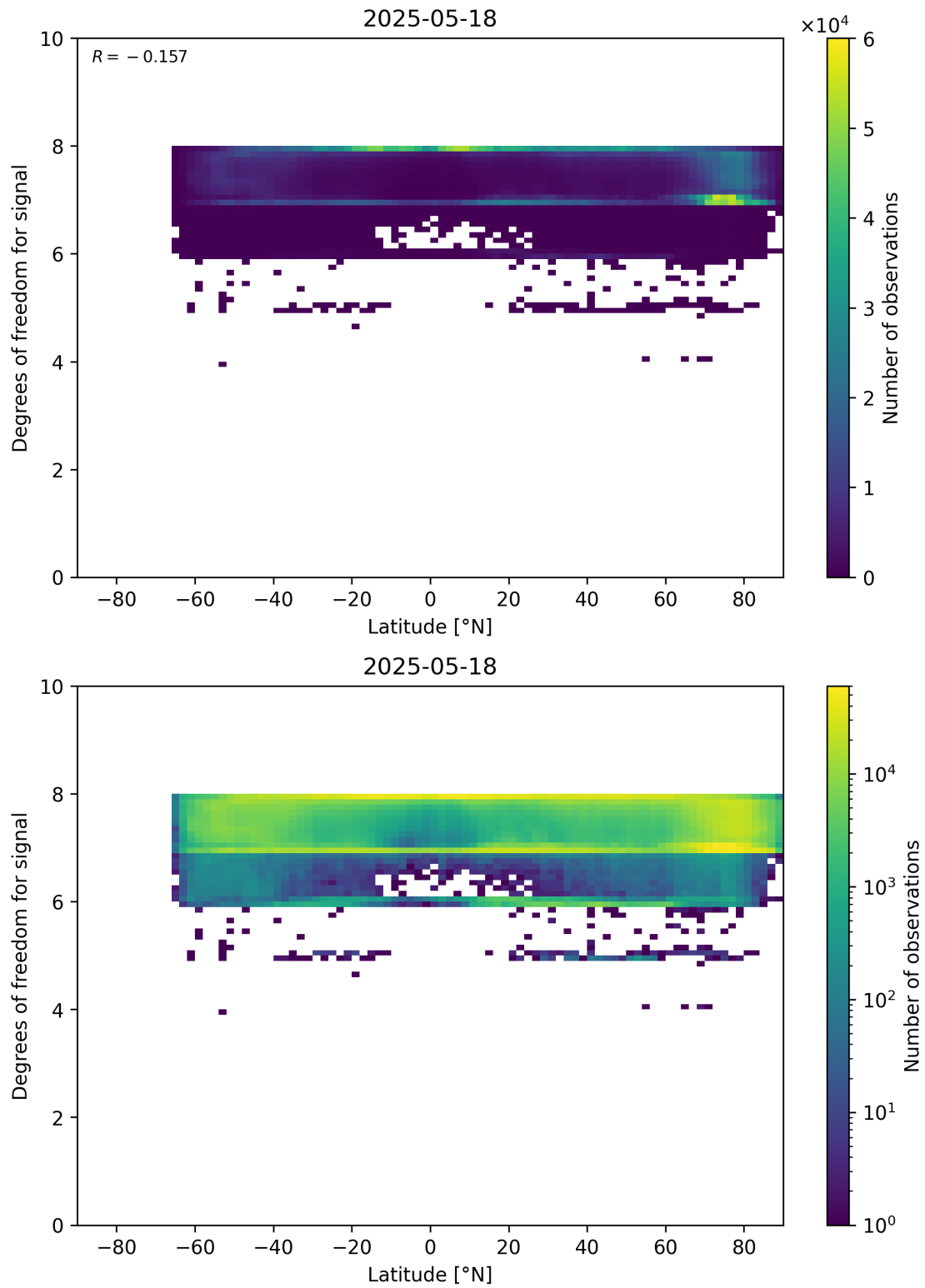
Figure 55: Scatter density plot of “Latitude” against “Degrees of freedom for signal” for 2025-05-17 to 2025-05-19.
