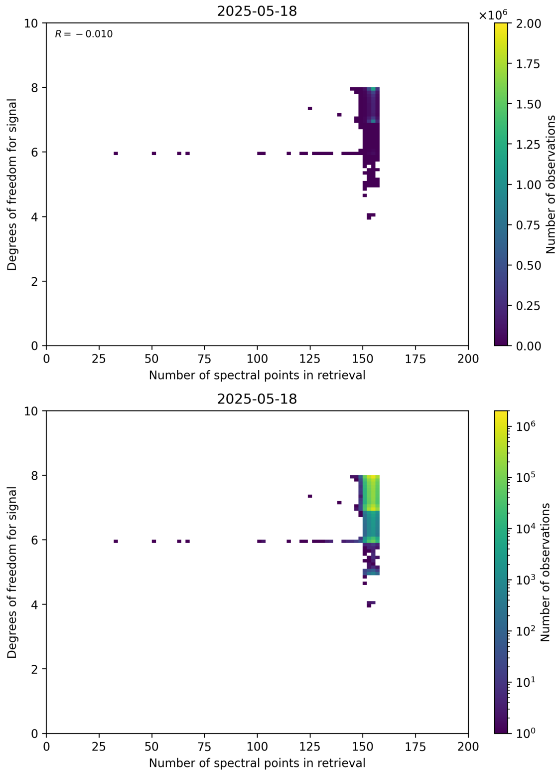
Figure 59: Scatter density plot of “Number of spectral points in retrieval” against “Degrees of freedom for signal” for 2025-05-17 to 2025-05-19.
