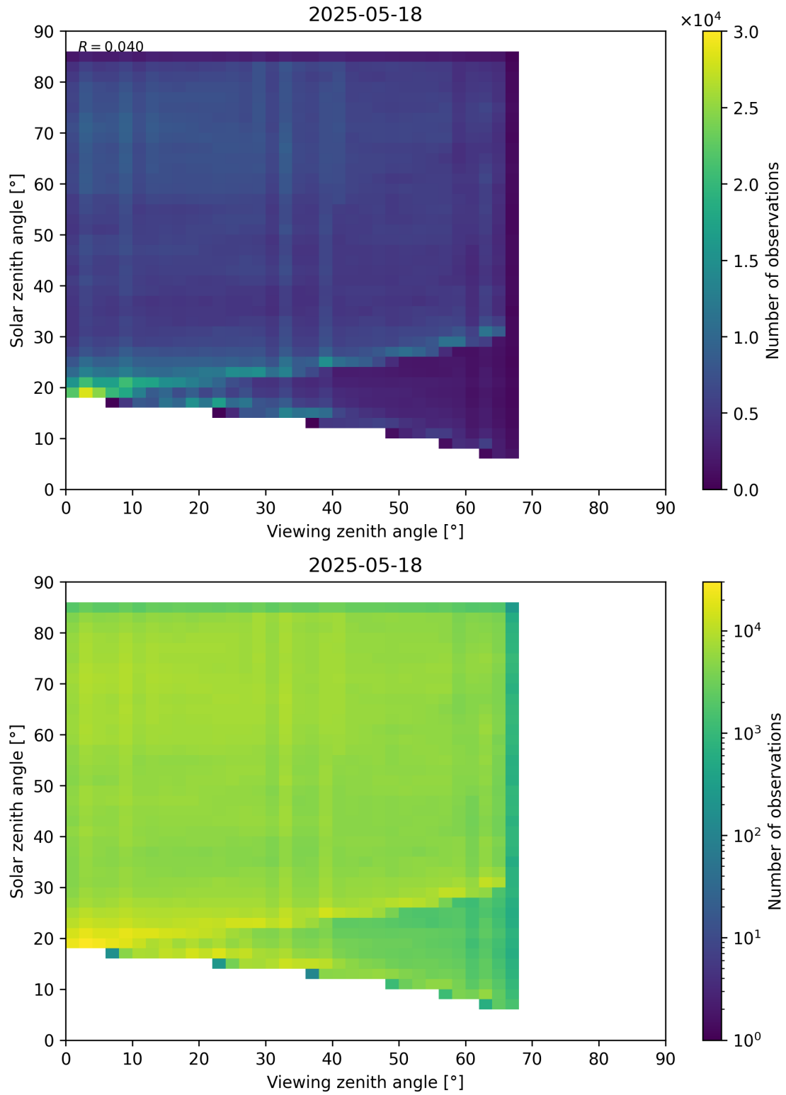
Figure 77: Scatter density plot of “Viewing zenith angle” against “Solar zenith angle” for 2025-05-17 to 2025-05-19.
