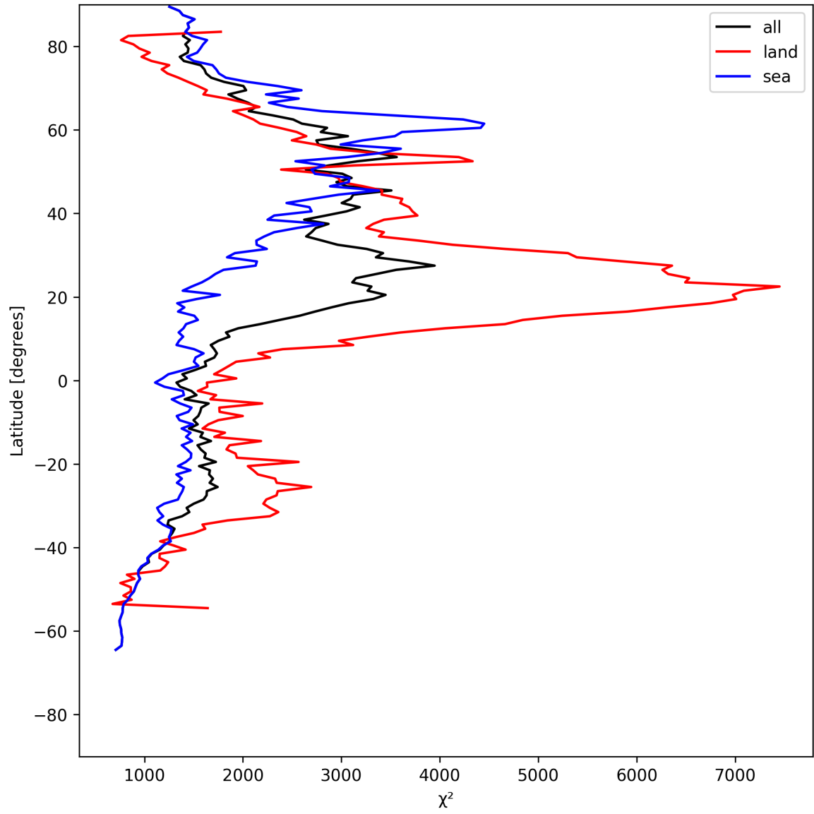
Figure 14: Zonal average of “ \chi^2 ” for 2025-05-17 to 2025-05-19.
