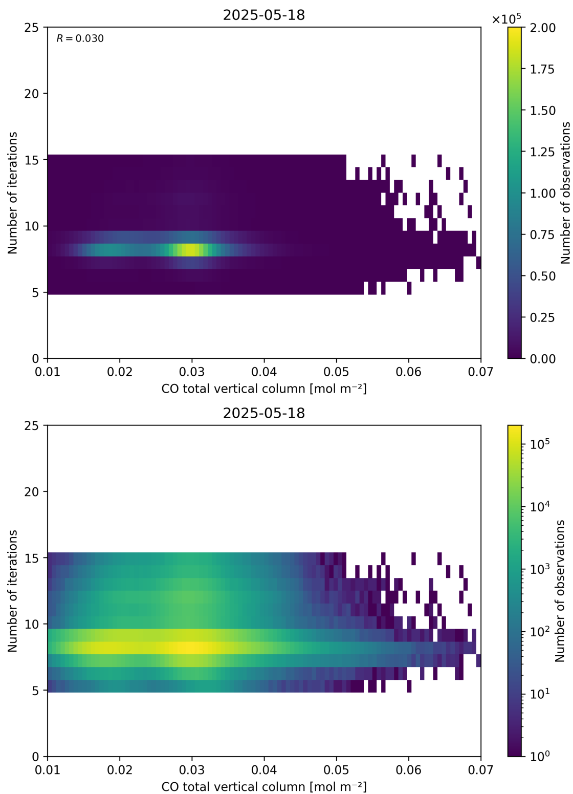
Figure 42: Scatter density plot of “CO total vertical column” against “Number of iterations” for 2025-05-17 to 2025-05-19.
