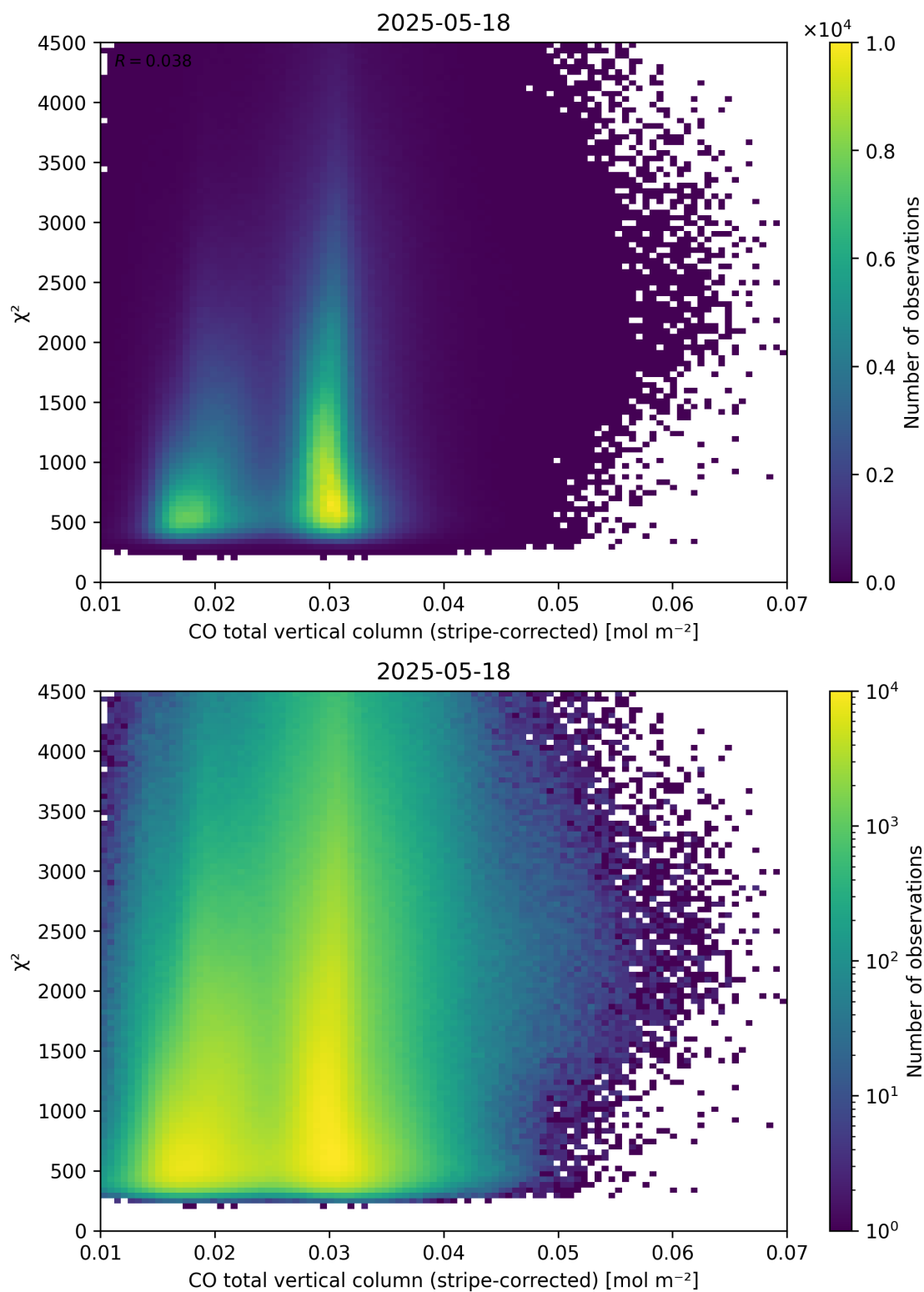
Figure 37: Scatter density plot of “CO total vertical column (stripe-corrected)” against “ \chi^2 ” for 2025-05-17 to 2025-05-19.
