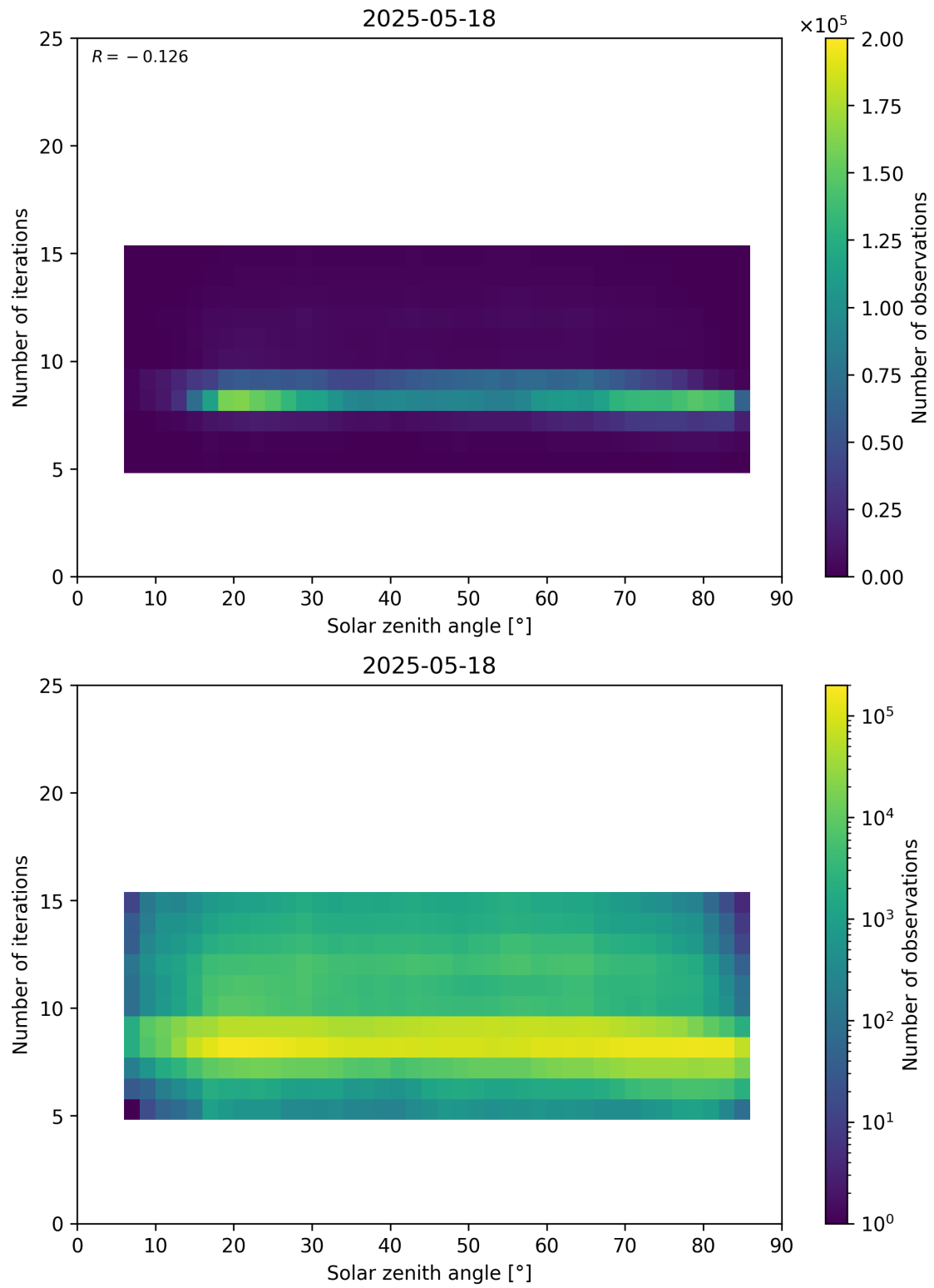
Figure 67: Scatter density plot of “Solar zenith angle” against “Number of iterations” for 2025-05-17 to 2025-05-19.
