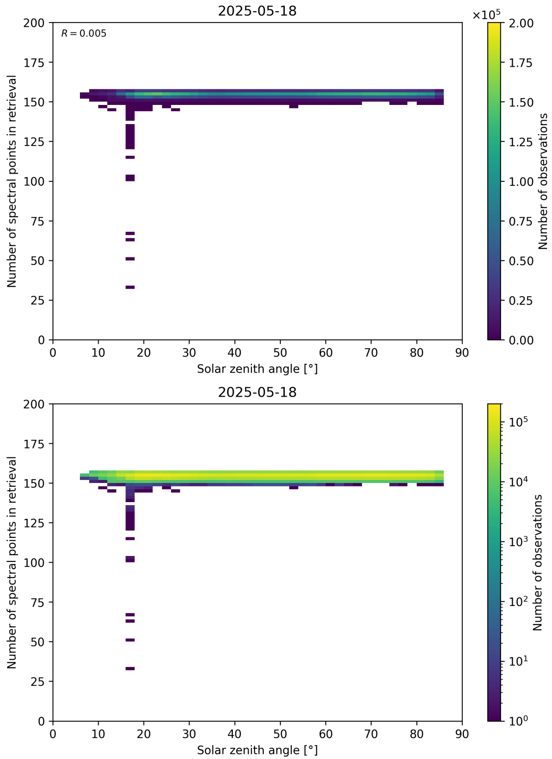
Figure 68: Scatter density plot of “Solar zenith angle” against “Number of spectral points in retrieval” for 2025-05-17 to 2025-05-19.
