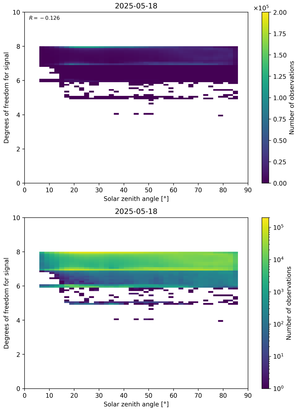
Figure 65: Scatter density plot of “Solar zenith angle” against “Degrees of freedom for signal” for 2025-05-17 to 2025-05-19.
