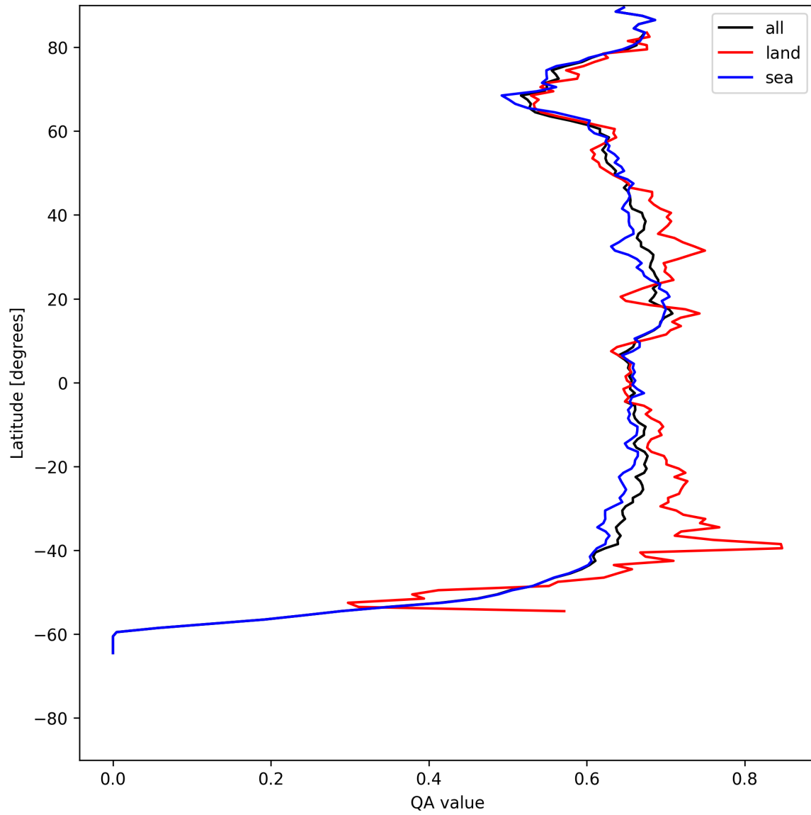
Figure 9: Zonal average of “QA value” for 2025-05-17 to 2025-05-19.
