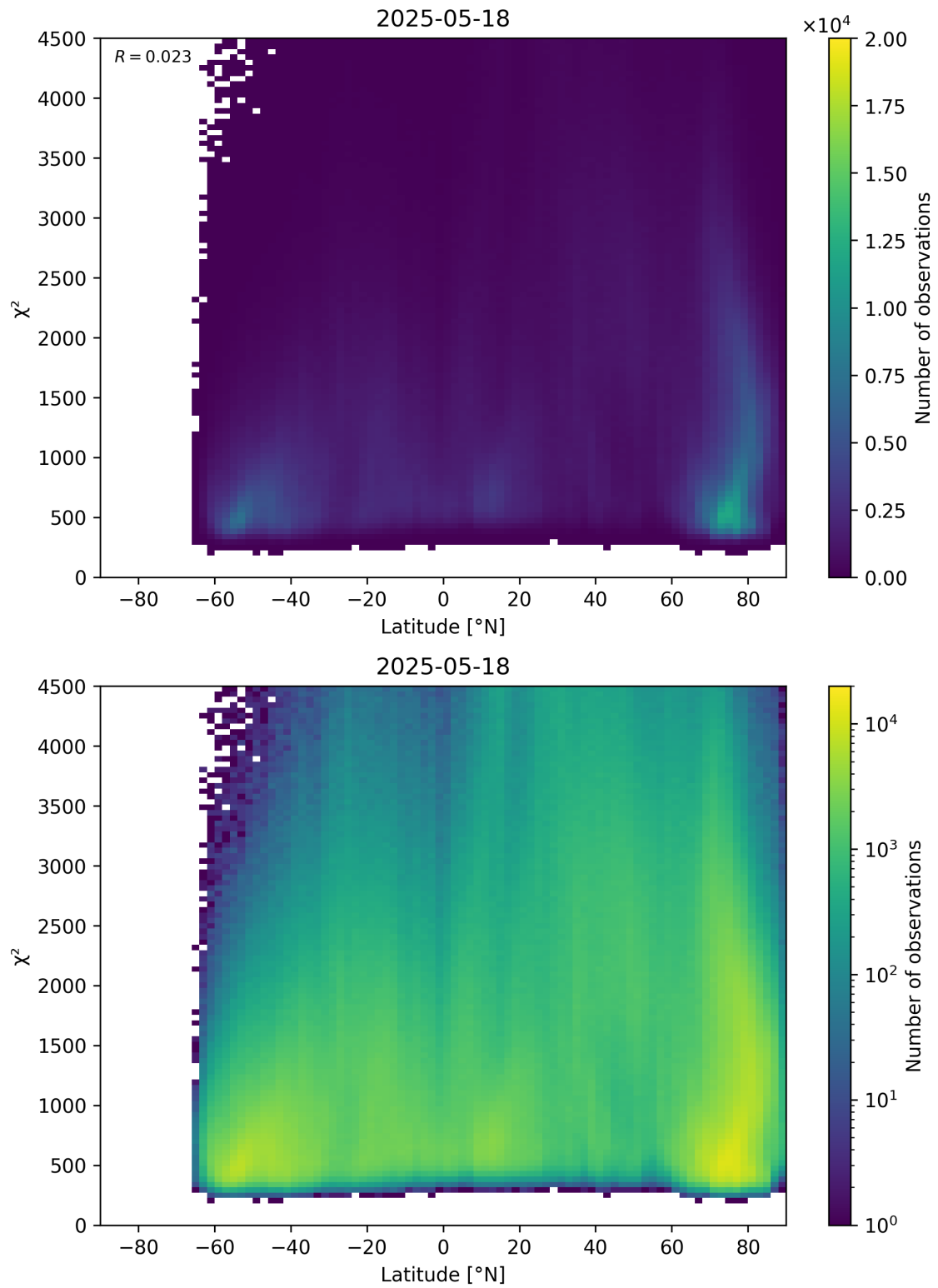
Figure 54: Scatter density plot of “Latitude” against “ \chi^2 ” for 2025-05-17 to 2025-05-19.
