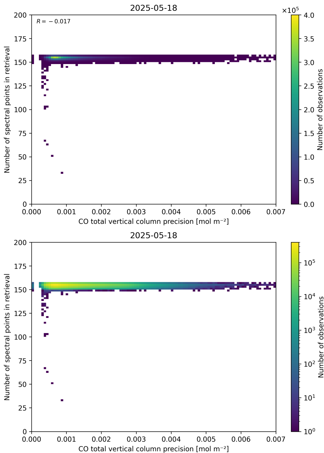
Figure 47: Scatter density plot of “CO total vertical column precision” against “Number of spectral points in retrieval” for 2025-05-17 to 2025-05-19.
