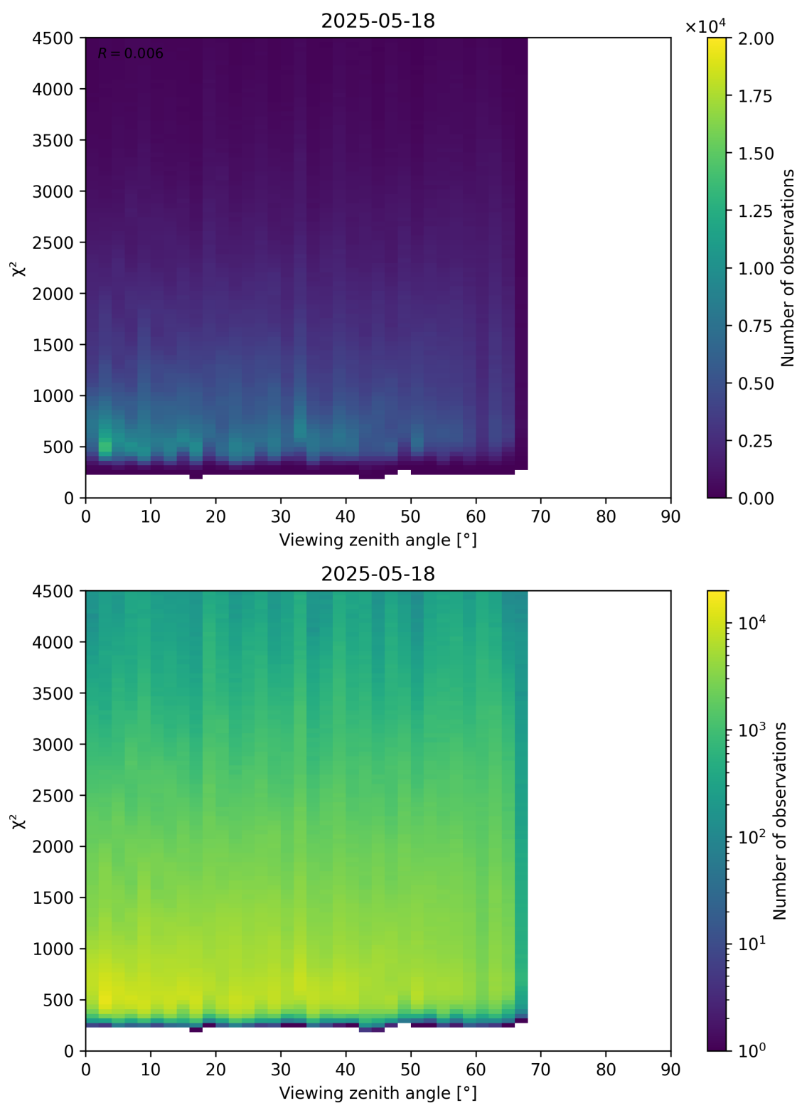
Figure 72: Scatter density plot of “Viewing zenith angle” against “ \chi^2 ” for 2025-05-17 to 2025-05-19.
