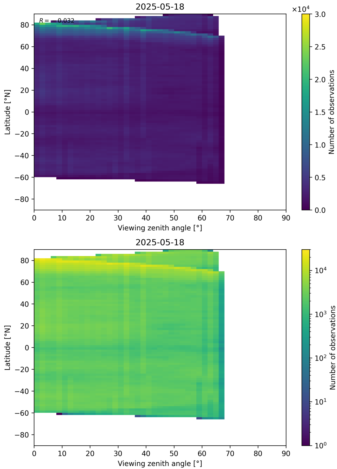
Figure 74: Scatter density plot of “Viewing zenith angle” against “Latitude” for 2025-05-17 to 2025-05-19.
