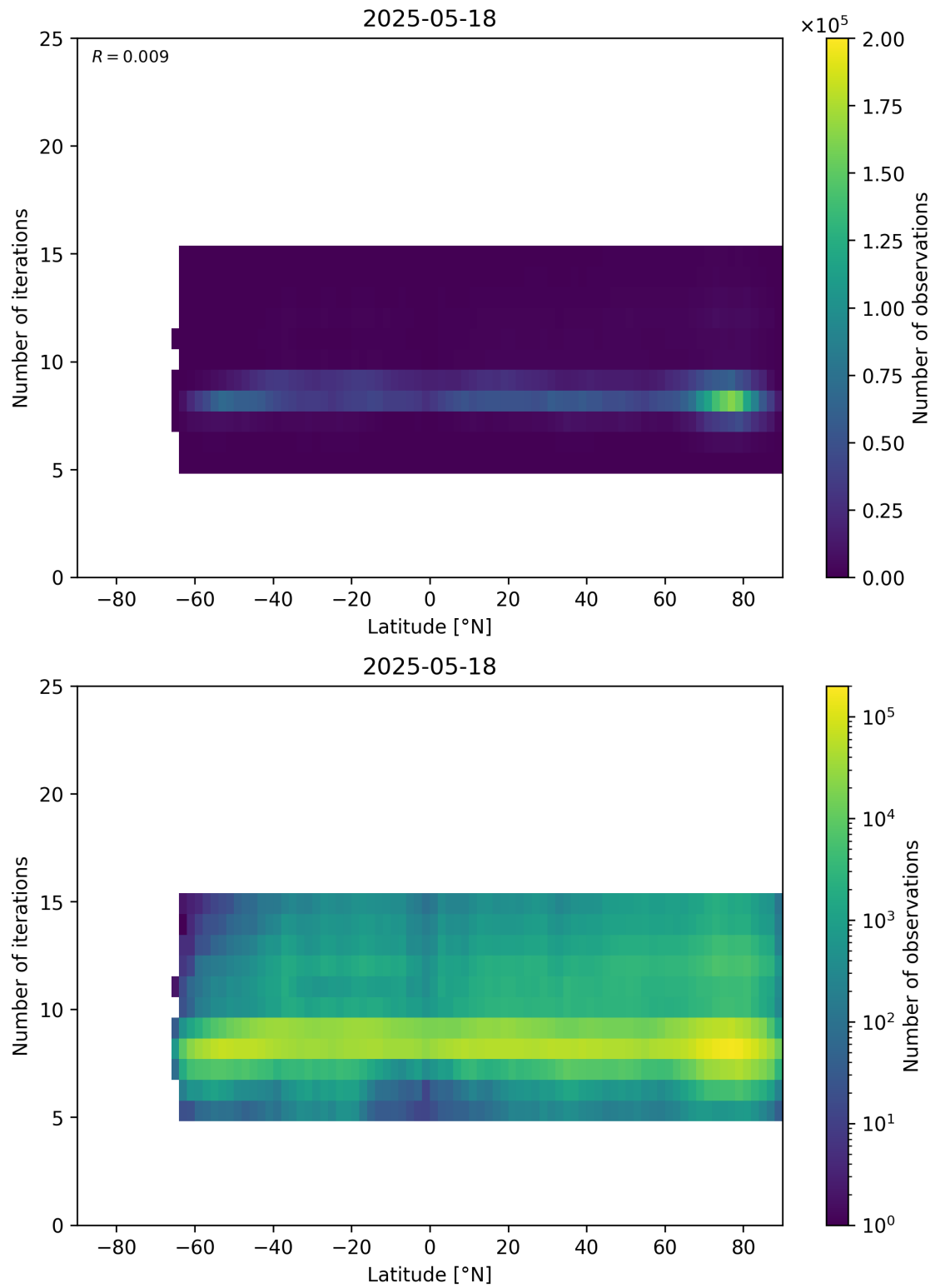
Figure 56: Scatter density plot of “Latitude” against “Number of iterations” for 2025-05-17 to 2025-05-19.
