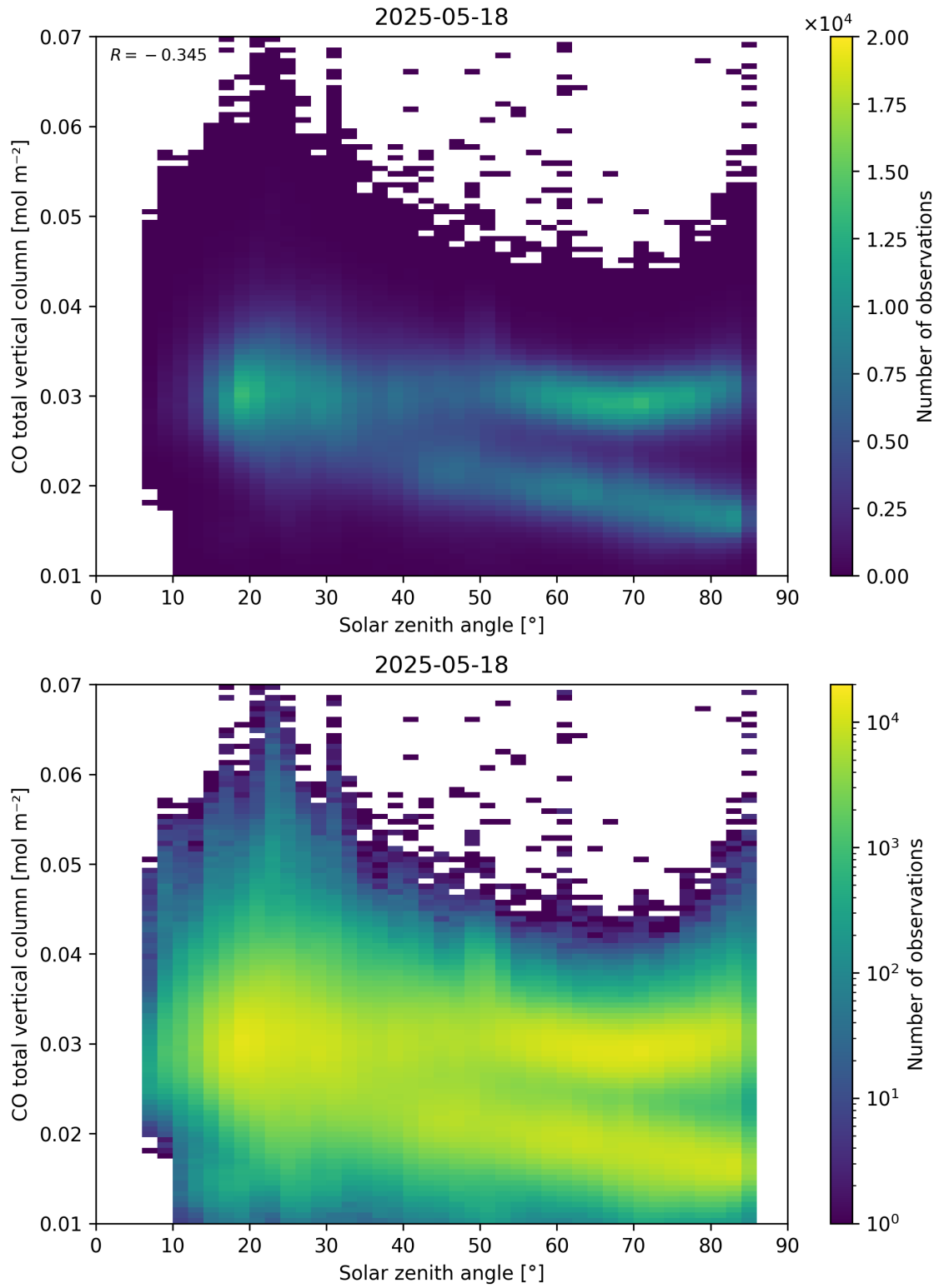
Figure 61: Scatter density plot of “Solar zenith angle” against “CO total vertical column” for 2025-05-17 to 2025-05-19.
