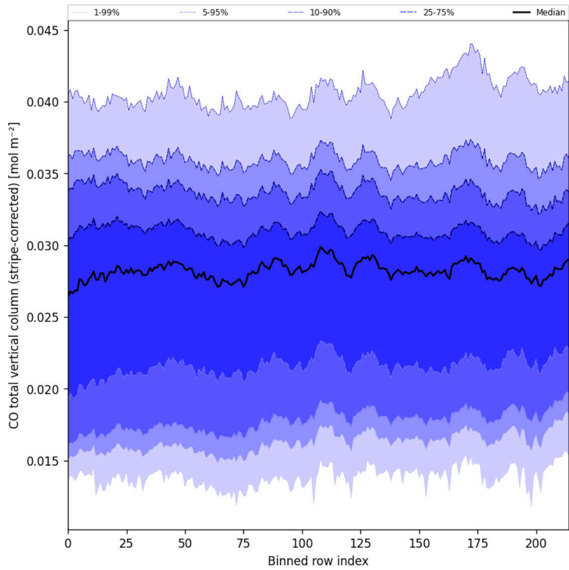
Figure 27: Along track statistics of “CO total vertical column (stripe-corrected)” for 2025-05-17 to 2025-05-19
