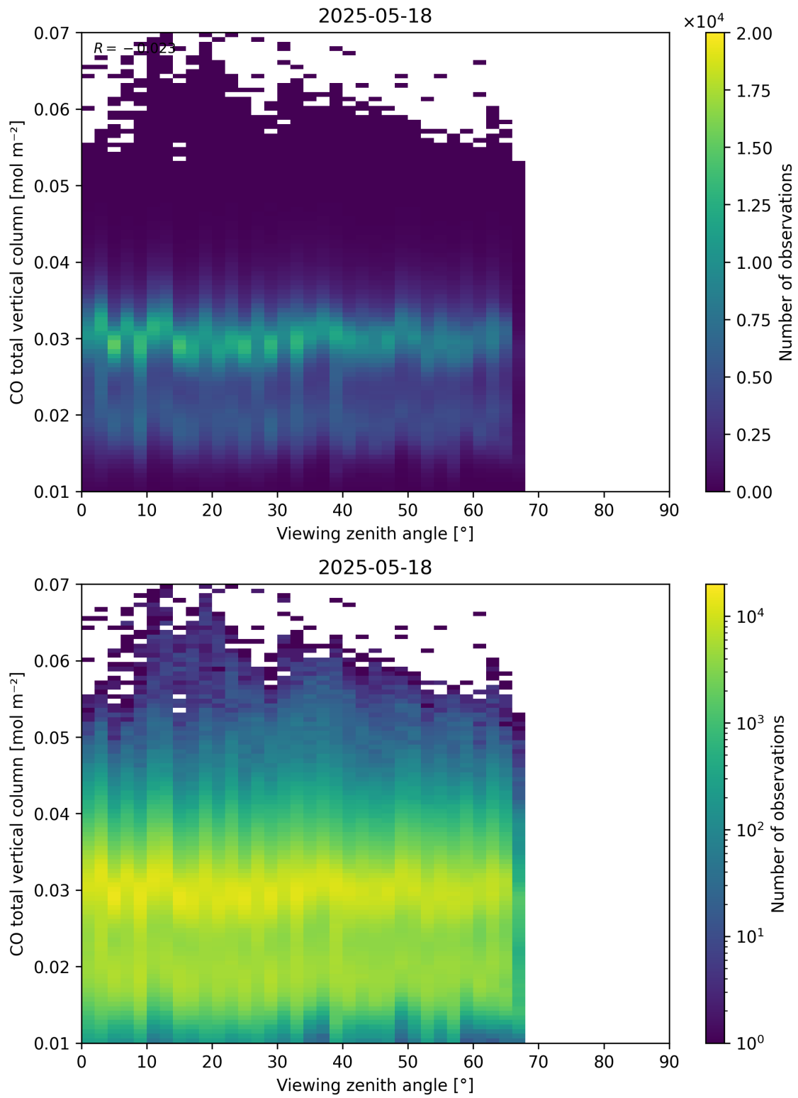
Figure 69: Scatter density plot of “Viewing zenith angle” against “CO total vertical column” for 2025-05-17 to 2025-05-19.
