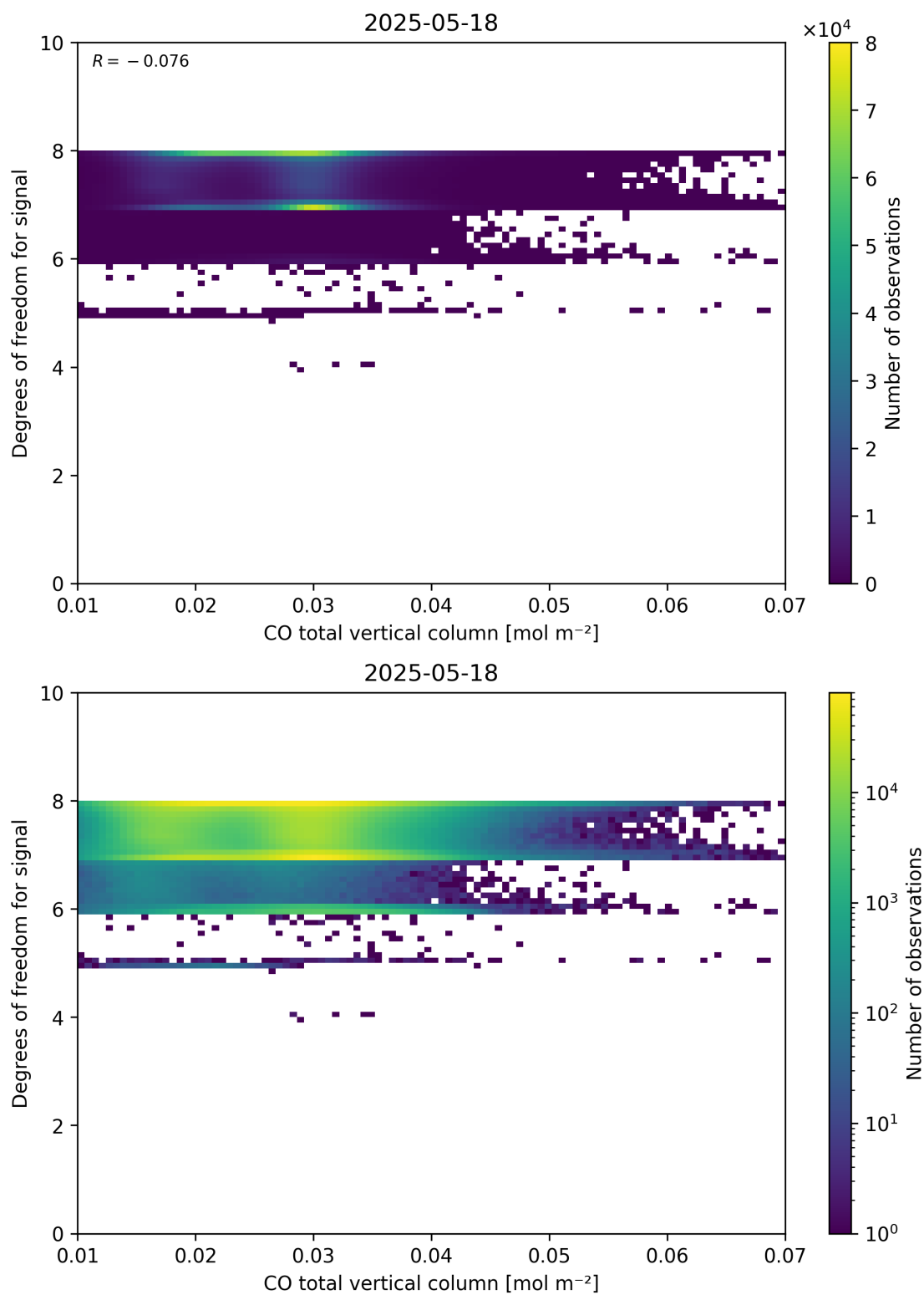
Figure 41: Scatter density plot of “CO total vertical column” against “Degrees of freedom for signal” for 2025-05-17 to 2025-05-19.
