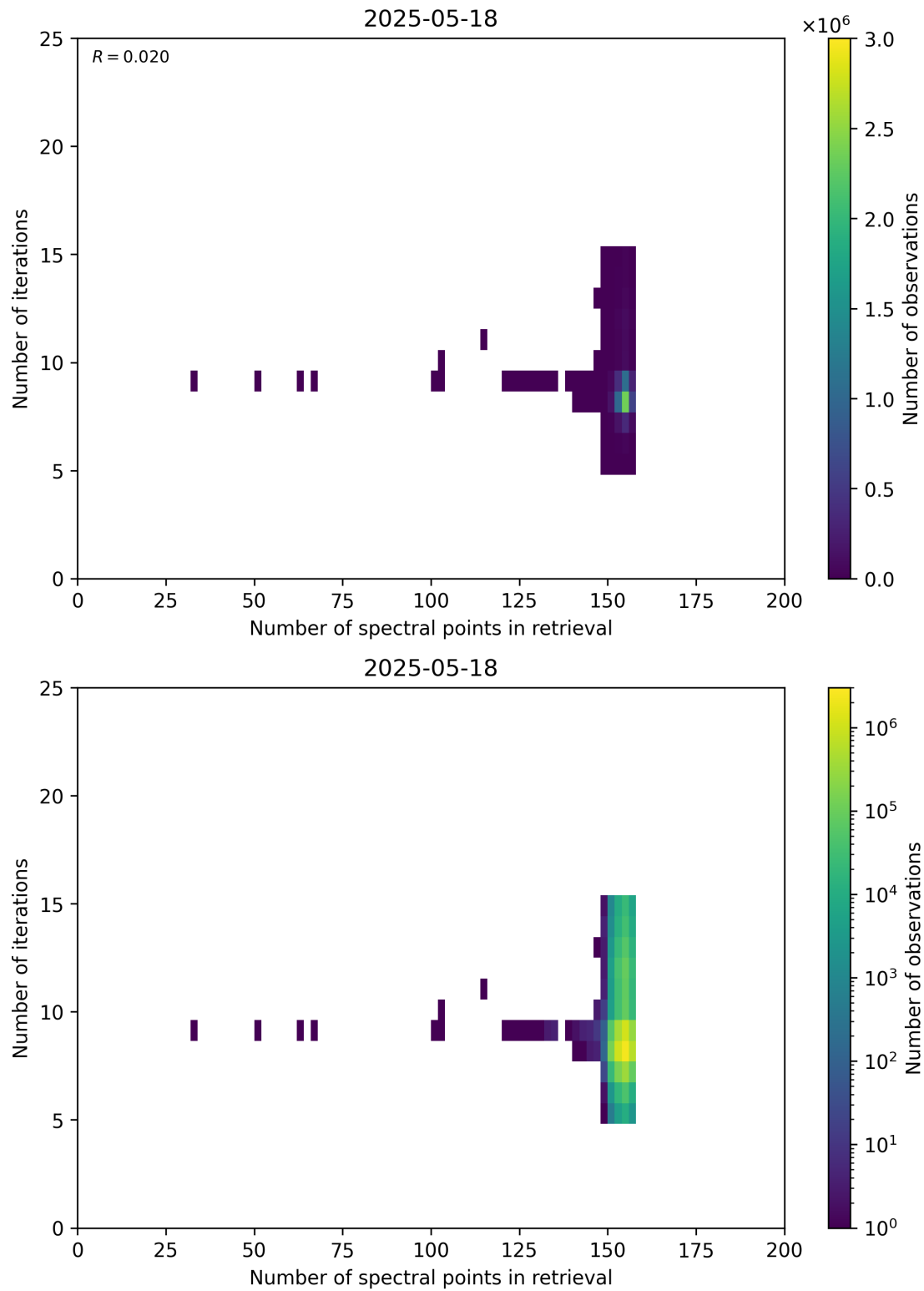
Figure 60: Scatter density plot of “Number of spectral points in retrieval” against “Number of iterations” for 2025-05-17 to 2025-05-19.
