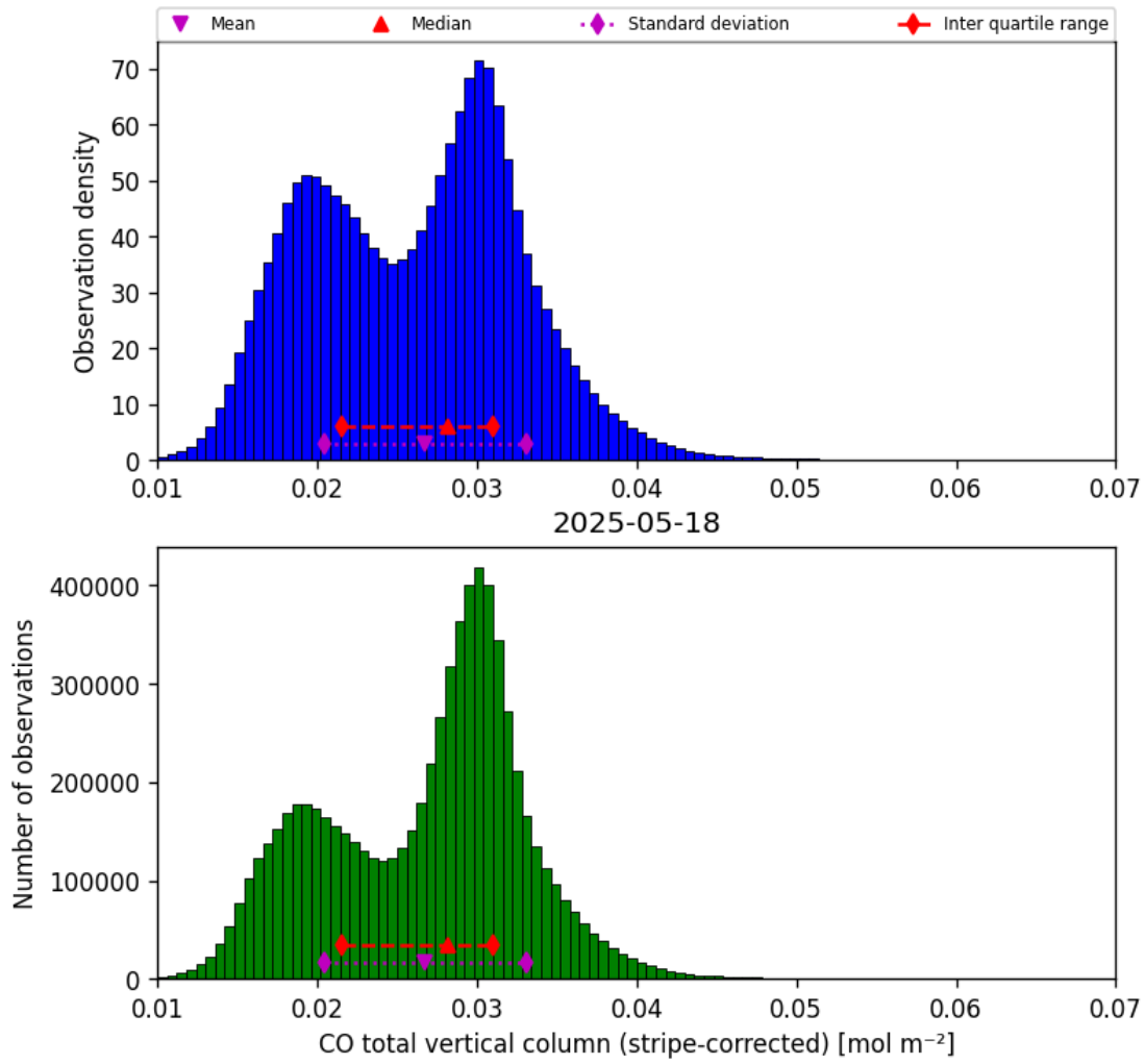
Figure 19: Histogram of “CO total vertical column (stripe-corrected)” for 2025-05-17 to 2025-05-19
