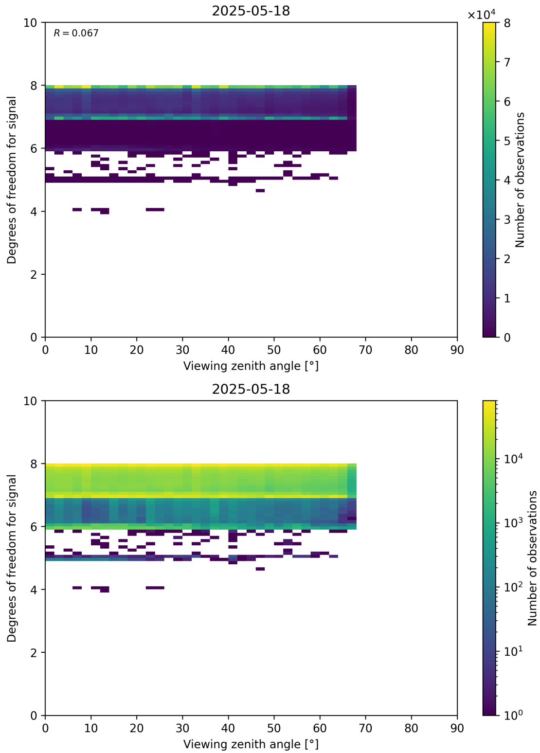
Figure 73: Scatter density plot of “Viewing zenith angle” against “Degrees of freedom for signal” for 2025-05-17 to 2025-05-19.
