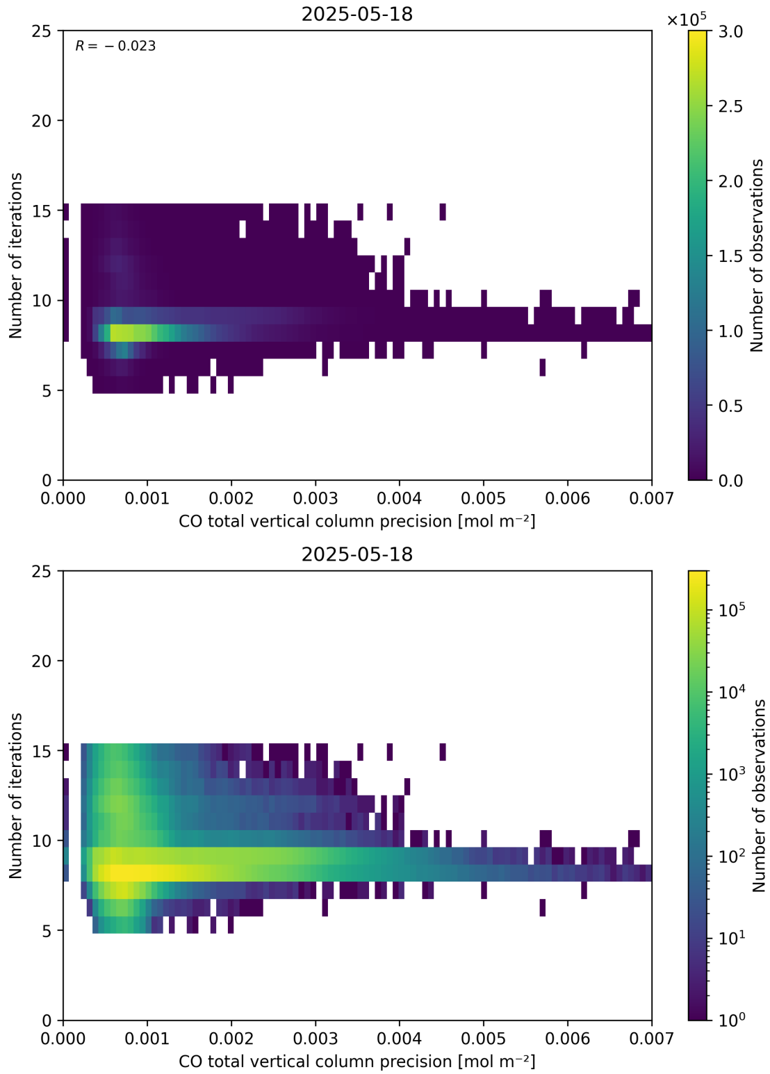
Figure 46: Scatter density plot of “CO total vertical column precision” against “Number of iterations” for 2025-05-17 to 2025-05-19.
