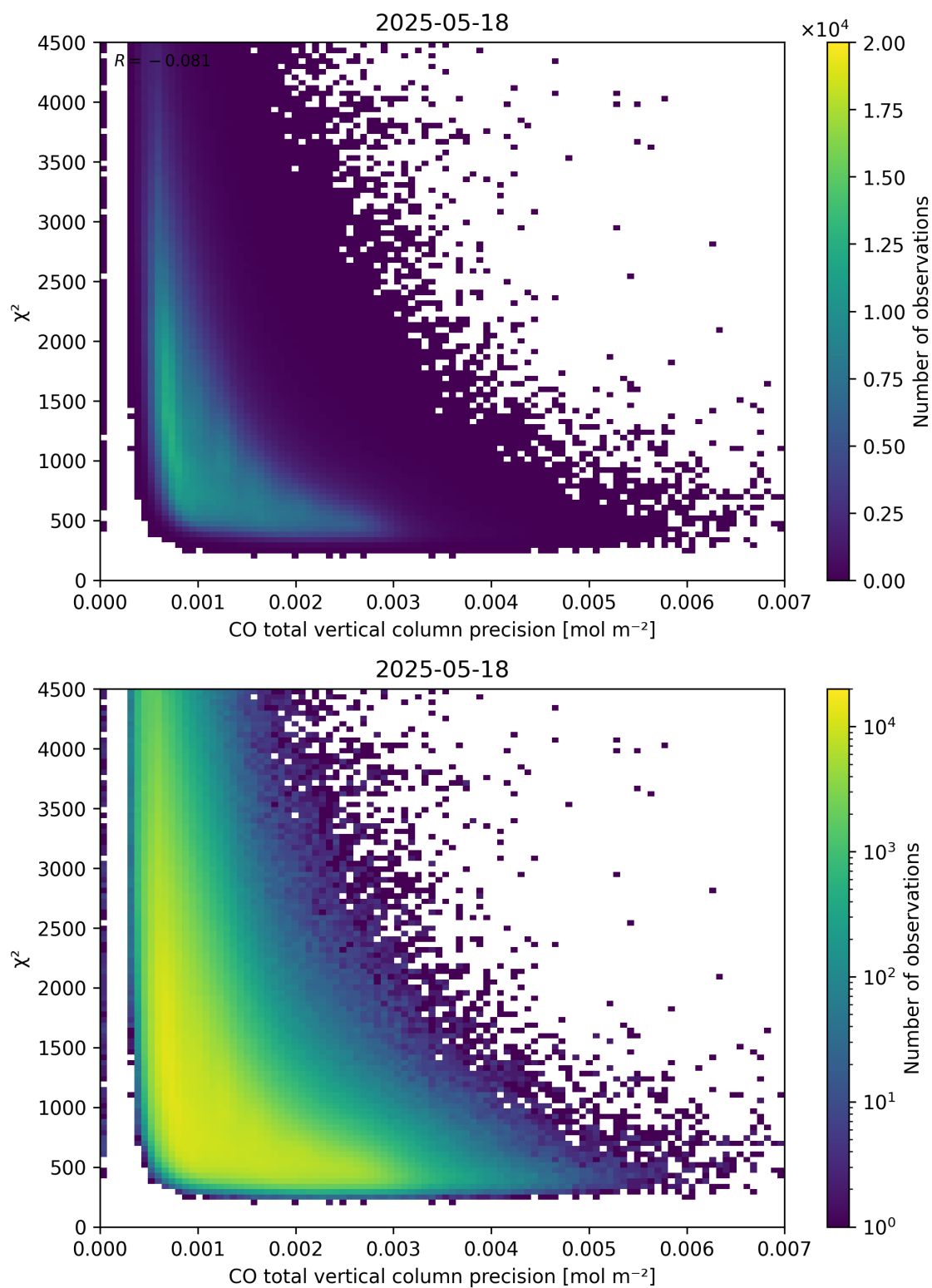
Figure 44: Scatter density plot of “CO total vertical column precision” against “ \chi^2 ” for 2025-05-17 to 2025-05-19.
