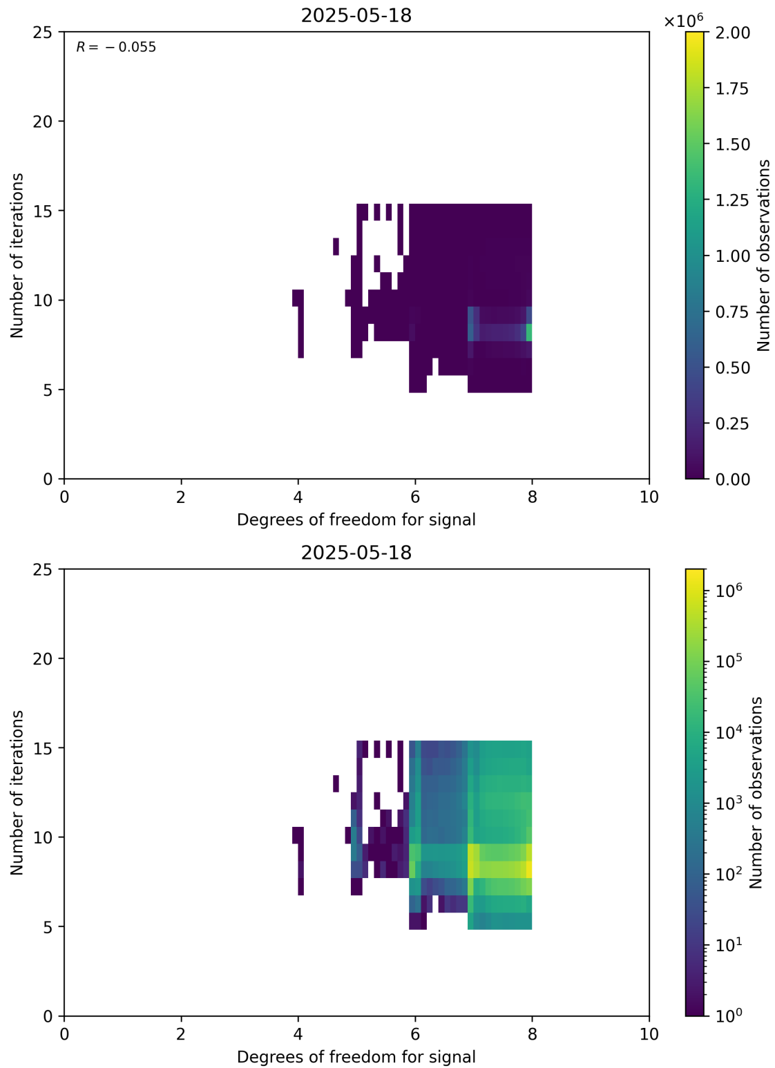
Figure 50: Scatter density plot of “Degrees of freedom for signal” against “Number of iterations” for 2025-05-17 to 2025-05-19.
