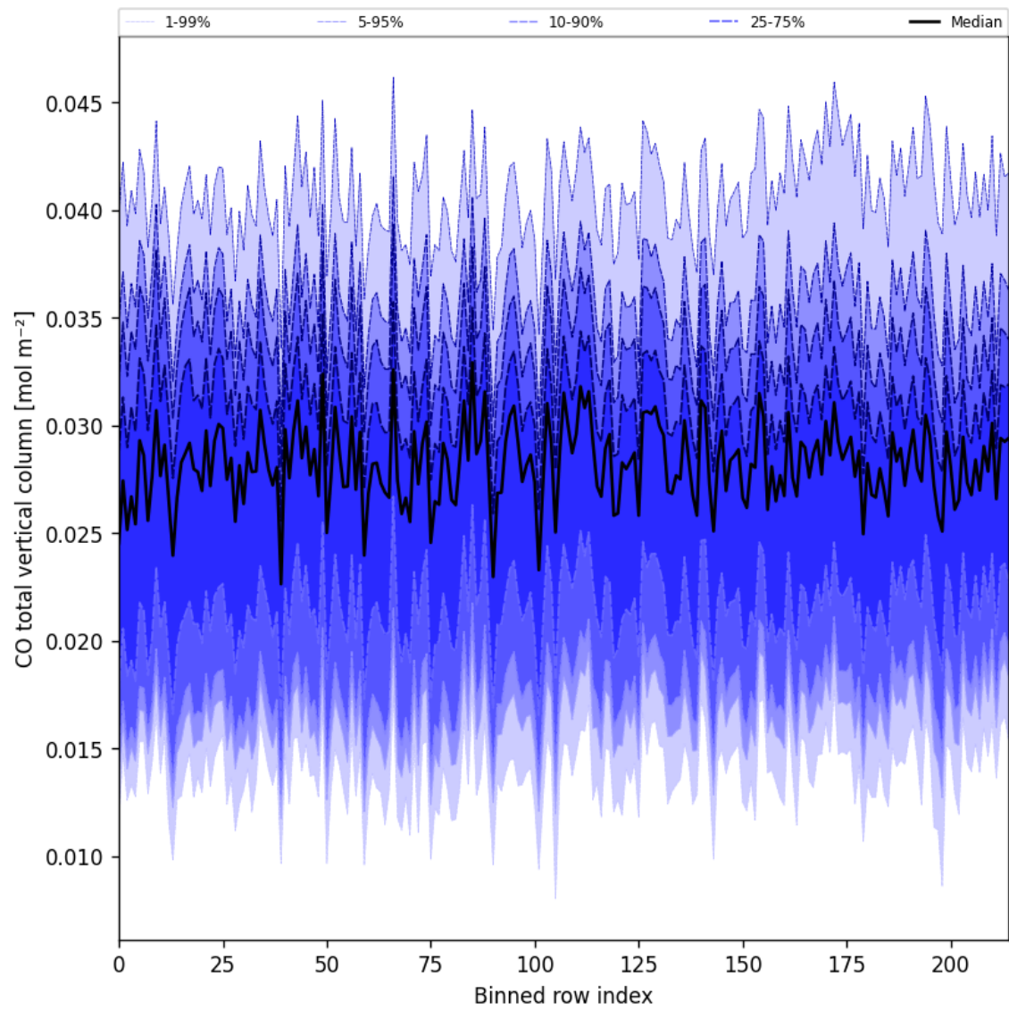
Figure 26: Along track statistics of “CO total vertical column” for 2025-05-17 to 2025-05-19
