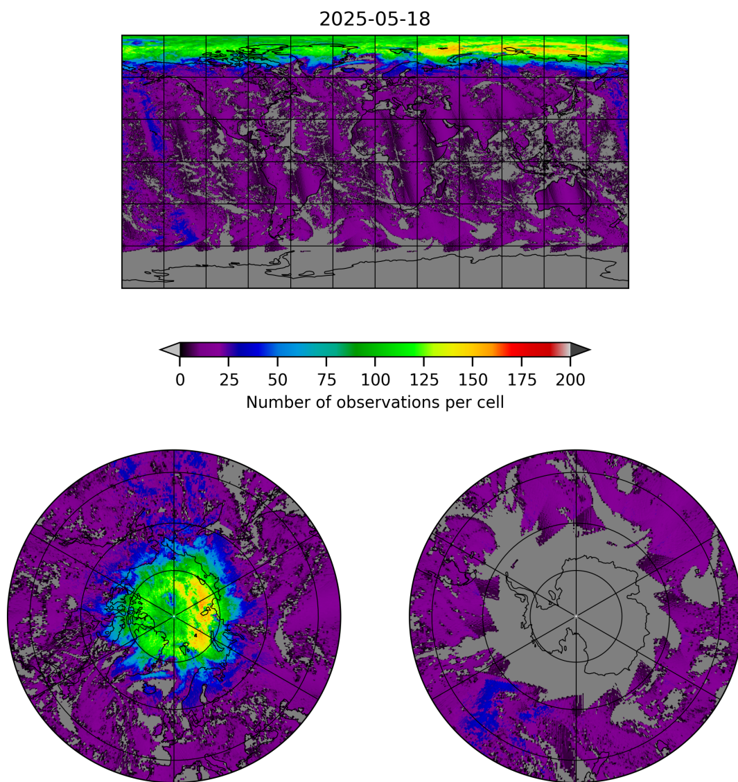
Figure 8: Map of the number of observations for 2025-05-17 to 2025-05-19
