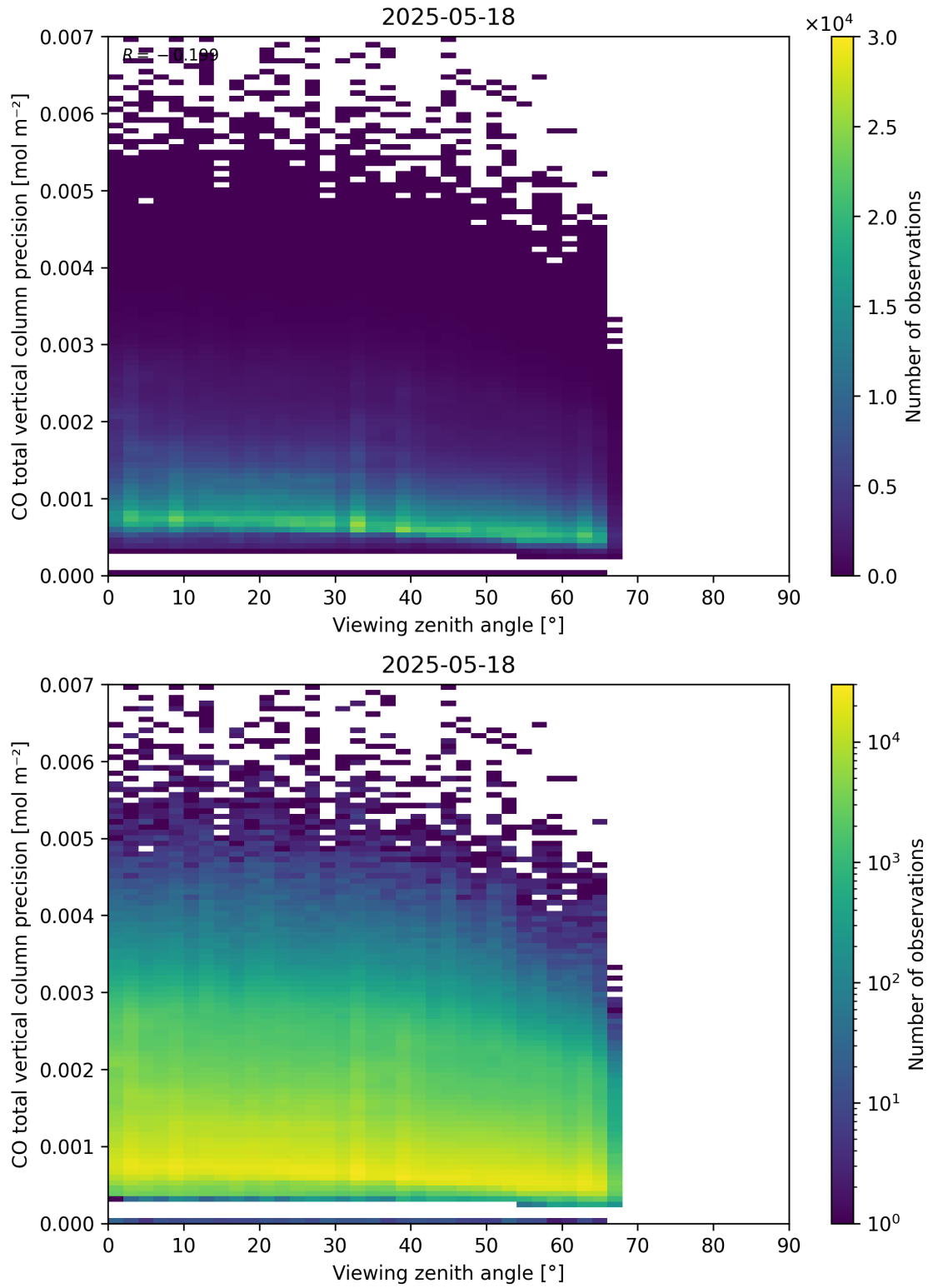
Figure 71: Scatter density plot of “Viewing zenith angle” against “CO total vertical column precision” for 2025-05-17 to 2025-05-19.
