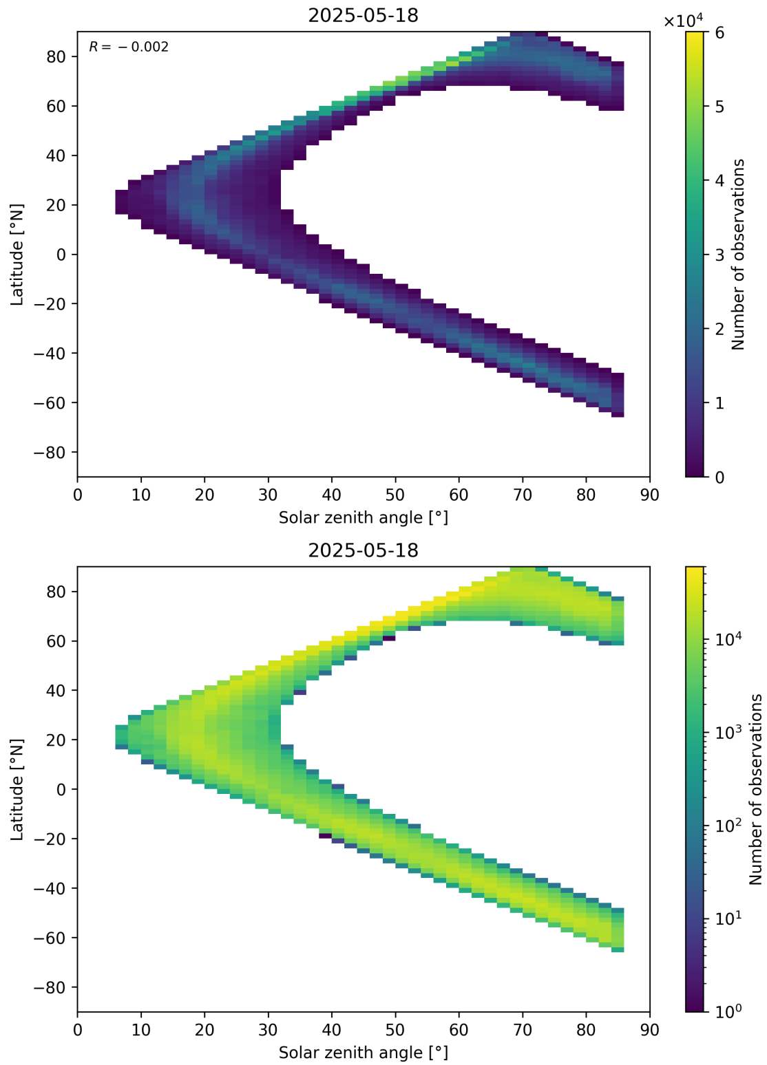
Figure 66: Scatter density plot of “Solar zenith angle” against “Latitude” for 2025-05-17 to 2025-05-19.
