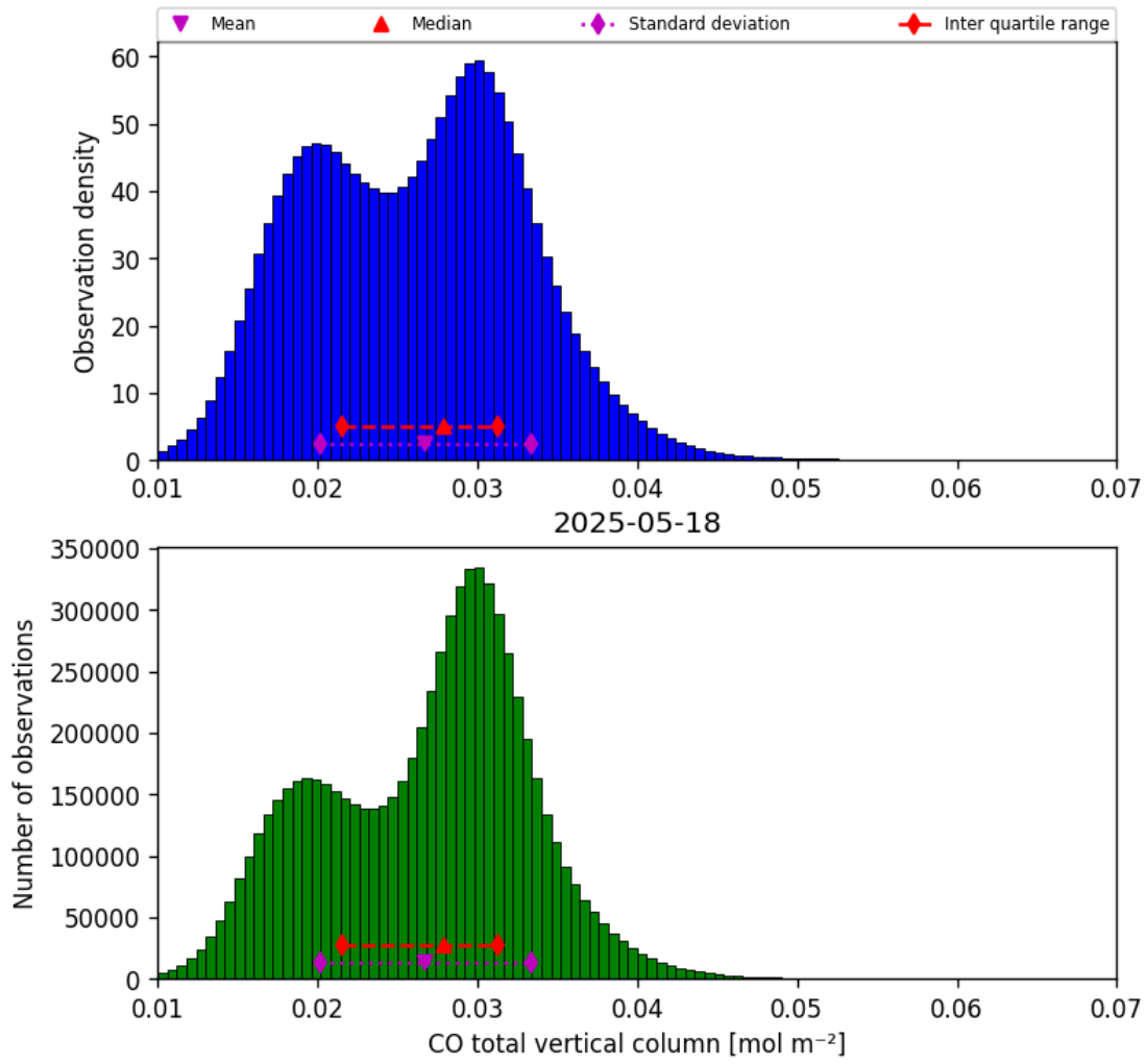
Figure 18: Histogram of “CO total vertical column” for 2025-05-17 to 2025-05-19
