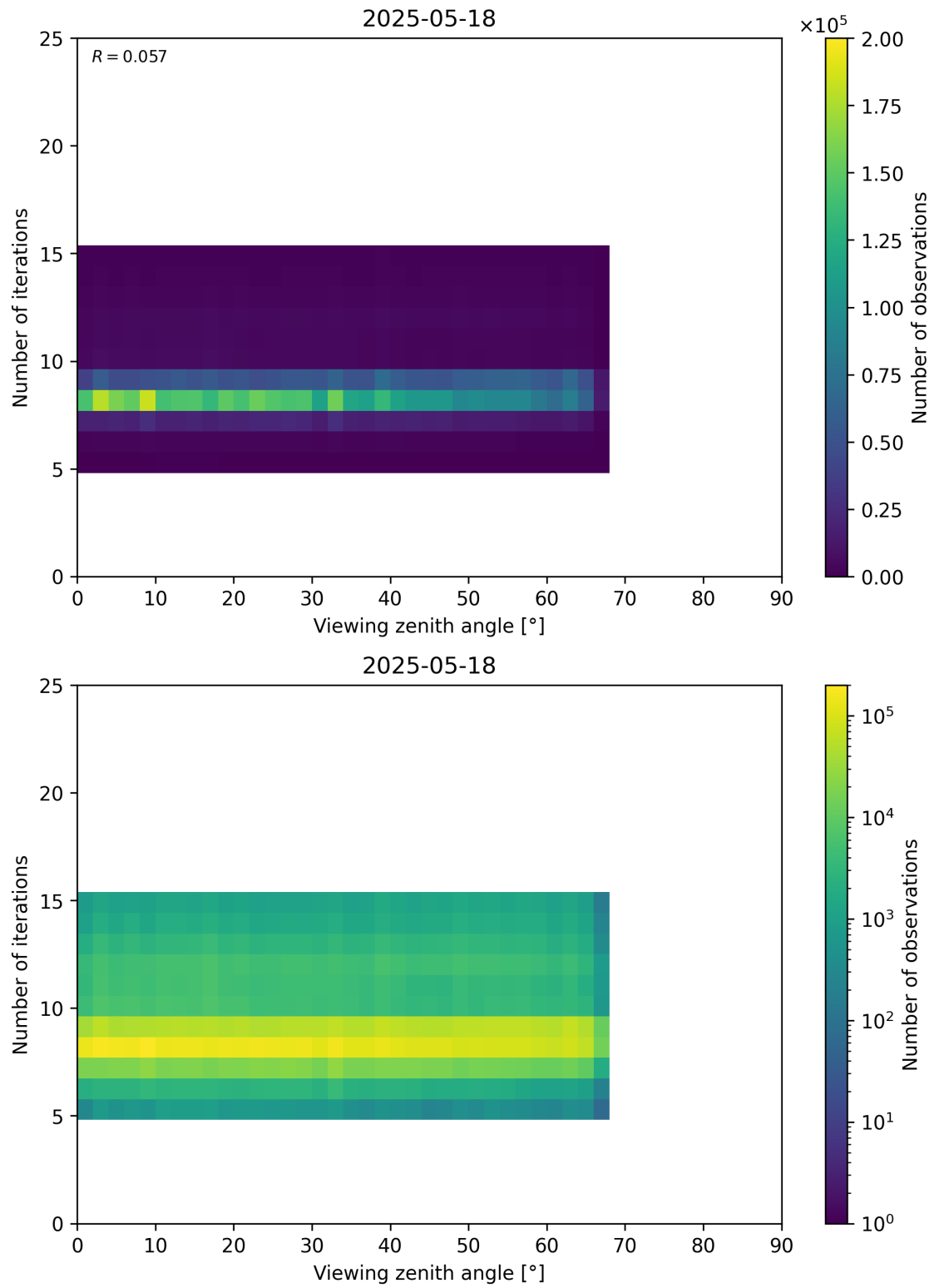
Figure 75: Scatter density plot of “Viewing zenith angle” against “Number of iterations” for 2025-05-17 to 2025-05-19.
