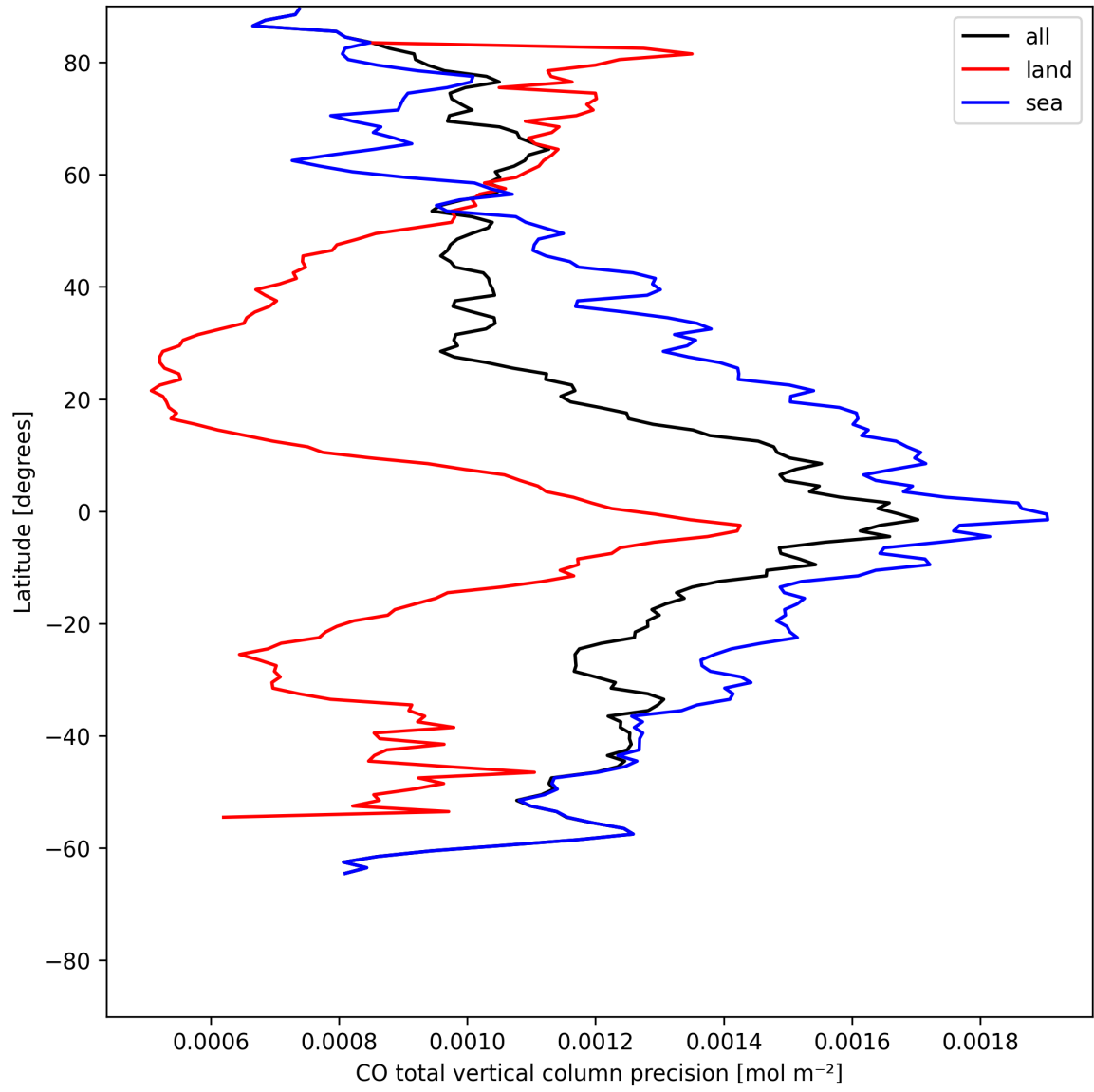
Figure 12: Zonal average of “CO total vertical column precision” for 2025-05-17 to 2025-05-19.
