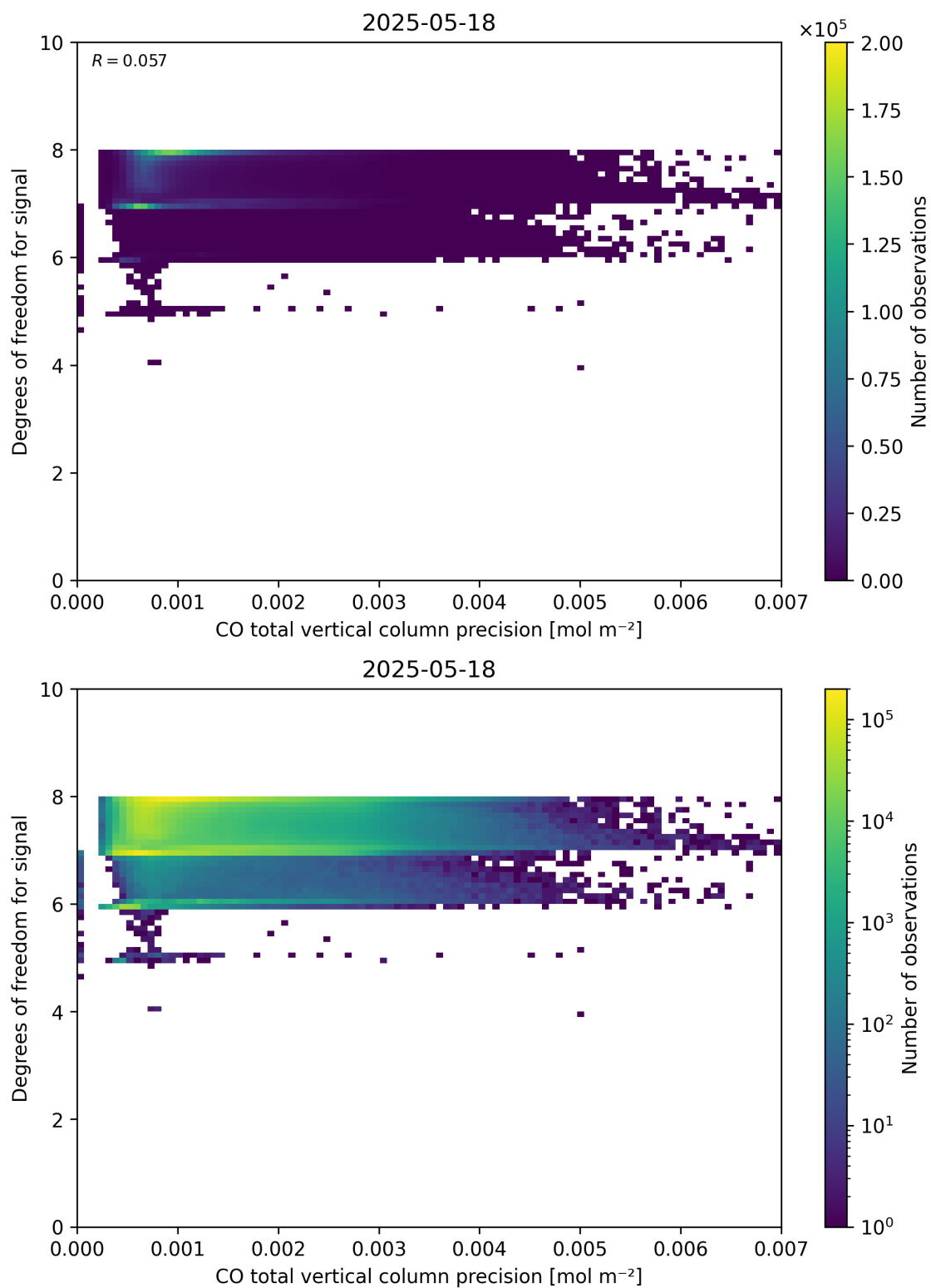
Figure 45: Scatter density plot of “CO total vertical column precision” against “Degrees of freedom for signal” for 2025-05-17 to 2025-05-19.
