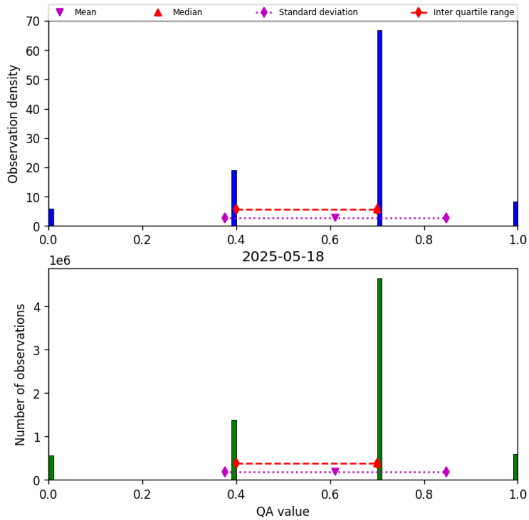
Figure 17: Histogram of “QA value” for 2025-05-17 to 2025-05-19
