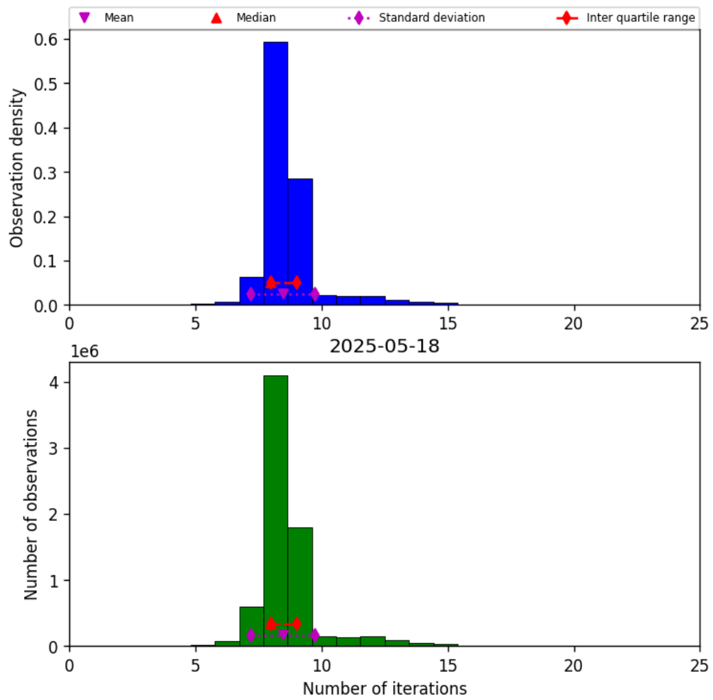
Figure 24: Histogram of “Number of iterations” for 2025-05-17 to 2025-05-19
