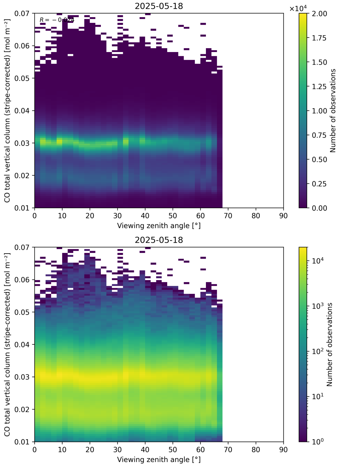
Figure 70: Scatter density plot of “Viewing zenith angle” against “CO total vertical column (stripe-corrected)” for 2025-05-17 to 2025-05-19.
