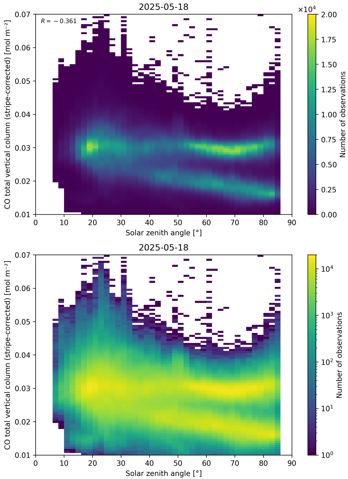
Figure 62: Scatter density plot of “Solar zenith angle” against “CO total vertical column (stripe-corrected)” for 2025-05-17 to 2025-05-19.
