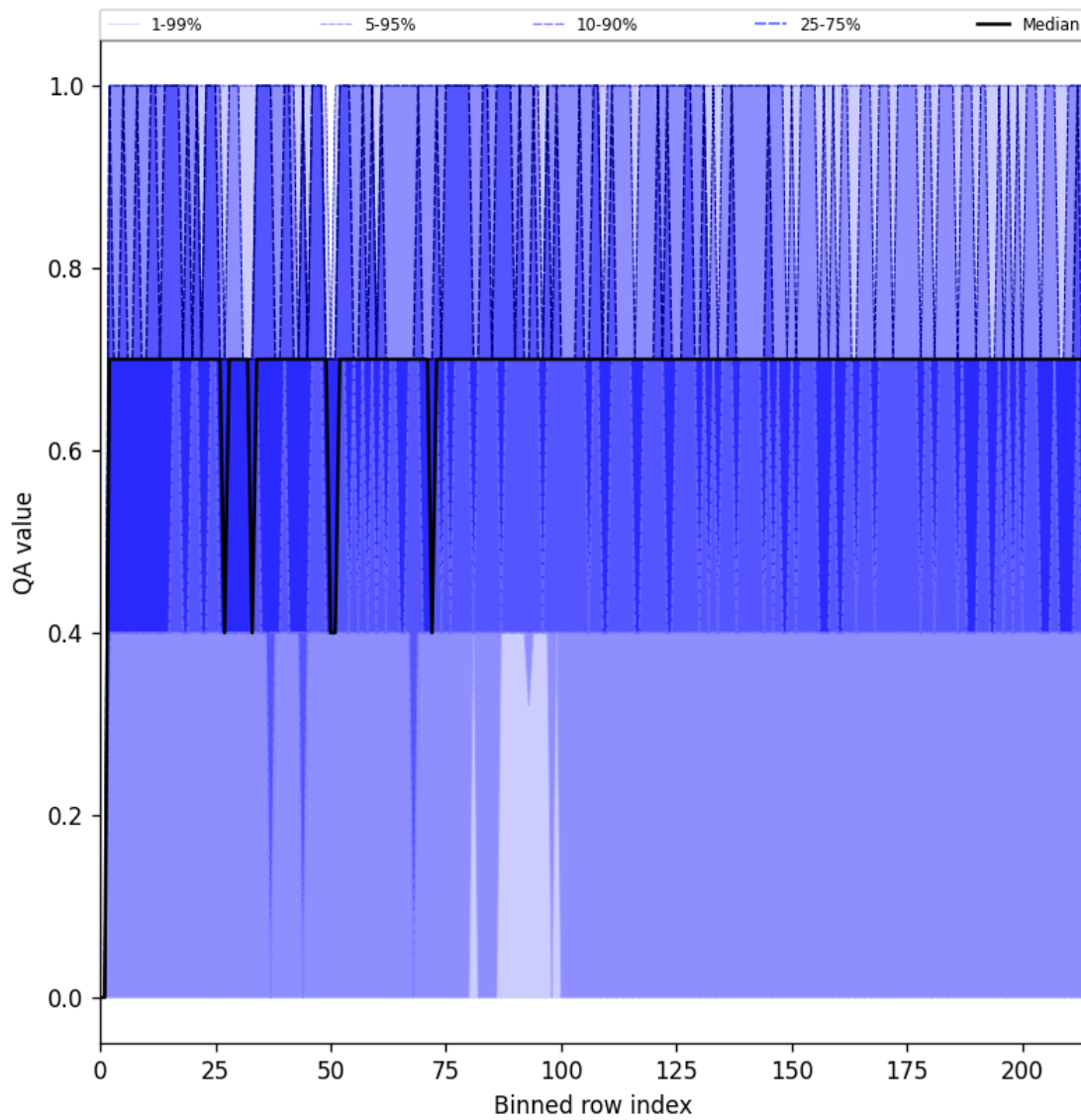
Figure 25: Along track statistics of “QA value” for 2025-05-17 to 2025-05-19
