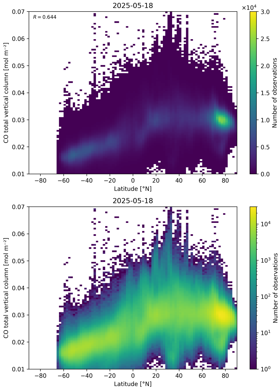
Figure 51: Scatter density plot of “Latitude” against “CO total vertical column” for 2025-05-17 to 2025-05-19.
