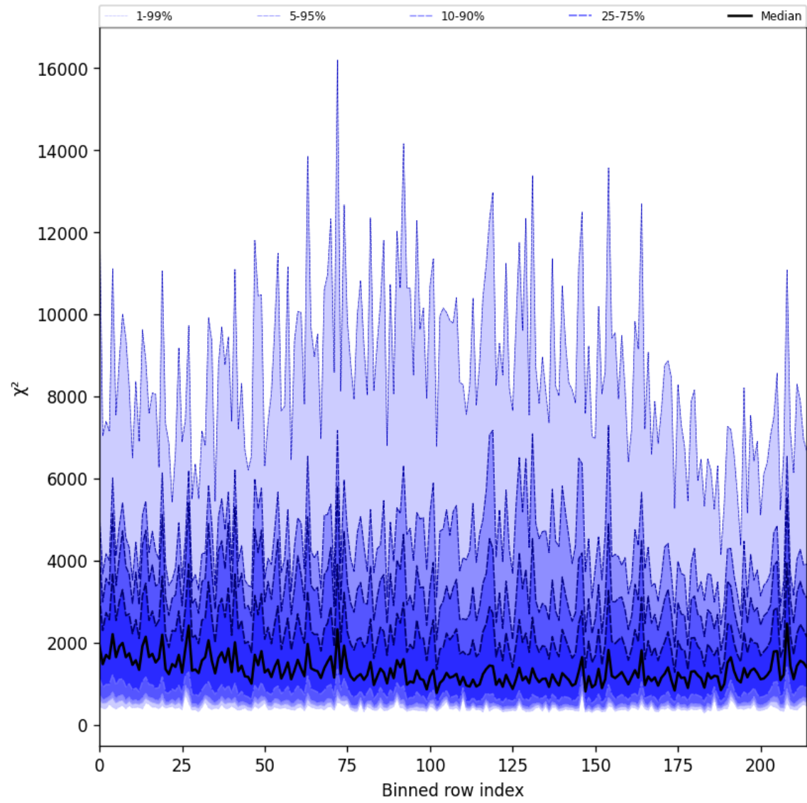
Figure 30: Along track statistics of “ \chi^2 ” for 2025-05-17 to 2025-05-19
