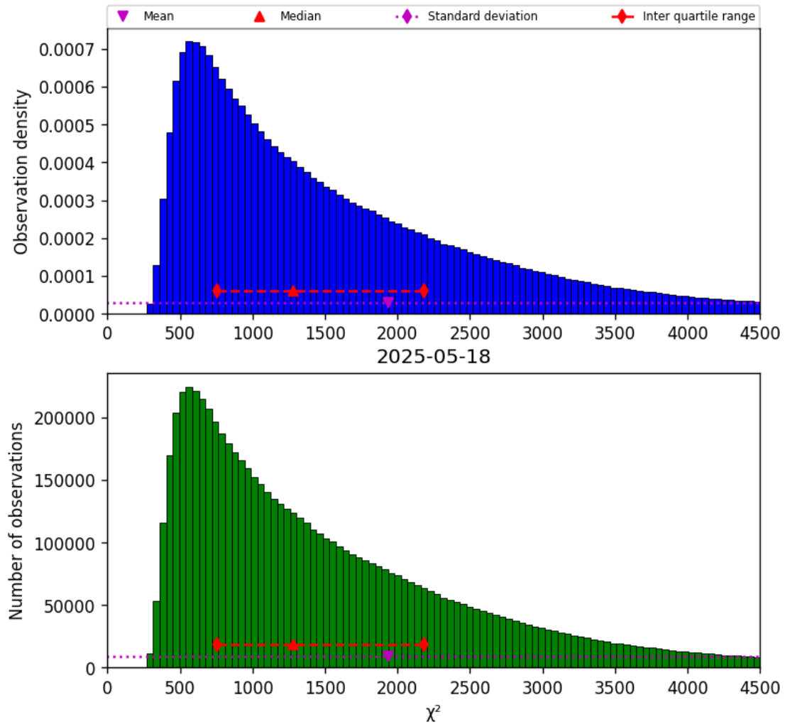
Figure 22: Histogram of “ \chi^2 ” for 2025-05-17 to 2025-05-19
