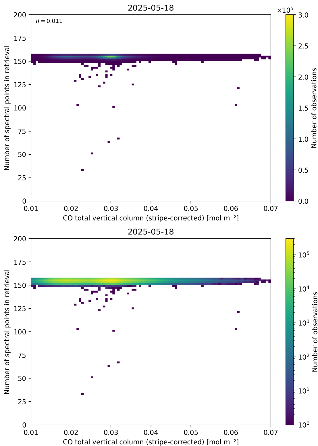
Figure 40: Scatter density plot of “CO total vertical column (stripe-corrected)” against “Number of spectral points in retrieval” for 2025-05-17 to 2025-05-19.
