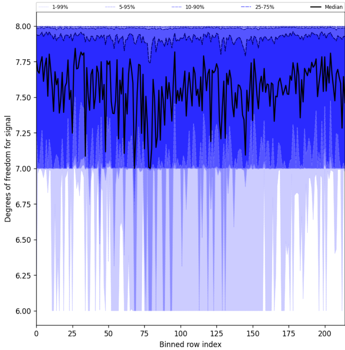
Figure 31: Along track statistics of “Degrees of freedom for signal” for 2025-05-17 to 2025-05-19
