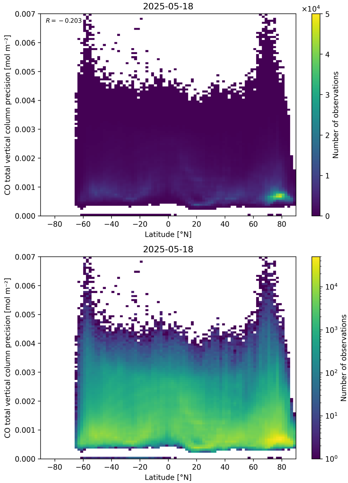
Figure 53: Scatter density plot of “Latitude” against “CO total vertical column precision” for 2025-05-17 to 2025-05-19.
