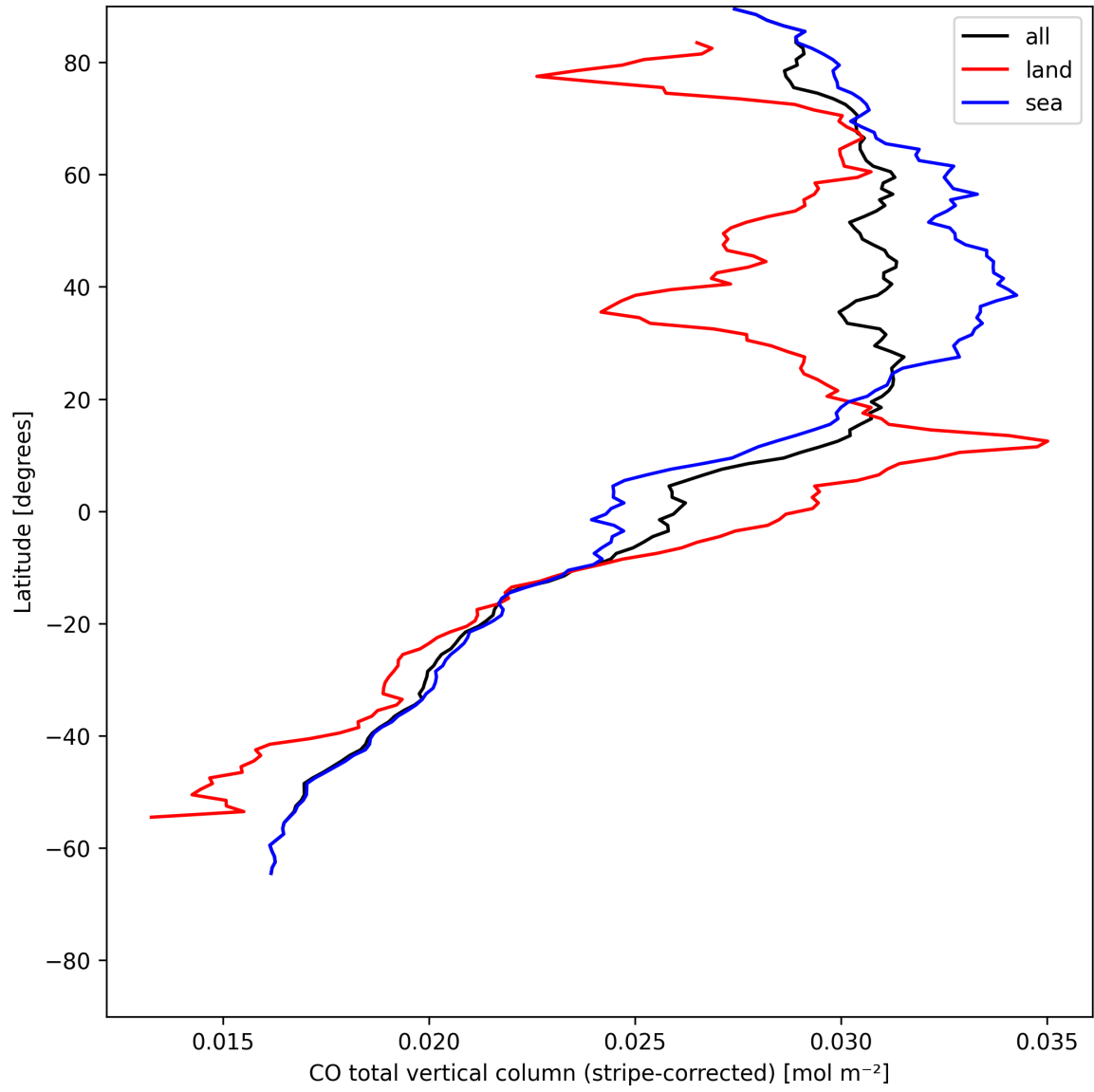
Figure 11: Zonal average of “CO total vertical column (stripe-corrected)” for 2025-05-17 to 2025-05-19.
