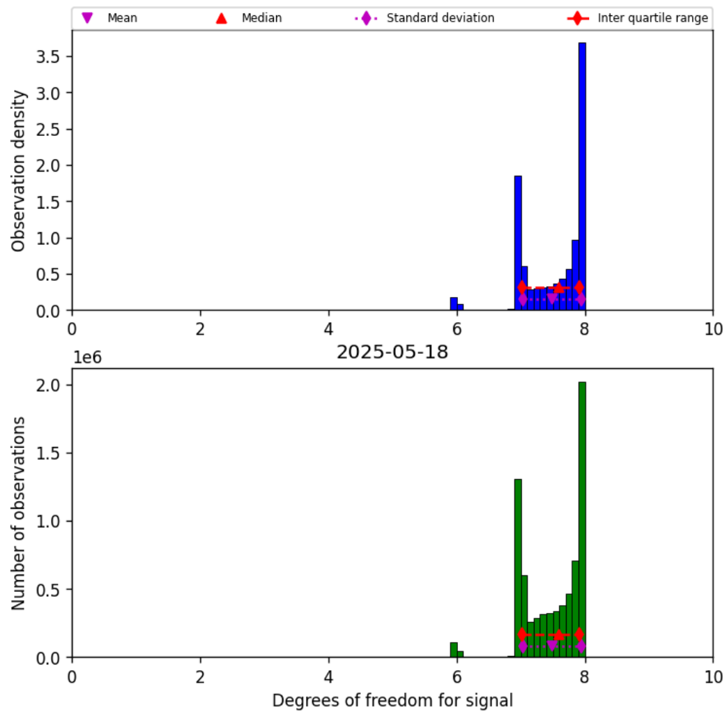
Figure 23: Histogram of “Degrees of freedom for signal” for 2025-05-17 to 2025-05-19
