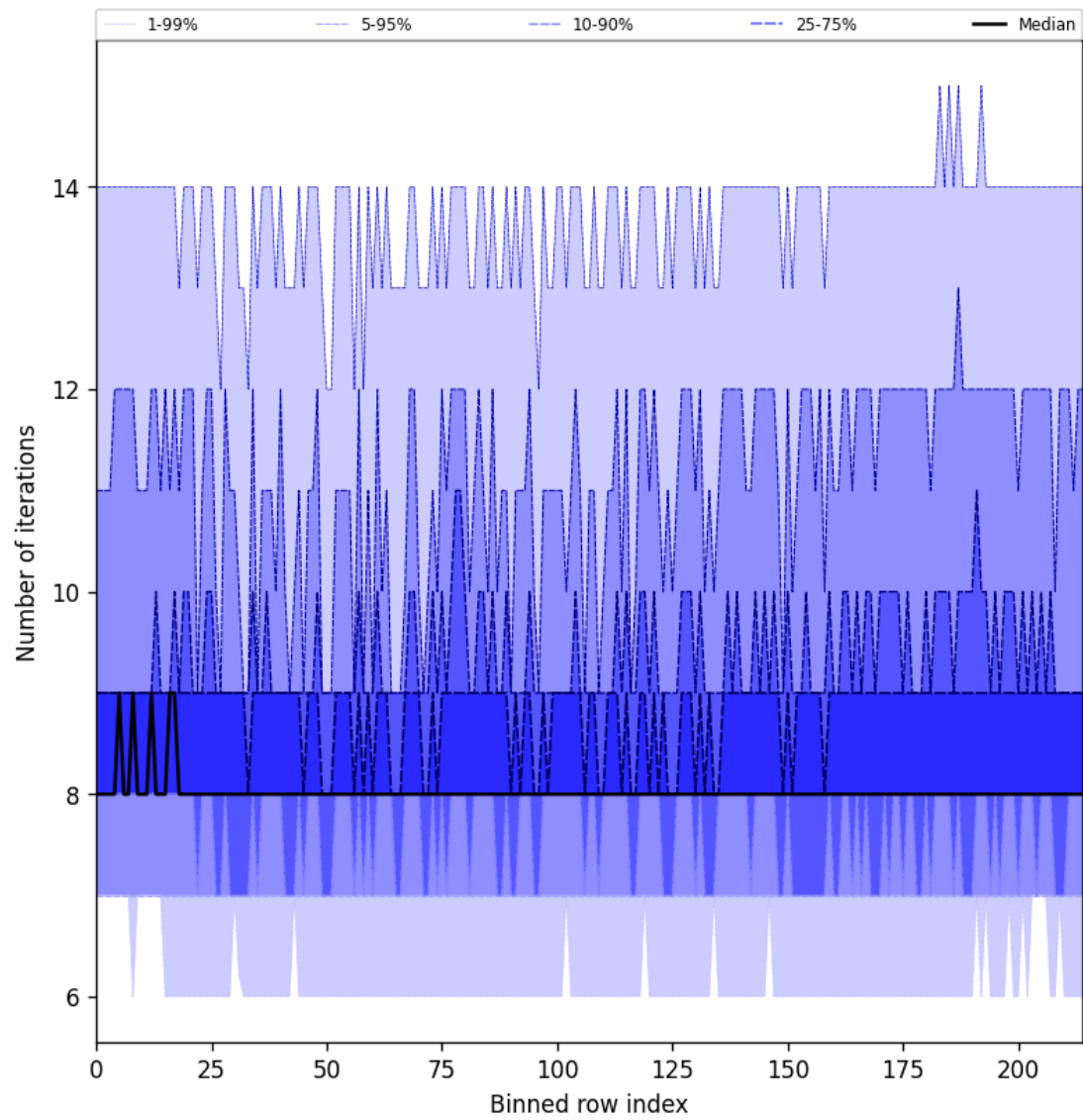
Figure 32: Along track statistics of “Number of iterations” for 2025-05-17 to 2025-05-19
