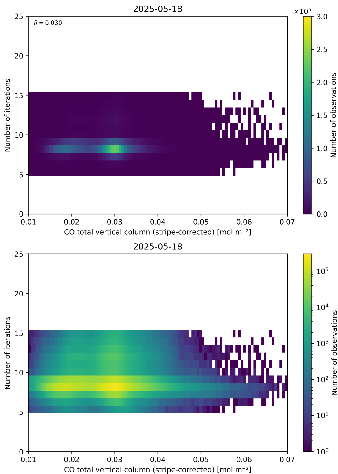
Figure 39: Scatter density plot of “CO total vertical column (stripe-corrected)” against “Number of iterations” for 2025-05-17 to 2025-05-19.
