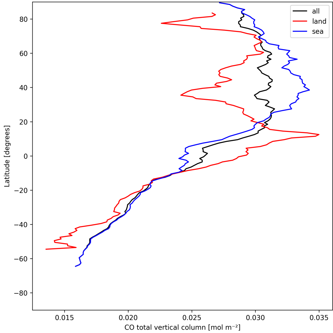
Figure 10: Zonal average of “CO total vertical column” for 2025-05-17 to 2025-05-19.
