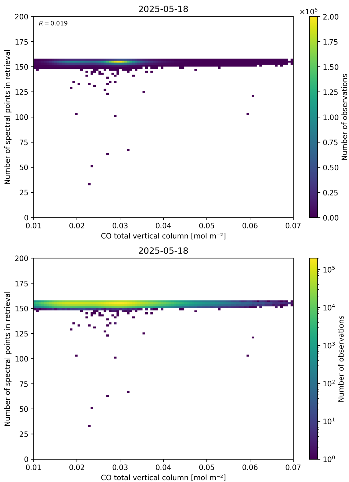
Figure 43: Scatter density plot of “CO total vertical column” against “Number of spectral points in retrieval” for 2025-05-17 to 2025-05-19.
