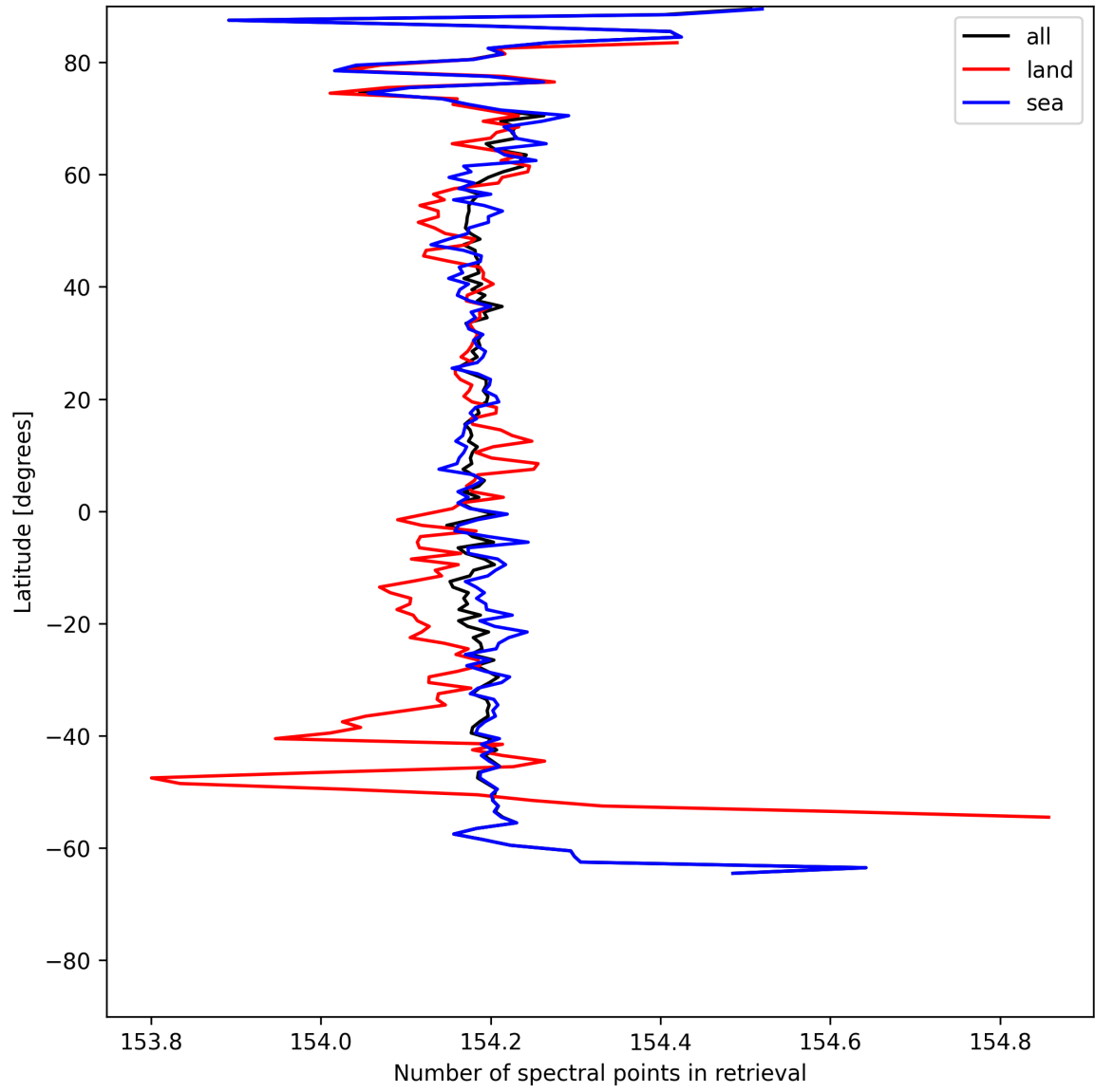
Figure 13: Zonal average of “Number of spectral points in retrieval” for 2025-05-17 to 2025-05-19.
