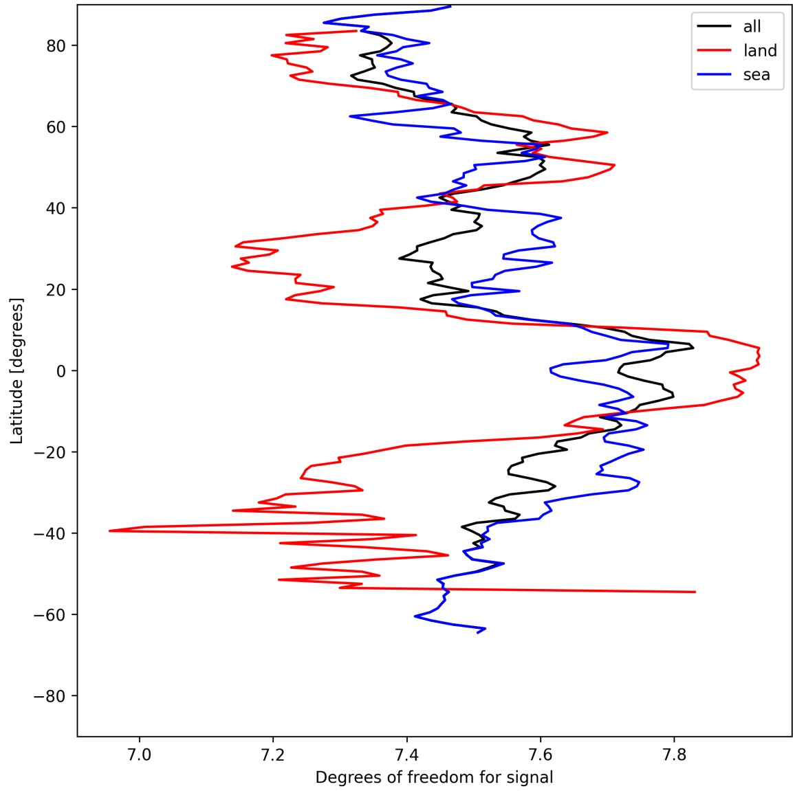
Figure 15: Zonal average of “Degrees of freedom for signal” for 2025-05-17 to 2025-05-19.
