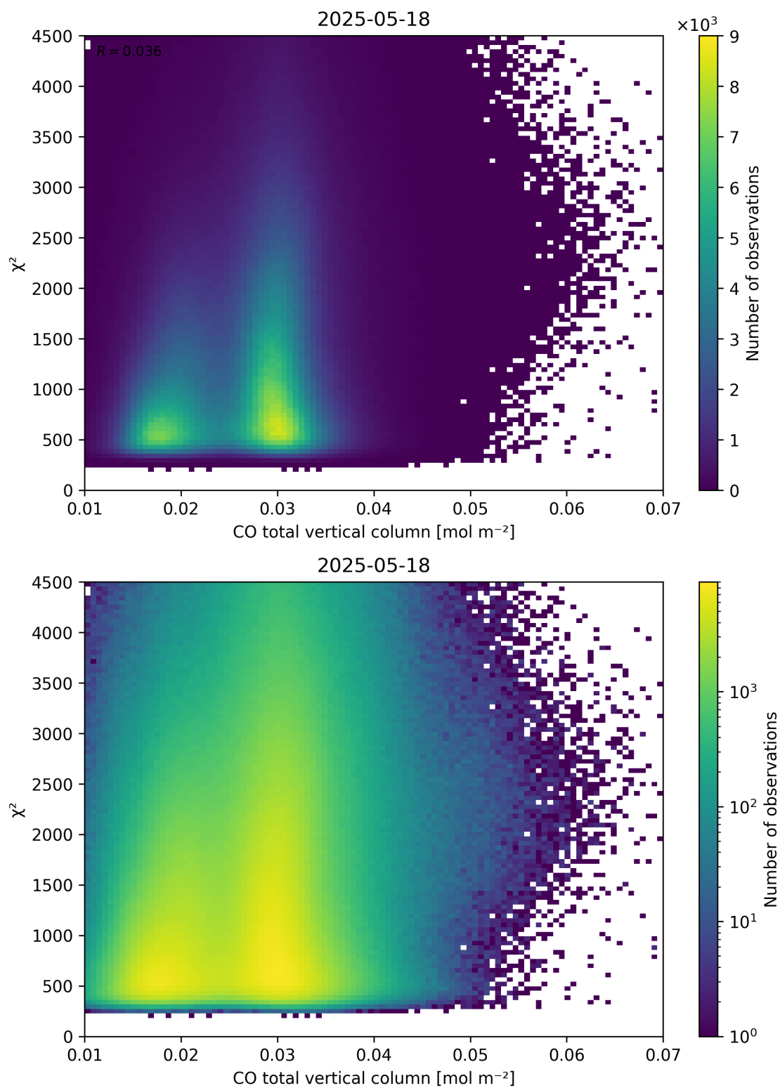
Figure 35: Scatter density plot of “CO total vertical column” against “ \chi^2 ” for 2025-05-17 to 2025-05-19.
