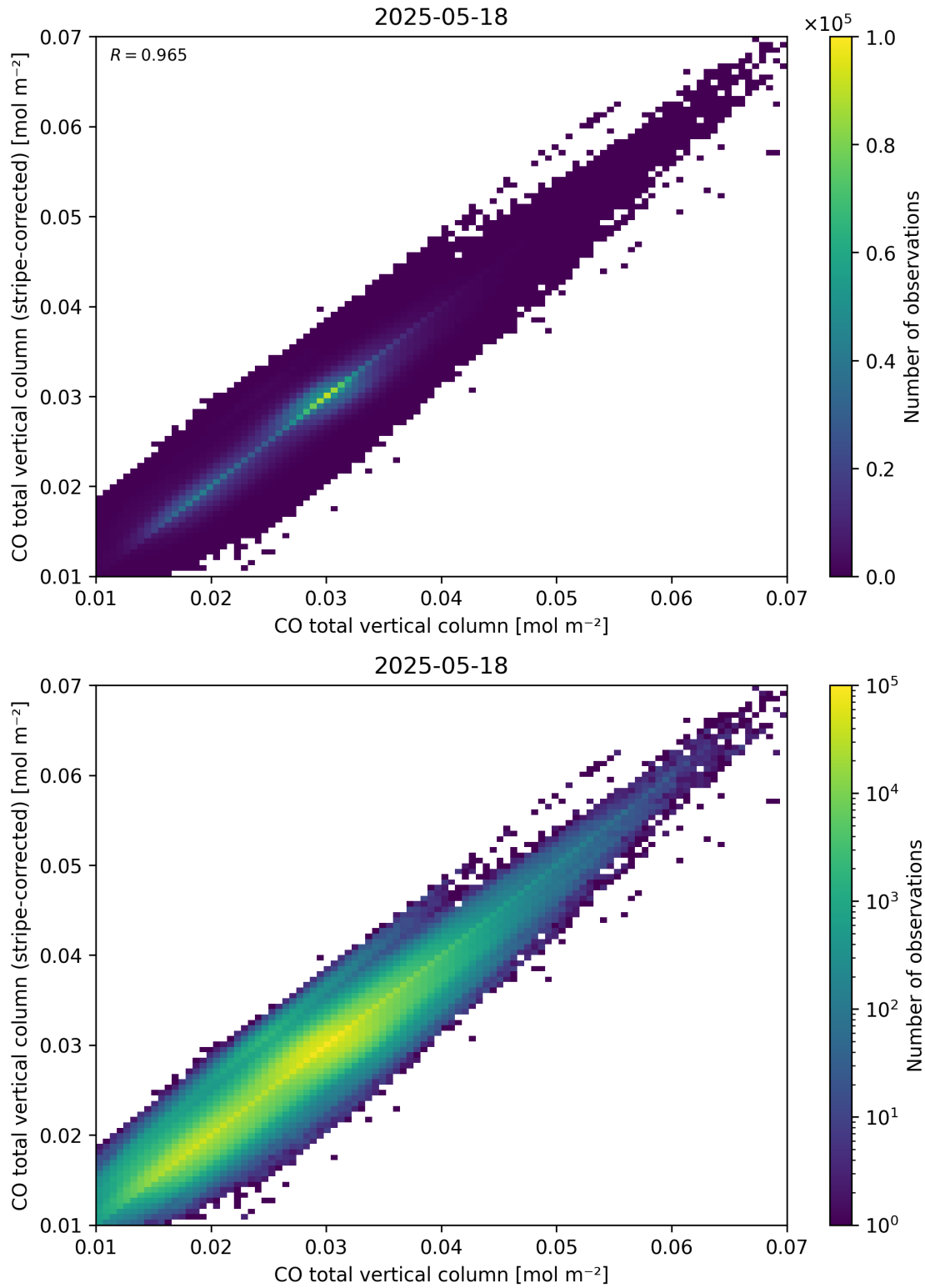
Figure 33: Scatter density plot of “CO total vertical column” against “CO total vertical column (stripe-corrected)” for 2025-05-17 to 2025-05-19.
