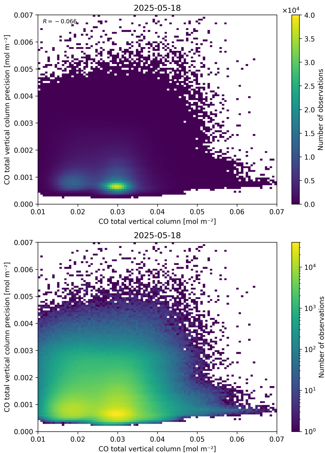
Figure 34: Scatter density plot of “CO total vertical column” against “CO total vertical column precision” for 2025-05-17 to 2025-05-19.
