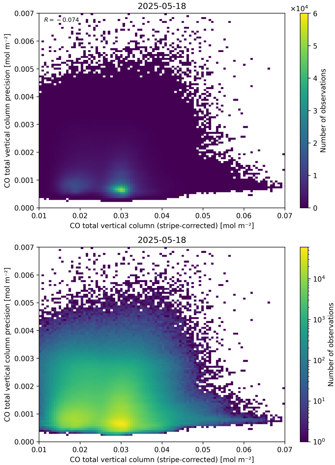
Figure 36: Scatter density plot of “CO total vertical column (stripe-corrected)” against “CO total vertical column precision” for 2025-05-17 to 2025-05-19.
