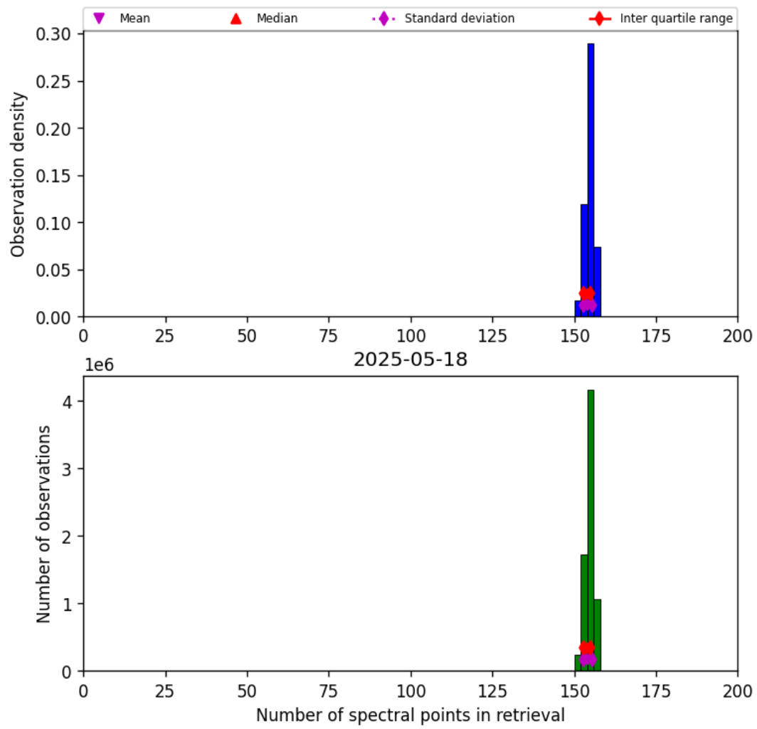
Figure 21: Histogram of “Number of spectral points in retrieval” for 2025-05-17 to 2025-05-19
