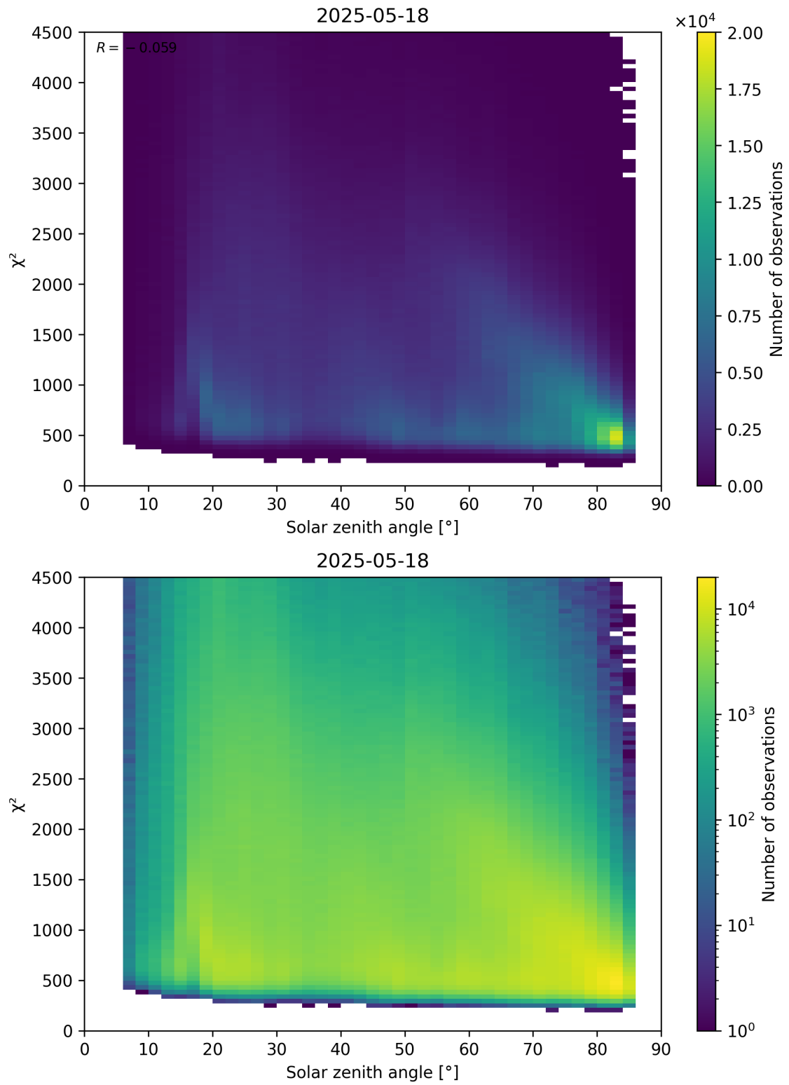
Figure 64: Scatter density plot of “Solar zenith angle” against “ \chi^2 ” for 2025-05-17 to 2025-05-19.
