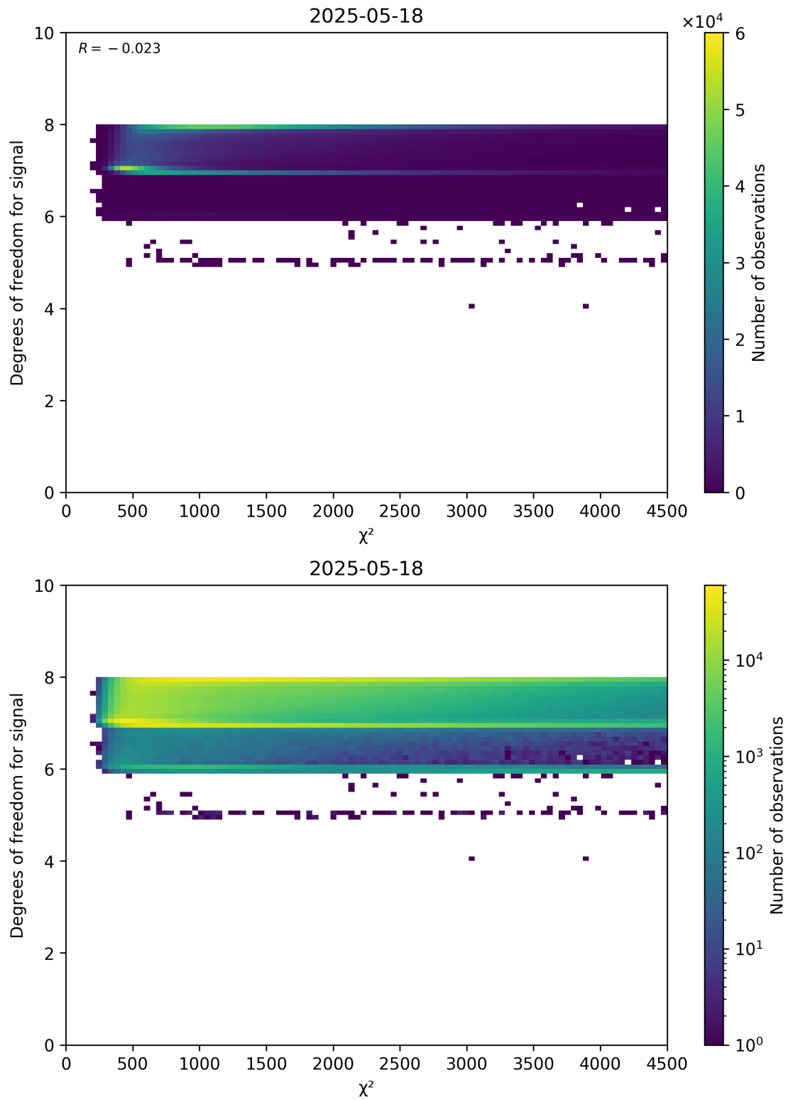
Figure 48: Scatter density plot of “ \chi^2 ” against “Degrees of freedom for signal” for 2025-05-17 to 2025-05-19.
