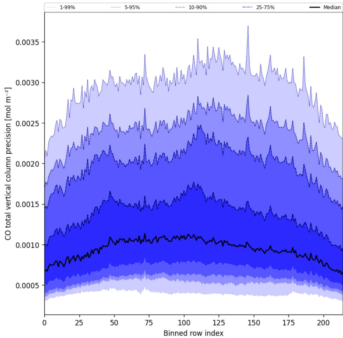
Figure 28: Along track statistics of "CO total vertical column precision" for 2025-05-17 to 2025-05-19
