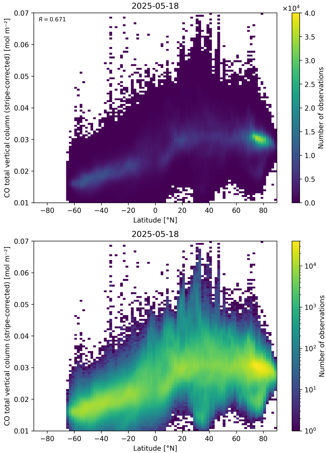
Figure 52: Scatter density plot of “Latitude” against “CO total vertical column (stripe-corrected)” for 2025-05-17 to 2025-05-19.
