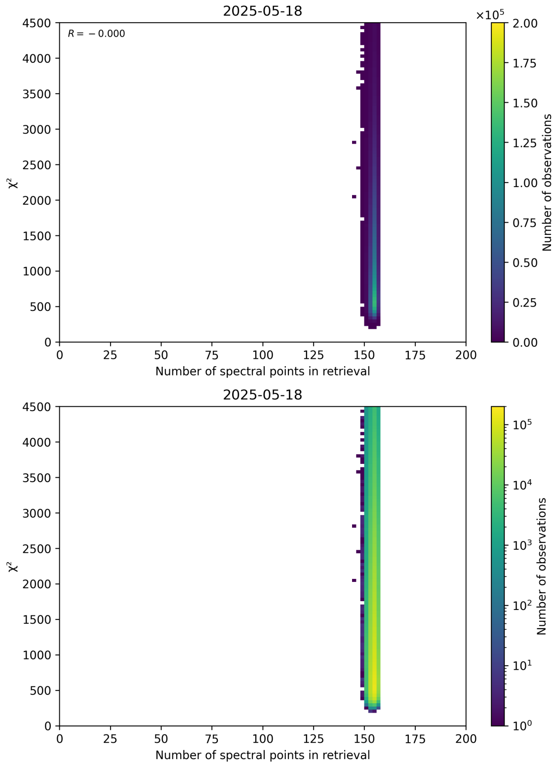
Figure 58: Scatter density plot of “Number of spectral points in retrieval” against “ \chi^2 ” for 2025-05-17 to 2025-05-19.
