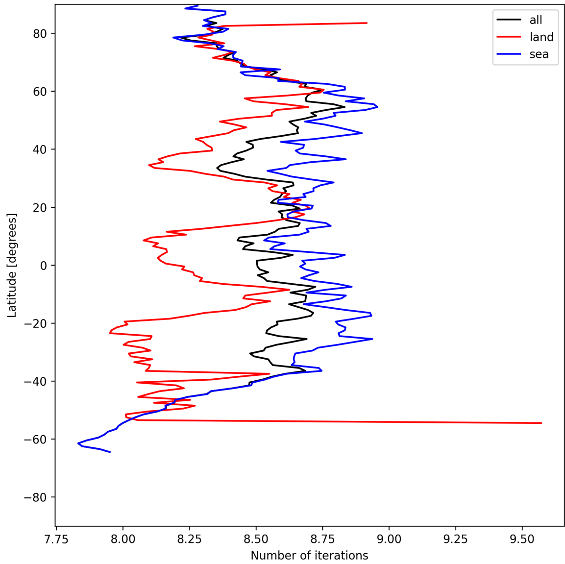
Figure 16: Zonal average of “Number of iterations” for 2025-05-17 to 2025-05-19.
