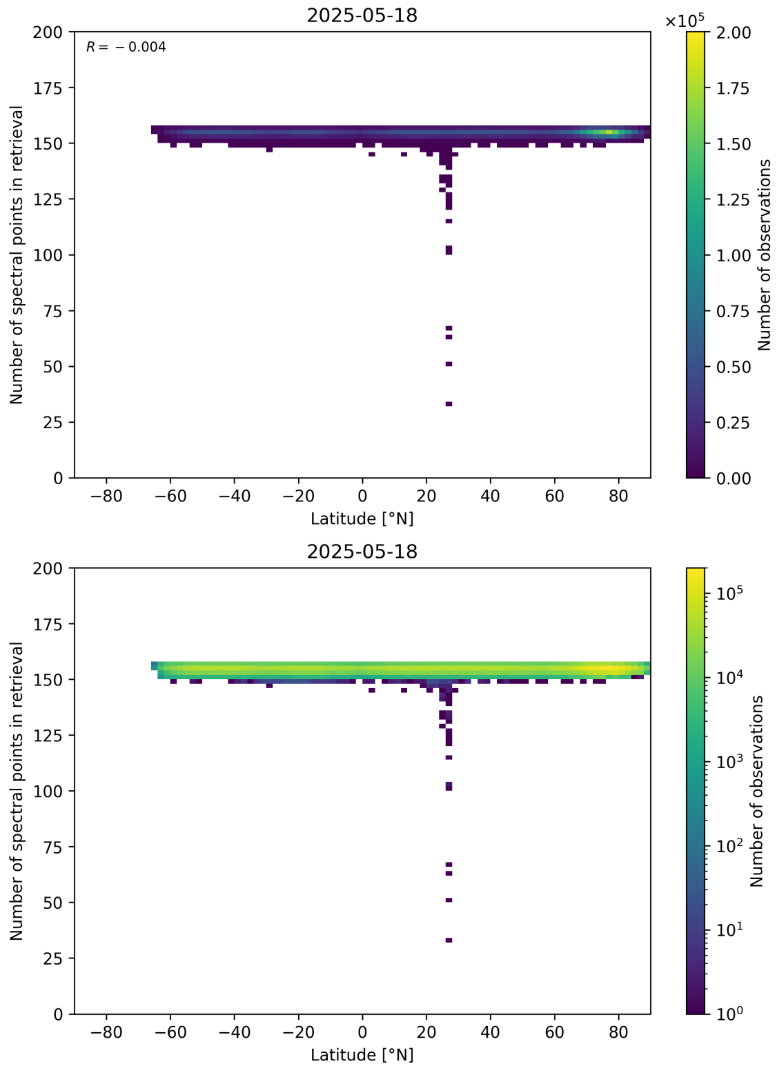
Figure 57: Scatter density plot of “Latitude” against “Number of spectral points in retrieval” for 2025-05-17 to 2025-05-19.
