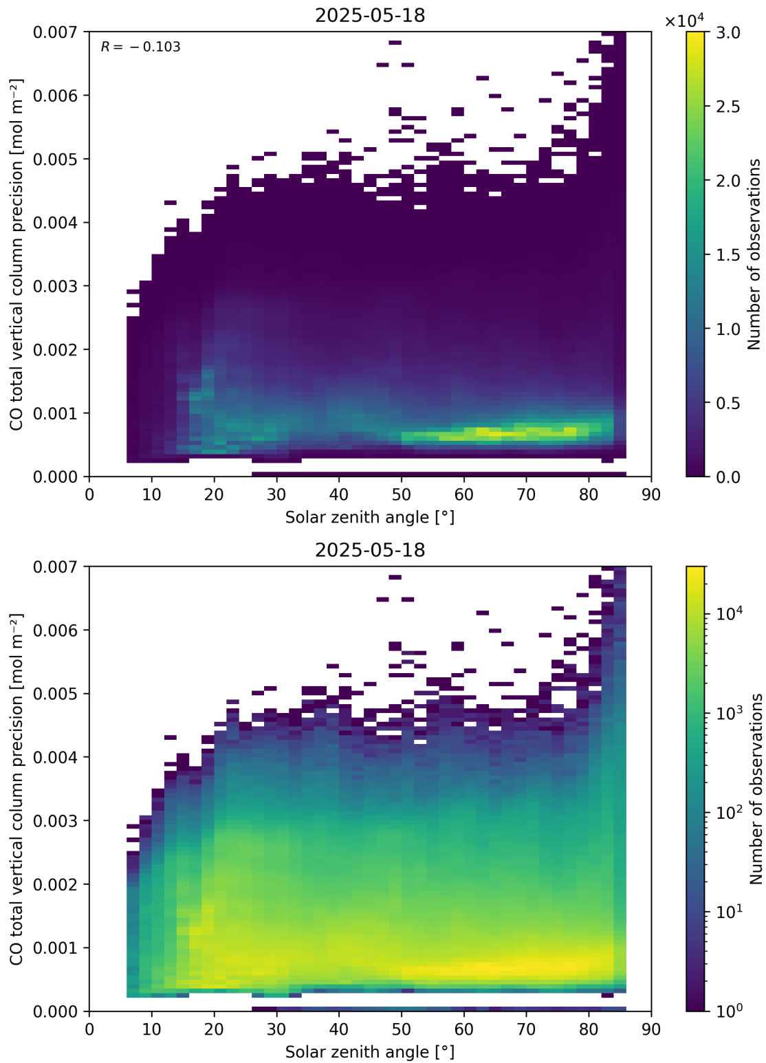
Figure 63: Scatter density plot of “Solar zenith angle” against “CO total vertical column precision” for 2025-05-17 to 2025-05-19.
