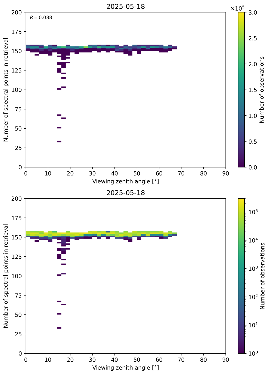
Figure 76: Scatter density plot of “Viewing zenith angle” against “Number of spectral points in retrieval” for 2025-05-17 to 2025-05-19.
