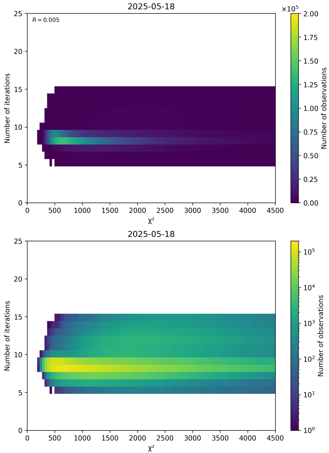
Figure 49: Scatter density plot of “ \chi^2 ” against “Number of iterations” for 2025-05-17 to 2025-05-19.
