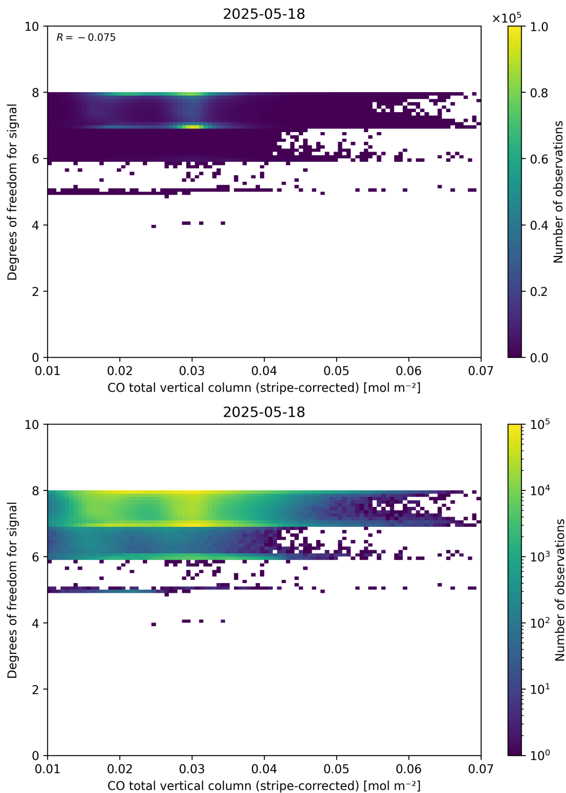
Figure 38: Scatter density plot of “CO total vertical column (stripe-corrected)” against “Degrees of freedom for signal” for 2025-05-17 to 2025-05-19.
