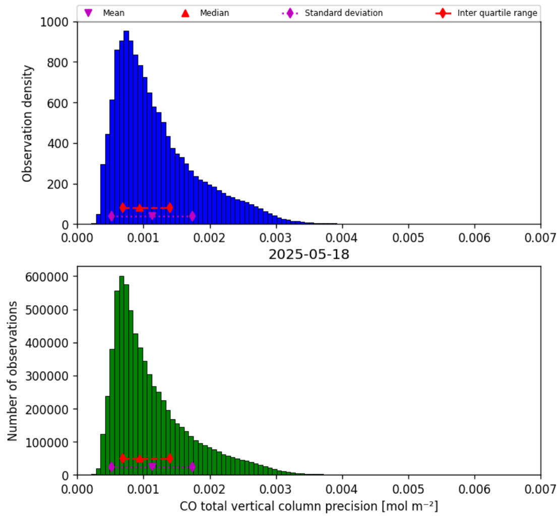
Figure 20: Histogram of “CO total vertical column precision” for 2025-05-17 to 2025-05-19
