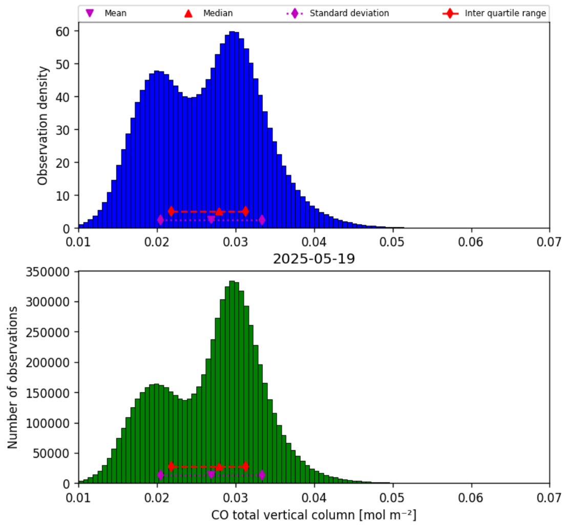
Figure 18: Histogram of “CO total vertical column” for 2025-05-18 to 2025-05-20
