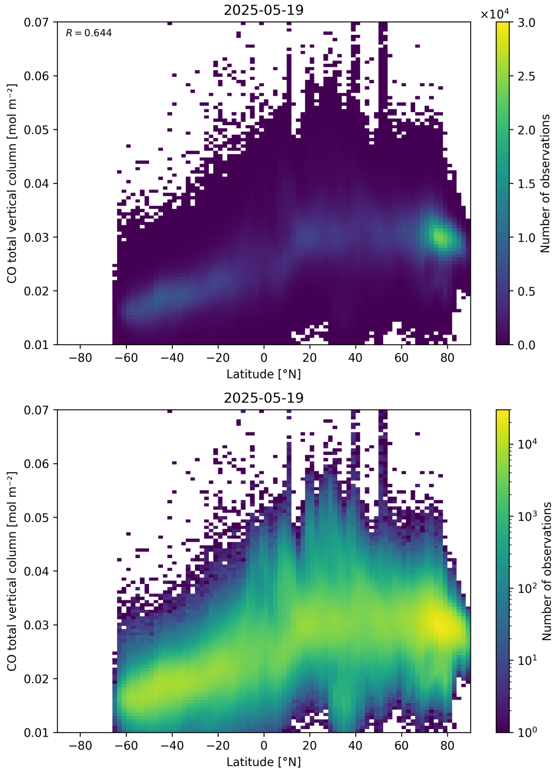
Figure 51: Scatter density plot of “Latitude” against “CO total vertical column” for 2025-05-18 to 2025-05-20.
