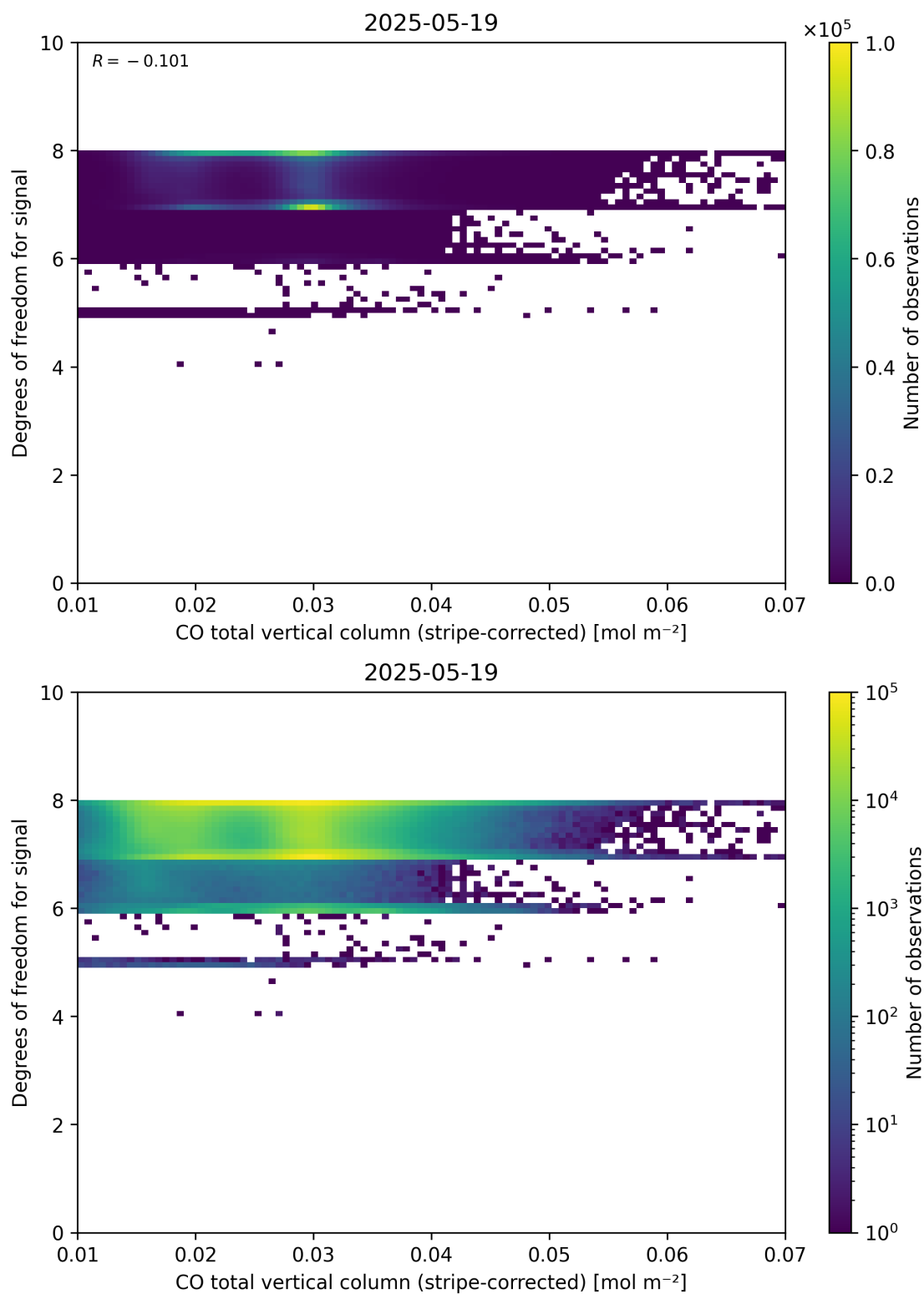
Figure 38: Scatter density plot of “CO total vertical column (stripe-corrected)” against “Degrees of freedom for signal” for 2025-05-18 to 2025-05-20.
