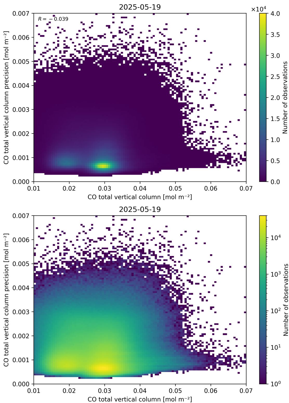
Figure 34: Scatter density plot of “CO total vertical column” against “CO total vertical column precision” for 2025-05-18 to 2025-05-20.
