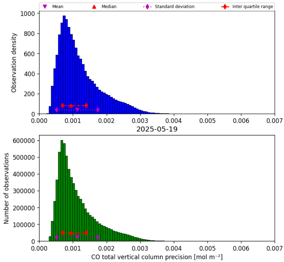
Figure 20: Histogram of “CO total vertical column precision” for 2025-05-18 to 2025-05-20
