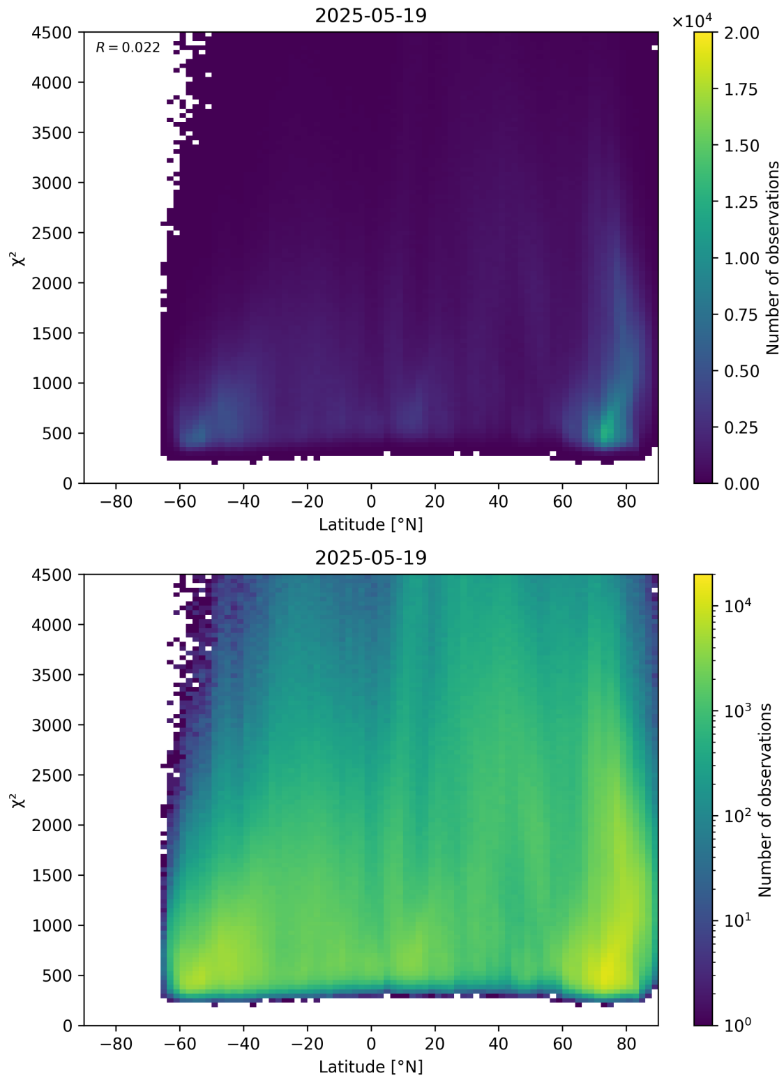
Figure 54: Scatter density plot of “Latitude” against “ \chi^2 ” for 2025-05-18 to 2025-05-20.
