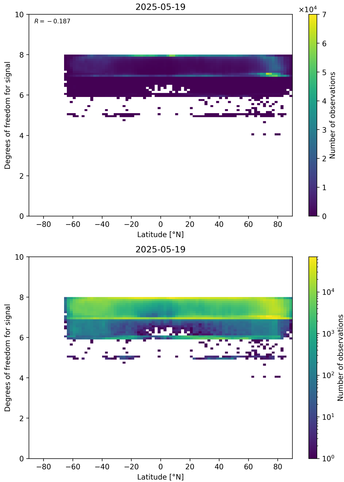
Figure 55: Scatter density plot of “Latitude” against “Degrees of freedom for signal” for 2025-05-18 to 2025-05-20.
