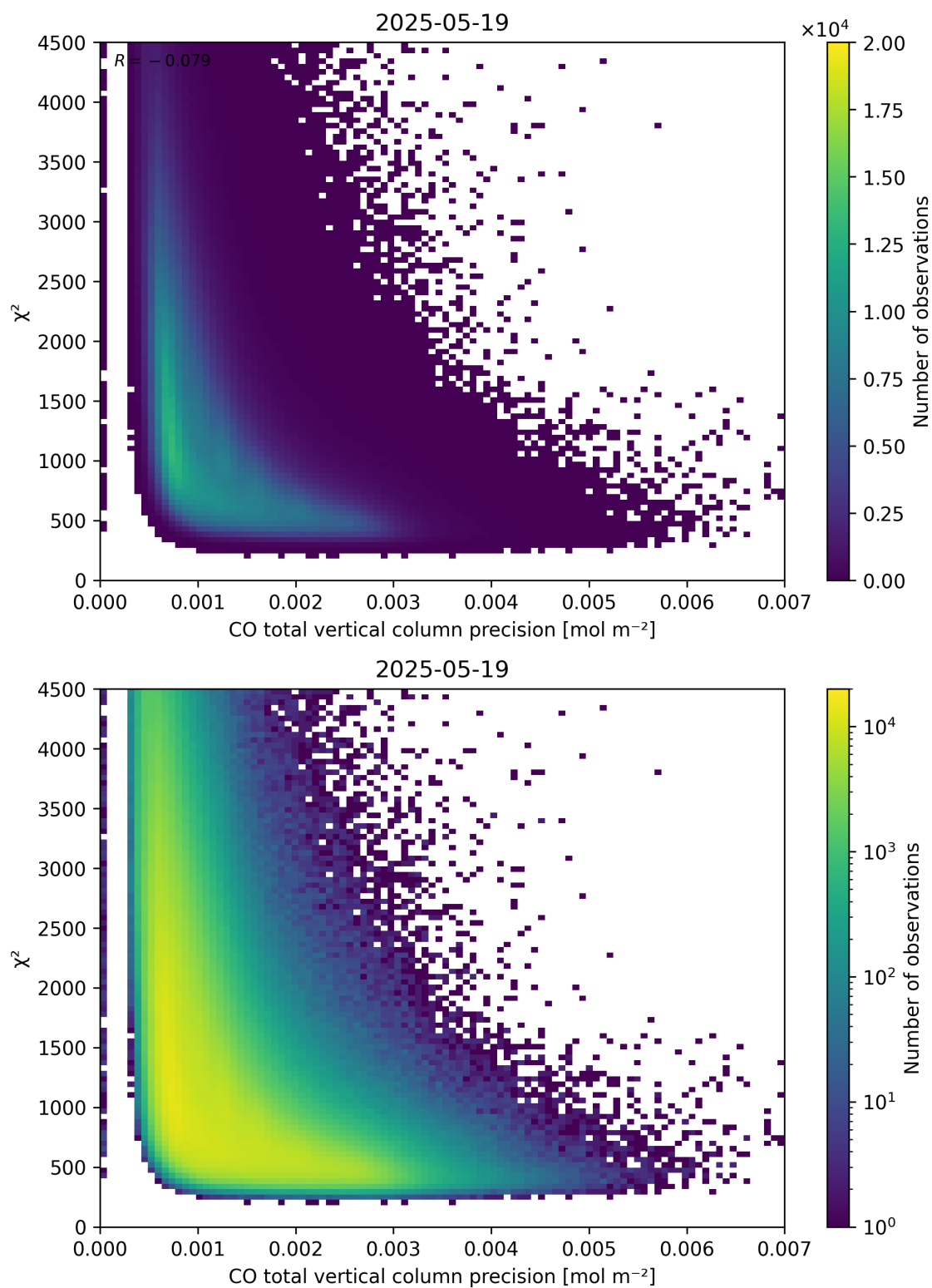
Figure 44: Scatter density plot of “CO total vertical column precision” against “ \chi^2 ” for 2025-05-18 to 2025-05-20.
