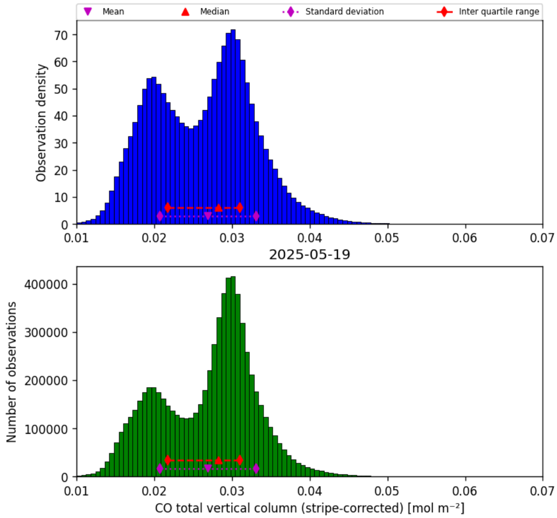
Figure 19: Histogram of “CO total vertical column (stripe-corrected)” for 2025-05-18 to 2025-05-20
