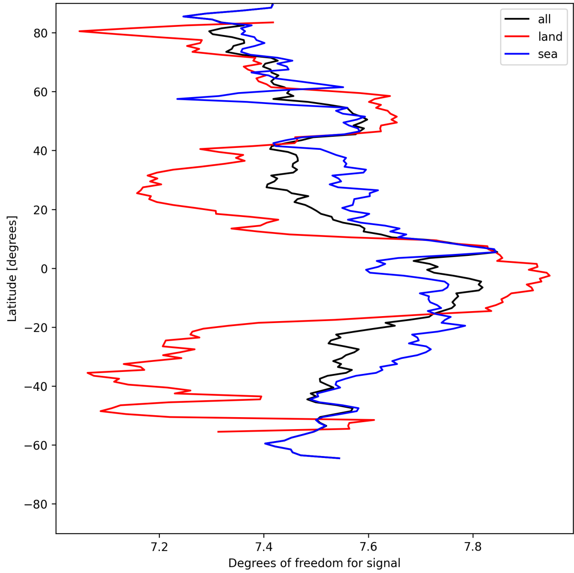
Figure 15: Zonal average of “Degrees of freedom for signal” for 2025-05-18 to 2025-05-20.
