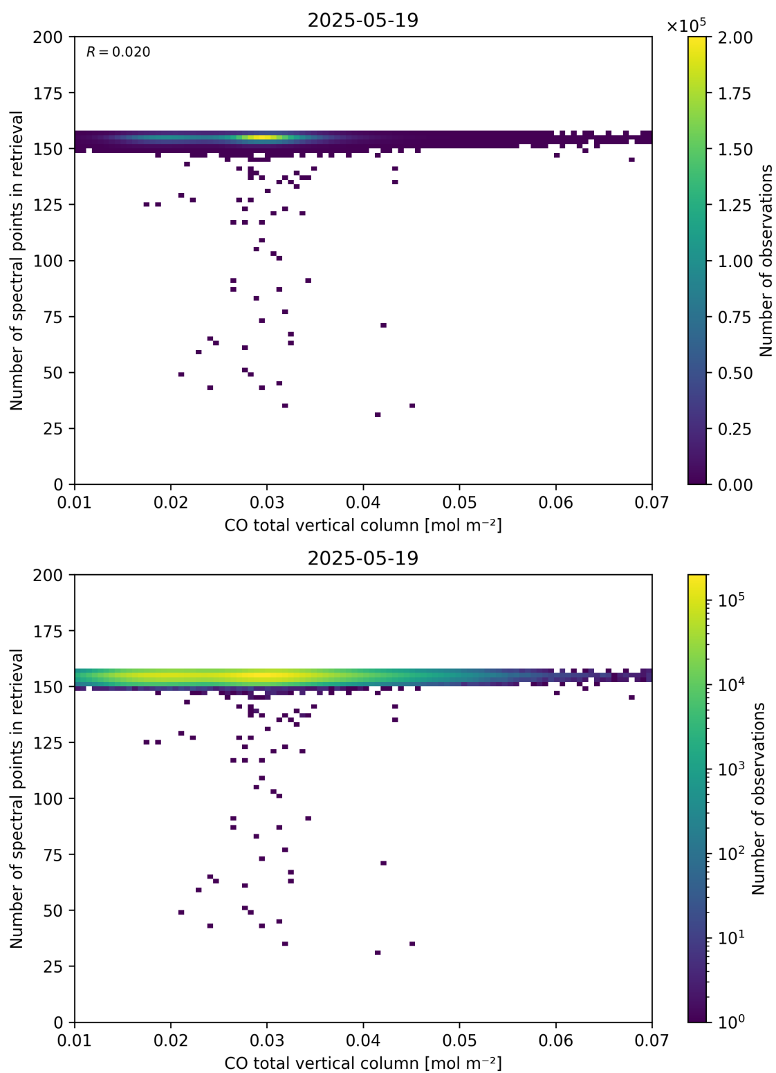
Figure 43: Scatter density plot of “CO total vertical column” against “Number of spectral points in retrieval” for 2025-05-18 to 2025-05-20.
