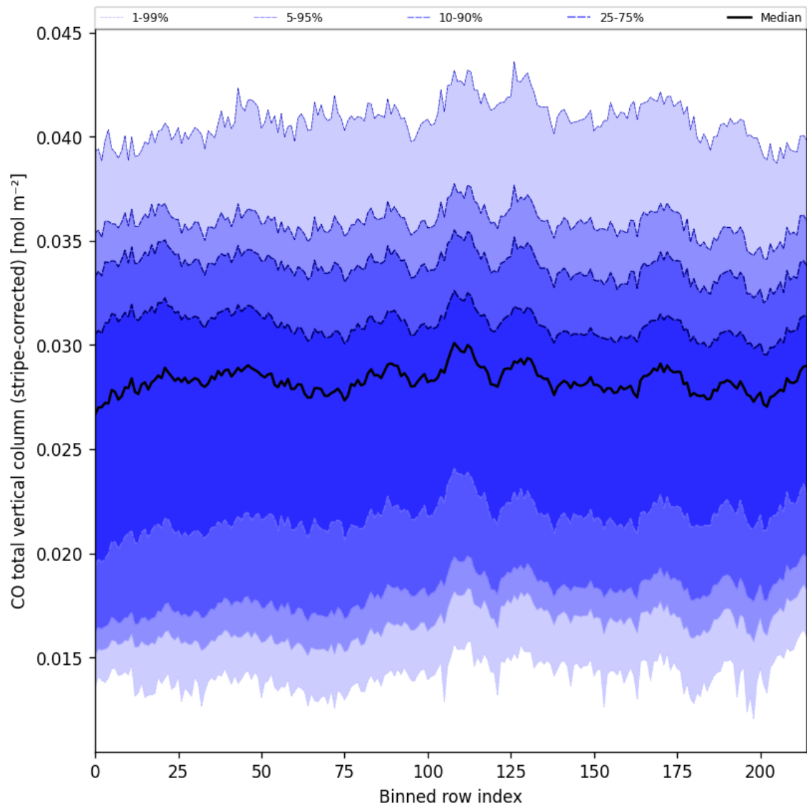
Figure 27: Along track statistics of “CO total vertical column (stripe-corrected)” for 2025-05-18 to 2025-05-20
