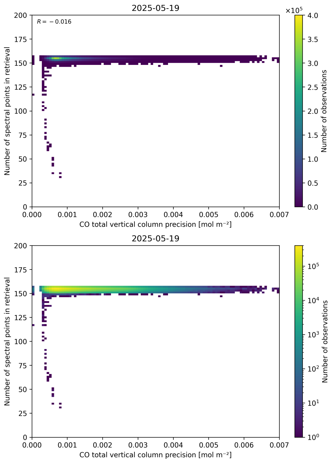
Figure 47: Scatter density plot of “CO total vertical column precision” against “Number of spectral points in retrieval” for 2025-05-18 to 2025-05-20.
