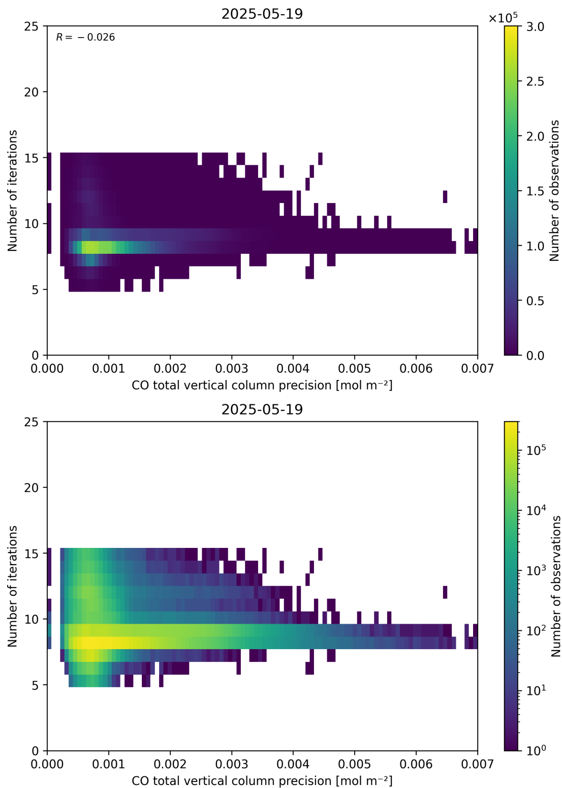
Figure 46: Scatter density plot of “CO total vertical column precision” against “Number of iterations” for 2025-05-18 to 2025-05-20.
