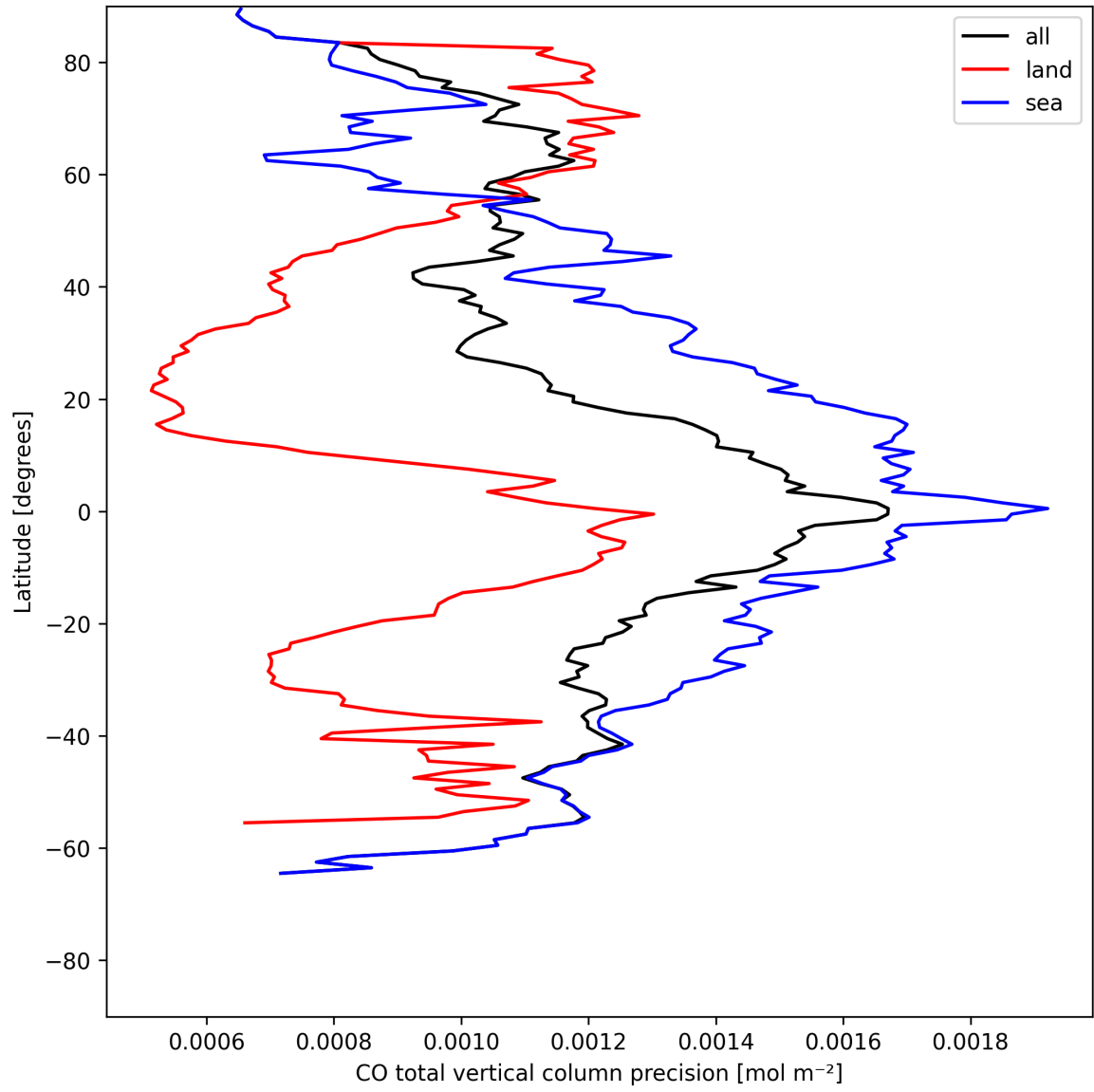
Figure 12: Zonal average of “CO total vertical column precision” for 2025-05-18 to 2025-05-20.
