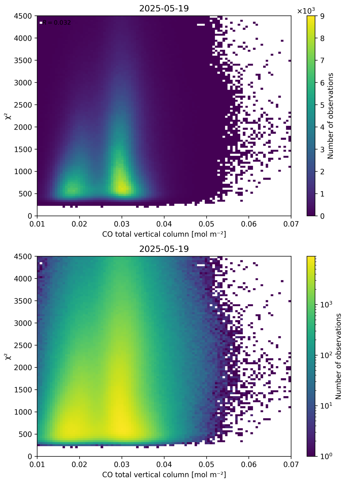
Figure 35: Scatter density plot of “CO total vertical column” against “ \chi^2 ” for 2025-05-18 to 2025-05-20.
