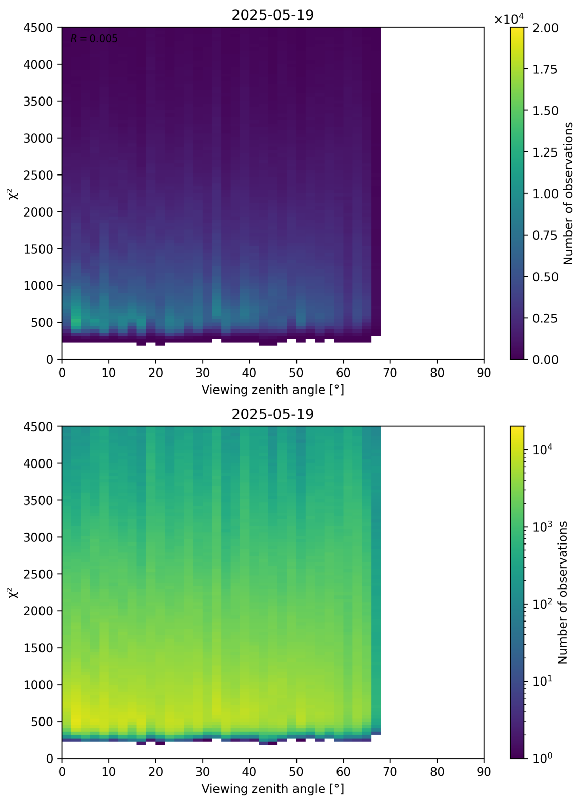
Figure 72: Scatter density plot of “Viewing zenith angle” against “ \chi^2 ” for 2025-05-18 to 2025-05-20.
