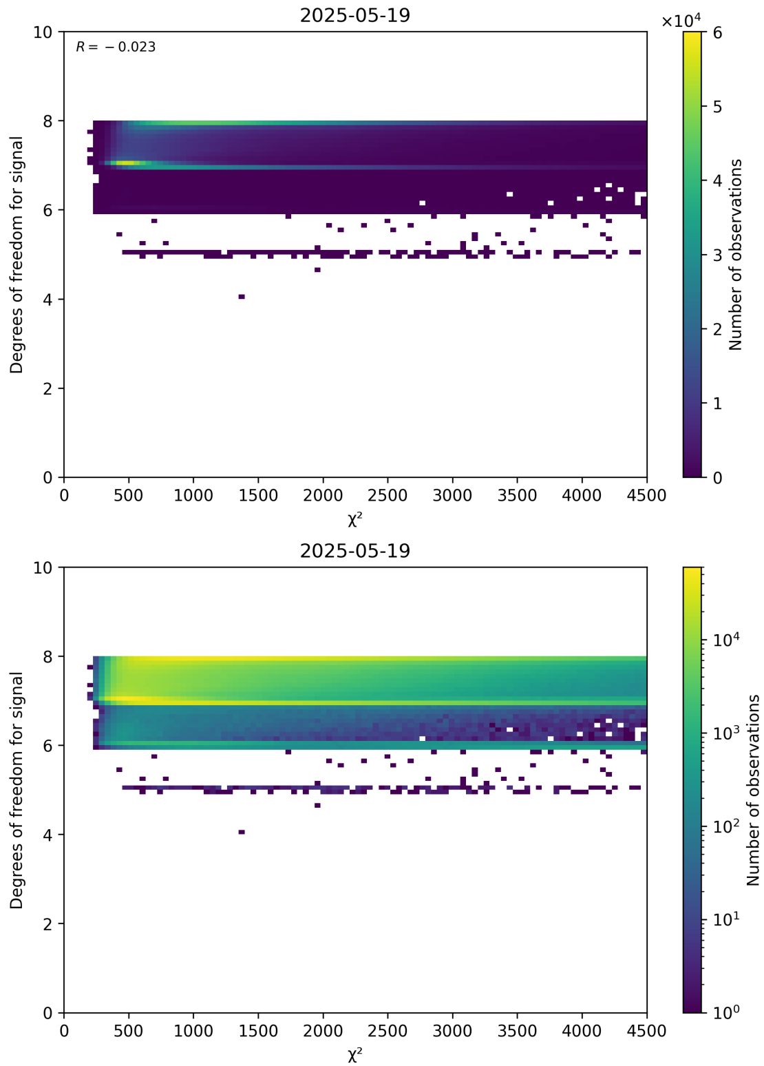
Figure 48: Scatter density plot of “ \chi^2 ” against “Degrees of freedom for signal” for 2025-05-18 to 2025-05-20.
