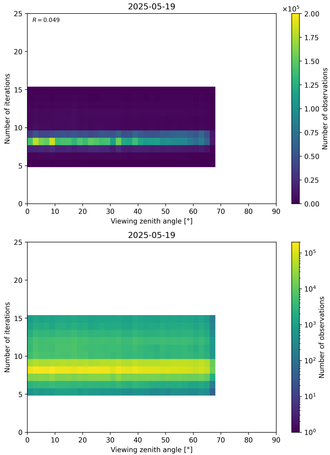
Figure 75: Scatter density plot of “Viewing zenith angle” against “Number of iterations” for 2025-05-18 to 2025-05-20.
