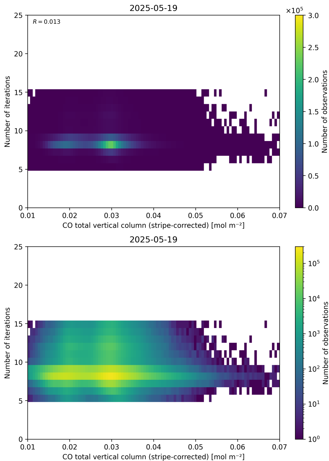
Figure 39: Scatter density plot of “CO total vertical column (stripe-corrected)” against “Number of iterations” for 2025-05-18 to 2025-05-20.
