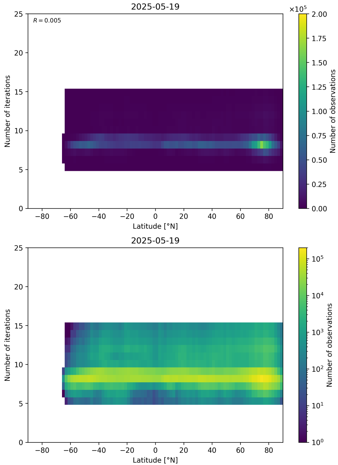
Figure 56: Scatter density plot of “Latitude” against “Number of iterations” for 2025-05-18 to 2025-05-20.
