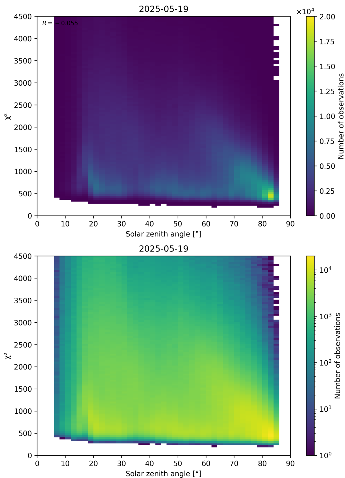
Figure 64: Scatter density plot of “Solar zenith angle” against “ \chi^2 ” for 2025-05-18 to 2025-05-20.
