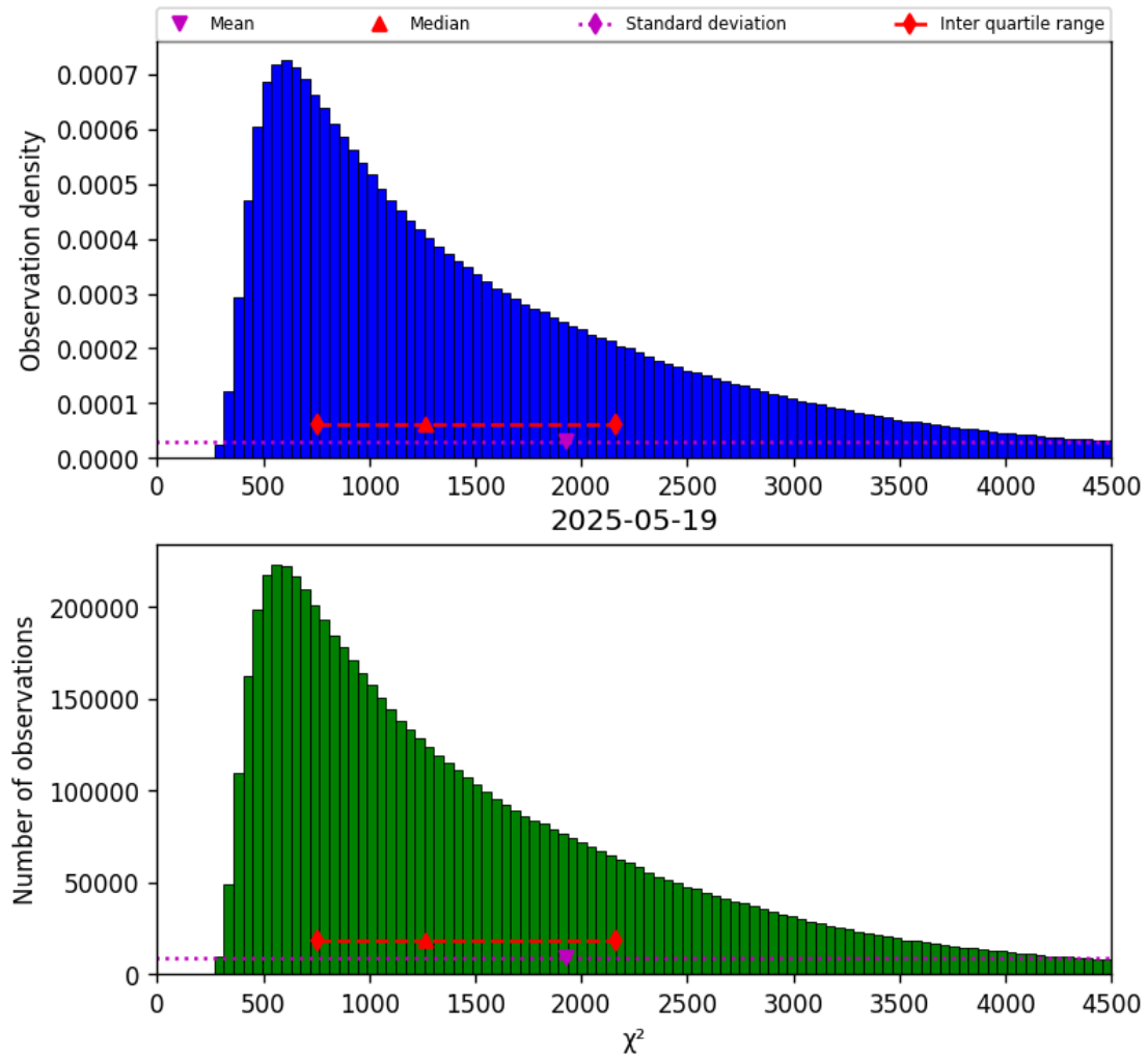
Figure 22: Histogram of “ \chi^2 ” for 2025-05-18 to 2025-05-20
