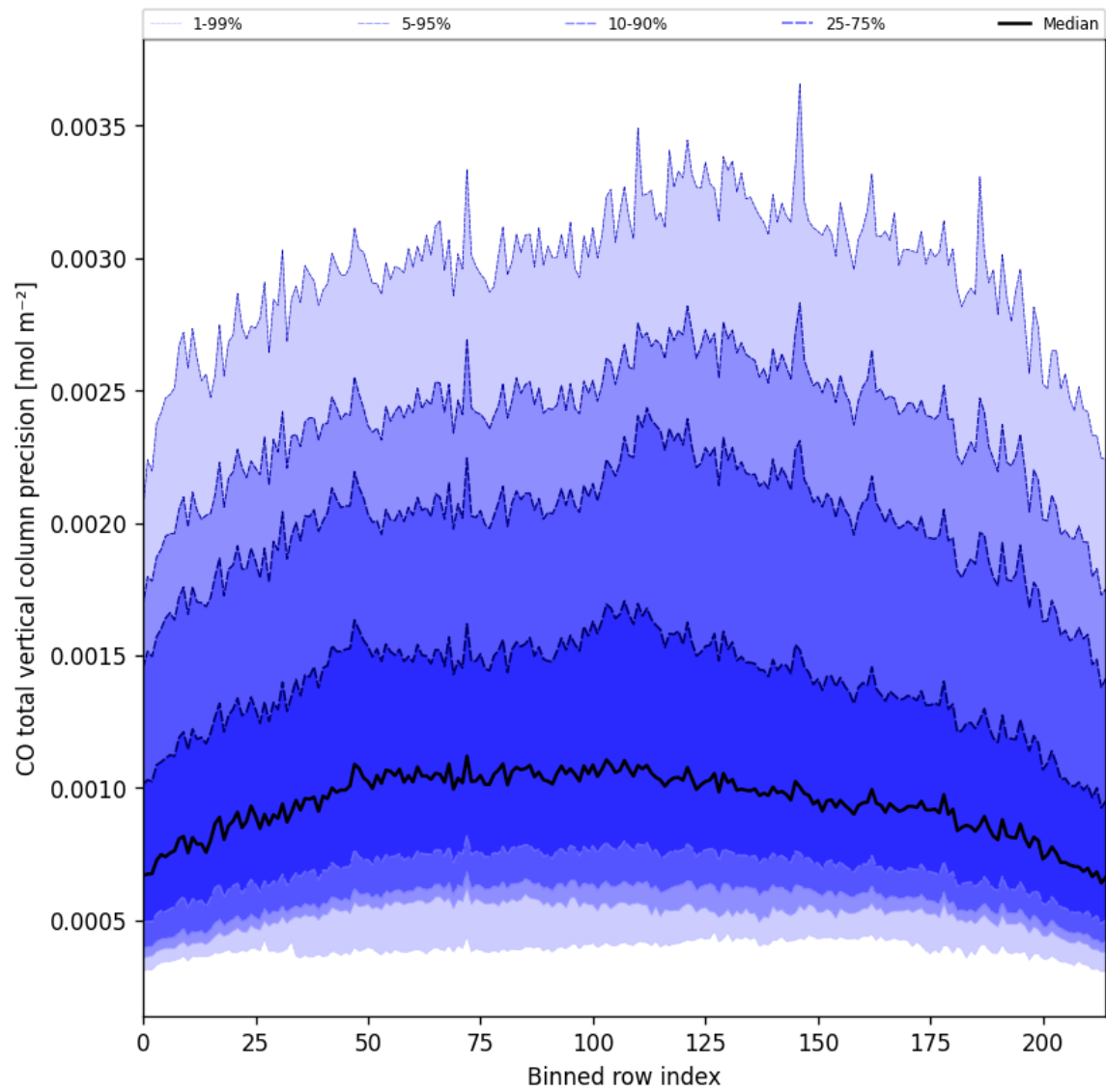
Figure 28: Along track statistics of “CO total vertical column precision” for 2025-05-18 to 2025-05-20
