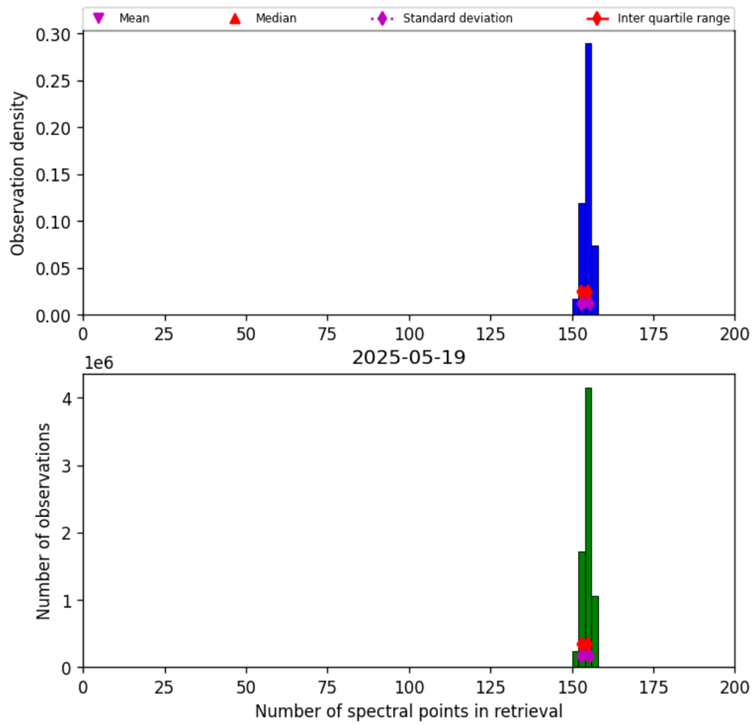
Figure 21: Histogram of “Number of spectral points in retrieval” for 2025-05-18 to 2025-05-20
