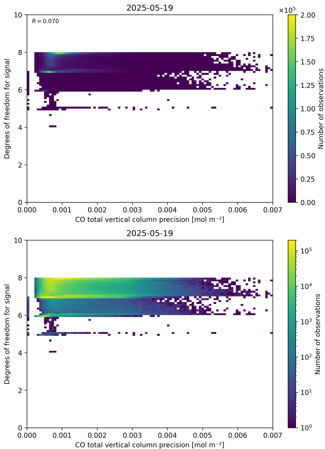
Figure 45: Scatter density plot of “CO total vertical column precision” against “Degrees of freedom for signal” for 2025-05-18 to 2025-05-20.
