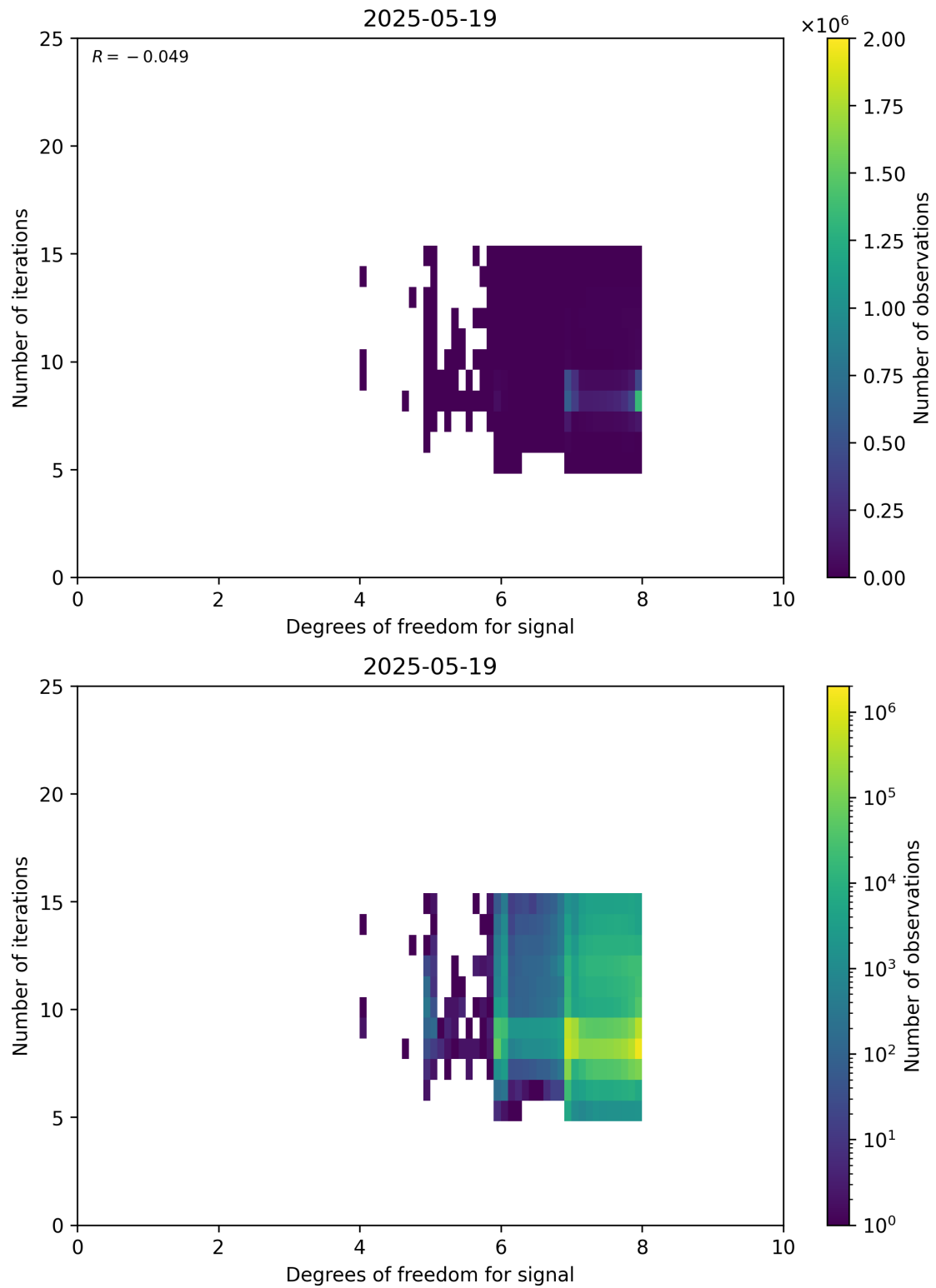
Figure 50: Scatter density plot of “Degrees of freedom for signal” against “Number of iterations” for 2025-05-18 to 2025-05-20.
