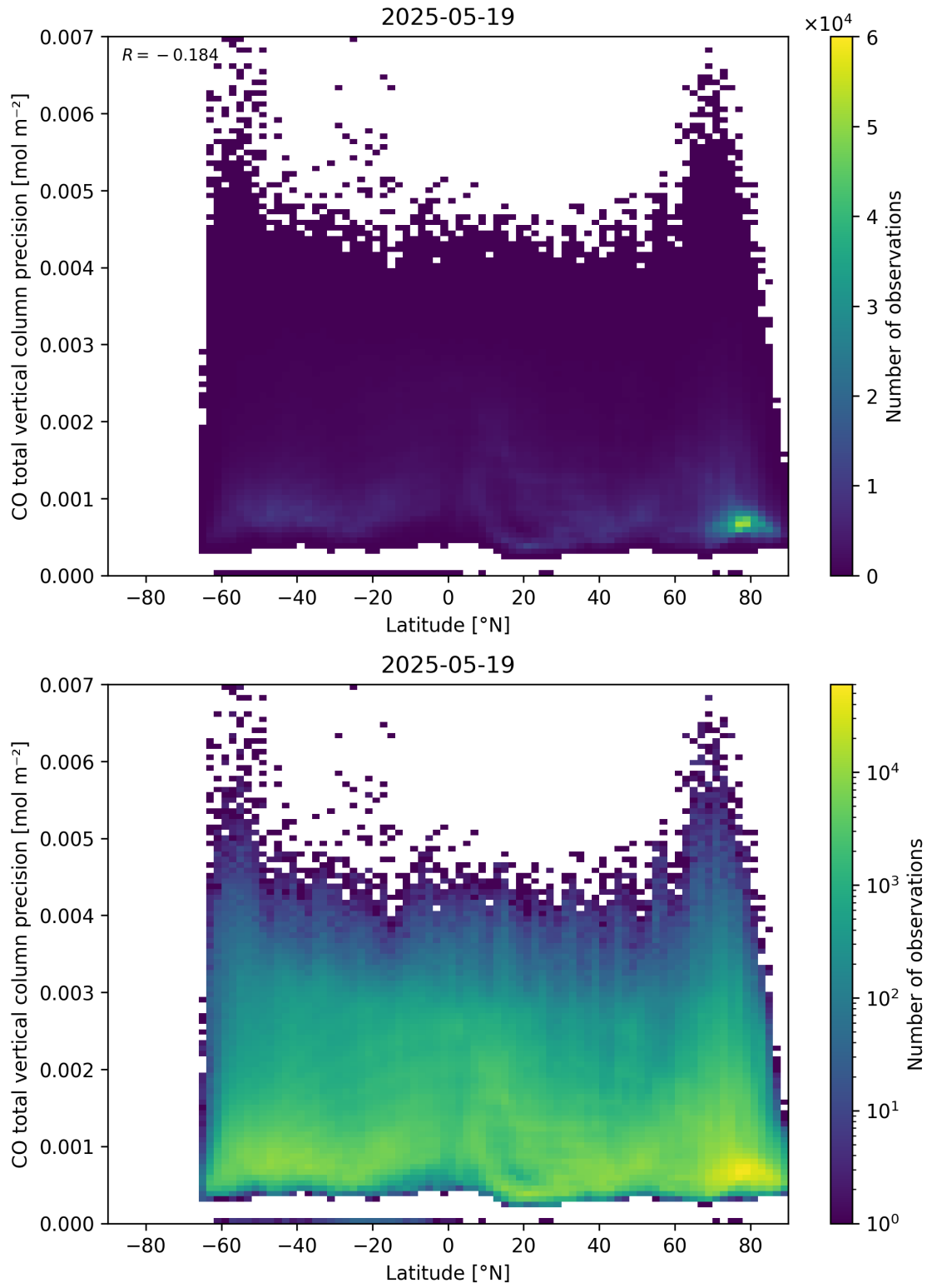
Figure 53: Scatter density plot of “Latitude” against “CO total vertical column precision” for 2025-05-18 to 2025-05-20.
