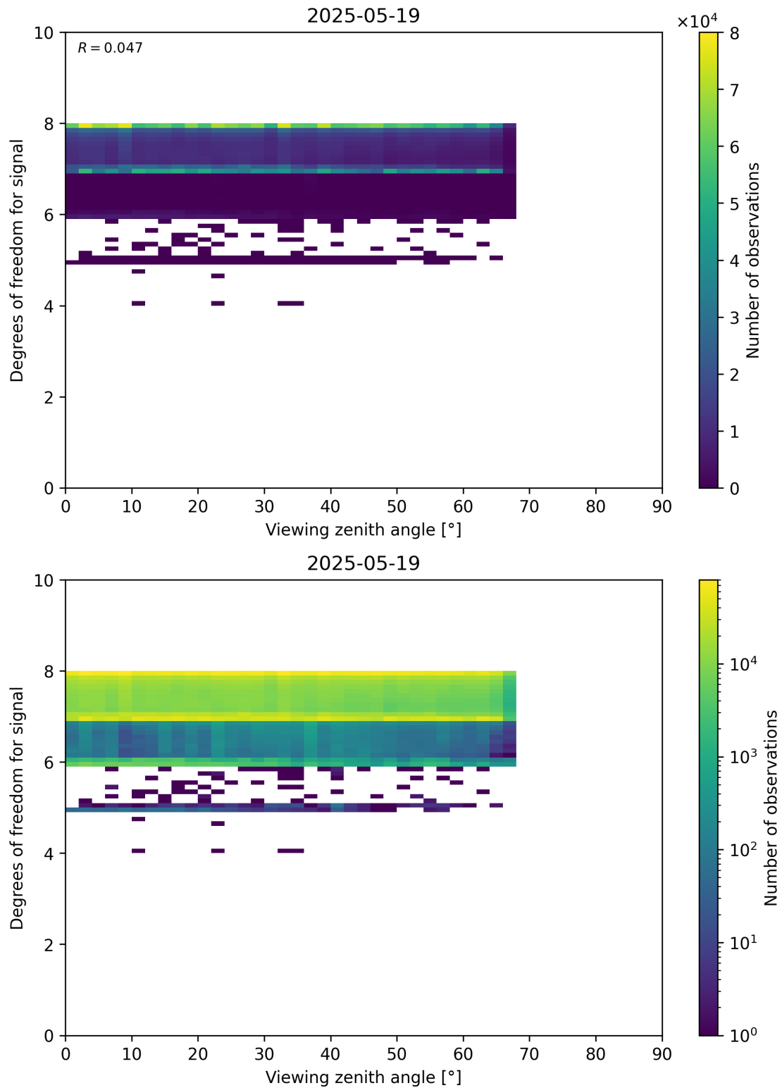
Figure 73: Scatter density plot of “Viewing zenith angle” against “Degrees of freedom for signal” for 2025-05-18 to 2025-05-20.
