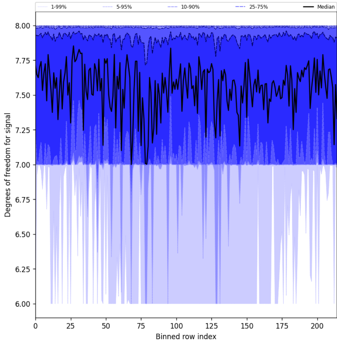
Figure 31: Along track statistics of “Degrees of freedom for signal” for 2025-05-18 to 2025-05-20
