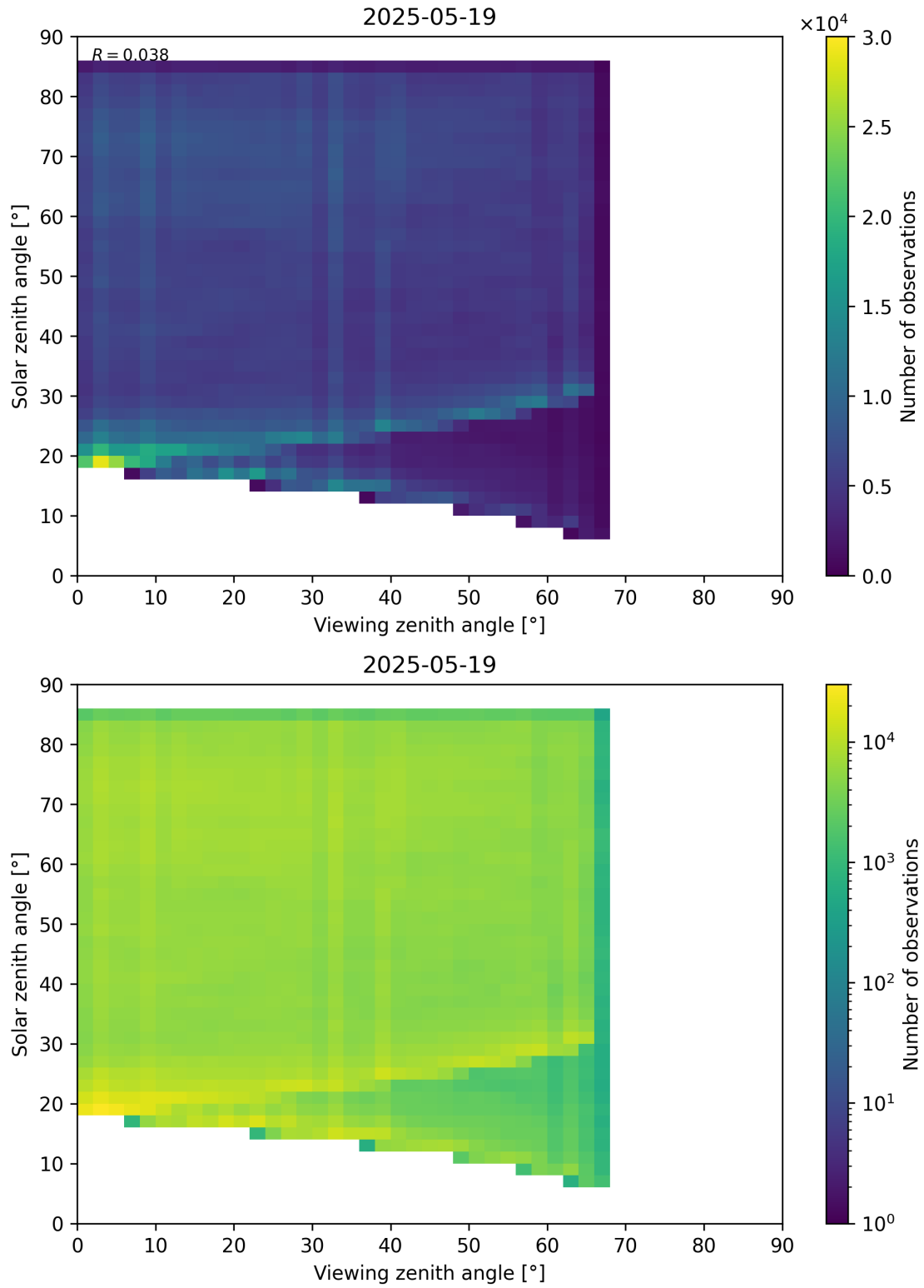
Figure 77: Scatter density plot of “Viewing zenith angle” against “Solar zenith angle” for 2025-05-18 to 2025-05-20.
