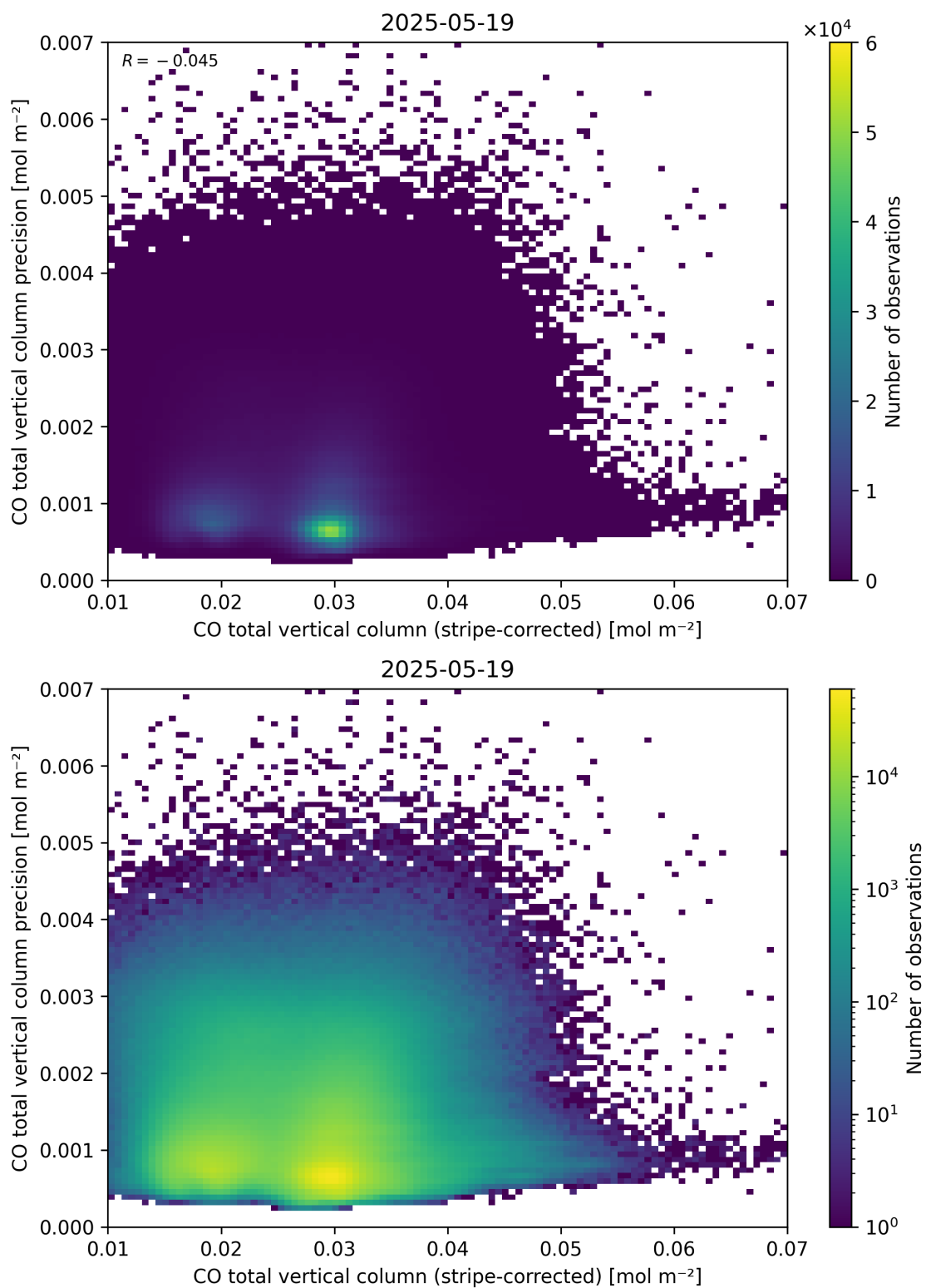
Figure 36: Scatter density plot of “CO total vertical column (stripe-corrected)” against “CO total vertical column precision” for 2025-05-18 to 2025-05-20.
