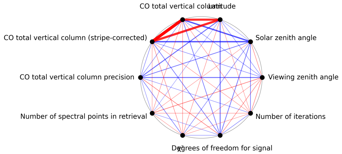
Figure 1: Map of correlation graph for 2025-05-18 to 2025-05-20.
