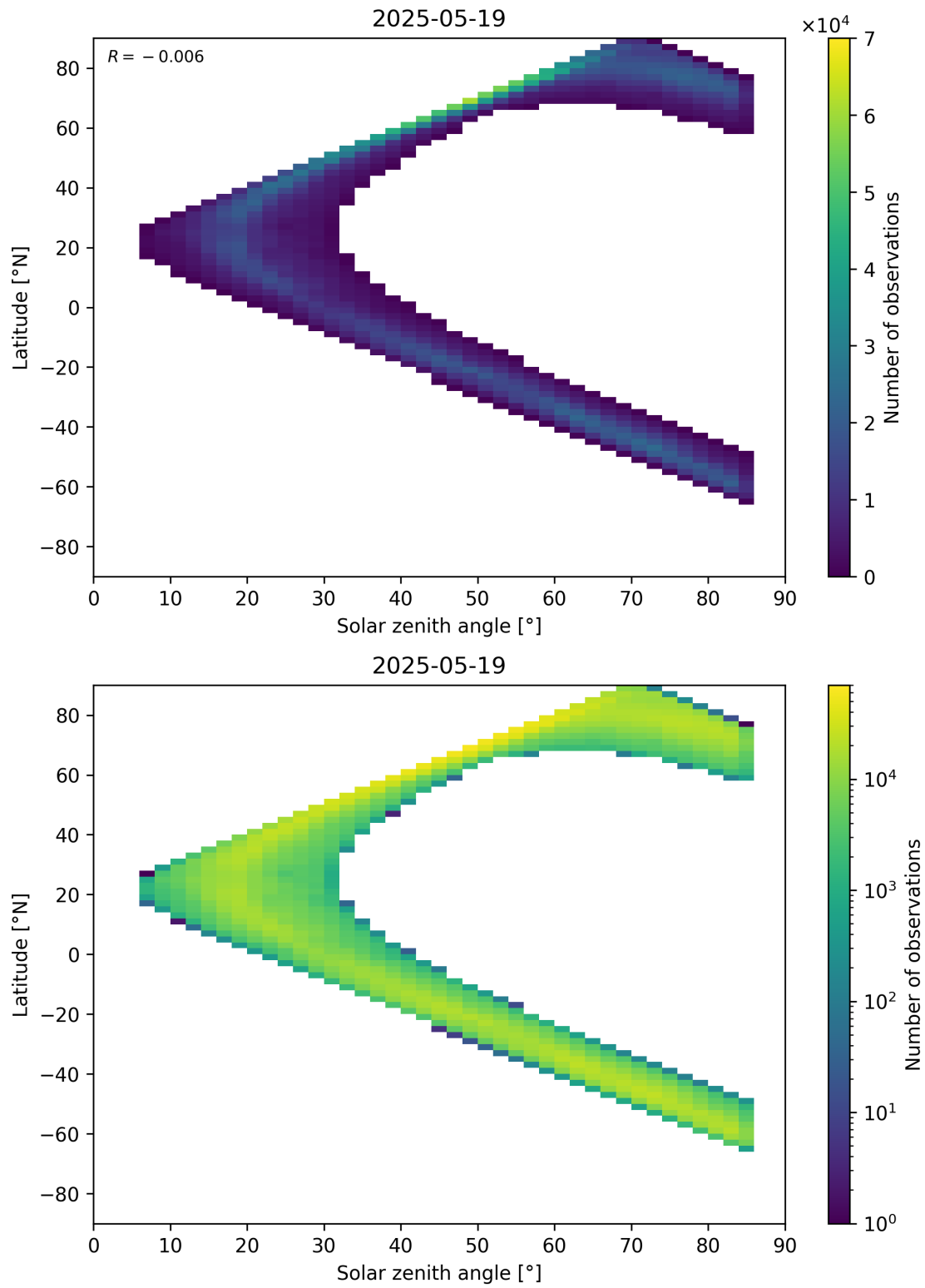
Figure 66: Scatter density plot of “Solar zenith angle” against “Latitude” for 2025-05-18 to 2025-05-20.
