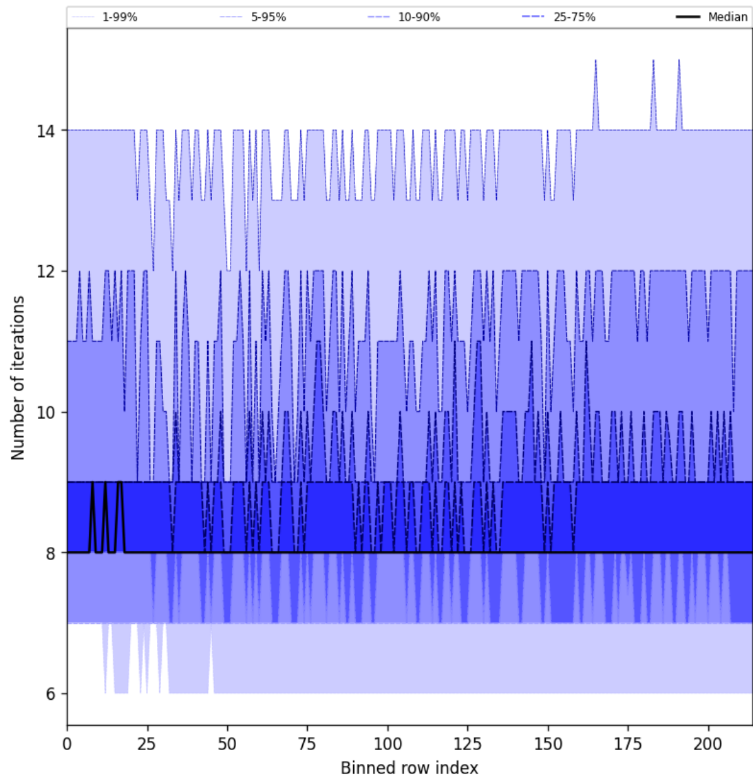
Figure 32: Along track statistics of “Number of iterations” for 2025-05-18 to 2025-05-20
