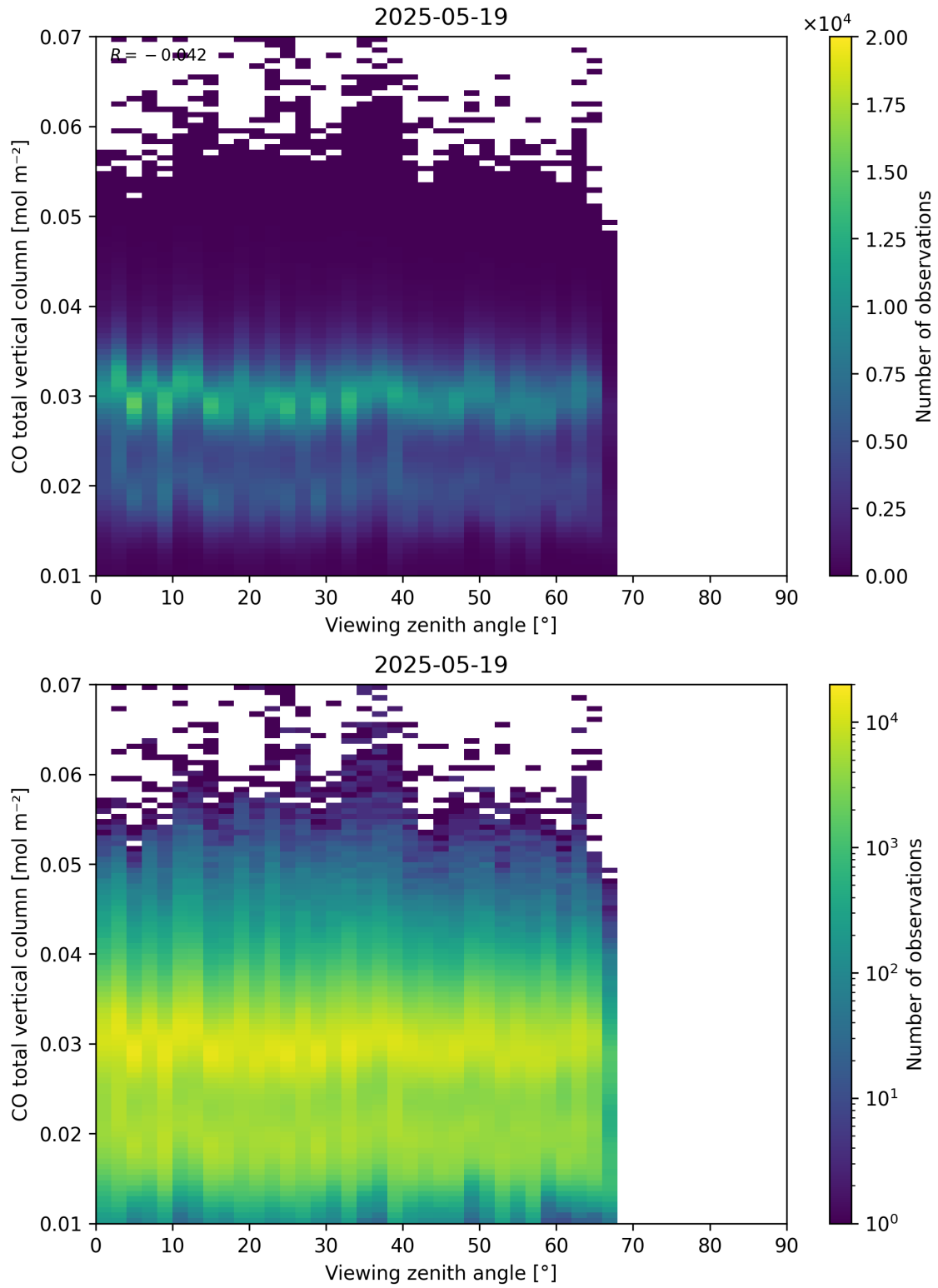
Figure 69: Scatter density plot of “Viewing zenith angle” against “CO total vertical column” for 2025-05-18 to 2025-05-20.
