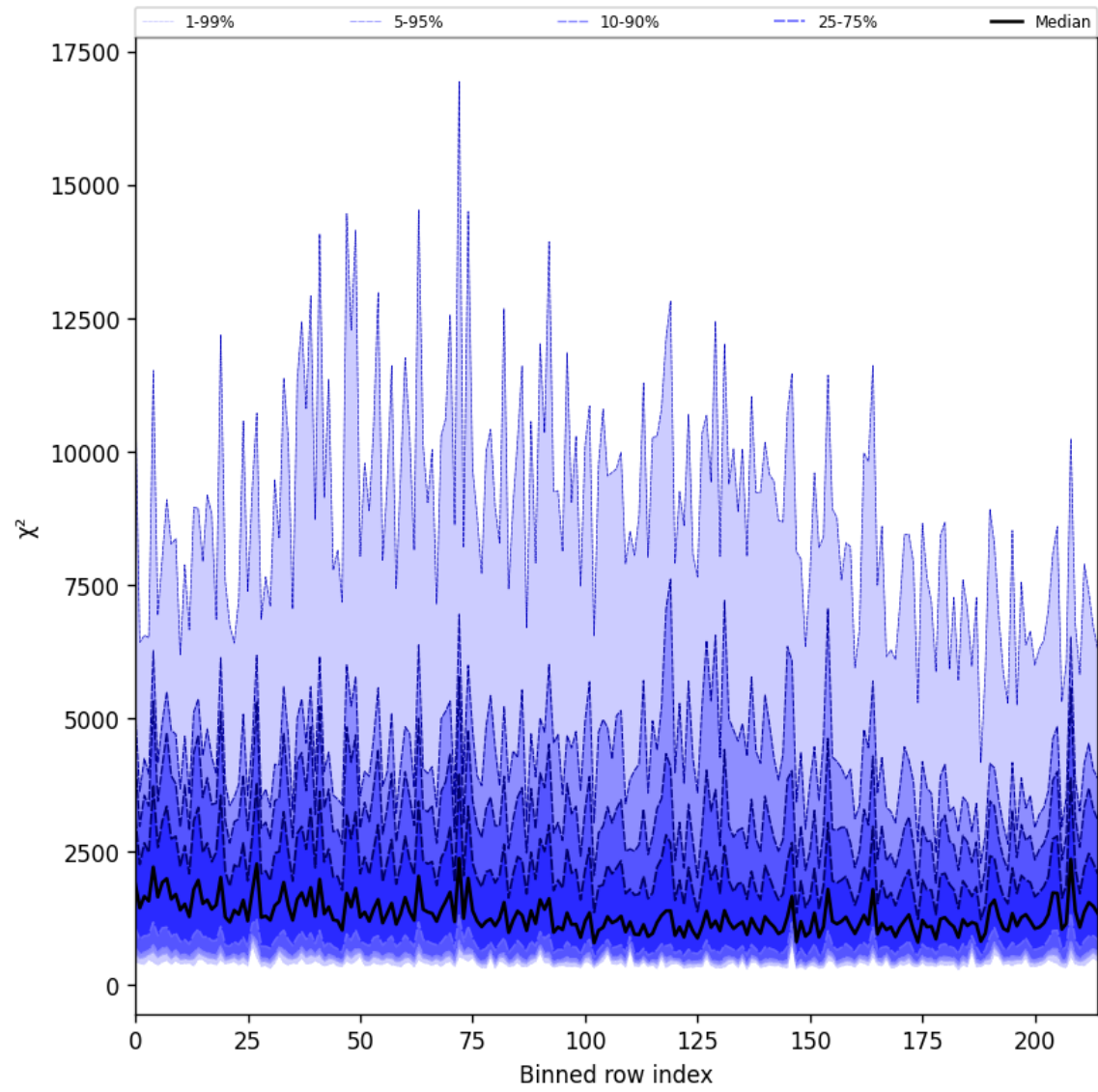
Figure 30: Along track statistics of “ \chi^2 ” for 2025-05-18 to 2025-05-20
