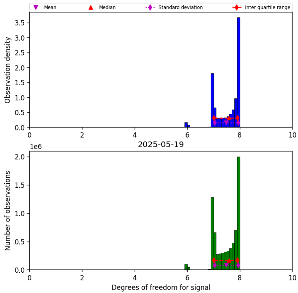
Figure 23: Histogram of “Degrees of freedom for signal” for 2025-05-18 to 2025-05-20
