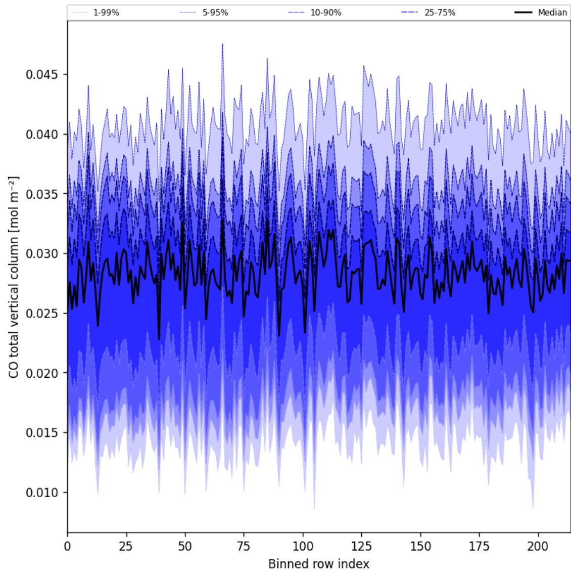
Figure 26: Along track statistics of “CO total vertical column” for 2025-05-18 to 2025-05-20
