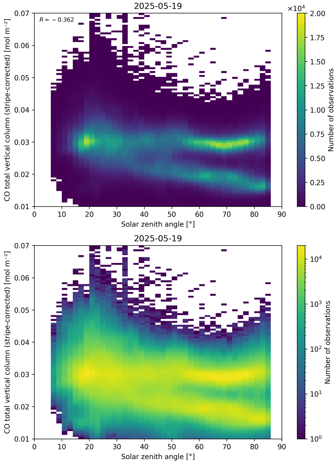
Figure 62: Scatter density plot of “Solar zenith angle” against “CO total vertical column (stripe-corrected)” for 2025-05-18 to 2025-05-20.
