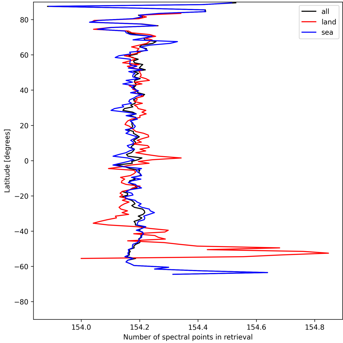
Figure 13: Zonal average of “Number of spectral points in retrieval” for 2025-05-18 to 2025-05-20.
