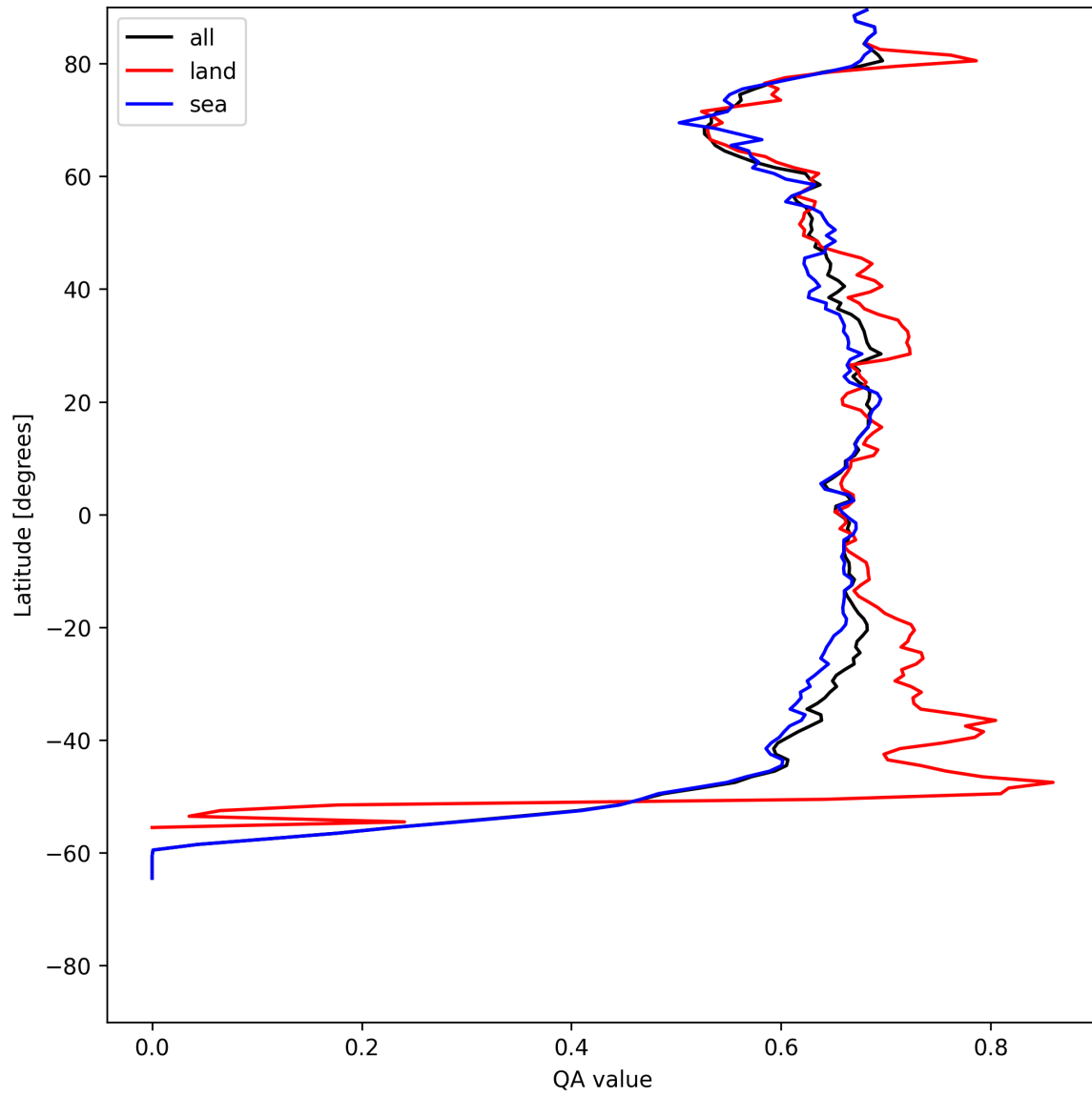
Figure 9: Zonal average of “QA value” for 2025-05-18 to 2025-05-20.
