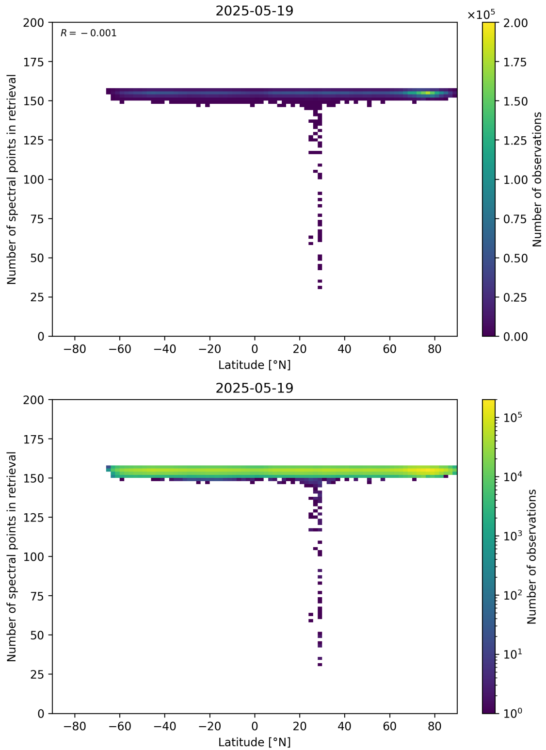
Figure 57: Scatter density plot of “Latitude” against “Number of spectral points in retrieval” for 2025-05-18 to 2025-05-20.
