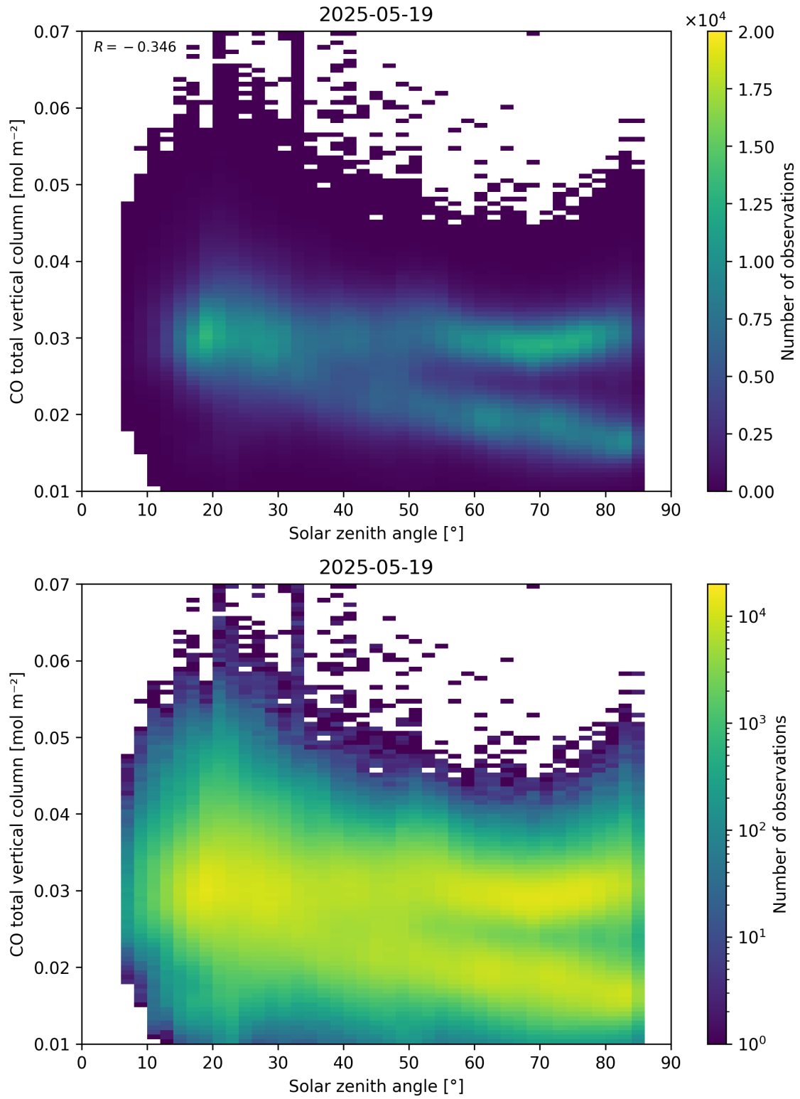
Figure 61: Scatter density plot of “Solar zenith angle” against “CO total vertical column” for 2025-05-18 to 2025-05-20.
