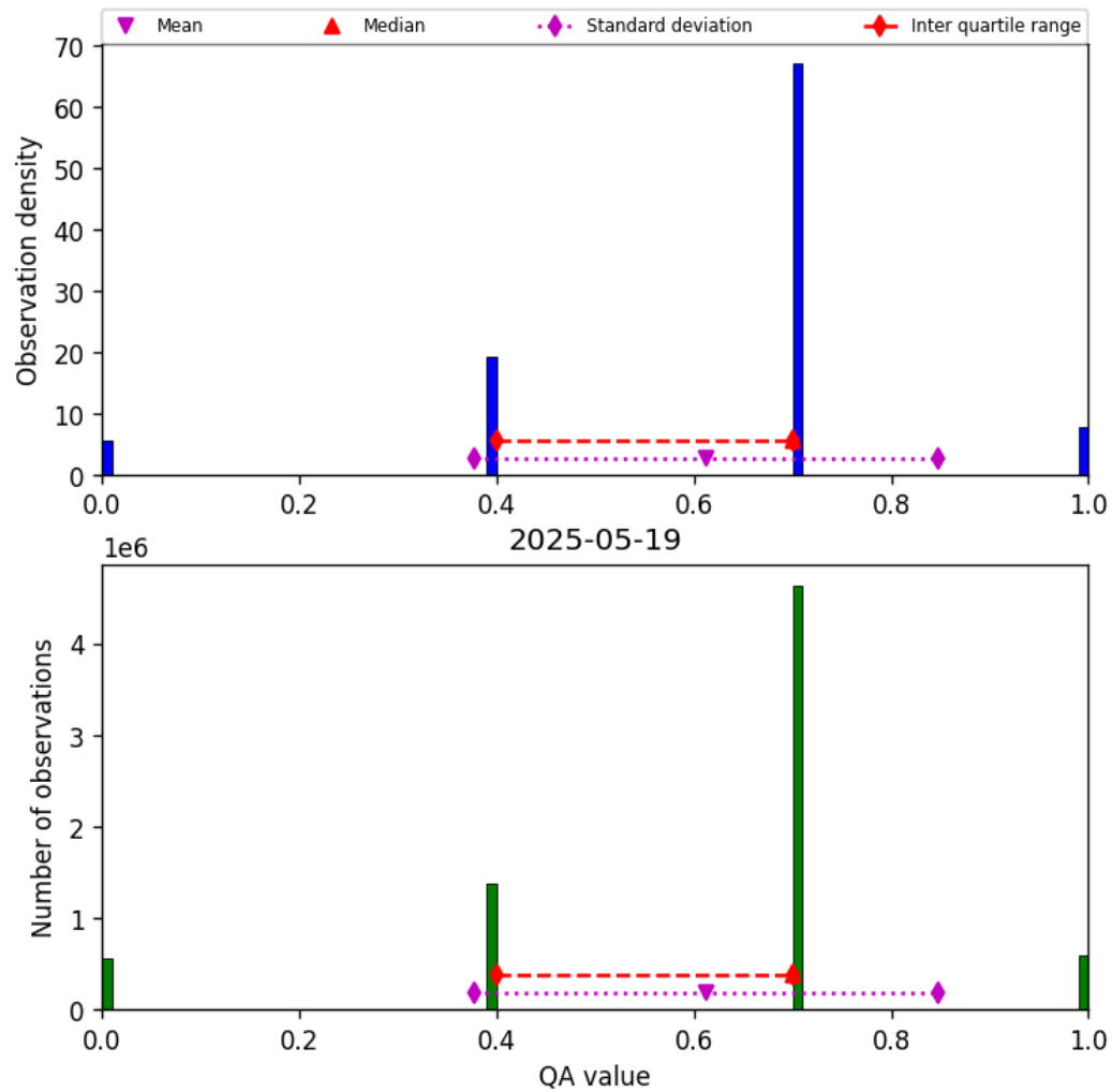
Figure 17: Histogram of “QA value” for 2025-05-18 to 2025-05-20
