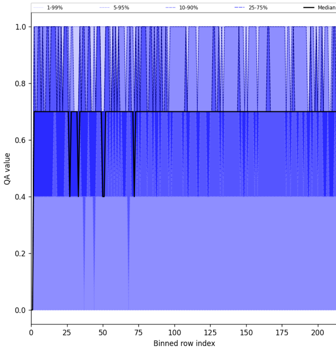
Figure 25: Along track statistics of “QA value” for 2025-05-18 to 2025-05-20
