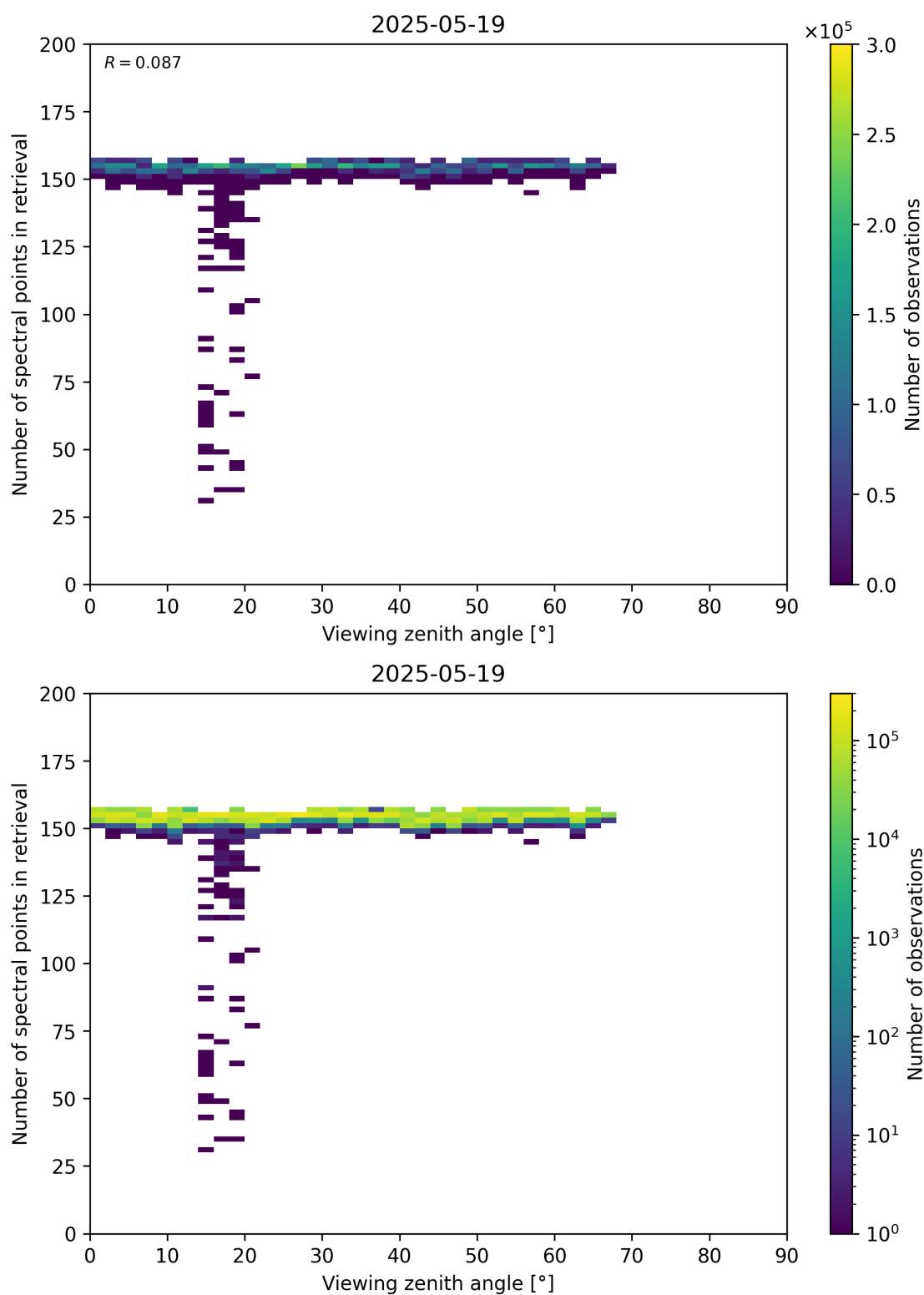
Figure 76: Scatter density plot of “Viewing zenith angle” against “Number of spectral points in retrieval” for 2025-05-18 to 2025-05-20.
