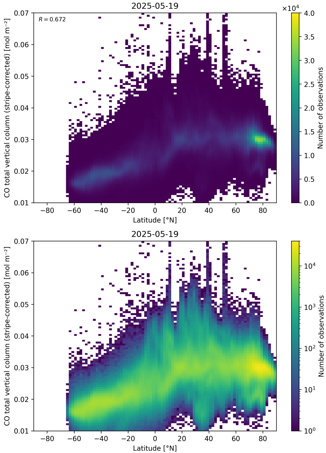
Figure 52: Scatter density plot of “Latitude” against “CO total vertical column (stripe-corrected)” for 2025-05-18 to 2025-05-20.
