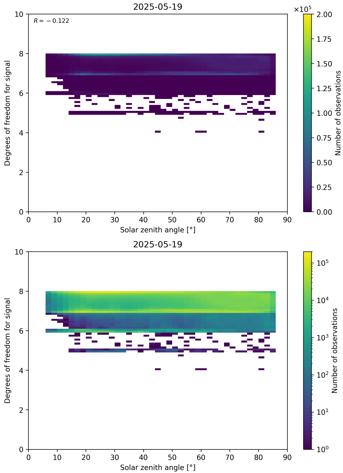
Figure 65: Scatter density plot of “Solar zenith angle” against “Degrees of freedom for signal” for 2025-05-18 to 2025-05-20.
