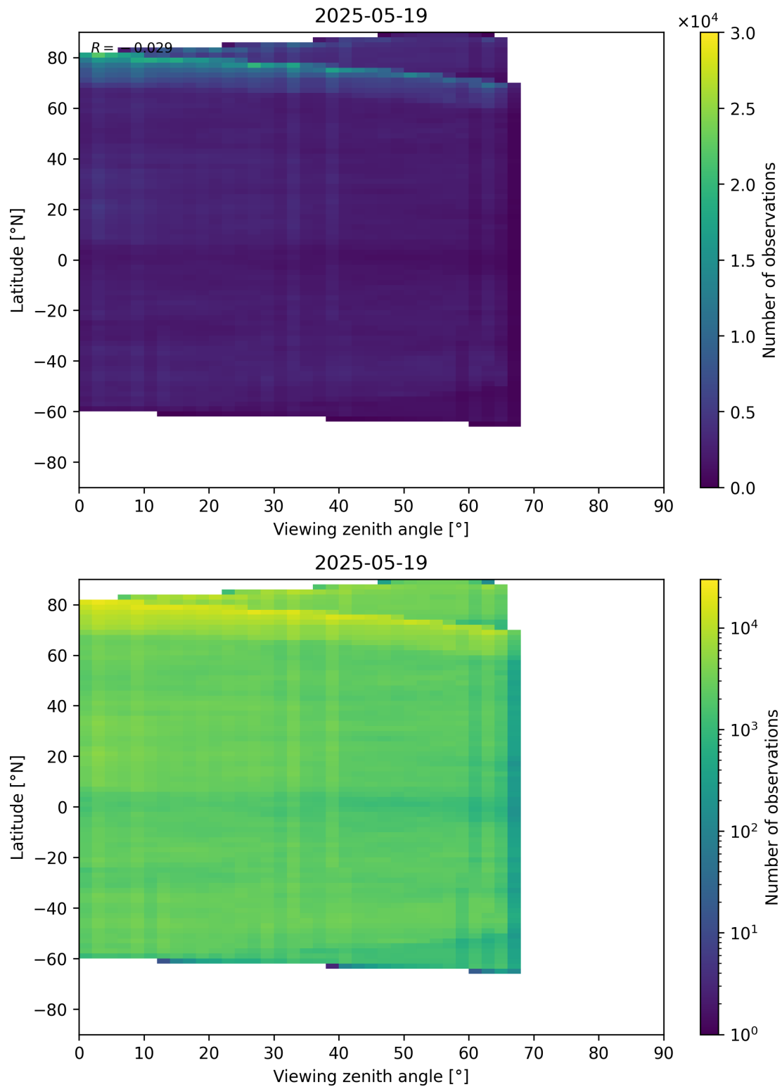
Figure 74: Scatter density plot of “Viewing zenith angle” against “Latitude” for 2025-05-18 to 2025-05-20.
