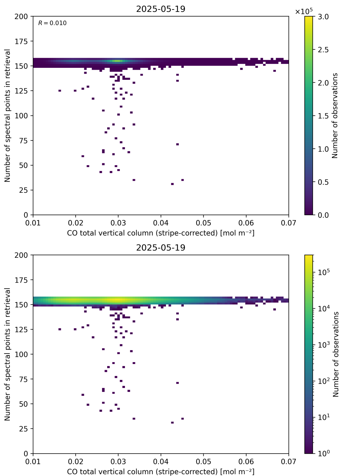
Figure 40: Scatter density plot of “CO total vertical column (stripe-corrected)” against “Number of spectral points in retrieval” for 2025-05-18 to 2025-05-20.
