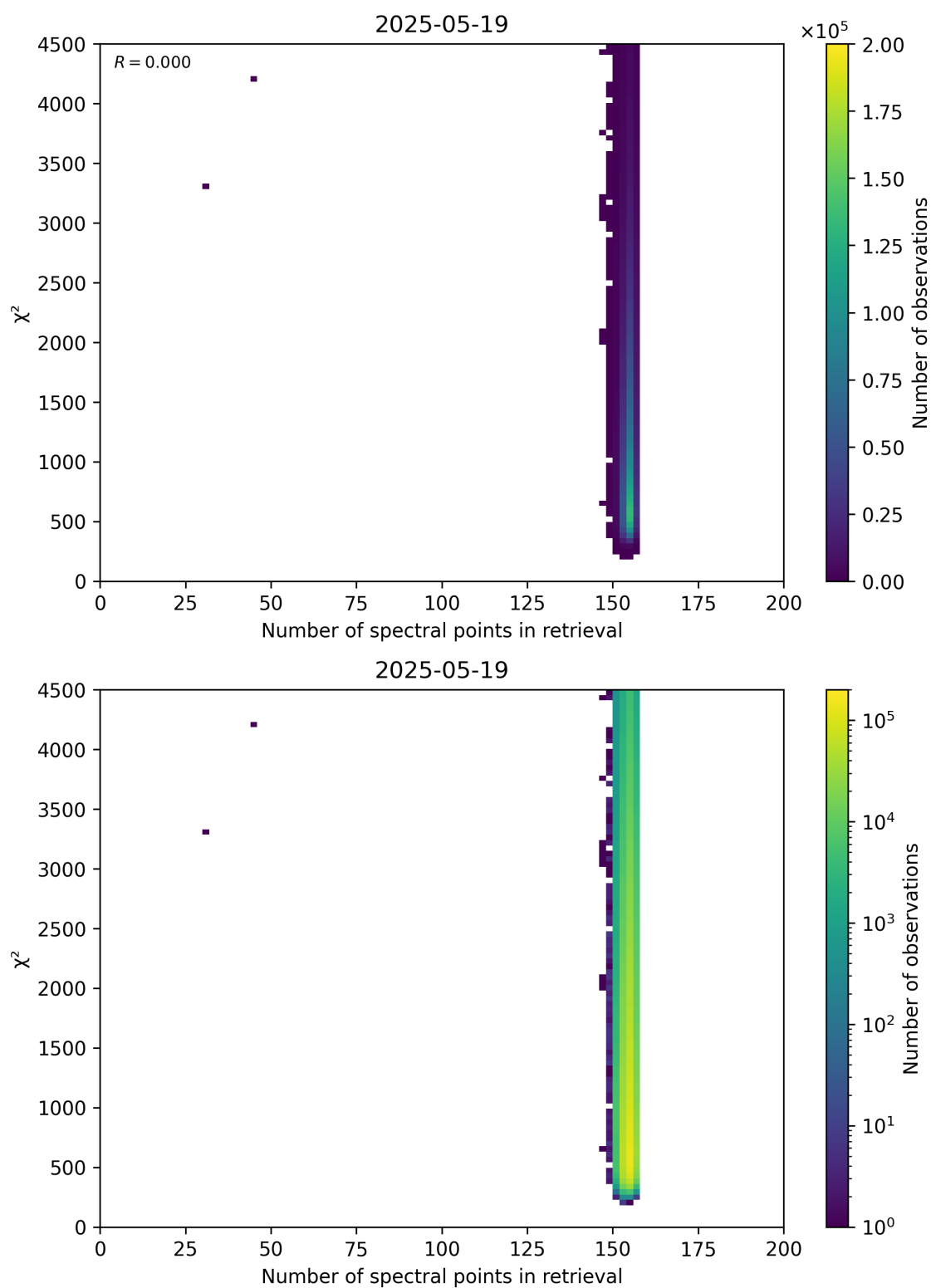
Figure 58: Scatter density plot of “Number of spectral points in retrieval” against “ \chi^2 ” for 2025-05-18 to 2025-05-20.
