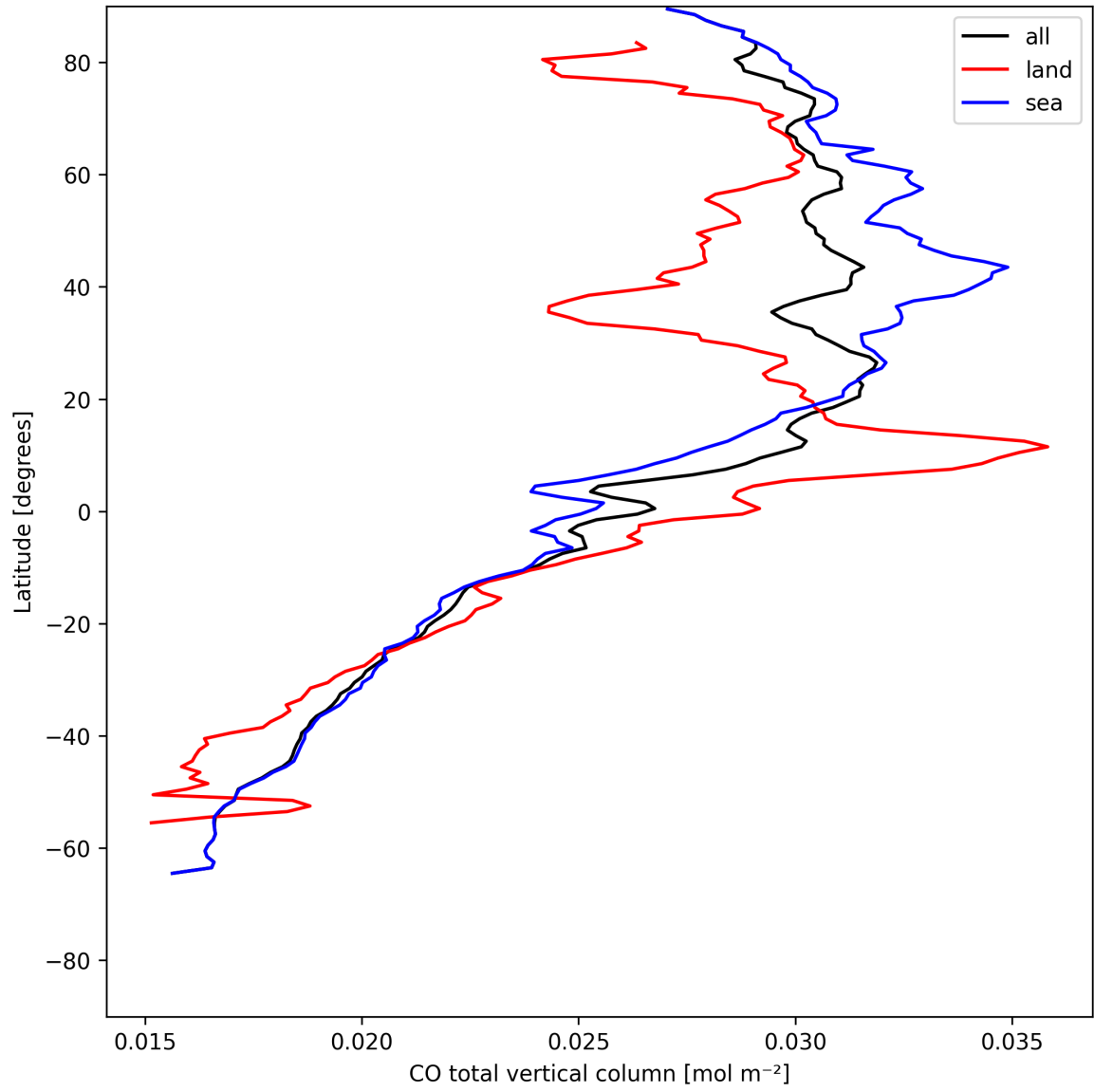
Figure 10: Zonal average of “CO total vertical column” for 2025-05-18 to 2025-05-20.
