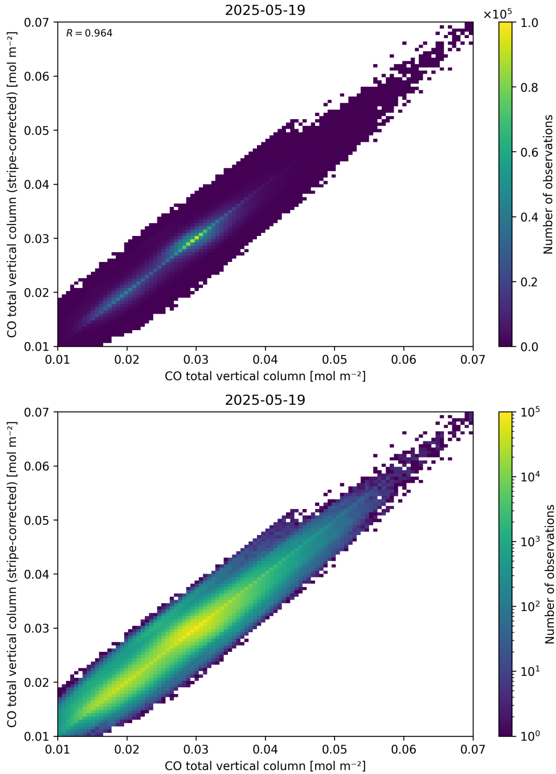
Figure 33: Scatter density plot of “CO total vertical column” against “CO total vertical column (stripe-corrected)” for 2025-05-18 to 2025-05-20.
