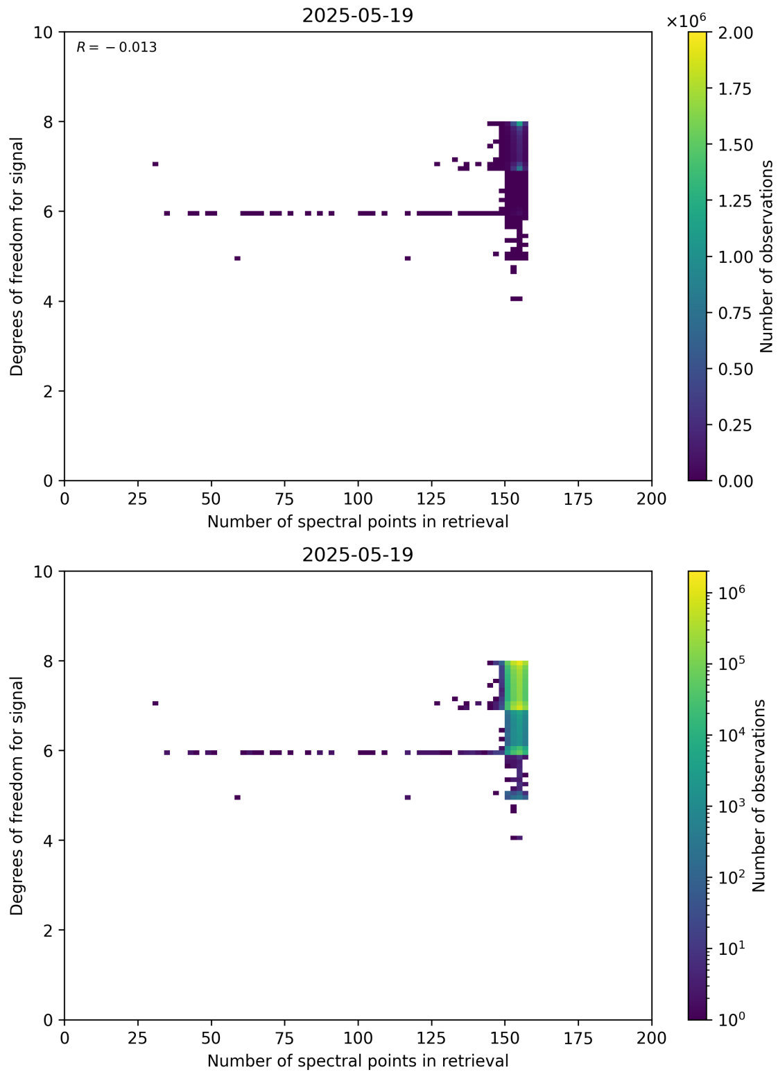
Figure 59: Scatter density plot of “Number of spectral points in retrieval” against “Degrees of freedom for signal” for 2025-05-18 to 2025-05-20.
