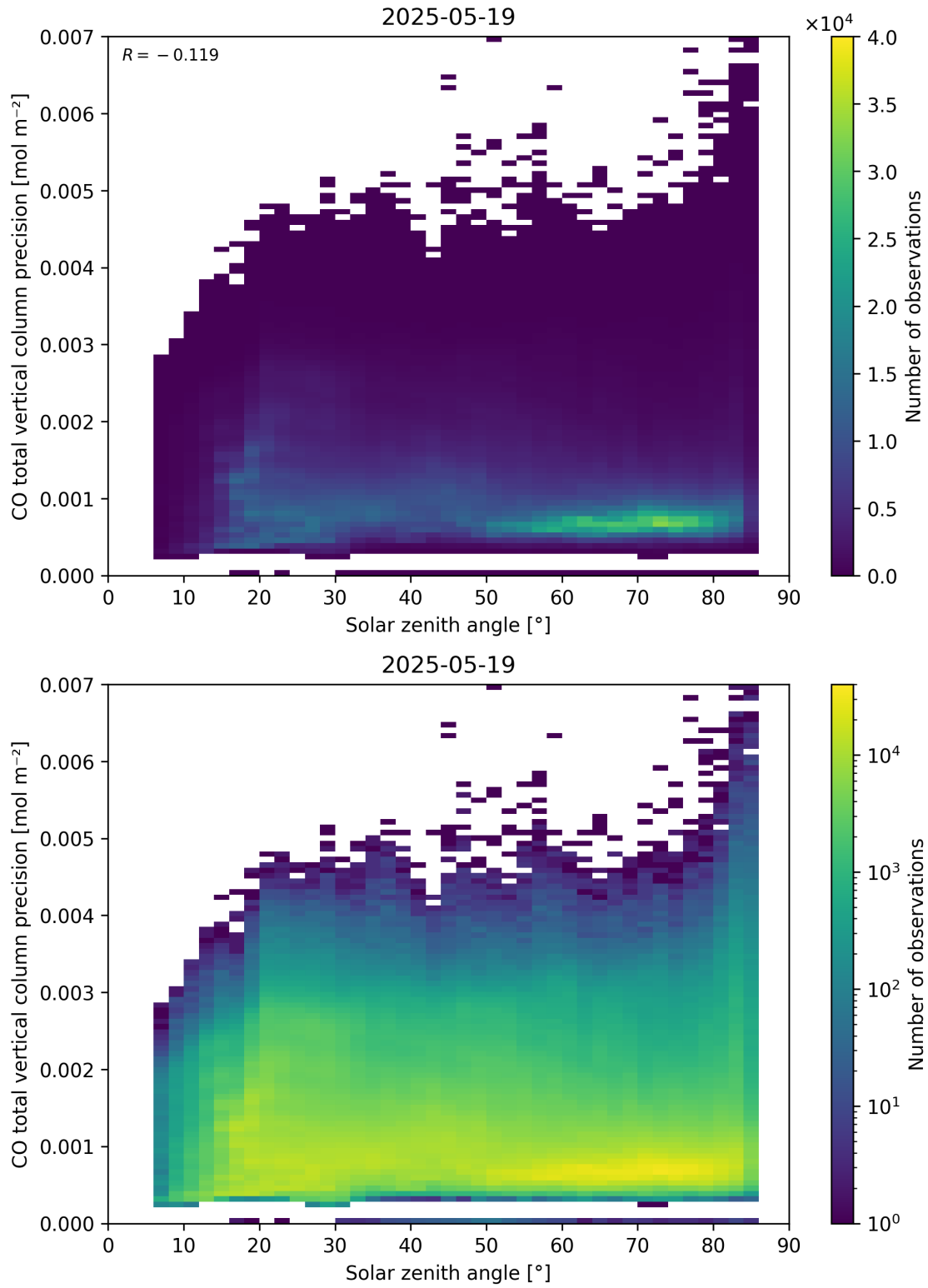
Figure 63: Scatter density plot of “Solar zenith angle” against “CO total vertical column precision” for 2025-05-18 to 2025-05-20.
