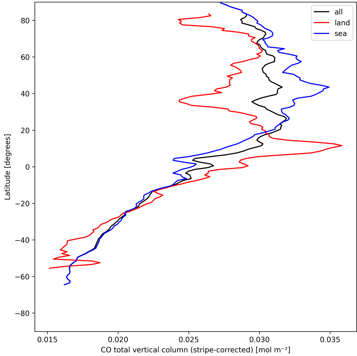
Figure 11: Zonal average of “CO total vertical column (stripe-corrected)” for 2025-05-18 to 2025-05-20.
