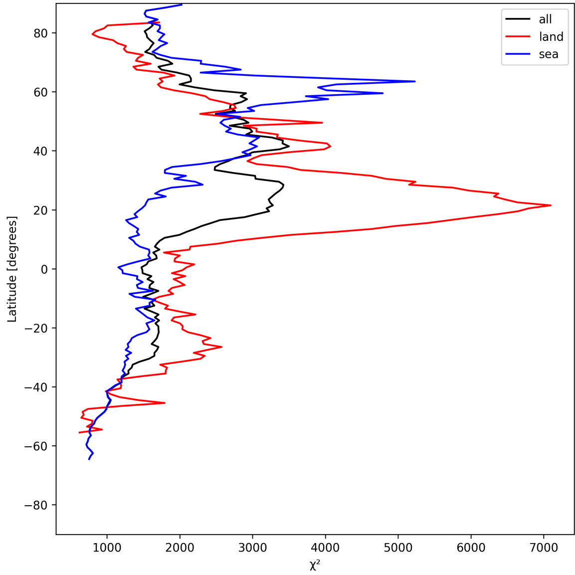
Figure 14: Zonal average of “ \chi^2 ” for 2025-05-18 to 2025-05-20.
