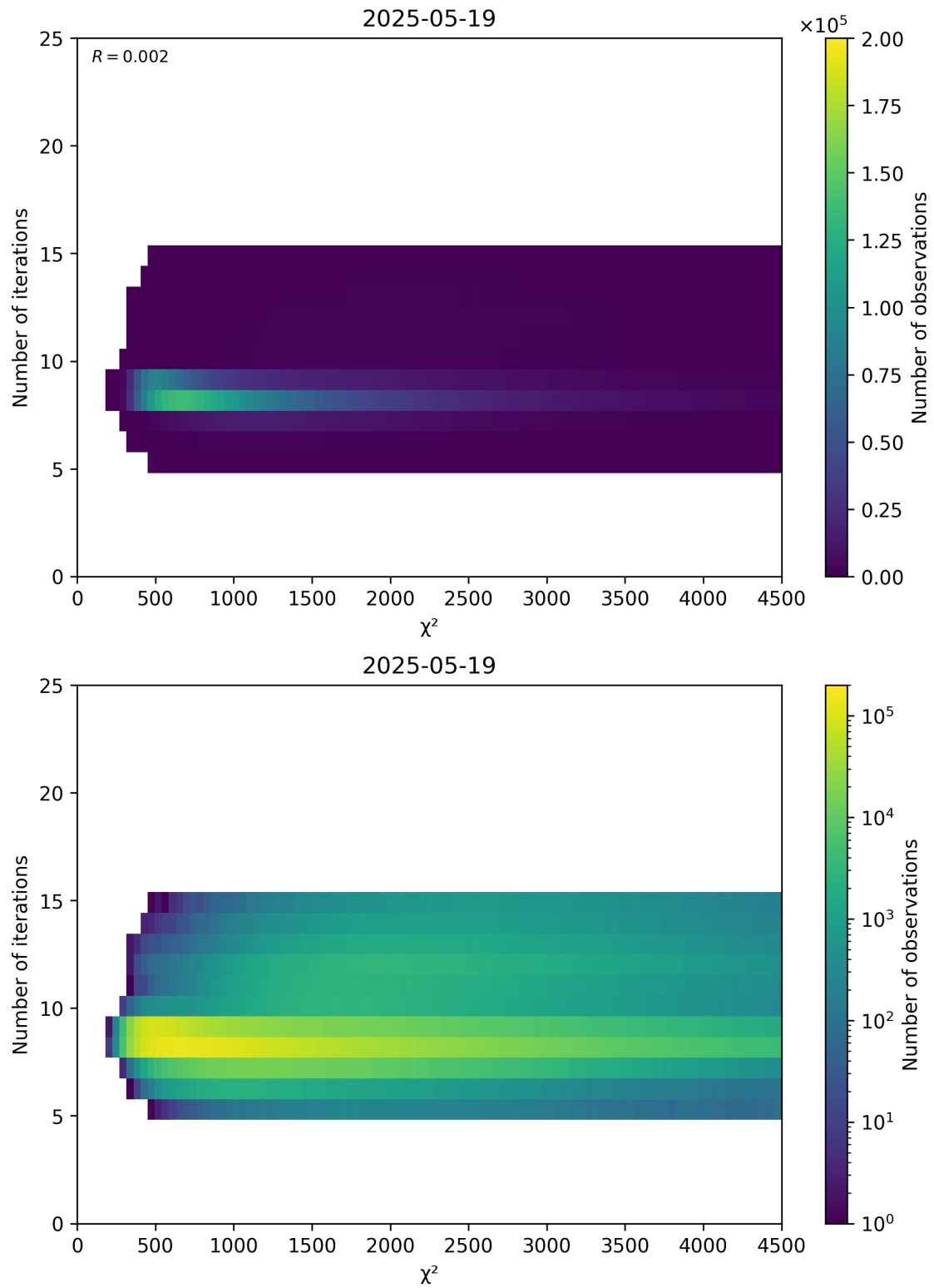
Figure 49: Scatter density plot of “ \chi^2 ” against “Number of iterations” for 2025-05-18 to 2025-05-20.
