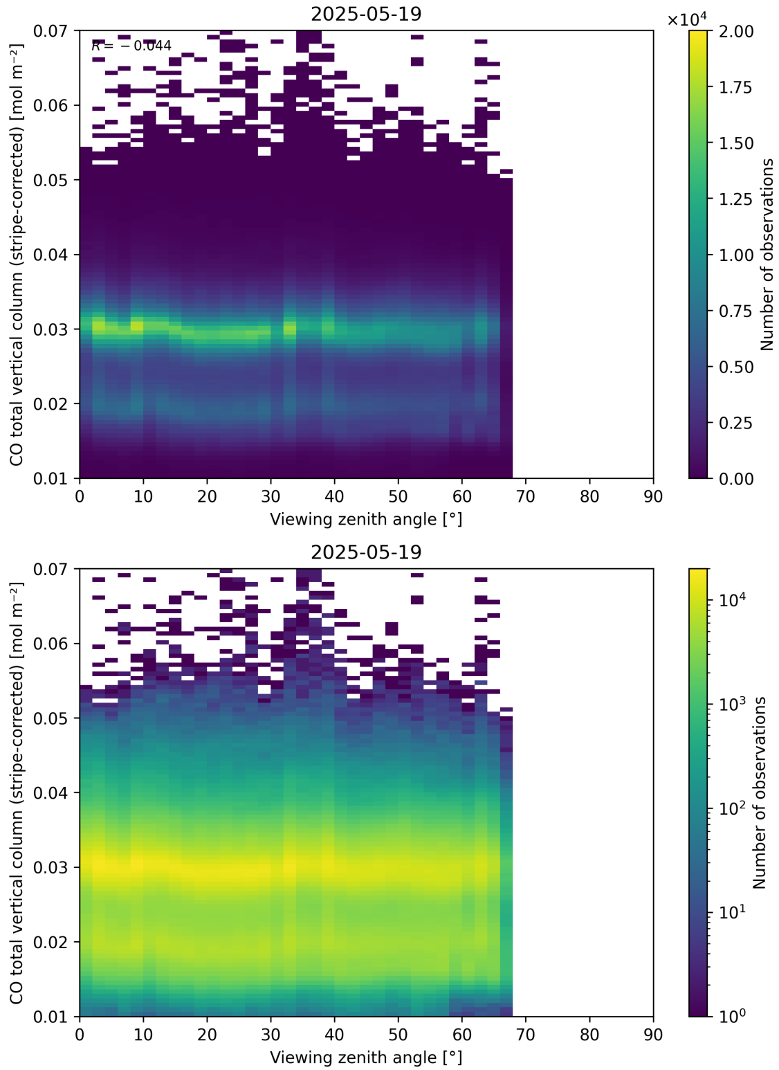
Figure 70: Scatter density plot of “Viewing zenith angle” against “CO total vertical column (stripe-corrected)” for 2025-05-18 to 2025-05-20.
