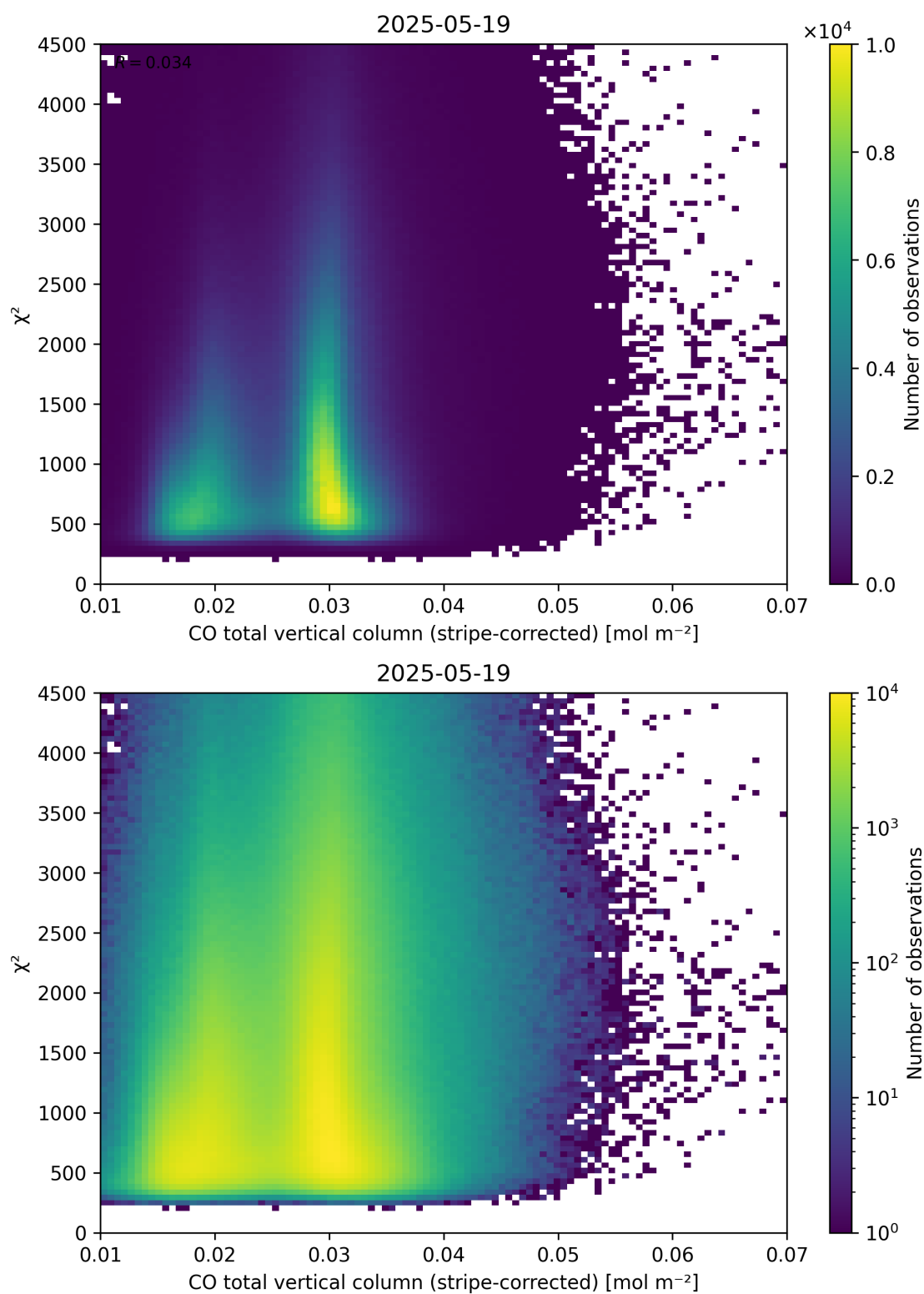
Figure 37: Scatter density plot of “CO total vertical column (stripe-corrected)” against “ \chi^2 ” for 2025-05-18 to 2025-05-20.
