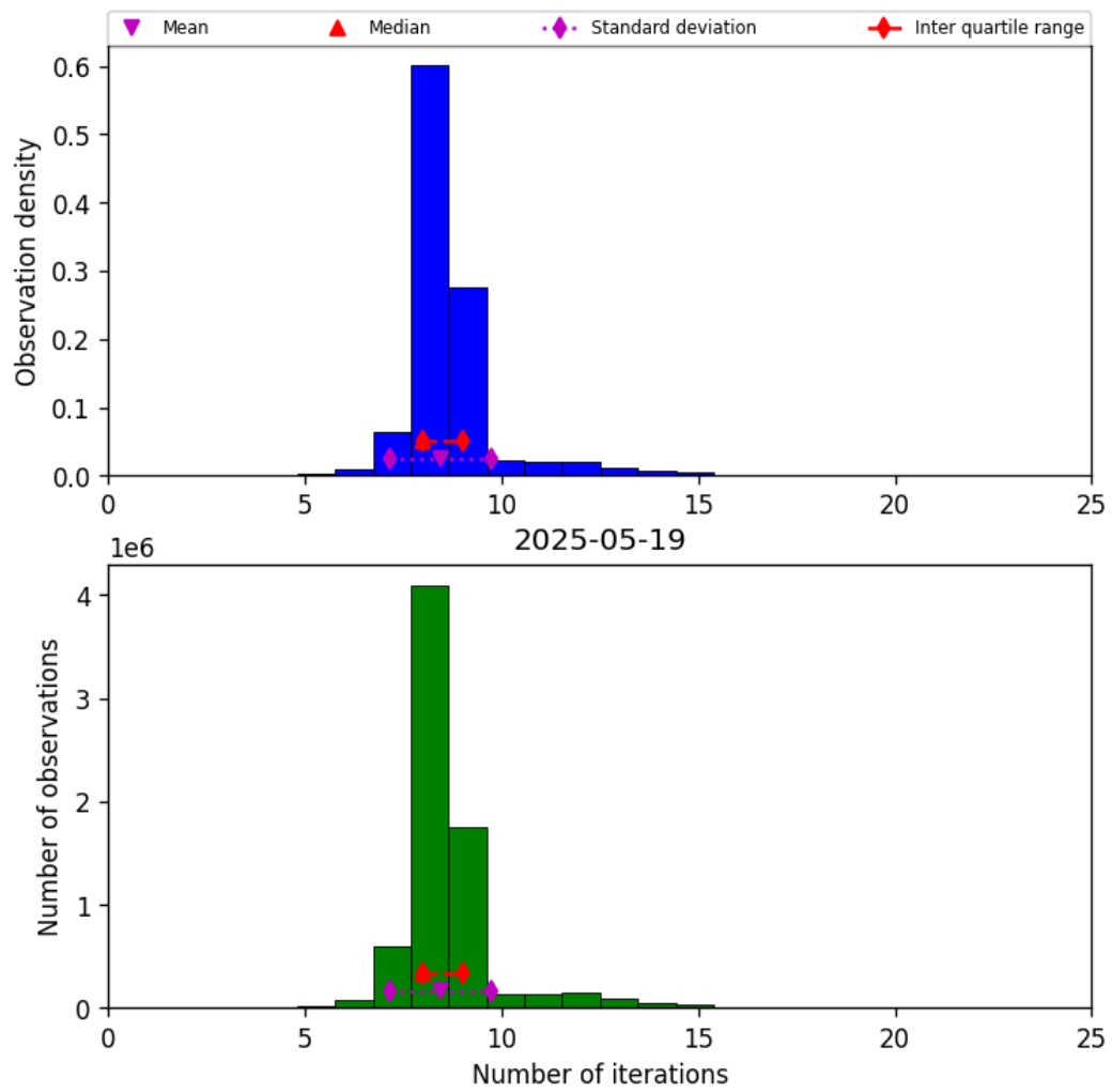
Figure 24: Histogram of “Number of iterations” for 2025-05-18 to 2025-05-20
