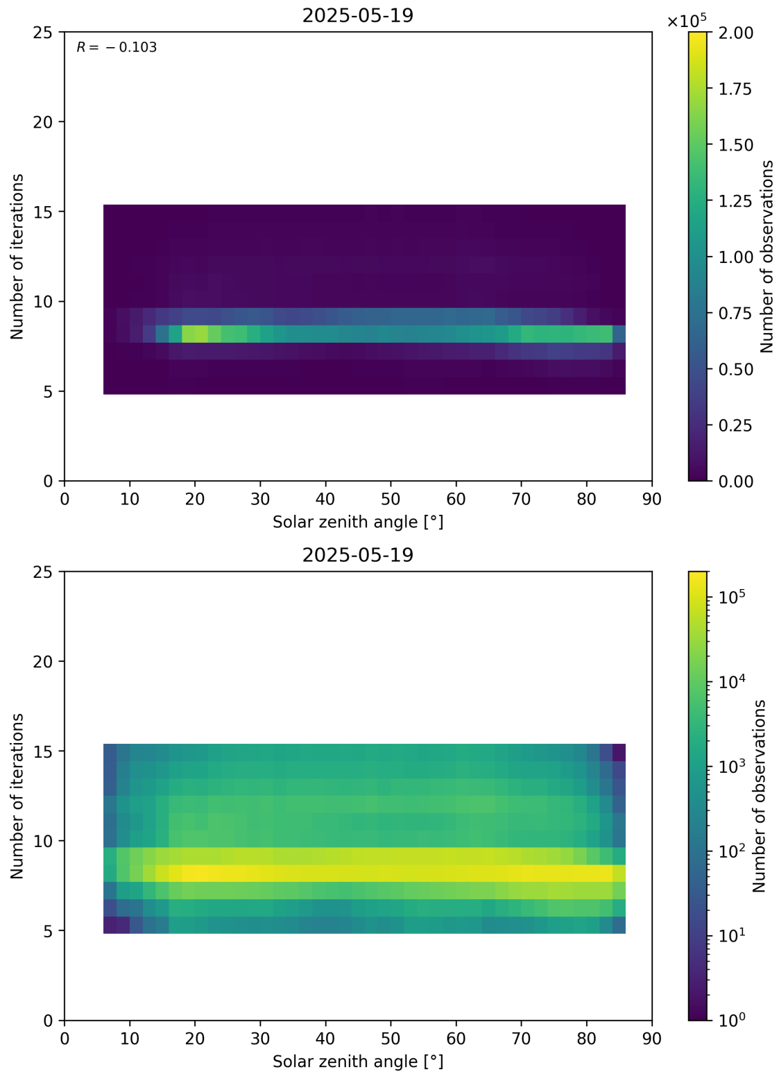
Figure 67: Scatter density plot of “Solar zenith angle” against “Number of iterations” for 2025-05-18 to 2025-05-20.
