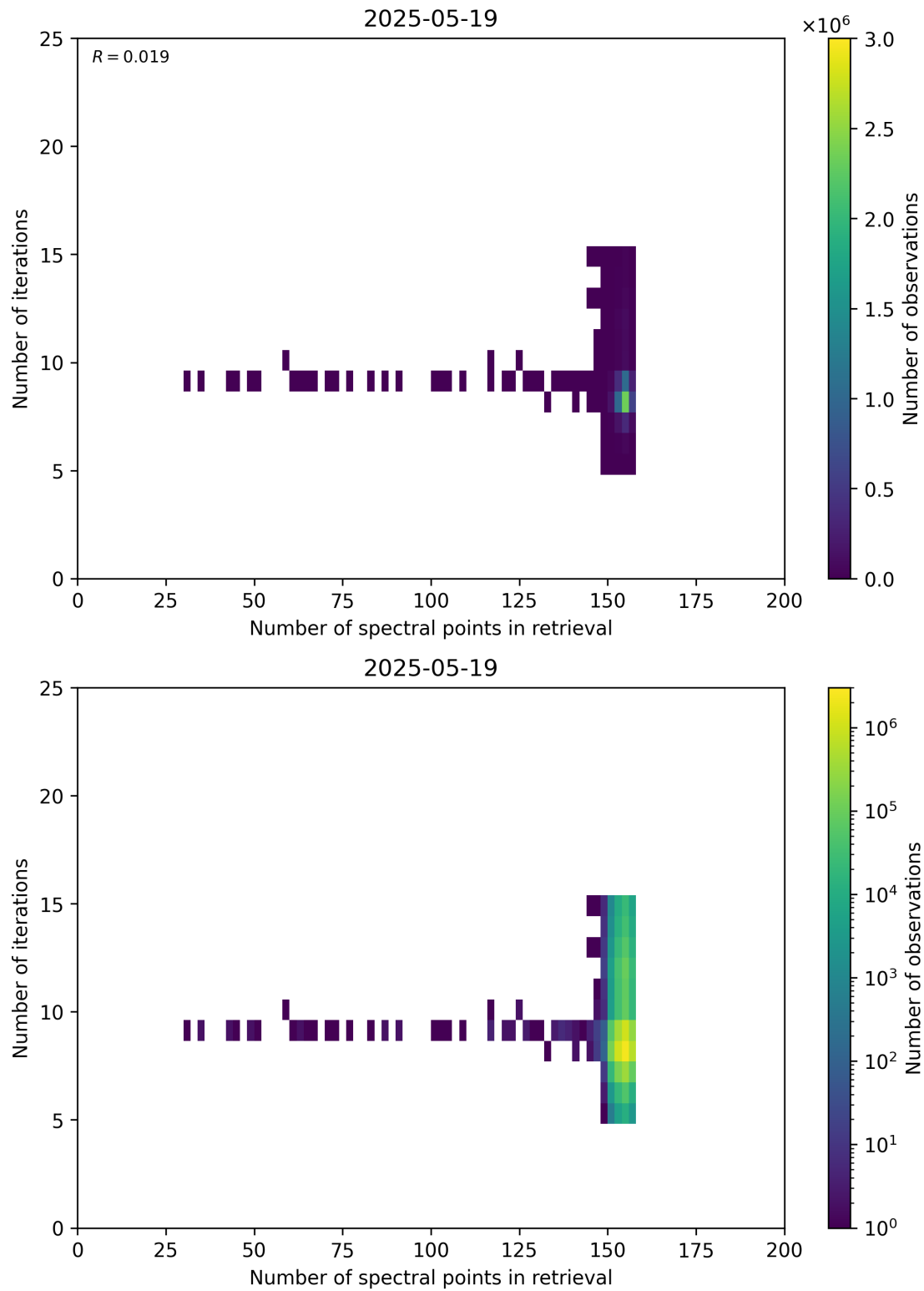
Figure 60: Scatter density plot of “Number of spectral points in retrieval” against “Number of iterations” for 2025-05-18 to 2025-05-20.
