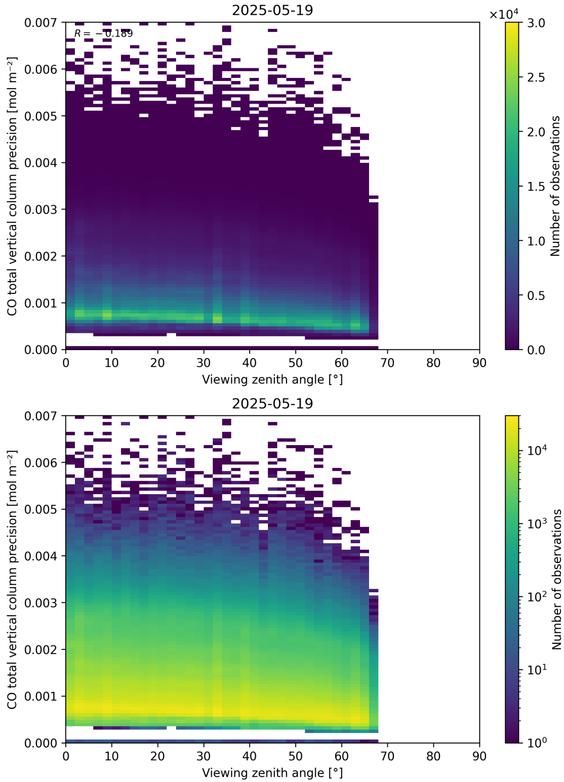
Figure 71: Scatter density plot of “Viewing zenith angle” against “CO total vertical column precision” for 2025-05-18 to 2025-05-20.
