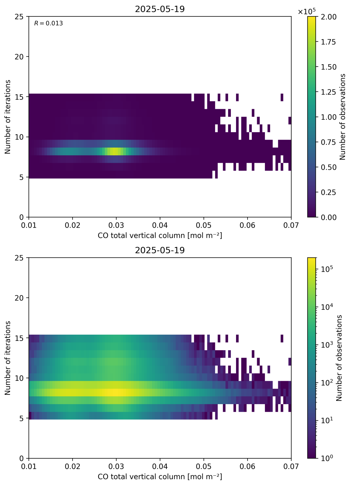
Figure 42: Scatter density plot of “CO total vertical column” against “Number of iterations” for 2025-05-18 to 2025-05-20.
