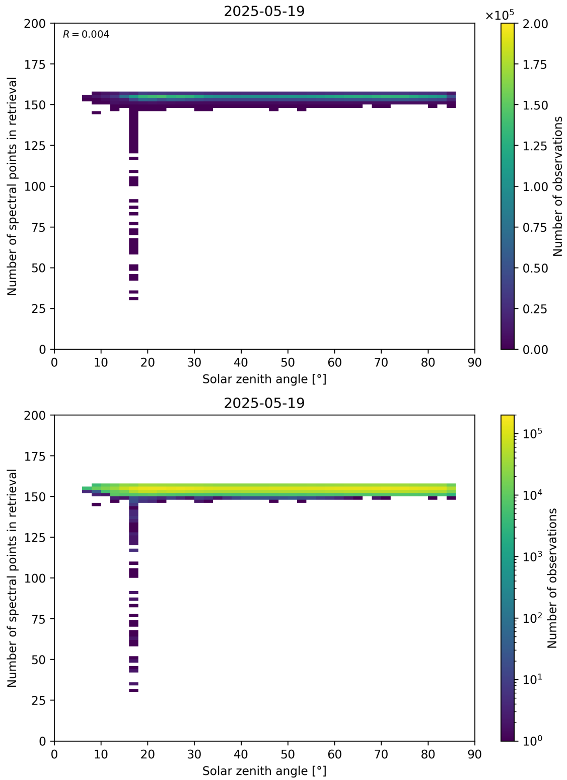
Figure 68: Scatter density plot of “Solar zenith angle” against “Number of spectral points in retrieval” for 2025-05-18 to 2025-05-20.
