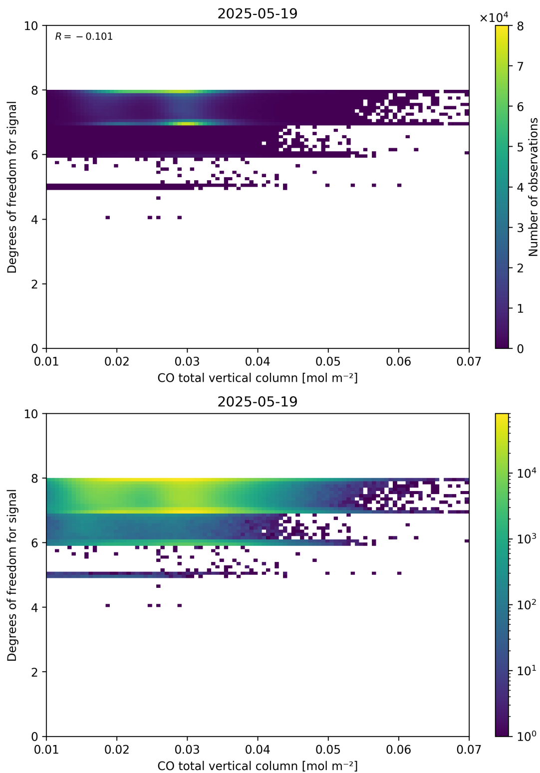
Figure 41: Scatter density plot of “CO total vertical column” against “Degrees of freedom for signal” for 2025-05-18 to 2025-05-20.
