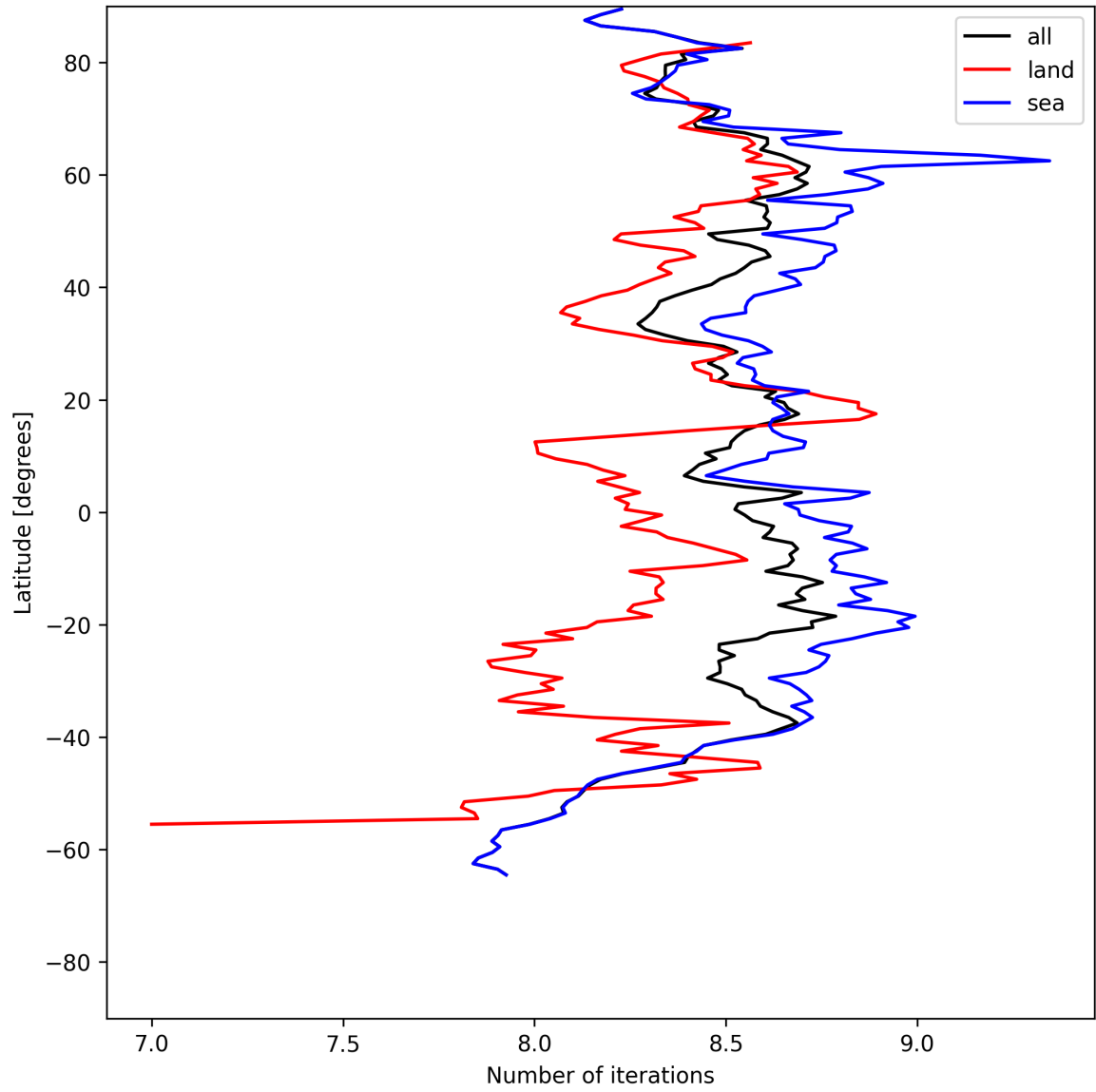
Figure 16: Zonal average of “Number of iterations” for 2025-05-18 to 2025-05-20.
