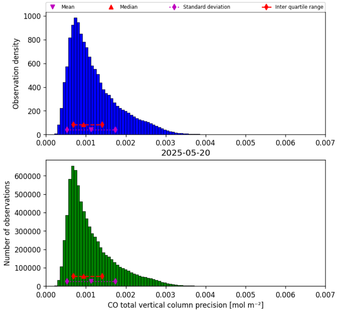
Figure 20: Histogram of “CO total vertical column precision” for 2025-05-19 to 2025-05-21
