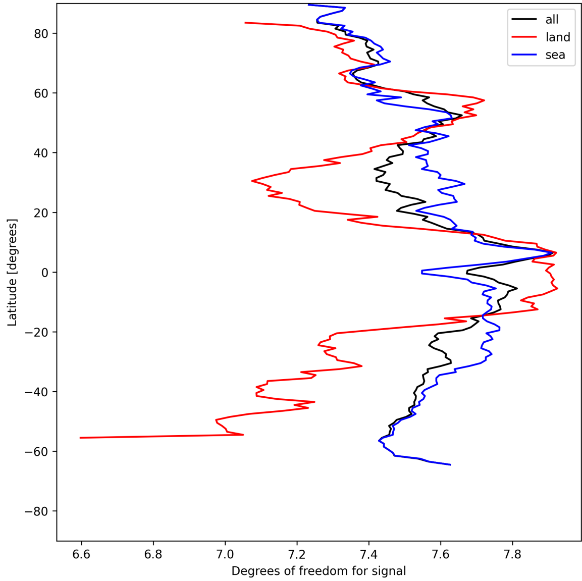
Figure 15: Zonal average of “Degrees of freedom for signal” for 2025-05-19 to 2025-05-21.
