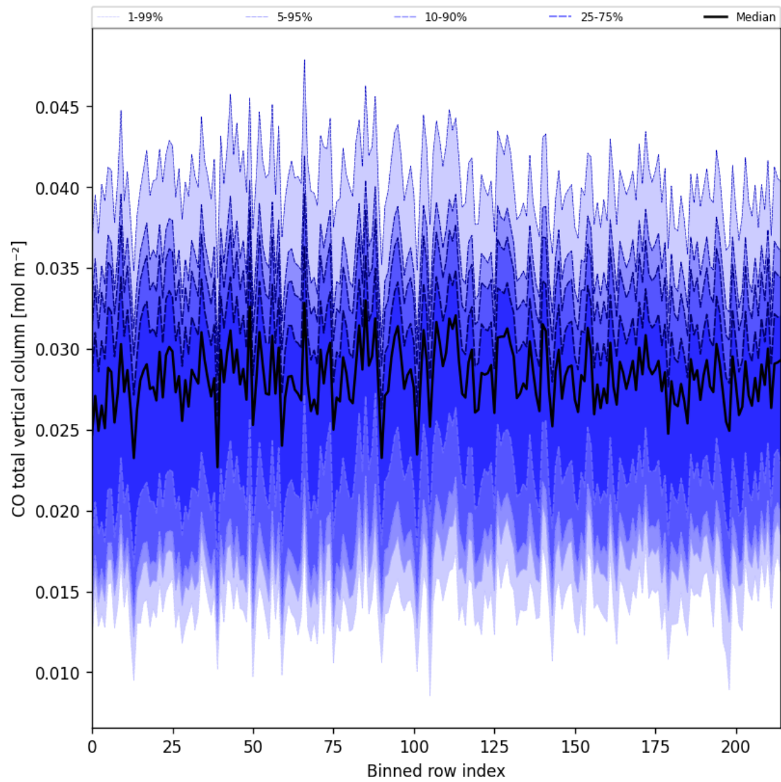
Figure 26: Along track statistics of “CO total vertical column” for 2025-05-19 to 2025-05-21
