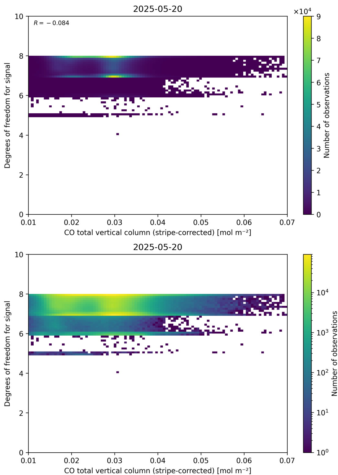
Figure 38: Scatter density plot of “CO total vertical column (stripe-corrected)” against “Degrees of freedom for signal” for 2025-05-19 to 2025-05-21.
