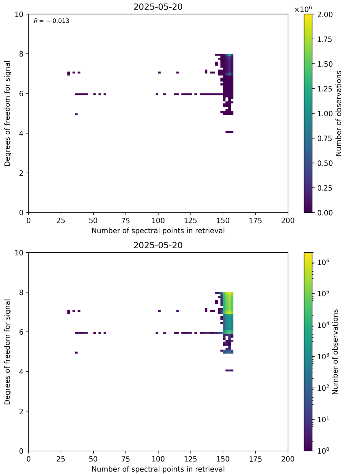
Figure 59: Scatter density plot of “Number of spectral points in retrieval” against “Degrees of freedom for signal” for 2025-05-19 to 2025-05-21.
