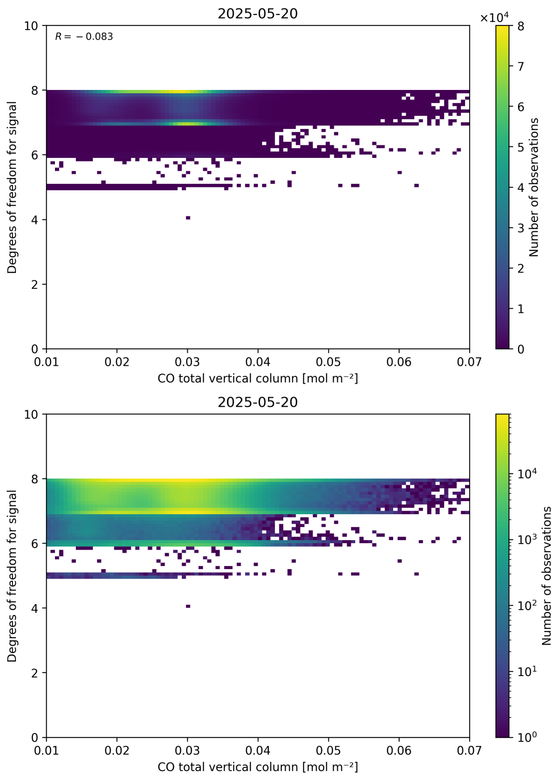
Figure 41: Scatter density plot of “CO total vertical column” against “Degrees of freedom for signal” for 2025-05-19 to 2025-05-21.
