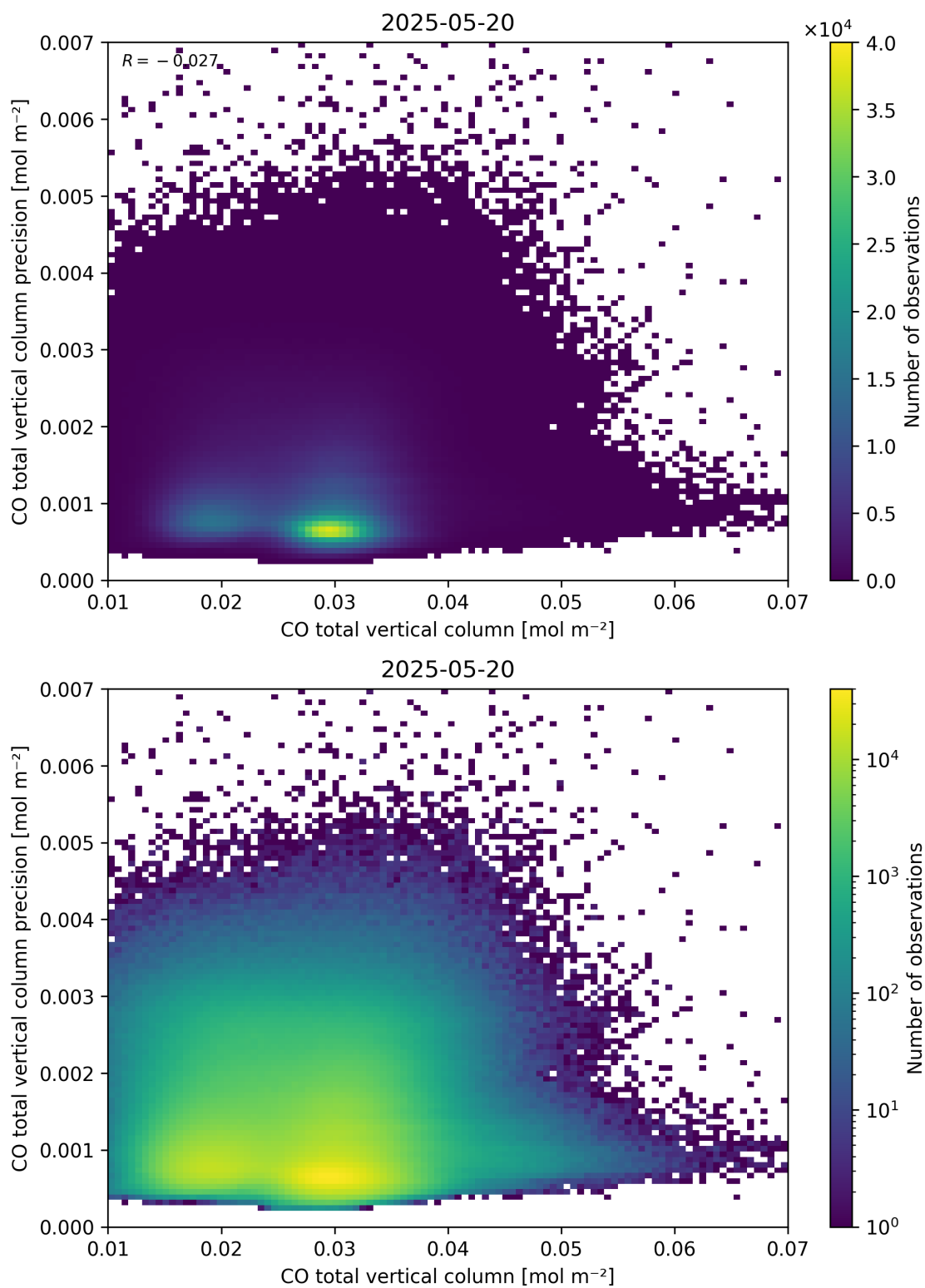
Figure 34: Scatter density plot of “CO total vertical column” against “CO total vertical column precision” for 2025-05-19 to 2025-05-21.
