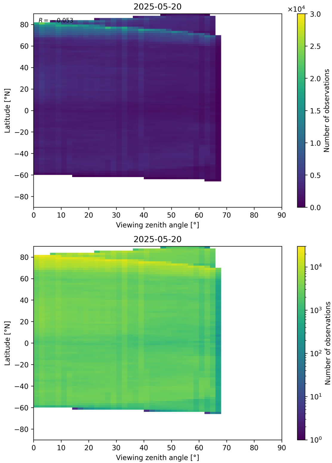
Figure 74: Scatter density plot of “Viewing zenith angle” against “Latitude” for 2025-05-19 to 2025-05-21.
