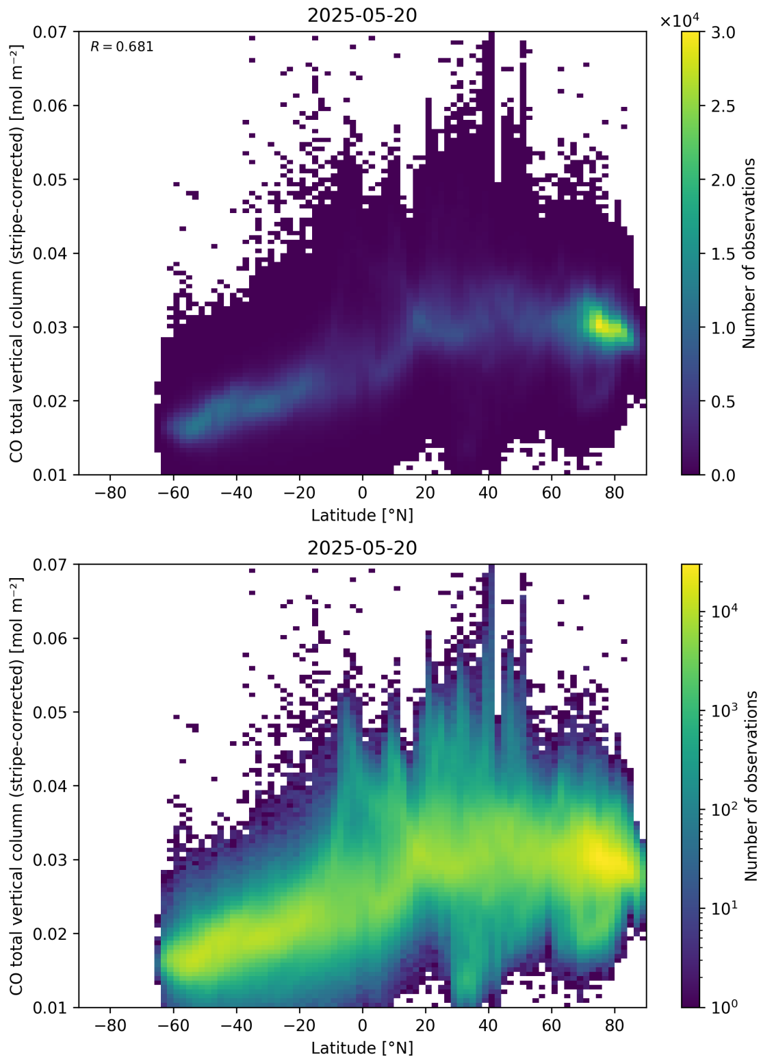
Figure 52: Scatter density plot of “Latitude” against “CO total vertical column (stripe-corrected)” for 2025-05-19 to 2025-05-21.
