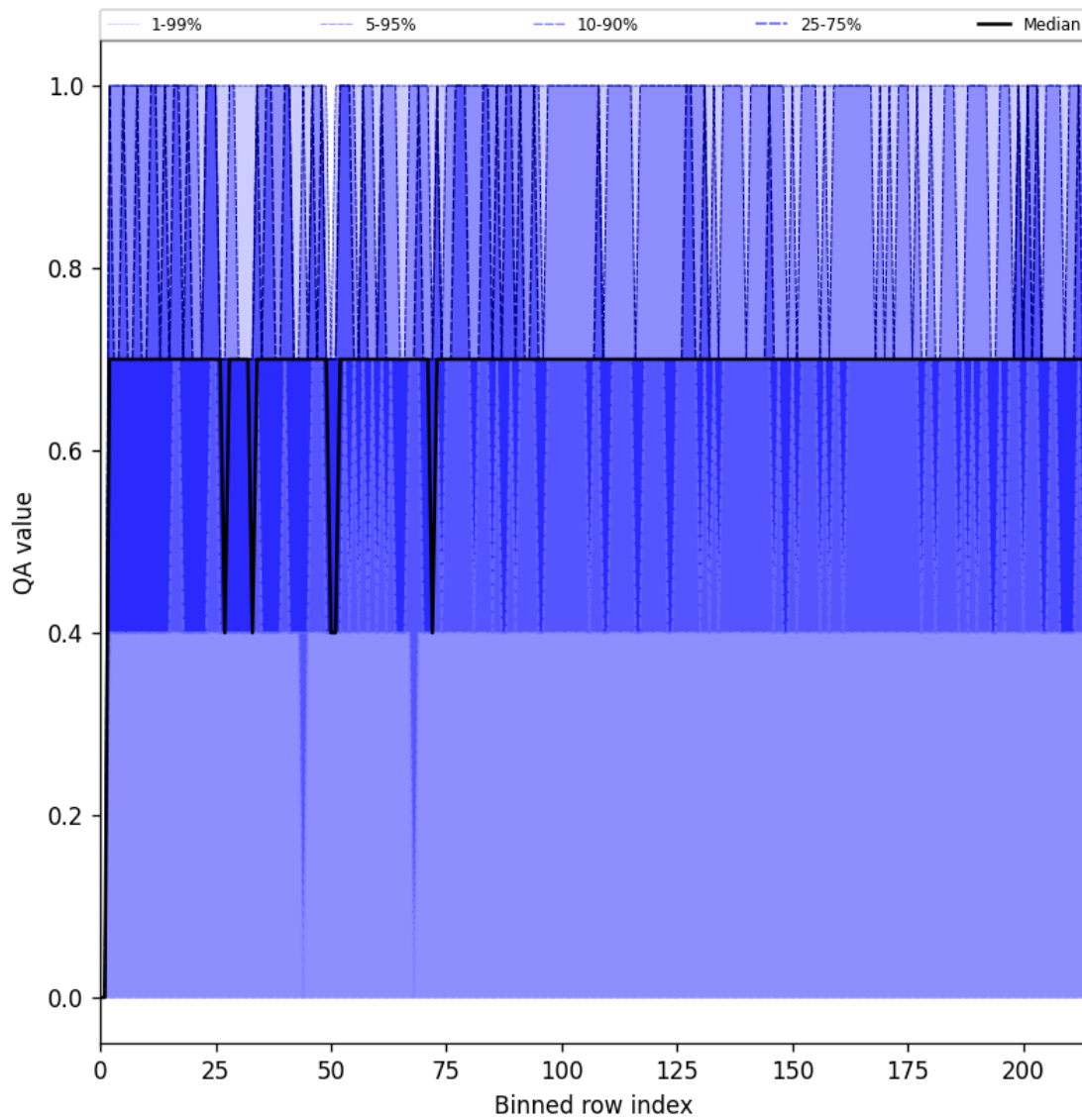
Figure 25: Along track statistics of “QA value” for 2025-05-19 to 2025-05-21
