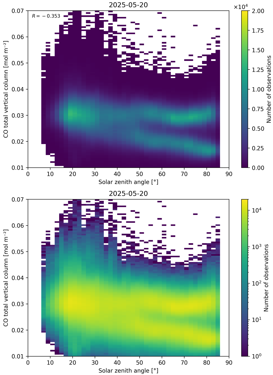
Figure 61: Scatter density plot of “Solar zenith angle” against “CO total vertical column” for 2025-05-19 to 2025-05-21.
