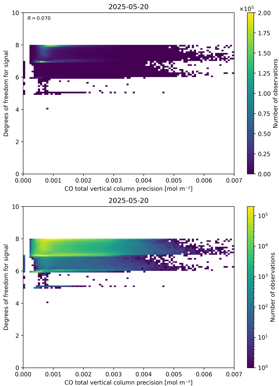
Figure 45: Scatter density plot of “CO total vertical column precision” against “Degrees of freedom for signal” for 2025-05-19 to 2025-05-21.
