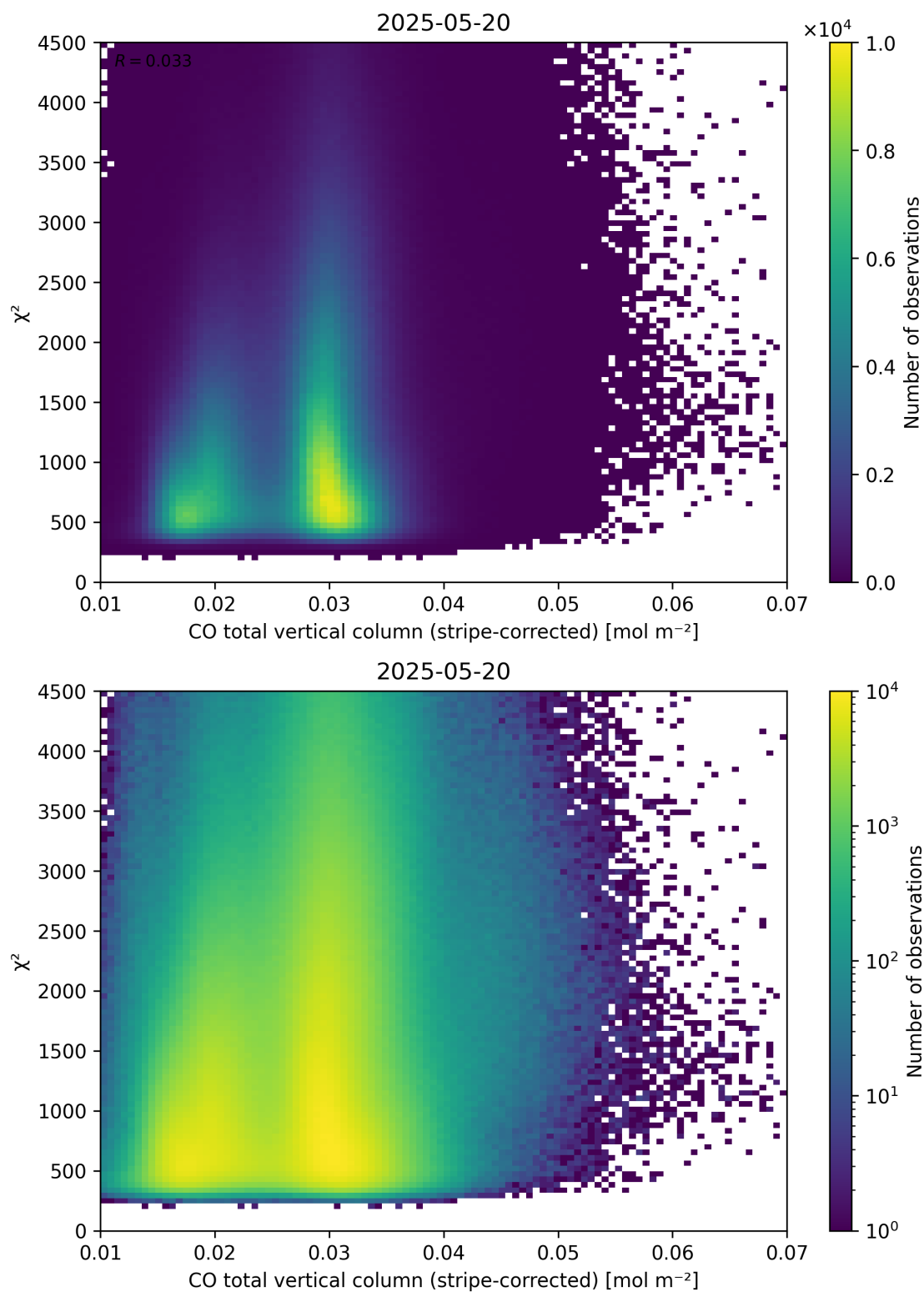
Figure 37: Scatter density plot of “CO total vertical column (stripe-corrected)” against “ \chi^2 ” for 2025-05-19 to 2025-05-21.
