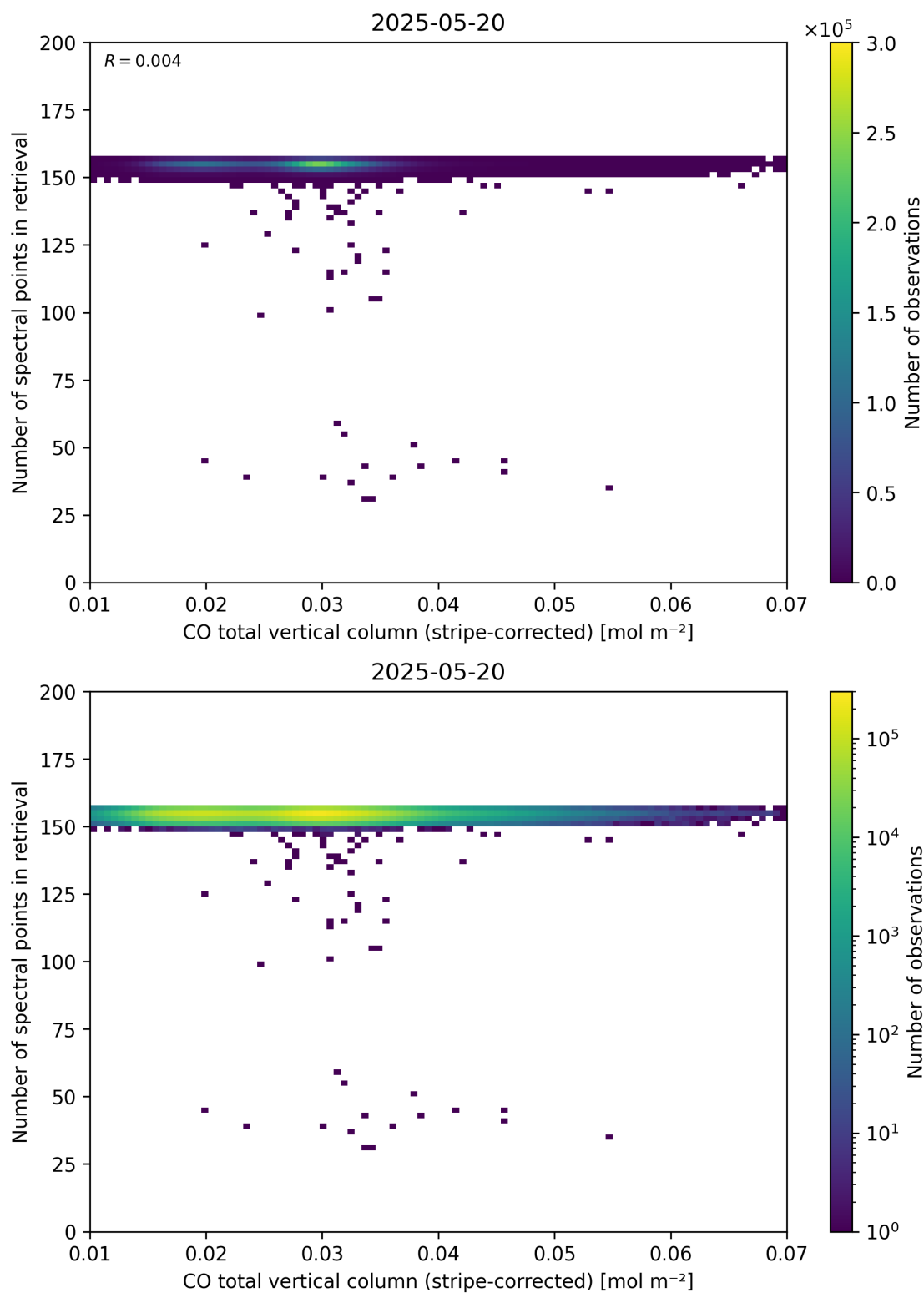
Figure 40: Scatter density plot of “CO total vertical column (stripe-corrected)” against “Number of spectral points in retrieval” for 2025-05-19 to 2025-05-21.
