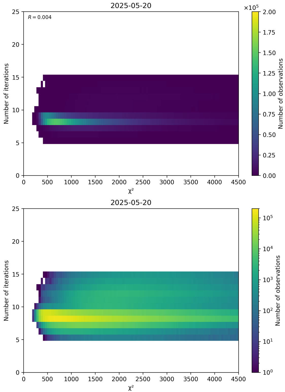
Figure 49: Scatter density plot of “ \chi^2 ” against “Number of iterations” for 2025-05-19 to 2025-05-21.
