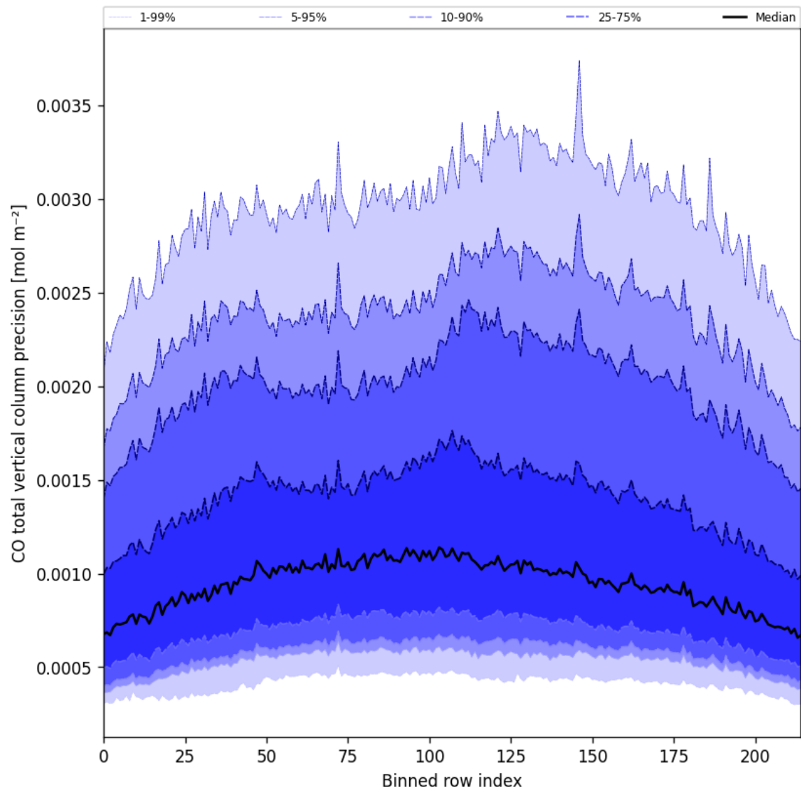
Figure 28: Along track statistics of “CO total vertical column precision” for 2025-05-19 to 2025-05-21
