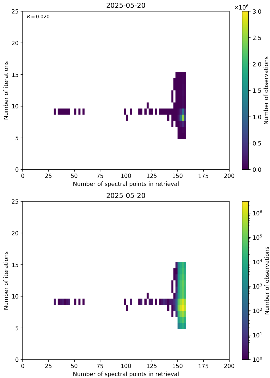
Figure 60: Scatter density plot of “Number of spectral points in retrieval” against “Number of iterations” for 2025-05-19 to 2025-05-21.
