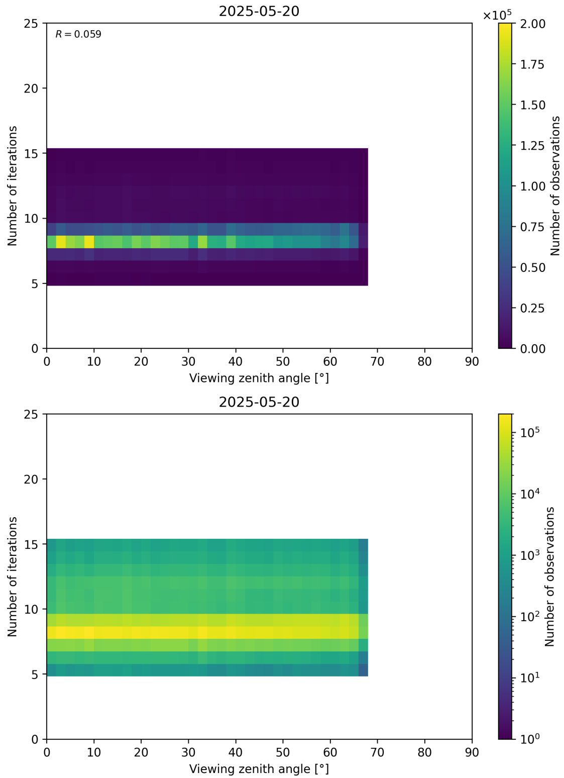
Figure 75: Scatter density plot of “Viewing zenith angle” against “Number of iterations” for 2025-05-19 to 2025-05-21.
