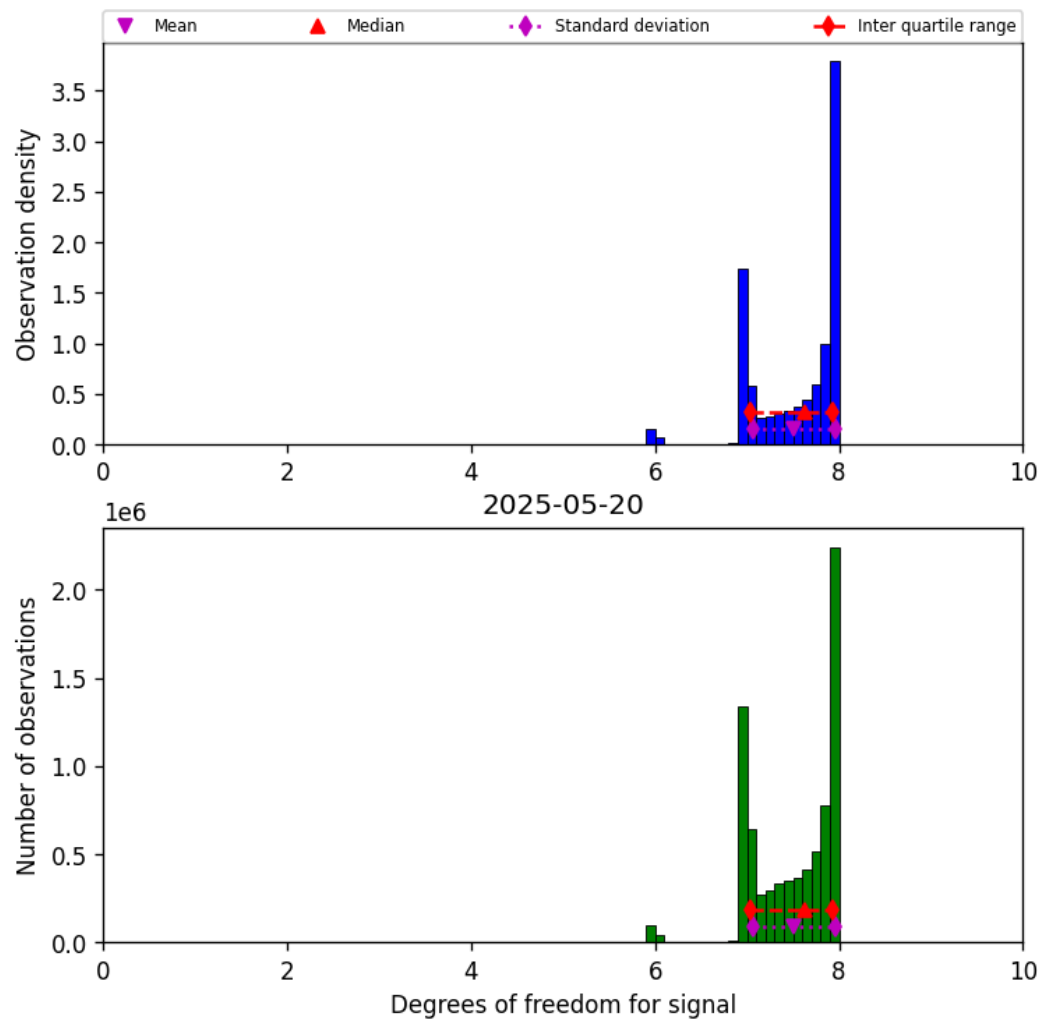
Figure 23: Histogram of “Degrees of freedom for signal” for 2025-05-19 to 2025-05-21
