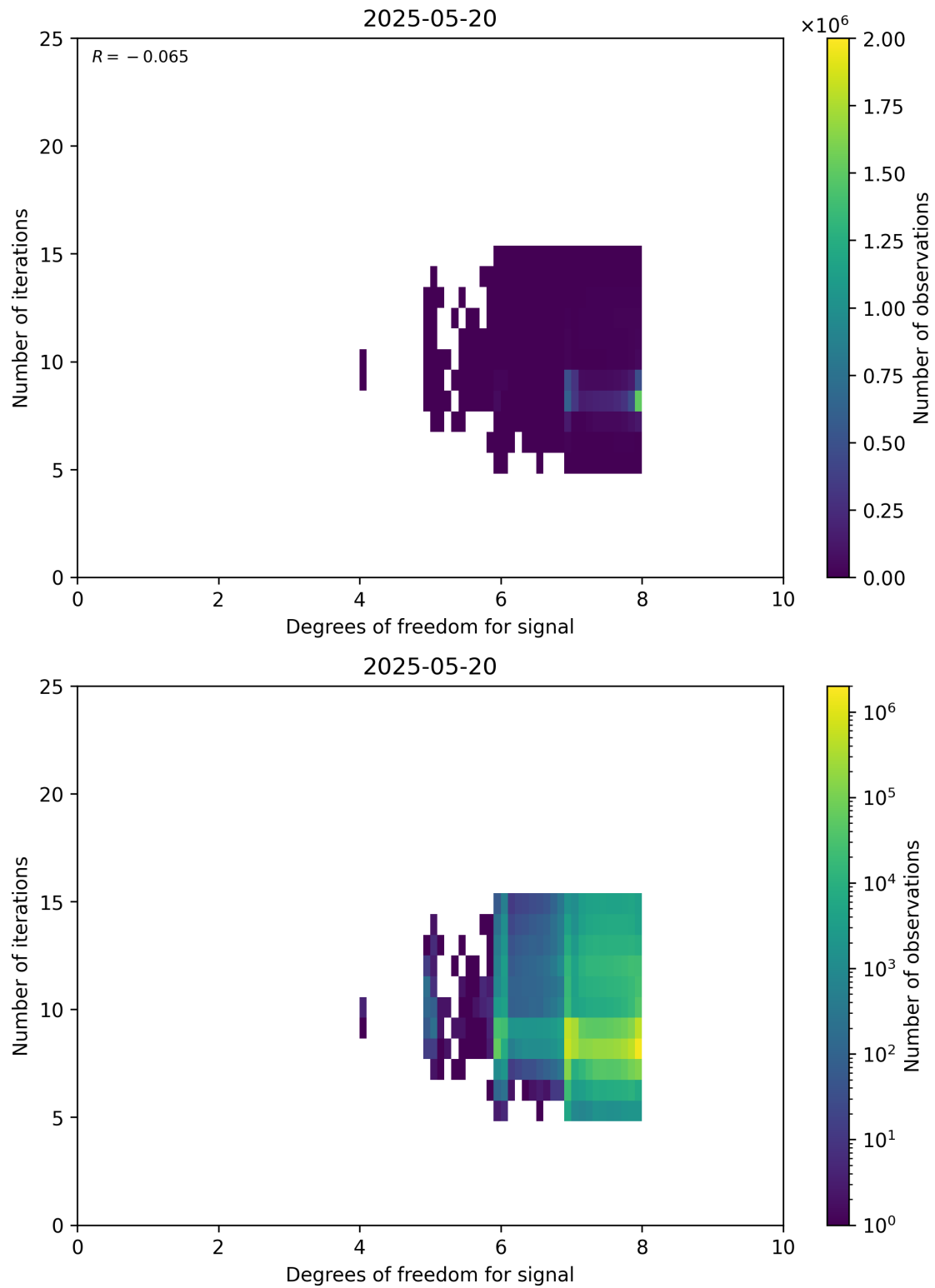
Figure 50: Scatter density plot of “Degrees of freedom for signal” against “Number of iterations” for 2025-05-19 to 2025-05-21.
