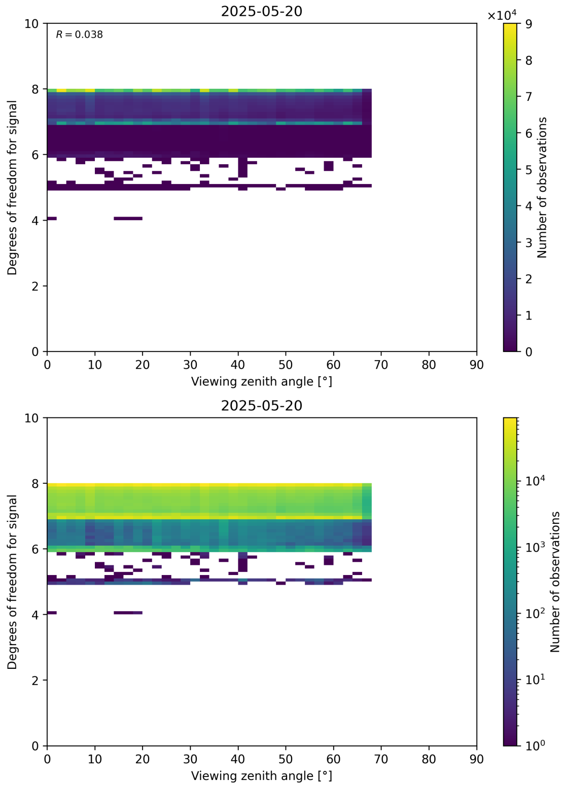
Figure 73: Scatter density plot of “Viewing zenith angle” against “Degrees of freedom for signal” for 2025-05-19 to 2025-05-21.
