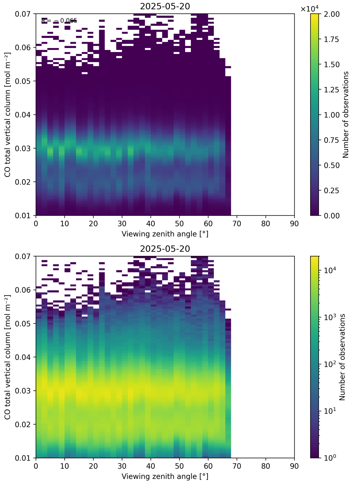
Figure 69: Scatter density plot of “Viewing zenith angle” against “CO total vertical column” for 2025-05-19 to 2025-05-21.
