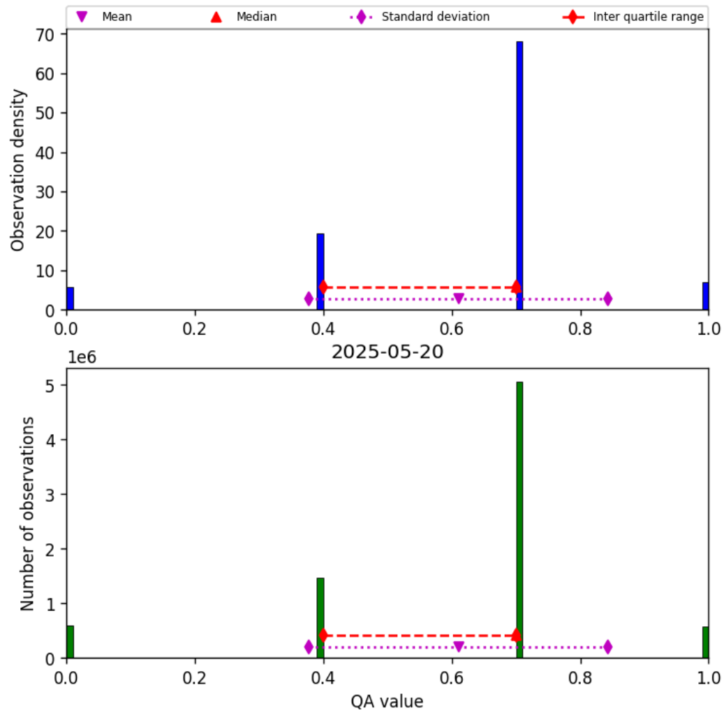
Figure 17: Histogram of “QA value” for 2025-05-19 to 2025-05-21
