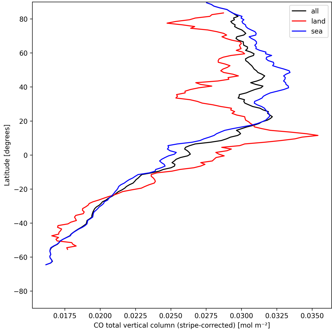
Figure 11: Zonal average of “CO total vertical column (stripe-corrected)” for 2025-05-19 to 2025-05-21.
