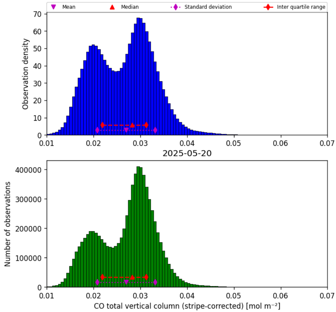
Figure 19: Histogram of “CO total vertical column (stripe-corrected)” for 2025-05-19 to 2025-05-21
