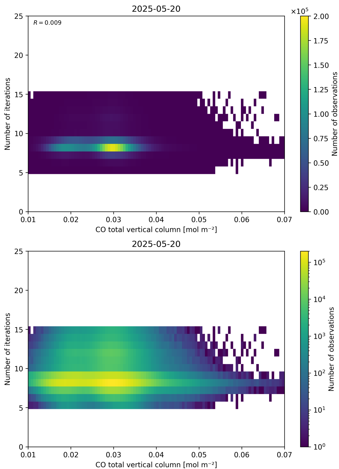
Figure 42: Scatter density plot of “CO total vertical column” against “Number of iterations” for 2025-05-19 to 2025-05-21.
