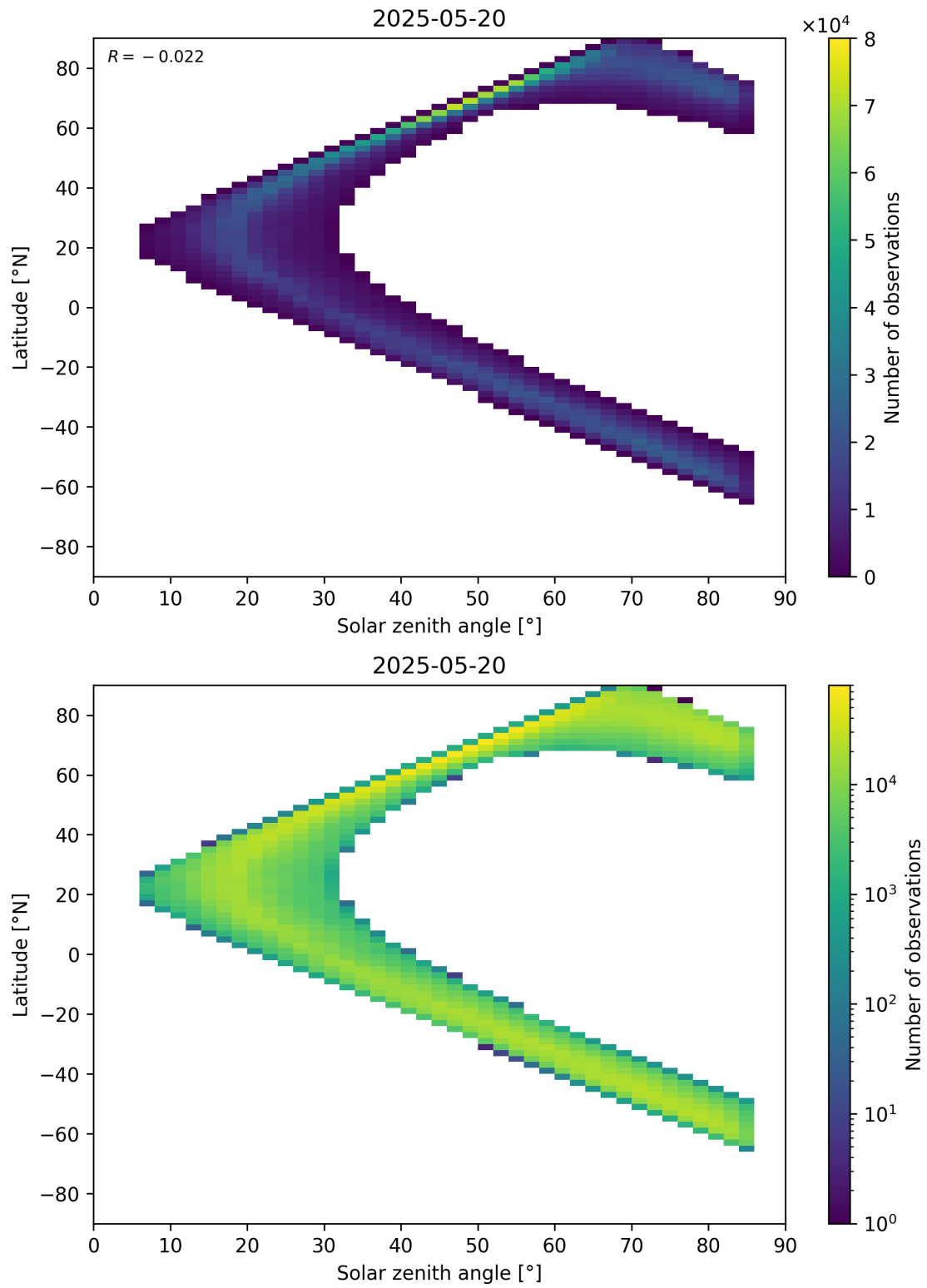
Figure 66: Scatter density plot of “Solar zenith angle” against “Latitude” for 2025-05-19 to 2025-05-21.
