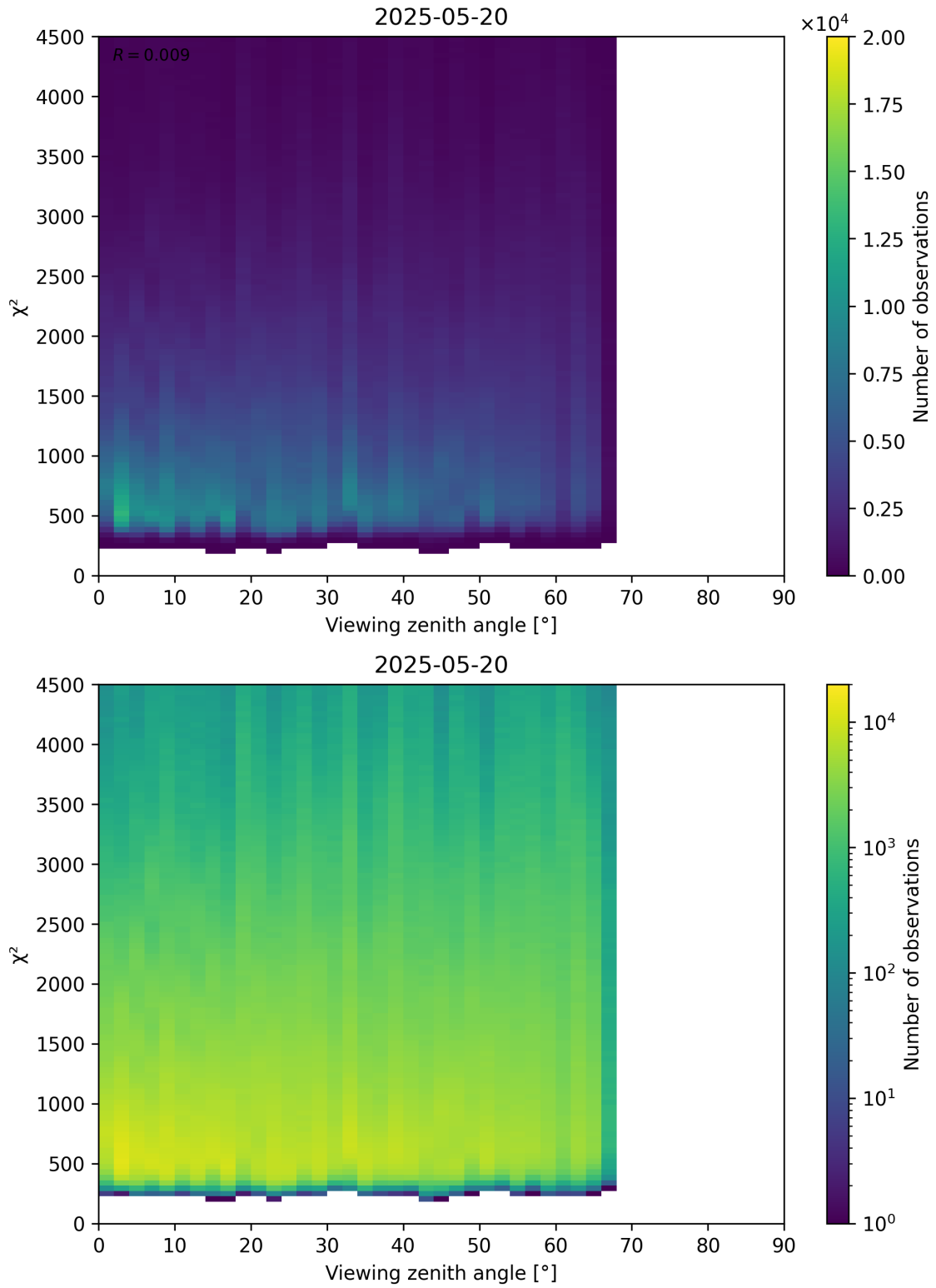
Figure 72: Scatter density plot of “Viewing zenith angle” against “ \chi^2 ” for 2025-05-19 to 2025-05-21.
