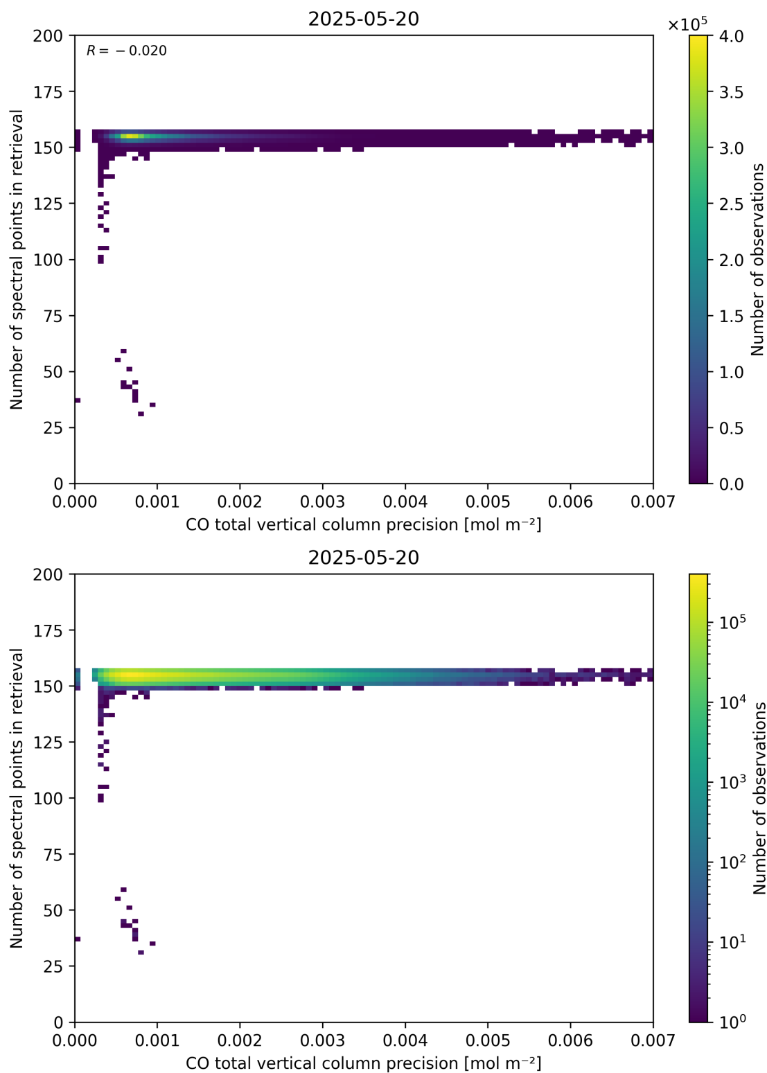
Figure 47: Scatter density plot of “CO total vertical column precision” against “Number of spectral points in retrieval” for 2025-05-19 to 2025-05-21.
