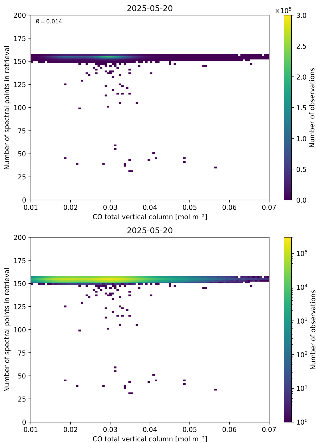
Figure 43: Scatter density plot of “CO total vertical column” against “Number of spectral points in retrieval” for 2025-05-19 to 2025-05-21.
