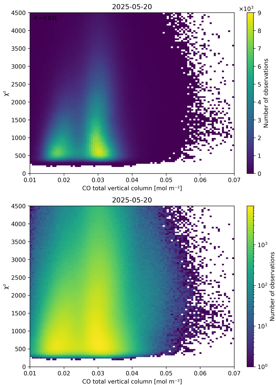
Figure 35: Scatter density plot of “CO total vertical column” against “ \chi^2 ” for 2025-05-19 to 2025-05-21.
