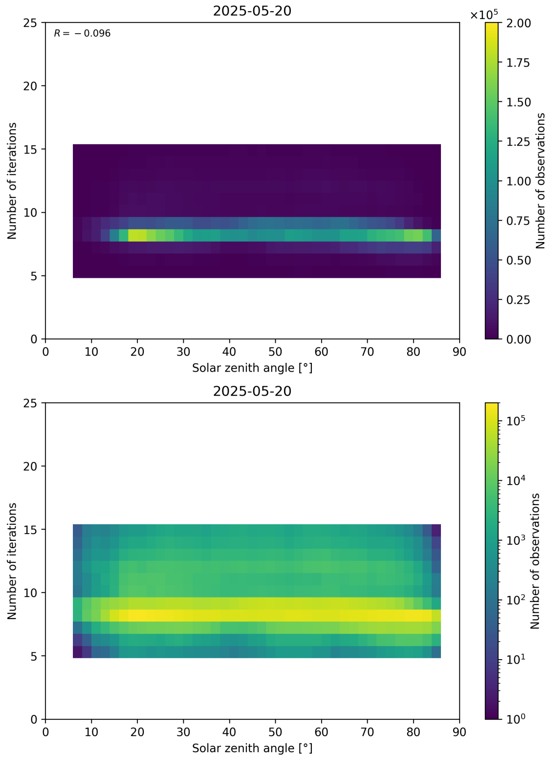
Figure 67: Scatter density plot of “Solar zenith angle” against “Number of iterations” for 2025-05-19 to 2025-05-21.
