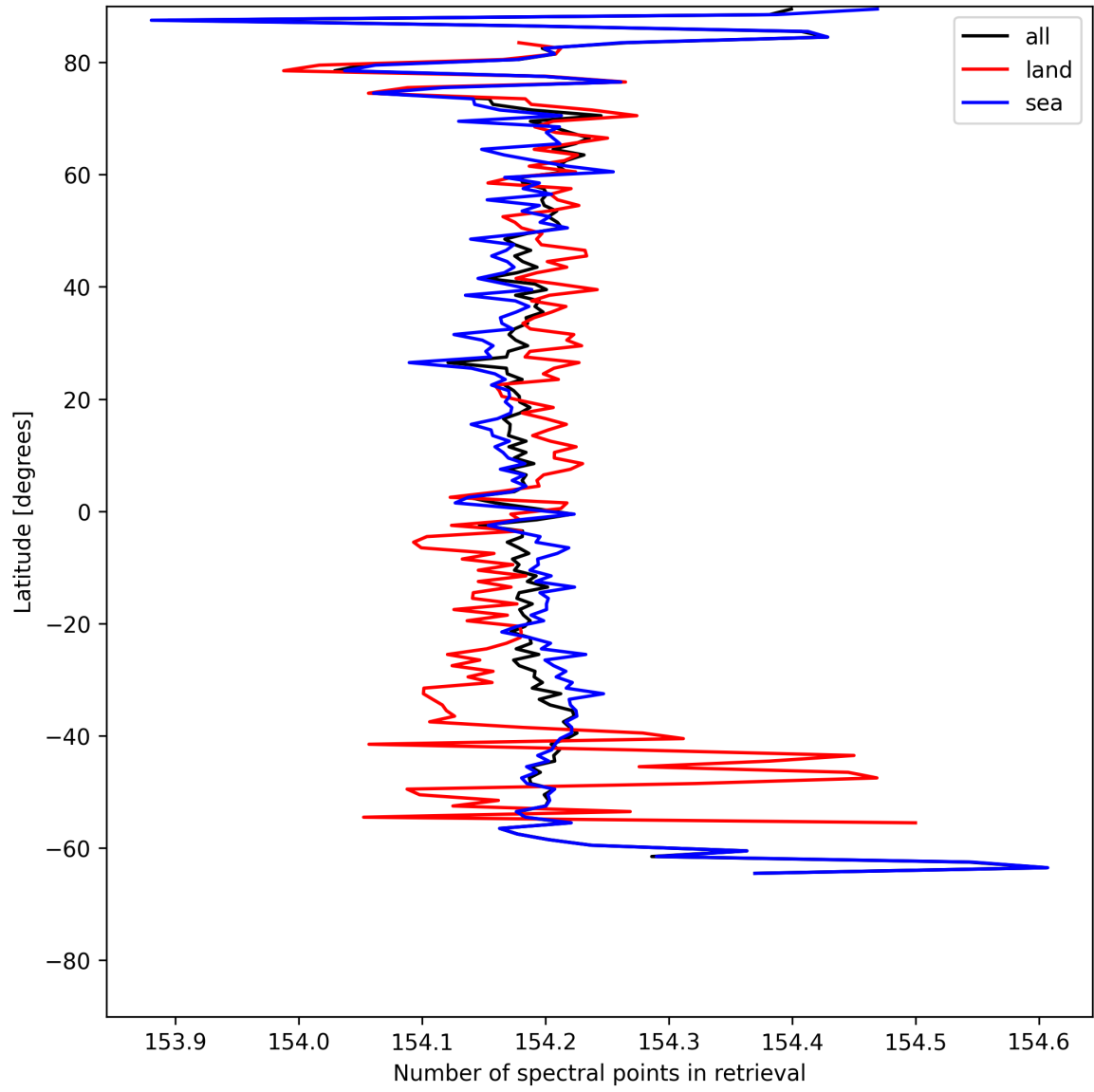
Figure 13: Zonal average of “Number of spectral points in retrieval” for 2025-05-19 to 2025-05-21.
