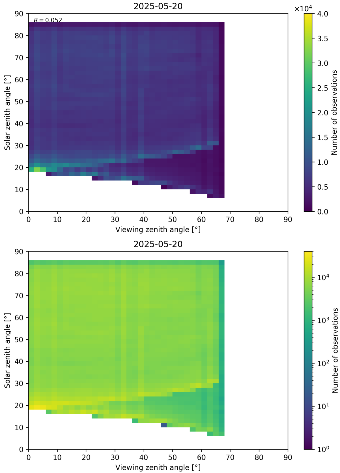
Figure 77: Scatter density plot of “Viewing zenith angle” against “Solar zenith angle” for 2025-05-19 to 2025-05-21.
