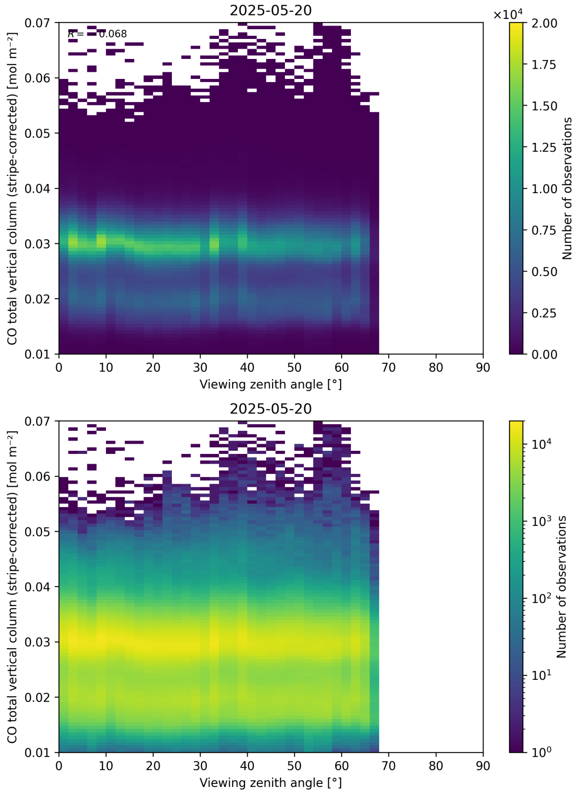
Figure 70: Scatter density plot of “Viewing zenith angle” against “CO total vertical column (stripe-corrected)” for 2025-05-19 to 2025-05-21.
