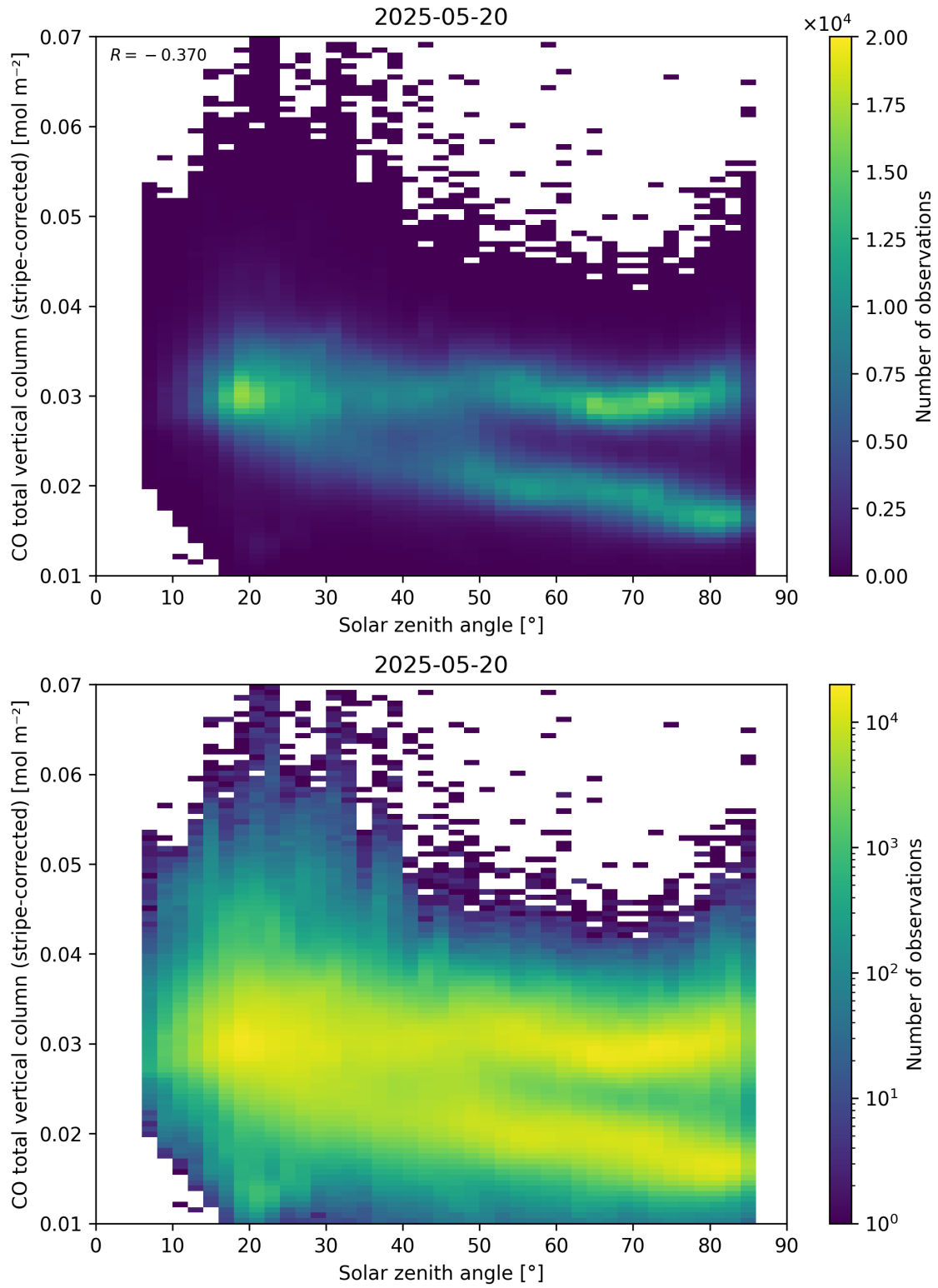
Figure 62: Scatter density plot of “Solar zenith angle” against “CO total vertical column (stripe-corrected)” for 2025-05-19 to 2025-05-21.
