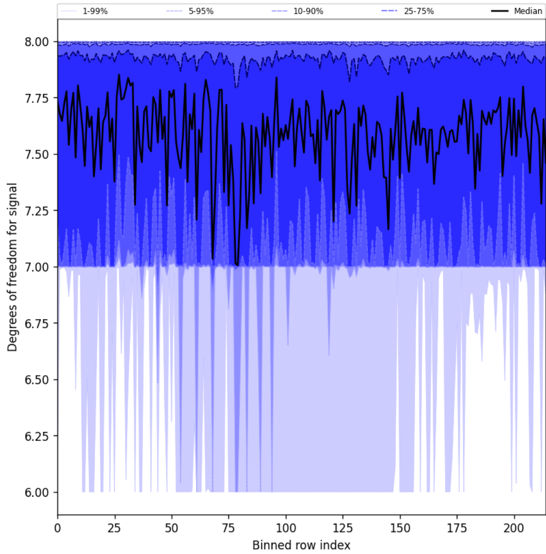
Figure 31: Along track statistics of “Degrees of freedom for signal” for 2025-05-19 to 2025-05-21
