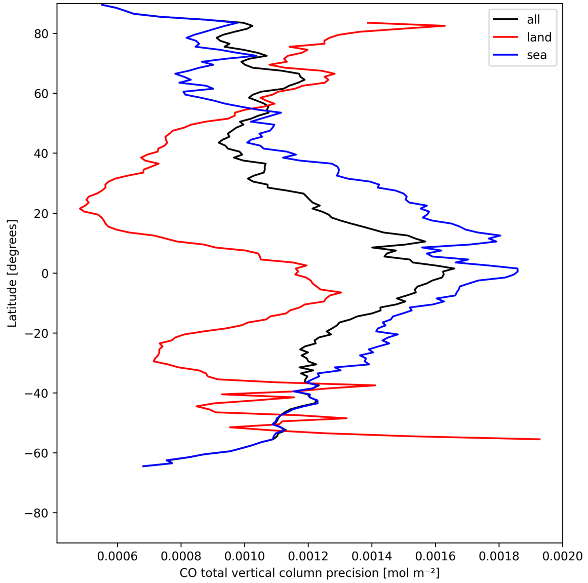
Figure 12: Zonal average of “CO total vertical column precision” for 2025-05-19 to 2025-05-21.
