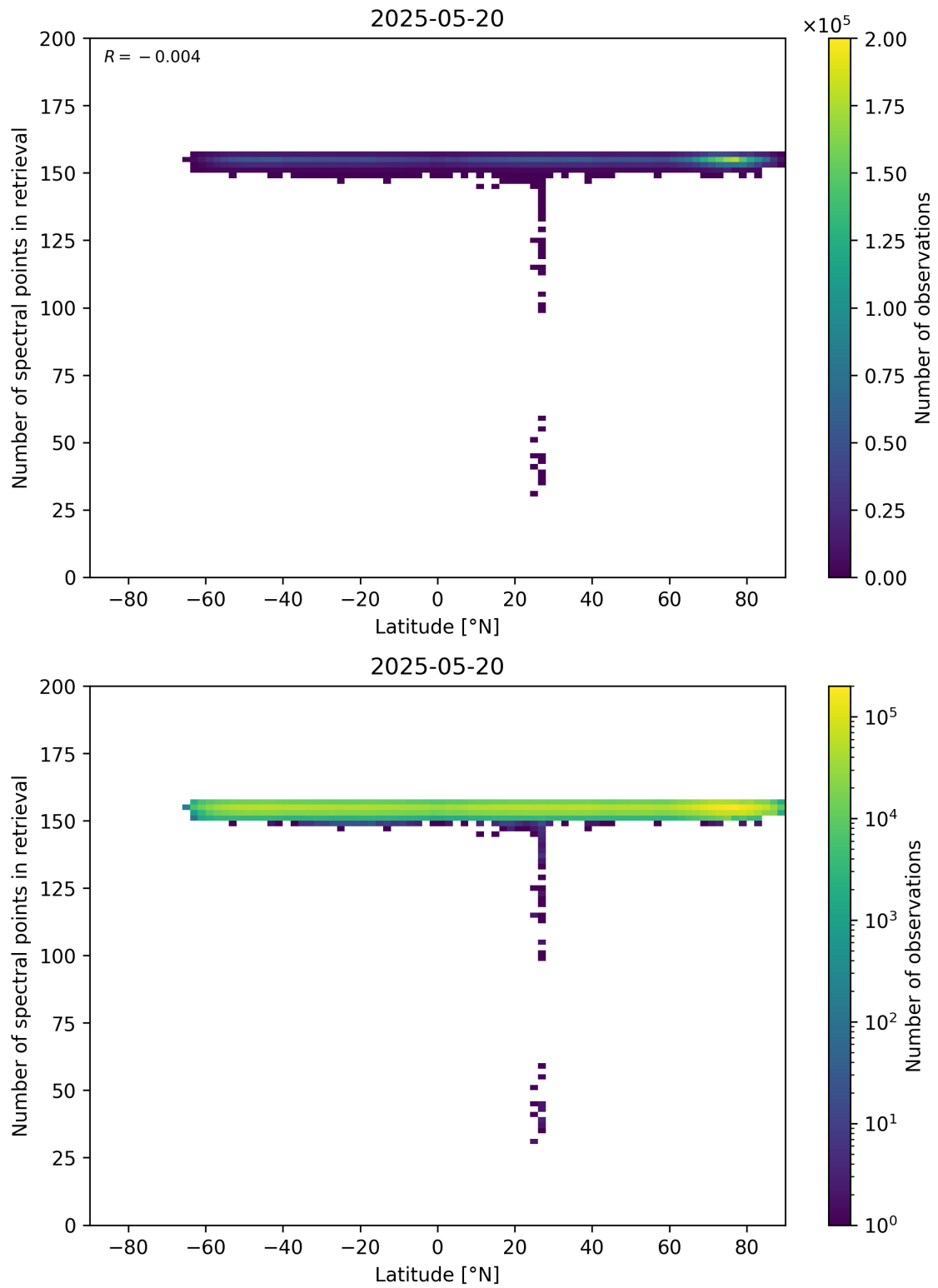
Figure 57: Scatter density plot of “Latitude” against “Number of spectral points in retrieval” for 2025-05-19 to 2025-05-21.
