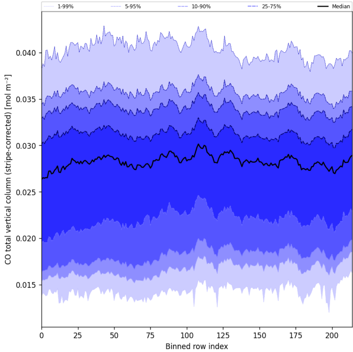
Figure 27: Along track statistics of “CO total vertical column (stripe-corrected)” for 2025-05-19 to 2025-05-21
