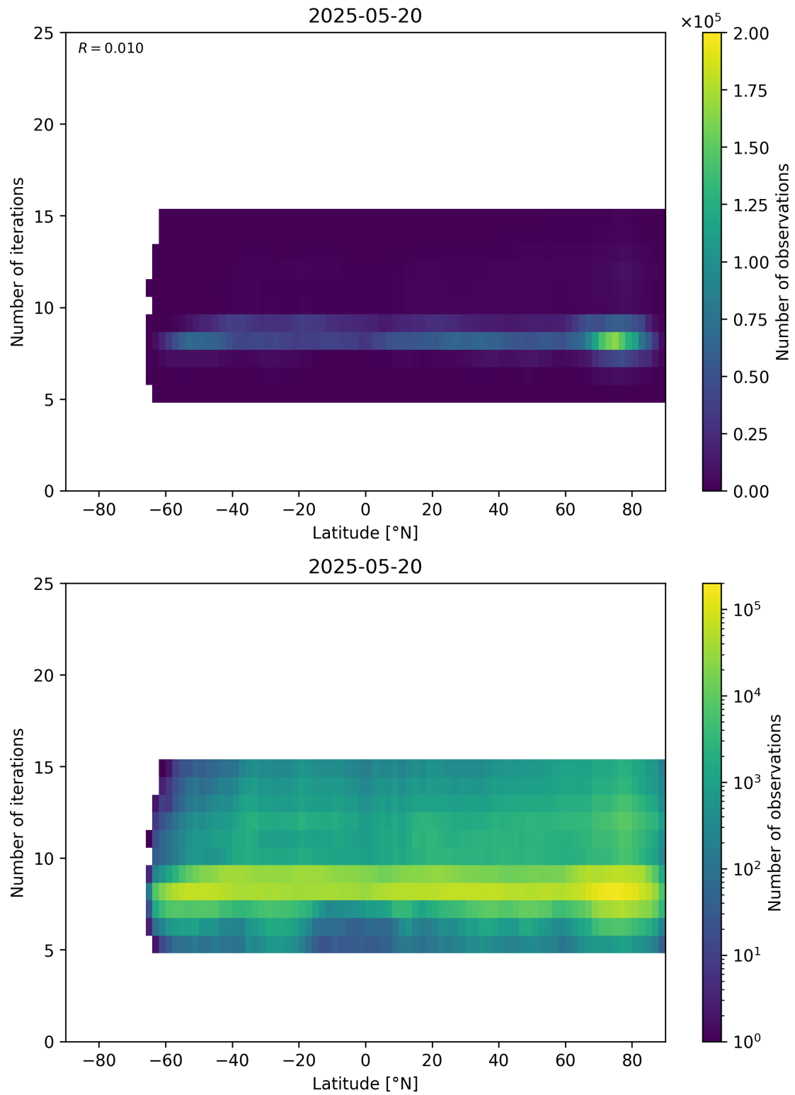
Figure 56: Scatter density plot of “Latitude” against “Number of iterations” for 2025-05-19 to 2025-05-21.
