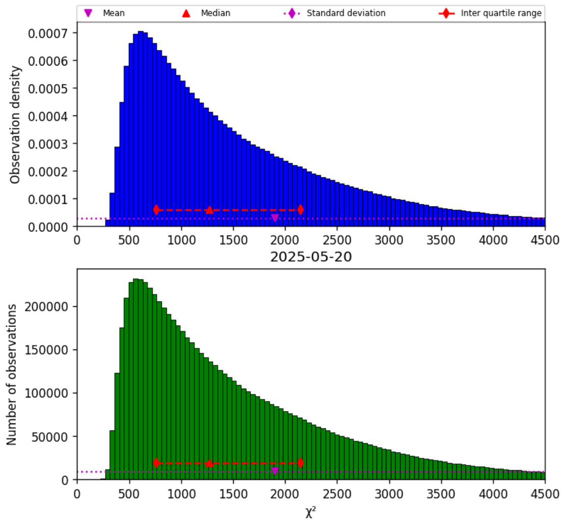
Figure 22: Histogram of “ \chi^2 ” for 2025-05-19 to 2025-05-21
