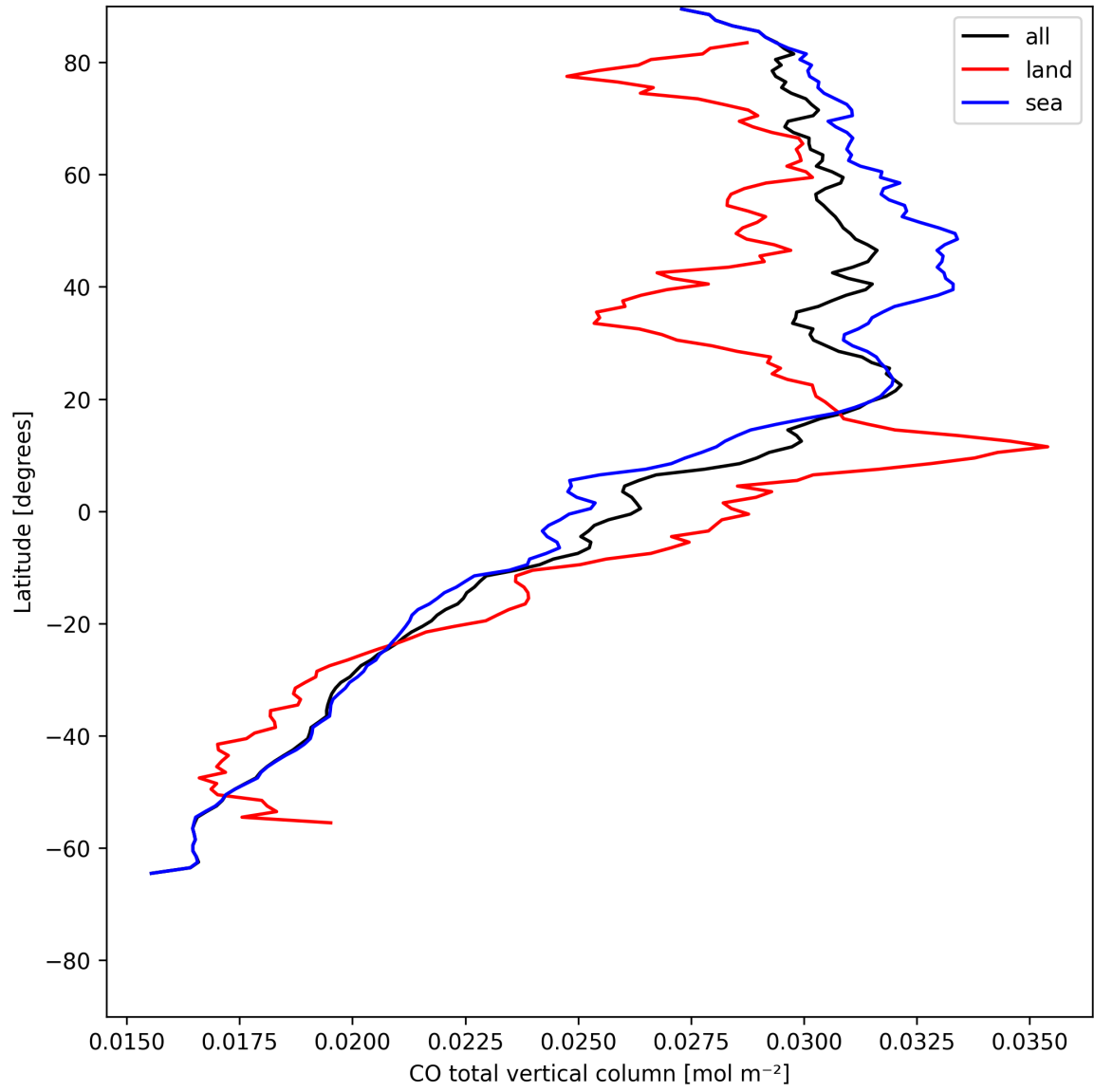
Figure 10: Zonal average of “CO total vertical column” for 2025-05-19 to 2025-05-21.
