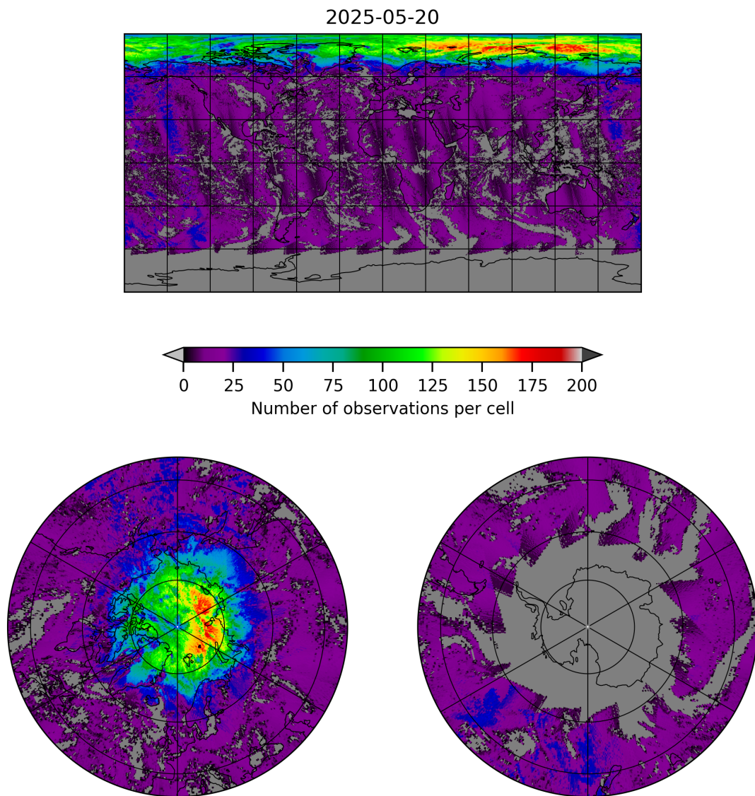
Figure 8: Map of the number of observations for 2025-05-19 to 2025-05-21
