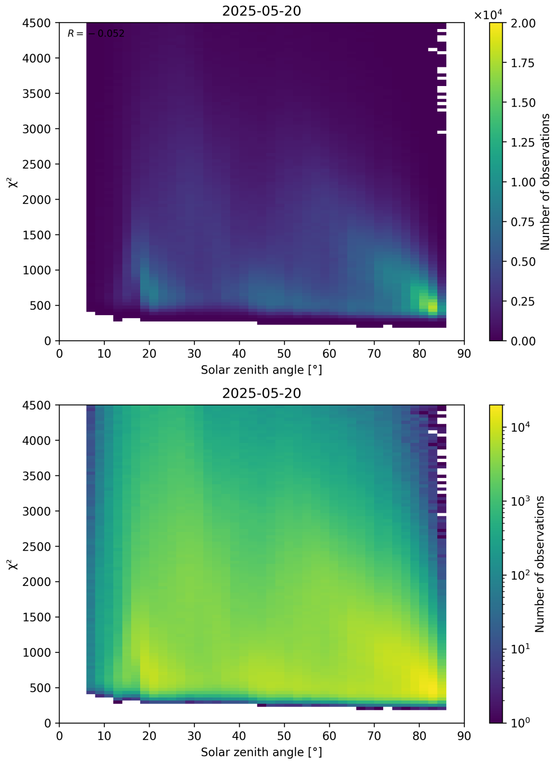
Figure 64: Scatter density plot of “Solar zenith angle” against “ \chi^2 ” for 2025-05-19 to 2025-05-21.
