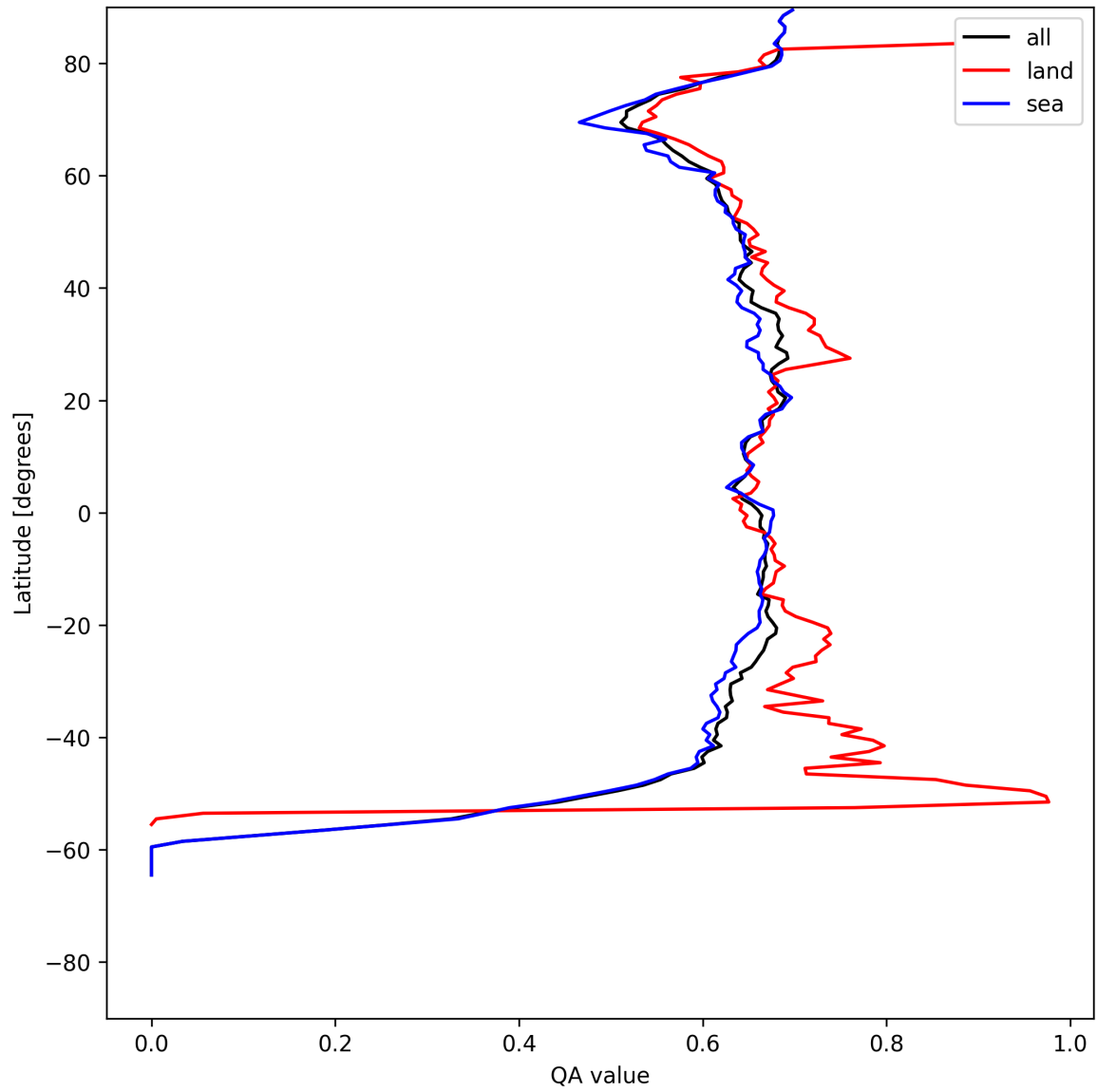
Figure 9: Zonal average of “QA value” for 2025-05-19 to 2025-05-21.
