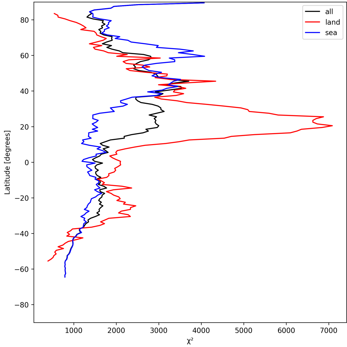
Figure 14: Zonal average of “ \chi^2 ” for 2025-05-19 to 2025-05-21.
