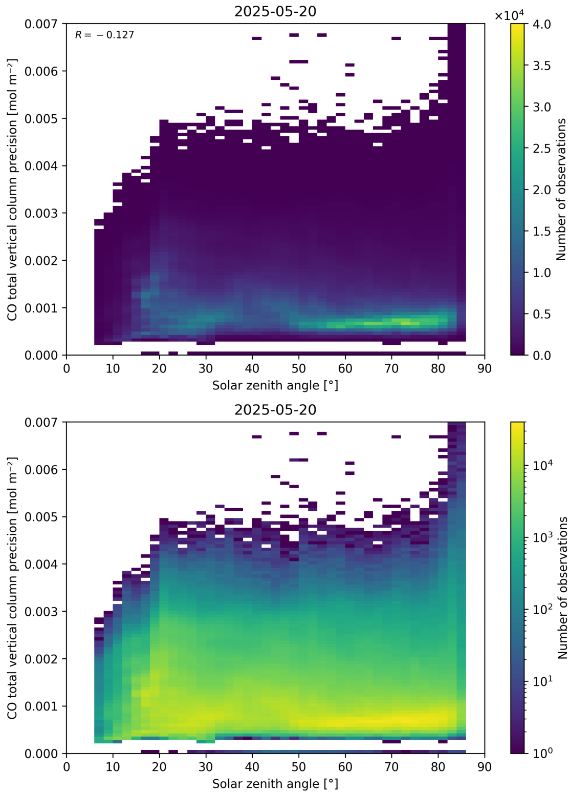
Figure 63: Scatter density plot of “Solar zenith angle” against “CO total vertical column precision” for 2025-05-19 to 2025-05-21.
