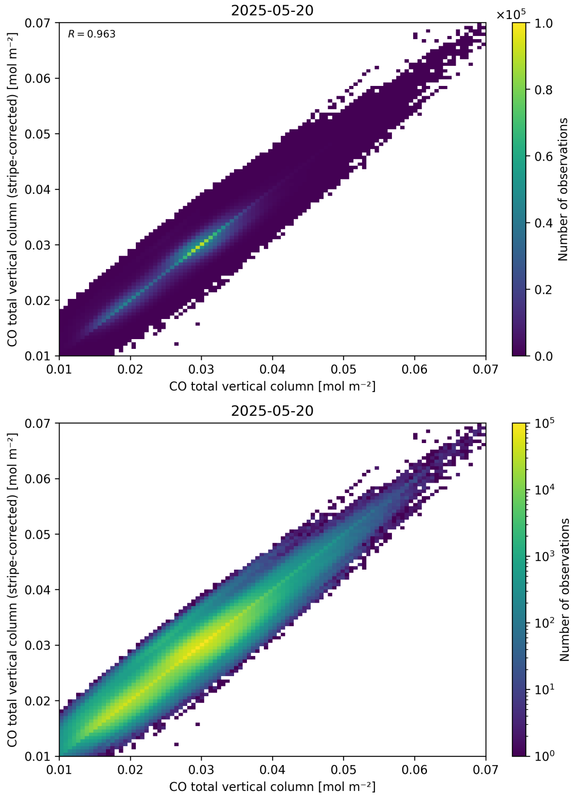
Figure 33: Scatter density plot of “CO total vertical column” against “CO total vertical column (stripe-corrected)” for 2025-05-19 to 2025-05-21.
