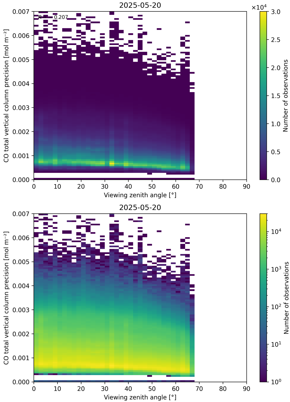
Figure 71: Scatter density plot of “Viewing zenith angle” against “CO total vertical column precision” for 2025-05-19 to 2025-05-21.
