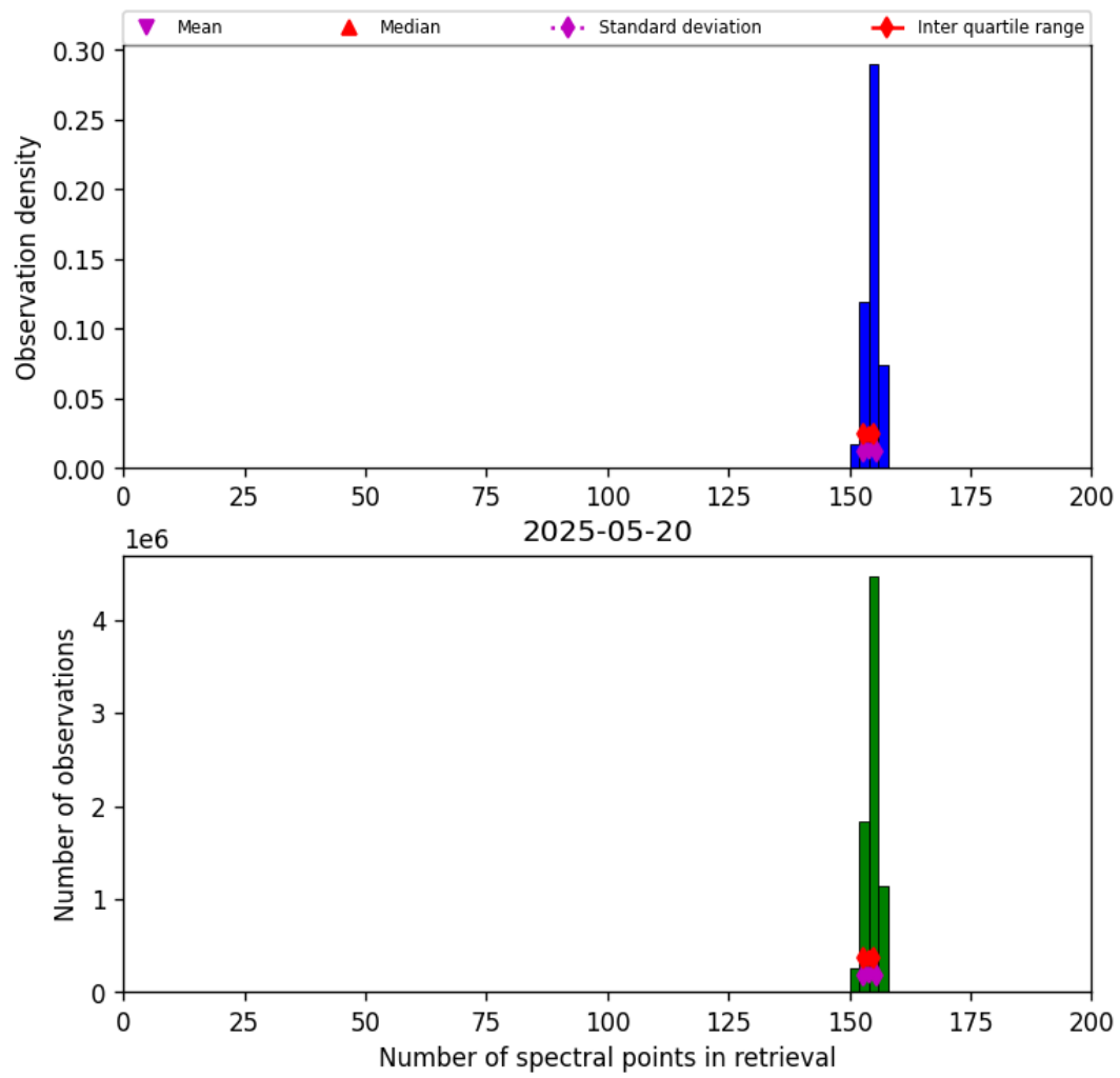
Figure 21: Histogram of “Number of spectral points in retrieval” for 2025-05-19 to 2025-05-21
