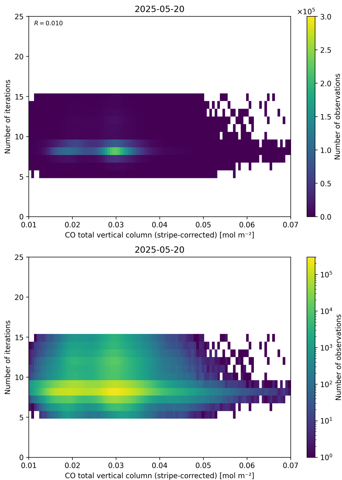
Figure 39: Scatter density plot of “CO total vertical column (stripe-corrected)” against “Number of iterations” for 2025-05-19 to 2025-05-21.
