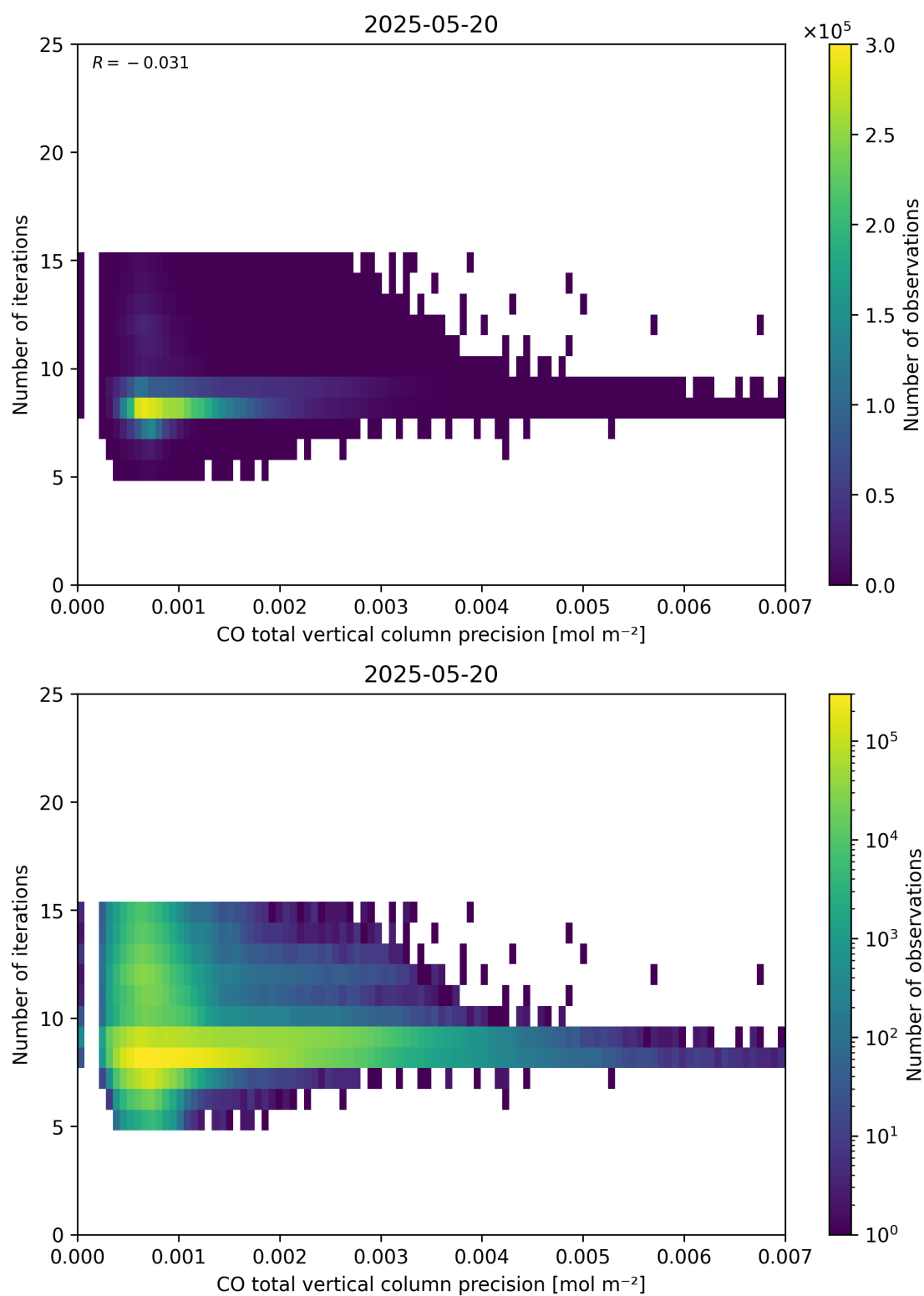
Figure 46: Scatter density plot of “CO total vertical column precision” against “Number of iterations” for 2025-05-19 to 2025-05-21.
