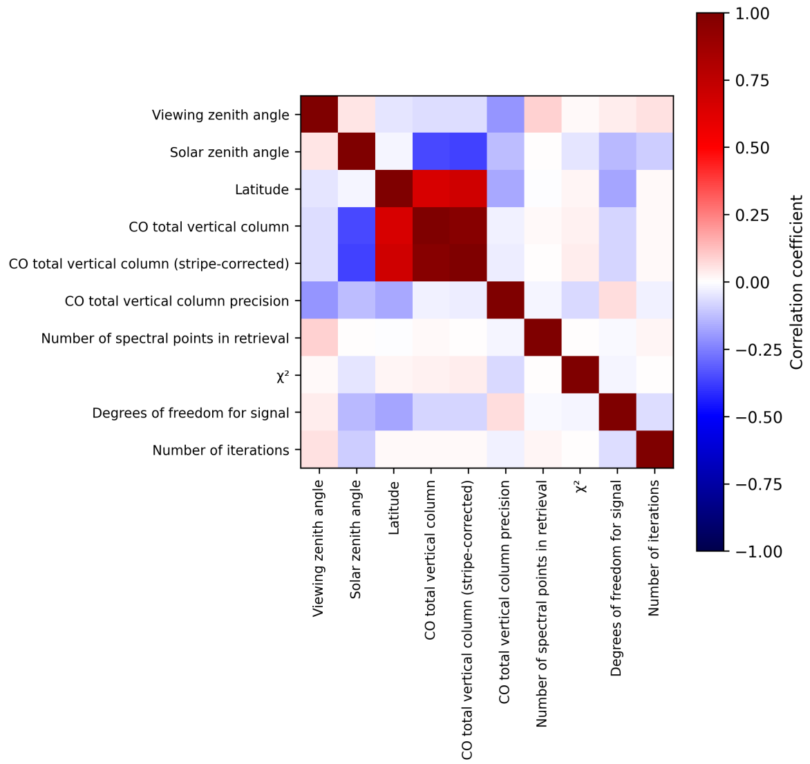
Figure 2: Map of correlation matrix for 2025-05-19 to 2025-05-21.
