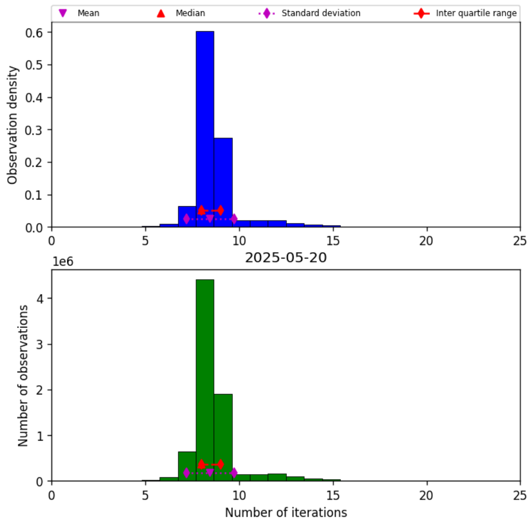
Figure 24: Histogram of “Number of iterations” for 2025-05-19 to 2025-05-21
