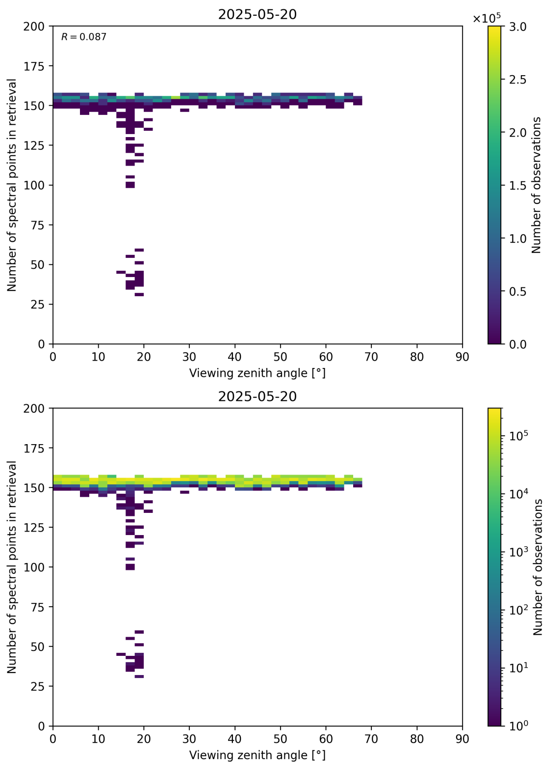
Figure 76: Scatter density plot of “Viewing zenith angle” against “Number of spectral points in retrieval” for 2025-05-19 to 2025-05-21.
