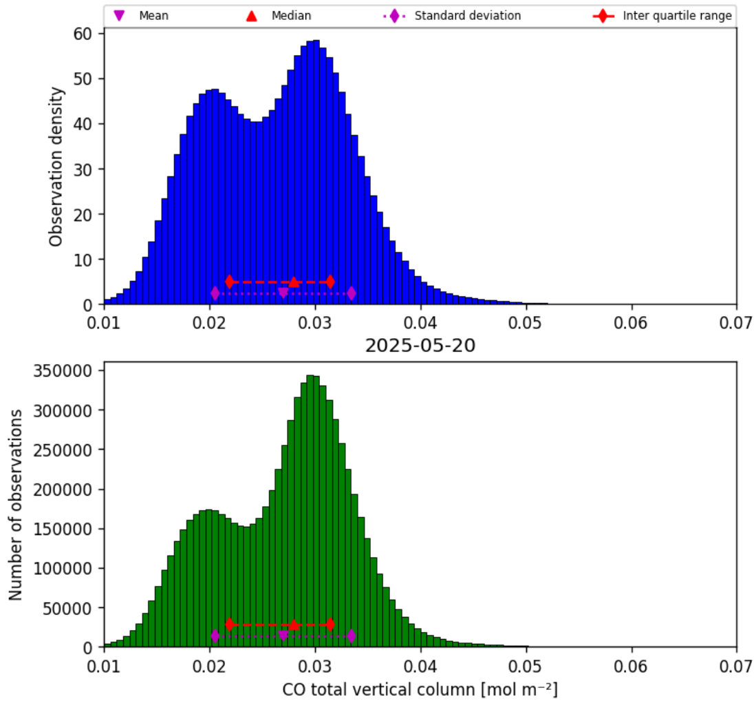
Figure 18: Histogram of “CO total vertical column” for 2025-05-19 to 2025-05-21
