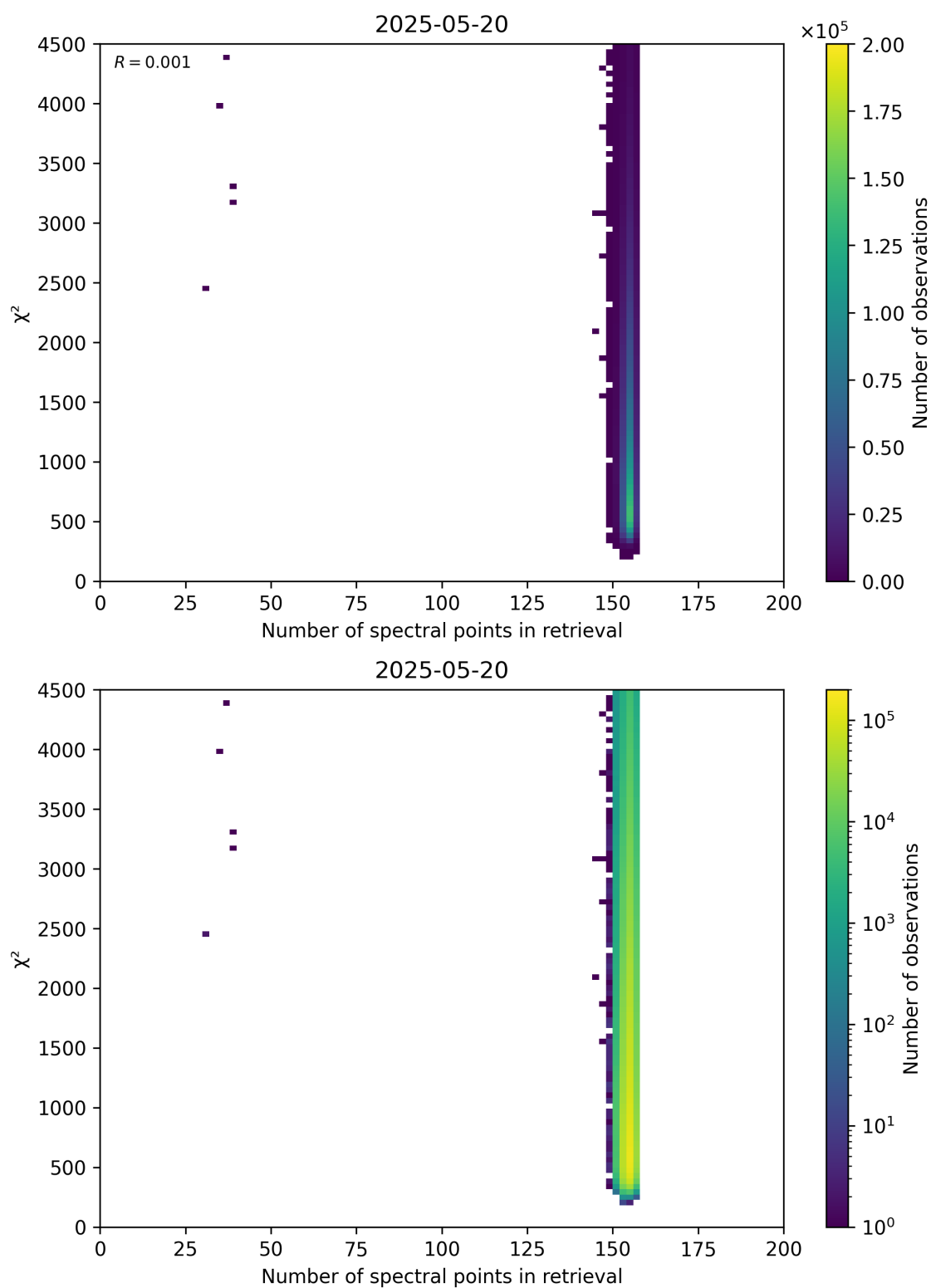
Figure 58: Scatter density plot of “Number of spectral points in retrieval” against “ \chi^2 ” for 2025-05-19 to 2025-05-21.
