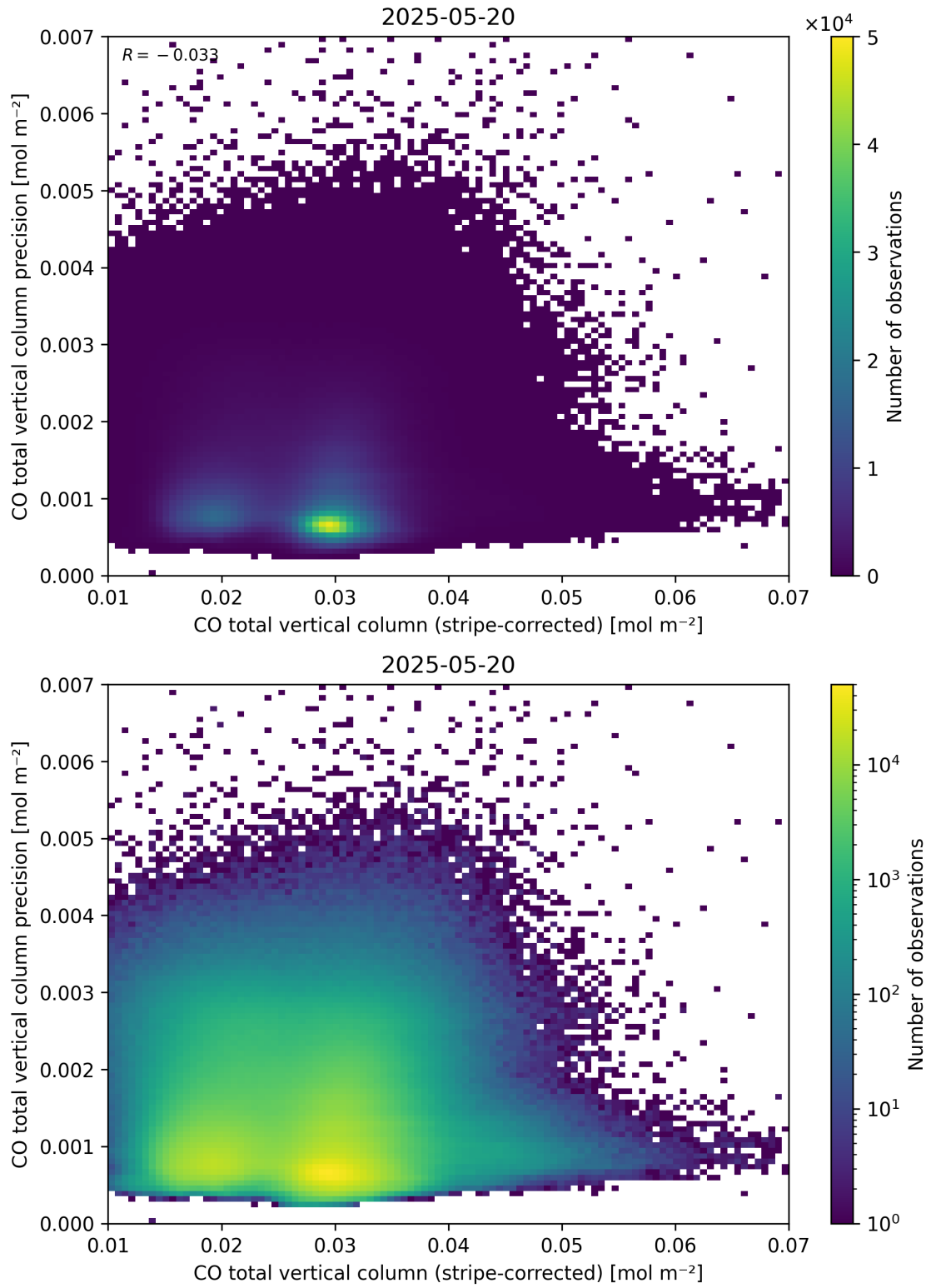
Figure 36: Scatter density plot of “CO total vertical column (stripe-corrected)” against “CO total vertical column precision” for 2025-05-19 to 2025-05-21.
