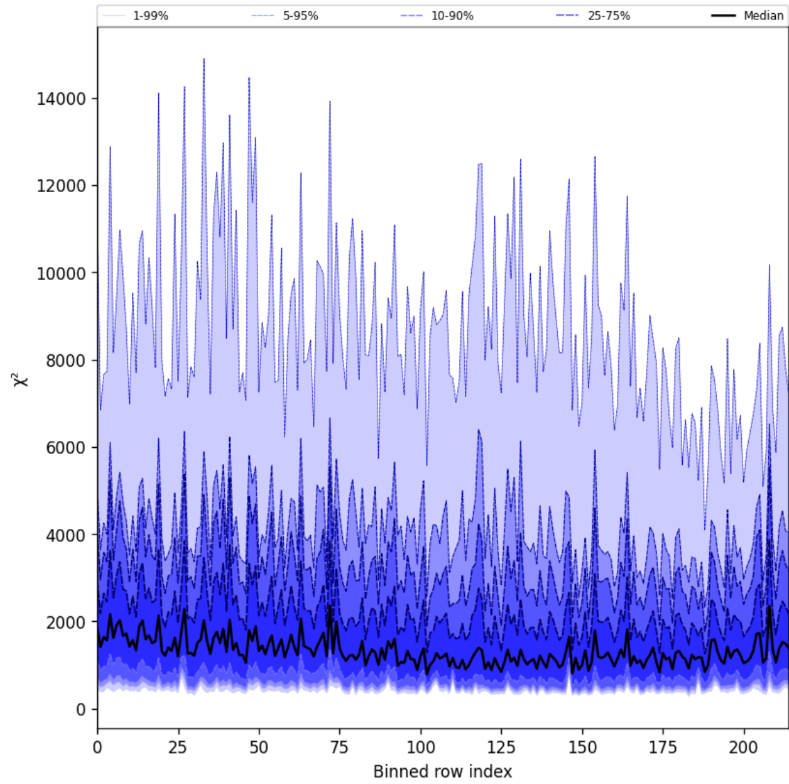
Figure 30: Along track statistics of “ \chi^2 ” for 2025-05-19 to 2025-05-21
