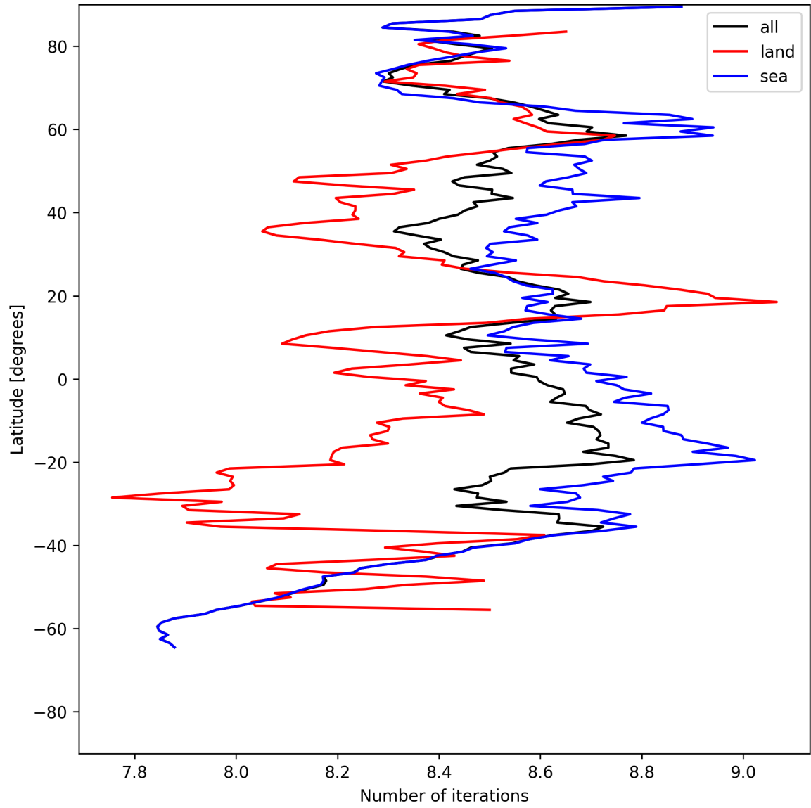
Figure 16: Zonal average of “Number of iterations” for 2025-05-19 to 2025-05-21.
