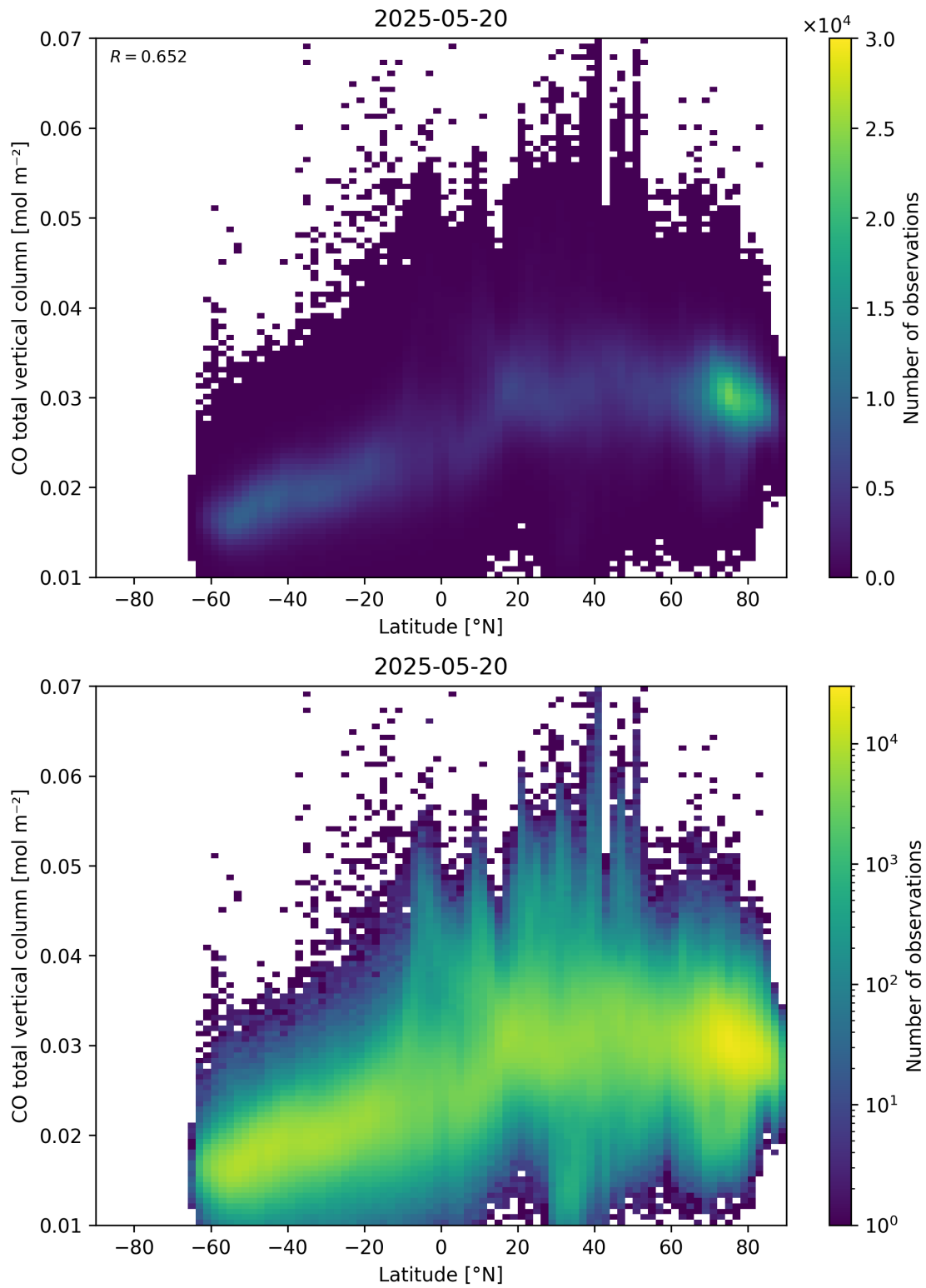
Figure 51: Scatter density plot of “Latitude” against “CO total vertical column” for 2025-05-19 to 2025-05-21.
