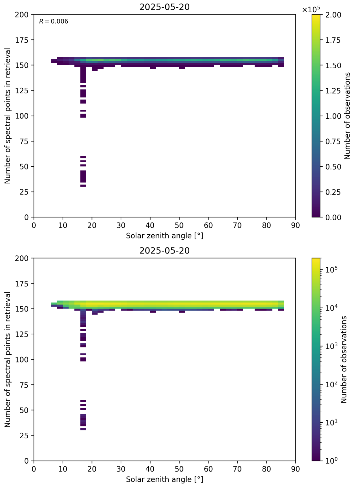
Figure 68: Scatter density plot of “Solar zenith angle” against “Number of spectral points in retrieval” for 2025-05-19 to 2025-05-21.
