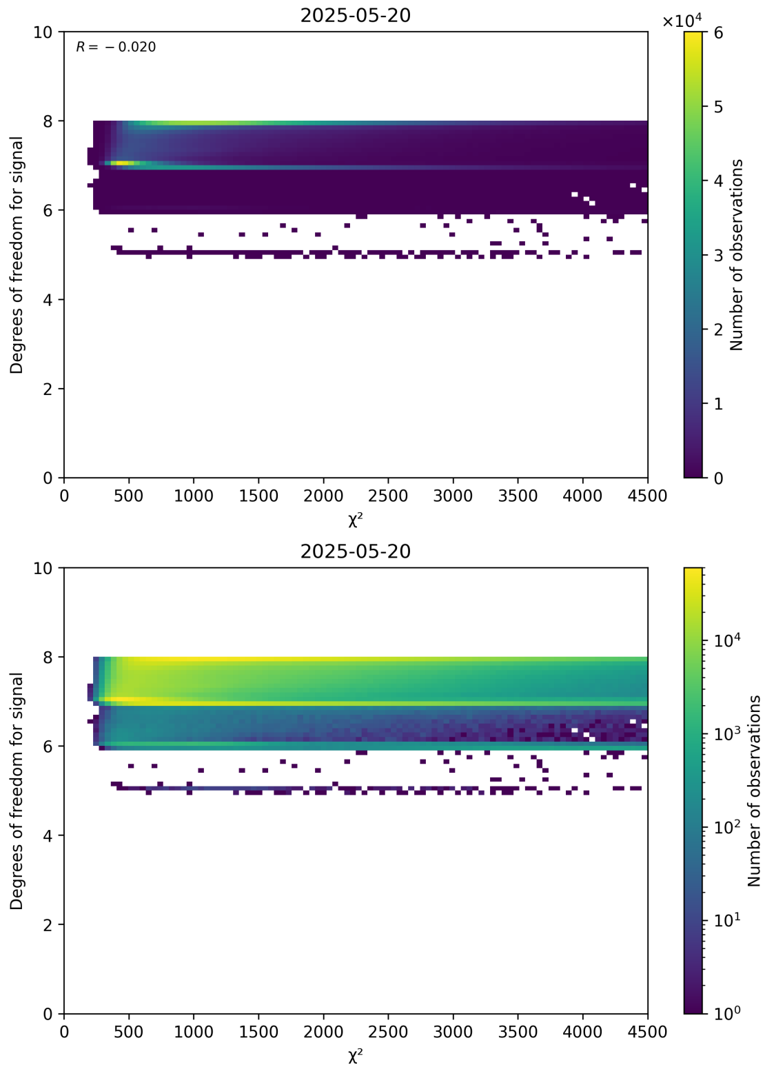
Figure 48: Scatter density plot of “ \chi^2 ” against “Degrees of freedom for signal” for 2025-05-19 to 2025-05-21.
