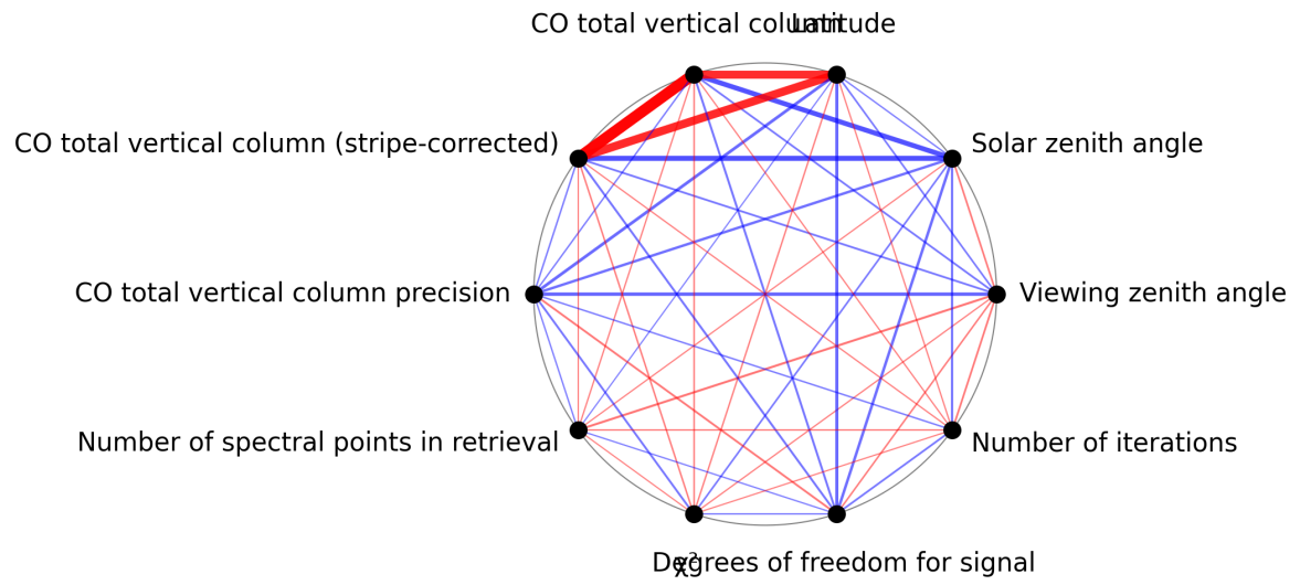
Figure 1: Map of correlation graph for 2025-05-19 to 2025-05-21.
