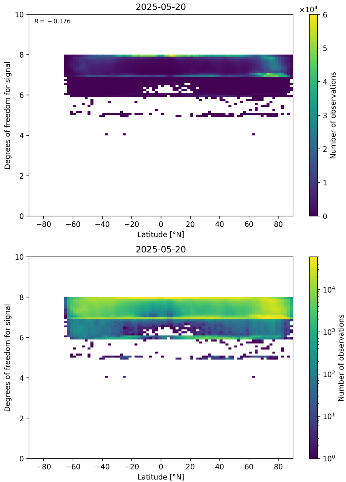
Figure 55: Scatter density plot of “Latitude” against “Degrees of freedom for signal” for 2025-05-19 to 2025-05-21.
