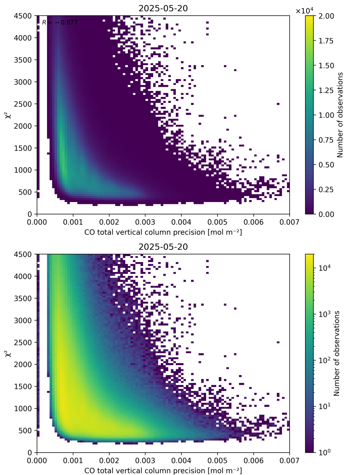
Figure 44: Scatter density plot of “CO total vertical column precision” against “ \chi^2 ” for 2025-05-19 to 2025-05-21.
