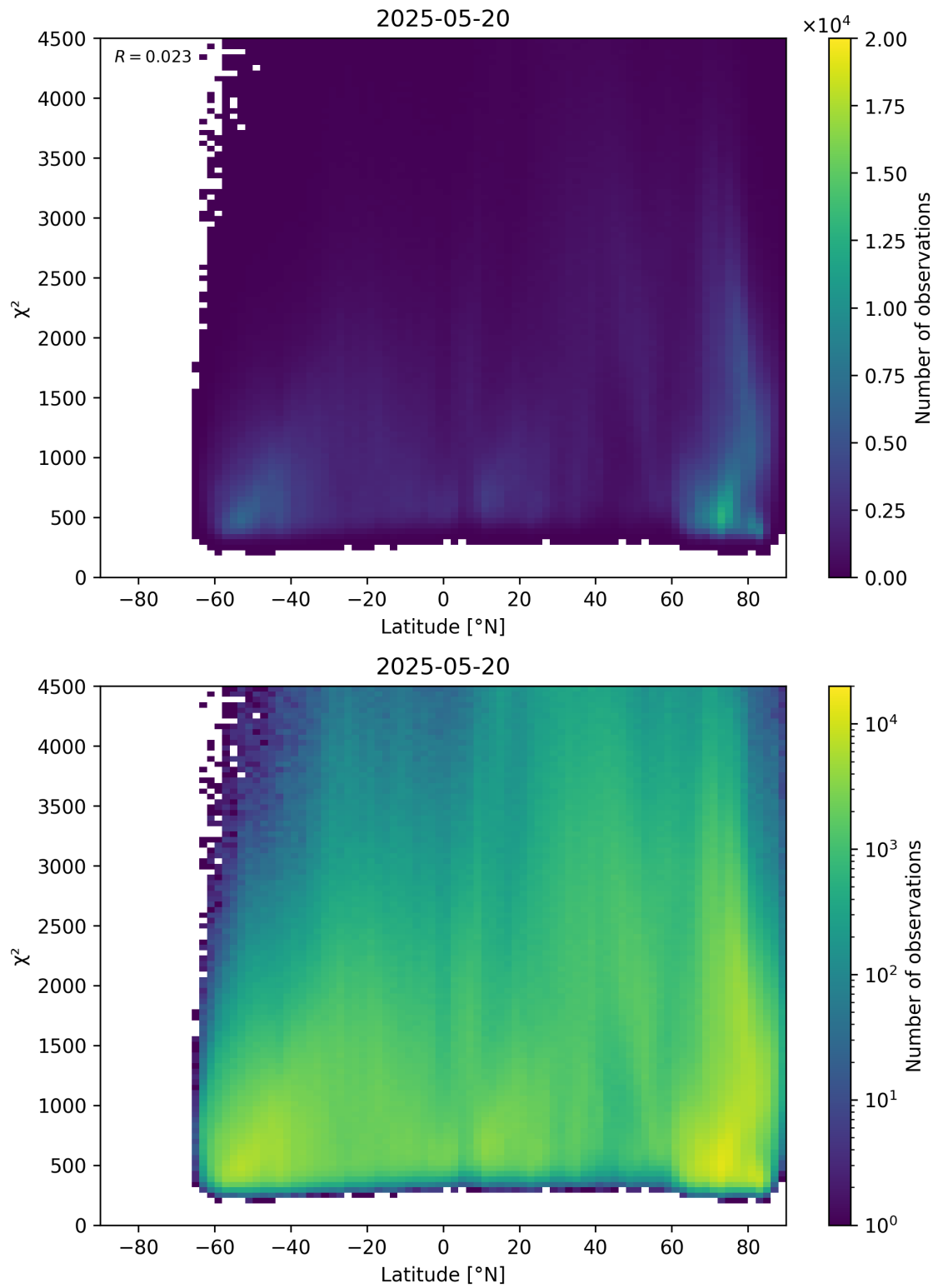
Figure 54: Scatter density plot of “Latitude” against “ \chi^2 ” for 2025-05-19 to 2025-05-21.
