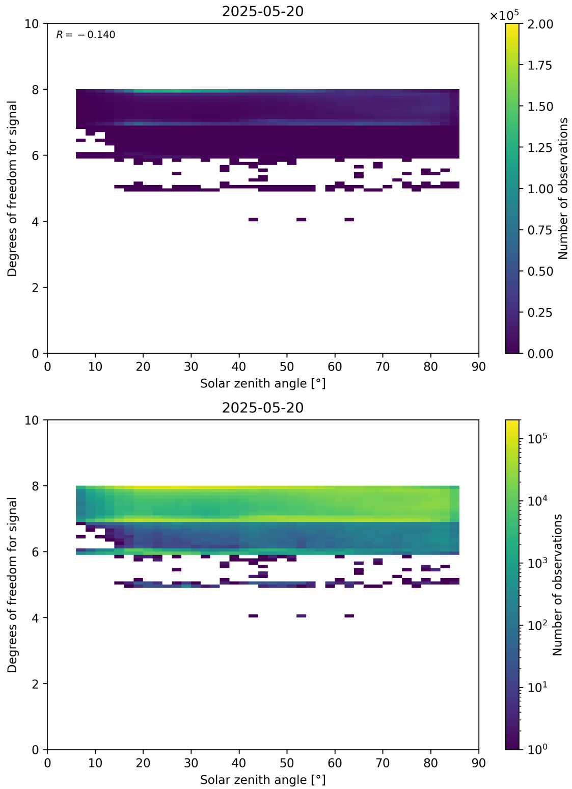
Figure 65: Scatter density plot of “Solar zenith angle” against “Degrees of freedom for signal” for 2025-05-19 to 2025-05-21.
