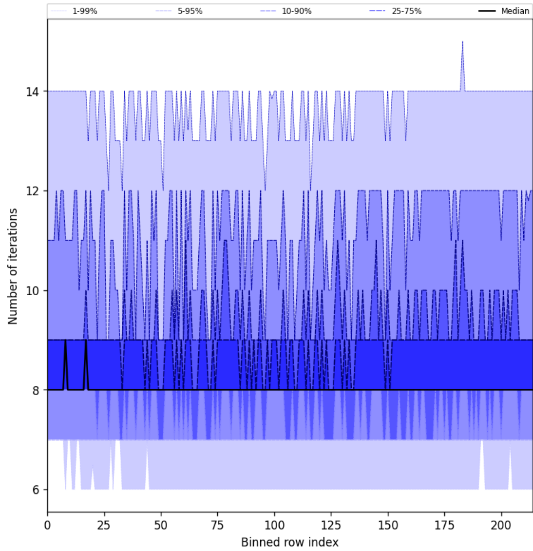
Figure 32: Along track statistics of “Number of iterations” for 2025-05-19 to 2025-05-21
