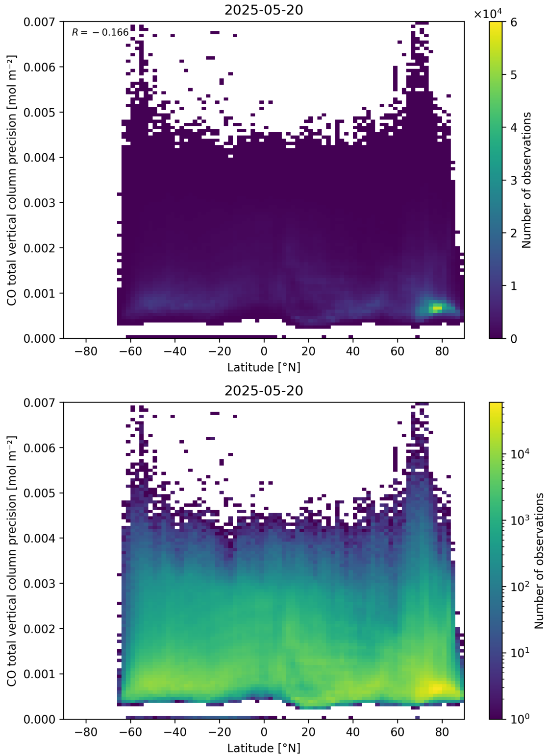
Figure 53: Scatter density plot of “Latitude” against “CO total vertical column precision” for 2025-05-19 to 2025-05-21.
