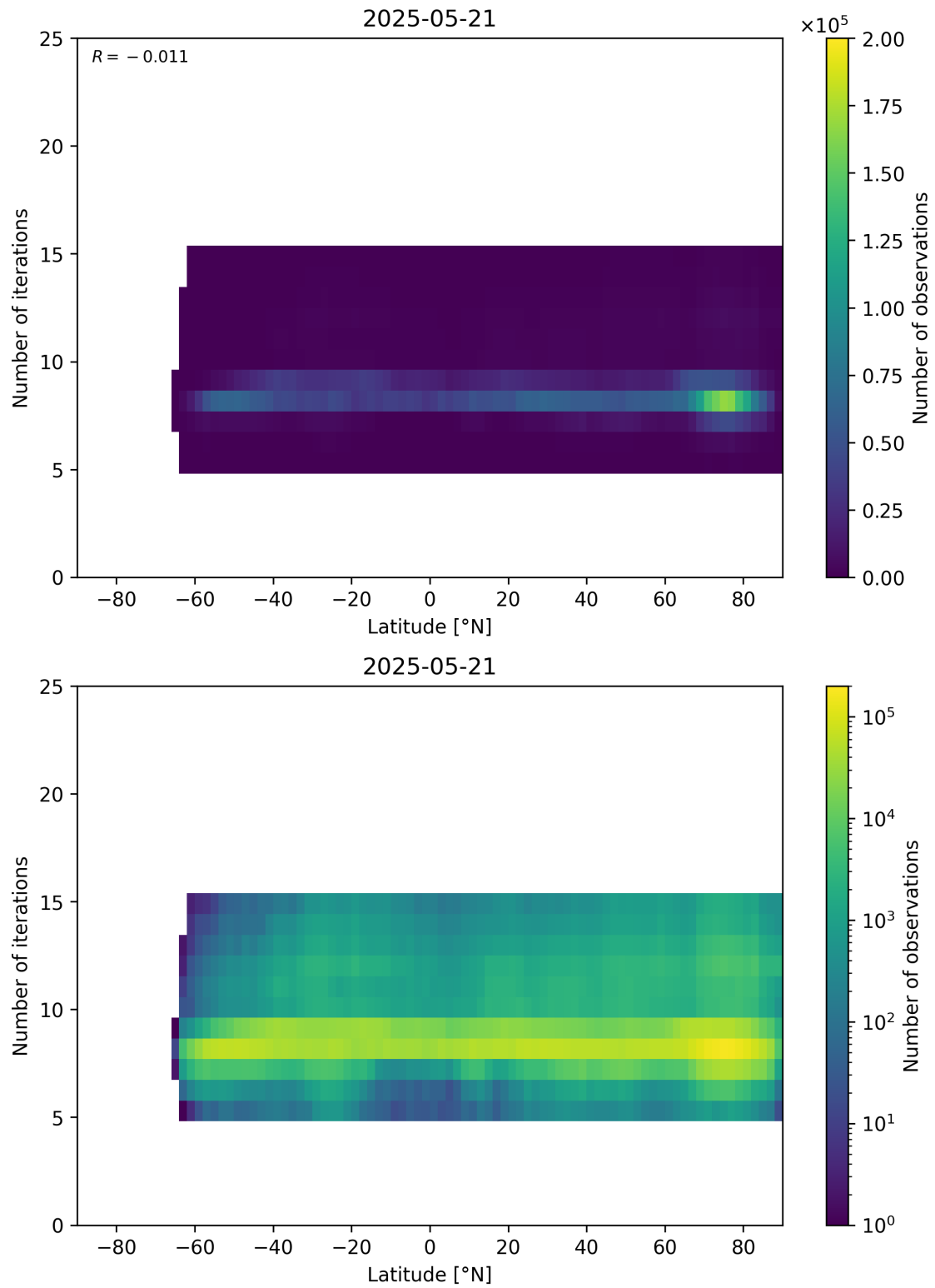
Figure 56: Scatter density plot of “Latitude” against “Number of iterations” for 2025-05-21 to 2025-05-22.
