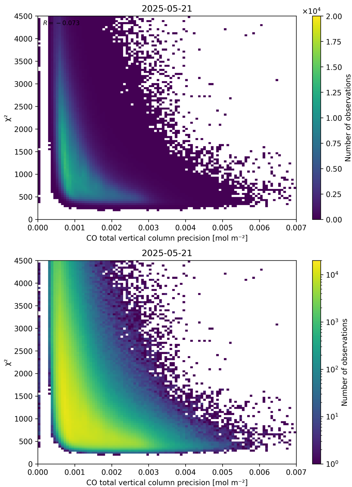
Figure 44: Scatter density plot of “CO total vertical column precision” against “ \chi^2 ” for 2025-05-21 to 2025-05-22.
