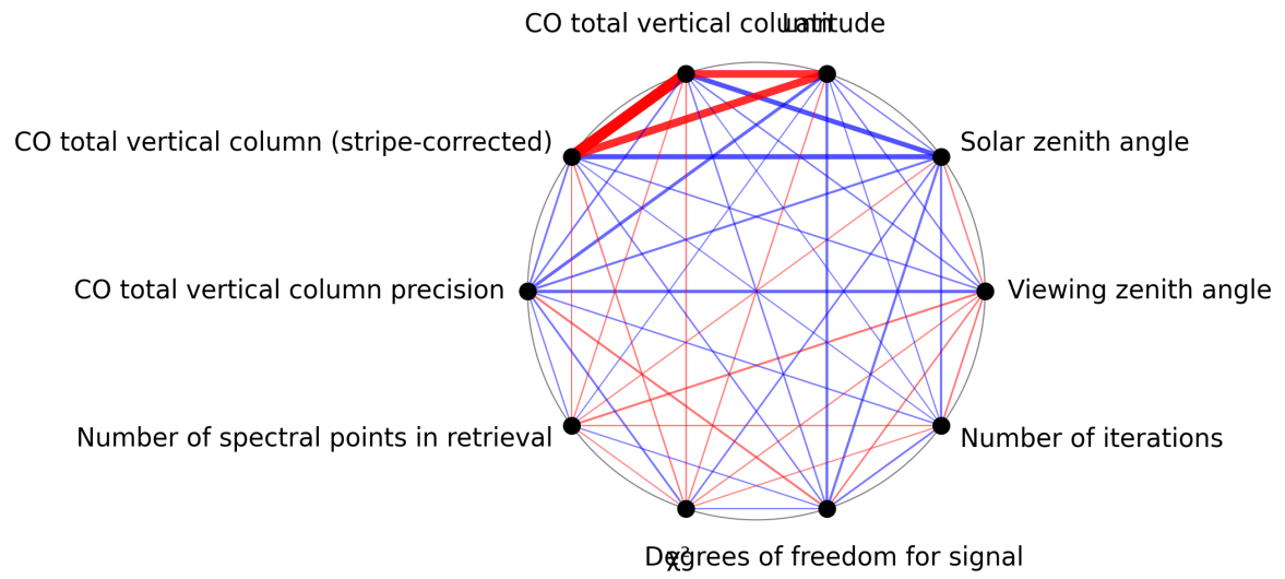
Figure 1: Map of correlation graph for 2025-05-21 to 2025-05-22.
