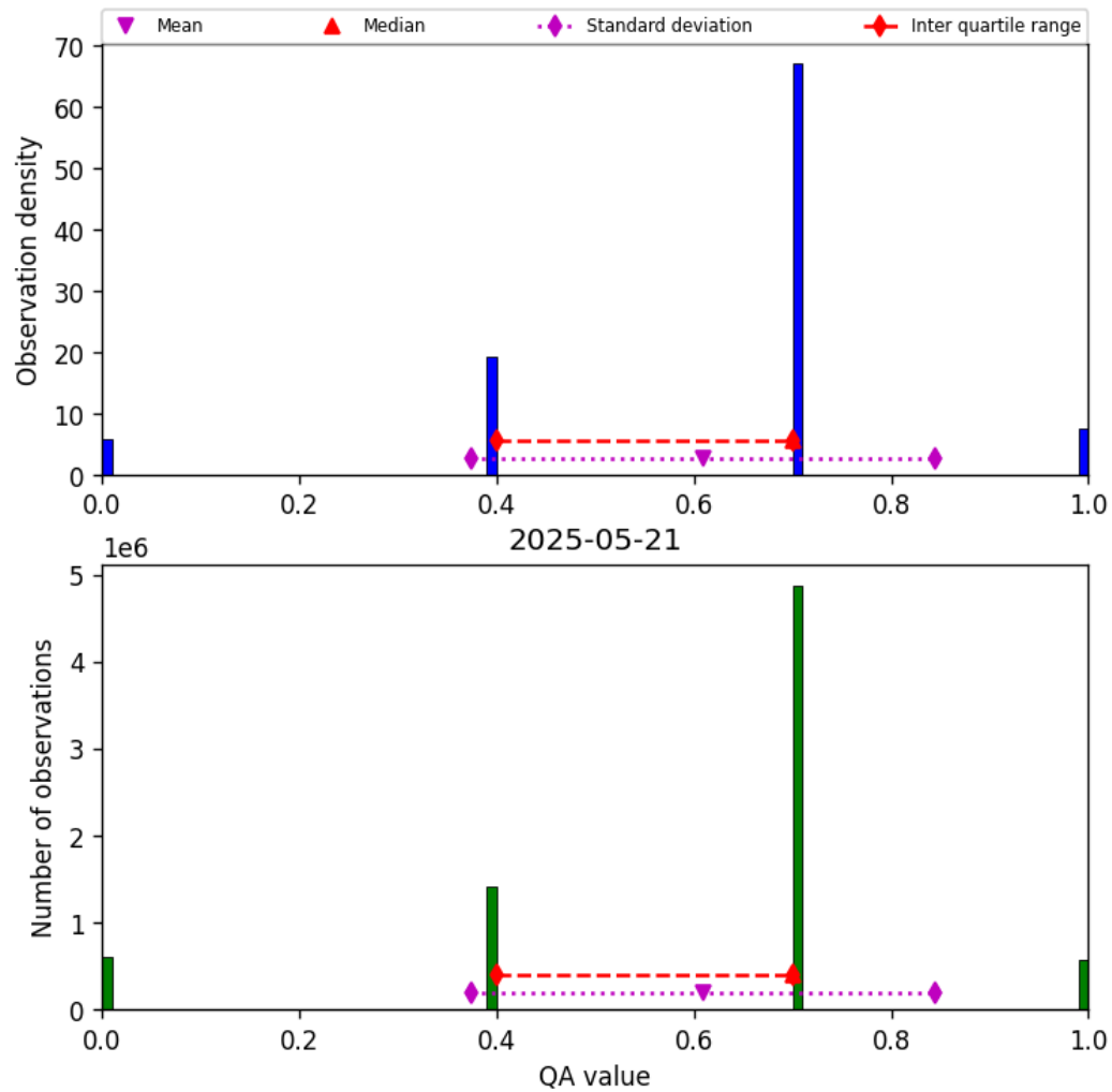
Figure 17: Histogram of “QA value” for 2025-05-21 to 2025-05-22
