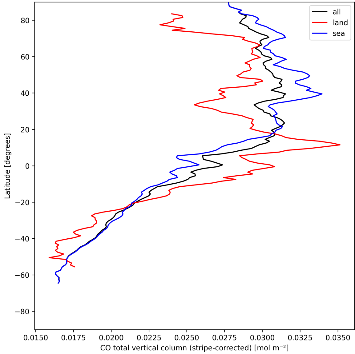
Figure 11: Zonal average of “CO total vertical column (stripe-corrected)” for 2025-05-21 to 2025-05-22.
