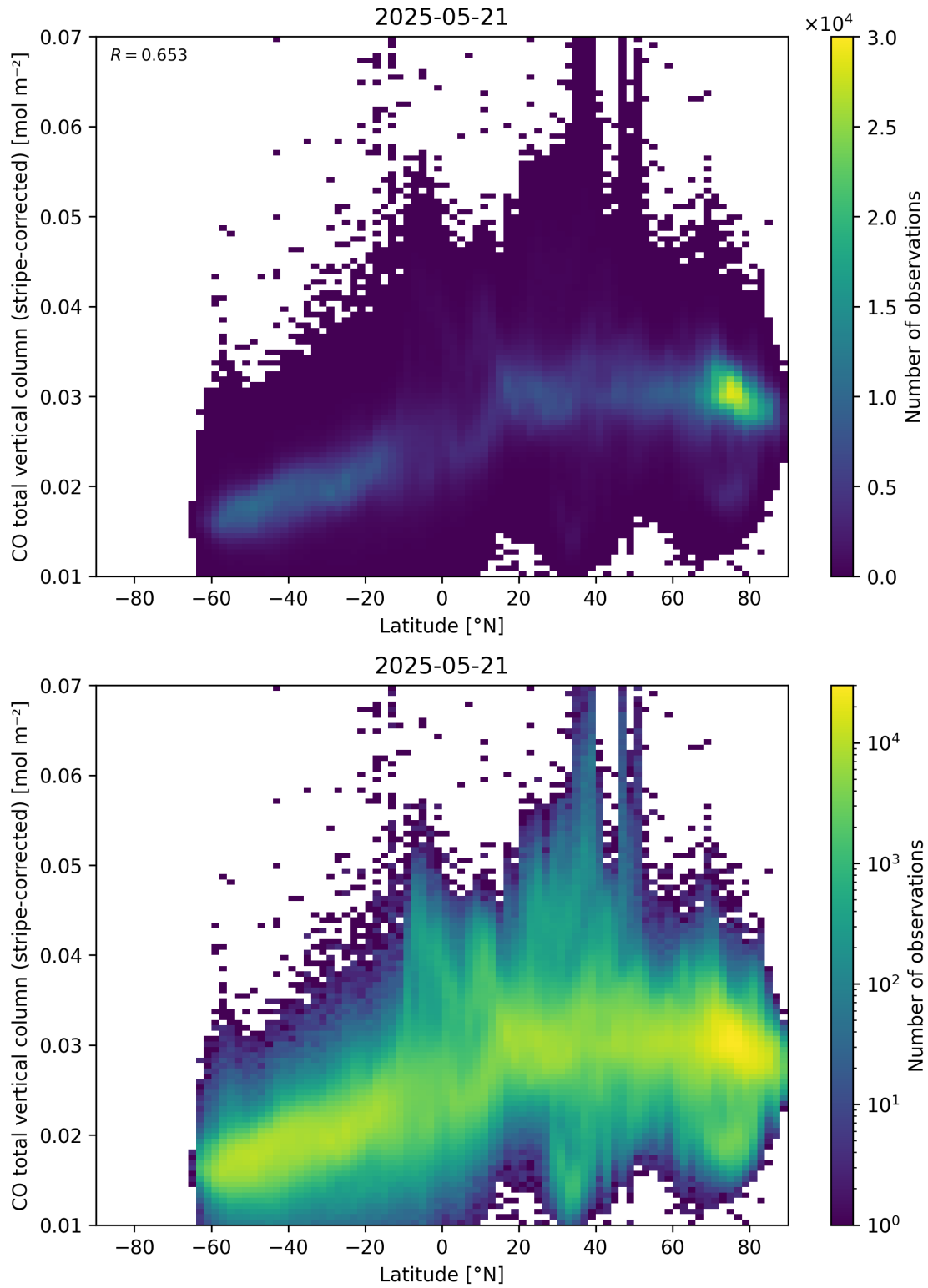
Figure 52: Scatter density plot of “Latitude” against “CO total vertical column (stripe-corrected)” for 2025-05-21 to 2025-05-22.
