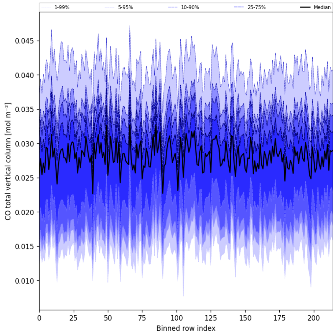
Figure 26: Along track statistics of "CO total vertical column" for 2025-05-21 to 2025-05-22
