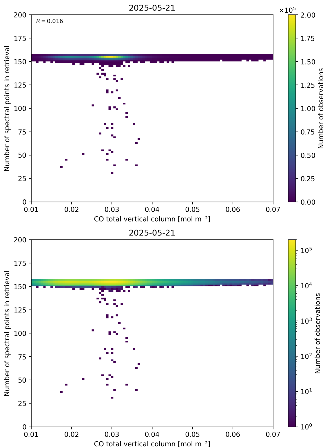
Figure 43: Scatter density plot of “CO total vertical column” against “Number of spectral points in retrieval” for 2025-05-21 to 2025-05-22.
