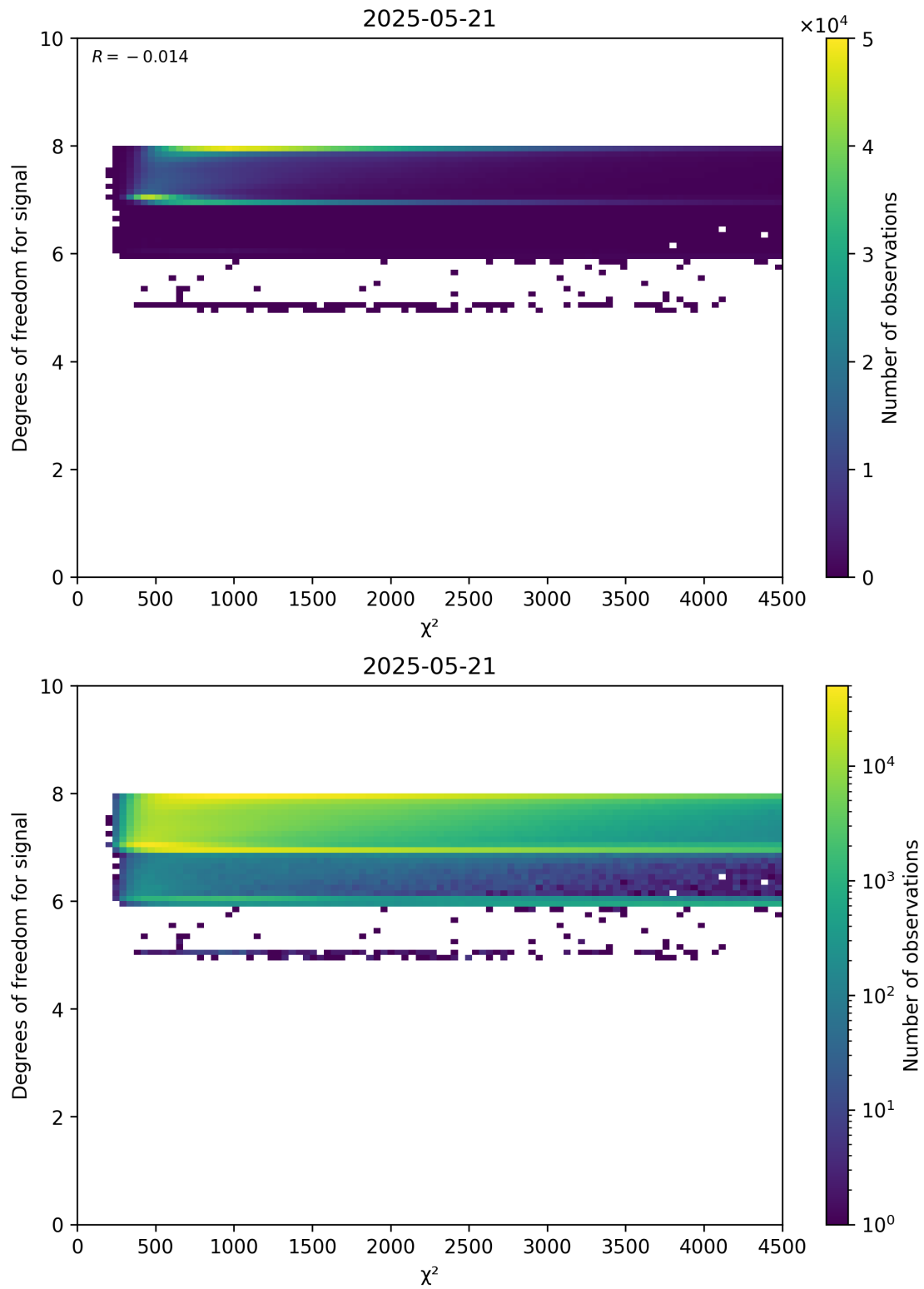
Figure 48: Scatter density plot of “ \chi^2 ” against “Degrees of freedom for signal” for 2025-05-21 to 2025-05-22.
