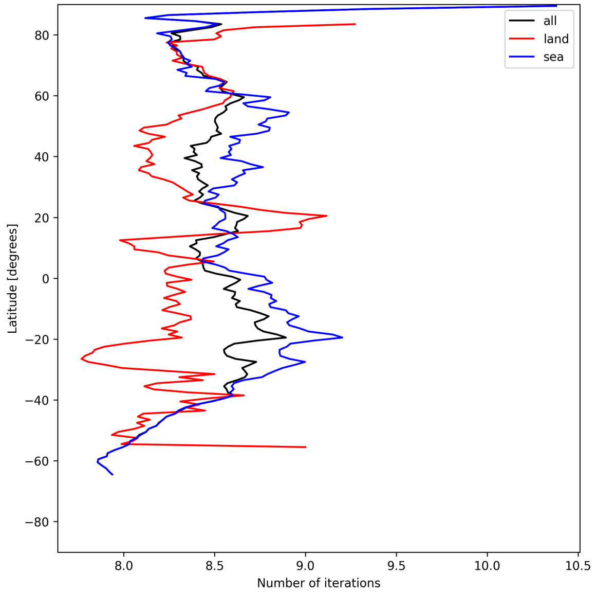
Figure 16: Zonal average of “Number of iterations” for 2025-05-21 to 2025-05-22.
