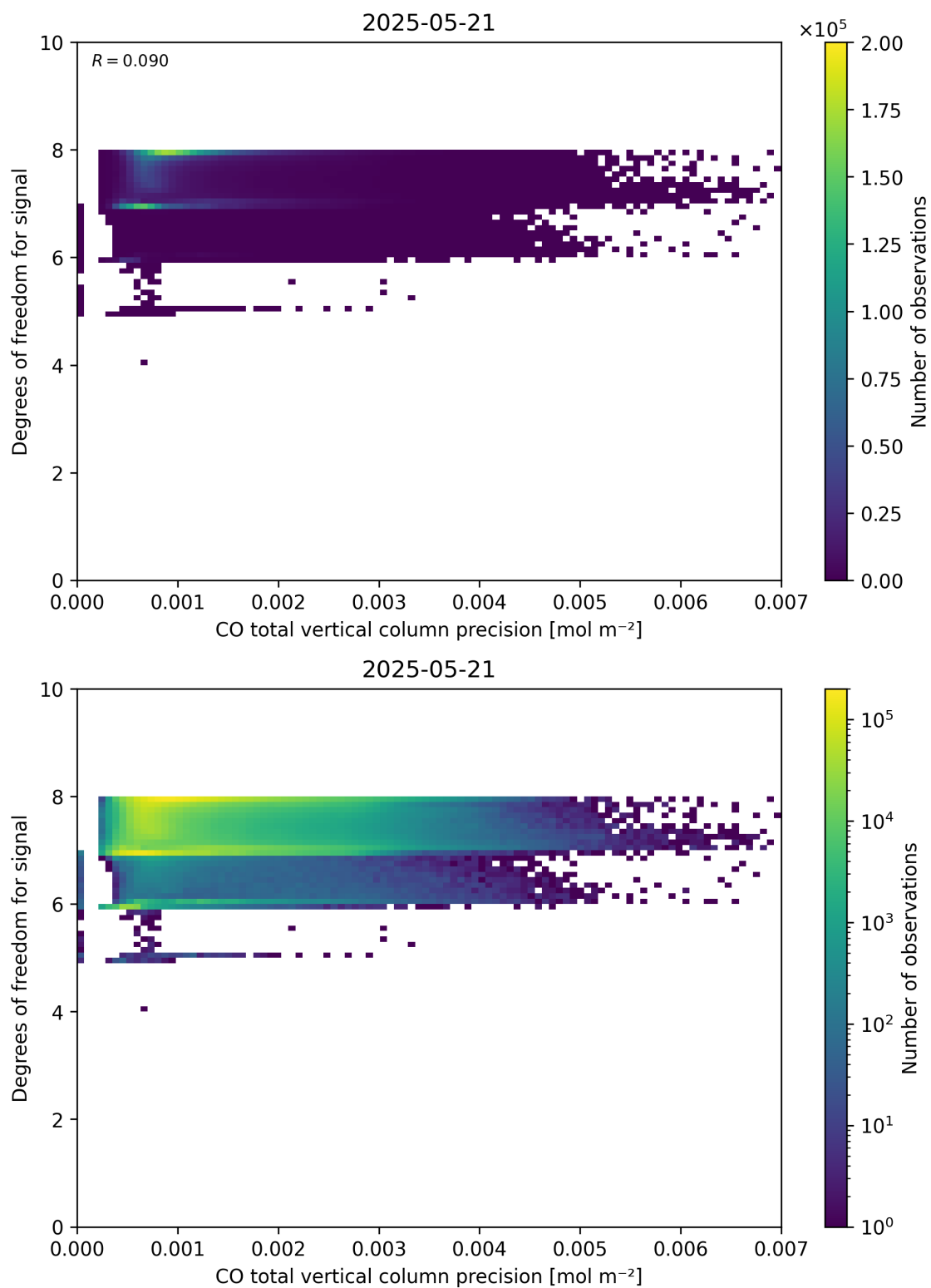
Figure 45: Scatter density plot of “CO total vertical column precision” against “Degrees of freedom for signal” for 2025-05-21 to 2025-05-22.
