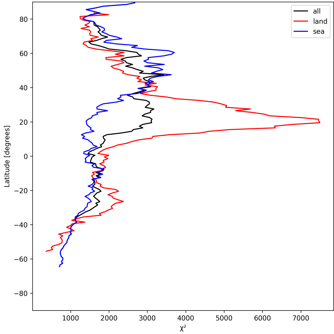
Figure 14: Zonal average of “ \chi^2 ” for 2025-05-21 to 2025-05-22.
