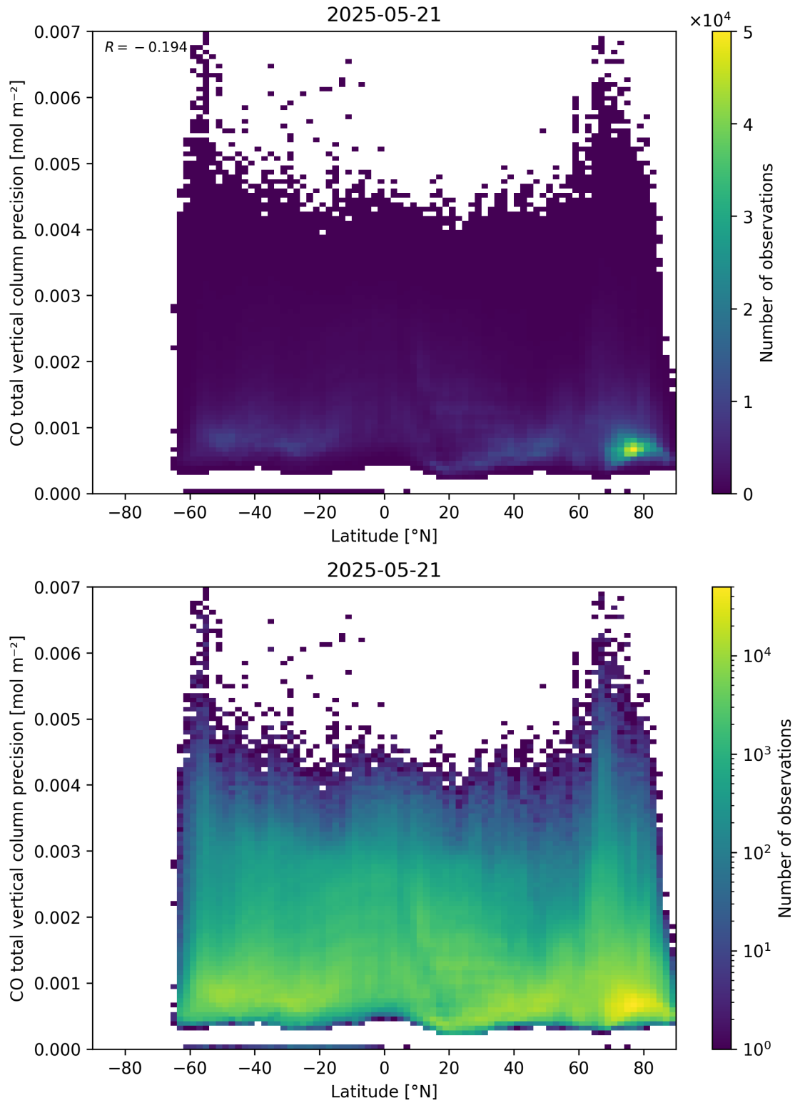
Figure 53: Scatter density plot of “Latitude” against “CO total vertical column precision” for 2025-05-21 to 2025-05-22.
