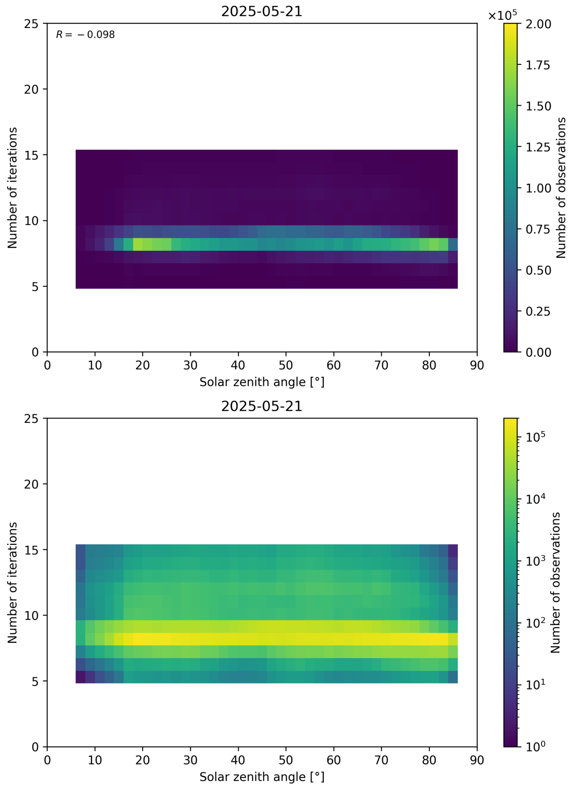
Figure 67: Scatter density plot of “Solar zenith angle” against “Number of iterations” for 2025-05-21 to 2025-05-22.
