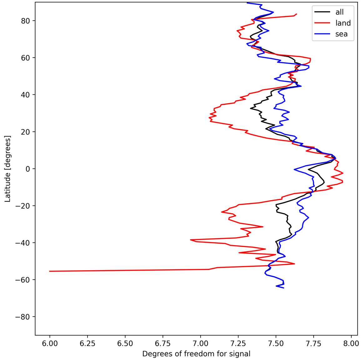
Figure 15: Zonal average of “Degrees of freedom for signal” for 2025-05-21 to 2025-05-22.
