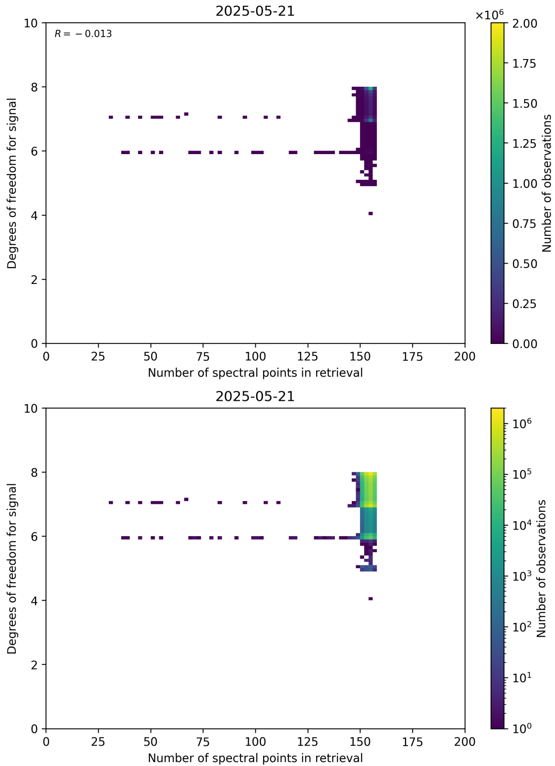
Figure 59: Scatter density plot of “Number of spectral points in retrieval” against “Degrees of freedom for signal” for 2025-05-21 to 2025-05-22.
