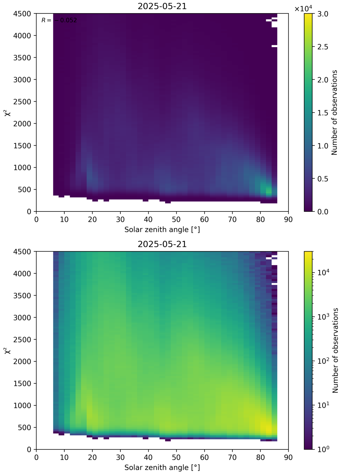
Figure 64: Scatter density plot of “Solar zenith angle” against “ \chi^2 ” for 2025-05-21 to 2025-05-22.
