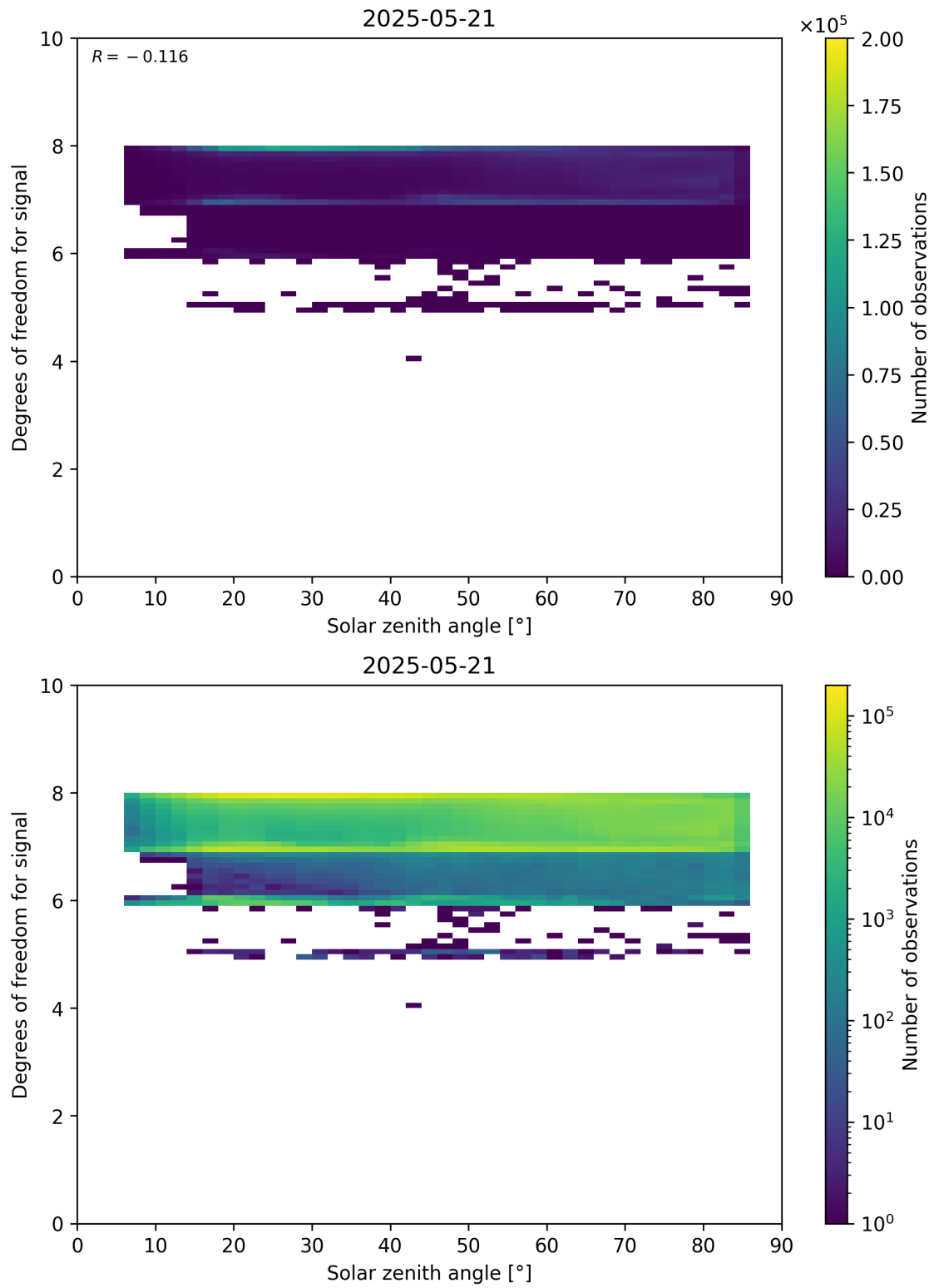
Figure 65: Scatter density plot of “Solar zenith angle” against “Degrees of freedom for signal” for 2025-05-21 to 2025-05-22.
