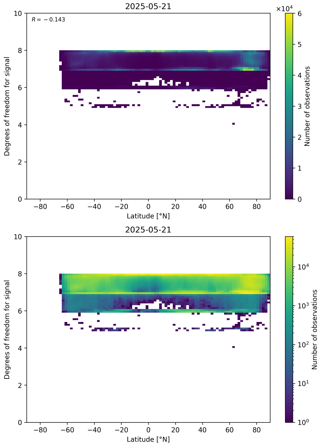
Figure 55: Scatter density plot of “Latitude” against “Degrees of freedom for signal” for 2025-05-21 to 2025-05-22.
