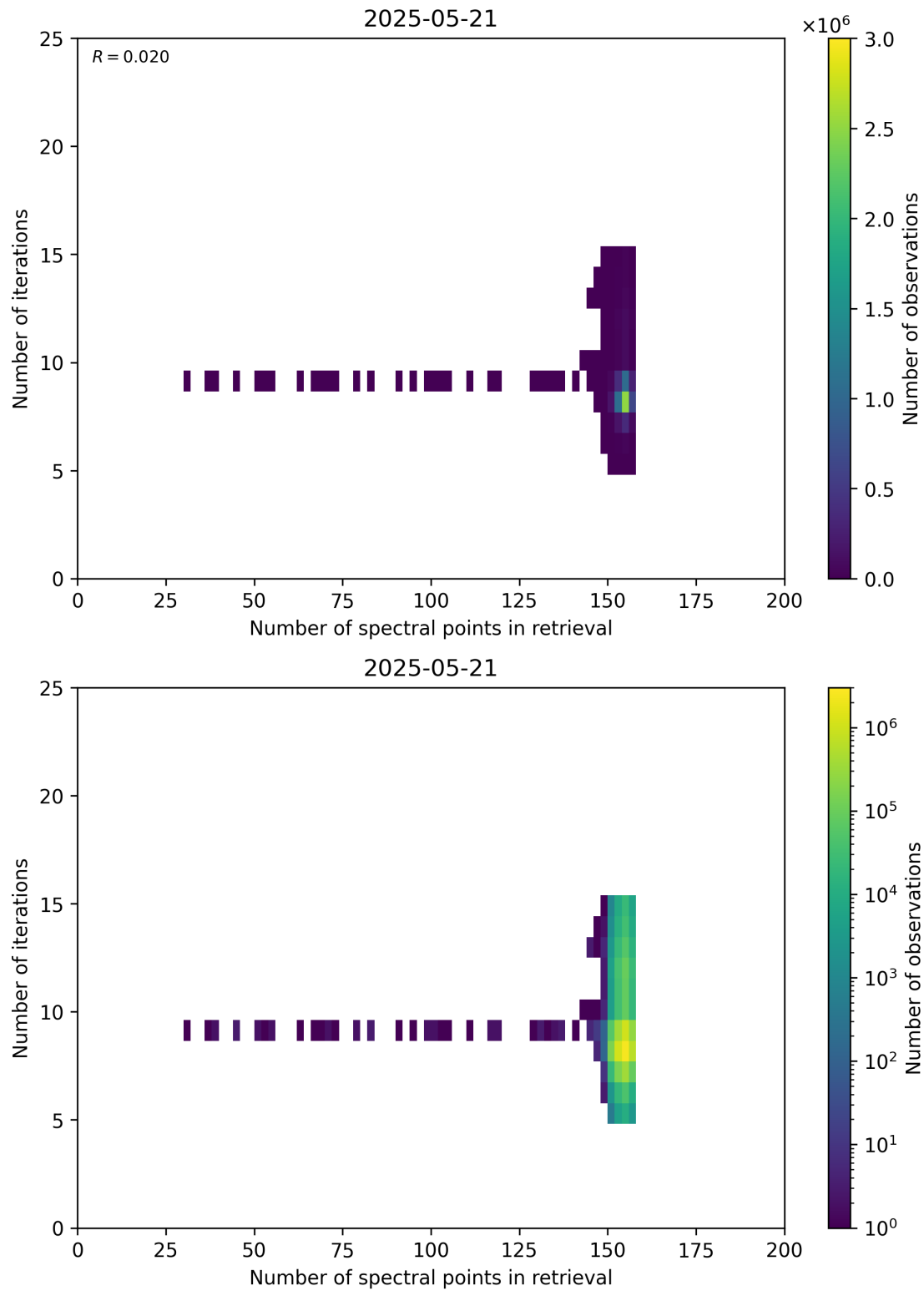
Figure 60: Scatter density plot of “Number of spectral points in retrieval” against “Number of iterations” for 2025-05-21 to 2025-05-22.
