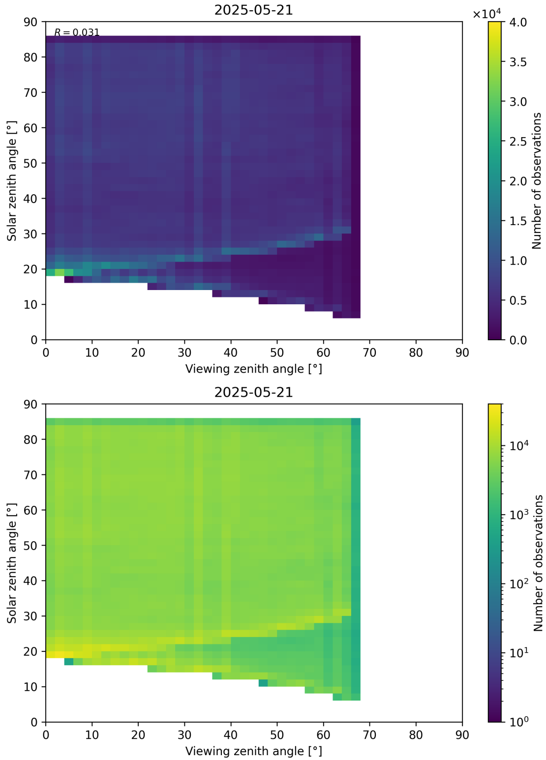
Figure 77: Scatter density plot of “Viewing zenith angle” against “Solar zenith angle” for 2025-05-21 to 2025-05-22.
