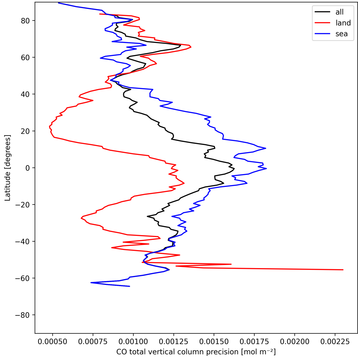
Figure 12: Zonal average of “CO total vertical column precision” for 2025-05-21 to 2025-05-22.
