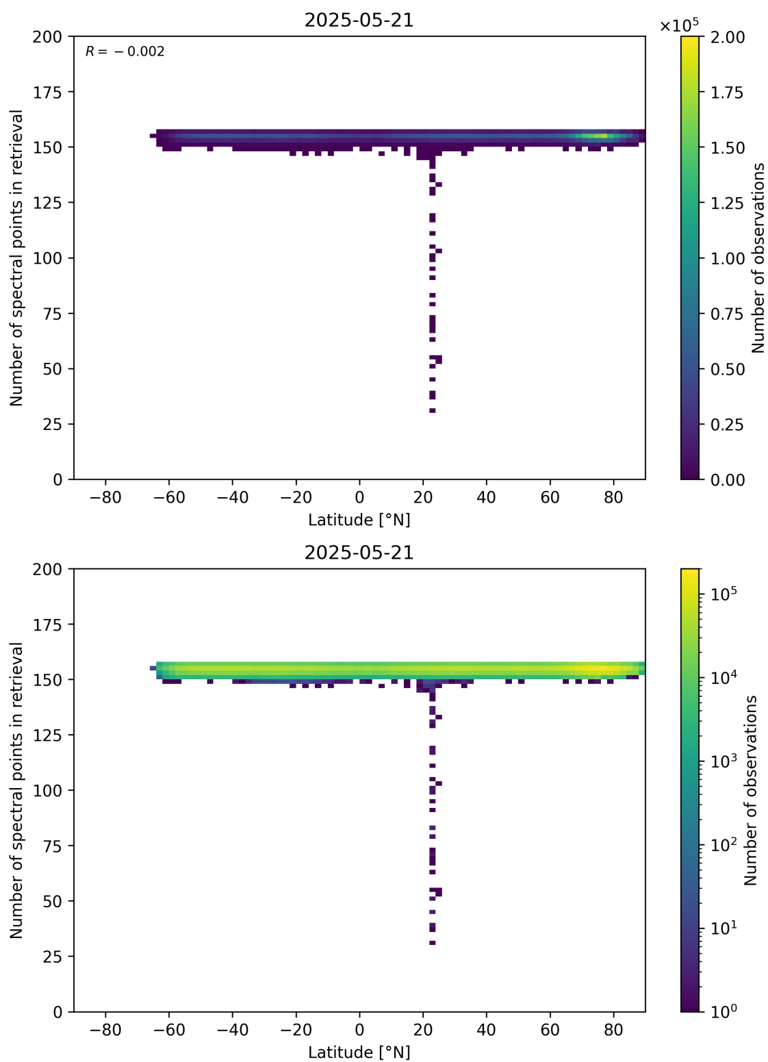
Figure 57: Scatter density plot of “Latitude” against “Number of spectral points in retrieval” for 2025-05-21 to 2025-05-22.
