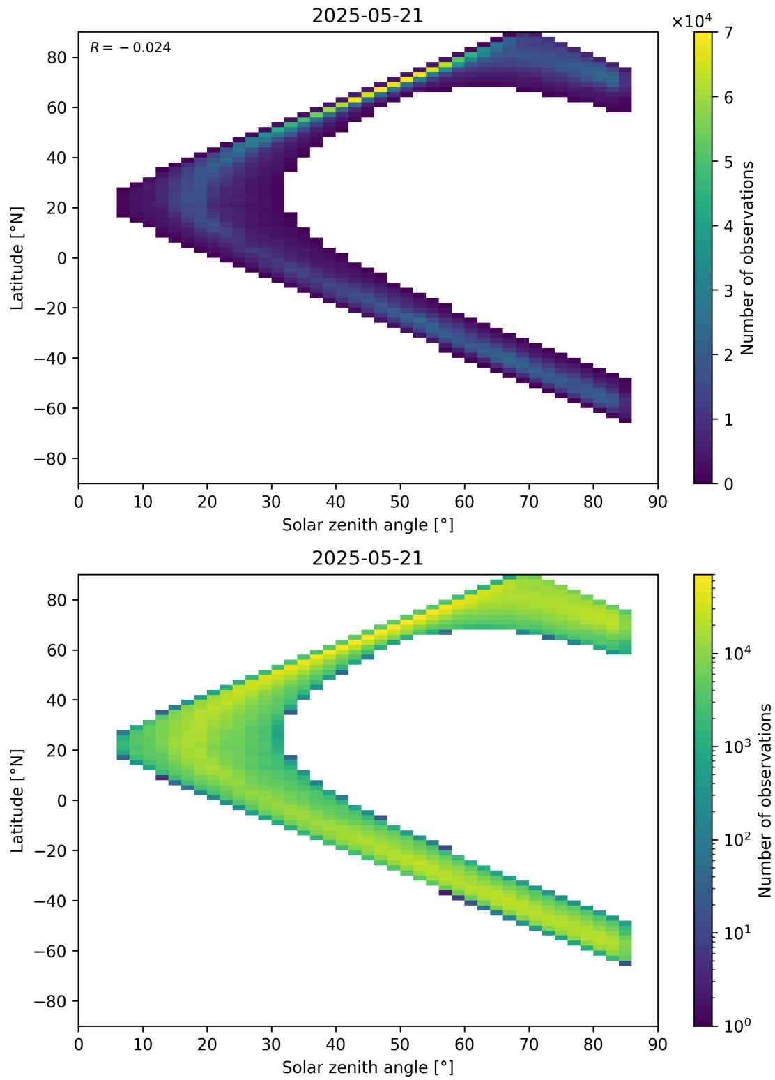
Figure 66: Scatter density plot of “Solar zenith angle” against “Latitude” for 2025-05-21 to 2025-05-22.
