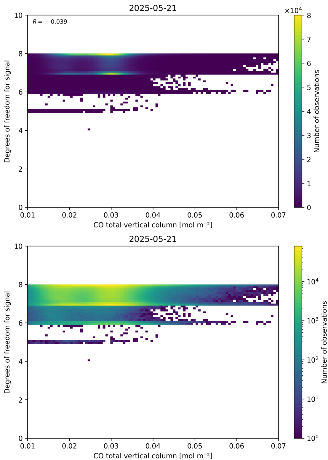
Figure 41: Scatter density plot of “CO total vertical column” against “Degrees of freedom for signal” for 2025-05-21 to 2025-05-22.
