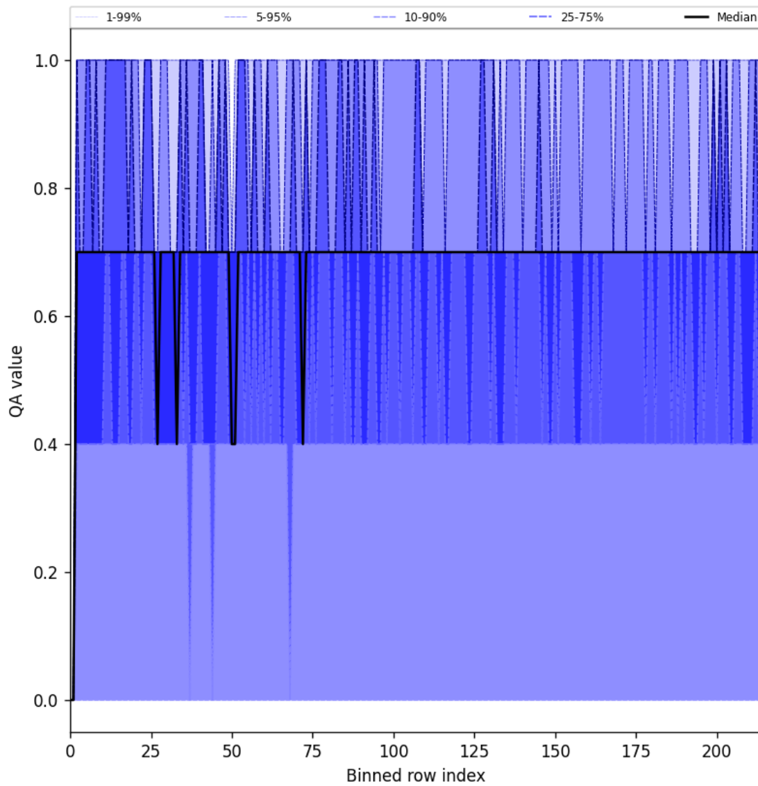
Figure 25: Along track statistics of “QA value” for 2025-05-21 to 2025-05-22
