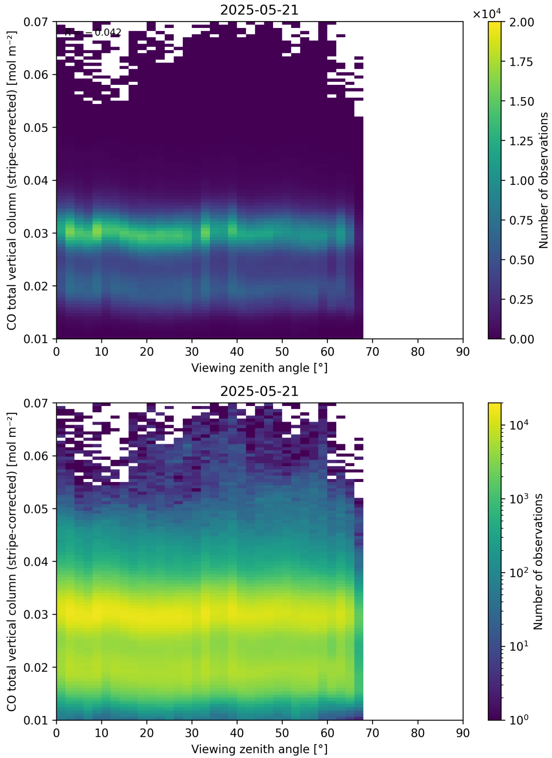
Figure 70: Scatter density plot of “Viewing zenith angle” against “CO total vertical column (stripe-corrected)” for 2025-05-21 to 2025-05-22.
