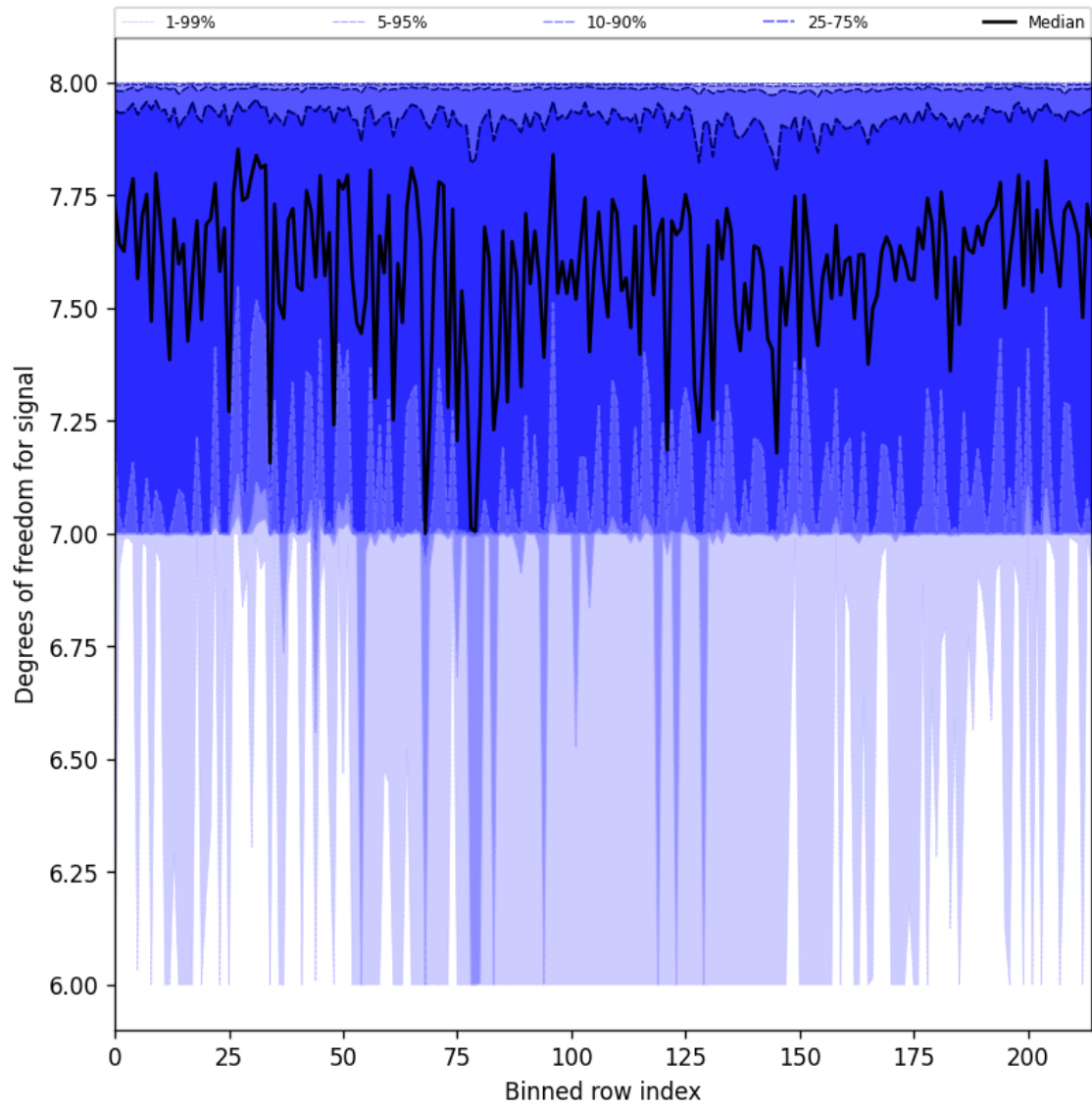
Figure 31: Along track statistics of “Degrees of freedom for signal” for 2025-05-21 to 2025-05-22
