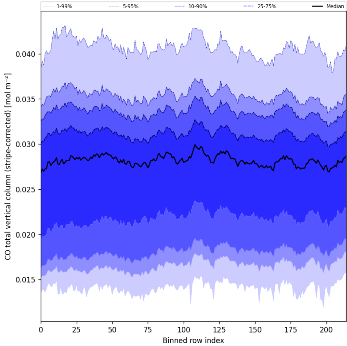
Figure 27: Along track statistics of “CO total vertical column (stripe-corrected)” for 2025-05-21 to 2025-05-22
