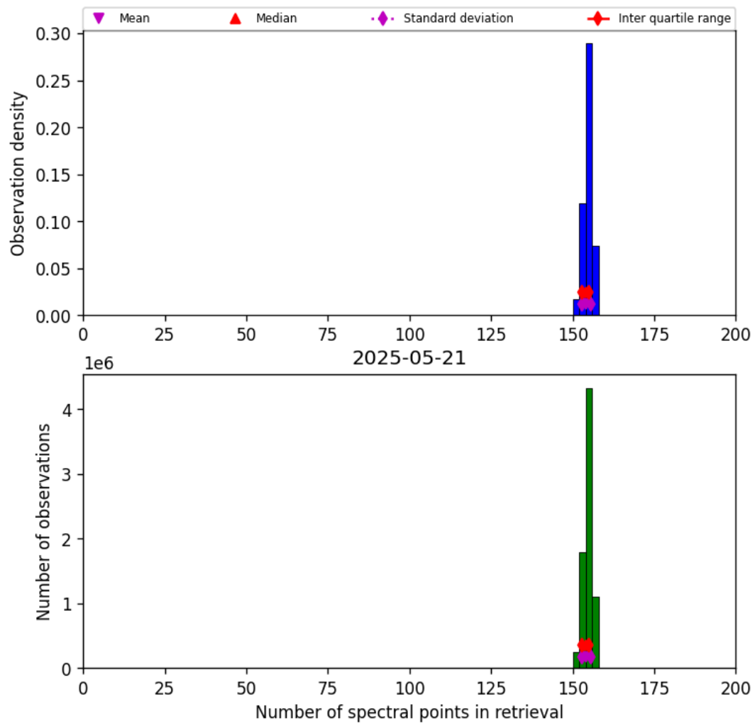
Figure 21: Histogram of “Number of spectral points in retrieval” for 2025-05-21 to 2025-05-22
