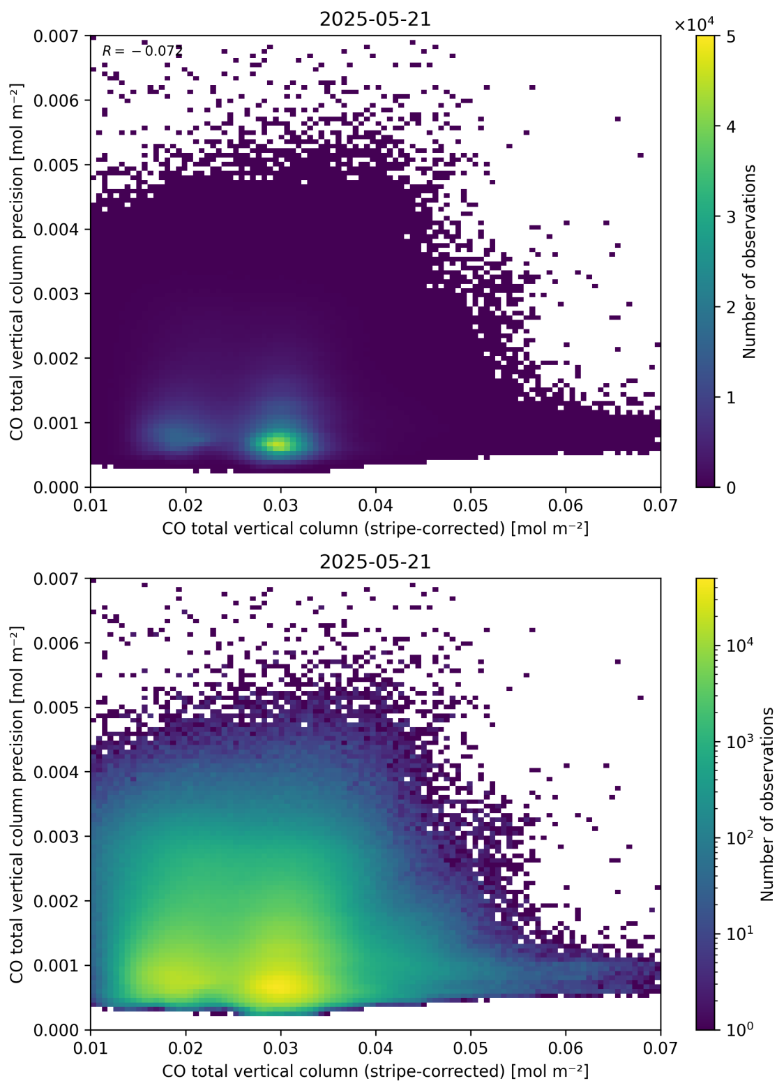
Figure 36: Scatter density plot of “CO total vertical column (stripe-corrected)” against “CO total vertical column precision” for 2025-05-21 to 2025-05-22.
