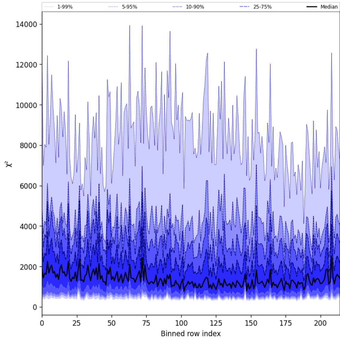
Figure 30: Along track statistics of “ \chi^2 ” for 2025-05-21 to 2025-05-22
