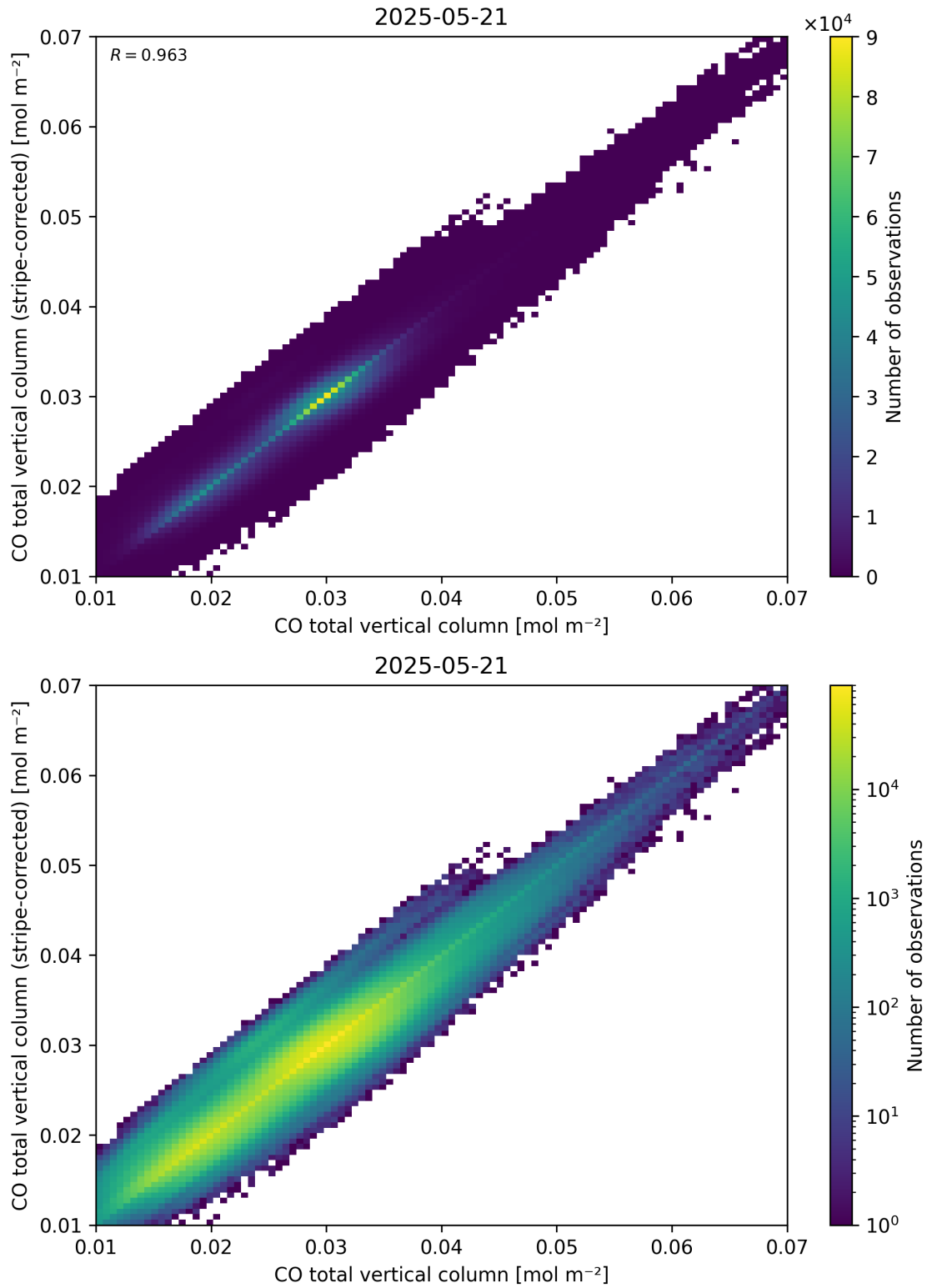
Figure 33: Scatter density plot of “CO total vertical column” against “CO total vertical column (stripe-corrected)” for 2025-05-21 to 2025-05-22.
