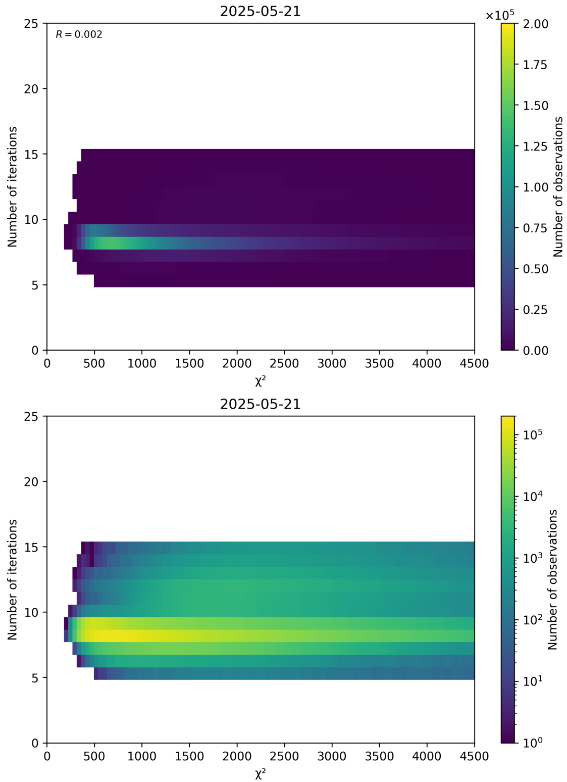
Figure 49: Scatter density plot of “ \chi^2 ” against “Number of iterations” for 2025-05-21 to 2025-05-22.
