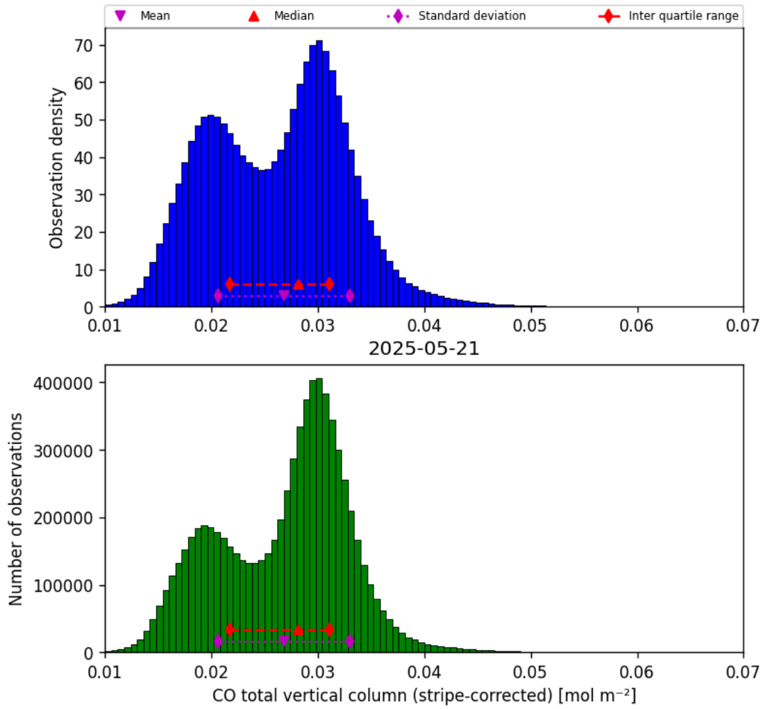
Figure 19: Histogram of “CO total vertical column (stripe-corrected)” for 2025-05-21 to 2025-05-22
