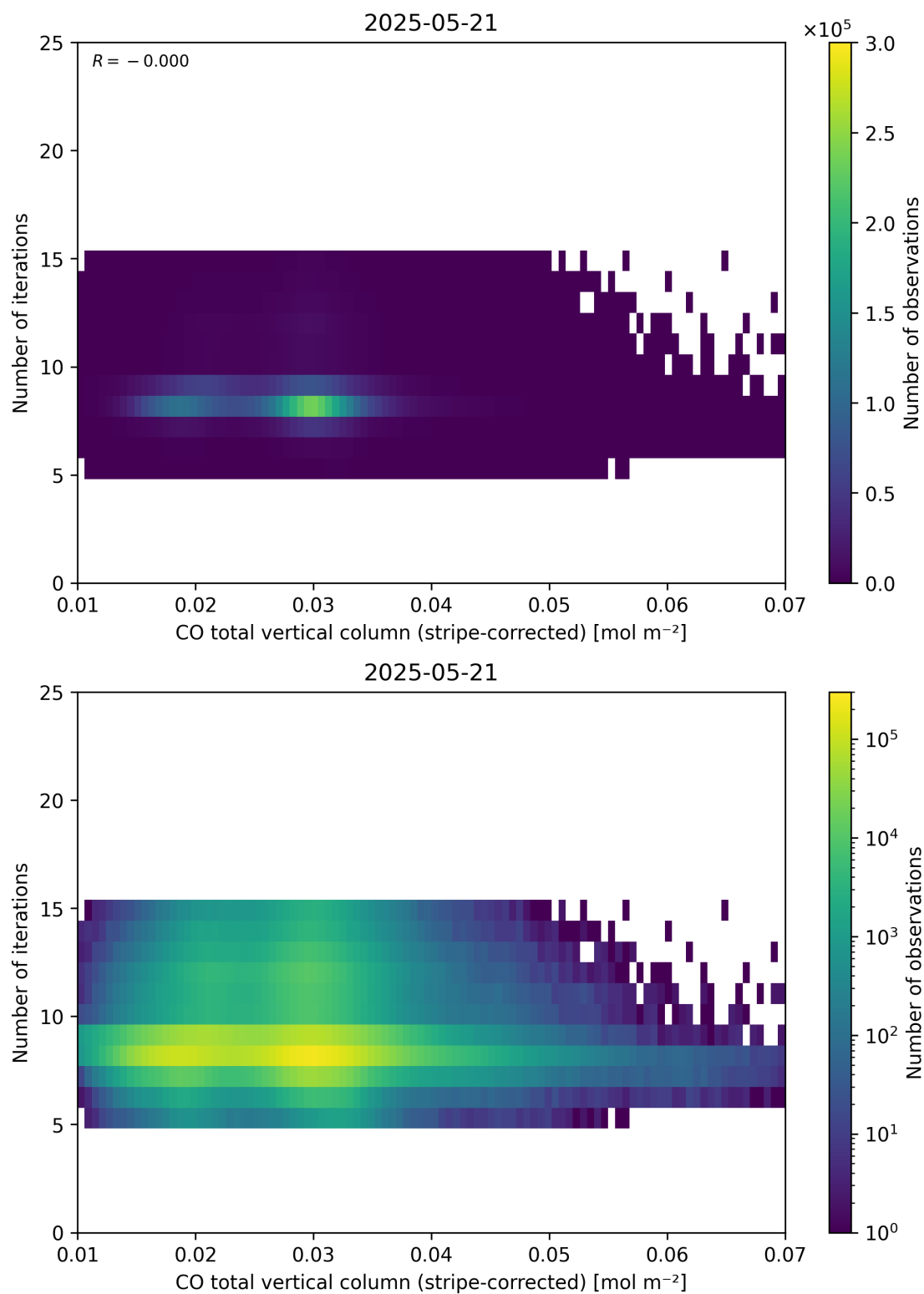
Figure 39: Scatter density plot of “CO total vertical column (stripe-corrected)” against “Number of iterations” for 2025-05-21 to 2025-05-22.
