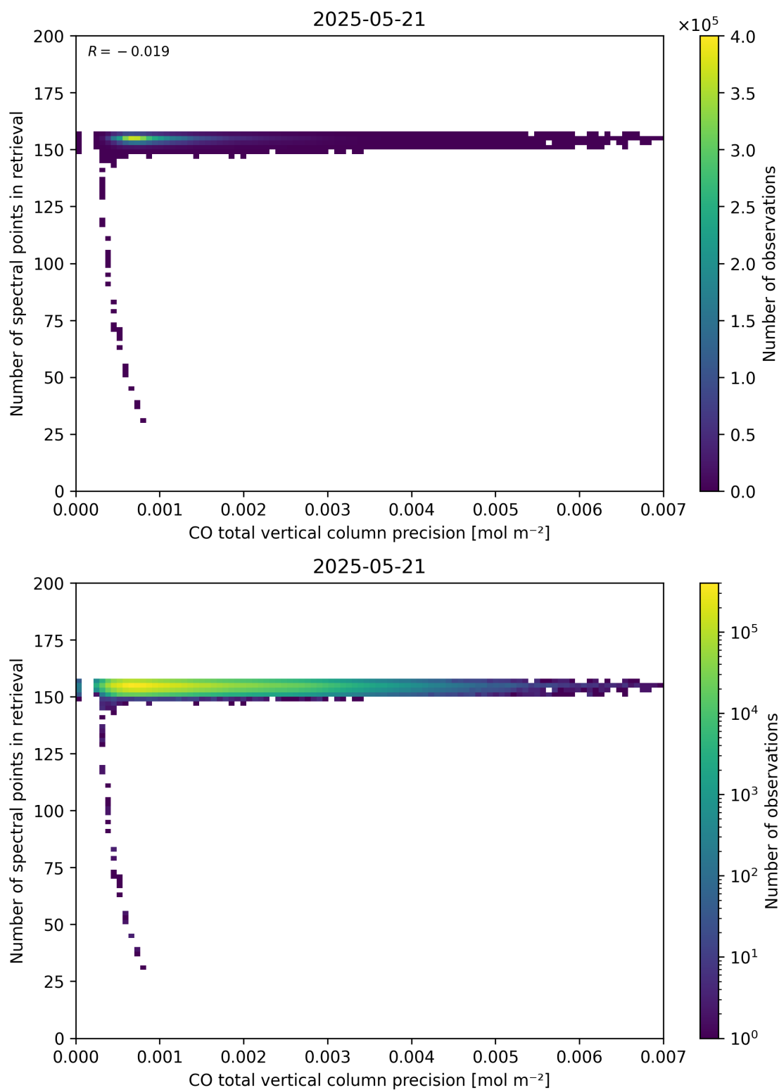
Figure 47: Scatter density plot of “CO total vertical column precision” against “Number of spectral points in retrieval” for 2025-05-21 to 2025-05-22.
