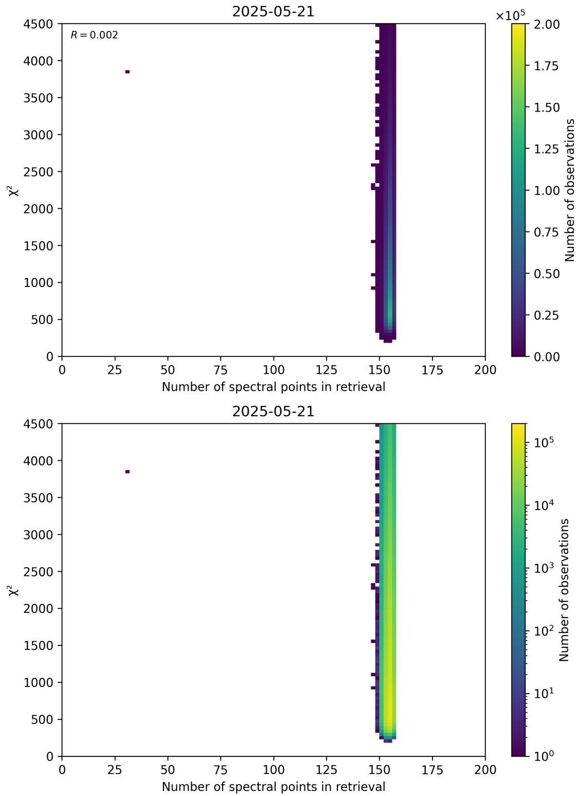
Figure 58: Scatter density plot of “Number of spectral points in retrieval” against “ \chi^2 ” for 2025-05-21 to 2025-05-22.
