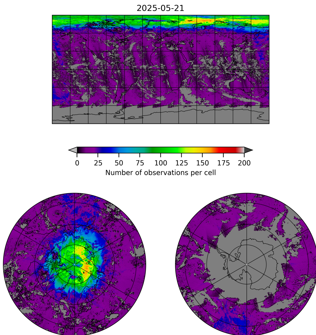
Figure 8: Map of the number of observations for 2025-05-21 to 2025-05-22
