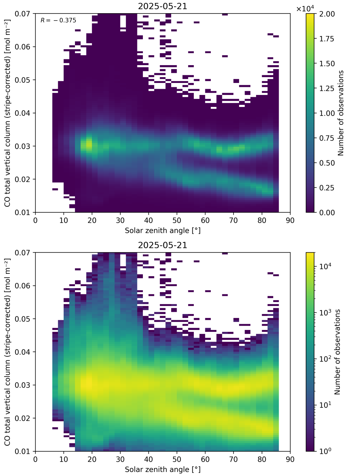
Figure 62: Scatter density plot of “Solar zenith angle” against “CO total vertical column (stripe-corrected)” for 2025-05-21 to 2025-05-22.
