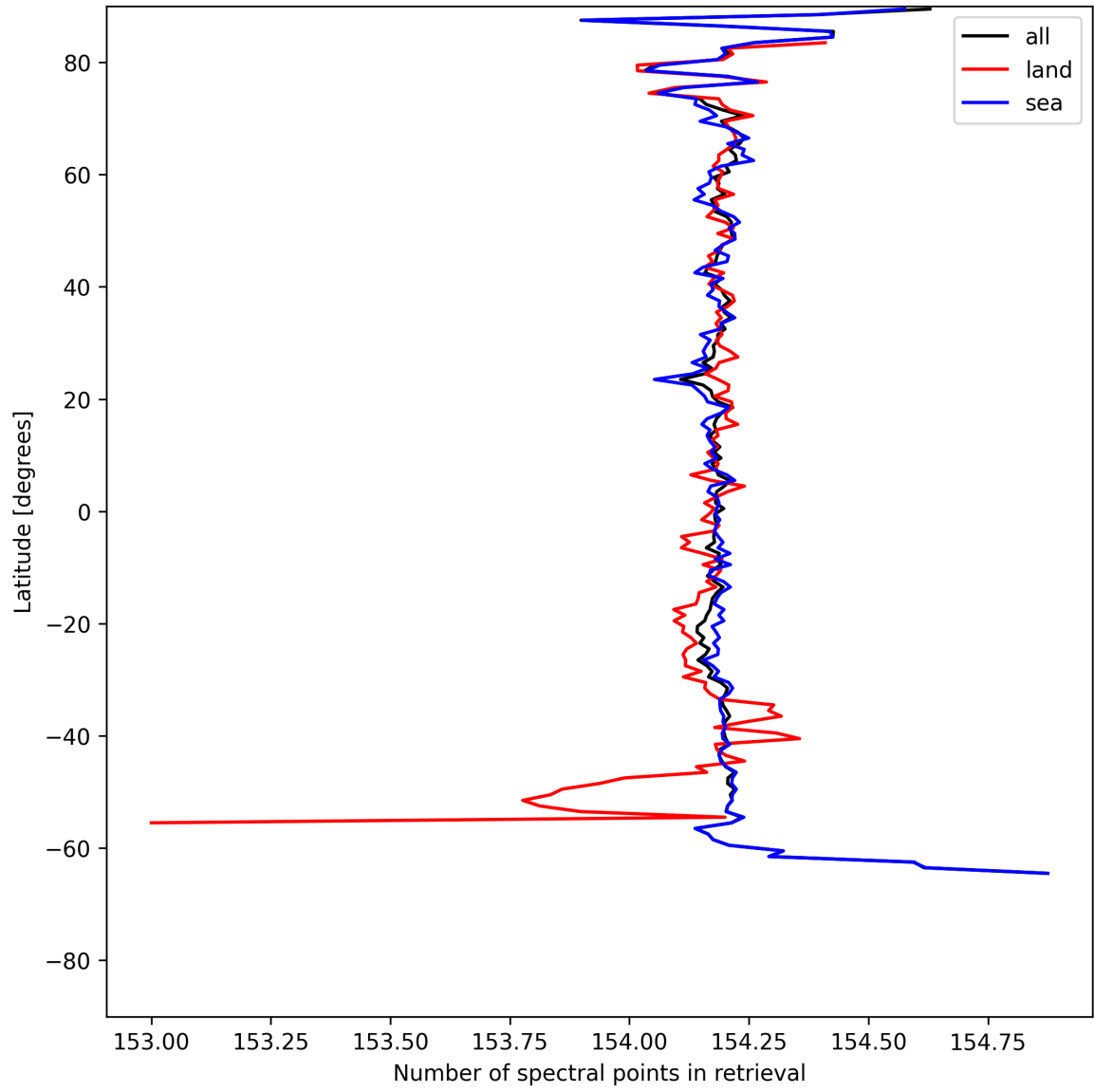
Figure 13: Zonal average of “Number of spectral points in retrieval” for 2025-05-21 to 2025-05-22.
