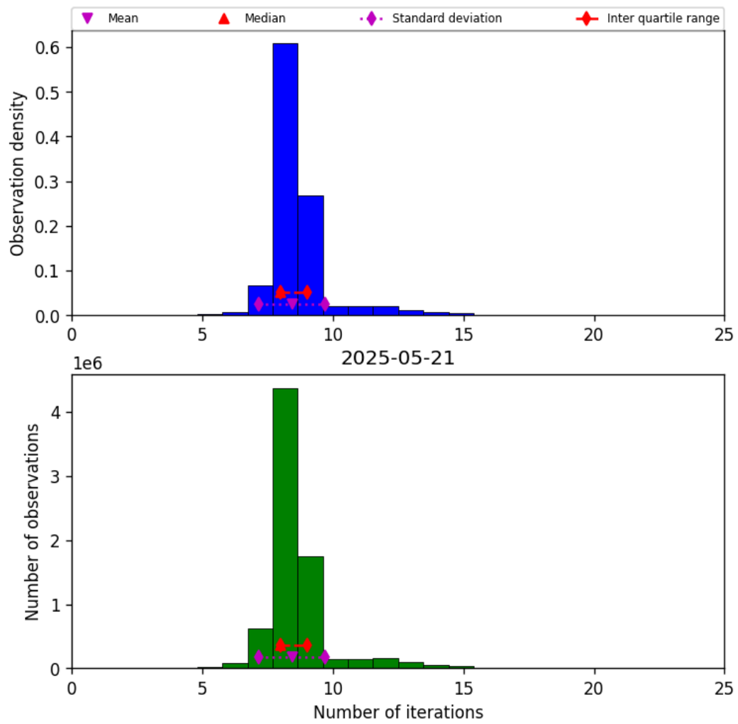
Figure 24: Histogram of “Number of iterations” for 2025-05-21 to 2025-05-22
