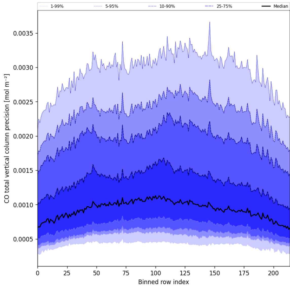
Figure 28: Along track statistics of “CO total vertical column precision” for 2025-05-21 to 2025-05-22
