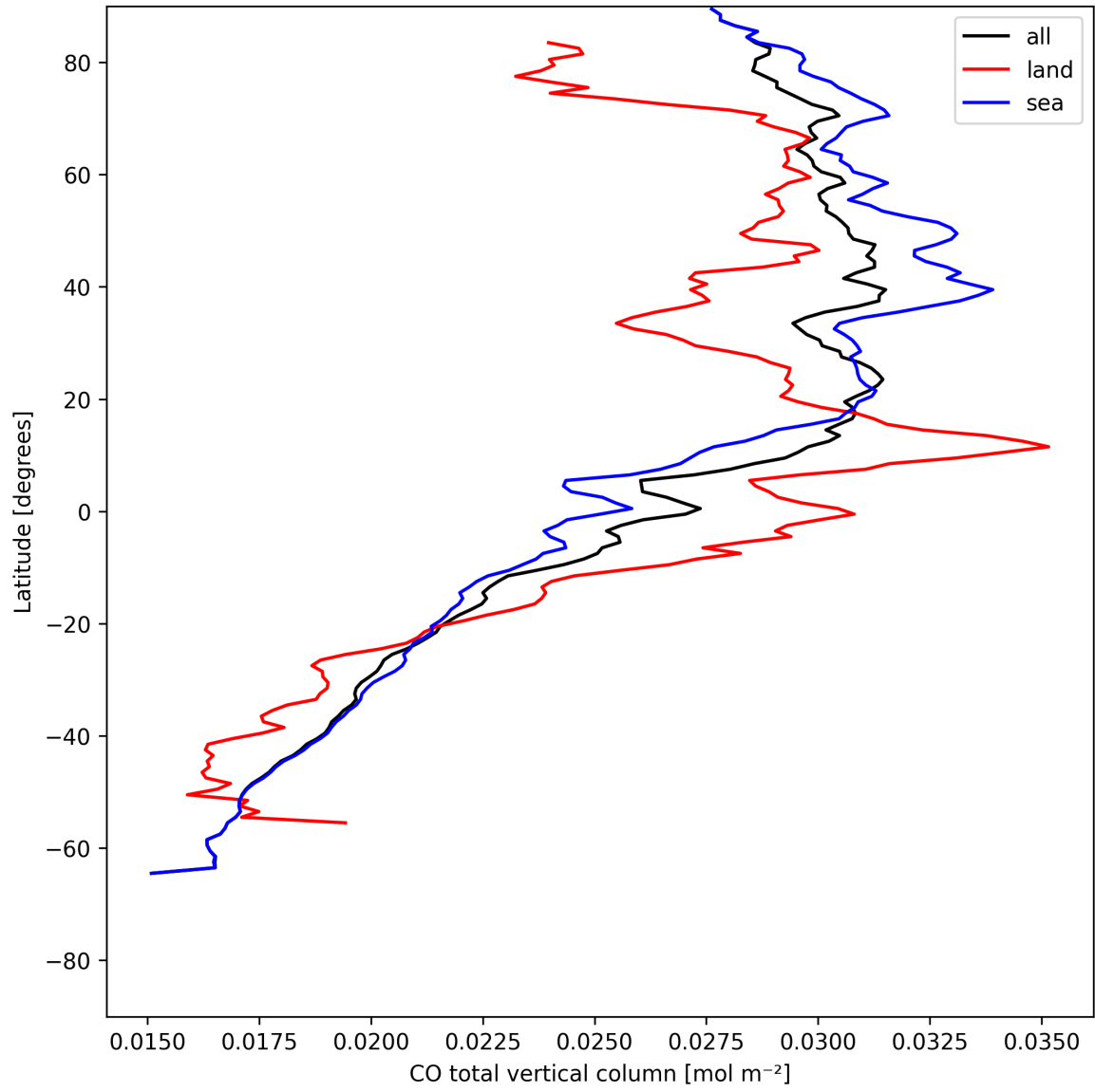
Figure 10: Zonal average of “CO total vertical column” for 2025-05-21 to 2025-05-22.
