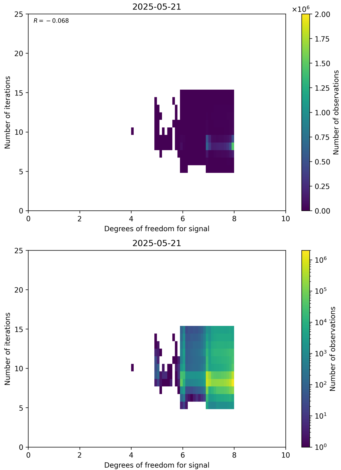
Figure 50: Scatter density plot of “Degrees of freedom for signal” against “Number of iterations” for 2025-05-21 to 2025-05-22.
