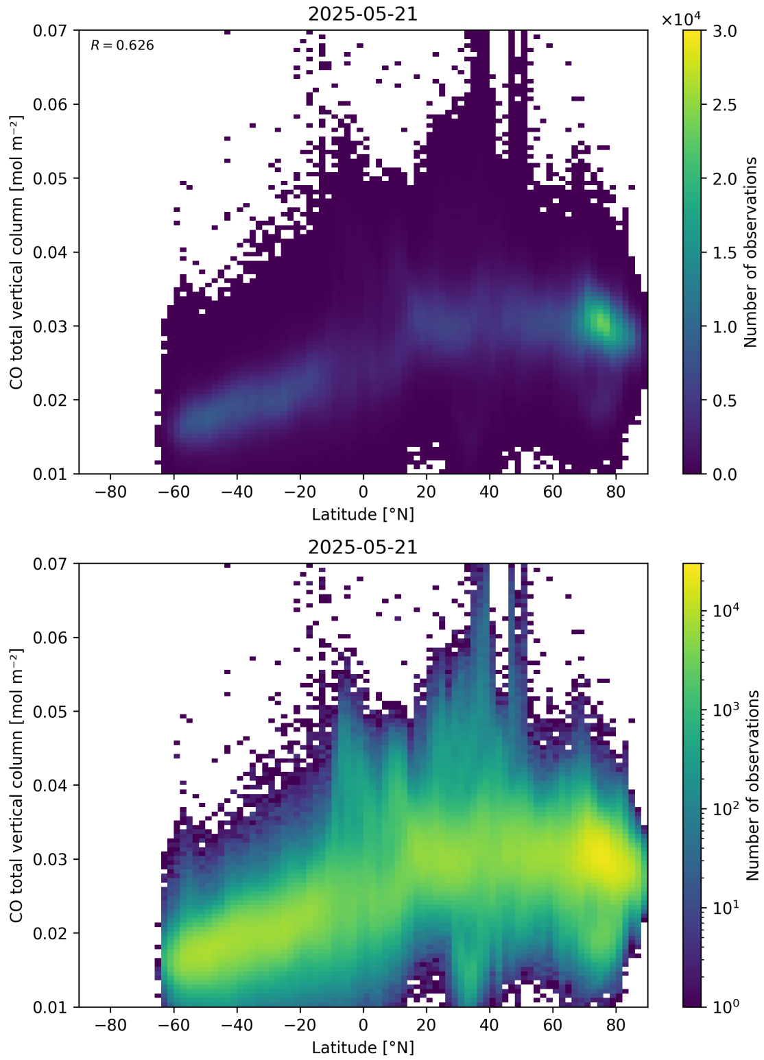
Figure 51: Scatter density plot of “Latitude” against “CO total vertical column” for 2025-05-21 to 2025-05-22.
