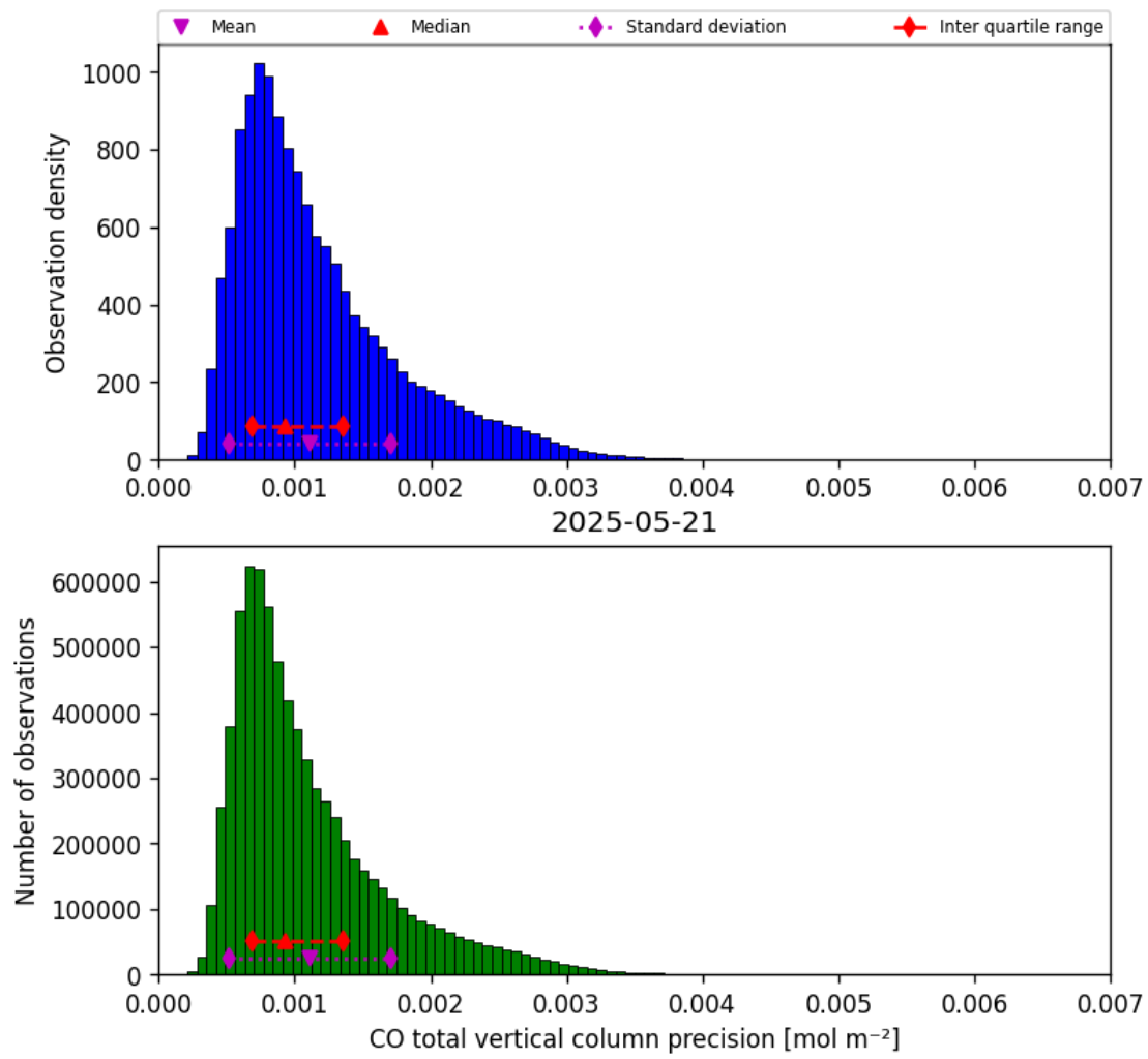
Figure 20: Histogram of “CO total vertical column precision” for 2025-05-21 to 2025-05-22
