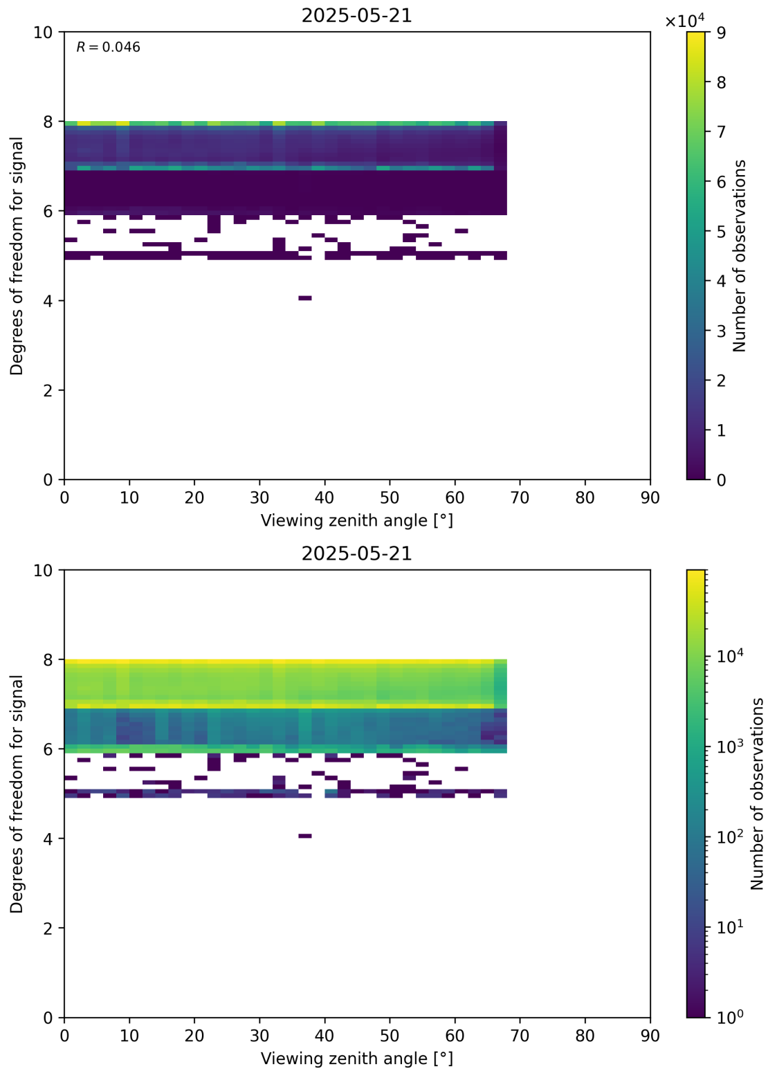
Figure 73: Scatter density plot of “Viewing zenith angle” against “Degrees of freedom for signal” for 2025-05-21 to 2025-05-22.
