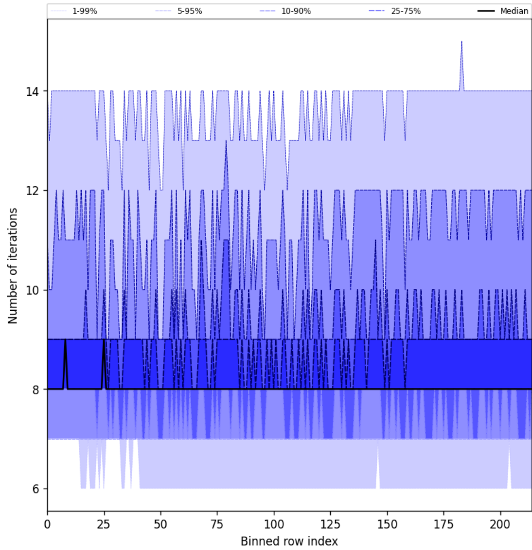
Figure 32: Along track statistics of “Number of iterations” for 2025-05-21 to 2025-05-22
