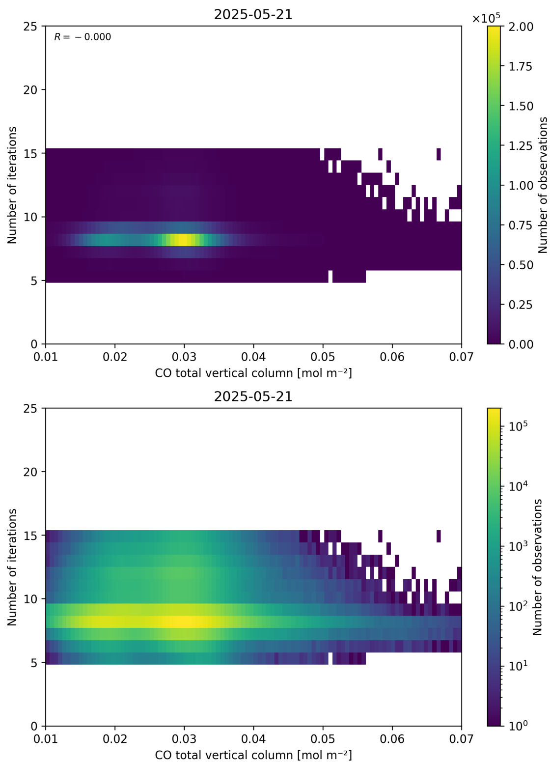
Figure 42: Scatter density plot of “CO total vertical column” against “Number of iterations” for 2025-05-21 to 2025-05-22.
