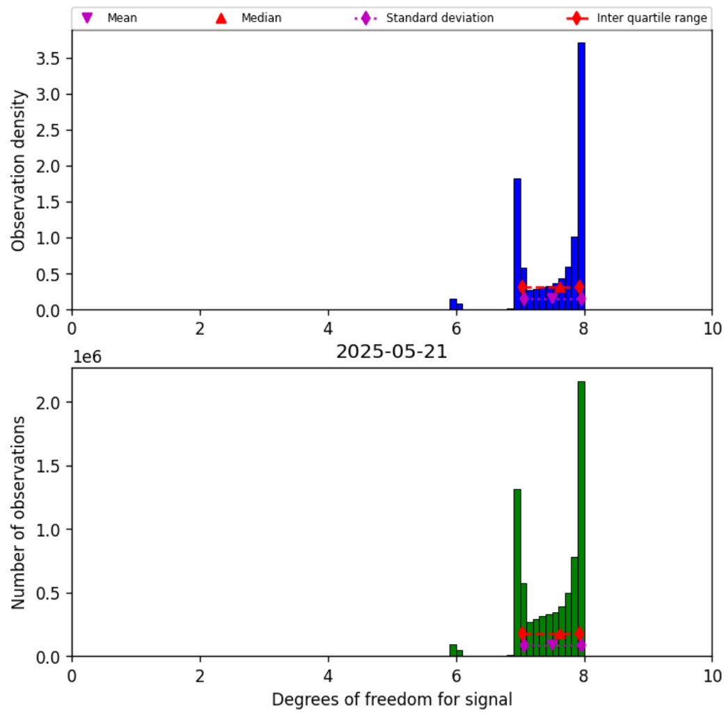
Figure 23: Histogram of “Degrees of freedom for signal” for 2025-05-21 to 2025-05-22
