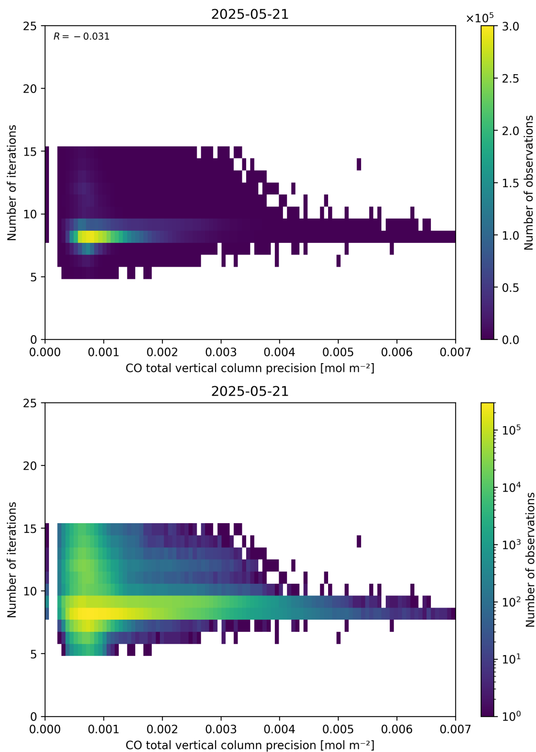
Figure 46: Scatter density plot of “CO total vertical column precision” against “Number of iterations” for 2025-05-21 to 2025-05-22.
