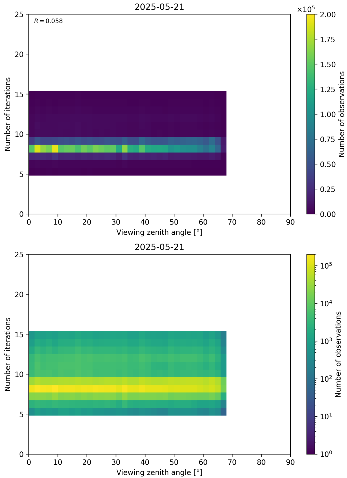
Figure 75: Scatter density plot of “Viewing zenith angle” against “Number of iterations” for 2025-05-21 to 2025-05-22.
