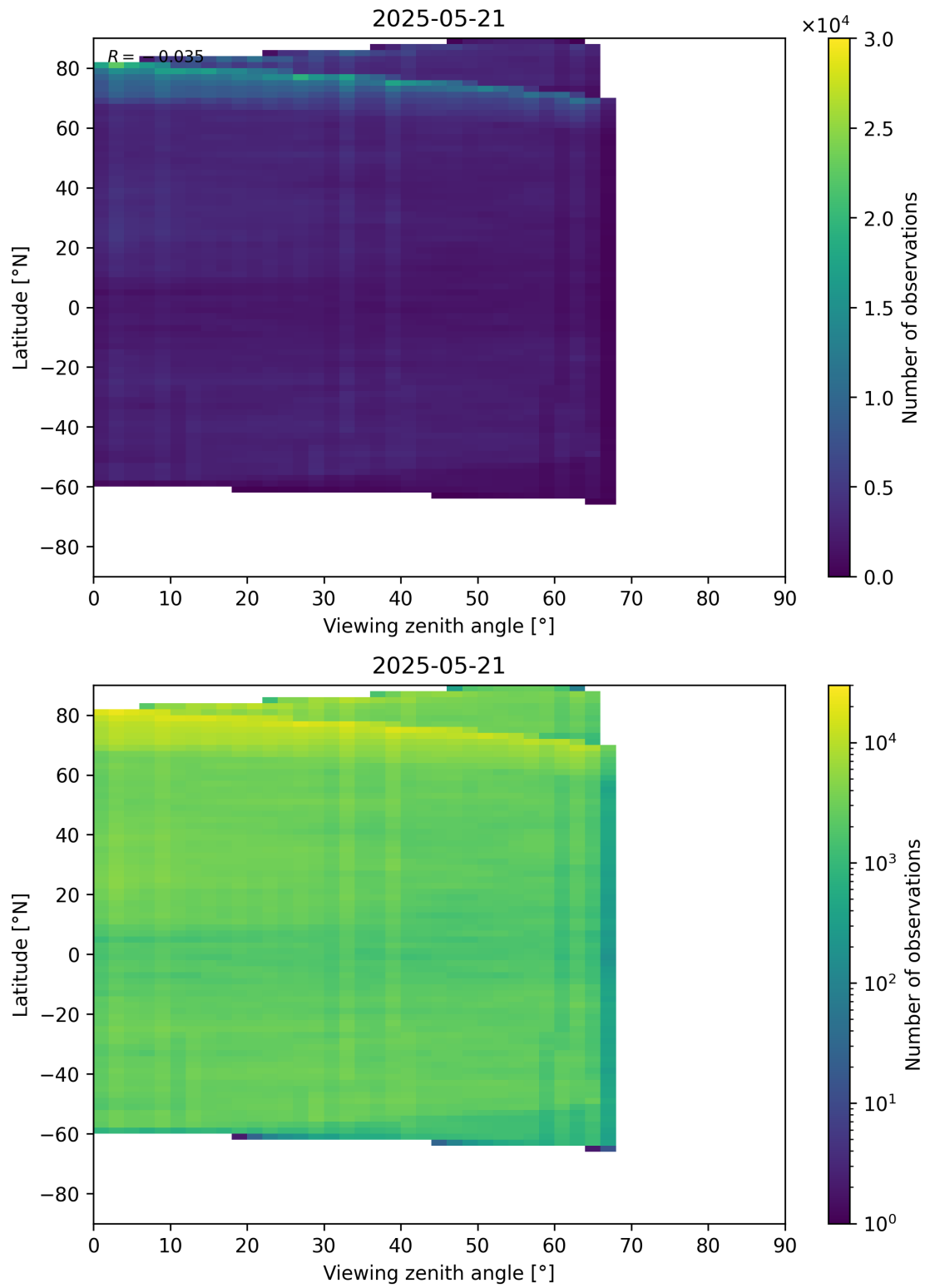
Figure 74: Scatter density plot of “Viewing zenith angle” against “Latitude” for 2025-05-21 to 2025-05-22.
