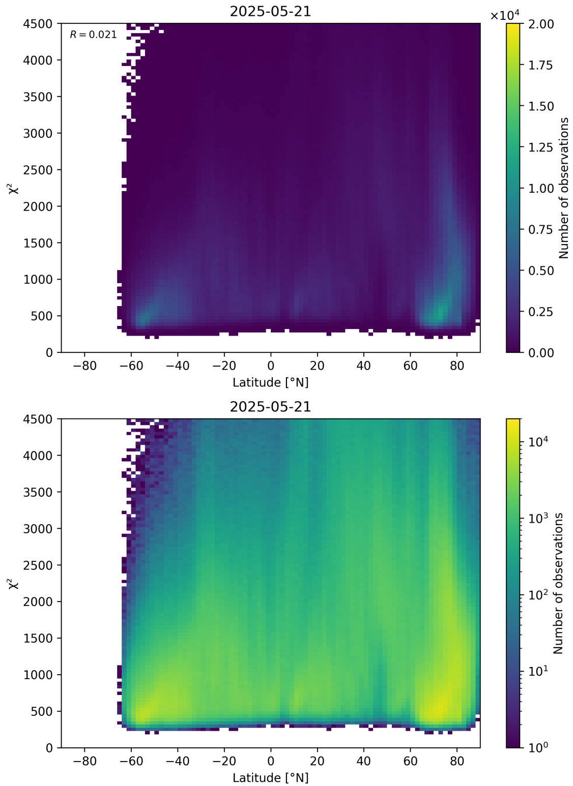
Figure 54: Scatter density plot of “Latitude” against “ \chi^2 ” for 2025-05-21 to 2025-05-22.
