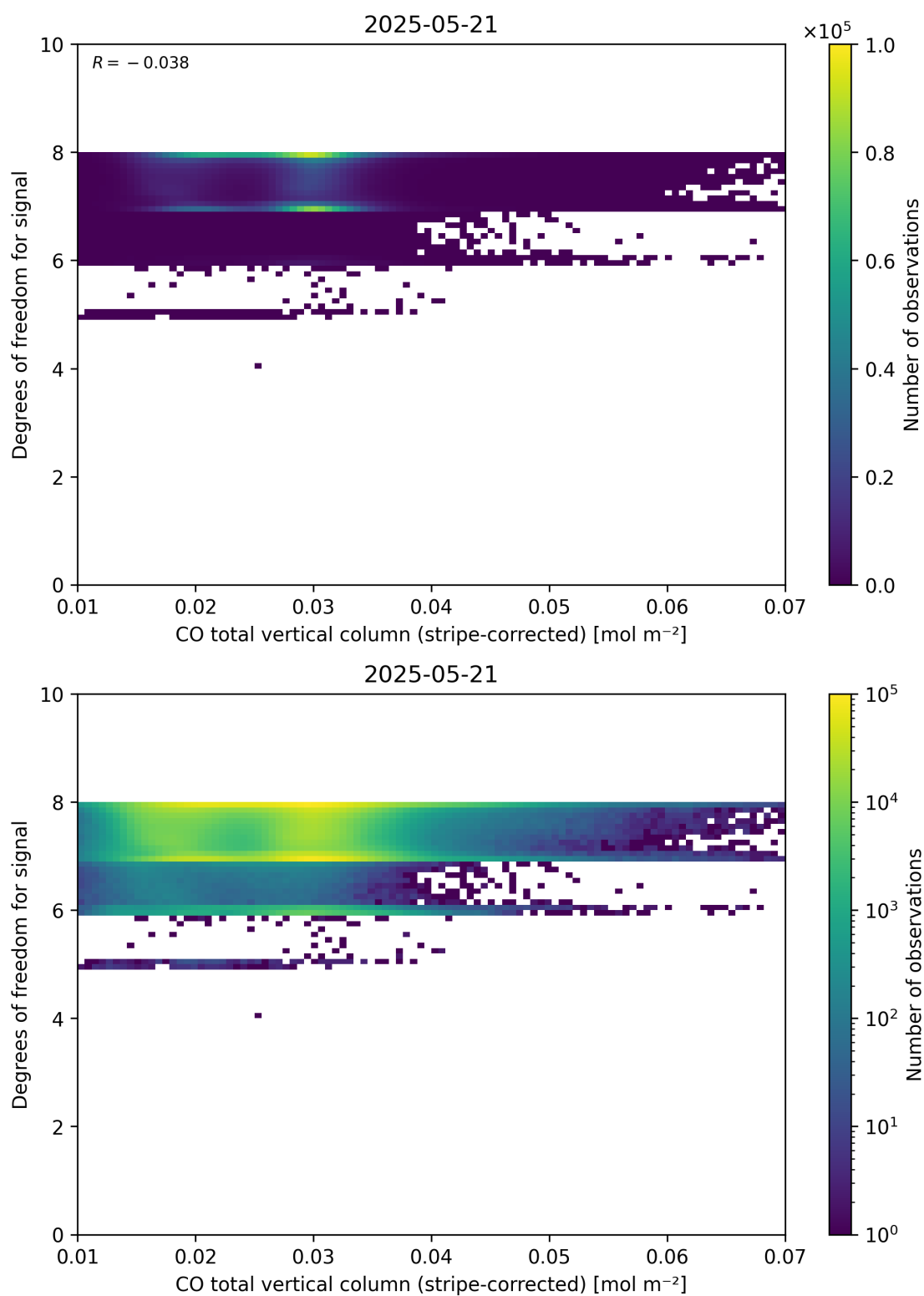
Figure 38: Scatter density plot of “CO total vertical column (stripe-corrected)” against “Degrees of freedom for signal” for 2025-05-21 to 2025-05-22.
