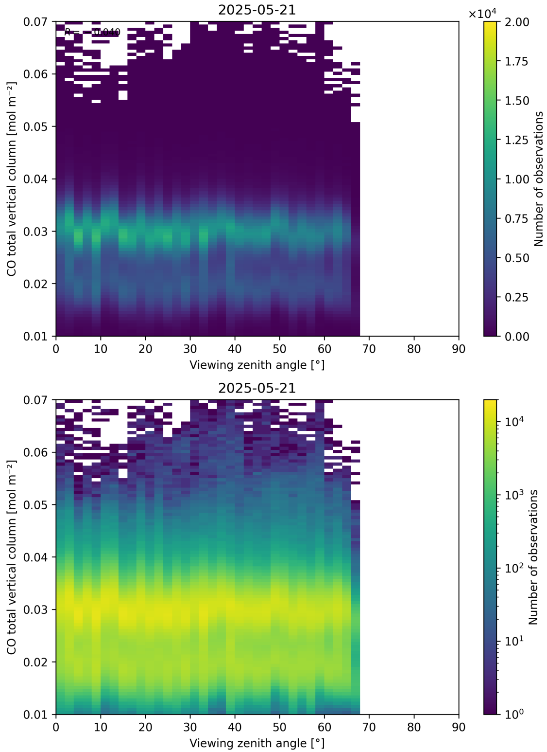
Figure 69: Scatter density plot of “Viewing zenith angle” against “CO total vertical column” for 2025-05-21 to 2025-05-22.
