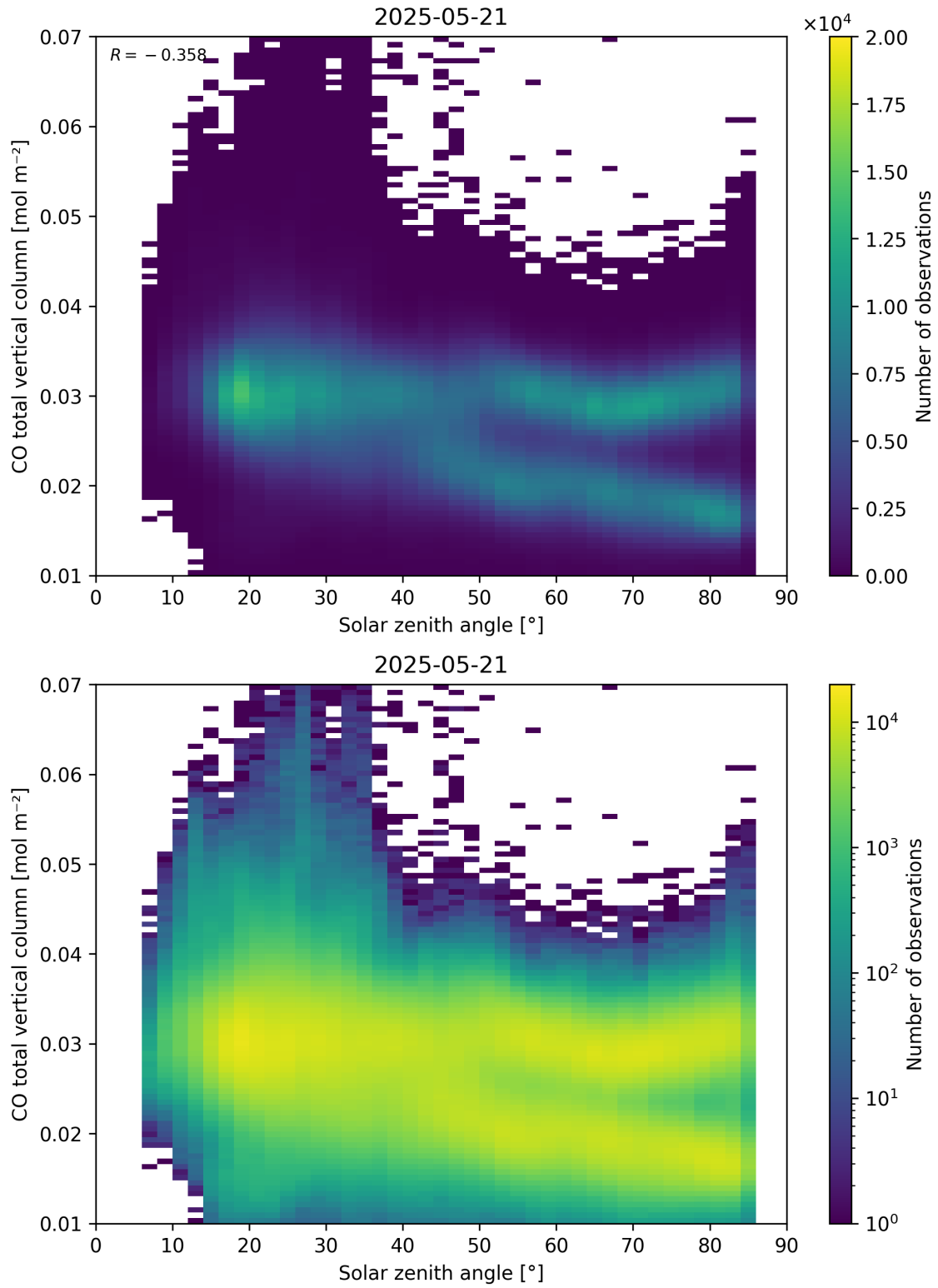
Figure 61: Scatter density plot of “Solar zenith angle” against “CO total vertical column” for 2025-05-21 to 2025-05-22.
