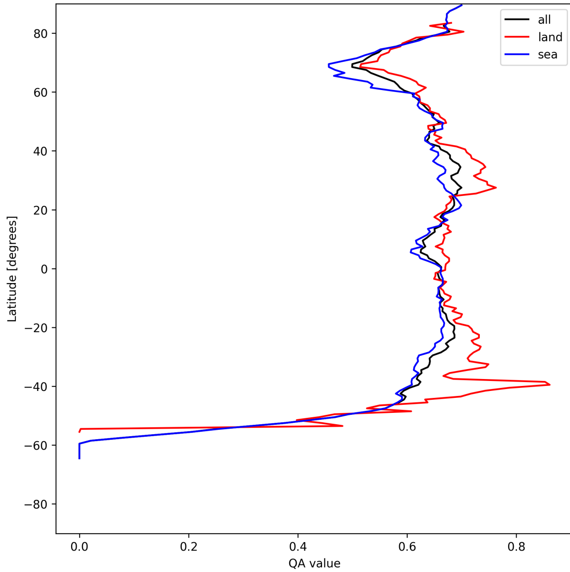
Figure 9: Zonal average of “QA value” for 2025-05-21 to 2025-05-22.
