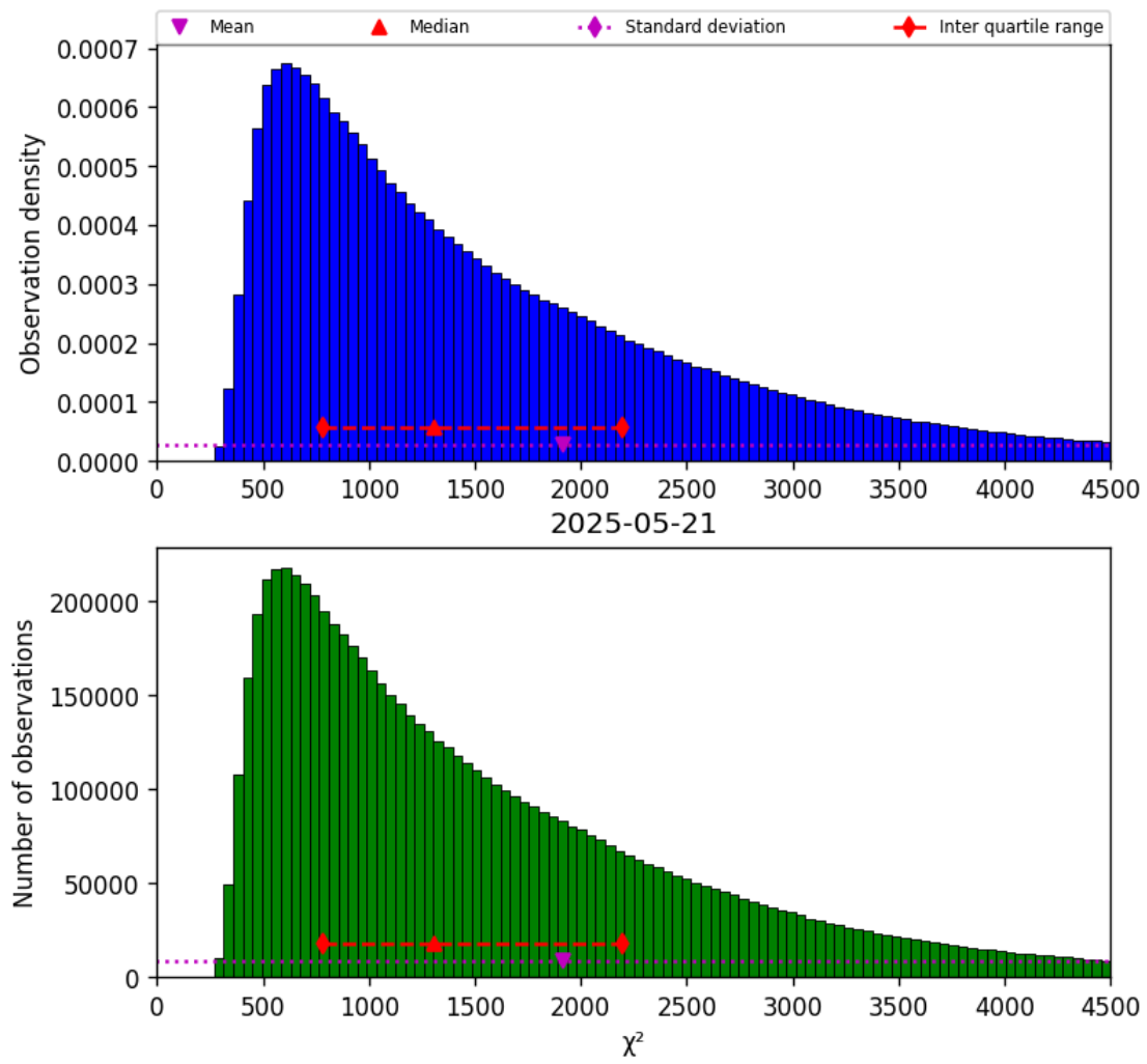
Figure 22: Histogram of “ \chi^2 ” for 2025-05-21 to 2025-05-22
