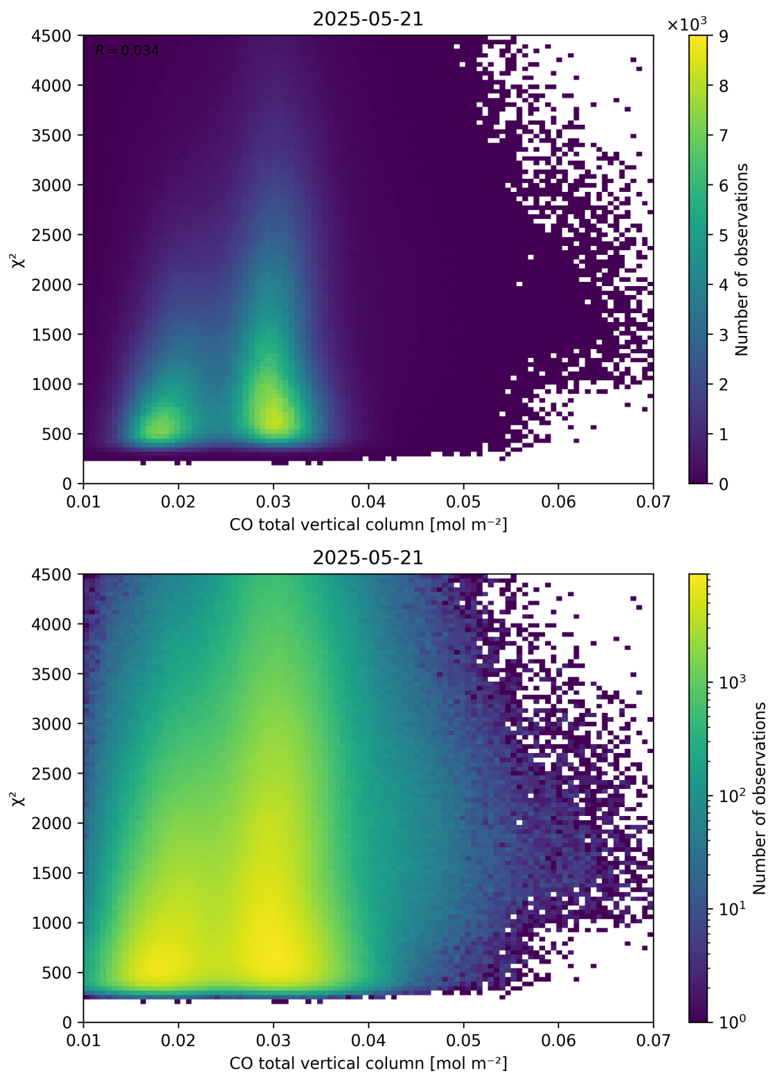
Figure 35: Scatter density plot of “CO total vertical column” against “ \chi^2 ” for 2025-05-21 to 2025-05-22.
