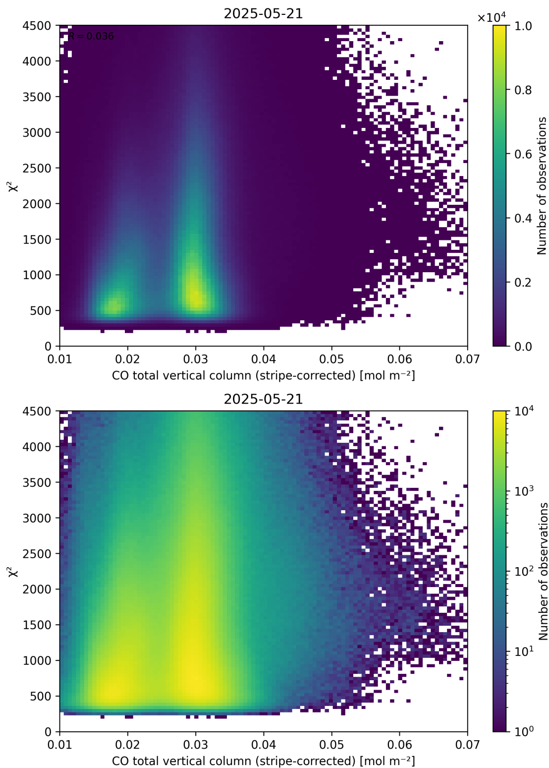
Figure 37: Scatter density plot of “CO total vertical column (stripe-corrected)” against “ \chi^2 ” for 2025-05-21 to 2025-05-22.
