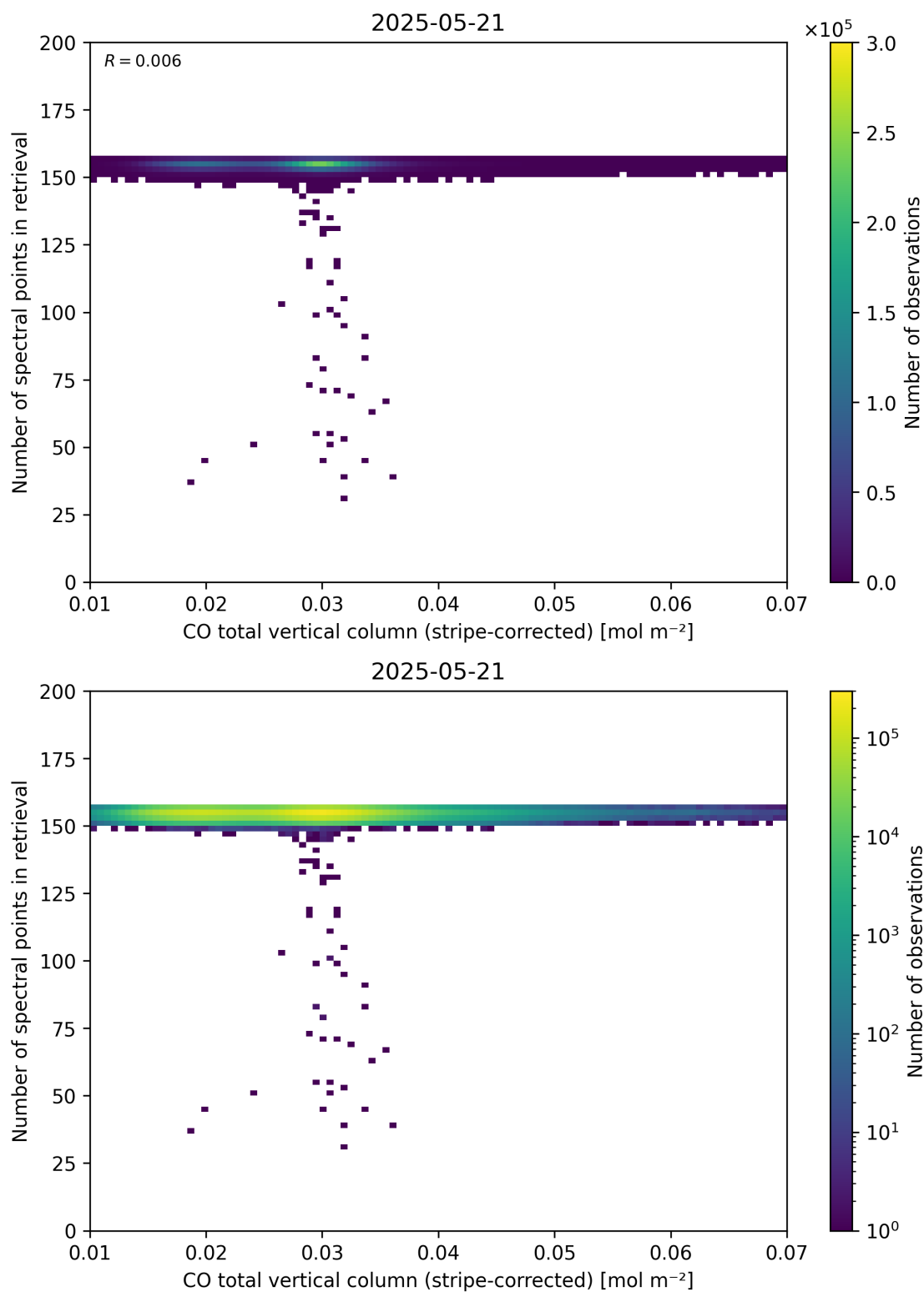
Figure 40: Scatter density plot of “CO total vertical column (stripe-corrected)” against “Number of spectral points in retrieval” for 2025-05-21 to 2025-05-22.
