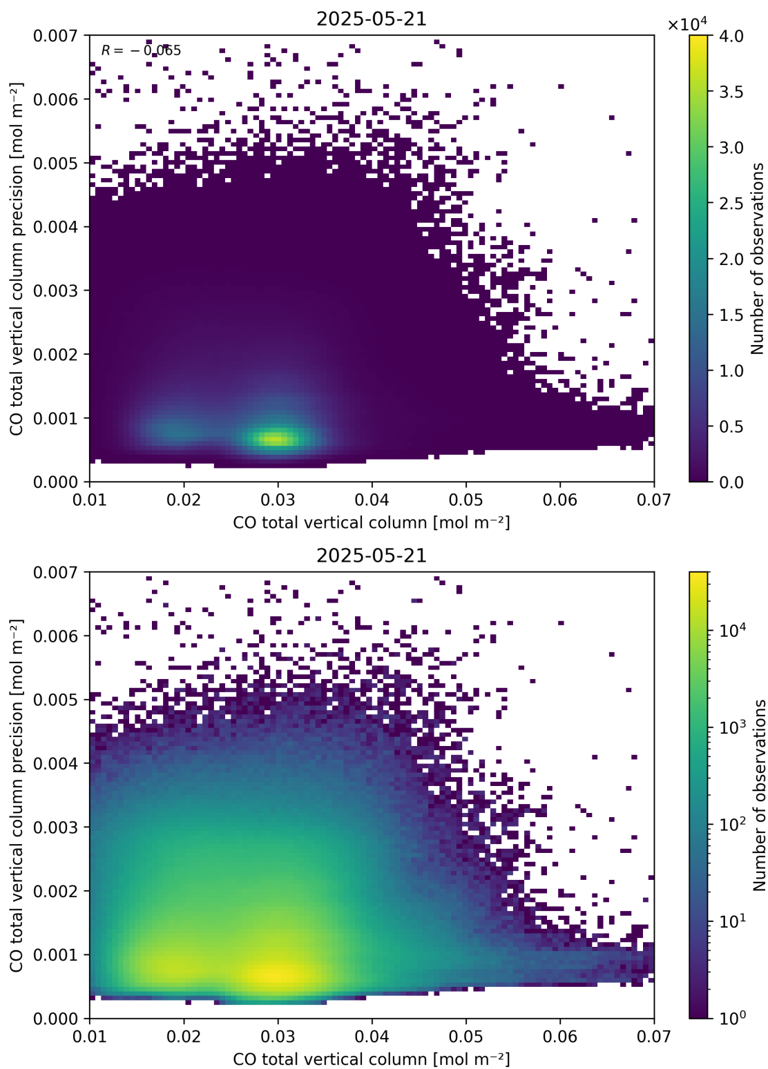
Figure 34: Scatter density plot of “CO total vertical column” against “CO total vertical column precision” for 2025-05-21 to 2025-05-22.
