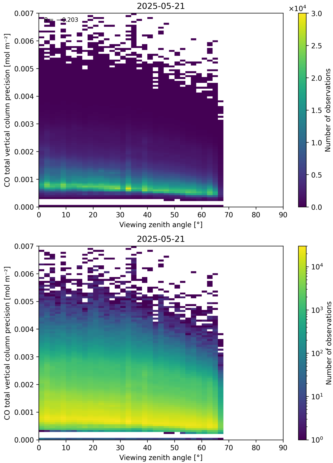
Figure 71: Scatter density plot of “Viewing zenith angle” against “CO total vertical column precision” for 2025-05-21 to 2025-05-22.
