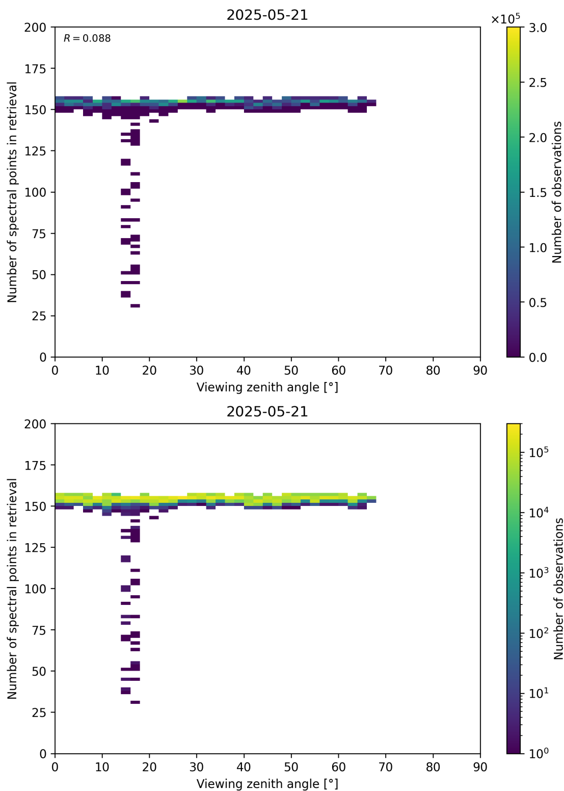
Figure 76: Scatter density plot of “Viewing zenith angle” against “Number of spectral points in retrieval” for 2025-05-21 to 2025-05-22.
