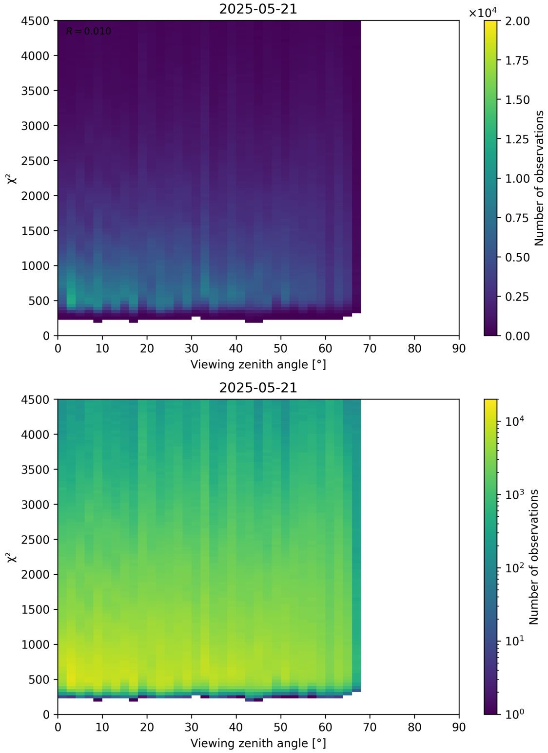
Figure 72: Scatter density plot of “Viewing zenith angle” against “ \chi^2 ” for 2025-05-21 to 2025-05-22.
