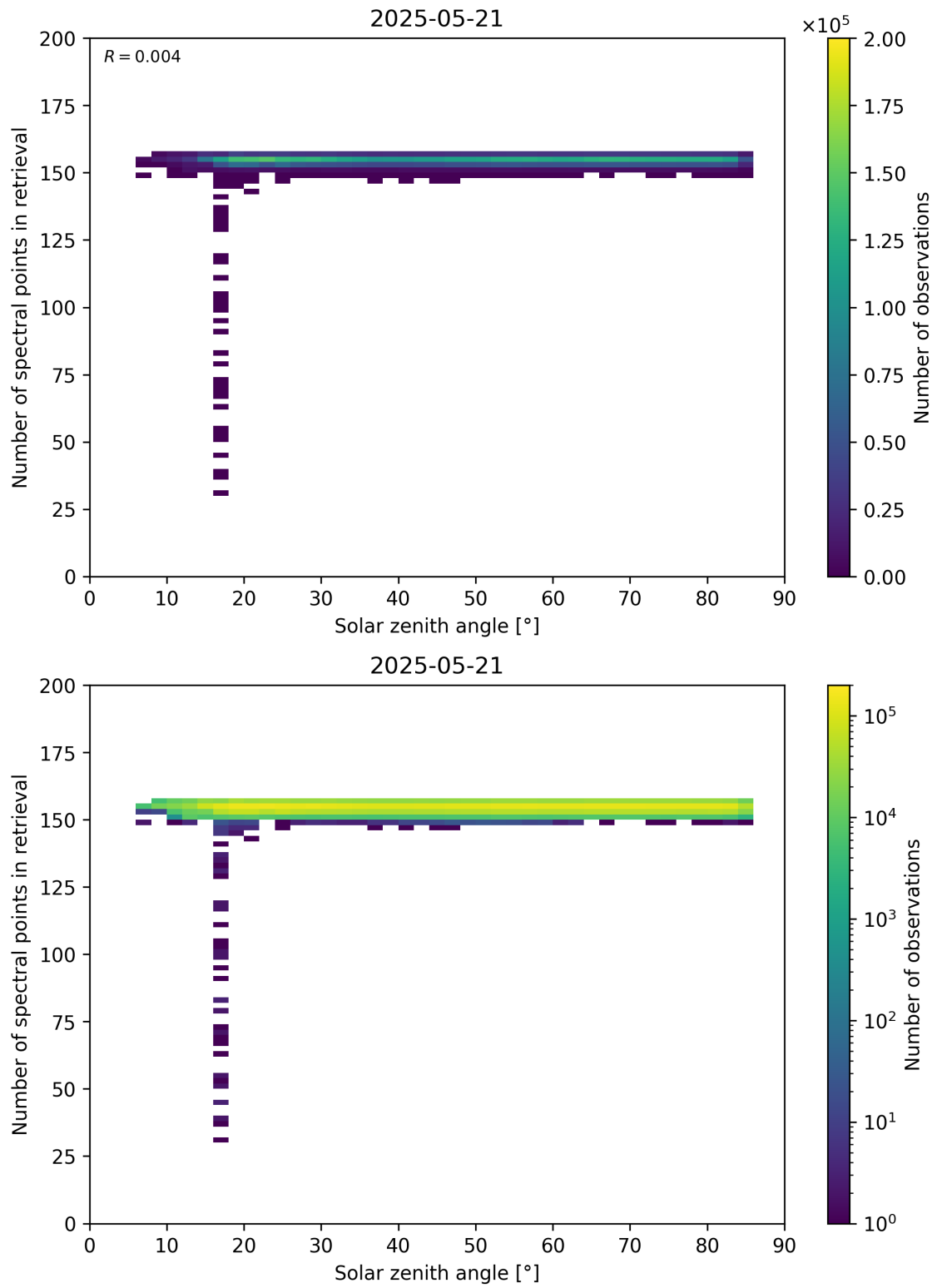
Figure 68: Scatter density plot of “Solar zenith angle” against “Number of spectral points in retrieval” for 2025-05-21 to 2025-05-22.
