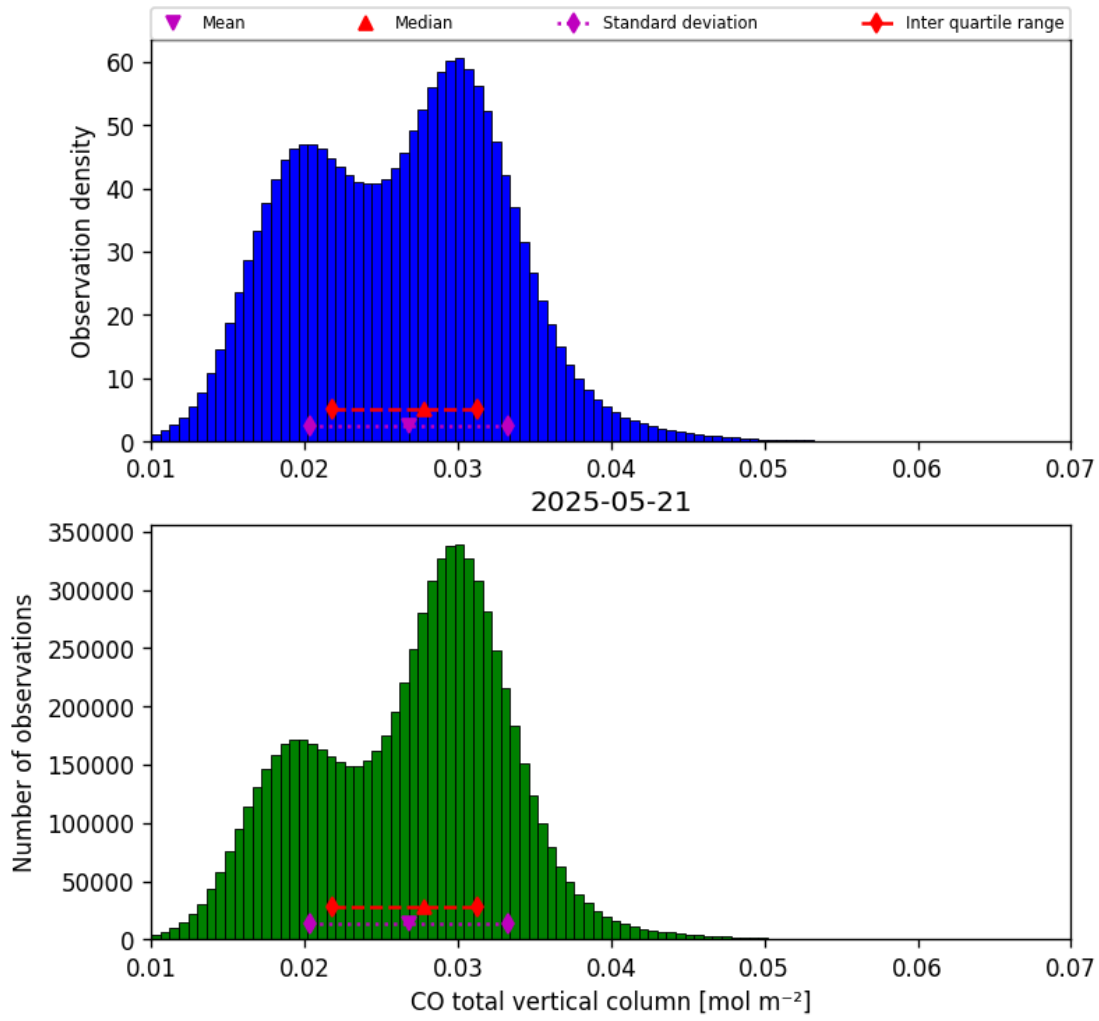
Figure 18: Histogram of “CO total vertical column” for 2025-05-21 to 2025-05-22
