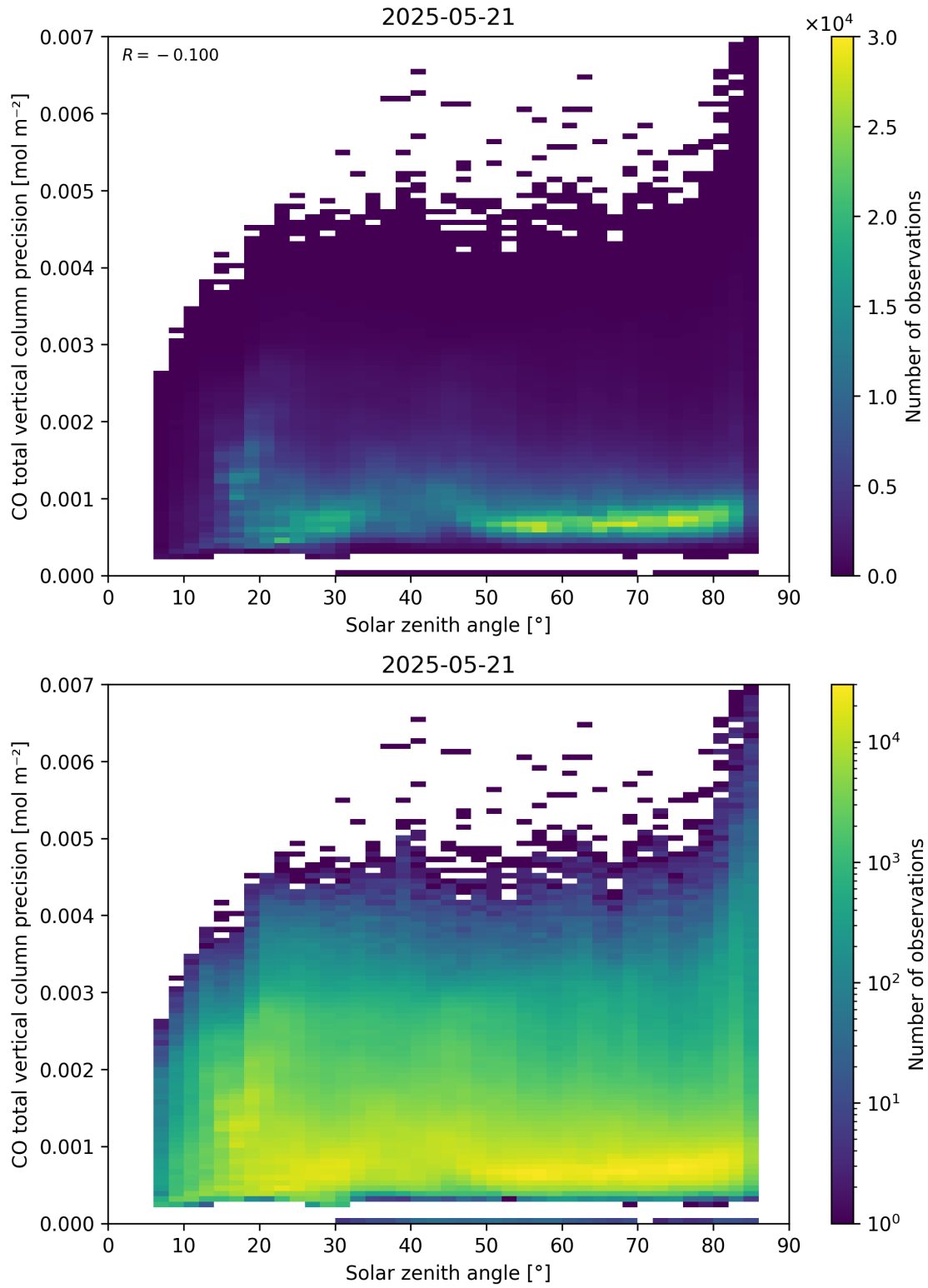
Figure 63: Scatter density plot of “Solar zenith angle” against “CO total vertical column precision” for 2025-05-21 to 2025-05-22.
