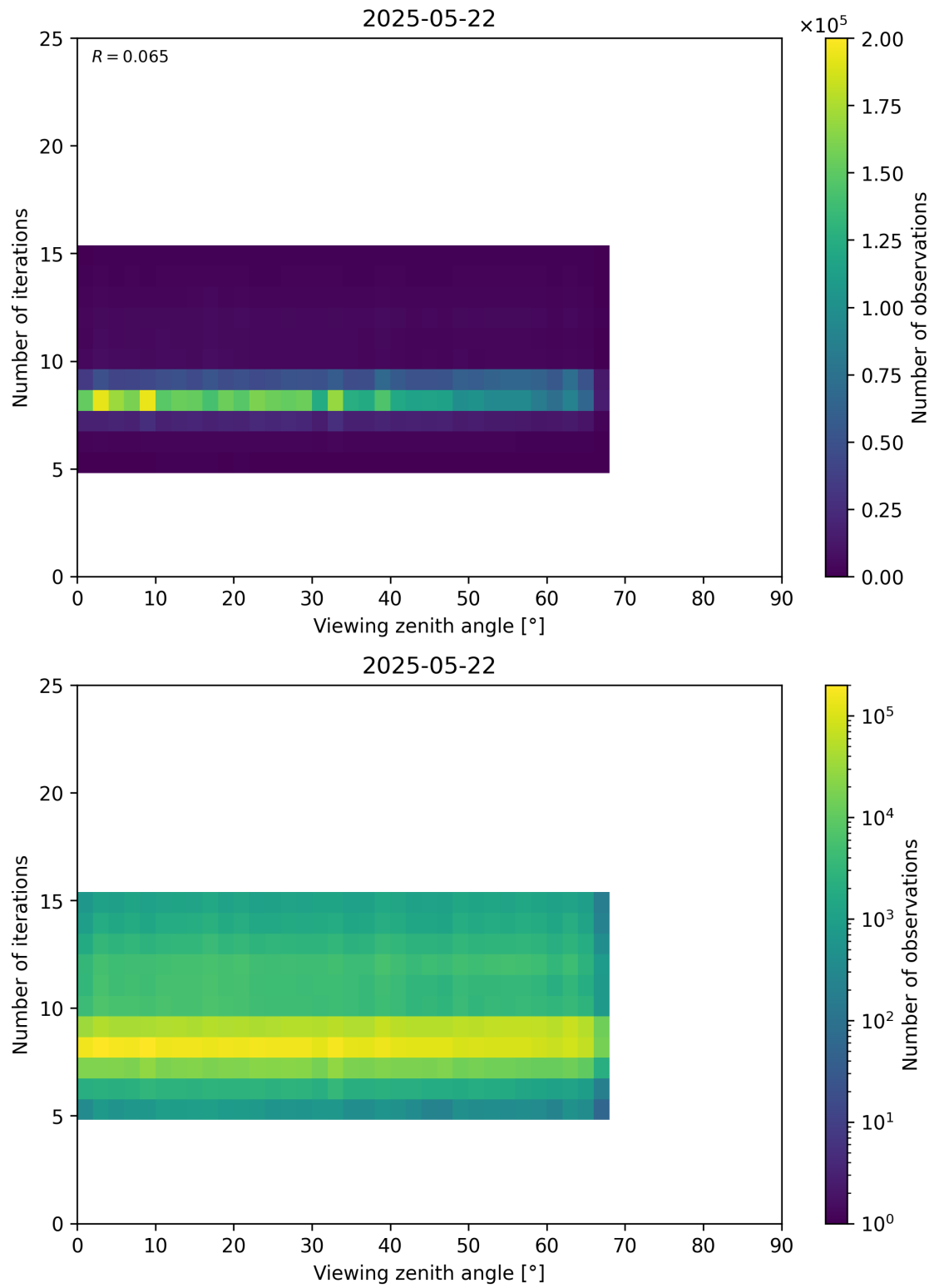
Figure 75: Scatter density plot of “Viewing zenith angle” against “Number of iterations” for 2025-05-21 to 2025-05-23.
