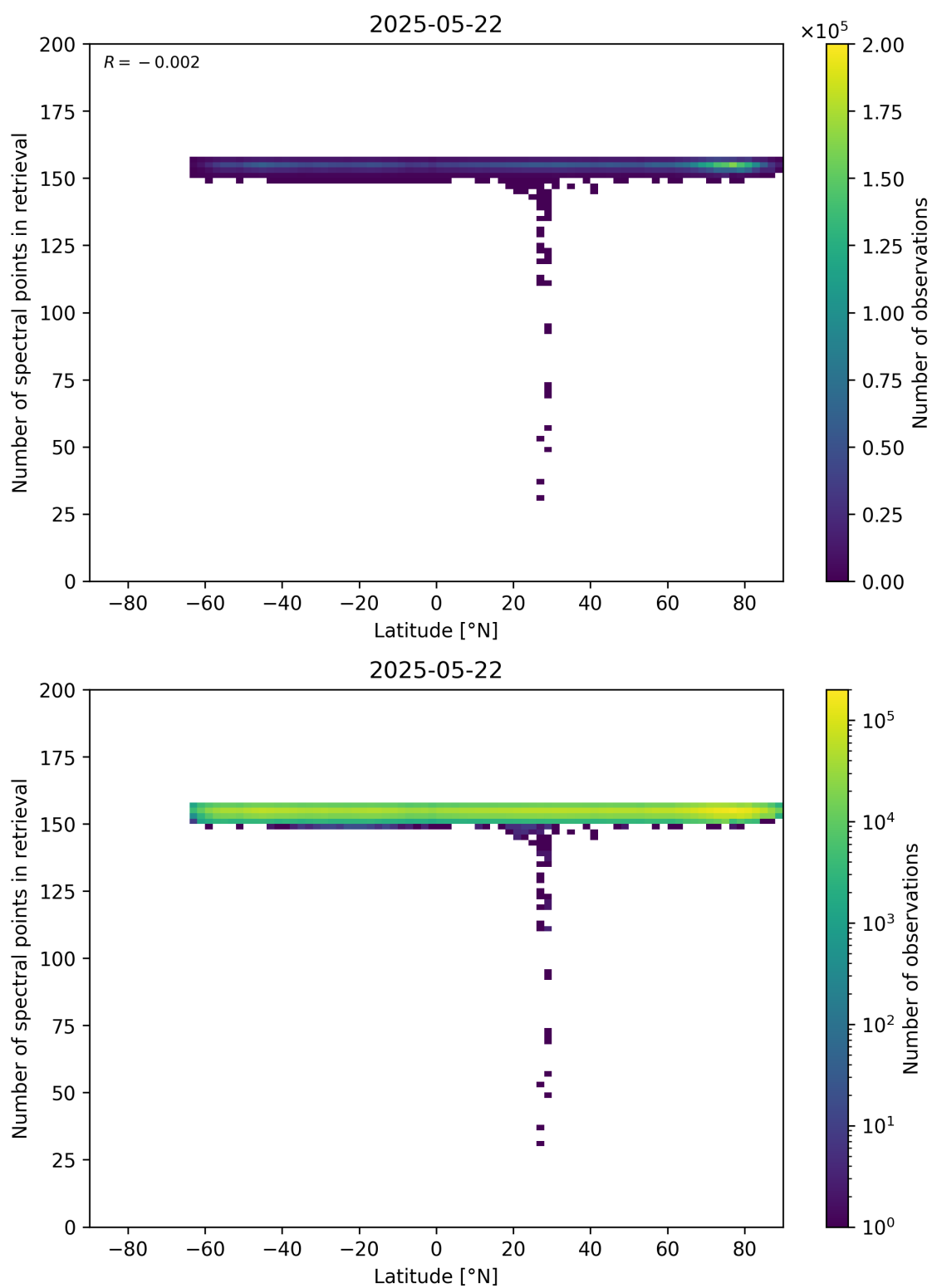
Figure 57: Scatter density plot of “Latitude” against “Number of spectral points in retrieval” for 2025-05-21 to 2025-05-23.
