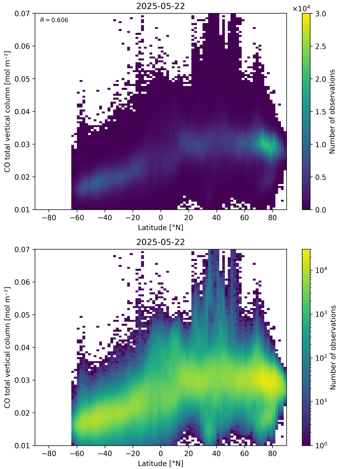
Figure 51: Scatter density plot of “Latitude” against “CO total vertical column” for 2025-05-21 to 2025-05-23.
