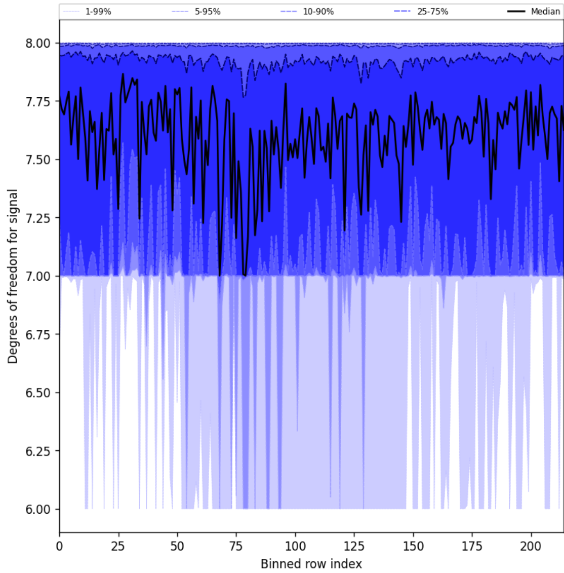
Figure 31: Along track statistics of “Degrees of freedom for signal” for 2025-05-21 to 2025-05-23
