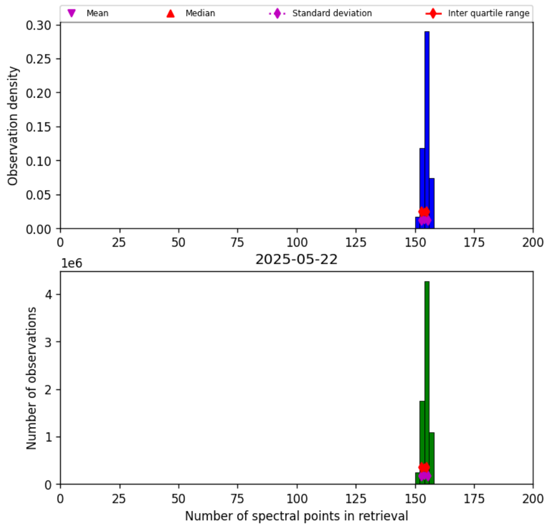
Figure 21: Histogram of “Number of spectral points in retrieval” for 2025-05-21 to 2025-05-23
