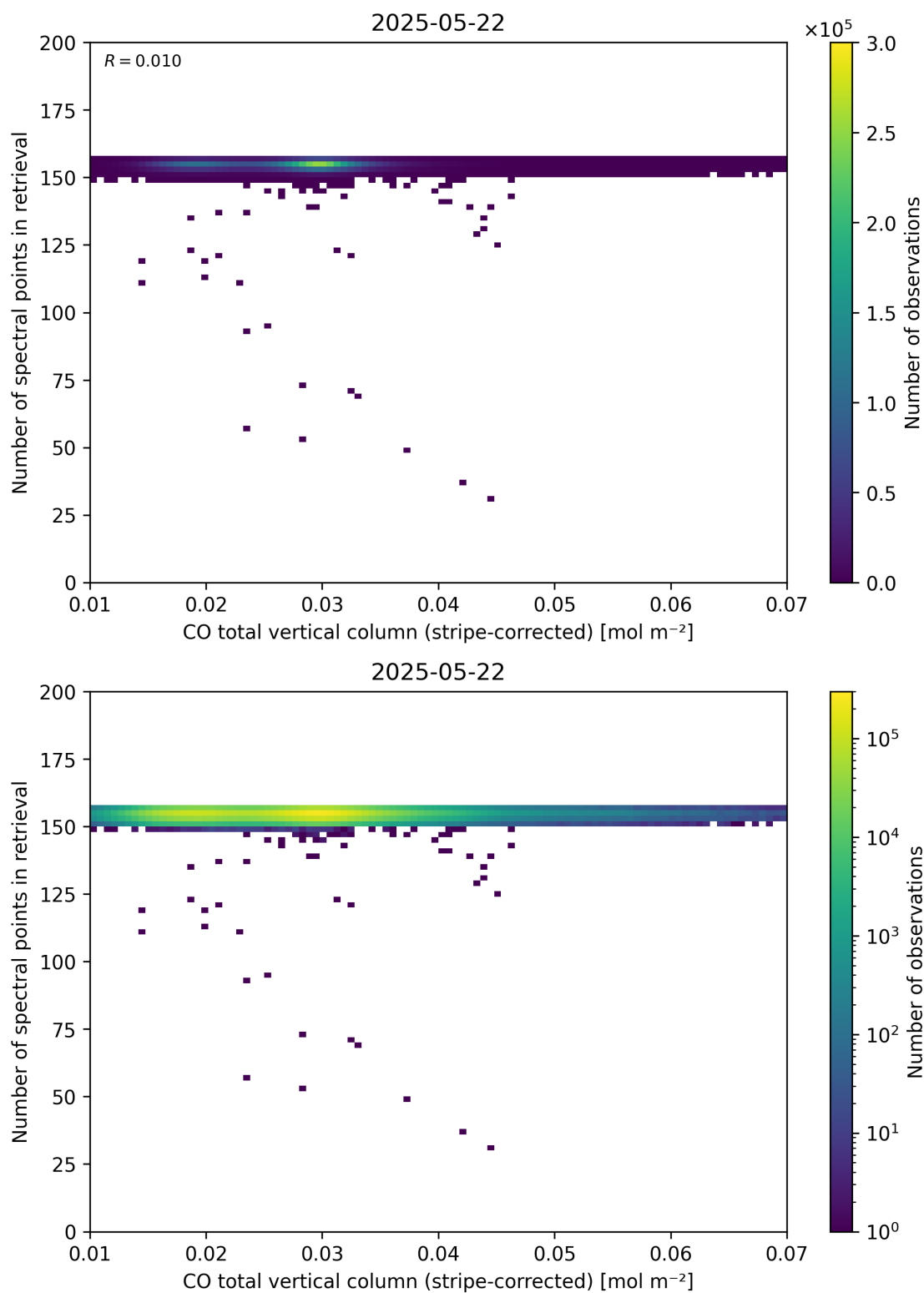
Figure 40: Scatter density plot of “CO total vertical column (stripe-corrected)” against “Number of spectral points in retrieval” for 2025-05-21 to 2025-05-23.
