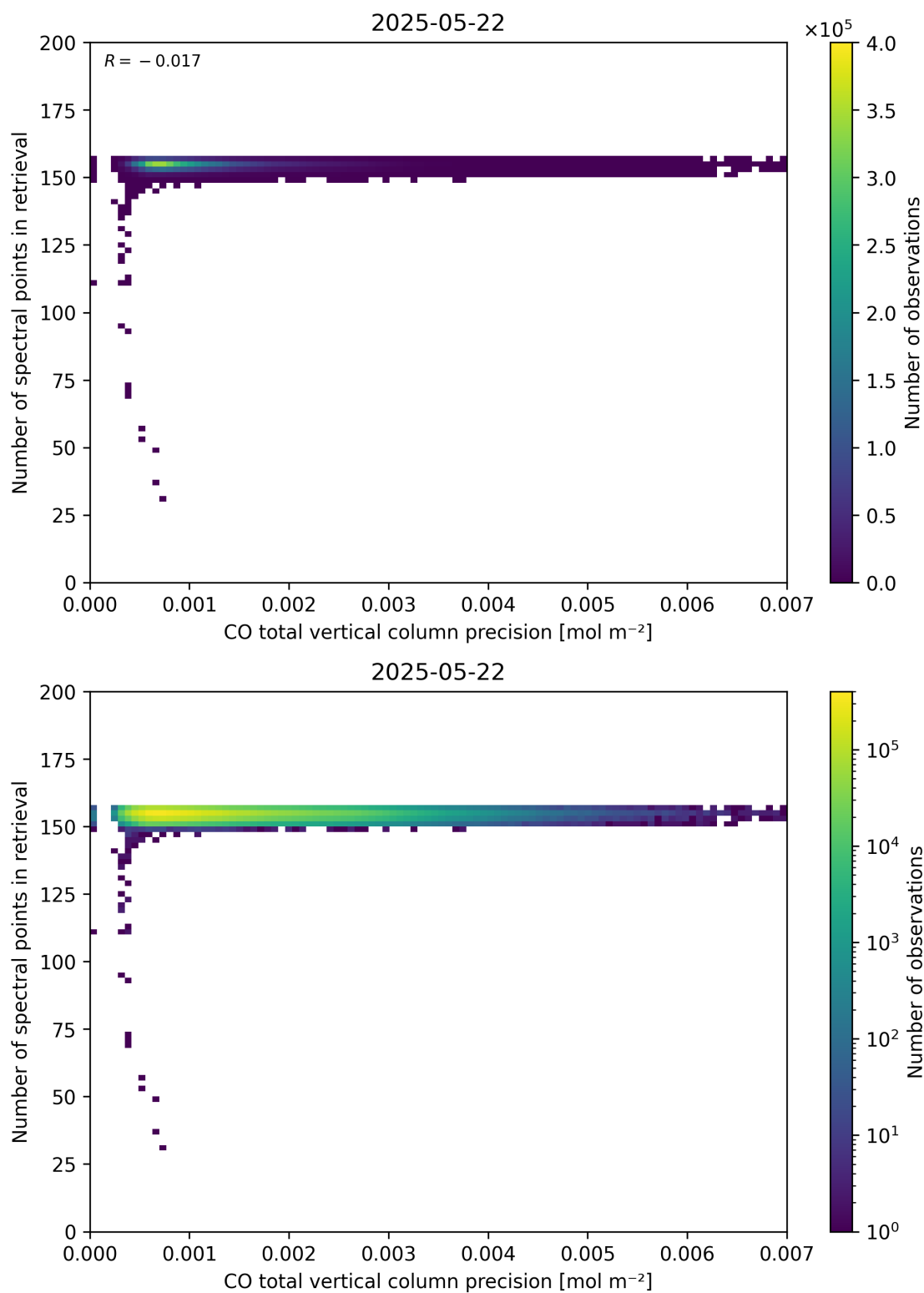
Figure 47: Scatter density plot of “CO total vertical column precision” against “Number of spectral points in retrieval” for 2025-05-21 to 2025-05-23.
