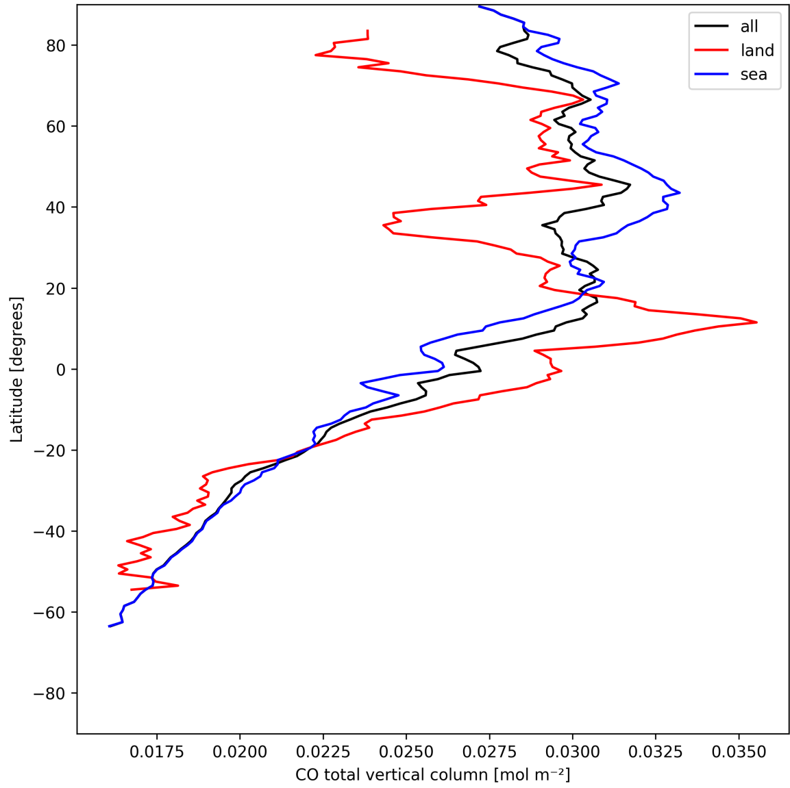
Figure 10: Zonal average of “CO total vertical column” for 2025-05-21 to 2025-05-23.
