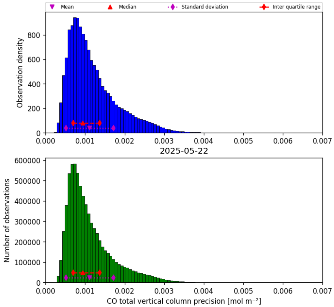
Figure 20: Histogram of “CO total vertical column precision” for 2025-05-21 to 2025-05-23
