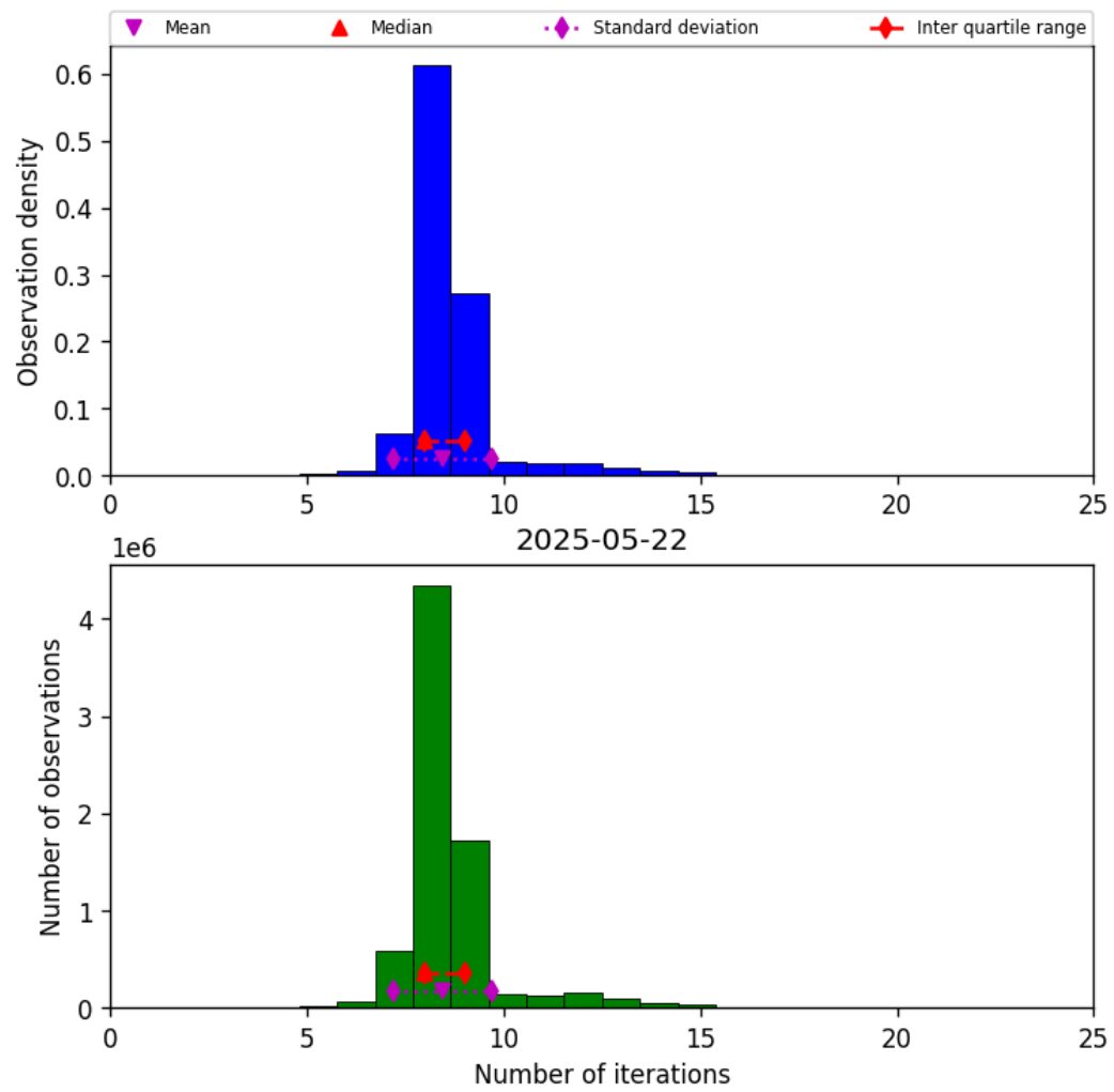
Figure 24: Histogram of “Number of iterations” for 2025-05-21 to 2025-05-23
