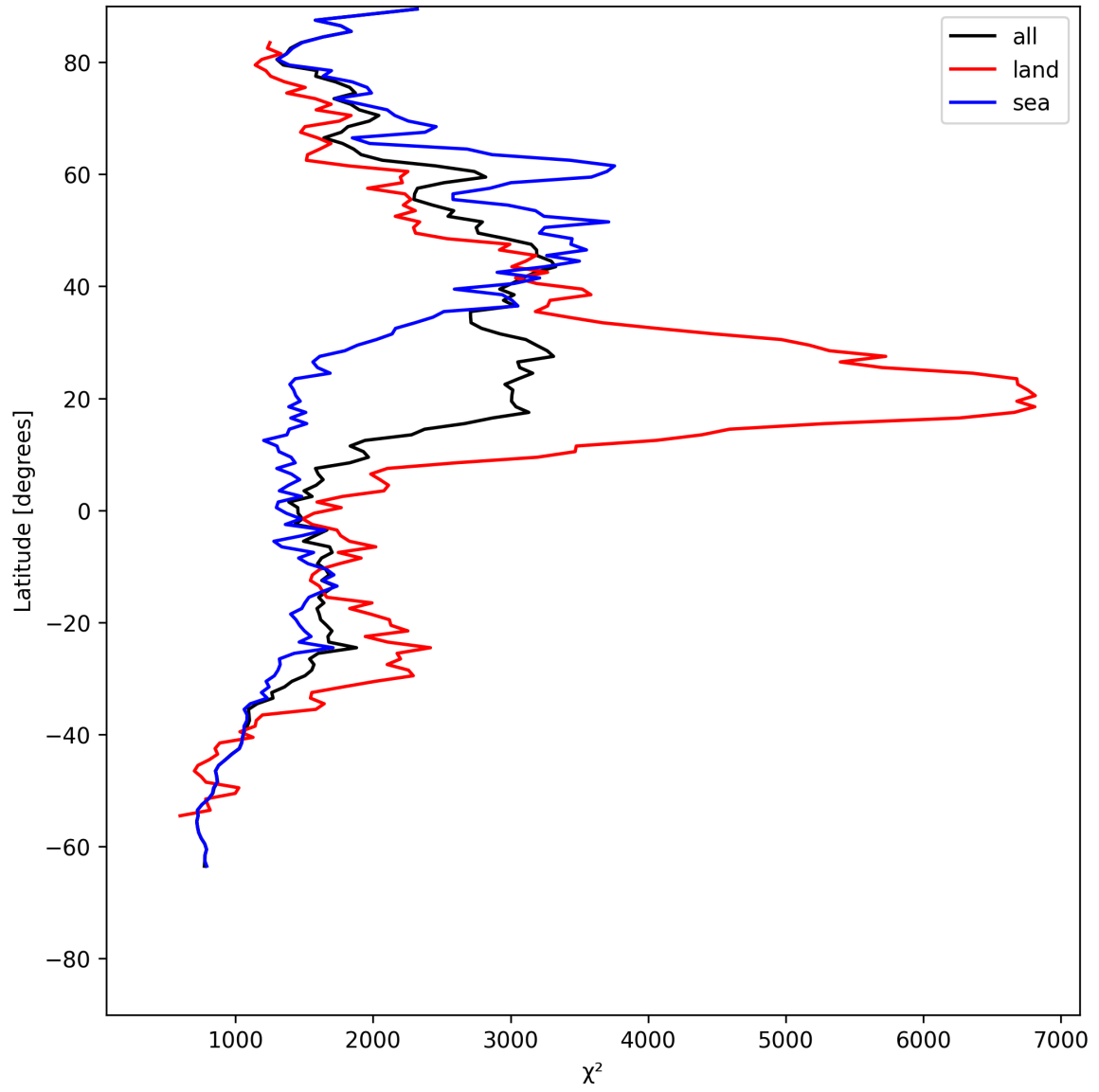
Figure 14: Zonal average of “ \chi^2 ” for 2025-05-21 to 2025-05-23.
