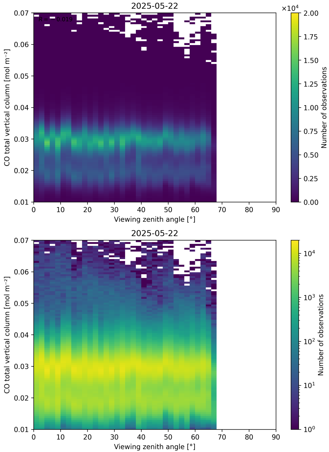
Figure 69: Scatter density plot of “Viewing zenith angle” against “CO total vertical column” for 2025-05-21 to 2025-05-23.
