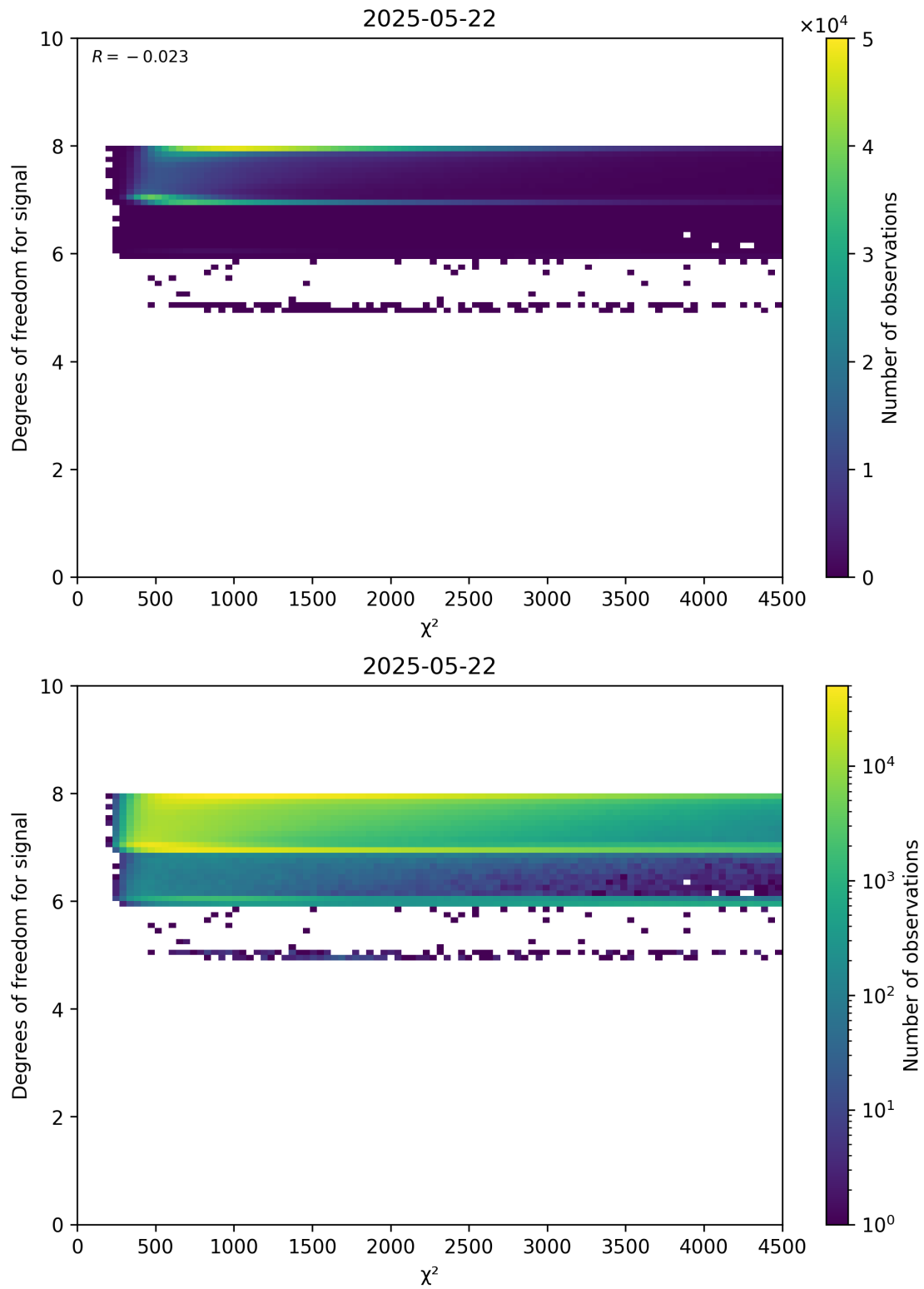
Figure 48: Scatter density plot of “ \chi^2 ” against “Degrees of freedom for signal” for 2025-05-21 to 2025-05-23.
