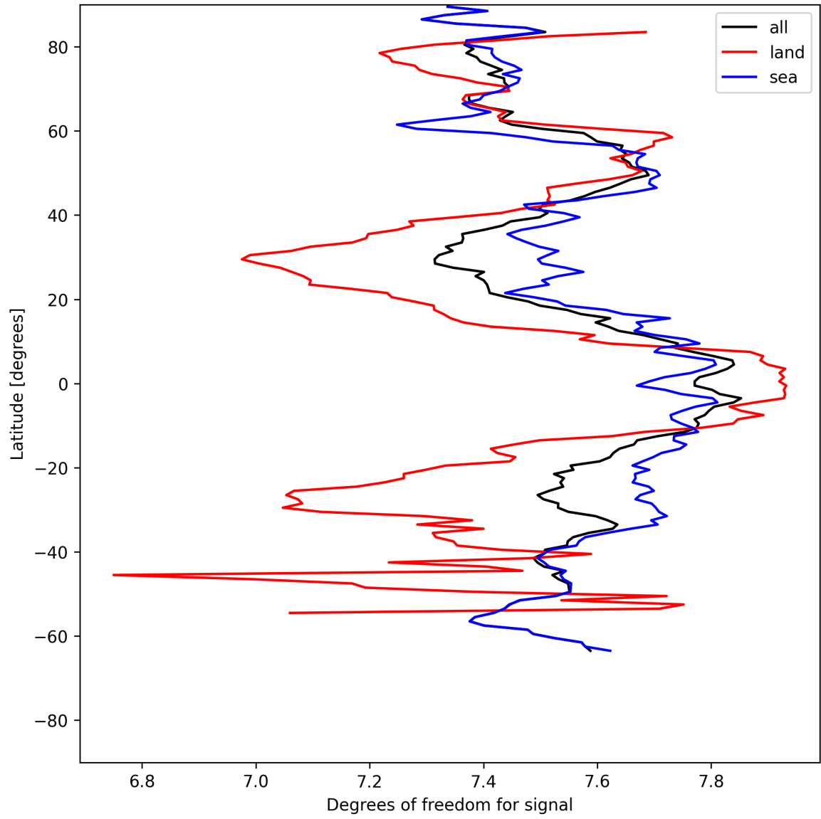
Figure 15: Zonal average of “Degrees of freedom for signal” for 2025-05-21 to 2025-05-23.
