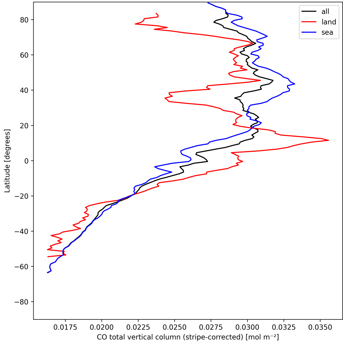
Figure 11: Zonal average of “CO total vertical column (stripe-corrected)” for 2025-05-21 to 2025-05-23.
