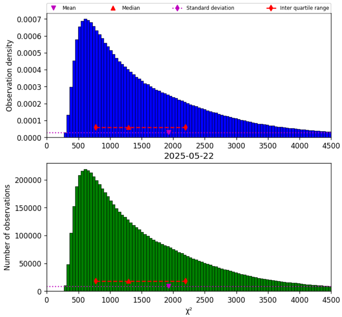
Figure 22: Histogram of " \chi^2 " for 2025-05-21 to 2025-05-23
