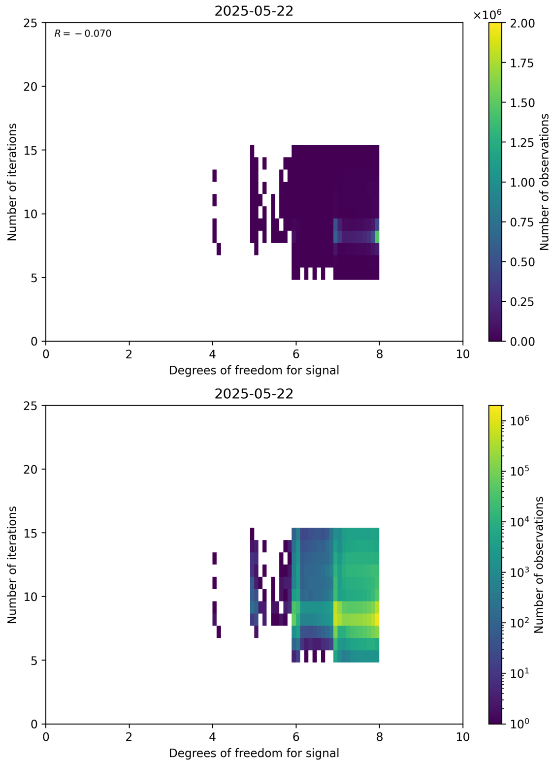
Figure 50: Scatter density plot of “Degrees of freedom for signal” against “Number of iterations” for 2025-05-21 to 2025-05-23.
