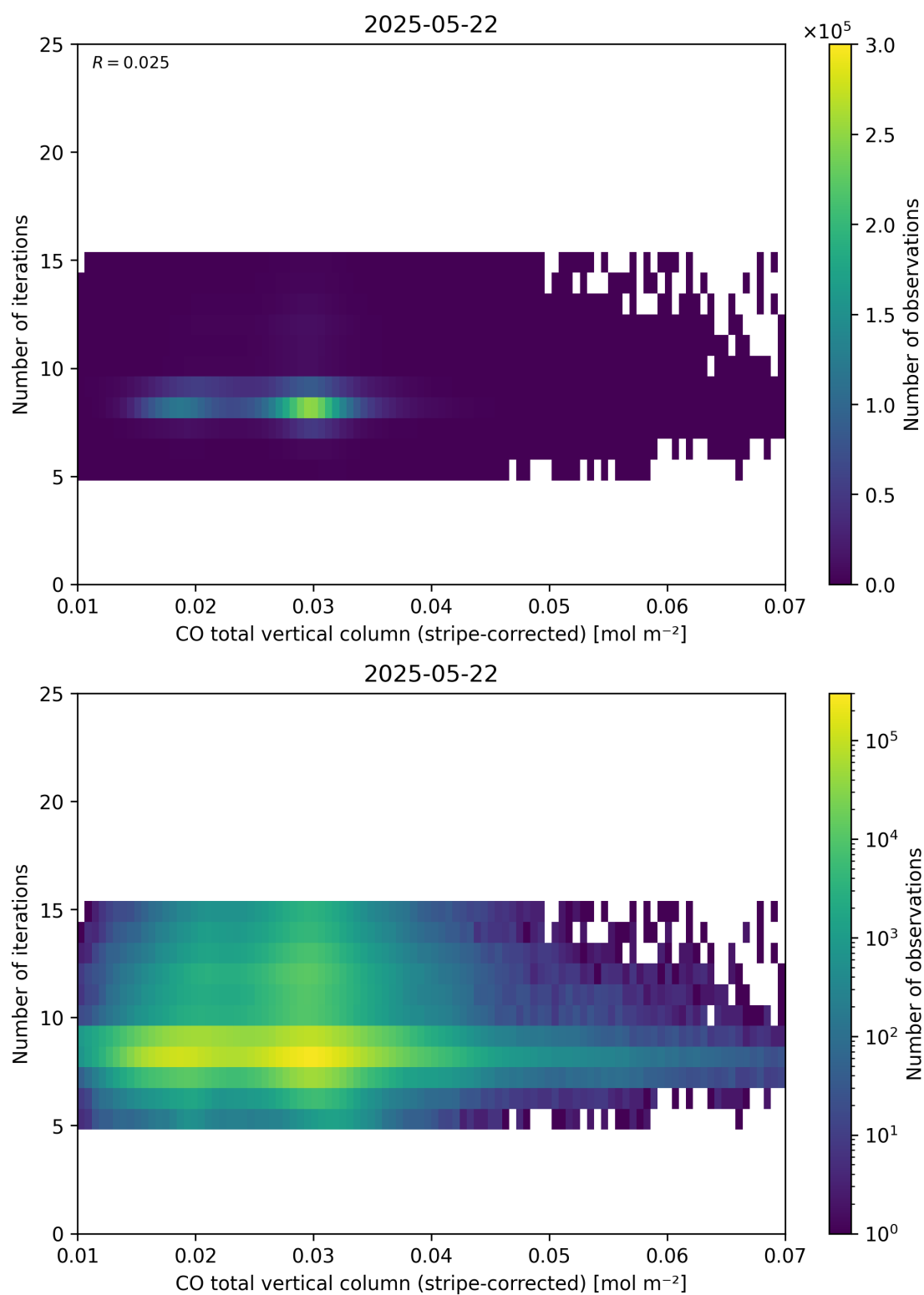
Figure 39: Scatter density plot of “CO total vertical column (stripe-corrected)” against “Number of iterations” for 2025-05-21 to 2025-05-23.
