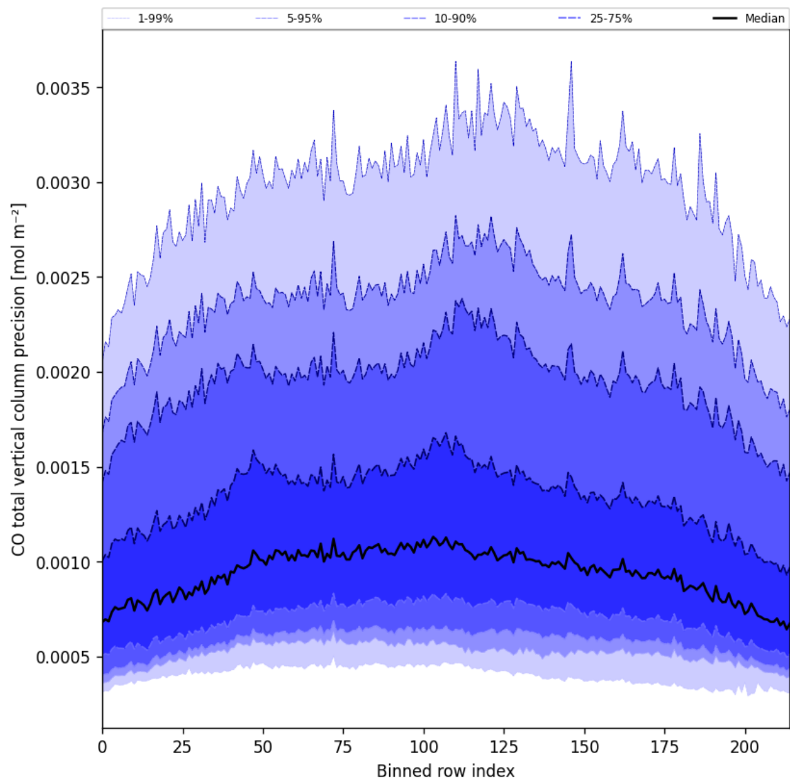
Figure 28: Along track statistics of “CO total vertical column precision” for 2025-05-21 to 2025-05-23
