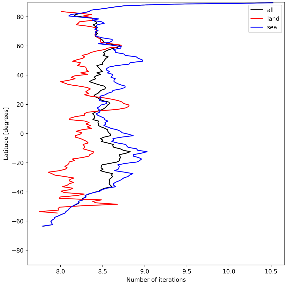
Figure 16: Zonal average of “Number of iterations” for 2025-05-21 to 2025-05-23.
