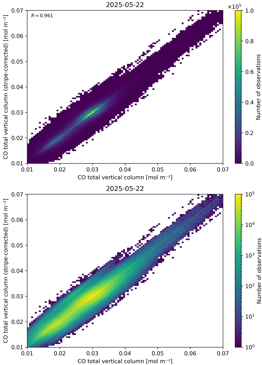
Figure 33: Scatter density plot of “CO total vertical column” against “CO total vertical column (stripe-corrected)” for 2025-05-21 to 2025-05-23.
