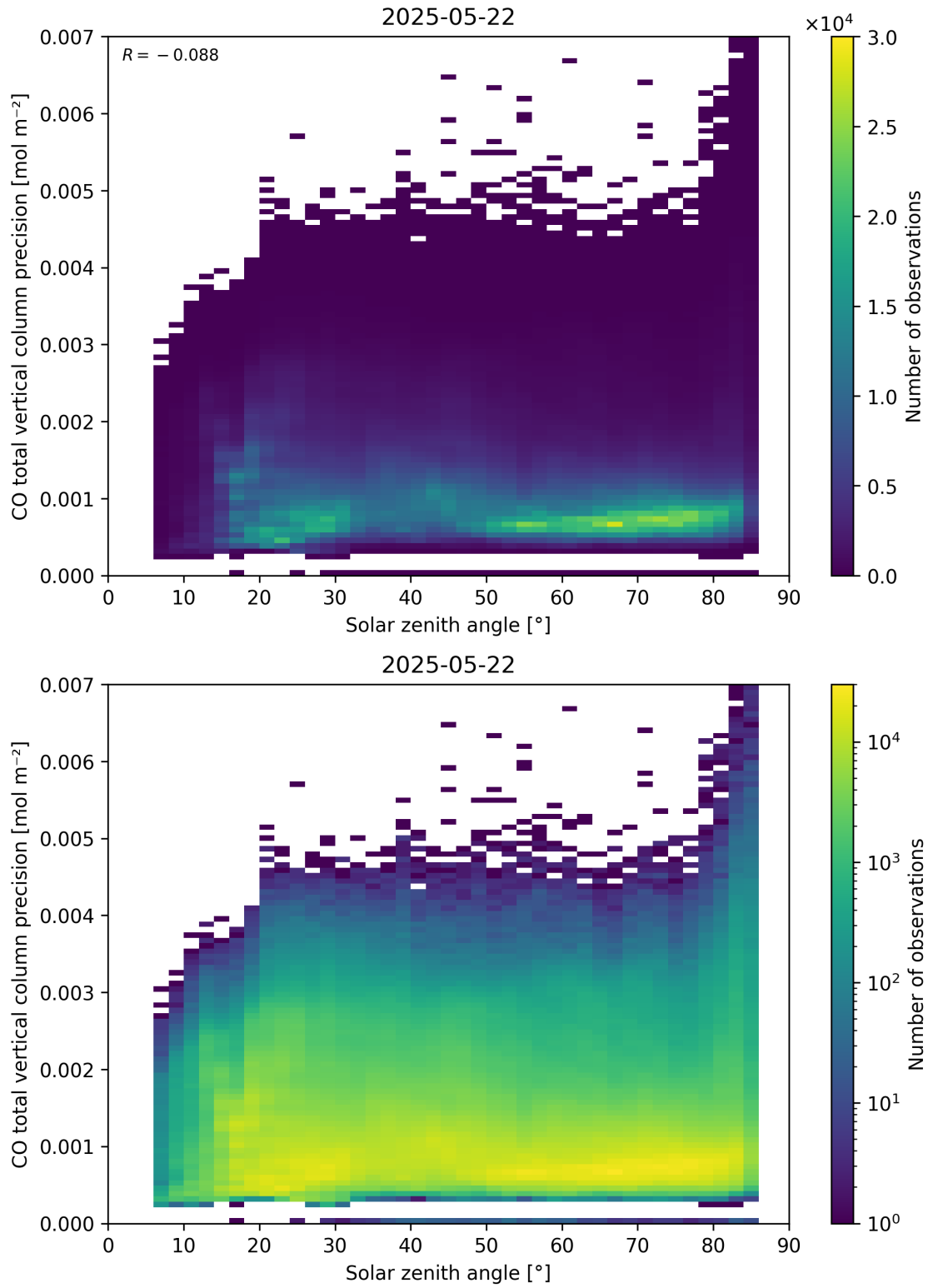
Figure 63: Scatter density plot of “Solar zenith angle” against “CO total vertical column precision” for 2025-05-21 to 2025-05-23.
