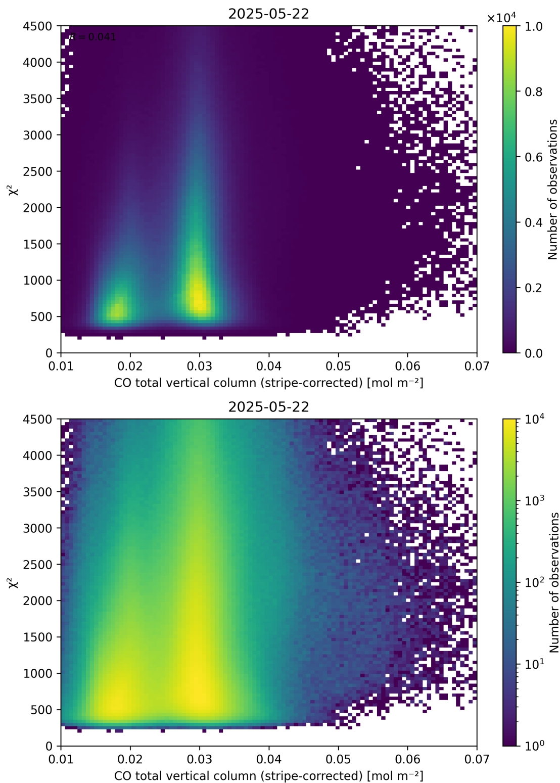
Figure 37: Scatter density plot of “CO total vertical column (stripe-corrected)” against “ \chi^2 ” for 2025-05-21 to 2025-05-23.
