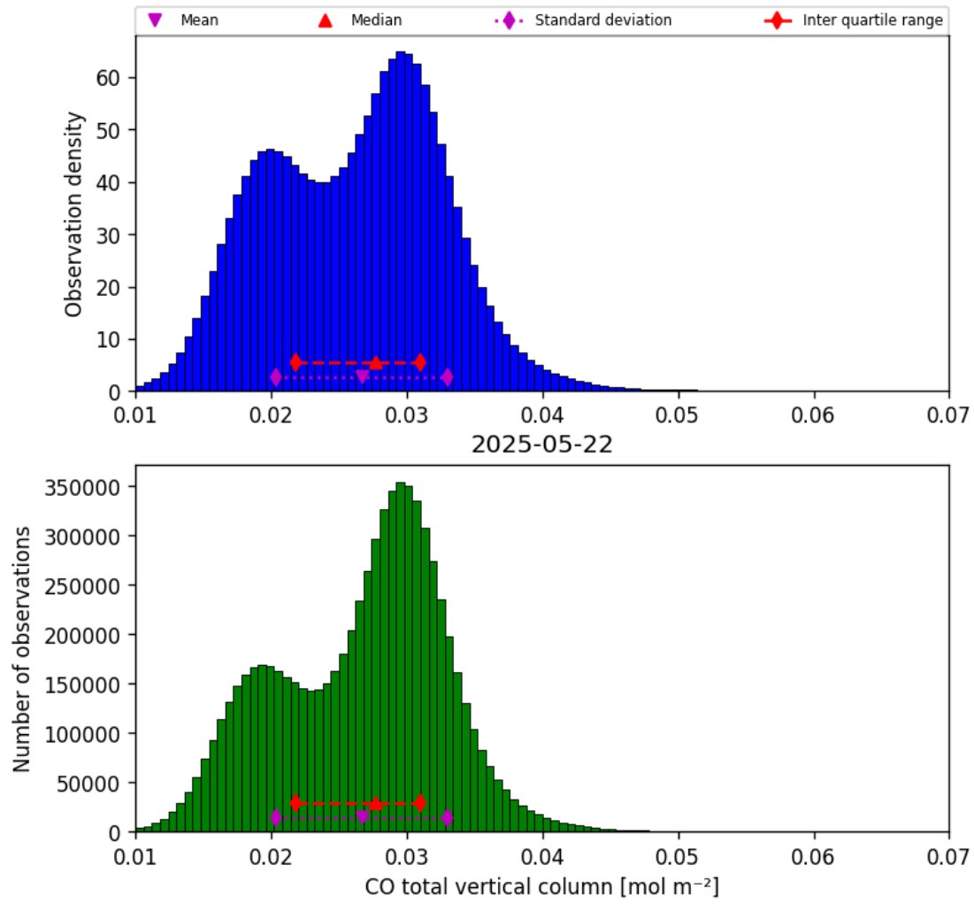
Figure 18: Histogram of “CO total vertical column” for 2025-05-21 to 2025-05-23
