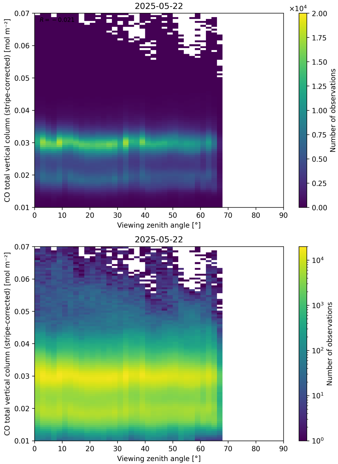
Figure 70: Scatter density plot of “Viewing zenith angle” against “CO total vertical column (stripe-corrected)” for 2025-05-21 to 2025-05-23.
