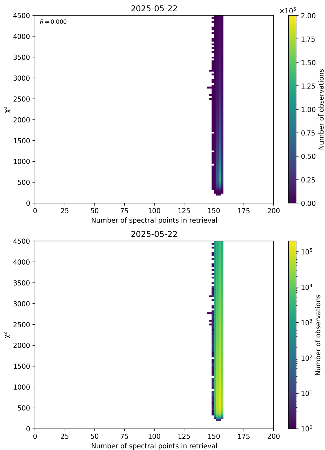
Figure 58: Scatter density plot of “Number of spectral points in retrieval” against “ \chi^2 ” for 2025-05-21 to 2025-05-23.
