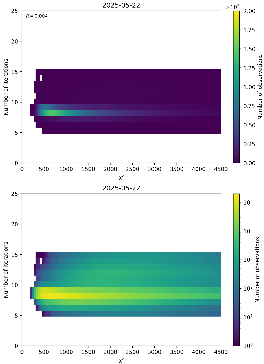
Figure 49: Scatter density plot of “ \chi^2 ” against “Number of iterations” for 2025-05-21 to 2025-05-23.
