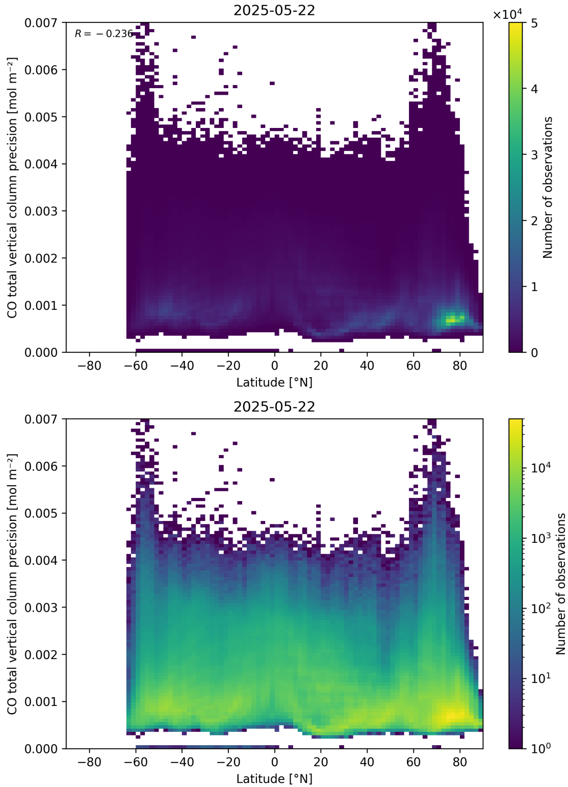
Figure 53: Scatter density plot of “Latitude” against “CO total vertical column precision” for 2025-05-21 to 2025-05-23.
