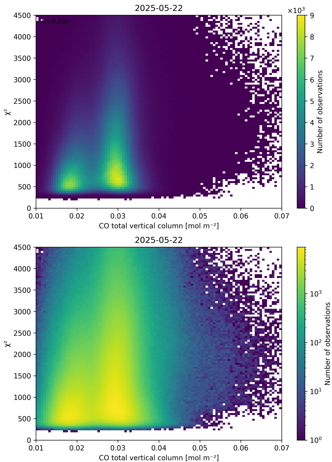
Figure 35: Scatter density plot of “CO total vertical column” against “ \chi^2 ” for 2025-05-21 to 2025-05-23.
