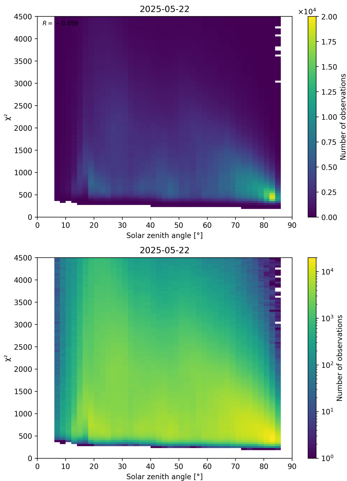
Figure 64: Scatter density plot of “Solar zenith angle” against “ \chi^2 ” for 2025-05-21 to 2025-05-23.
