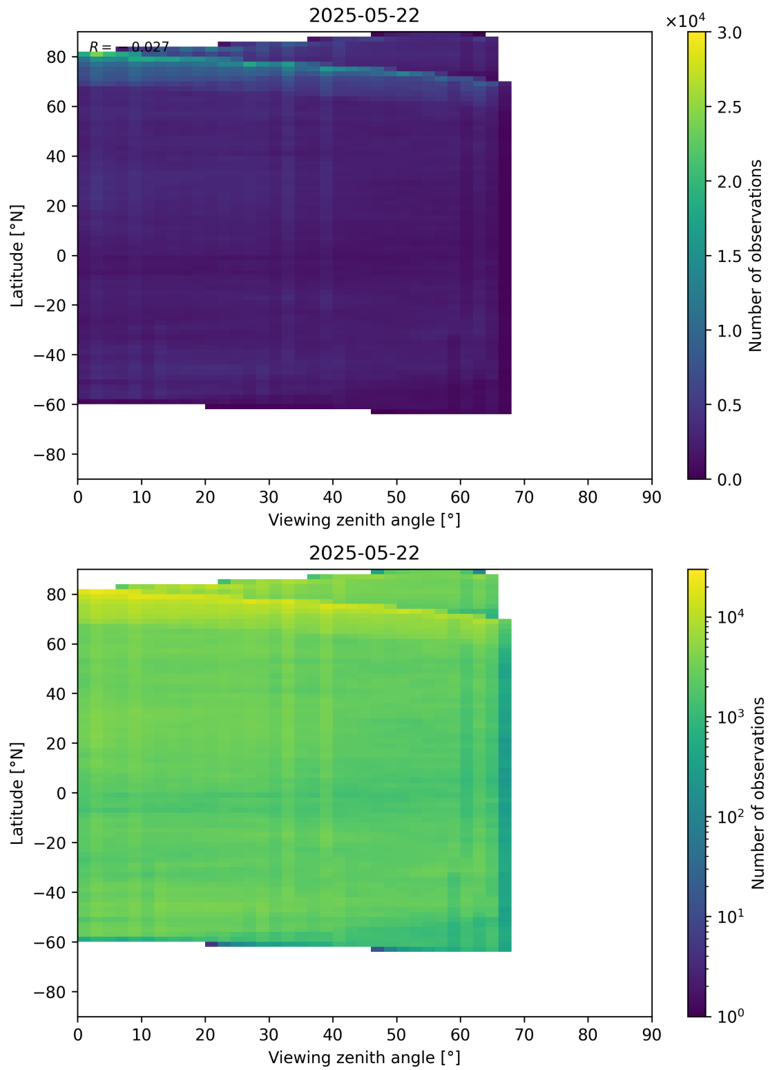
Figure 74: Scatter density plot of “Viewing zenith angle” against “Latitude” for 2025-05-21 to 2025-05-23.
