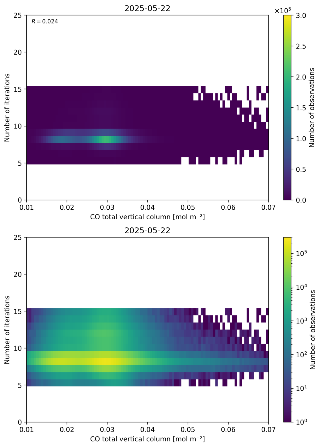
Figure 42: Scatter density plot of “CO total vertical column” against “Number of iterations” for 2025-05-21 to 2025-05-23.
