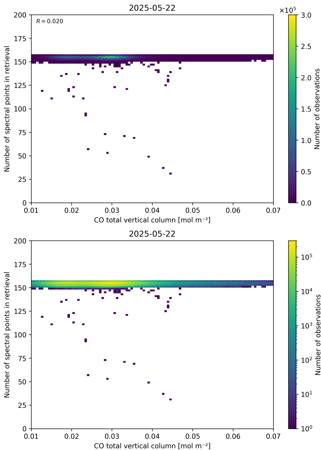
Figure 43: Scatter density plot of “CO total vertical column” against “Number of spectral points in retrieval” for 2025-05-21 to 2025-05-23.
