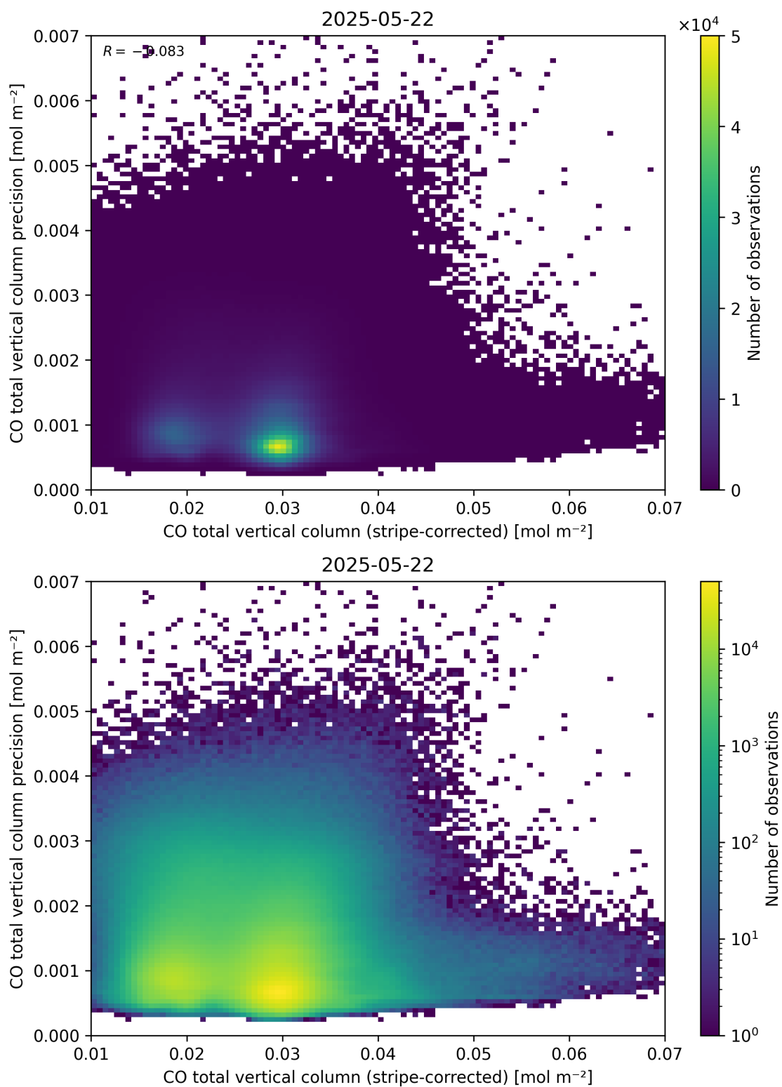
Figure 36: Scatter density plot of “CO total vertical column (stripe-corrected)” against “CO total vertical column precision” for 2025-05-21 to 2025-05-23.
