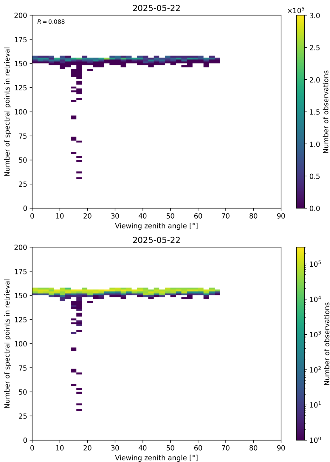
Figure 76: Scatter density plot of “Viewing zenith angle” against “Number of spectral points in retrieval” for 2025-05-21 to 2025-05-23.
