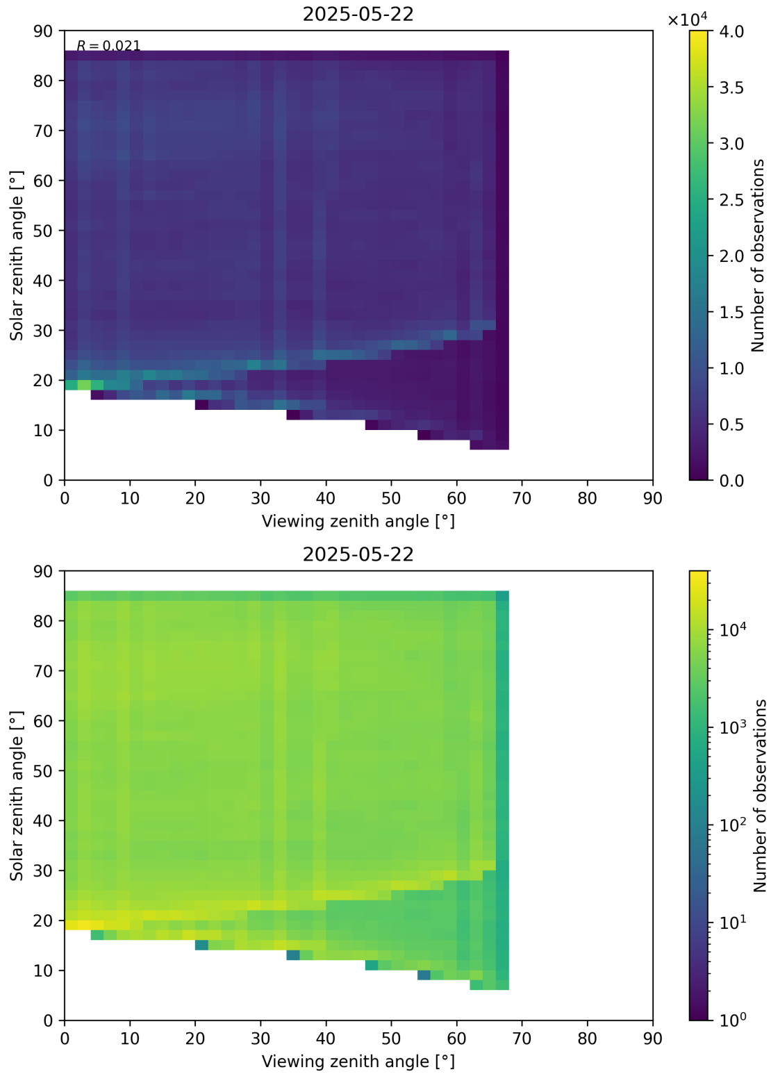
Figure 77: Scatter density plot of “Viewing zenith angle” against “Solar zenith angle” for 2025-05-21 to 2025-05-23.
