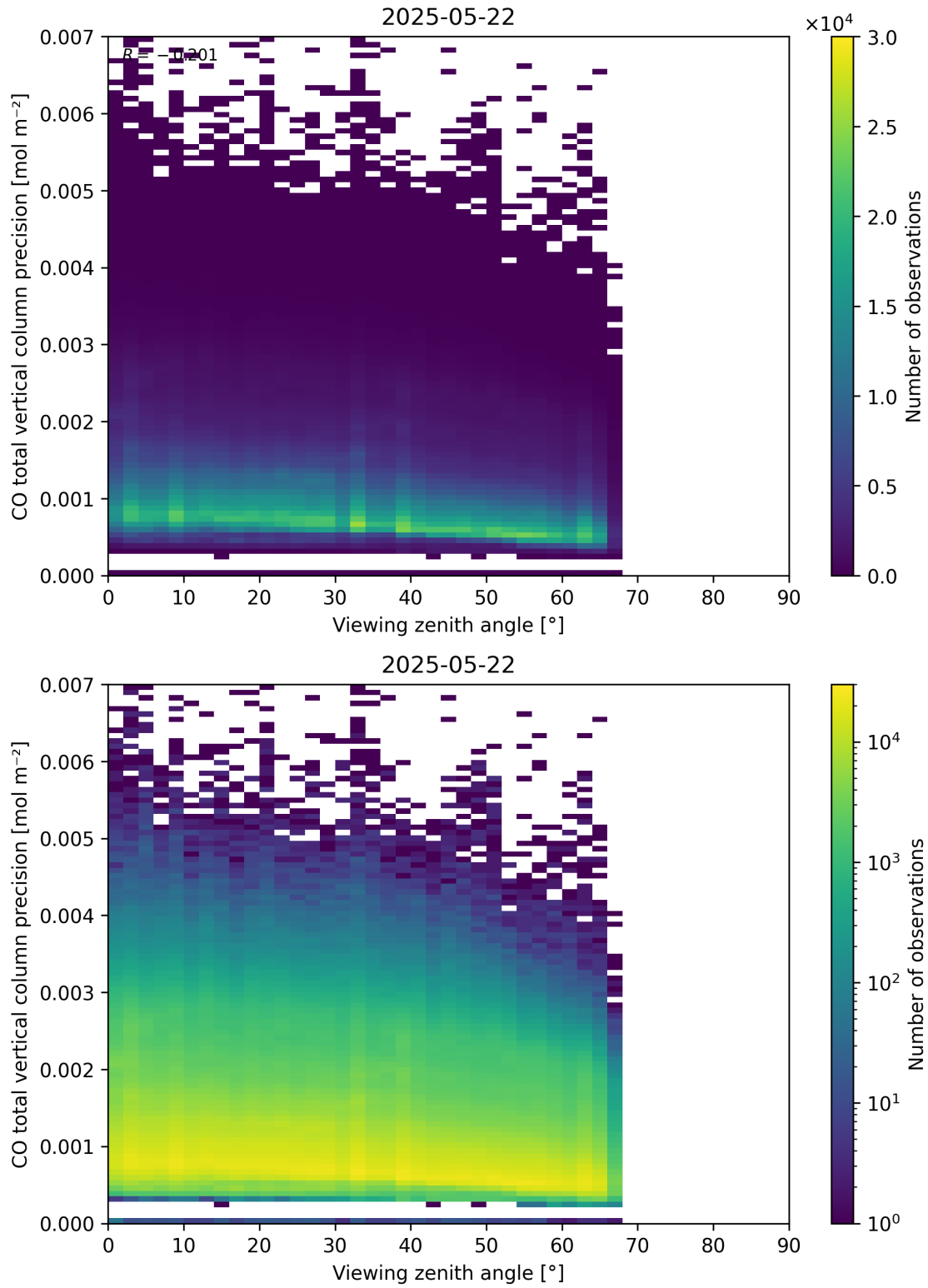
Figure 71: Scatter density plot of “Viewing zenith angle” against “CO total vertical column precision” for 2025-05-21 to 2025-05-23.
