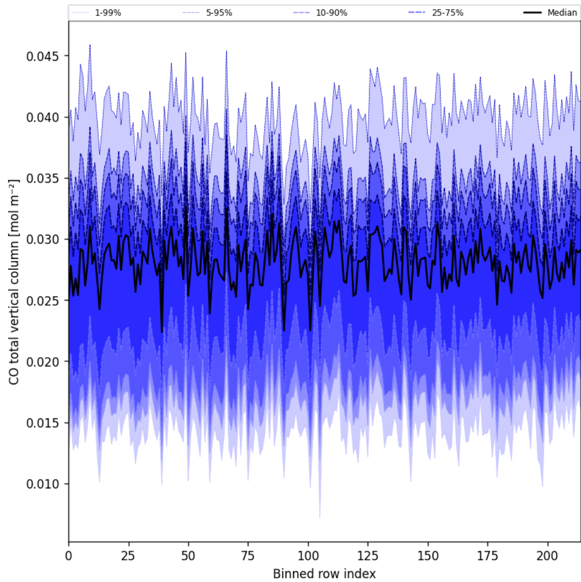
Figure 26: Along track statistics of “CO total vertical column” for 2025-05-21 to 2025-05-23
