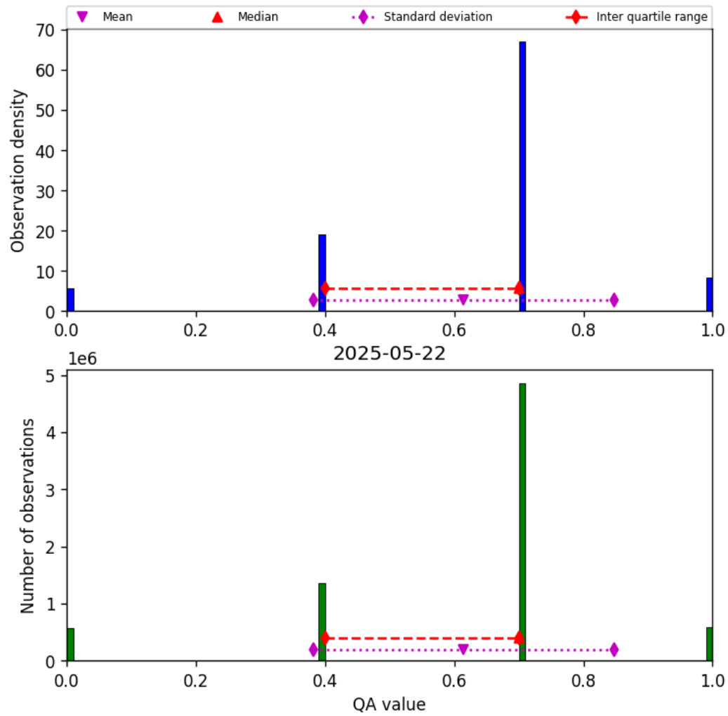
Figure 17: Histogram of “QA value” for 2025-05-21 to 2025-05-23
