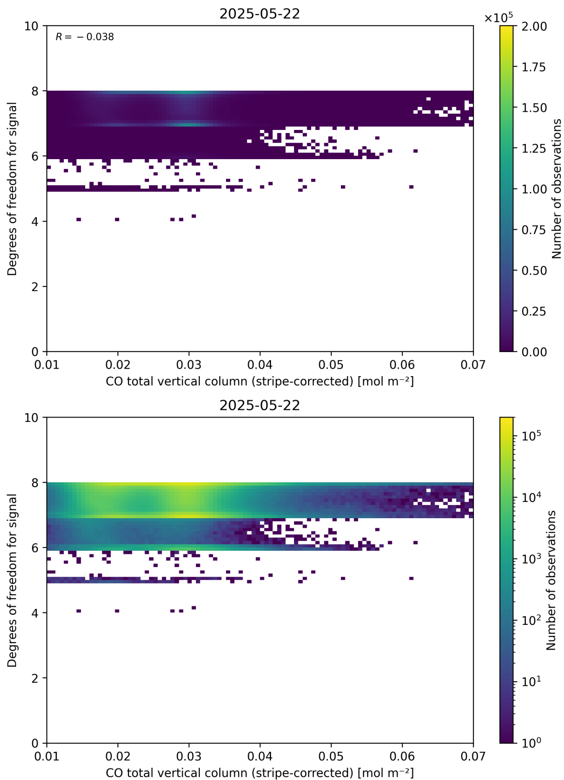
Figure 38: Scatter density plot of “CO total vertical column (stripe-corrected)” against “Degrees of freedom for signal” for 2025-05-21 to 2025-05-23.
