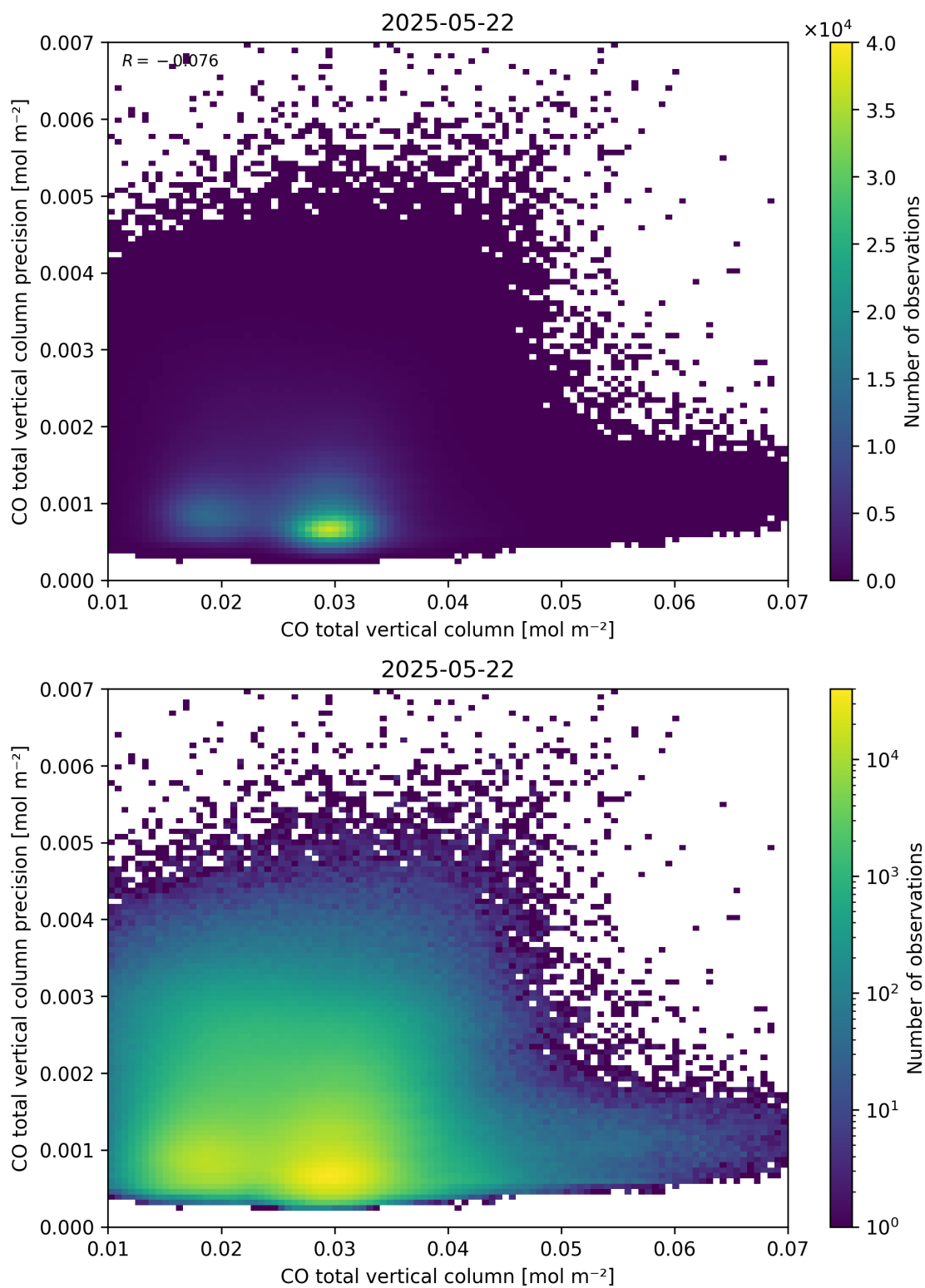
Figure 34: Scatter density plot of “CO total vertical column” against “CO total vertical column precision” for 2025-05-21 to 2025-05-23.
