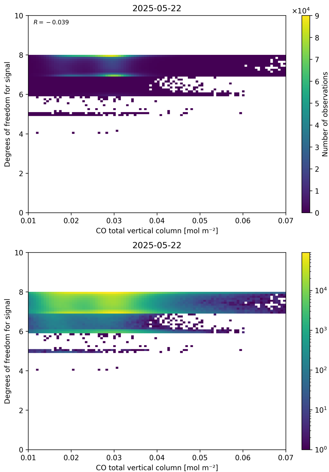
Figure 41: Scatter density plot of “CO total vertical column” against “Degrees of freedom for signal” for 2025-05-21 to 2025-05-23.
