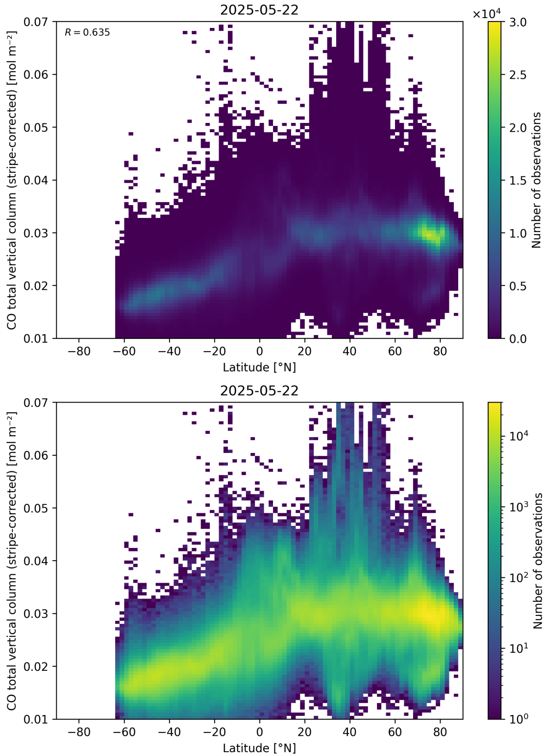
Figure 52: Scatter density plot of “Latitude” against “CO total vertical column (stripe-corrected)” for 2025-05-21 to 2025-05-23.
