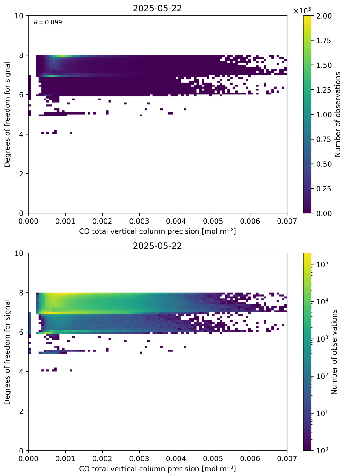
Figure 45: Scatter density plot of “CO total vertical column precision” against “Degrees of freedom for signal” for 2025-05-21 to 2025-05-23.
