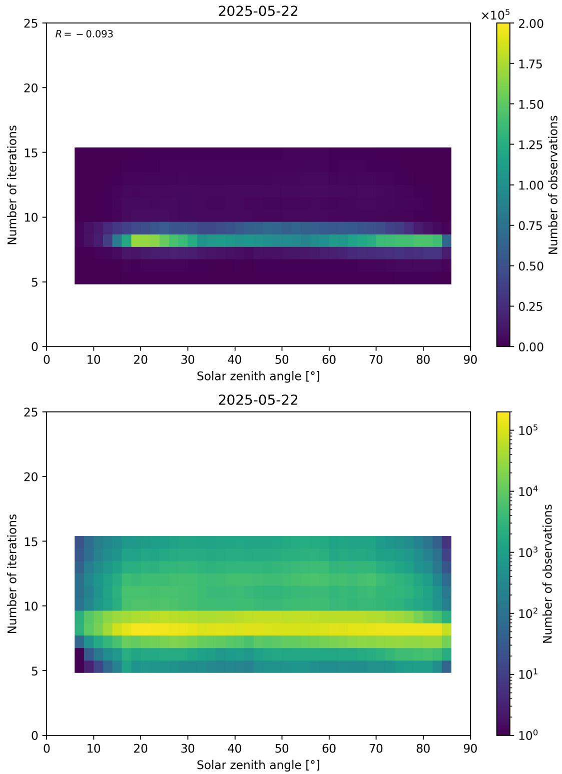
Figure 67: Scatter density plot of “Solar zenith angle” against “Number of iterations” for 2025-05-21 to 2025-05-23.
