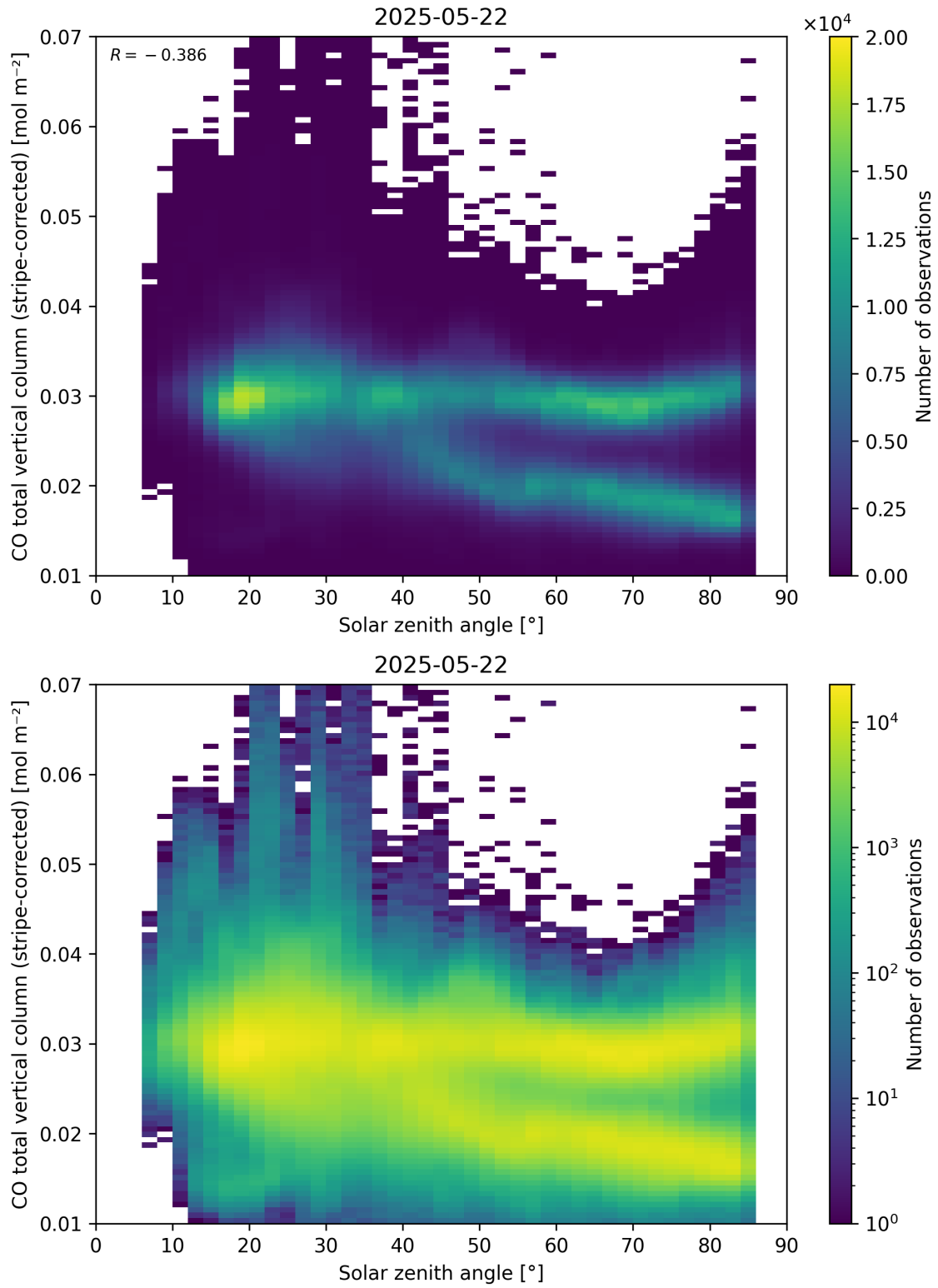
Figure 62: Scatter density plot of “Solar zenith angle” against “CO total vertical column (stripe-corrected)” for 2025-05-21 to 2025-05-23.
