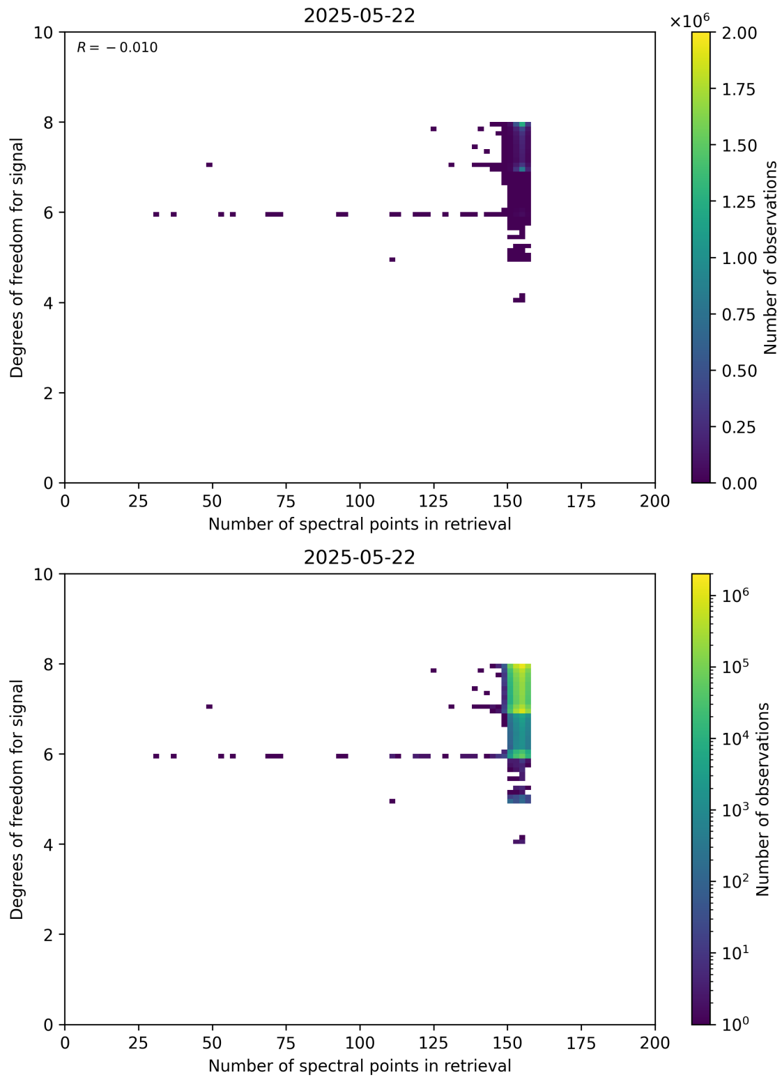
Figure 59: Scatter density plot of “Number of spectral points in retrieval” against “Degrees of freedom for signal” for 2025-05-21 to 2025-05-23.
