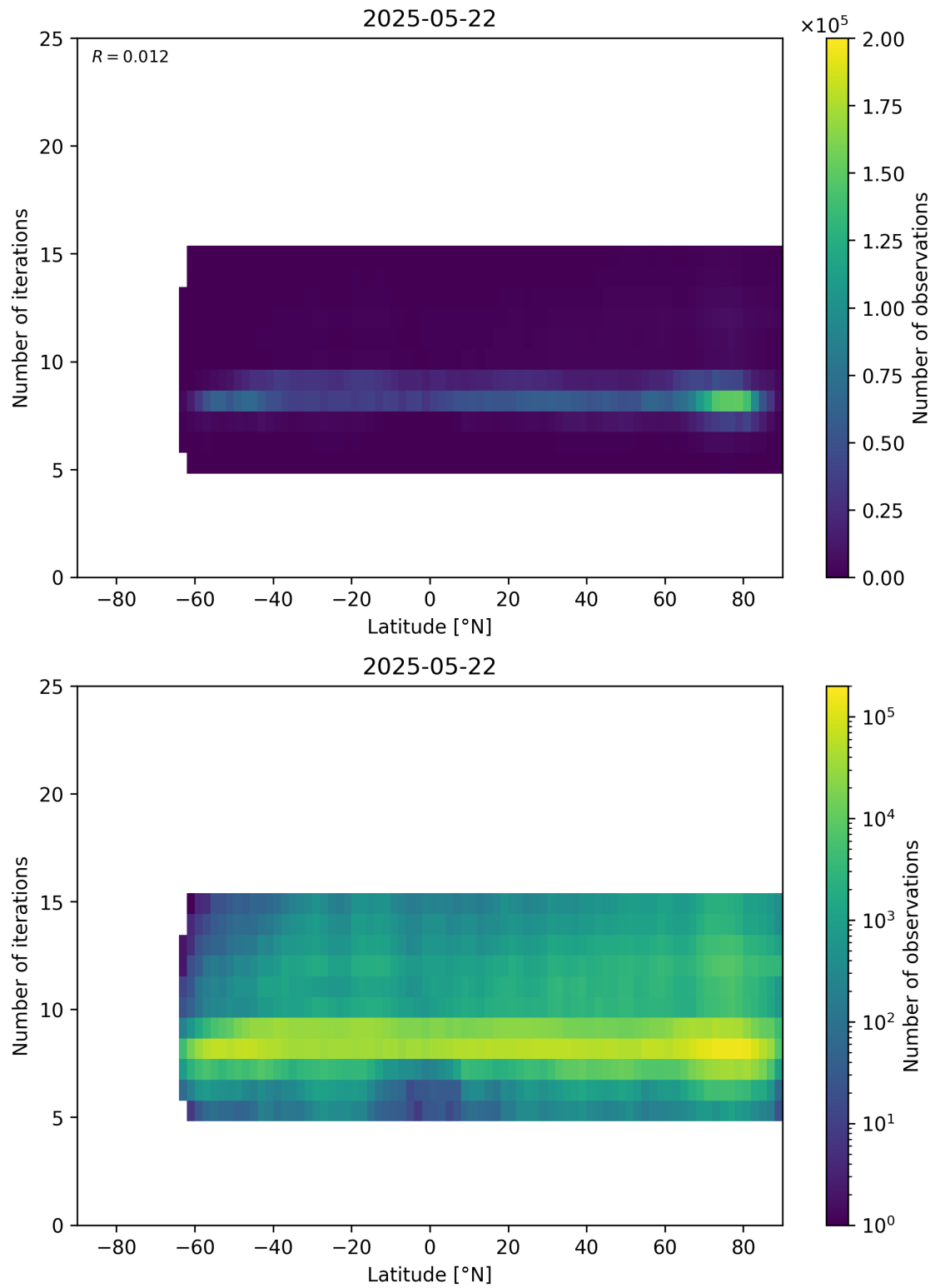
Figure 56: Scatter density plot of “Latitude” against “Number of iterations” for 2025-05-21 to 2025-05-23.
