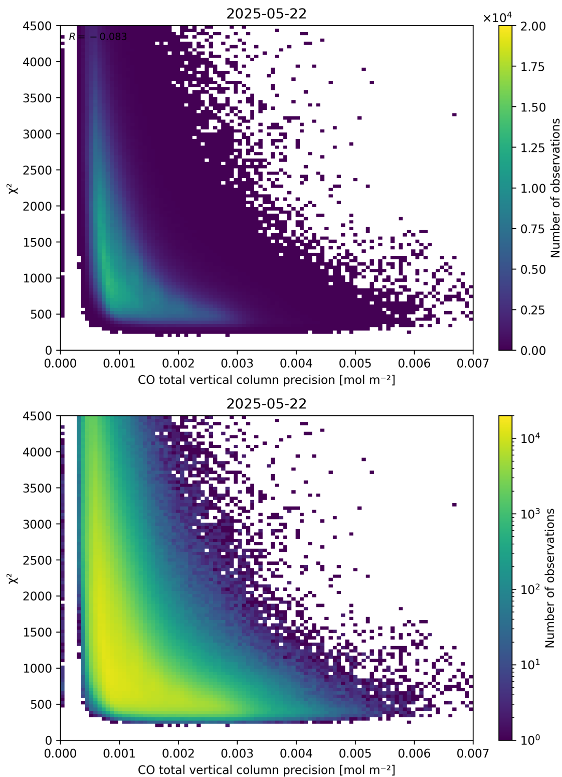
Figure 44: Scatter density plot of “CO total vertical column precision” against “ \chi^2 ” for 2025-05-21 to 2025-05-23.
