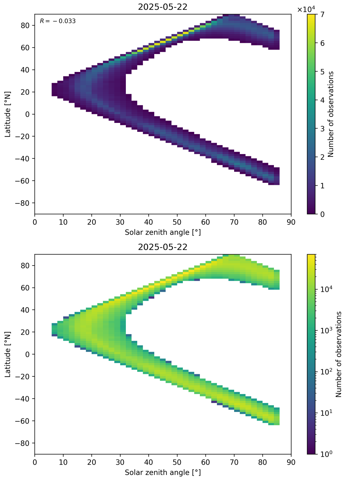
Figure 66: Scatter density plot of “Solar zenith angle” against “Latitude” for 2025-05-21 to 2025-05-23.
