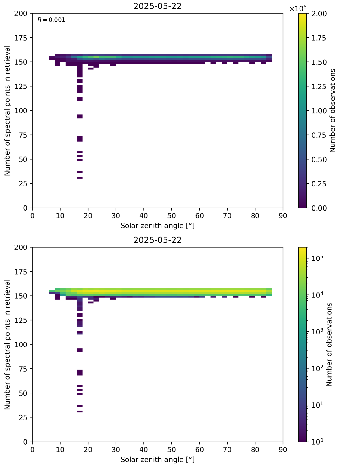
Figure 68: Scatter density plot of “Solar zenith angle” against “Number of spectral points in retrieval” for 2025-05-21 to 2025-05-23.
