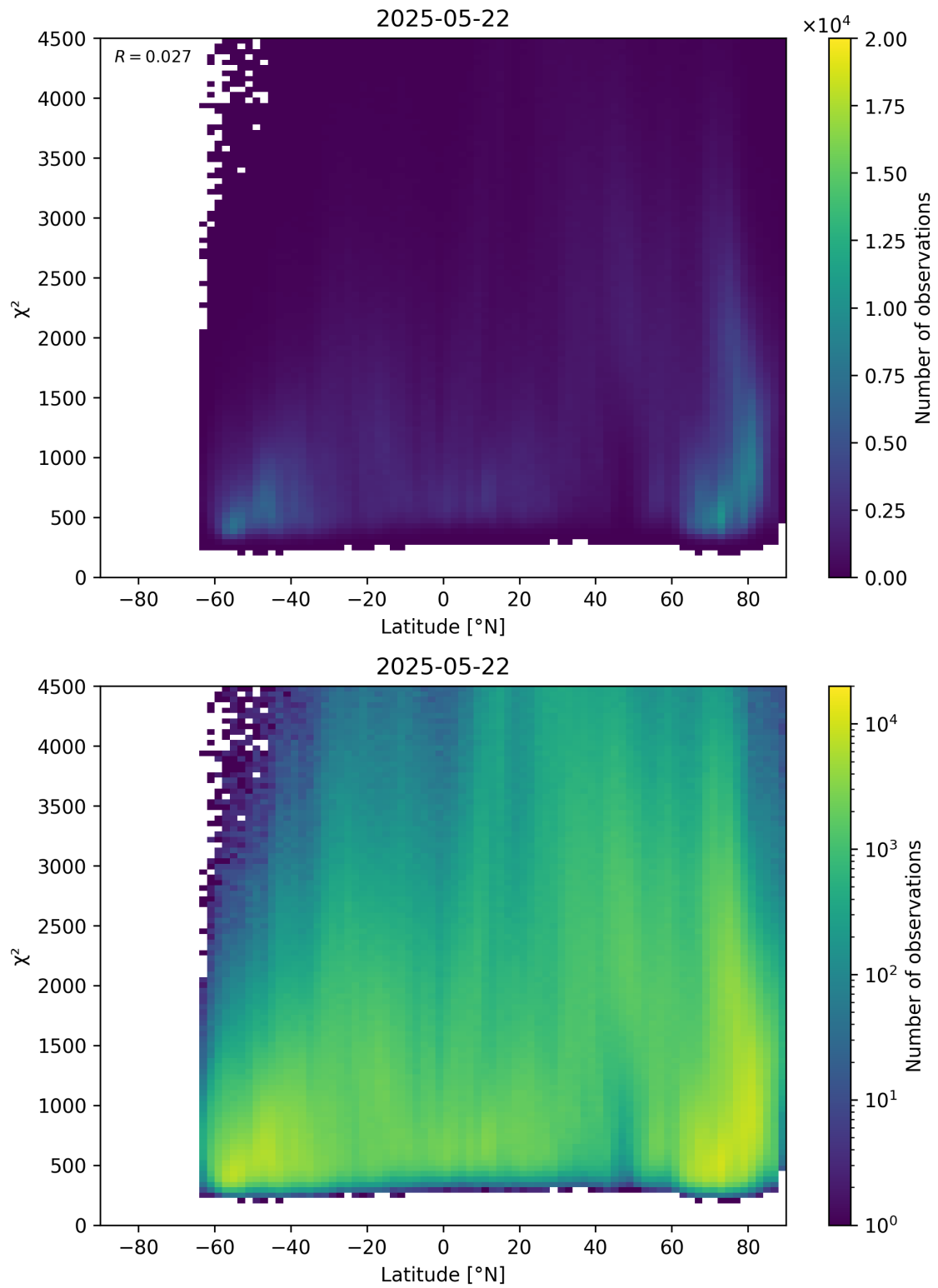
Figure 54: Scatter density plot of “Latitude” against “ \chi^2 ” for 2025-05-21 to 2025-05-23.
