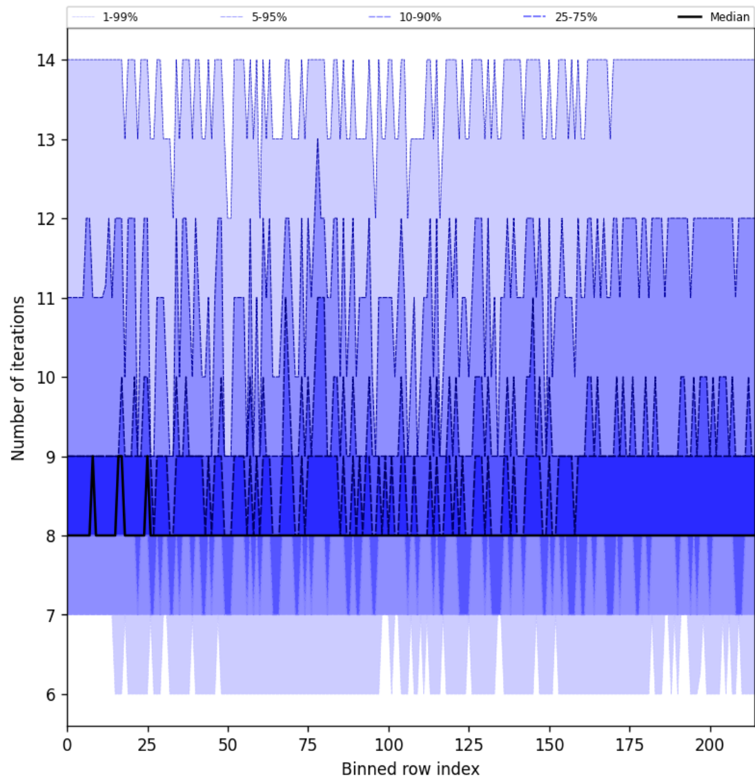
Figure 32: Along track statistics of “Number of iterations” for 2025-05-21 to 2025-05-23
