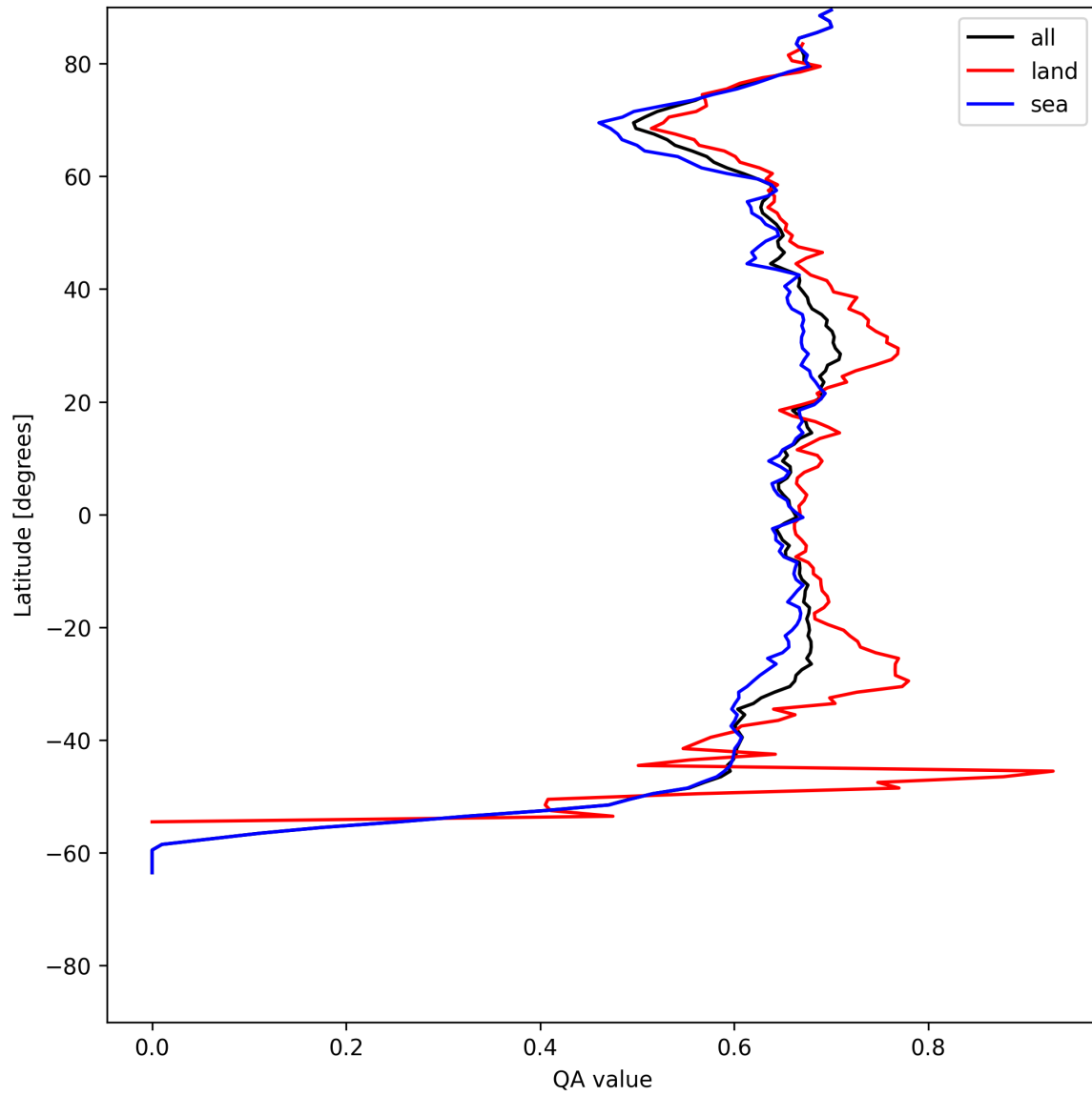
Figure 9: Zonal average of “QA value” for 2025-05-21 to 2025-05-23.
