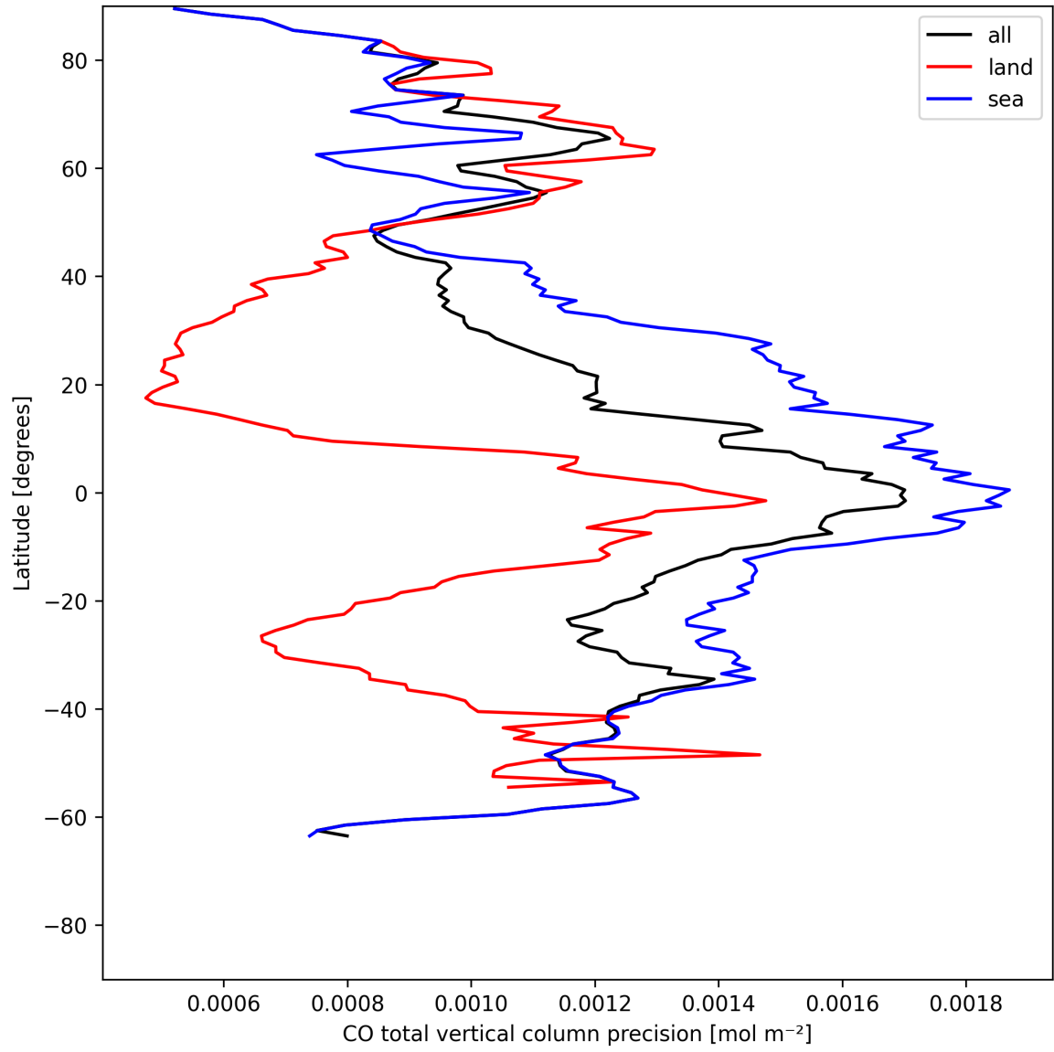
Figure 12: Zonal average of “CO total vertical column precision” for 2025-05-21 to 2025-05-23.
