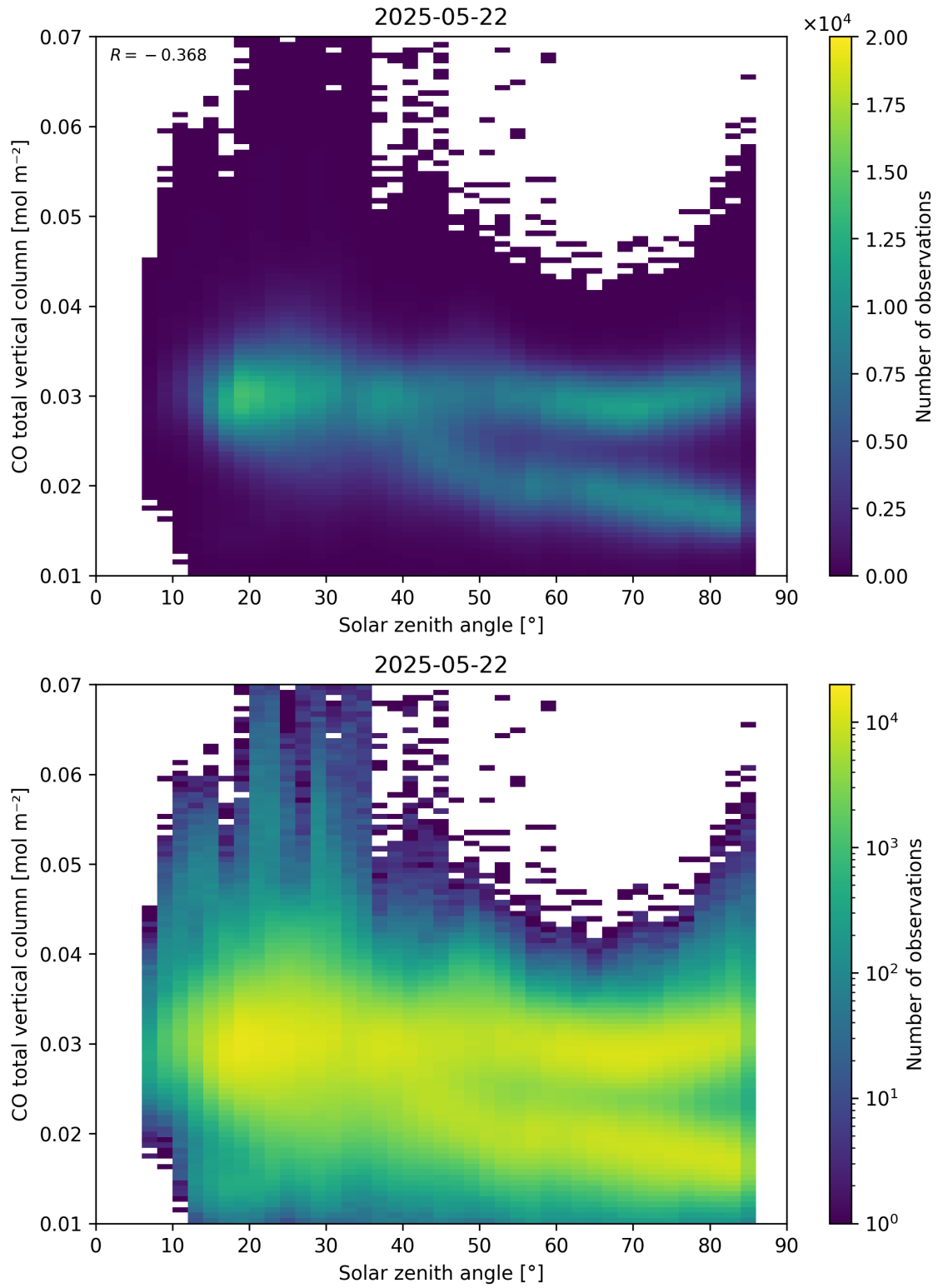
Figure 61: Scatter density plot of “Solar zenith angle” against “CO total vertical column” for 2025-05-21 to 2025-05-23.
