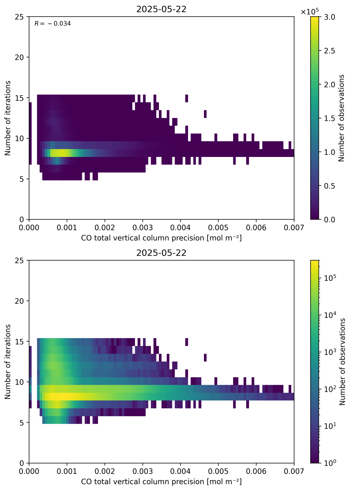
Figure 46: Scatter density plot of “CO total vertical column precision” against “Number of iterations” for 2025-05-21 to 2025-05-23.
