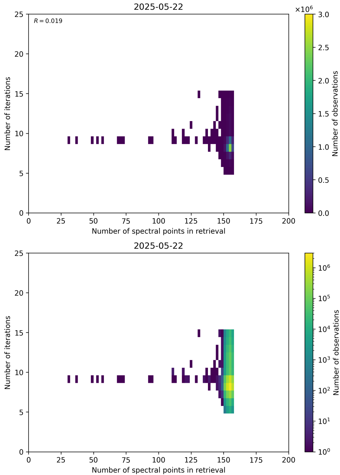
Figure 60: Scatter density plot of “Number of spectral points in retrieval” against “Number of iterations” for 2025-05-21 to 2025-05-23.
