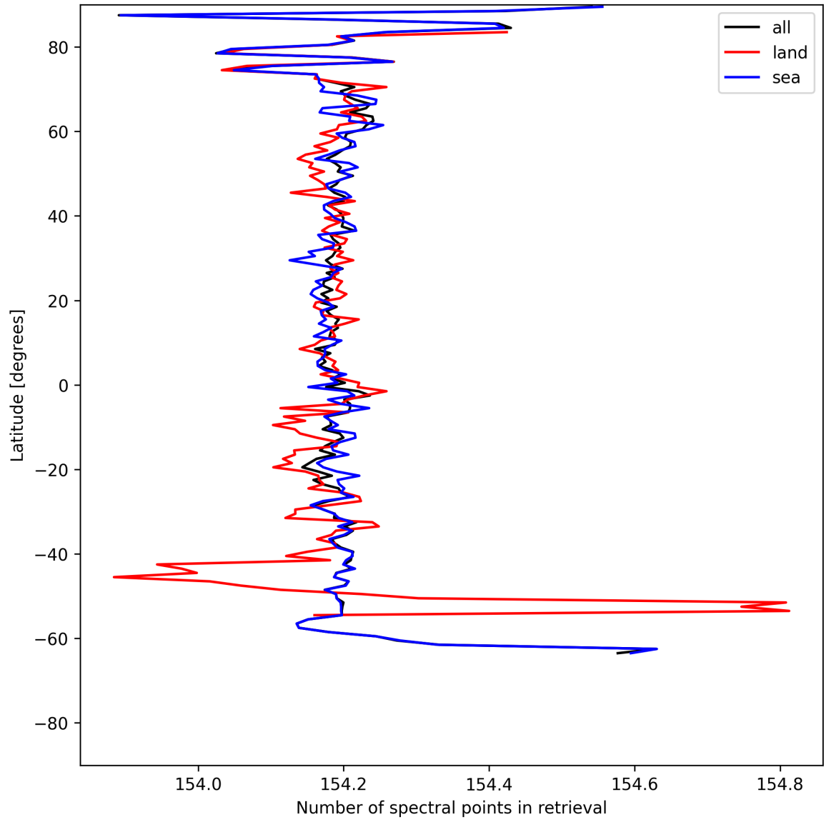
Figure 13: Zonal average of “Number of spectral points in retrieval” for 2025-05-21 to 2025-05-23.
