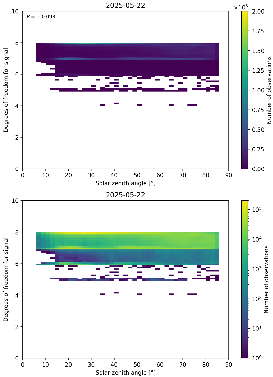
Figure 65: Scatter density plot of “Solar zenith angle” against “Degrees of freedom for signal” for 2025-05-21 to 2025-05-23.
