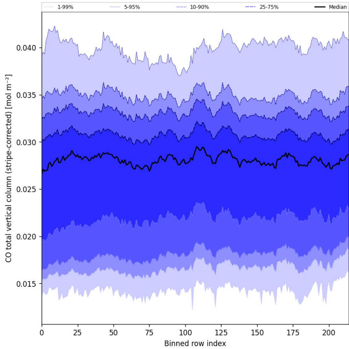
Figure 27: Along track statistics of “CO total vertical column (stripe-corrected)” for 2025-05-21 to 2025-05-23
