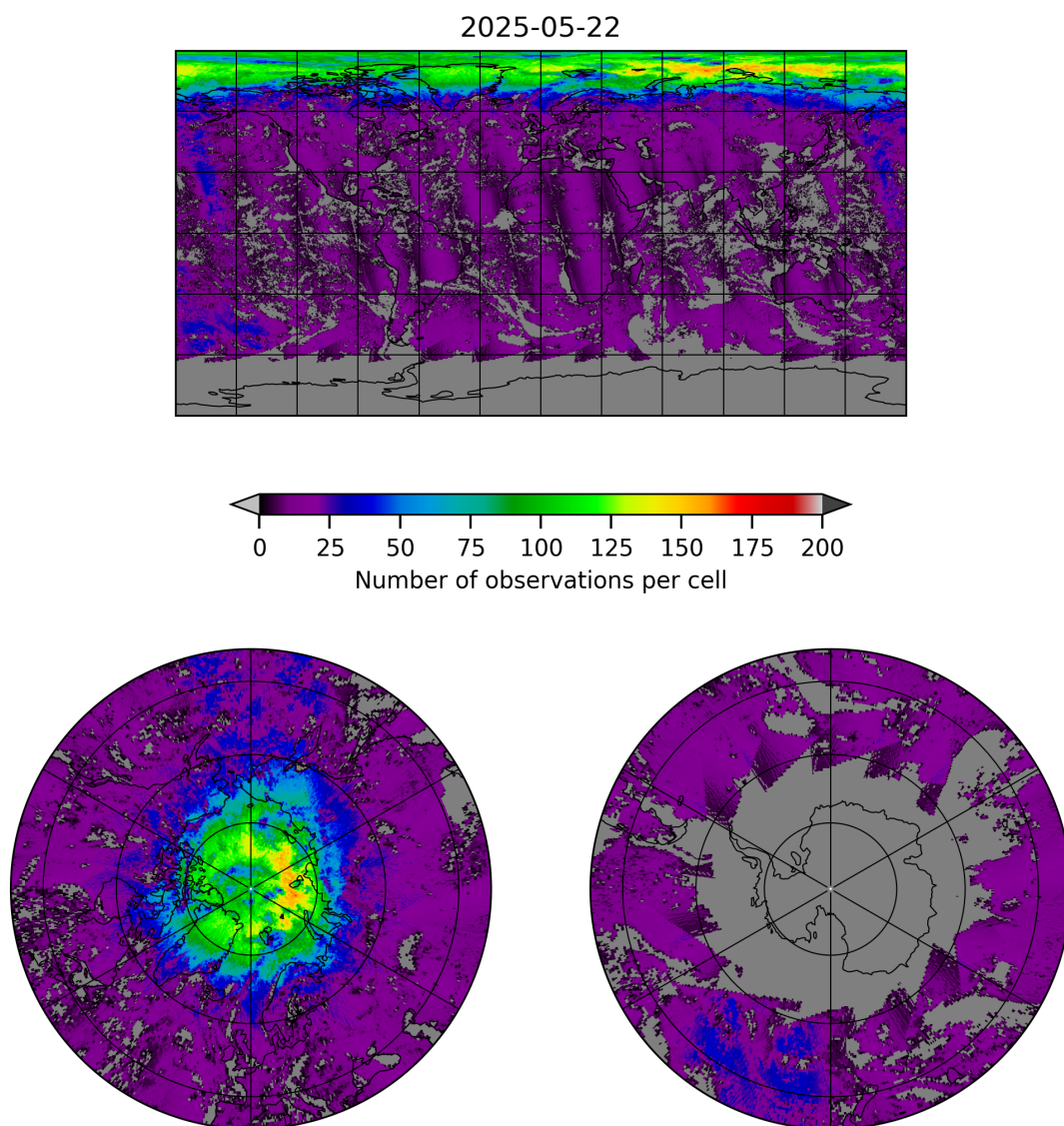
Figure 8: Map of the number of observations for 2025-05-21 to 2025-05-23
