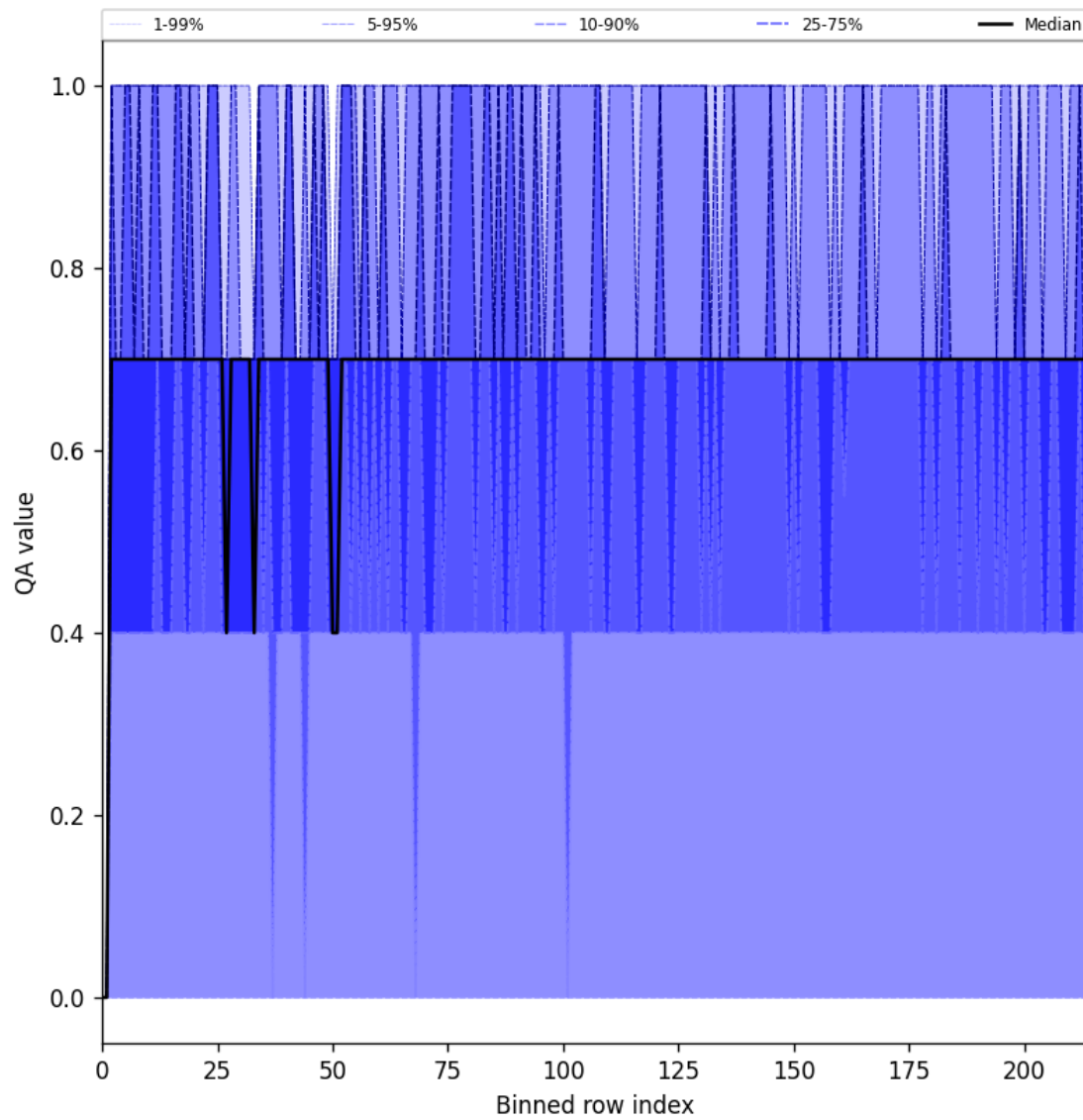
Figure 25: Along track statistics of “QA value” for 2025-05-21 to 2025-05-23
