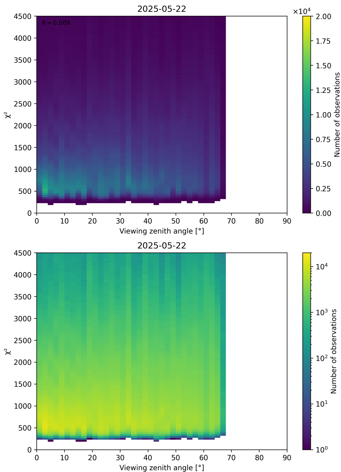
Figure 72: Scatter density plot of “Viewing zenith angle” against “ \chi^2 ” for 2025-05-21 to 2025-05-23.
