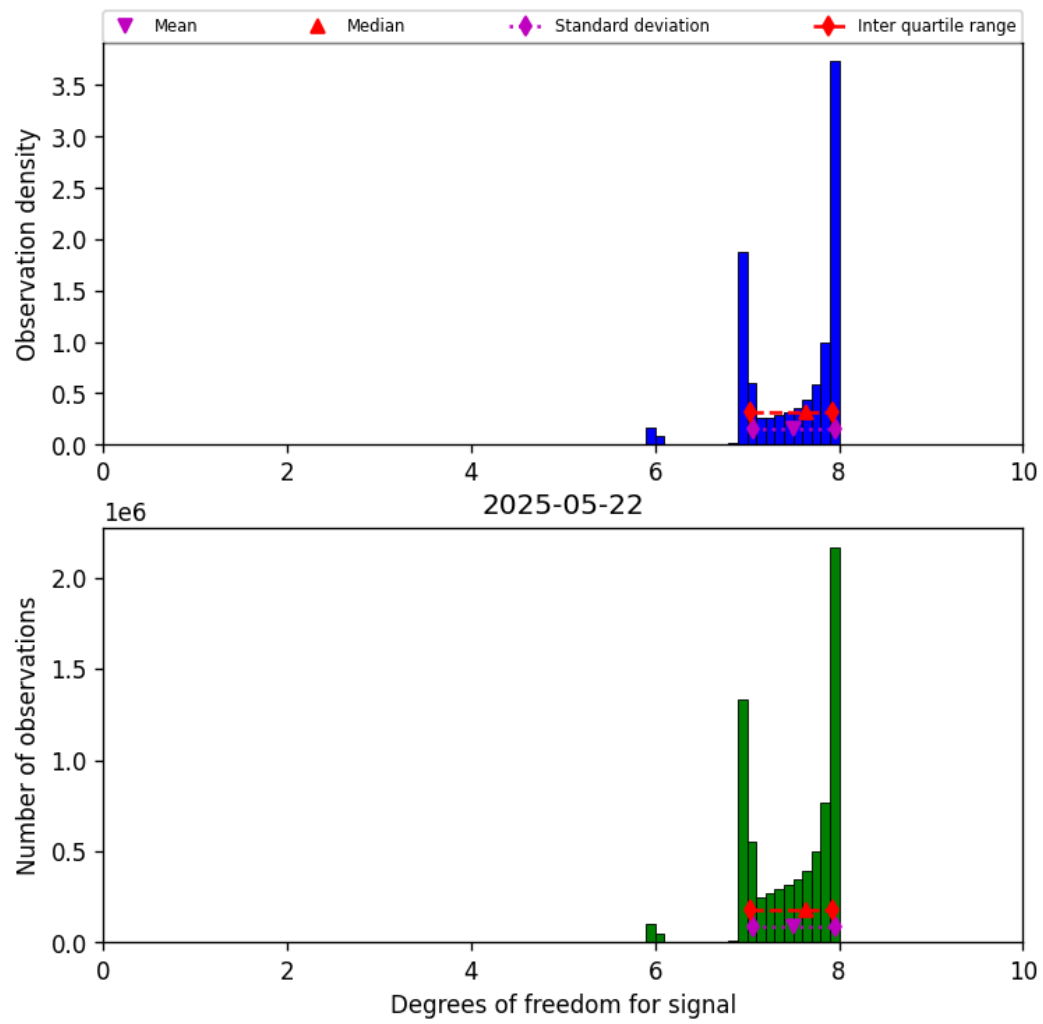
Figure 23: Histogram of “Degrees of freedom for signal” for 2025-05-21 to 2025-05-23
