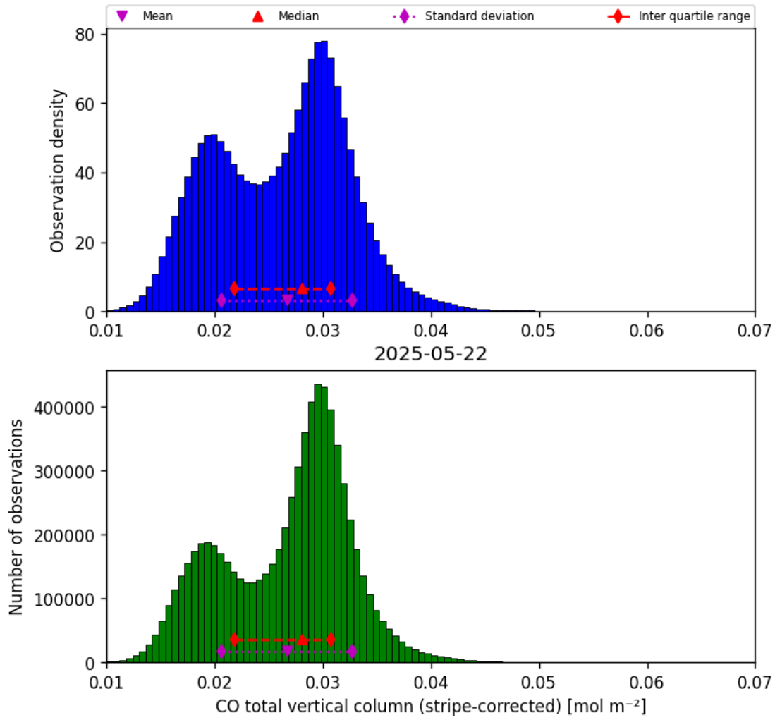
Figure 19: Histogram of “CO total vertical column (stripe-corrected)” for 2025-05-21 to 2025-05-23
