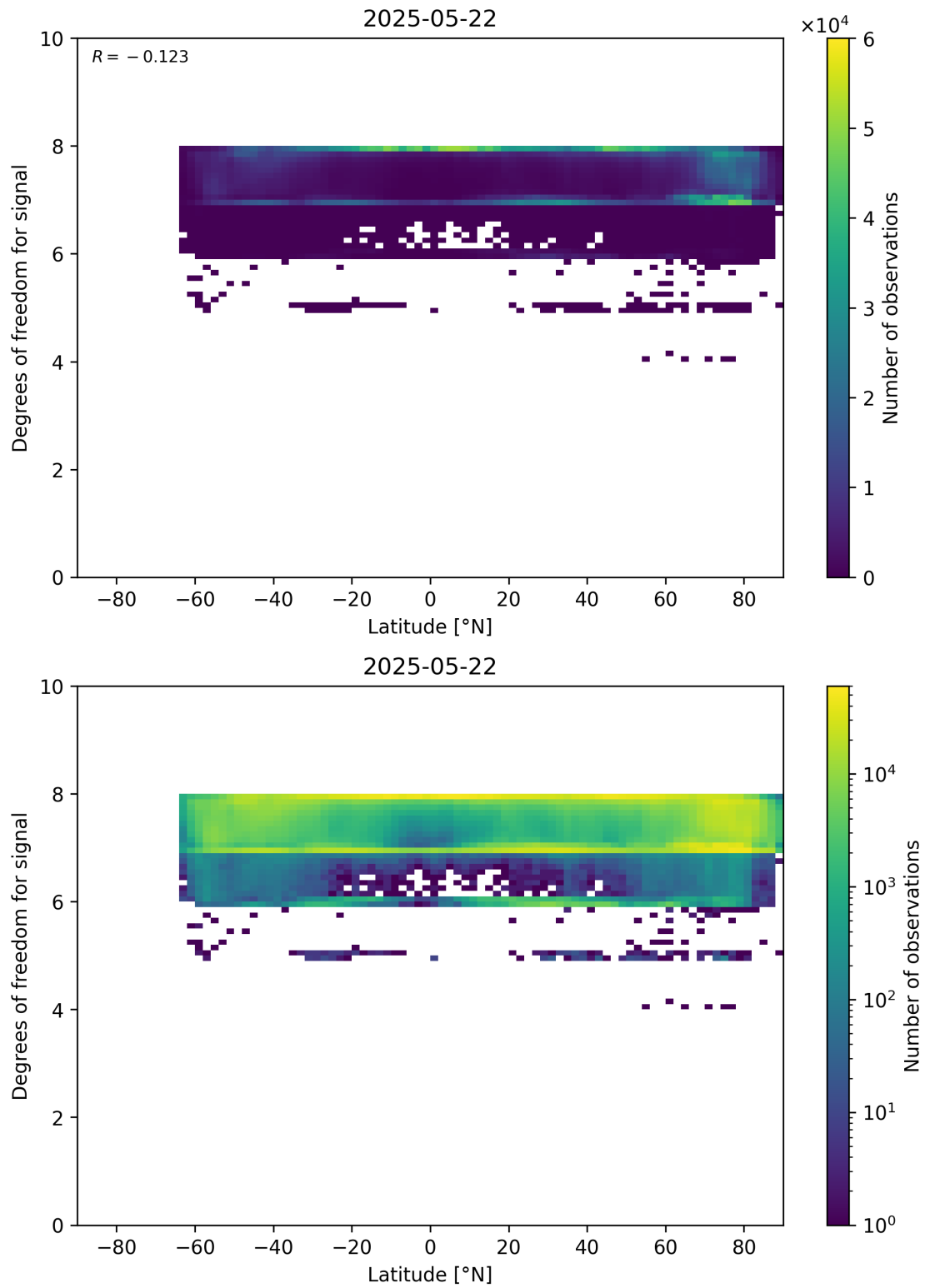
Figure 55: Scatter density plot of “Latitude” against “Degrees of freedom for signal” for 2025-05-21 to 2025-05-23.
