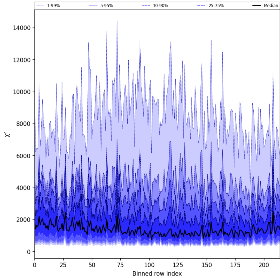
Figure 30: Along track statistics of “ \chi^2 ” for 2025-05-21 to 2025-05-23
