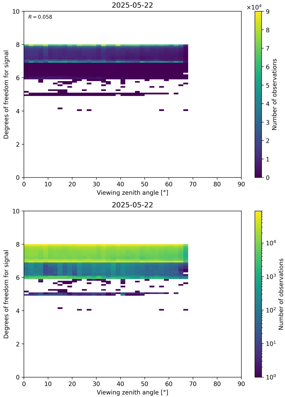
Figure 73: Scatter density plot of “Viewing zenith angle” against “Degrees of freedom for signal” for 2025-05-21 to 2025-05-23.
