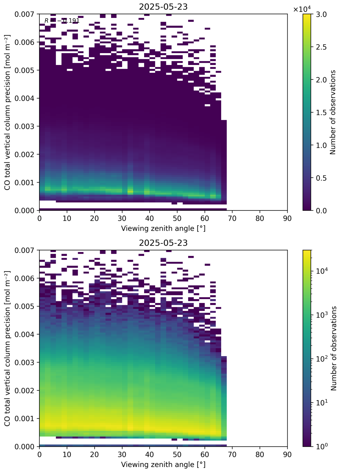
Figure 71: Scatter density plot of “Viewing zenith angle” against “CO total vertical column precision” for 2025-05-22 to 2025-05-24.
