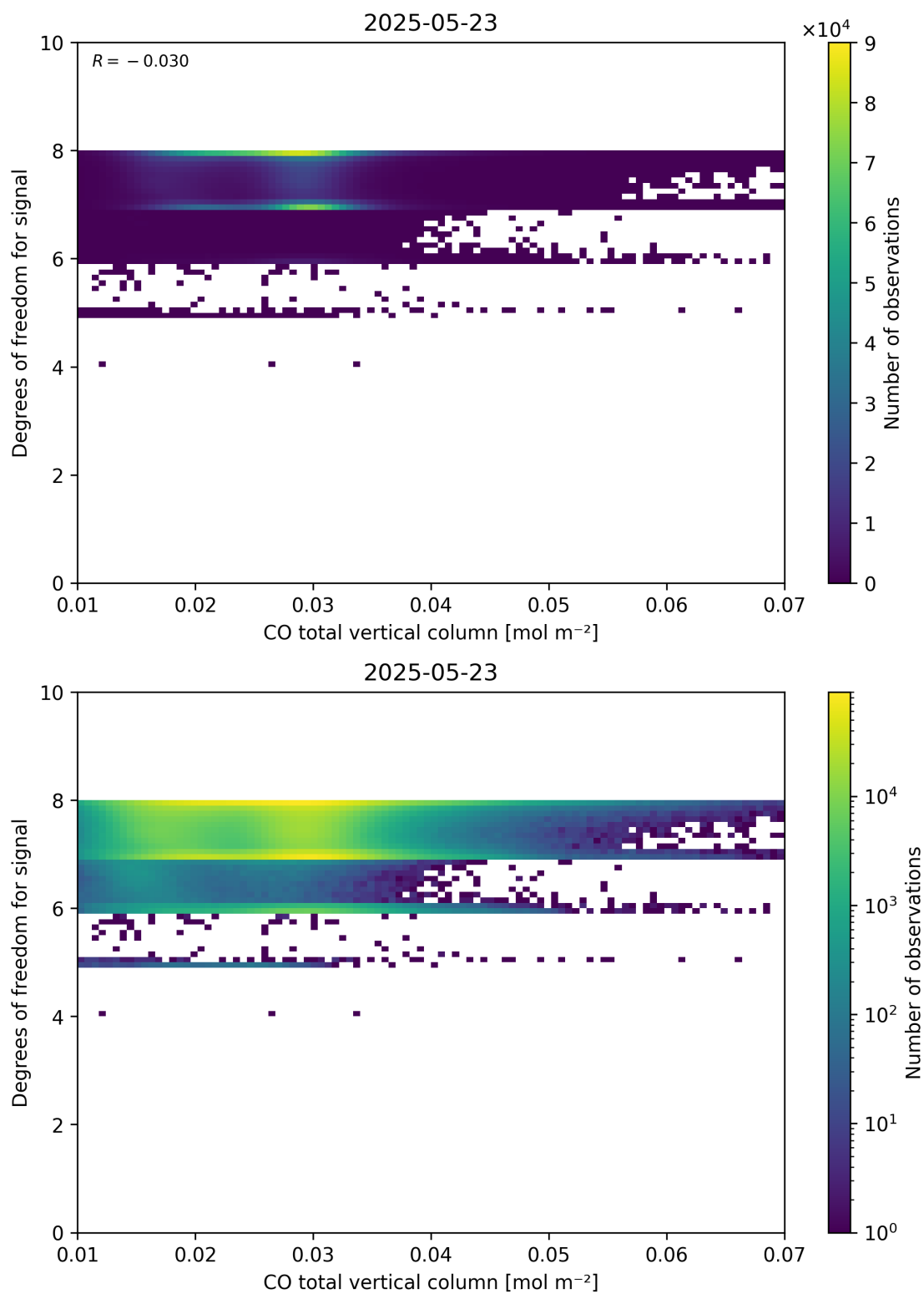
Figure 41: Scatter density plot of “CO total vertical column” against “Degrees of freedom for signal” for 2025-05-22 to 2025-05-24.
