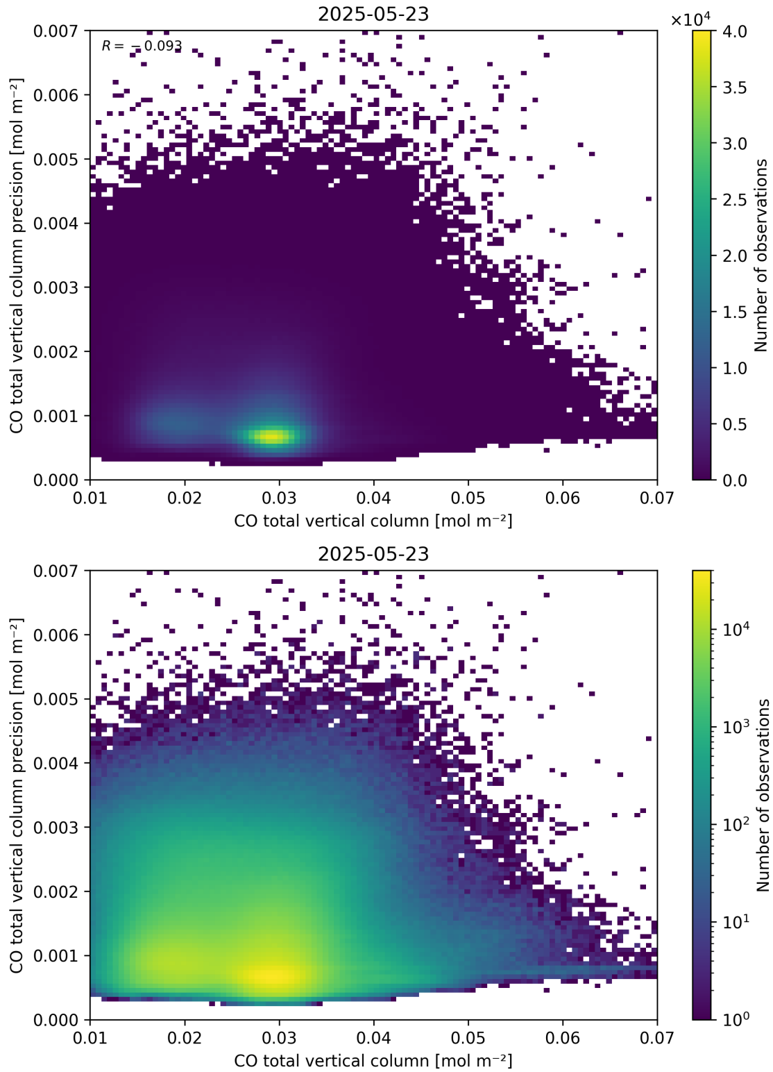
Figure 34: Scatter density plot of “CO total vertical column” against “CO total vertical column precision” for 2025-05-22 to 2025-05-24.
