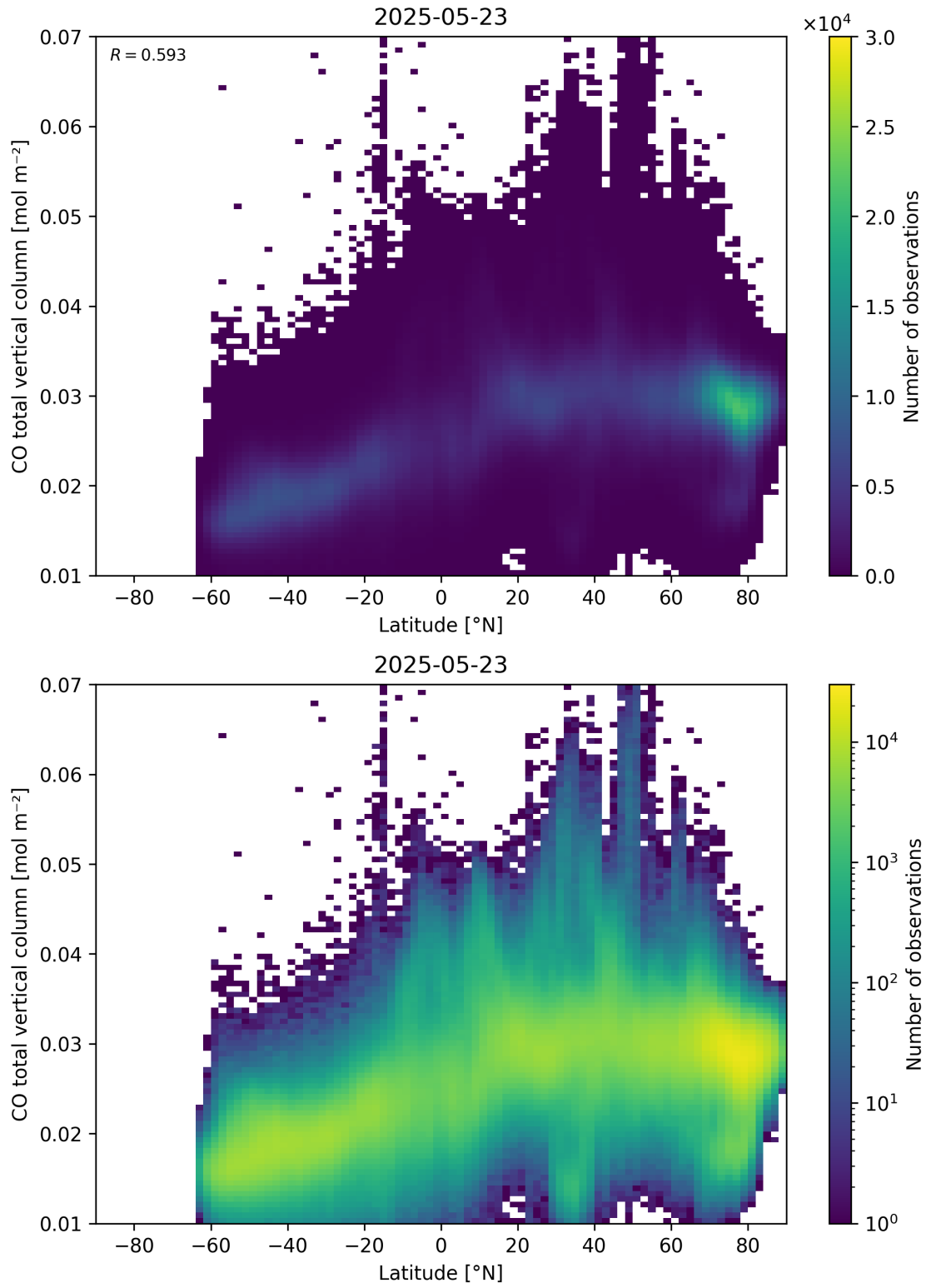
Figure 51: Scatter density plot of “Latitude” against “CO total vertical column” for 2025-05-22 to 2025-05-24.
