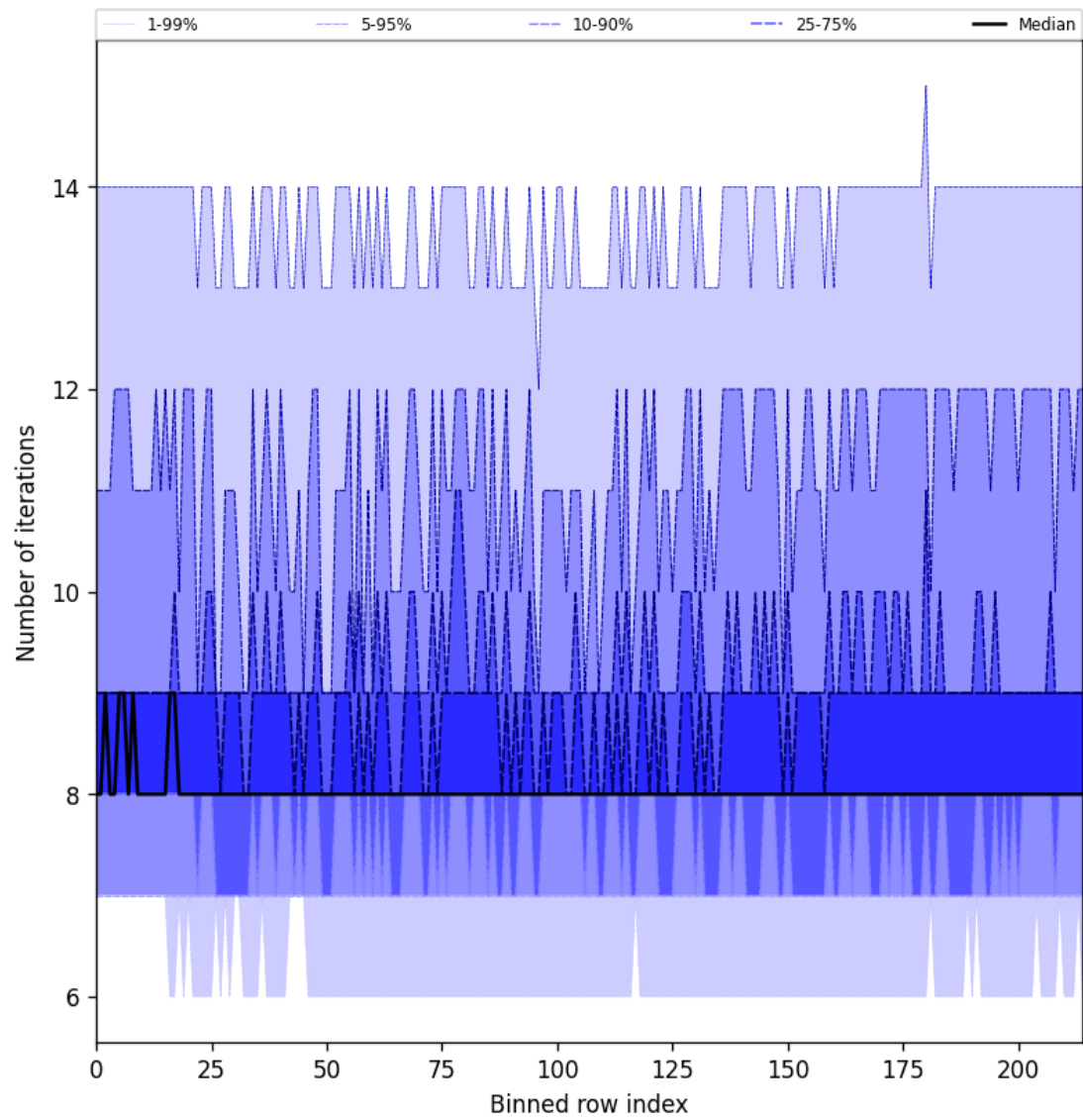
Figure 32: Along track statistics of “Number of iterations” for 2025-05-22 to 2025-05-24
