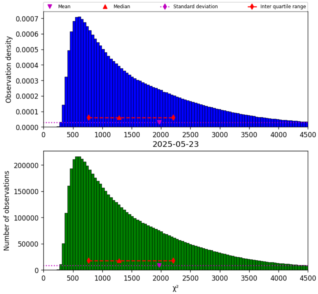
Figure 22: Histogram of " \chi^2 " for 2025-05-22 to 2025-05-24
