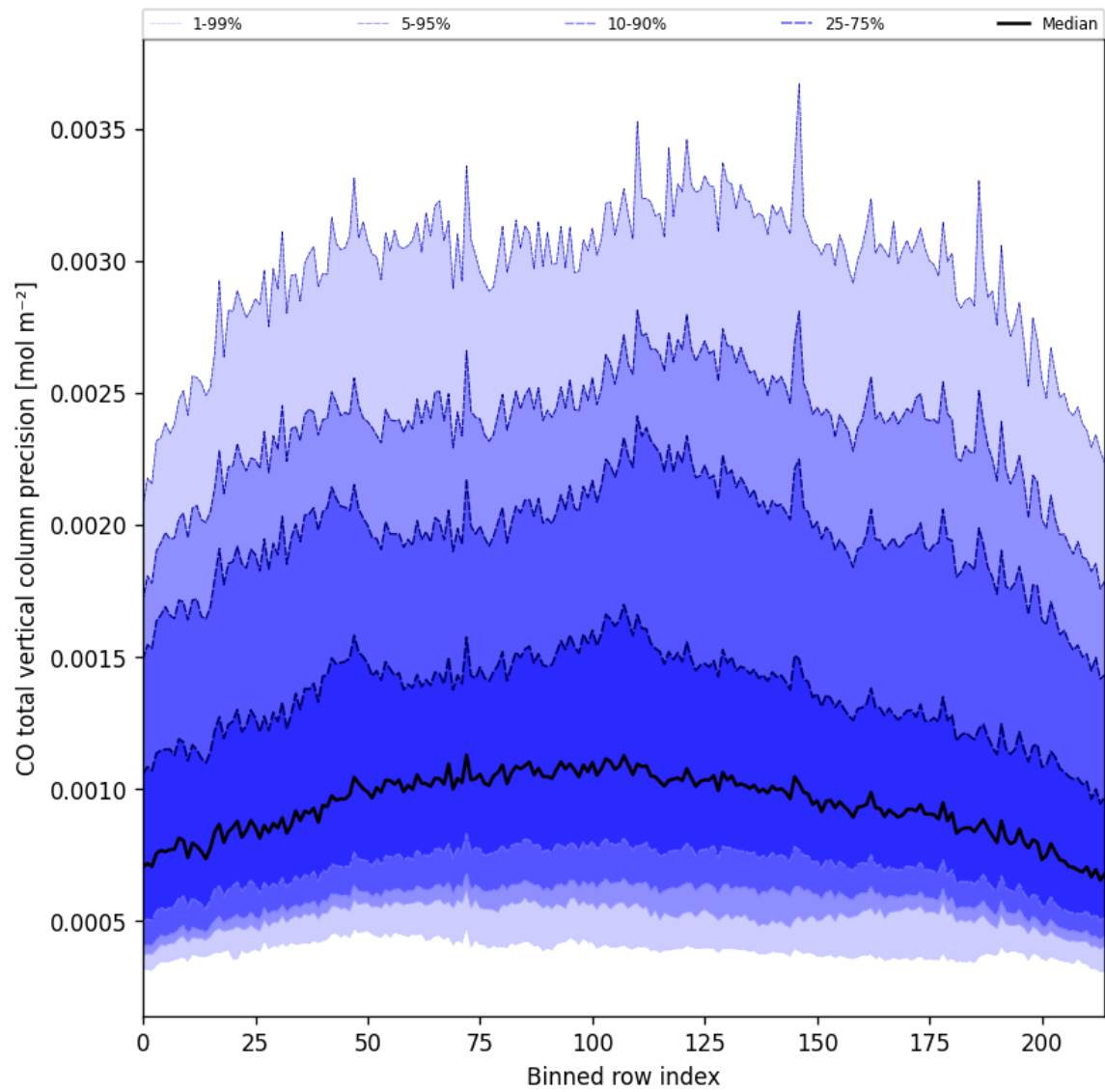
Figure 28: Along track statistics of “CO total vertical column precision” for 2025-05-22 to 2025-05-24
