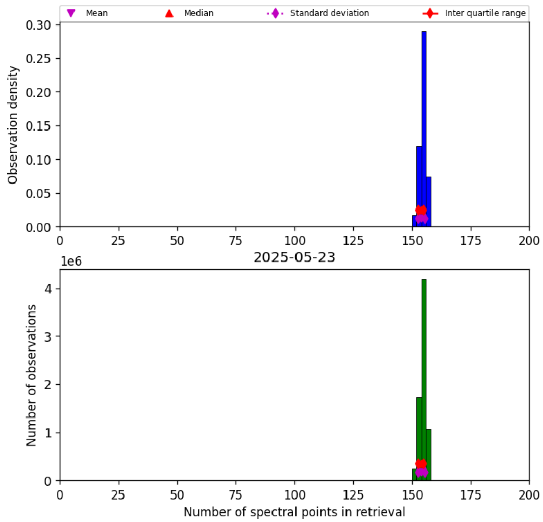
Figure 21: Histogram of “Number of spectral points in retrieval” for 2025-05-22 to 2025-05-24
