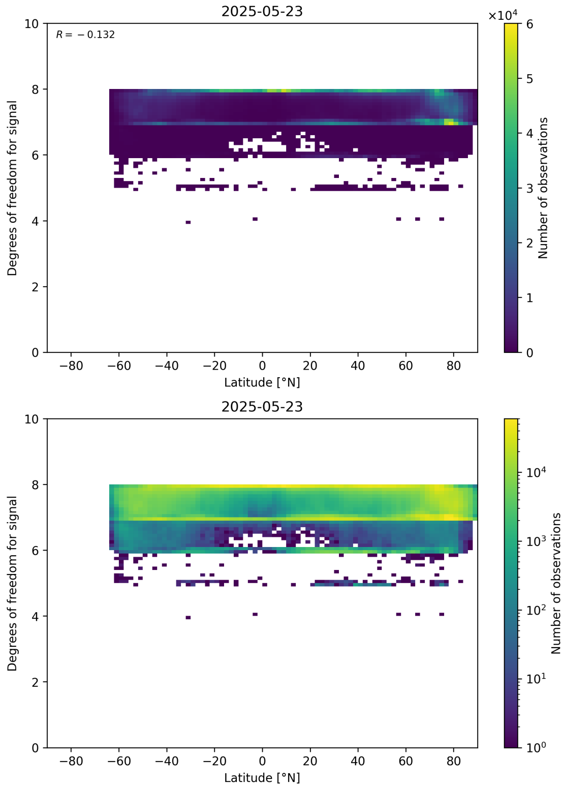
Figure 55: Scatter density plot of “Latitude” against “Degrees of freedom for signal” for 2025-05-22 to 2025-05-24.
