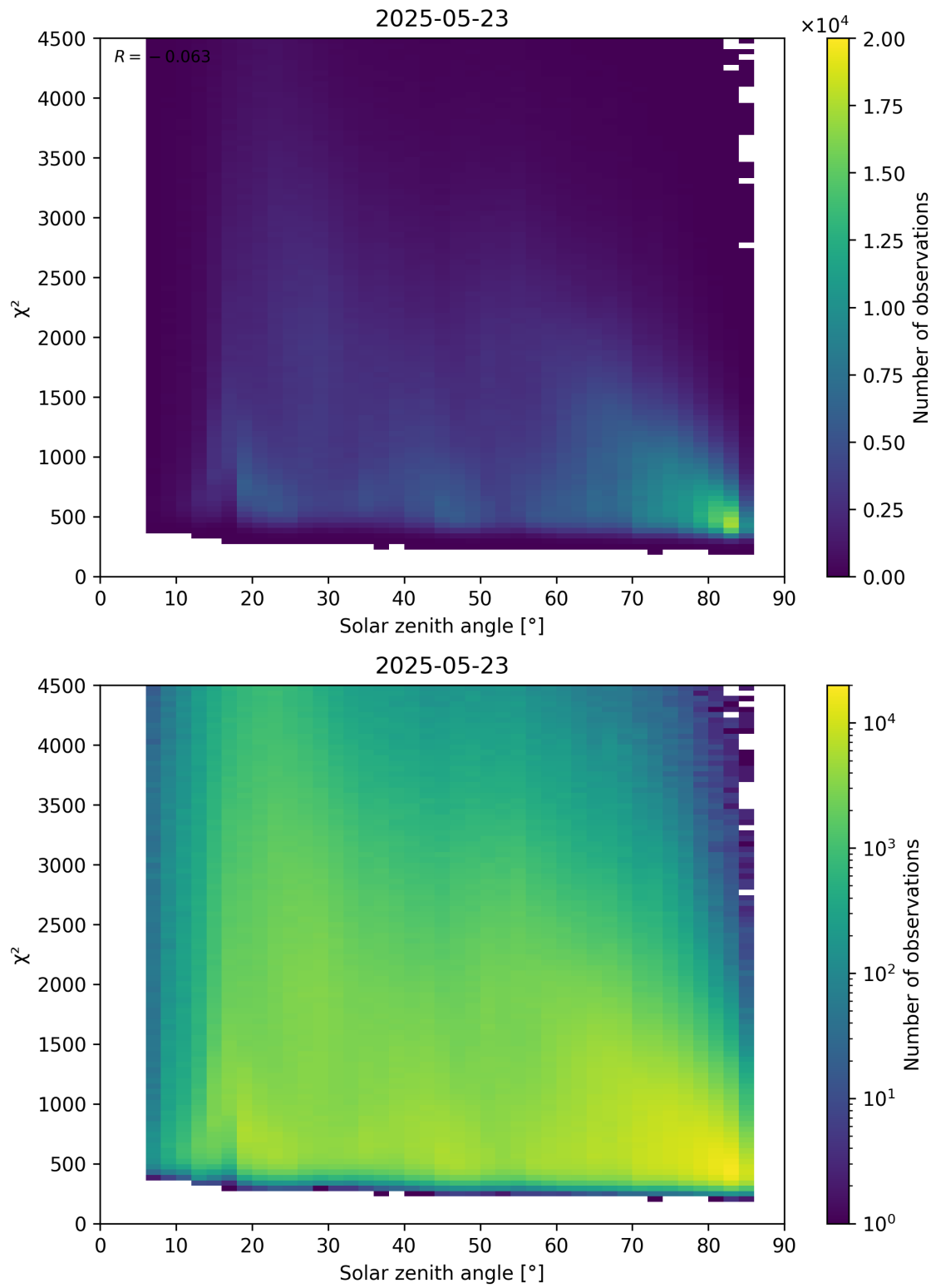
Figure 64: Scatter density plot of “Solar zenith angle” against “ \chi^2 ” for 2025-05-22 to 2025-05-24.
