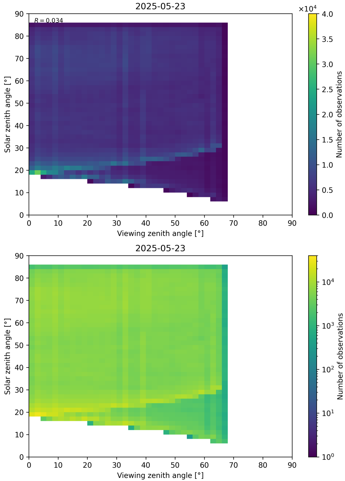
Figure 77: Scatter density plot of “Viewing zenith angle” against “Solar zenith angle” for 2025-05-22 to 2025-05-24.
