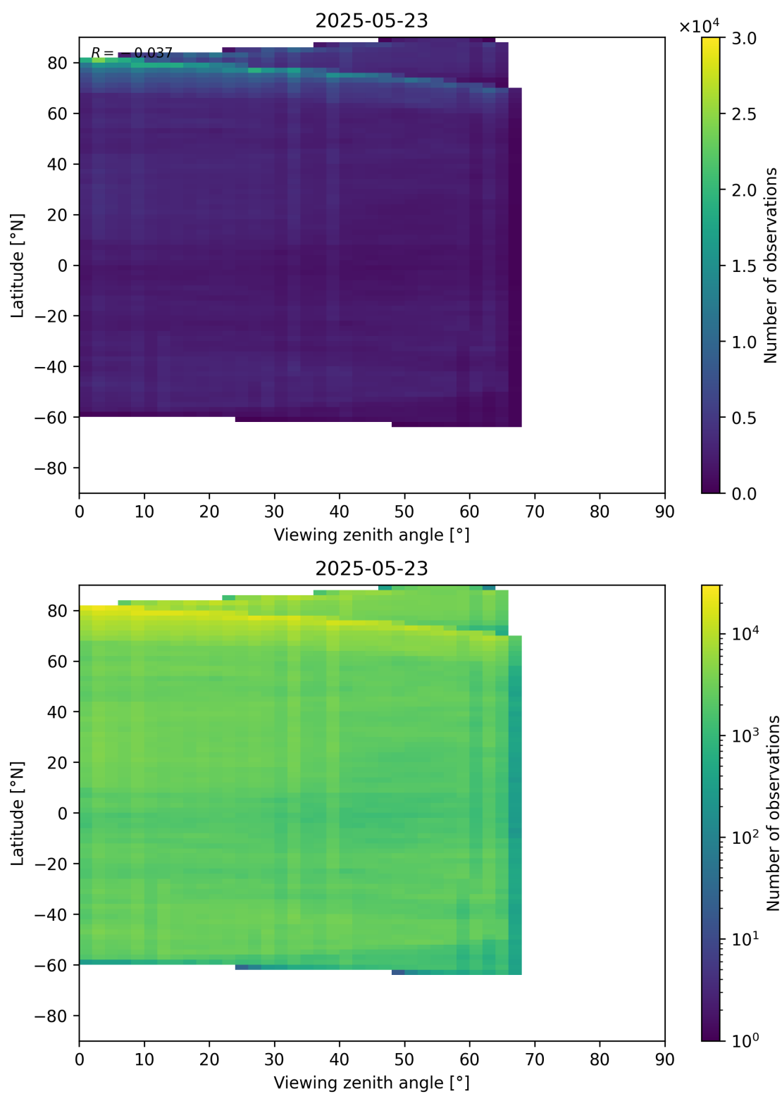
Figure 74: Scatter density plot of “Viewing zenith angle” against “Latitude” for 2025-05-22 to 2025-05-24.
