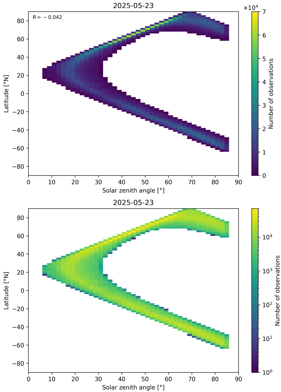
Figure 66: Scatter density plot of “Solar zenith angle” against “Latitude” for 2025-05-22 to 2025-05-24.
