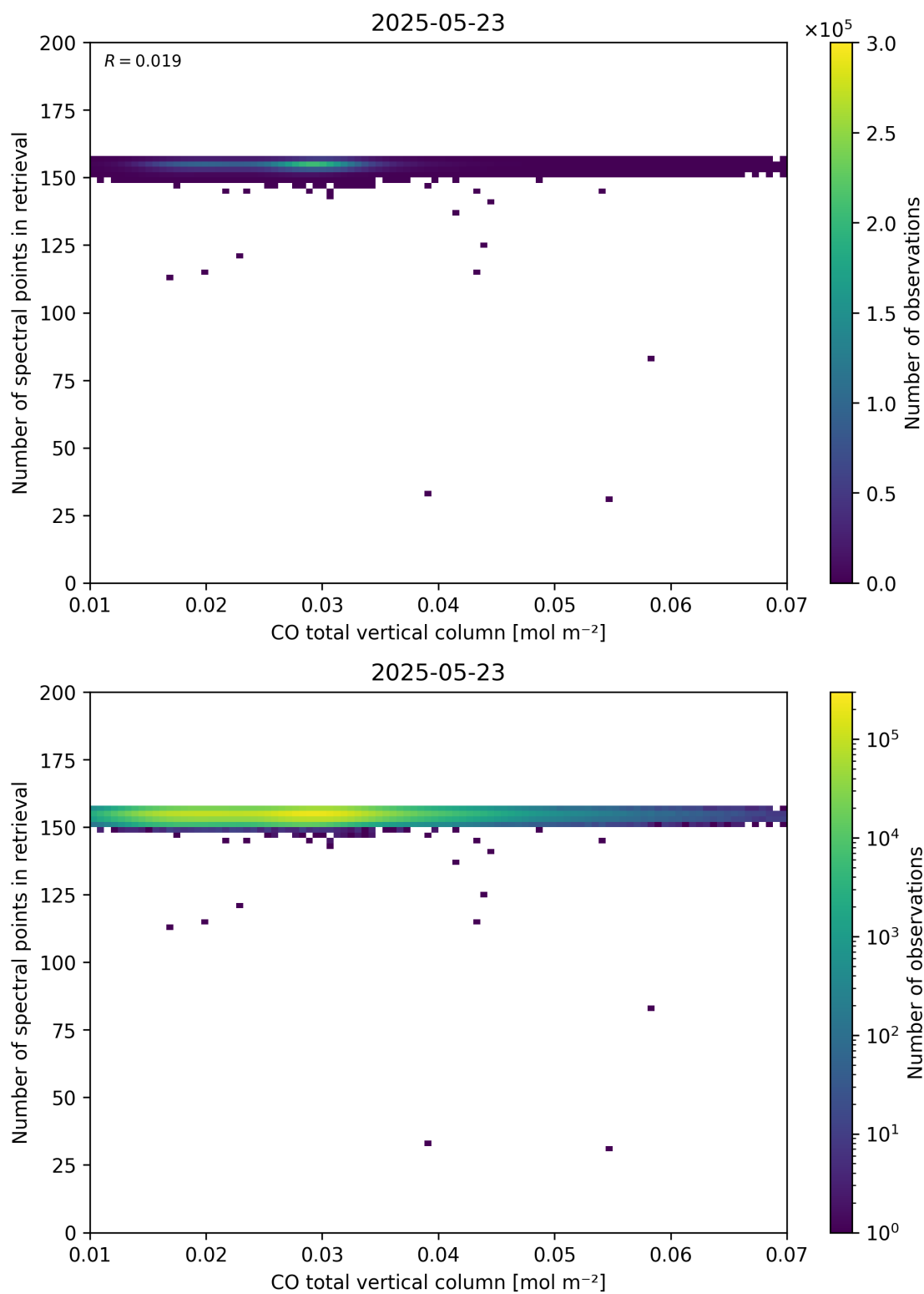
Figure 43: Scatter density plot of “CO total vertical column” against “Number of spectral points in retrieval” for 2025-05-22 to 2025-05-24.
