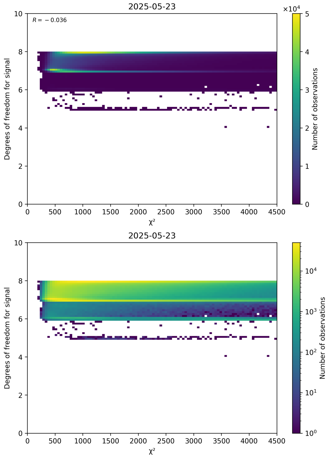
Figure 48: Scatter density plot of “ \chi^2 ” against “Degrees of freedom for signal” for 2025-05-22 to 2025-05-24.
