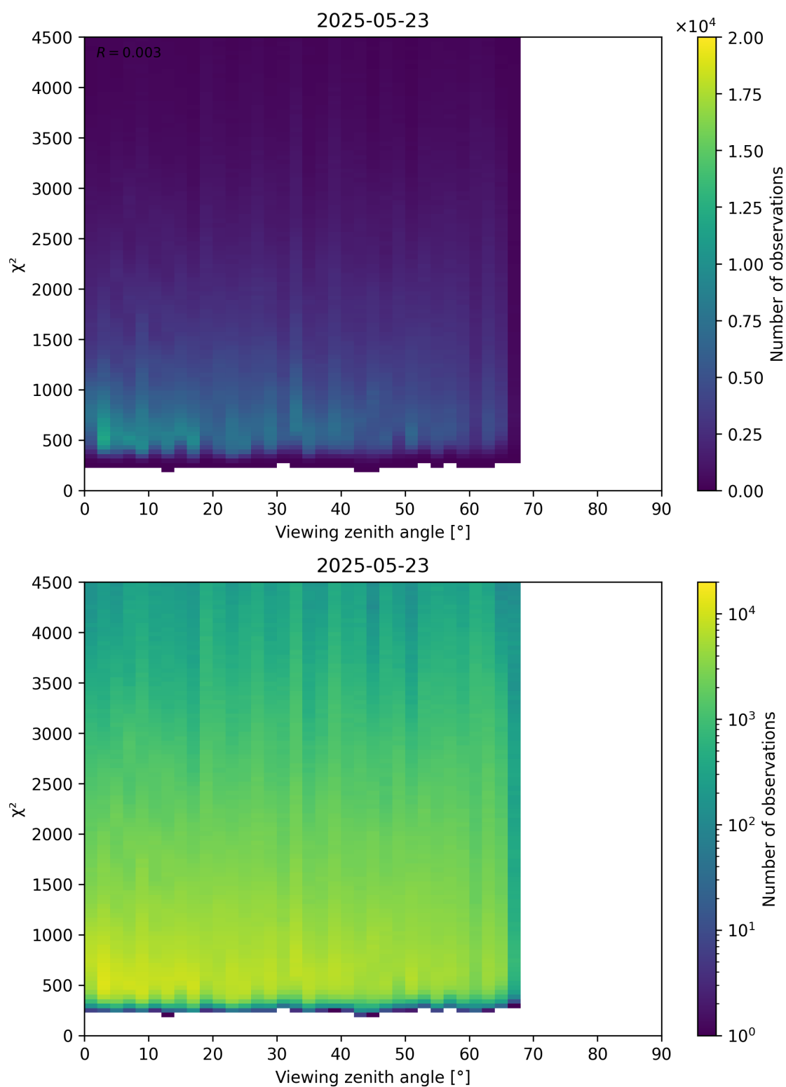
Figure 72: Scatter density plot of “Viewing zenith angle” against “ \chi^2 ” for 2025-05-22 to 2025-05-24.
