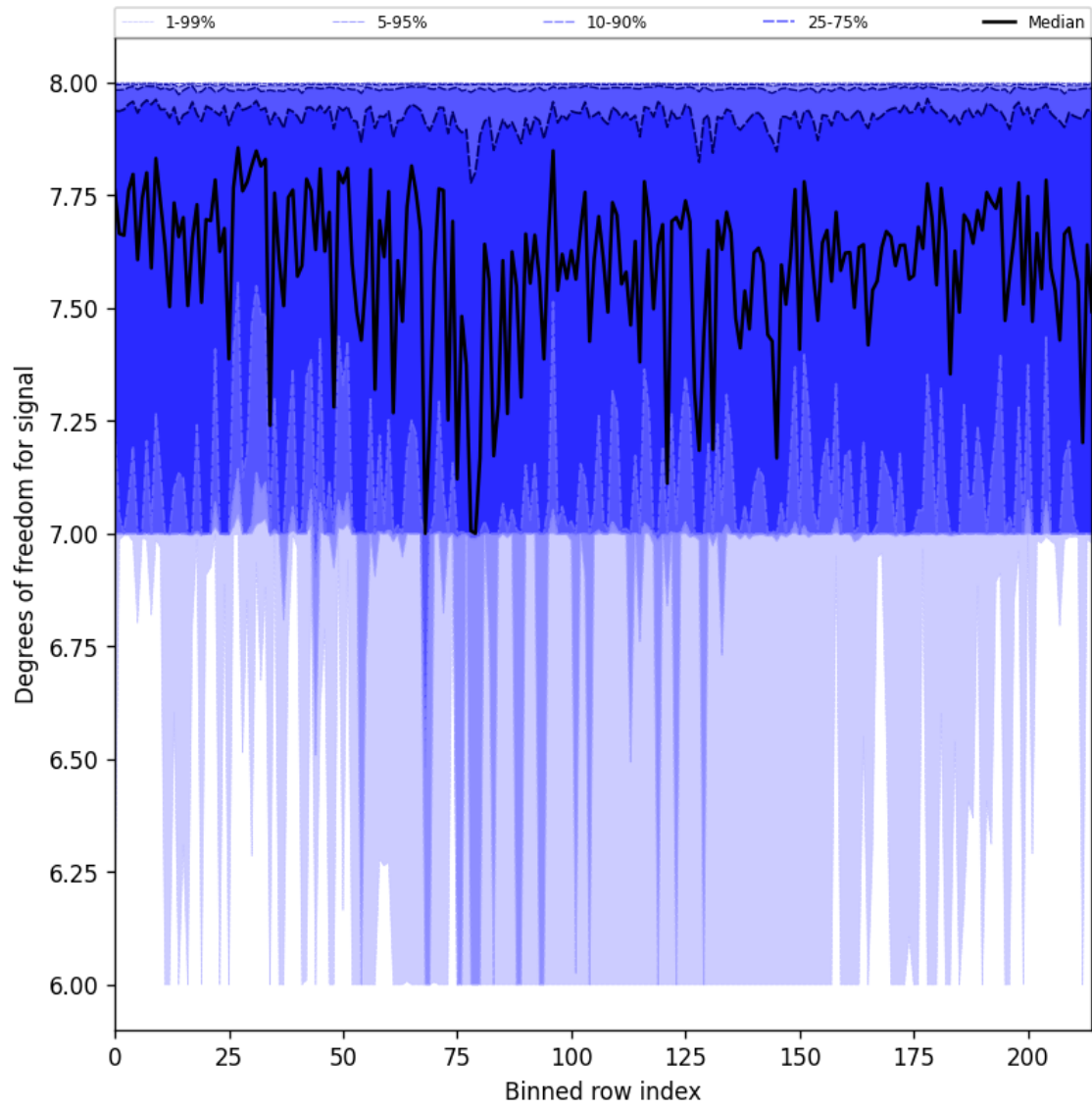
Figure 31: Along track statistics of “Degrees of freedom for signal” for 2025-05-22 to 2025-05-24
