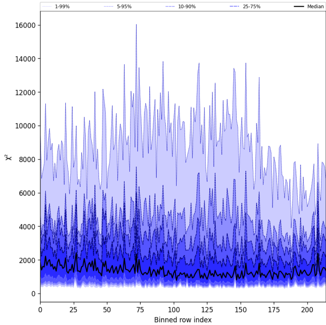
Figure 30: Along track statistics of “ \chi^2 ” for 2025-05-22 to 2025-05-24
