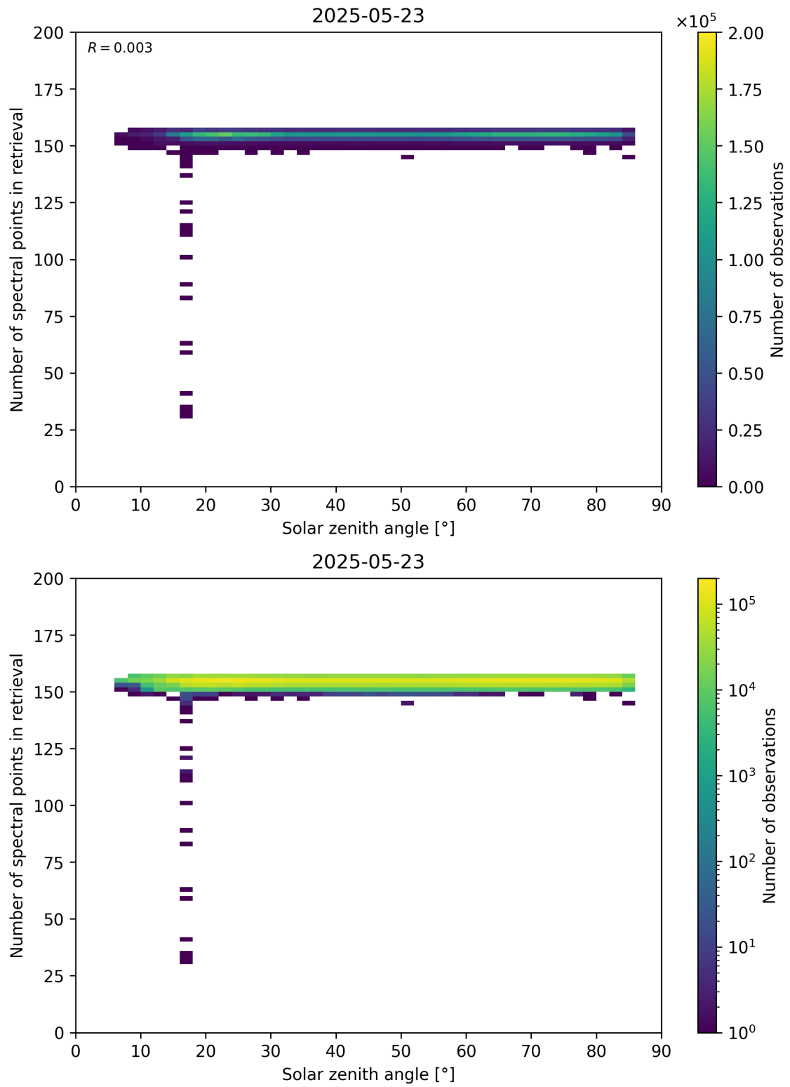
Figure 68: Scatter density plot of “Solar zenith angle” against “Number of spectral points in retrieval” for 2025-05-22 to 2025-05-24.
