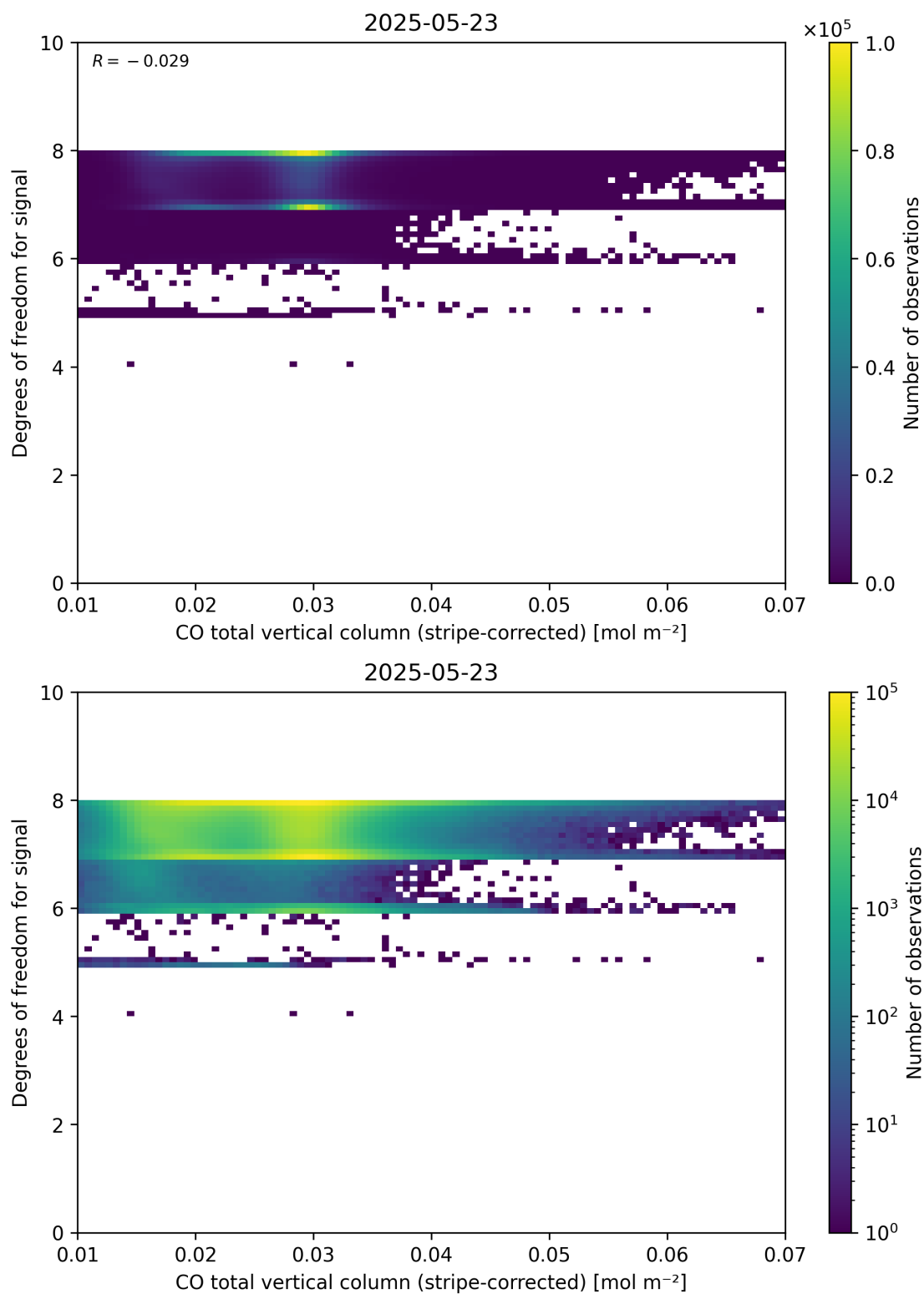
Figure 38: Scatter density plot of “CO total vertical column (stripe-corrected)” against “Degrees of freedom for signal” for 2025-05-22 to 2025-05-24.
