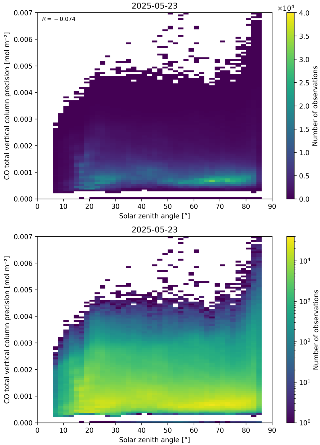
Figure 63: Scatter density plot of “Solar zenith angle” against “CO total vertical column precision” for 2025-05-22 to 2025-05-24.
