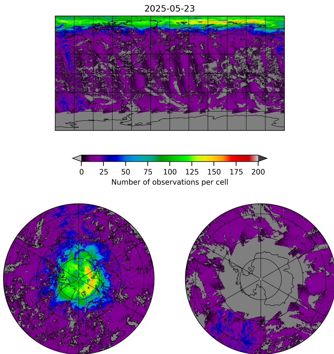
Figure 8: Map of the number of observations for 2025-05-22 to 2025-05-24
