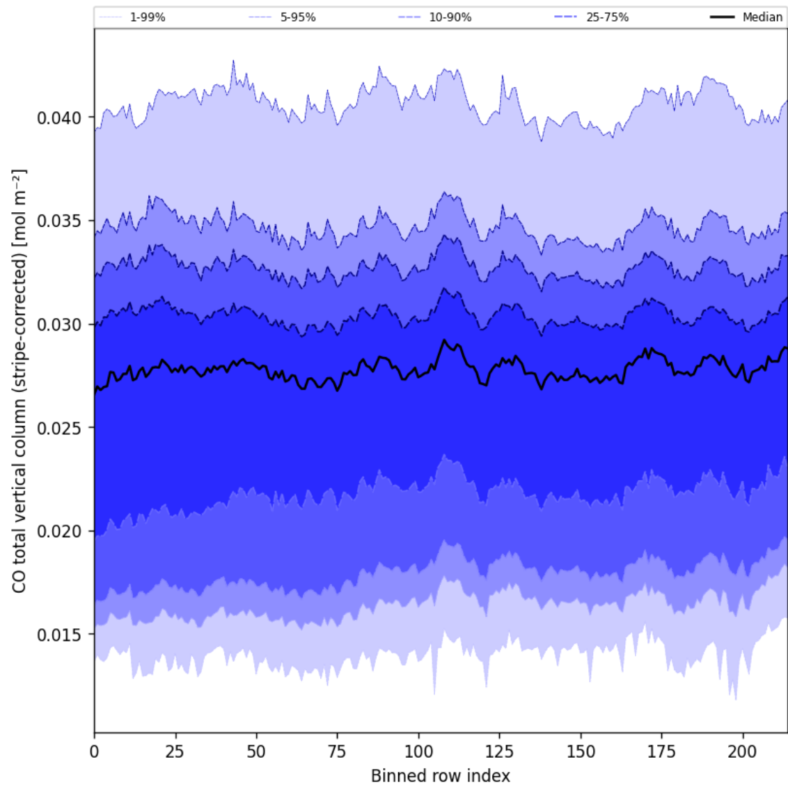
Figure 27: Along track statistics of “CO total vertical column (stripe-corrected)” for 2025-05-22 to 2025-05-24
