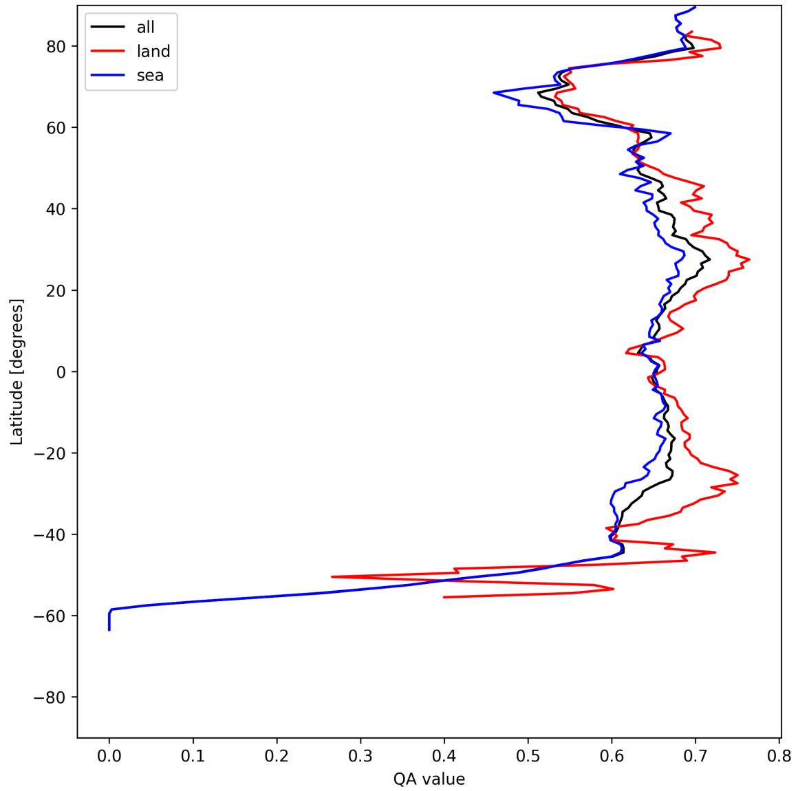
Figure 9: Zonal average of “QA value” for 2025-05-22 to 2025-05-24.
