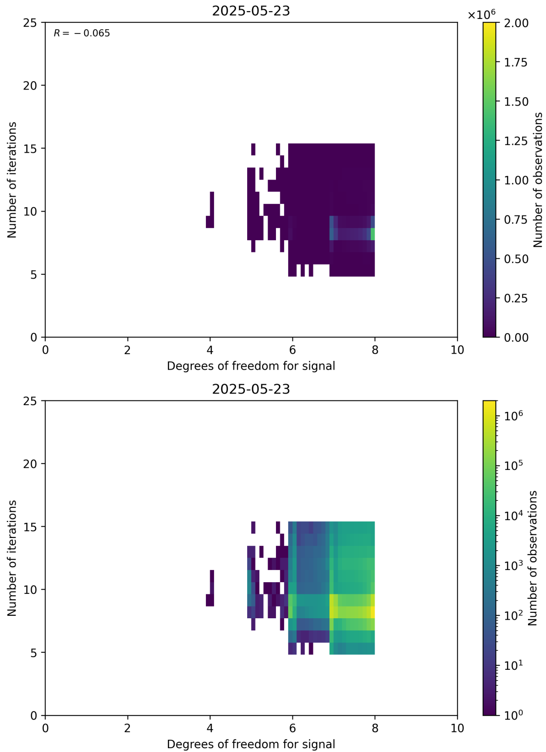
Figure 50: Scatter density plot of “Degrees of freedom for signal” against “Number of iterations” for 2025-05-22 to 2025-05-24.
