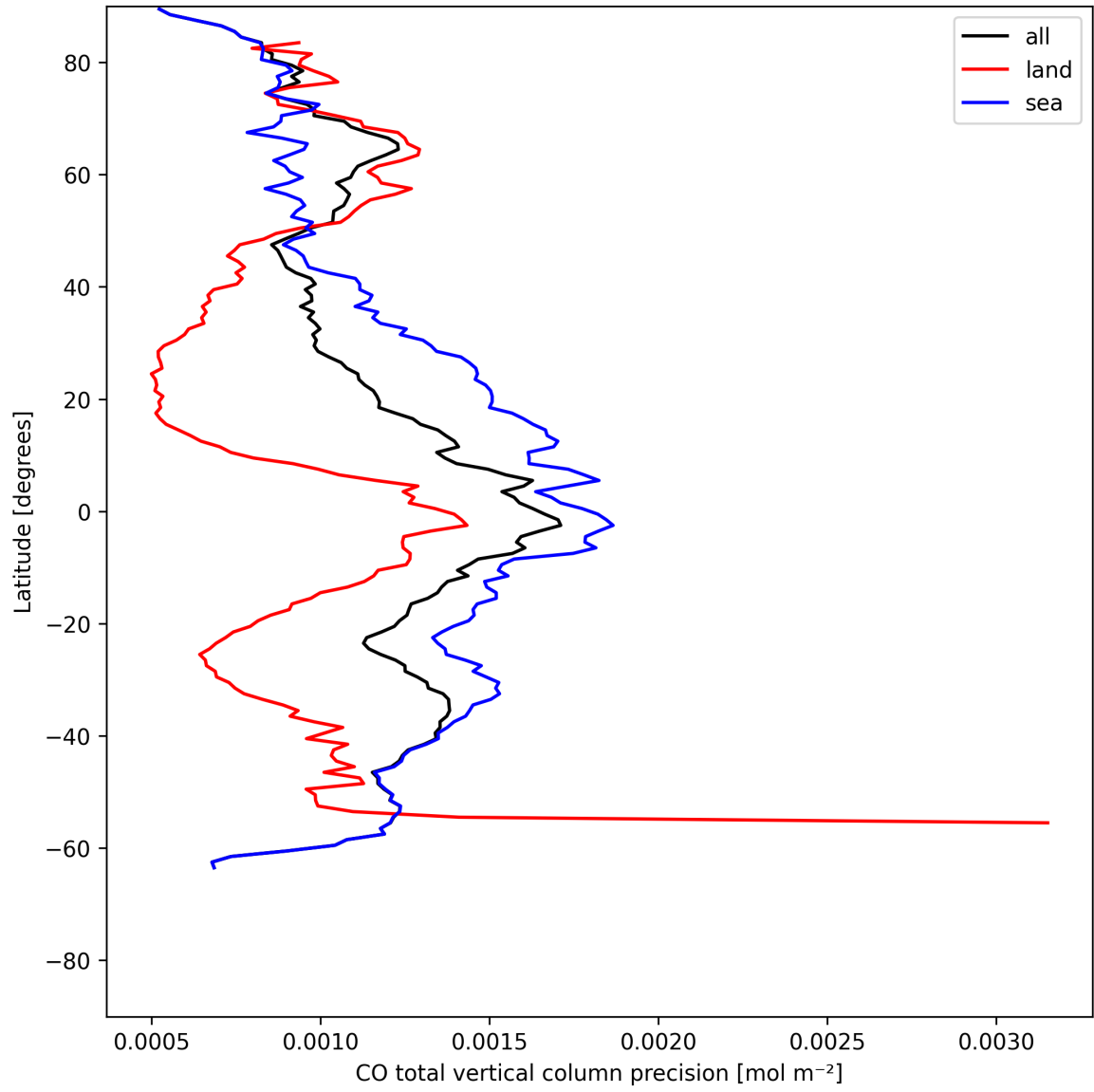
Figure 12: Zonal average of “CO total vertical column precision” for 2025-05-22 to 2025-05-24.
