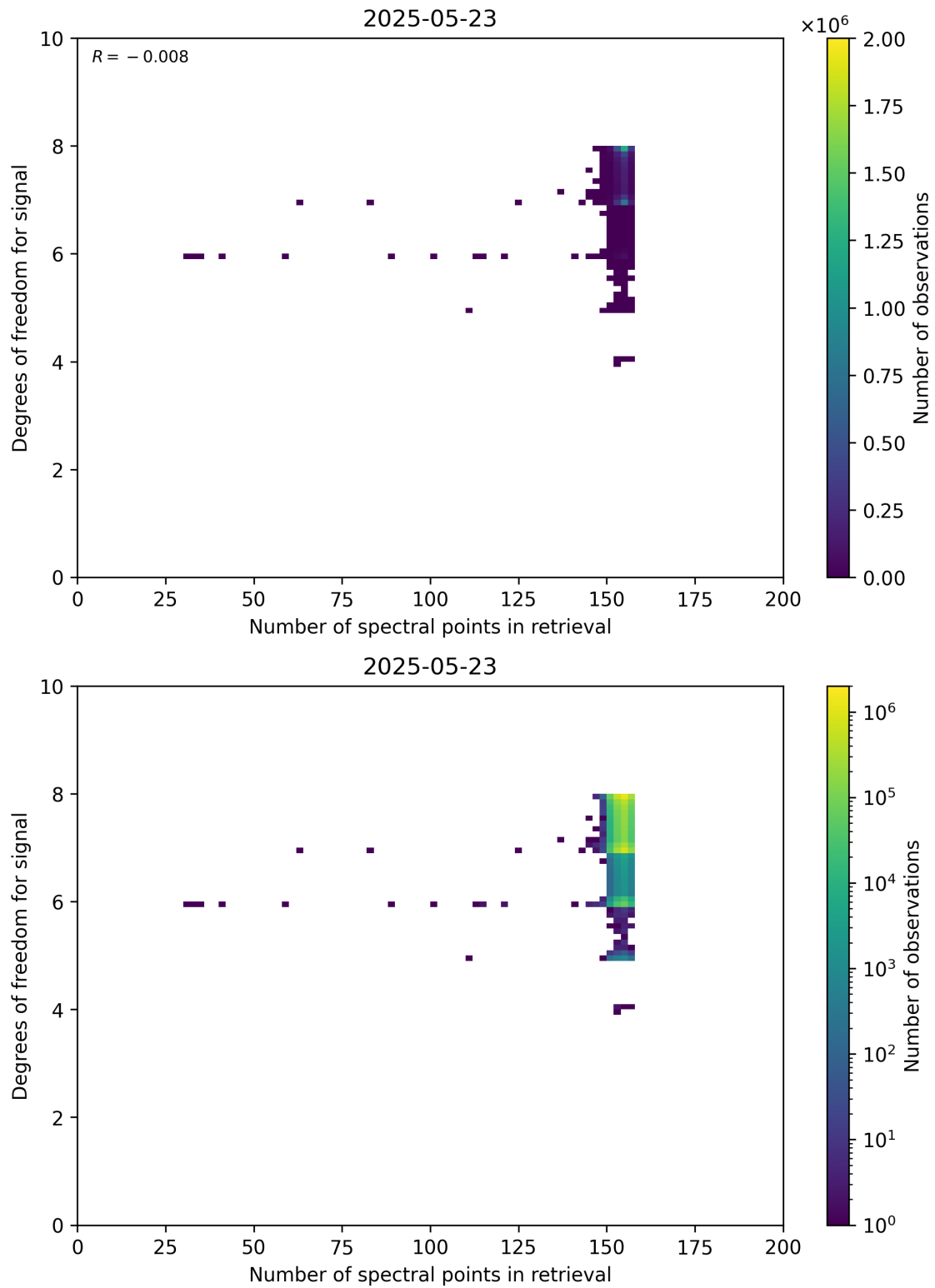
Figure 59: Scatter density plot of “Number of spectral points in retrieval” against “Degrees of freedom for signal” for 2025-05-22 to 2025-05-24.
