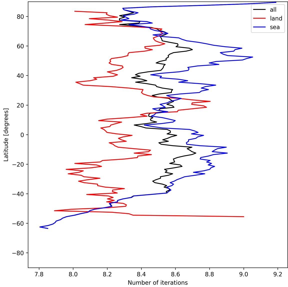
Figure 16: Zonal average of “Number of iterations” for 2025-05-22 to 2025-05-24.
