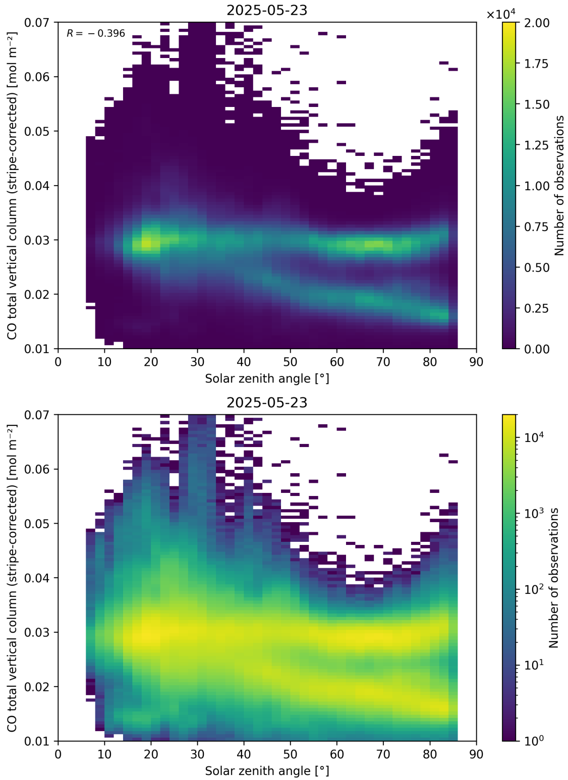
Figure 62: Scatter density plot of “Solar zenith angle” against “CO total vertical column (stripe-corrected)” for 2025-05-22 to 2025-05-24.
