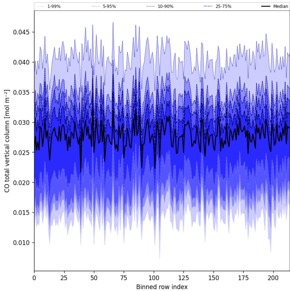
Figure 26: Along track statistics of “CO total vertical column” for 2025-05-22 to 2025-05-24
