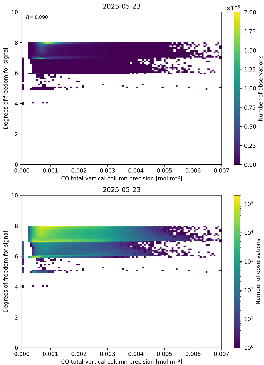
Figure 45: Scatter density plot of “CO total vertical column precision” against “Degrees of freedom for signal” for 2025-05-22 to 2025-05-24.
