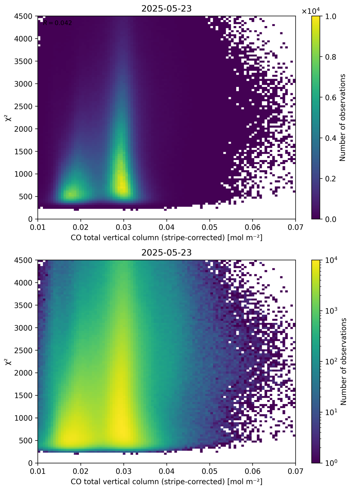
Figure 37: Scatter density plot of “CO total vertical column (stripe-corrected)” against “ \chi^2 ” for 2025-05-22 to 2025-05-24.
