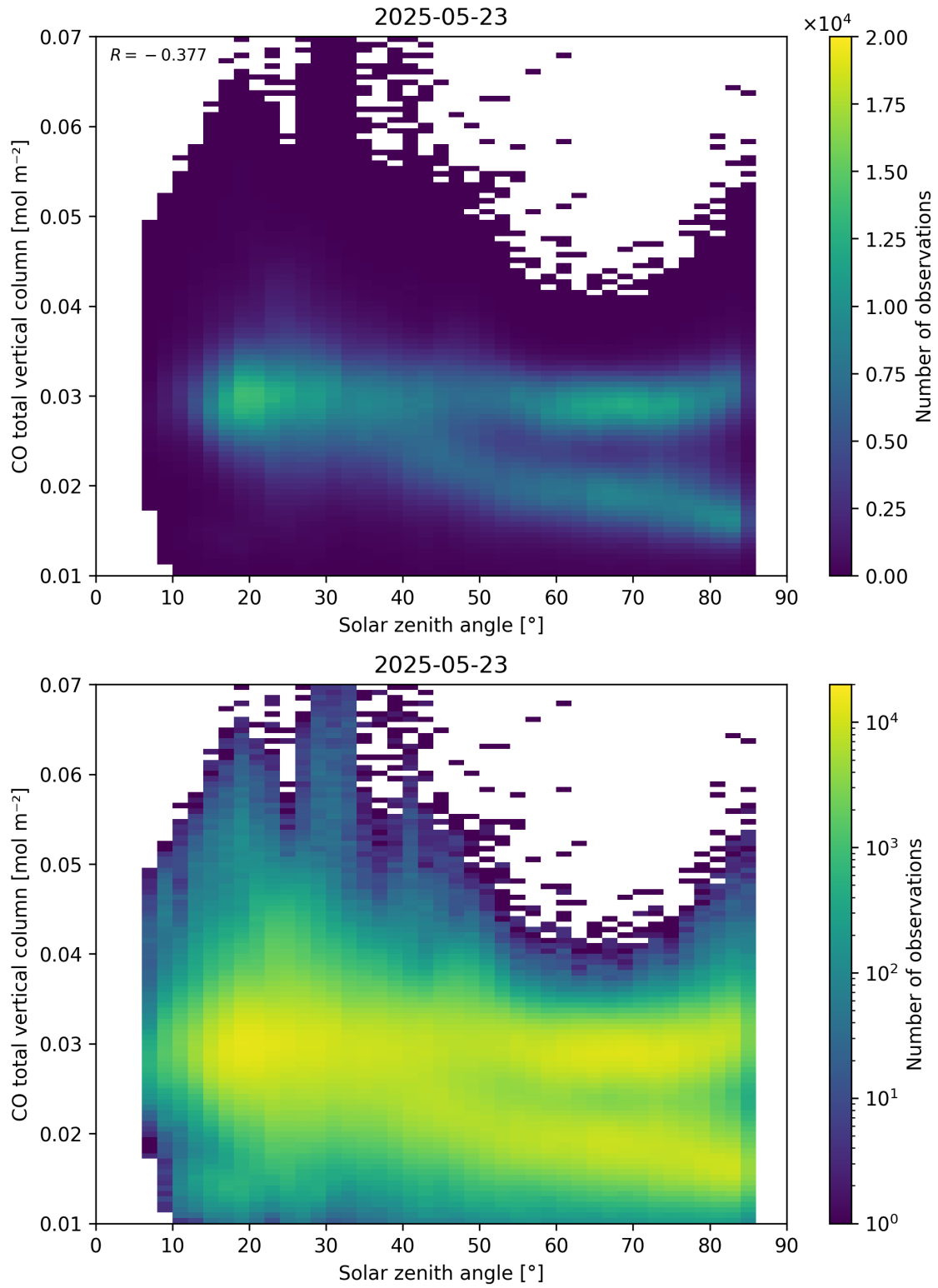
Figure 61: Scatter density plot of “Solar zenith angle” against “CO total vertical column” for 2025-05-22 to 2025-05-24.
