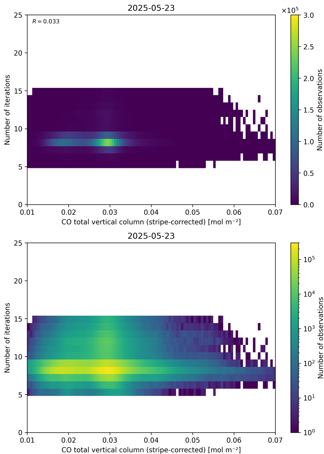
Figure 39: Scatter density plot of “CO total vertical column (stripe-corrected)” against “Number of iterations” for 2025-05-22 to 2025-05-24.
