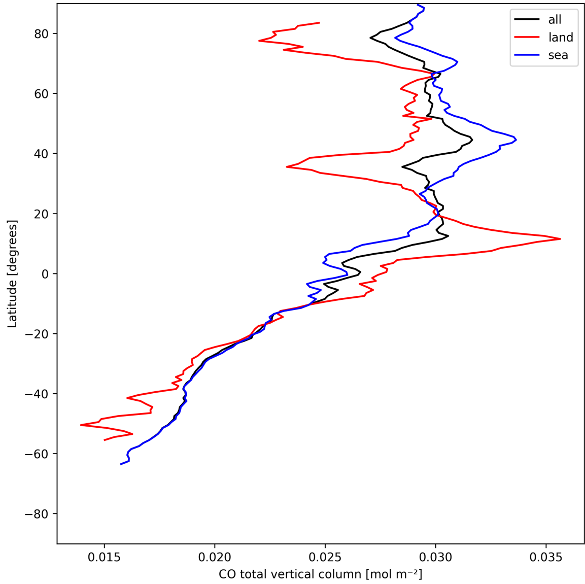
Figure 10: Zonal average of “CO total vertical column” for 2025-05-22 to 2025-05-24.
