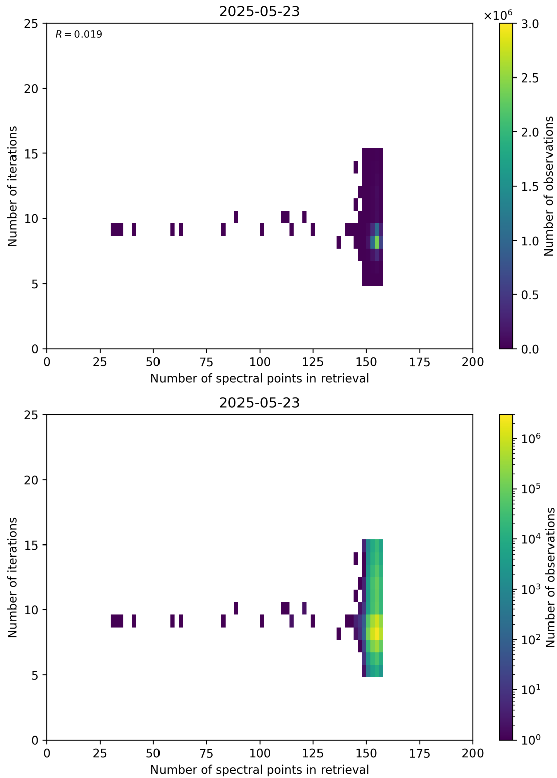
Figure 60: Scatter density plot of “Number of spectral points in retrieval” against “Number of iterations” for 2025-05-22 to 2025-05-24.
