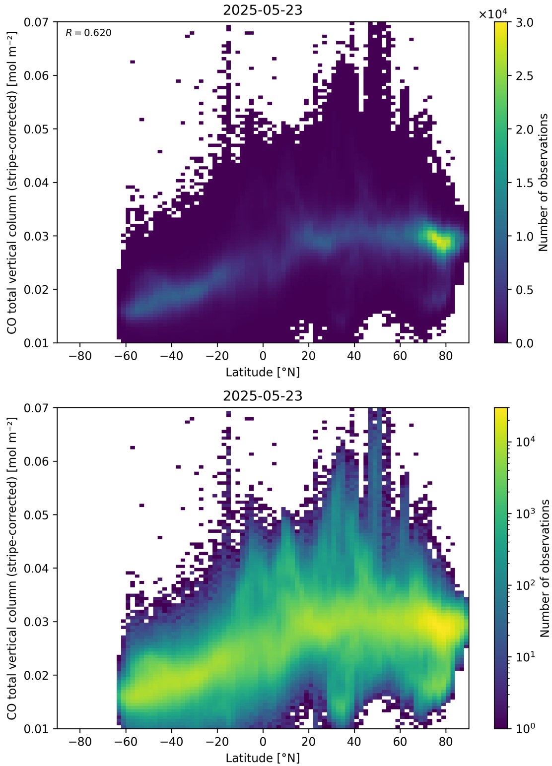
Figure 52: Scatter density plot of “Latitude” against “CO total vertical column (stripe-corrected)” for 2025-05-22 to 2025-05-24.
