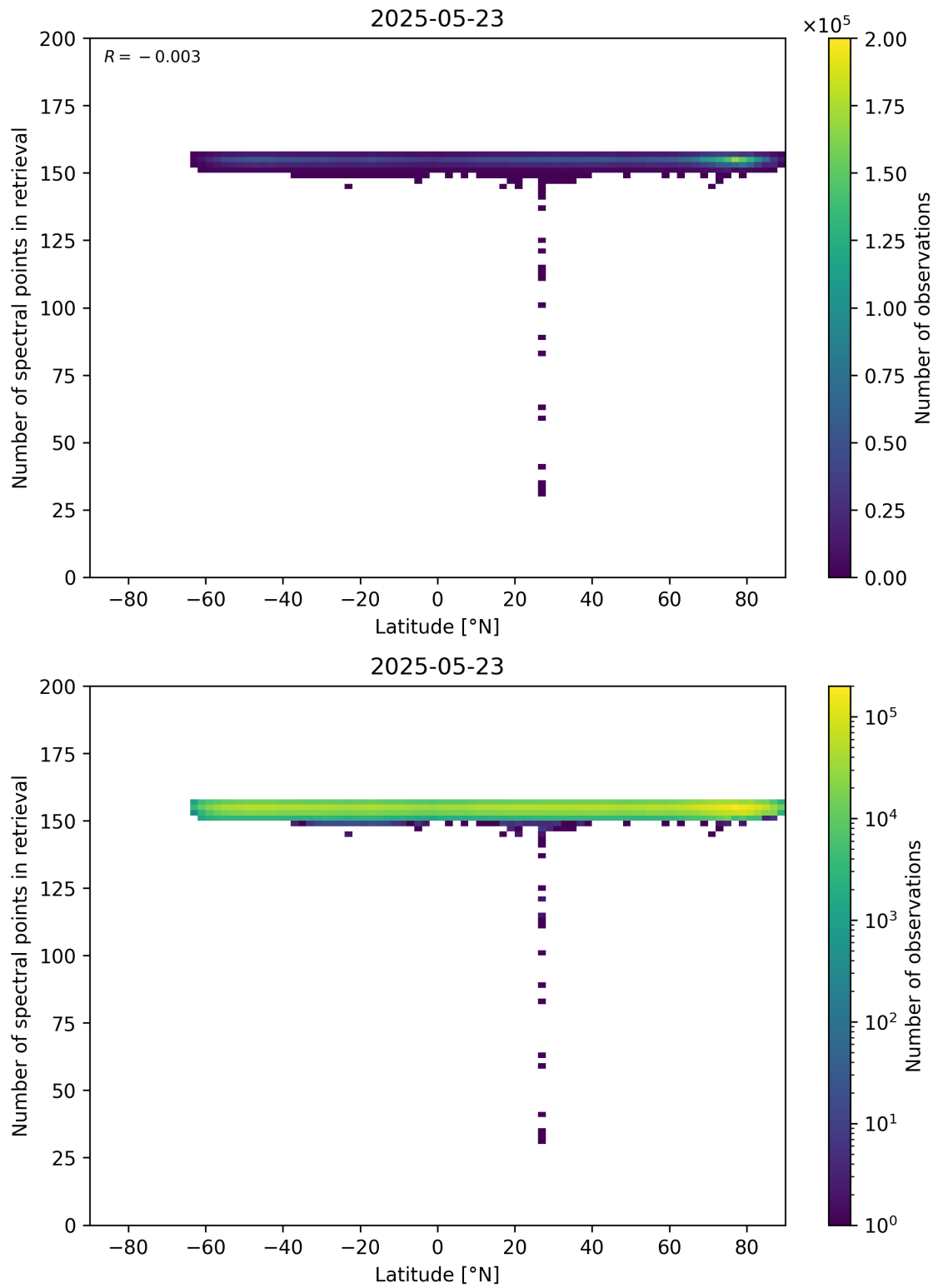
Figure 57: Scatter density plot of “Latitude” against “Number of spectral points in retrieval” for 2025-05-22 to 2025-05-24.
