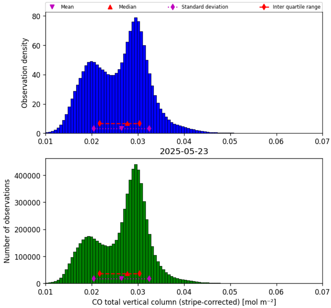
Figure 19: Histogram of “CO total vertical column (stripe-corrected)” for 2025-05-22 to 2025-05-24
