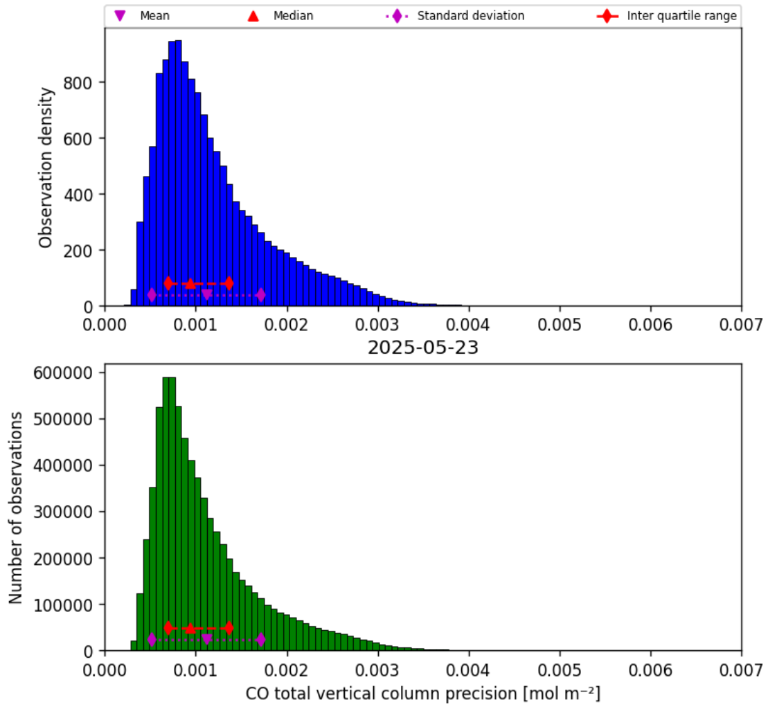
Figure 20: Histogram of “CO total vertical column precision” for 2025-05-22 to 2025-05-24
