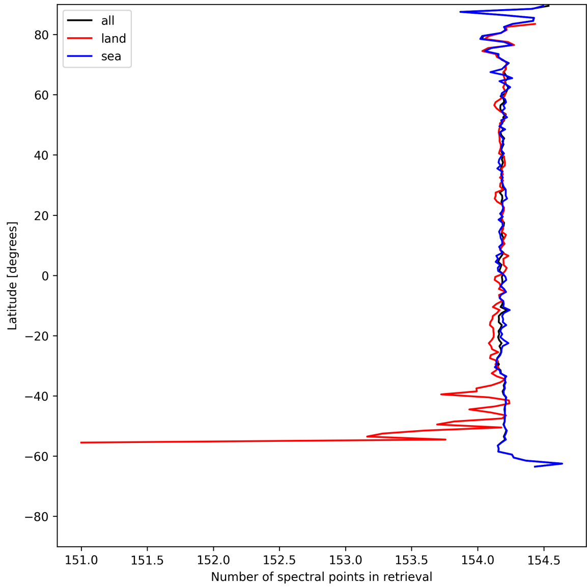
Figure 13: Zonal average of “Number of spectral points in retrieval” for 2025-05-22 to 2025-05-24.
