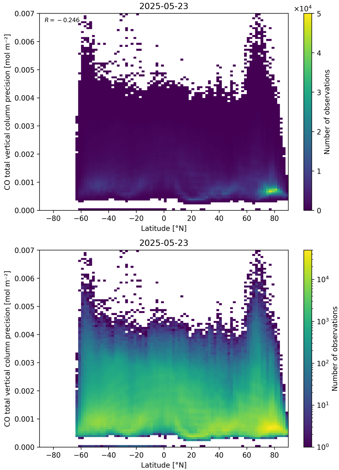
Figure 53: Scatter density plot of “Latitude” against “CO total vertical column precision” for 2025-05-22 to 2025-05-24.
