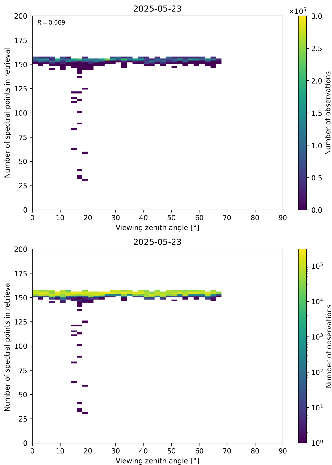
Figure 76: Scatter density plot of “Viewing zenith angle” against “Number of spectral points in retrieval” for 2025-05-22 to 2025-05-24.
