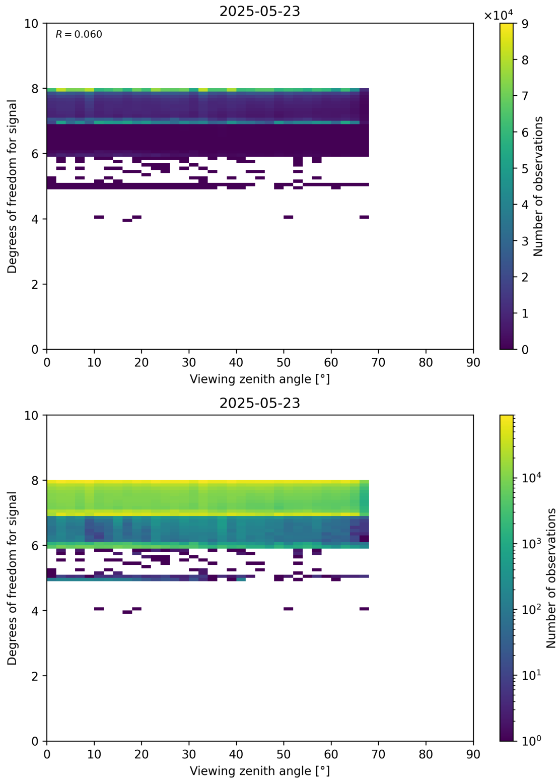
Figure 73: Scatter density plot of “Viewing zenith angle” against “Degrees of freedom for signal” for 2025-05-22 to 2025-05-24.
