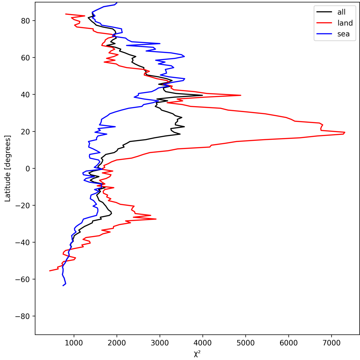
Figure 14: Zonal average of “ \chi^2 ” for 2025-05-22 to 2025-05-24.
