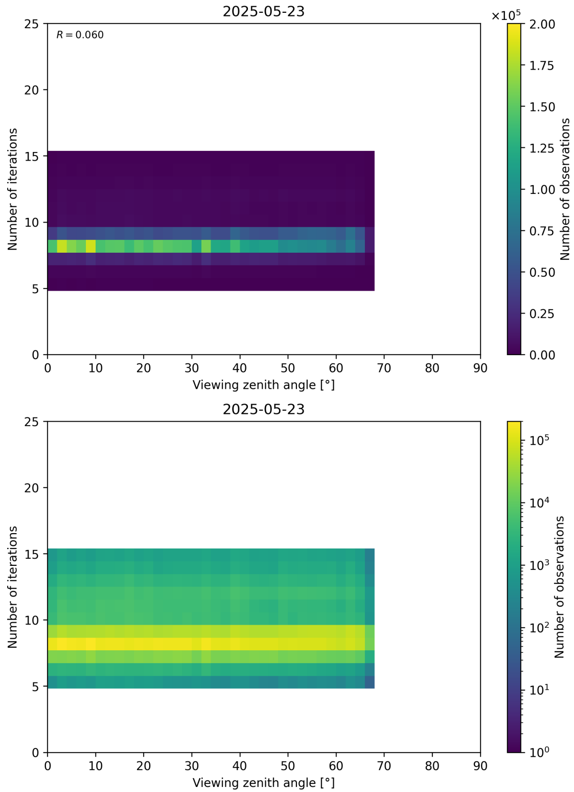
Figure 75: Scatter density plot of “Viewing zenith angle” against “Number of iterations” for 2025-05-22 to 2025-05-24.
