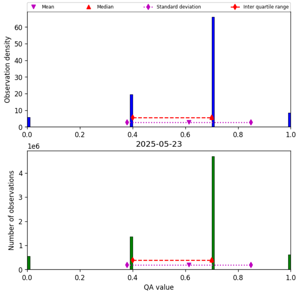
Figure 17: Histogram of “QA value” for 2025-05-22 to 2025-05-24
