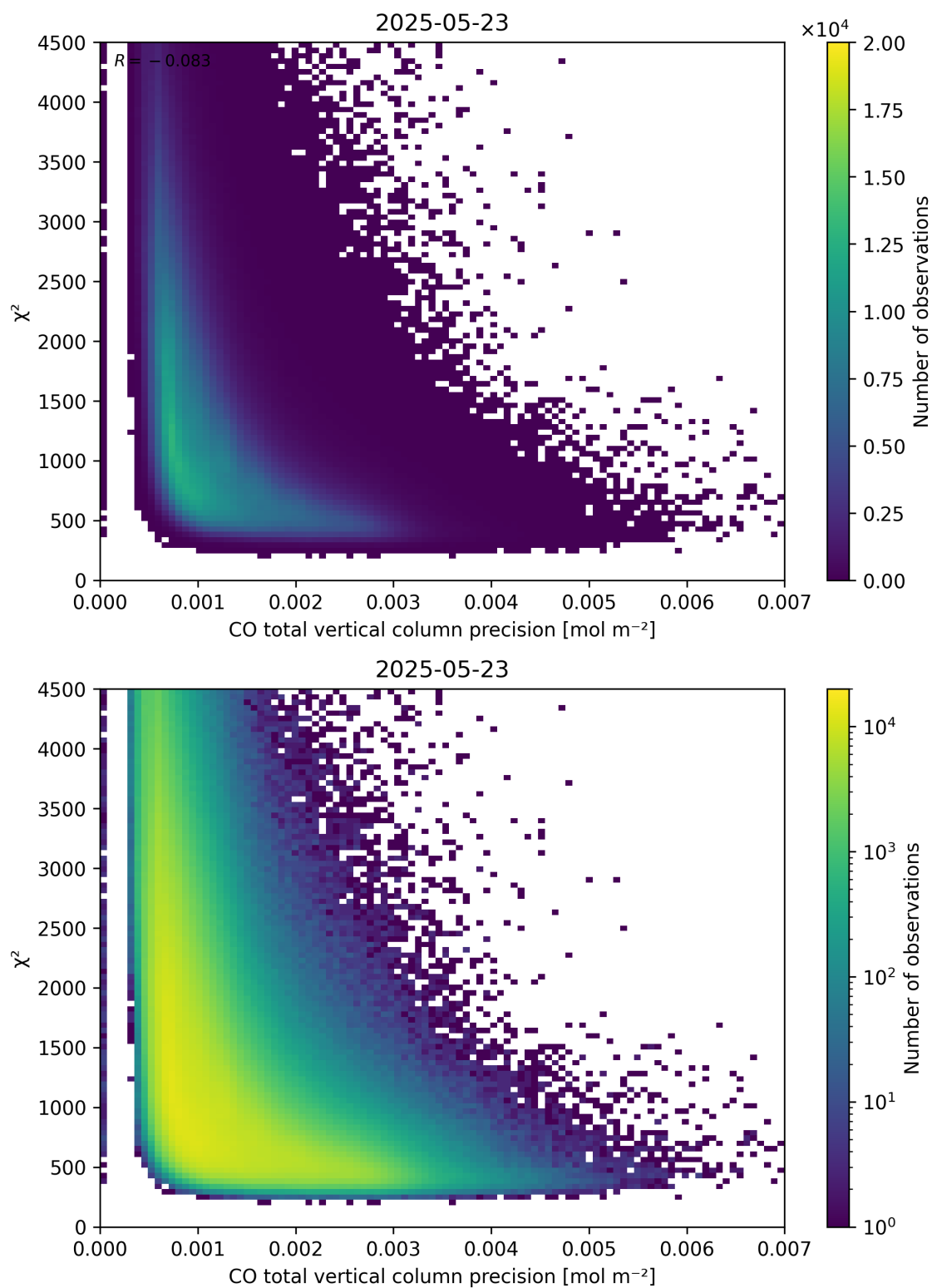
Figure 44: Scatter density plot of “CO total vertical column precision” against “ \chi^2 ” for 2025-05-22 to 2025-05-24.
