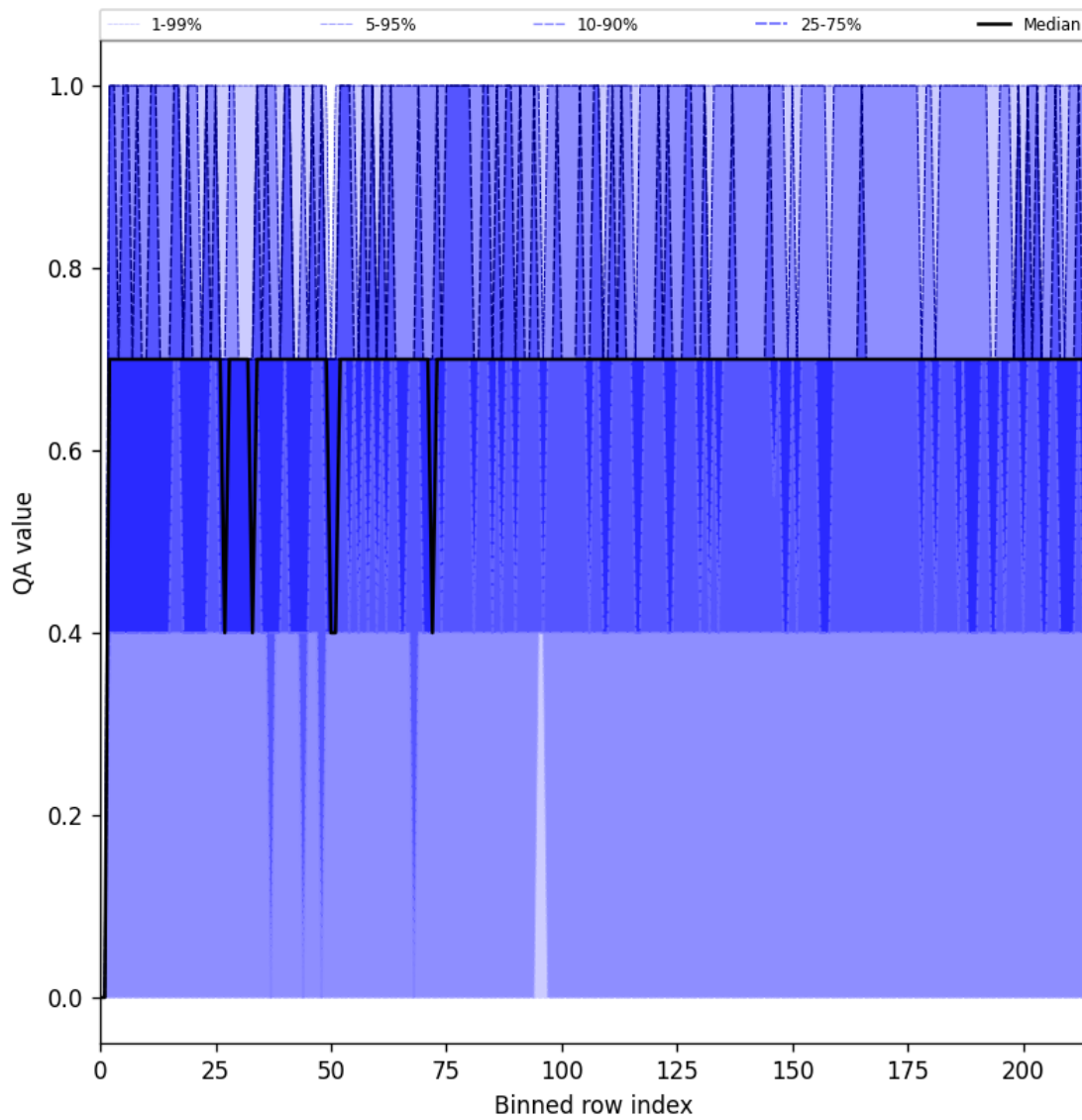
Figure 25: Along track statistics of “QA value” for 2025-05-22 to 2025-05-24
