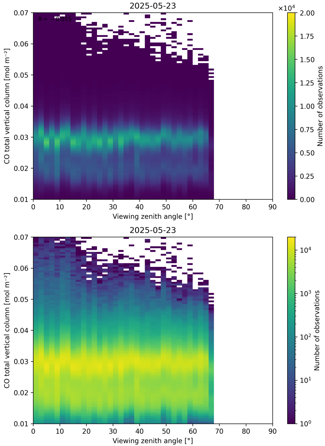
Figure 69: Scatter density plot of “Viewing zenith angle” against “CO total vertical column” for 2025-05-22 to 2025-05-24.
