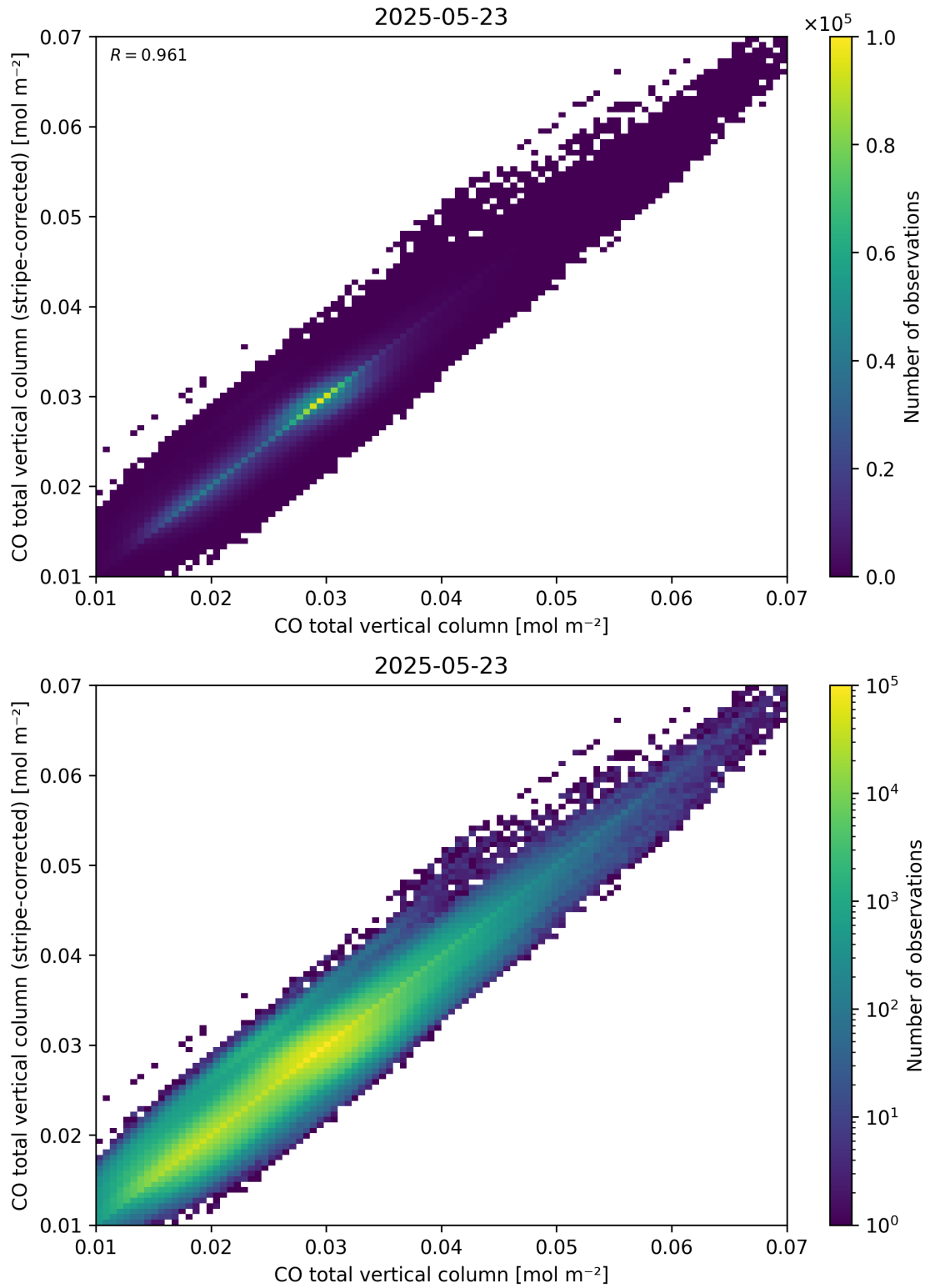
Figure 33: Scatter density plot of “CO total vertical column” against “CO total vertical column (stripe-corrected)” for 2025-05-22 to 2025-05-24.
