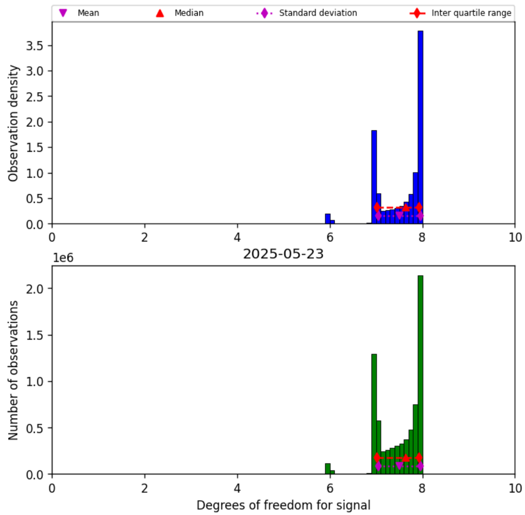
Figure 23: Histogram of “Degrees of freedom for signal” for 2025-05-22 to 2025-05-24
