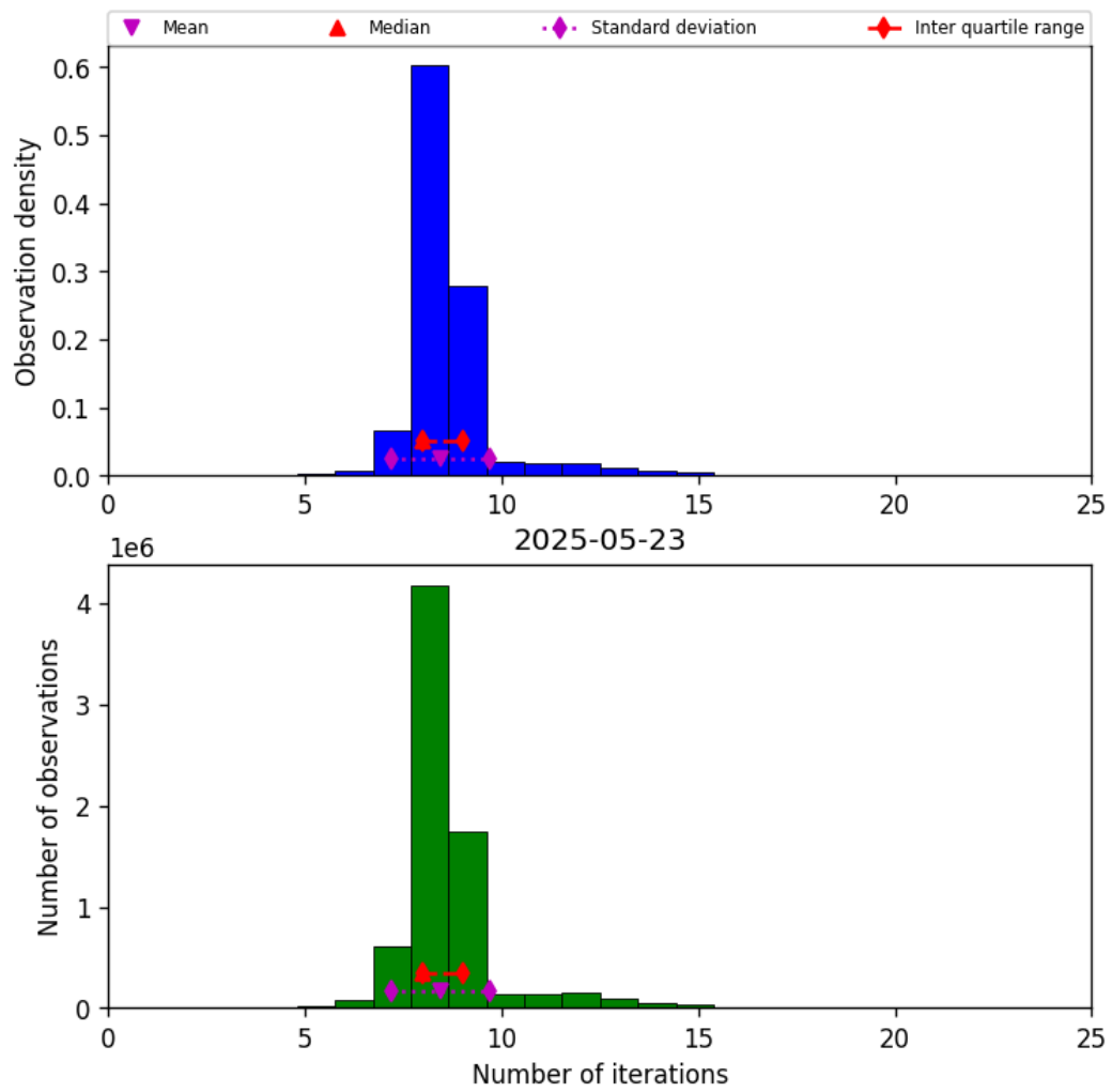
Figure 24: Histogram of “Number of iterations” for 2025-05-22 to 2025-05-24
