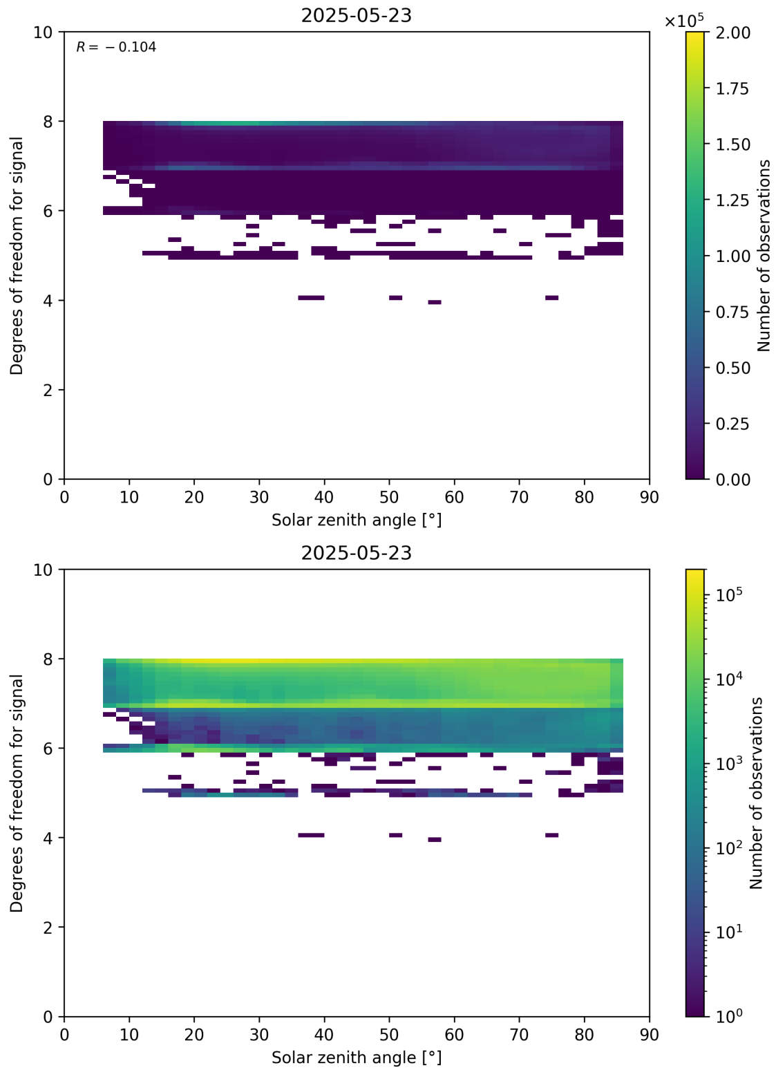
Figure 65: Scatter density plot of “Solar zenith angle” against “Degrees of freedom for signal” for 2025-05-22 to 2025-05-24.
