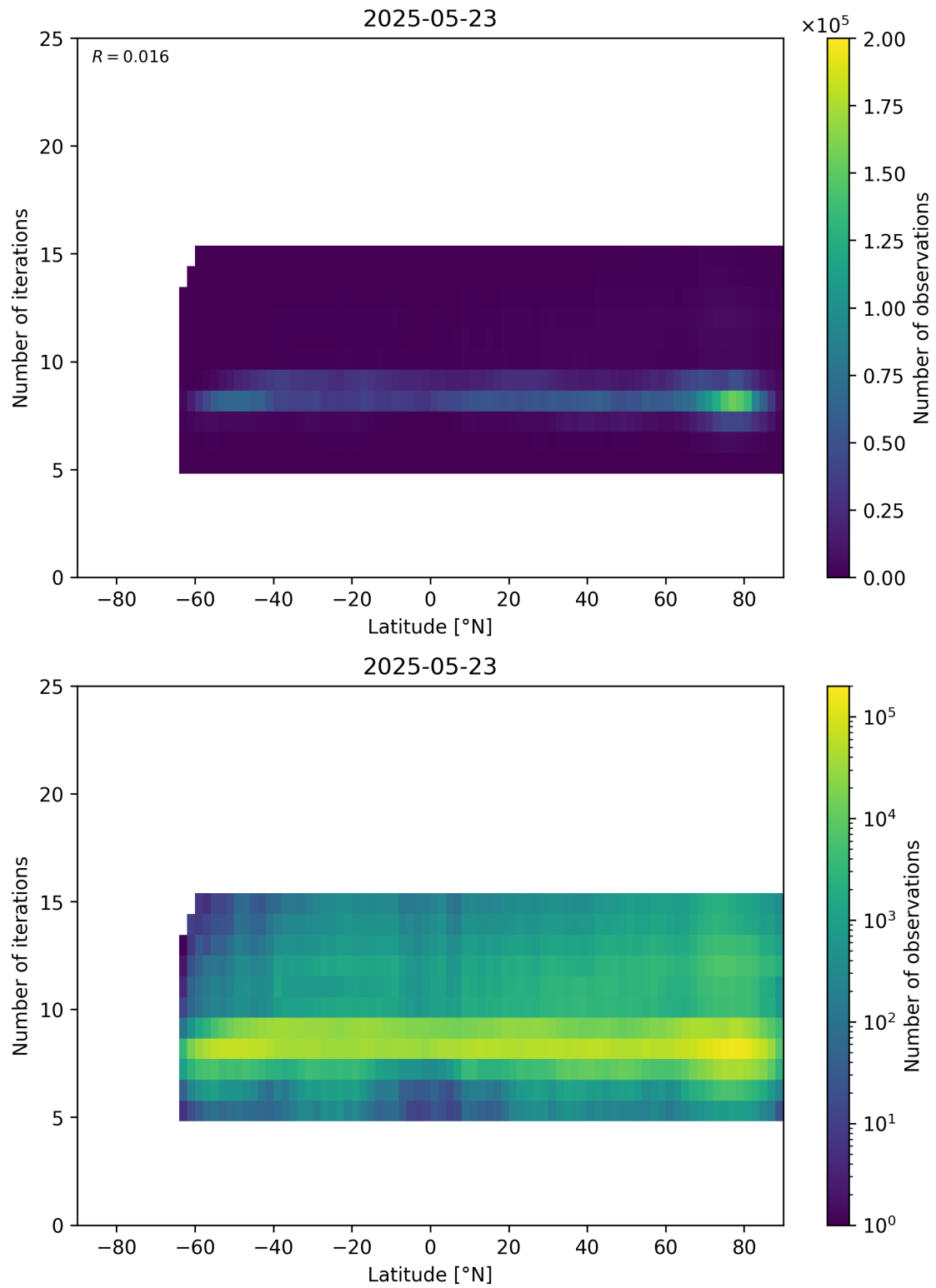
Figure 56: Scatter density plot of “Latitude” against “Number of iterations” for 2025-05-22 to 2025-05-24.
