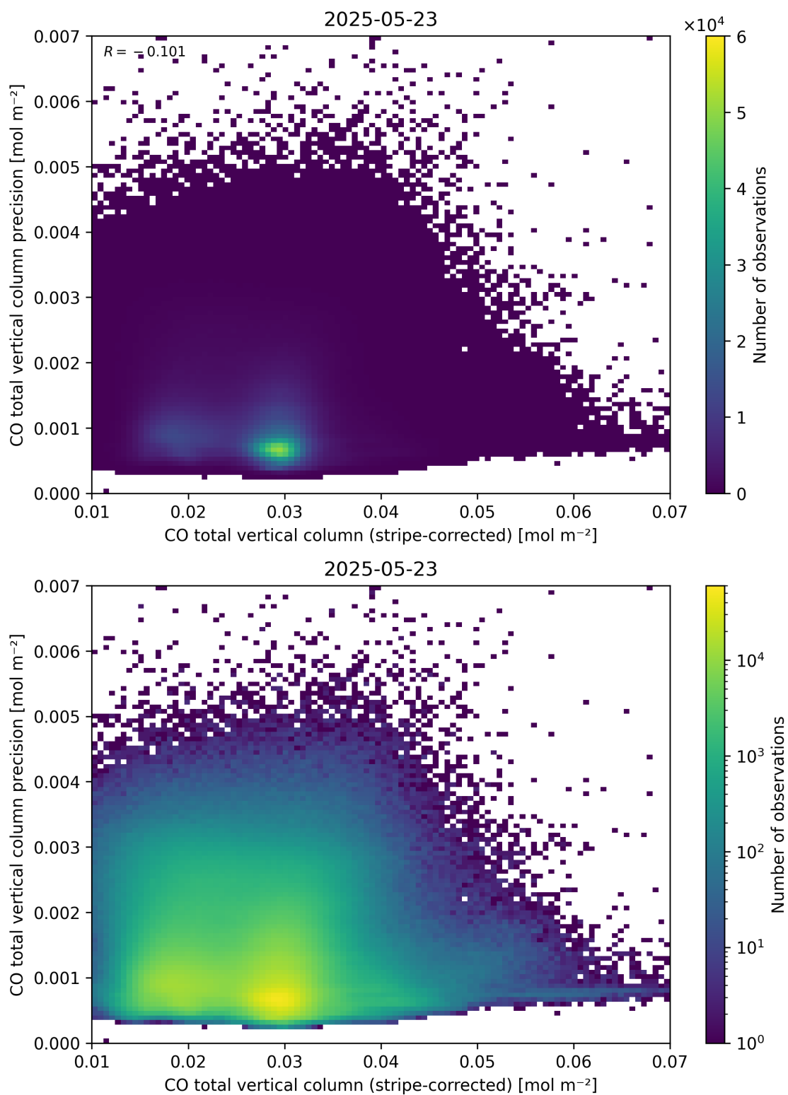
Figure 36: Scatter density plot of “CO total vertical column (stripe-corrected)” against “CO total vertical column precision” for 2025-05-22 to 2025-05-24.
