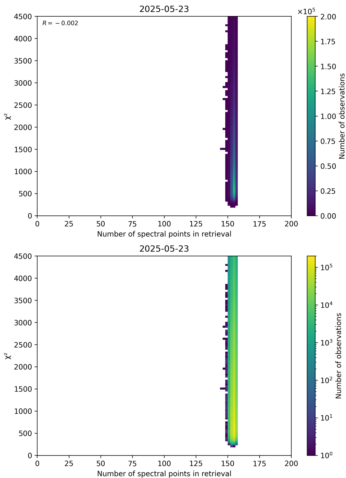
Figure 58: Scatter density plot of “Number of spectral points in retrieval” against “ \chi^2 ” for 2025-05-22 to 2025-05-24.
