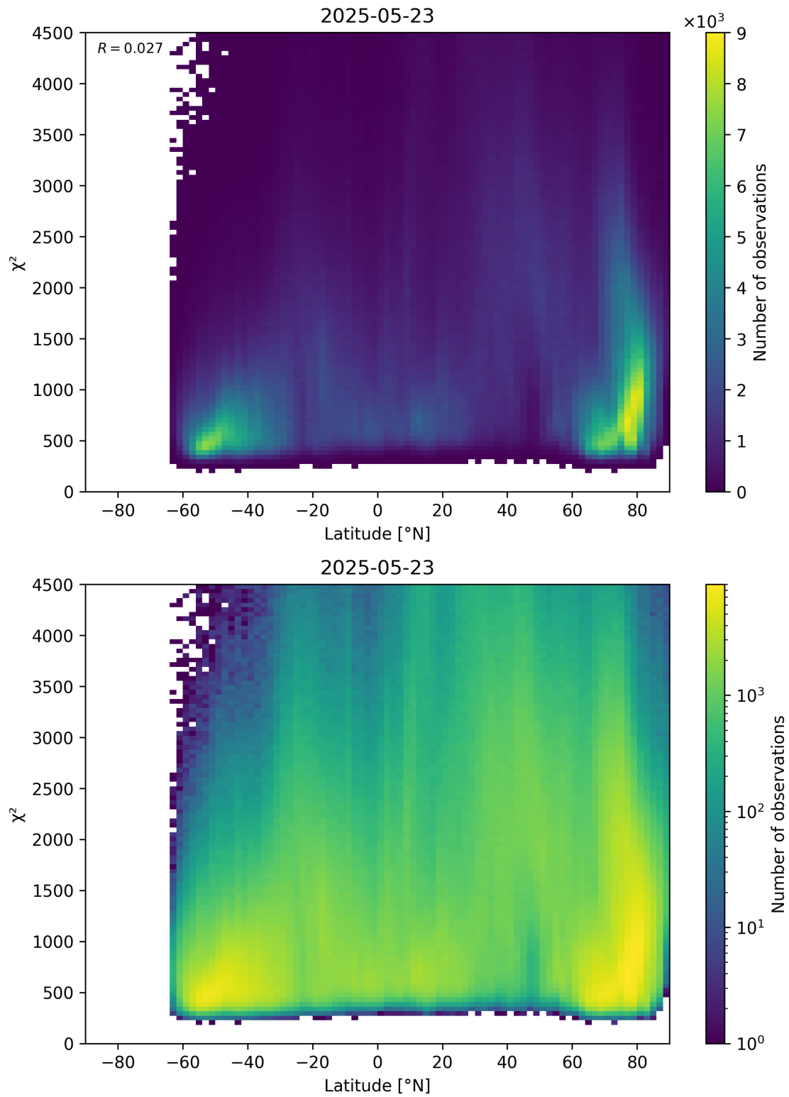
Figure 54: Scatter density plot of “Latitude” against “ \chi^2 ” for 2025-05-22 to 2025-05-24.
