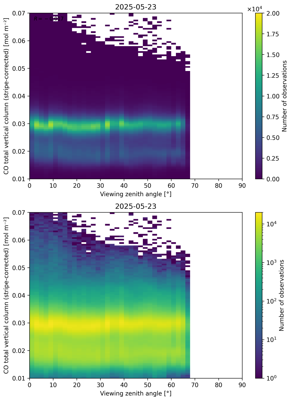
Figure 70: Scatter density plot of “Viewing zenith angle” against “CO total vertical column (stripe-corrected)” for 2025-05-22 to 2025-05-24.
