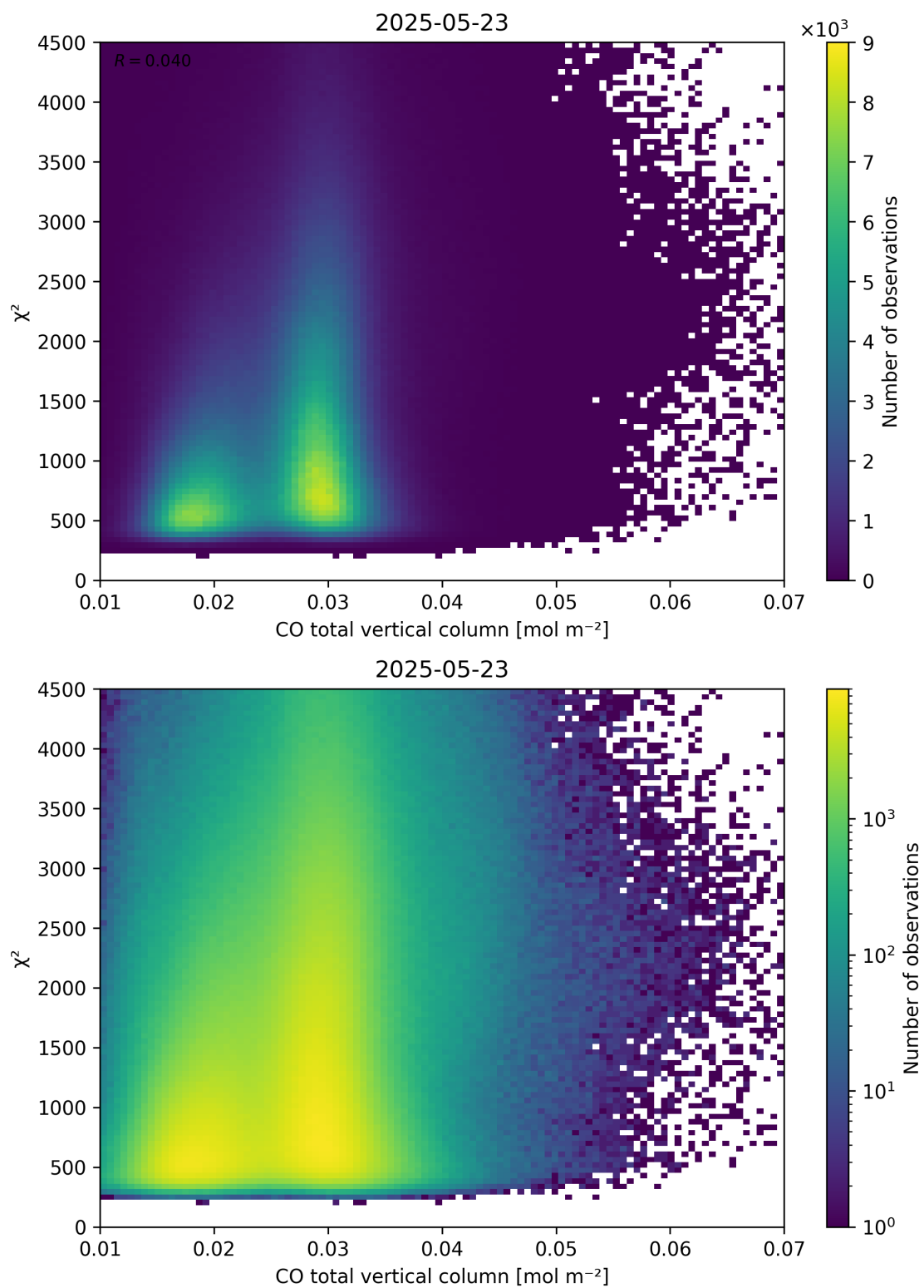
Figure 35: Scatter density plot of “CO total vertical column” against “ \chi^2 ” for 2025-05-22 to 2025-05-24.
