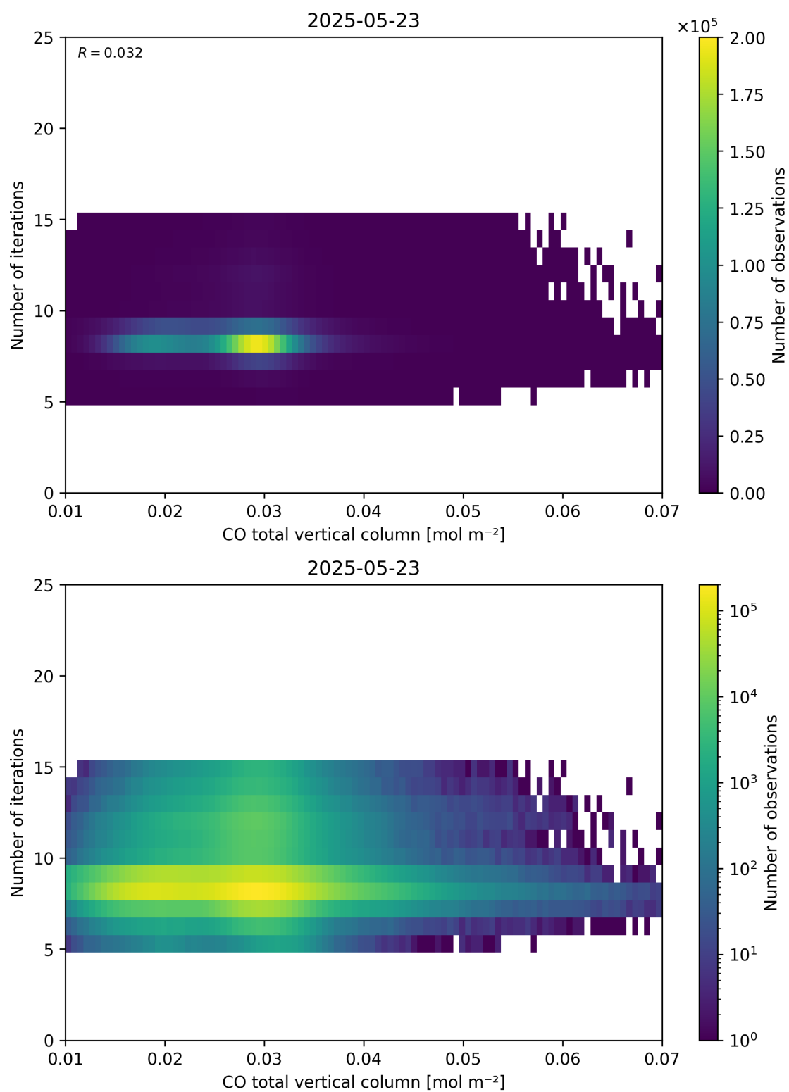
Figure 42: Scatter density plot of “CO total vertical column” against “Number of iterations” for 2025-05-22 to 2025-05-24.
