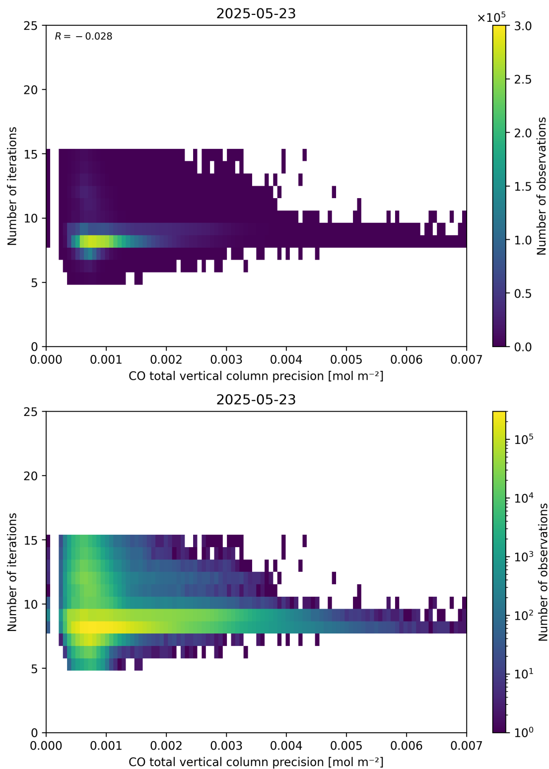
Figure 46: Scatter density plot of “CO total vertical column precision” against “Number of iterations” for 2025-05-22 to 2025-05-24.
