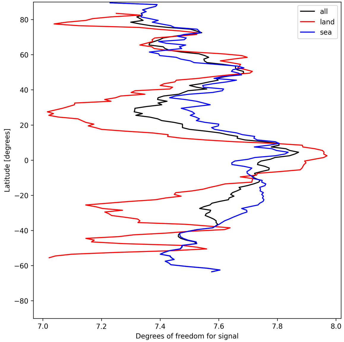
Figure 15: Zonal average of “Degrees of freedom for signal” for 2025-05-22 to 2025-05-24.
