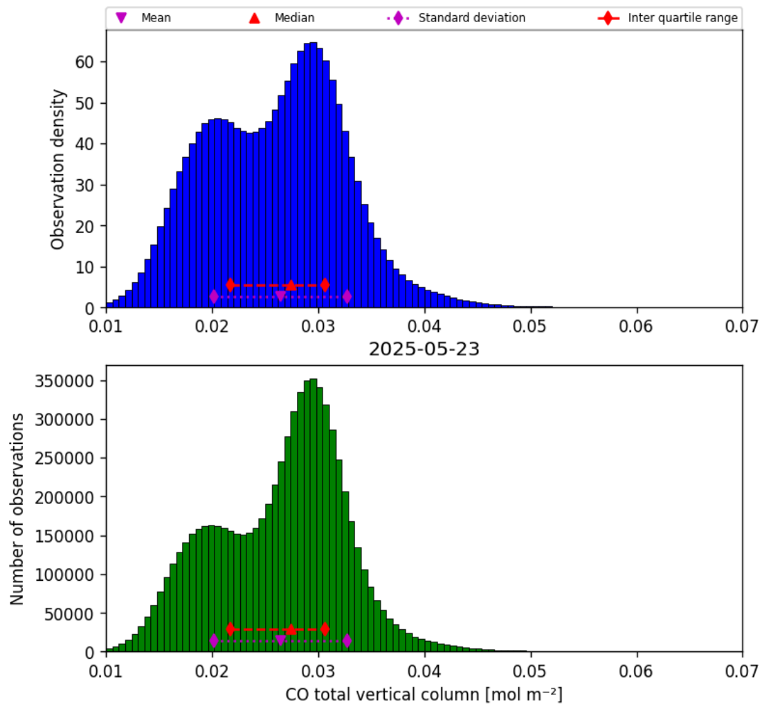
Figure 18: Histogram of “CO total vertical column” for 2025-05-22 to 2025-05-24
