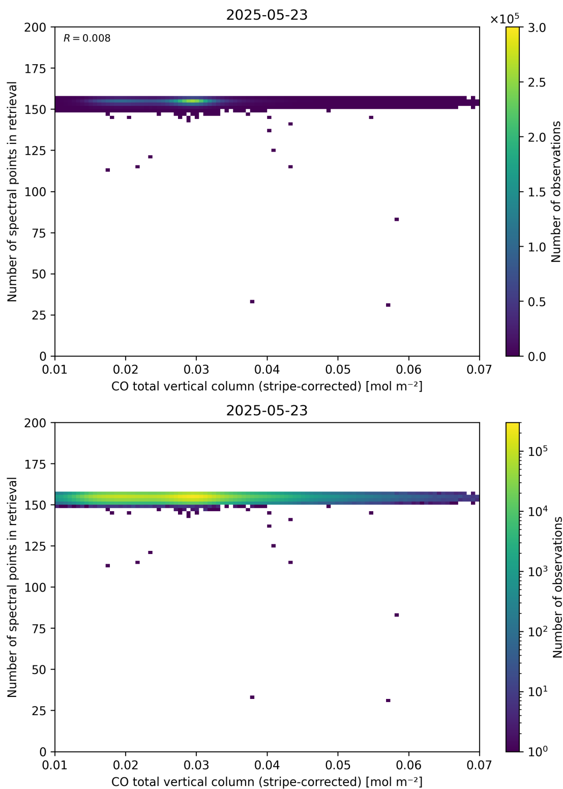
Figure 40: Scatter density plot of “CO total vertical column (stripe-corrected)” against “Number of spectral points in retrieval” for 2025-05-22 to 2025-05-24.
