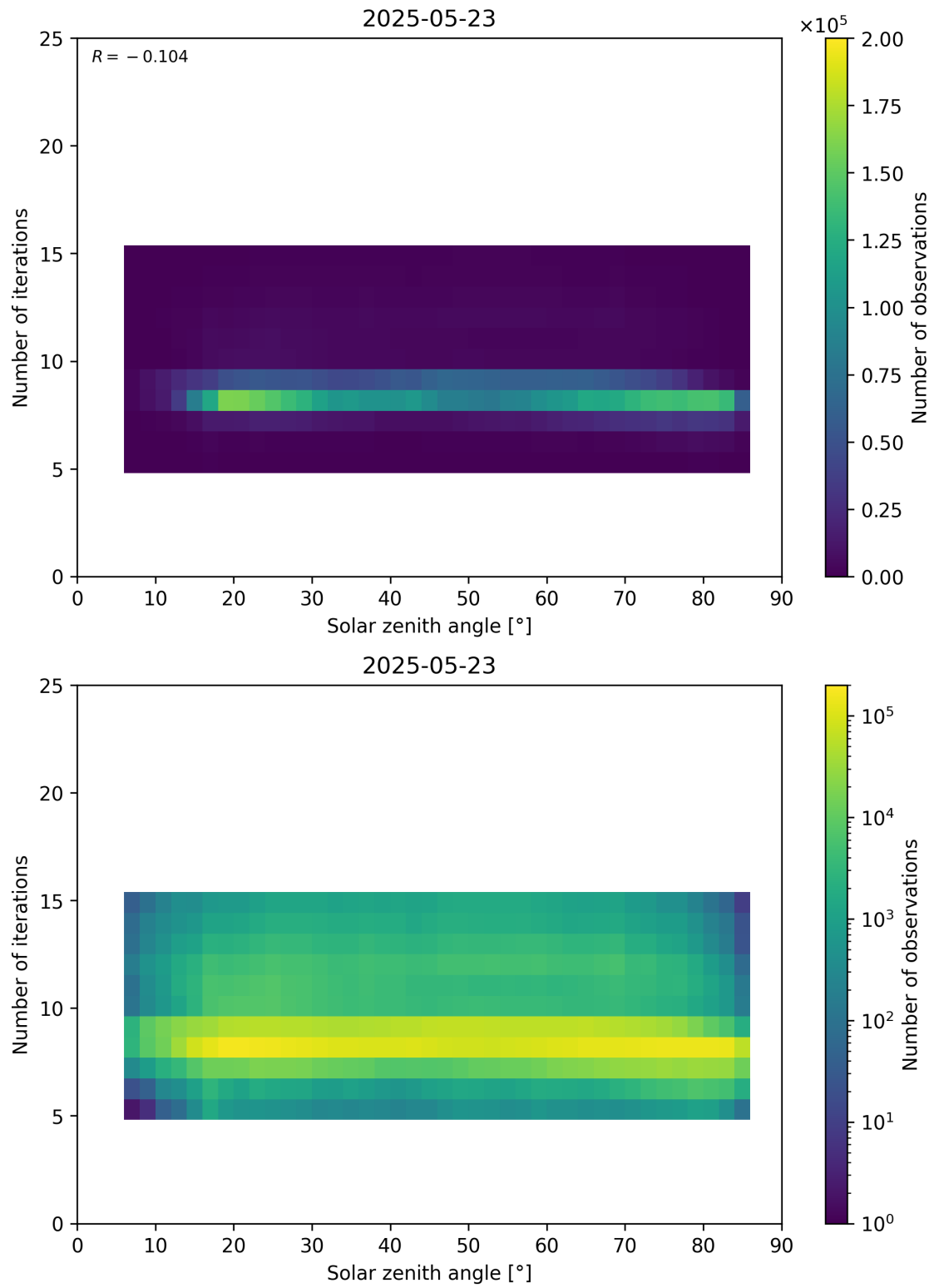
Figure 67: Scatter density plot of “Solar zenith angle” against “Number of iterations” for 2025-05-22 to 2025-05-24.
