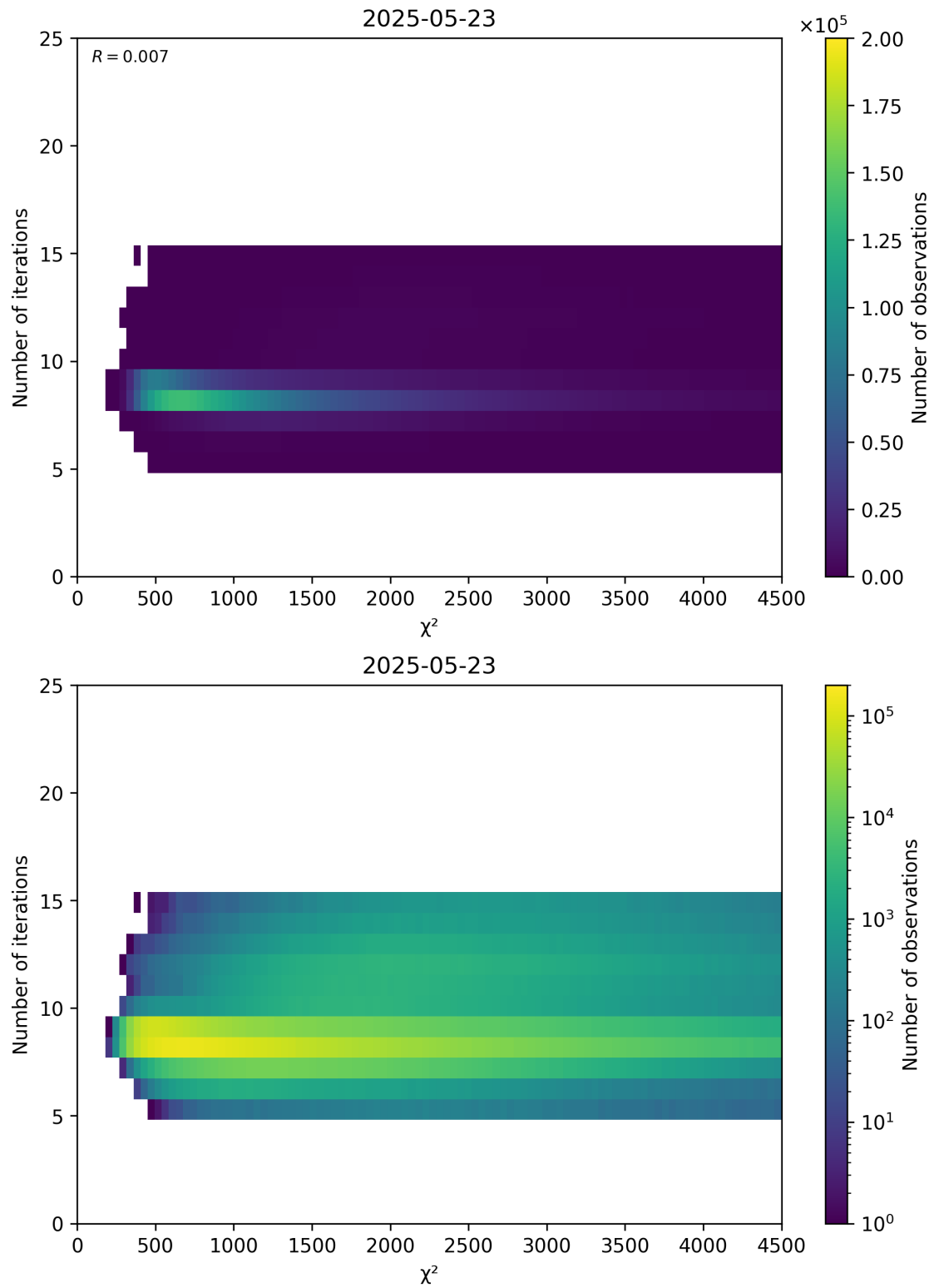
Figure 49: Scatter density plot of “ \chi^2 ” against “Number of iterations” for 2025-05-22 to 2025-05-24.
