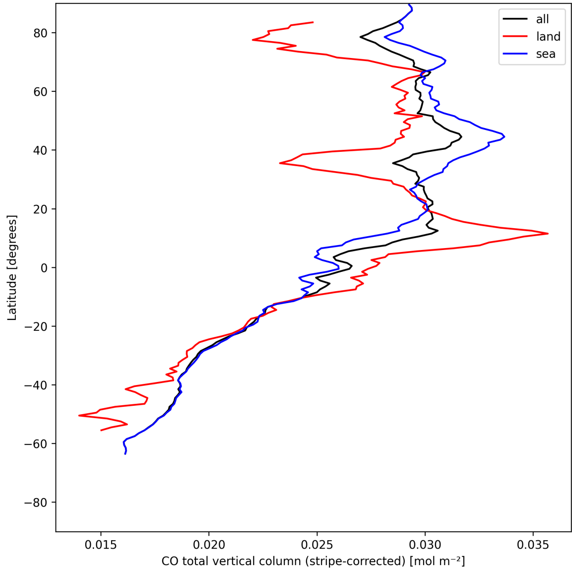
Figure 11: Zonal average of “CO total vertical column (stripe-corrected)” for 2025-05-22 to 2025-05-24.
