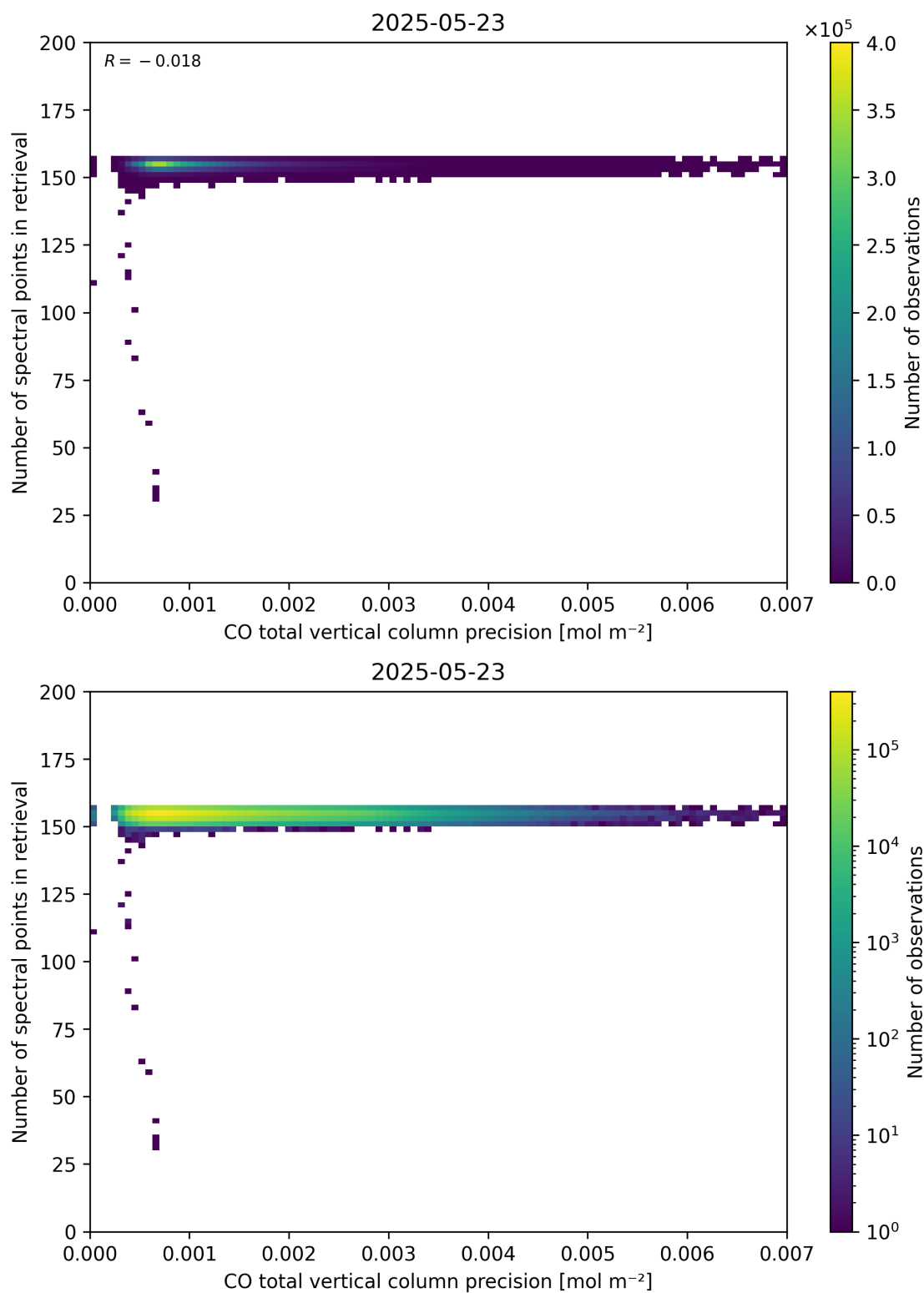
Figure 47: Scatter density plot of “CO total vertical column precision” against “Number of spectral points in retrieval” for 2025-05-22 to 2025-05-24.
