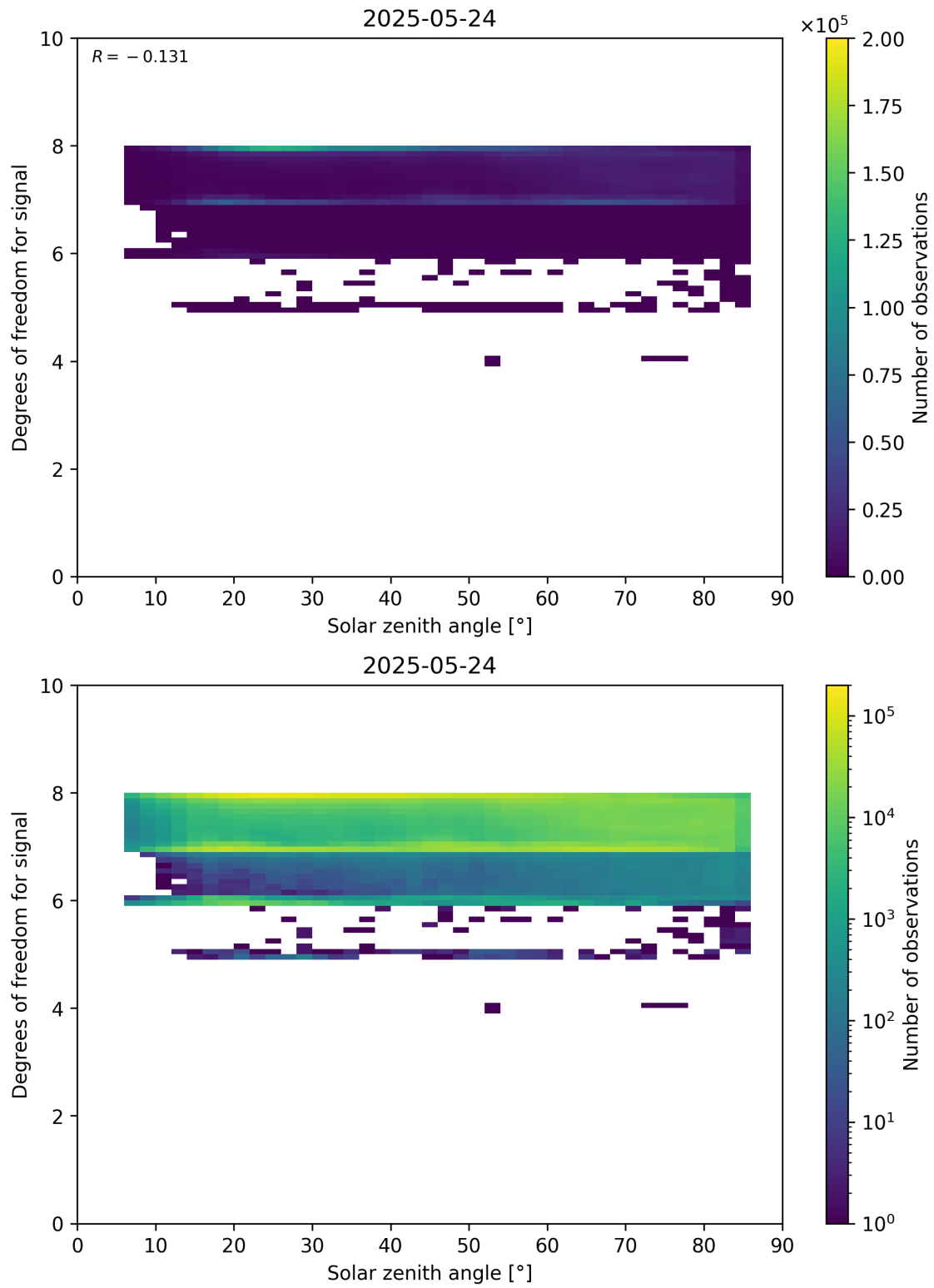
Figure 65: Scatter density plot of “Solar zenith angle” against “Degrees of freedom for signal” for 2025-05-23 to 2025-05-25.
