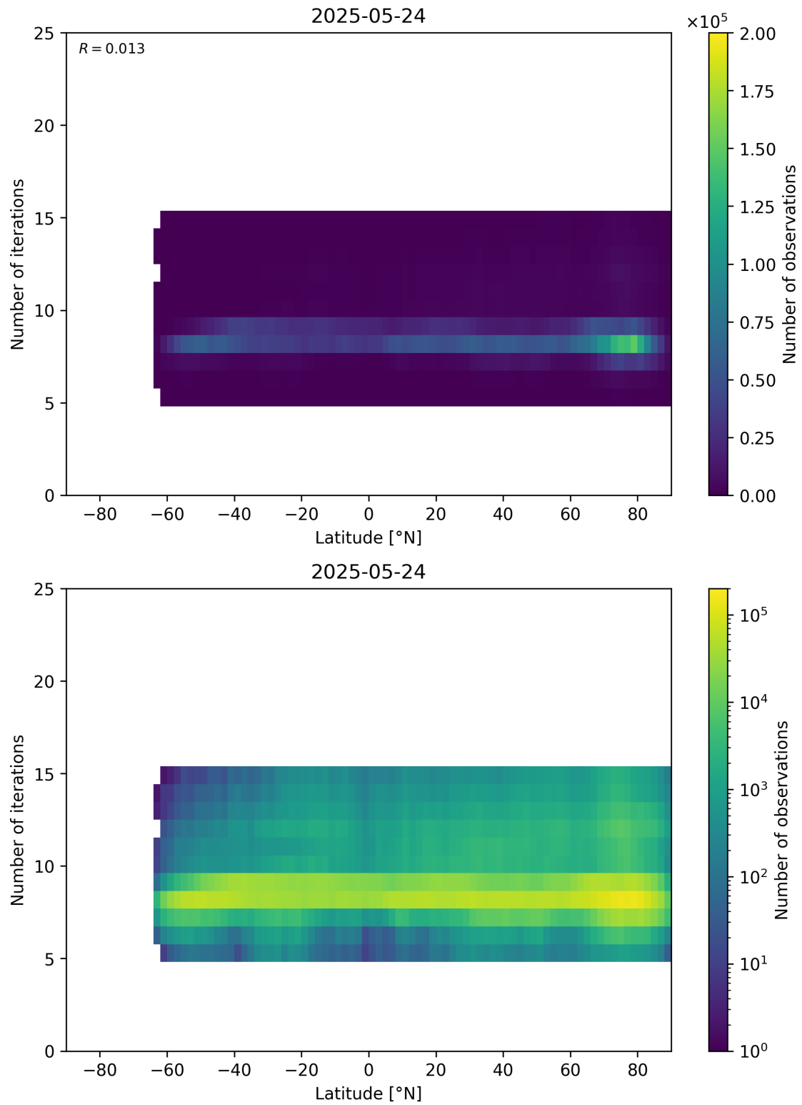
Figure 56: Scatter density plot of “Latitude” against “Number of iterations” for 2025-05-23 to 2025-05-25.
