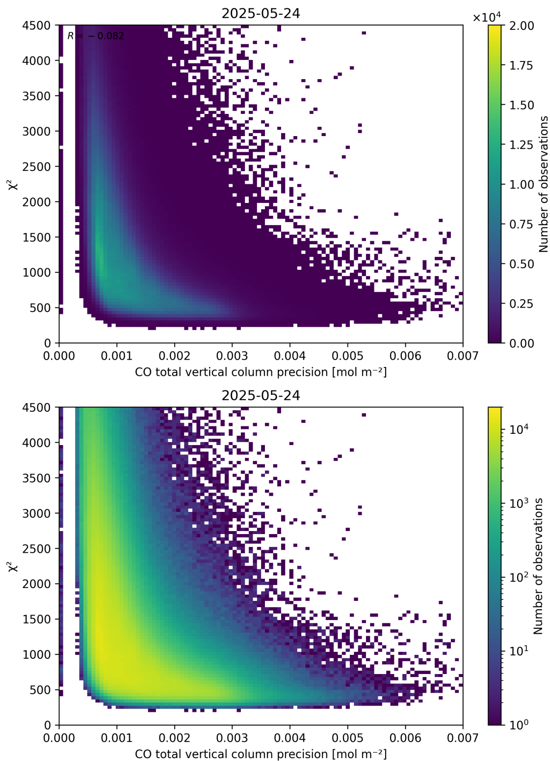
Figure 44: Scatter density plot of “CO total vertical column precision” against “ \chi^2 ” for 2025-05-23 to 2025-05-25.
