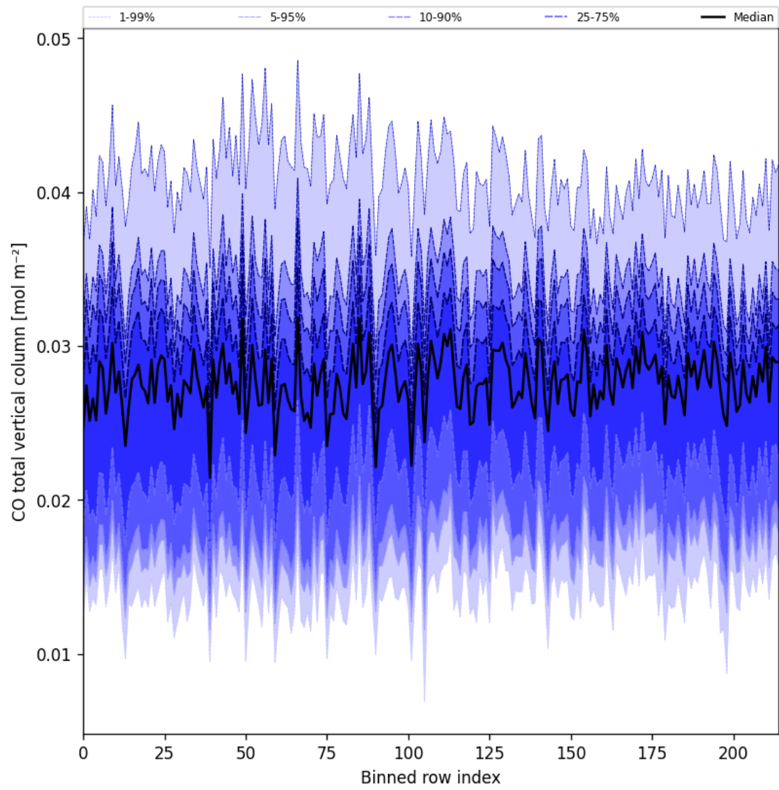
Figure 26: Along track statistics of “CO total vertical column” for 2025-05-23 to 2025-05-25
