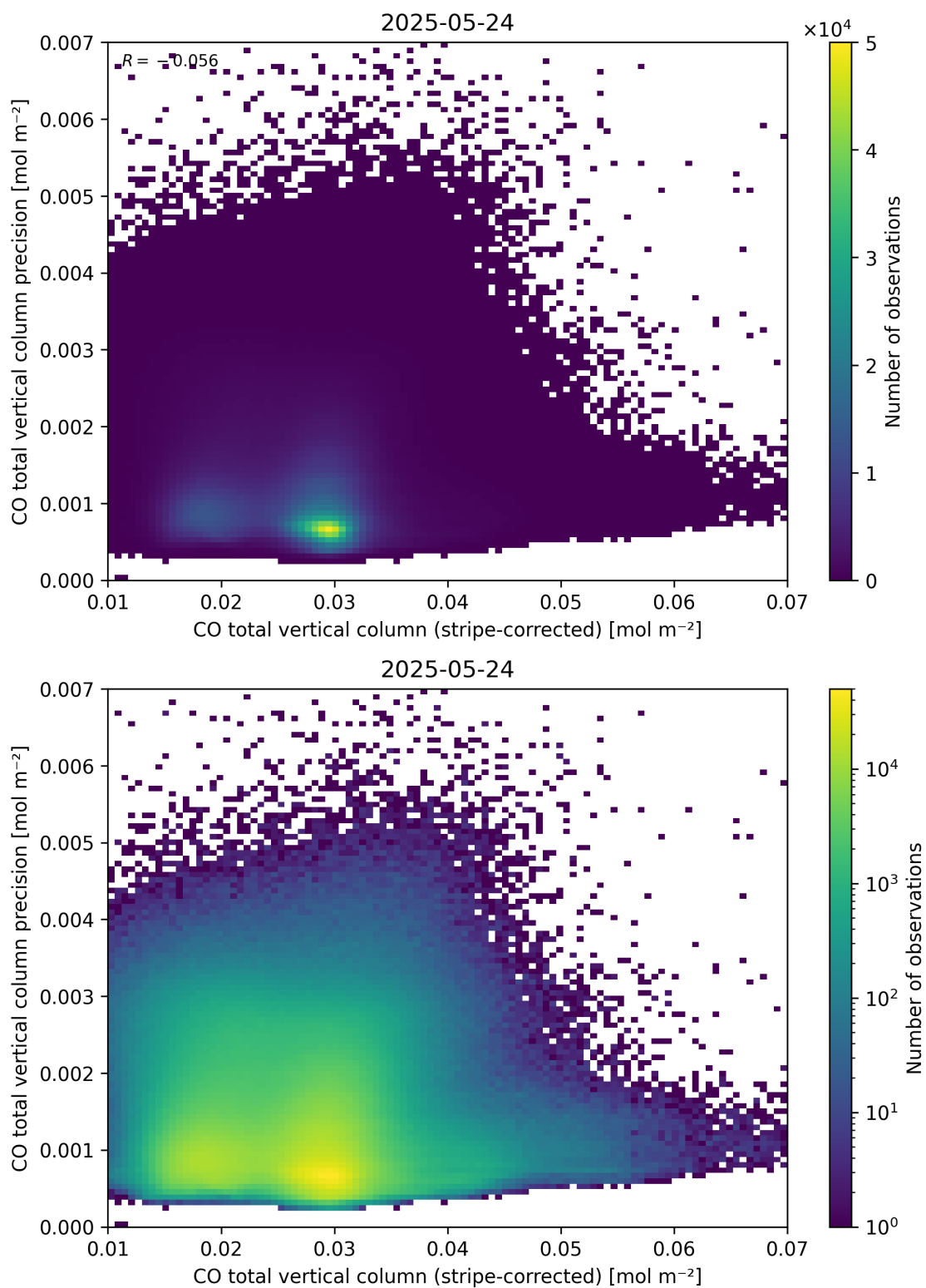
Figure 36: Scatter density plot of “CO total vertical column (stripe-corrected)” against “CO total vertical column precision” for 2025-05-23 to 2025-05-25.
