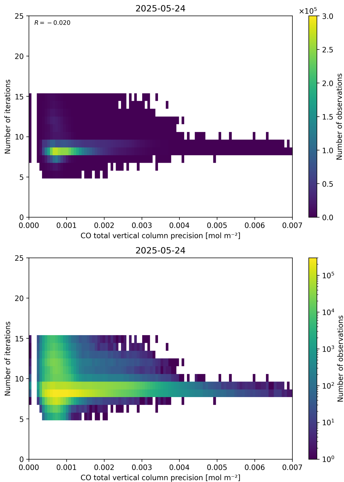
Figure 46: Scatter density plot of “CO total vertical column precision” against “Number of iterations” for 2025-05-23 to 2025-05-25.
