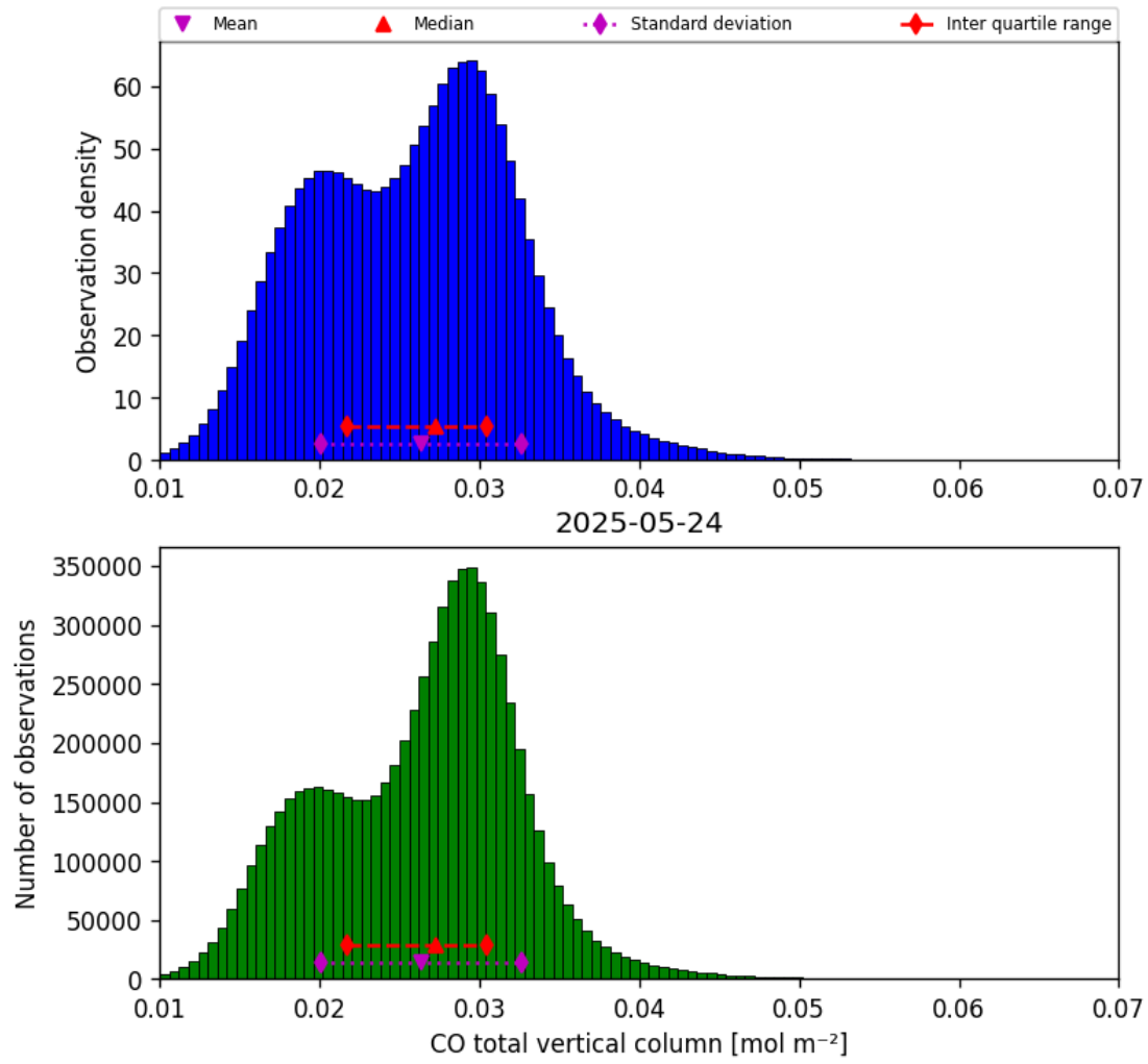
Figure 18: Histogram of “CO total vertical column” for 2025-05-23 to 2025-05-25
