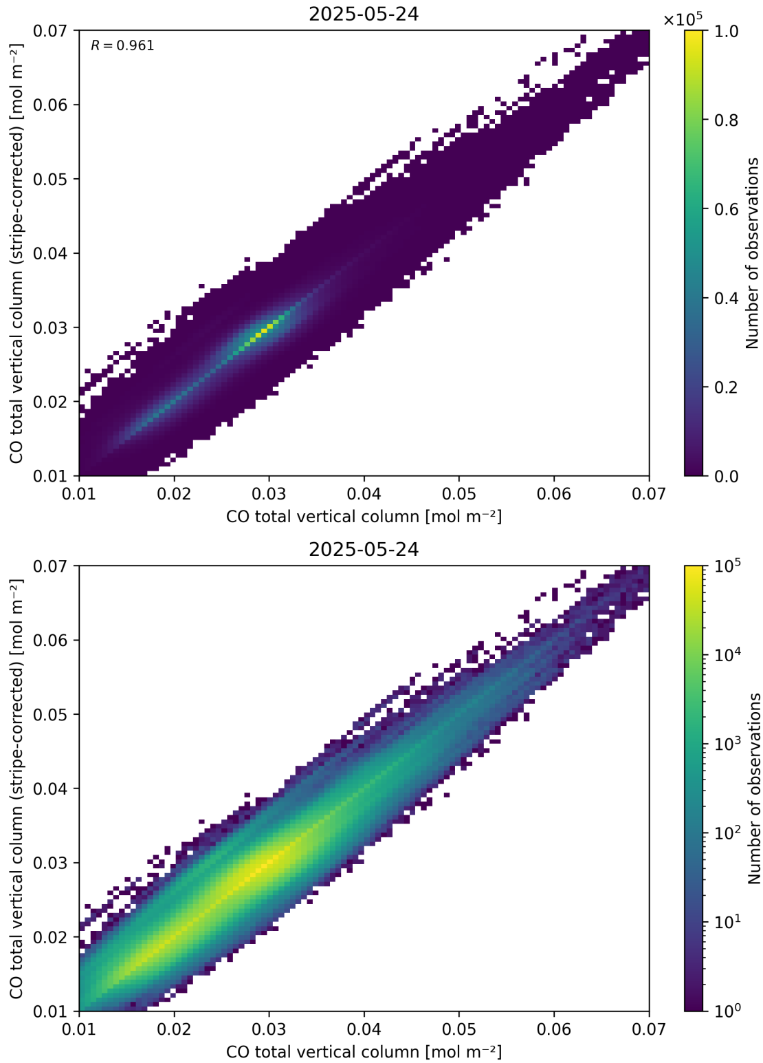
Figure 33: Scatter density plot of “CO total vertical column” against “CO total vertical column (stripe-corrected)” for 2025-05-23 to 2025-05-25.
