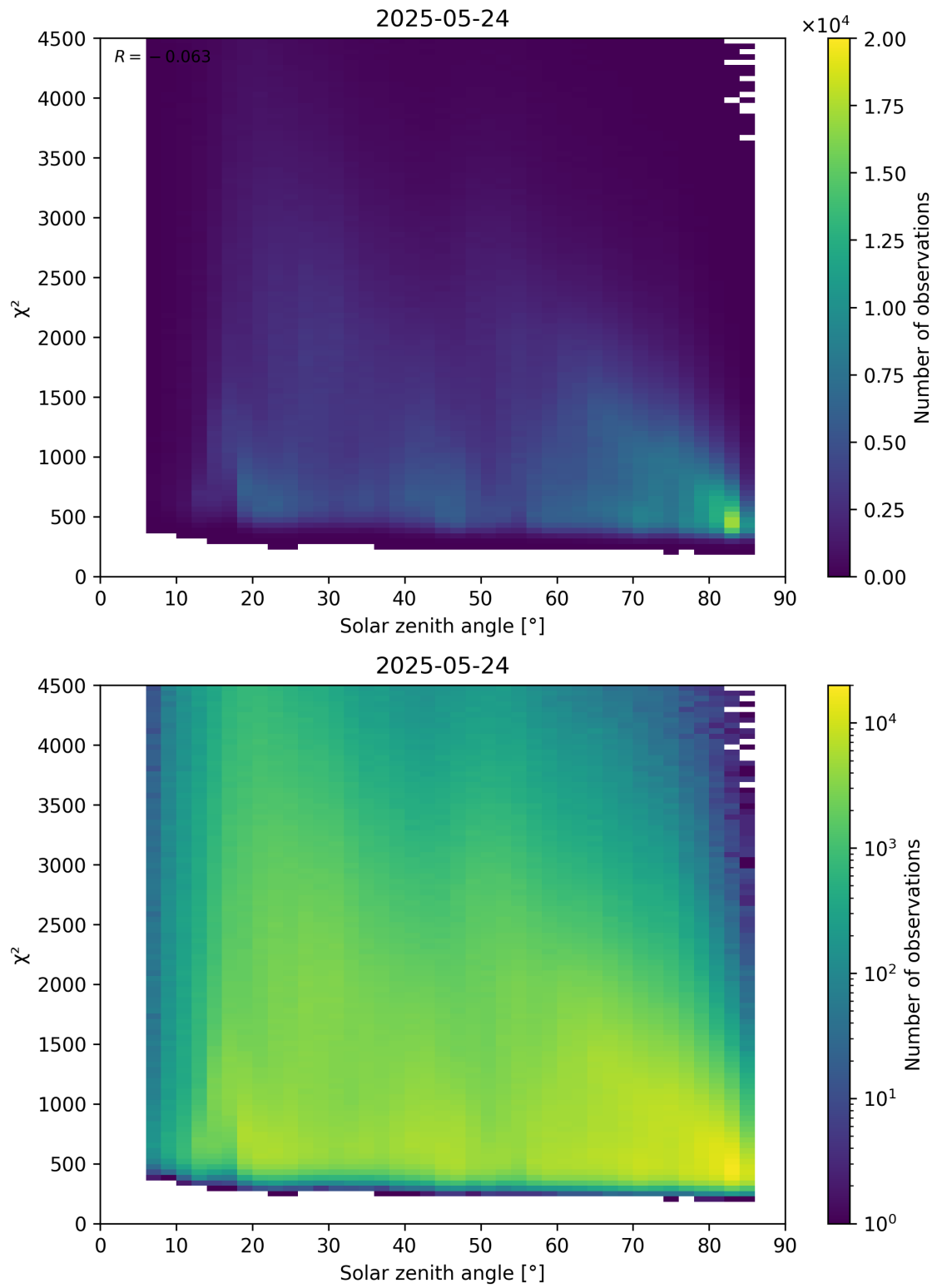
Figure 64: Scatter density plot of “Solar zenith angle” against “ \chi^2 ” for 2025-05-23 to 2025-05-25.
