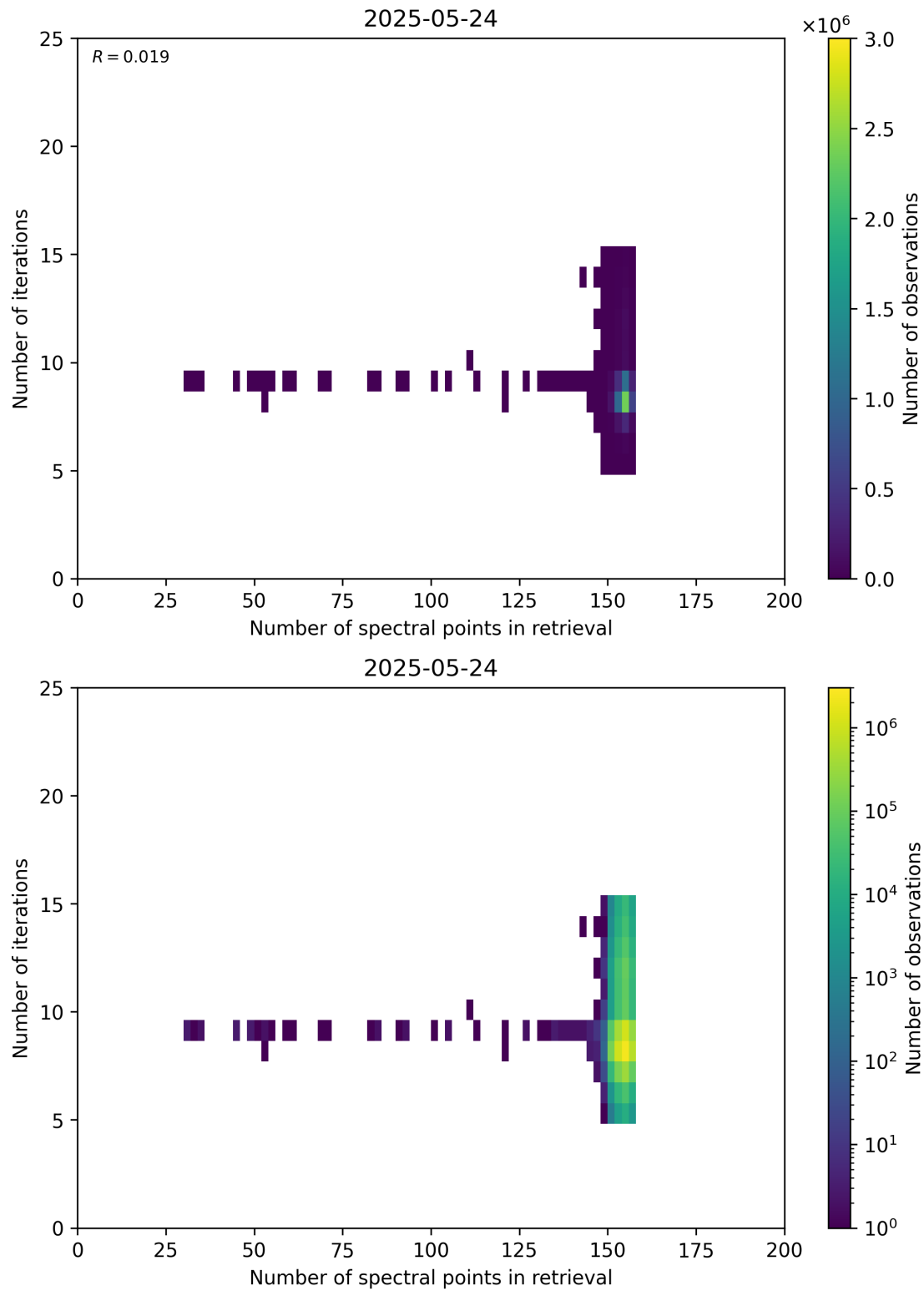
Figure 60: Scatter density plot of “Number of spectral points in retrieval” against “Number of iterations” for 2025-05-23 to 2025-05-25.
