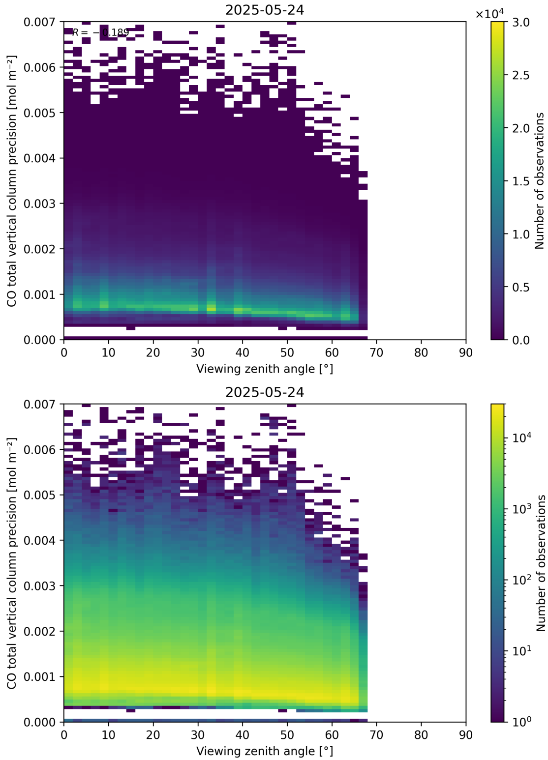
Figure 71: Scatter density plot of “Viewing zenith angle” against “CO total vertical column precision” for 2025-05-23 to 2025-05-25.
