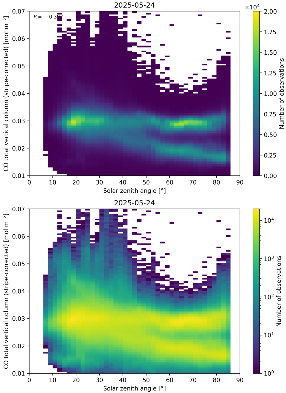
Figure 62: Scatter density plot of “Solar zenith angle” against “CO total vertical column (stripe-corrected)” for 2025-05-23 to 2025-05-25.
