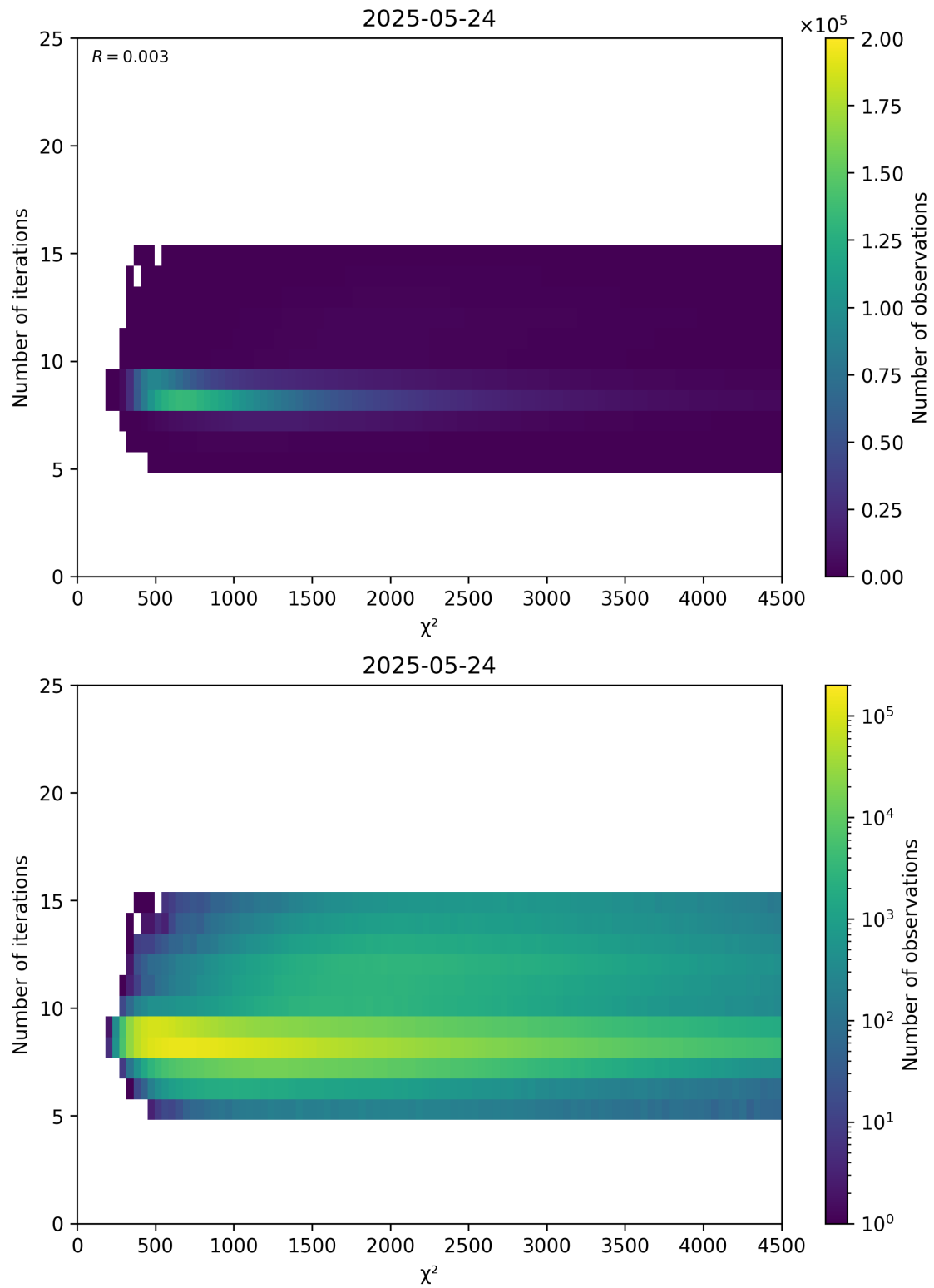
Figure 49: Scatter density plot of “ \chi^2 ” against “Number of iterations” for 2025-05-23 to 2025-05-25.
