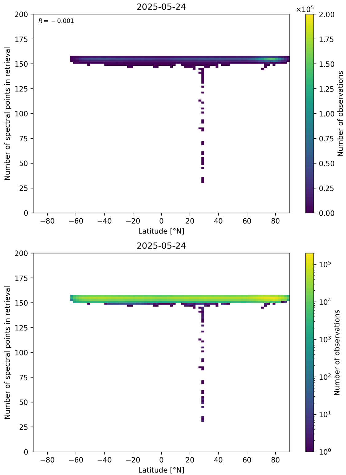
Figure 57: Scatter density plot of “Latitude” against “Number of spectral points in retrieval” for 2025-05-23 to 2025-05-25.
