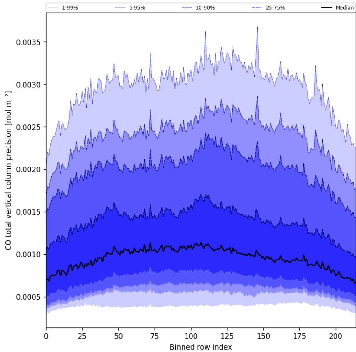
Figure 28: Along track statistics of “CO total vertical column precision” for 2025-05-23 to 2025-05-25
