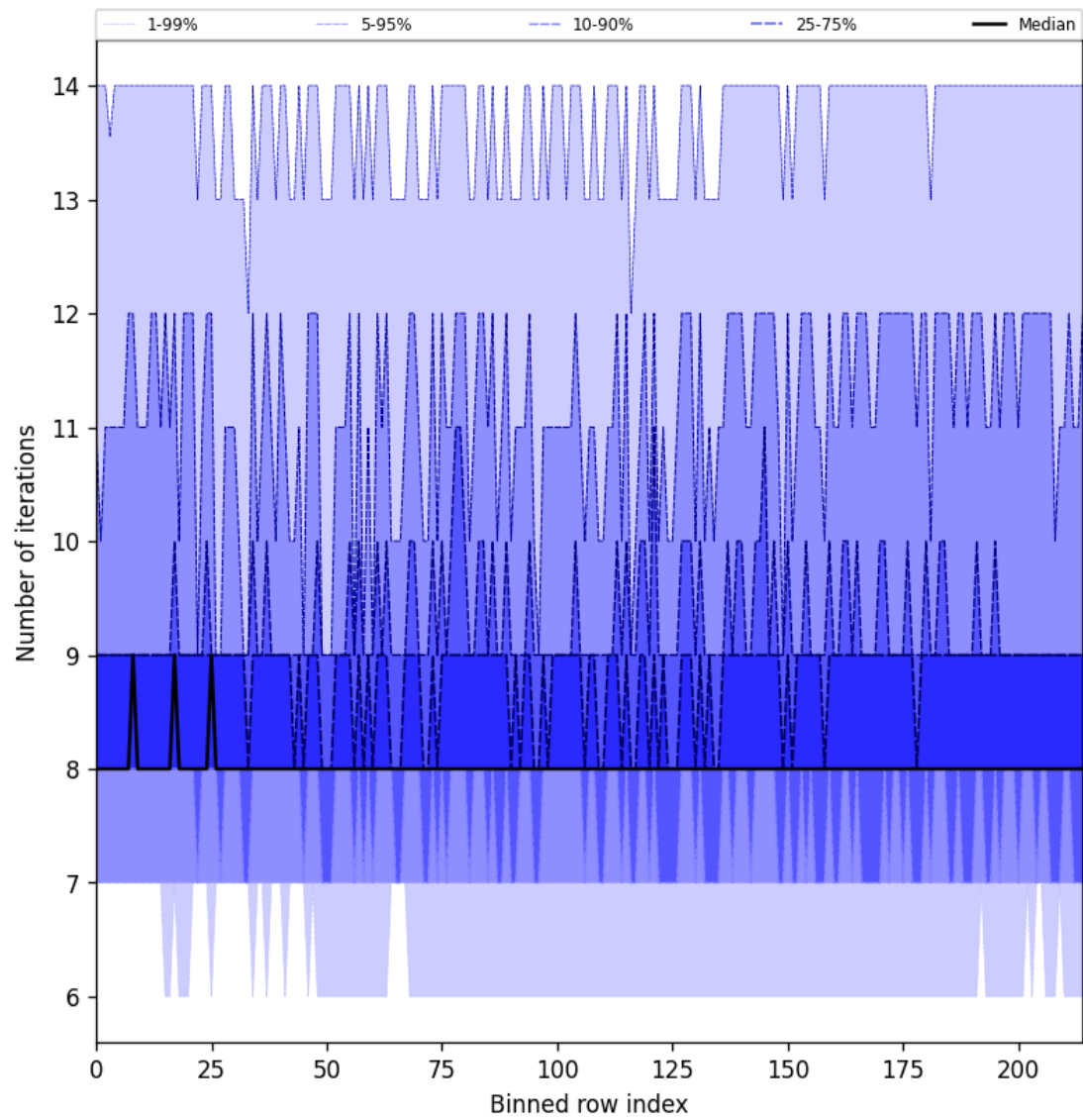
Figure 32: Along track statistics of “Number of iterations” for 2025-05-23 to 2025-05-25
