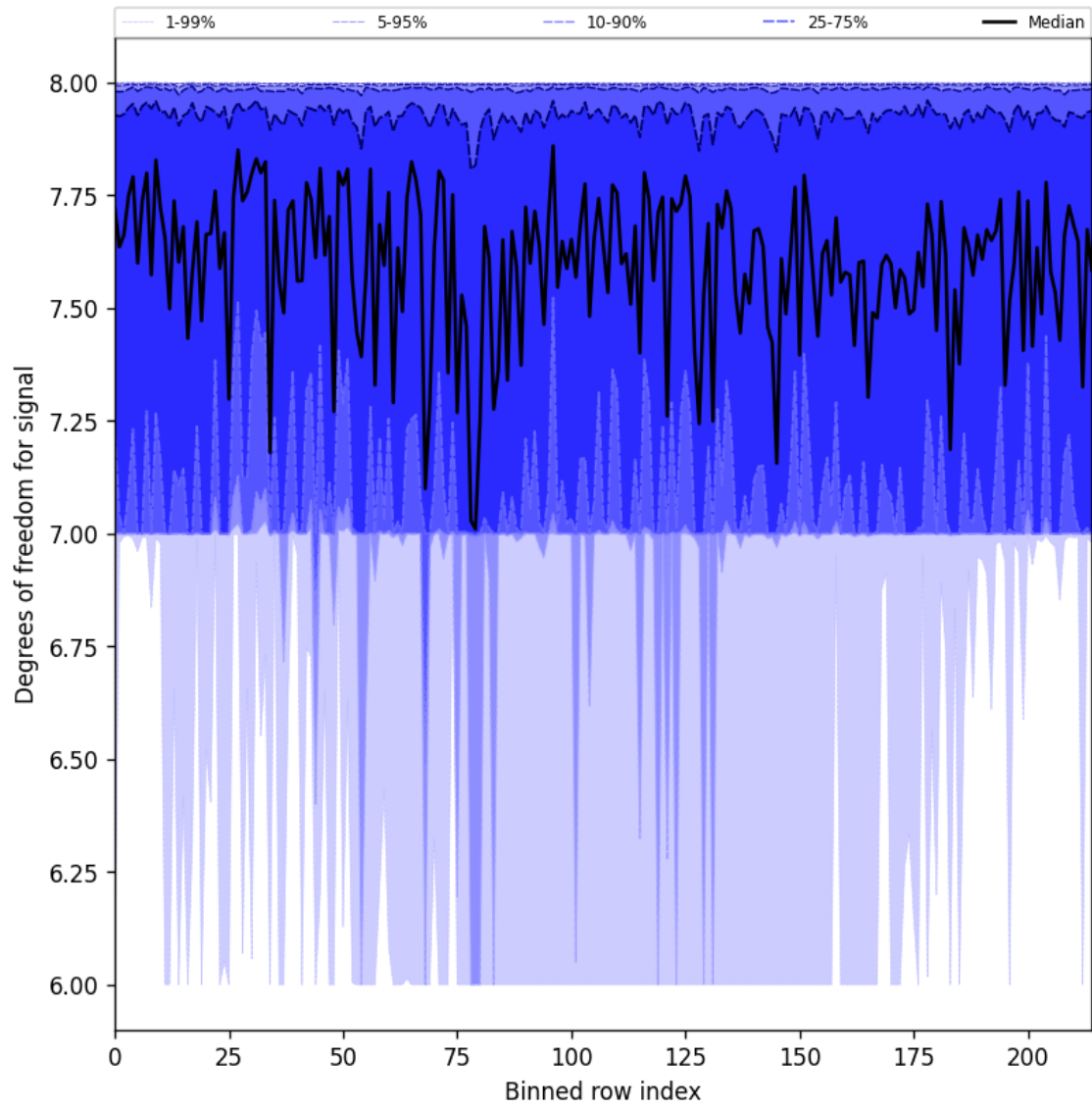
Figure 31: Along track statistics of “Degrees of freedom for signal” for 2025-05-23 to 2025-05-25
