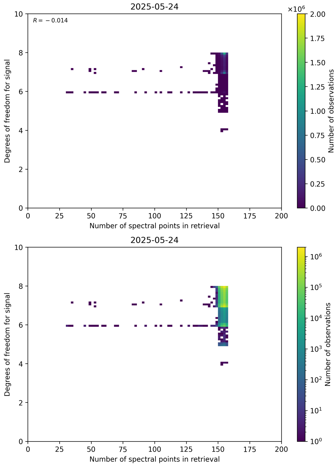
Figure 59: Scatter density plot of “Number of spectral points in retrieval” against “Degrees of freedom for signal” for 2025-05-23 to 2025-05-25.
