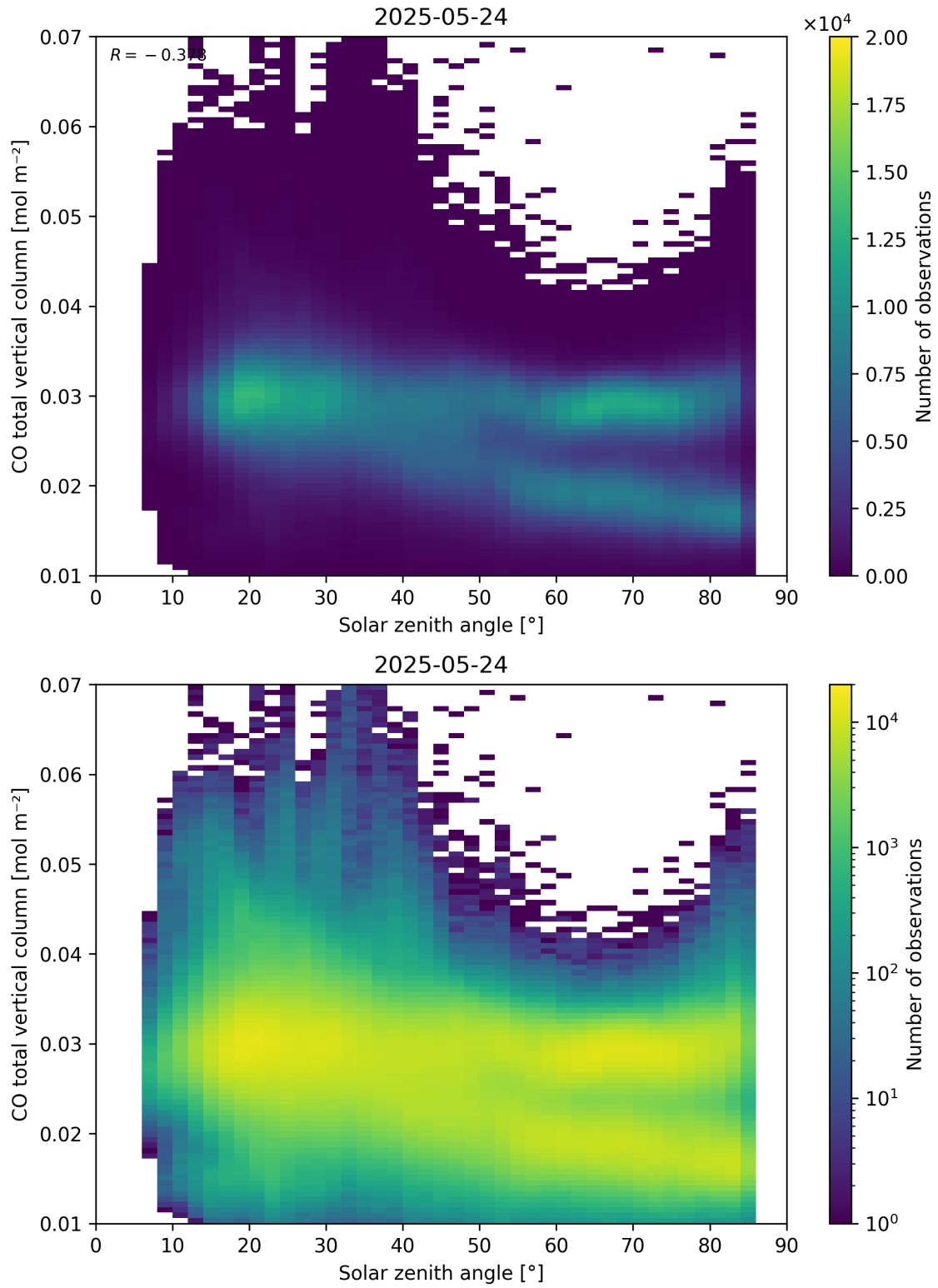
Figure 61: Scatter density plot of “Solar zenith angle” against “CO total vertical column” for 2025-05-23 to 2025-05-25.
