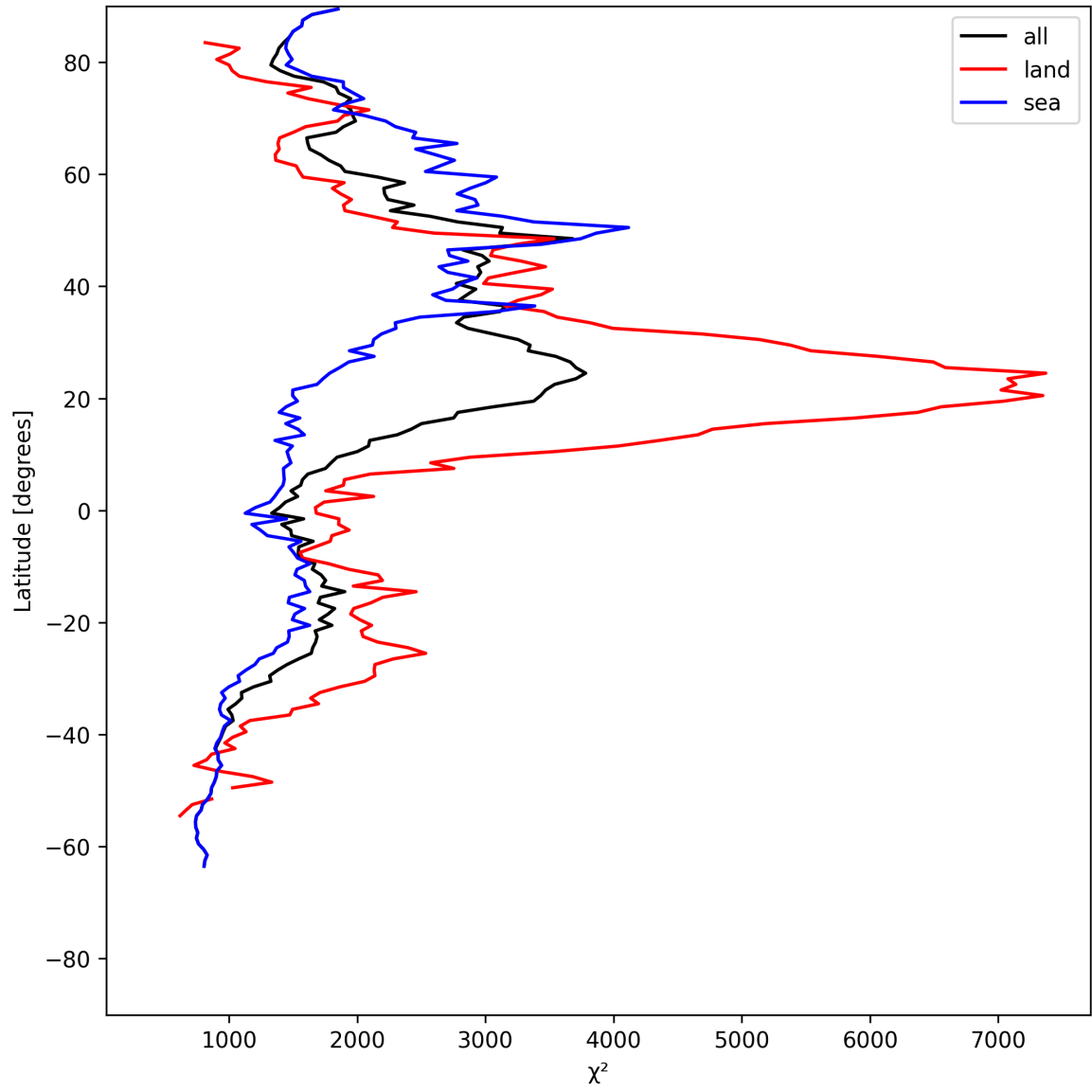
Figure 14: Zonal average of “ \chi^2 ” for 2025-05-23 to 2025-05-25.
