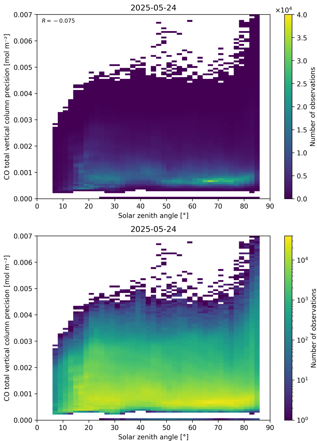
Figure 63: Scatter density plot of “Solar zenith angle” against “CO total vertical column precision” for 2025-05-23 to 2025-05-25.
