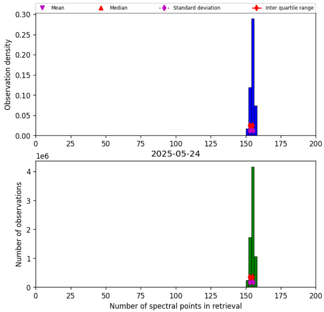
Figure 21: Histogram of “Number of spectral points in retrieval” for 2025-05-23 to 2025-05-25
