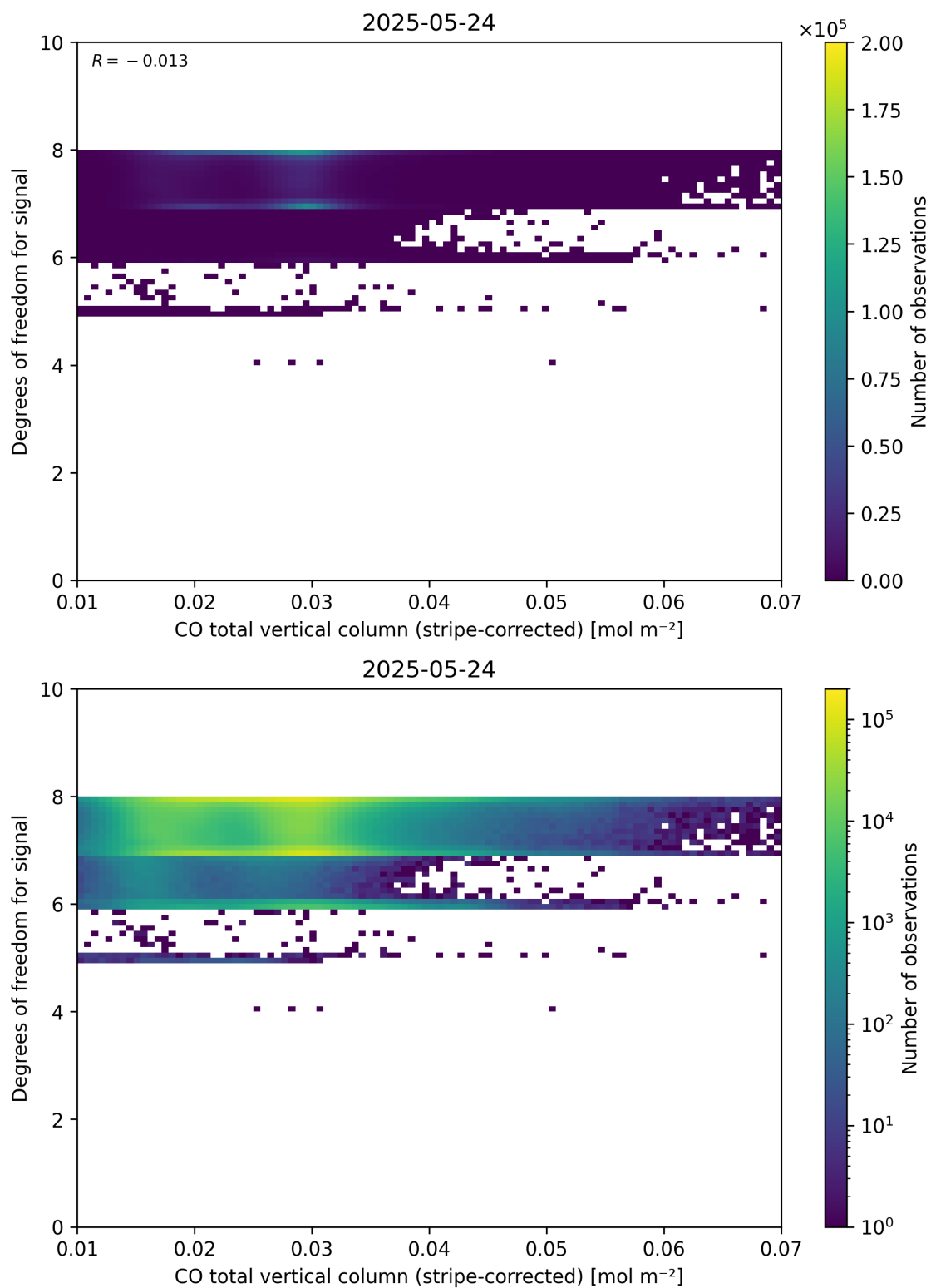
Figure 38: Scatter density plot of “CO total vertical column (stripe-corrected)” against “Degrees of freedom for signal” for 2025-05-23 to 2025-05-25.
