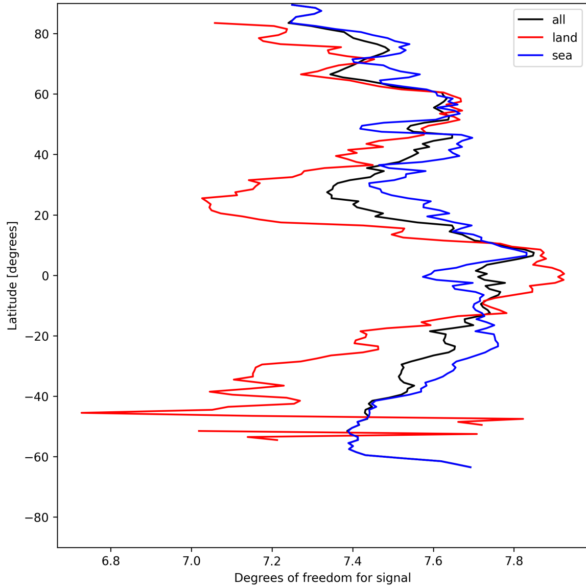
Figure 15: Zonal average of “Degrees of freedom for signal” for 2025-05-23 to 2025-05-25.
