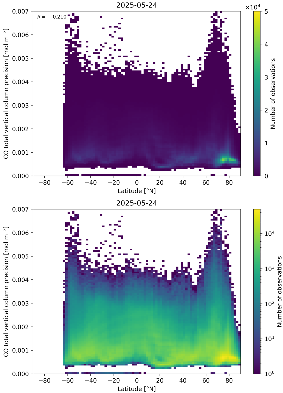
Figure 53: Scatter density plot of “Latitude” against “CO total vertical column precision” for 2025-05-23 to 2025-05-25.
