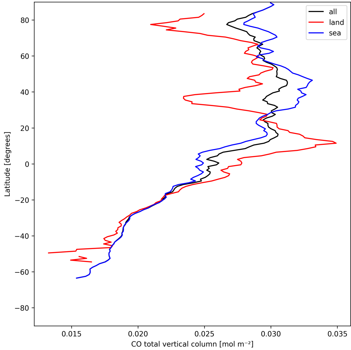
Figure 10: Zonal average of “CO total vertical column” for 2025-05-23 to 2025-05-25.
