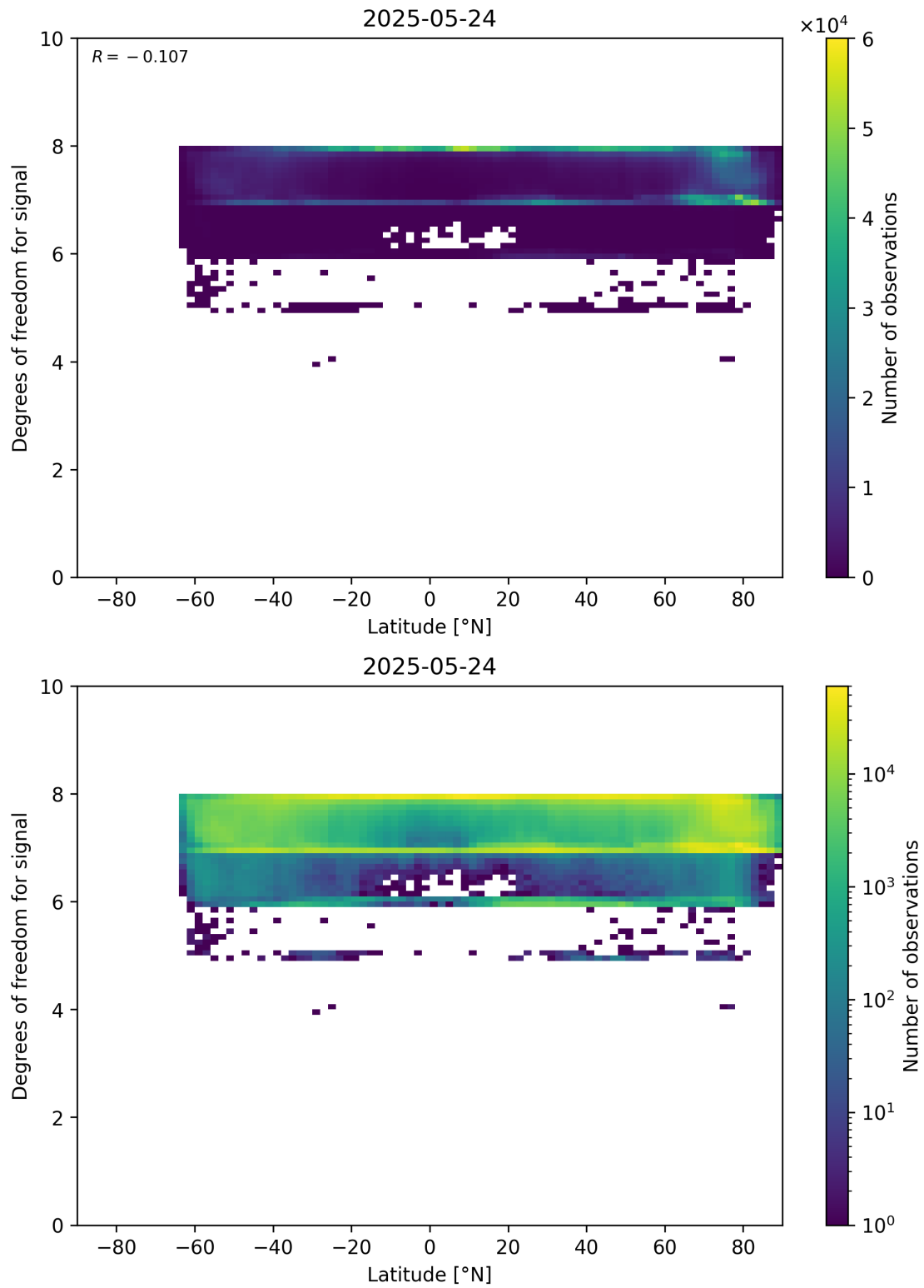
Figure 55: Scatter density plot of “Latitude” against “Degrees of freedom for signal” for 2025-05-23 to 2025-05-25.
