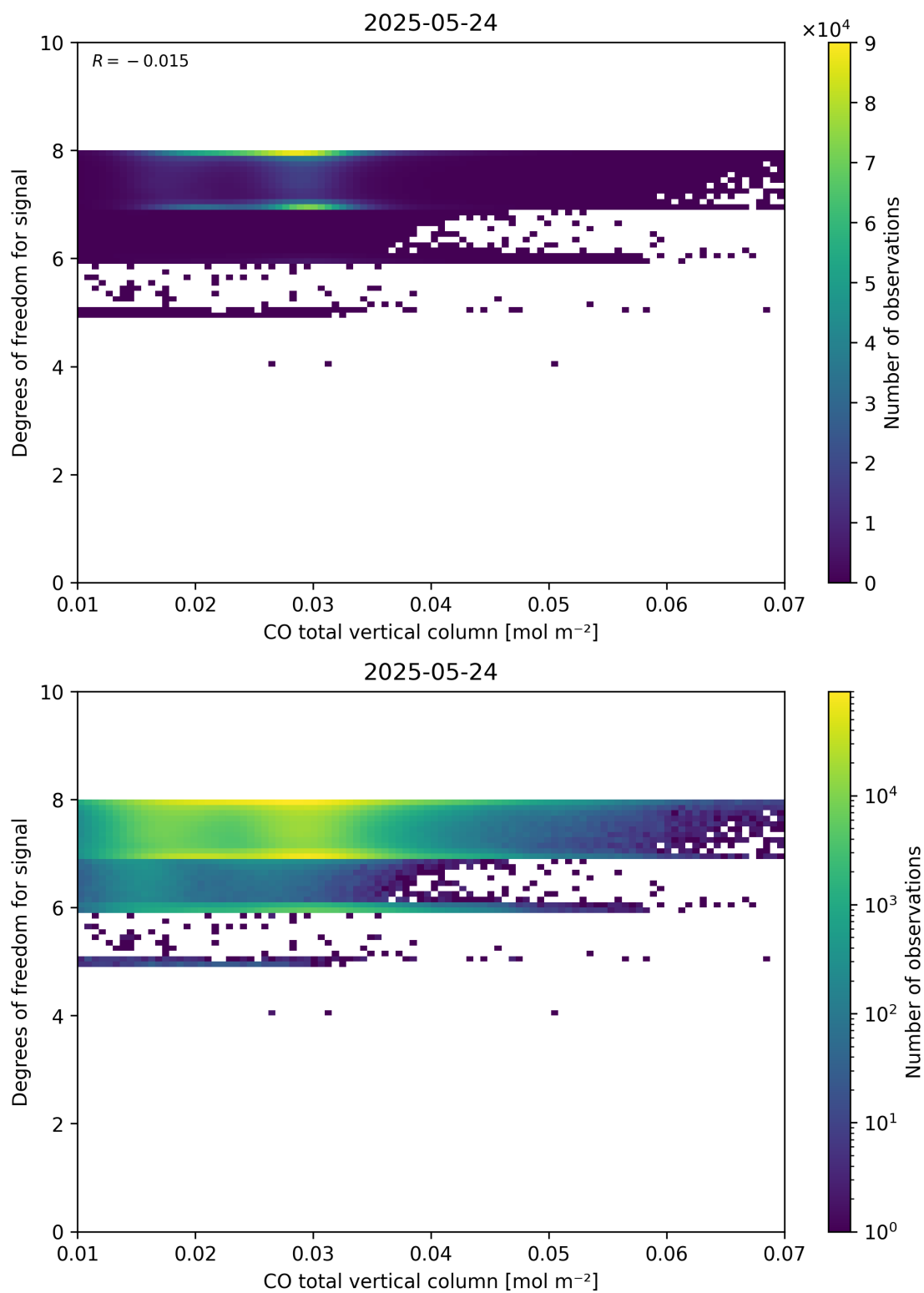
Figure 41: Scatter density plot of “CO total vertical column” against “Degrees of freedom for signal” for 2025-05-23 to 2025-05-25.
