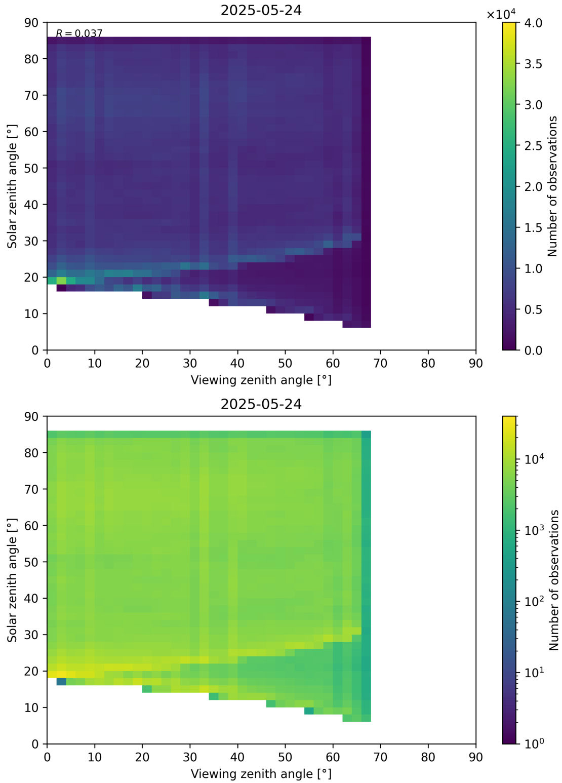
Figure 77: Scatter density plot of “Viewing zenith angle” against “Solar zenith angle” for 2025-05-23 to 2025-05-25.
