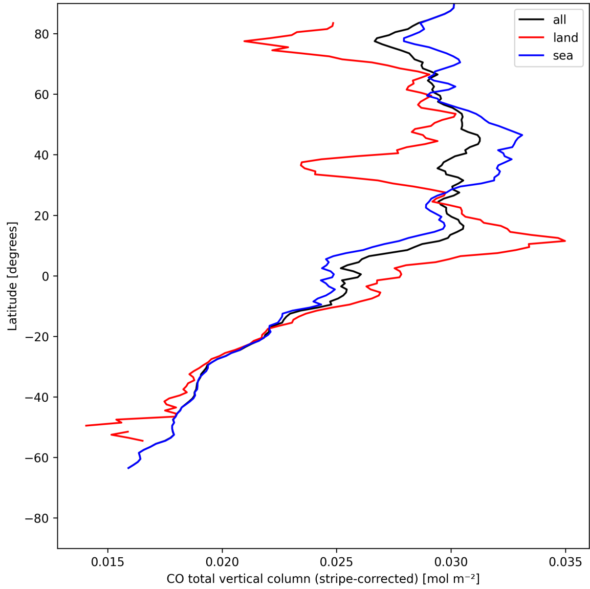
Figure 11: Zonal average of “CO total vertical column (stripe-corrected)” for 2025-05-23 to 2025-05-25.
