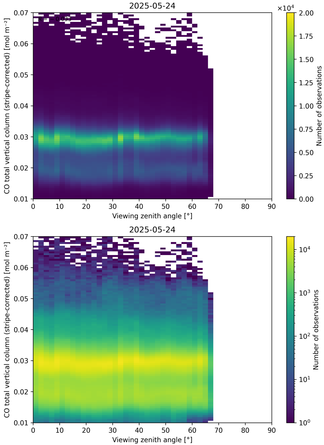
Figure 70: Scatter density plot of “Viewing zenith angle” against “CO total vertical column (stripe-corrected)” for 2025-05-23 to 2025-05-25.
