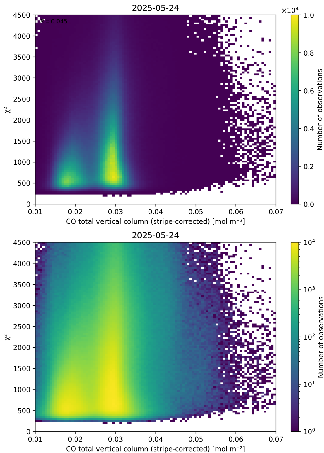
Figure 37: Scatter density plot of “CO total vertical column (stripe-corrected)” against “ \chi^2 ” for 2025-05-23 to 2025-05-25.
