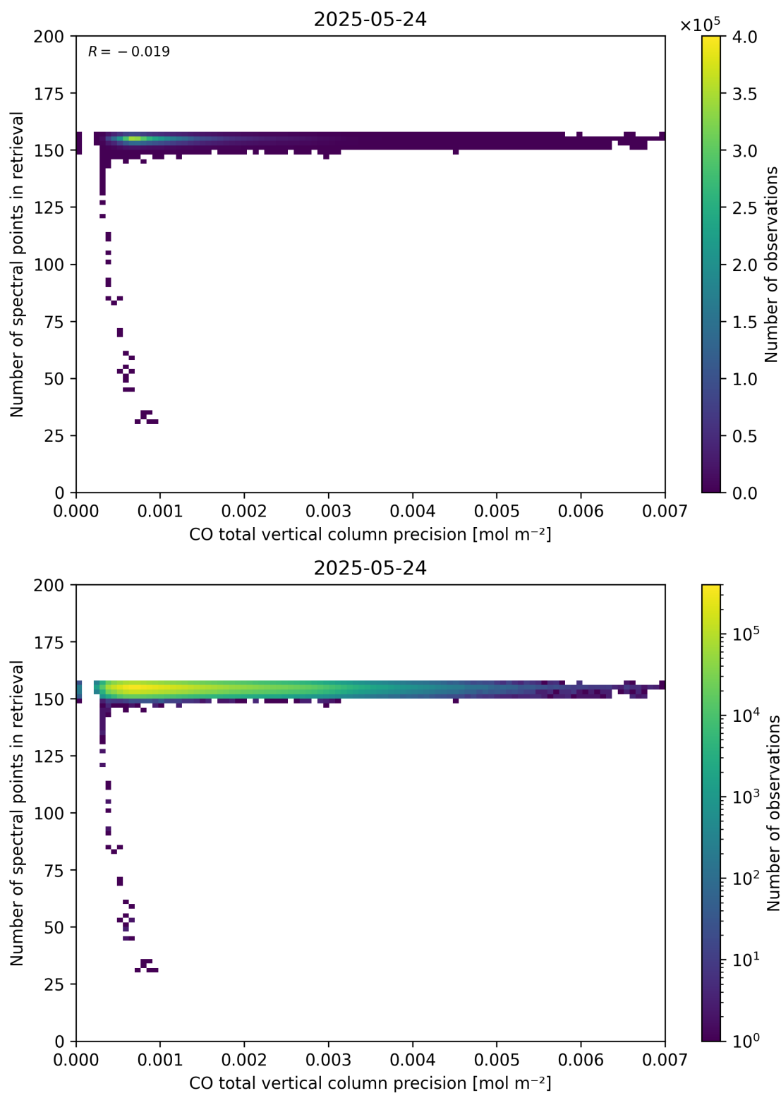
Figure 47: Scatter density plot of “CO total vertical column precision” against “Number of spectral points in retrieval” for 2025-05-23 to 2025-05-25.
