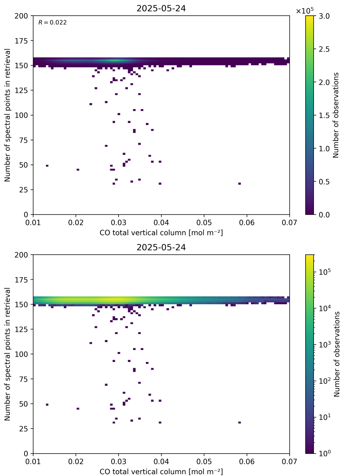
Figure 43: Scatter density plot of “CO total vertical column” against “Number of spectral points in retrieval” for 2025-05-23 to 2025-05-25.
