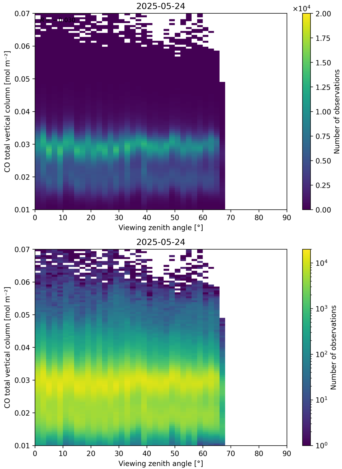
Figure 69: Scatter density plot of “Viewing zenith angle” against “CO total vertical column” for 2025-05-23 to 2025-05-25.
