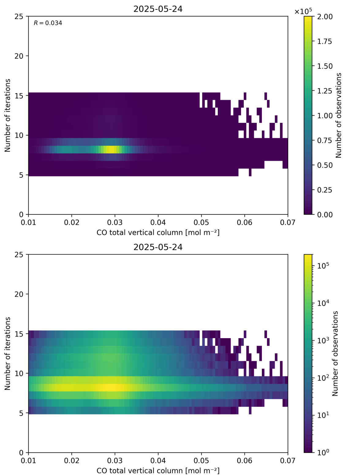
Figure 42: Scatter density plot of “CO total vertical column” against “Number of iterations” for 2025-05-23 to 2025-05-25.
