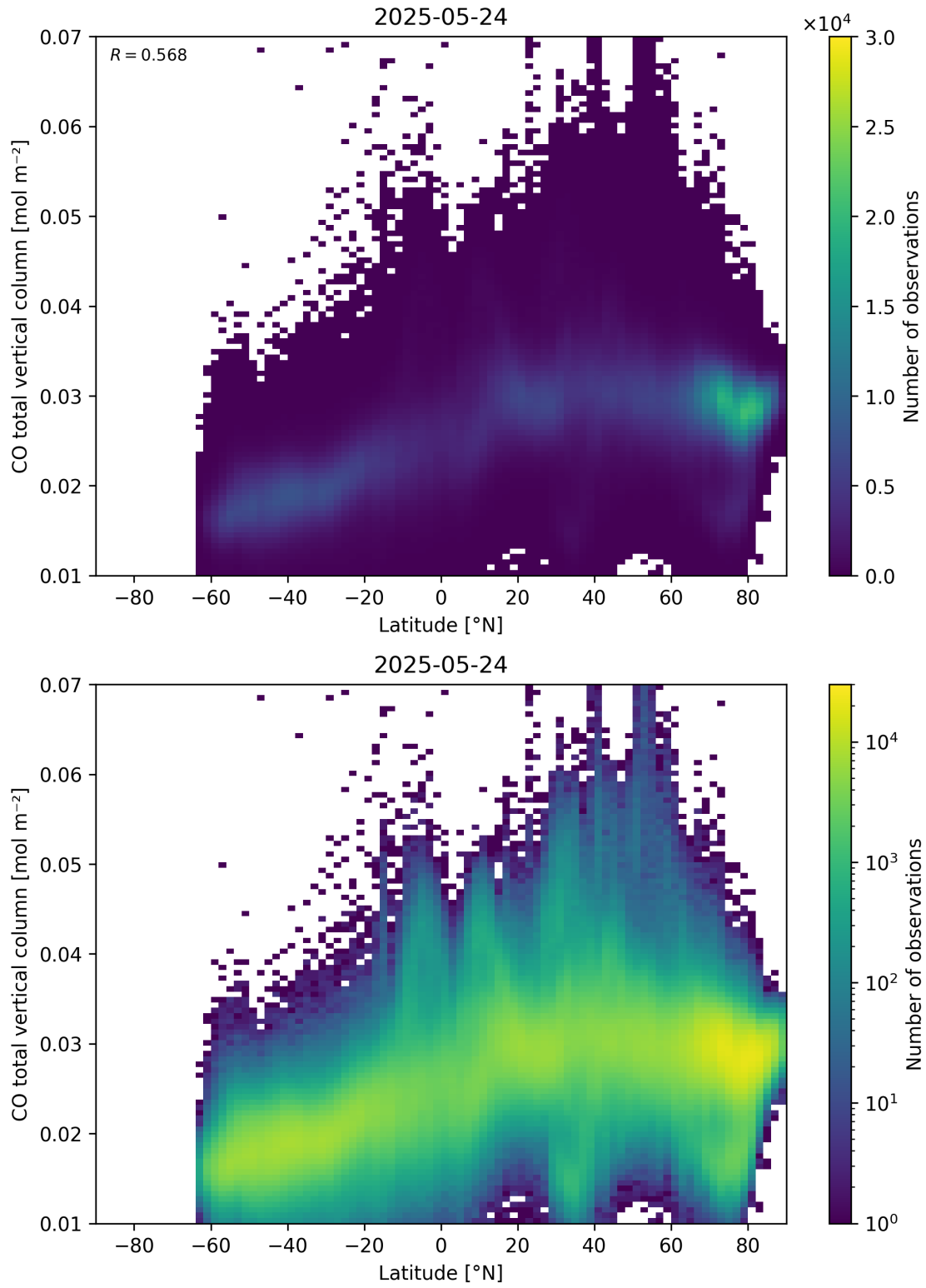
Figure 51: Scatter density plot of “Latitude” against “CO total vertical column” for 2025-05-23 to 2025-05-25.
