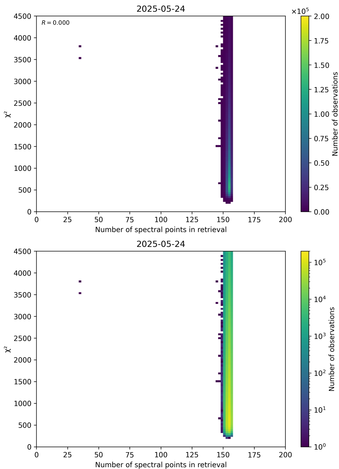
Figure 58: Scatter density plot of “Number of spectral points in retrieval” against “ \chi^2 ” for 2025-05-23 to 2025-05-25.
