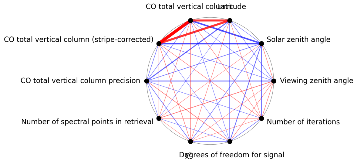
Figure 1: Map of correlation graph for 2025-05-23 to 2025-05-25.
