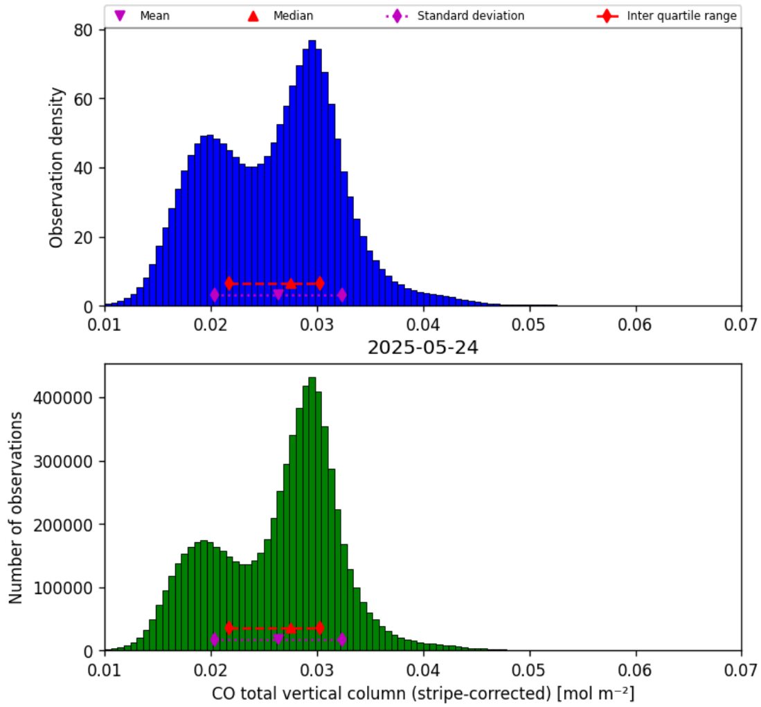
Figure 19: Histogram of “CO total vertical column (stripe-corrected)” for 2025-05-23 to 2025-05-25
