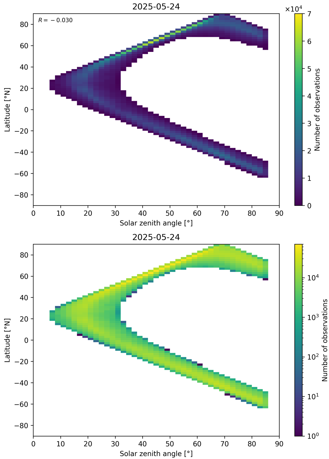
Figure 66: Scatter density plot of “Solar zenith angle” against “Latitude” for 2025-05-23 to 2025-05-25.
