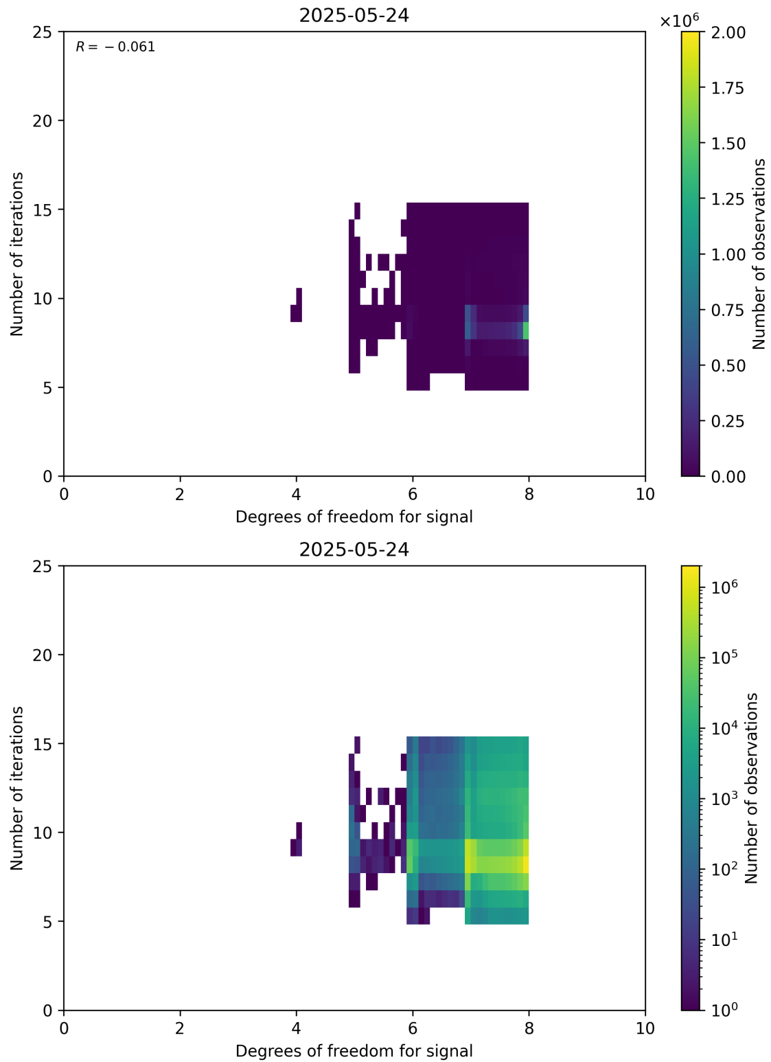
Figure 50: Scatter density plot of “Degrees of freedom for signal” against “Number of iterations” for 2025-05-23 to 2025-05-25.
