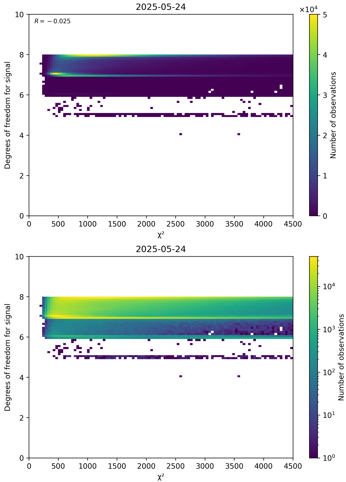
Figure 48: Scatter density plot of “ \chi^2 ” against “Degrees of freedom for signal” for 2025-05-23 to 2025-05-25.
