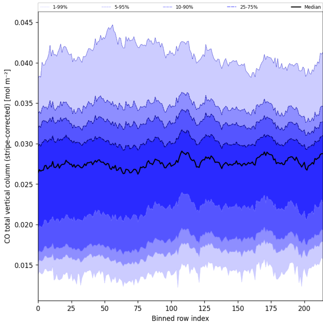
Figure 27: Along track statistics of “CO total vertical column (stripe-corrected)” for 2025-05-23 to 2025-05-25
