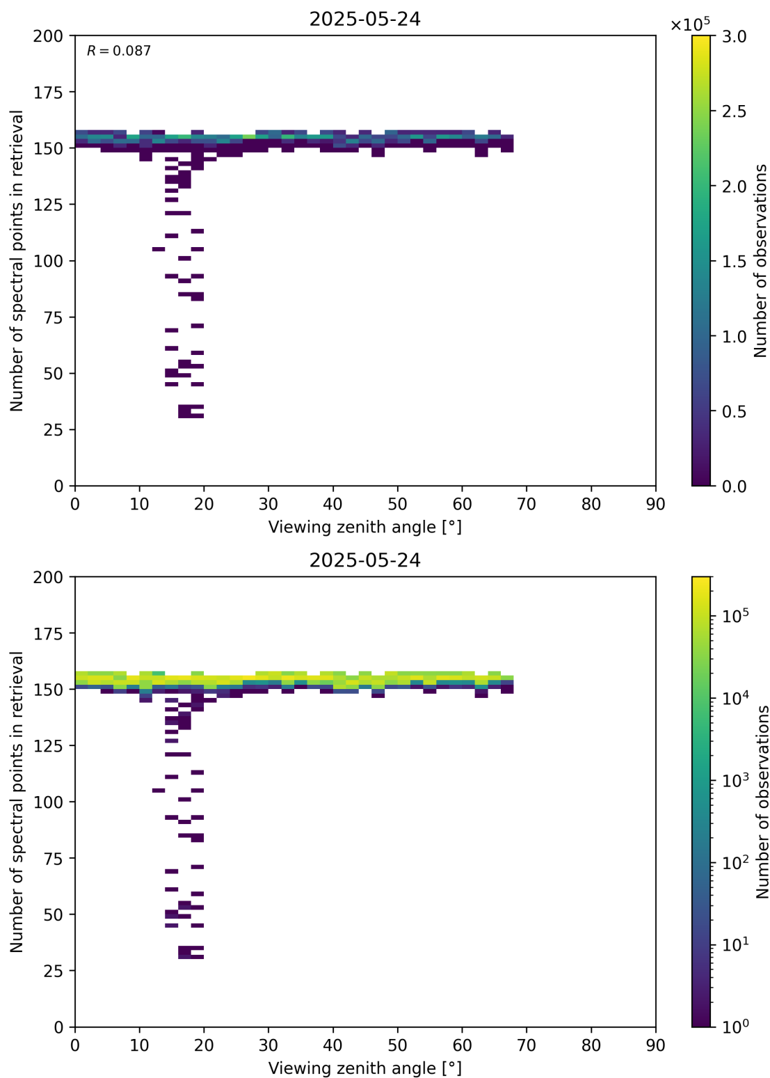
Figure 76: Scatter density plot of “Viewing zenith angle” against “Number of spectral points in retrieval” for 2025-05-23 to 2025-05-25.
