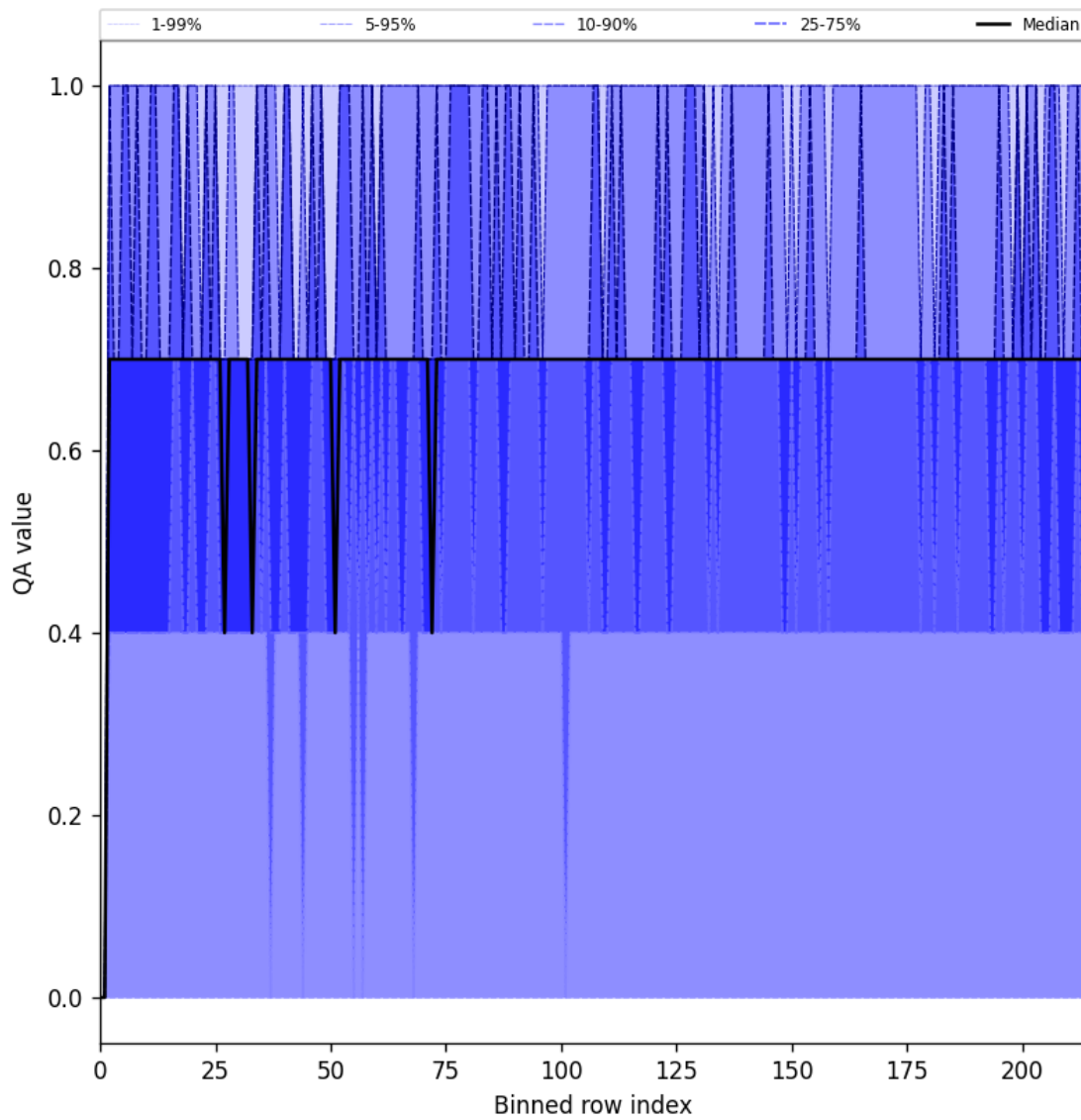
Figure 25: Along track statistics of “QA value” for 2025-05-23 to 2025-05-25
