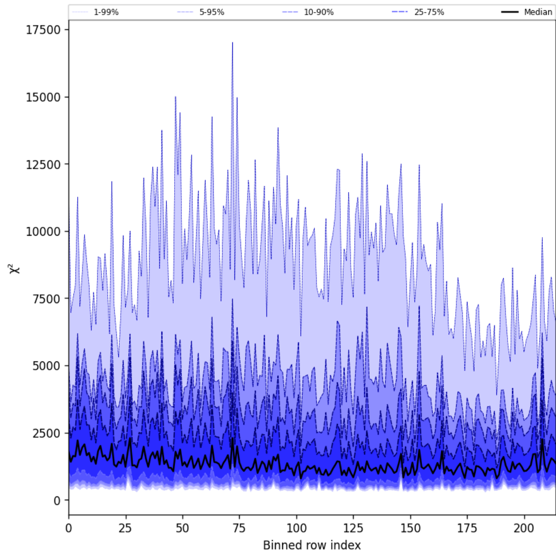
Figure 30: Along track statistics of “ \chi^2 ” for 2025-05-23 to 2025-05-25
