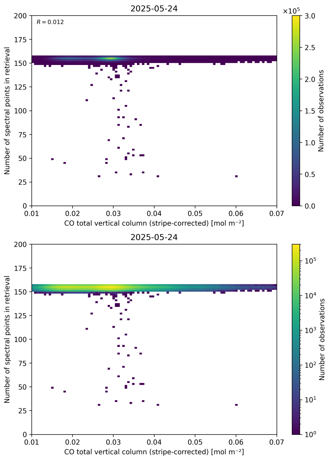
Figure 40: Scatter density plot of “CO total vertical column (stripe-corrected)” against “Number of spectral points in retrieval” for 2025-05-23 to 2025-05-25.
