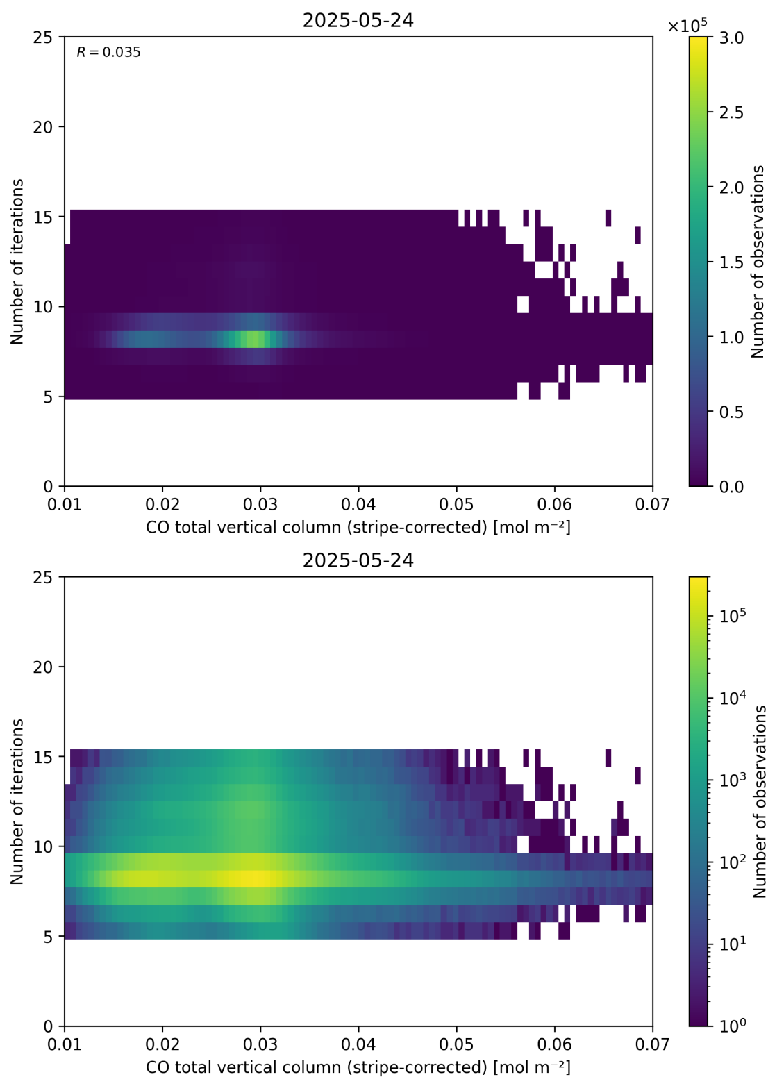
Figure 39: Scatter density plot of “CO total vertical column (stripe-corrected)” against “Number of iterations” for 2025-05-23 to 2025-05-25.
