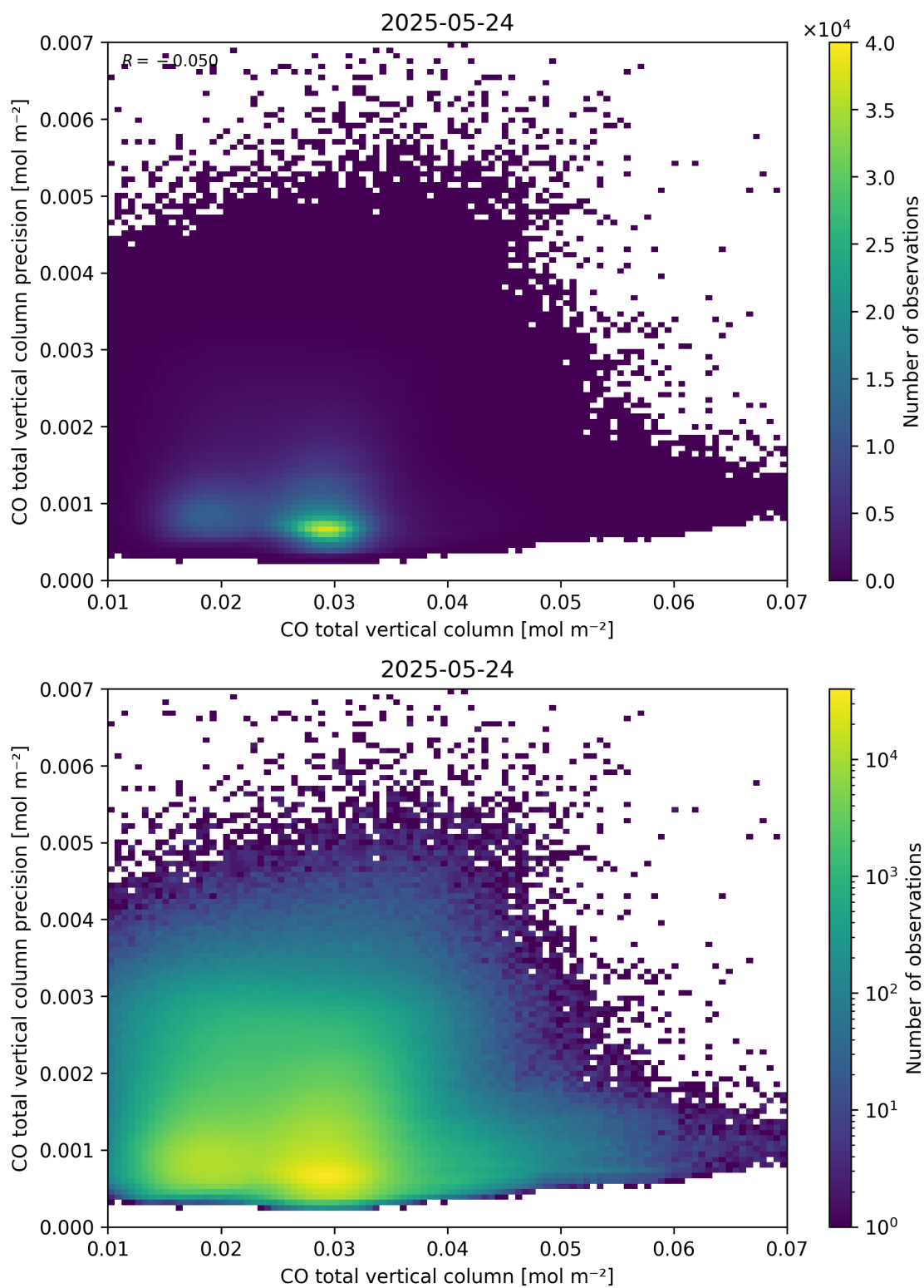
Figure 34: Scatter density plot of “CO total vertical column” against “CO total vertical column precision” for 2025-05-23 to 2025-05-25.
