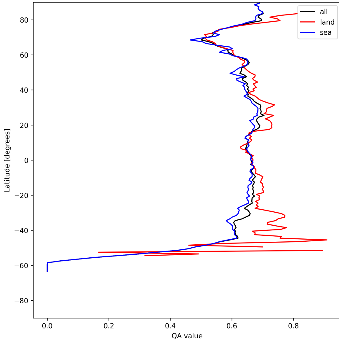
Figure 9: Zonal average of “QA value” for 2025-05-23 to 2025-05-25.
