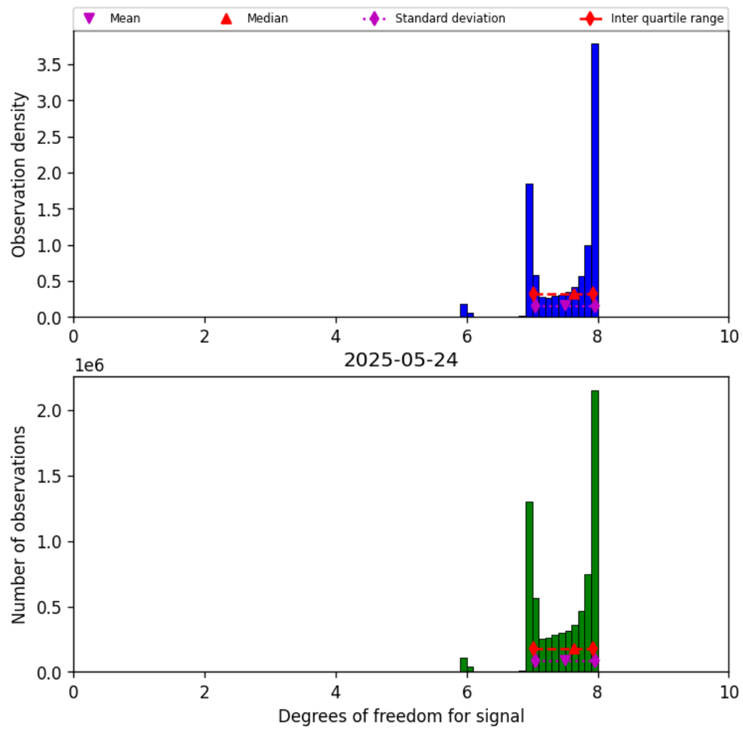
Figure 23: Histogram of “Degrees of freedom for signal” for 2025-05-23 to 2025-05-25
