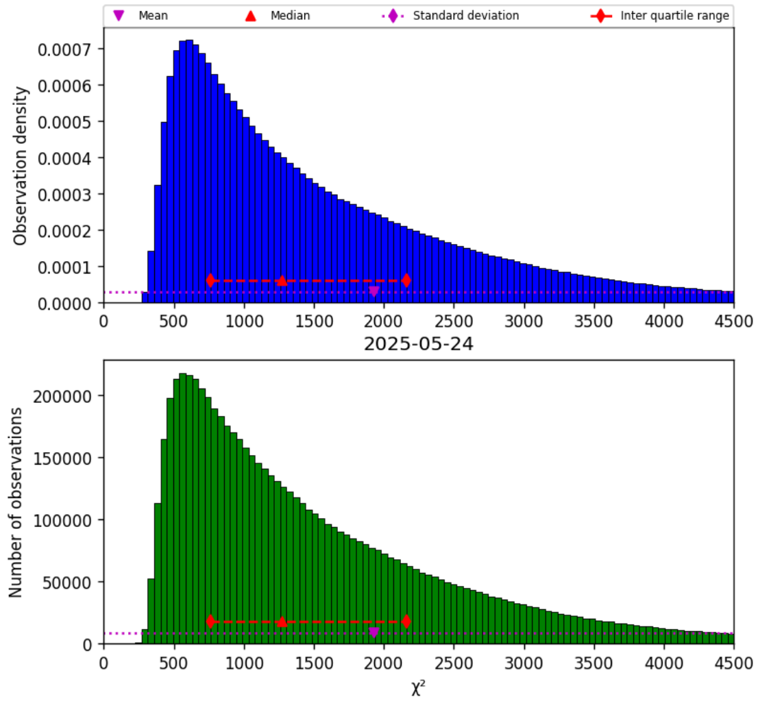
Figure 22: Histogram of “ \chi^2 ” for 2025-05-23 to 2025-05-25
