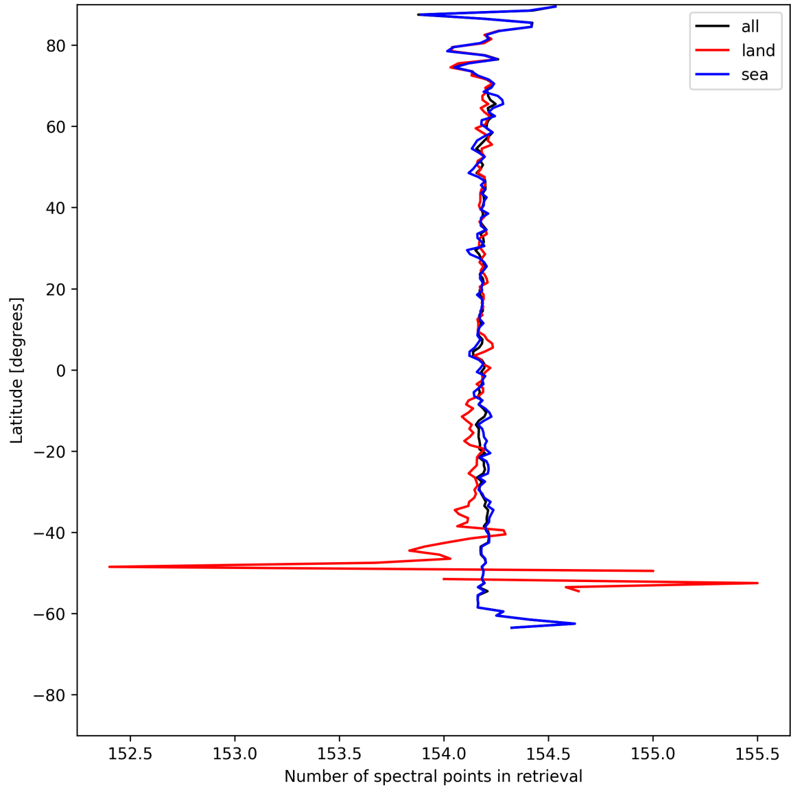
Figure 13: Zonal average of “Number of spectral points in retrieval” for 2025-05-23 to 2025-05-25.
