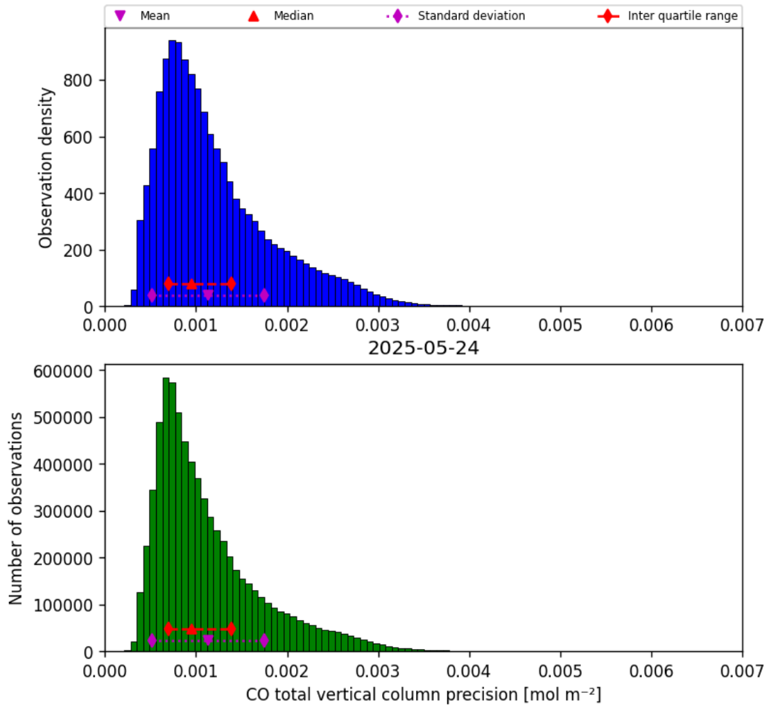
Figure 20: Histogram of “CO total vertical column precision” for 2025-05-23 to 2025-05-25
