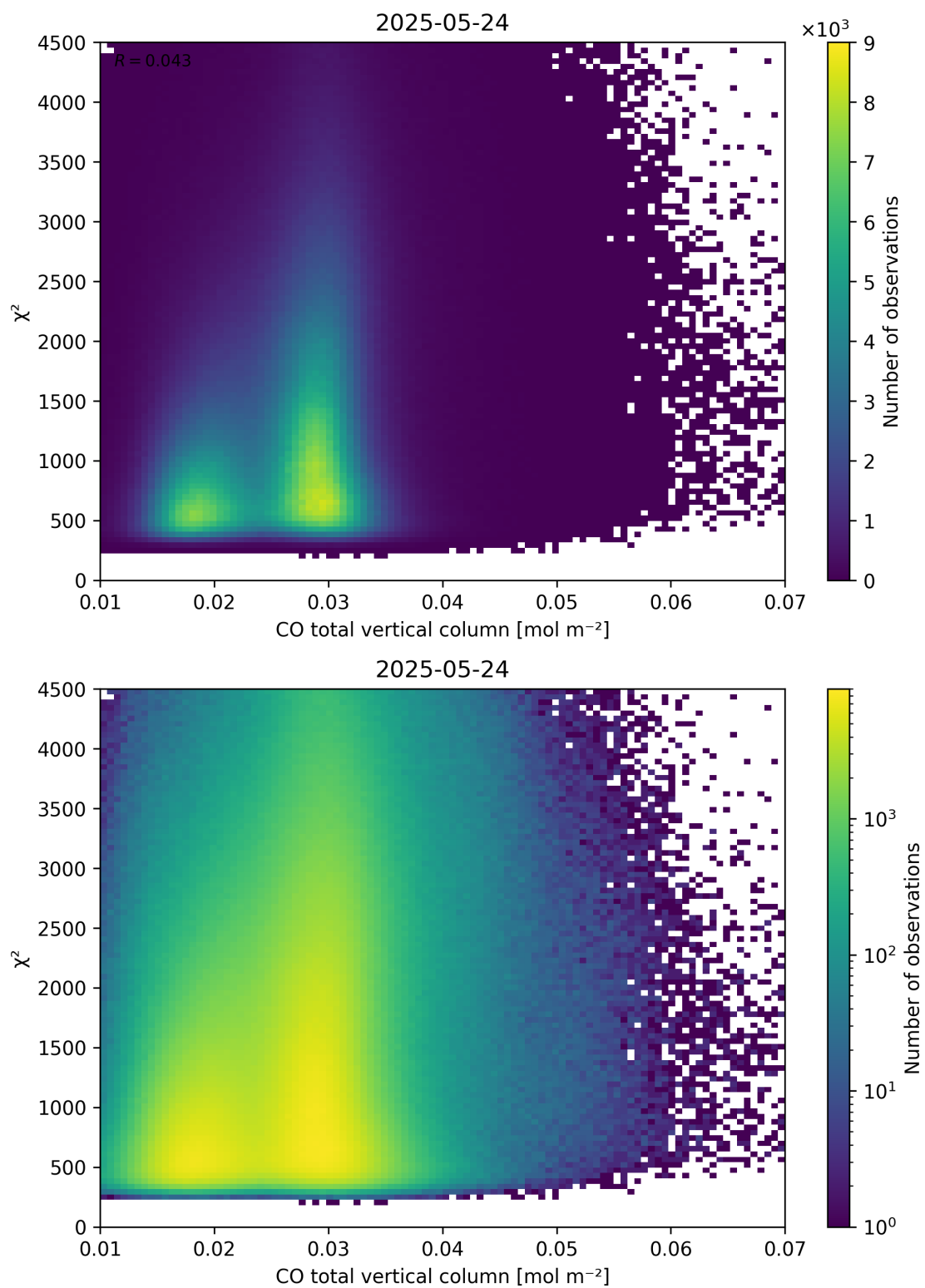
Figure 35: Scatter density plot of “CO total vertical column” against “ \chi^2 ” for 2025-05-23 to 2025-05-25.
