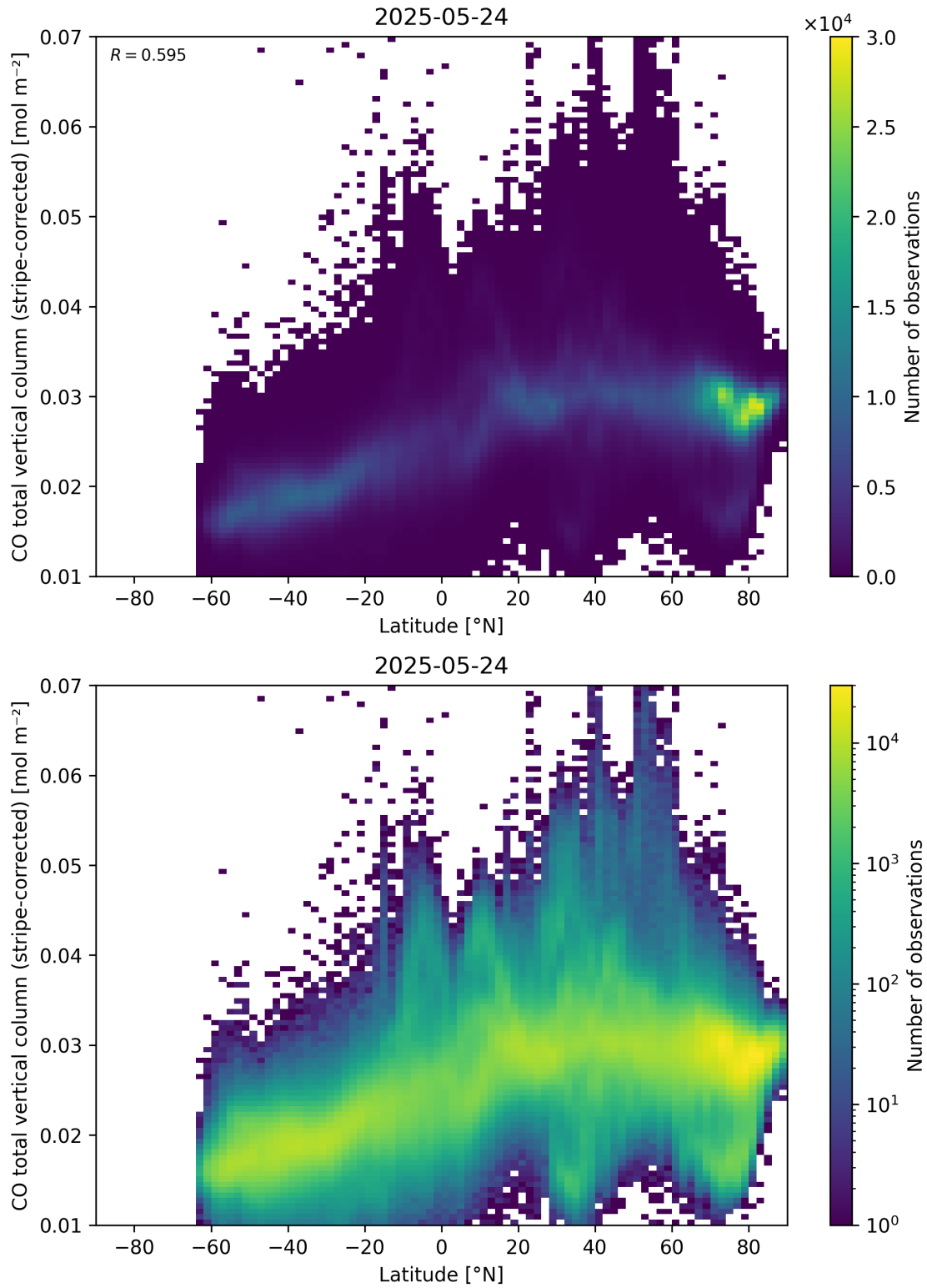
Figure 52: Scatter density plot of “Latitude” against “CO total vertical column (stripe-corrected)” for 2025-05-23 to 2025-05-25.
