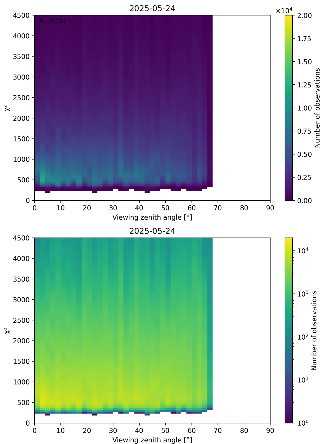
Figure 72: Scatter density plot of “Viewing zenith angle” against “ \chi^2 ” for 2025-05-23 to 2025-05-25.
