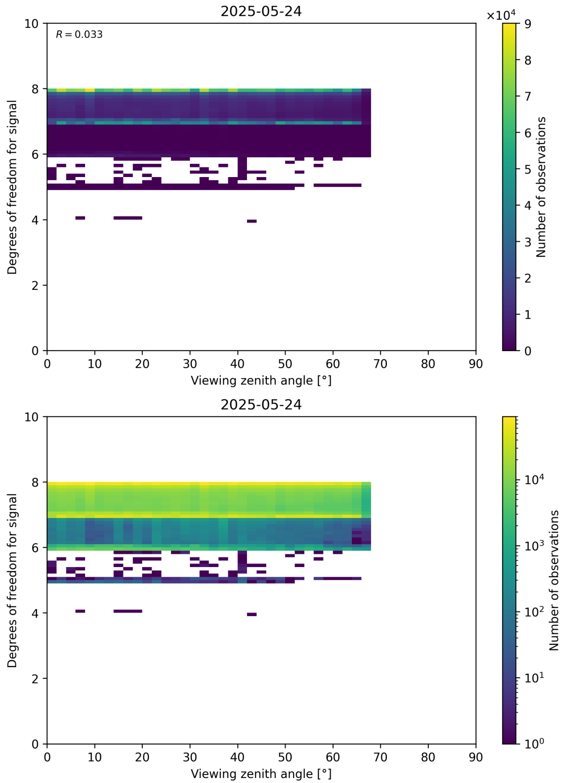
Figure 73: Scatter density plot of “Viewing zenith angle” against “Degrees of freedom for signal” for 2025-05-23 to 2025-05-25.
