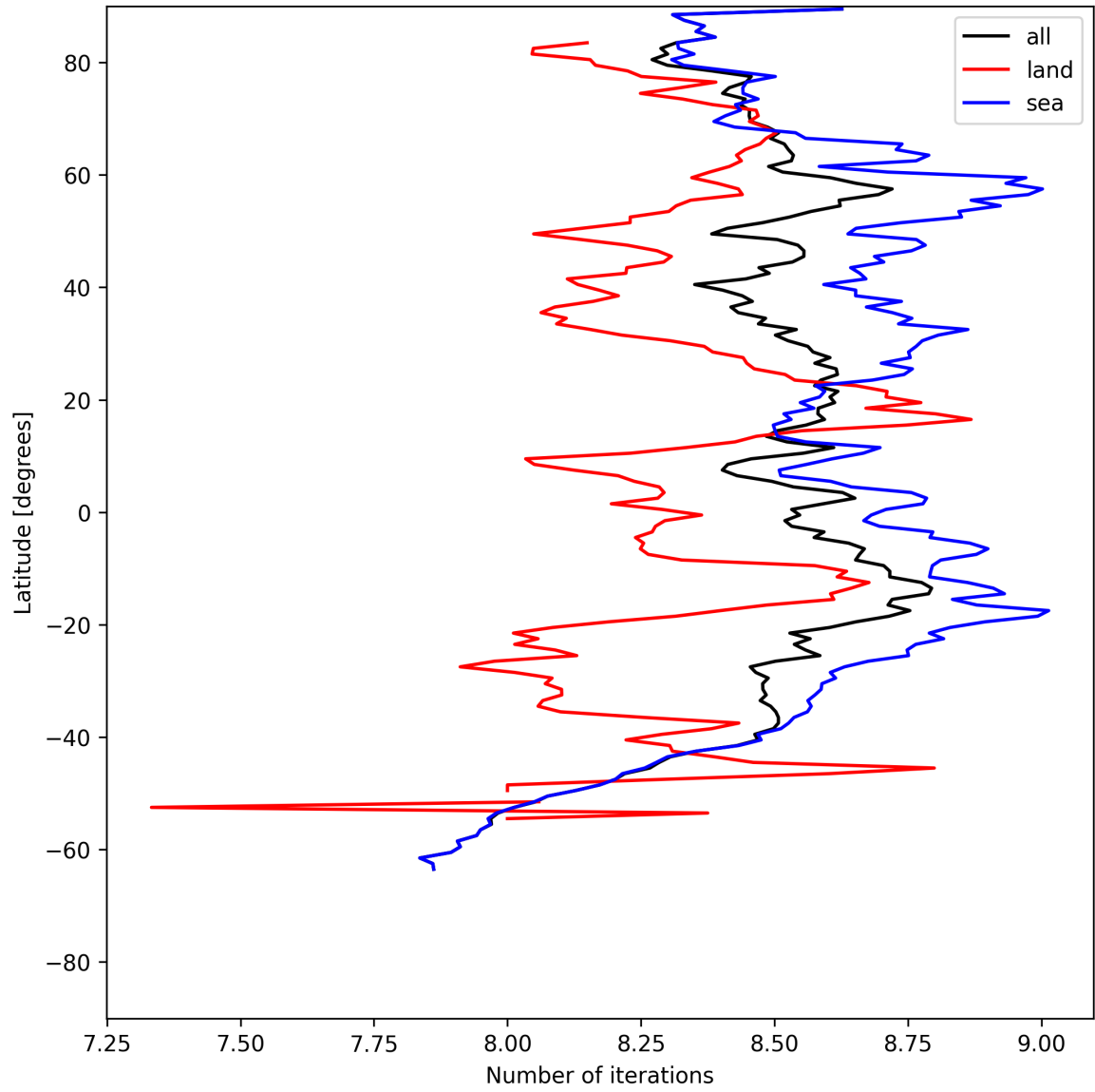
Figure 16: Zonal average of “Number of iterations” for 2025-05-23 to 2025-05-25.
