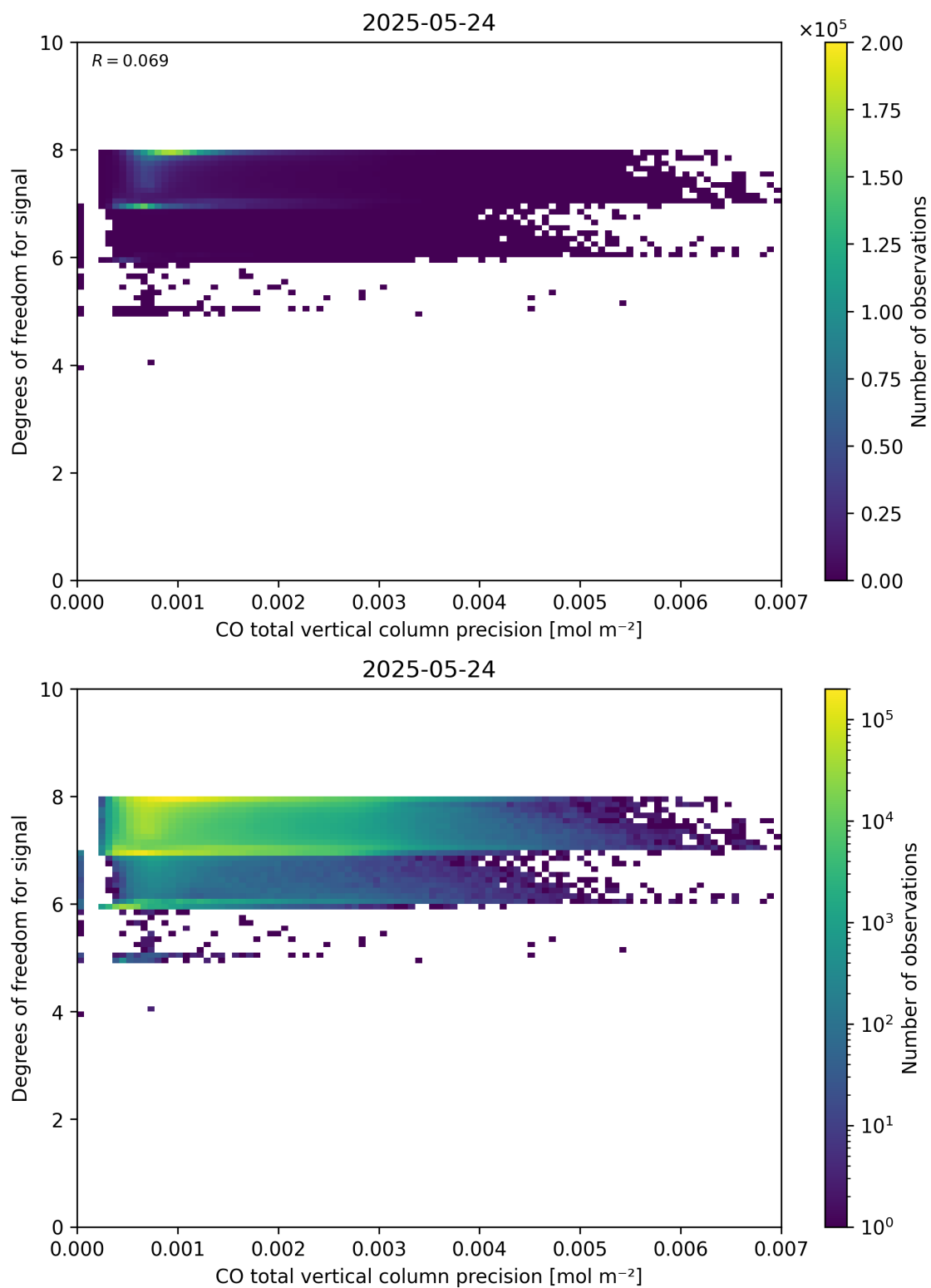
Figure 45: Scatter density plot of “CO total vertical column precision” against “Degrees of freedom for signal” for 2025-05-23 to 2025-05-25.
