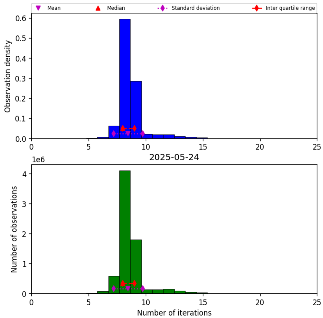
Figure 24: Histogram of “Number of iterations” for 2025-05-23 to 2025-05-25
