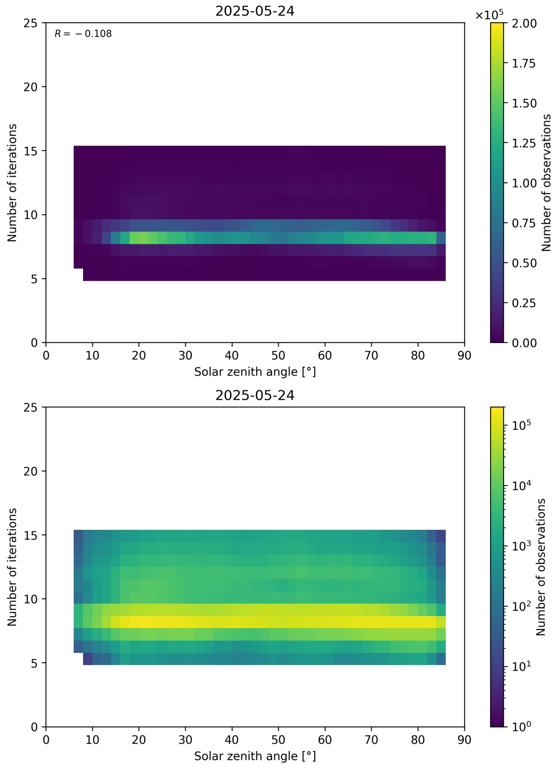
Figure 67: Scatter density plot of “Solar zenith angle” against “Number of iterations” for 2025-05-23 to 2025-05-25.
