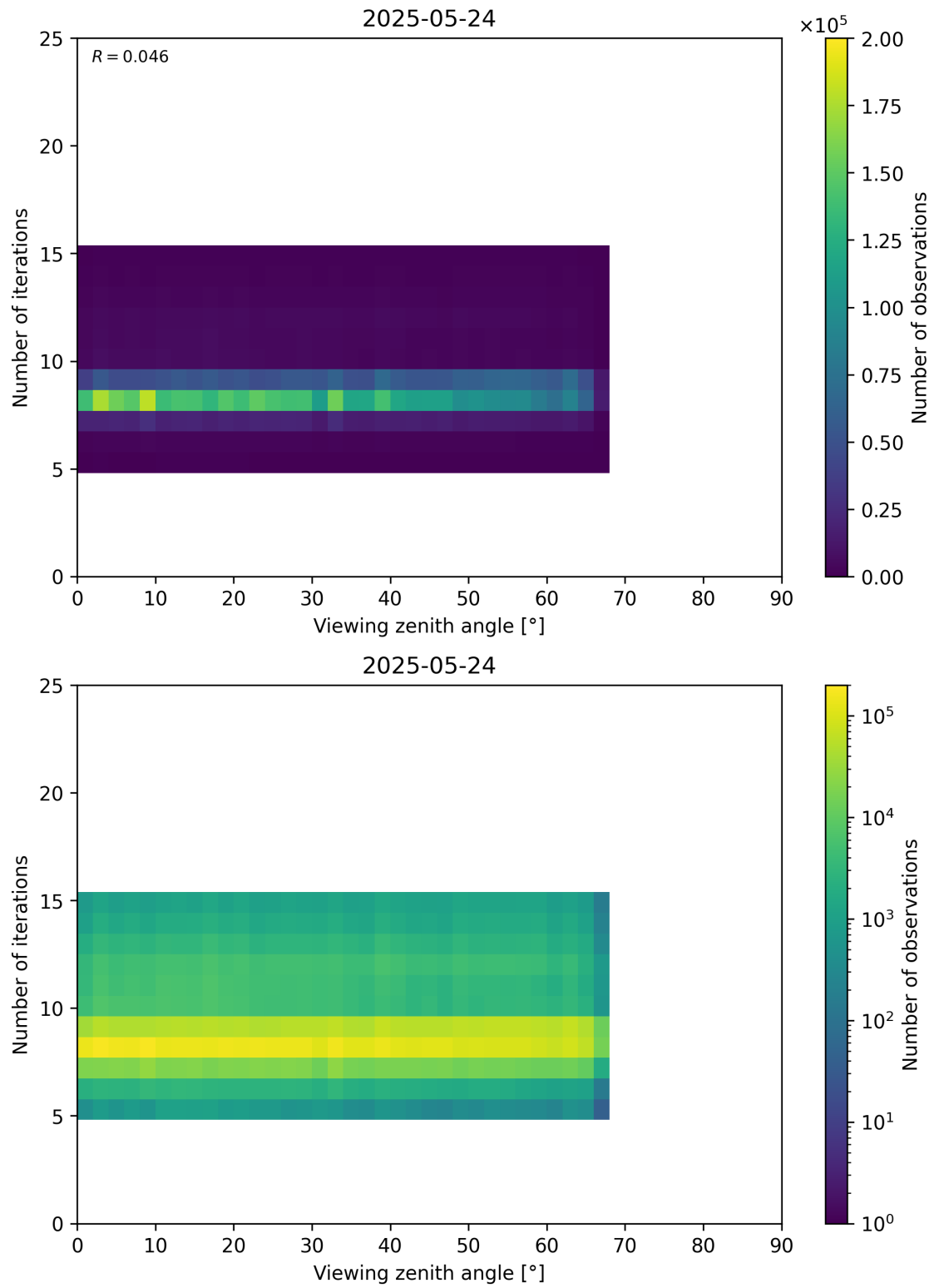
Figure 75: Scatter density plot of “Viewing zenith angle” against “Number of iterations” for 2025-05-23 to 2025-05-25.
