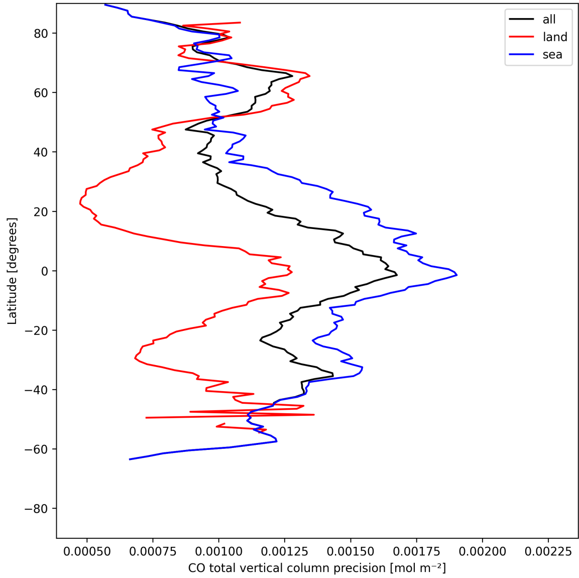
Figure 12: Zonal average of “CO total vertical column precision” for 2025-05-23 to 2025-05-25.
