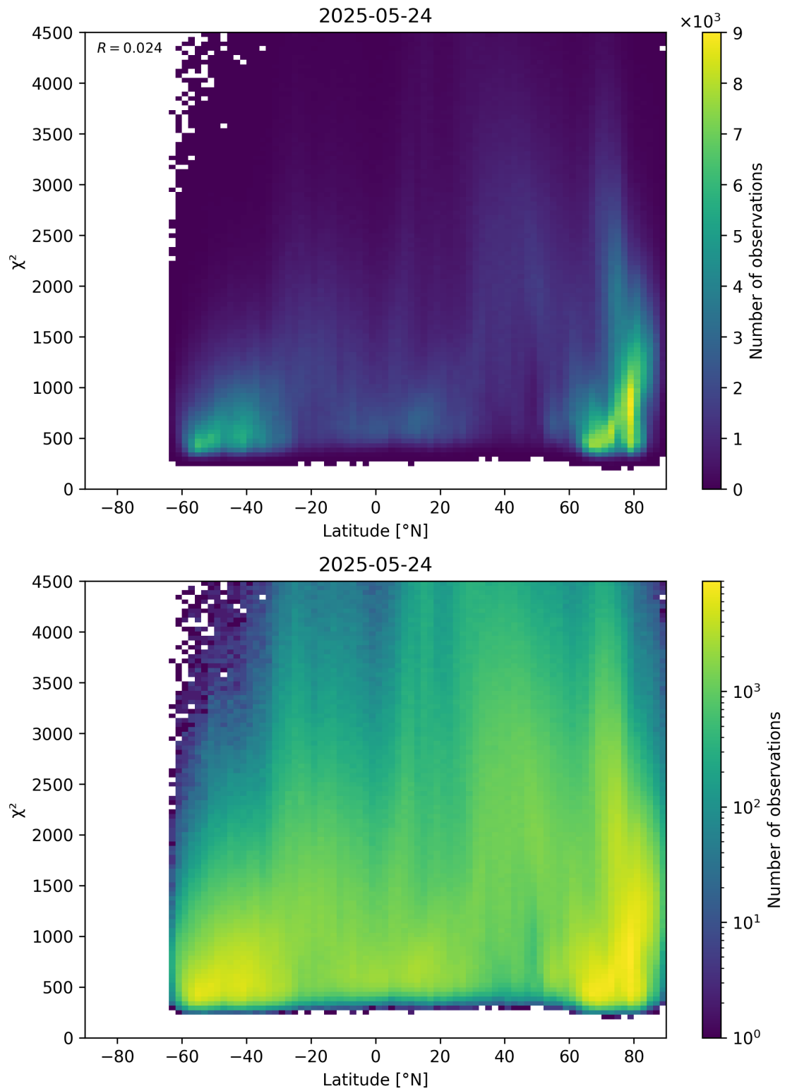
Figure 54: Scatter density plot of “Latitude” against “ \chi^2 ” for 2025-05-23 to 2025-05-25.
