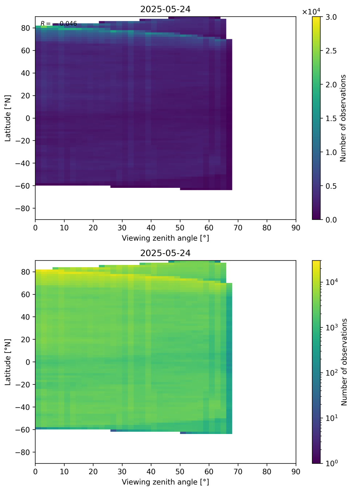
Figure 74: Scatter density plot of “Viewing zenith angle” against “Latitude” for 2025-05-23 to 2025-05-25.
