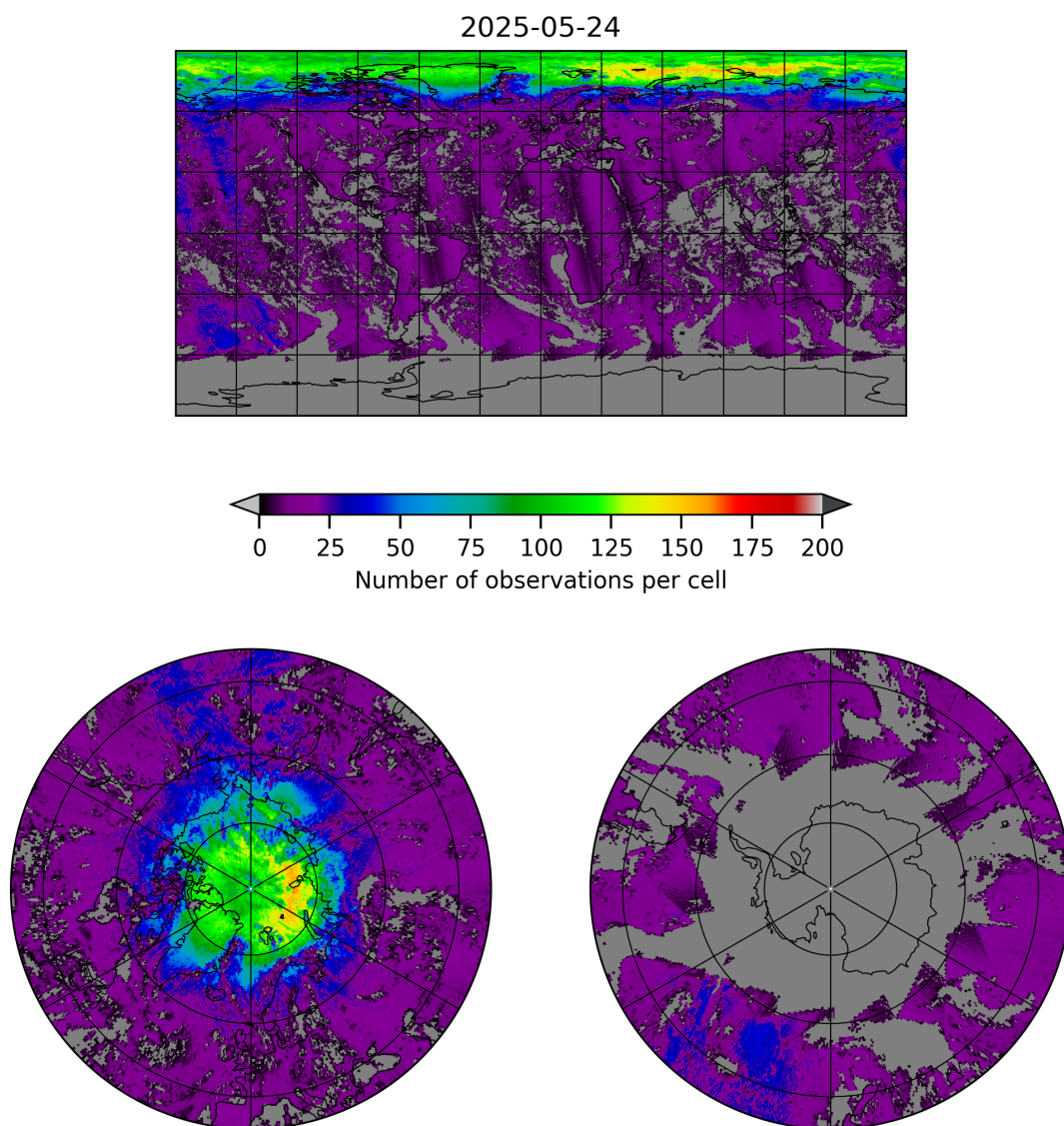
Figure 8: Map of the number of observations for 2025-05-23 to 2025-05-25
