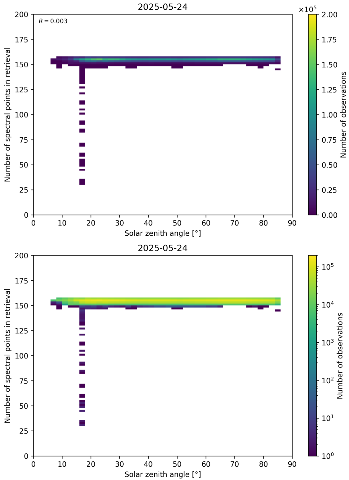
Figure 68: Scatter density plot of “Solar zenith angle” against “Number of spectral points in retrieval” for 2025-05-23 to 2025-05-25.
