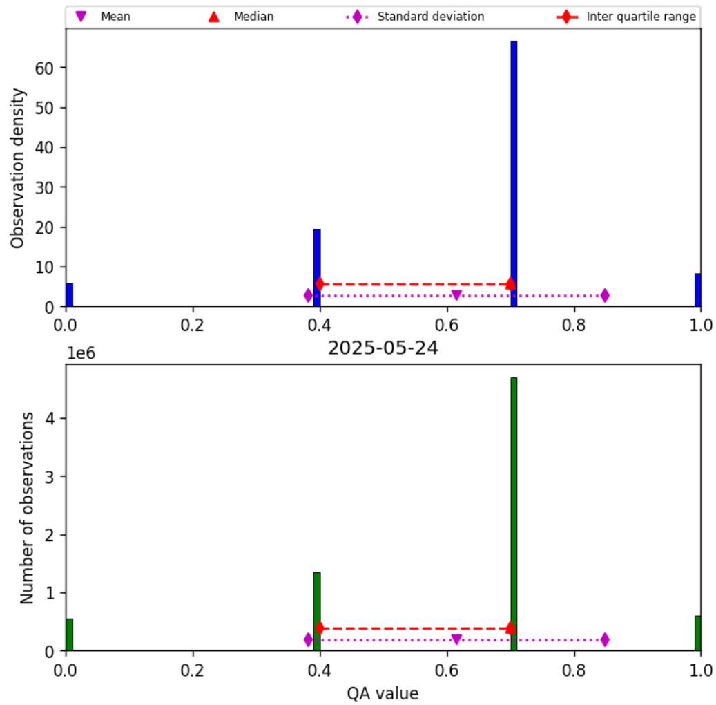
Figure 17: Histogram of “QA value” for 2025-05-23 to 2025-05-25
