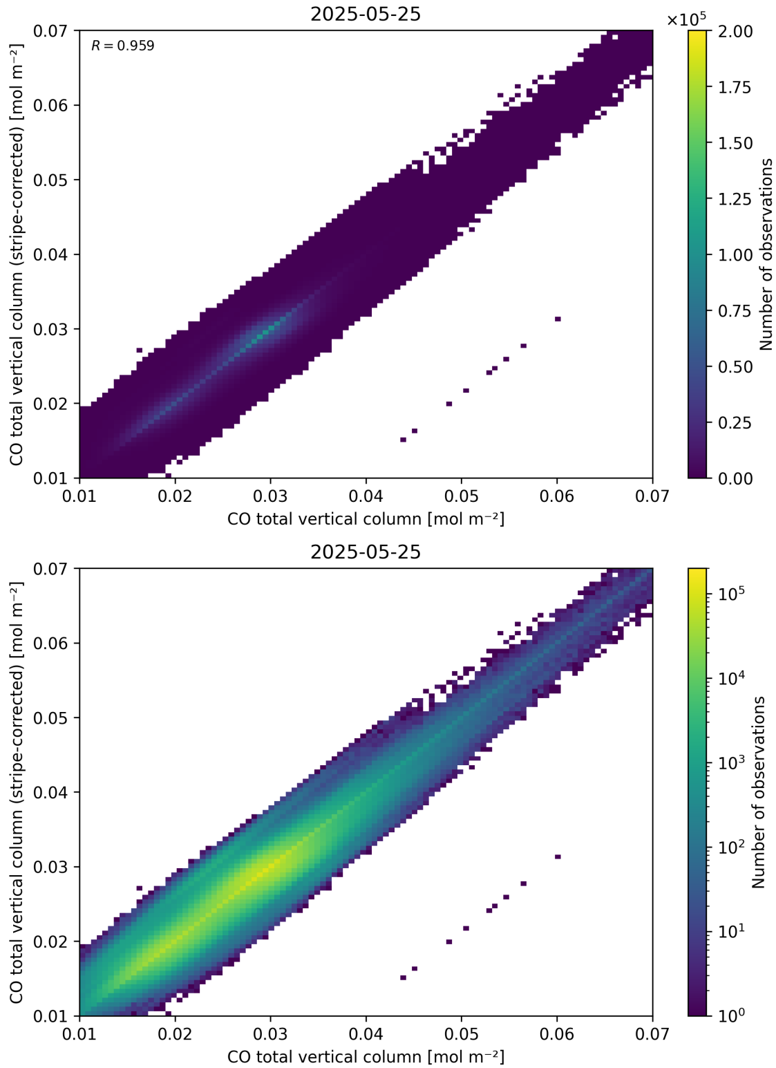
Figure 33: Scatter density plot of “CO total vertical column” against “CO total vertical column (stripe-corrected)” for 2025-05-24 to 2025-05-26.
