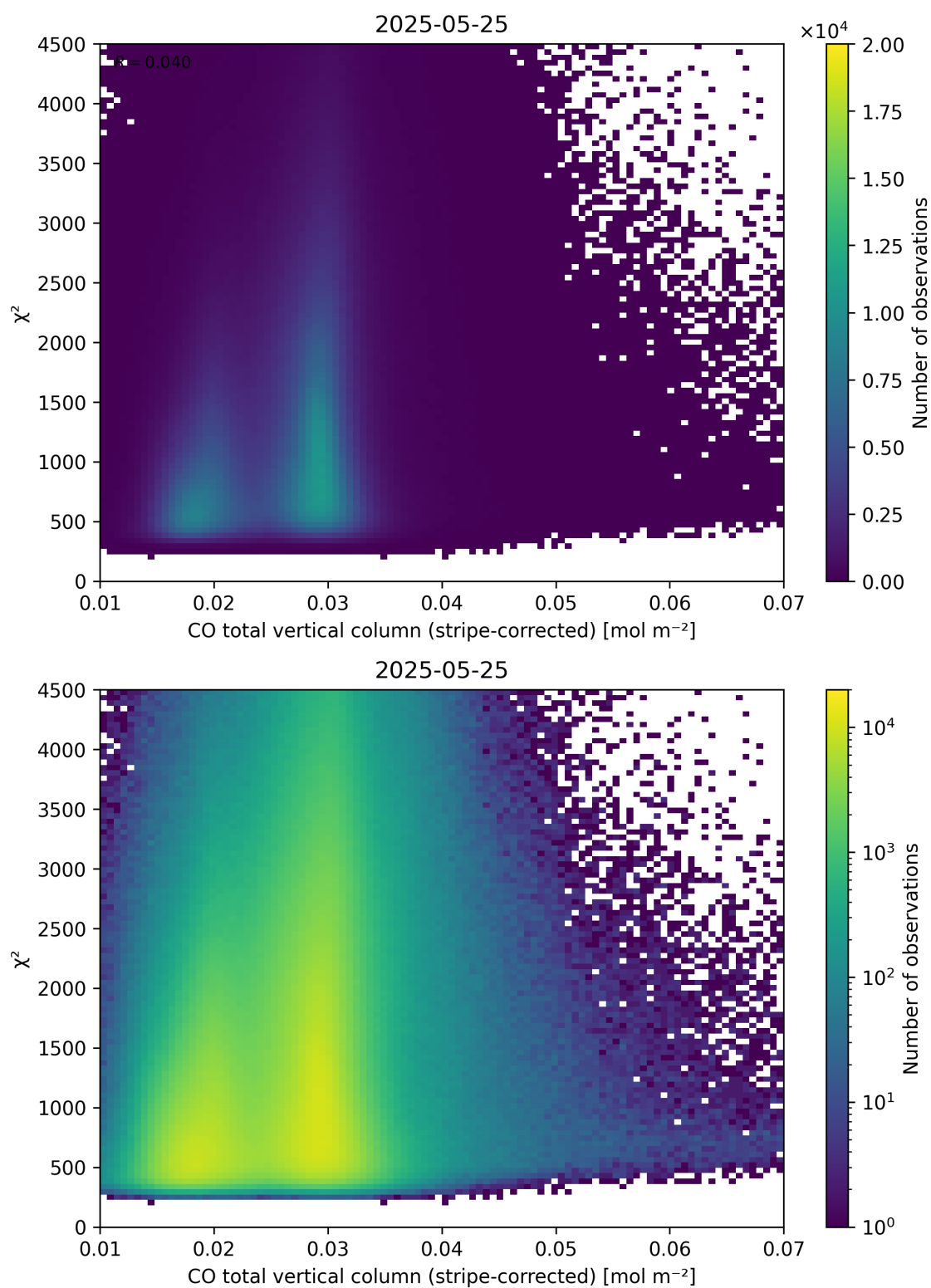
Figure 37: Scatter density plot of “CO total vertical column (stripe-corrected)” against “ \chi^2 ” for 2025-05-24 to 2025-05-26.
