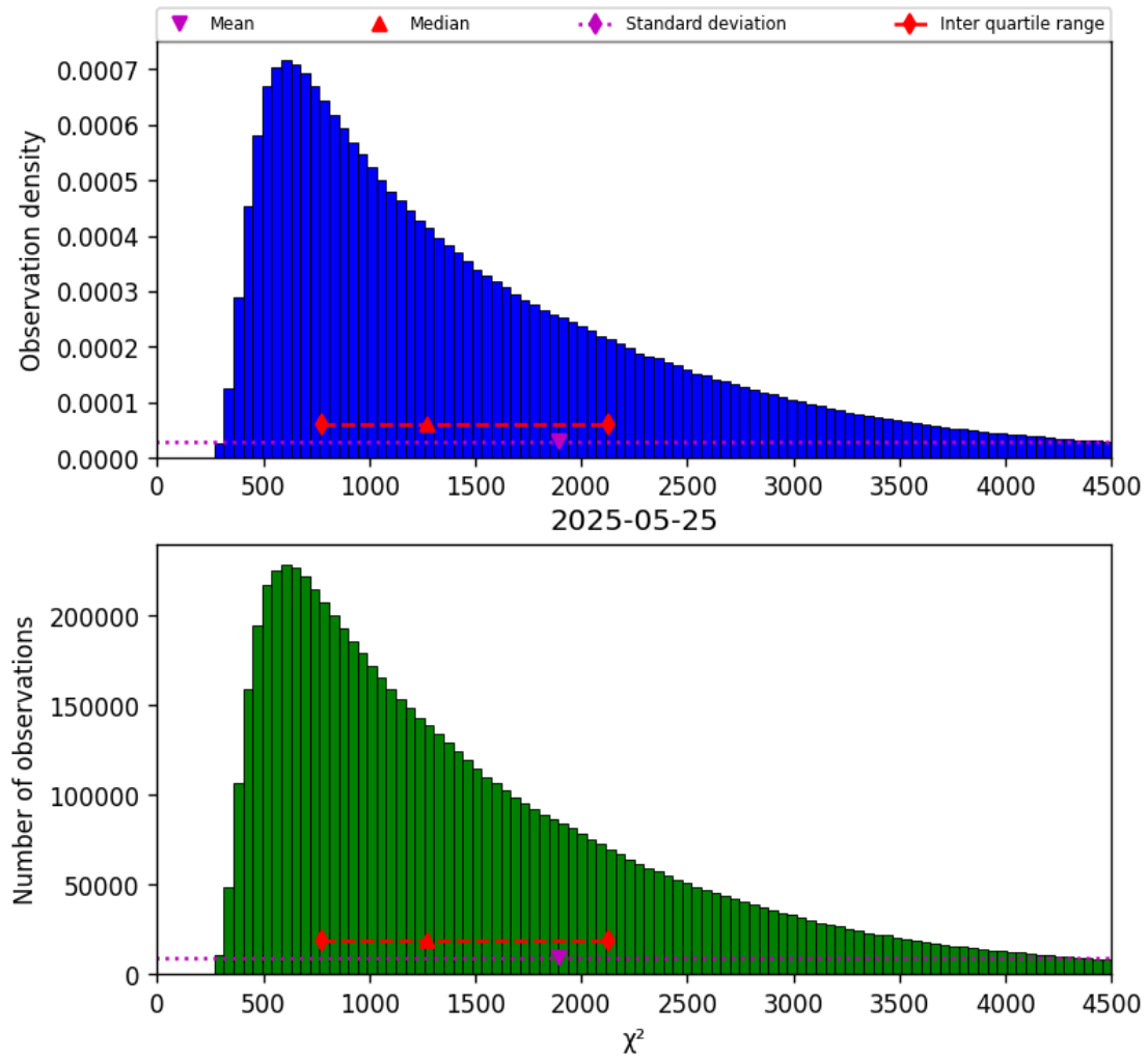
Figure 22: Histogram of “ \chi^2 ” for 2025-05-24 to 2025-05-26
