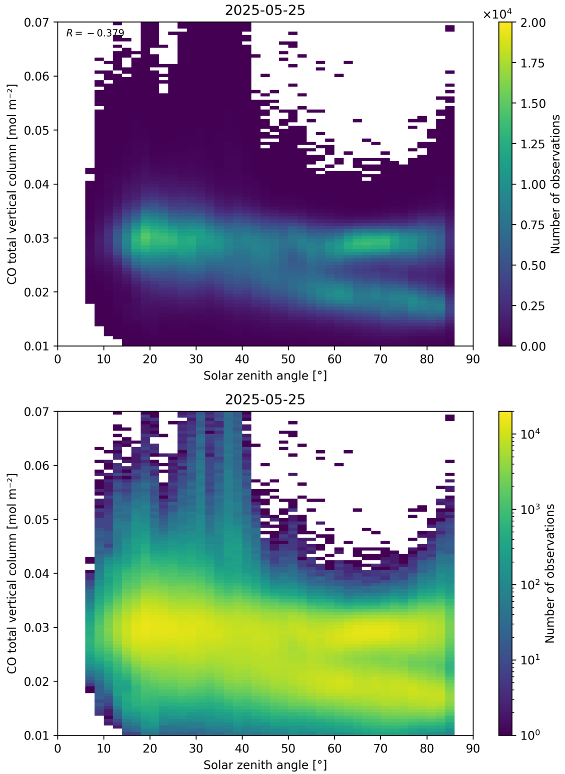
Figure 61: Scatter density plot of “Solar zenith angle” against “CO total vertical column” for 2025-05-24 to 2025-05-26.
