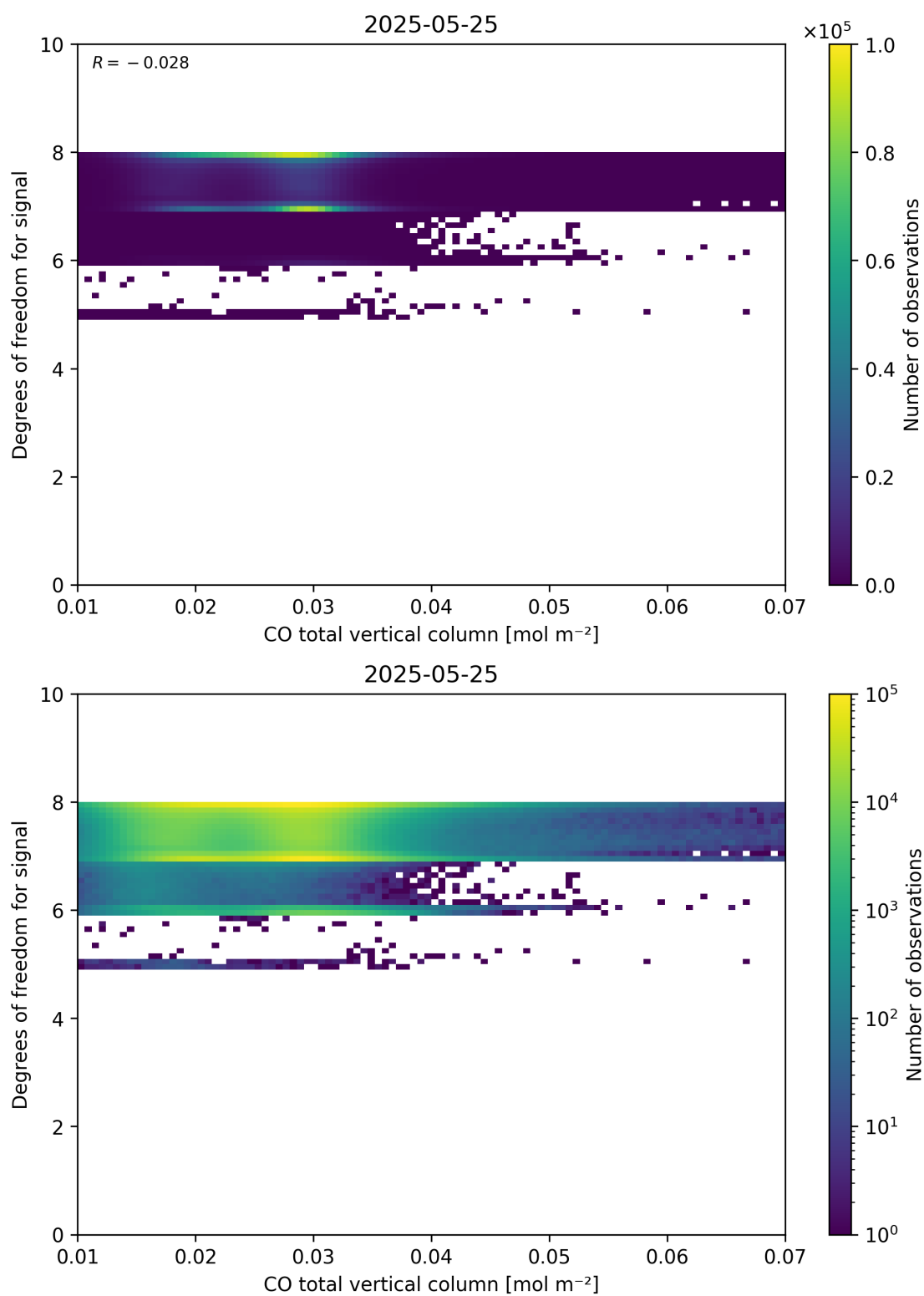
Figure 41: Scatter density plot of “CO total vertical column” against “Degrees of freedom for signal” for 2025-05-24 to 2025-05-26.
