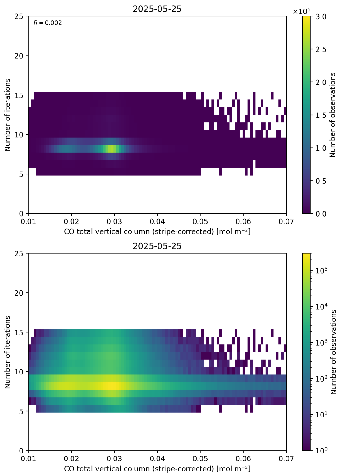
Figure 39: Scatter density plot of “CO total vertical column (stripe-corrected)” against “Number of iterations” for 2025-05-24 to 2025-05-26.
