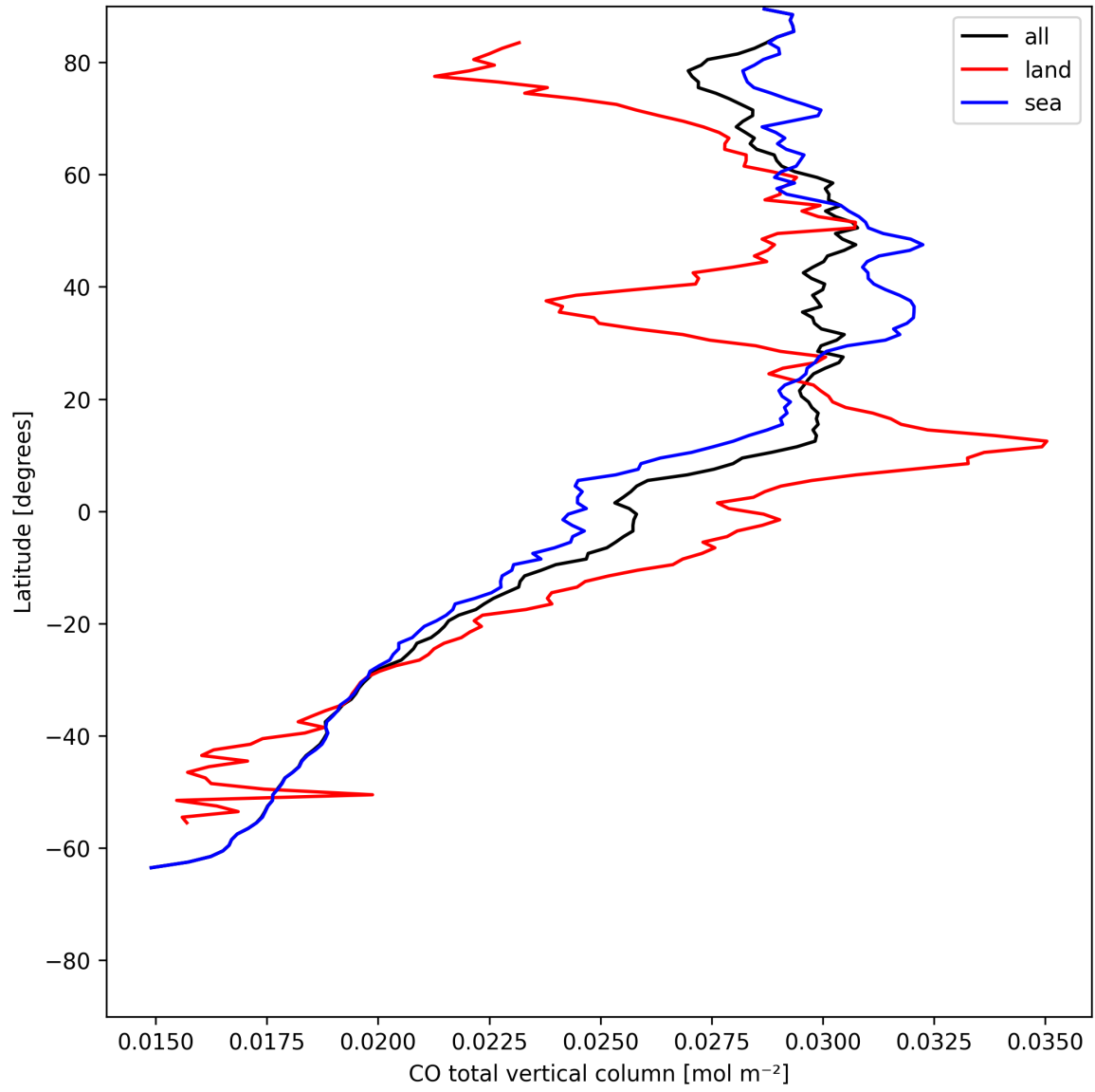
Figure 10: Zonal average of “CO total vertical column” for 2025-05-24 to 2025-05-26.
