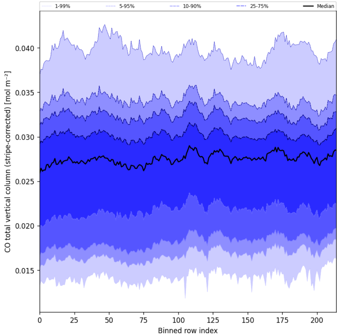
Figure 27: Along track statistics of “CO total vertical column (stripe-corrected)” for 2025-05-24 to 2025-05-26
