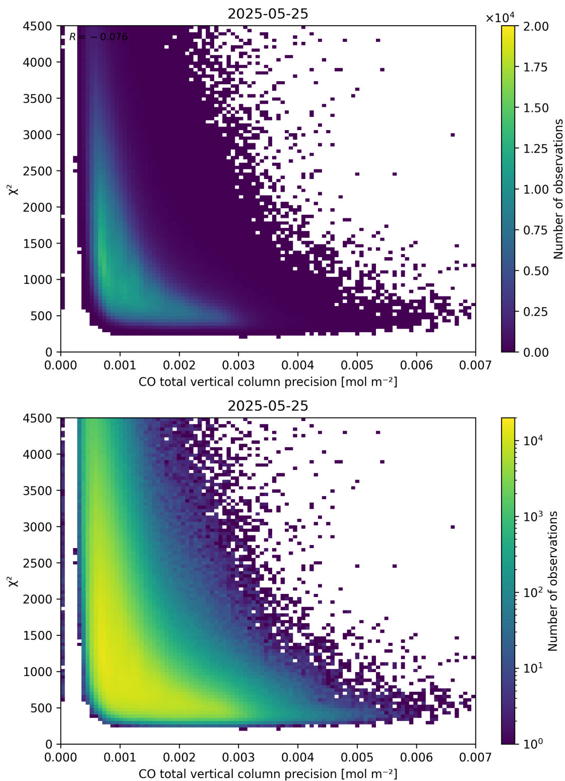
Figure 44: Scatter density plot of “CO total vertical column precision” against “ \chi^2 ” for 2025-05-24 to 2025-05-26.
