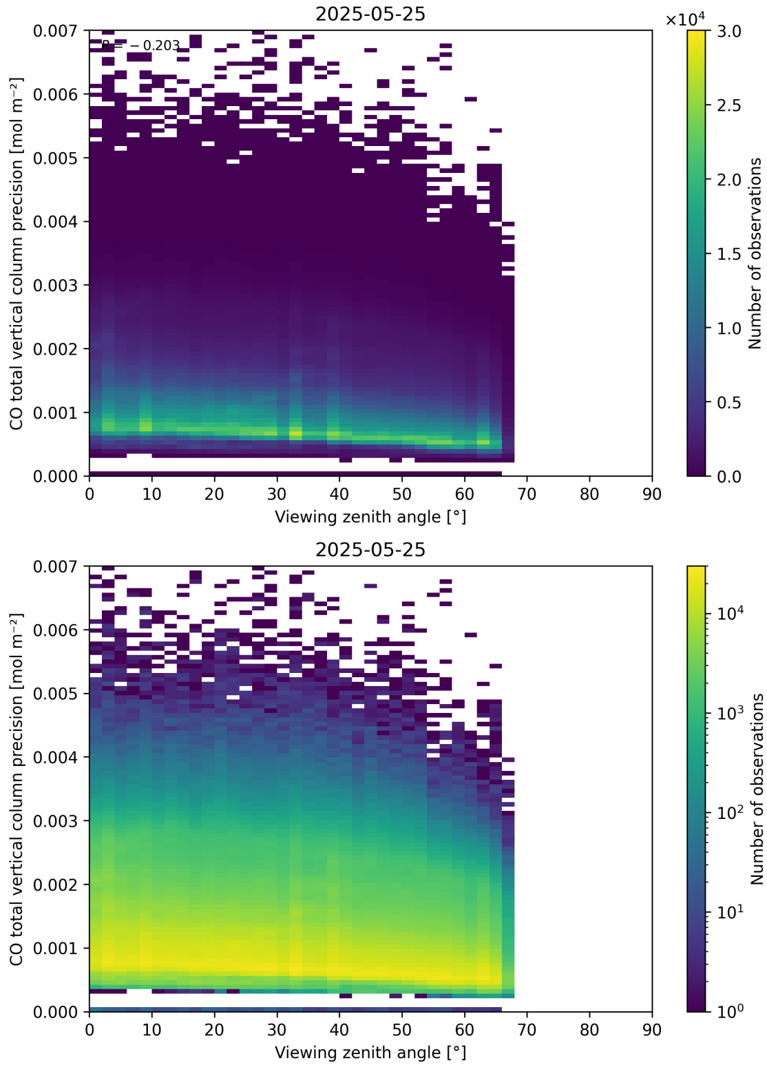
Figure 71: Scatter density plot of “Viewing zenith angle” against “CO total vertical column precision” for 2025-05-24 to 2025-05-26.
