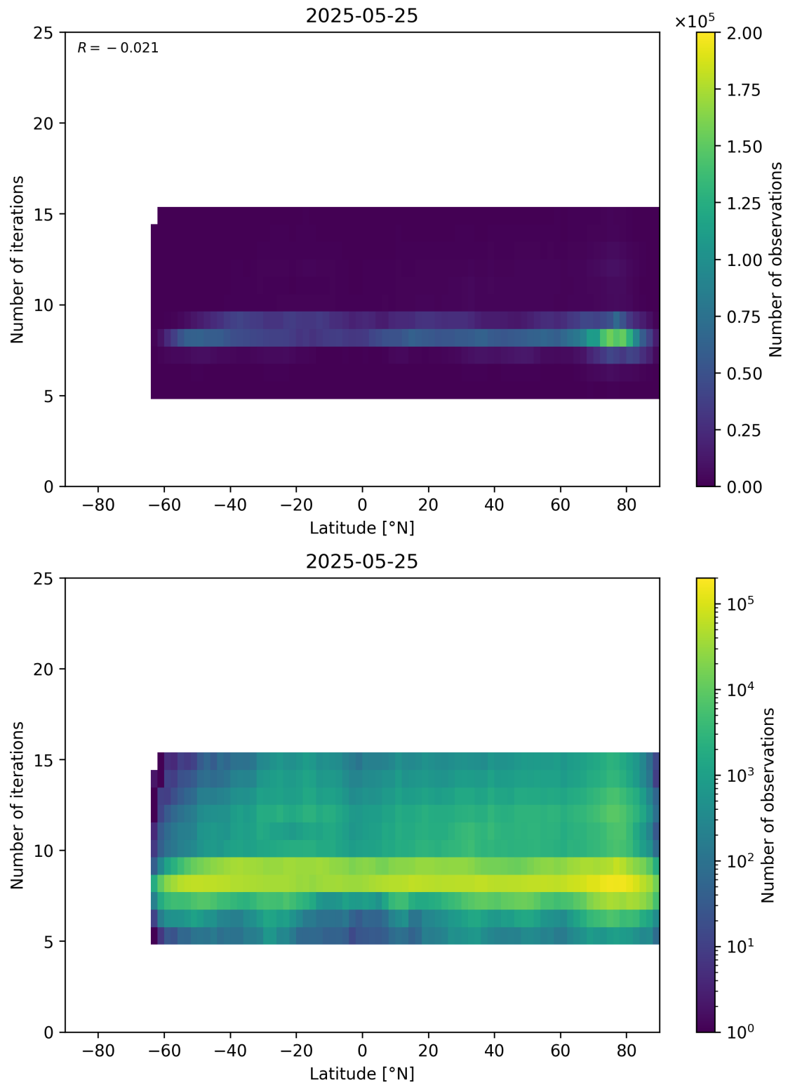
Figure 56: Scatter density plot of “Latitude” against “Number of iterations” for 2025-05-24 to 2025-05-26.
