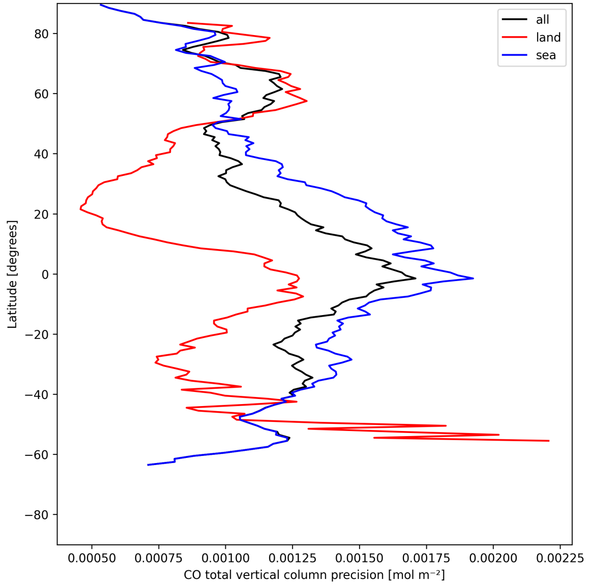
Figure 12: Zonal average of “CO total vertical column precision” for 2025-05-24 to 2025-05-26.
