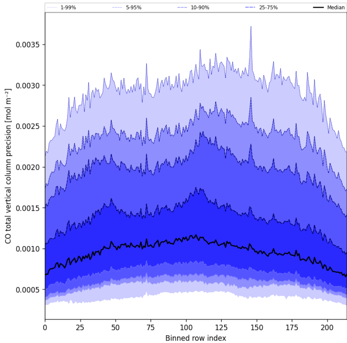
Figure 28: Along track statistics of “CO total vertical column precision” for 2025-05-24 to 2025-05-26
