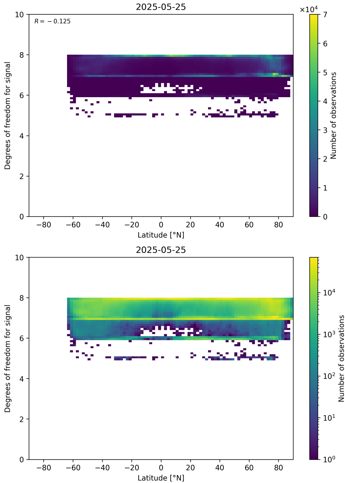
Figure 55: Scatter density plot of “Latitude” against “Degrees of freedom for signal” for 2025-05-24 to 2025-05-26.
