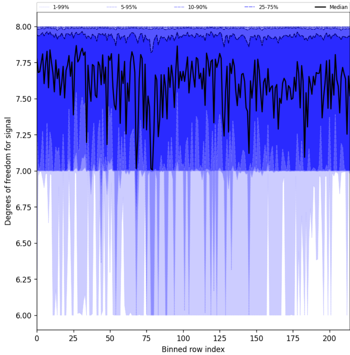
Figure 31: Along track statistics of “Degrees of freedom for signal” for 2025-05-24 to 2025-05-26
