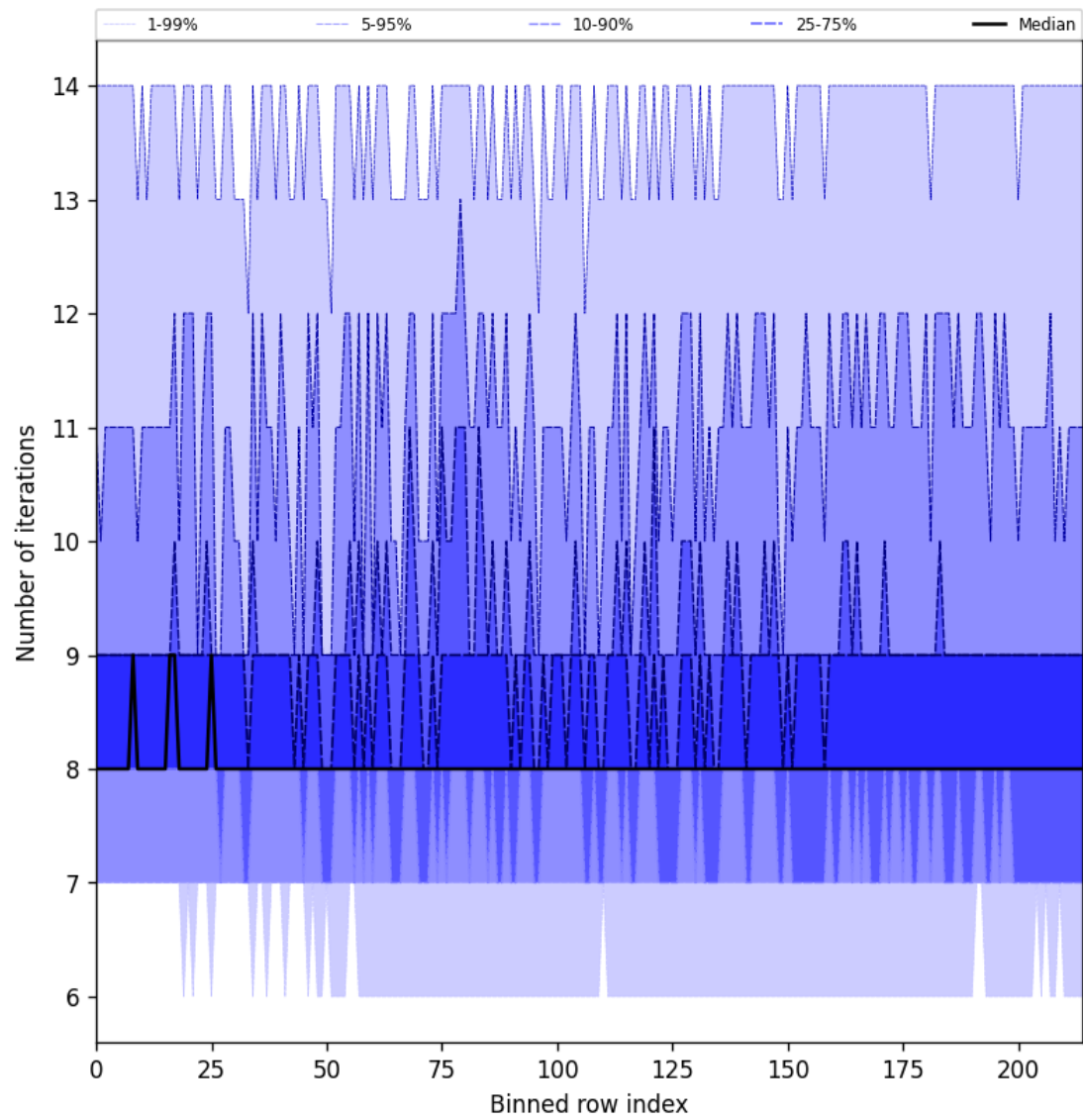
Figure 32: Along track statistics of “Number of iterations” for 2025-05-24 to 2025-05-26
