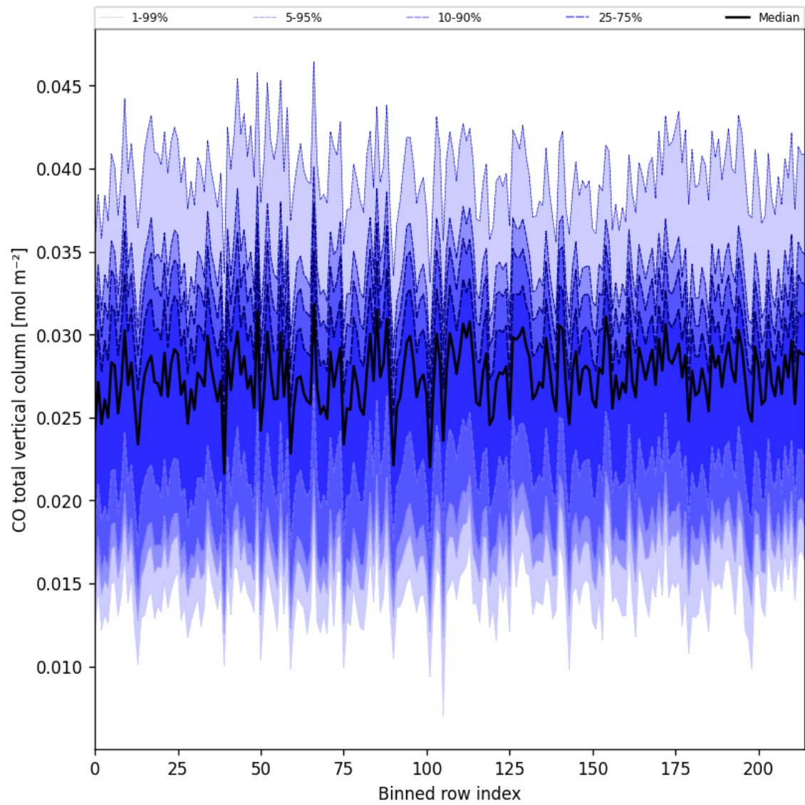
Figure 26: Along track statistics of “CO total vertical column” for 2025-05-24 to 2025-05-26
