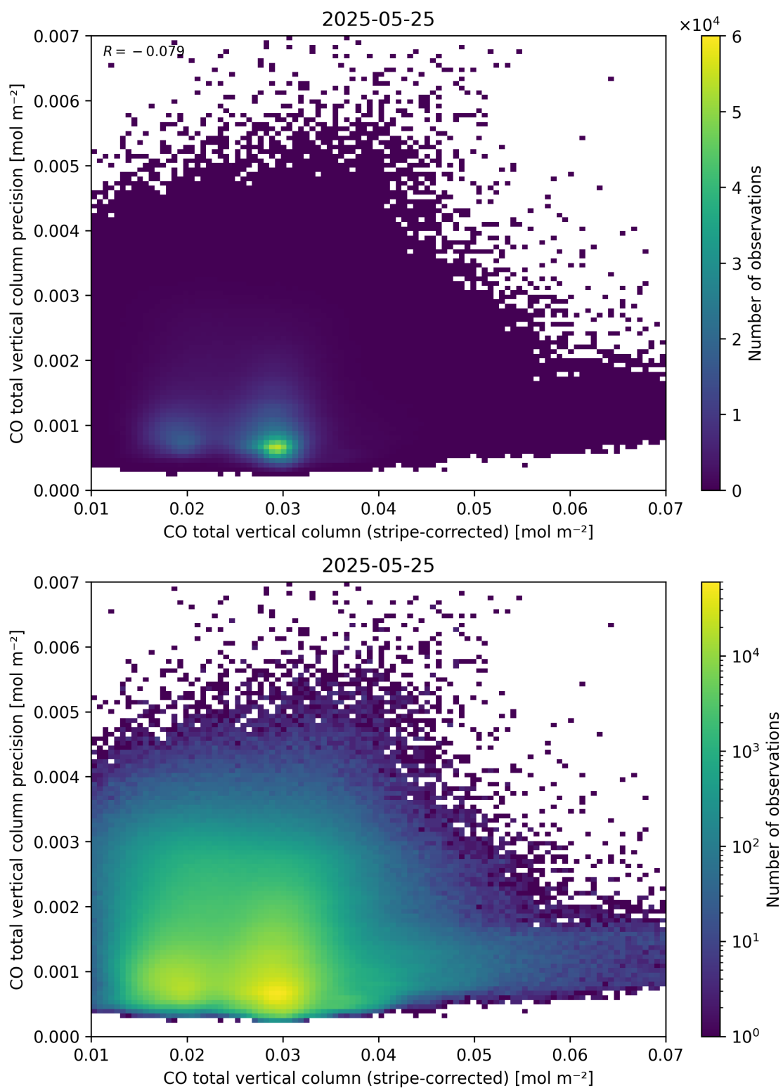
Figure 36: Scatter density plot of “CO total vertical column (stripe-corrected)” against “CO total vertical column precision” for 2025-05-24 to 2025-05-26.
