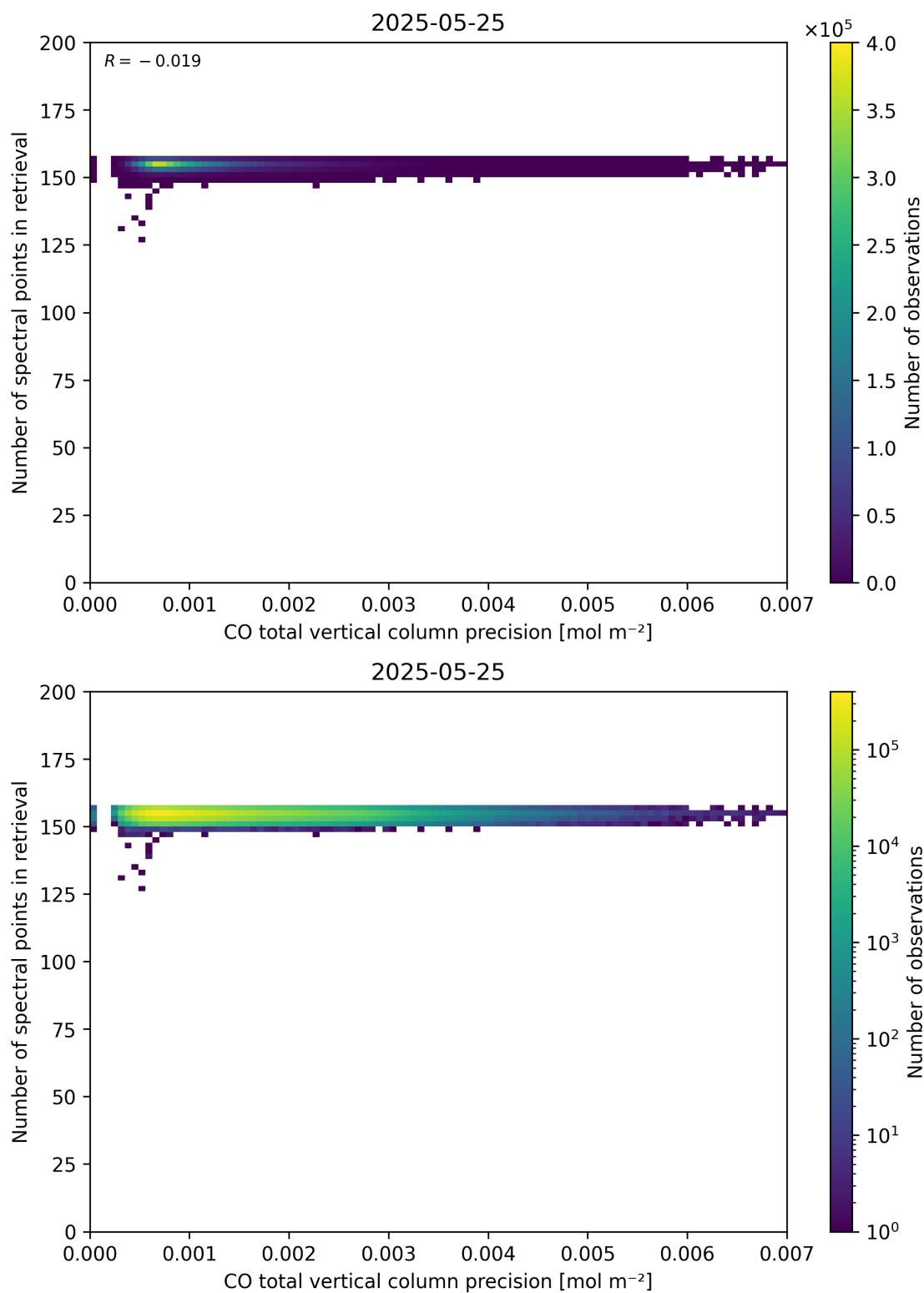
Figure 47: Scatter density plot of “CO total vertical column precision” against “Number of spectral points in retrieval” for 2025-05-24 to 2025-05-26.
