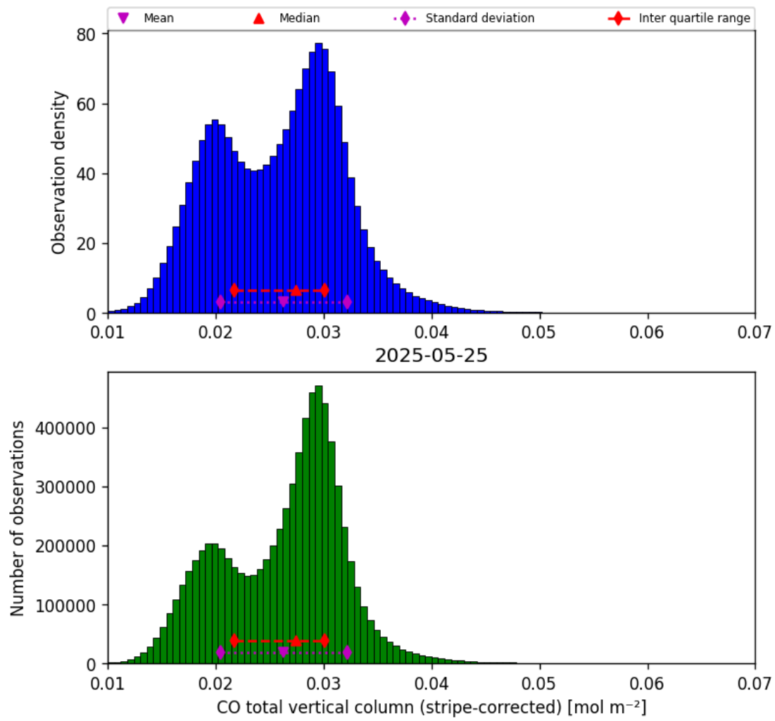
Figure 19: Histogram of “CO total vertical column (stripe-corrected)” for 2025-05-24 to 2025-05-26
