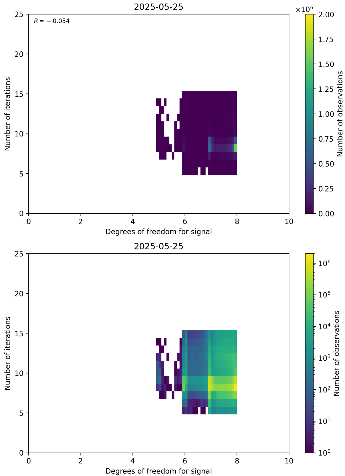
Figure 50: Scatter density plot of “Degrees of freedom for signal” against “Number of iterations” for 2025-05-24 to 2025-05-26.
