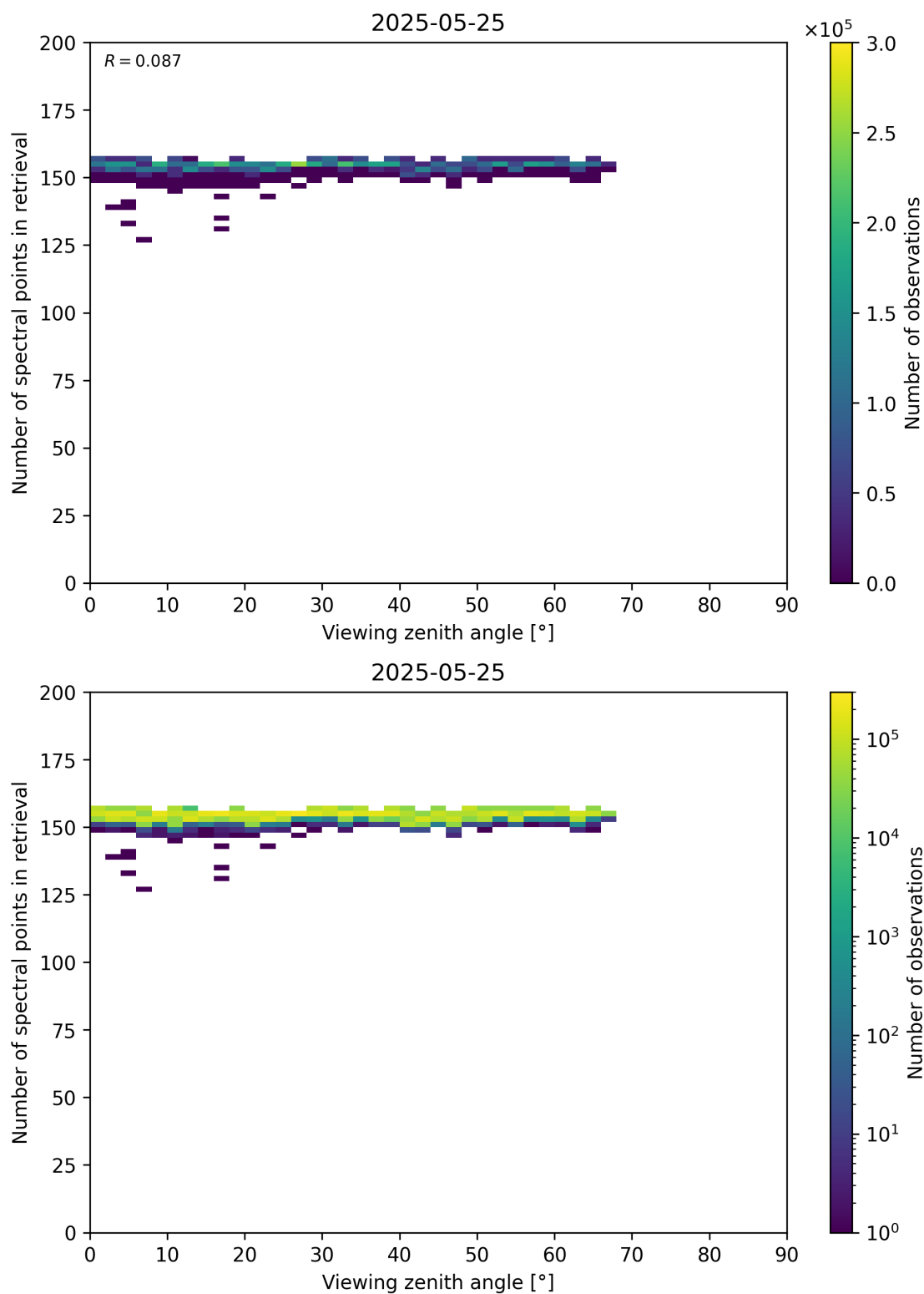
Figure 76: Scatter density plot of “Viewing zenith angle” against “Number of spectral points in retrieval” for 2025-05-24 to 2025-05-26.
