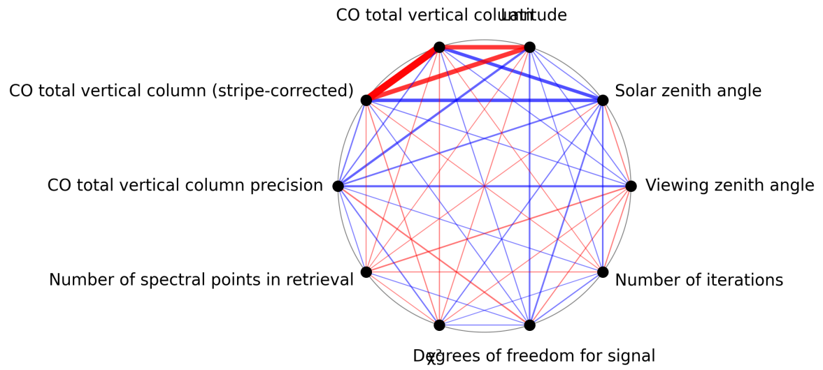
Figure 1: Map of correlation graph for 2025-05-24 to 2025-05-26.
