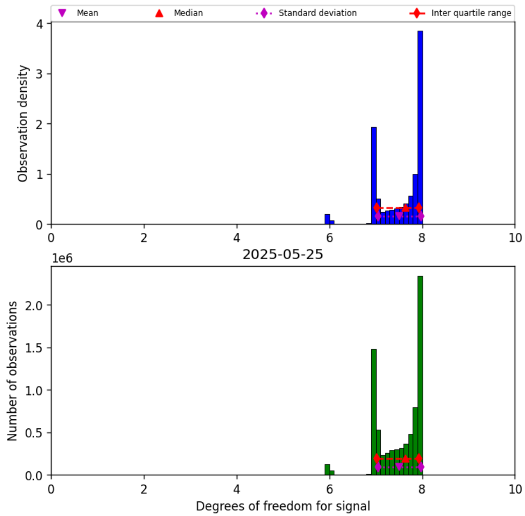
Figure 23: Histogram of “Degrees of freedom for signal” for 2025-05-24 to 2025-05-26
