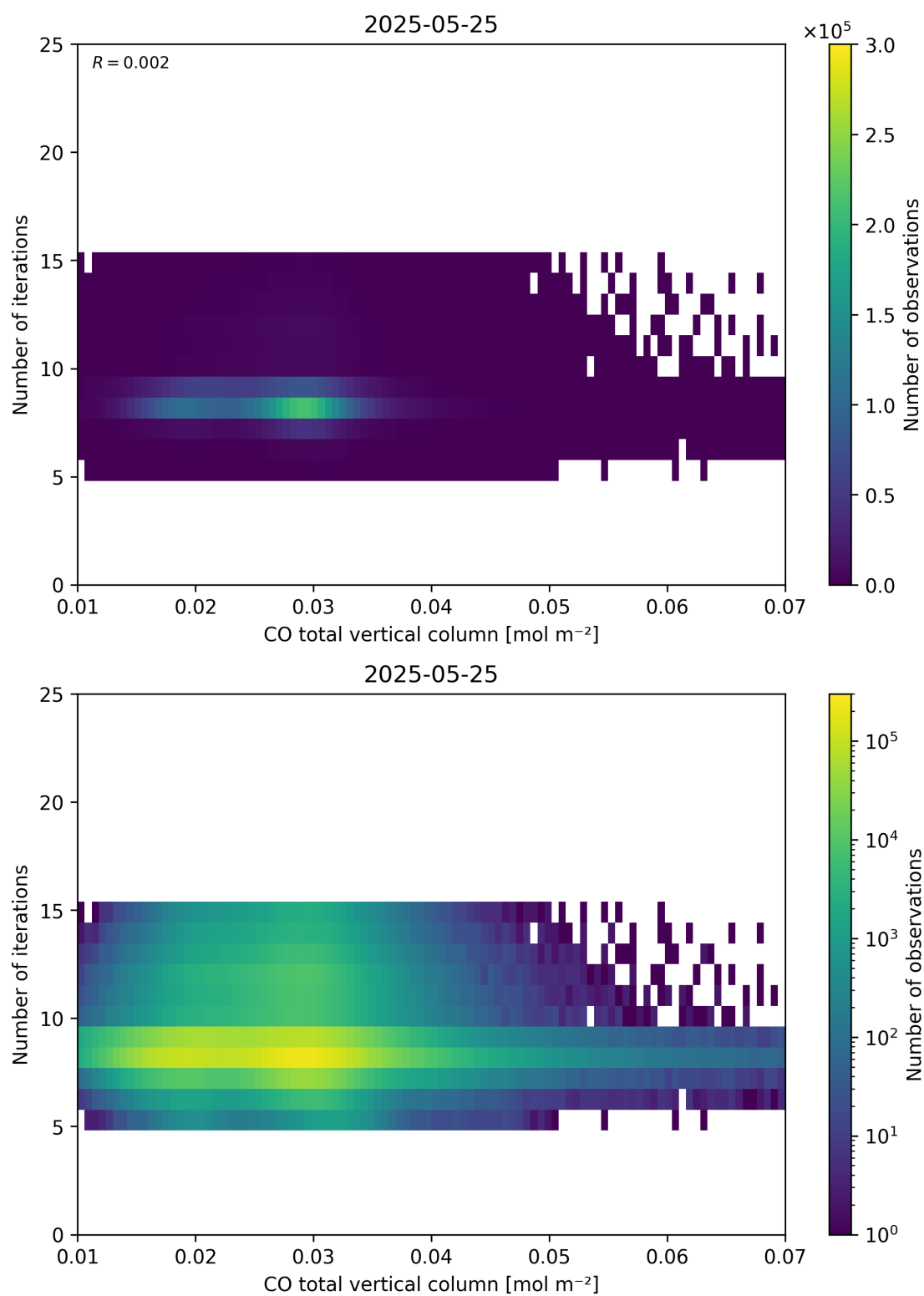
Figure 42: Scatter density plot of “CO total vertical column” against “Number of iterations” for 2025-05-24 to 2025-05-26.
