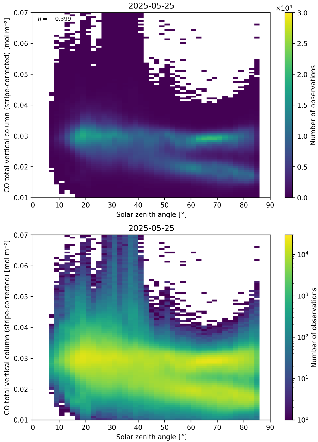
Figure 62: Scatter density plot of “Solar zenith angle” against “CO total vertical column (stripe-corrected)” for 2025-05-24 to 2025-05-26.
