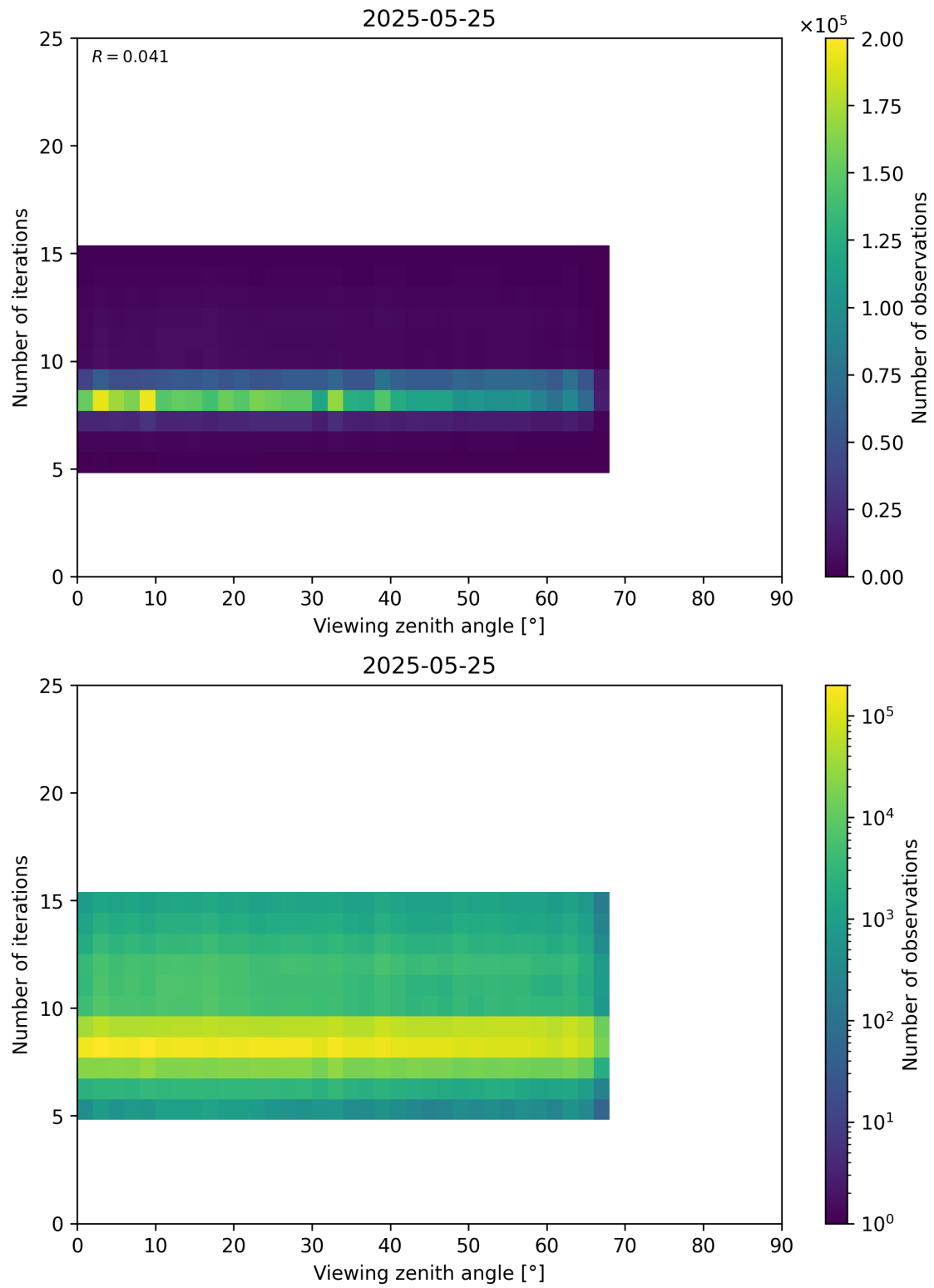
Figure 75: Scatter density plot of “Viewing zenith angle” against “Number of iterations” for 2025-05-24 to 2025-05-26.
