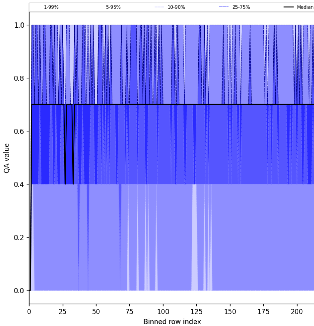
Figure 25: Along track statistics of “QA value” for 2025-05-24 to 2025-05-26
