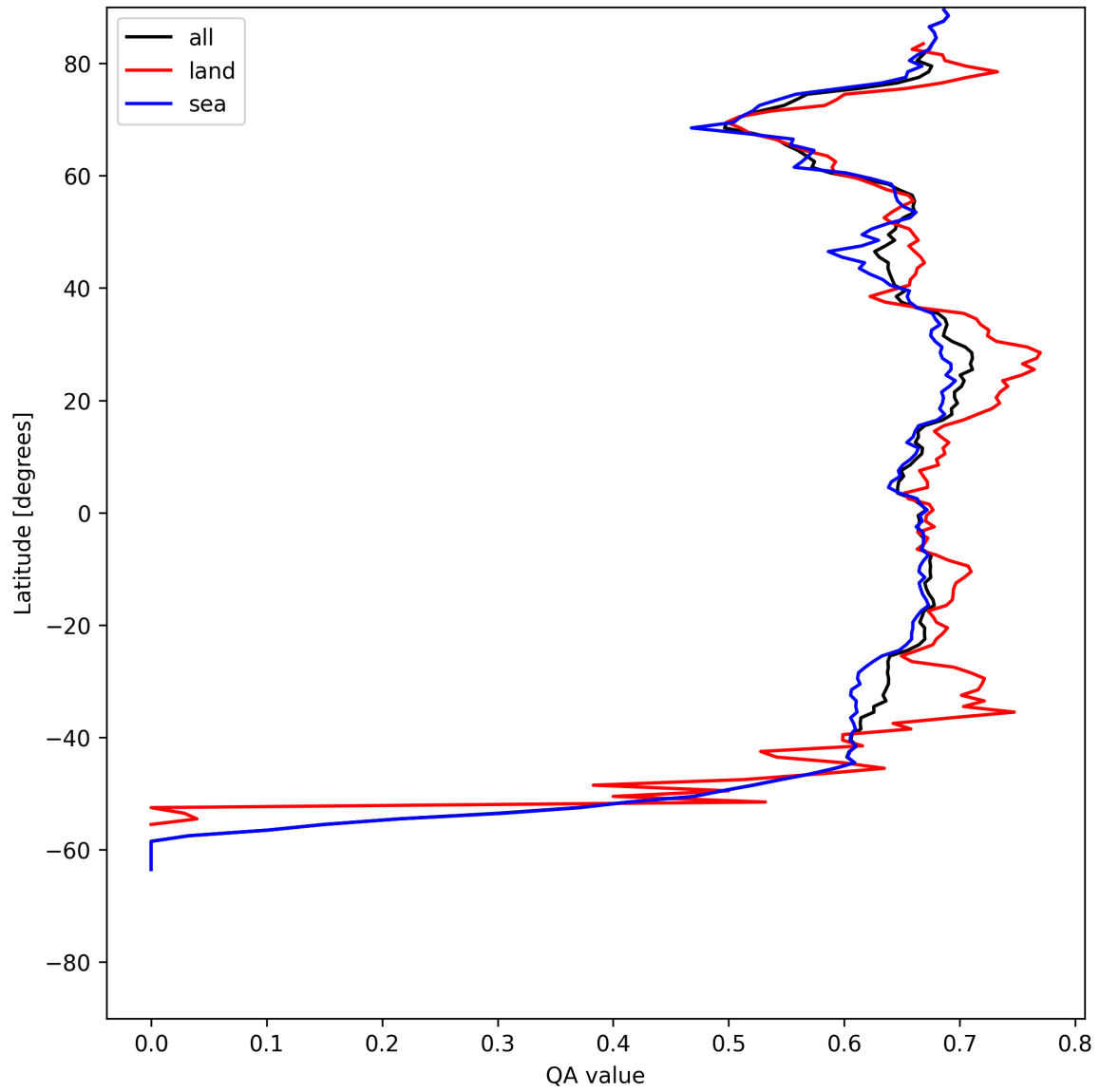
Figure 9: Zonal average of “QA value” for 2025-05-24 to 2025-05-26.
