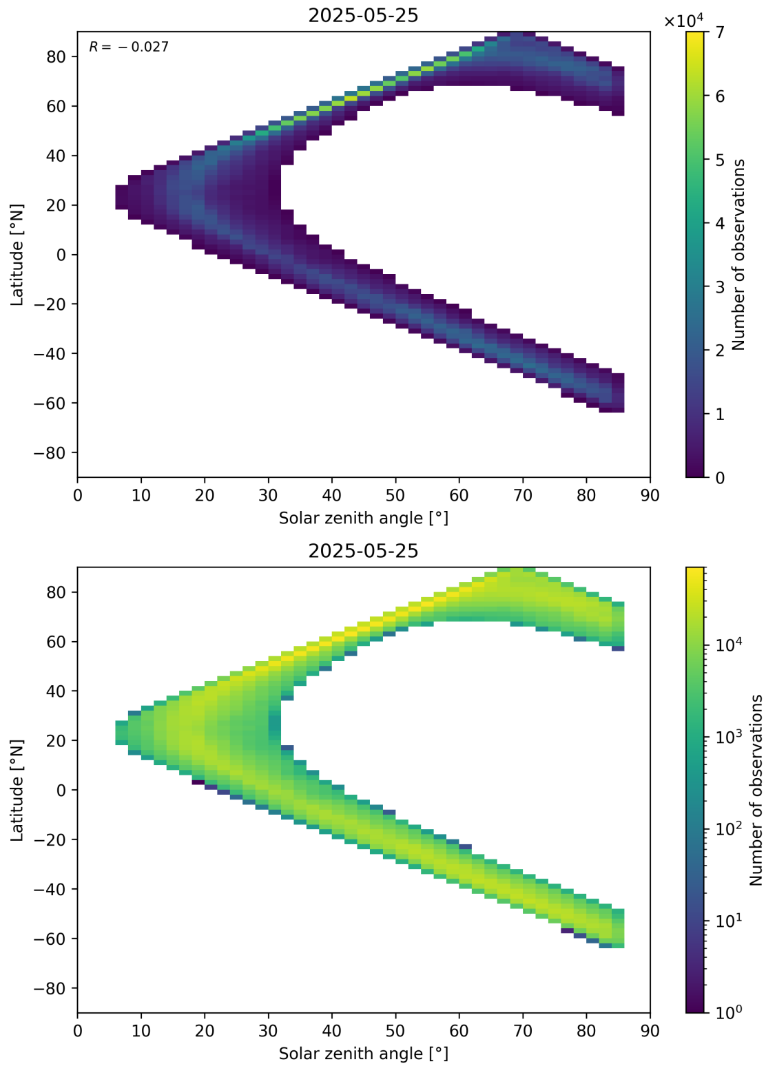
Figure 66: Scatter density plot of “Solar zenith angle” against “Latitude” for 2025-05-24 to 2025-05-26.
