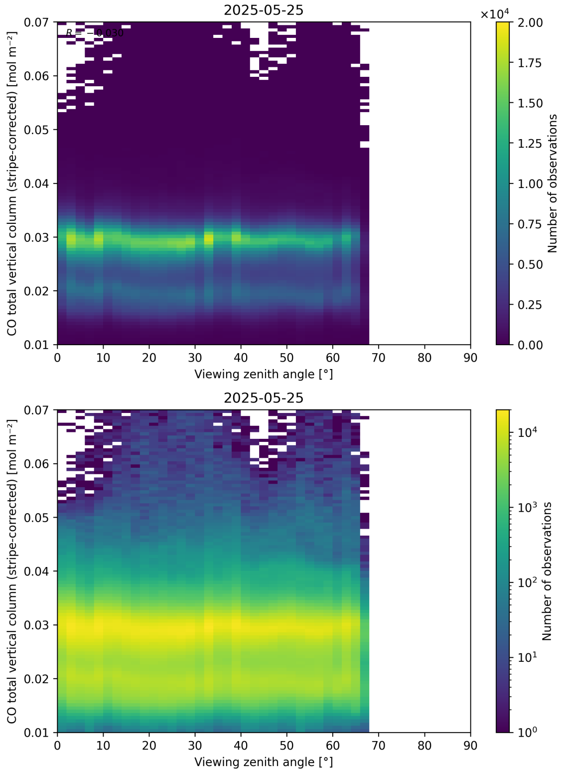
Figure 70: Scatter density plot of “Viewing zenith angle” against “CO total vertical column (stripe-corrected)” for 2025-05-24 to 2025-05-26.
