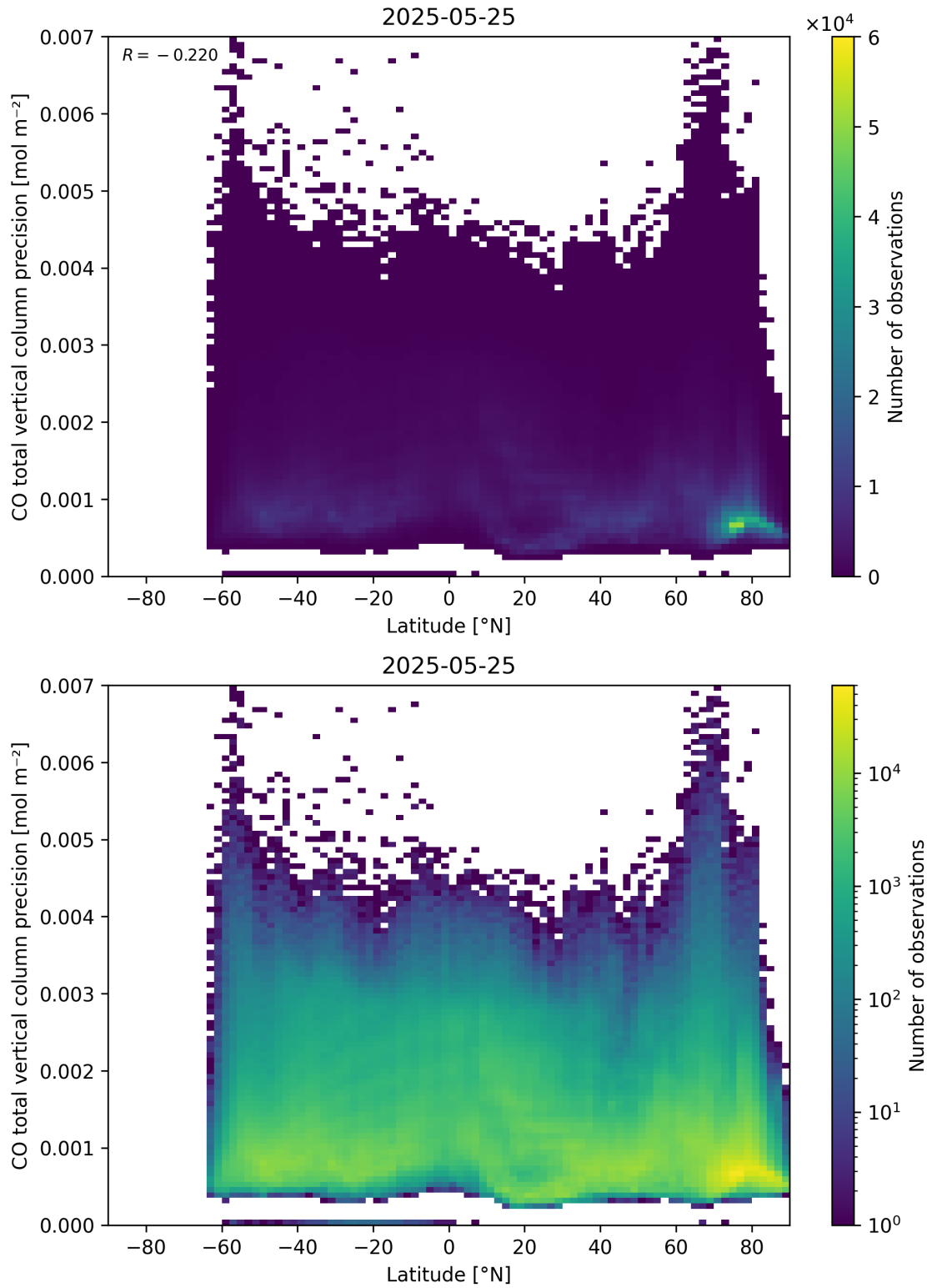
Figure 53: Scatter density plot of “Latitude” against “CO total vertical column precision” for 2025-05-24 to 2025-05-26.
