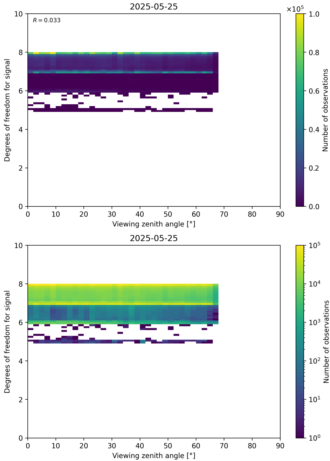
Figure 73: Scatter density plot of “Viewing zenith angle” against “Degrees of freedom for signal” for 2025-05-24 to 2025-05-26.
