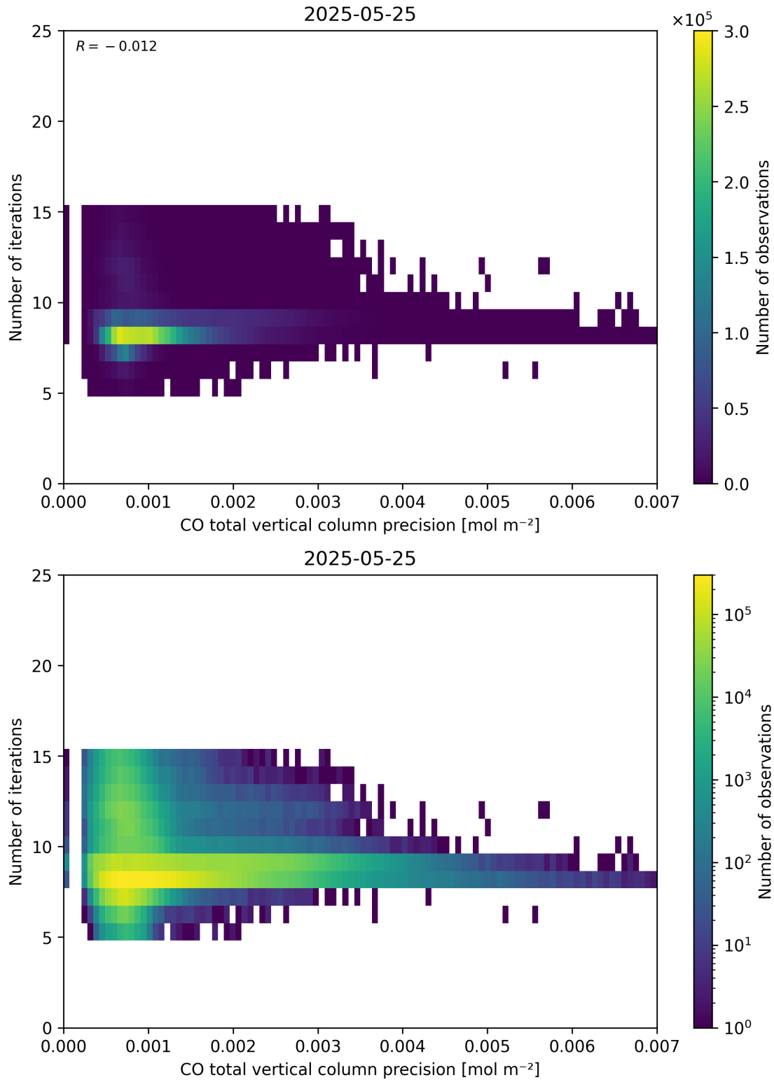
Figure 46: Scatter density plot of “CO total vertical column precision” against “Number of iterations” for 2025-05-24 to 2025-05-26.
