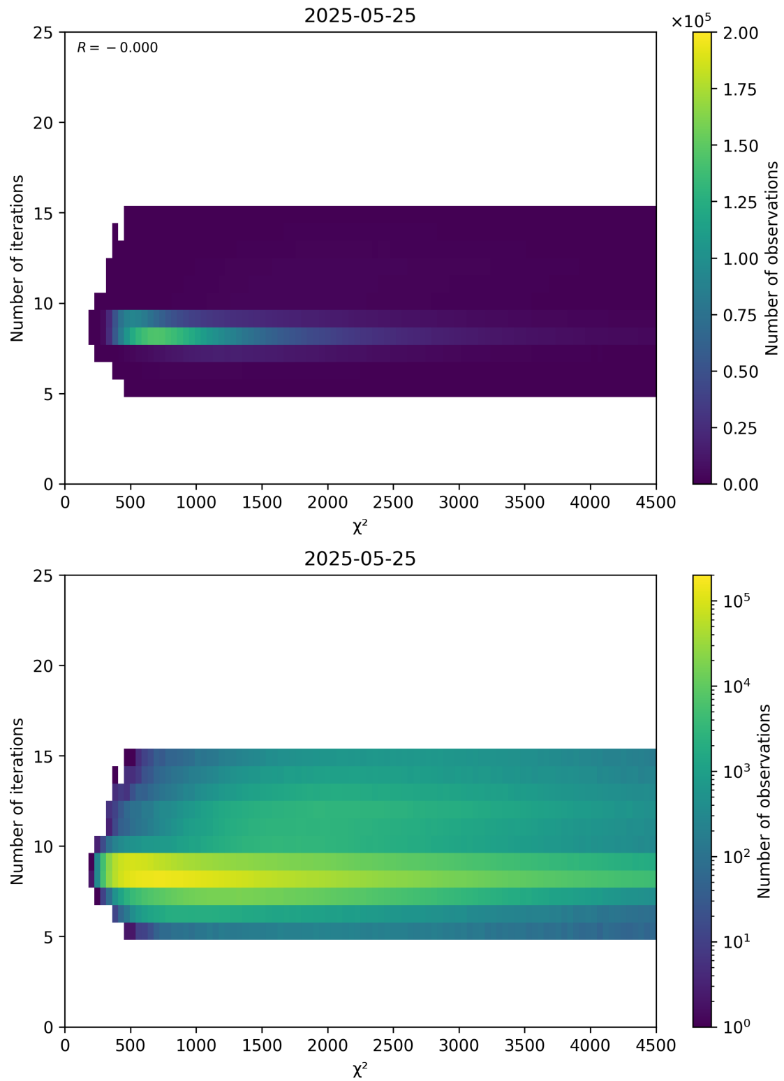
Figure 49: Scatter density plot of “ \chi^2 ” against “Number of iterations” for 2025-05-24 to 2025-05-26.
