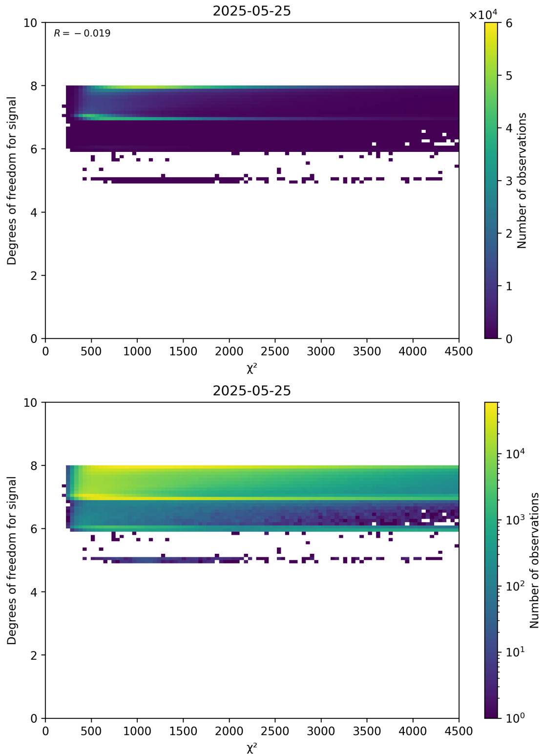
Figure 48: Scatter density plot of “ \chi^2 ” against “Degrees of freedom for signal” for 2025-05-24 to 2025-05-26.
