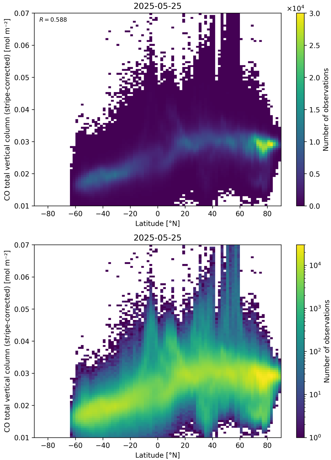
Figure 52: Scatter density plot of “Latitude” against “CO total vertical column (stripe-corrected)” for 2025-05-24 to 2025-05-26.
