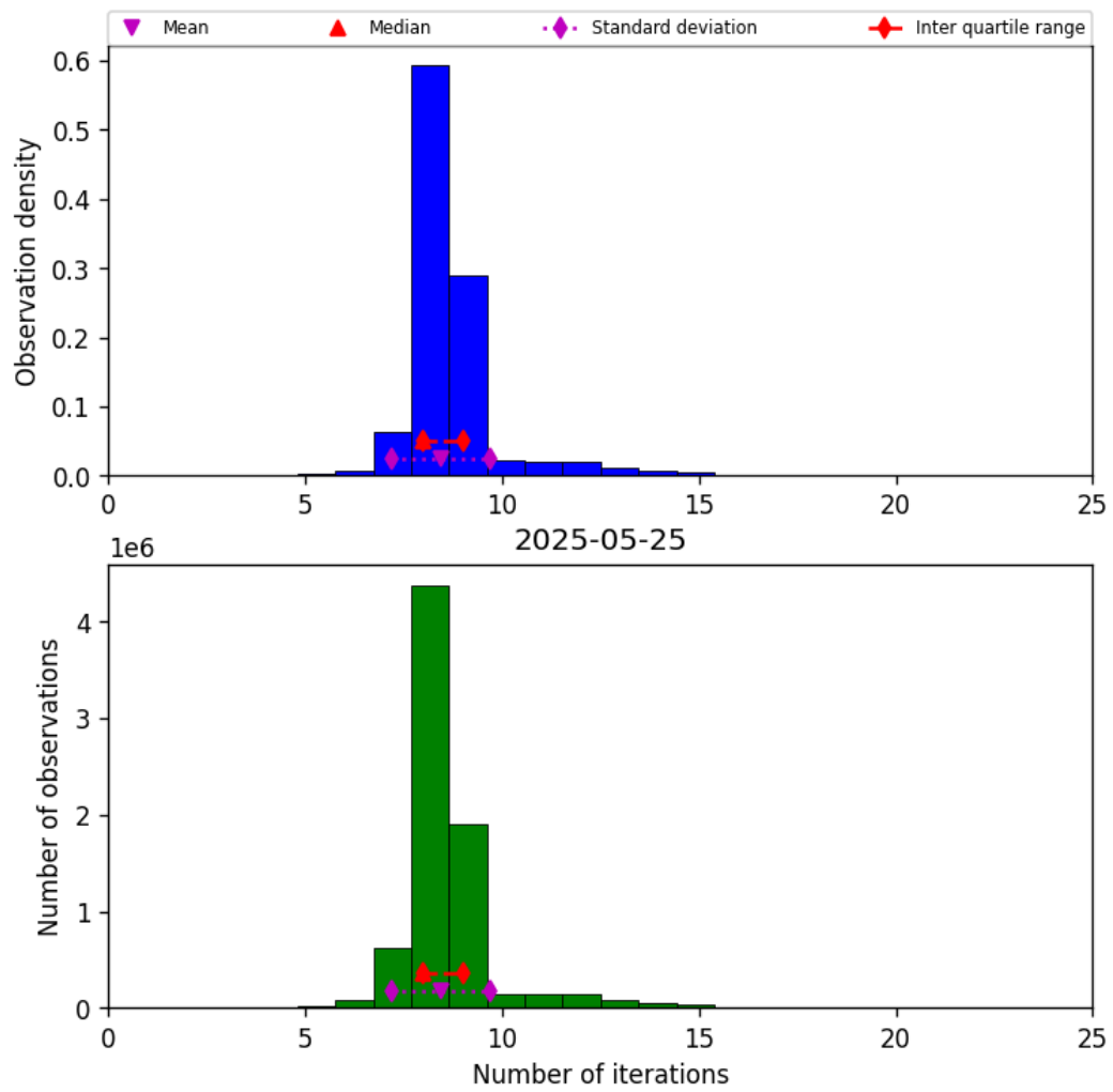
Figure 24: Histogram of “Number of iterations” for 2025-05-24 to 2025-05-26
