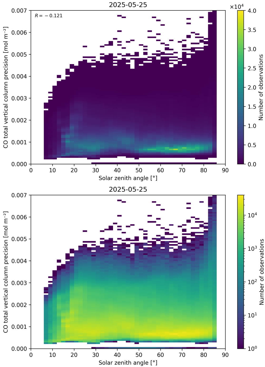
Figure 63: Scatter density plot of “Solar zenith angle” against “CO total vertical column precision” for 2025-05-24 to 2025-05-26.
