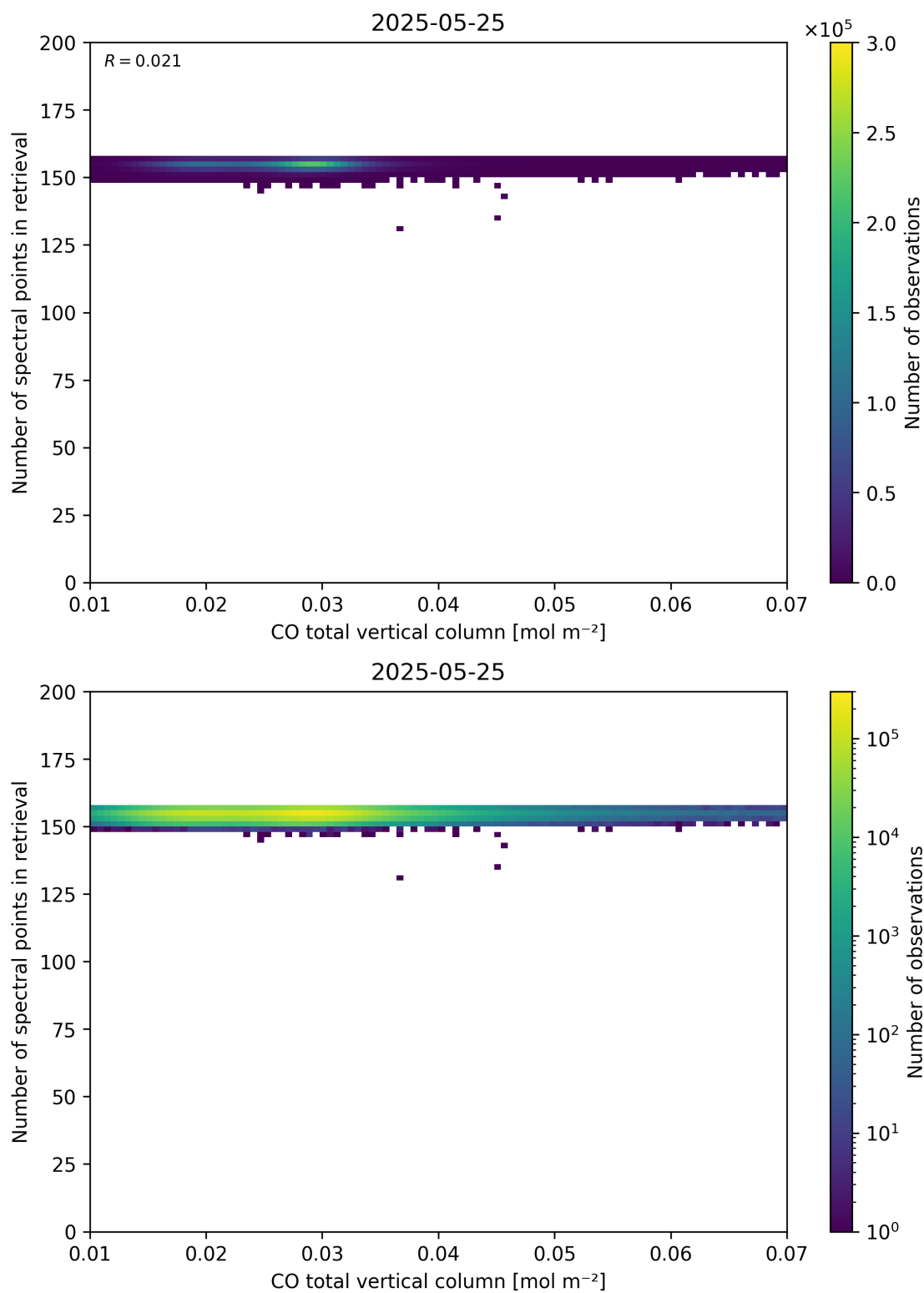
Figure 43: Scatter density plot of “CO total vertical column” against “Number of spectral points in retrieval” for 2025-05-24 to 2025-05-26.
