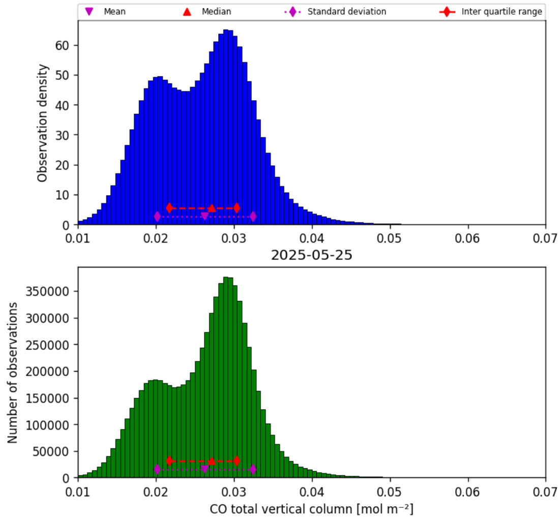
Figure 18: Histogram of “CO total vertical column” for 2025-05-24 to 2025-05-26
