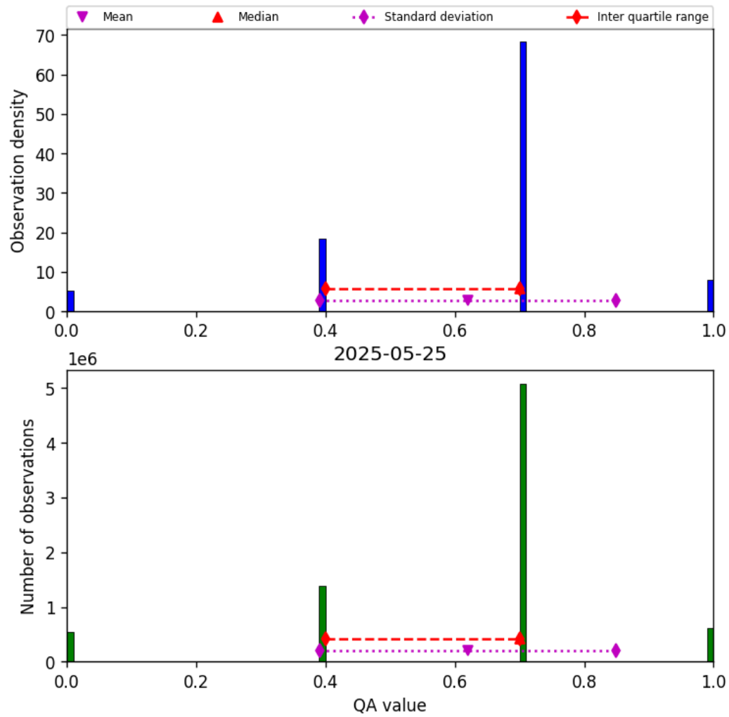
Figure 17: Histogram of “QA value” for 2025-05-24 to 2025-05-26
