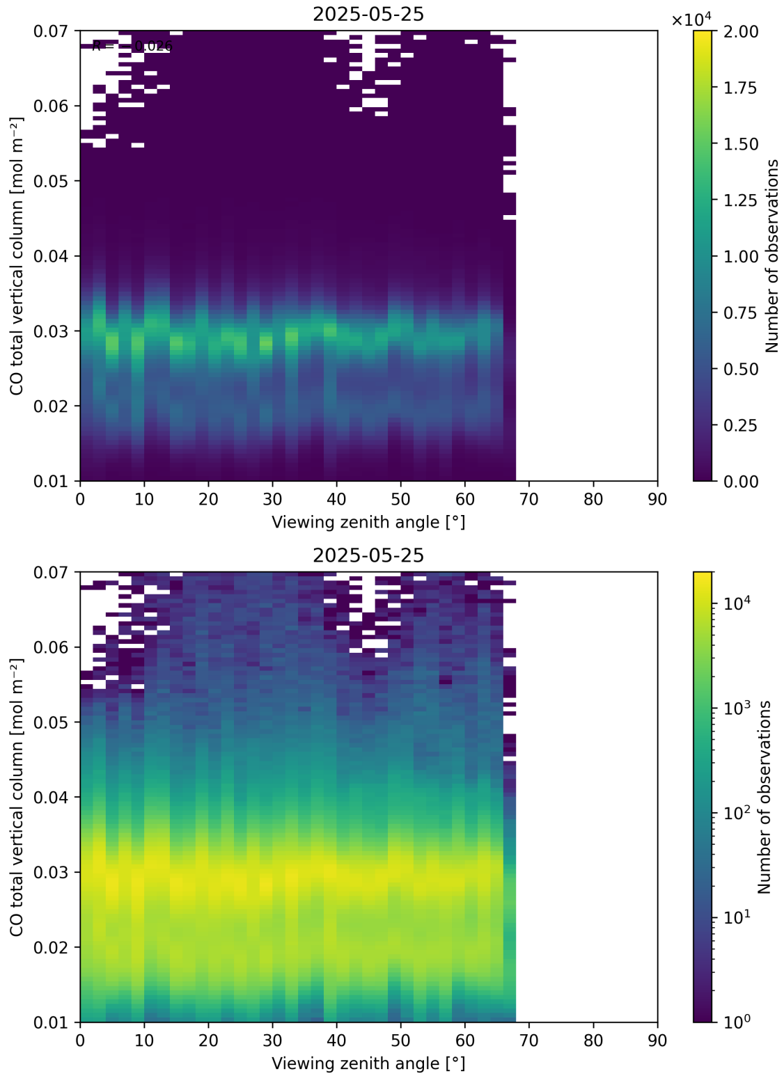
Figure 69: Scatter density plot of “Viewing zenith angle” against “CO total vertical column” for 2025-05-24 to 2025-05-26.
