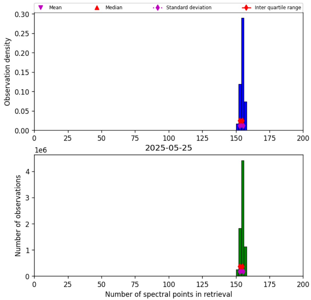
Figure 21: Histogram of “Number of spectral points in retrieval” for 2025-05-24 to 2025-05-26
