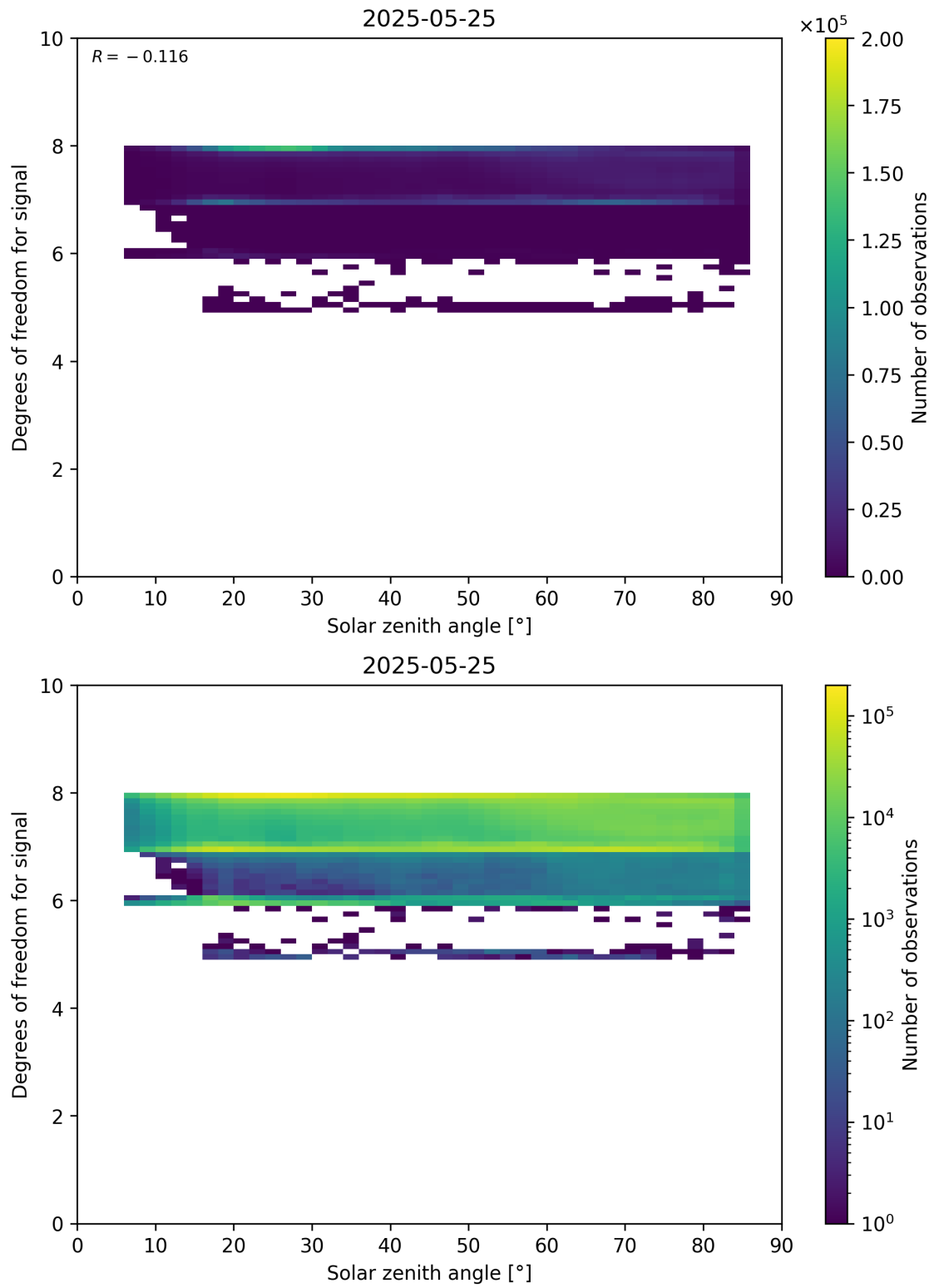
Figure 65: Scatter density plot of “Solar zenith angle” against “Degrees of freedom for signal” for 2025-05-24 to 2025-05-26.
