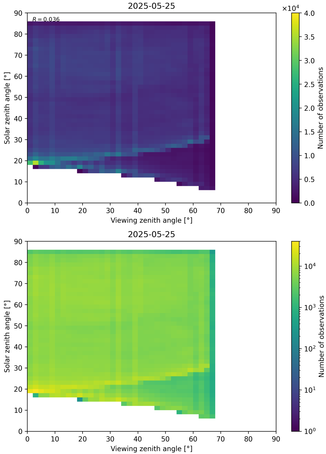
Figure 77: Scatter density plot of “Viewing zenith angle” against “Solar zenith angle” for 2025-05-24 to 2025-05-26.
