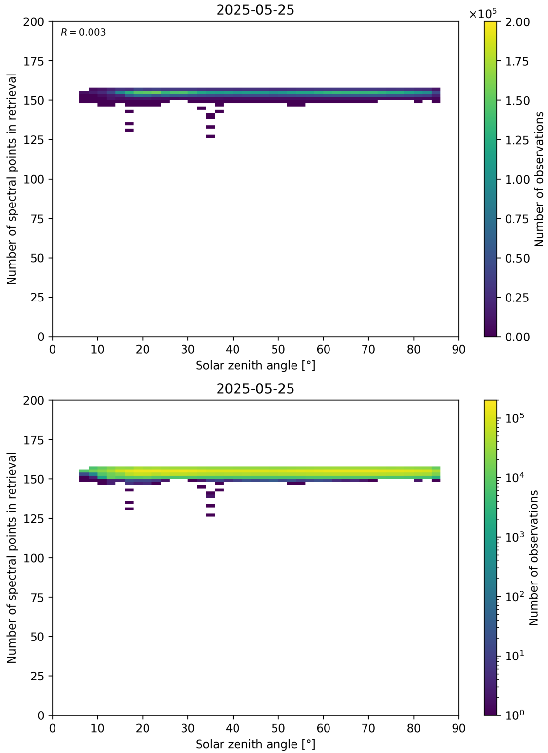
Figure 68: Scatter density plot of “Solar zenith angle” against “Number of spectral points in retrieval” for 2025-05-24 to 2025-05-26.
