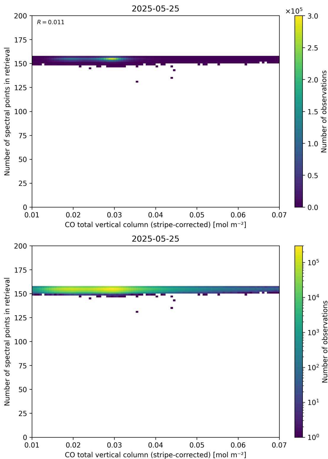
Figure 40: Scatter density plot of “CO total vertical column (stripe-corrected)” against “Number of spectral points in retrieval” for 2025-05-24 to 2025-05-26.
