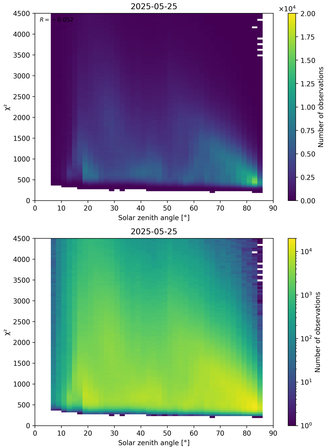
Figure 64: Scatter density plot of “Solar zenith angle” against “ \chi^2 ” for 2025-05-24 to 2025-05-26.
