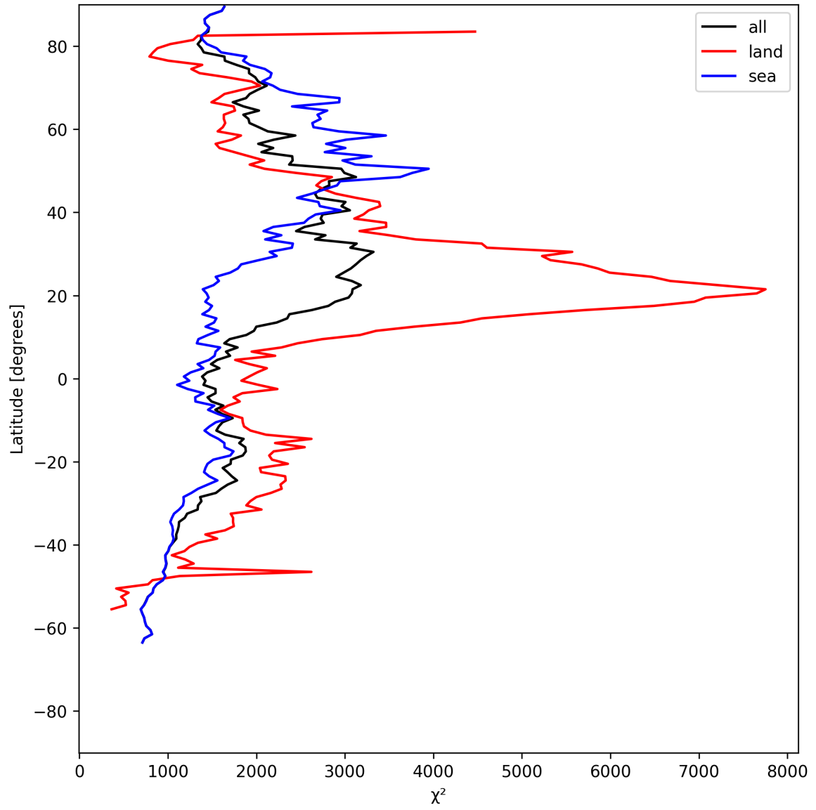
Figure 14: Zonal average of “ \chi^2 ” for 2025-05-24 to 2025-05-26.
