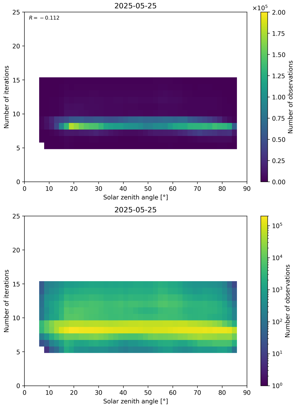
Figure 67: Scatter density plot of “Solar zenith angle” against “Number of iterations” for 2025-05-24 to 2025-05-26.
