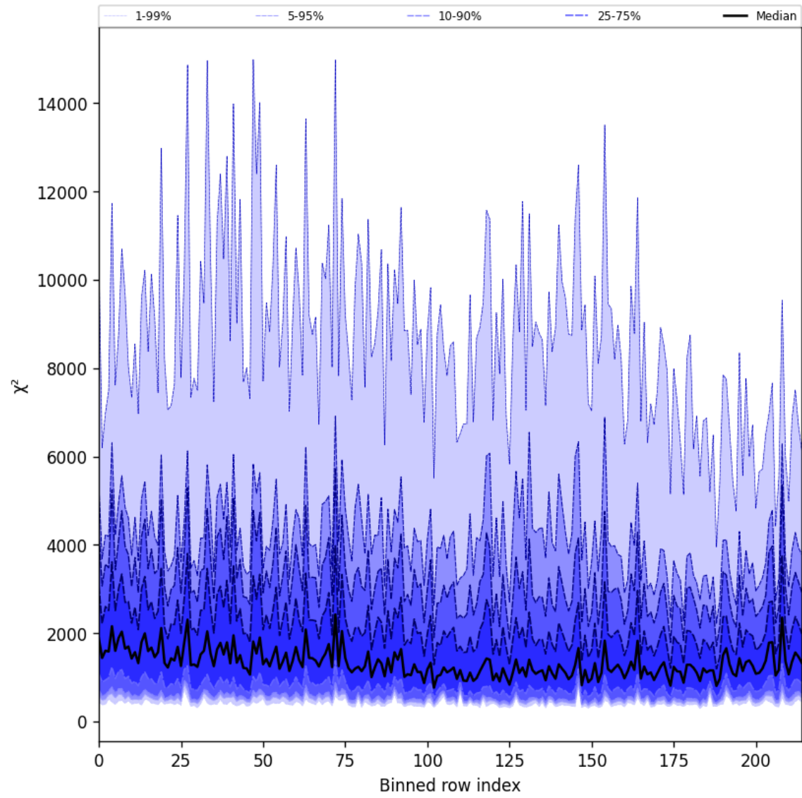
Figure 30: Along track statistics of “ \chi^2 ” for 2025-05-24 to 2025-05-26
