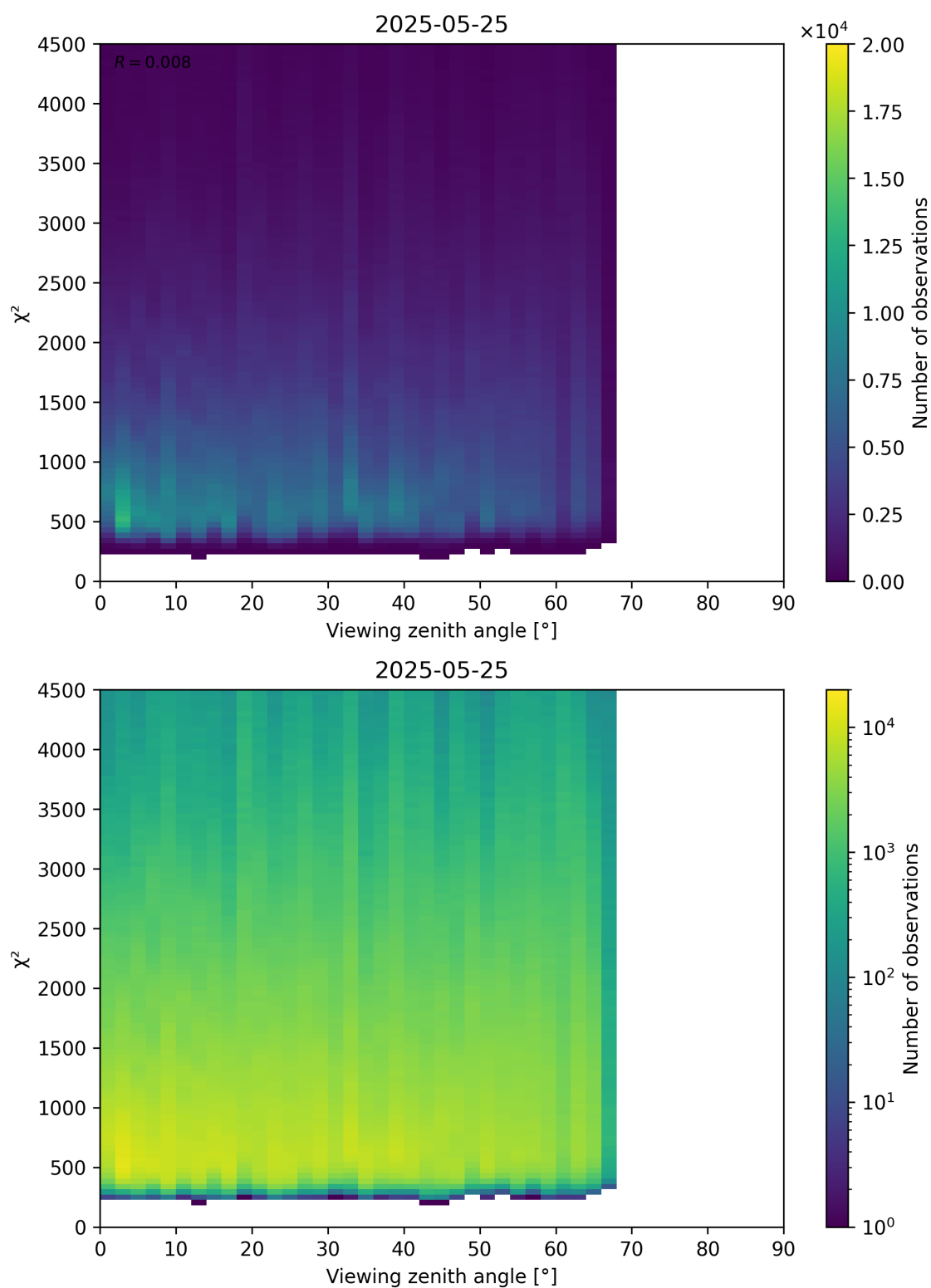
Figure 72: Scatter density plot of “Viewing zenith angle” against “ \chi^2 ” for 2025-05-24 to 2025-05-26.
