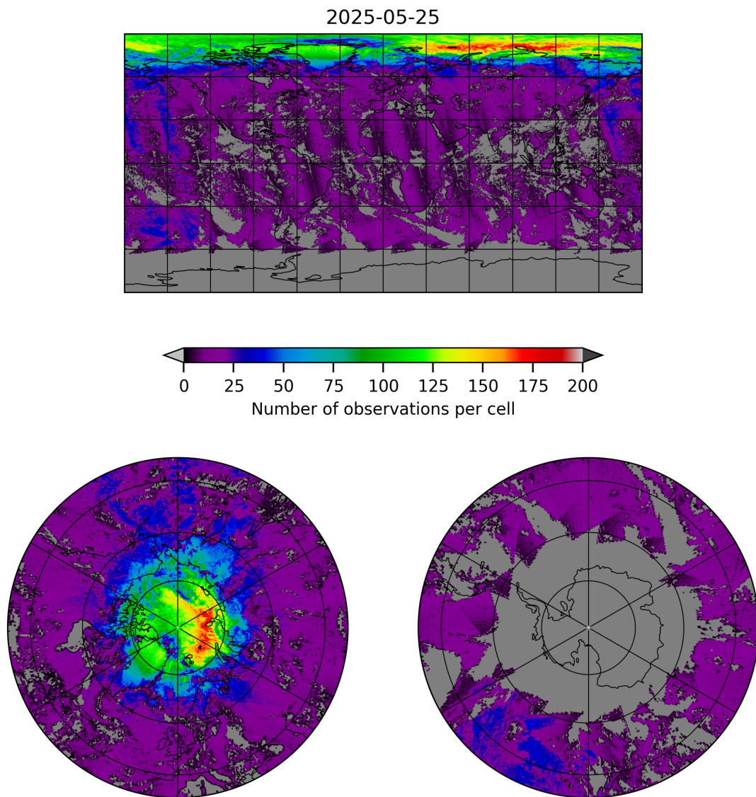
Figure 8: Map of the number of observations for 2025-05-24 to 2025-05-26
