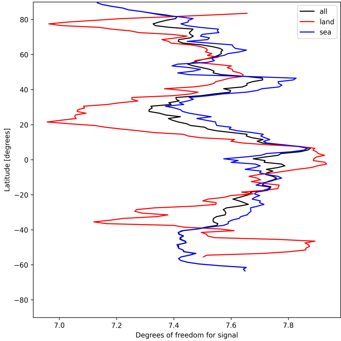
Figure 15: Zonal average of “Degrees of freedom for signal” for 2025-05-24 to 2025-05-26.
