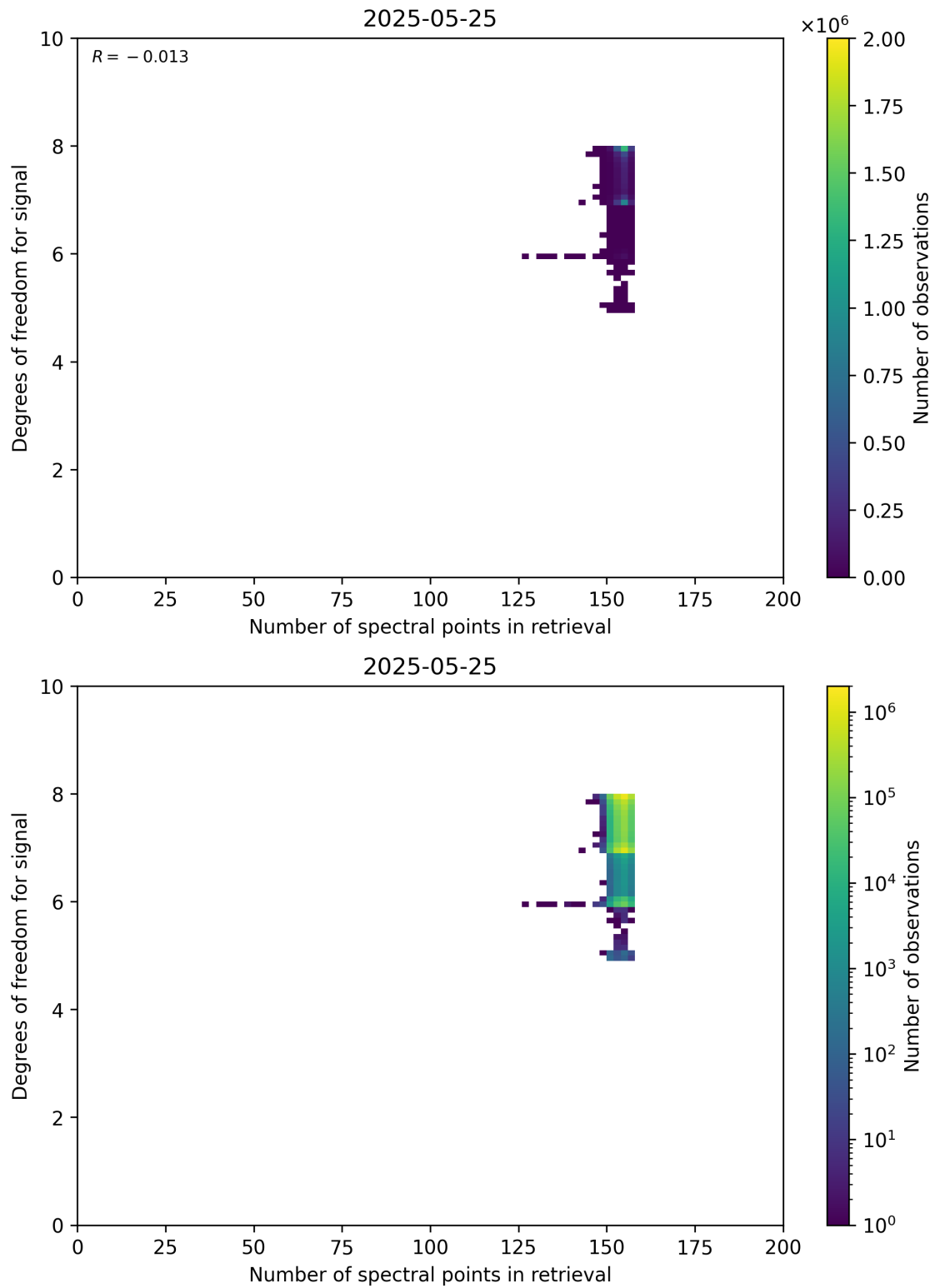
Figure 59: Scatter density plot of “Number of spectral points in retrieval” against “Degrees of freedom for signal” for 2025-05-24 to 2025-05-26.
