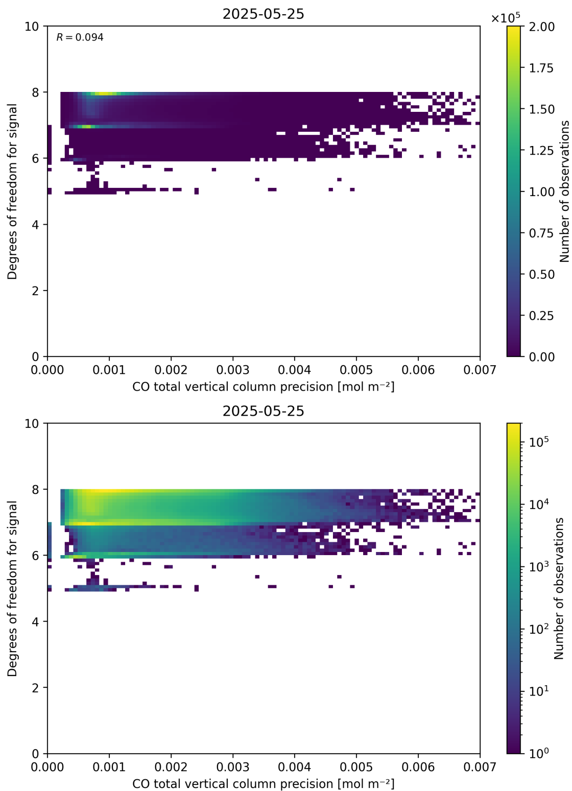
Figure 45: Scatter density plot of “CO total vertical column precision” against “Degrees of freedom for signal” for 2025-05-24 to 2025-05-26.
