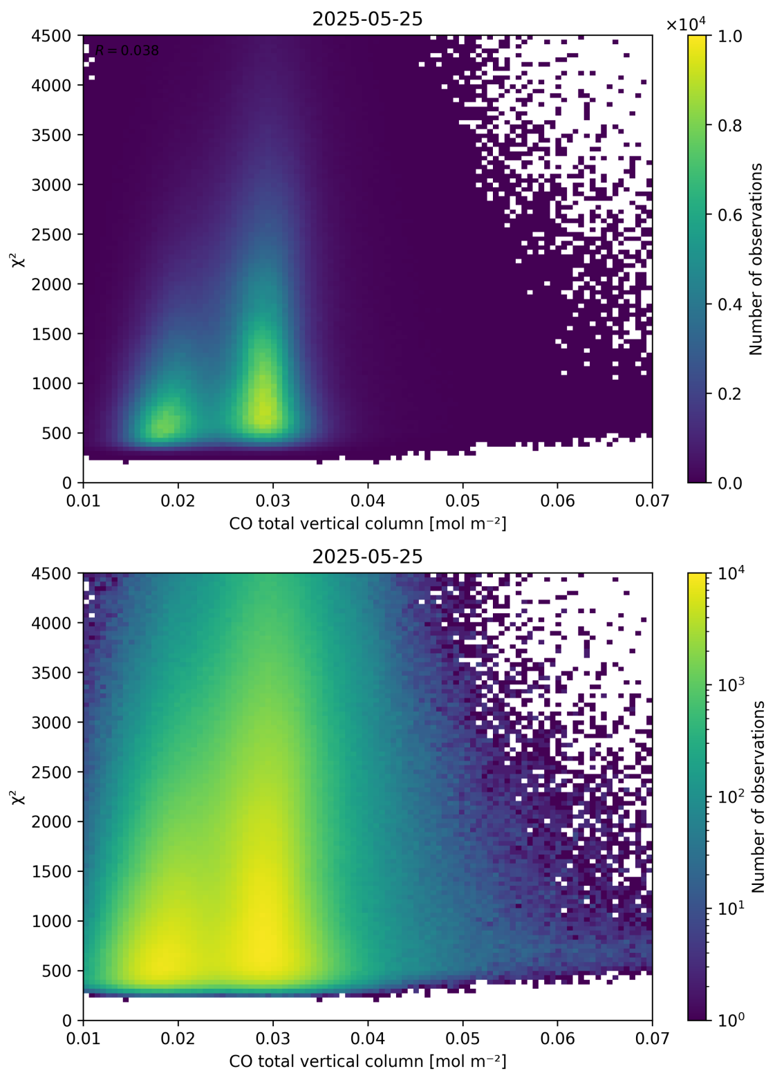
Figure 35: Scatter density plot of “CO total vertical column” against “ \chi^2 ” for 2025-05-24 to 2025-05-26.
