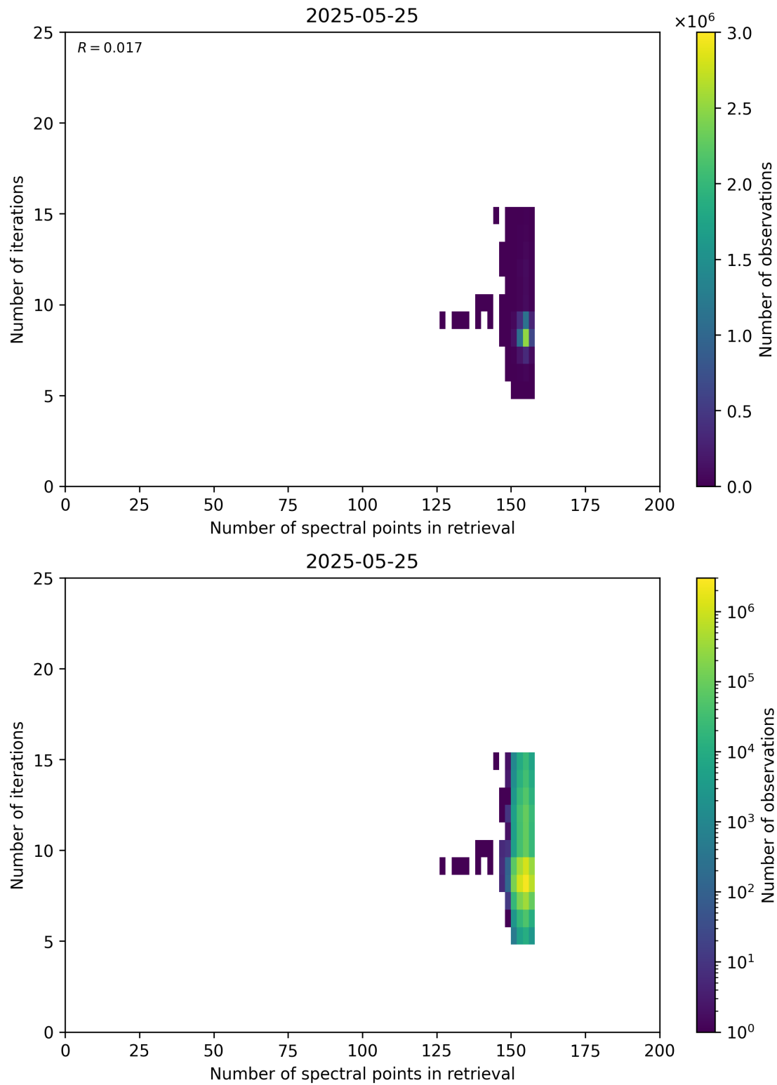
Figure 60: Scatter density plot of “Number of spectral points in retrieval” against “Number of iterations” for 2025-05-24 to 2025-05-26.
