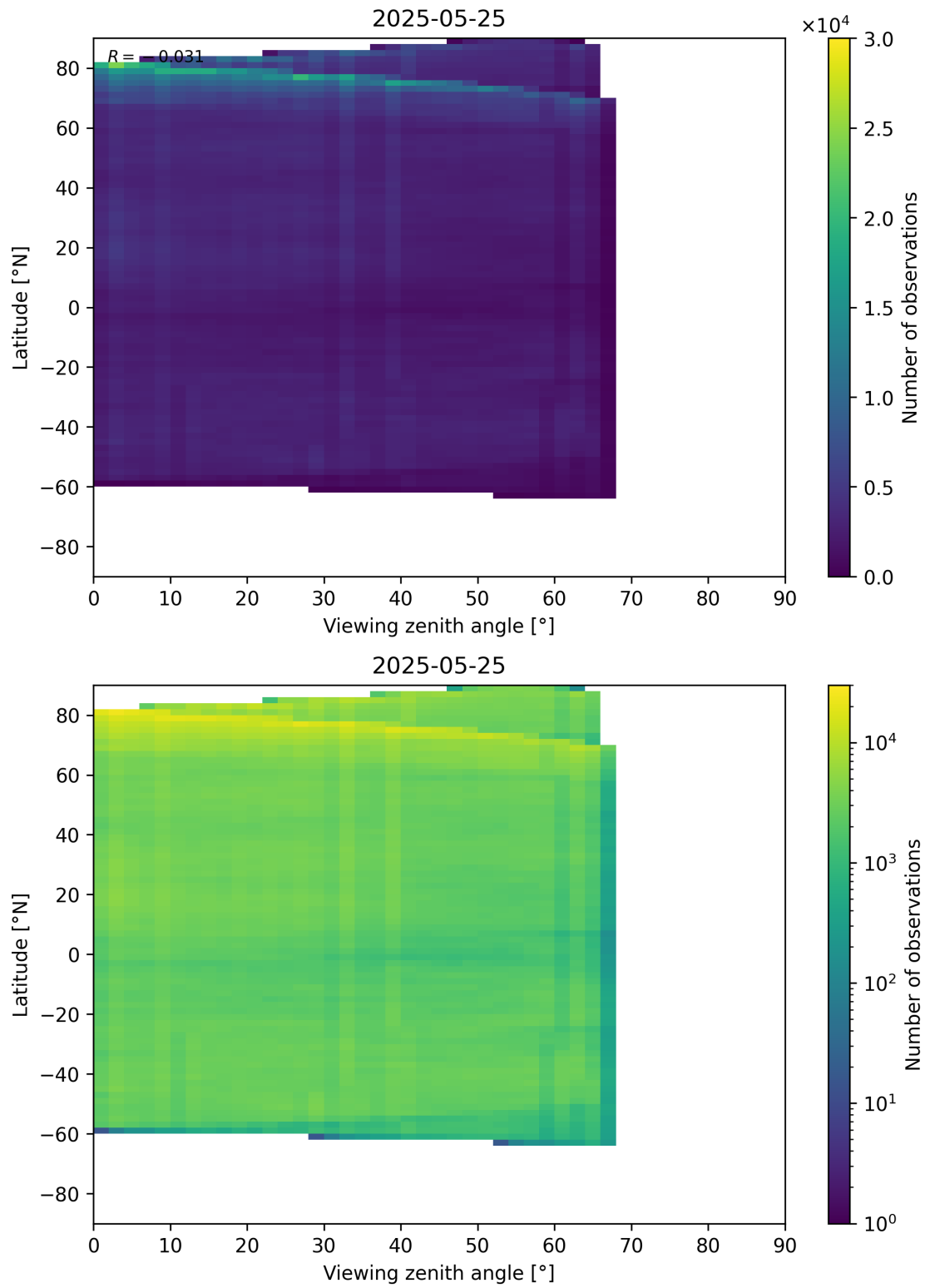
Figure 74: Scatter density plot of “Viewing zenith angle” against “Latitude” for 2025-05-24 to 2025-05-26.
