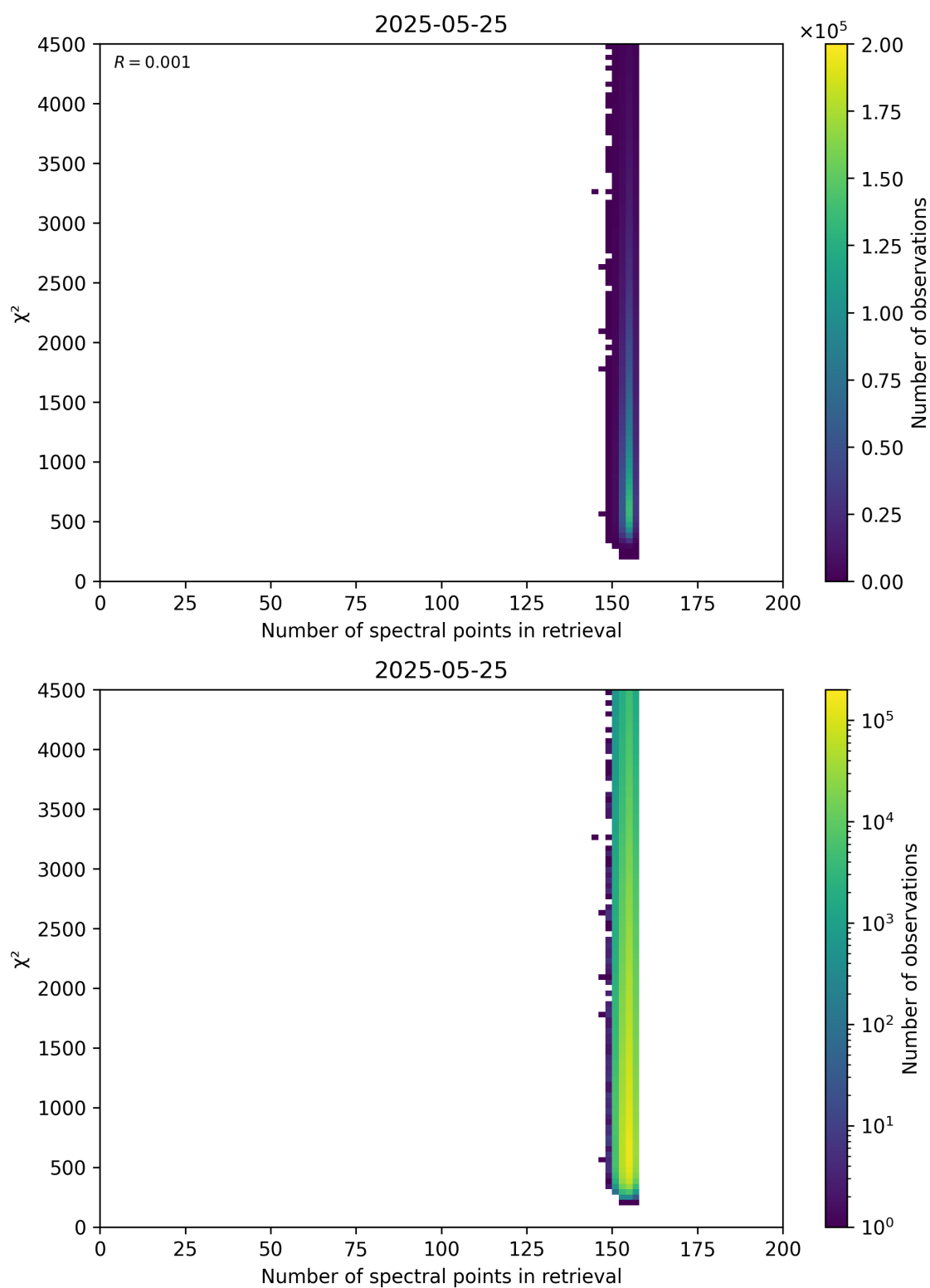
Figure 58: Scatter density plot of “Number of spectral points in retrieval” against “ \chi^2 ” for 2025-05-24 to 2025-05-26.
