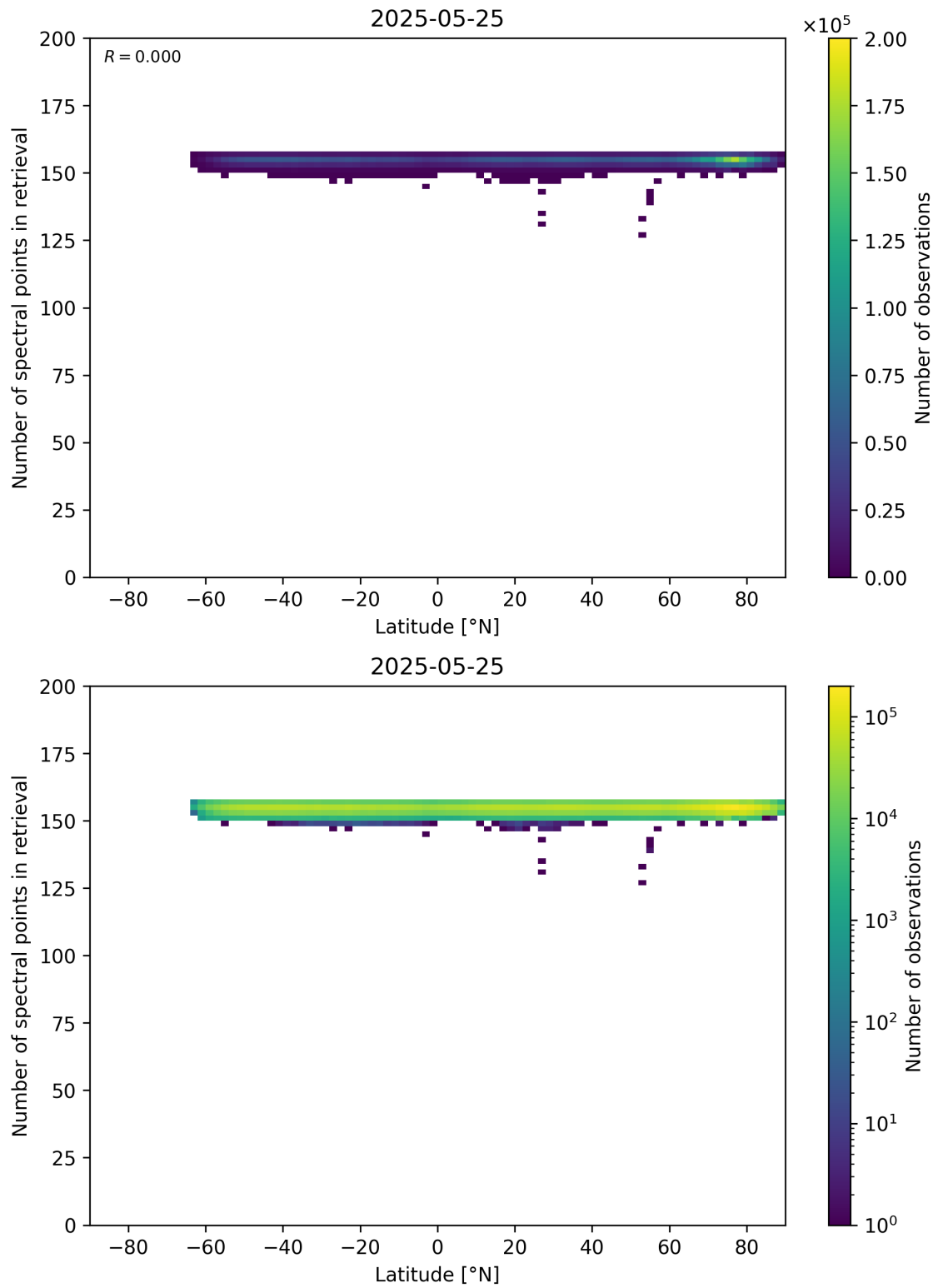
Figure 57: Scatter density plot of “Latitude” against “Number of spectral points in retrieval” for 2025-05-24 to 2025-05-26.
