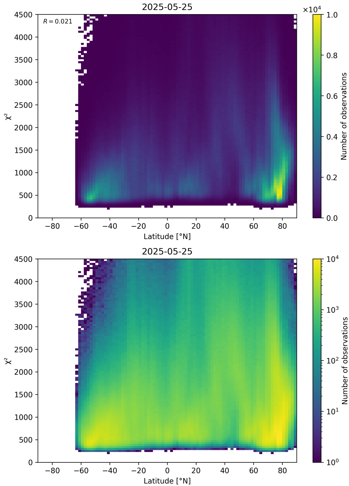
Figure 54: Scatter density plot of “Latitude” against “ \chi^2 ” for 2025-05-24 to 2025-05-26.
