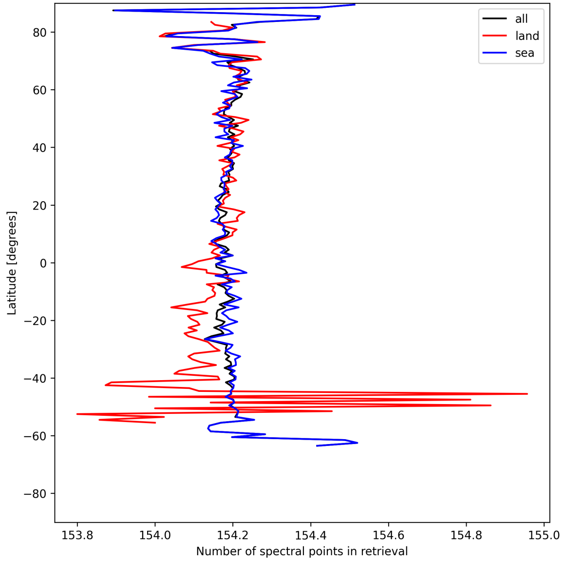
Figure 13: Zonal average of “Number of spectral points in retrieval” for 2025-05-24 to 2025-05-26.
