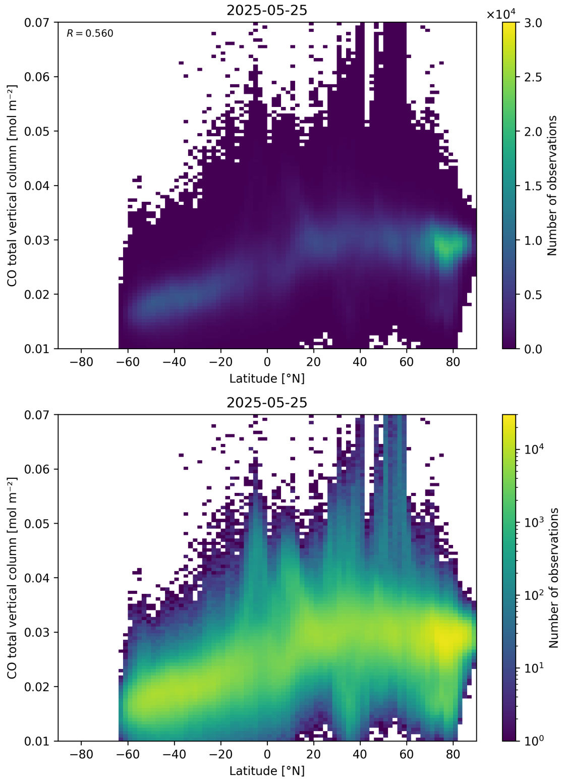
Figure 51: Scatter density plot of “Latitude” against “CO total vertical column” for 2025-05-24 to 2025-05-26.
