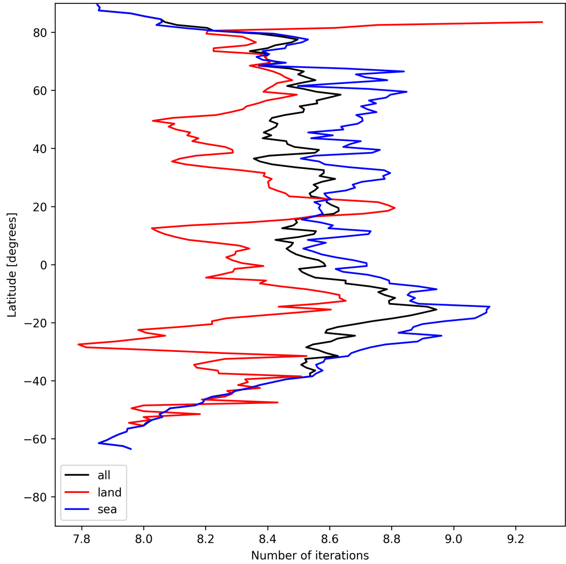
Figure 16: Zonal average of “Number of iterations” for 2025-05-24 to 2025-05-26.
