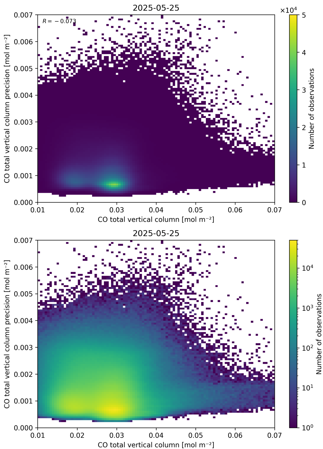
Figure 34: Scatter density plot of “CO total vertical column” against “CO total vertical column precision” for 2025-05-24 to 2025-05-26.
