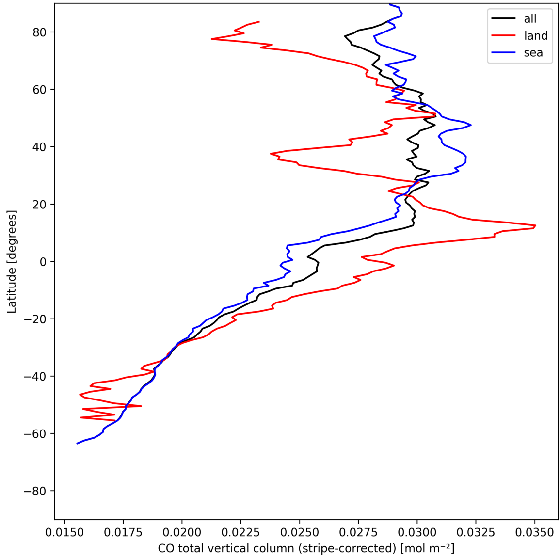
Figure 11: Zonal average of “CO total vertical column (stripe-corrected)” for 2025-05-24 to 2025-05-26.
