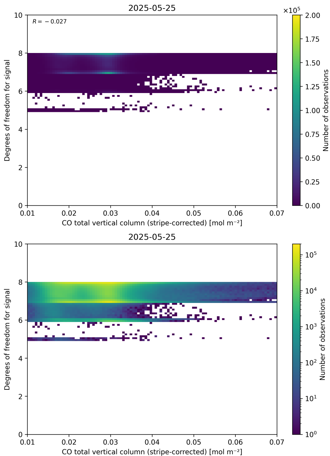
Figure 38: Scatter density plot of “CO total vertical column (stripe-corrected)” against “Degrees of freedom for signal” for 2025-05-24 to 2025-05-26.
