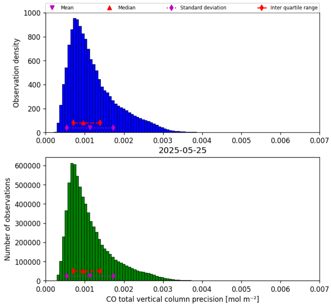
Figure 20: Histogram of “CO total vertical column precision” for 2025-05-24 to 2025-05-26
