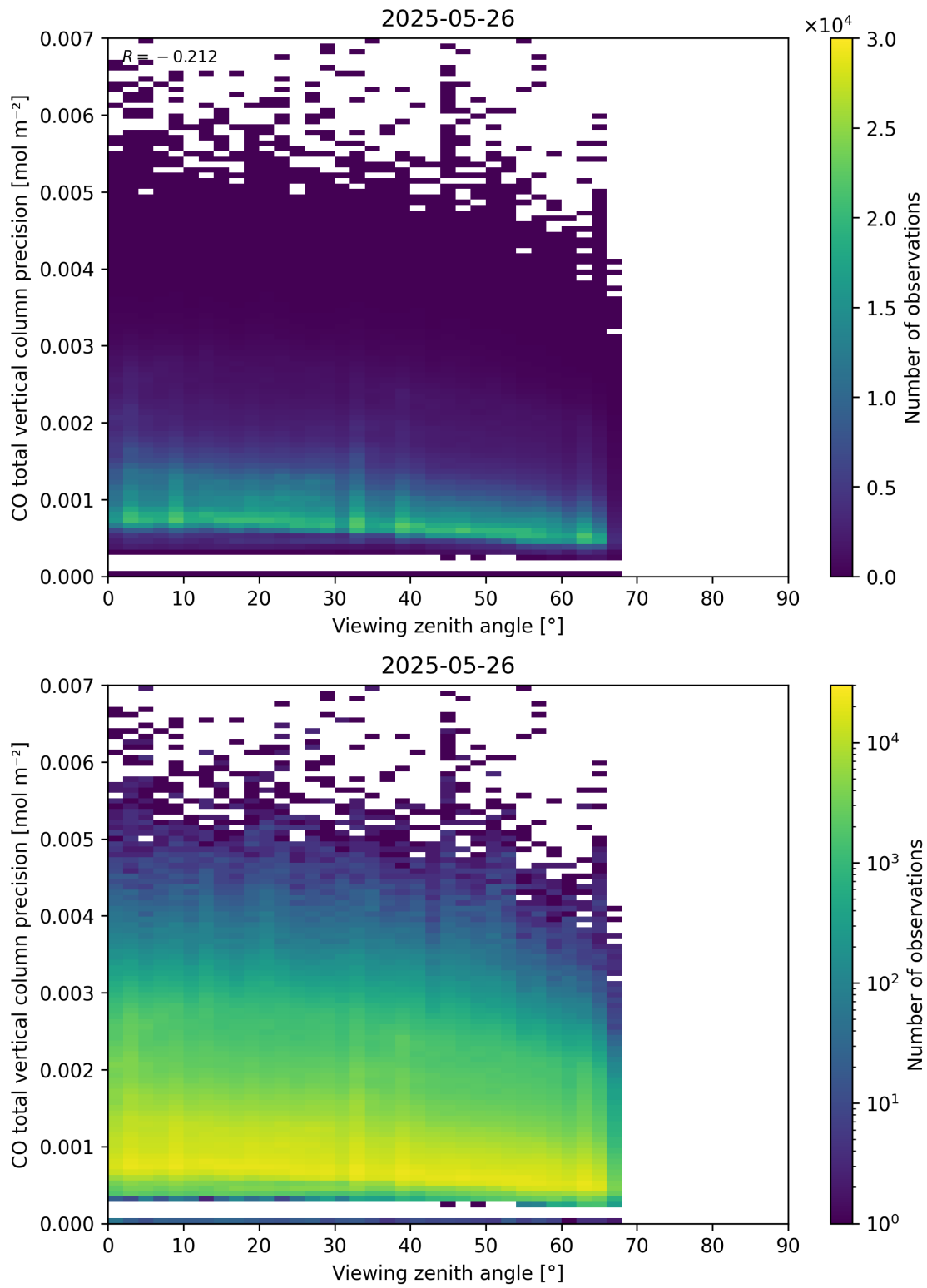
Figure 71: Scatter density plot of “Viewing zenith angle” against “CO total vertical column precision” for 2025-05-26 to 2025-05-27.
