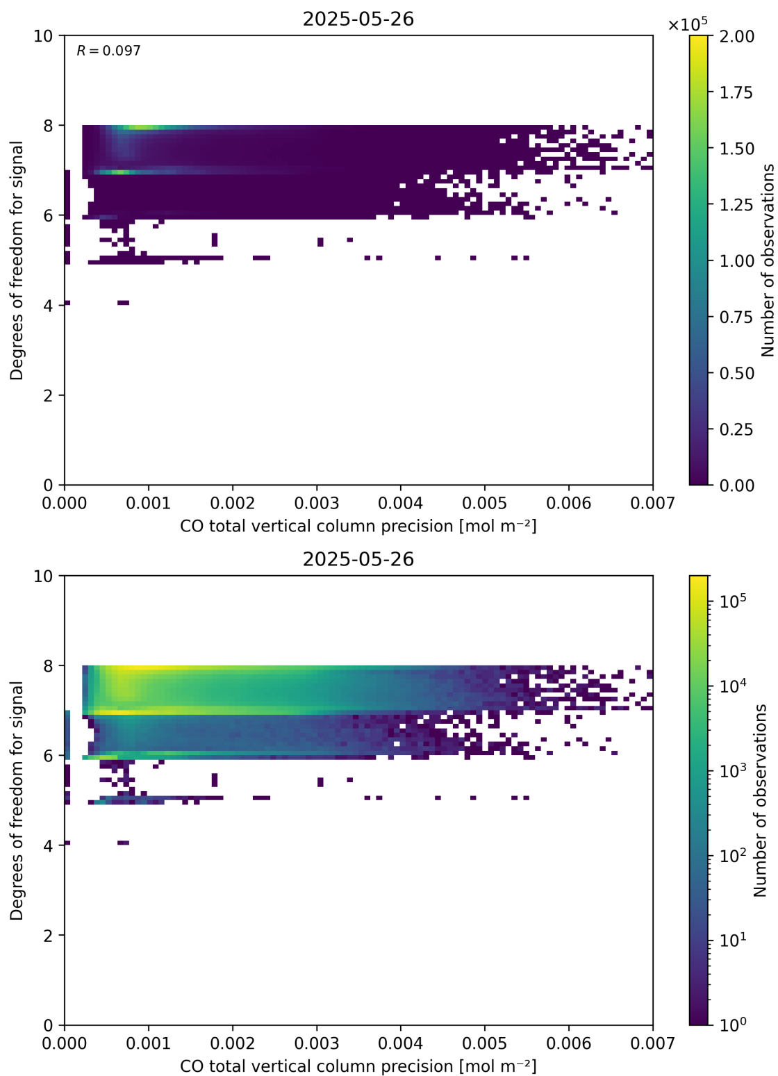
Figure 45: Scatter density plot of “CO total vertical column precision” against “Degrees of freedom for signal” for 2025-05-26 to 2025-05-27.
