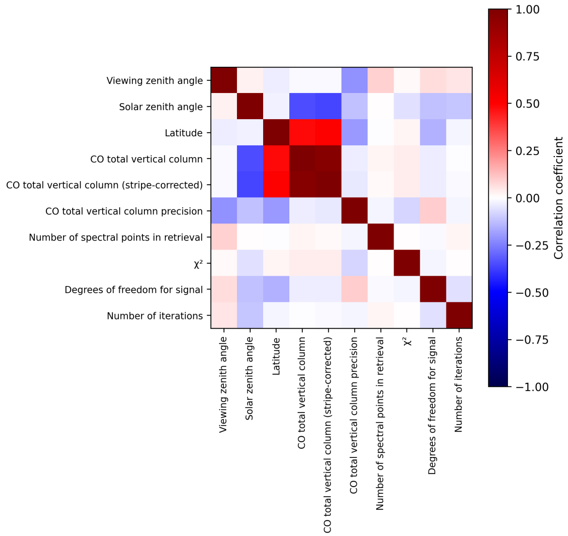
Figure 2: Map of correlation matrix for 2025-05-26 to 2025-05-27.
