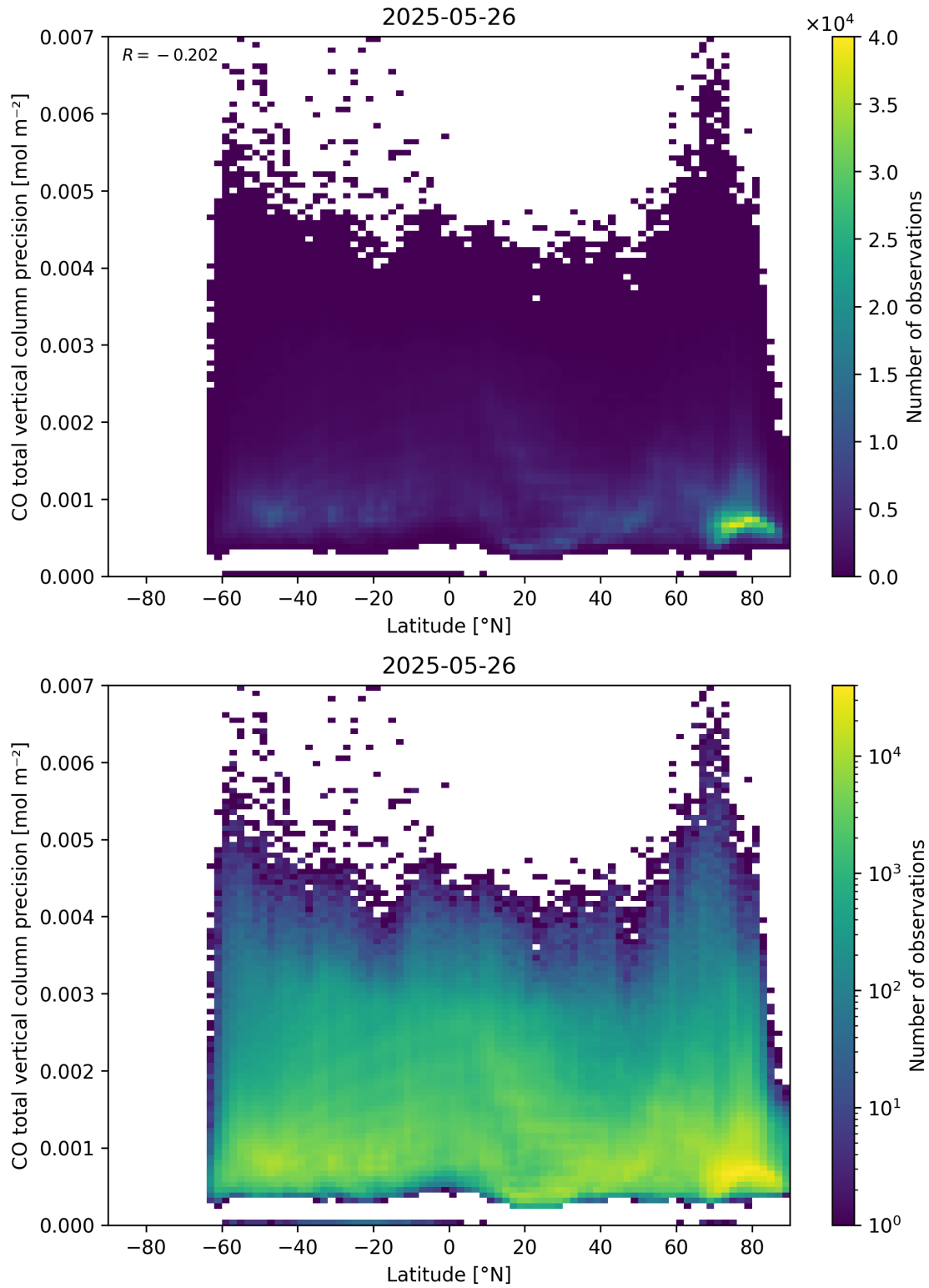
Figure 53: Scatter density plot of “Latitude” against “CO total vertical column precision” for 2025-05-26 to 2025-05-27.
