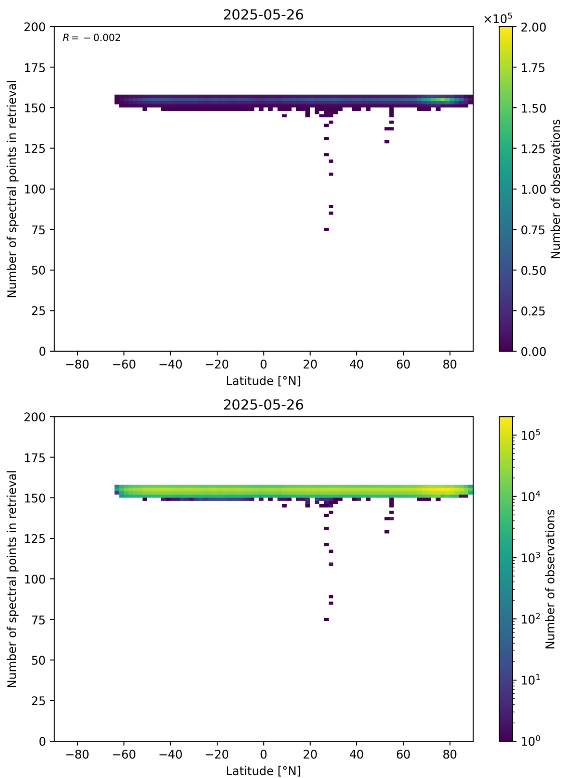
Figure 57: Scatter density plot of “Latitude” against “Number of spectral points in retrieval” for 2025-05-26 to 2025-05-27.
