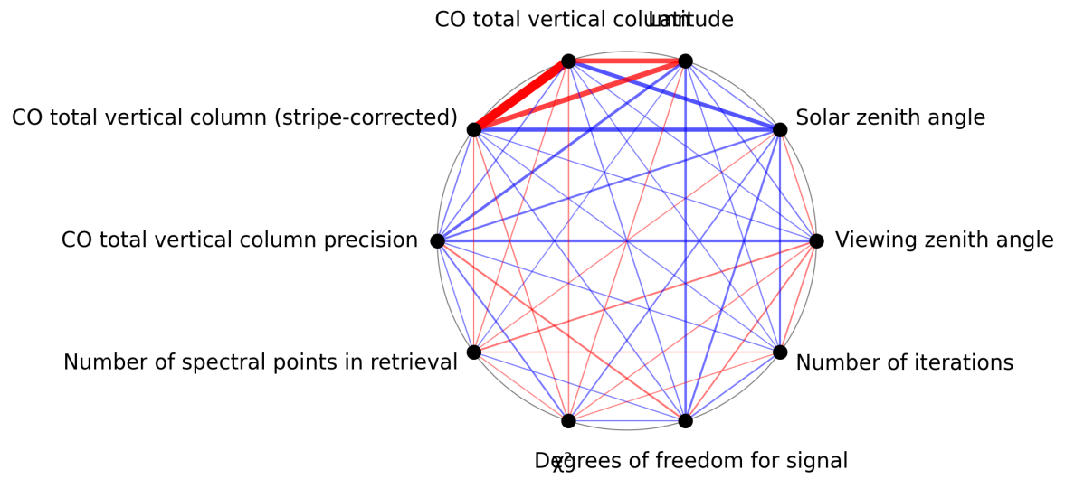
Figure 1: Map of correlation graph for 2025-05-26 to 2025-05-27.
