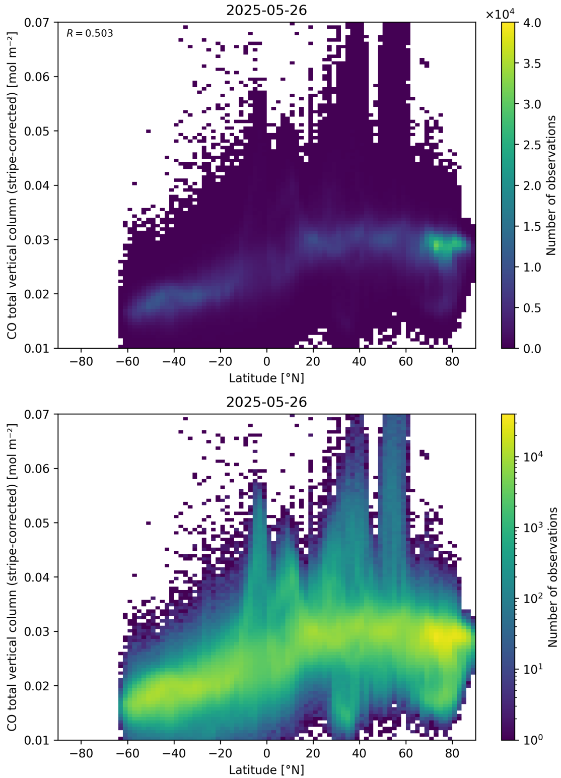
Figure 52: Scatter density plot of “Latitude” against “CO total vertical column (stripe-corrected)” for 2025-05-26 to 2025-05-27.
