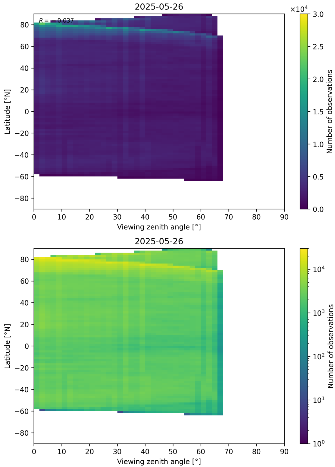
Figure 74: Scatter density plot of “Viewing zenith angle” against “Latitude” for 2025-05-26 to 2025-05-27.
