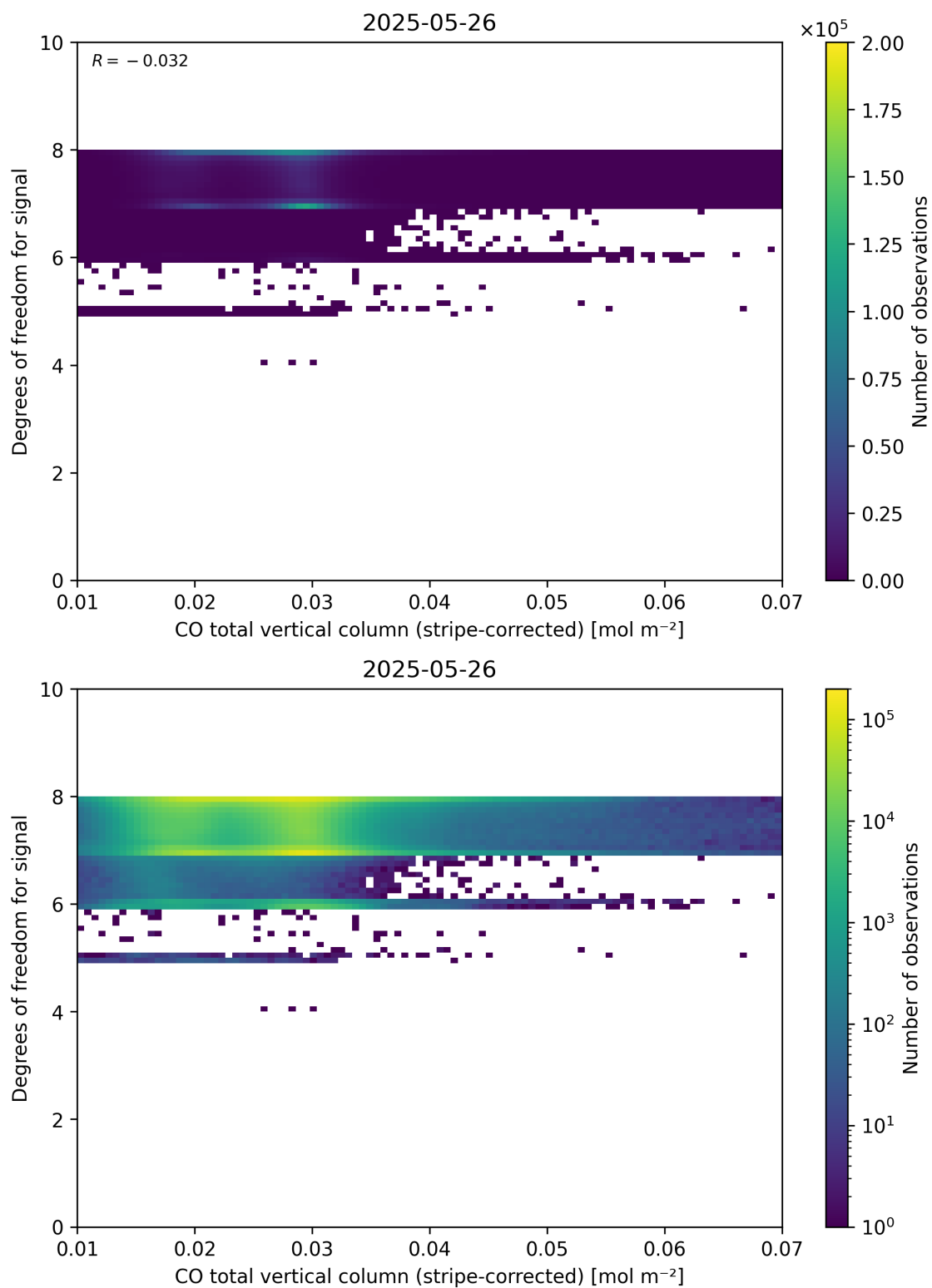
Figure 38: Scatter density plot of “CO total vertical column (stripe-corrected)” against “Degrees of freedom for signal” for 2025-05-26 to 2025-05-27.
