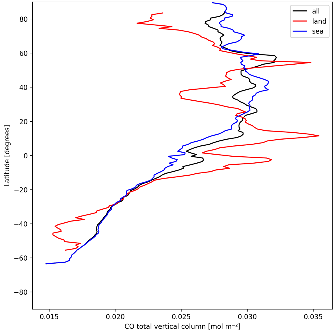
Figure 10: Zonal average of “CO total vertical column” for 2025-05-26 to 2025-05-27.
