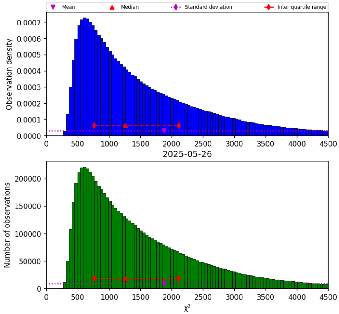
Figure 22: Histogram of “ \chi^2 ” for 2025-05-26 to 2025-05-27
