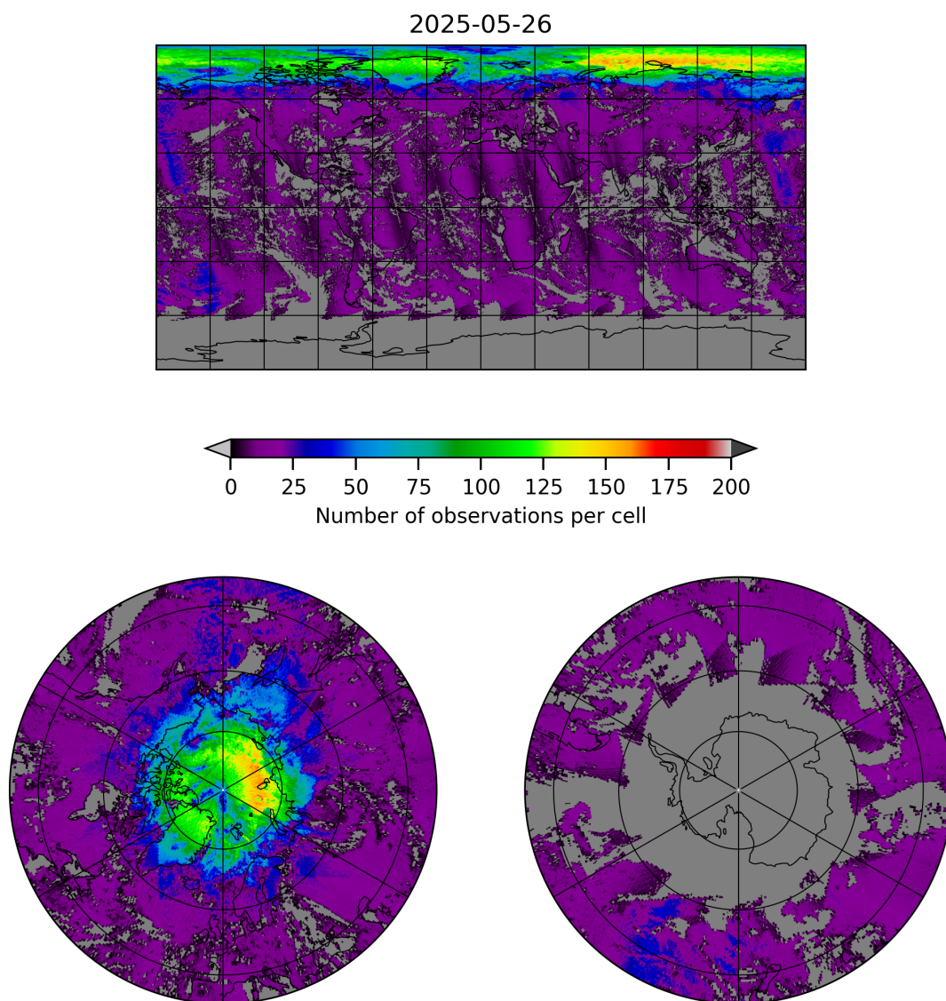
Figure 8: Map of the number of observations for 2025-05-26 to 2025-05-27
