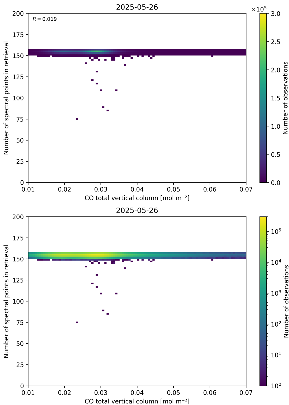
Figure 43: Scatter density plot of “CO total vertical column” against “Number of spectral points in retrieval” for 2025-05-26 to 2025-05-27.
