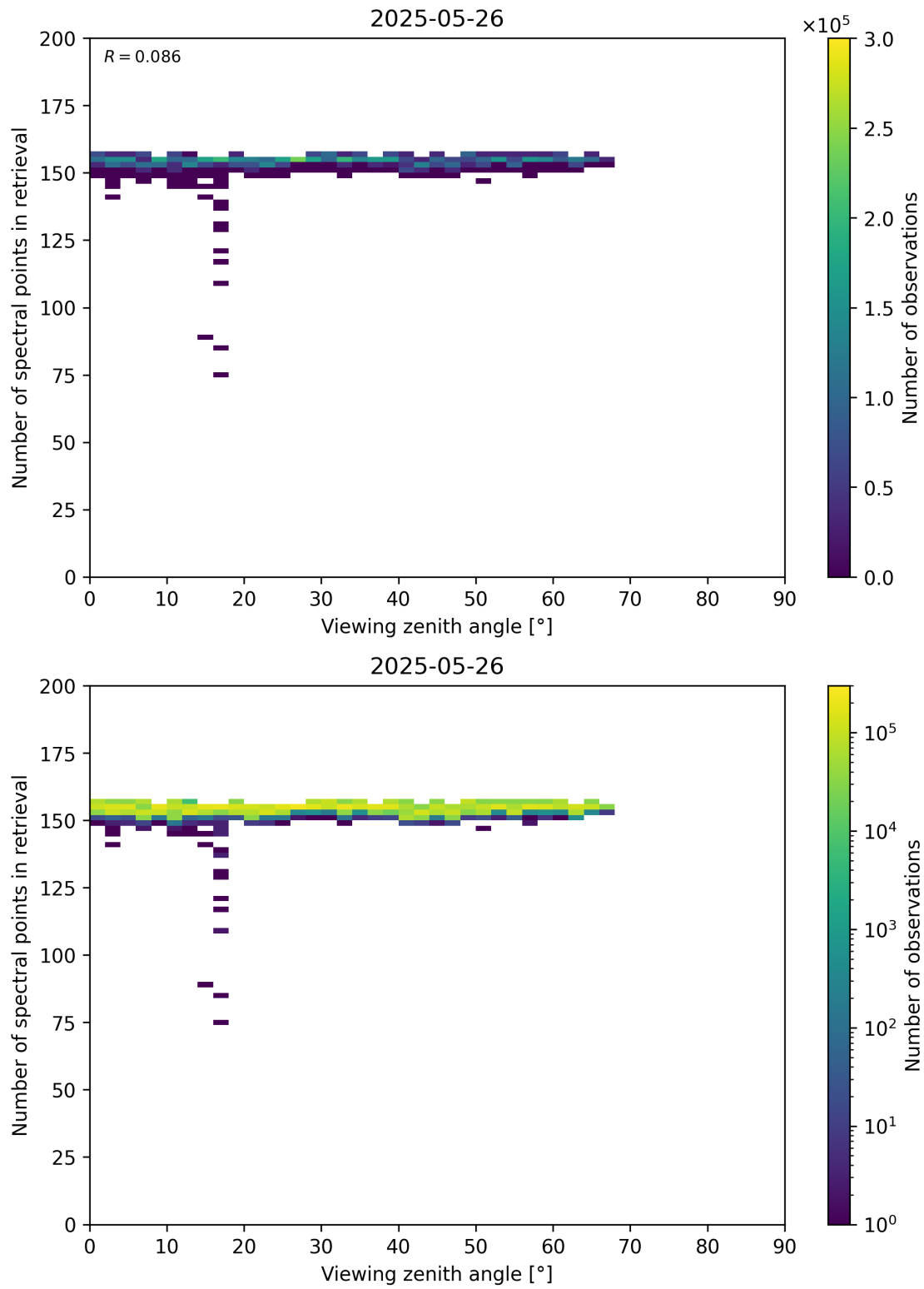
Figure 76: Scatter density plot of “Viewing zenith angle” against “Number of spectral points in retrieval” for 2025-05-26 to 2025-05-27.
