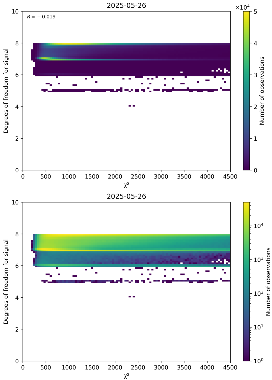
Figure 48: Scatter density plot of “ \chi^2 ” against “Degrees of freedom for signal” for 2025-05-26 to 2025-05-27.
