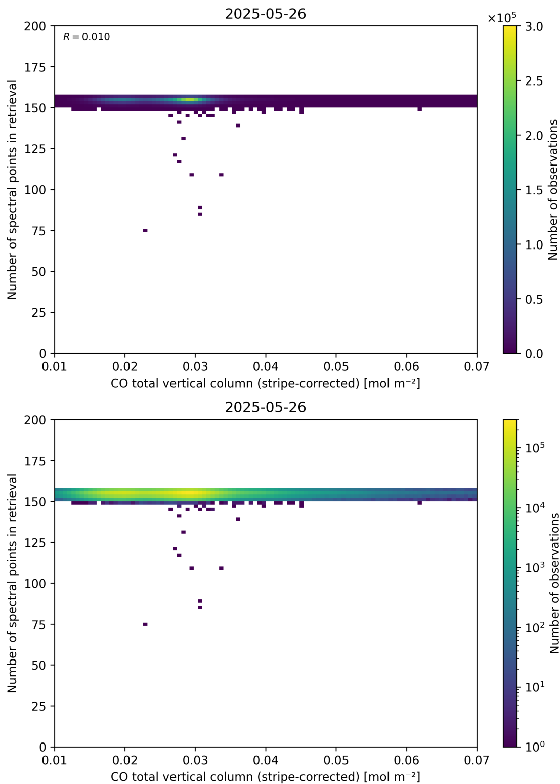
Figure 40: Scatter density plot of “CO total vertical column (stripe-corrected)” against “Number of spectral points in retrieval” for 2025-05-26 to 2025-05-27.
