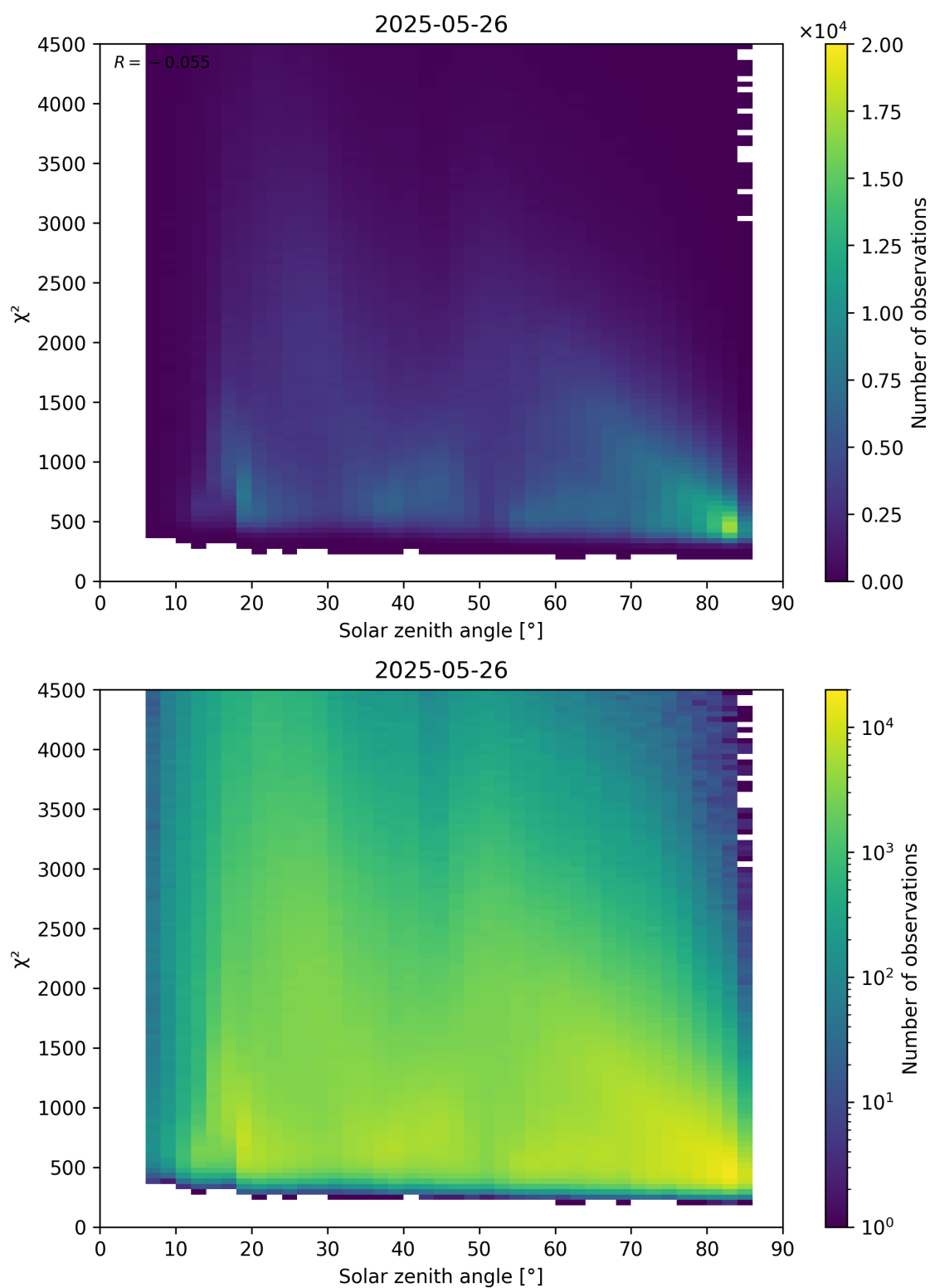
Figure 64: Scatter density plot of “Solar zenith angle” against “ \chi^2 ” for 2025-05-26 to 2025-05-27.
