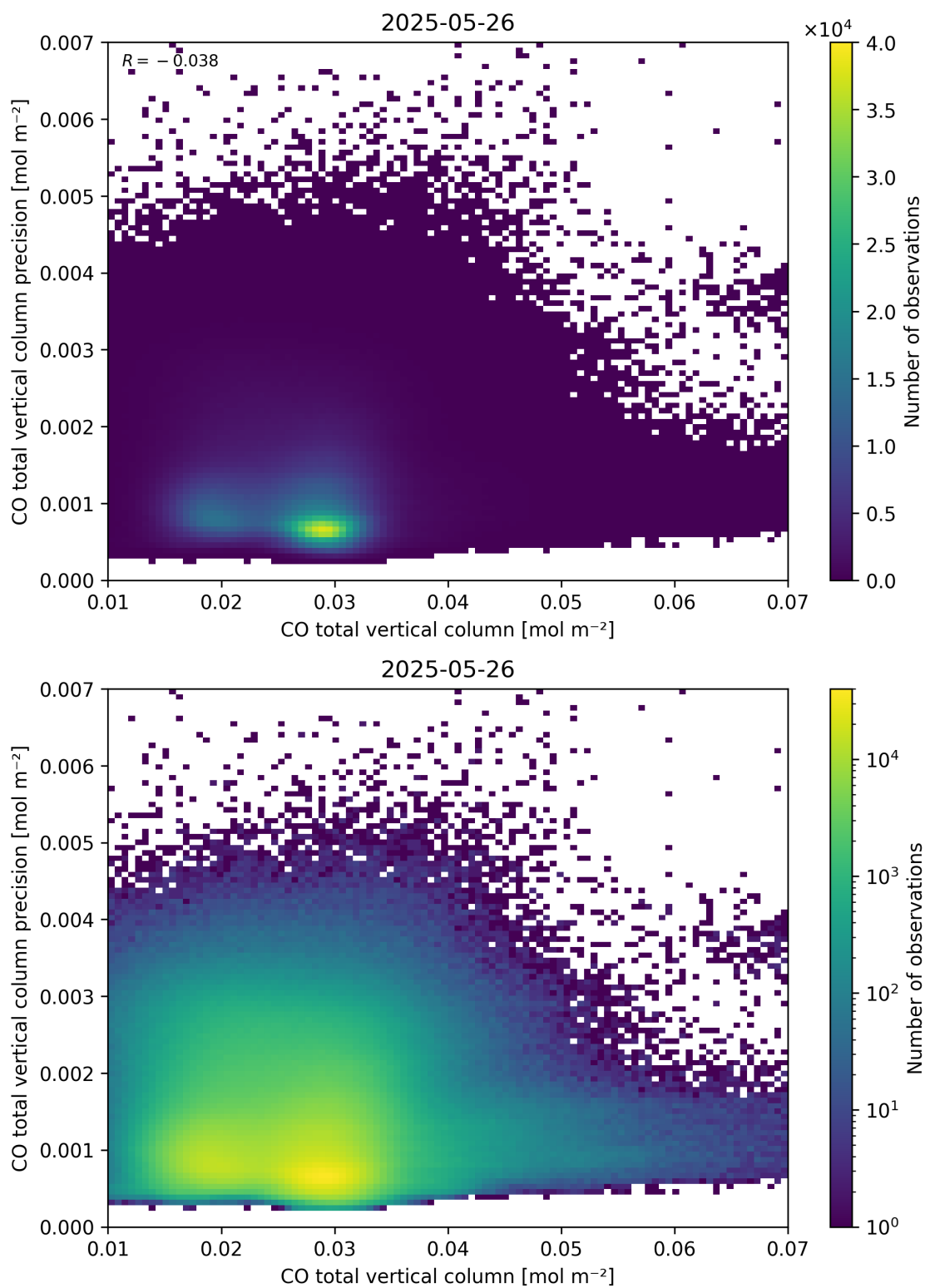
Figure 34: Scatter density plot of “CO total vertical column” against “CO total vertical column precision” for 2025-05-26 to 2025-05-27.
