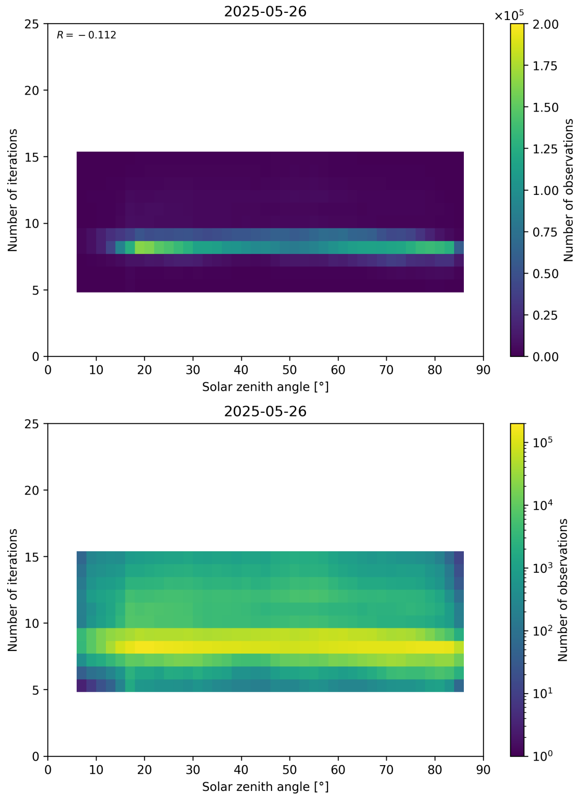
Figure 67: Scatter density plot of “Solar zenith angle” against “Number of iterations” for 2025-05-26 to 2025-05-27.
