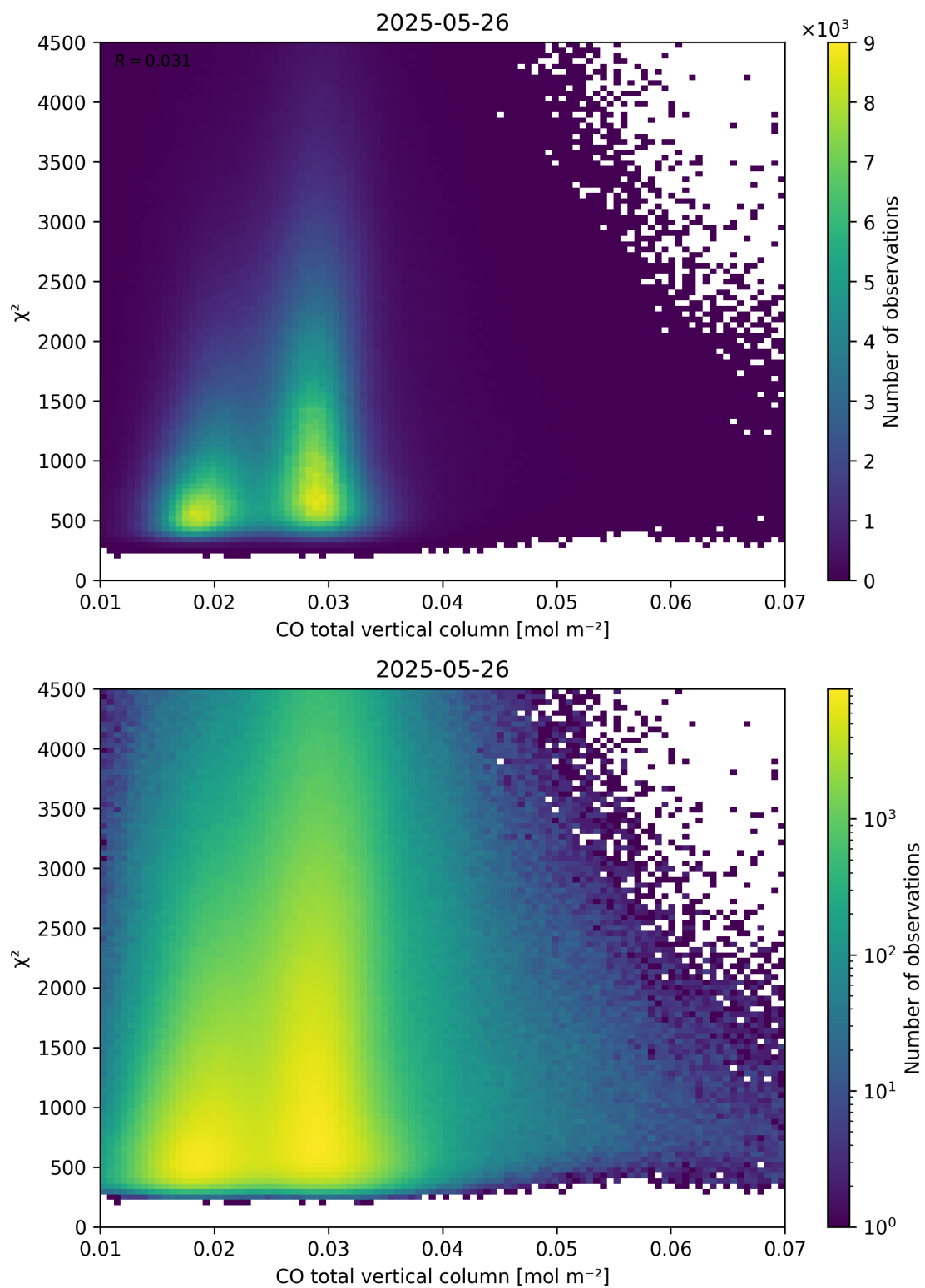
Figure 35: Scatter density plot of “CO total vertical column” against “ \chi^2 ” for 2025-05-26 to 2025-05-27.
