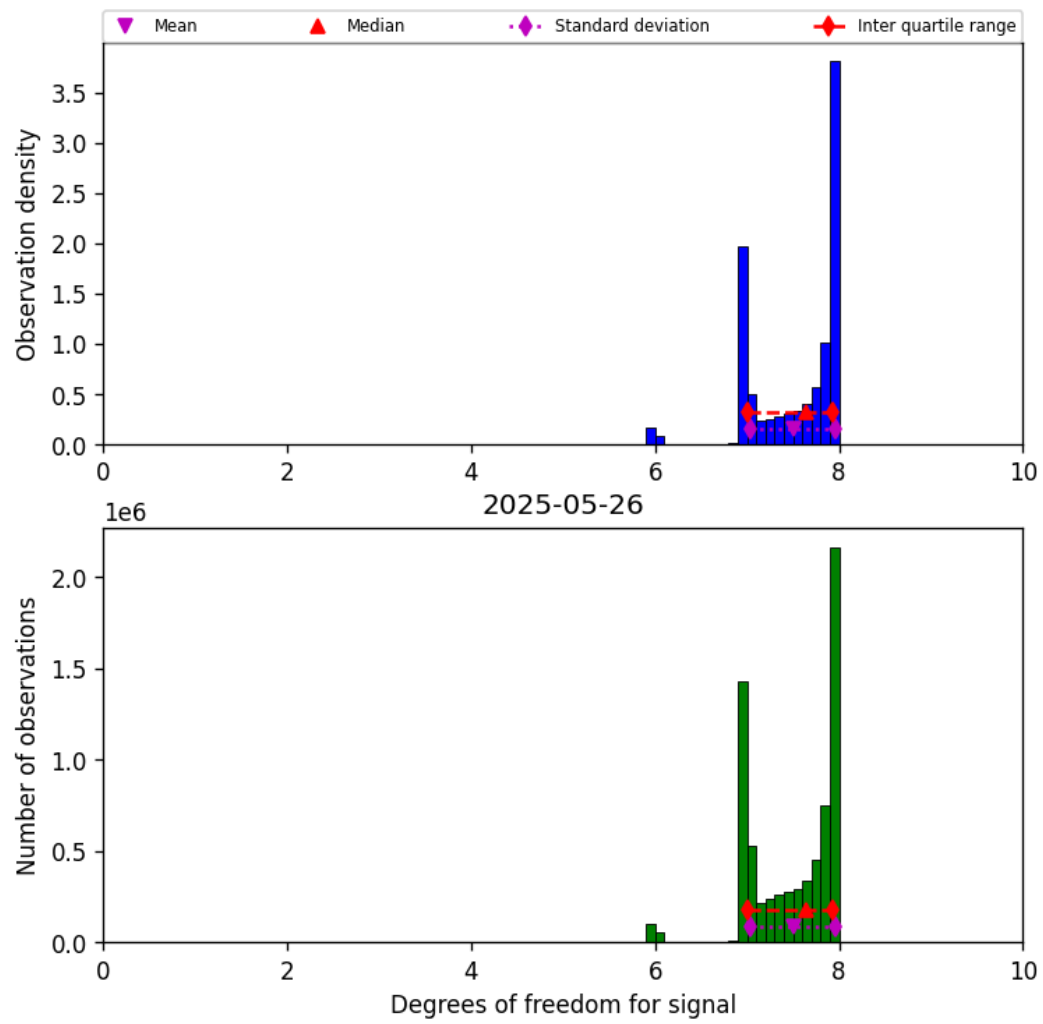
Figure 23: Histogram of “Degrees of freedom for signal” for 2025-05-26 to 2025-05-27
