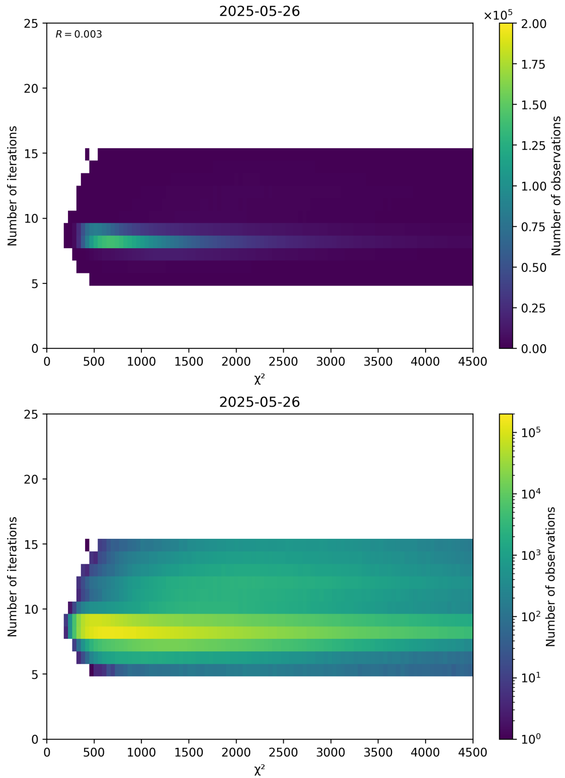
Figure 49: Scatter density plot of “ \chi^2 ” against “Number of iterations” for 2025-05-26 to 2025-05-27.
