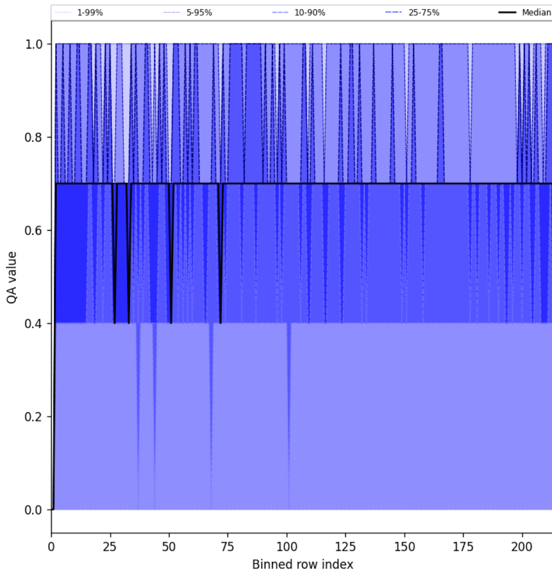
Figure 25: Along track statistics of “QA value” for 2025-05-26 to 2025-05-27
