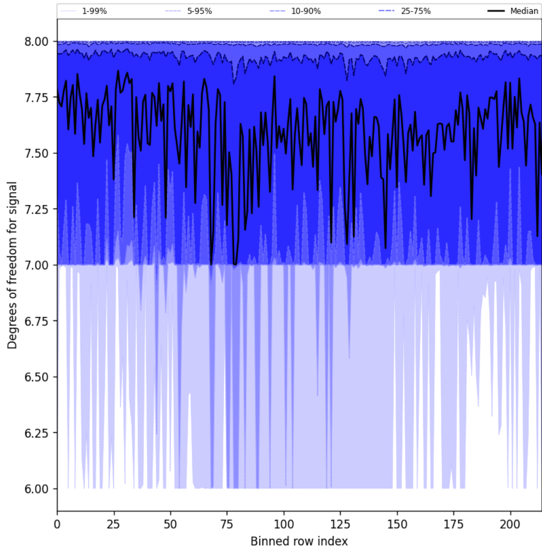
Figure 31: Along track statistics of “Degrees of freedom for signal” for 2025-05-26 to 2025-05-27
