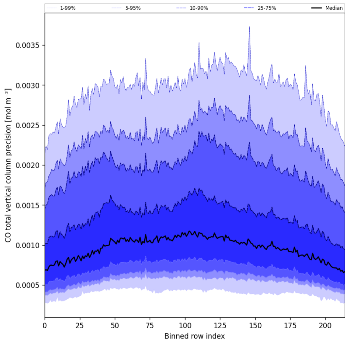
Figure 28: Along track statistics of “CO total vertical column precision” for 2025-05-26 to 2025-05-27
