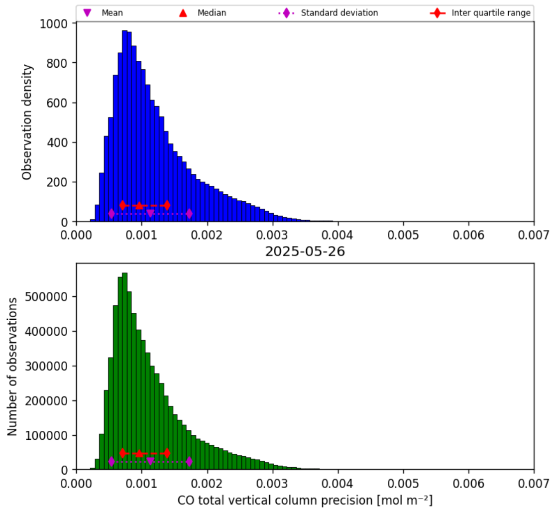
Figure 20: Histogram of “CO total vertical column precision” for 2025-05-26 to 2025-05-27
