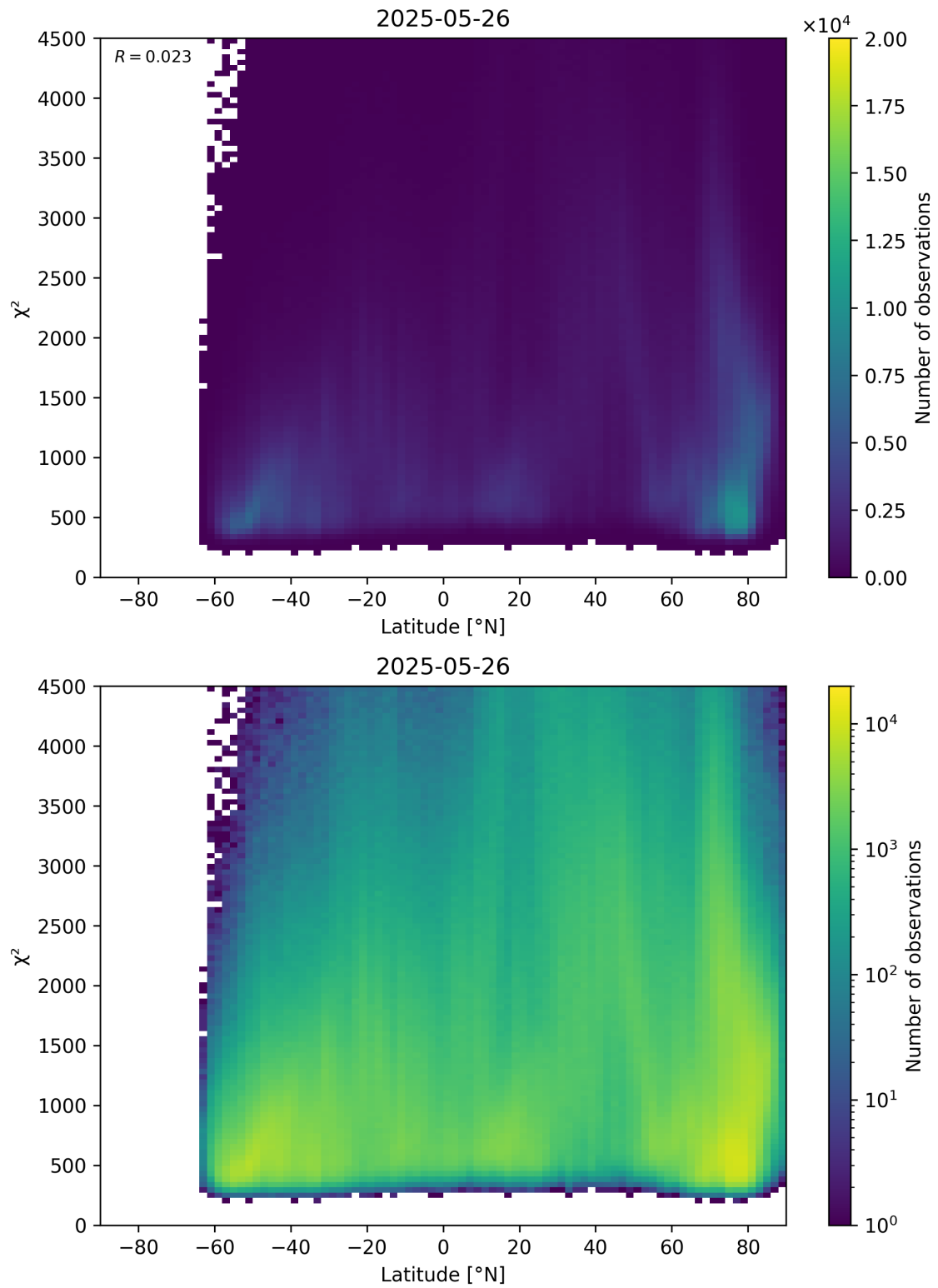
Figure 54: Scatter density plot of “Latitude” against “ \chi^2 ” for 2025-05-26 to 2025-05-27.
