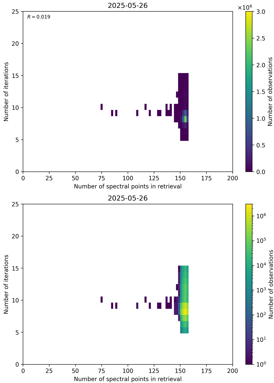
Figure 60: Scatter density plot of “Number of spectral points in retrieval” against “Number of iterations” for 2025-05-26 to 2025-05-27.
