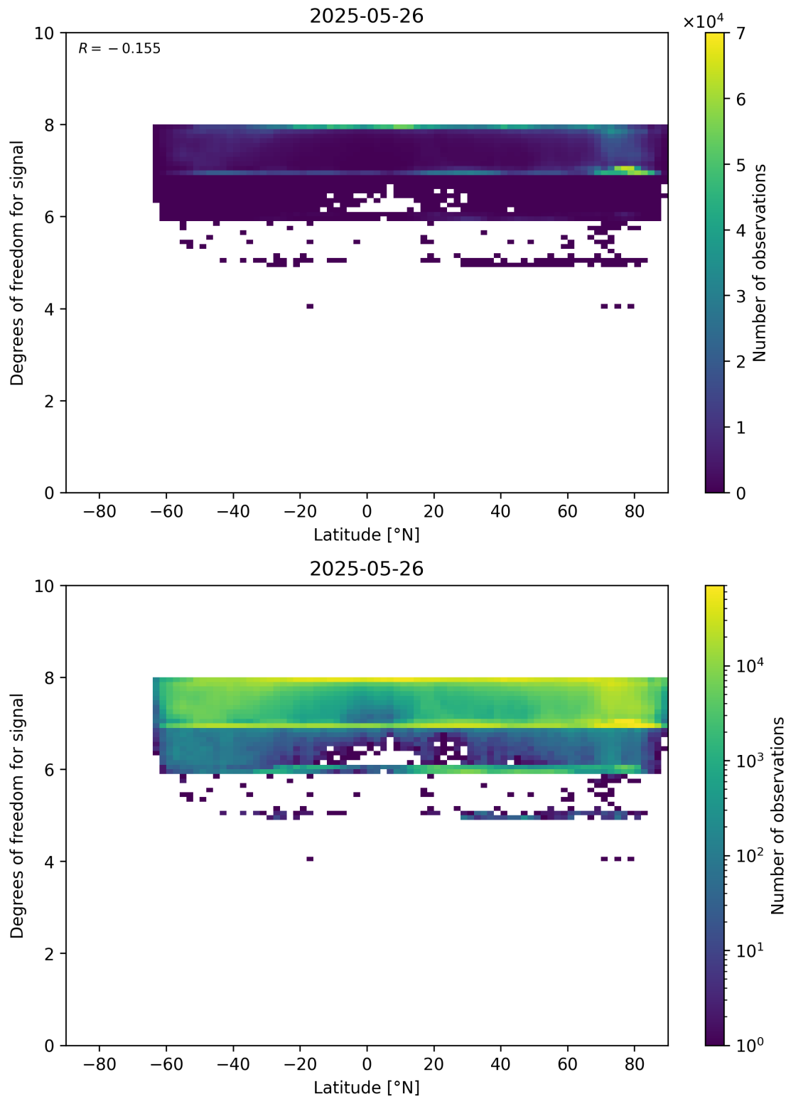
Figure 55: Scatter density plot of “Latitude” against “Degrees of freedom for signal” for 2025-05-26 to 2025-05-27.
