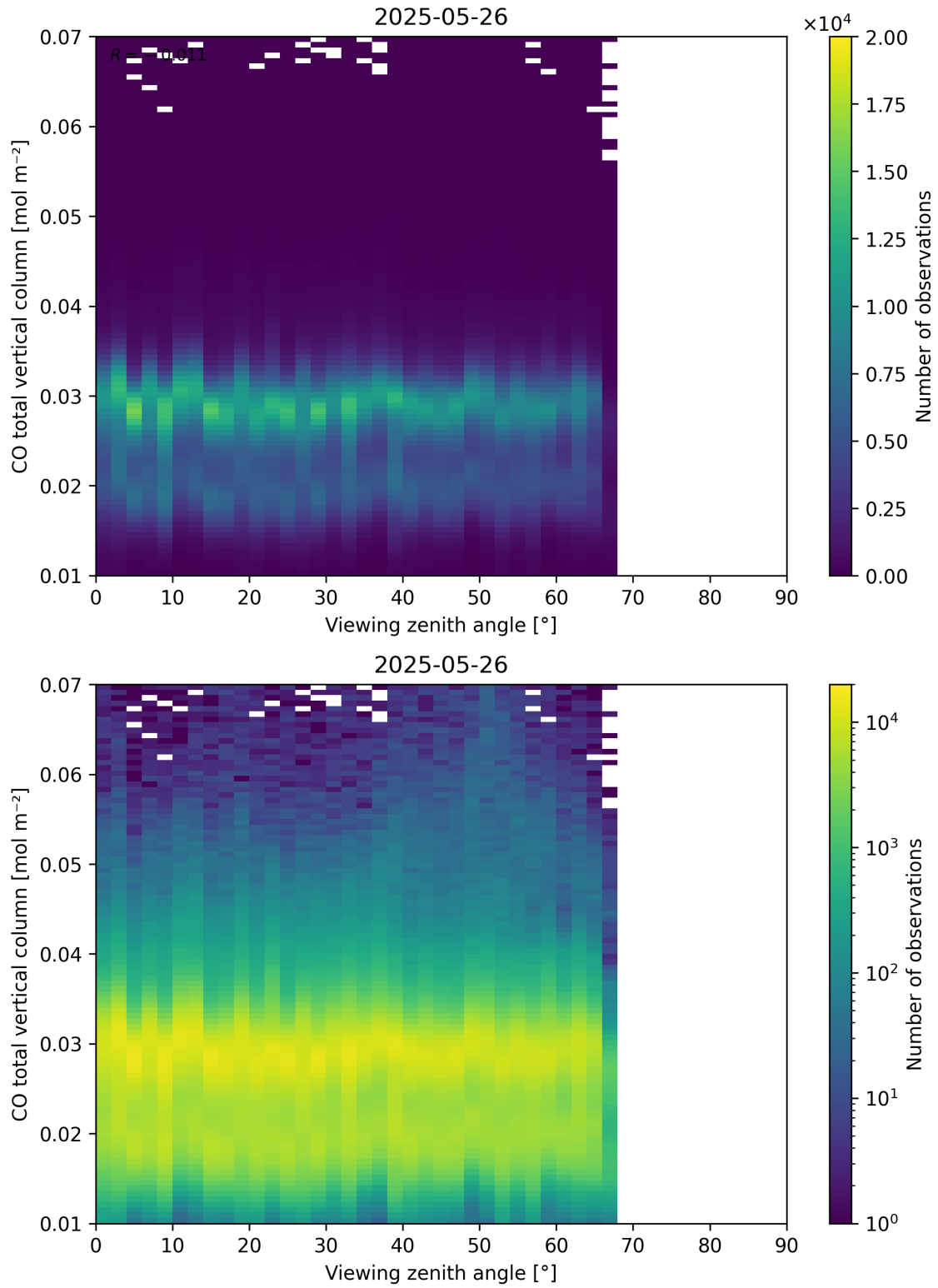
Figure 69: Scatter density plot of “Viewing zenith angle” against “CO total vertical column” for 2025-05-26 to 2025-05-27.
