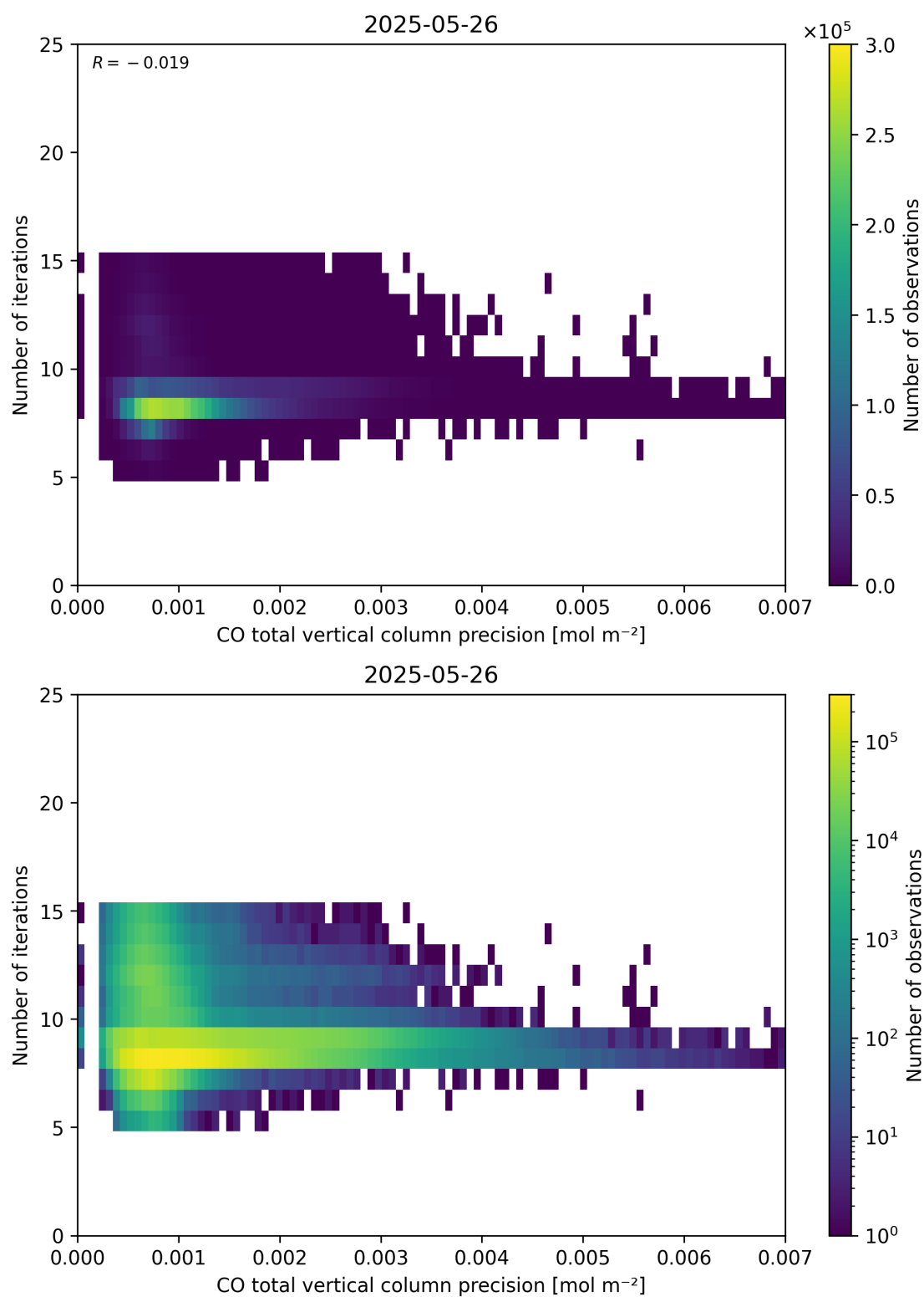
Figure 46: Scatter density plot of “CO total vertical column precision” against “Number of iterations” for 2025-05-26 to 2025-05-27.
