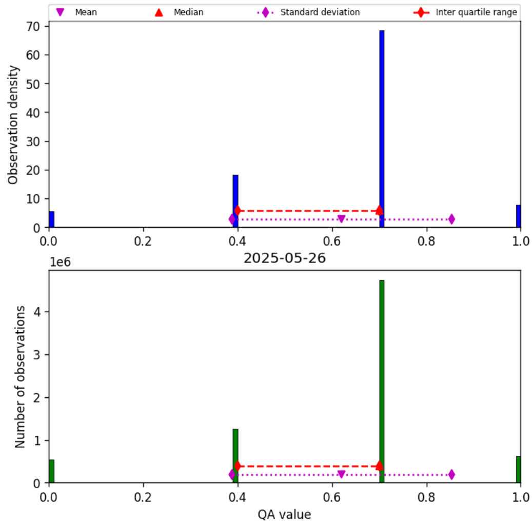
Figure 17: Histogram of “QA value” for 2025-05-26 to 2025-05-27
