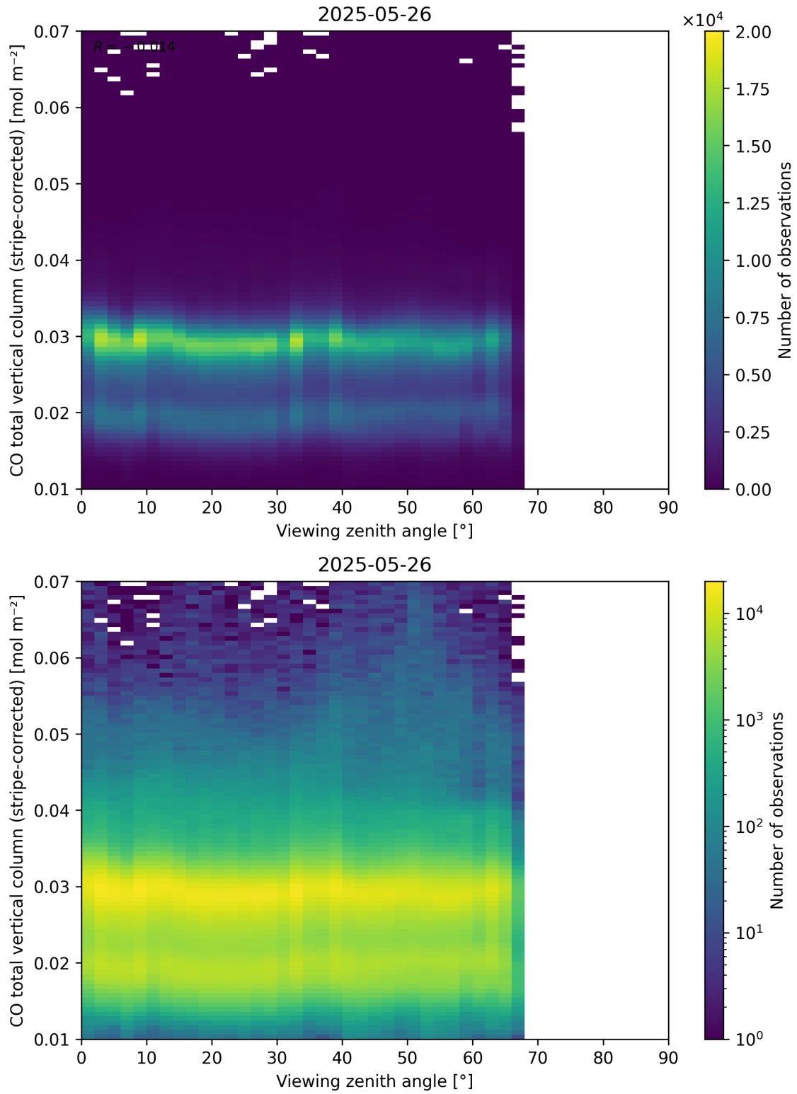
Figure 70: Scatter density plot of “Viewing zenith angle” against “CO total vertical column (stripe-corrected)” for 2025-05-26 to 2025-05-27.
