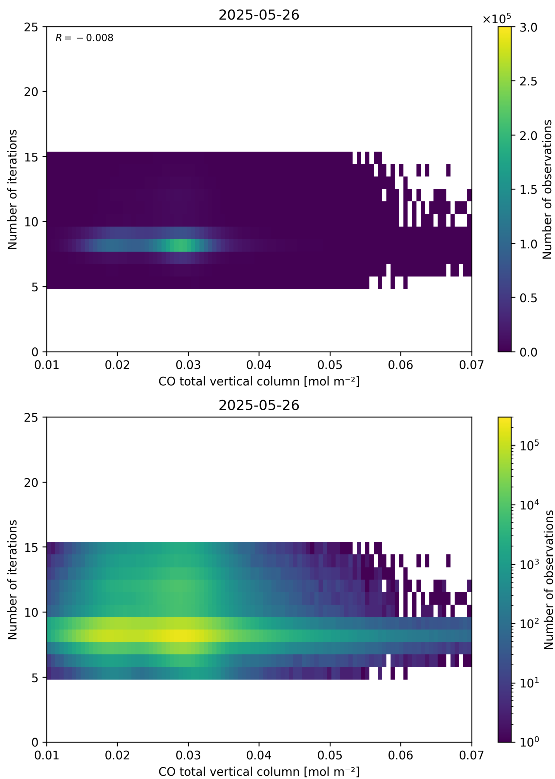
Figure 42: Scatter density plot of “CO total vertical column” against “Number of iterations” for 2025-05-26 to 2025-05-27.
