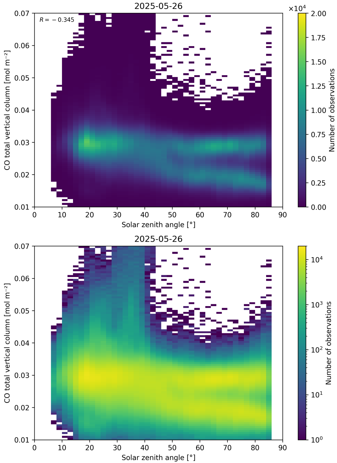
Figure 61: Scatter density plot of “Solar zenith angle” against “CO total vertical column” for 2025-05-26 to 2025-05-27.
