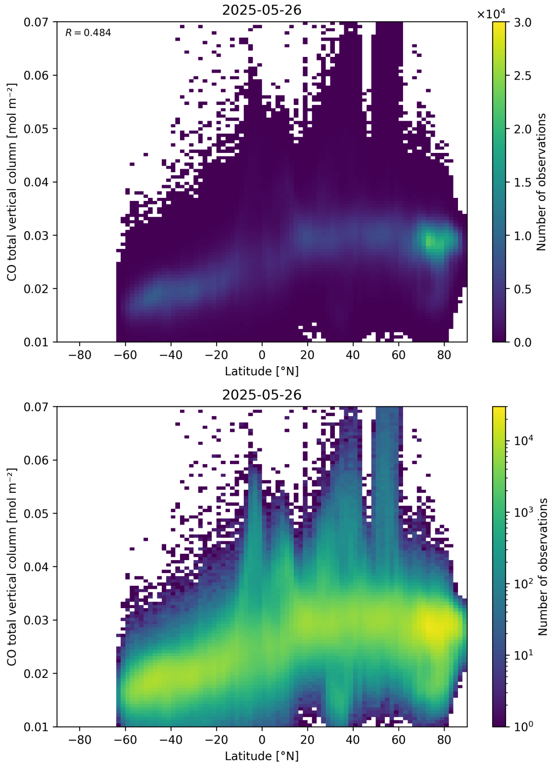
Figure 51: Scatter density plot of “Latitude” against “CO total vertical column” for 2025-05-26 to 2025-05-27.
