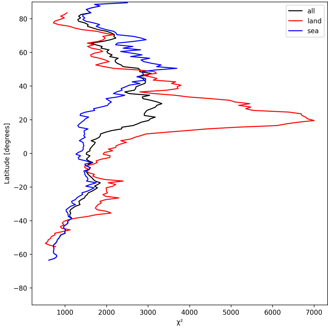
Figure 14: Zonal average of “ \chi^2 ” for 2025-05-26 to 2025-05-27.
