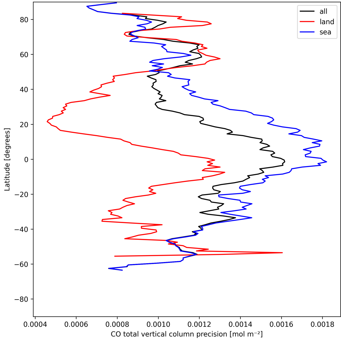
Figure 12: Zonal average of “CO total vertical column precision” for 2025-05-26 to 2025-05-27.
