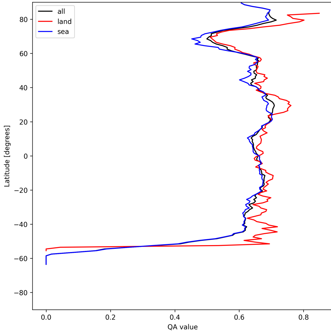
Figure 9: Zonal average of “QA value” for 2025-05-26 to 2025-05-27.
