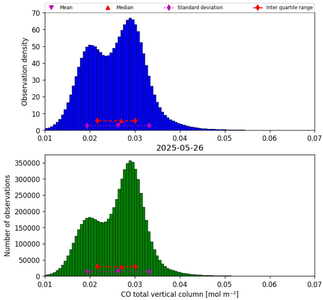
Figure 18: Histogram of “CO total vertical column” for 2025-05-26 to 2025-05-27
