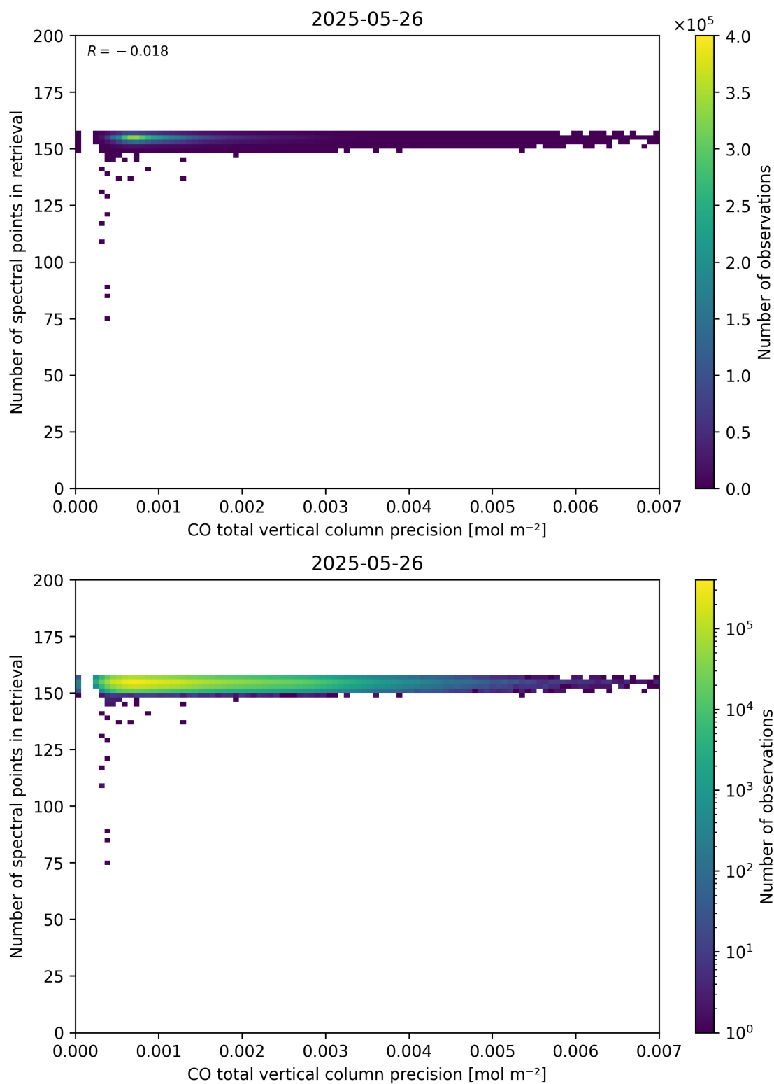
Figure 47: Scatter density plot of “CO total vertical column precision” against “Number of spectral points in retrieval” for 2025-05-26 to 2025-05-27.
