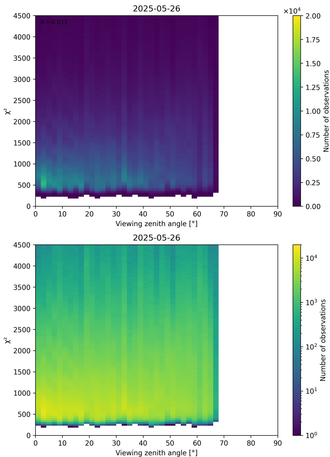
Figure 72: Scatter density plot of “Viewing zenith angle” against “ \chi^2 ” for 2025-05-26 to 2025-05-27.
