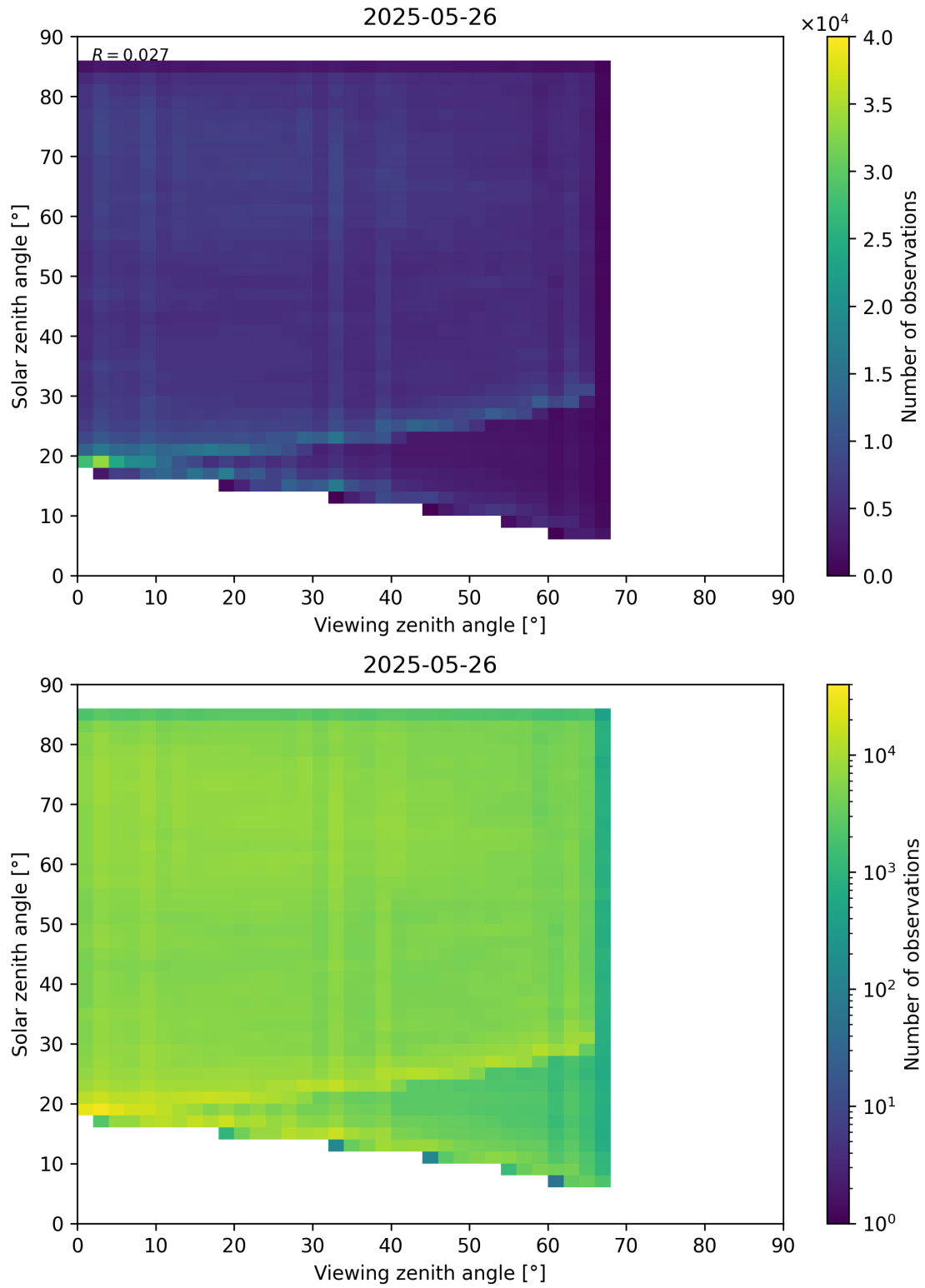
Figure 77: Scatter density plot of “Viewing zenith angle” against “Solar zenith angle” for 2025-05-26 to 2025-05-27.
