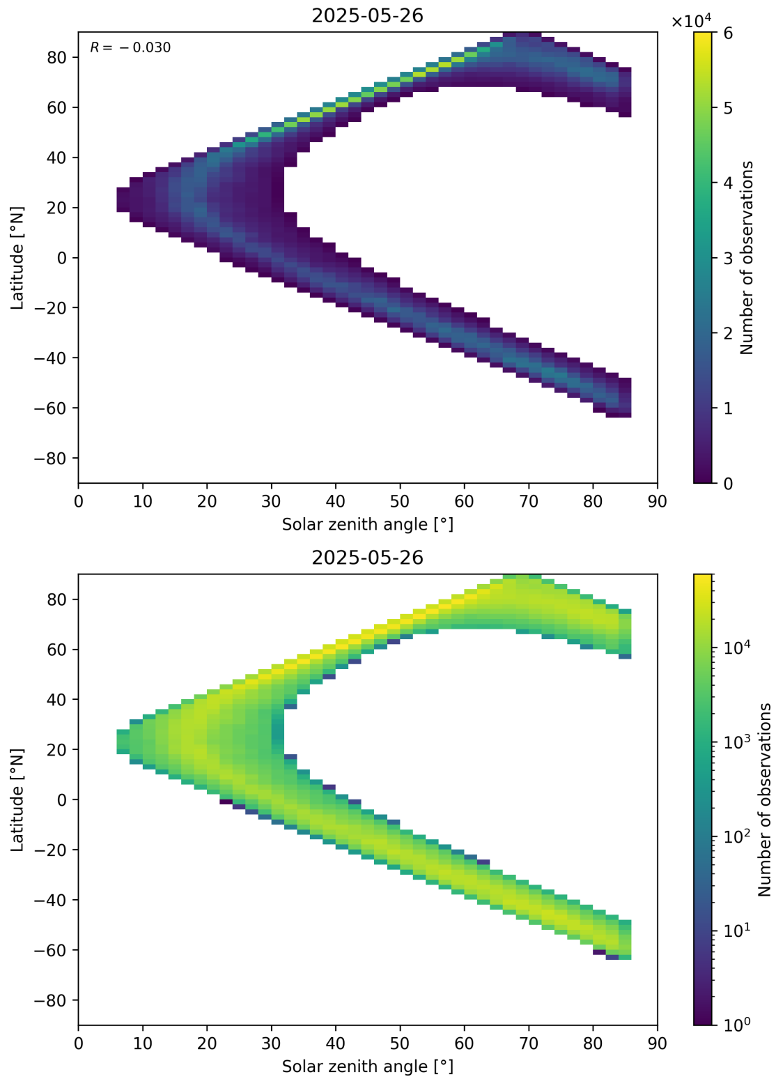
Figure 66: Scatter density plot of “Solar zenith angle” against “Latitude” for 2025-05-26 to 2025-05-27.
