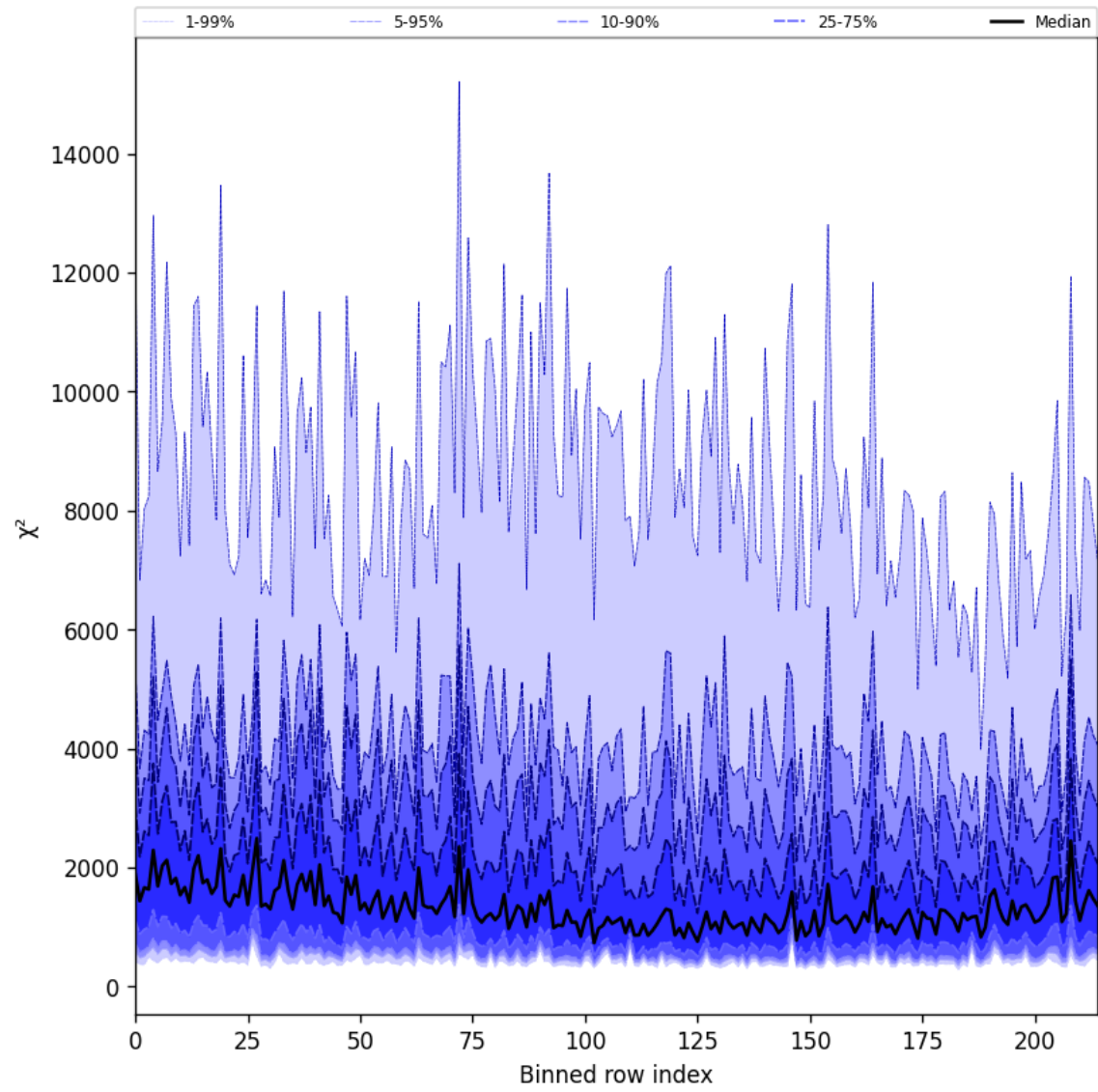
Figure 30: Along track statistics of “ \chi^2 ” for 2025-05-26 to 2025-05-27
