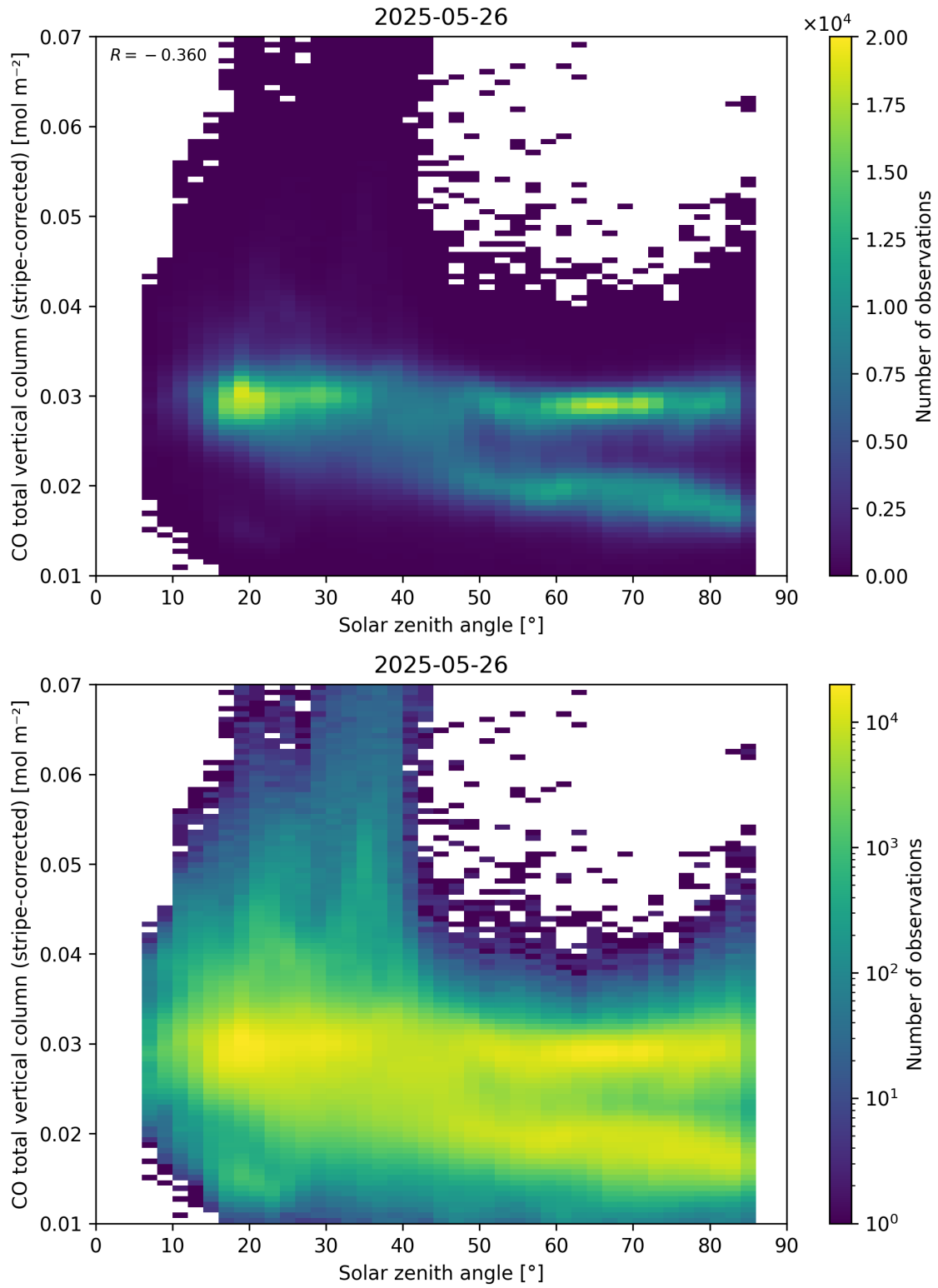
Figure 62: Scatter density plot of “Solar zenith angle” against “CO total vertical column (stripe-corrected)” for 2025-05-26 to 2025-05-27.
