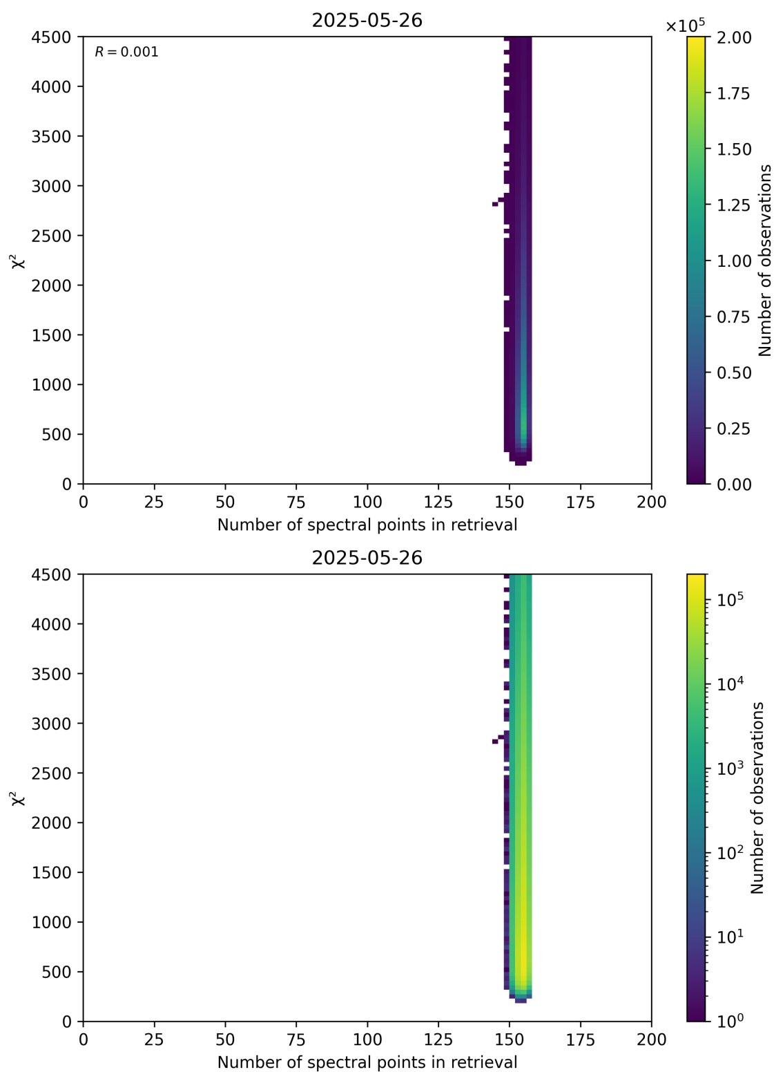
Figure 58: Scatter density plot of “Number of spectral points in retrieval” against “ \chi^2 ” for 2025-05-26 to 2025-05-27.
