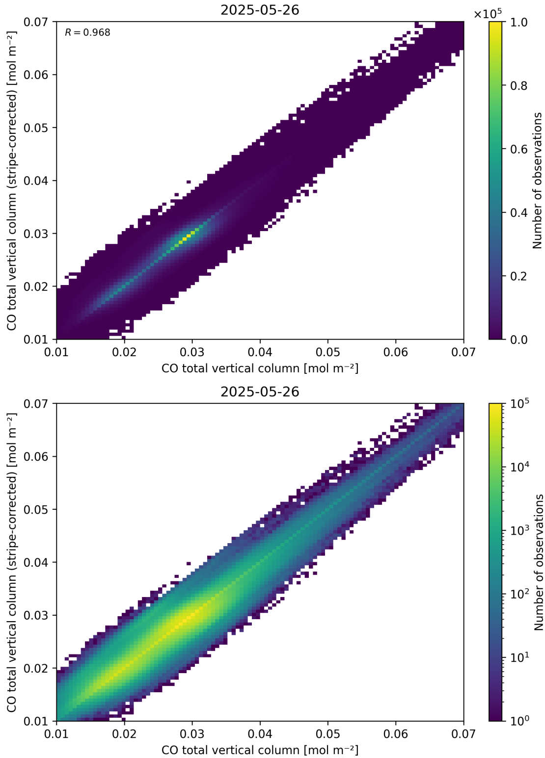
Figure 33: Scatter density plot of “CO total vertical column” against “CO total vertical column (stripe-corrected)” for 2025-05-26 to 2025-05-27.
