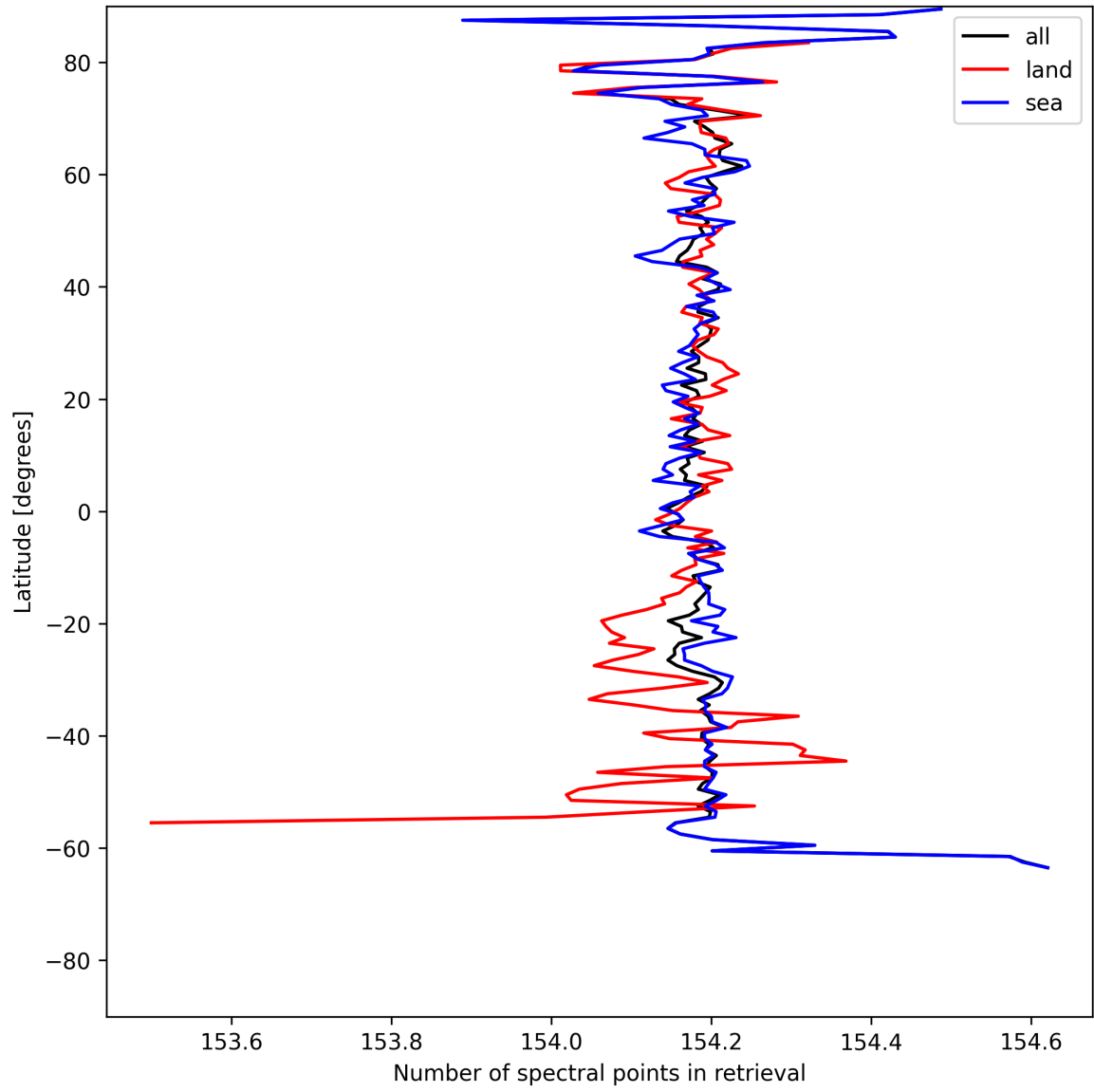
Figure 13: Zonal average of “Number of spectral points in retrieval” for 2025-05-26 to 2025-05-27.
