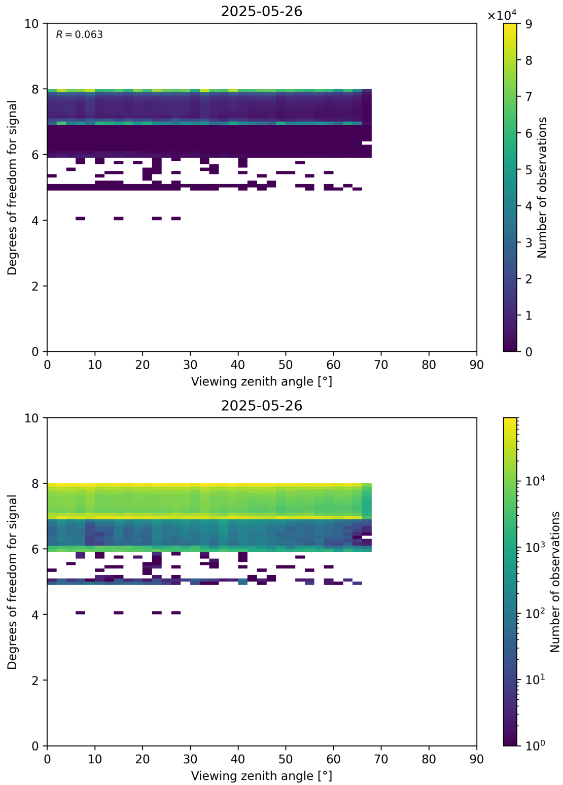
Figure 73: Scatter density plot of “Viewing zenith angle” against “Degrees of freedom for signal” for 2025-05-26 to 2025-05-27.
