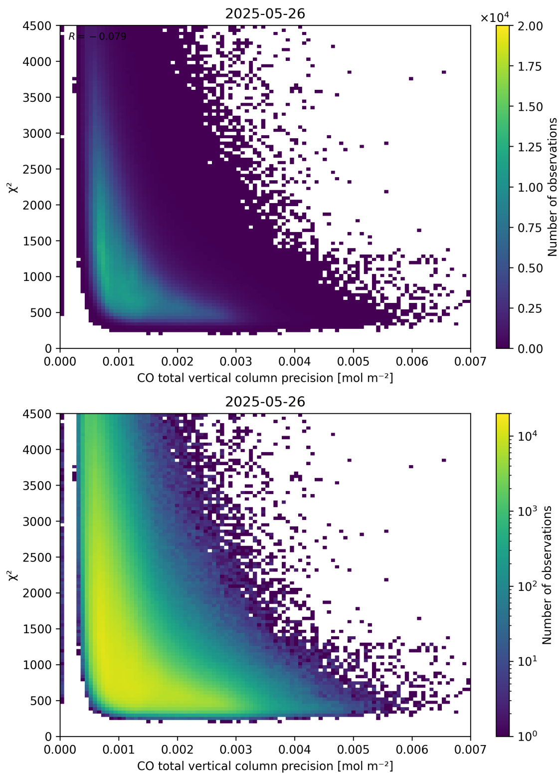
Figure 44: Scatter density plot of “CO total vertical column precision” against “ \chi^2 ” for 2025-05-26 to 2025-05-27.
