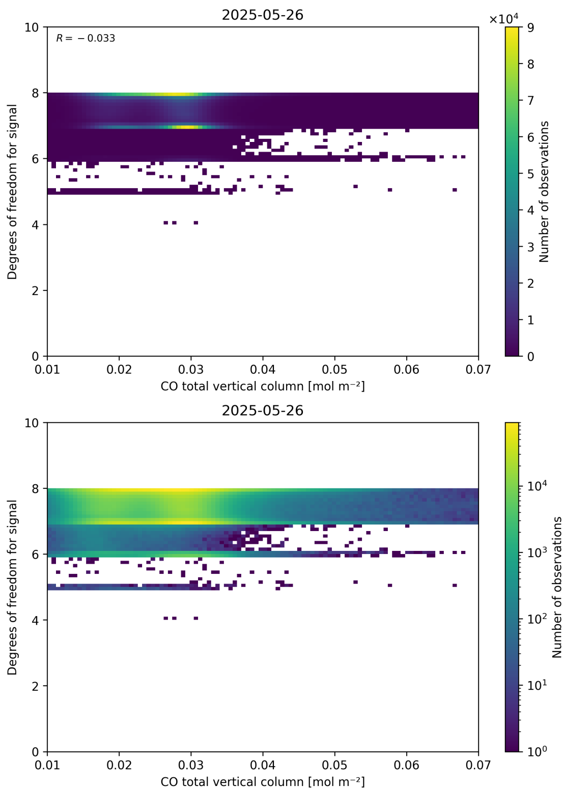
Figure 41: Scatter density plot of “CO total vertical column” against “Degrees of freedom for signal” for 2025-05-26 to 2025-05-27.
