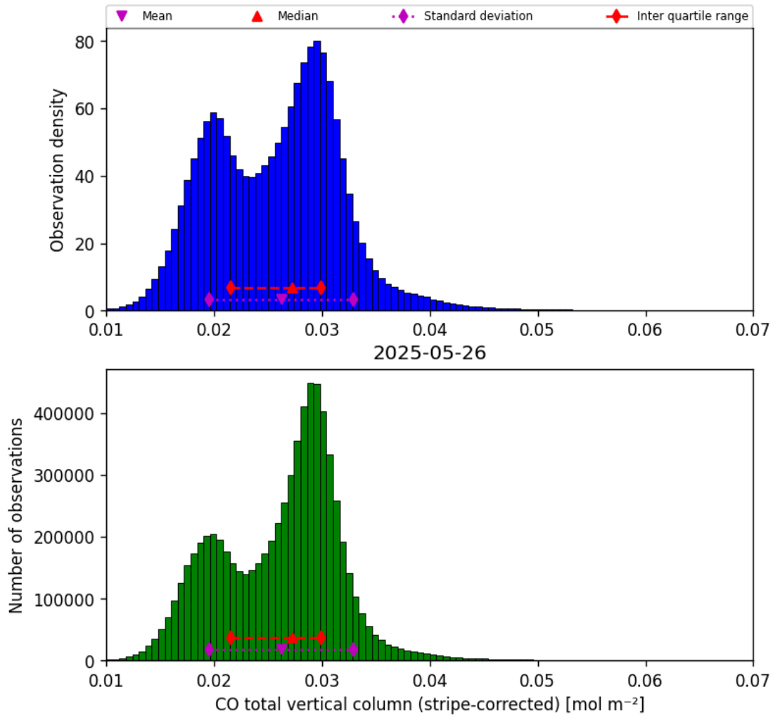
Figure 19: Histogram of “CO total vertical column (stripe-corrected)” for 2025-05-26 to 2025-05-27
