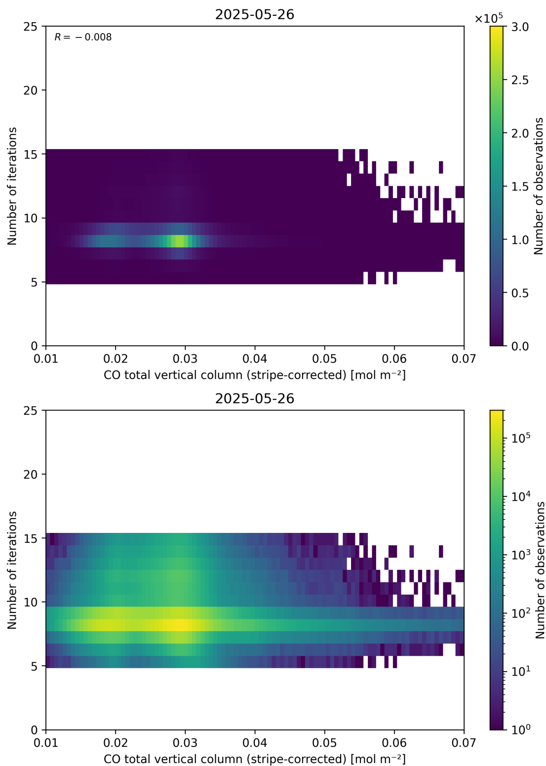
Figure 39: Scatter density plot of “CO total vertical column (stripe-corrected)” against “Number of iterations” for 2025-05-26 to 2025-05-27.
