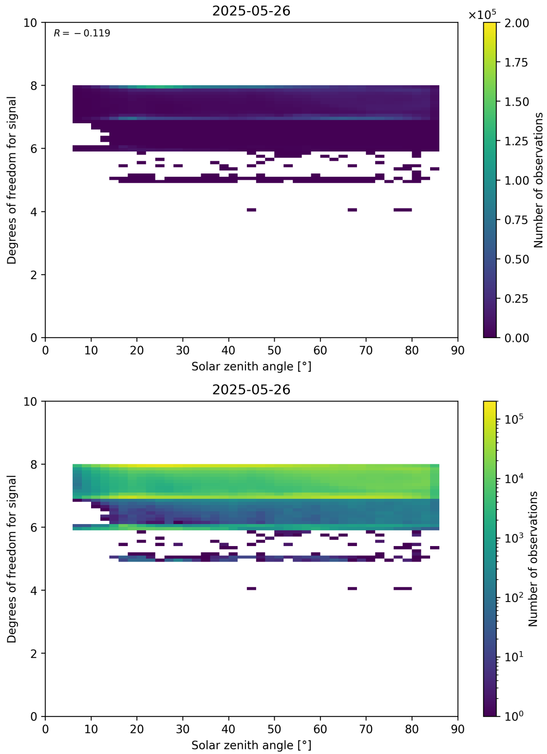
Figure 65: Scatter density plot of “Solar zenith angle” against “Degrees of freedom for signal” for 2025-05-26 to 2025-05-27.
