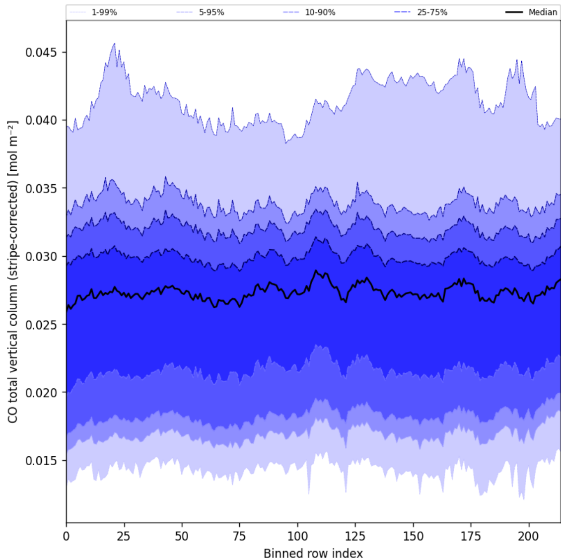
Figure 27: Along track statistics of “CO total vertical column (stripe-corrected)” for 2025-05-26 to 2025-05-27
