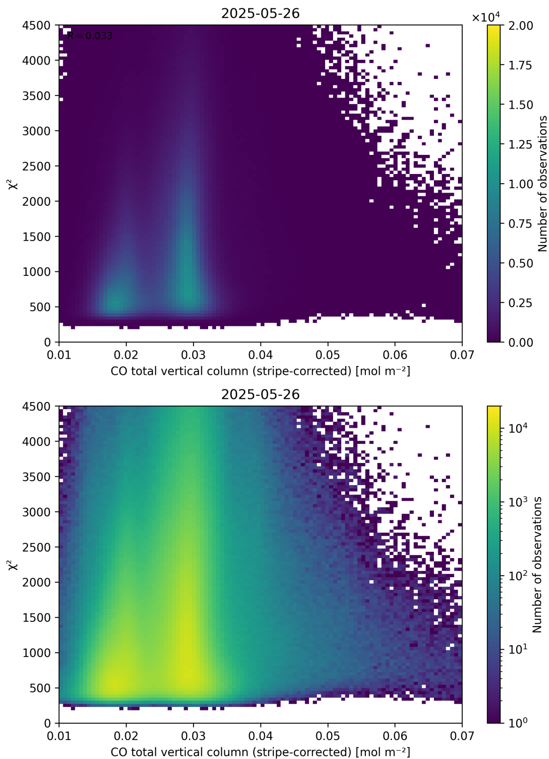
Figure 37: Scatter density plot of “CO total vertical column (stripe-corrected)” against “ \chi^2 ” for 2025-05-26 to 2025-05-27.
