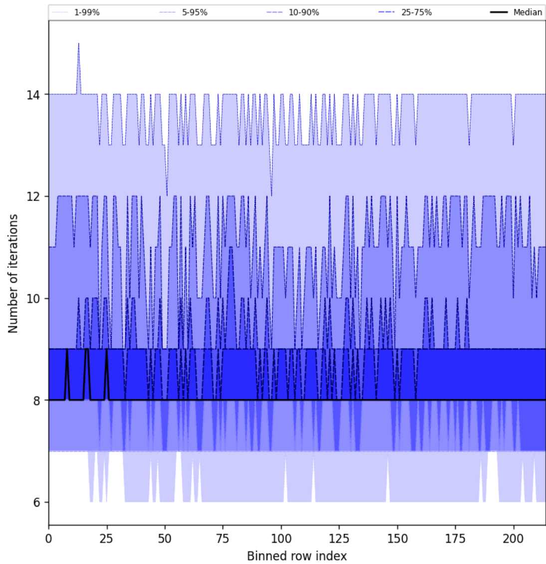
Figure 32: Along track statistics of “Number of iterations” for 2025-05-26 to 2025-05-27
