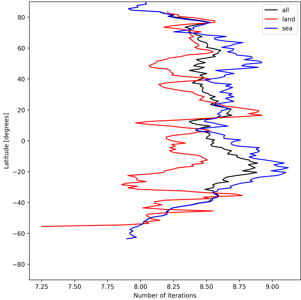
Figure 16: Zonal average of “Number of iterations” for 2025-05-26 to 2025-05-27.
