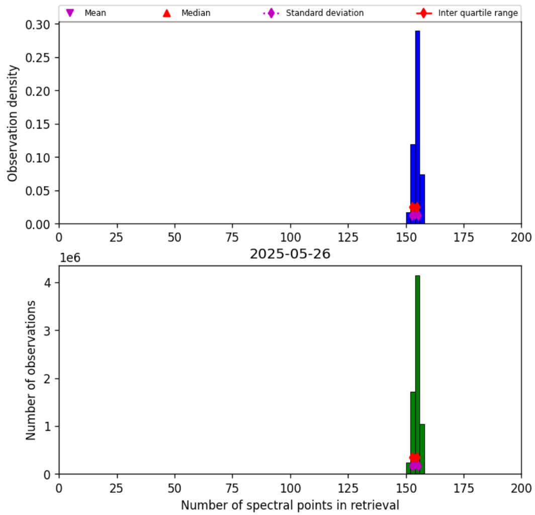
Figure 21: Histogram of “Number of spectral points in retrieval” for 2025-05-26 to 2025-05-27
