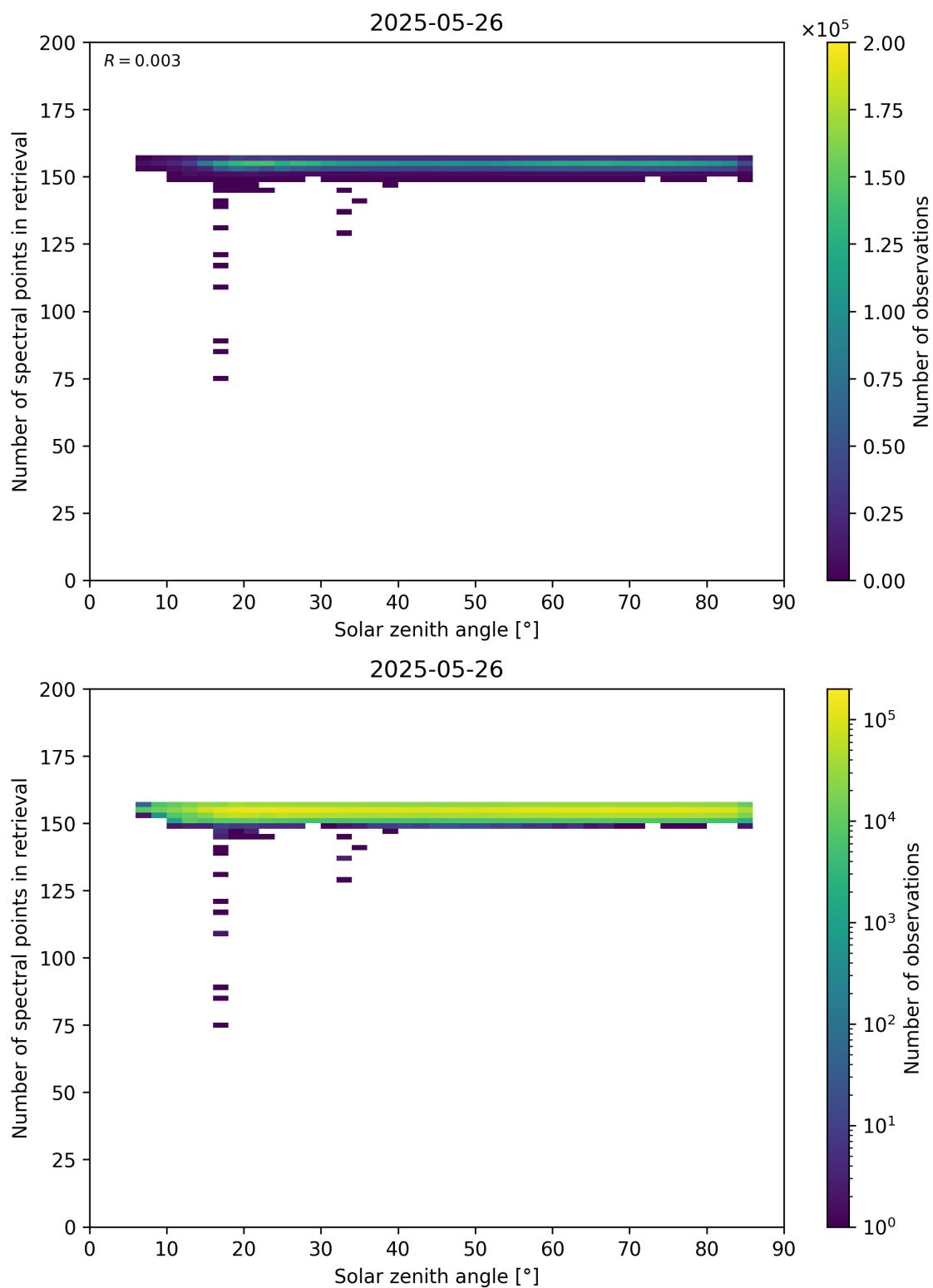
Figure 68: Scatter density plot of “Solar zenith angle” against “Number of spectral points in retrieval” for 2025-05-26 to 2025-05-27.
