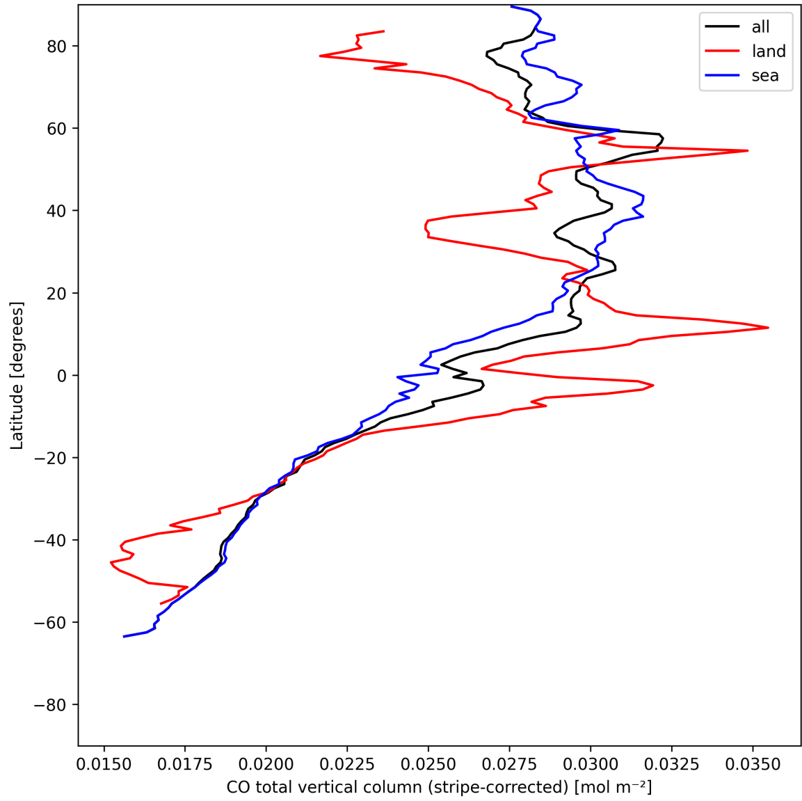
Figure 11: Zonal average of “CO total vertical column (stripe-corrected)” for 2025-05-26 to 2025-05-27.
