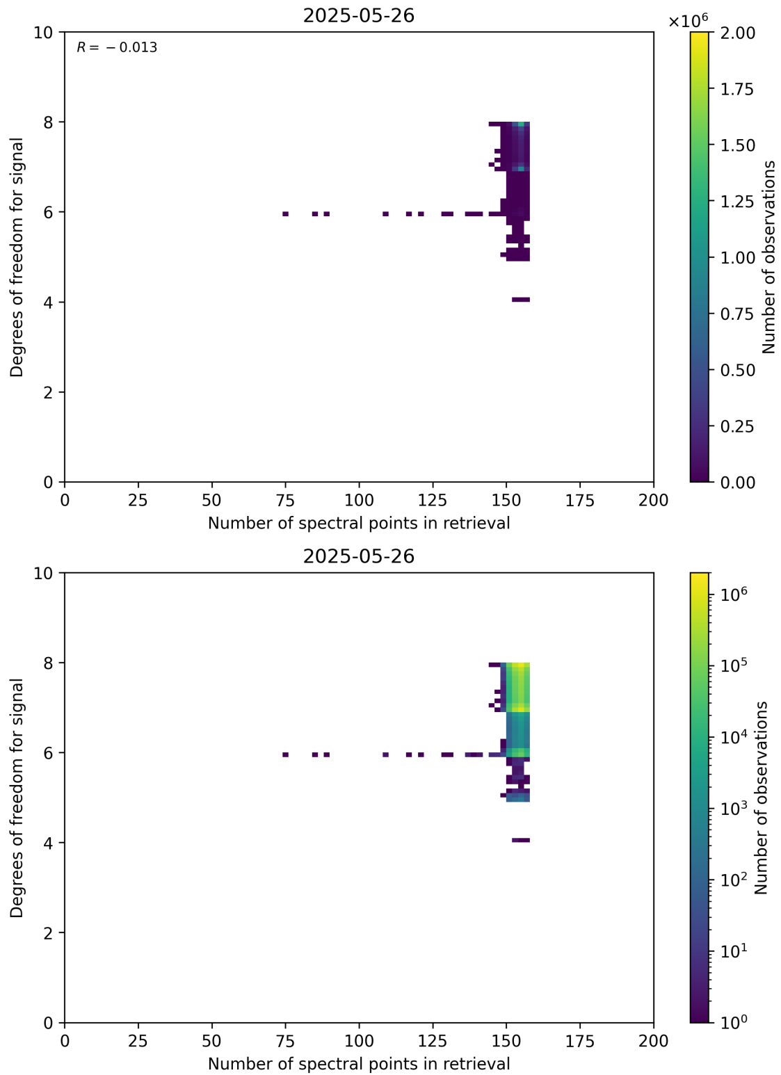
Figure 59: Scatter density plot of “Number of spectral points in retrieval” against “Degrees of freedom for signal” for 2025-05-26 to 2025-05-27.
