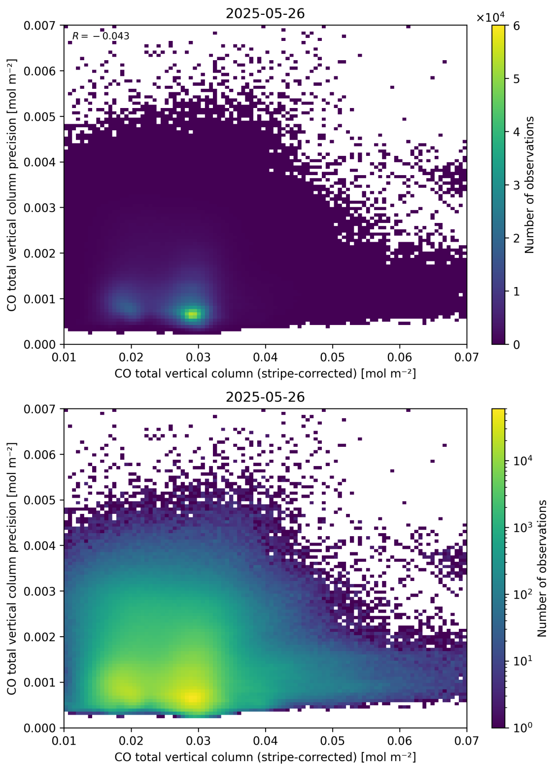
Figure 36: Scatter density plot of “CO total vertical column (stripe-corrected)” against “CO total vertical column precision” for 2025-05-26 to 2025-05-27.
