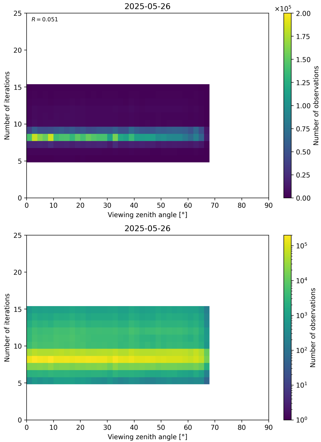
Figure 75: Scatter density plot of “Viewing zenith angle” against “Number of iterations” for 2025-05-26 to 2025-05-27.
