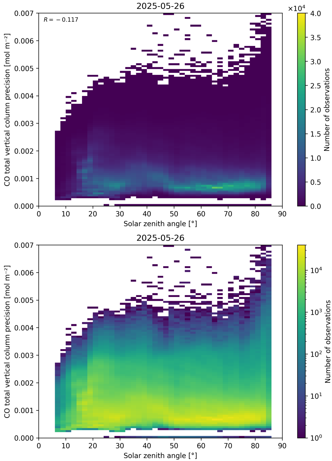
Figure 63: Scatter density plot of “Solar zenith angle” against “CO total vertical column precision” for 2025-05-26 to 2025-05-27.
