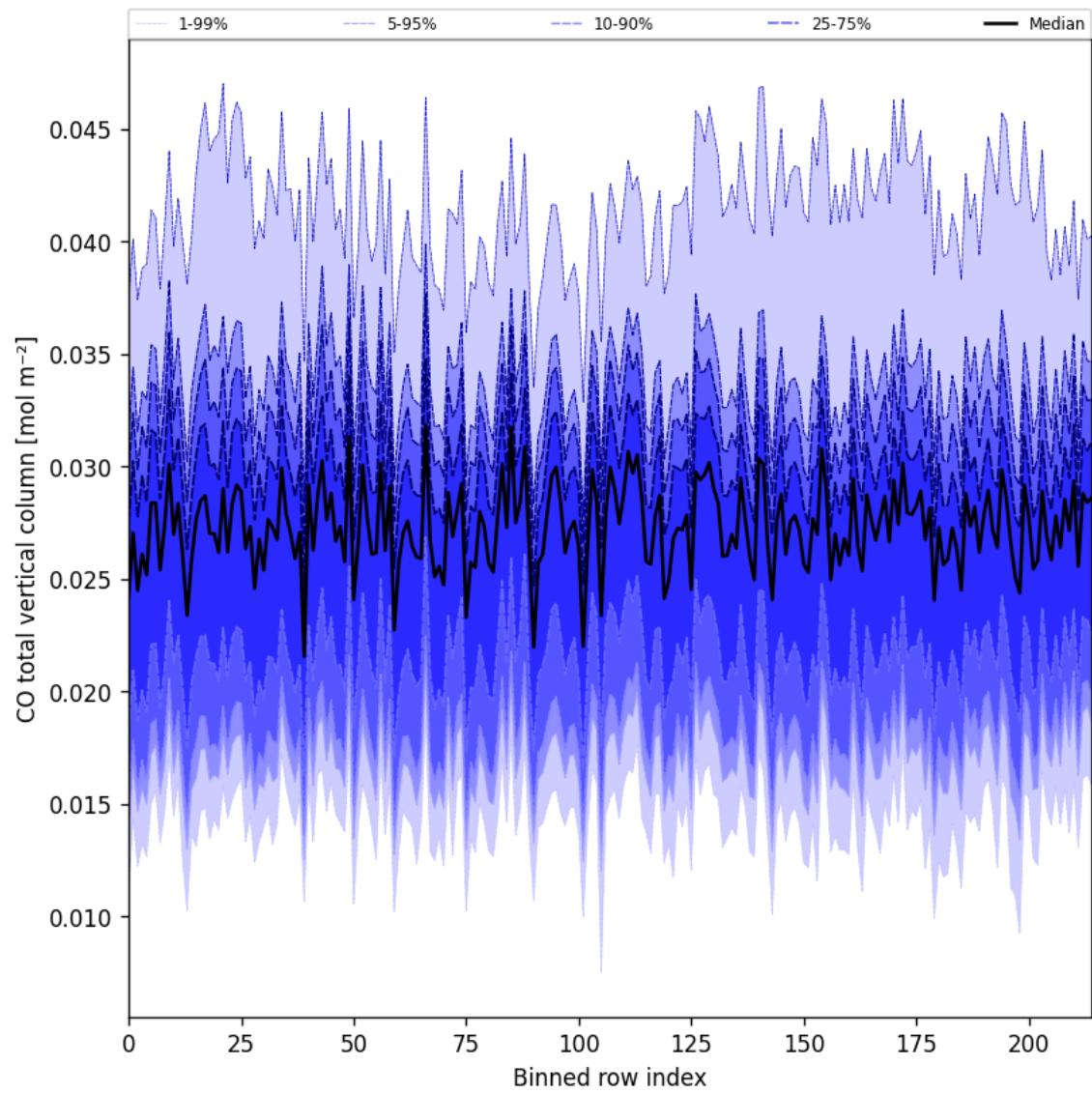
Figure 26: Along track statistics of “CO total vertical column” for 2025-05-26 to 2025-05-27
