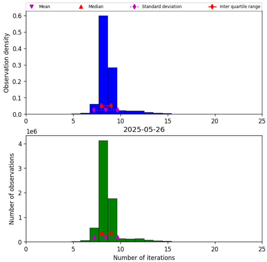
Figure 24: Histogram of “Number of iterations” for 2025-05-26 to 2025-05-27
