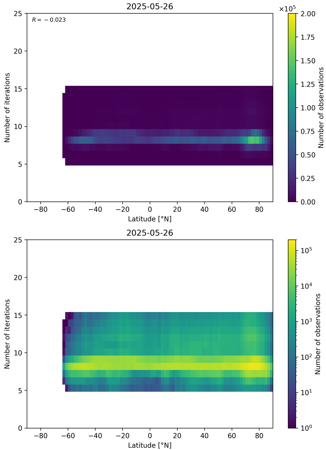
Figure 56: Scatter density plot of “Latitude” against “Number of iterations” for 2025-05-26 to 2025-05-27.
