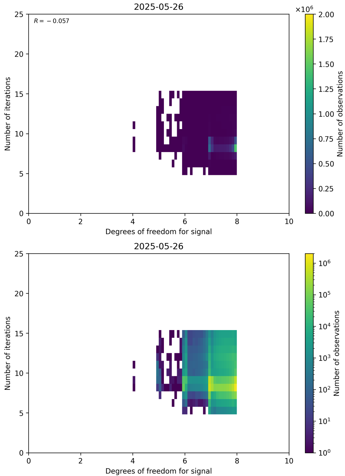
Figure 50: Scatter density plot of “Degrees of freedom for signal” against “Number of iterations” for 2025-05-26 to 2025-05-27.
