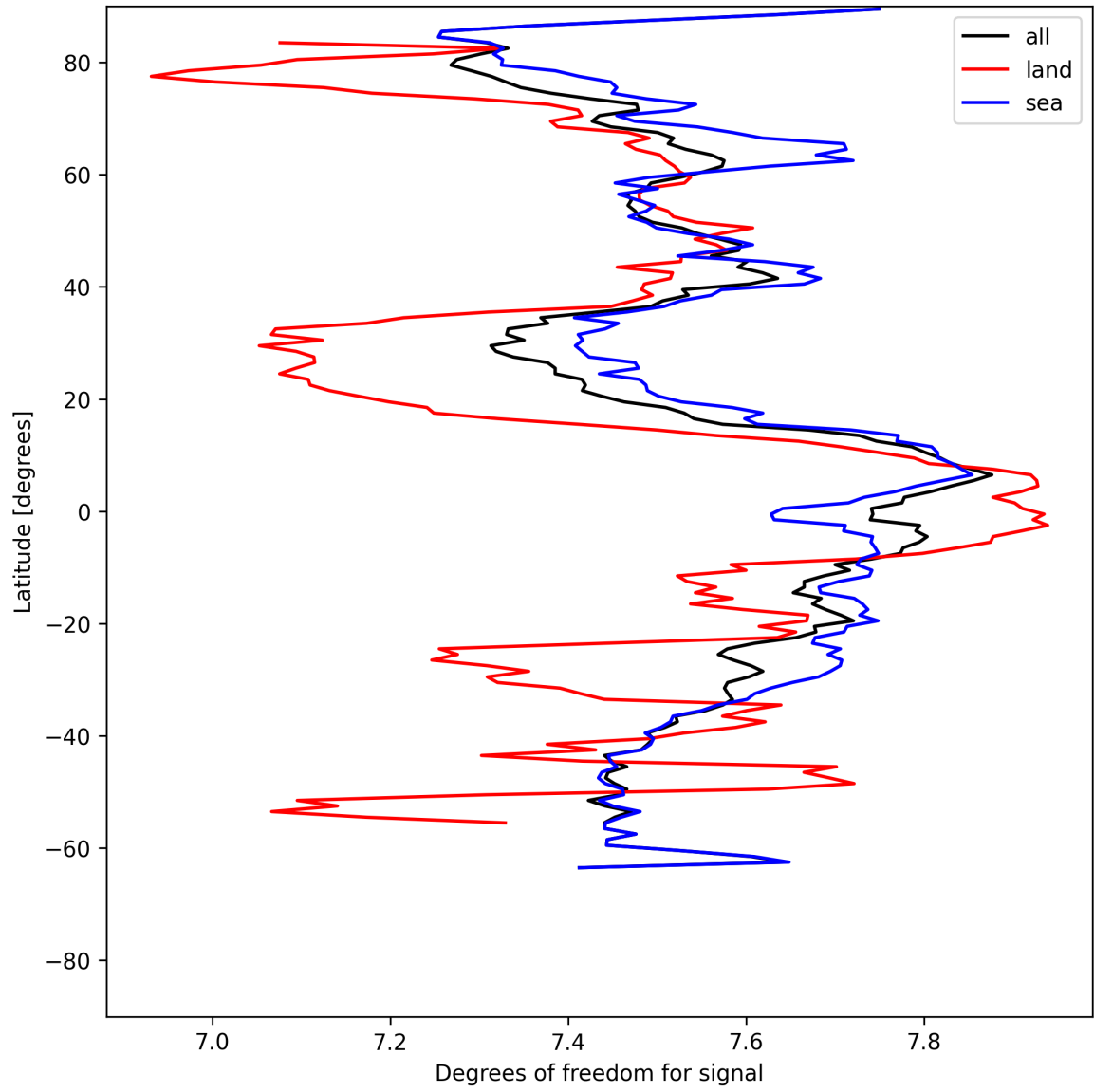
Figure 15: Zonal average of “Degrees of freedom for signal” for 2025-05-26 to 2025-05-27.
