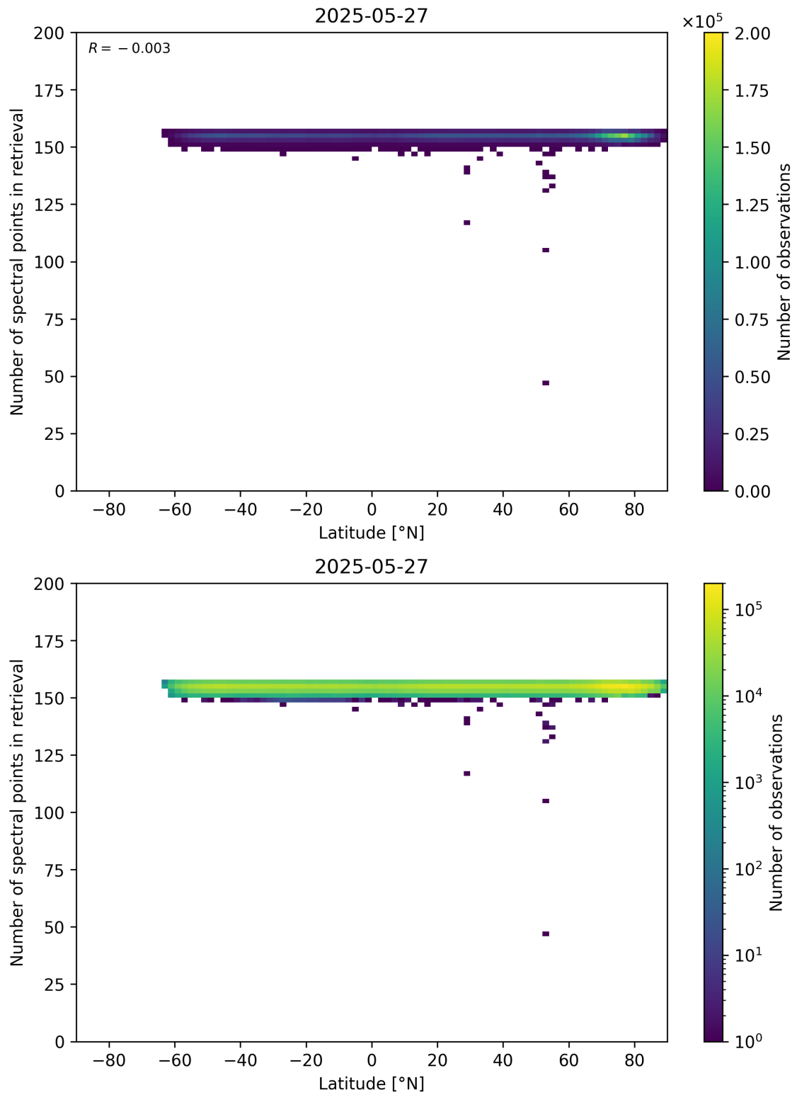
Figure 57: Scatter density plot of “Latitude” against “Number of spectral points in retrieval” for 2025-05-26 to 2025-05-28.
