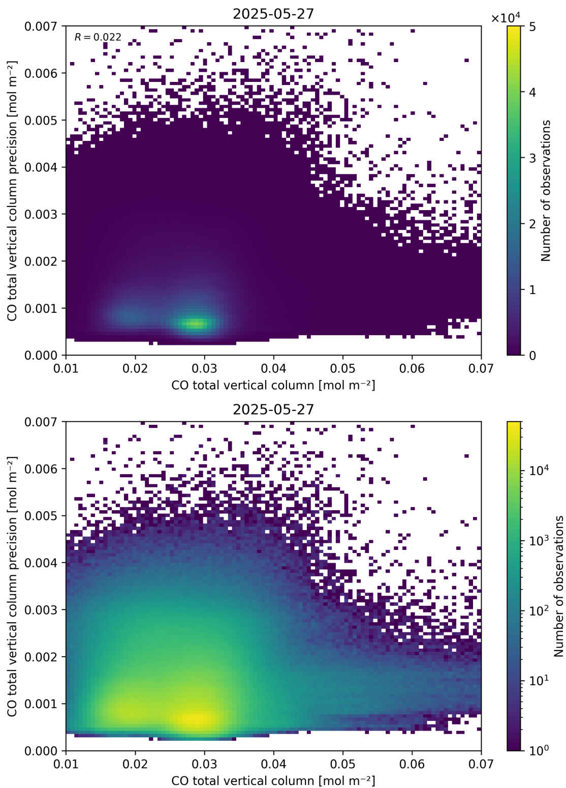
Figure 34: Scatter density plot of “CO total vertical column” against “CO total vertical column precision” for 2025-05-26 to 2025-05-28.
