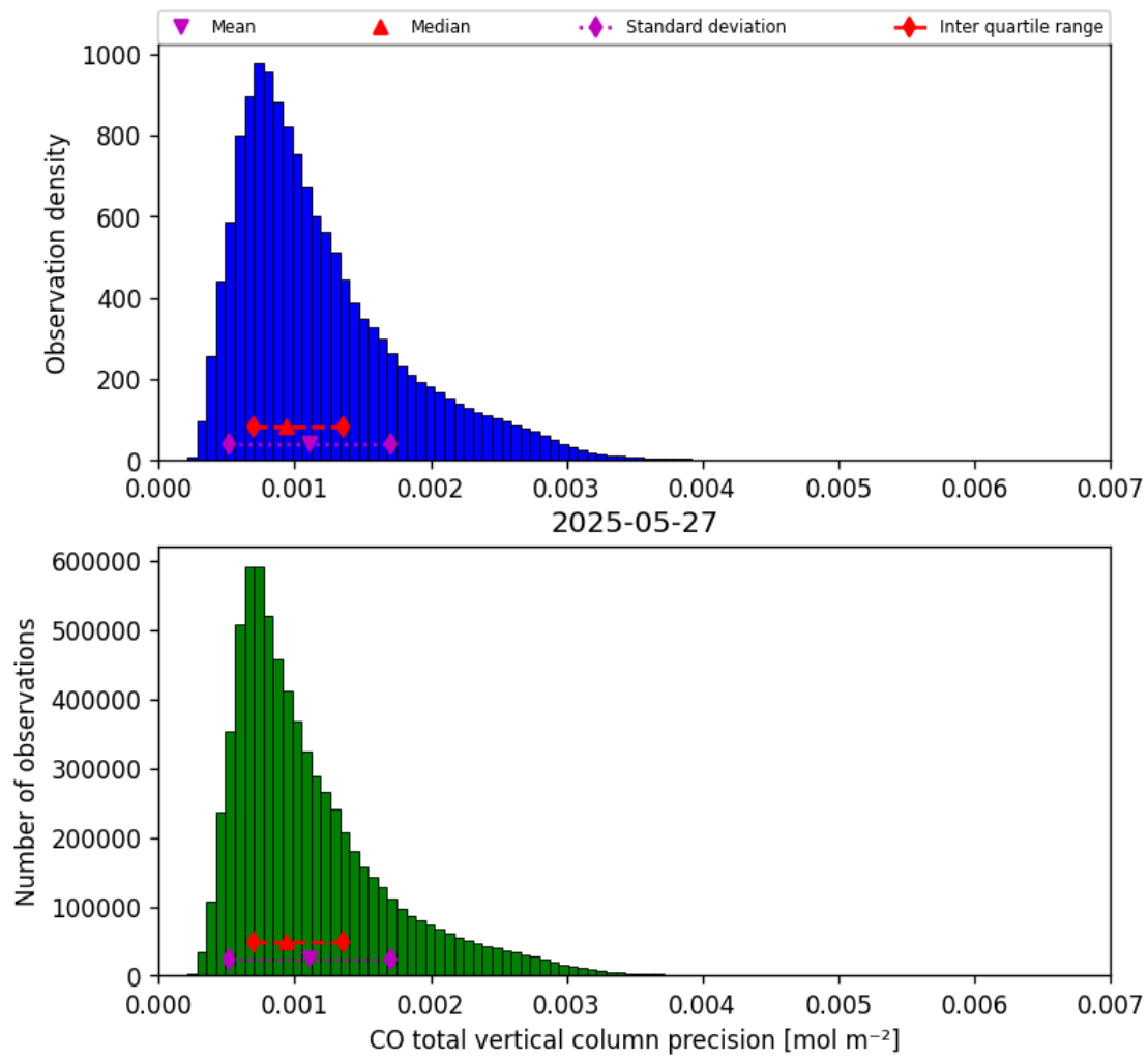
Figure 20: Histogram of “CO total vertical column precision” for 2025-05-26 to 2025-05-28
