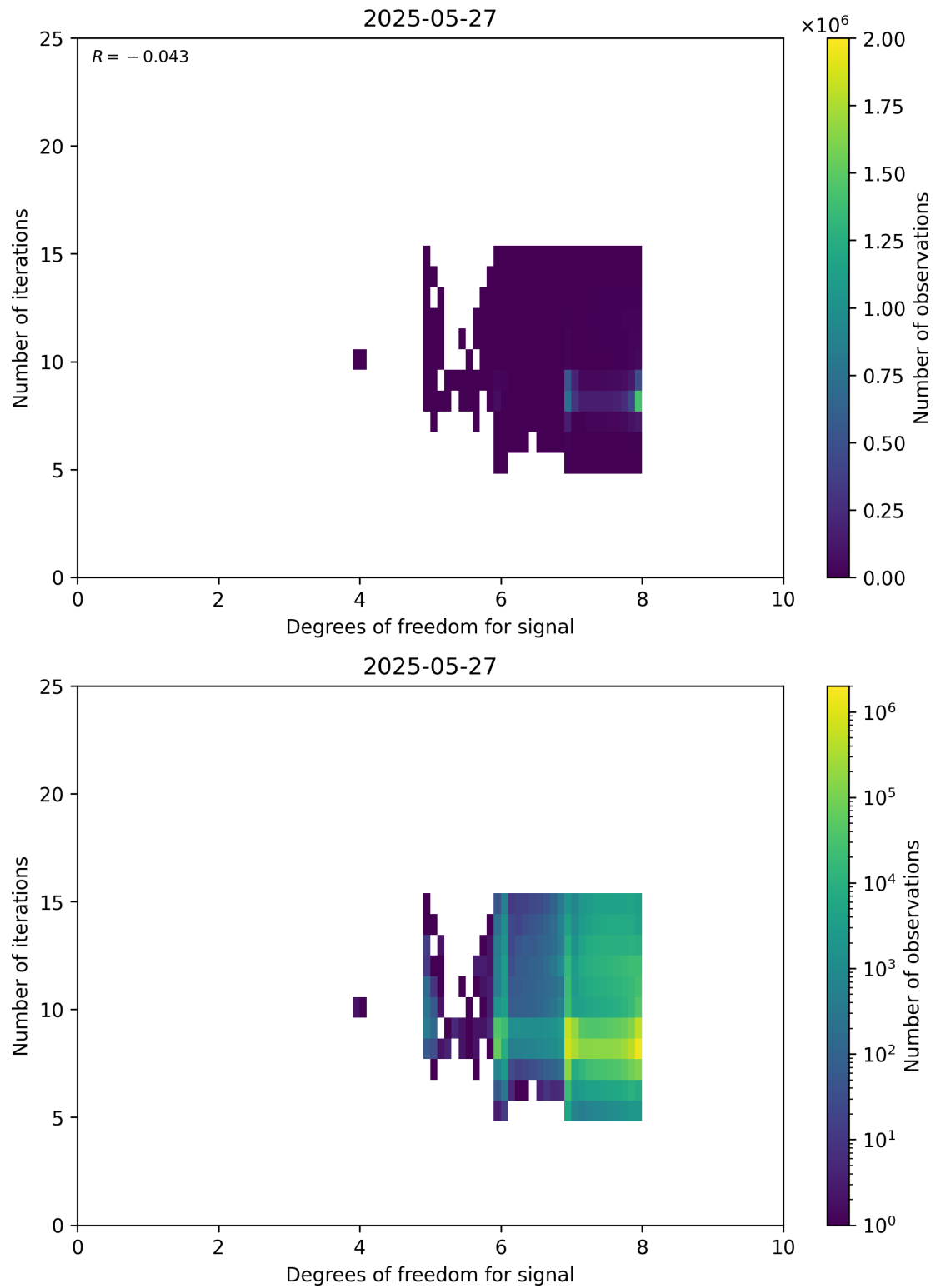
Figure 50: Scatter density plot of “Degrees of freedom for signal” against “Number of iterations” for 2025-05-26 to 2025-05-28.
