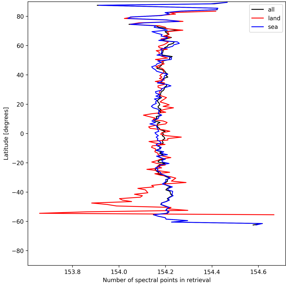
Figure 13: Zonal average of “Number of spectral points in retrieval” for 2025-05-26 to 2025-05-28.
