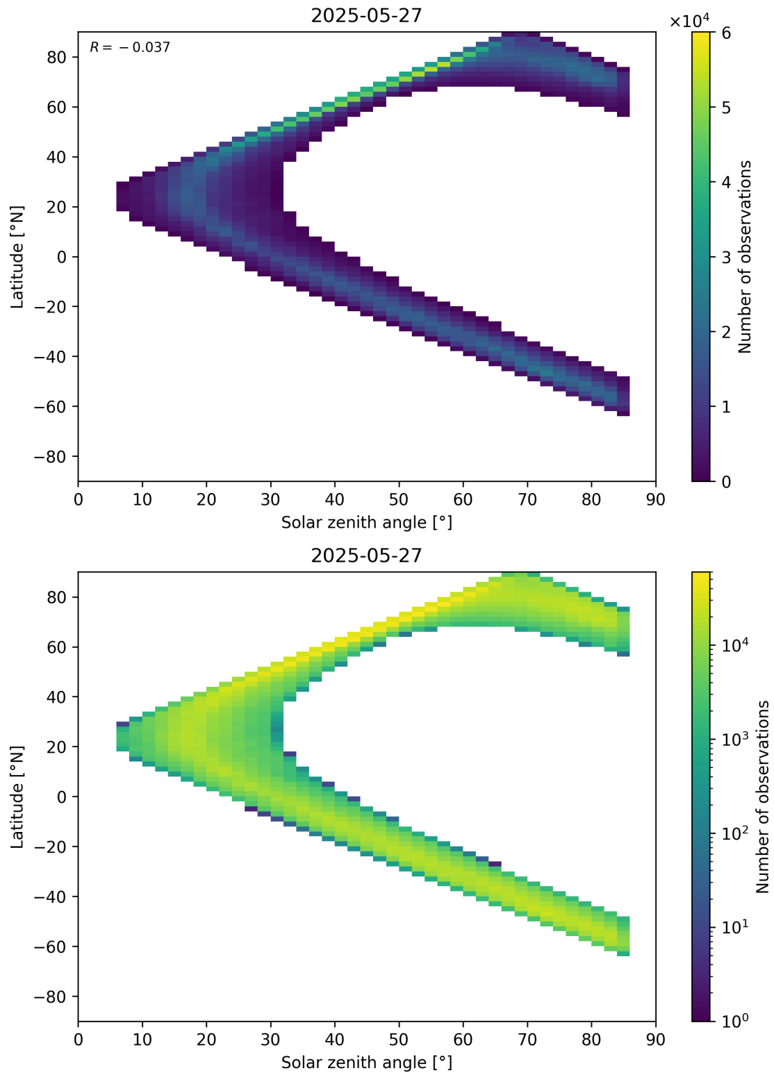
Figure 66: Scatter density plot of “Solar zenith angle” against “Latitude” for 2025-05-26 to 2025-05-28.
