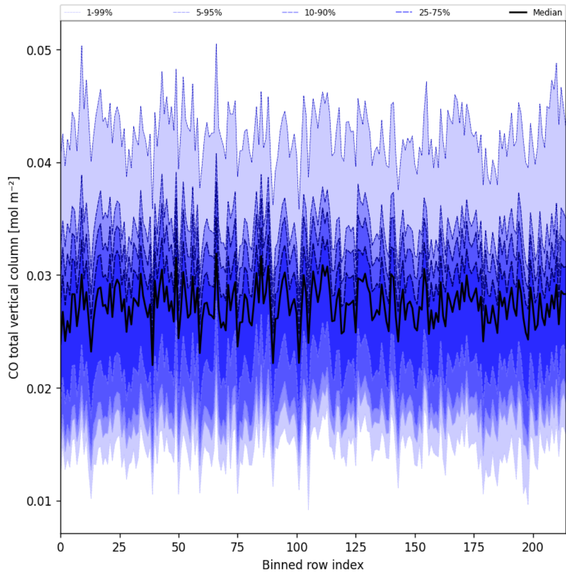
Figure 26: Along track statistics of “CO total vertical column” for 2025-05-26 to 2025-05-28
