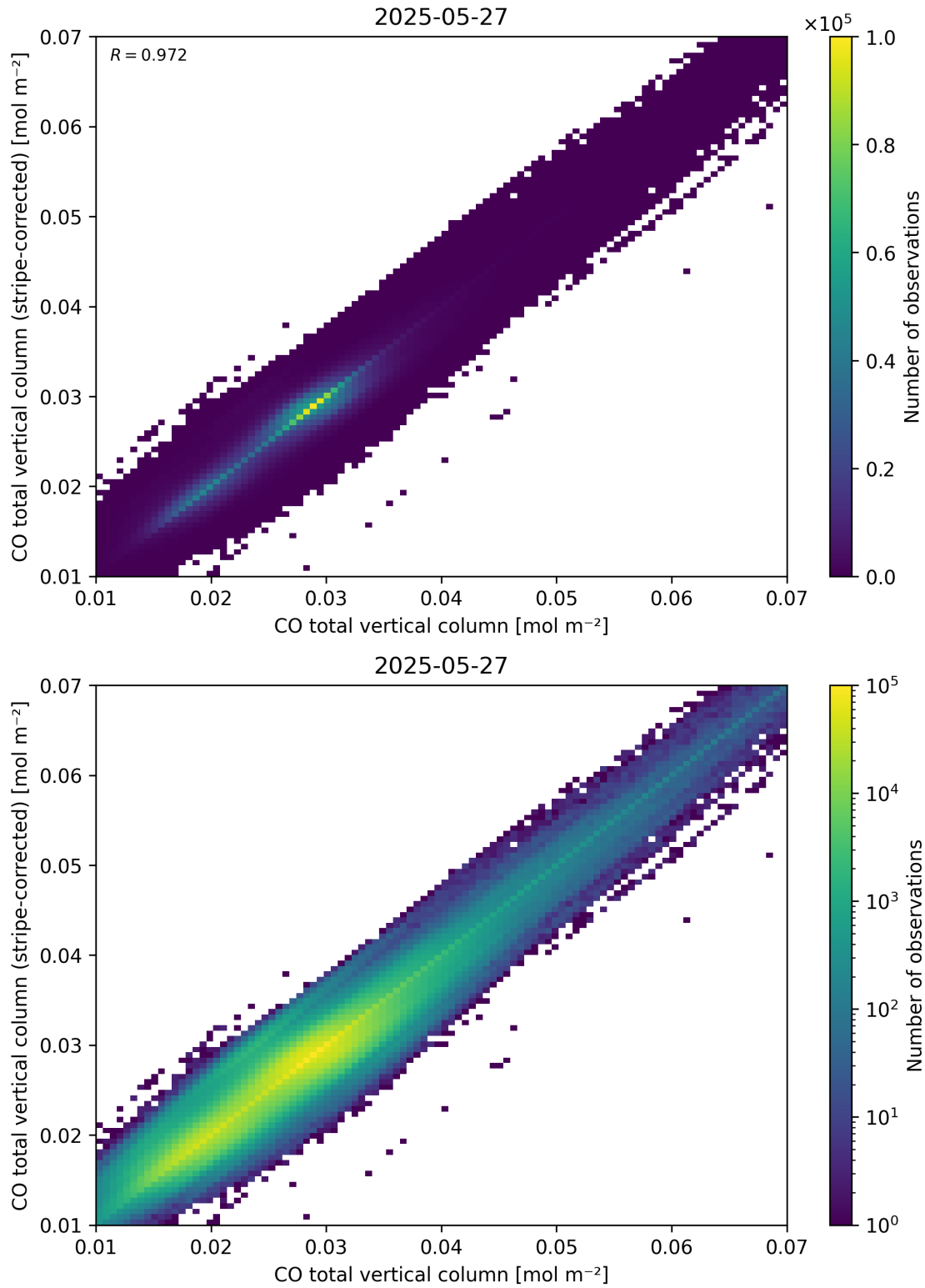
Figure 33: Scatter density plot of “CO total vertical column” against “CO total vertical column (stripe-corrected)” for 2025-05-26 to 2025-05-28.
