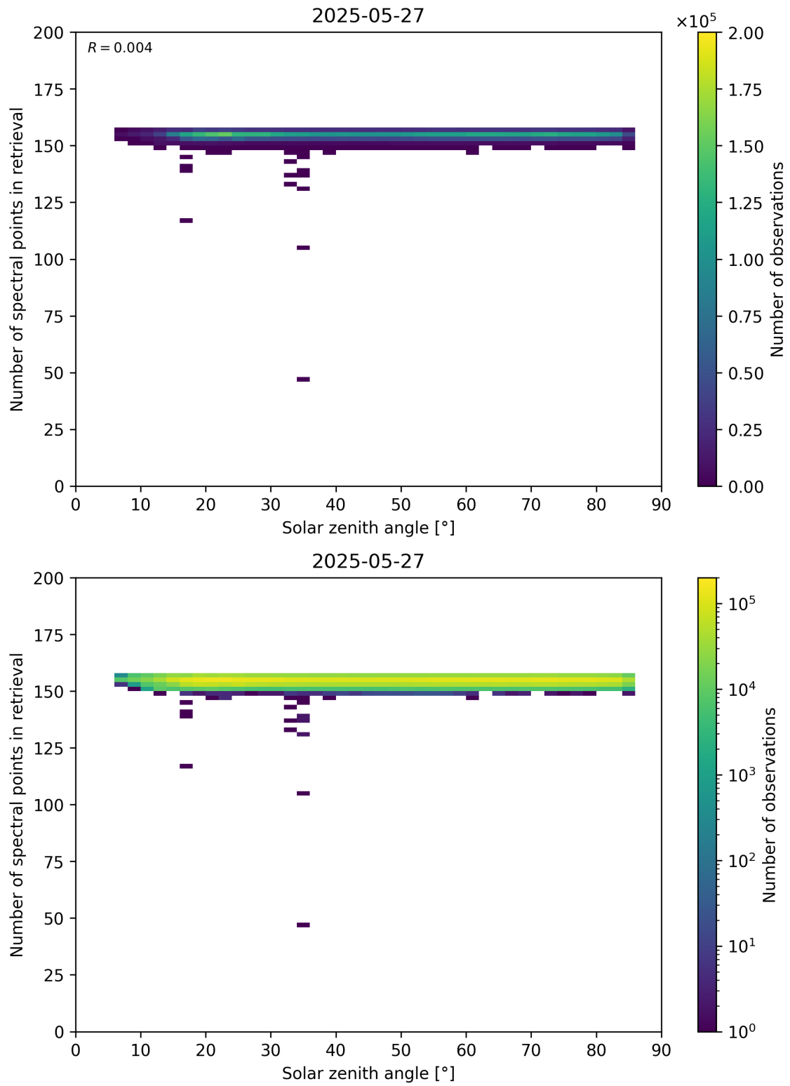
Figure 68: Scatter density plot of “Solar zenith angle” against “Number of spectral points in retrieval” for 2025-05-26 to 2025-05-28.
