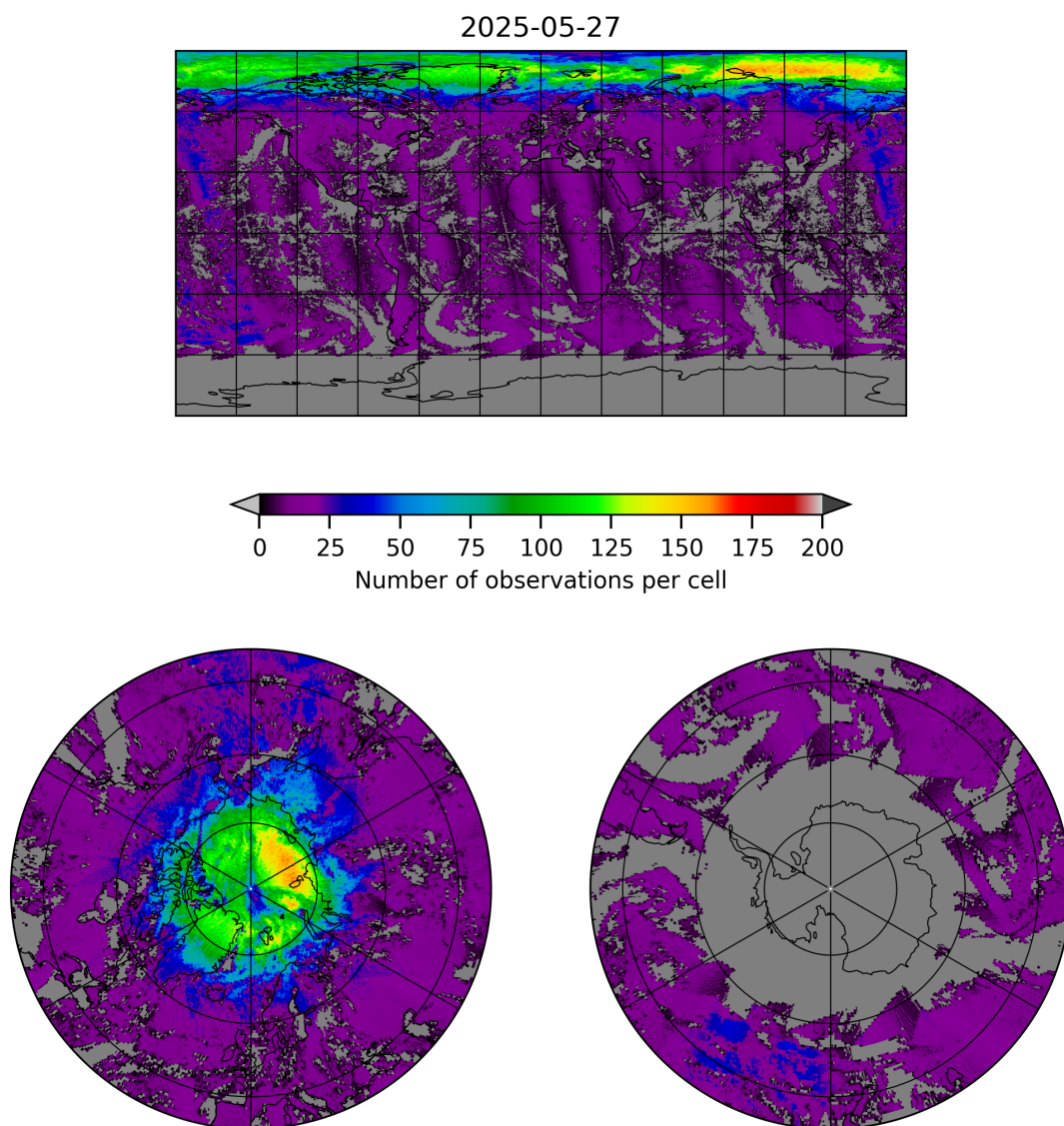
Figure 8: Map of the number of observations for 2025-05-26 to 2025-05-28
