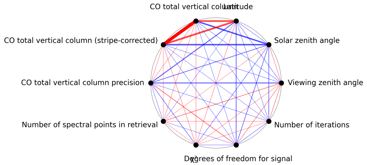
Figure 1: Map of correlation graph for 2025-05-26 to 2025-05-28.
