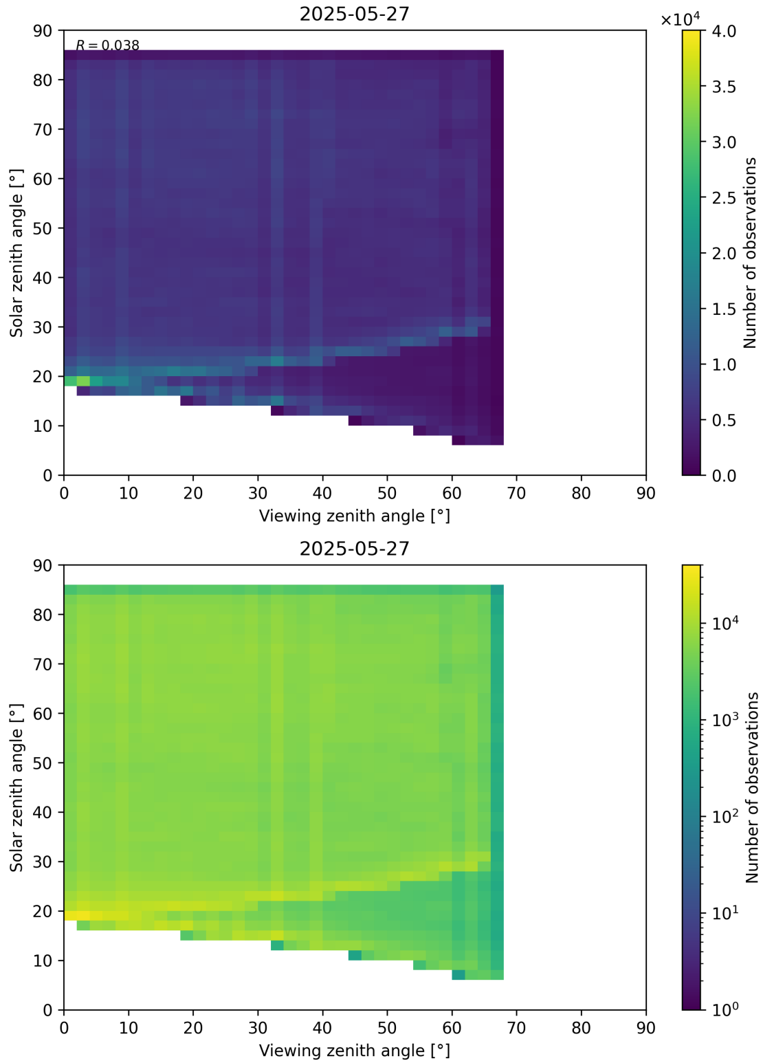
Figure 77: Scatter density plot of “Viewing zenith angle” against “Solar zenith angle” for 2025-05-26 to 2025-05-28.
