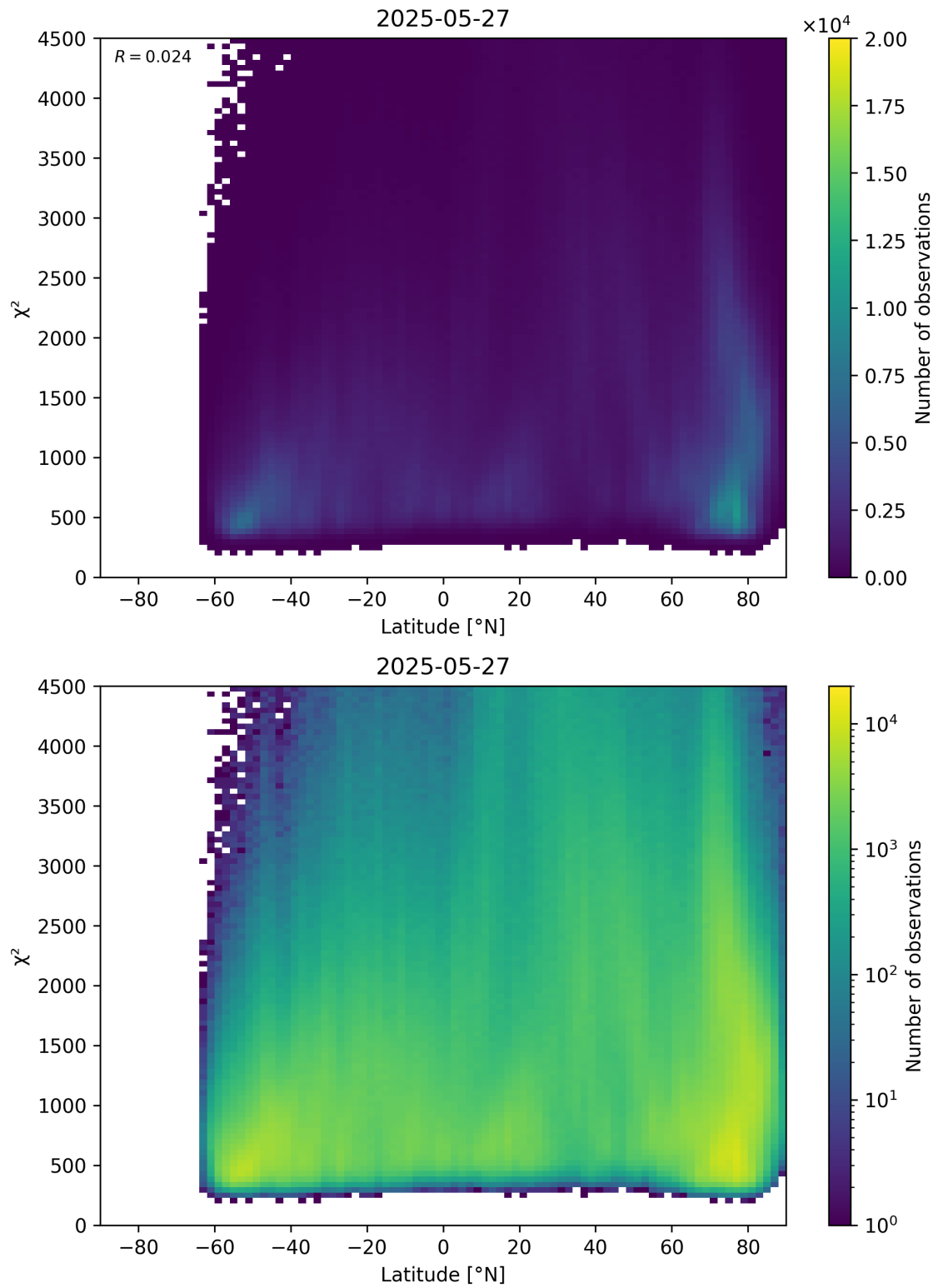
Figure 54: Scatter density plot of “Latitude” against “ \chi^2 ” for 2025-05-26 to 2025-05-28.
