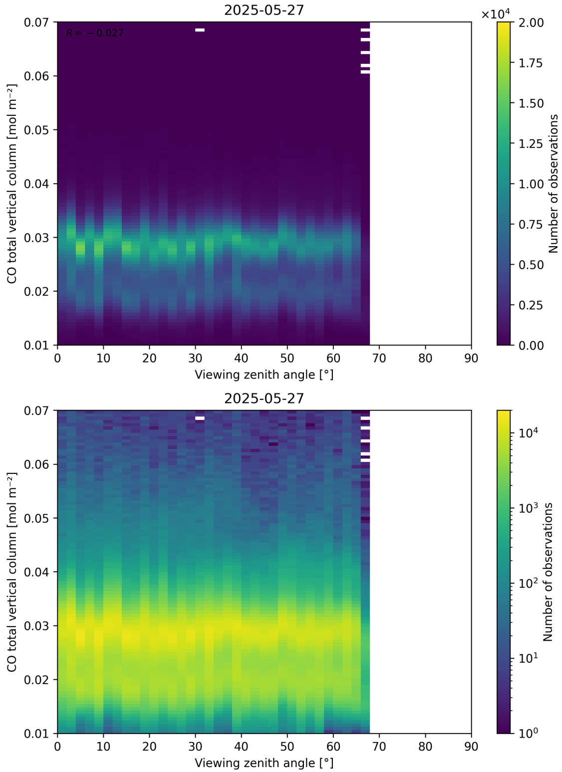
Figure 69: Scatter density plot of “Viewing zenith angle” against “CO total vertical column” for 2025-05-26 to 2025-05-28.
