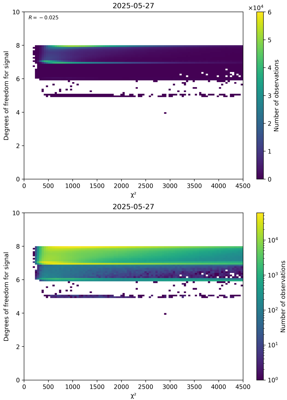
Figure 48: Scatter density plot of “ \chi^2 ” against “Degrees of freedom for signal” for 2025-05-26 to 2025-05-28.
