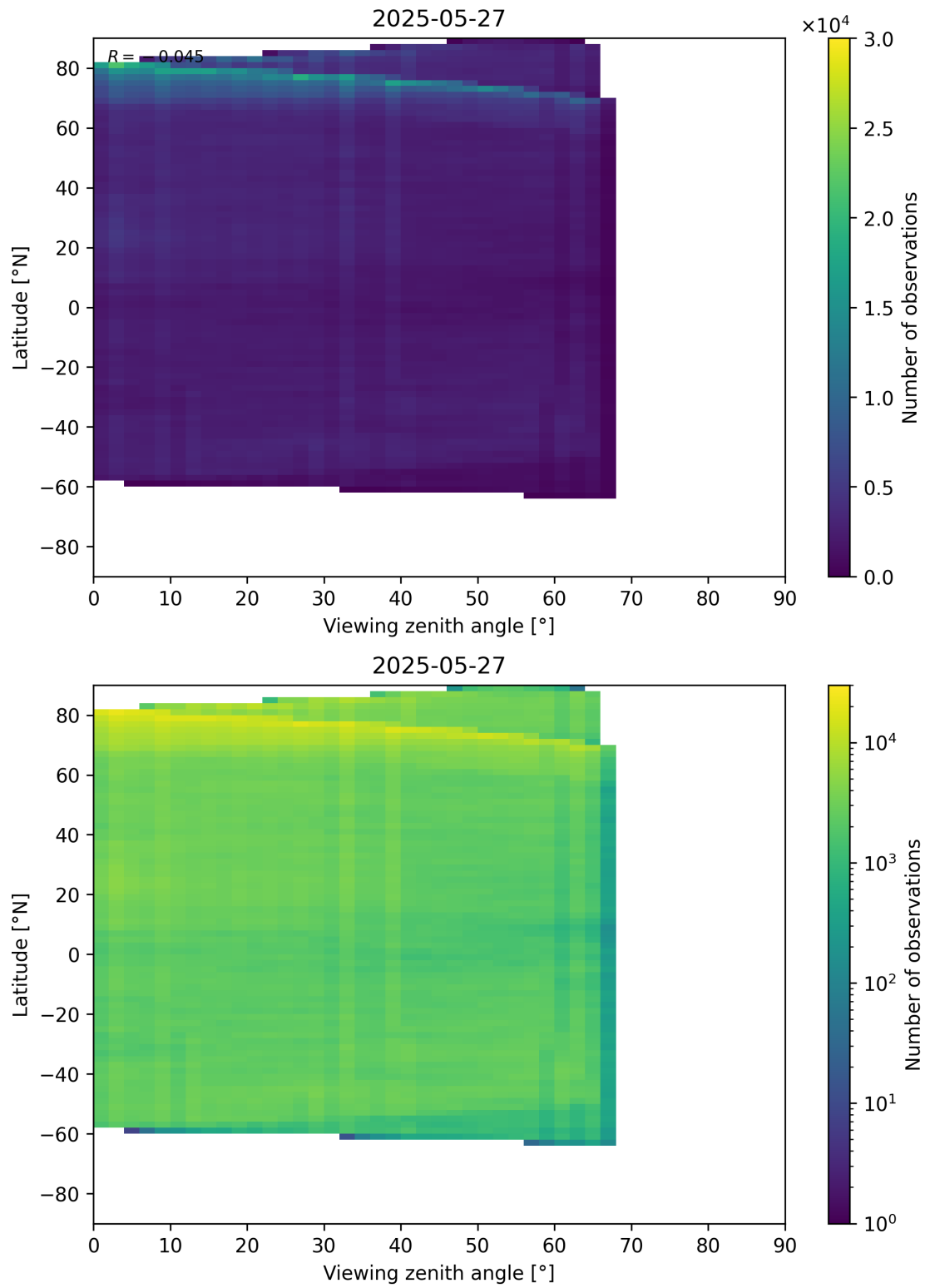
Figure 74: Scatter density plot of “Viewing zenith angle” against “Latitude” for 2025-05-26 to 2025-05-28.
