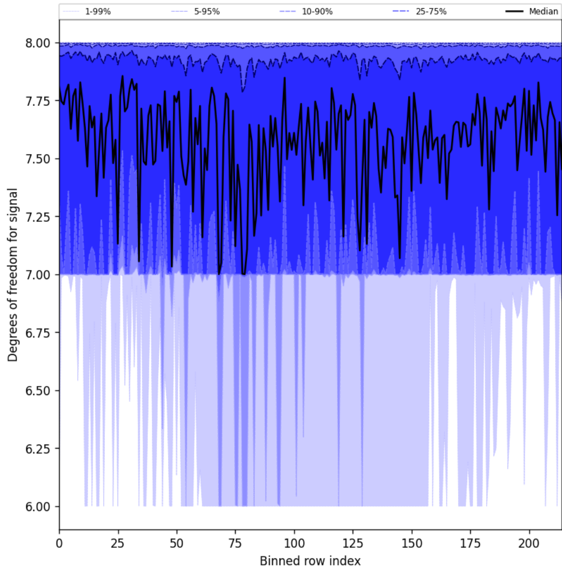
Figure 31: Along track statistics of “Degrees of freedom for signal” for 2025-05-26 to 2025-05-28
