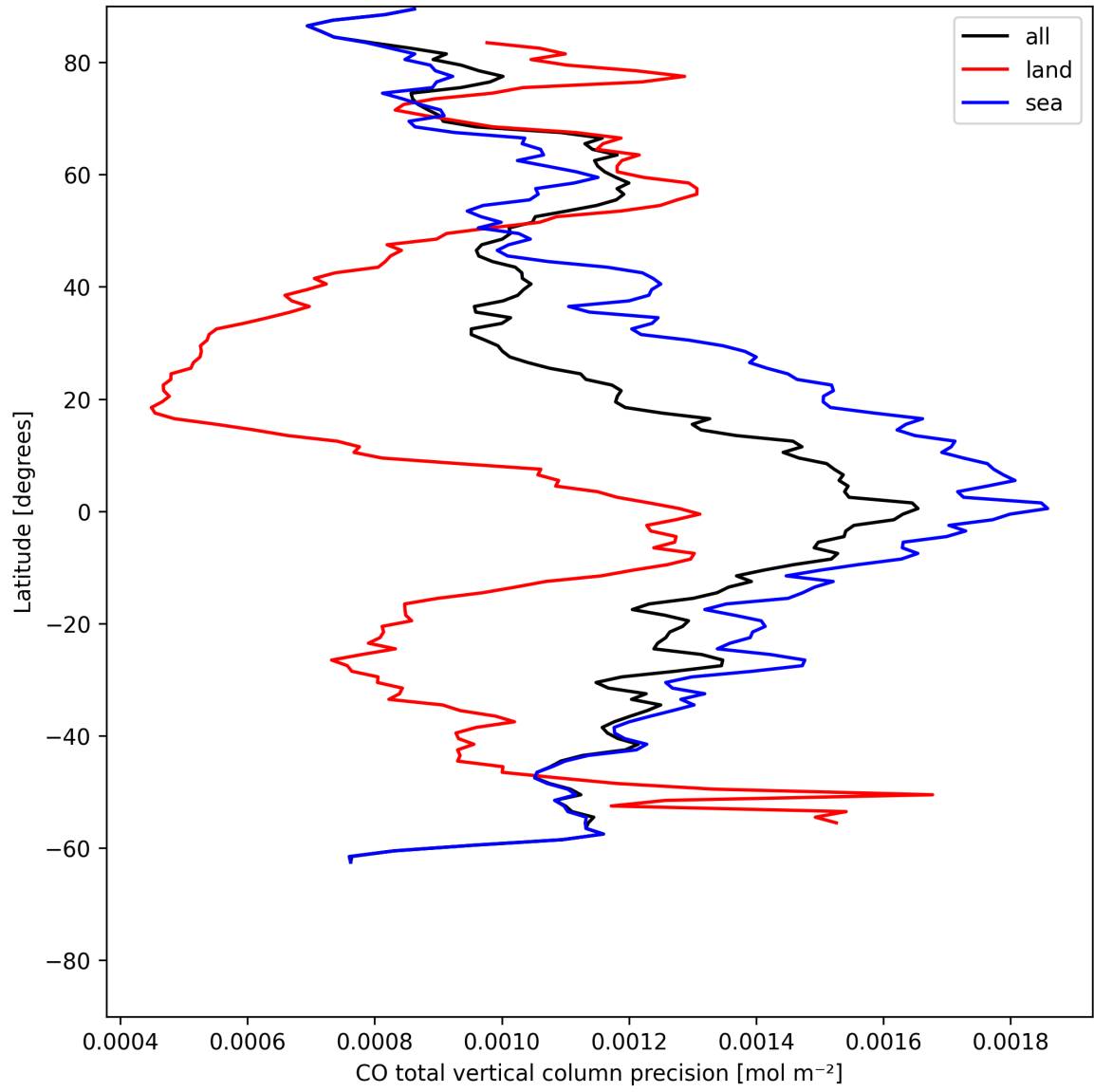
Figure 12: Zonal average of “CO total vertical column precision” for 2025-05-26 to 2025-05-28.
