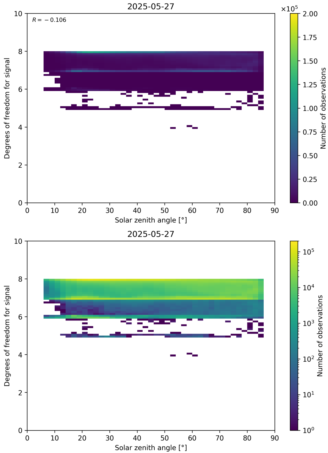
Figure 65: Scatter density plot of “Solar zenith angle” against “Degrees of freedom for signal” for 2025-05-26 to 2025-05-28.
