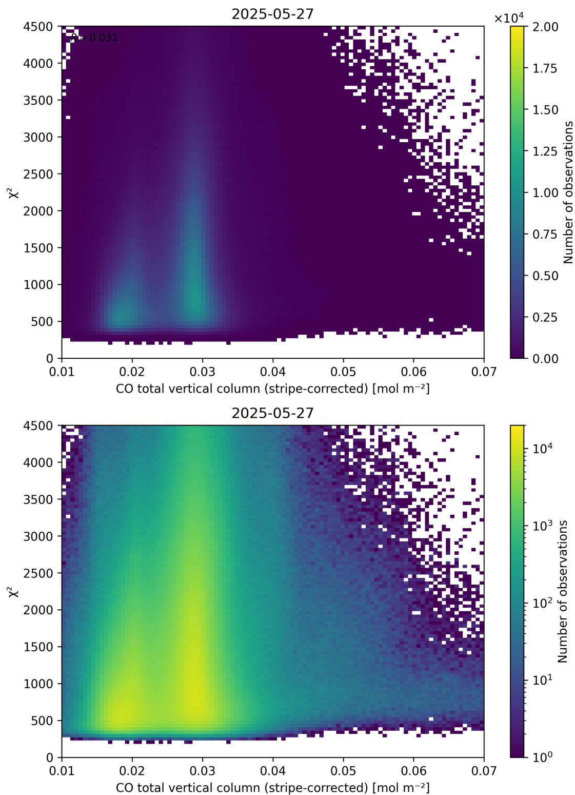
Figure 37: Scatter density plot of “CO total vertical column (stripe-corrected)” against “ \chi^2 ” for 2025-05-26 to 2025-05-28.
