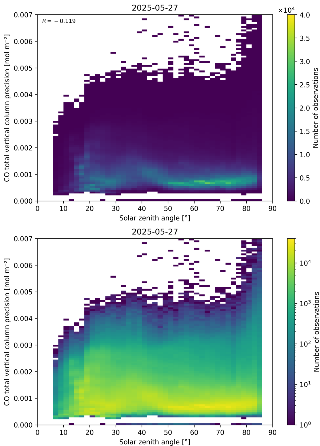
Figure 63: Scatter density plot of “Solar zenith angle” against “CO total vertical column precision” for 2025-05-26 to 2025-05-28.
