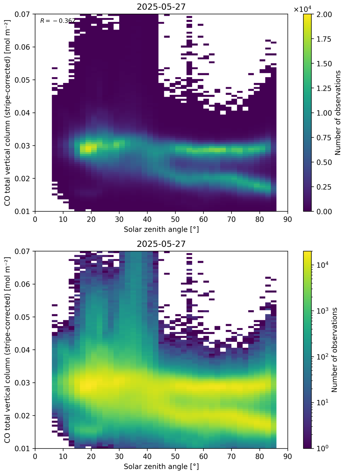
Figure 62: Scatter density plot of “Solar zenith angle” against “CO total vertical column (stripe-corrected)” for 2025-05-26 to 2025-05-28.
