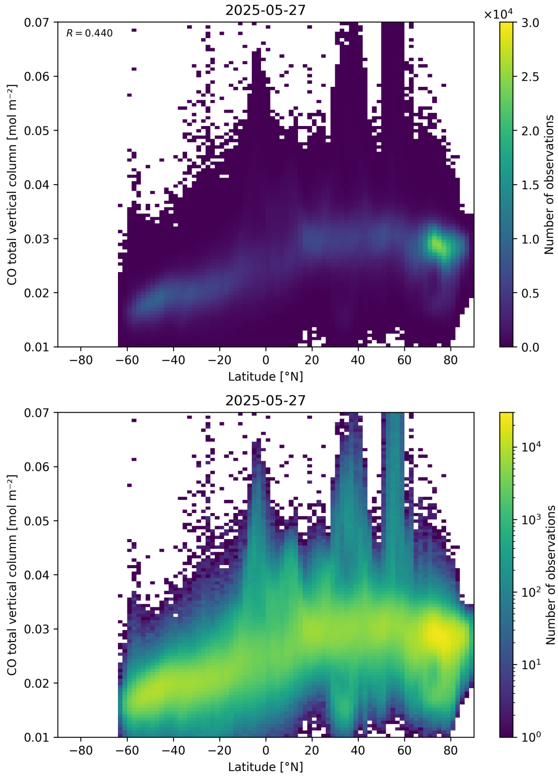
Figure 51: Scatter density plot of “Latitude” against “CO total vertical column” for 2025-05-26 to 2025-05-28.
