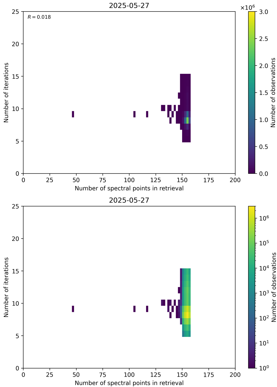
Figure 60: Scatter density plot of “Number of spectral points in retrieval” against “Number of iterations” for 2025-05-26 to 2025-05-28.
