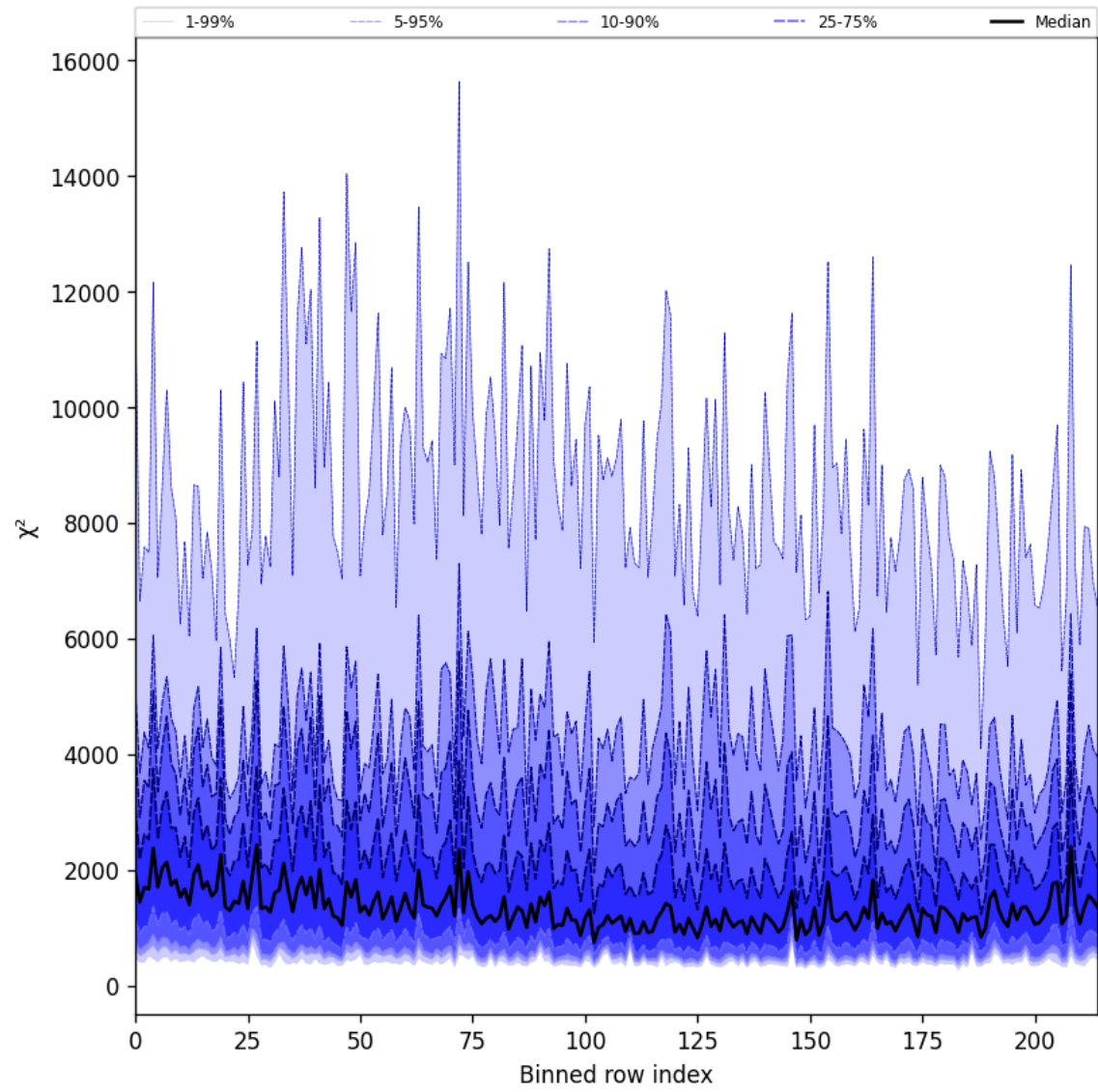
Figure 30: Along track statistics of “ \chi^2 ” for 2025-05-26 to 2025-05-28
