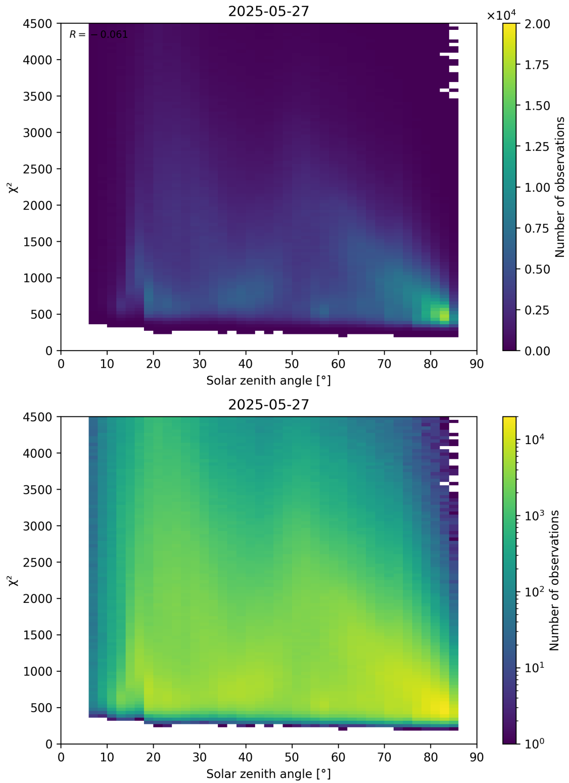
Figure 64: Scatter density plot of “Solar zenith angle” against “ \chi^2 ” for 2025-05-26 to 2025-05-28.
