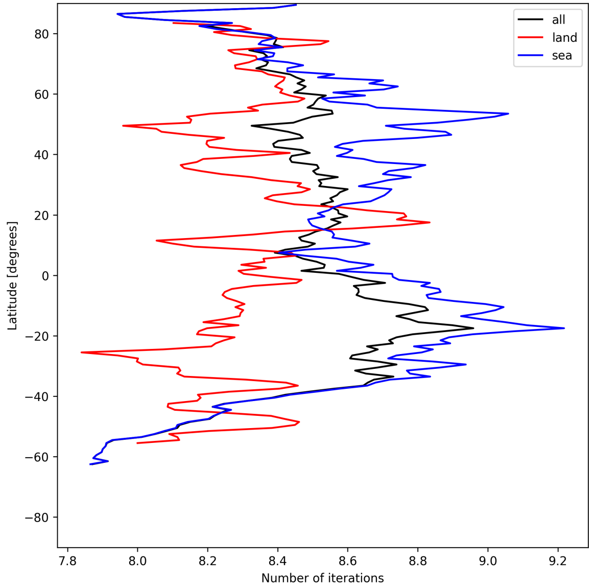
Figure 16: Zonal average of “Number of iterations” for 2025-05-26 to 2025-05-28.
