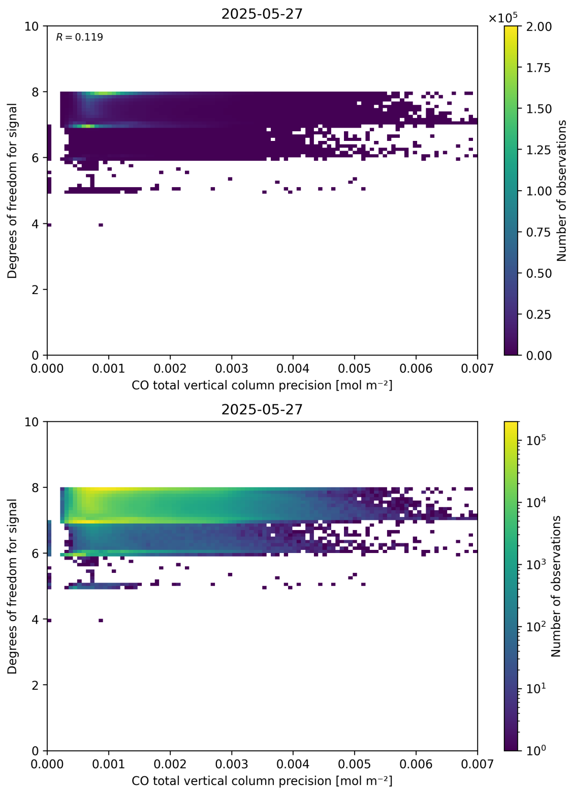
Figure 45: Scatter density plot of “CO total vertical column precision” against “Degrees of freedom for signal” for 2025-05-26 to 2025-05-28.
