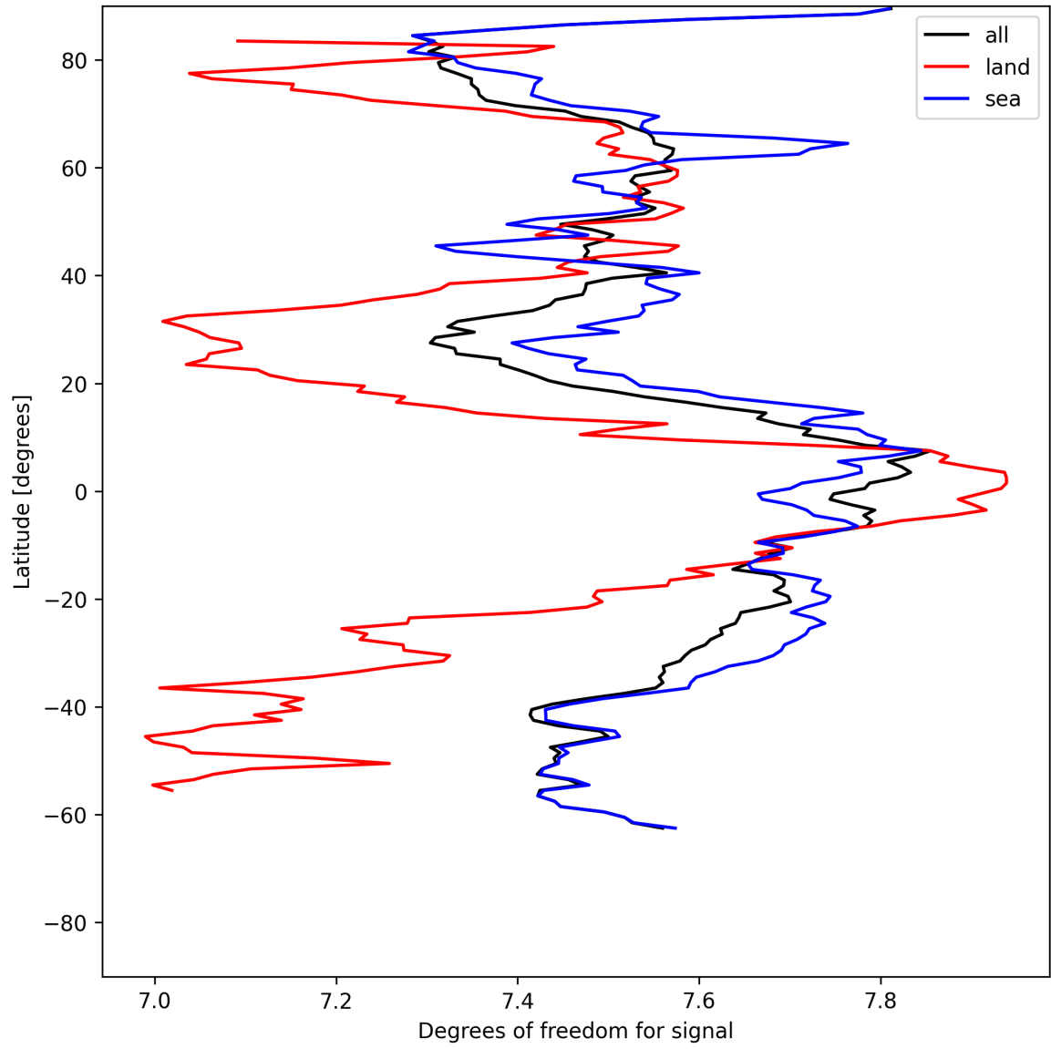
Figure 15: Zonal average of “Degrees of freedom for signal” for 2025-05-26 to 2025-05-28.
