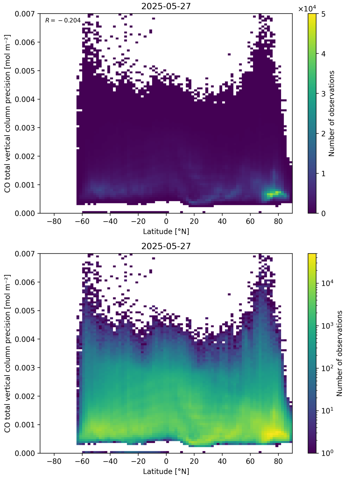
Figure 53: Scatter density plot of “Latitude” against “CO total vertical column precision” for 2025-05-26 to 2025-05-28.
