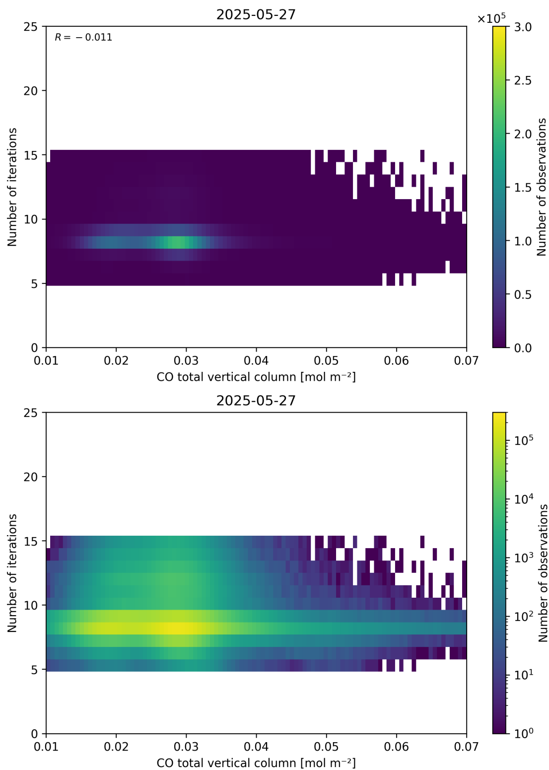
Figure 42: Scatter density plot of “CO total vertical column” against “Number of iterations” for 2025-05-26 to 2025-05-28.
