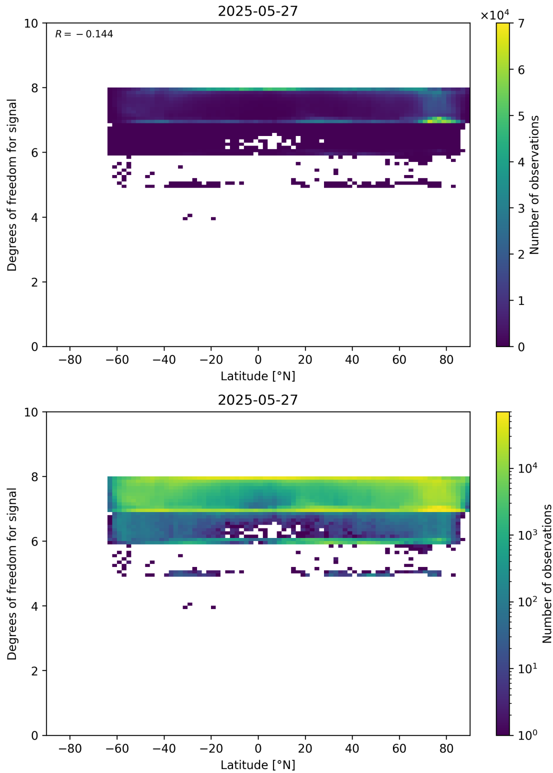
Figure 55: Scatter density plot of “Latitude” against “Degrees of freedom for signal” for 2025-05-26 to 2025-05-28.
