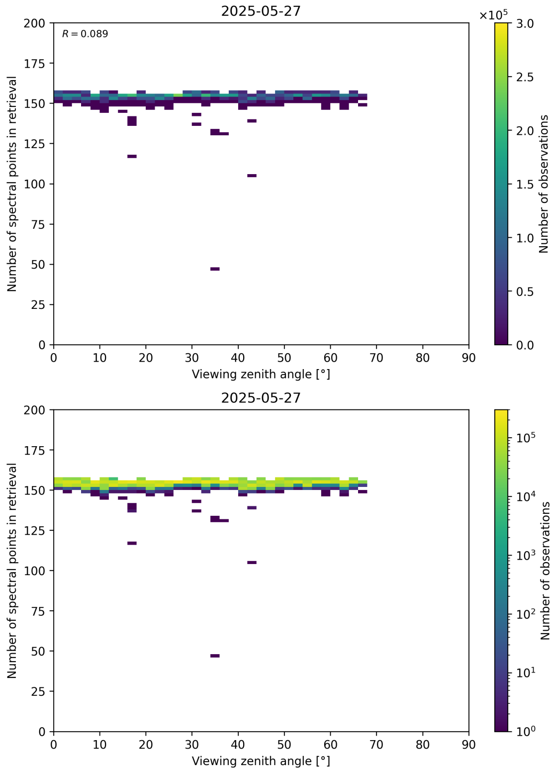
Figure 76: Scatter density plot of “Viewing zenith angle” against “Number of spectral points in retrieval” for 2025-05-26 to 2025-05-28.
