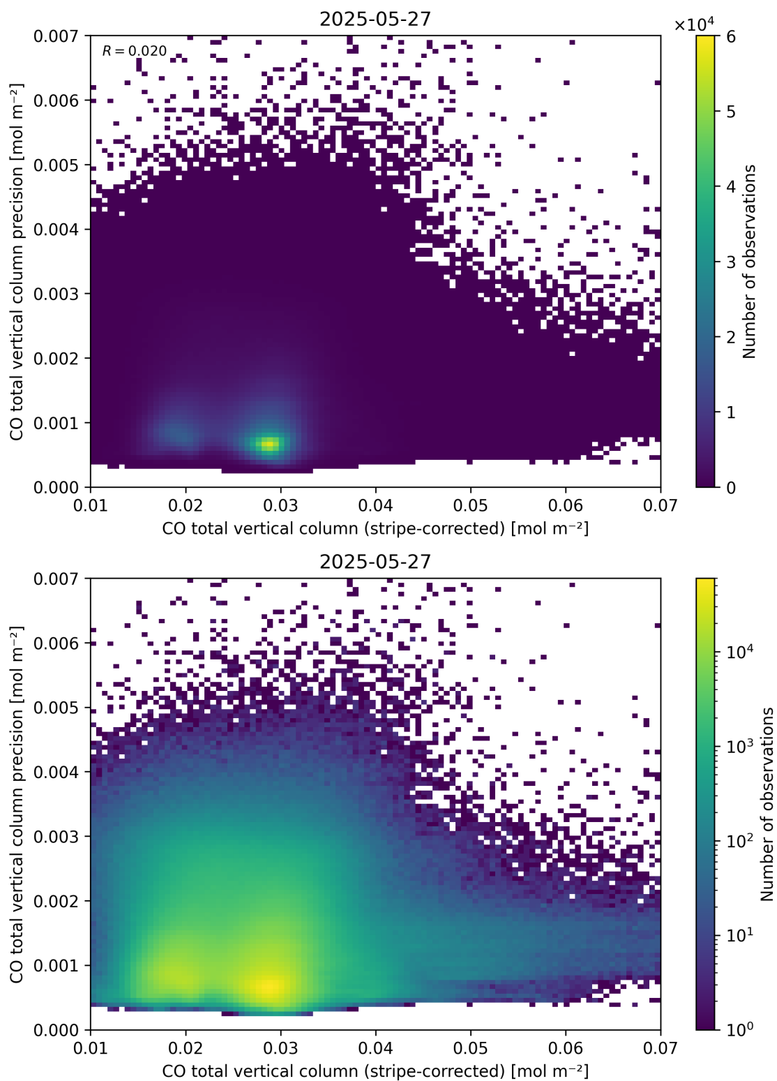
Figure 36: Scatter density plot of “CO total vertical column (stripe-corrected)” against “CO total vertical column precision” for 2025-05-26 to 2025-05-28.
