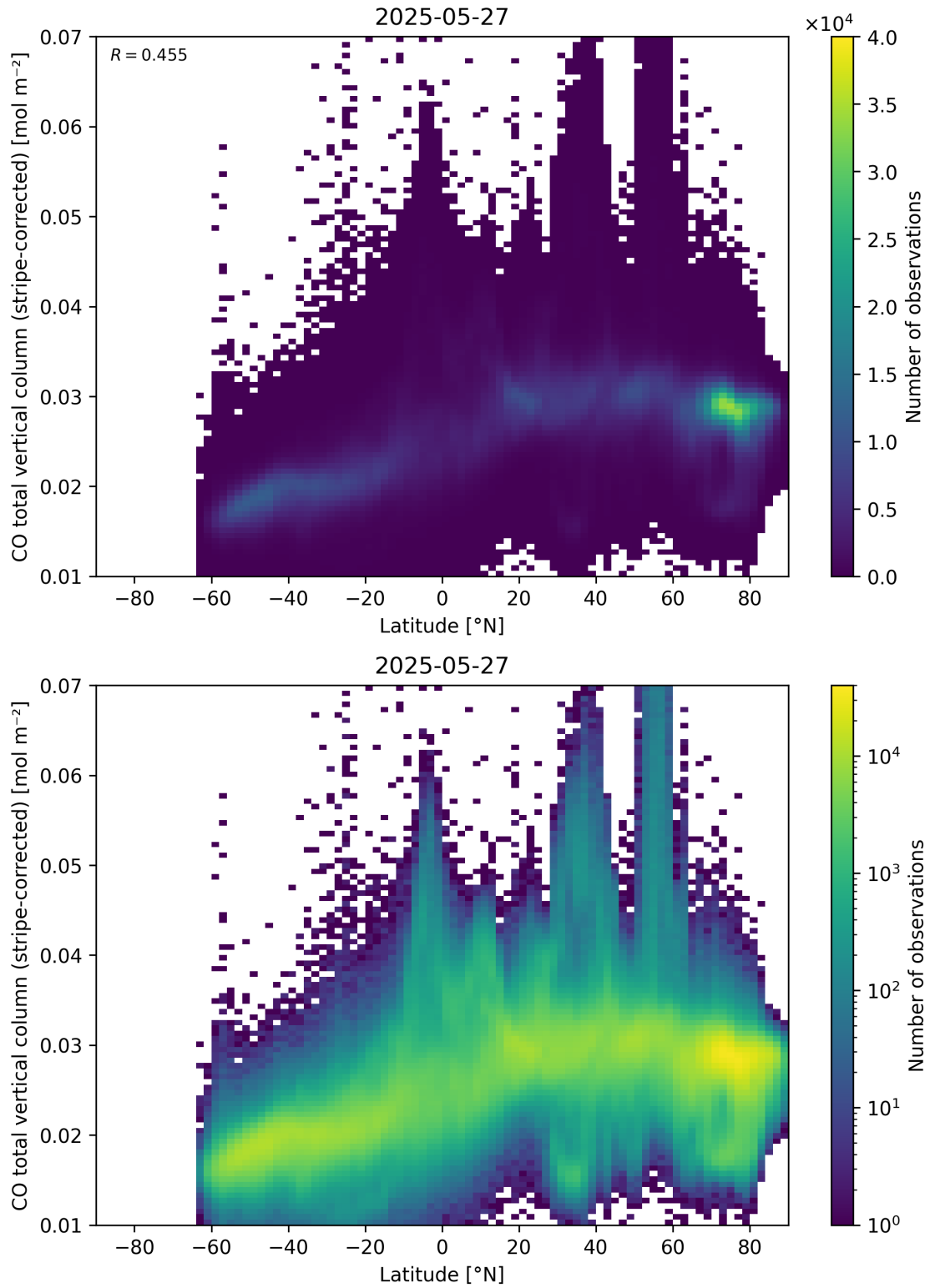
Figure 52: Scatter density plot of “Latitude” against “CO total vertical column (stripe-corrected)” for 2025-05-26 to 2025-05-28.
