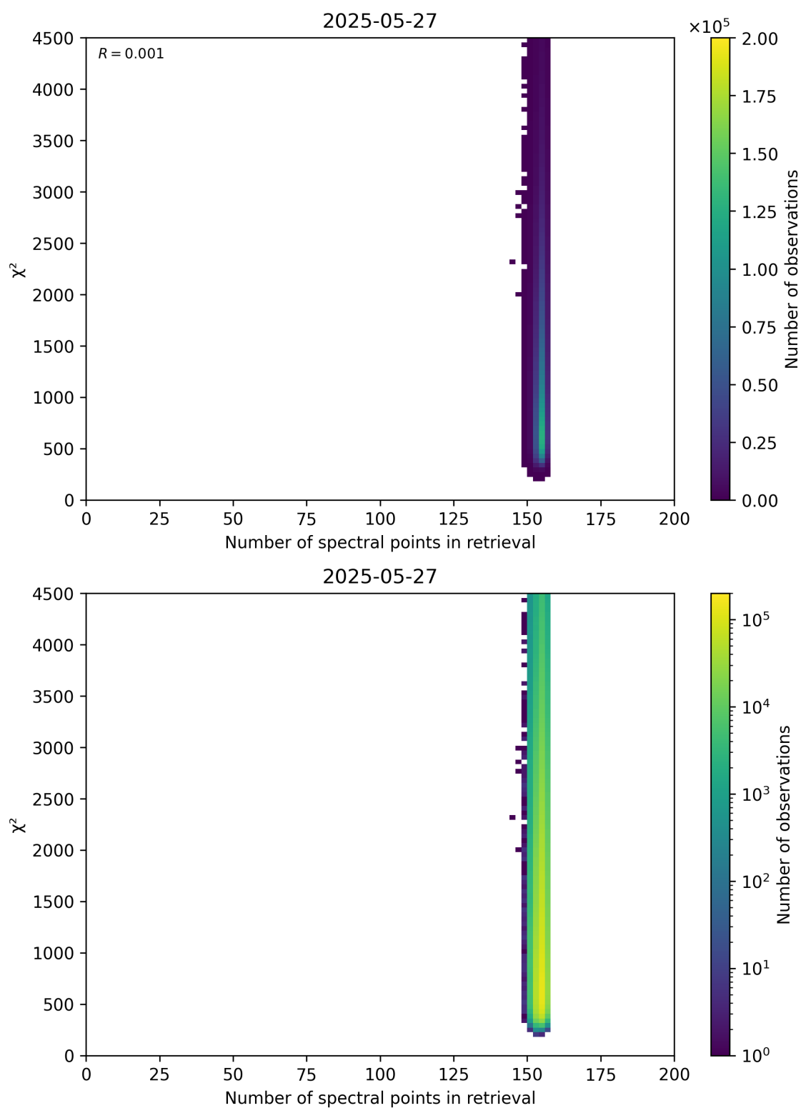
Figure 58: Scatter density plot of “Number of spectral points in retrieval” against “ \chi^2 ” for 2025-05-26 to 2025-05-28.
