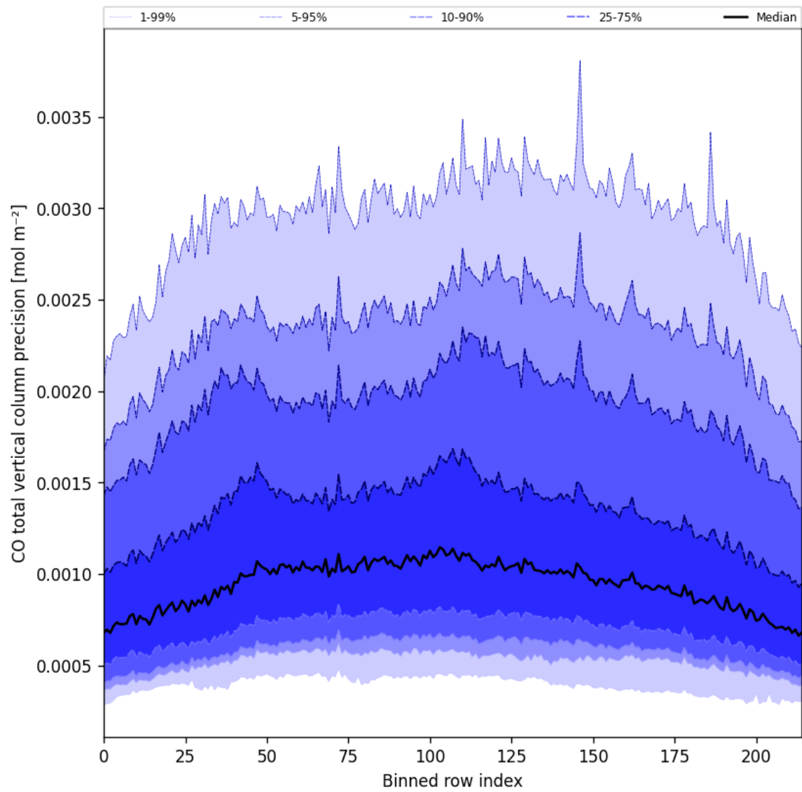
Figure 28: Along track statistics of “CO total vertical column precision” for 2025-05-26 to 2025-05-28
