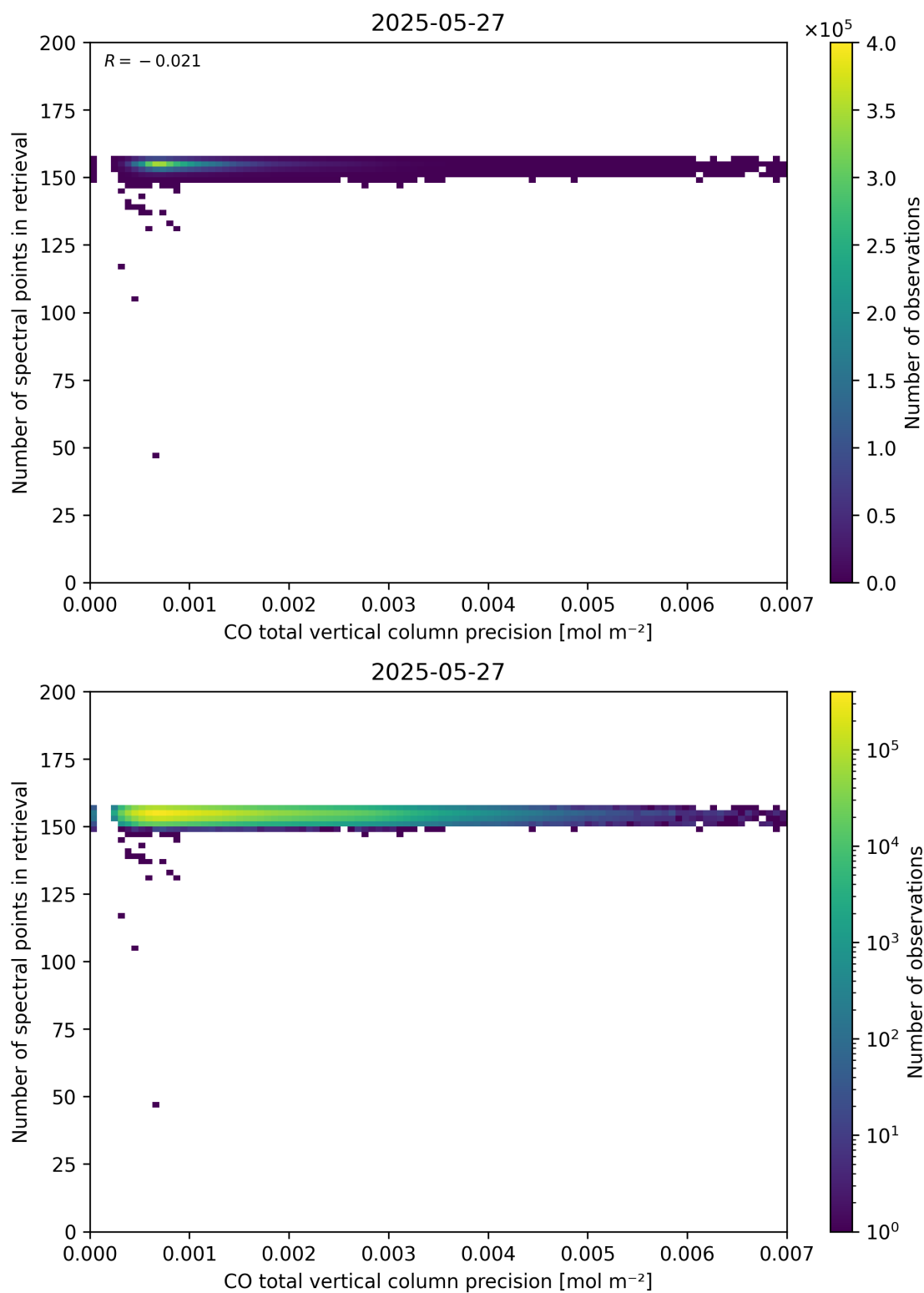
Figure 47: Scatter density plot of “CO total vertical column precision” against “Number of spectral points in retrieval” for 2025-05-26 to 2025-05-28.
