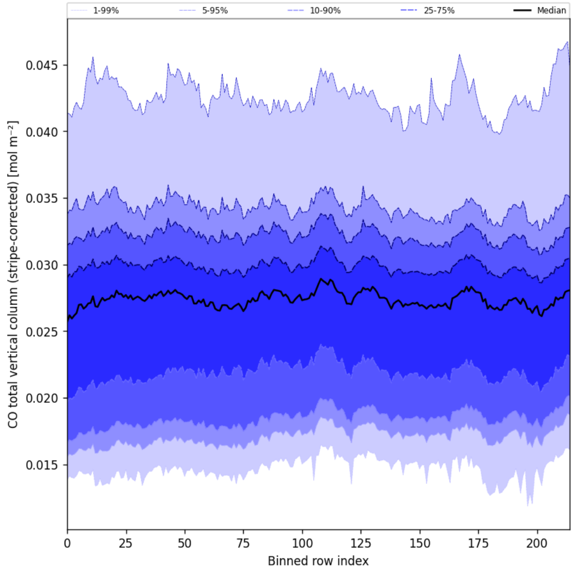
Figure 27: Along track statistics of “CO total vertical column (stripe-corrected)” for 2025-05-26 to 2025-05-28
