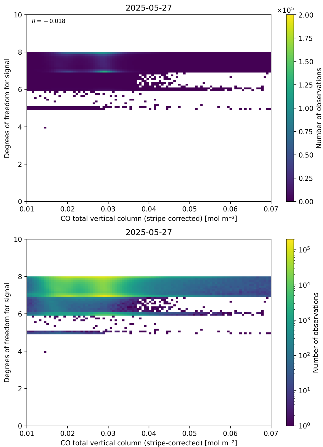
Figure 38: Scatter density plot of “CO total vertical column (stripe-corrected)” against “Degrees of freedom for signal” for 2025-05-26 to 2025-05-28.
