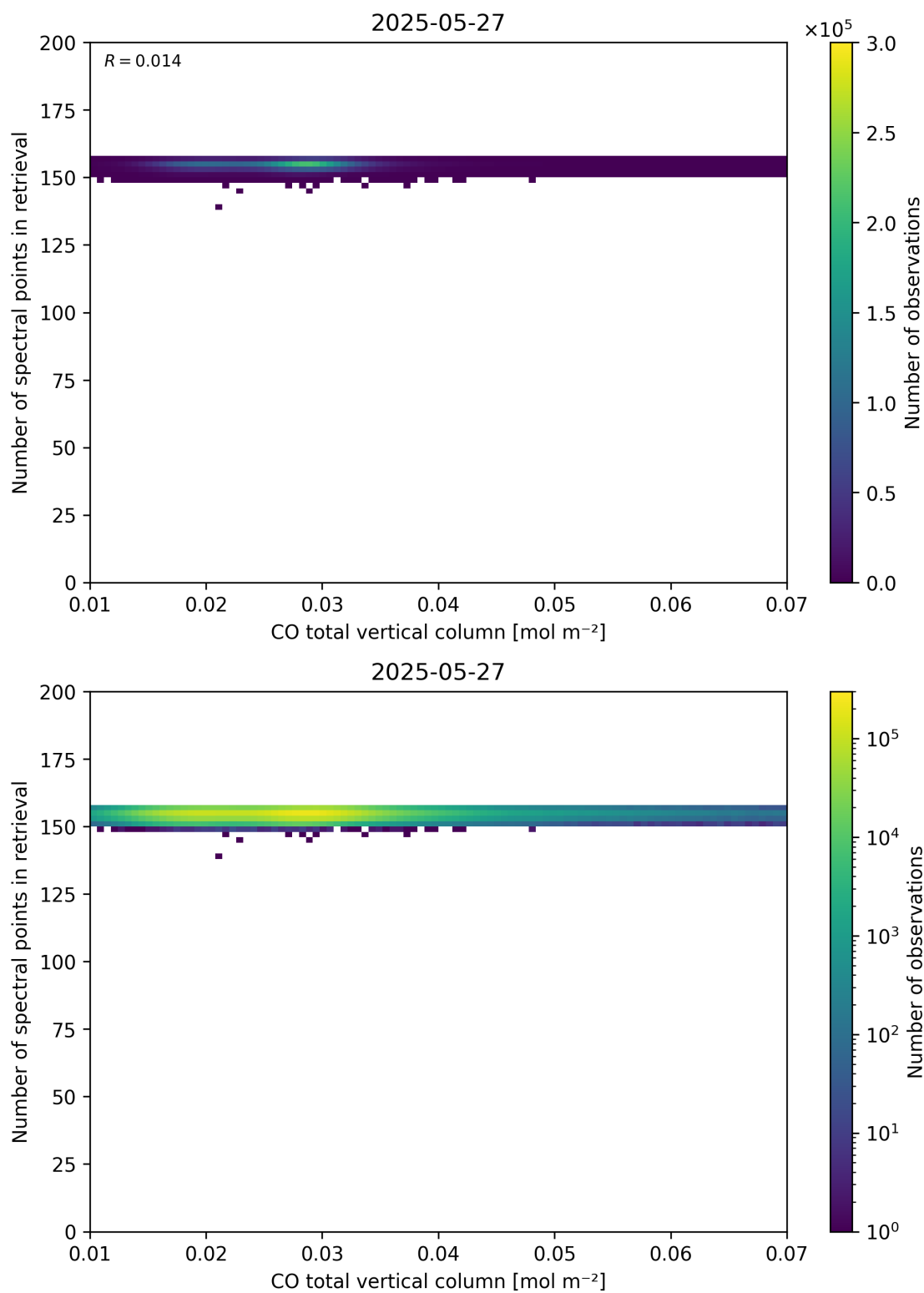
Figure 43: Scatter density plot of “CO total vertical column” against “Number of spectral points in retrieval” for 2025-05-26 to 2025-05-28.
