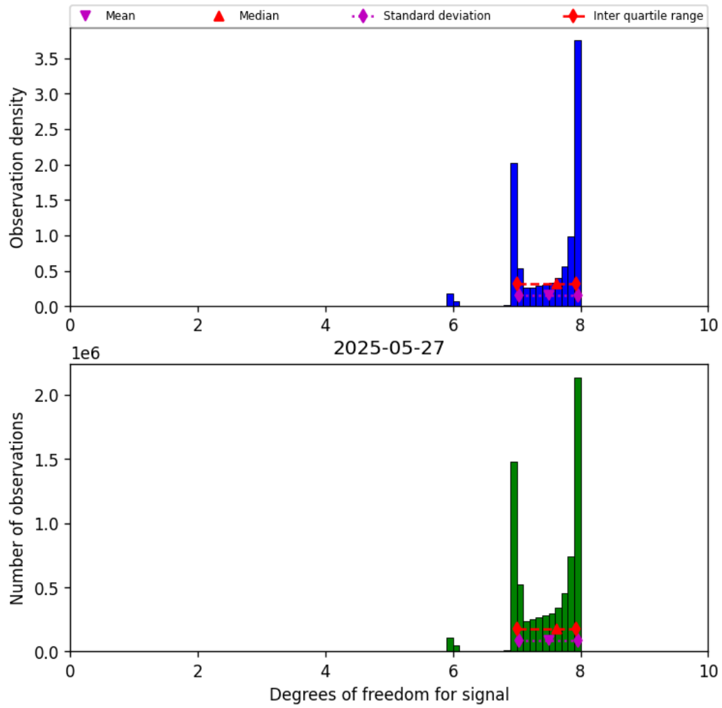
Figure 23: Histogram of “Degrees of freedom for signal” for 2025-05-26 to 2025-05-28
