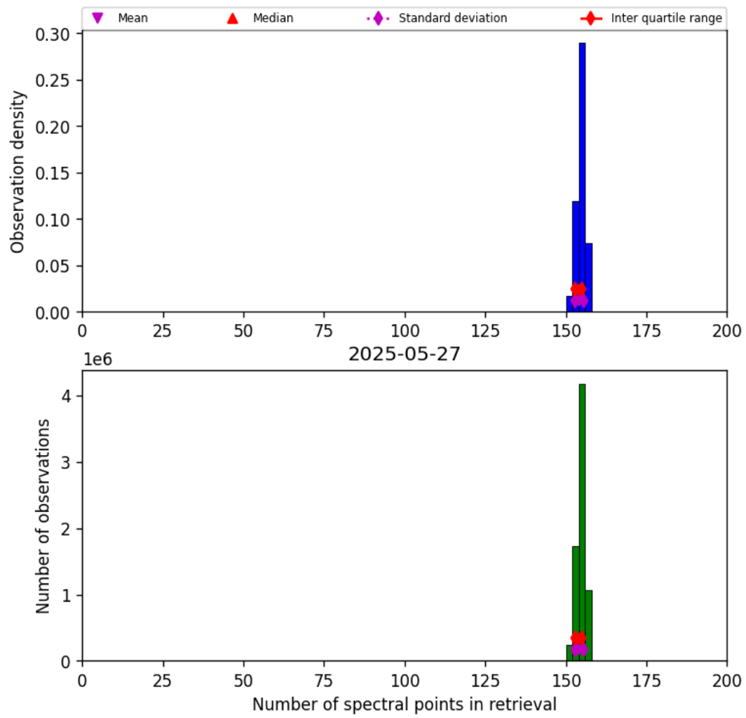
Figure 21: Histogram of “Number of spectral points in retrieval” for 2025-05-26 to 2025-05-28
