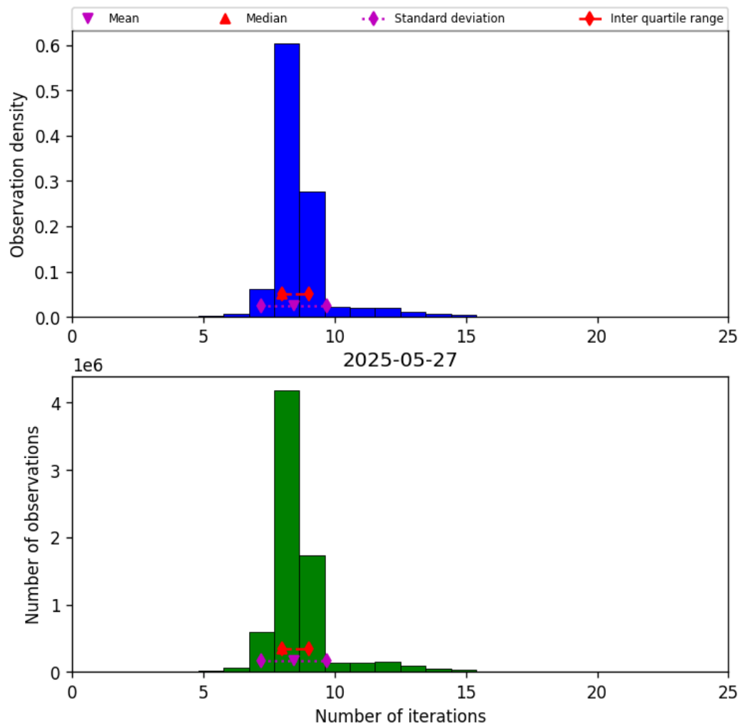
Figure 24: Histogram of “Number of iterations” for 2025-05-26 to 2025-05-28
