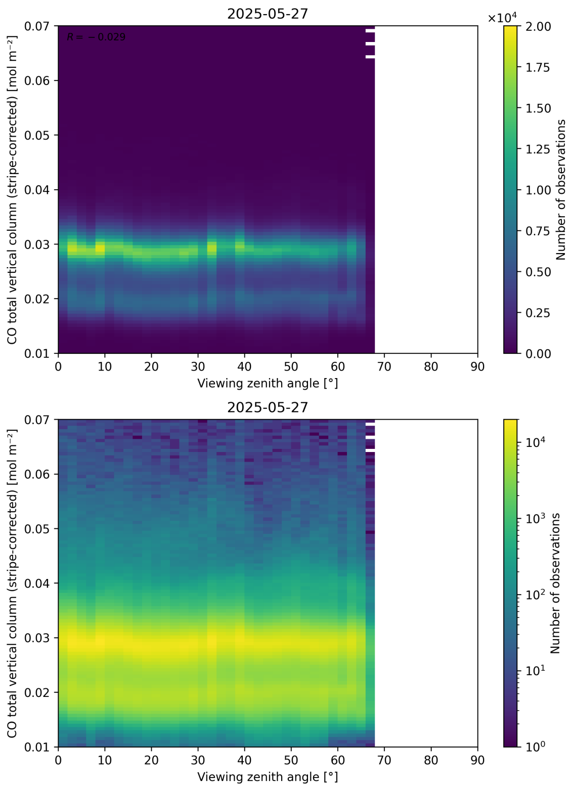
Figure 70: Scatter density plot of “Viewing zenith angle” against “CO total vertical column (stripe-corrected)” for 2025-05-26 to 2025-05-28.
