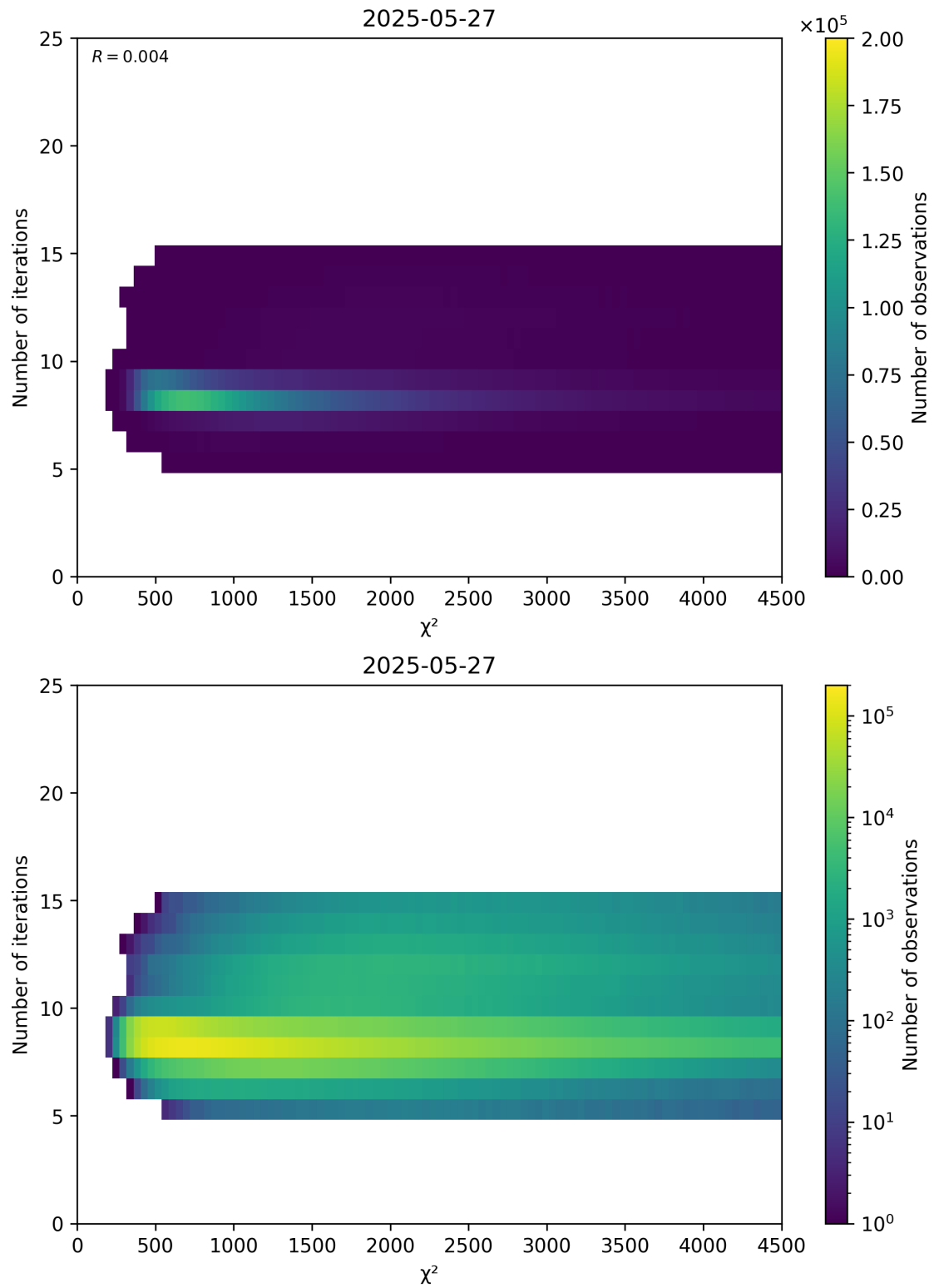
Figure 49: Scatter density plot of “ \chi^2 ” against “Number of iterations” for 2025-05-26 to 2025-05-28.
