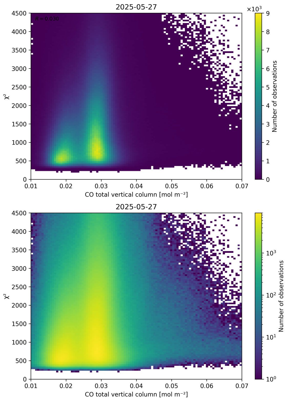
Figure 35: Scatter density plot of “CO total vertical column” against “ \chi^2 ” for 2025-05-26 to 2025-05-28.
