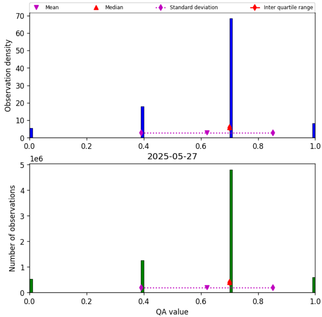
Figure 17: Histogram of “QA value” for 2025-05-26 to 2025-05-28
