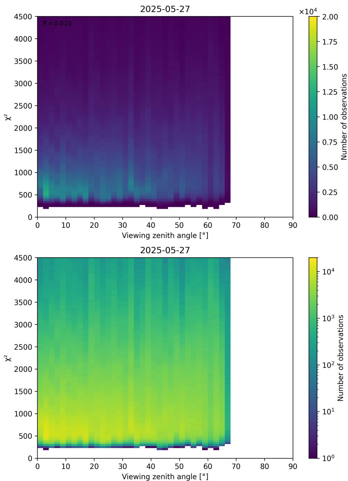
Figure 72: Scatter density plot of “Viewing zenith angle” against “ \chi^2 ” for 2025-05-26 to 2025-05-28.
