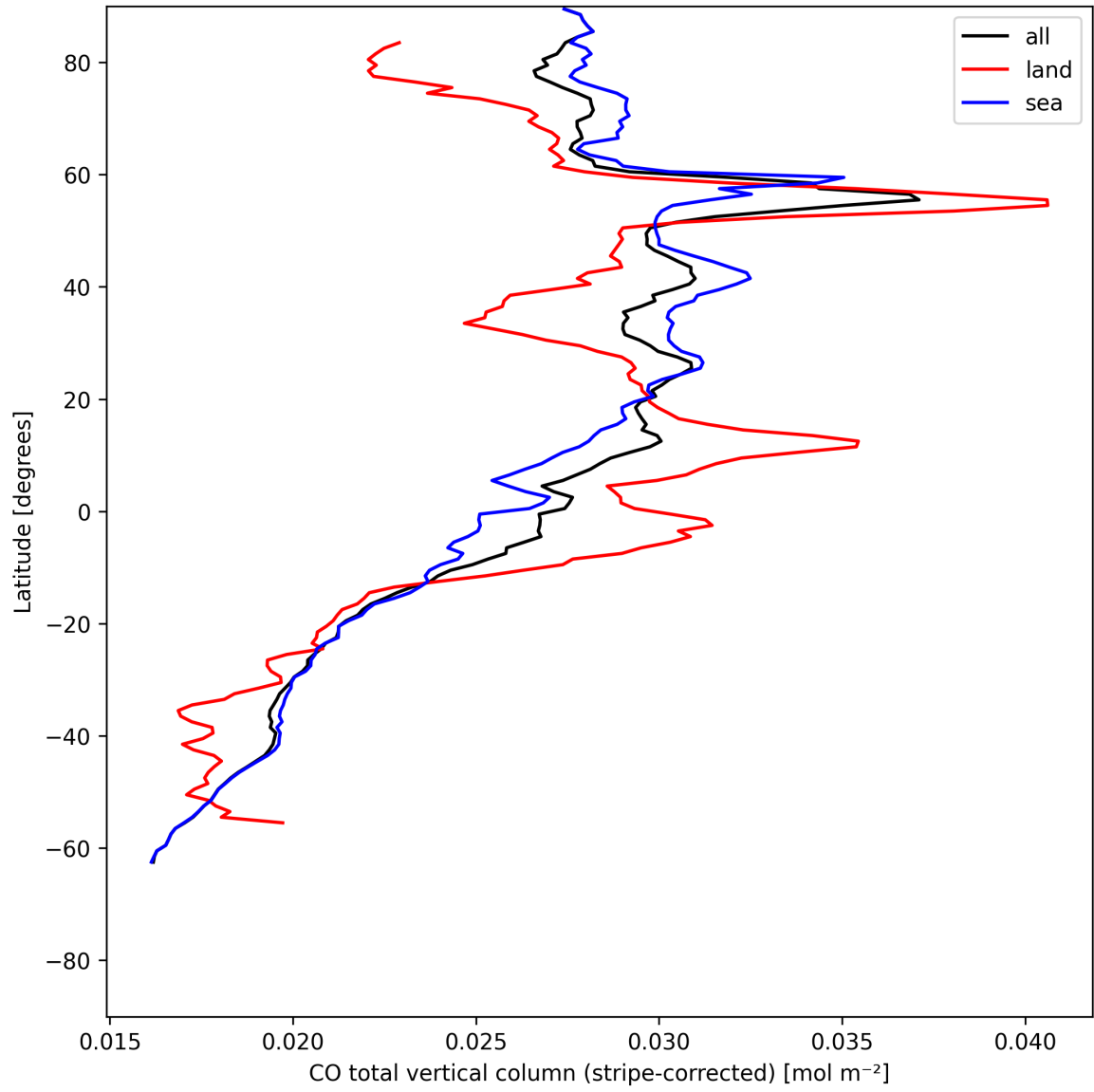
Figure 11: Zonal average of “CO total vertical column (stripe-corrected)” for 2025-05-26 to 2025-05-28.
