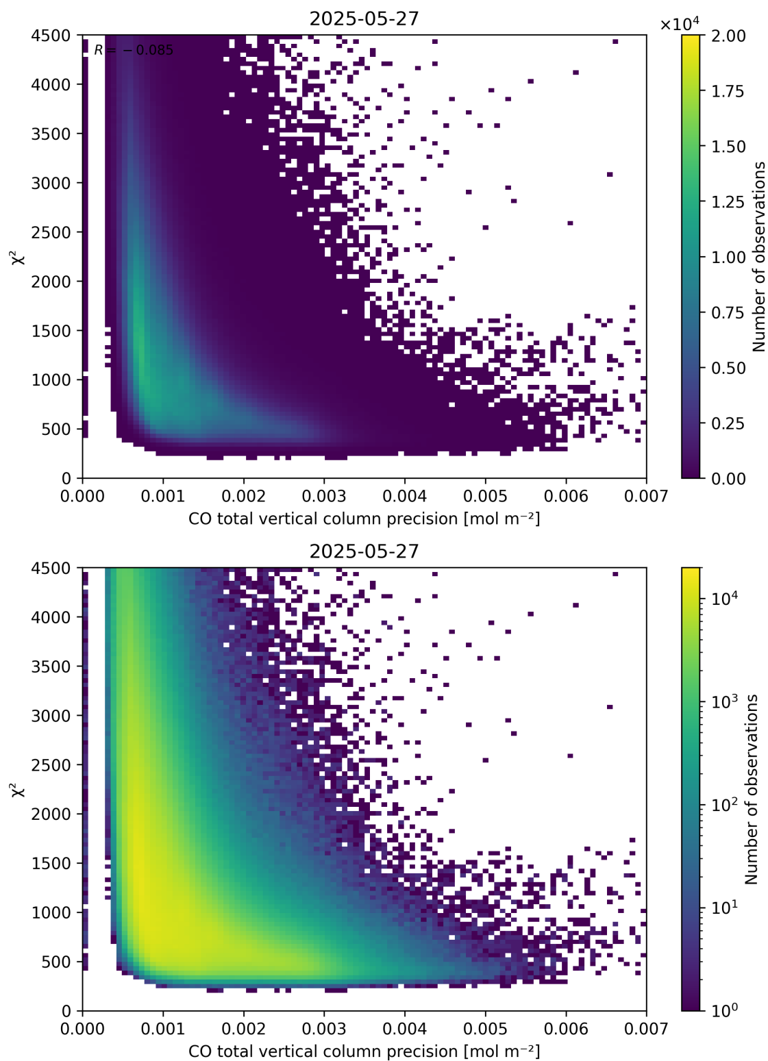
Figure 44: Scatter density plot of “CO total vertical column precision” against “ \chi^2 ” for 2025-05-26 to 2025-05-28.
