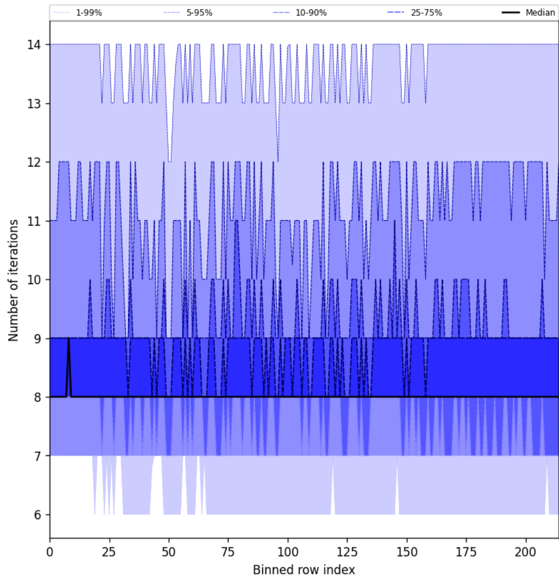
Figure 32: Along track statistics of “Number of iterations” for 2025-05-26 to 2025-05-28
