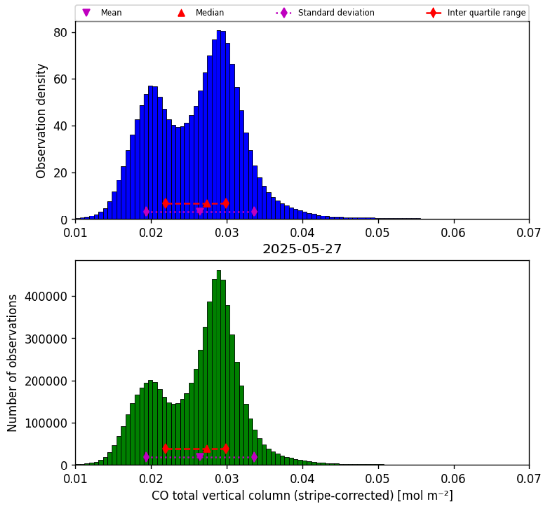
Figure 19: Histogram of “CO total vertical column (stripe-corrected)” for 2025-05-26 to 2025-05-28
