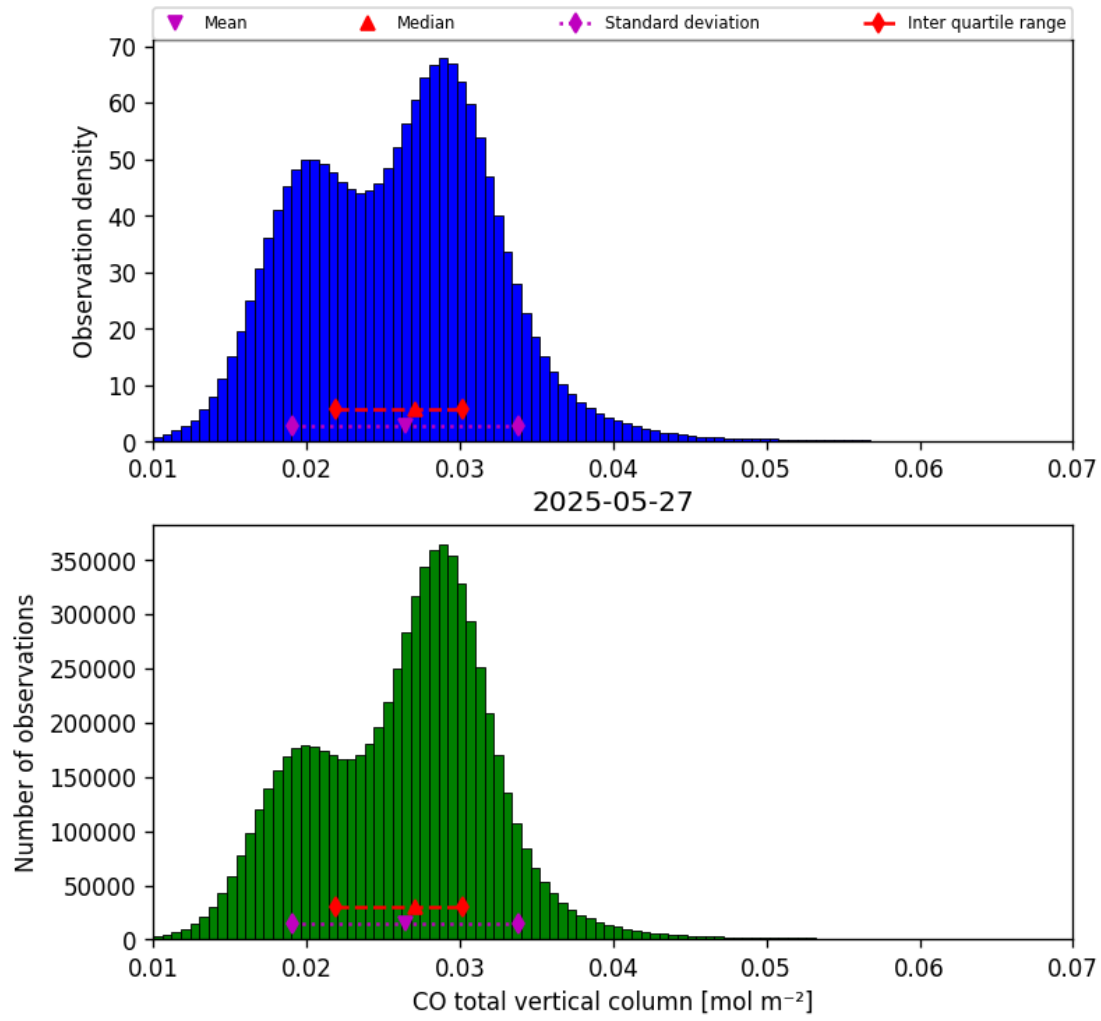
Figure 18: Histogram of “CO total vertical column” for 2025-05-26 to 2025-05-28
