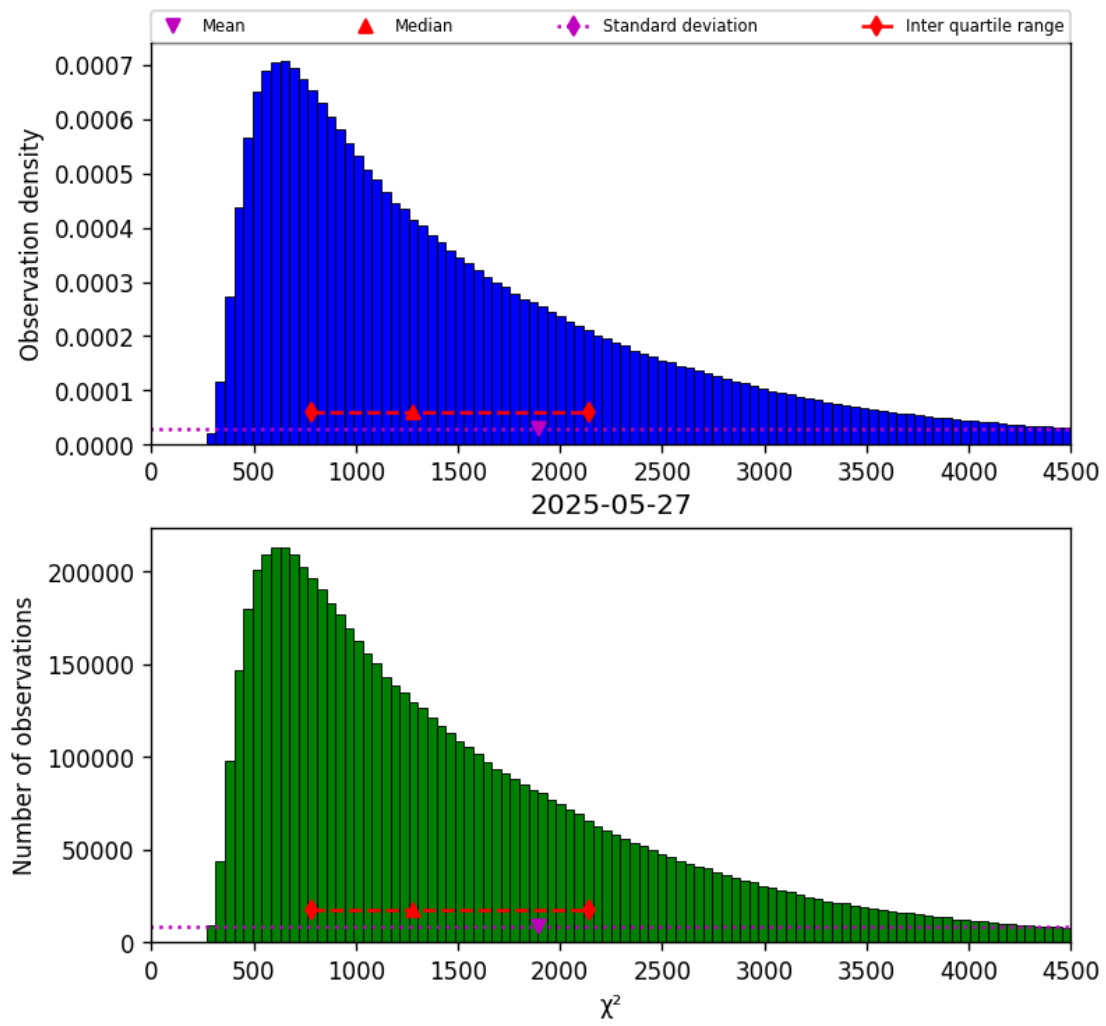
Figure 22: Histogram of “ \chi^2 ” for 2025-05-26 to 2025-05-28
