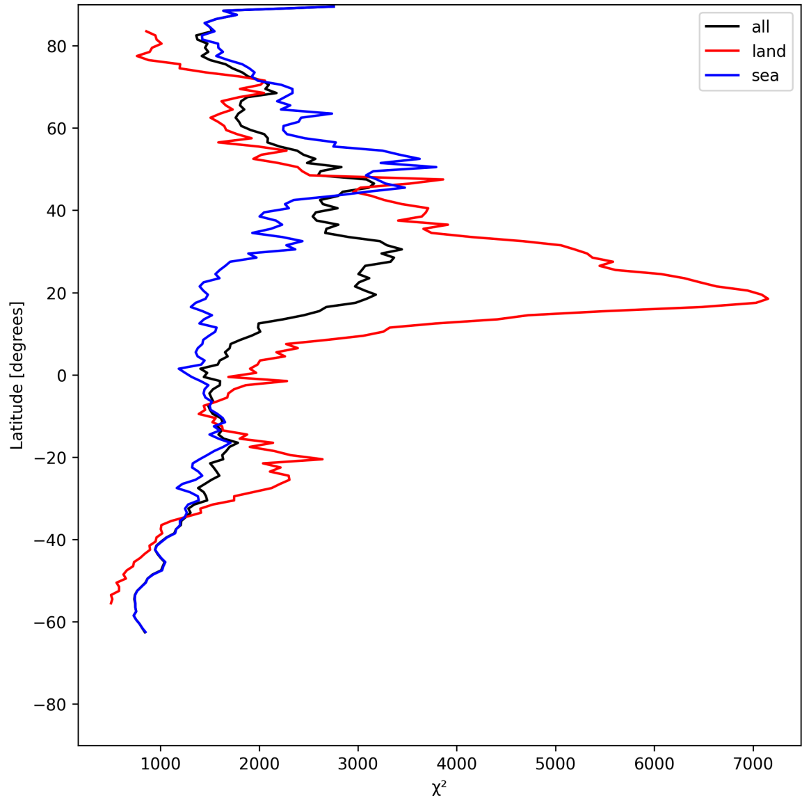
Figure 14: Zonal average of “ \chi^2 ” for 2025-05-26 to 2025-05-28.
