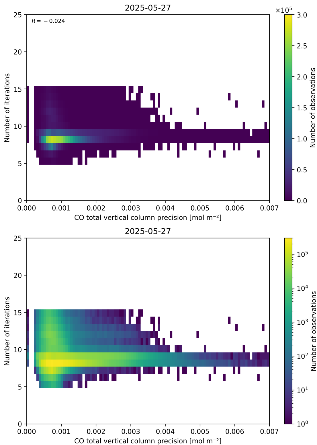
Figure 46: Scatter density plot of “CO total vertical column precision” against “Number of iterations” for 2025-05-26 to 2025-05-28.
