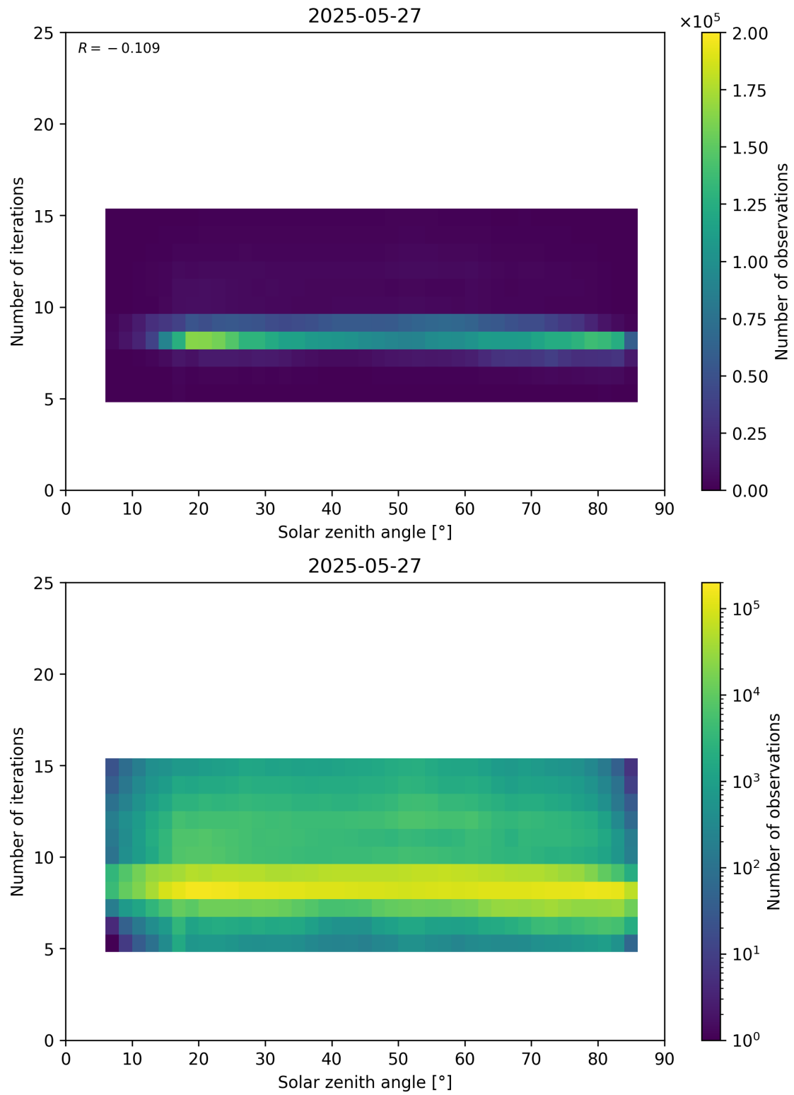
Figure 67: Scatter density plot of “Solar zenith angle” against “Number of iterations” for 2025-05-26 to 2025-05-28.
