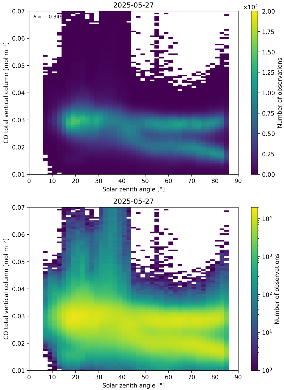
Figure 61: Scatter density plot of “Solar zenith angle” against “CO total vertical column” for 2025-05-26 to 2025-05-28.
