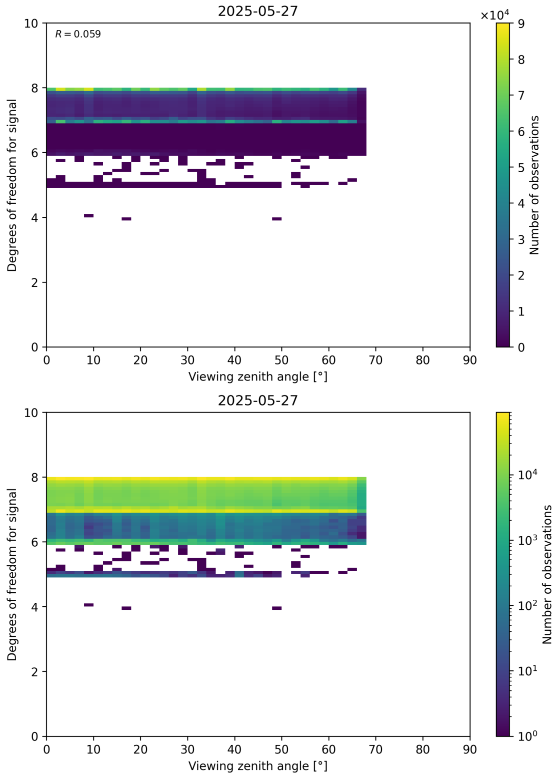
Figure 73: Scatter density plot of “Viewing zenith angle” against “Degrees of freedom for signal” for 2025-05-26 to 2025-05-28.
