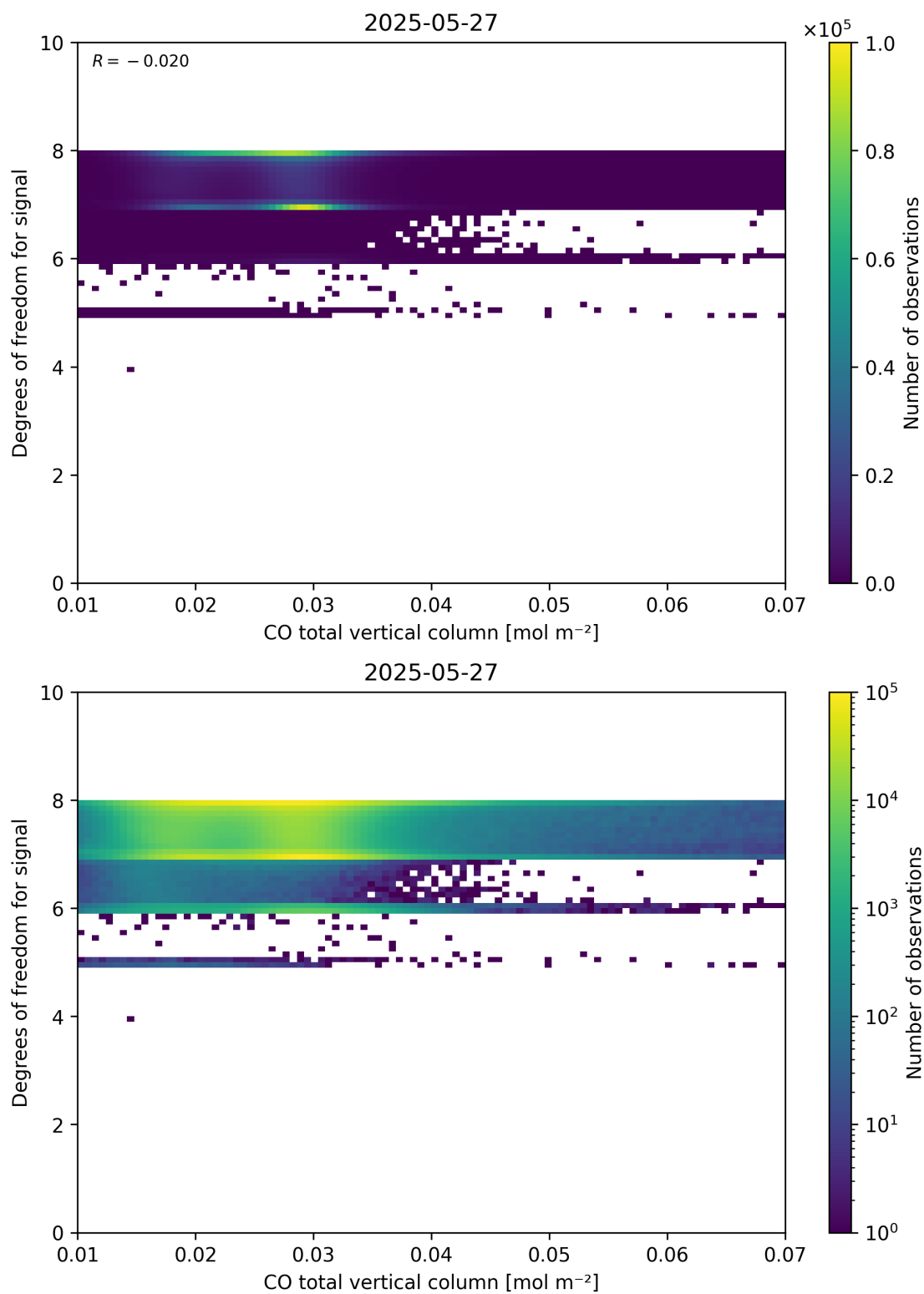
Figure 41: Scatter density plot of “CO total vertical column” against “Degrees of freedom for signal” for 2025-05-26 to 2025-05-28.
