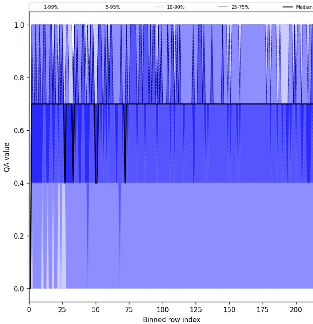
Figure 25: Along track statistics of “QA value” for 2025-05-26 to 2025-05-28
