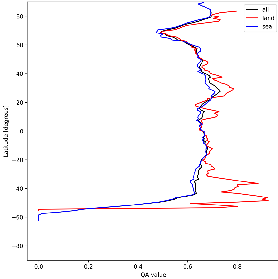
Figure 9: Zonal average of “QA value” for 2025-05-26 to 2025-05-28.
