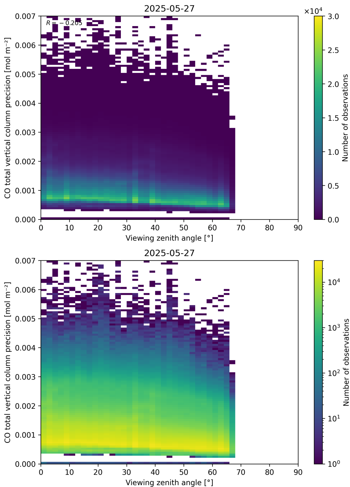
Figure 71: Scatter density plot of “Viewing zenith angle” against “CO total vertical column precision” for 2025-05-26 to 2025-05-28.
