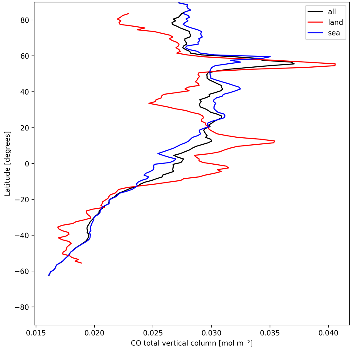
Figure 10: Zonal average of “CO total vertical column” for 2025-05-26 to 2025-05-28.
