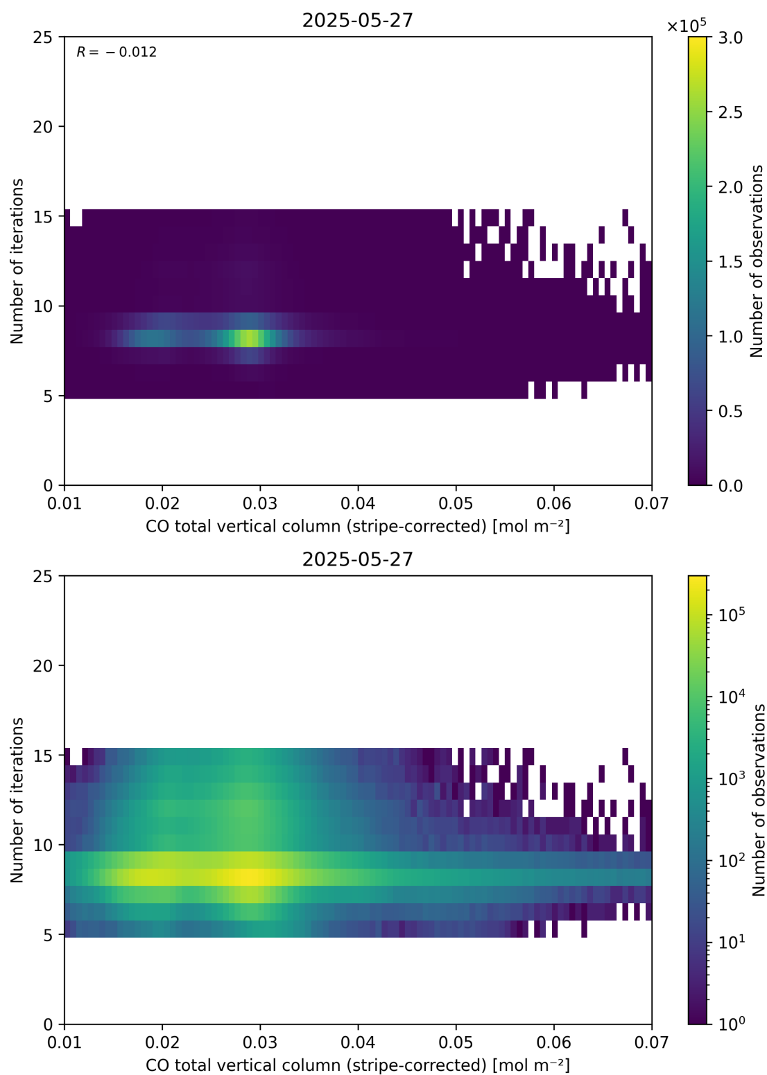
Figure 39: Scatter density plot of “CO total vertical column (stripe-corrected)” against “Number of iterations” for 2025-05-26 to 2025-05-28.
