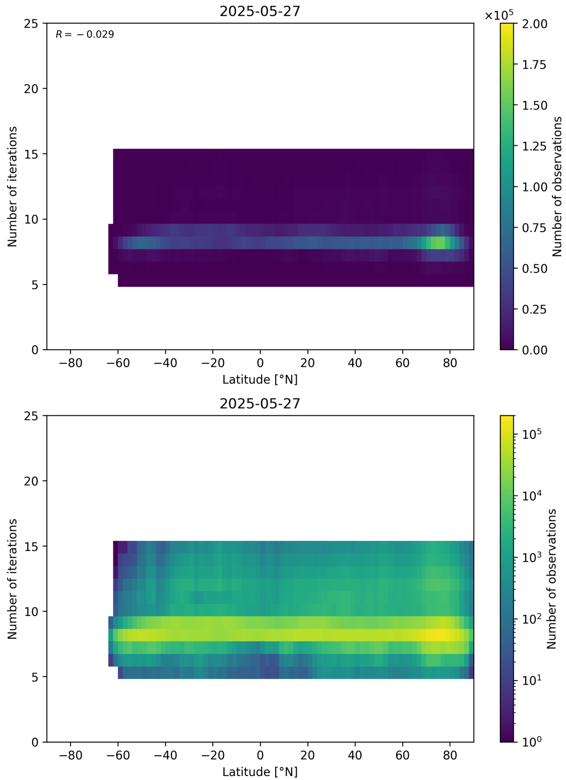
Figure 56: Scatter density plot of “Latitude” against “Number of iterations” for 2025-05-26 to 2025-05-28.
