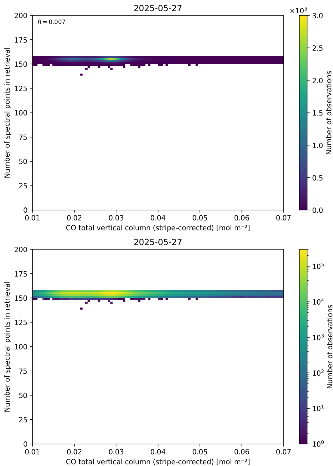
Figure 40: Scatter density plot of “CO total vertical column (stripe-corrected)” against “Number of spectral points in retrieval” for 2025-05-26 to 2025-05-28.
