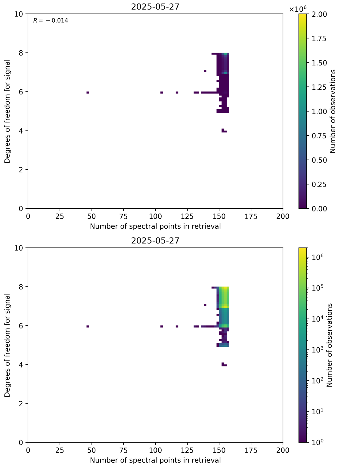
Figure 59: Scatter density plot of “Number of spectral points in retrieval” against “Degrees of freedom for signal” for 2025-05-26 to 2025-05-28.
