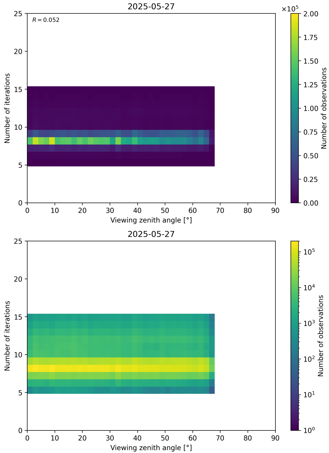
Figure 75: Scatter density plot of “Viewing zenith angle” against “Number of iterations” for 2025-05-26 to 2025-05-28.
