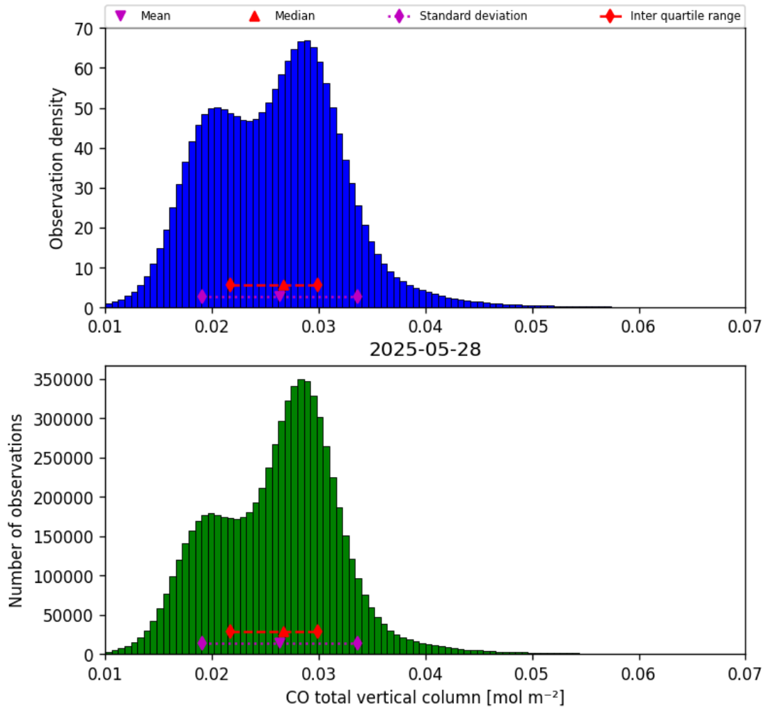
Figure 18: Histogram of “CO total vertical column” for 2025-05-27 to 2025-05-29
