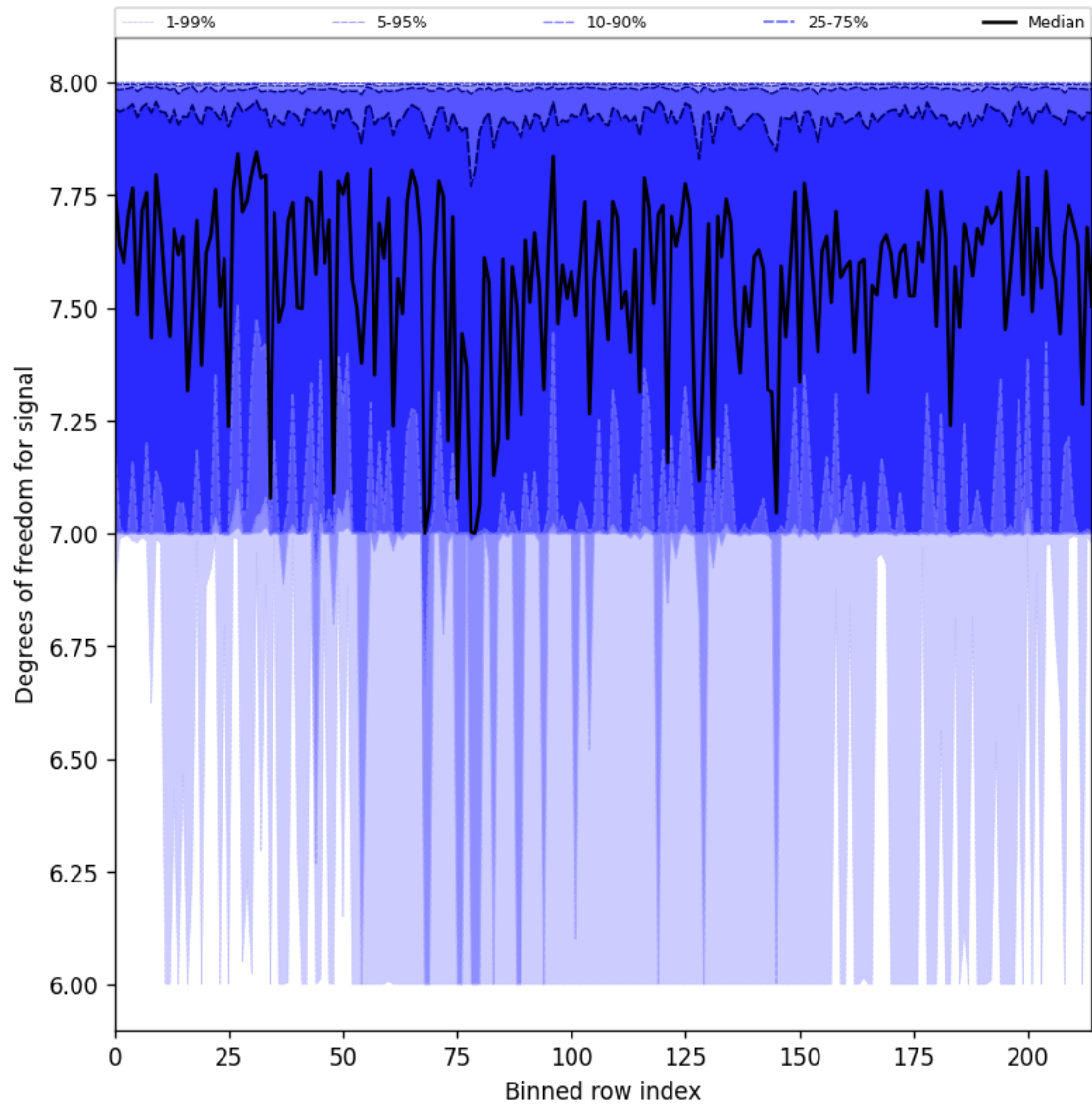
Figure 31: Along track statistics of “Degrees of freedom for signal” for 2025-05-27 to 2025-05-29
