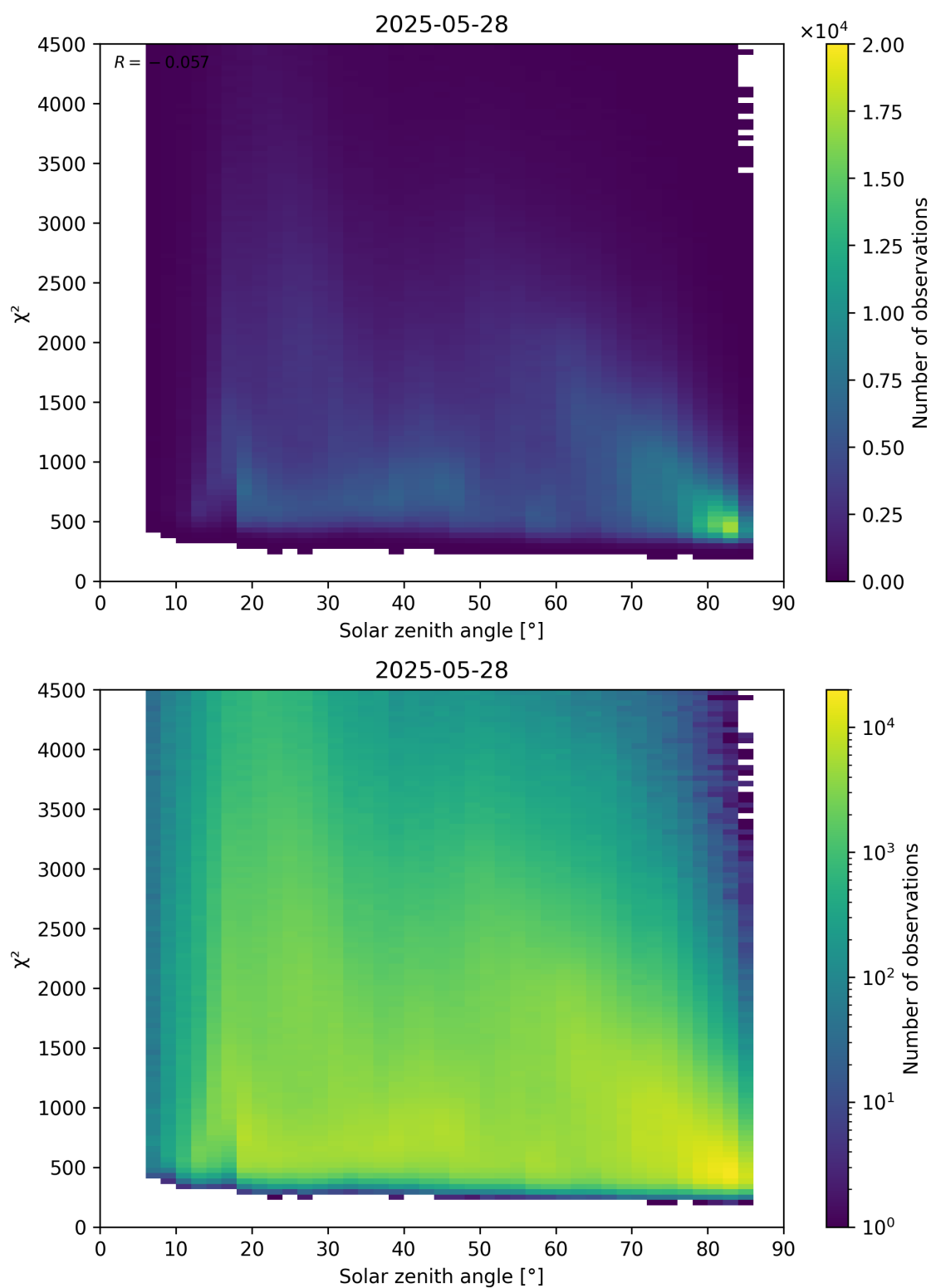
Figure 64: Scatter density plot of “Solar zenith angle” against “ \chi^2 ” for 2025-05-27 to 2025-05-29.
