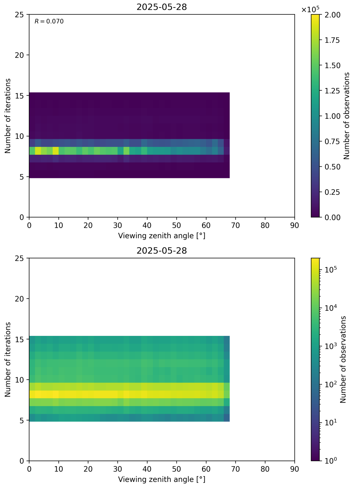
Figure 75: Scatter density plot of “Viewing zenith angle” against “Number of iterations” for 2025-05-27 to 2025-05-29.
