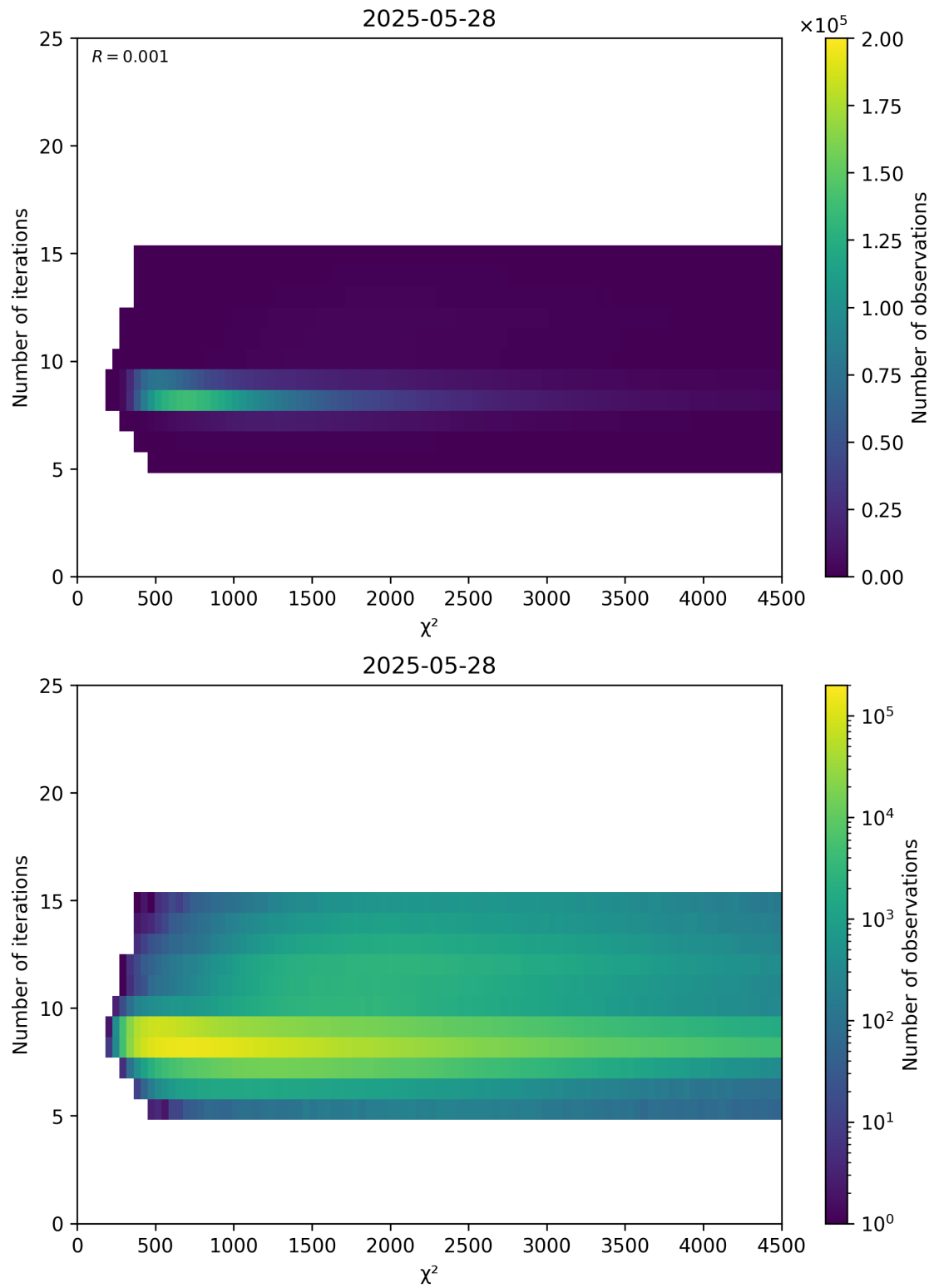
Figure 49: Scatter density plot of “ \chi^2 ” against “Number of iterations” for 2025-05-27 to 2025-05-29.
