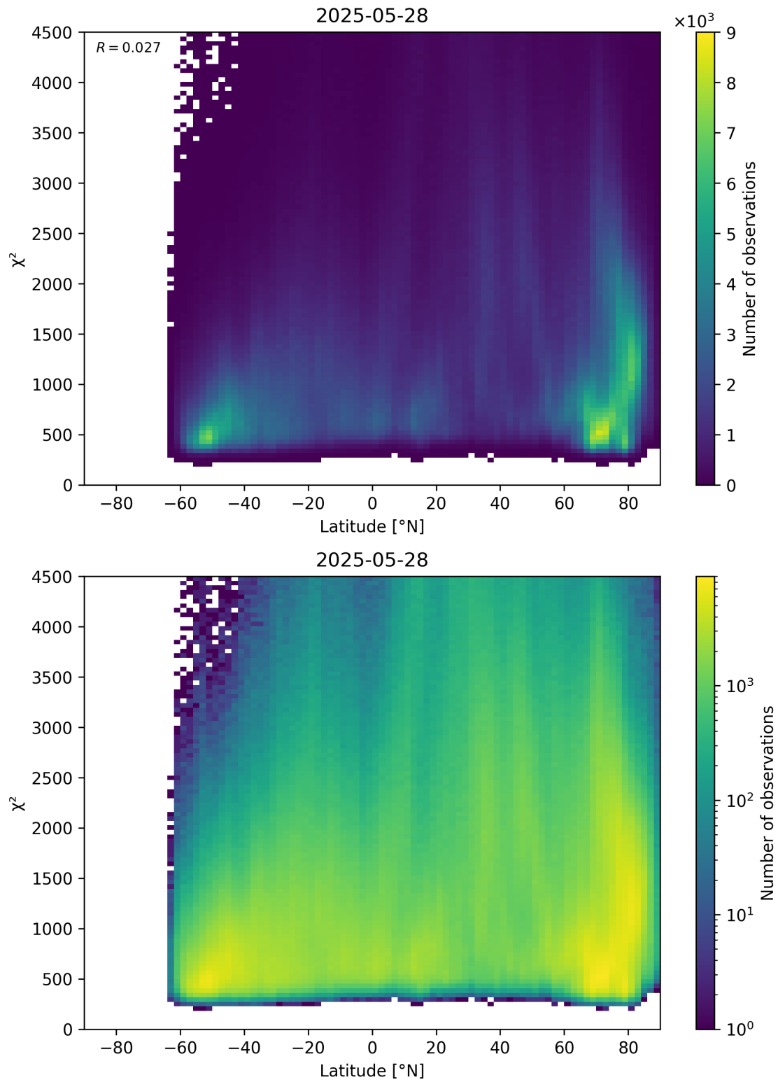
Figure 54: Scatter density plot of “Latitude” against “ \chi^2 ” for 2025-05-27 to 2025-05-29.
