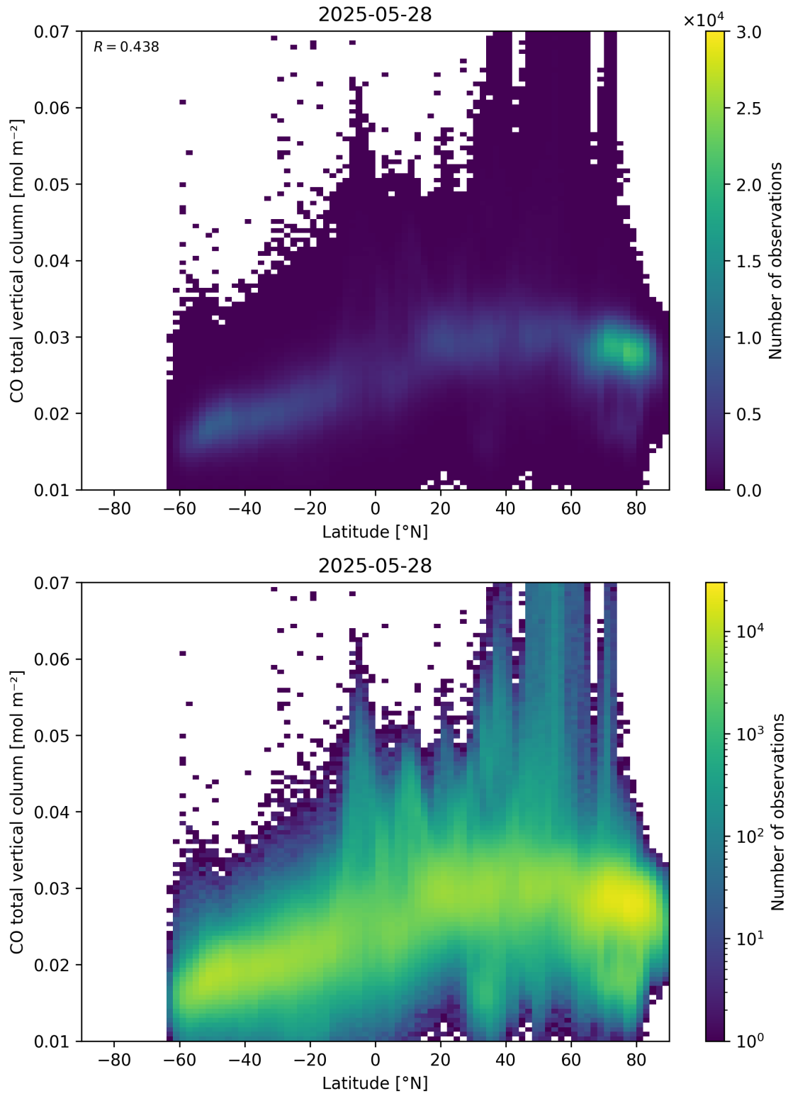
Figure 51: Scatter density plot of “Latitude” against “CO total vertical column” for 2025-05-27 to 2025-05-29.
