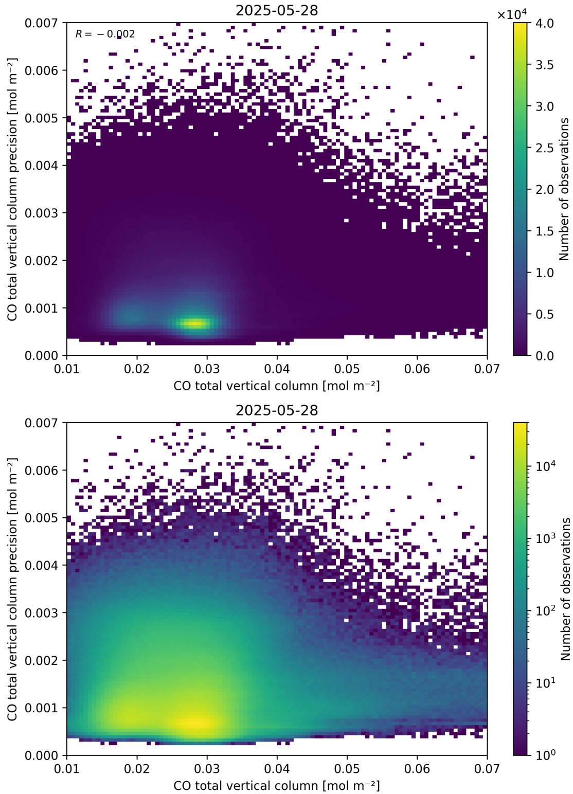
Figure 34: Scatter density plot of “CO total vertical column” against “CO total vertical column precision” for 2025-05-27 to 2025-05-29.
