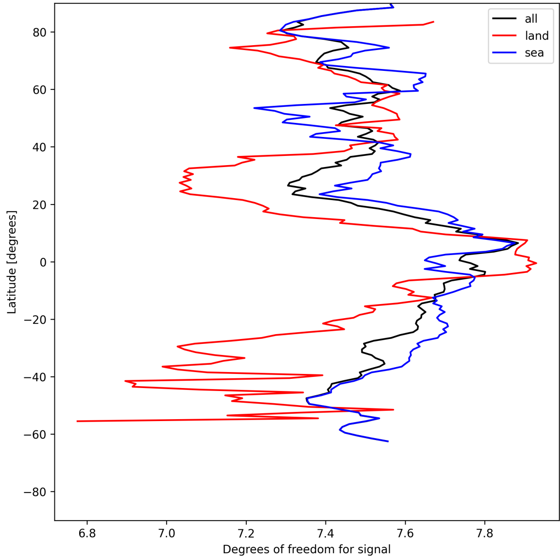
Figure 15: Zonal average of “Degrees of freedom for signal” for 2025-05-27 to 2025-05-29.
