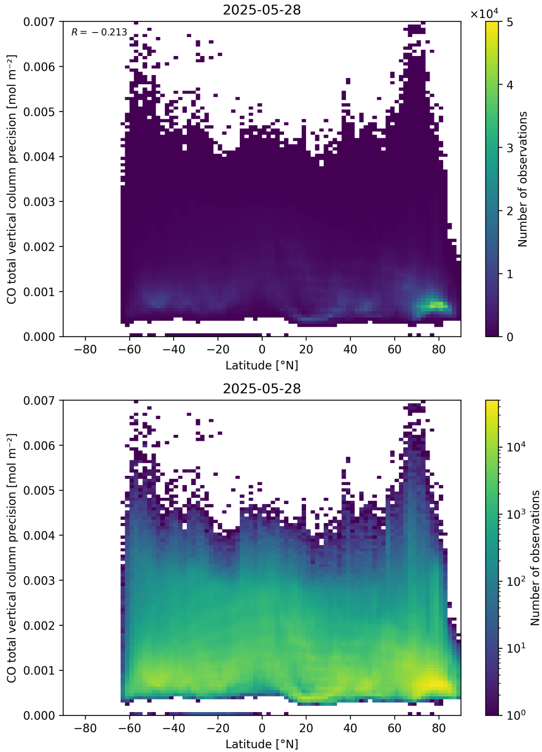
Figure 53: Scatter density plot of “Latitude” against “CO total vertical column precision” for 2025-05-27 to 2025-05-29.
