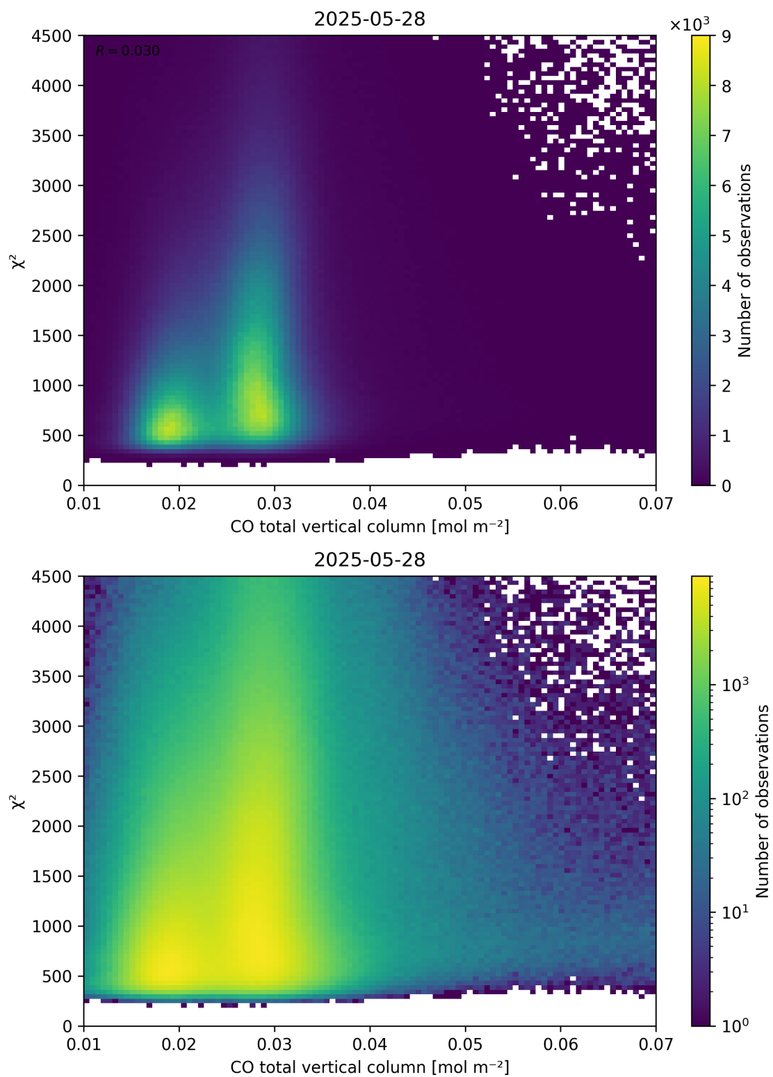
Figure 35: Scatter density plot of “CO total vertical column” against “ \chi^2 ” for 2025-05-27 to 2025-05-29.
