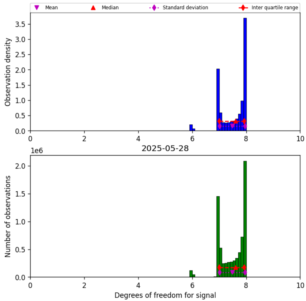
Figure 23: Histogram of “Degrees of freedom for signal” for 2025-05-27 to 2025-05-29
