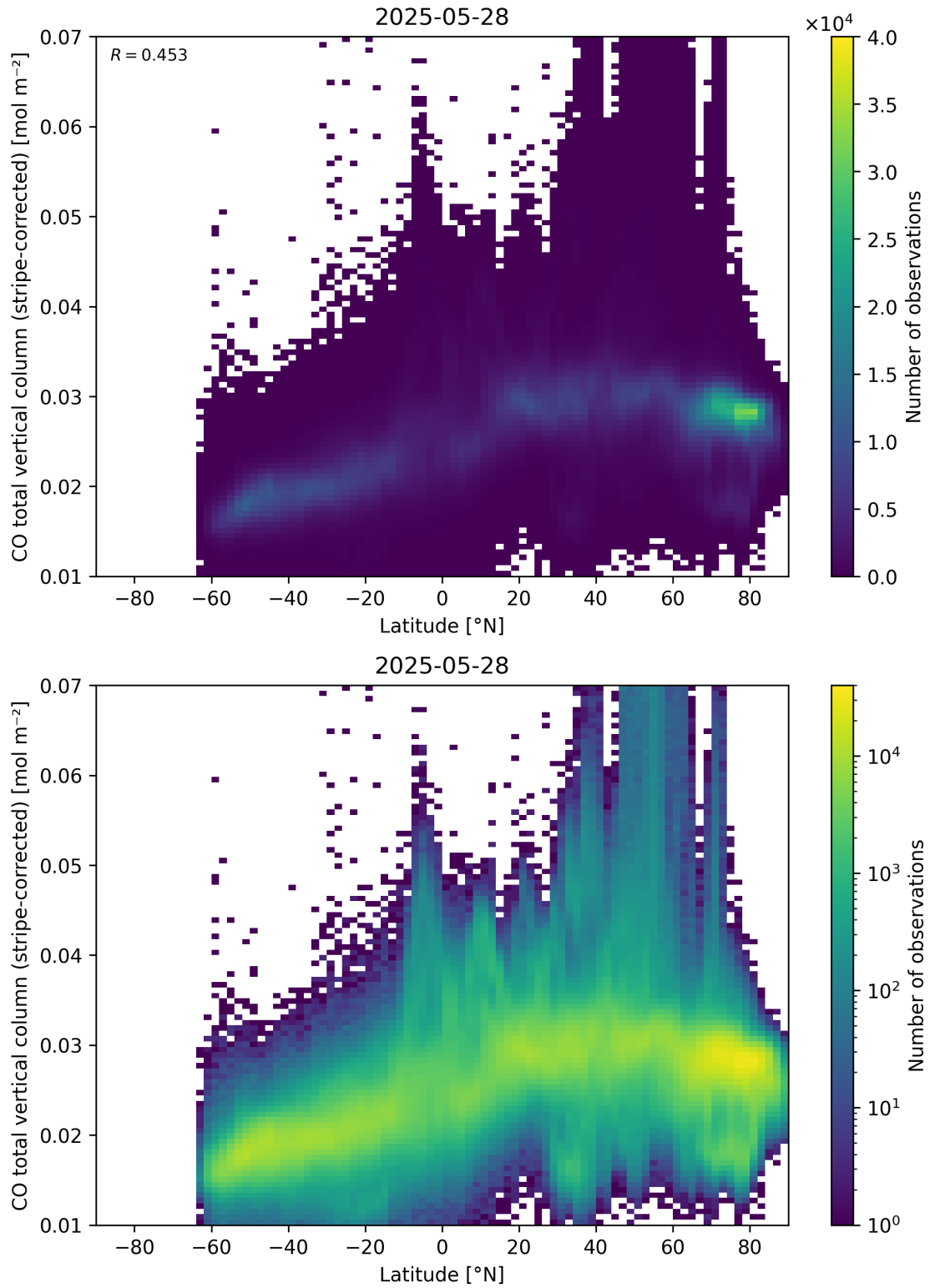
Figure 52: Scatter density plot of “Latitude” against “CO total vertical column (stripe-corrected)” for 2025-05-27 to 2025-05-29.
