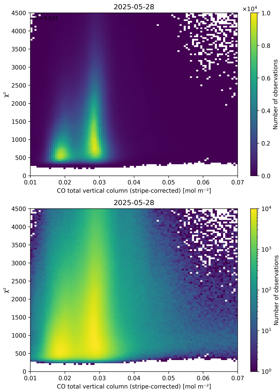
Figure 37: Scatter density plot of “CO total vertical column (stripe-corrected)” against “ \chi^2 ” for 2025-05-27 to 2025-05-29.
