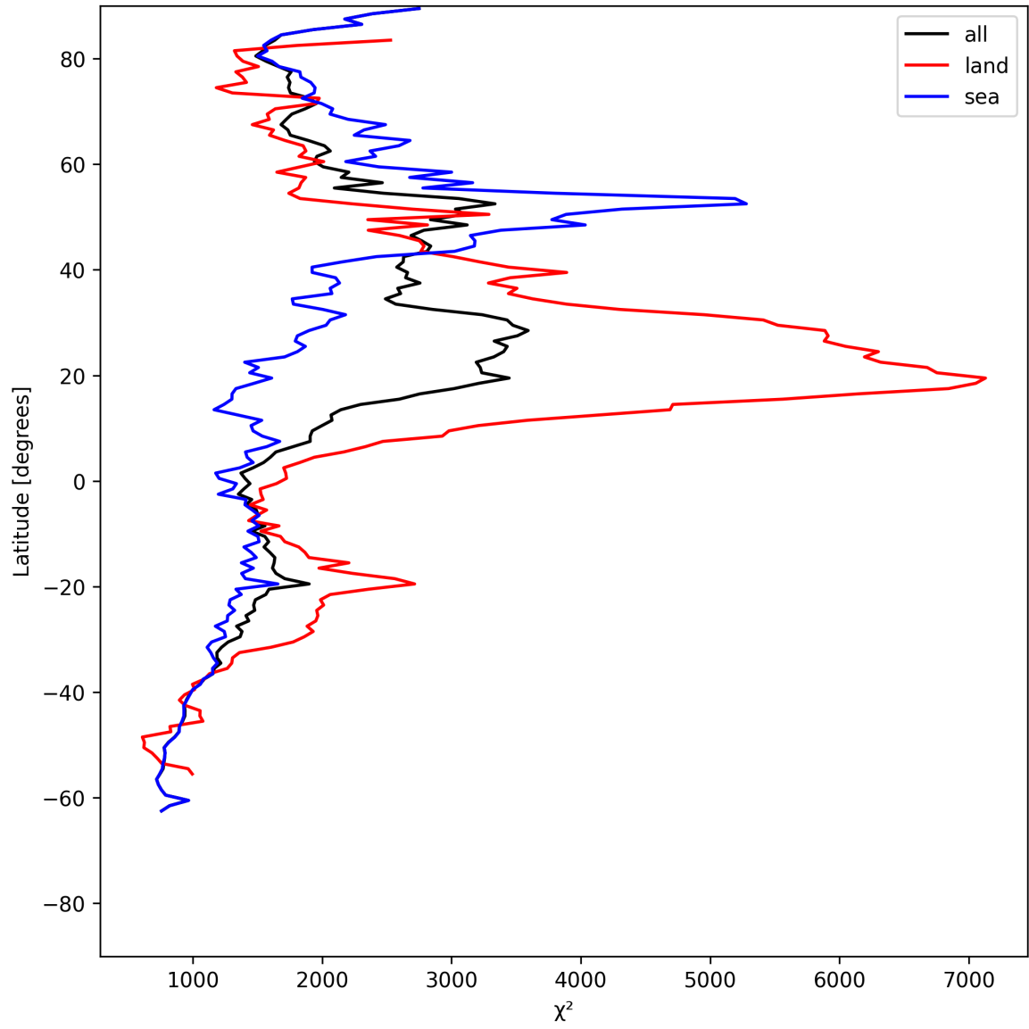
Figure 14: Zonal average of “ \chi^2 ” for 2025-05-27 to 2025-05-29.
