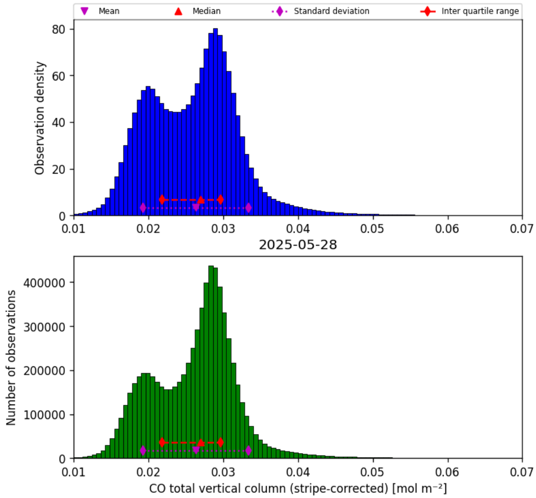
Figure 19: Histogram of “CO total vertical column (stripe-corrected)” for 2025-05-27 to 2025-05-29
