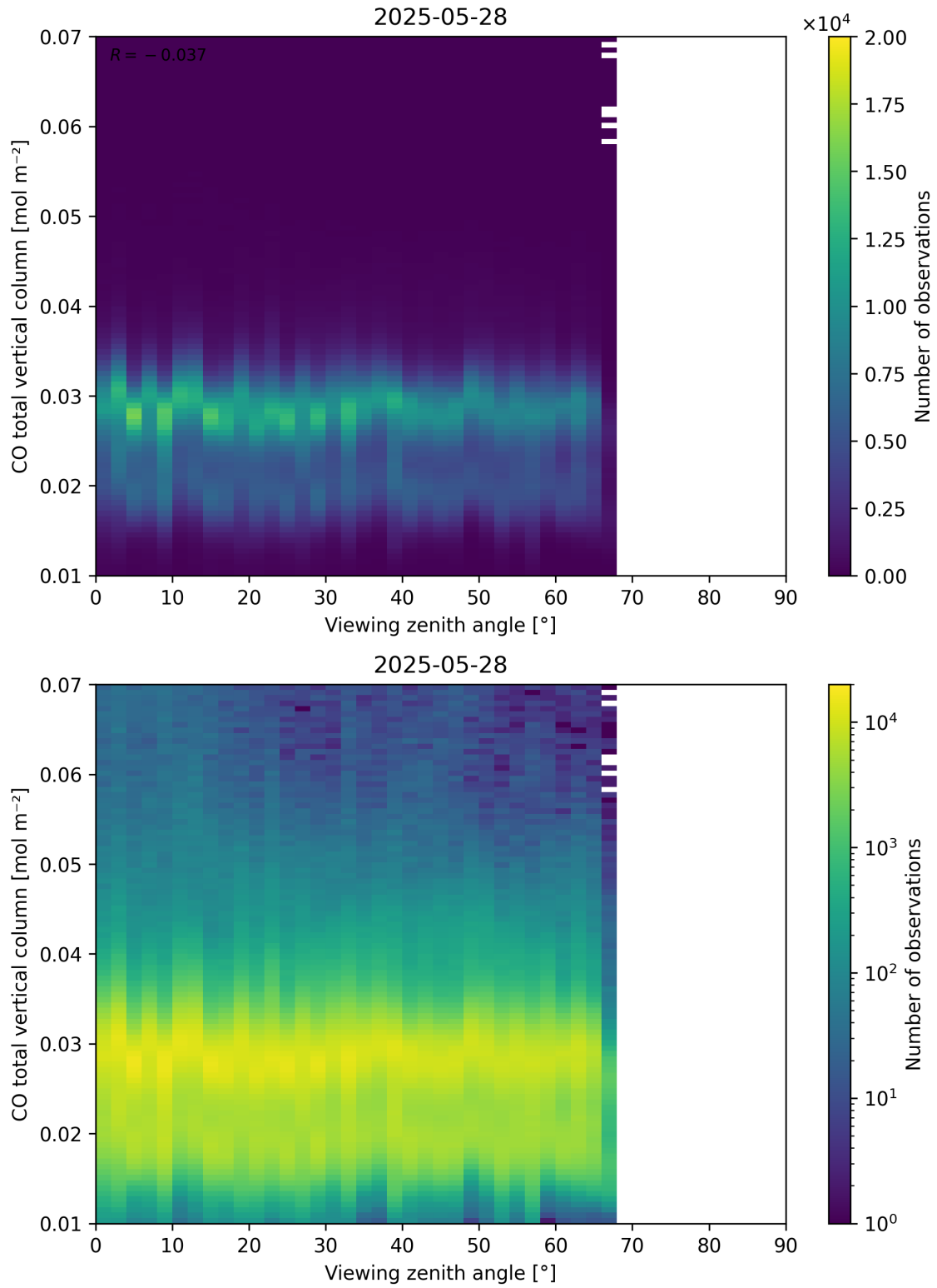
Figure 69: Scatter density plot of “Viewing zenith angle” against “CO total vertical column” for 2025-05-27 to 2025-05-29.
