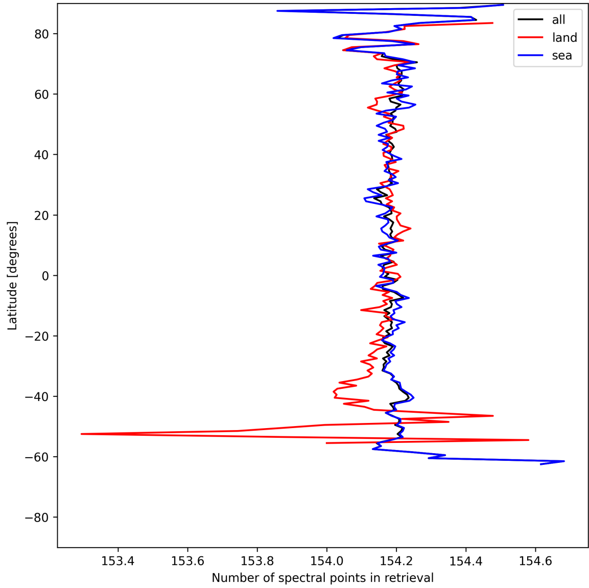
Figure 13: Zonal average of “Number of spectral points in retrieval” for 2025-05-27 to 2025-05-29.
