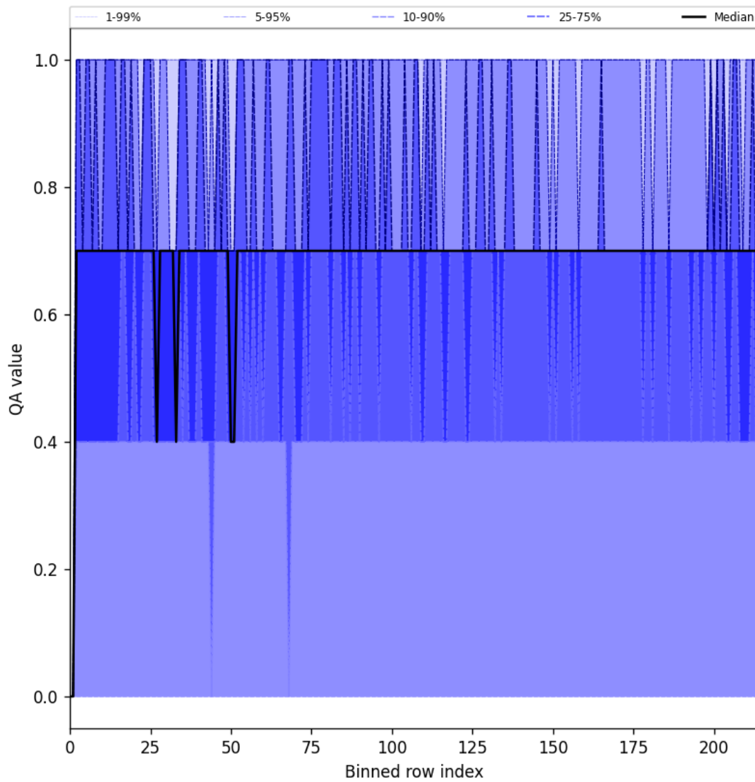
Figure 25: Along track statistics of “QA value” for 2025-05-27 to 2025-05-29
