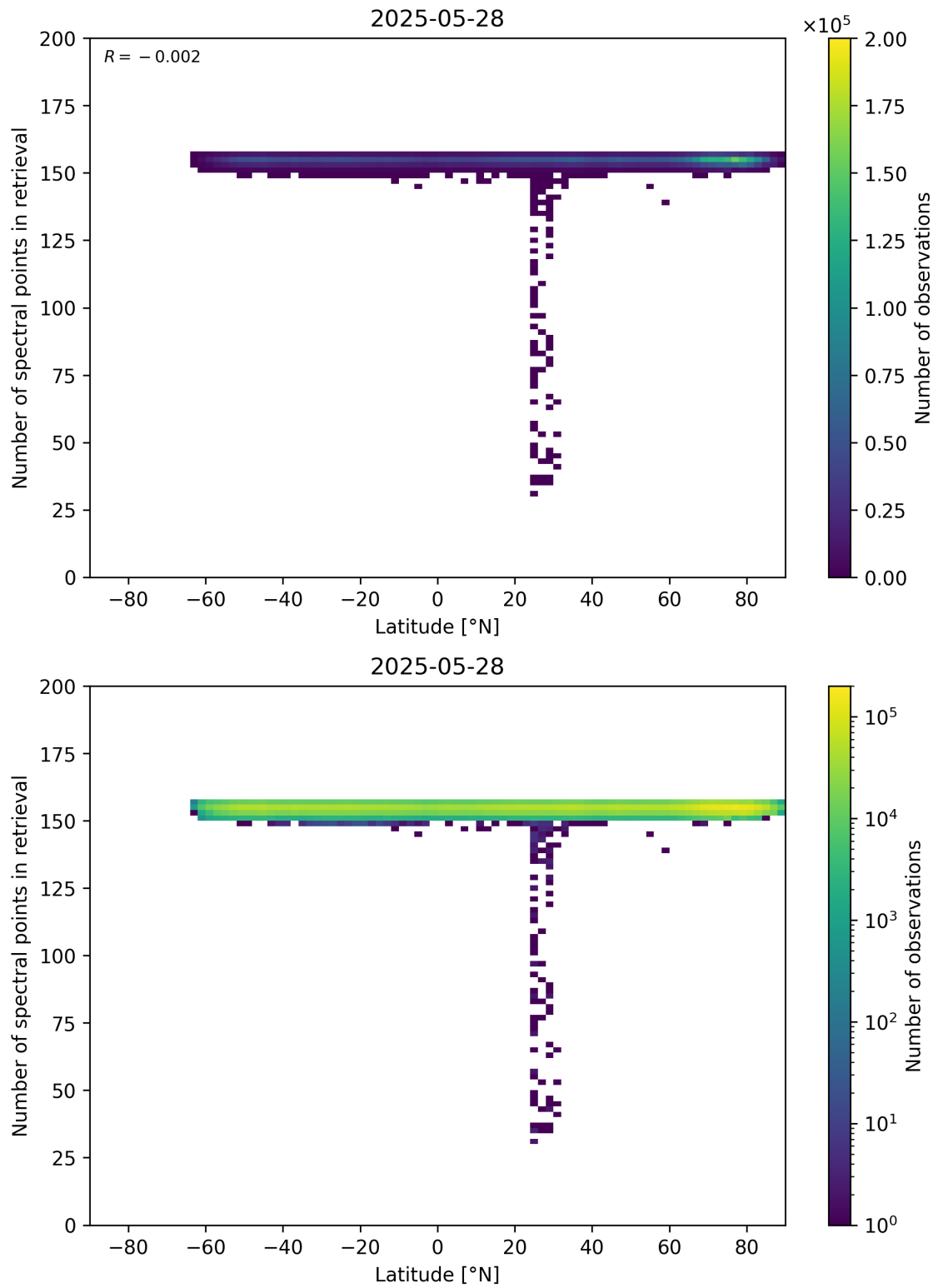
Figure 57: Scatter density plot of “Latitude” against “Number of spectral points in retrieval” for 2025-05-27 to 2025-05-29.
