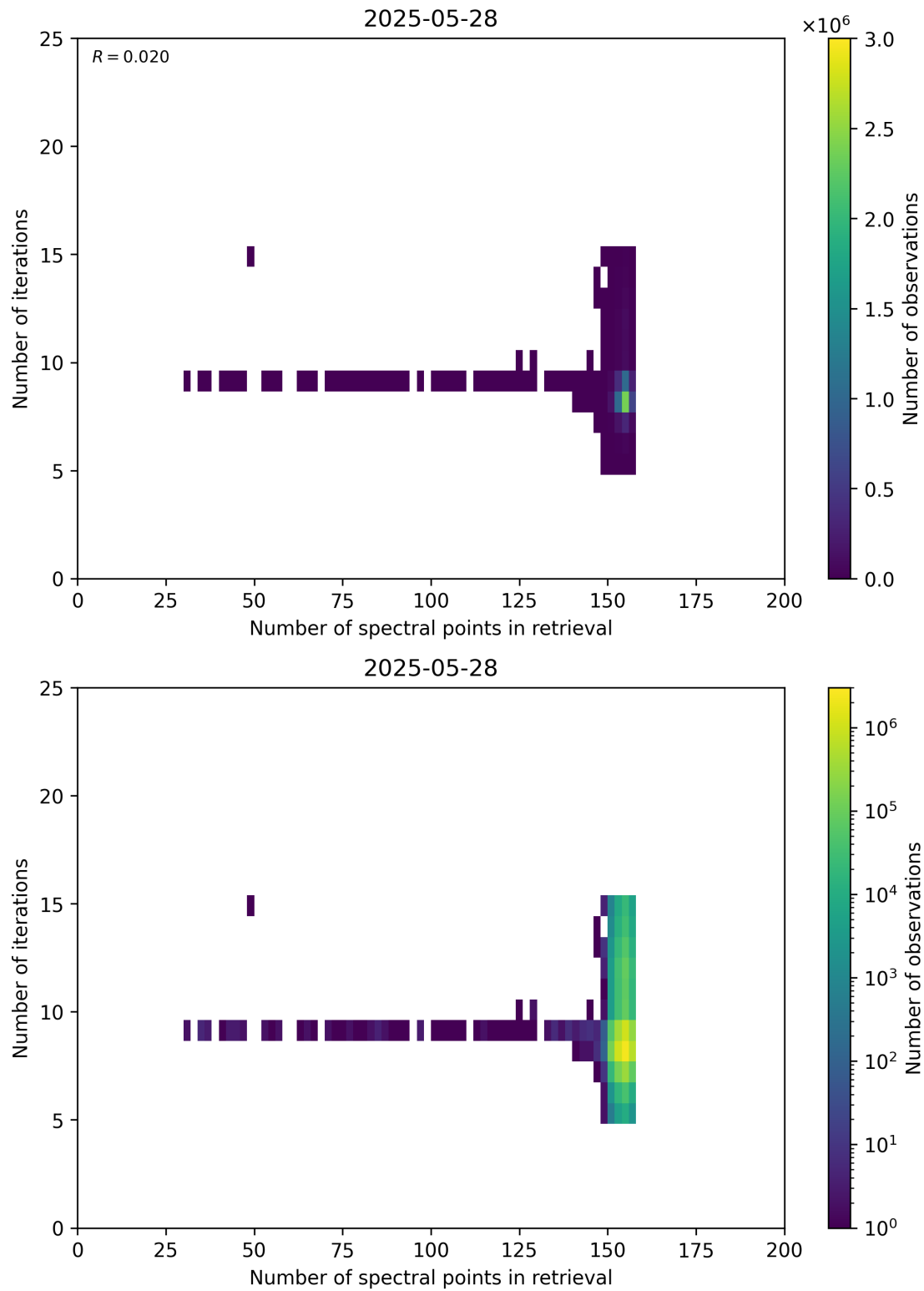
Figure 60: Scatter density plot of “Number of spectral points in retrieval” against “Number of iterations” for 2025-05-27 to 2025-05-29.
