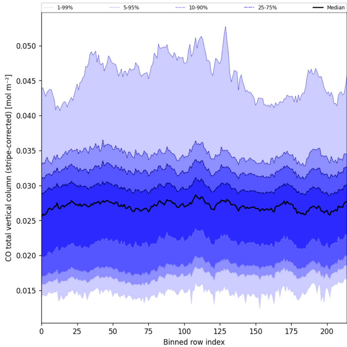
Figure 27: Along track statistics of “CO total vertical column (stripe-corrected)” for 2025-05-27 to 2025-05-29
