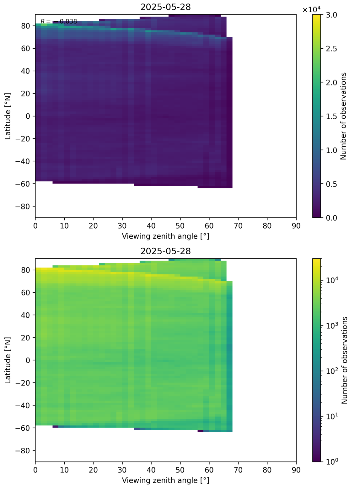
Figure 74: Scatter density plot of “Viewing zenith angle” against “Latitude” for 2025-05-27 to 2025-05-29.
