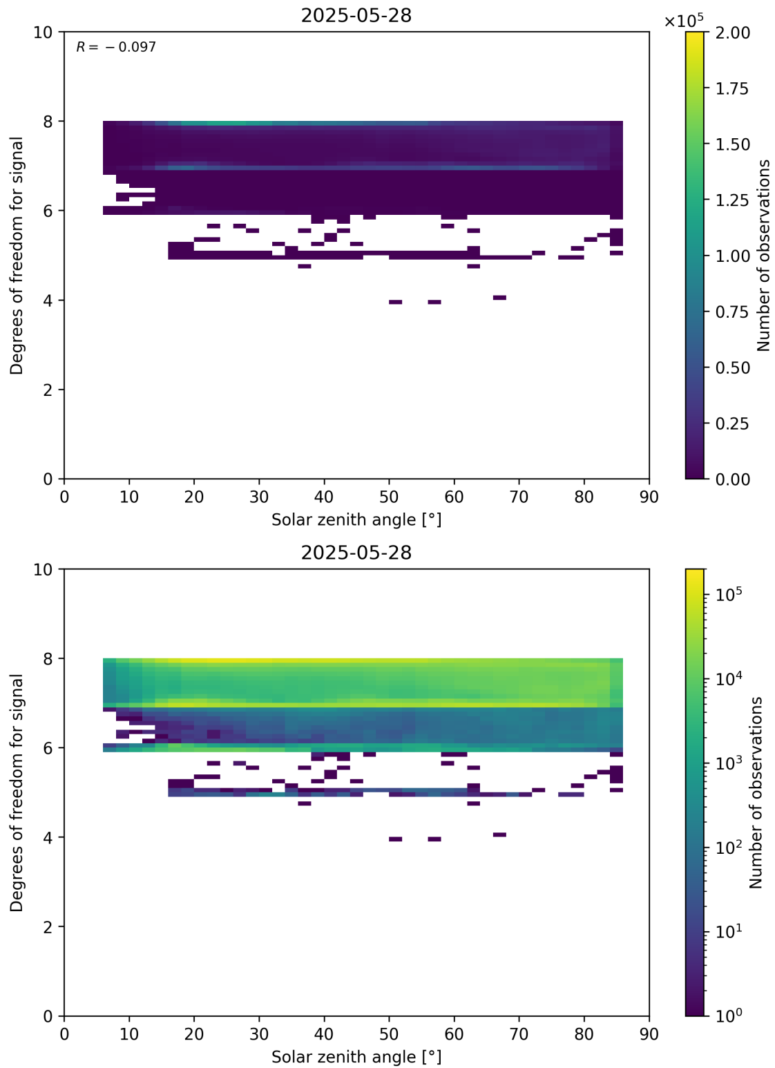
Figure 65: Scatter density plot of “Solar zenith angle” against “Degrees of freedom for signal” for 2025-05-27 to 2025-05-29.
