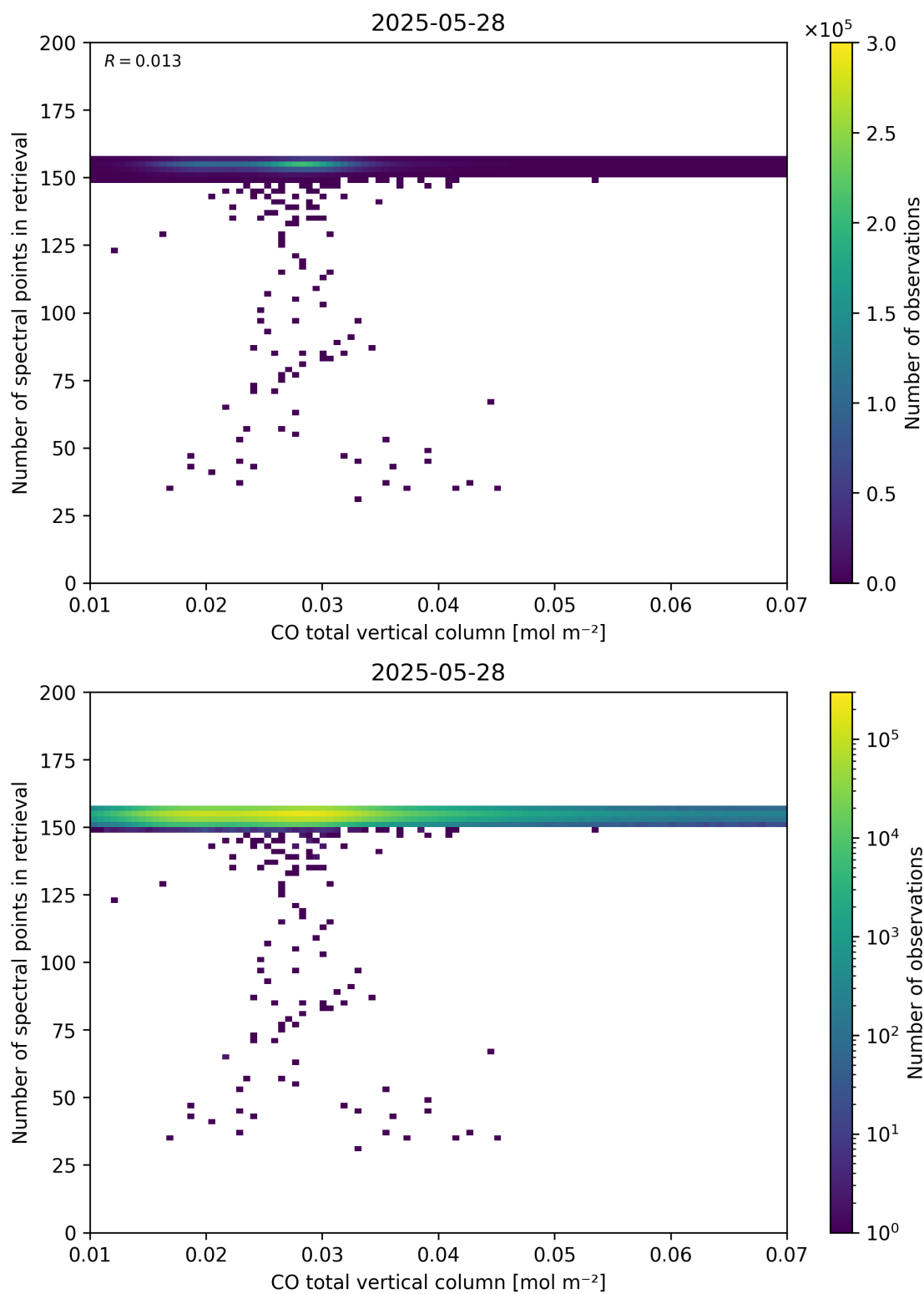
Figure 43: Scatter density plot of “CO total vertical column” against “Number of spectral points in retrieval” for 2025-05-27 to 2025-05-29.
