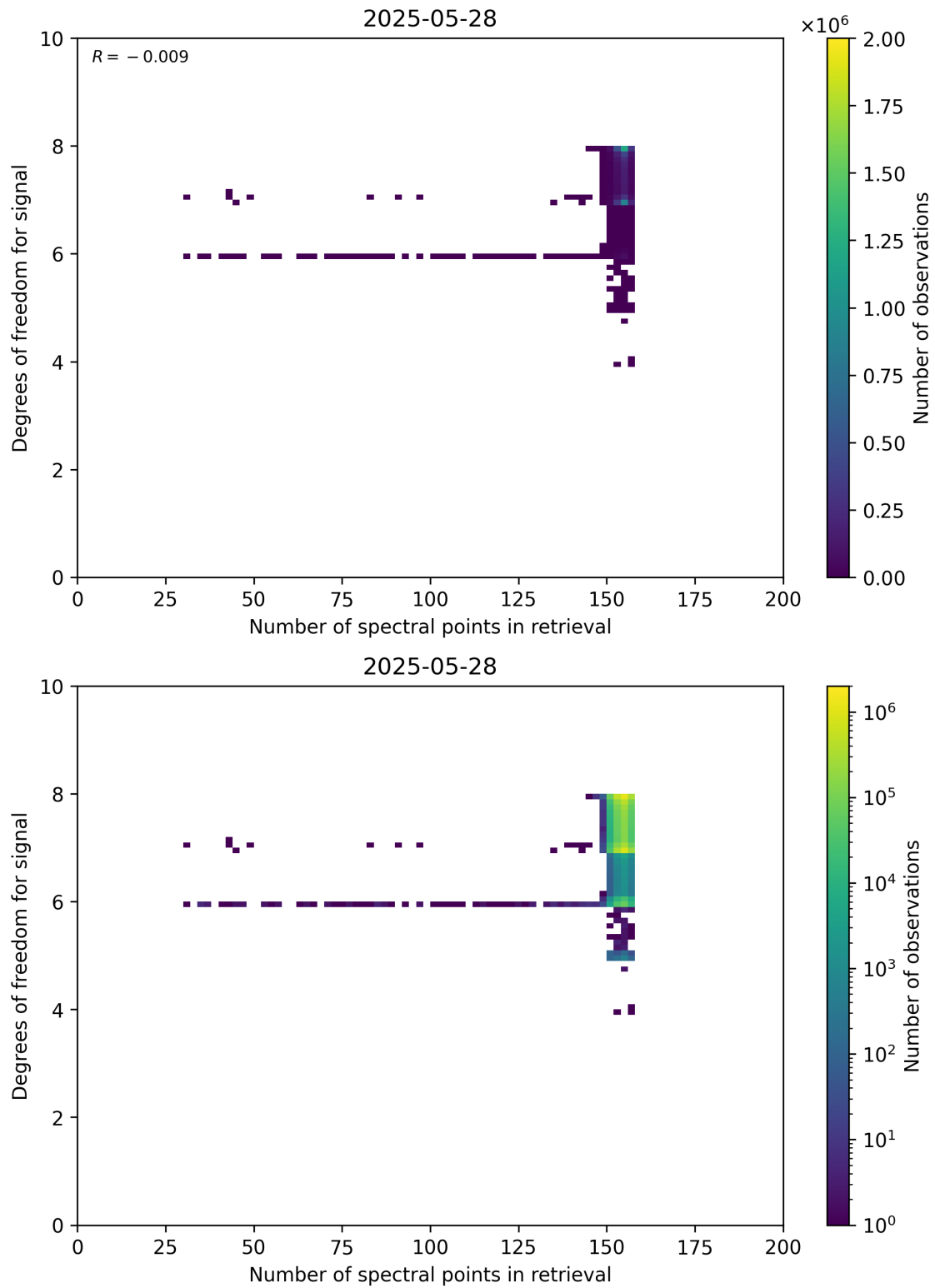
Figure 59: Scatter density plot of “Number of spectral points in retrieval” against “Degrees of freedom for signal” for 2025-05-27 to 2025-05-29.
