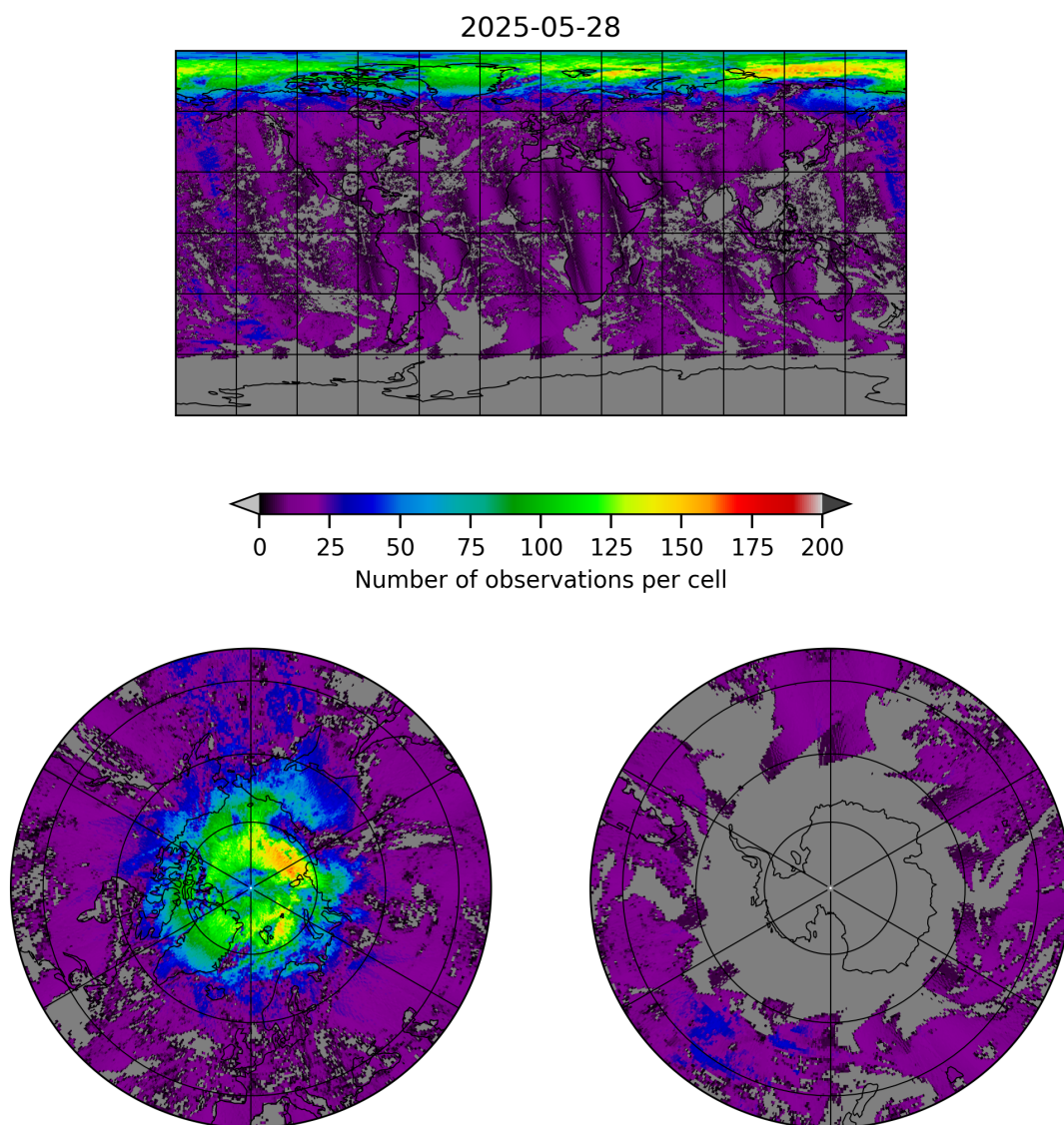
Figure 8: Map of the number of observations for 2025-05-27 to 2025-05-29
