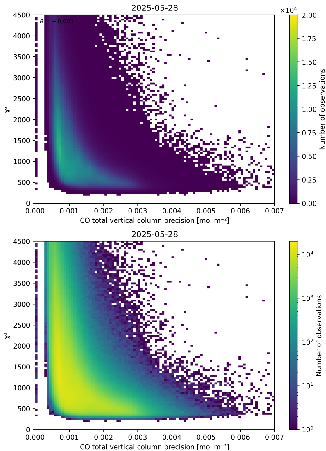
Figure 44: Scatter density plot of “CO total vertical column precision” against “ \chi^2 ” for 2025-05-27 to 2025-05-29.
