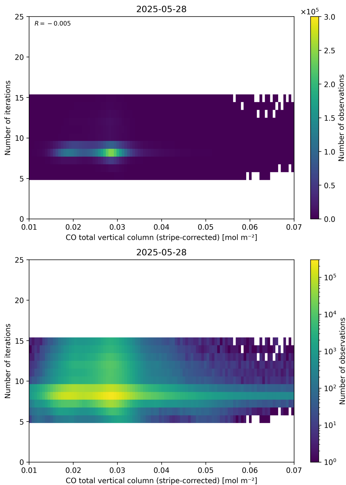
Figure 39: Scatter density plot of “CO total vertical column (stripe-corrected)” against “Number of iterations” for 2025-05-27 to 2025-05-29.
