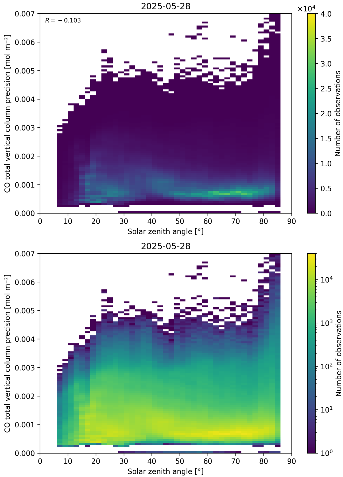
Figure 63: Scatter density plot of “Solar zenith angle” against “CO total vertical column precision” for 2025-05-27 to 2025-05-29.
