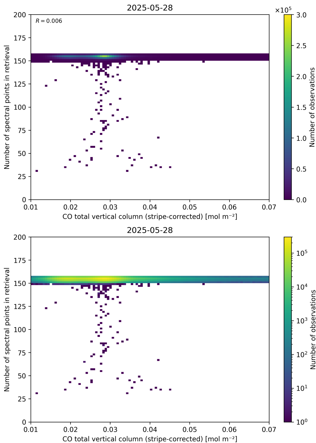
Figure 40: Scatter density plot of “CO total vertical column (stripe-corrected)” against “Number of spectral points in retrieval” for 2025-05-27 to 2025-05-29.
