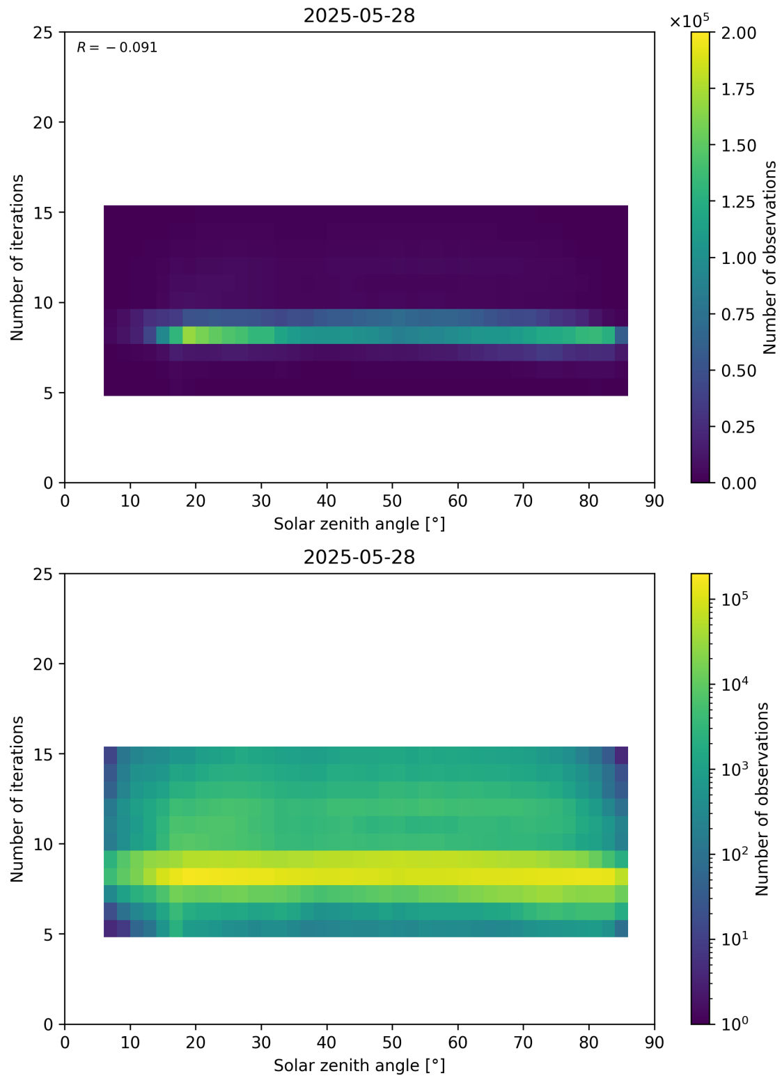
Figure 67: Scatter density plot of “Solar zenith angle” against “Number of iterations” for 2025-05-27 to 2025-05-29.
