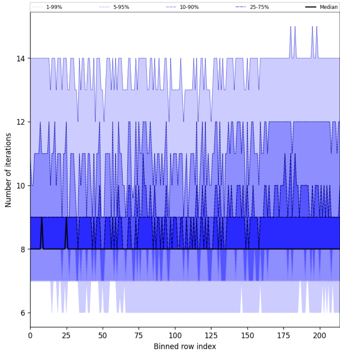
Figure 32: Along track statistics of “Number of iterations” for 2025-05-27 to 2025-05-29
