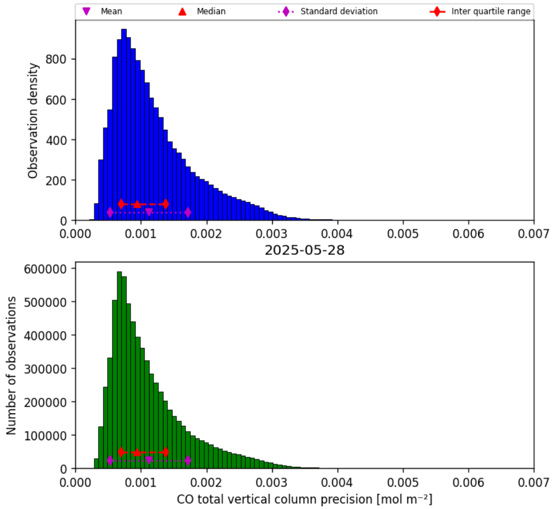
Figure 20: Histogram of “CO total vertical column precision” for 2025-05-27 to 2025-05-29
