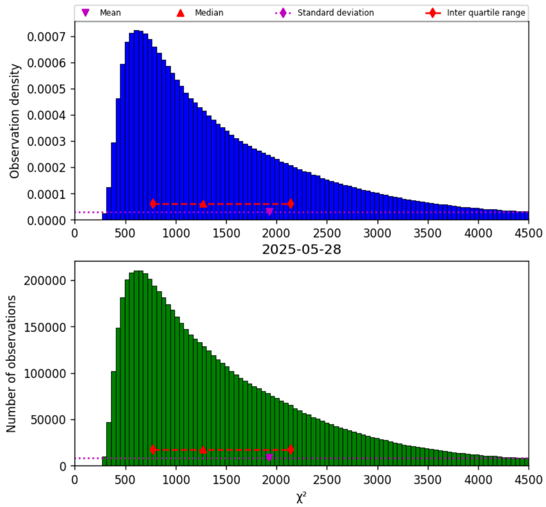
Figure 22: Histogram of “ \chi^2 ” for 2025-05-27 to 2025-05-29
