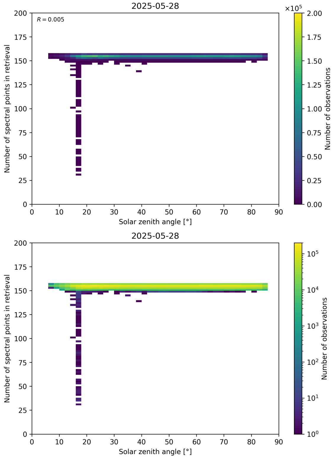
Figure 68: Scatter density plot of “Solar zenith angle” against “Number of spectral points in retrieval” for 2025-05-27 to 2025-05-29.
