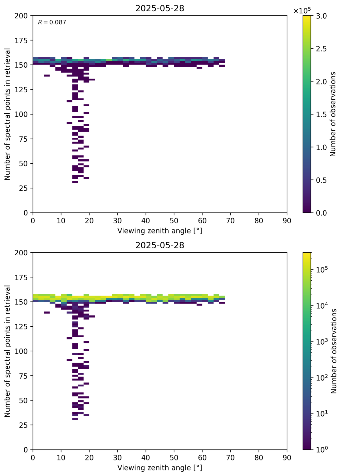
Figure 76: Scatter density plot of “Viewing zenith angle” against “Number of spectral points in retrieval” for 2025-05-27 to 2025-05-29.
