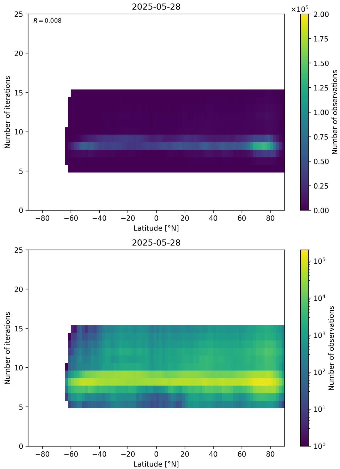
Figure 56: Scatter density plot of “Latitude” against “Number of iterations” for 2025-05-27 to 2025-05-29.
