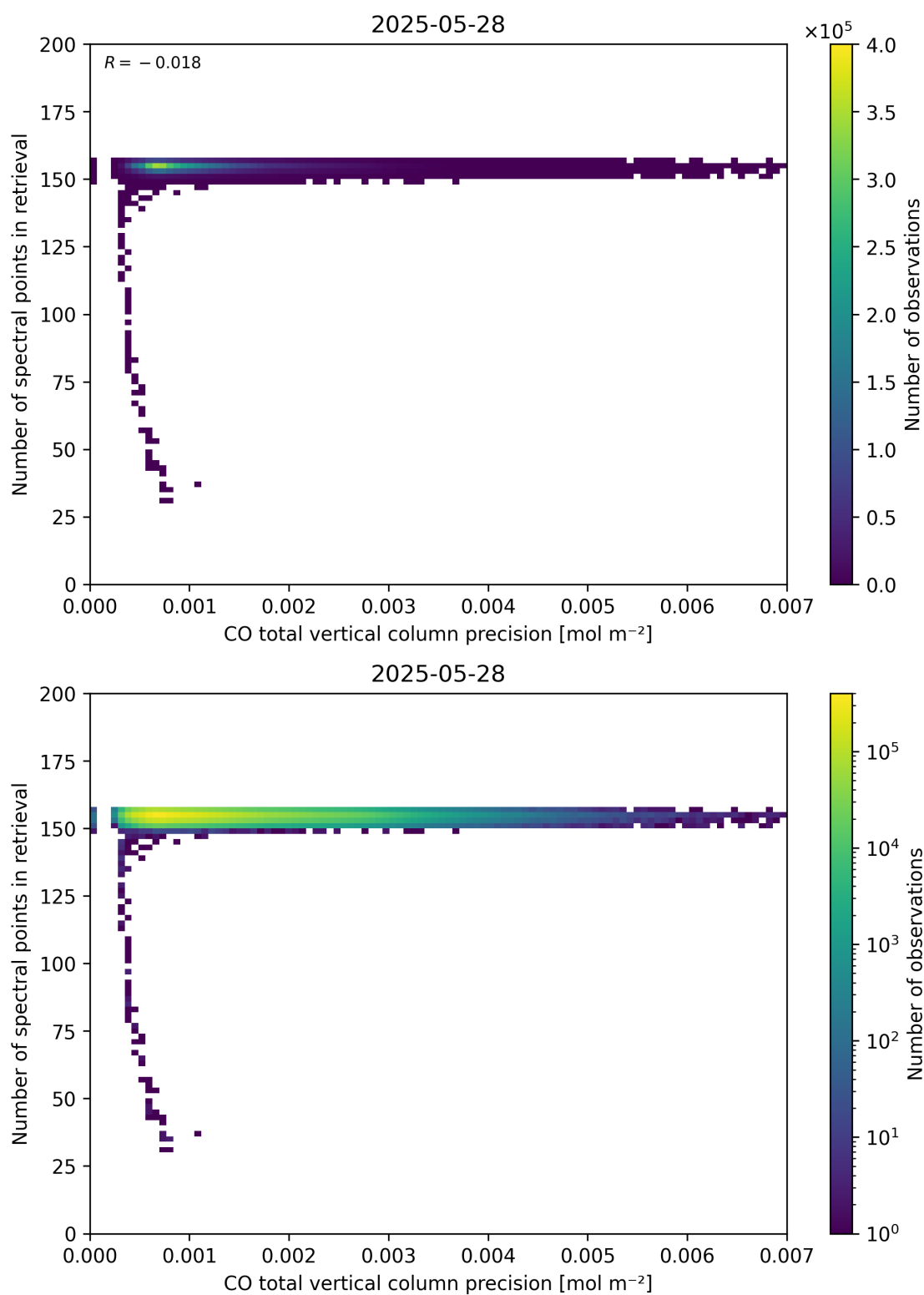
Figure 47: Scatter density plot of “CO total vertical column precision” against “Number of spectral points in retrieval” for 2025-05-27 to 2025-05-29.
