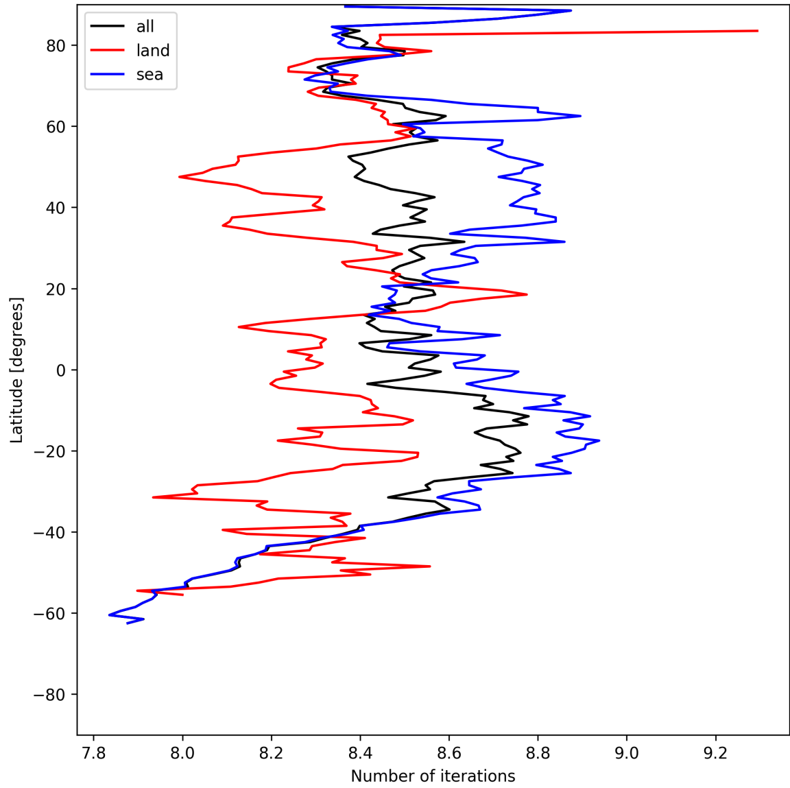
Figure 16: Zonal average of “Number of iterations” for 2025-05-27 to 2025-05-29.
