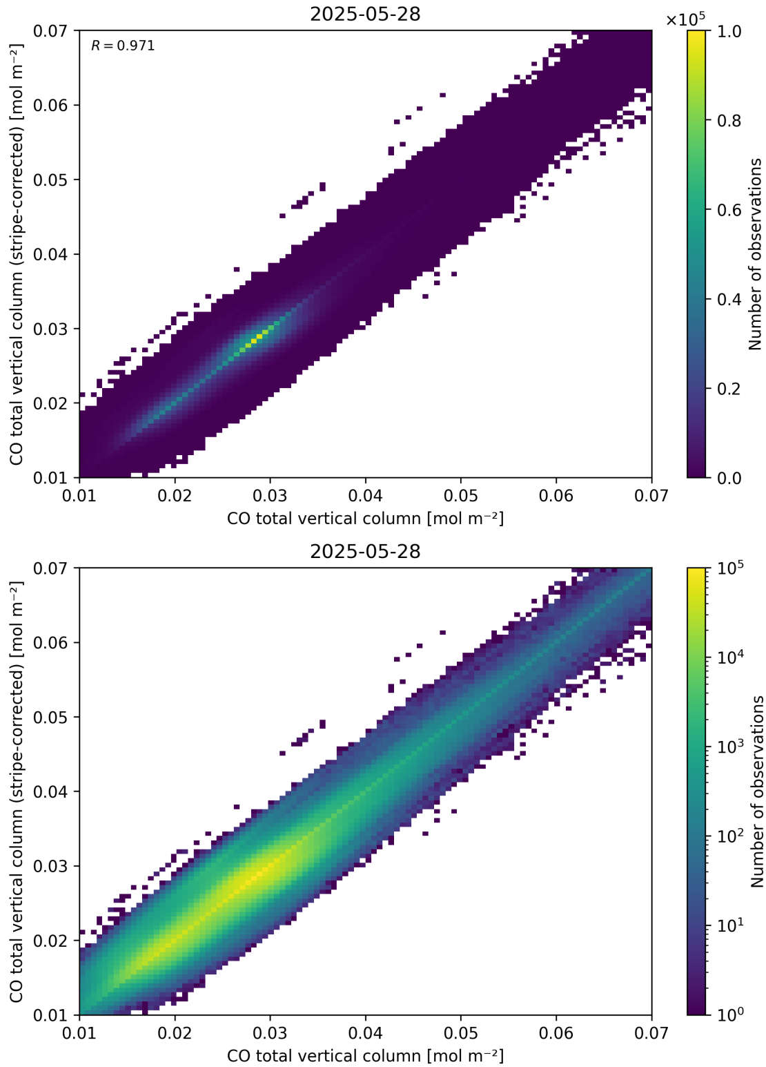
Figure 33: Scatter density plot of “CO total vertical column” against “CO total vertical column (stripe-corrected)” for 2025-05-27 to 2025-05-29.
