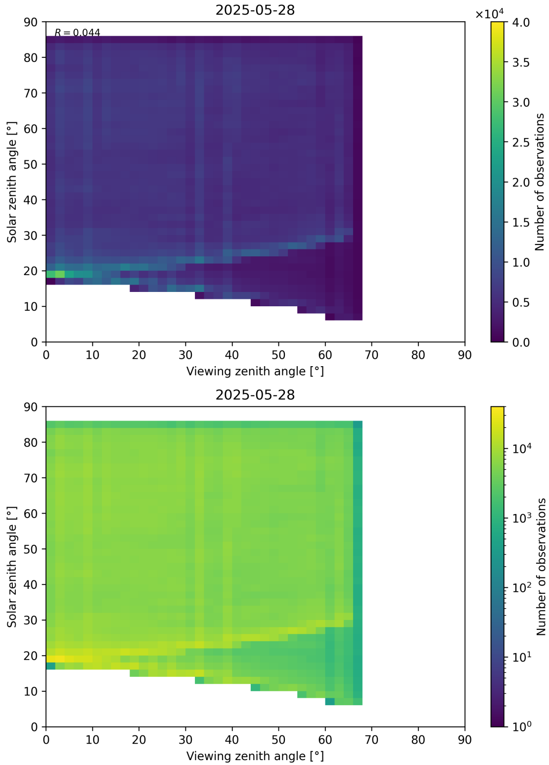
Figure 77: Scatter density plot of “Viewing zenith angle” against “Solar zenith angle” for 2025-05-27 to 2025-05-29.
