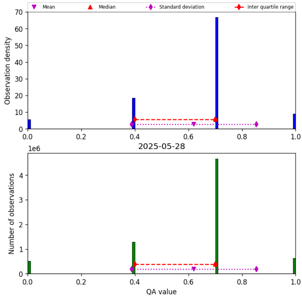
Figure 17: Histogram of “QA value” for 2025-05-27 to 2025-05-29
