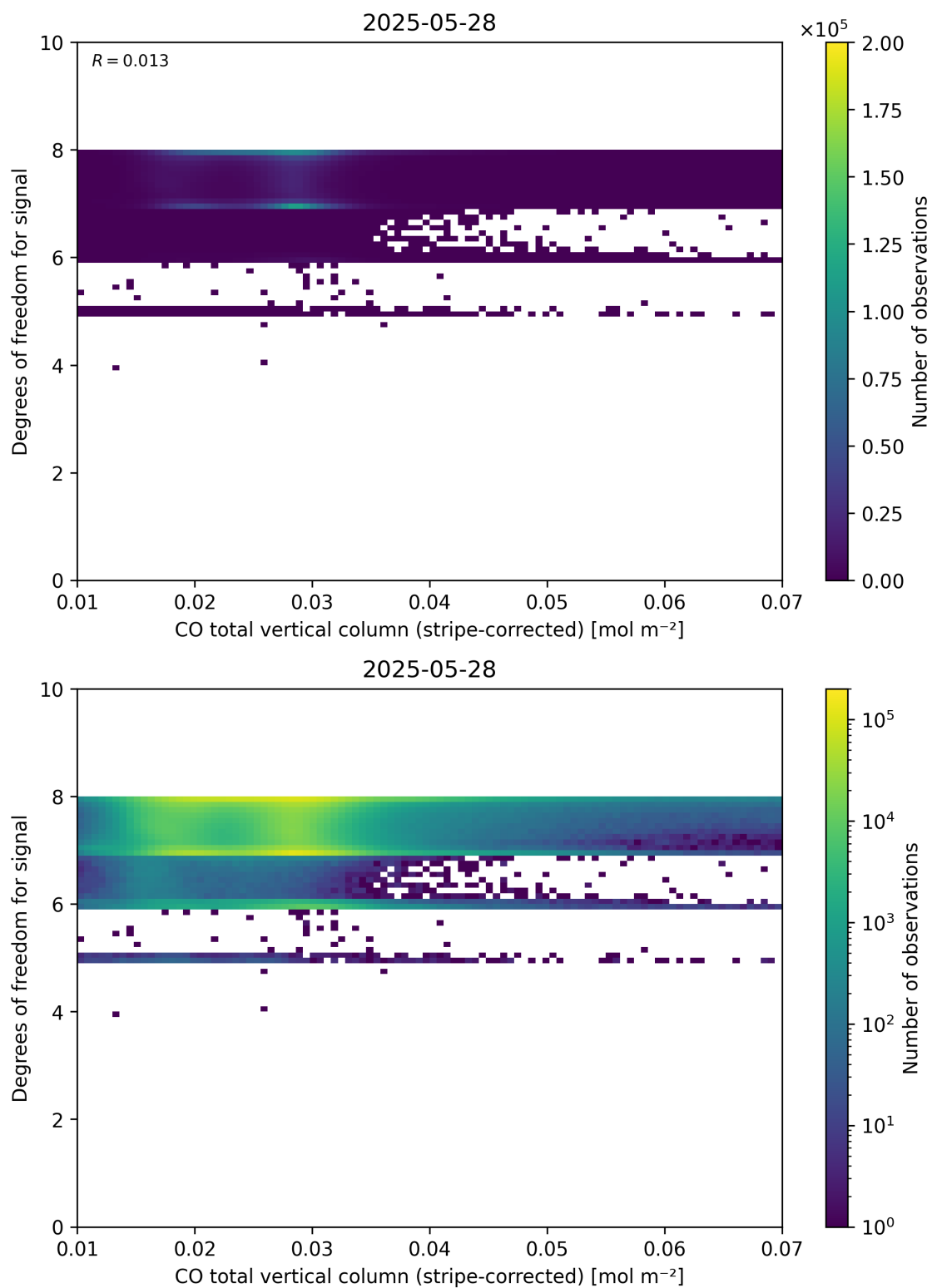
Figure 38: Scatter density plot of “CO total vertical column (stripe-corrected)” against “Degrees of freedom for signal” for 2025-05-27 to 2025-05-29.
