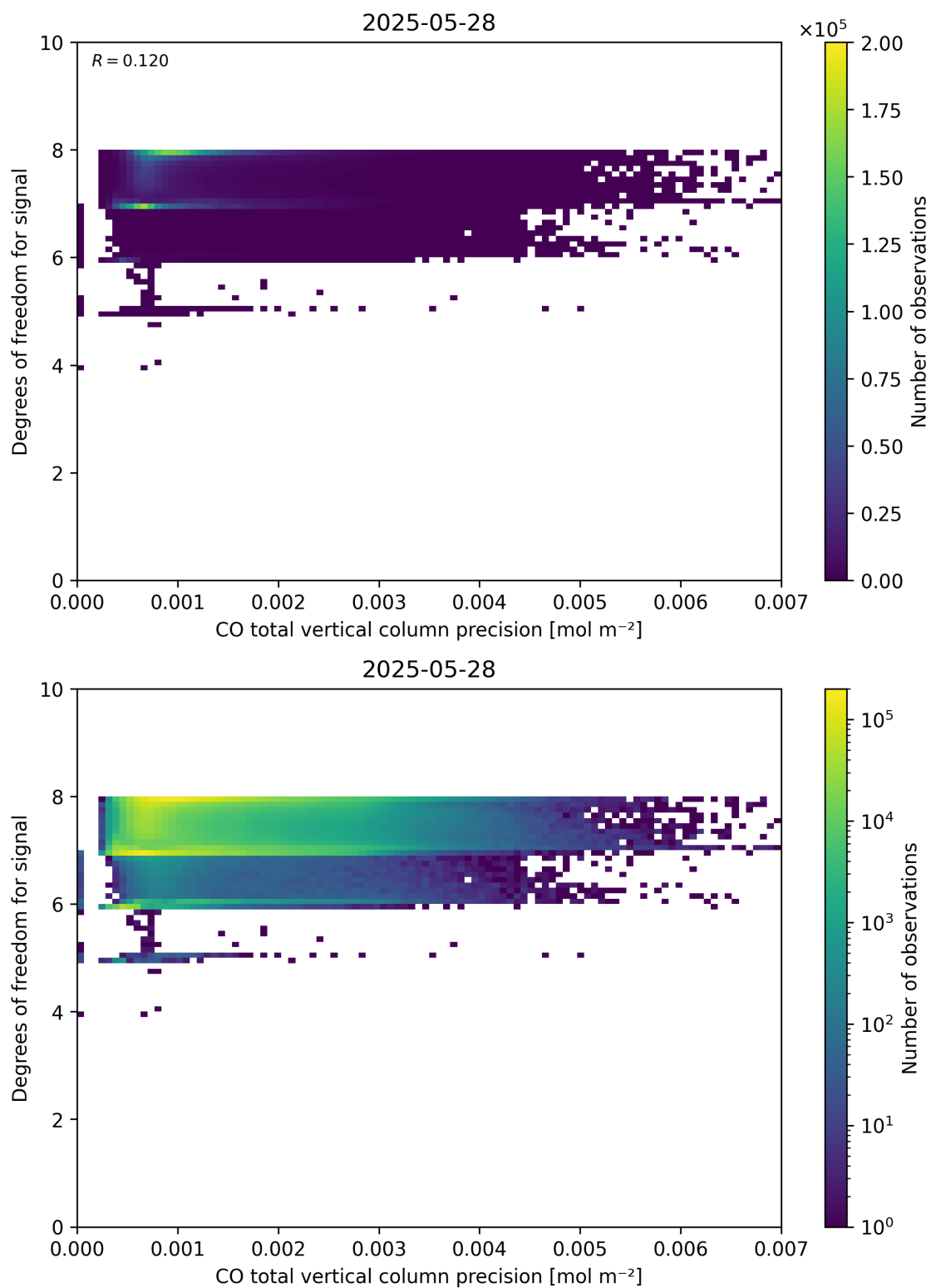
Figure 45: Scatter density plot of “CO total vertical column precision” against “Degrees of freedom for signal” for 2025-05-27 to 2025-05-29.
