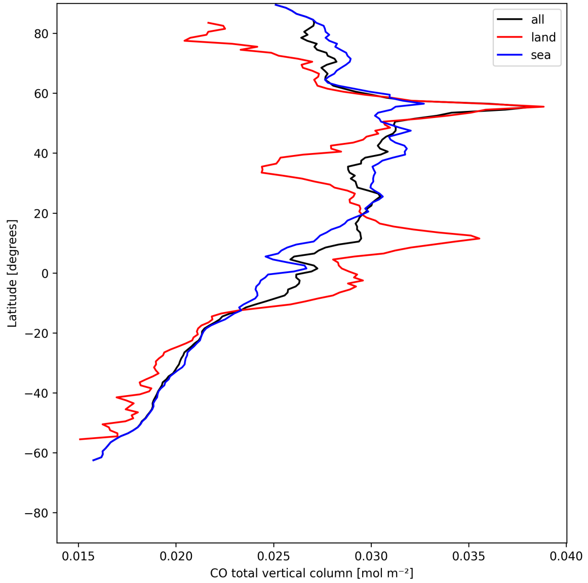
Figure 10: Zonal average of “CO total vertical column” for 2025-05-27 to 2025-05-29.
