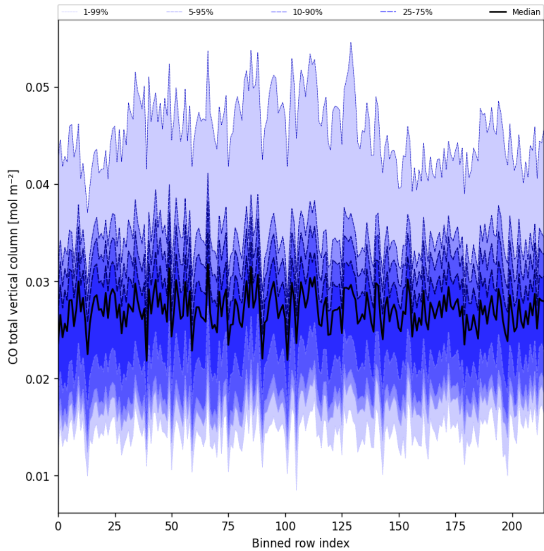
Figure 26: Along track statistics of “CO total vertical column” for 2025-05-27 to 2025-05-29
