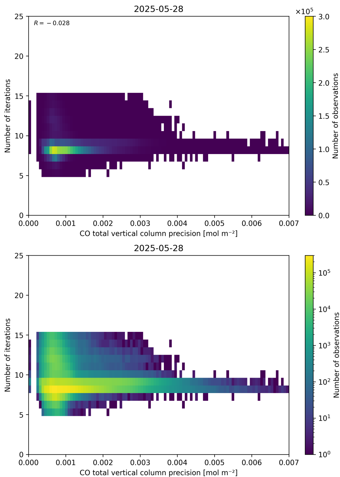
Figure 46: Scatter density plot of “CO total vertical column precision” against “Number of iterations” for 2025-05-27 to 2025-05-29.
