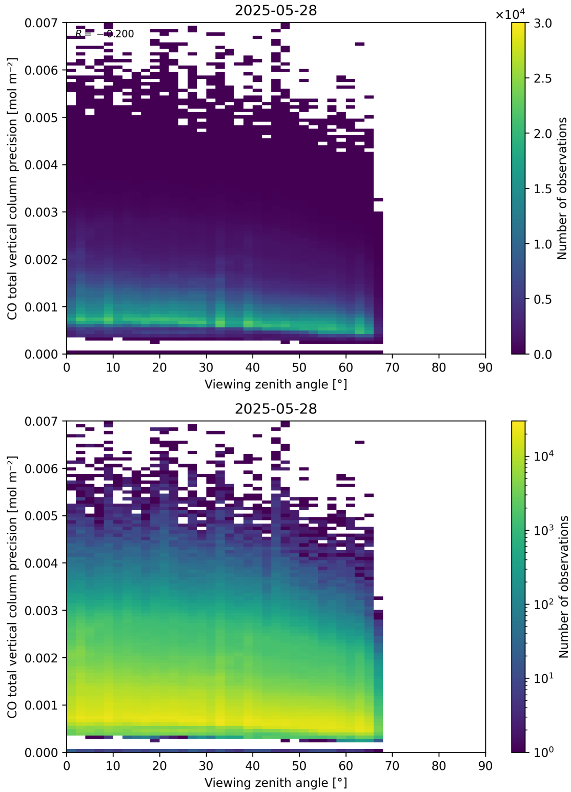
Figure 71: Scatter density plot of “Viewing zenith angle” against “CO total vertical column precision” for 2025-05-27 to 2025-05-29.
