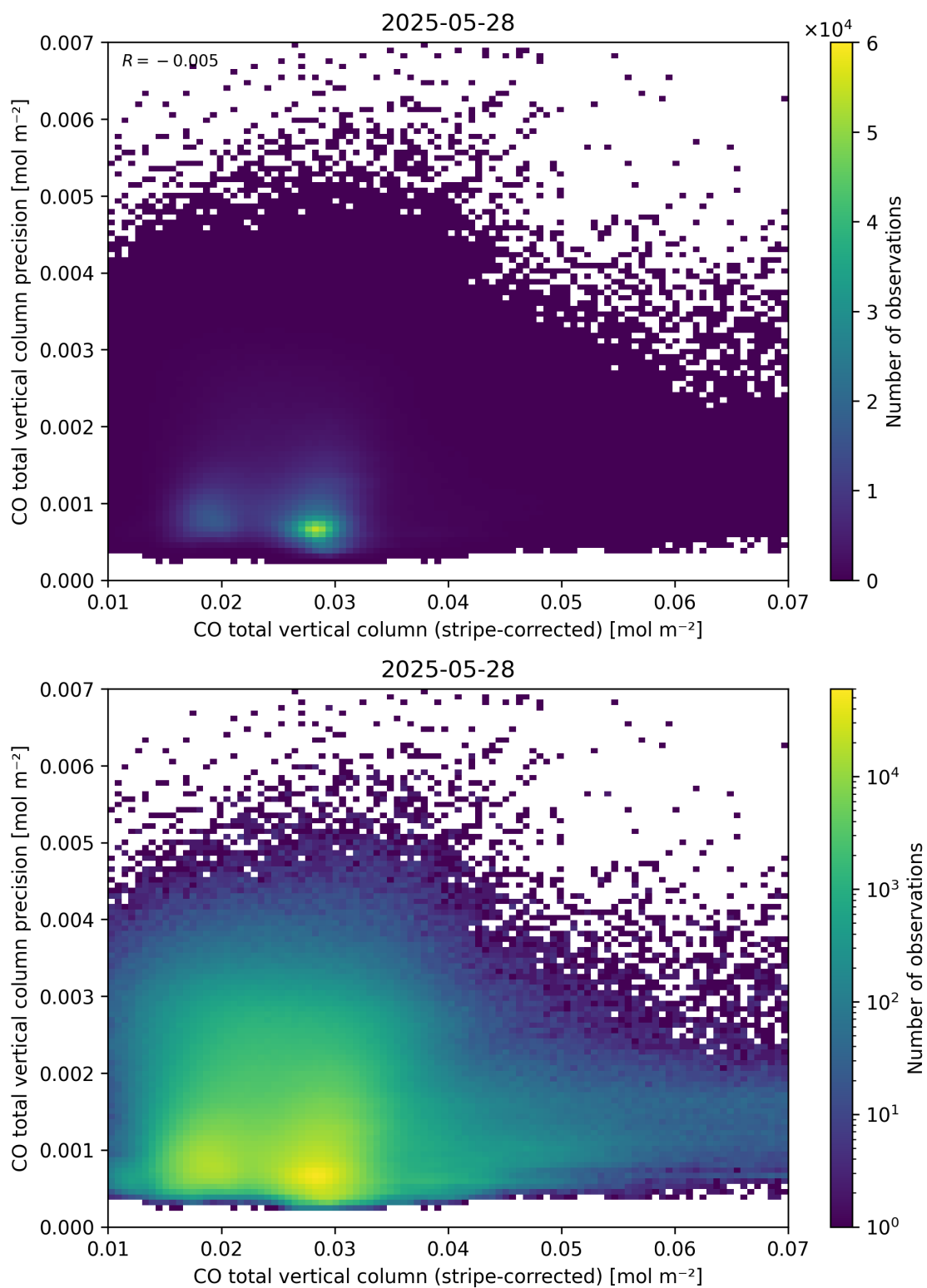
Figure 36: Scatter density plot of “CO total vertical column (stripe-corrected)” against “CO total vertical column precision” for 2025-05-27 to 2025-05-29.
