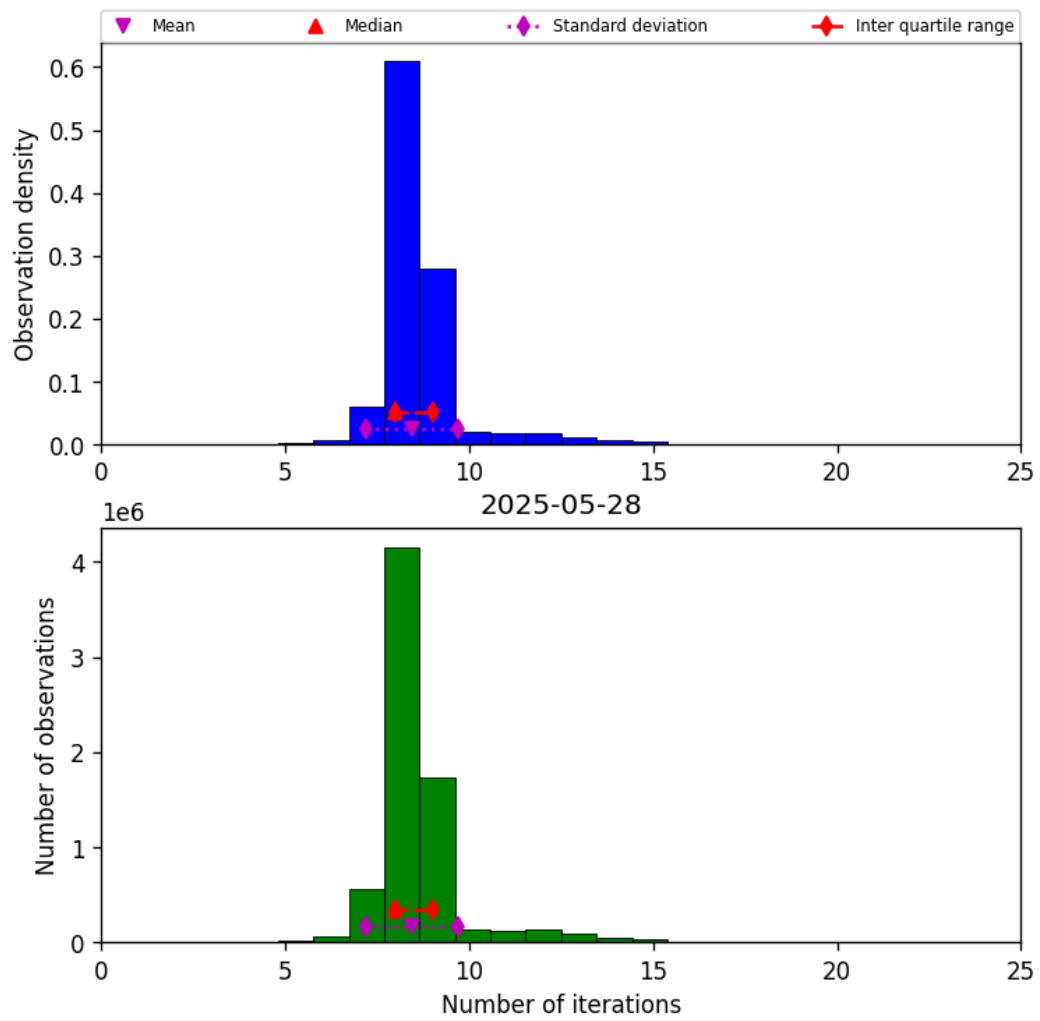
Figure 24: Histogram of “Number of iterations” for 2025-05-27 to 2025-05-29
