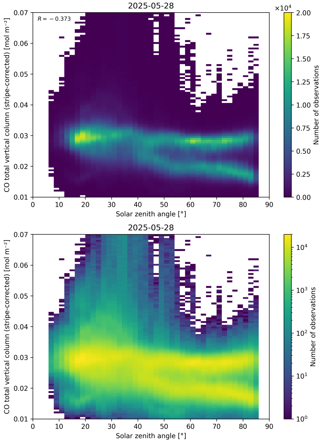
Figure 62: Scatter density plot of “Solar zenith angle” against “CO total vertical column (stripe-corrected)” for 2025-05-27 to 2025-05-29.
