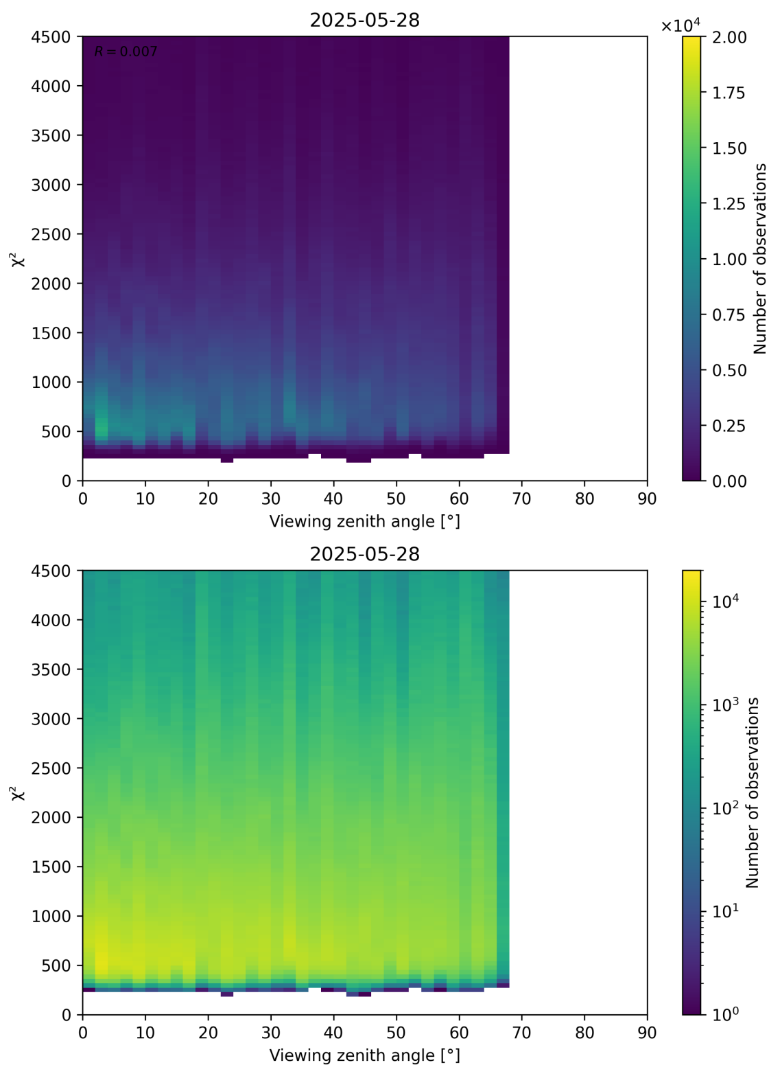
Figure 72: Scatter density plot of “Viewing zenith angle” against “ \chi^2 ” for 2025-05-27 to 2025-05-29.
