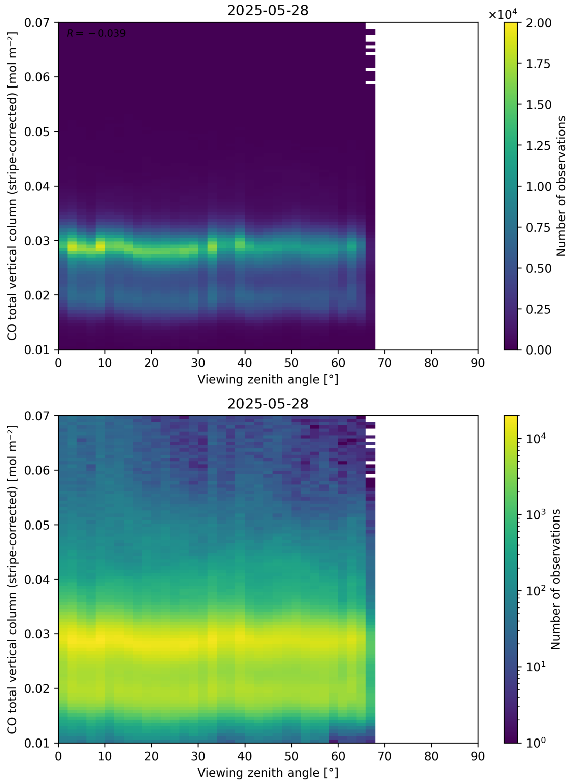
Figure 70: Scatter density plot of “Viewing zenith angle” against “CO total vertical column (stripe-corrected)” for 2025-05-27 to 2025-05-29.
