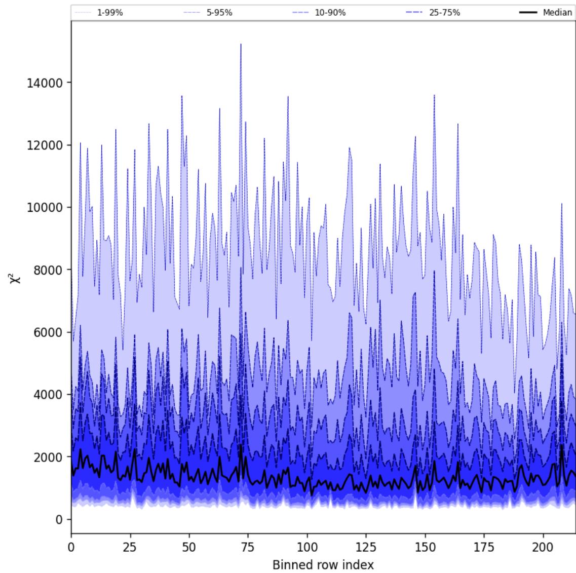
Figure 30: Along track statistics of “ \chi^2 ” for 2025-05-27 to 2025-05-29
