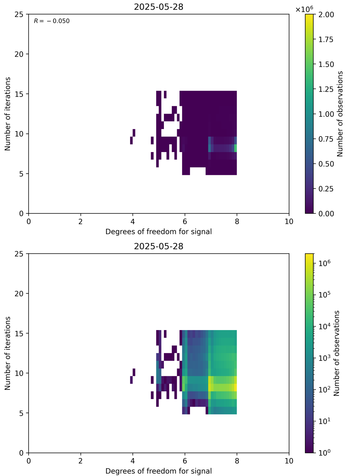
Figure 50: Scatter density plot of “Degrees of freedom for signal” against “Number of iterations” for 2025-05-27 to 2025-05-29.
