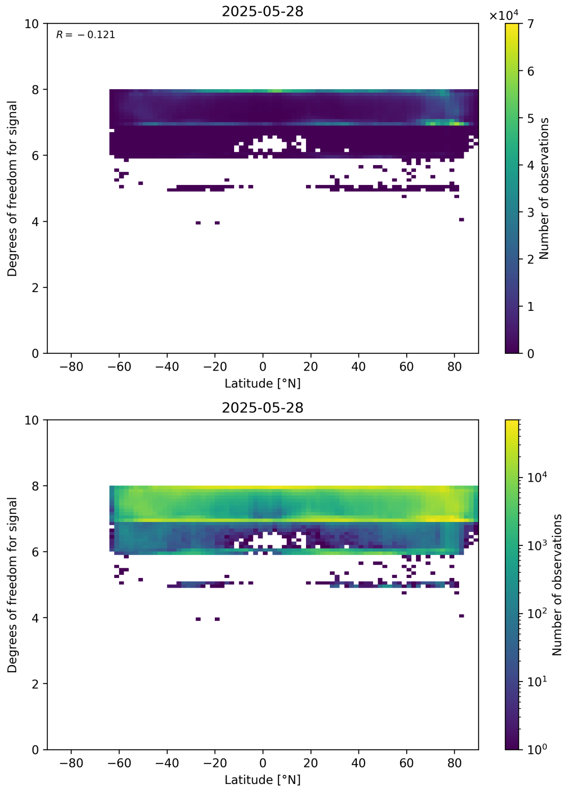
Figure 55: Scatter density plot of “Latitude” against “Degrees of freedom for signal” for 2025-05-27 to 2025-05-29.
