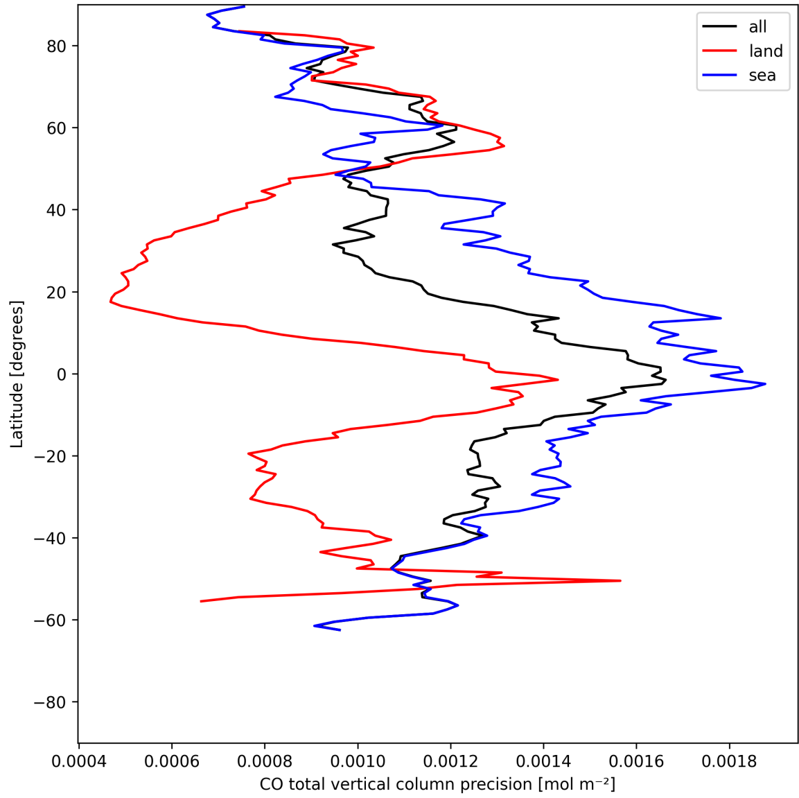
Figure 12: Zonal average of “CO total vertical column precision” for 2025-05-27 to 2025-05-29.
