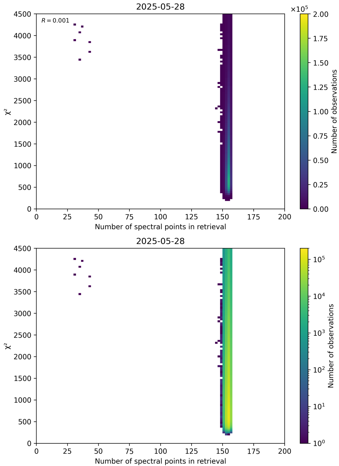
Figure 58: Scatter density plot of “Number of spectral points in retrieval” against “ \chi^2 ” for 2025-05-27 to 2025-05-29.
