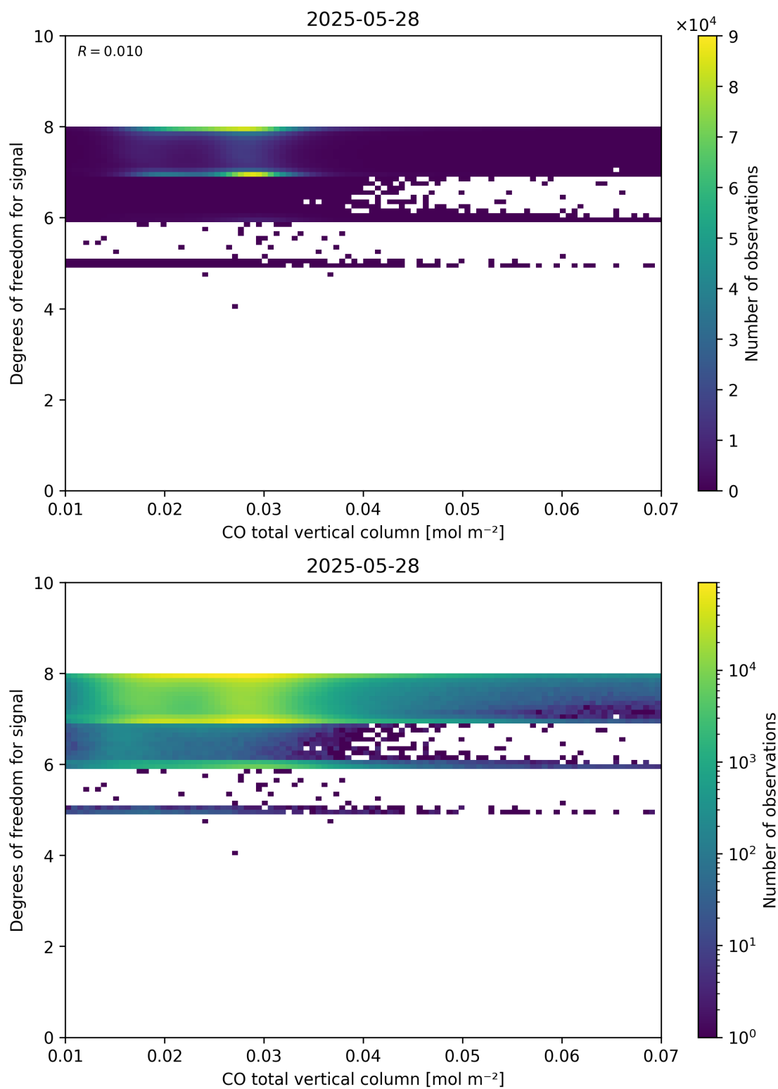
Figure 41: Scatter density plot of “CO total vertical column” against “Degrees of freedom for signal” for 2025-05-27 to 2025-05-29.
