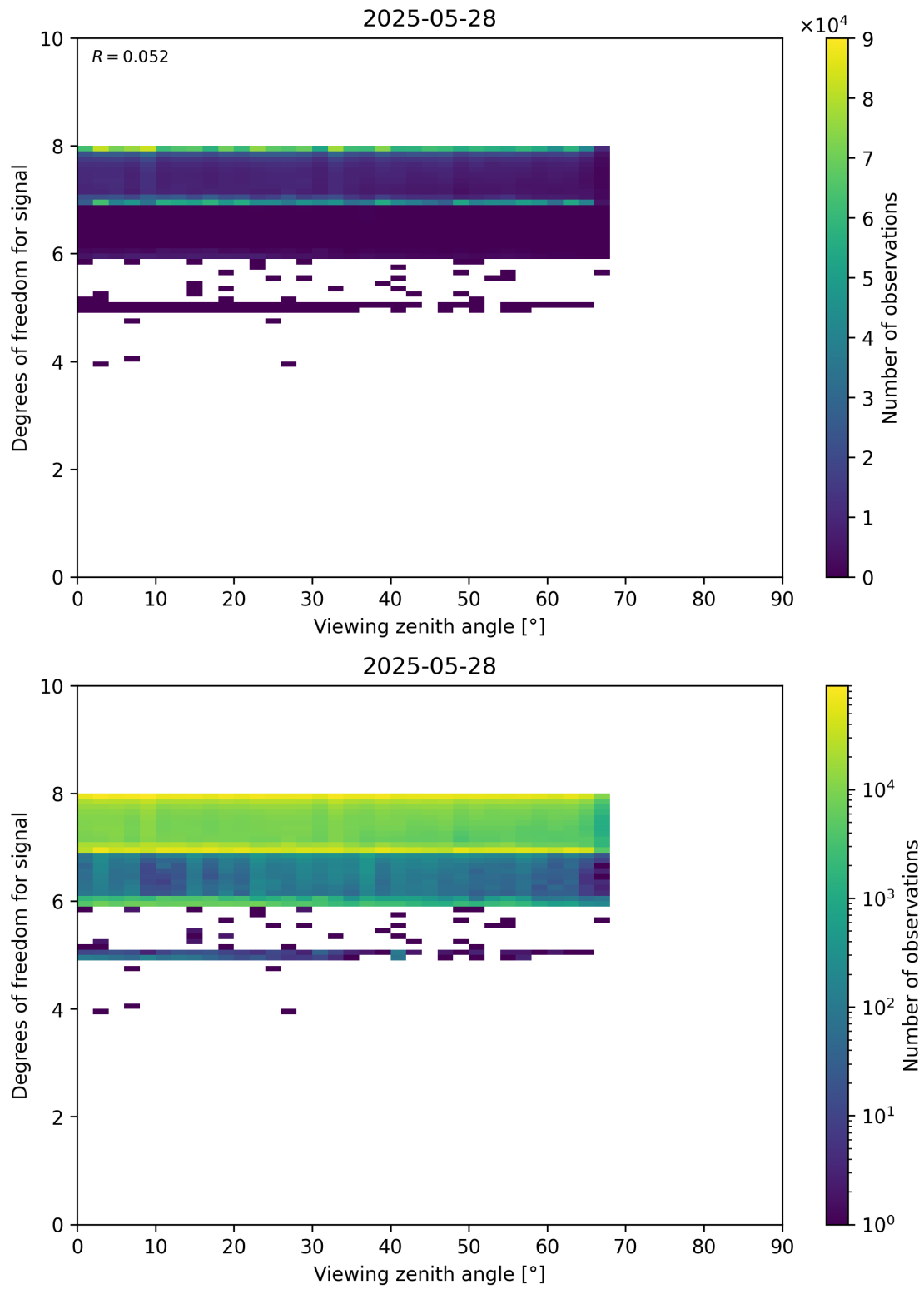
Figure 73: Scatter density plot of “Viewing zenith angle” against “Degrees of freedom for signal” for 2025-05-27 to 2025-05-29.
