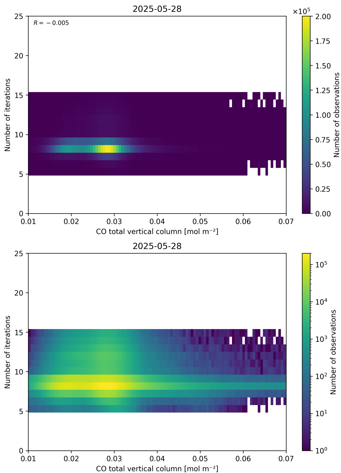
Figure 42: Scatter density plot of “CO total vertical column” against “Number of iterations” for 2025-05-27 to 2025-05-29.
