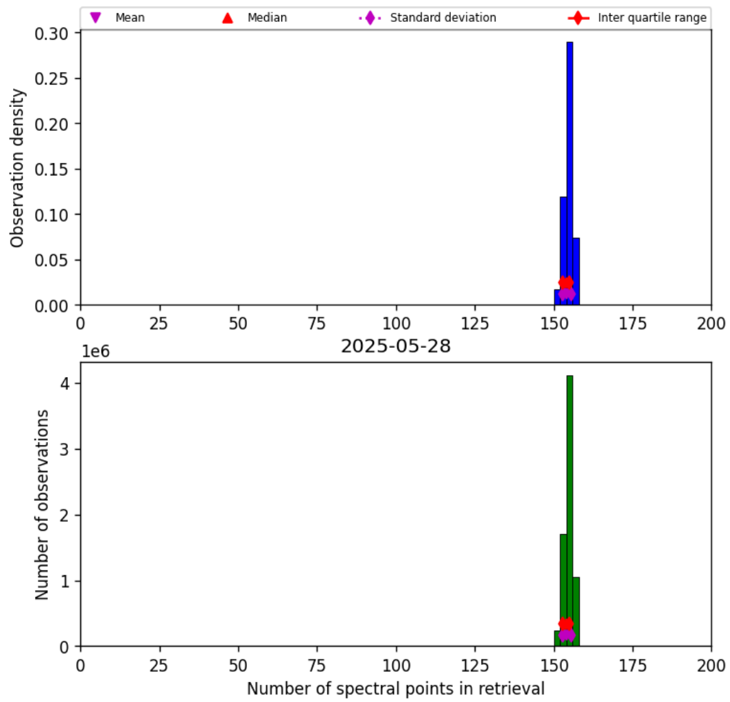
Figure 21: Histogram of “Number of spectral points in retrieval” for 2025-05-27 to 2025-05-29
