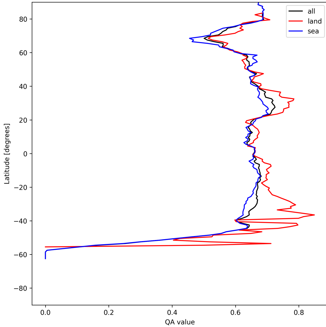
Figure 9: Zonal average of “QA value” for 2025-05-27 to 2025-05-29.
