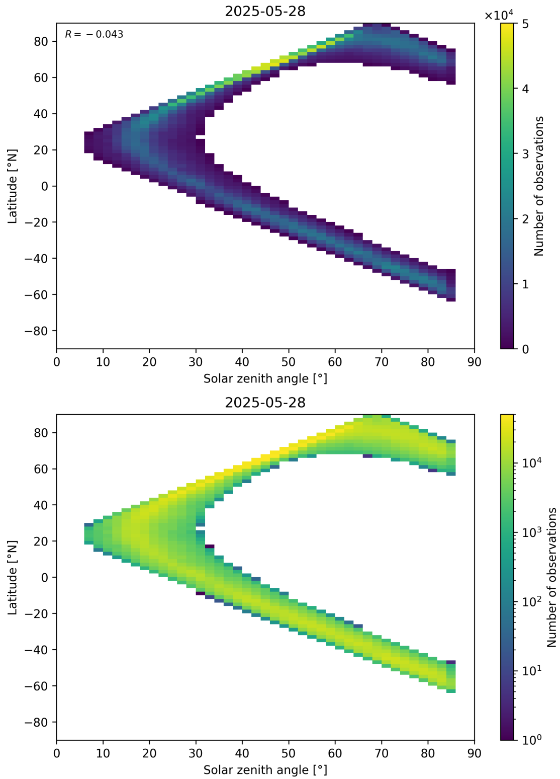
Figure 66: Scatter density plot of “Solar zenith angle” against “Latitude” for 2025-05-27 to 2025-05-29.
