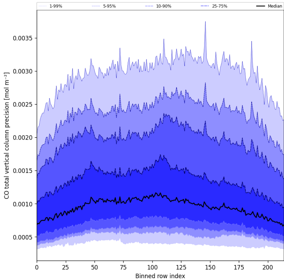
Figure 28: Along track statistics of “CO total vertical column precision” for 2025-05-27 to 2025-05-29
