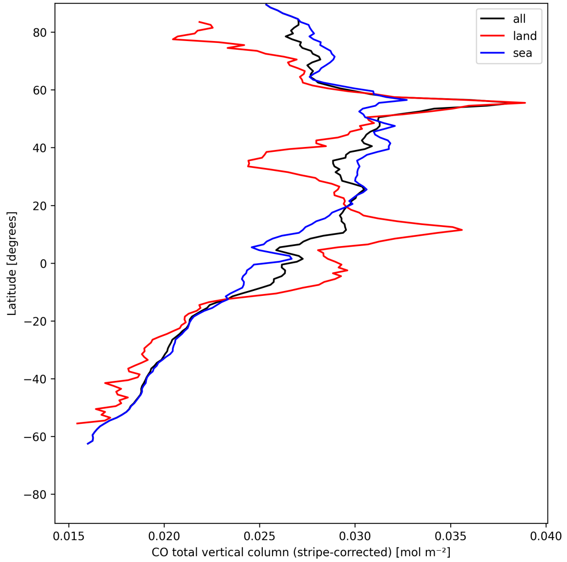
Figure 11: Zonal average of “CO total vertical column (stripe-corrected)” for 2025-05-27 to 2025-05-29.
