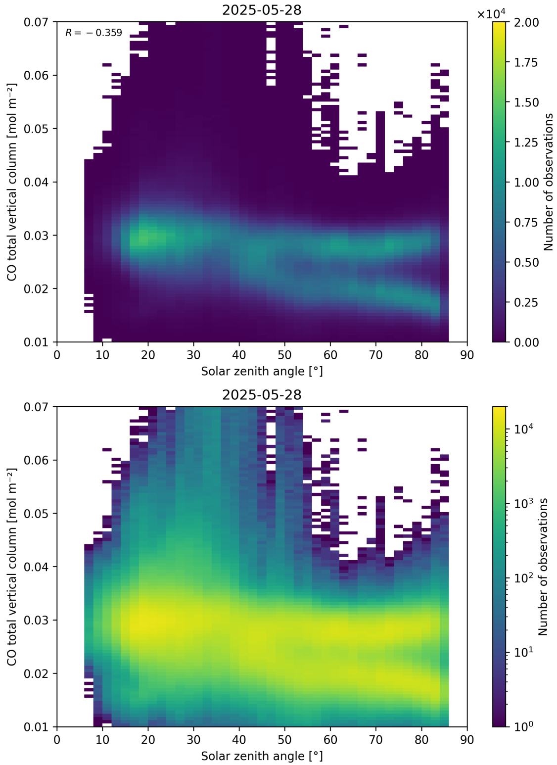
Figure 61: Scatter density plot of “Solar zenith angle” against “CO total vertical column” for 2025-05-27 to 2025-05-29.
