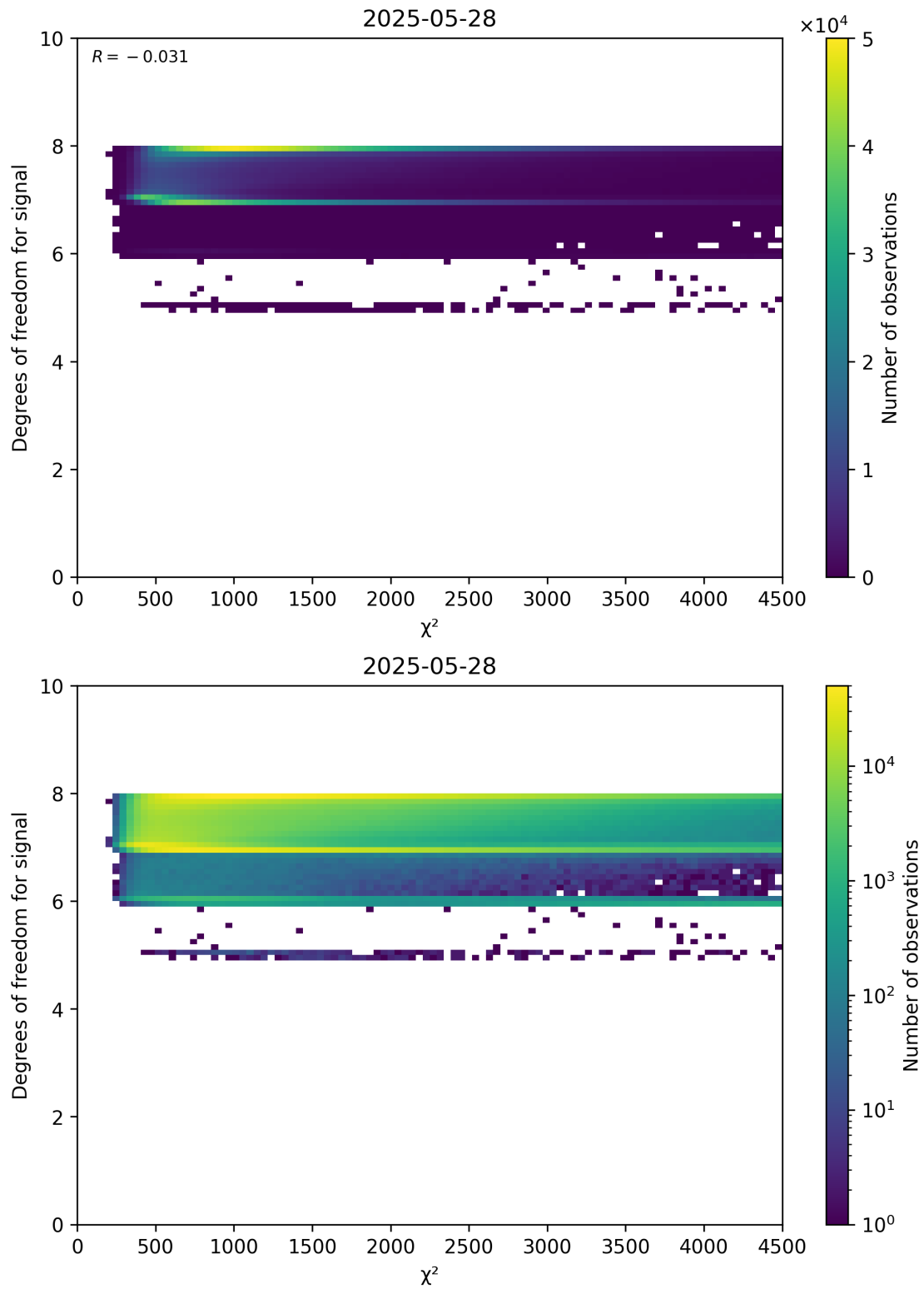
Figure 48: Scatter density plot of “ \chi^2 ” against “Degrees of freedom for signal” for 2025-05-27 to 2025-05-29.
