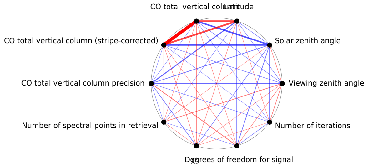
Figure 1: Map of correlation graph for 2025-05-27 to 2025-05-29.
