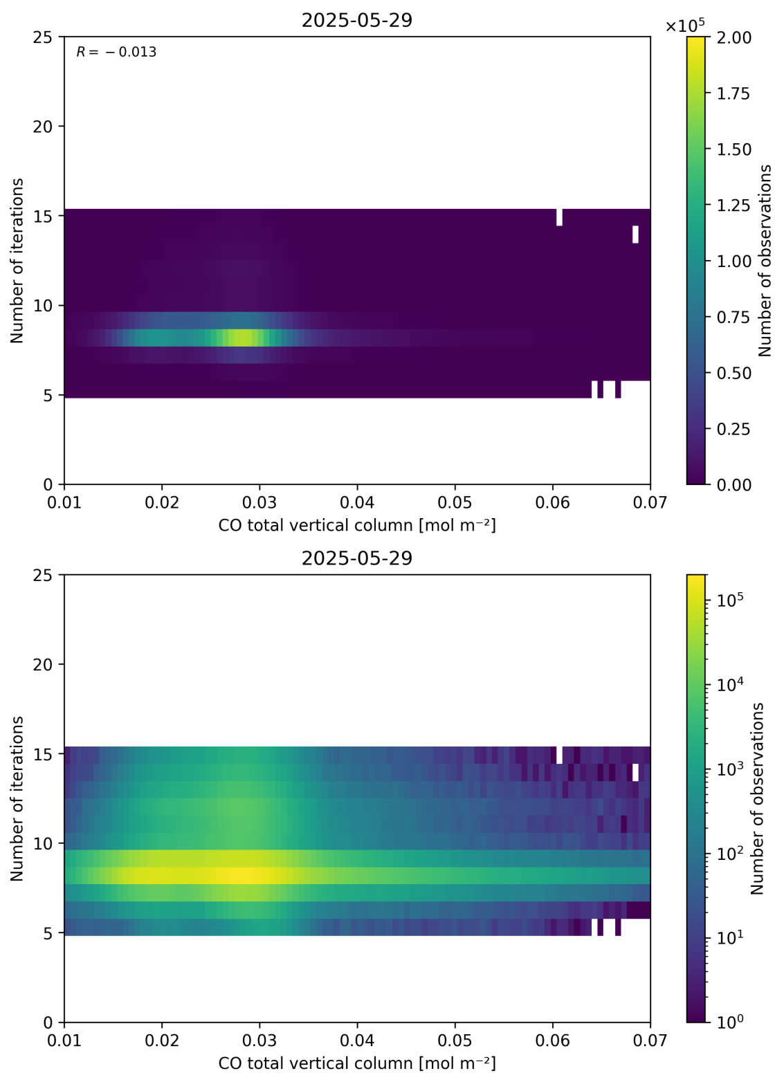
Figure 42: Scatter density plot of “CO total vertical column” against “Number of iterations” for 2025-05-28 to 2025-05-30.
