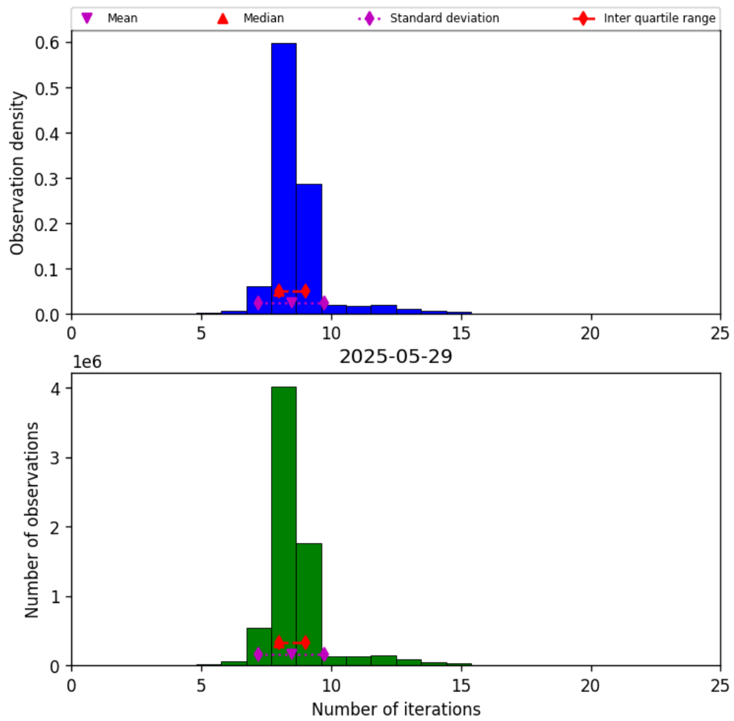
Figure 24: Histogram of “Number of iterations” for 2025-05-28 to 2025-05-30
