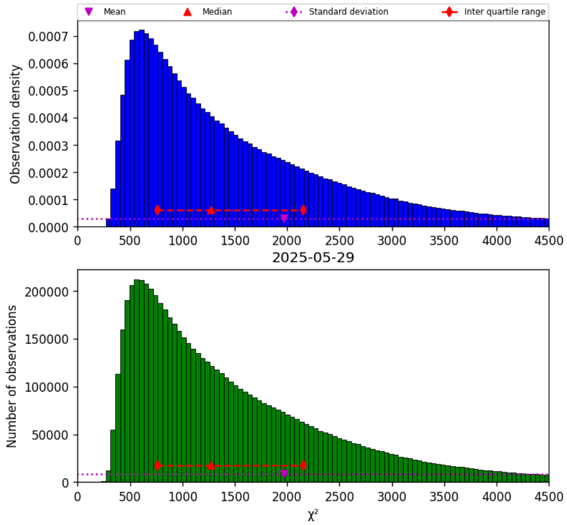
Figure 22: Histogram of “ \chi^2 ” for 2025-05-28 to 2025-05-30
