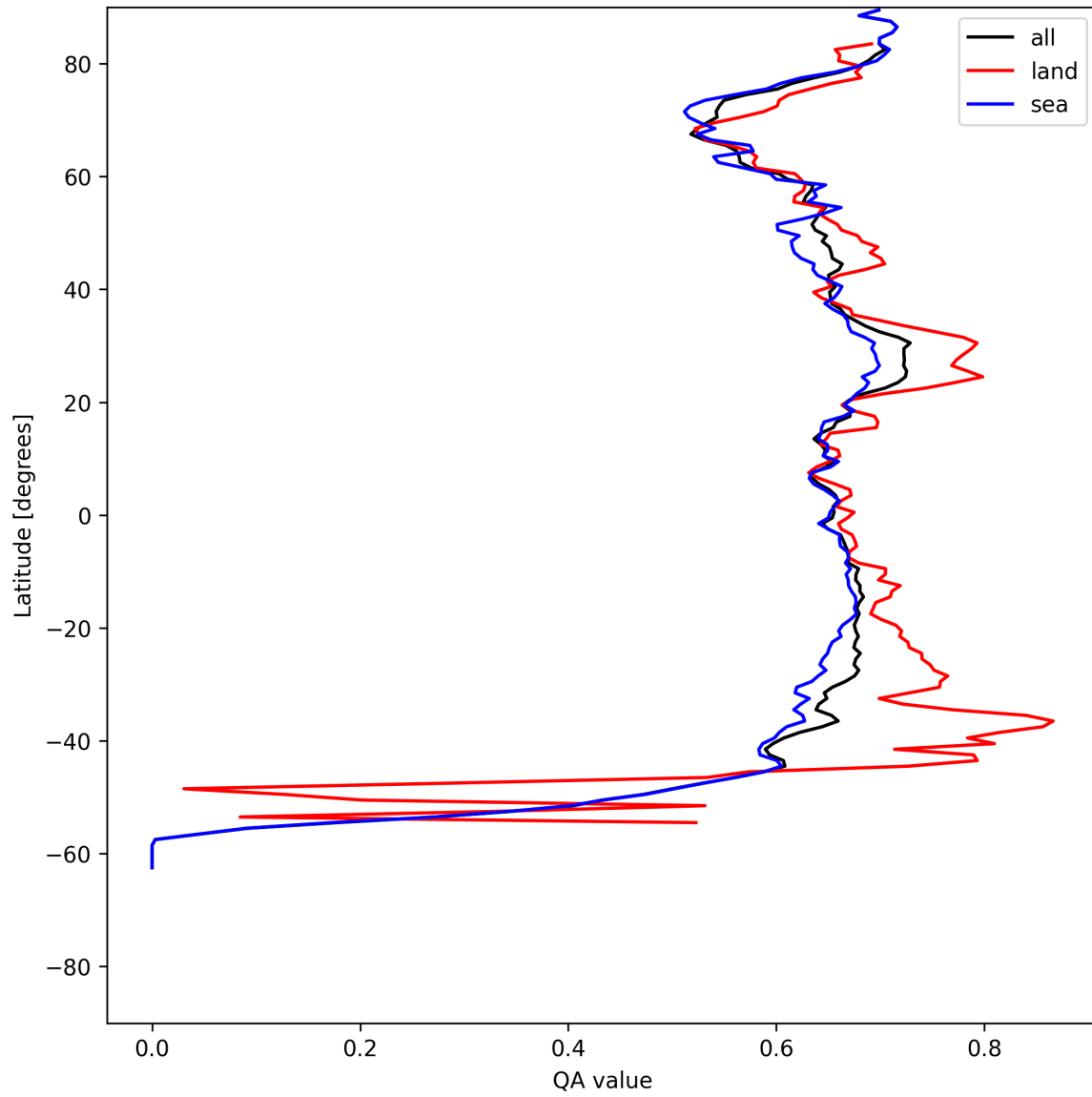
Figure 9: Zonal average of “QA value” for 2025-05-28 to 2025-05-30.
