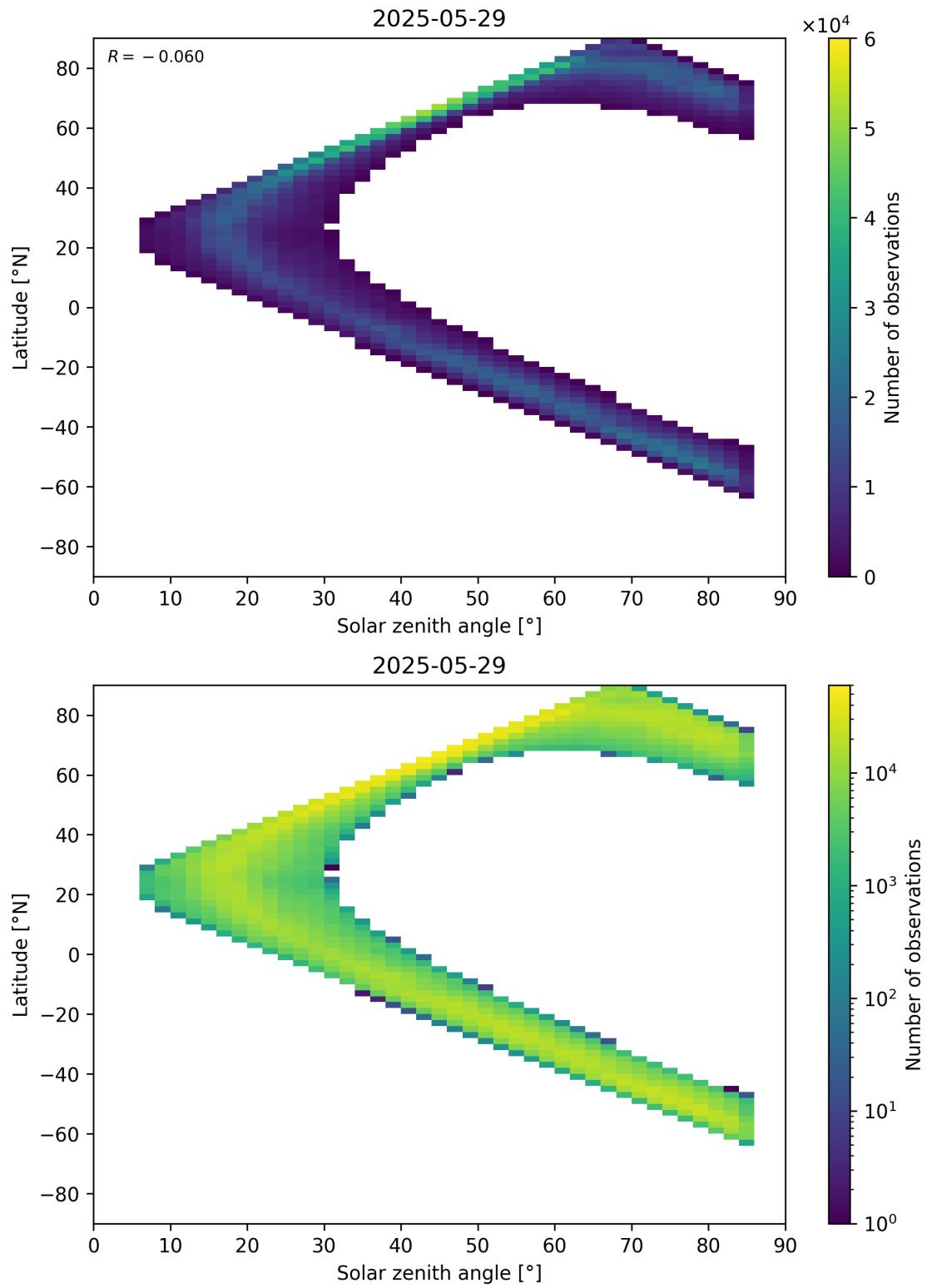
Figure 66: Scatter density plot of “Solar zenith angle” against “Latitude” for 2025-05-28 to 2025-05-30.
