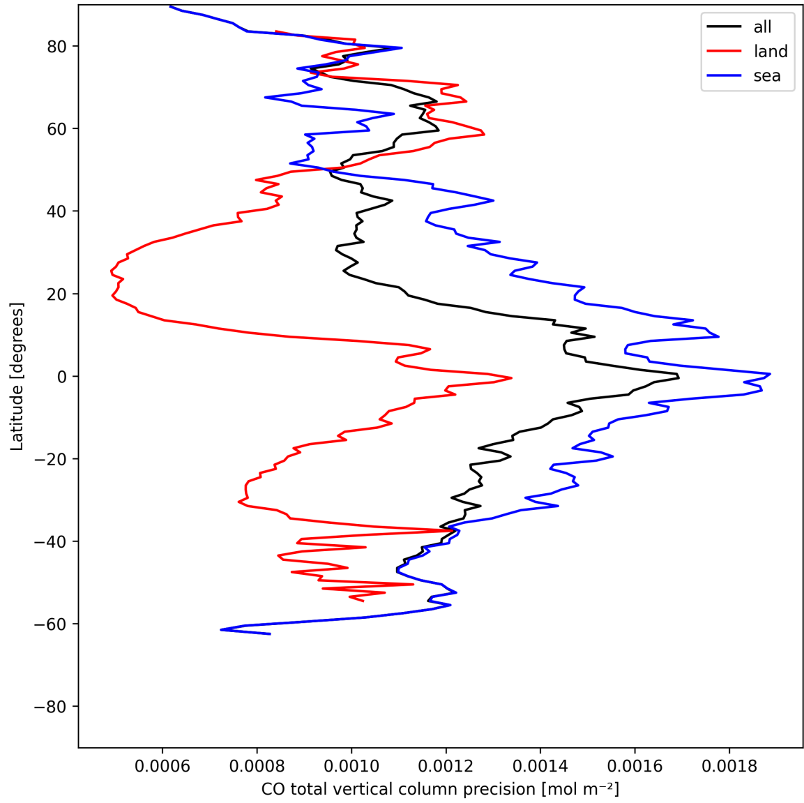
Figure 12: Zonal average of “CO total vertical column precision” for 2025-05-28 to 2025-05-30.
