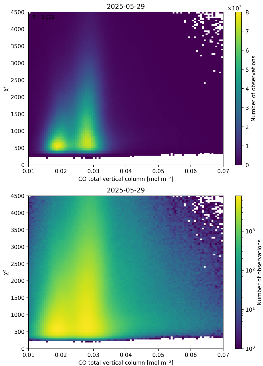
Figure 35: Scatter density plot of “CO total vertical column” against “ \chi^2 ” for 2025-05-28 to 2025-05-30.
