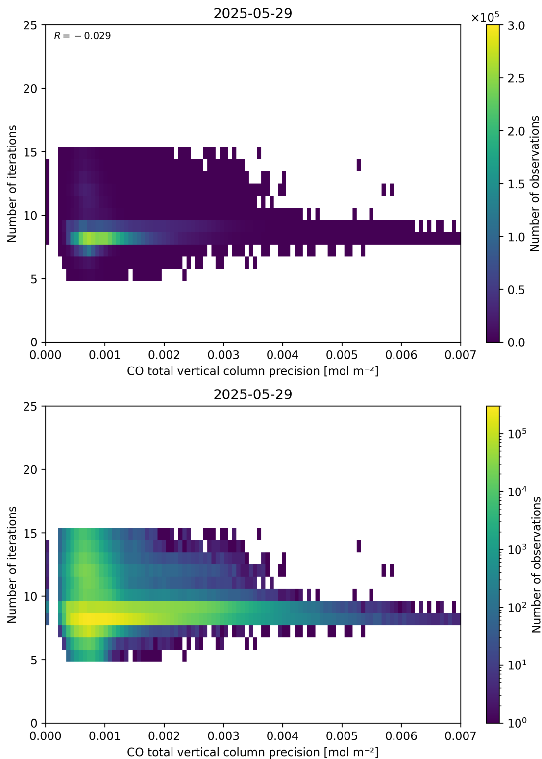
Figure 46: Scatter density plot of “CO total vertical column precision” against “Number of iterations” for 2025-05-28 to 2025-05-30.
