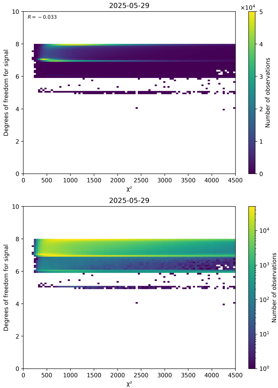
Figure 48: Scatter density plot of “ \chi^2 ” against “Degrees of freedom for signal” for 2025-05-28 to 2025-05-30.
