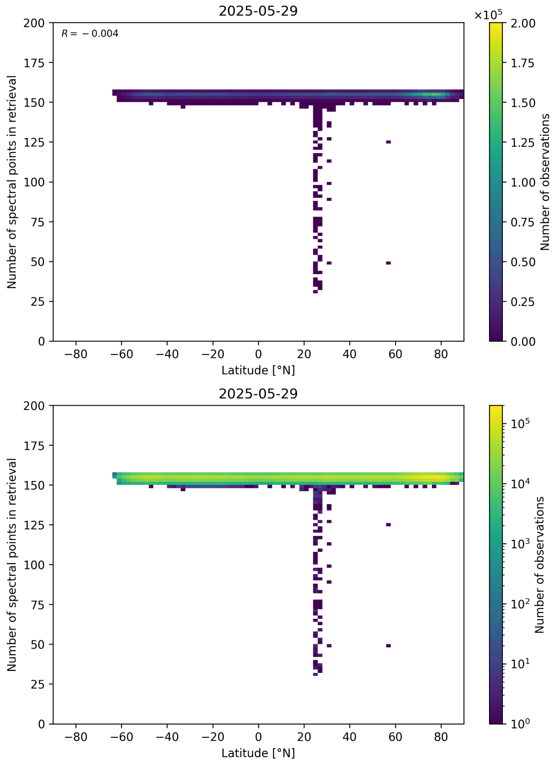
Figure 57: Scatter density plot of “Latitude” against “Number of spectral points in retrieval” for 2025-05-28 to 2025-05-30.
