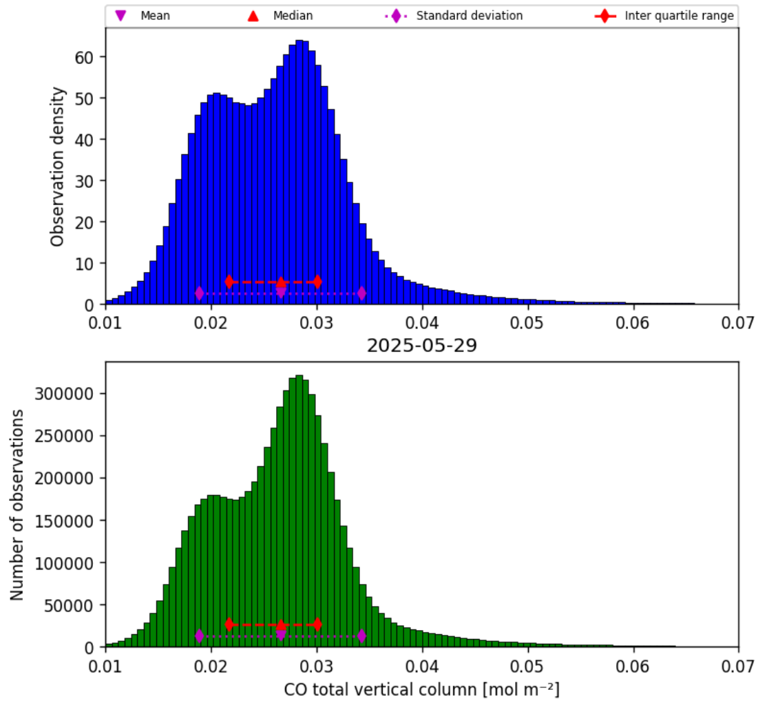
Figure 18: Histogram of “CO total vertical column” for 2025-05-28 to 2025-05-30
