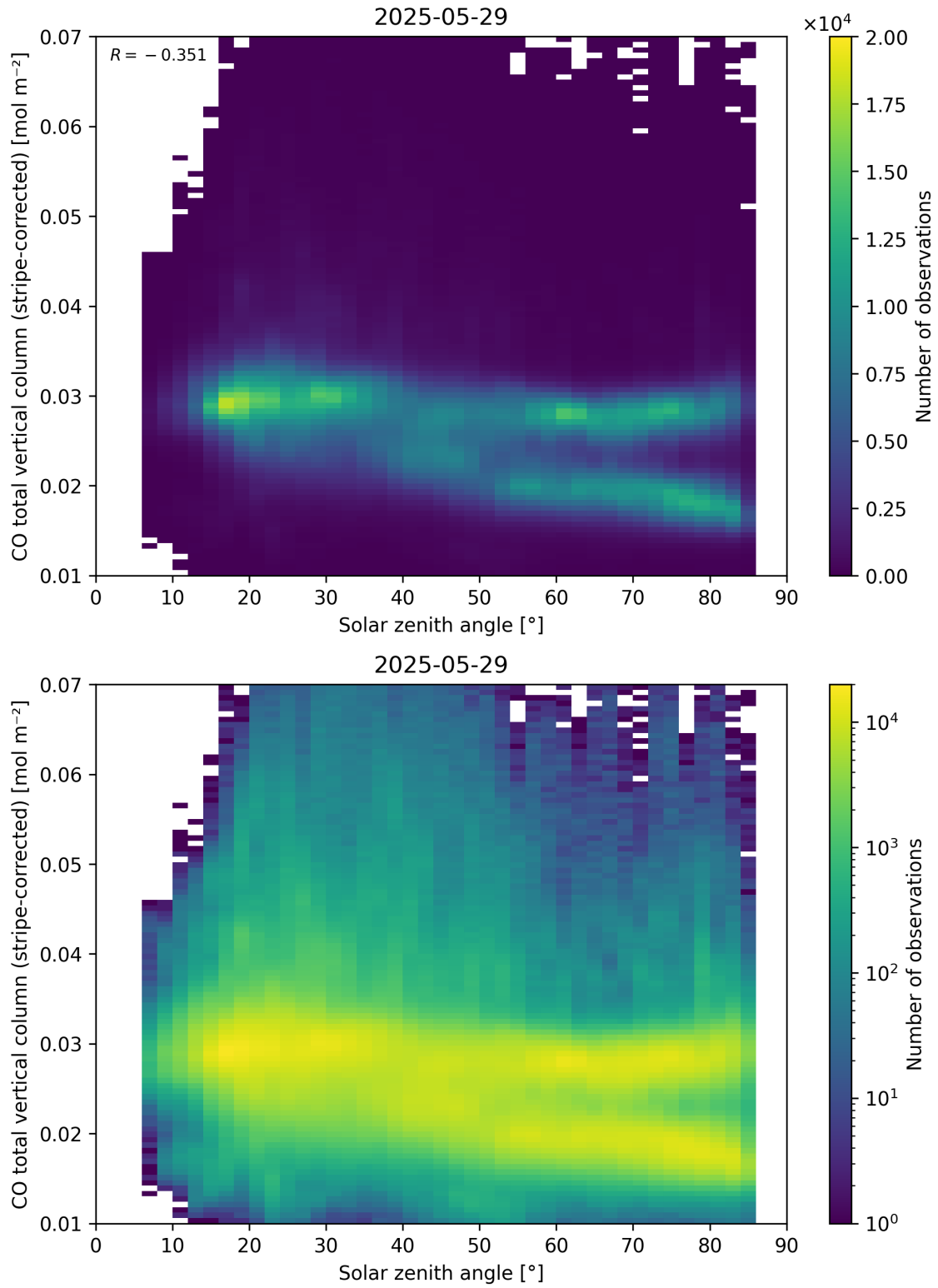
Figure 62: Scatter density plot of “Solar zenith angle” against “CO total vertical column (stripe-corrected)” for 2025-05-28 to 2025-05-30.
