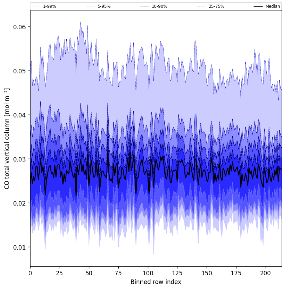
Figure 26: Along track statistics of “CO total vertical column” for 2025-05-28 to 2025-05-30
