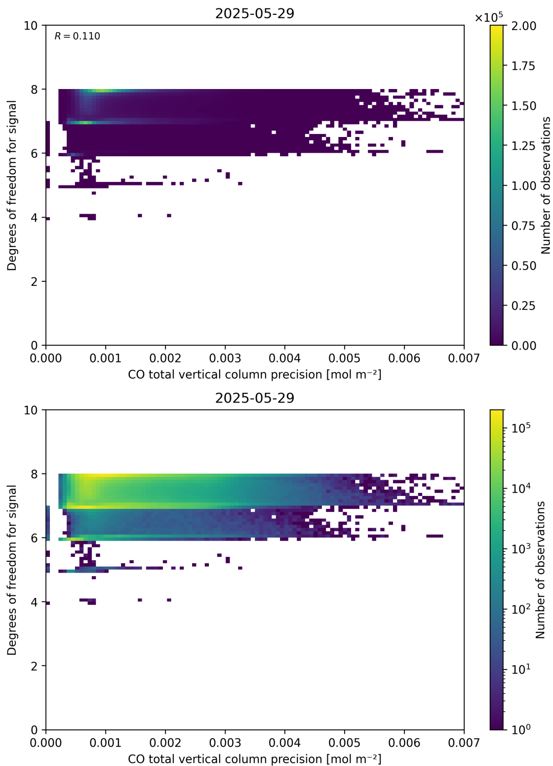
Figure 45: Scatter density plot of “CO total vertical column precision” against “Degrees of freedom for signal” for 2025-05-28 to 2025-05-30.
