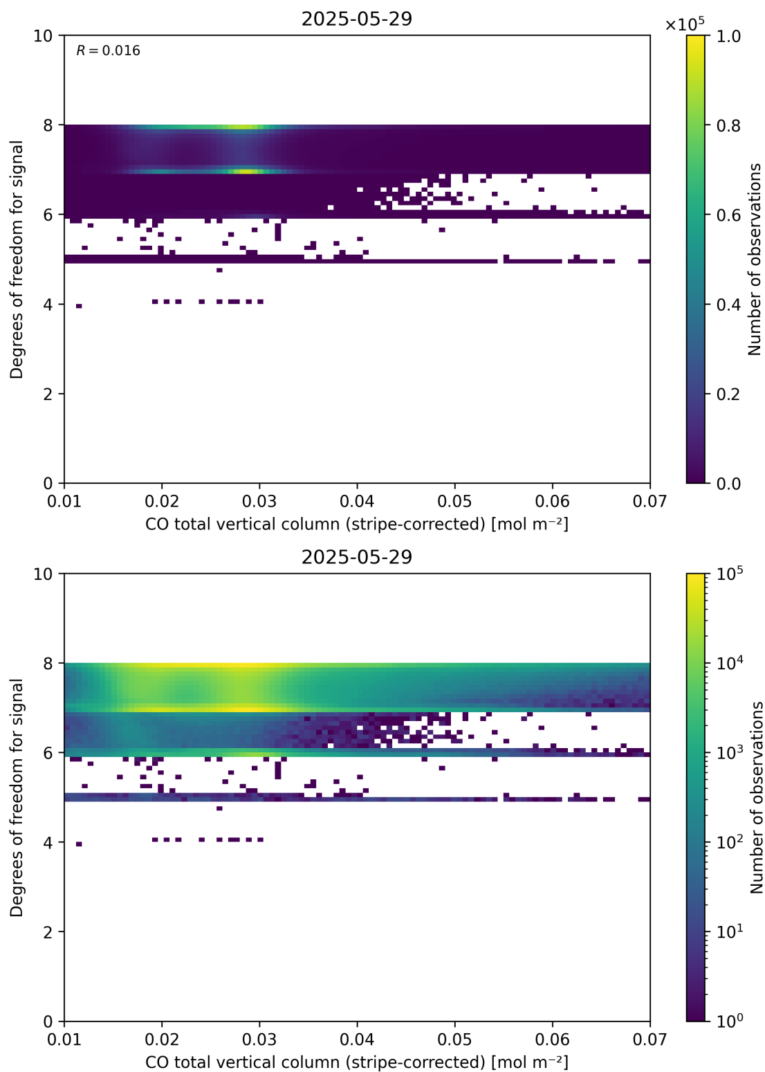
Figure 38: Scatter density plot of “CO total vertical column (stripe-corrected)” against “Degrees of freedom for signal” for 2025-05-28 to 2025-05-30.
