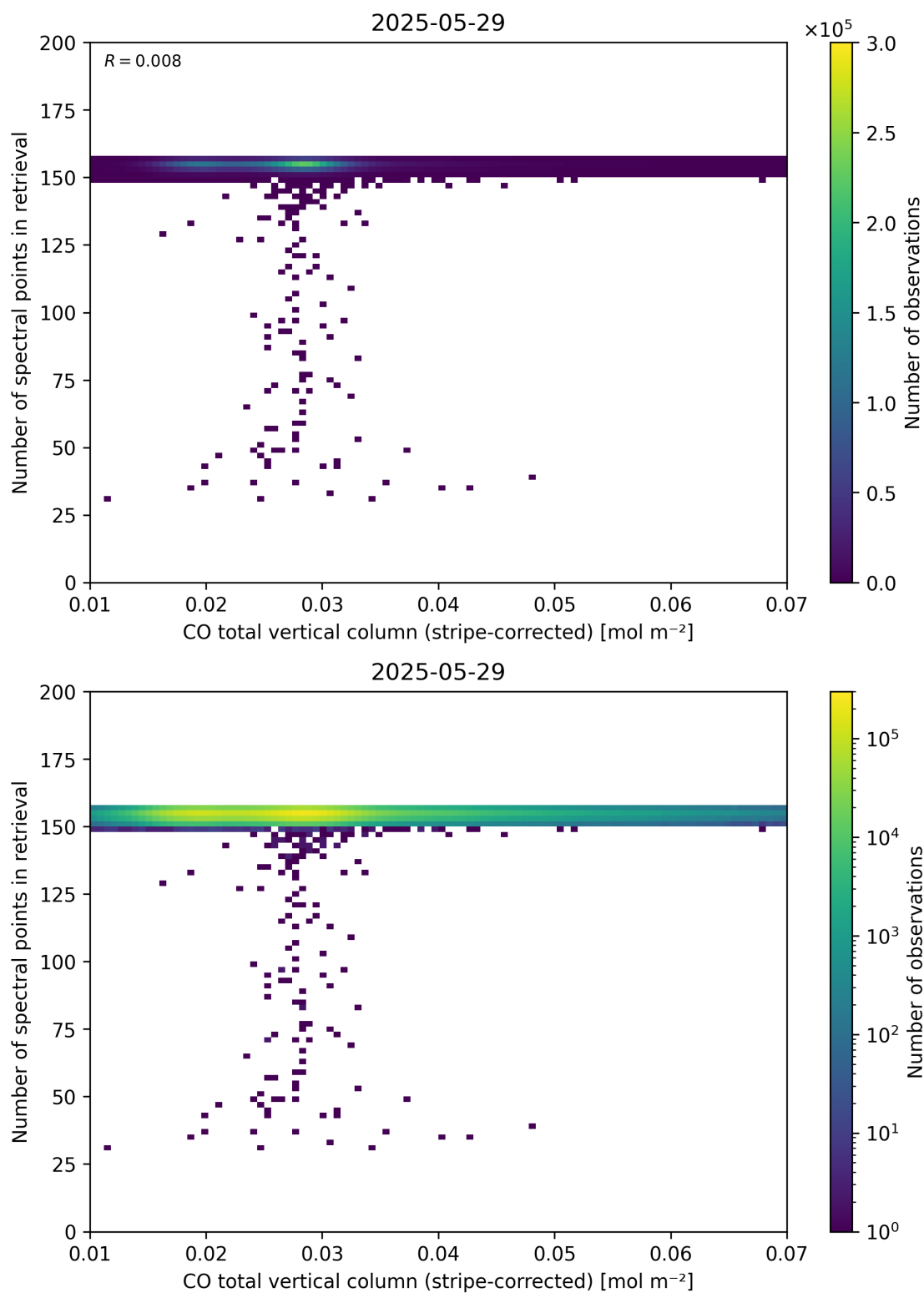
Figure 40: Scatter density plot of “CO total vertical column (stripe-corrected)” against “Number of spectral points in retrieval” for 2025-05-28 to 2025-05-30.
