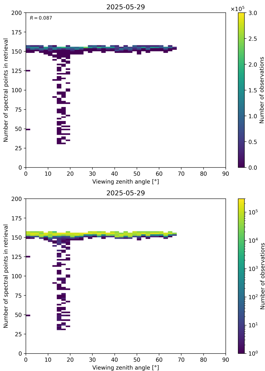
Figure 76: Scatter density plot of “Viewing zenith angle” against “Number of spectral points in retrieval” for 2025-05-28 to 2025-05-30.
