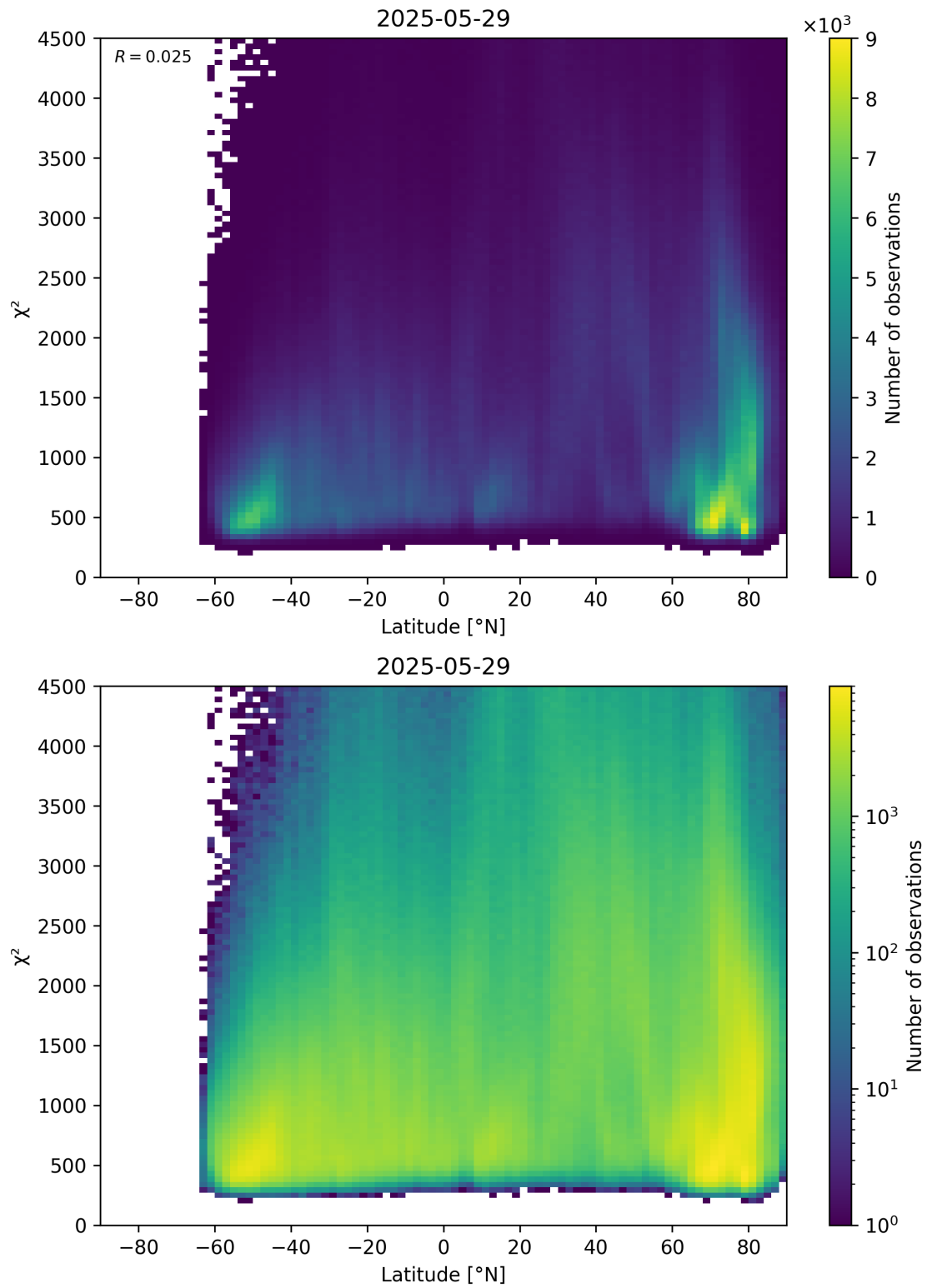
Figure 54: Scatter density plot of “Latitude” against “ \chi^2 ” for 2025-05-28 to 2025-05-30.
