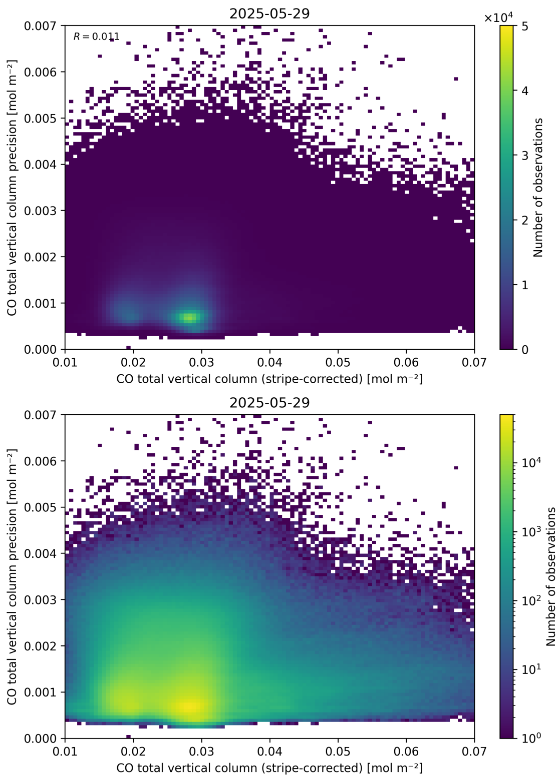
Figure 36: Scatter density plot of “CO total vertical column (stripe-corrected)” against “CO total vertical column precision” for 2025-05-28 to 2025-05-30.
