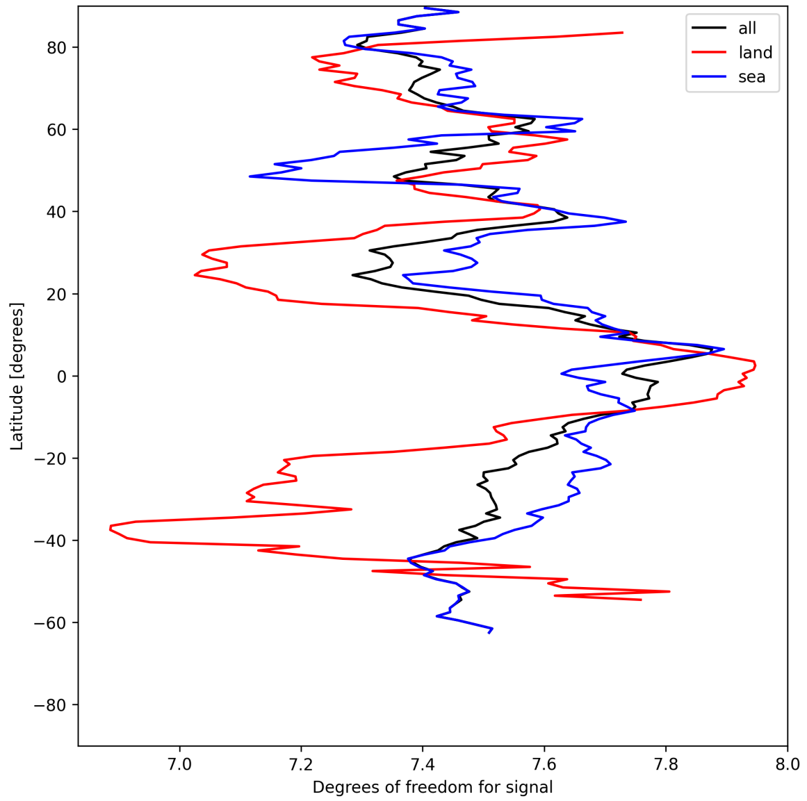
Figure 15: Zonal average of “Degrees of freedom for signal” for 2025-05-28 to 2025-05-30.
