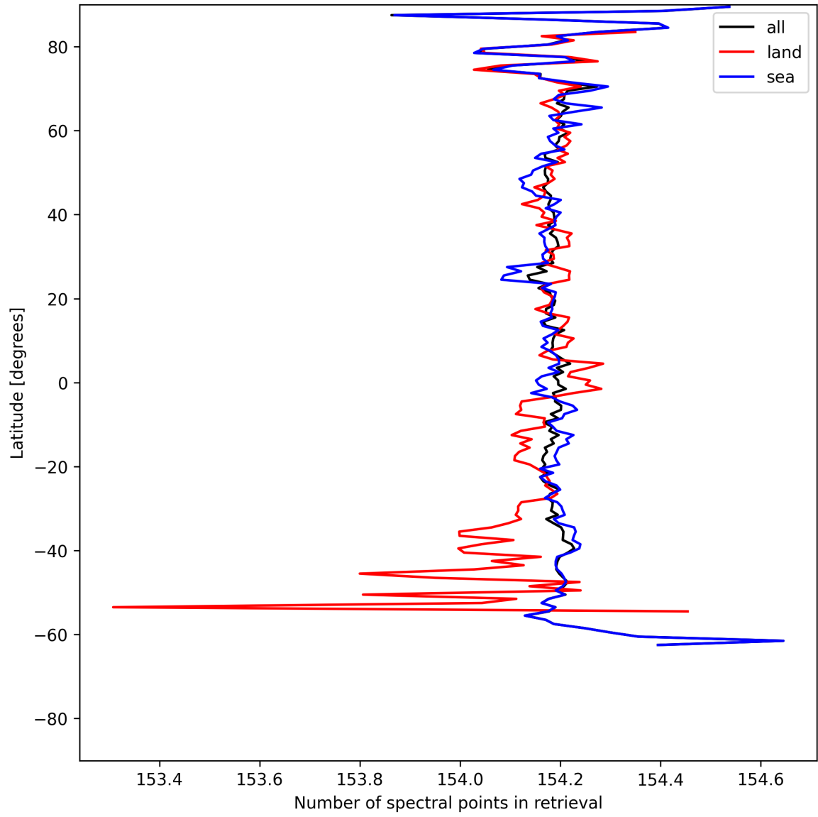
Figure 13: Zonal average of “Number of spectral points in retrieval” for 2025-05-28 to 2025-05-30.
