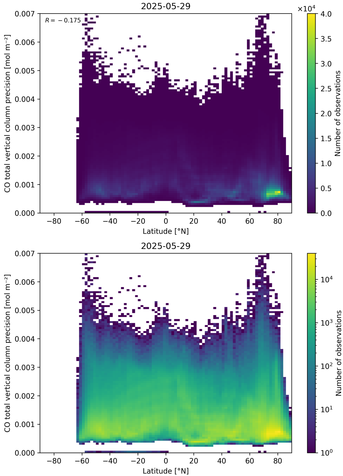
Figure 53: Scatter density plot of “Latitude” against “CO total vertical column precision” for 2025-05-28 to 2025-05-30.
