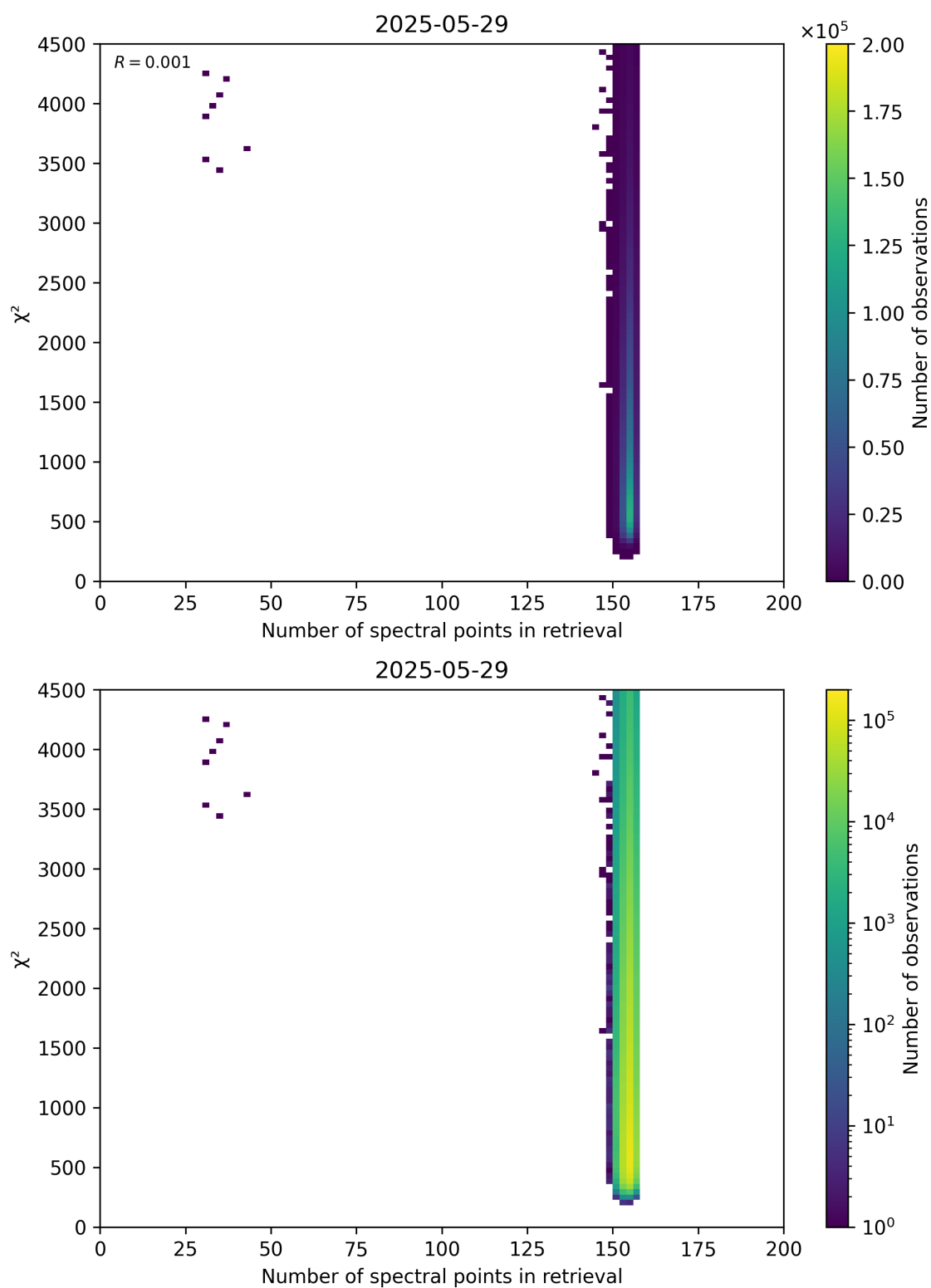
Figure 58: Scatter density plot of “Number of spectral points in retrieval” against “ \chi^2 ” for 2025-05-28 to 2025-05-30.
