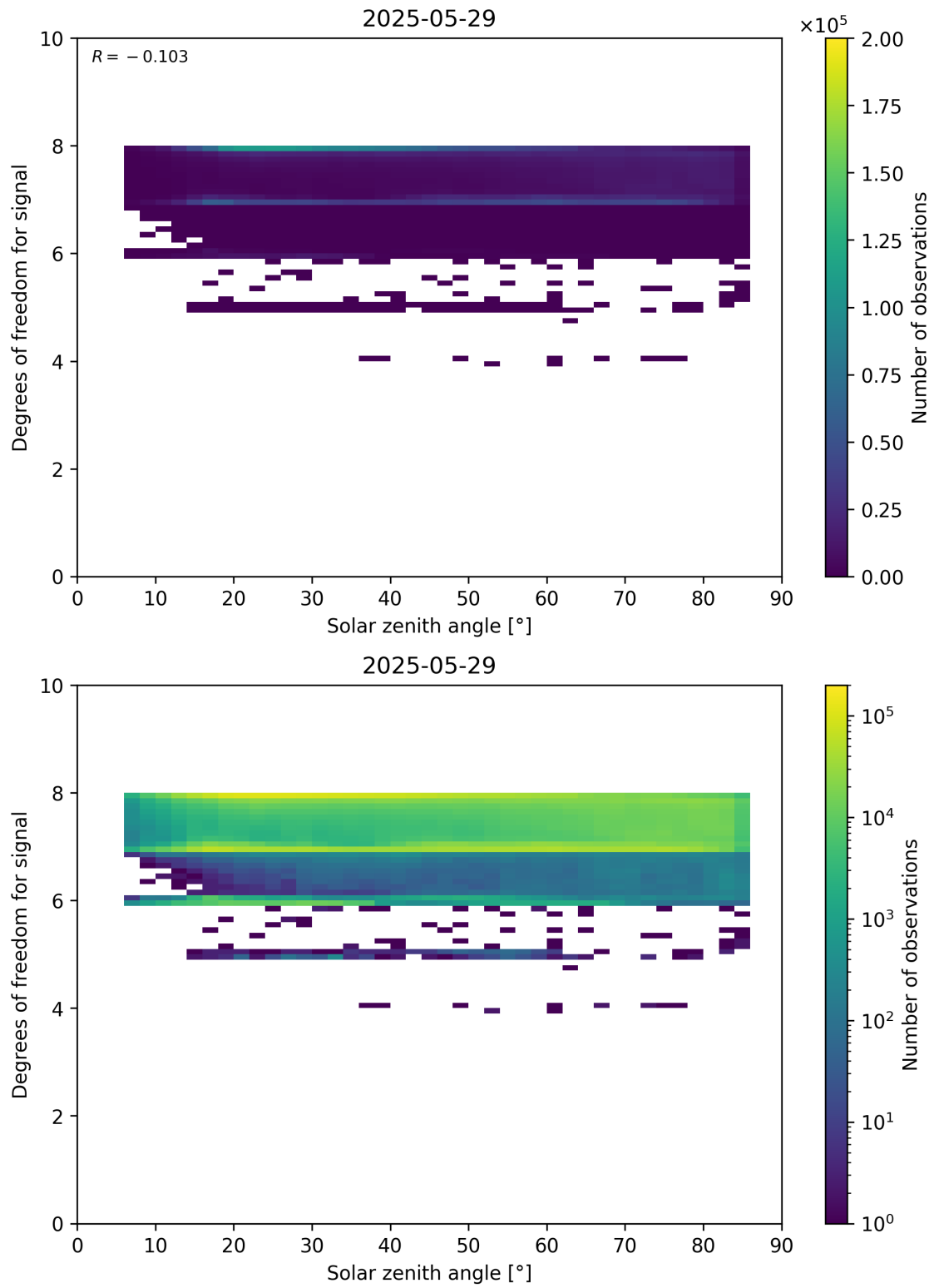
Figure 65: Scatter density plot of “Solar zenith angle” against “Degrees of freedom for signal” for 2025-05-28 to 2025-05-30.
