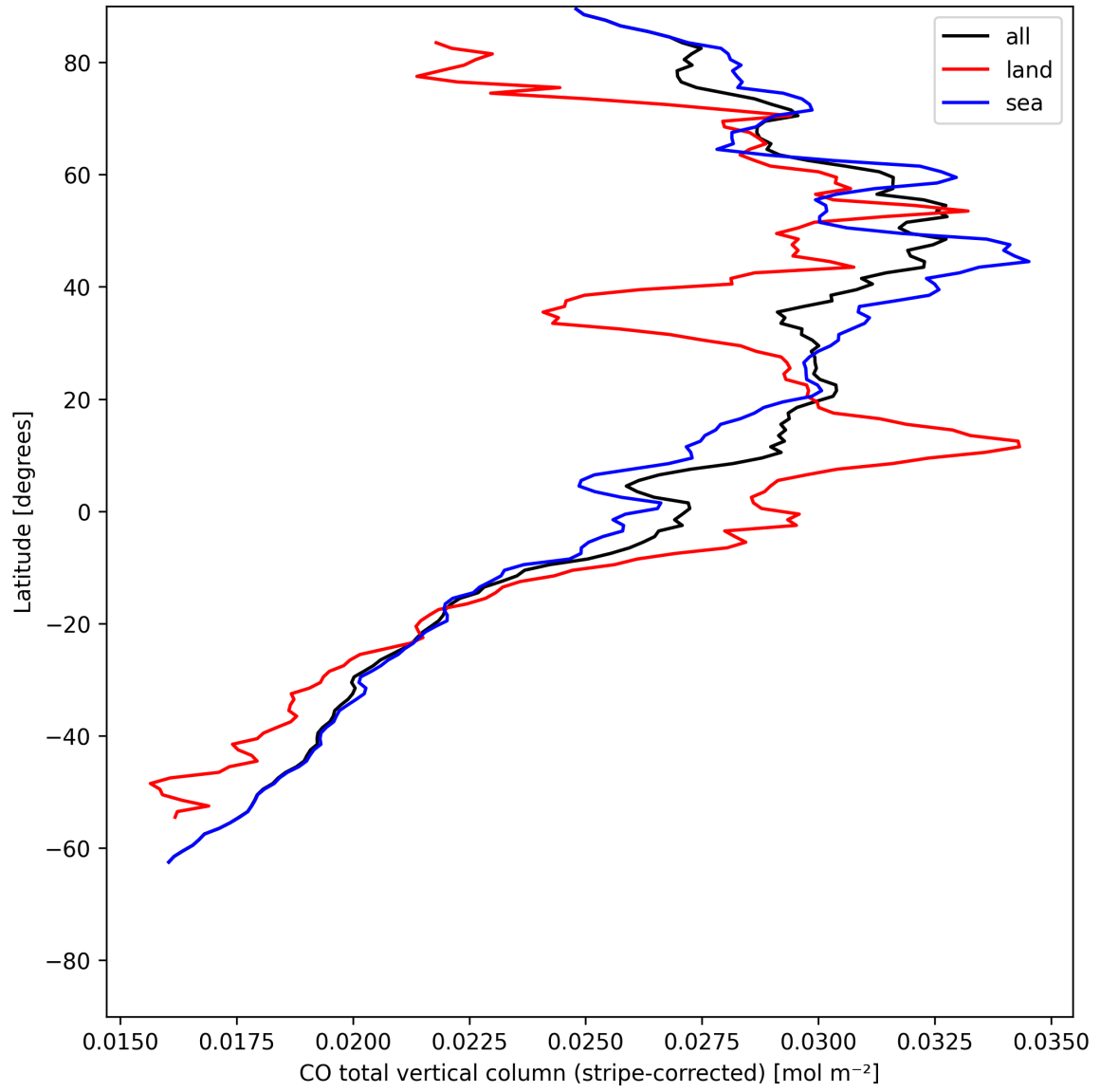
Figure 11: Zonal average of “CO total vertical column (stripe-corrected)” for 2025-05-28 to 2025-05-30.
