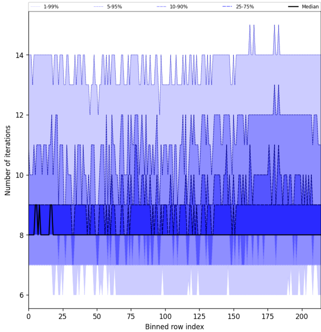
Figure 32: Along track statistics of “Number of iterations” for 2025-05-28 to 2025-05-30
