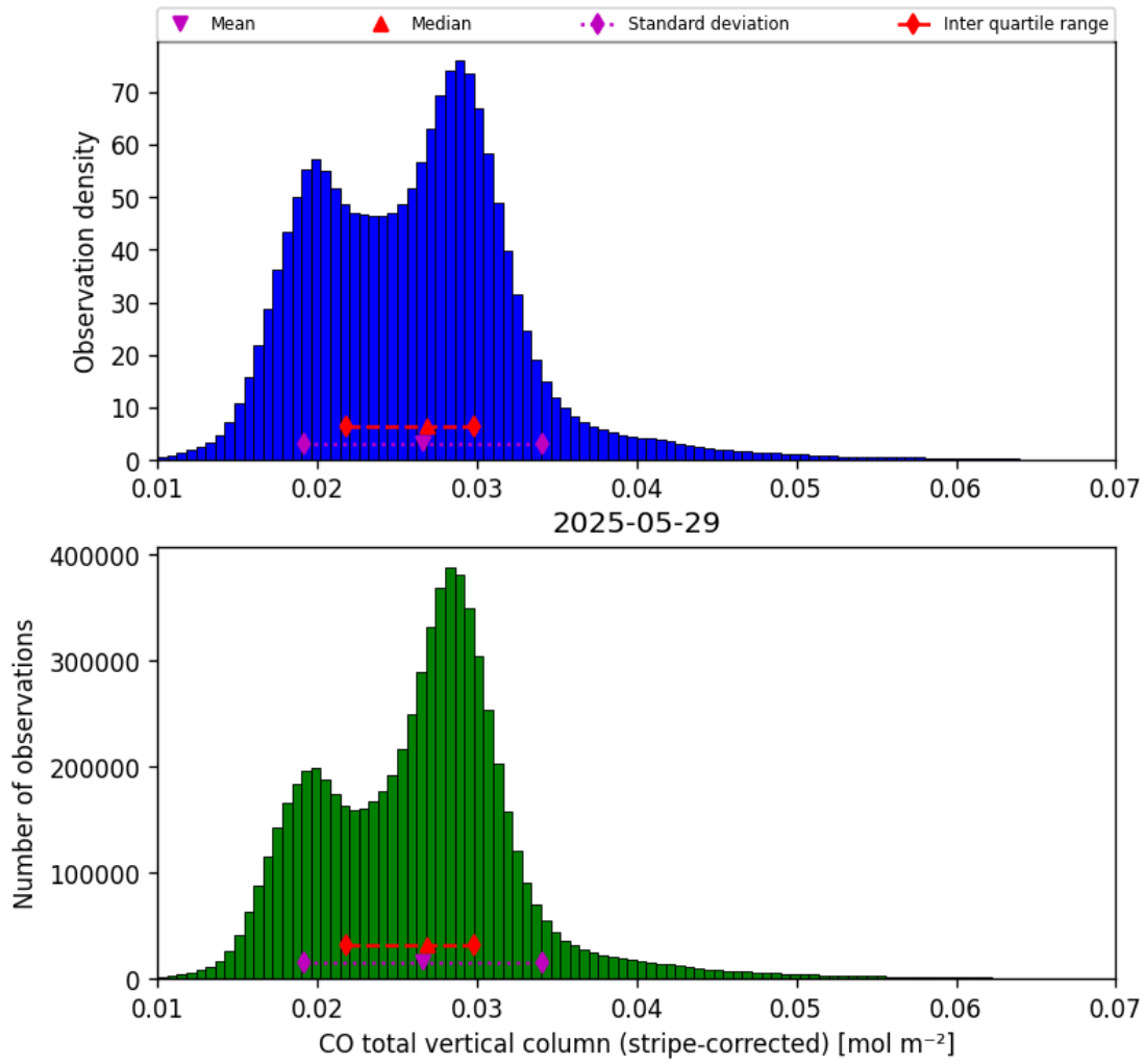
Figure 19: Histogram of “CO total vertical column (stripe-corrected)” for 2025-05-28 to 2025-05-30
