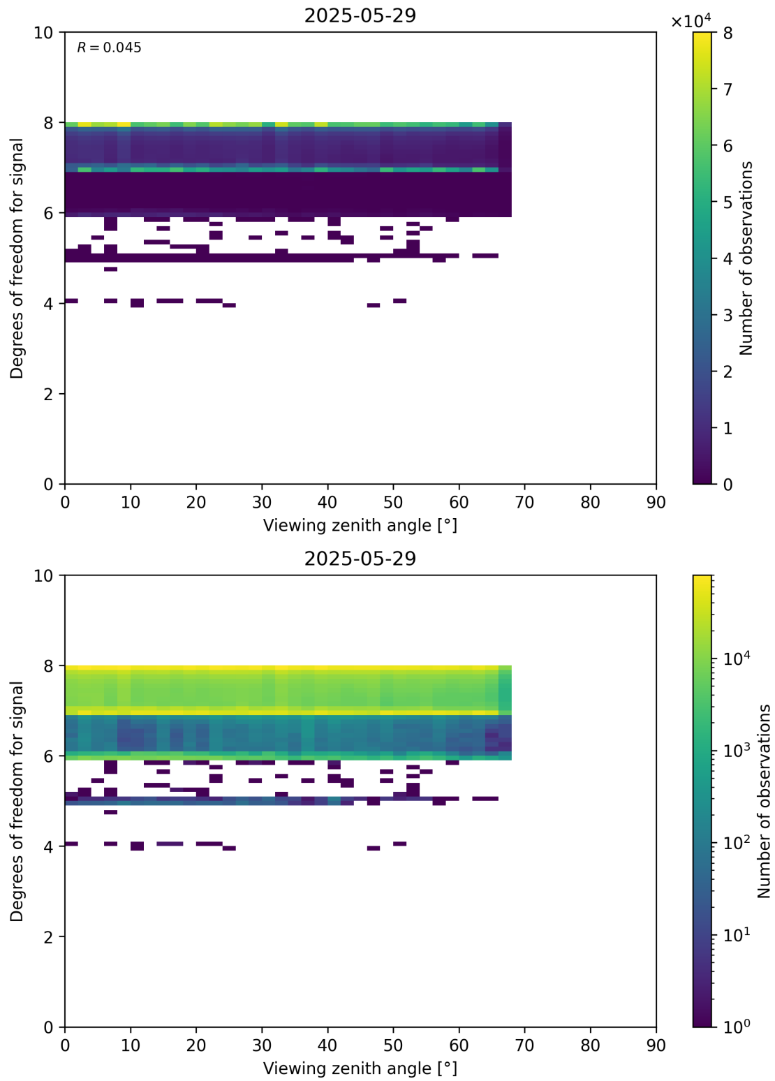
Figure 73: Scatter density plot of “Viewing zenith angle” against “Degrees of freedom for signal” for 2025-05-28 to 2025-05-30.
