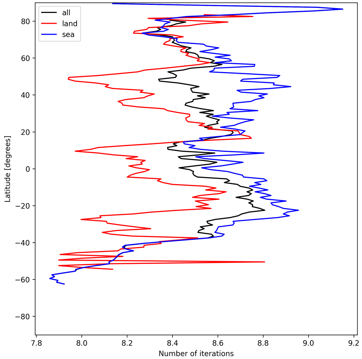
Figure 16: Zonal average of “Number of iterations” for 2025-05-28 to 2025-05-30.
