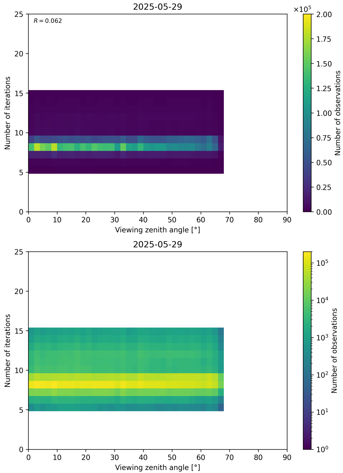
Figure 75: Scatter density plot of “Viewing zenith angle” against “Number of iterations” for 2025-05-28 to 2025-05-30.
