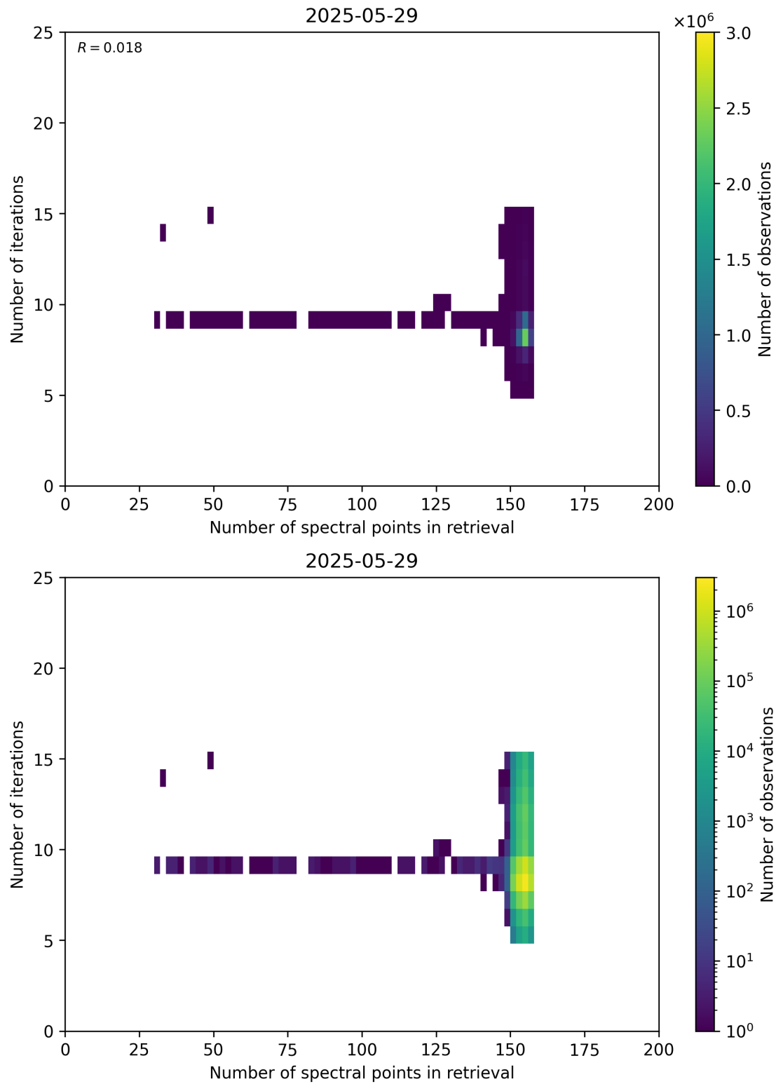
Figure 60: Scatter density plot of “Number of spectral points in retrieval” against “Number of iterations” for 2025-05-28 to 2025-05-30.
