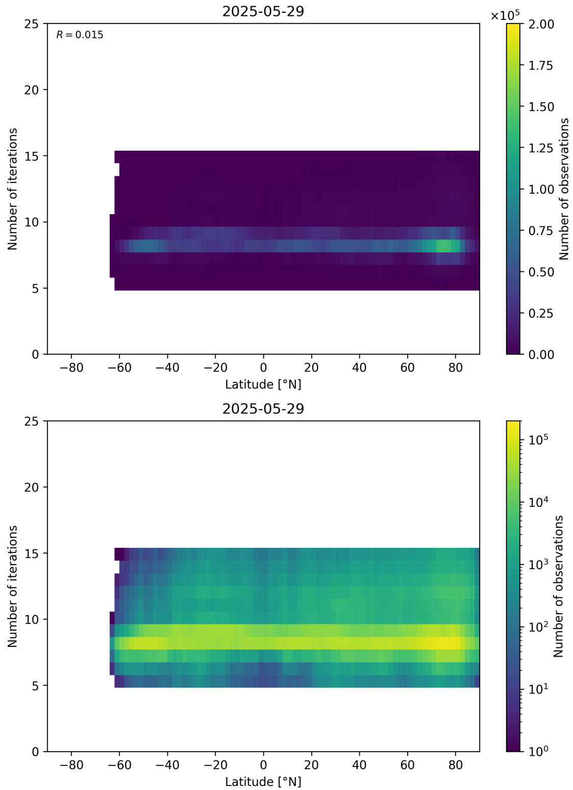
Figure 56: Scatter density plot of “Latitude” against “Number of iterations” for 2025-05-28 to 2025-05-30.
