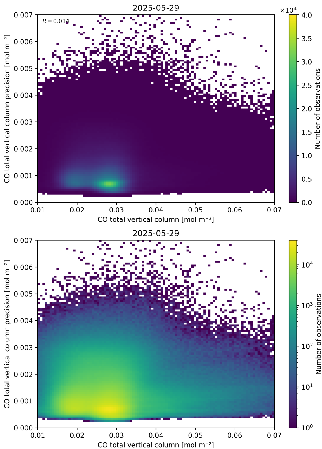
Figure 34: Scatter density plot of “CO total vertical column” against “CO total vertical column precision” for 2025-05-28 to 2025-05-30.
