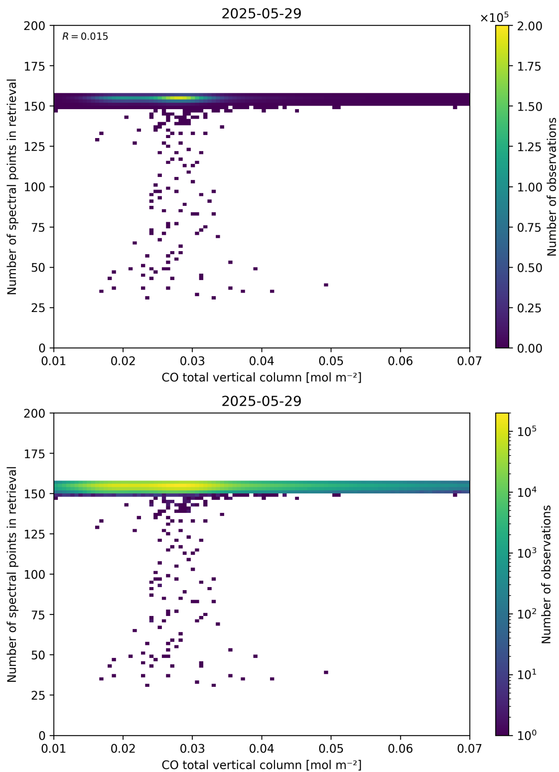
Figure 43: Scatter density plot of “CO total vertical column” against “Number of spectral points in retrieval” for 2025-05-28 to 2025-05-30.
