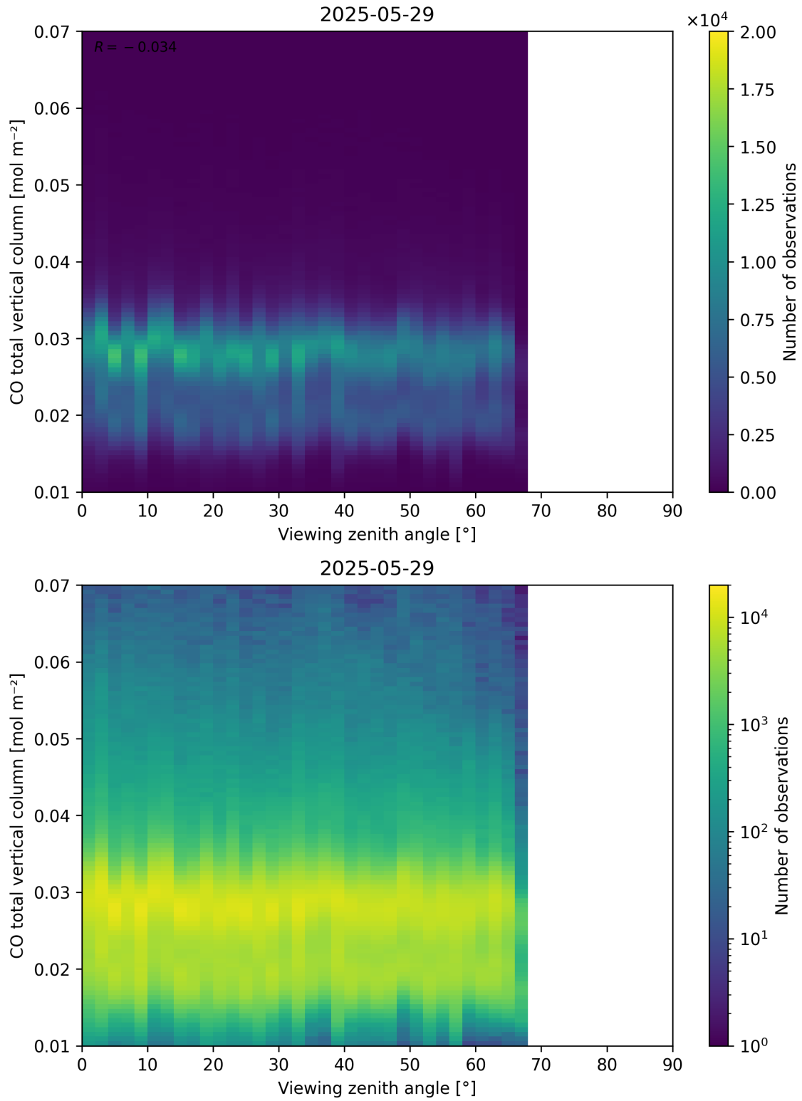
Figure 69: Scatter density plot of “Viewing zenith angle” against “CO total vertical column” for 2025-05-28 to 2025-05-30.
