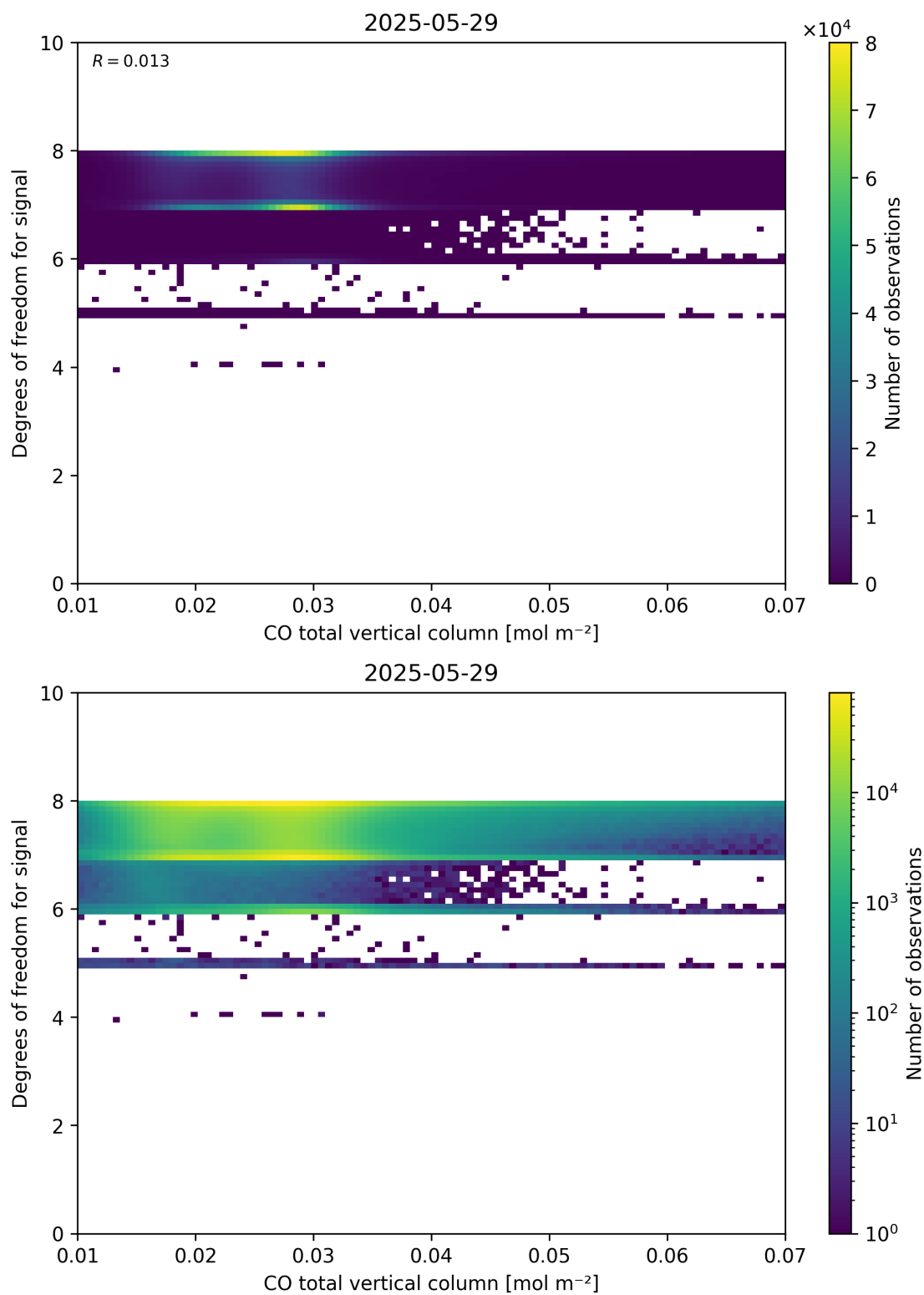
Figure 41: Scatter density plot of “CO total vertical column” against “Degrees of freedom for signal” for 2025-05-28 to 2025-05-30.
