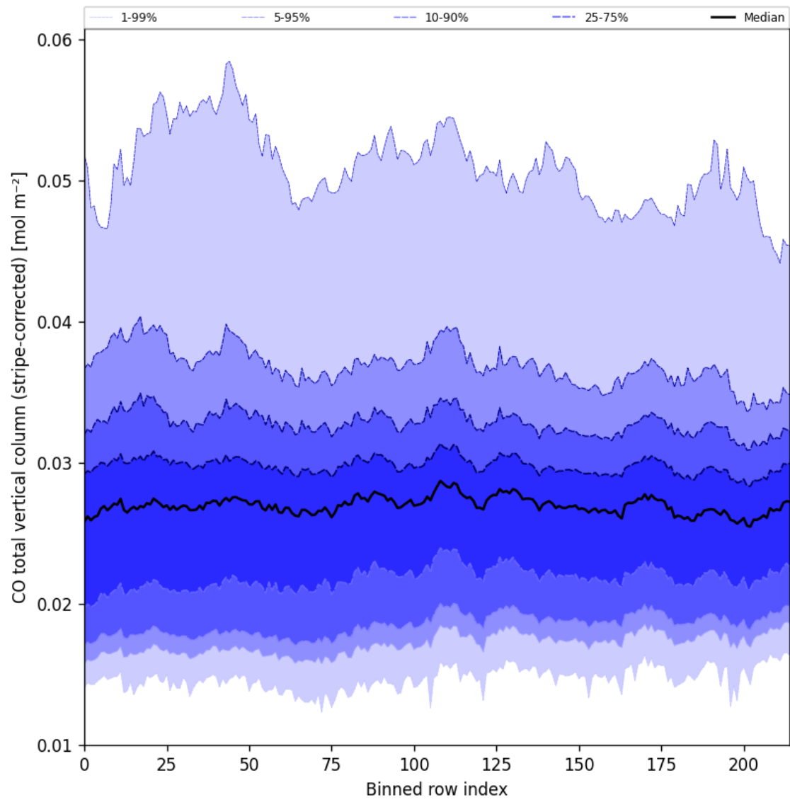
Figure 27: Along track statistics of “CO total vertical column (stripe-corrected)” for 2025-05-28 to 2025-05-30
