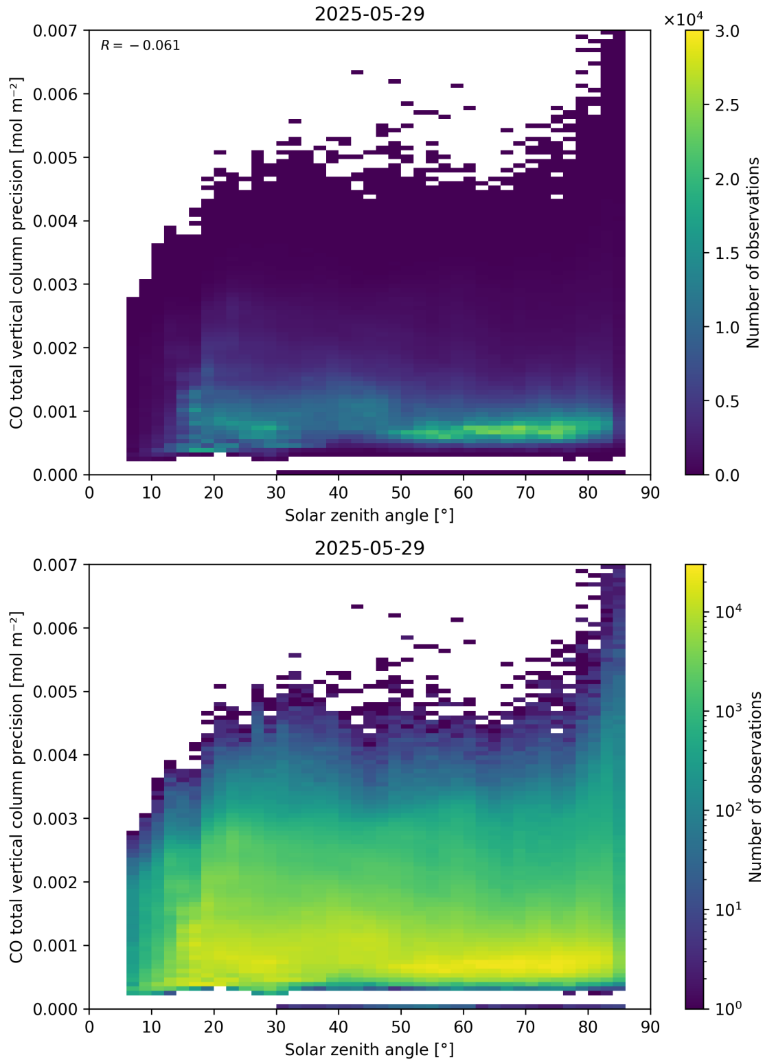
Figure 63: Scatter density plot of “Solar zenith angle” against “CO total vertical column precision” for 2025-05-28 to 2025-05-30.
