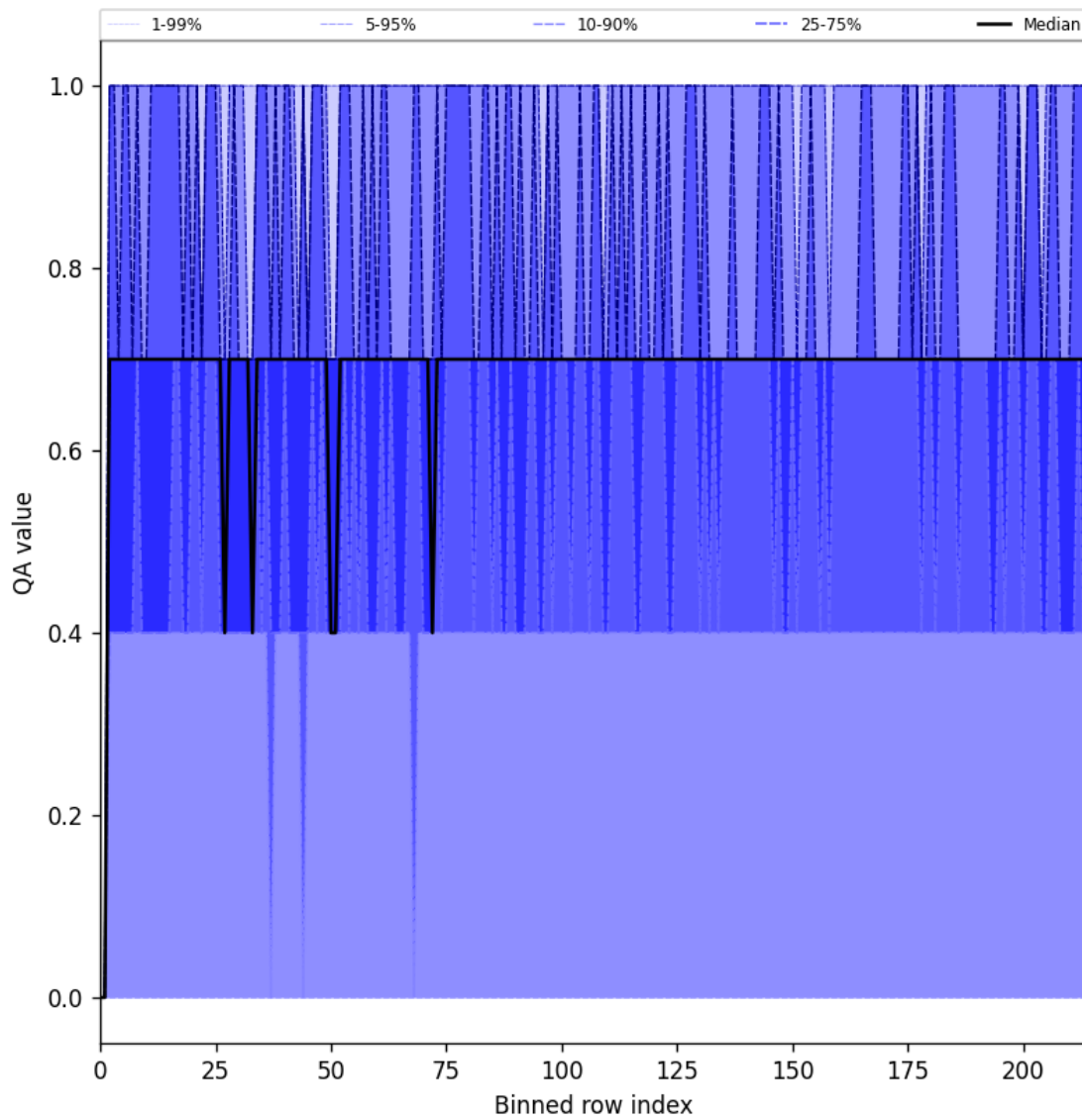
Figure 25: Along track statistics of “QA value” for 2025-05-28 to 2025-05-30
