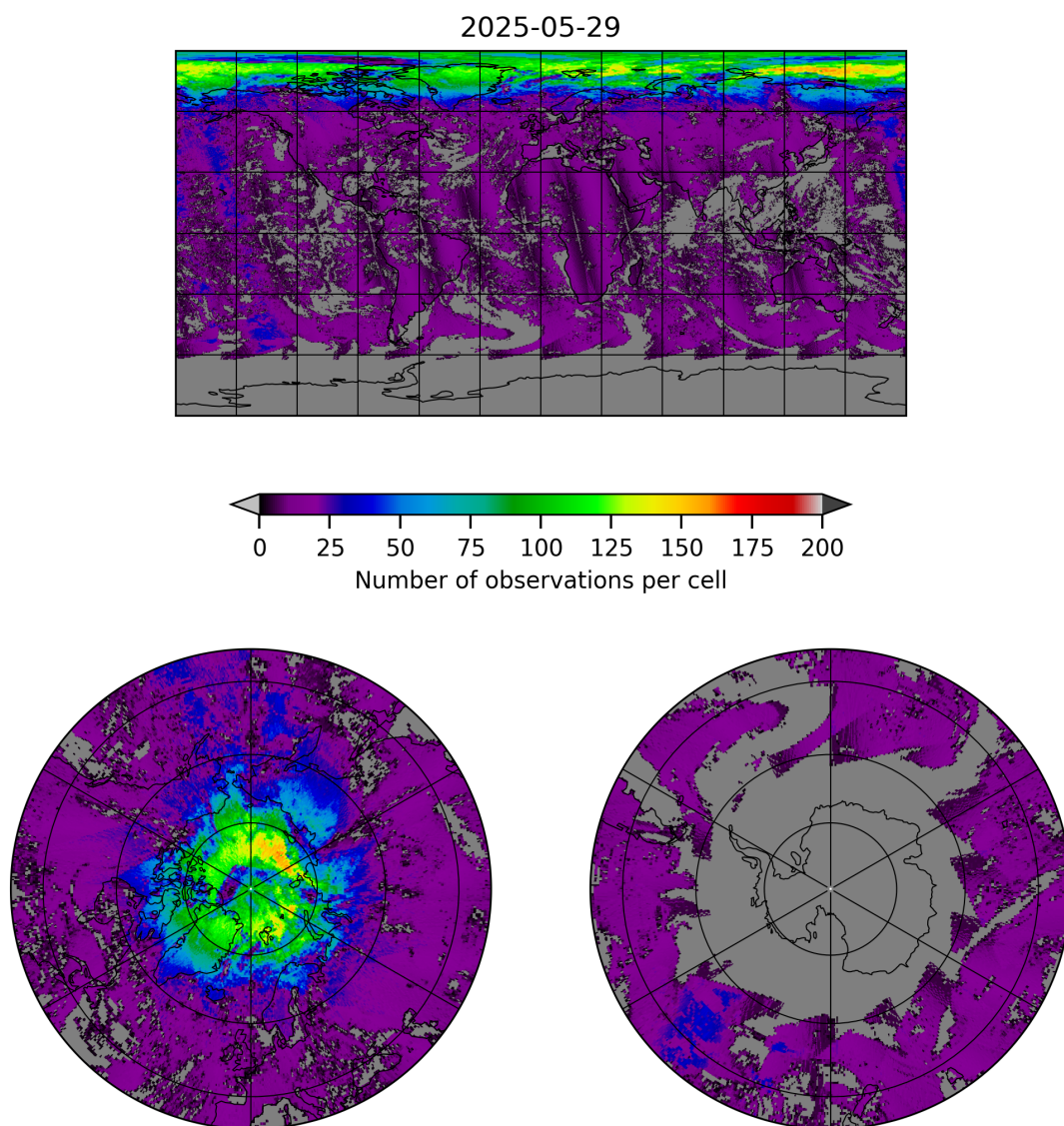
Figure 8: Map of the number of observations for 2025-05-28 to 2025-05-30
