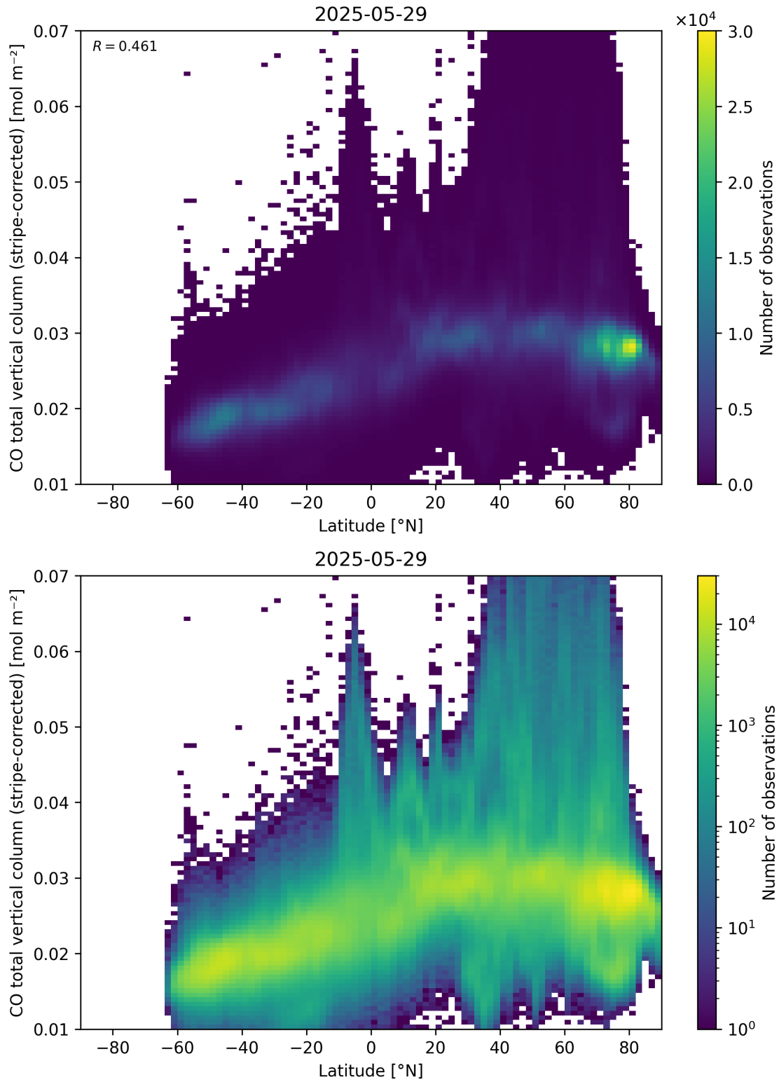
Figure 52: Scatter density plot of “Latitude” against “CO total vertical column (stripe-corrected)” for 2025-05-28 to 2025-05-30.
