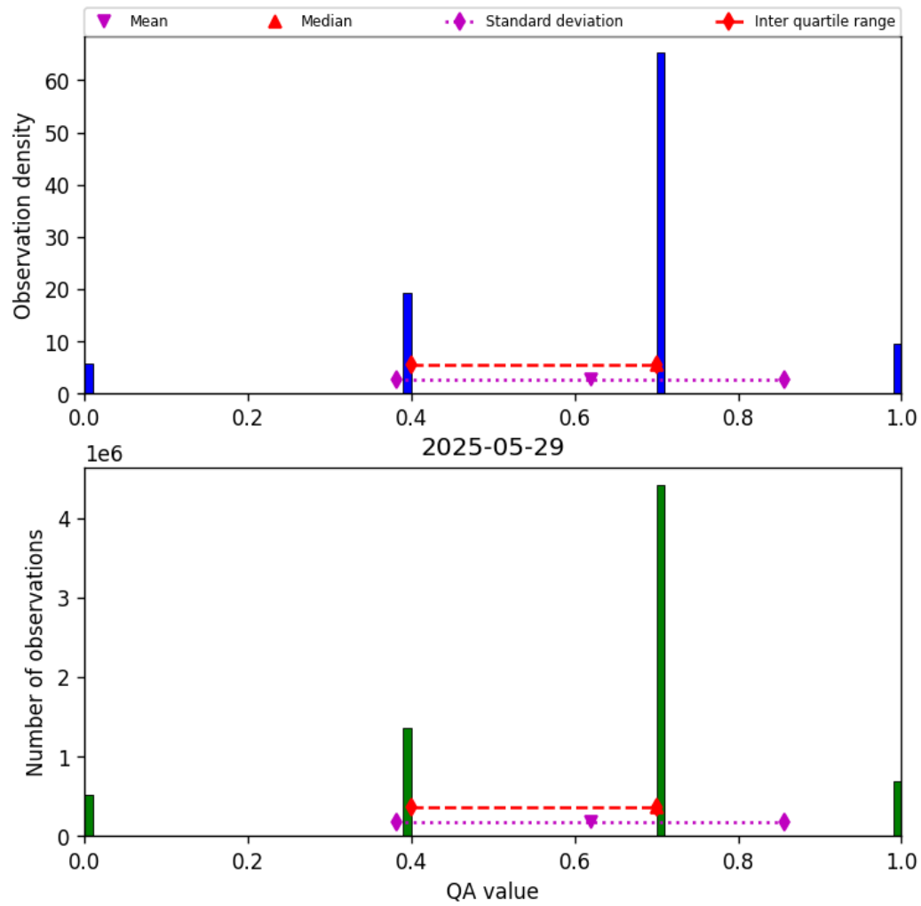
Figure 17: Histogram of “QA value” for 2025-05-28 to 2025-05-30
