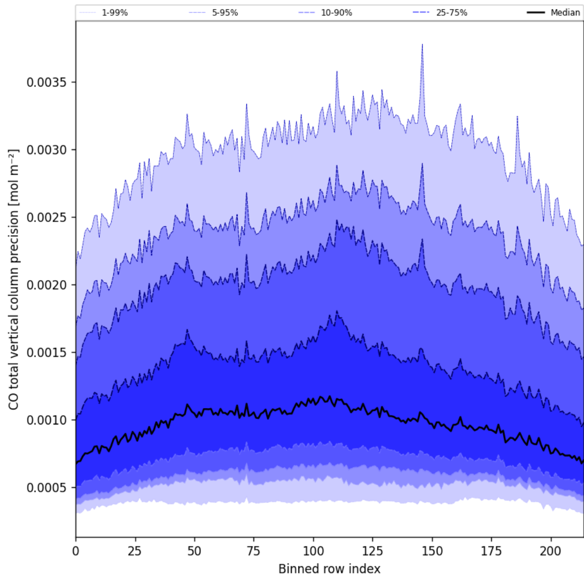
Figure 28: Along track statistics of “CO total vertical column precision” for 2025-05-28 to 2025-05-30
