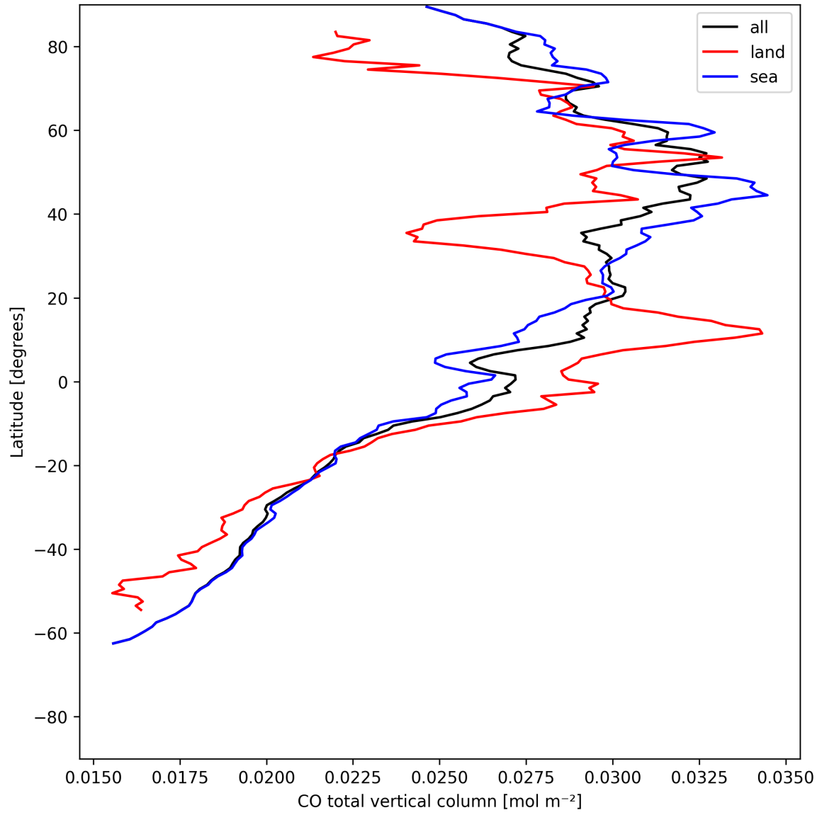
Figure 10: Zonal average of “CO total vertical column” for 2025-05-28 to 2025-05-30.
