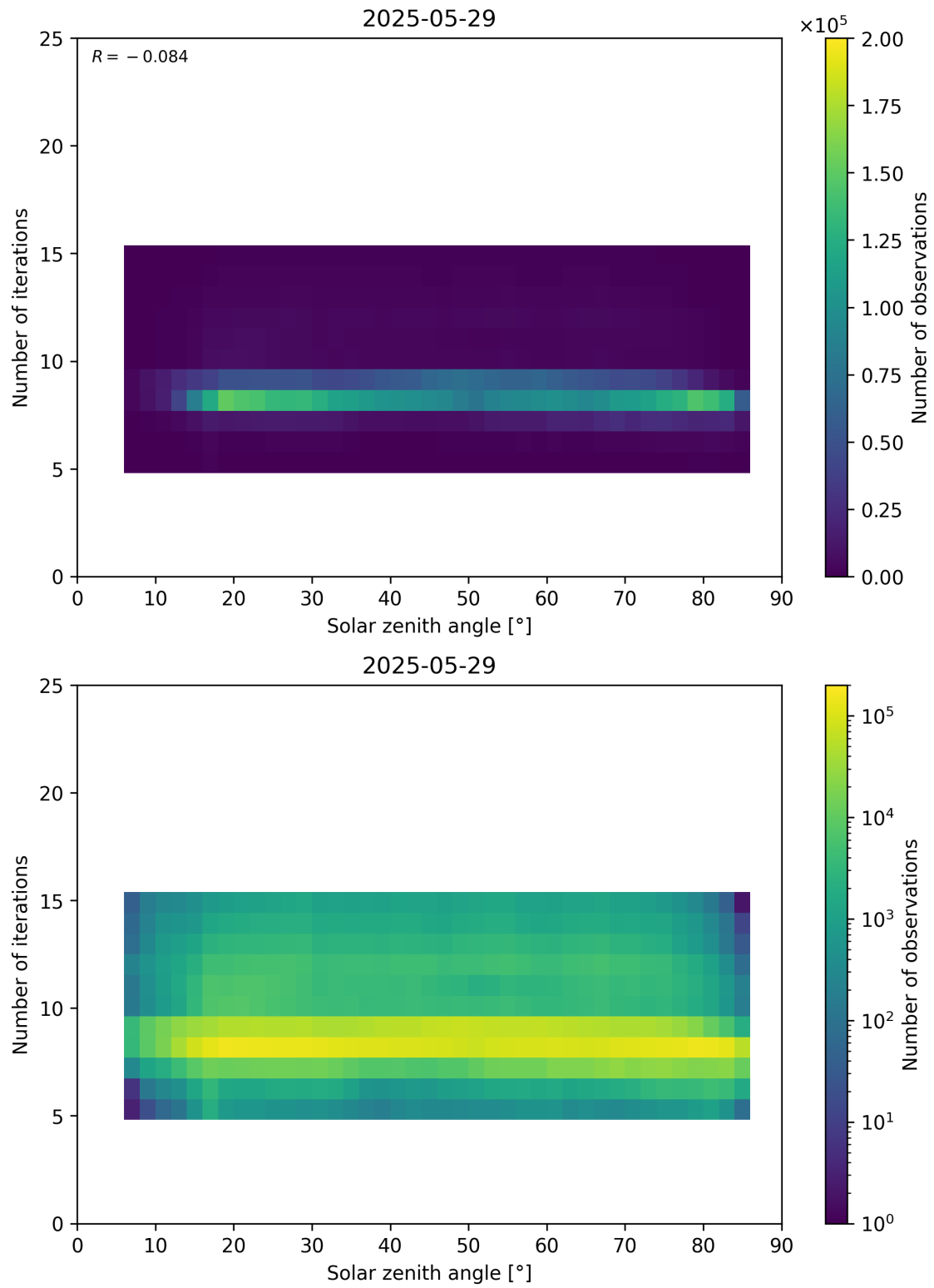
Figure 67: Scatter density plot of “Solar zenith angle” against “Number of iterations” for 2025-05-28 to 2025-05-30.
