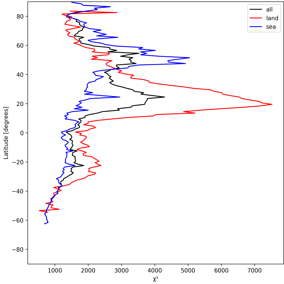
Figure 14: Zonal average of “ \chi^2 ” for 2025-05-28 to 2025-05-30.
