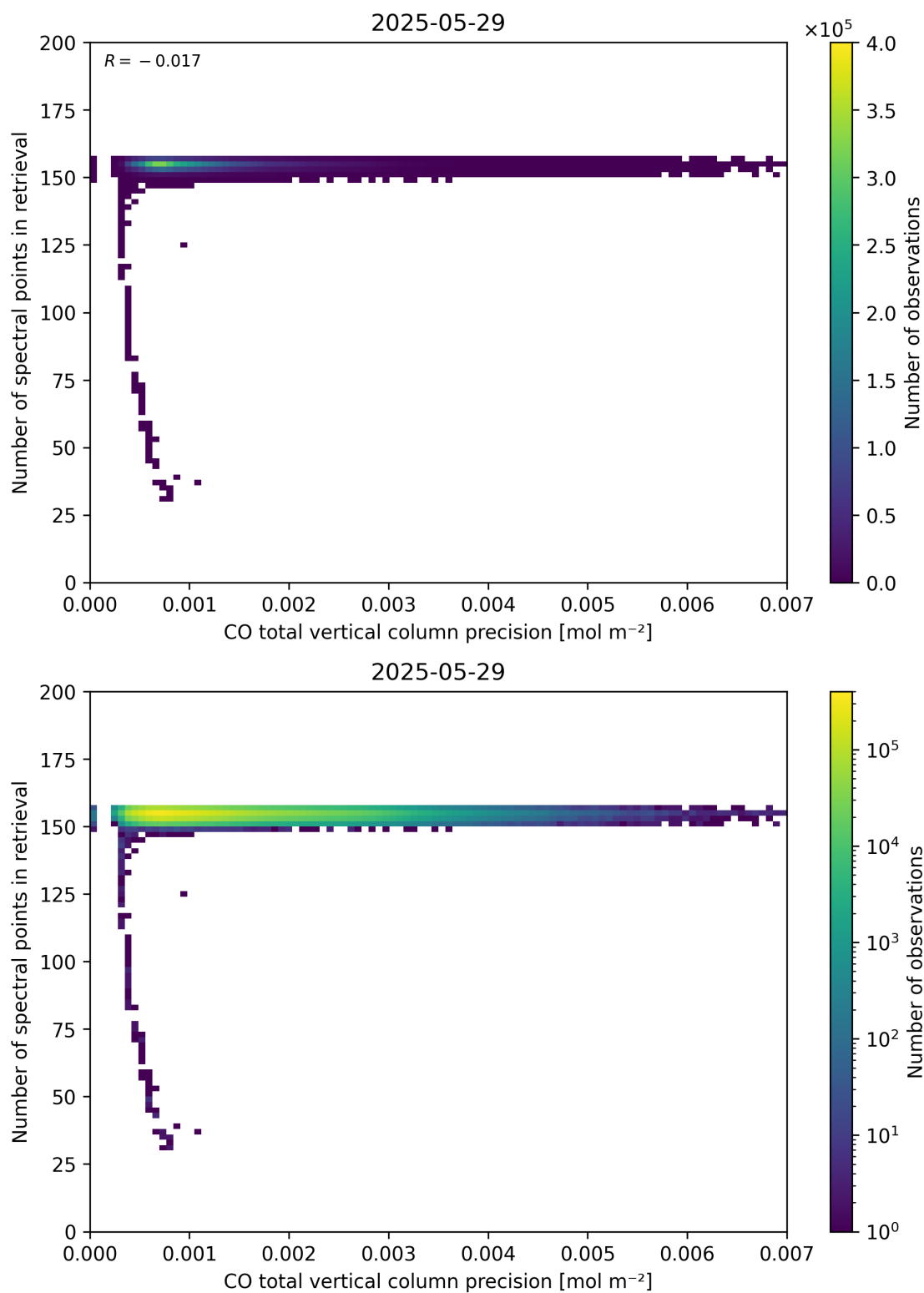
Figure 47: Scatter density plot of “CO total vertical column precision” against “Number of spectral points in retrieval” for 2025-05-28 to 2025-05-30.
