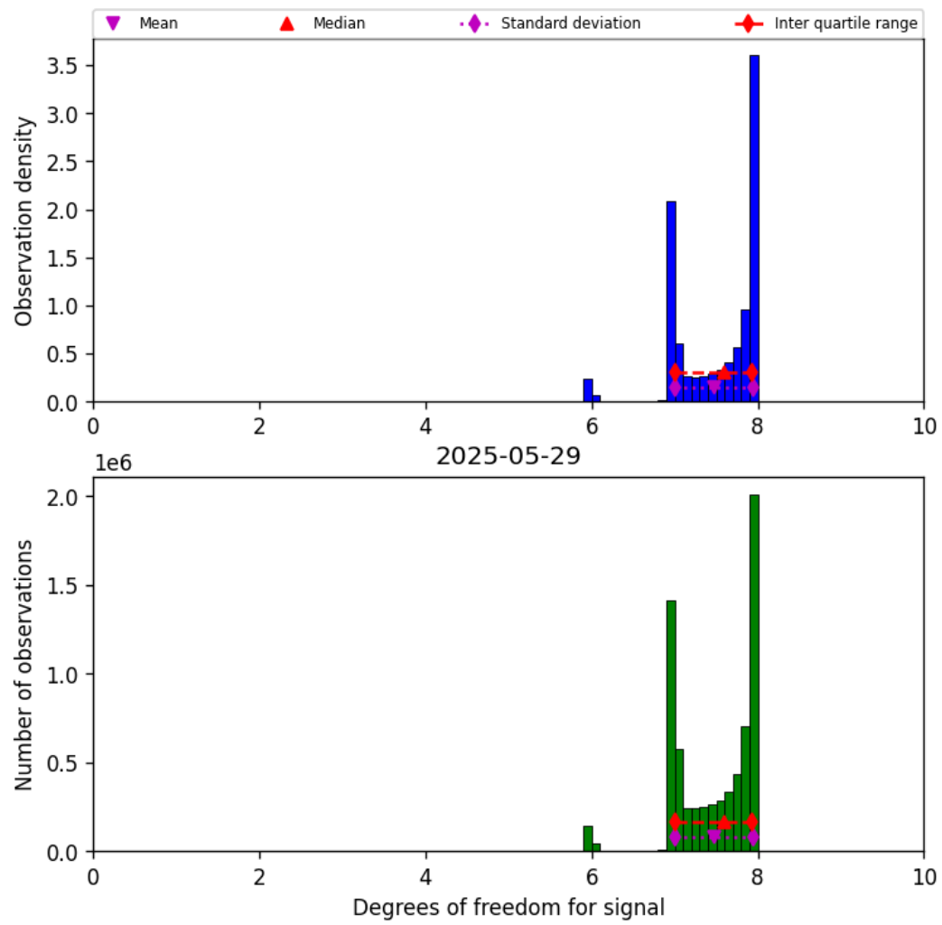
Figure 23: Histogram of “Degrees of freedom for signal” for 2025-05-28 to 2025-05-30
