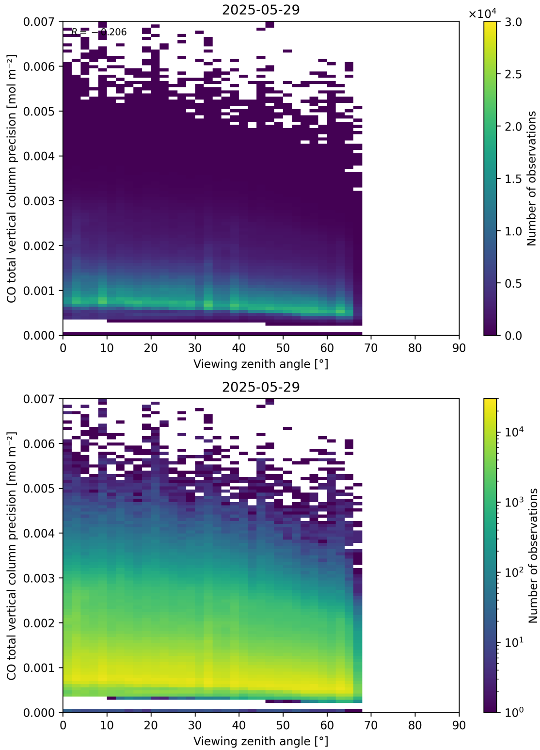
Figure 71: Scatter density plot of “Viewing zenith angle” against “CO total vertical column precision” for 2025-05-28 to 2025-05-30.
