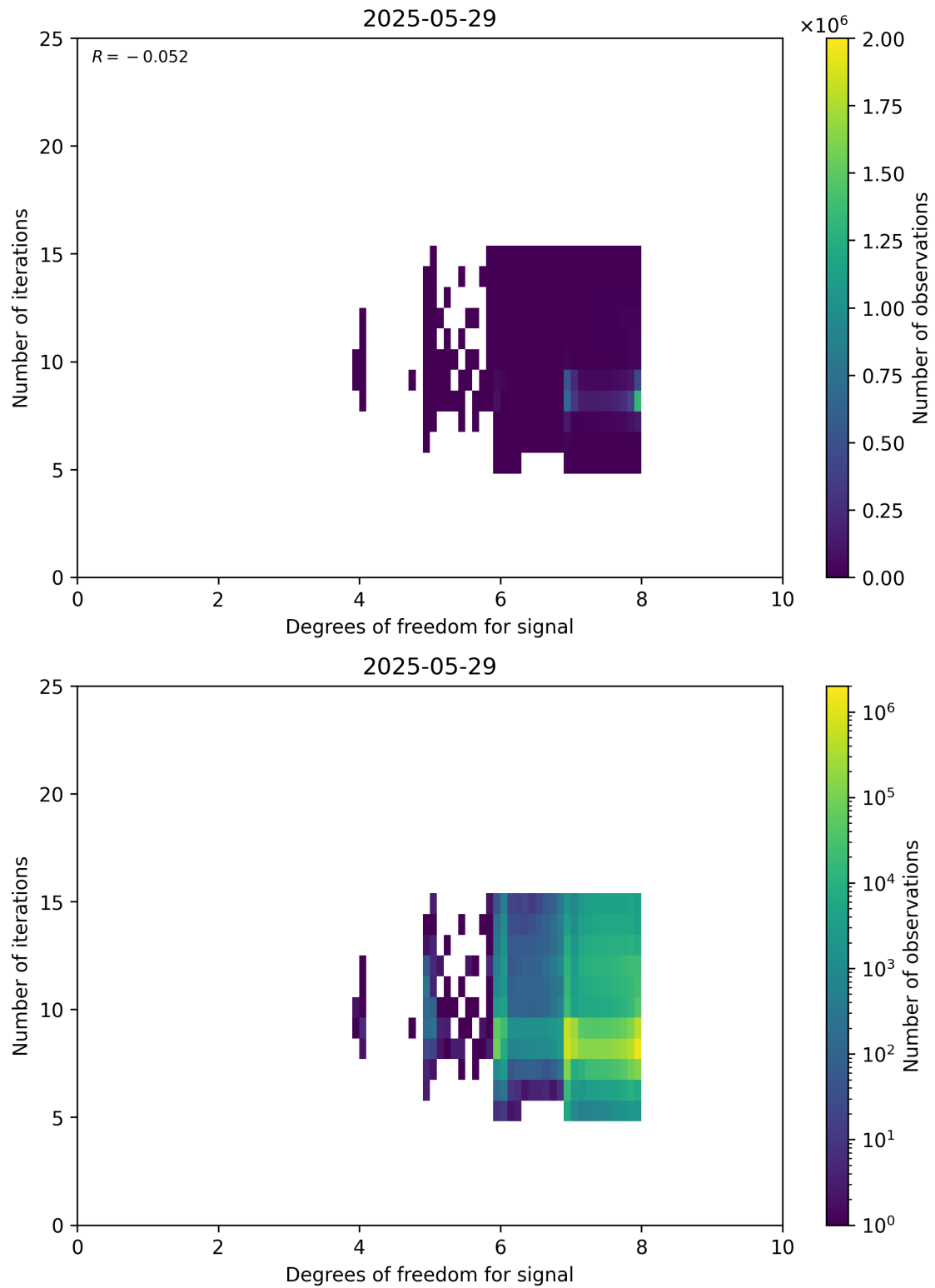
Figure 50: Scatter density plot of “Degrees of freedom for signal” against “Number of iterations” for 2025-05-28 to 2025-05-30.
