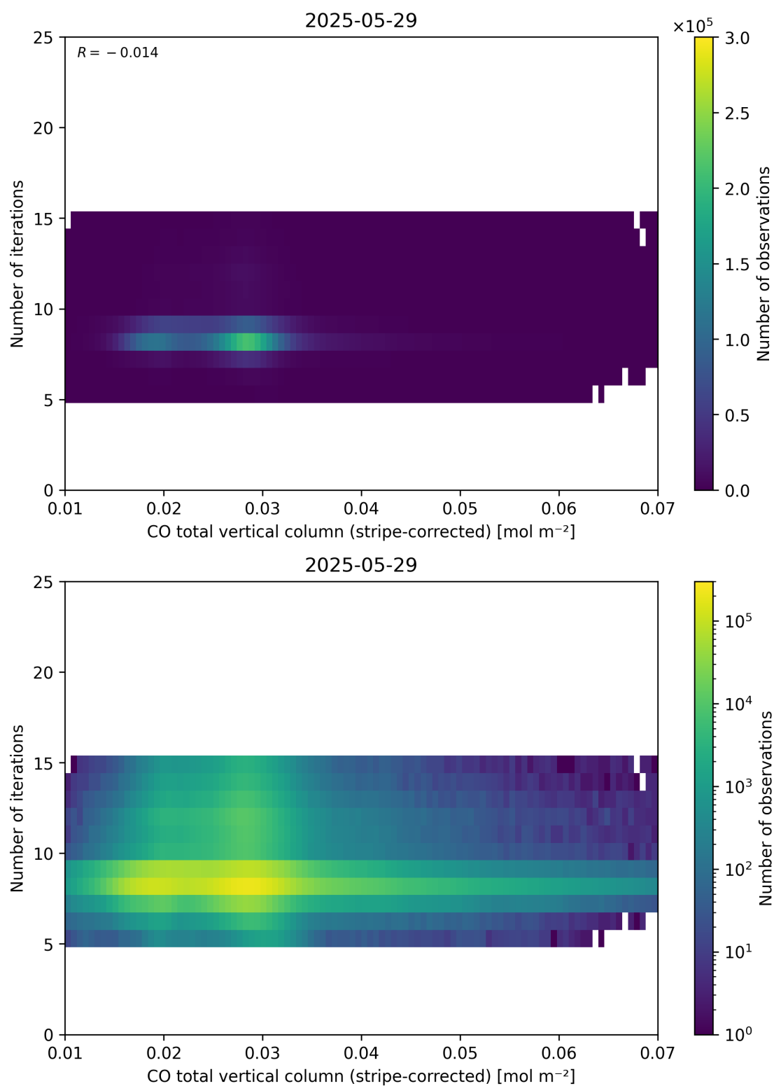
Figure 39: Scatter density plot of “CO total vertical column (stripe-corrected)” against “Number of iterations” for 2025-05-28 to 2025-05-30.
