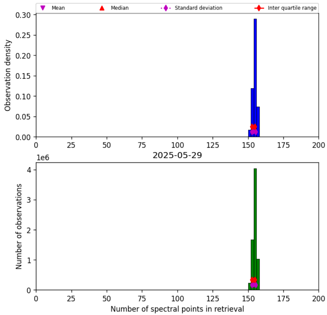
Figure 21: Histogram of “Number of spectral points in retrieval” for 2025-05-28 to 2025-05-30
