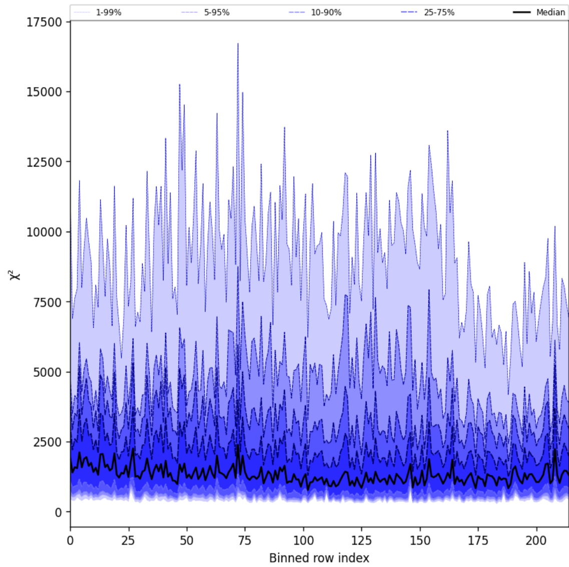
Figure 30: Along track statistics of “ \chi^2 ” for 2025-05-28 to 2025-05-30
