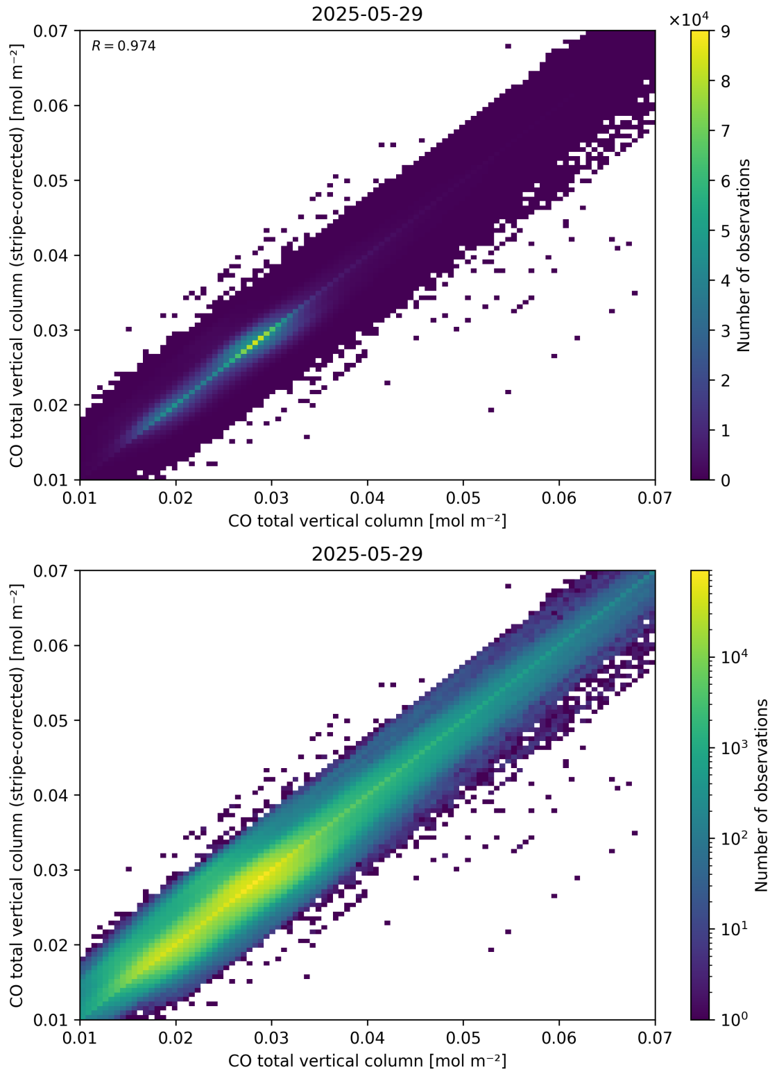
Figure 33: Scatter density plot of “CO total vertical column” against “CO total vertical column (stripe-corrected)” for 2025-05-28 to 2025-05-30.
