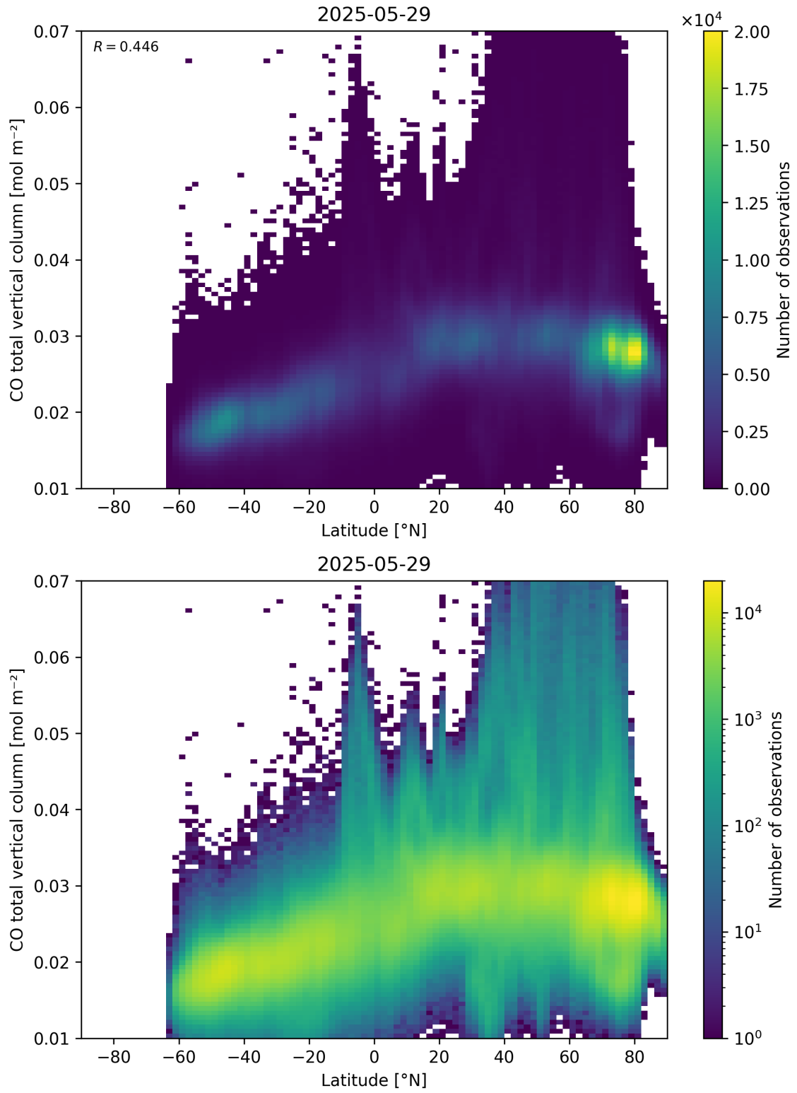
Figure 51: Scatter density plot of “Latitude” against “CO total vertical column” for 2025-05-28 to 2025-05-30.
