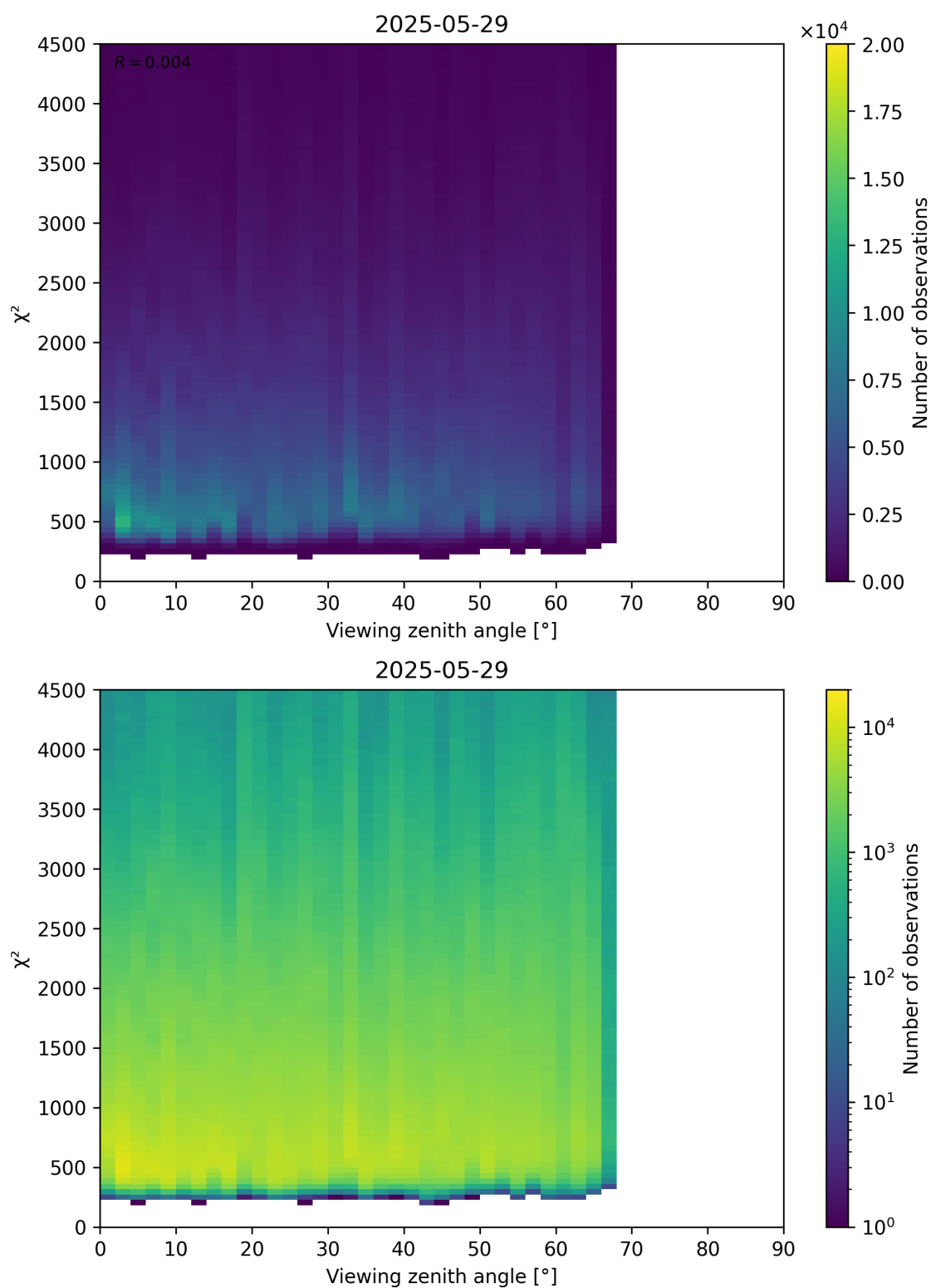
Figure 72: Scatter density plot of “Viewing zenith angle” against “ \chi^2 ” for 2025-05-28 to 2025-05-30.
