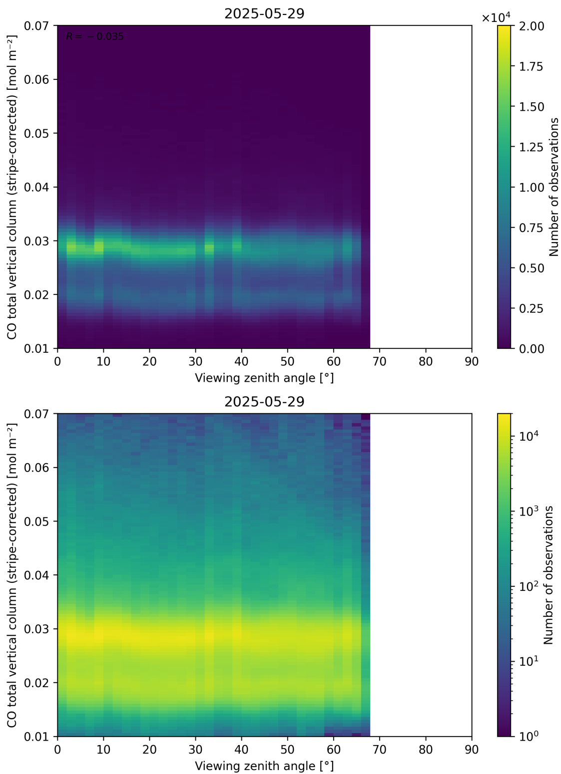
Figure 70: Scatter density plot of “Viewing zenith angle” against “CO total vertical column (stripe-corrected)” for 2025-05-28 to 2025-05-30.
