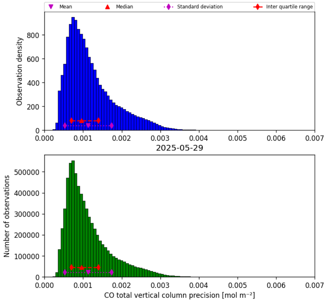
Figure 20: Histogram of “CO total vertical column precision” for 2025-05-28 to 2025-05-30
