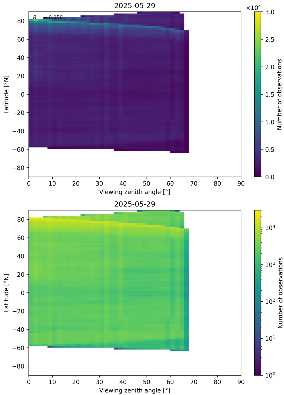
Figure 74: Scatter density plot of “Viewing zenith angle” against “Latitude” for 2025-05-28 to 2025-05-30.
