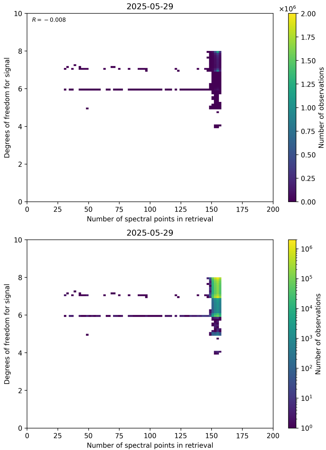
Figure 59: Scatter density plot of “Number of spectral points in retrieval” against “Degrees of freedom for signal” for 2025-05-28 to 2025-05-30.
