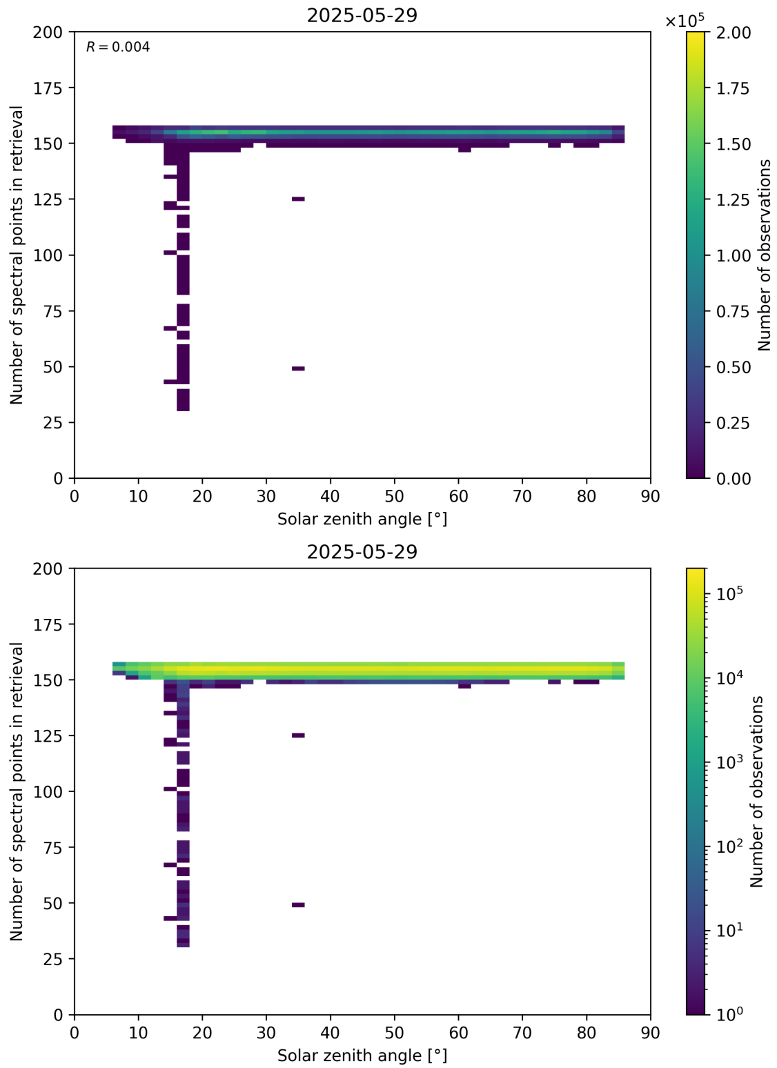
Figure 68: Scatter density plot of “Solar zenith angle” against “Number of spectral points in retrieval” for 2025-05-28 to 2025-05-30.
