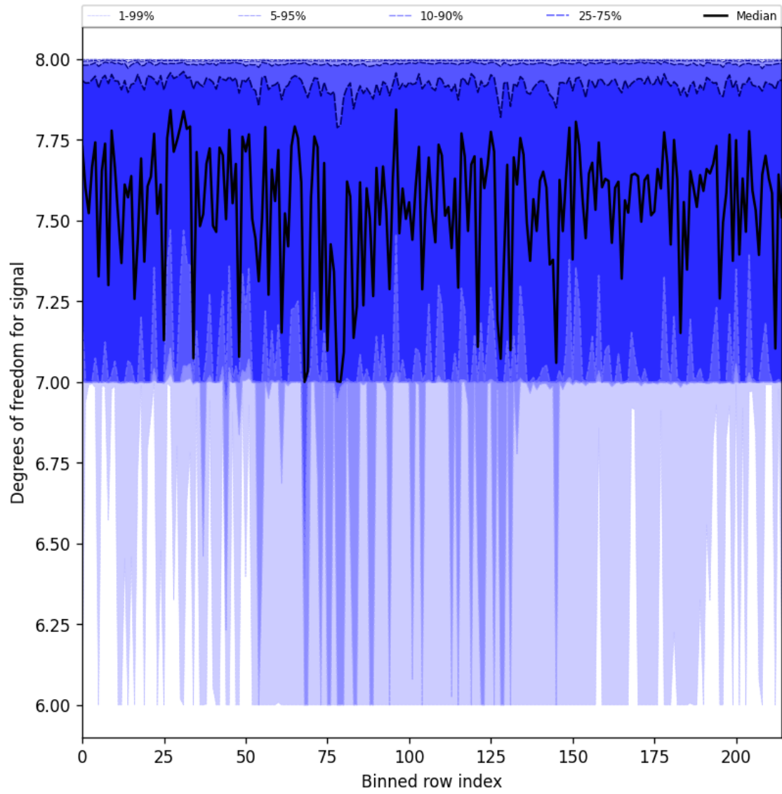
Figure 31: Along track statistics of “Degrees of freedom for signal” for 2025-05-28 to 2025-05-30
