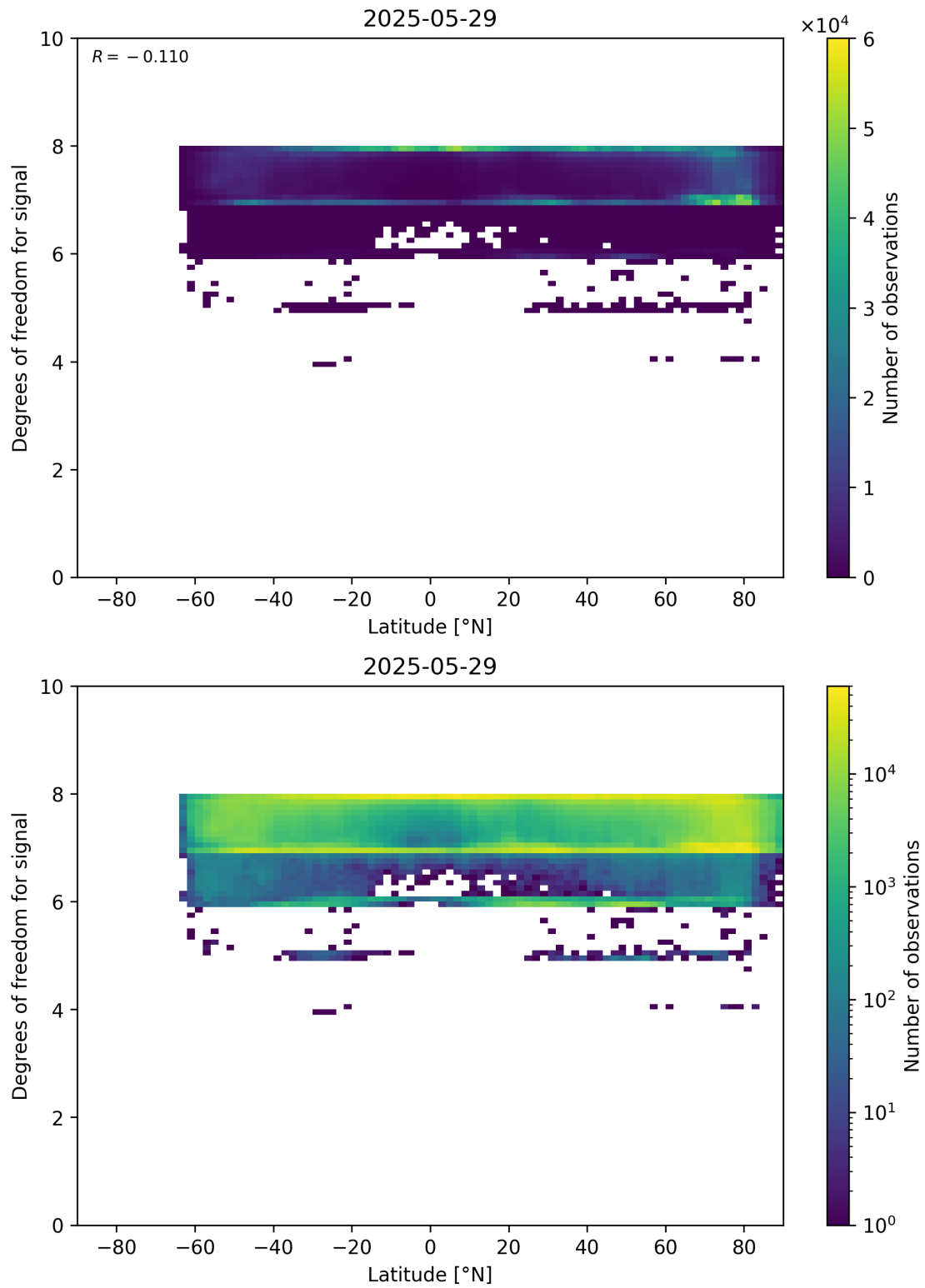
Figure 55: Scatter density plot of “Latitude” against “Degrees of freedom for signal” for 2025-05-28 to 2025-05-30.
