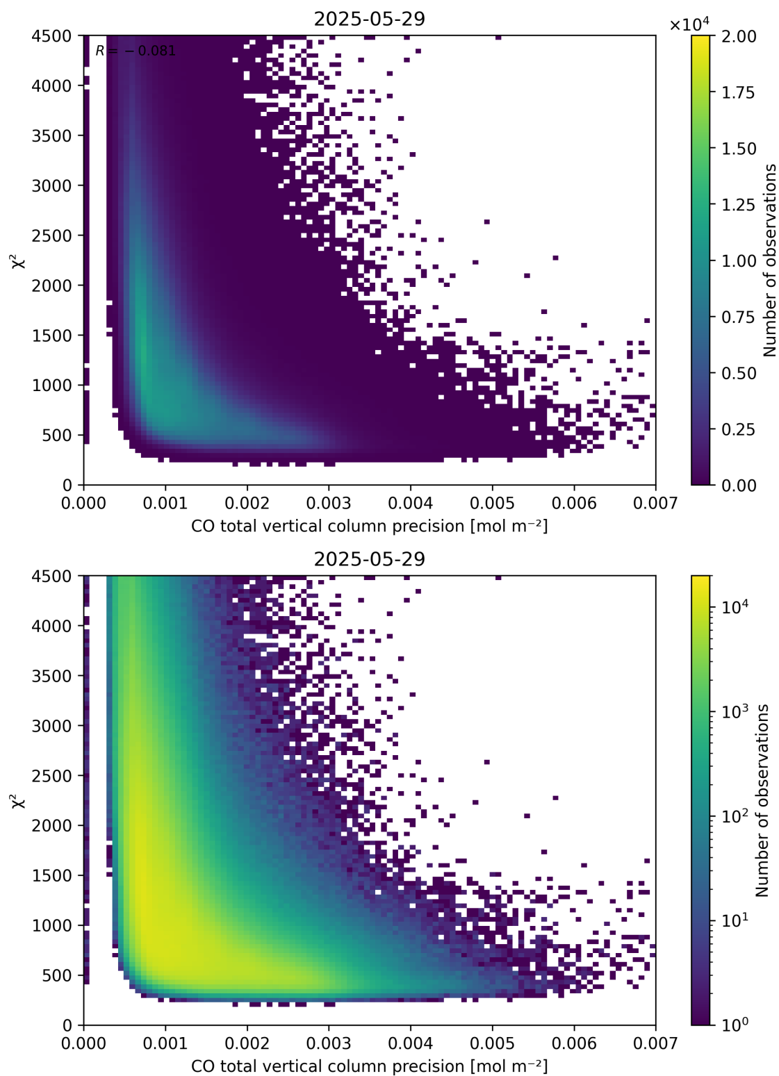
Figure 44: Scatter density plot of “CO total vertical column precision” against “ \chi^2 ” for 2025-05-28 to 2025-05-30.
