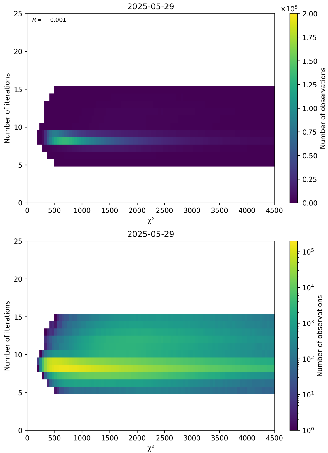
Figure 49: Scatter density plot of “ \chi^2 ” against “Number of iterations” for 2025-05-28 to 2025-05-30.
