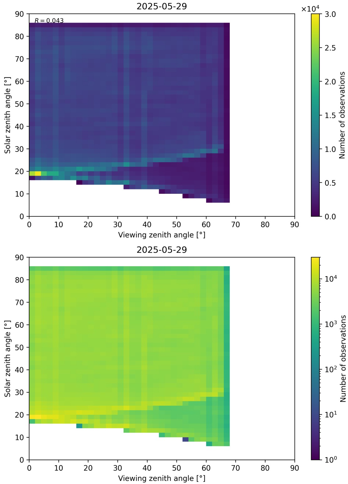
Figure 77: Scatter density plot of “Viewing zenith angle” against “Solar zenith angle” for 2025-05-28 to 2025-05-30.
