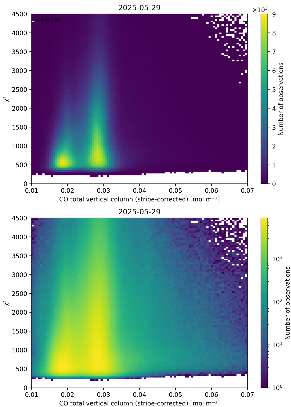
Figure 37: Scatter density plot of “CO total vertical column (stripe-corrected)” against “ \chi^2 ” for 2025-05-28 to 2025-05-30.
