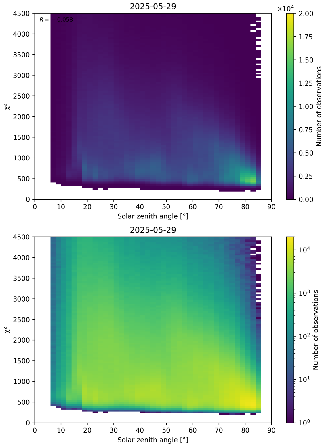
Figure 64: Scatter density plot of “Solar zenith angle” against “ \chi^2 ” for 2025-05-28 to 2025-05-30.
