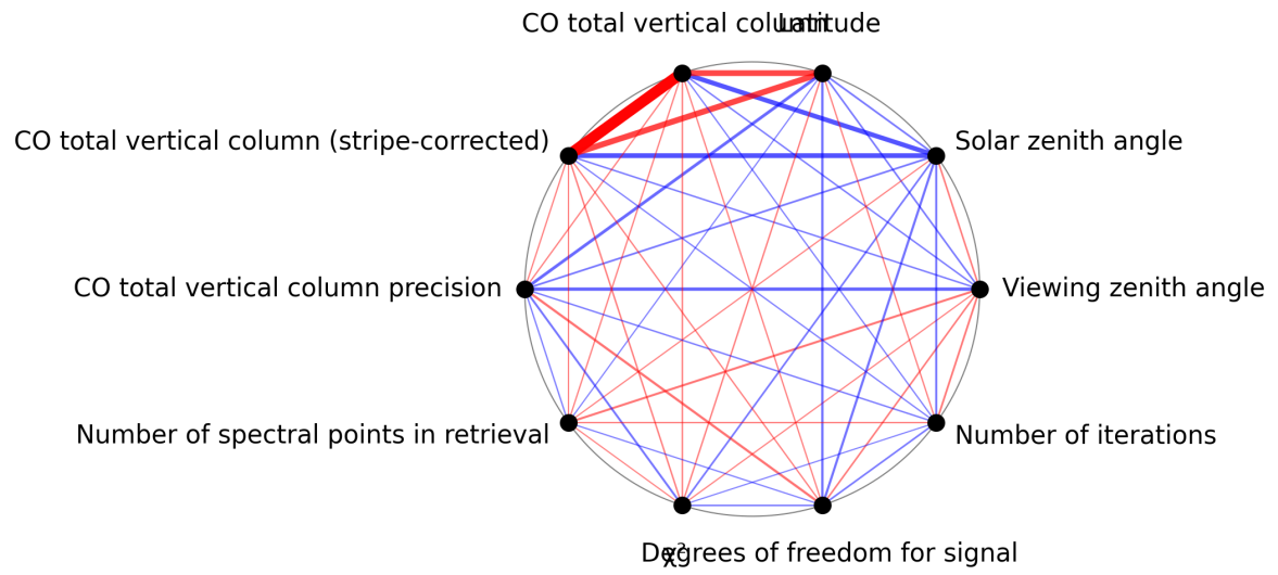
Figure 1: Map of correlation graph for 2025-05-28 to 2025-05-30.
