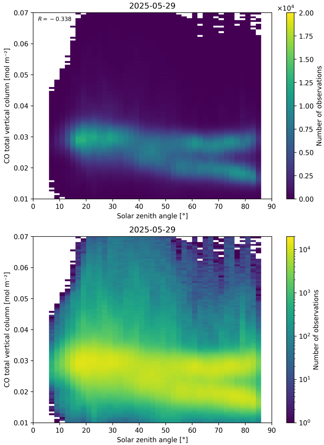
Figure 61: Scatter density plot of “Solar zenith angle” against “CO total vertical column” for 2025-05-28 to 2025-05-30.
