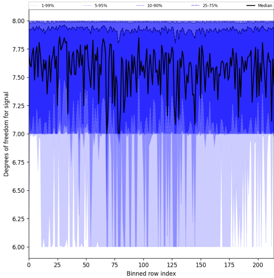
Figure 31: Along track statistics of “Degrees of freedom for signal” for 2025-05-29 to 2025-05-31
