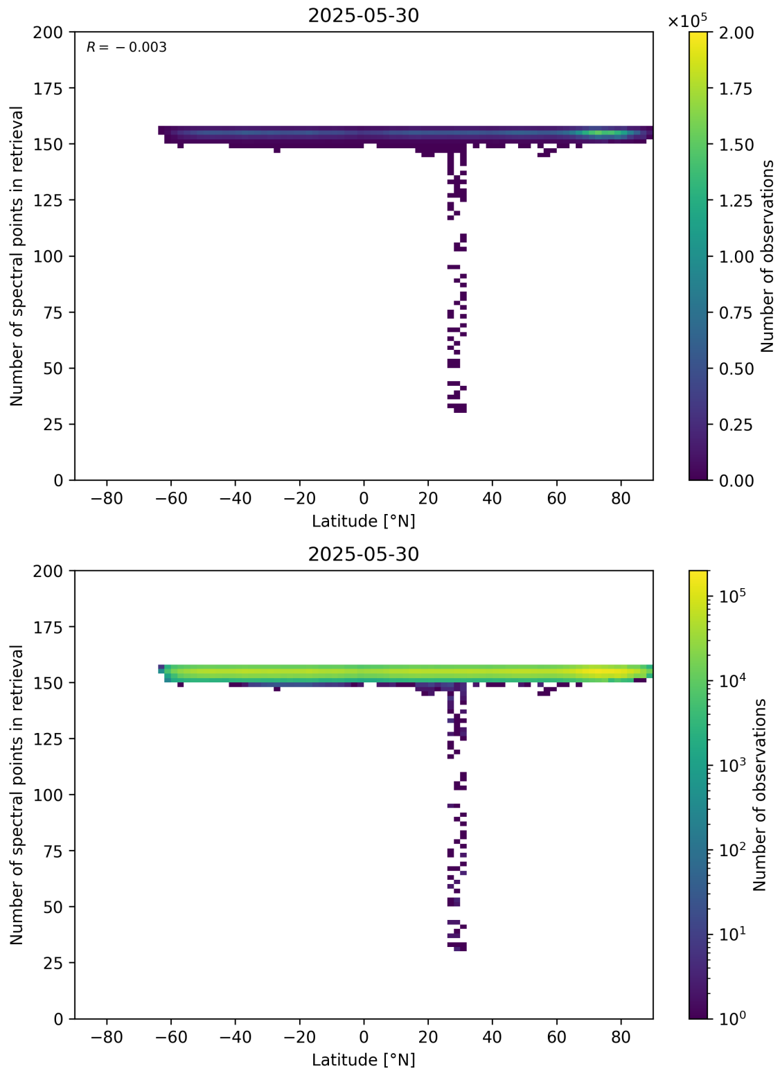
Figure 57: Scatter density plot of “Latitude” against “Number of spectral points in retrieval” for 2025-05-29 to 2025-05-31.
