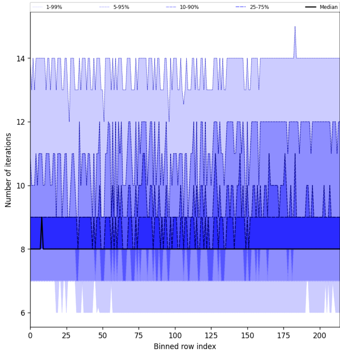
Figure 32: Along track statistics of “Number of iterations” for 2025-05-29 to 2025-05-31
