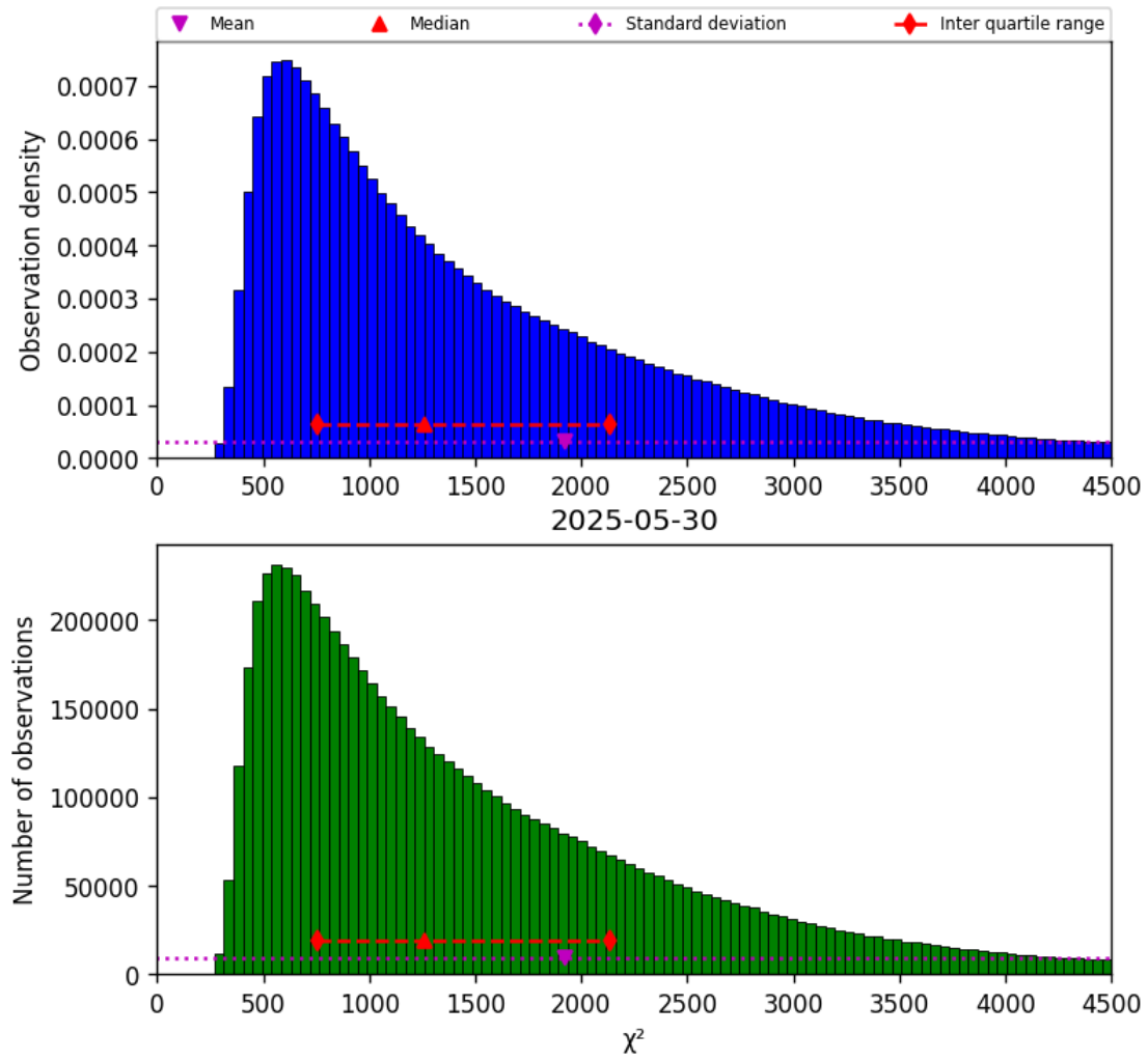
Figure 22: Histogram of “ \chi^2 ” for 2025-05-29 to 2025-05-31
