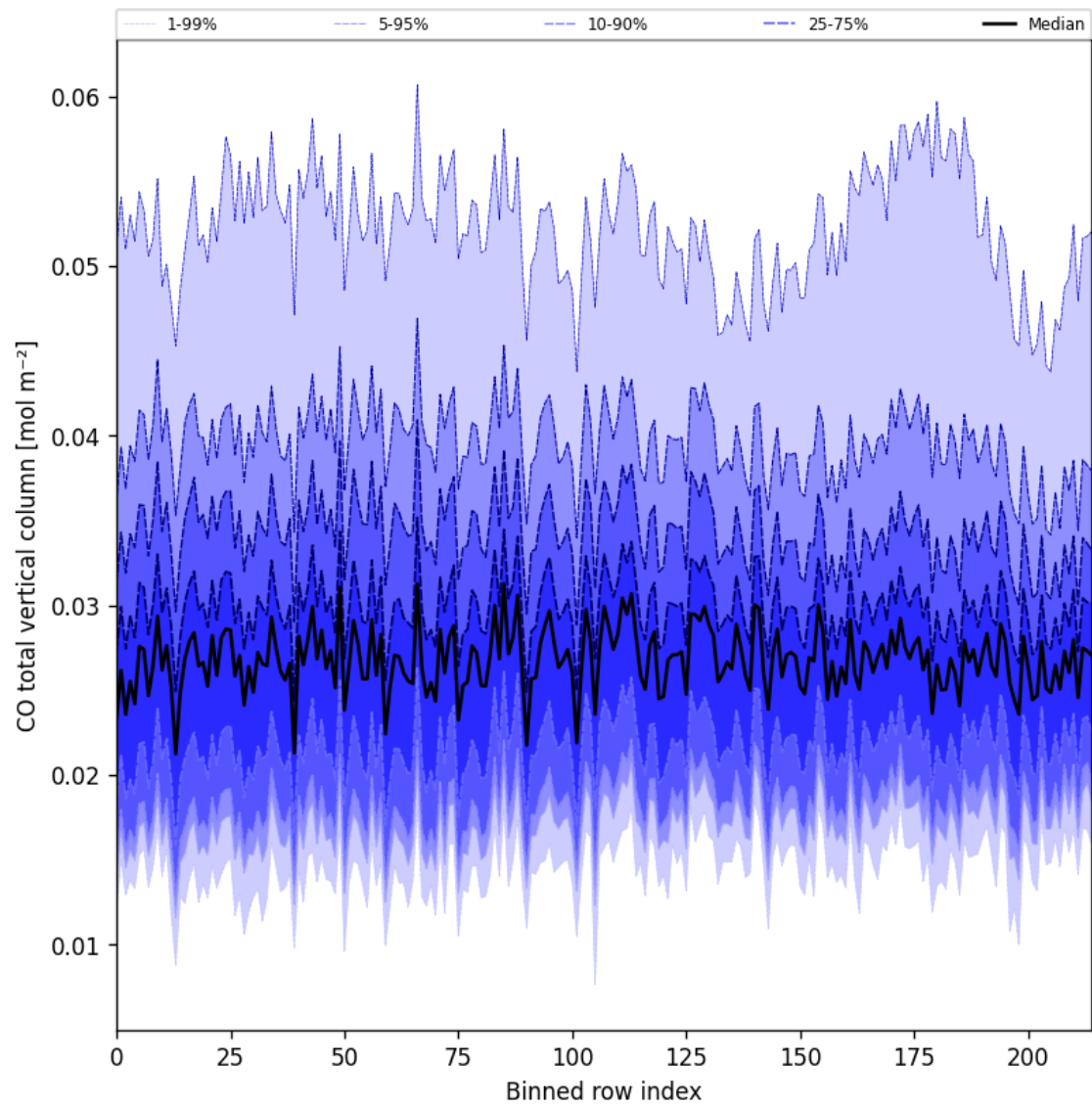
Figure 26: Along track statistics of “CO total vertical column” for 2025-05-29 to 2025-05-31
