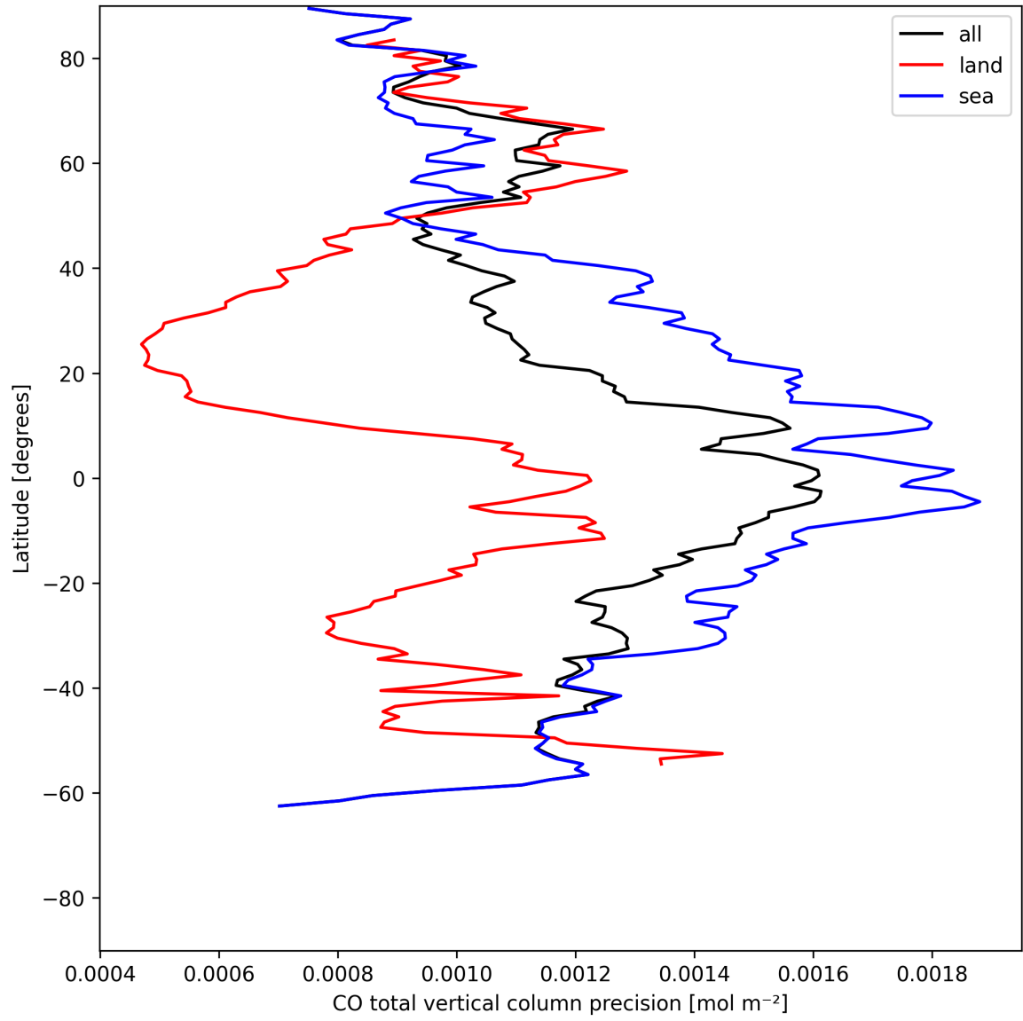
Figure 12: Zonal average of “CO total vertical column precision” for 2025-05-29 to 2025-05-31.
