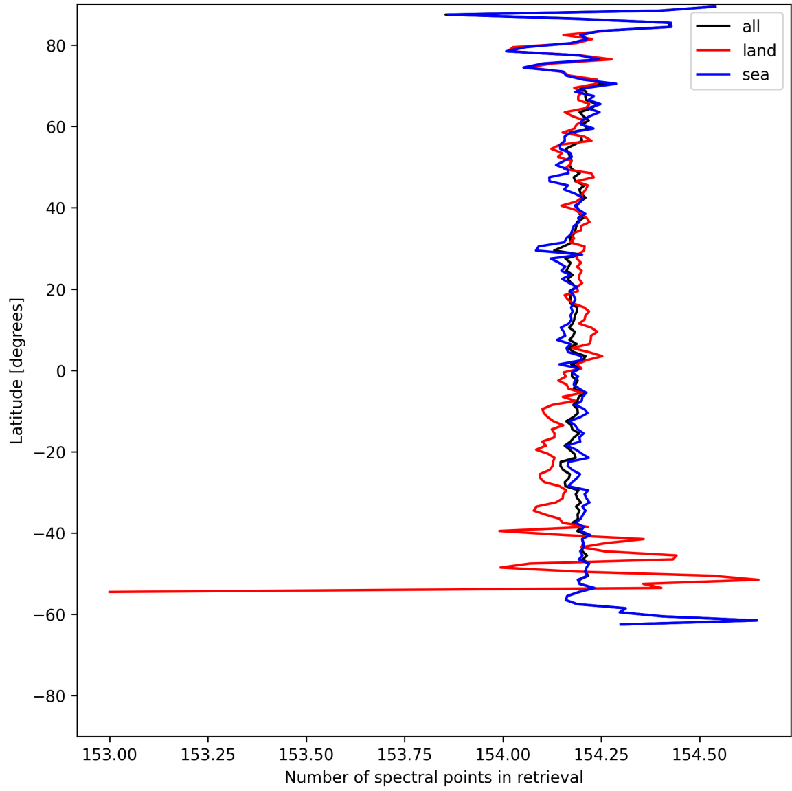
Figure 13: Zonal average of “Number of spectral points in retrieval” for 2025-05-29 to 2025-05-31.
