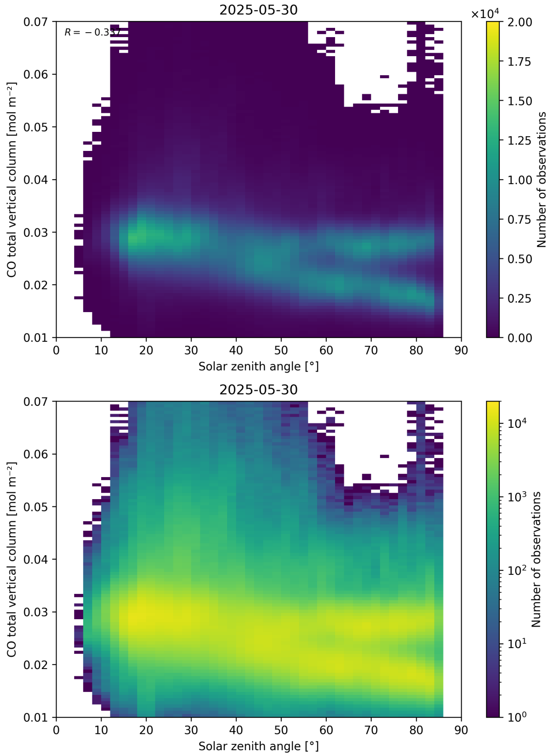
Figure 61: Scatter density plot of “Solar zenith angle” against “CO total vertical column” for 2025-05-29 to 2025-05-31.
