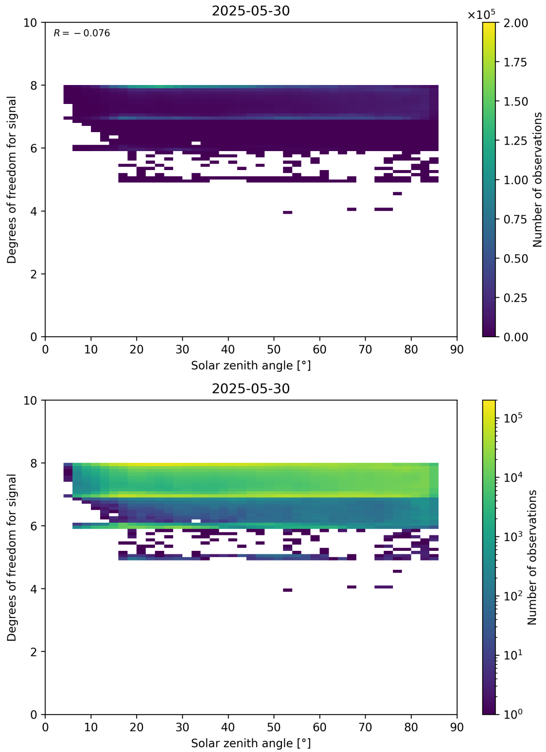
Figure 65: Scatter density plot of “Solar zenith angle” against “Degrees of freedom for signal” for 2025-05-29 to 2025-05-31.
