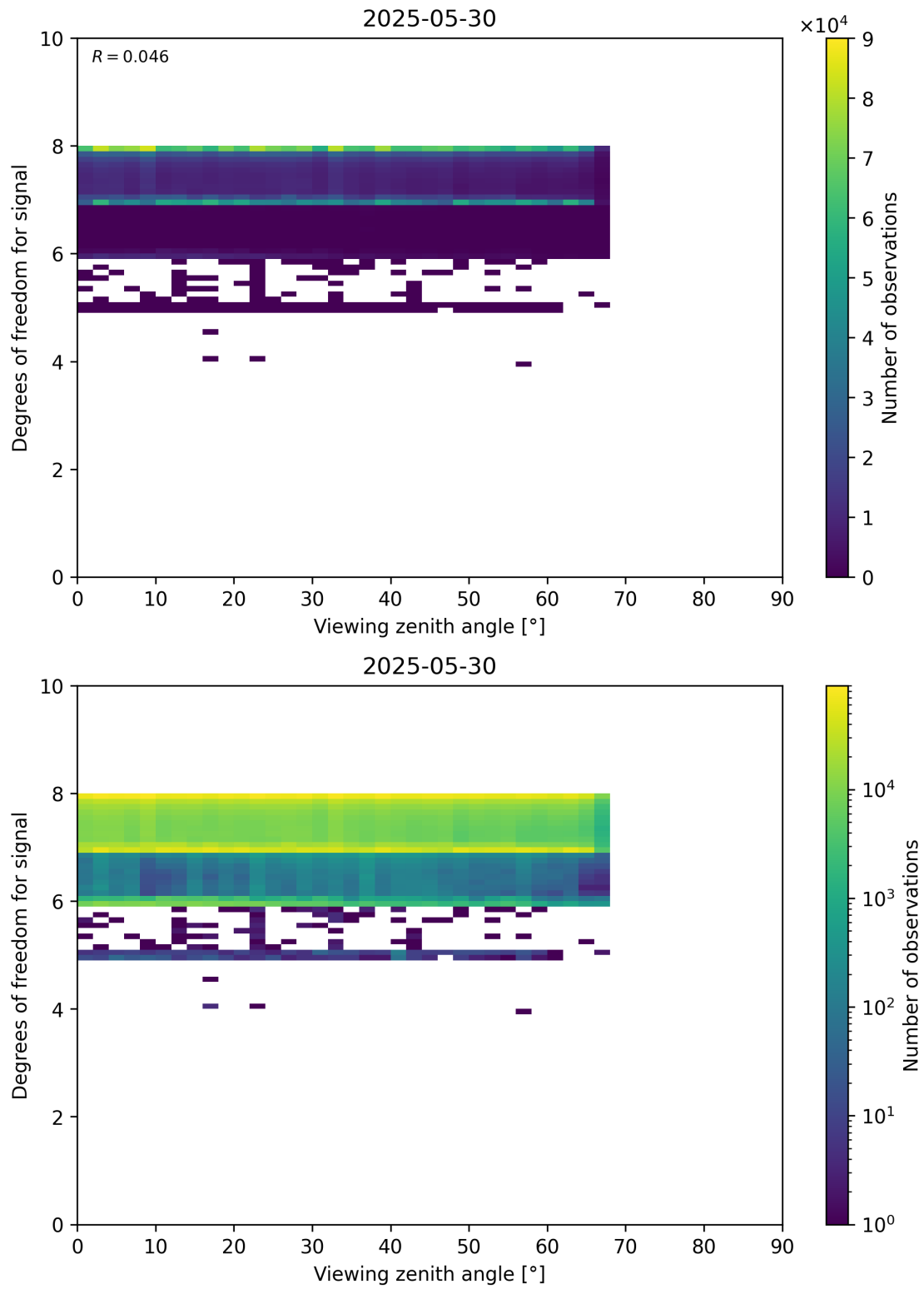
Figure 73: Scatter density plot of “Viewing zenith angle” against “Degrees of freedom for signal” for 2025-05-29 to 2025-05-31.
