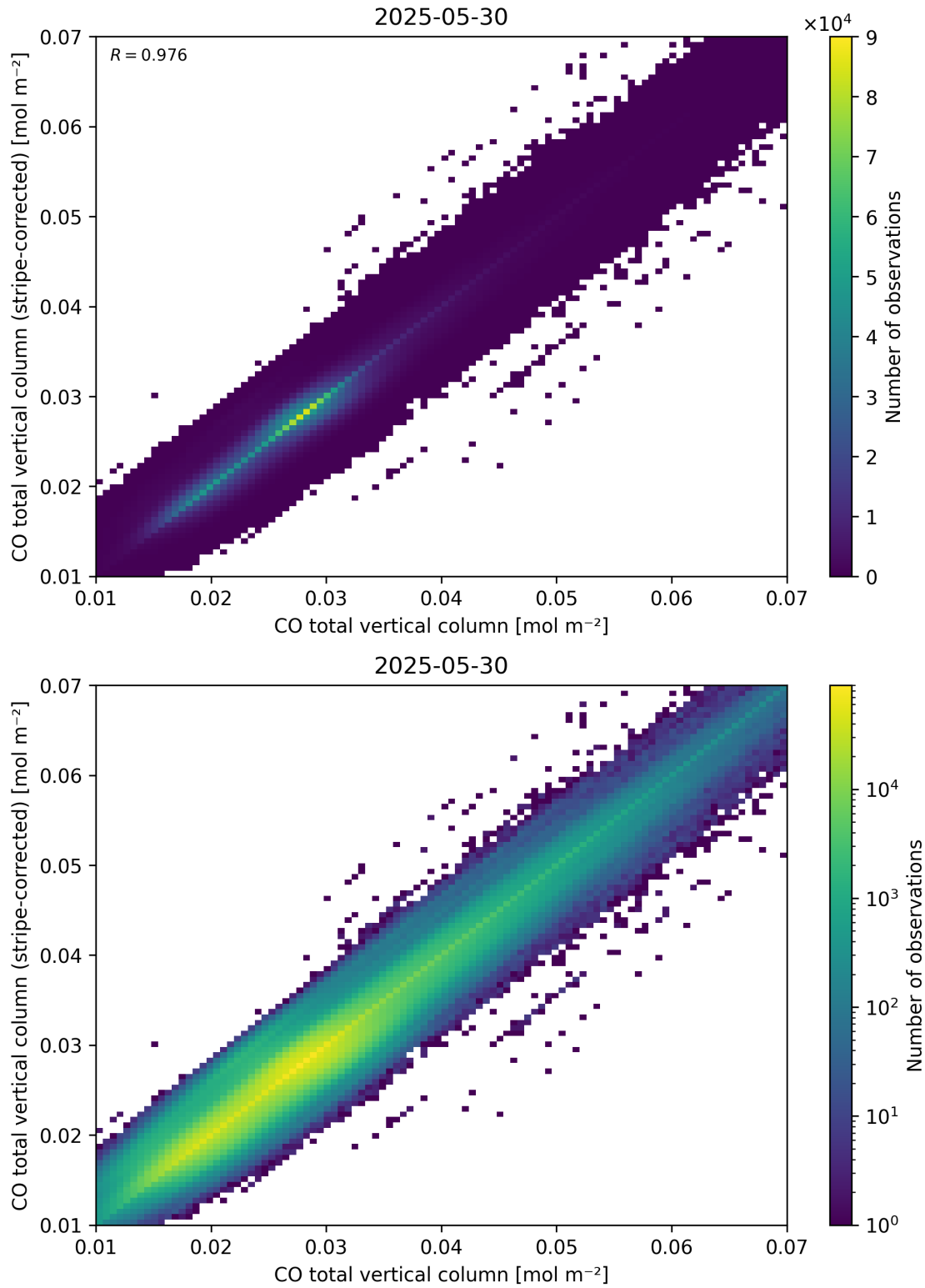
Figure 33: Scatter density plot of “CO total vertical column” against “CO total vertical column (stripe-corrected)” for 2025-05-29 to 2025-05-31.
