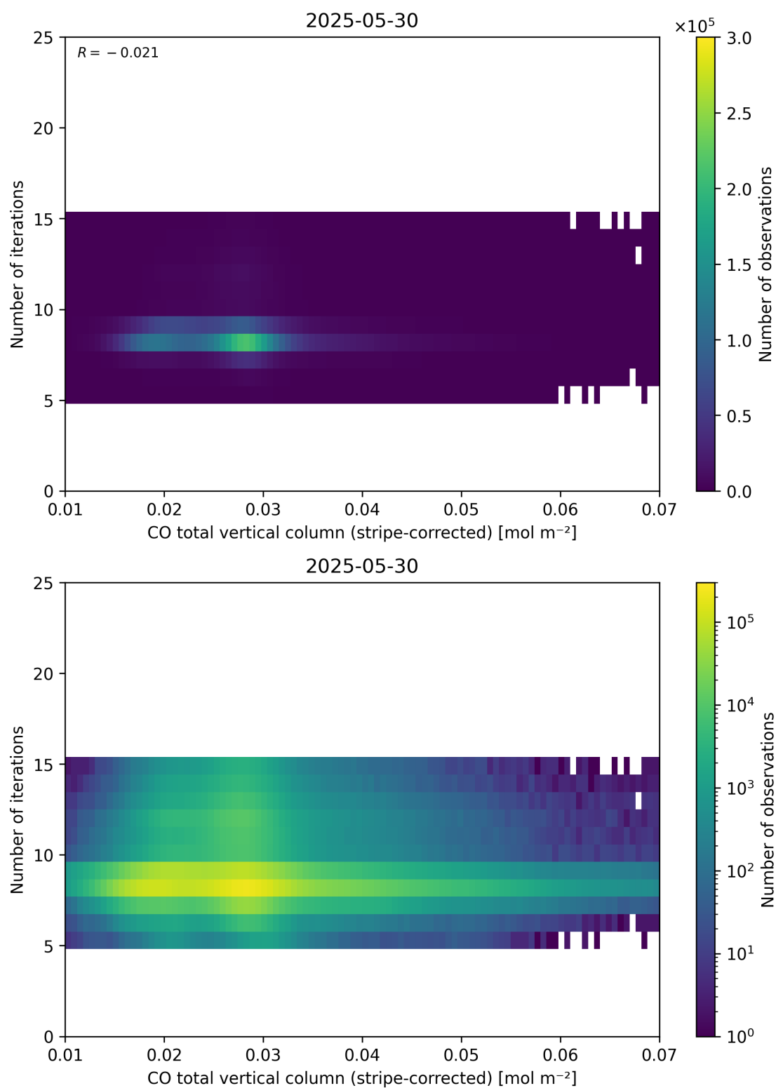
Figure 39: Scatter density plot of “CO total vertical column (stripe-corrected)” against “Number of iterations” for 2025-05-29 to 2025-05-31.
