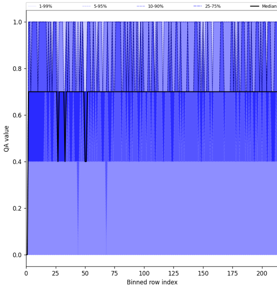
Figure 25: Along track statistics of “QA value” for 2025-05-29 to 2025-05-31
