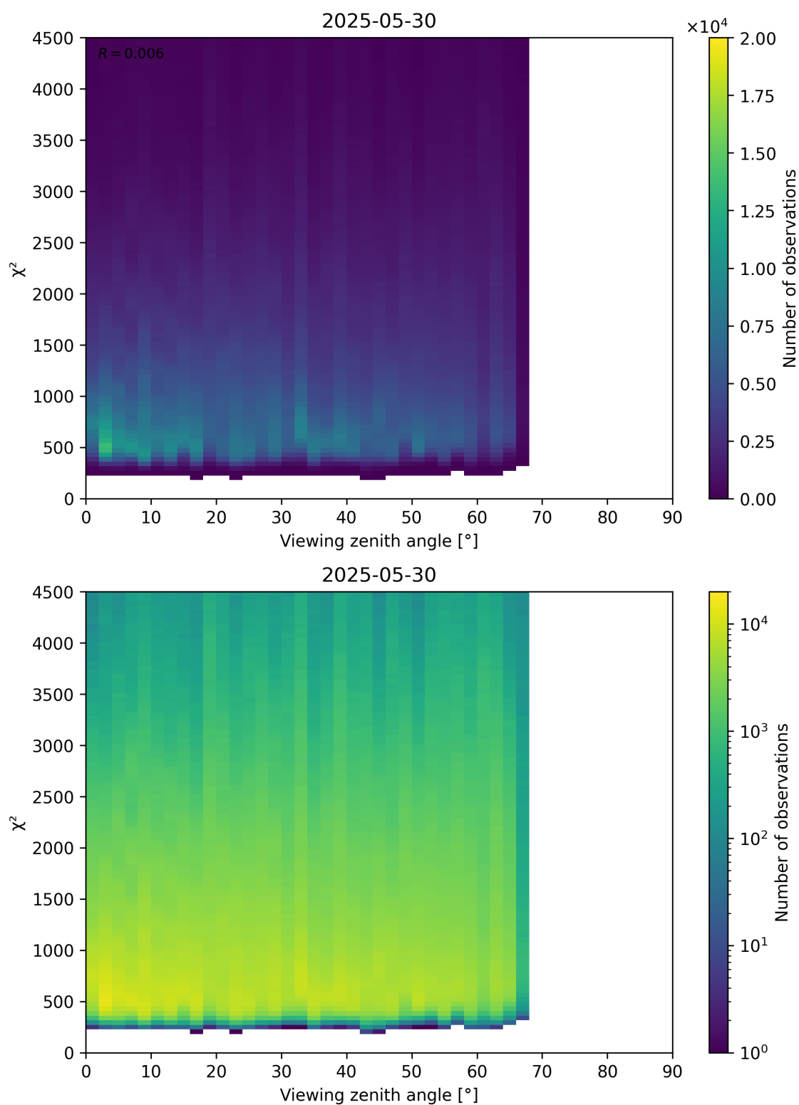
Figure 72: Scatter density plot of “Viewing zenith angle” against “ \chi^2 ” for 2025-05-29 to 2025-05-31.
