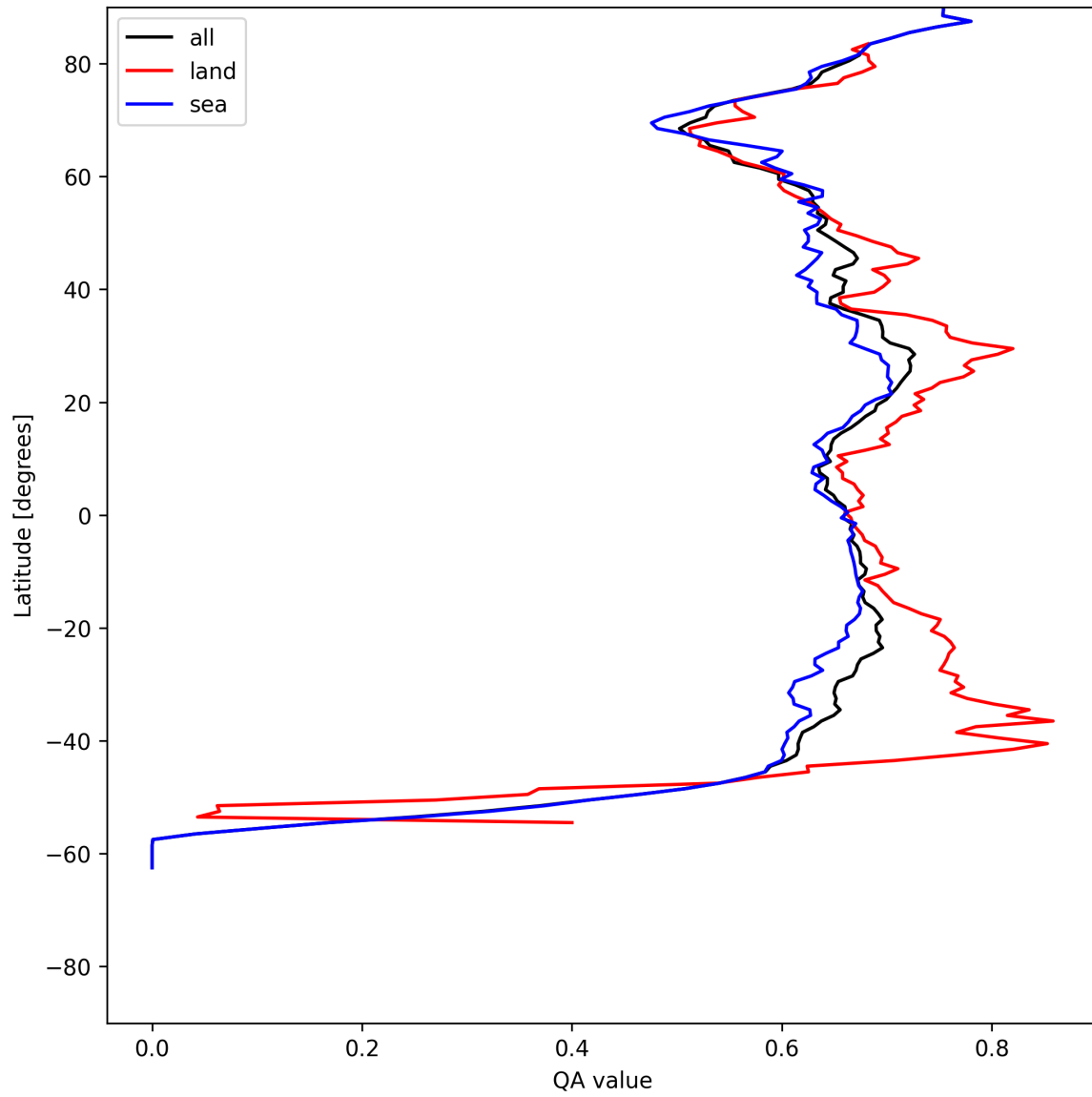
Figure 9: Zonal average of “QA value” for 2025-05-29 to 2025-05-31.
