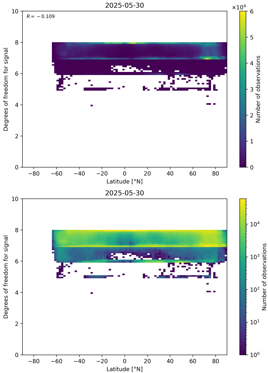
Figure 55: Scatter density plot of “Latitude” against “Degrees of freedom for signal” for 2025-05-29 to 2025-05-31.
