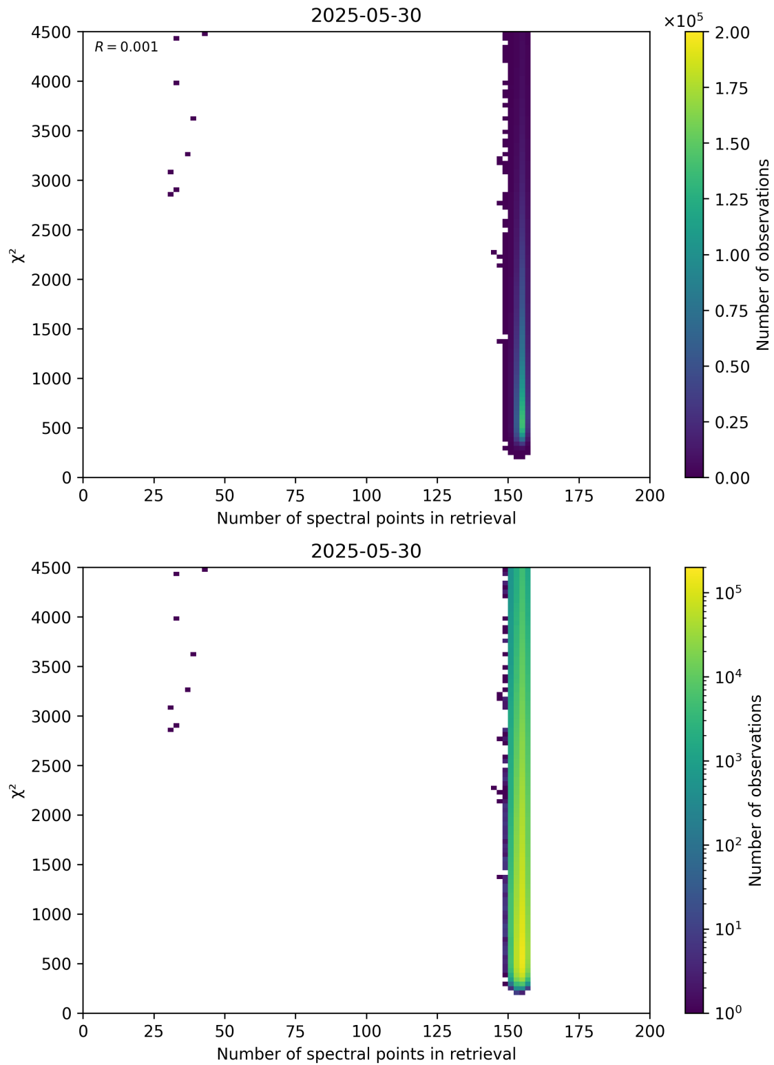
Figure 58: Scatter density plot of “Number of spectral points in retrieval” against “ \chi^2 ” for 2025-05-29 to 2025-05-31.
