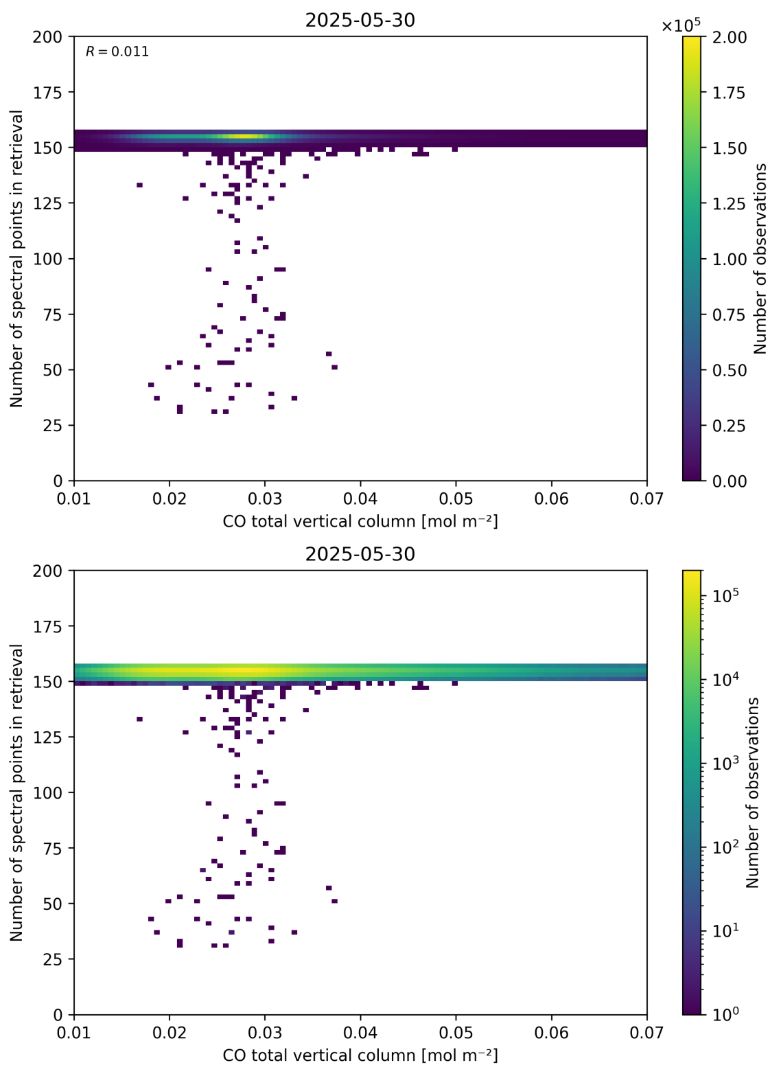
Figure 43: Scatter density plot of “CO total vertical column” against “Number of spectral points in retrieval” for 2025-05-29 to 2025-05-31.
