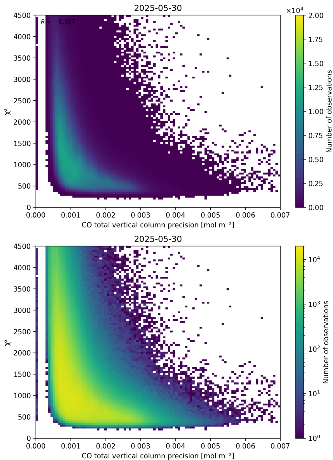
Figure 44: Scatter density plot of “CO total vertical column precision” against “ \chi^2 ” for 2025-05-29 to 2025-05-31.
