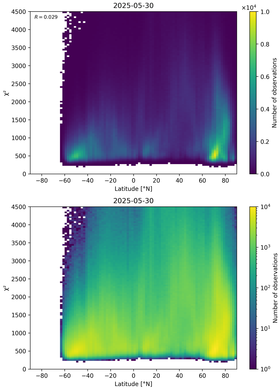
Figure 54: Scatter density plot of “Latitude” against “ \chi^2 ” for 2025-05-29 to 2025-05-31.
