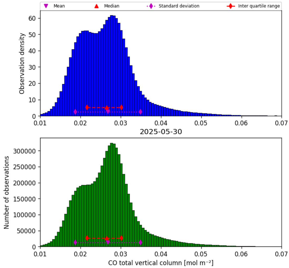
Figure 18: Histogram of “CO total vertical column” for 2025-05-29 to 2025-05-31
