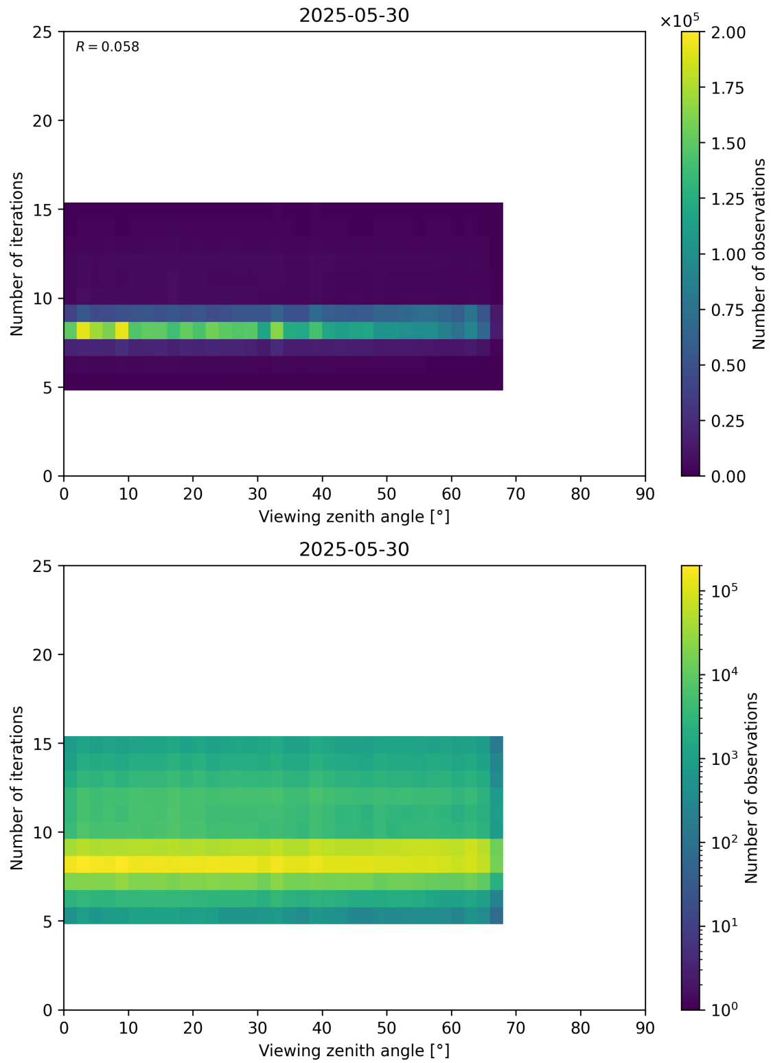
Figure 75: Scatter density plot of “Viewing zenith angle” against “Number of iterations” for 2025-05-29 to 2025-05-31.
