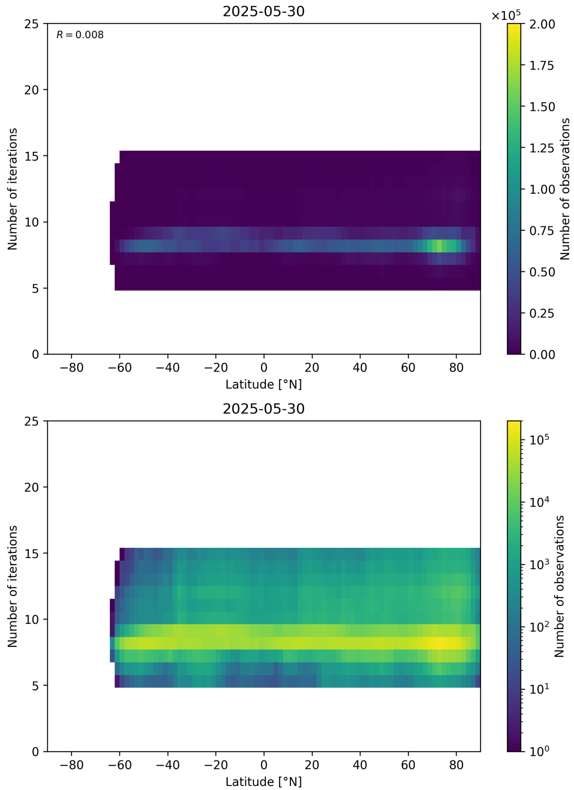
Figure 56: Scatter density plot of “Latitude” against “Number of iterations” for 2025-05-29 to 2025-05-31.
