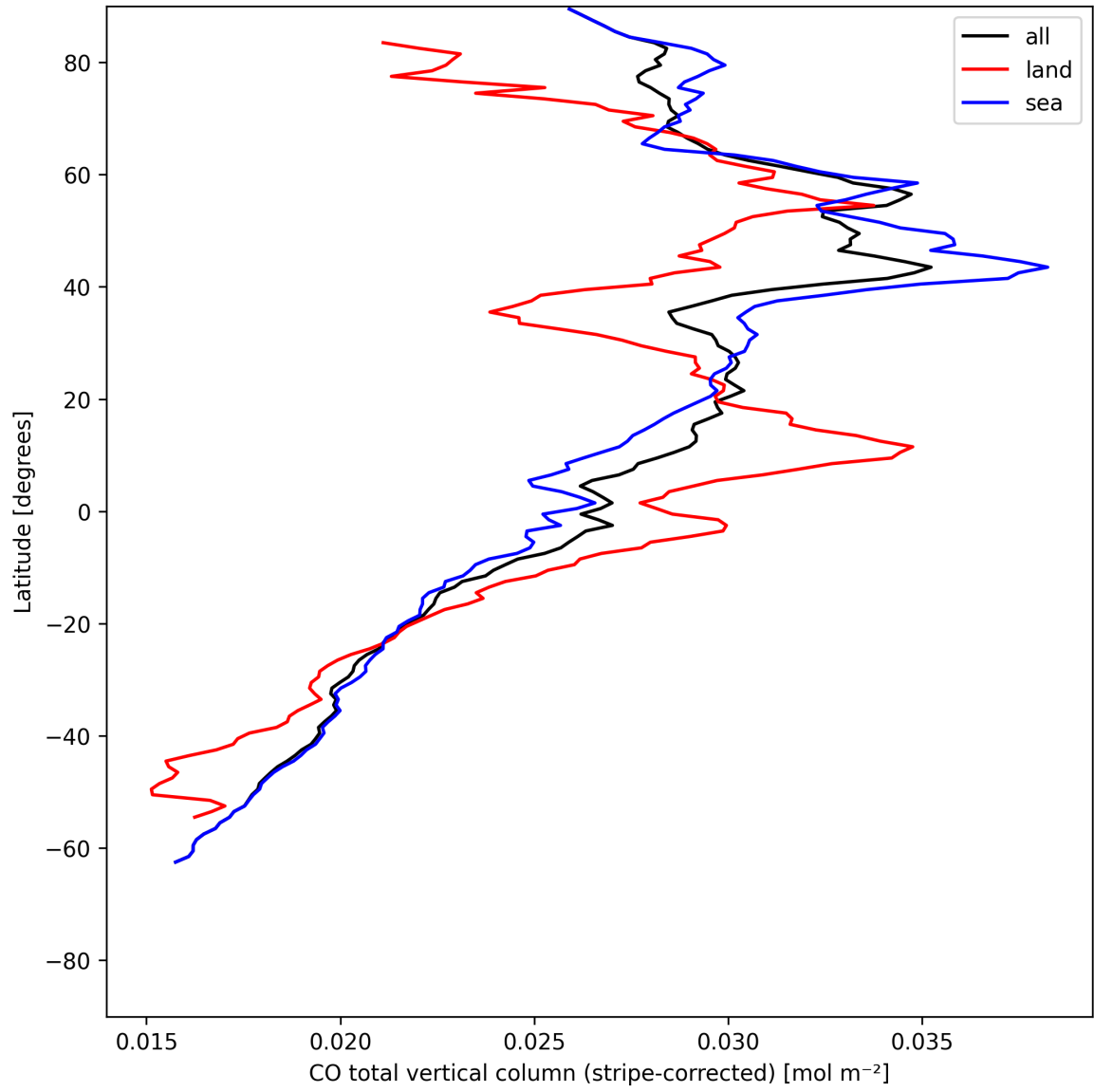
Figure 11: Zonal average of “CO total vertical column (stripe-corrected)” for 2025-05-29 to 2025-05-31.
