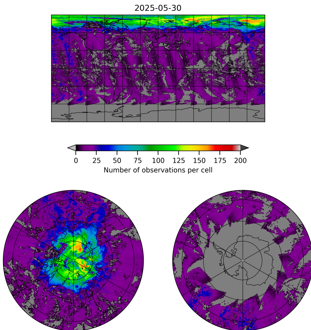
Figure 8: Map of the number of observations for 2025-05-29 to 2025-05-31
