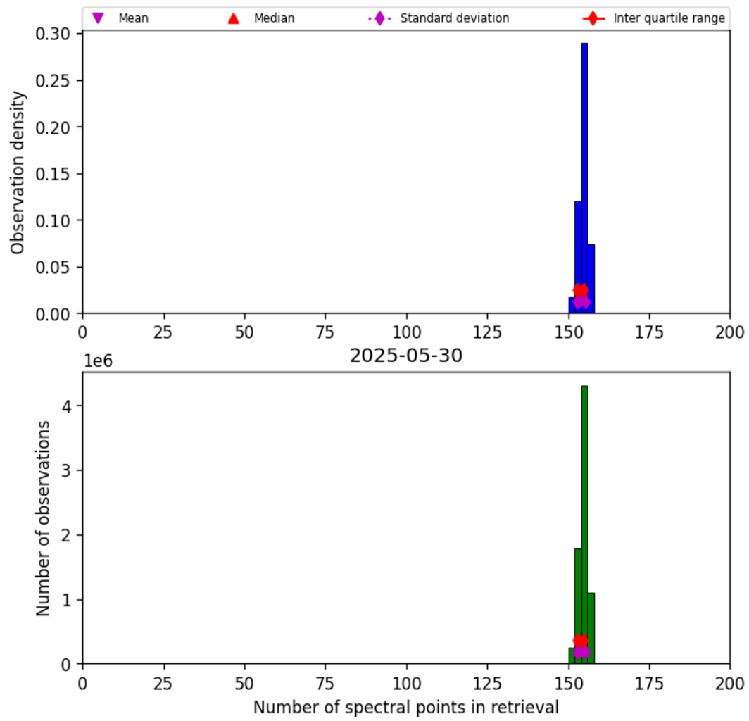
Figure 21: Histogram of “Number of spectral points in retrieval” for 2025-05-29 to 2025-05-31
