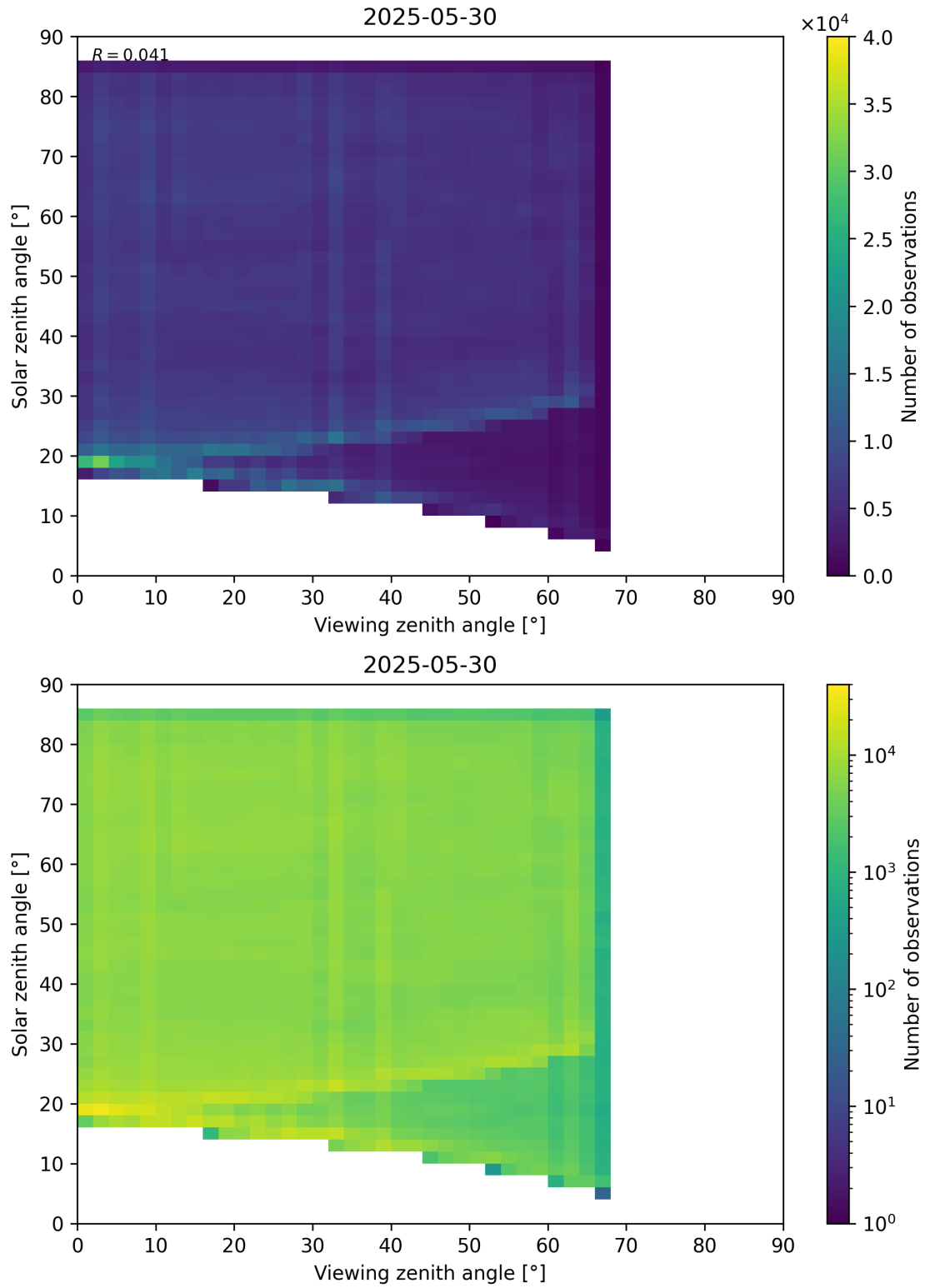
Figure 77: Scatter density plot of “Viewing zenith angle” against “Solar zenith angle” for 2025-05-29 to 2025-05-31.
