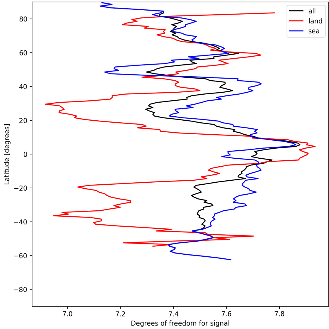
Figure 15: Zonal average of “Degrees of freedom for signal” for 2025-05-29 to 2025-05-31.
