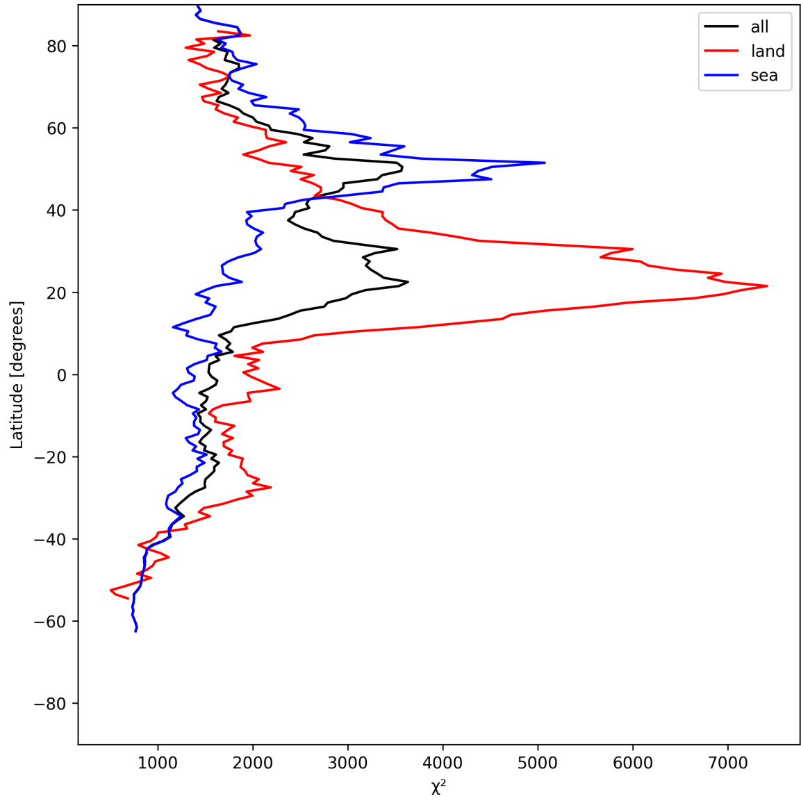
Figure 14: Zonal average of “ \chi^2 ” for 2025-05-29 to 2025-05-31.
