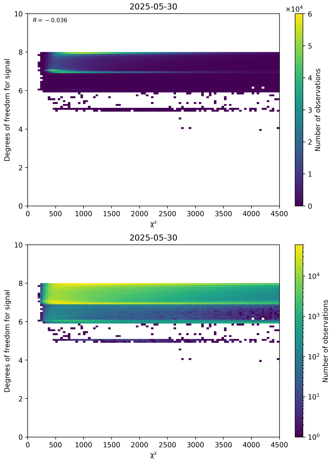
Figure 48: Scatter density plot of “ \chi^2 ” against “Degrees of freedom for signal” for 2025-05-29 to 2025-05-31.
