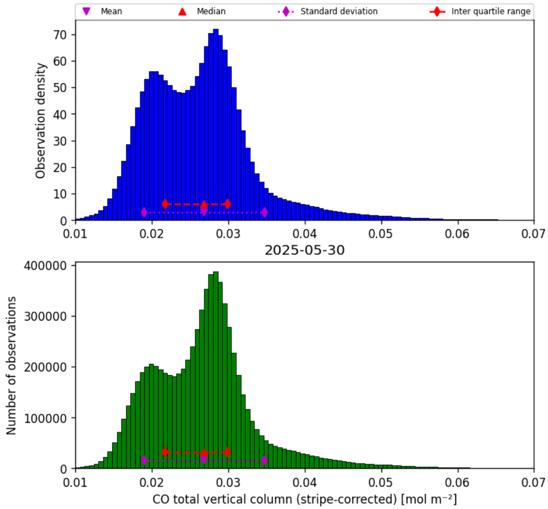
Figure 19: Histogram of “CO total vertical column (stripe-corrected)” for 2025-05-29 to 2025-05-31
