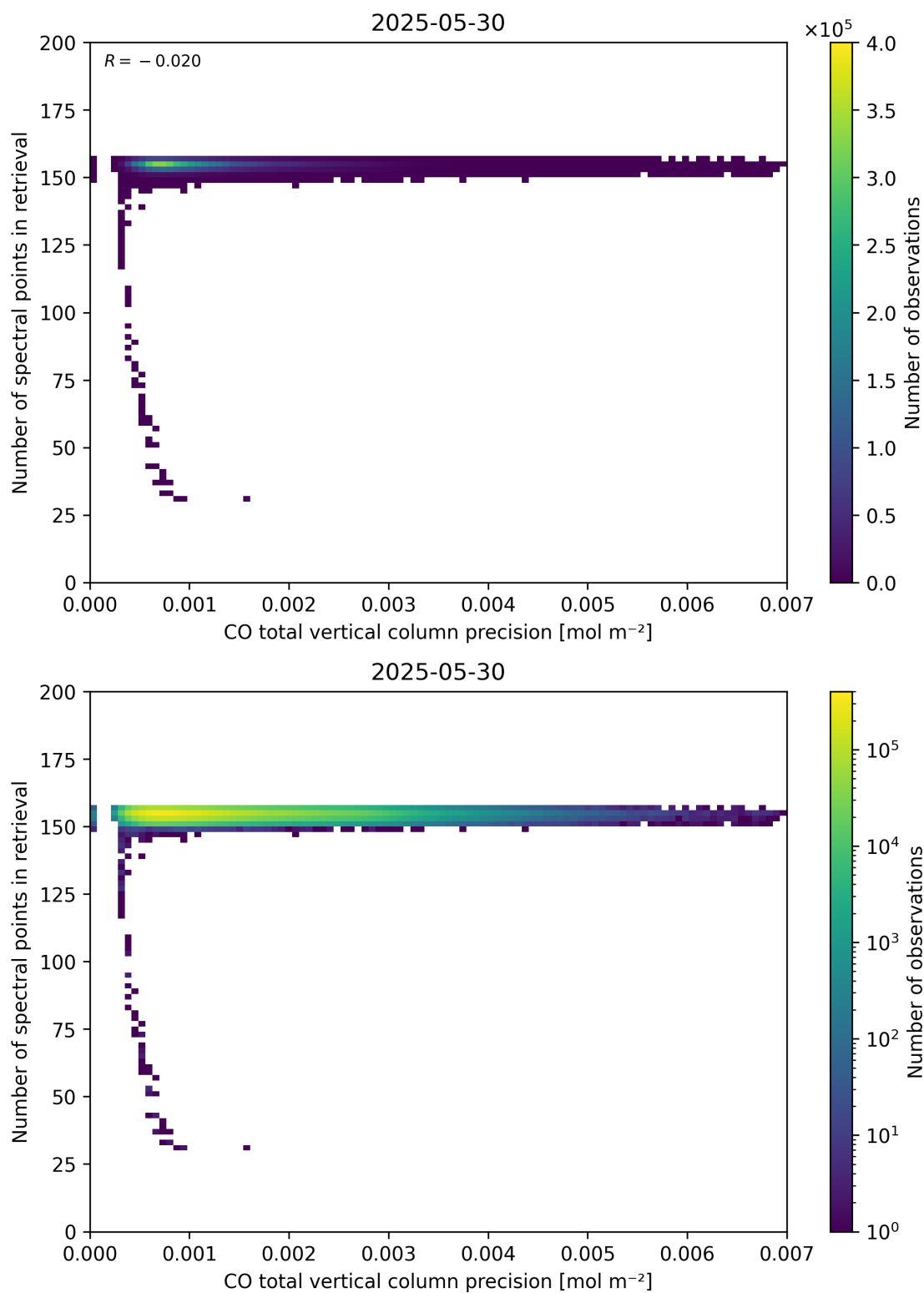
Figure 47: Scatter density plot of “CO total vertical column precision” against “Number of spectral points in retrieval” for 2025-05-29 to 2025-05-31.
