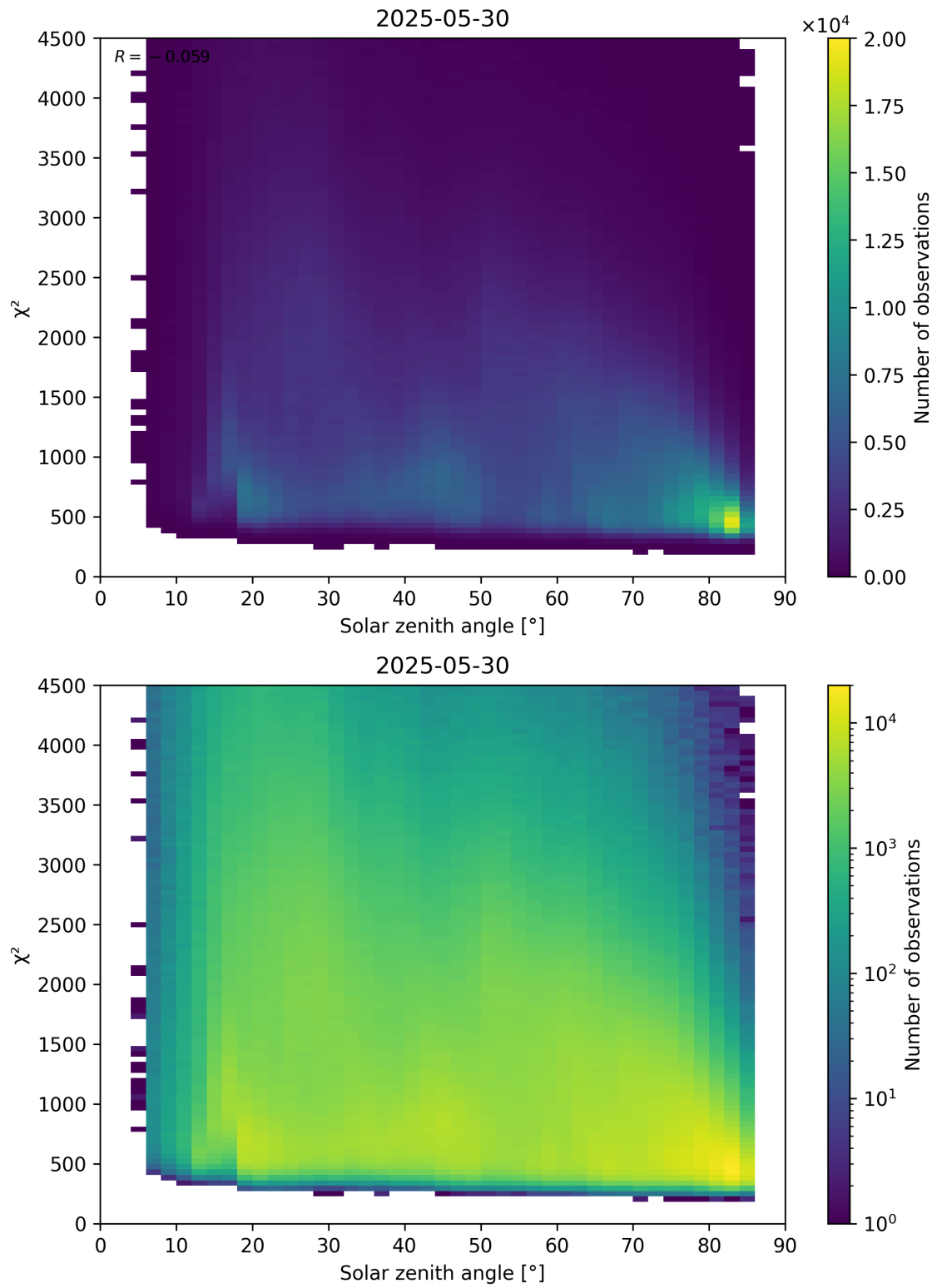
Figure 64: Scatter density plot of “Solar zenith angle” against “ \chi^2 ” for 2025-05-29 to 2025-05-31.
