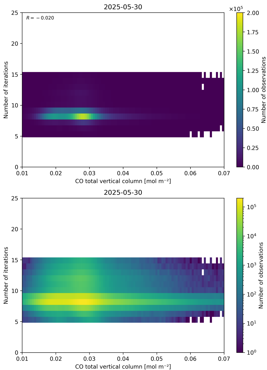
Figure 42: Scatter density plot of “CO total vertical column” against “Number of iterations” for 2025-05-29 to 2025-05-31.
