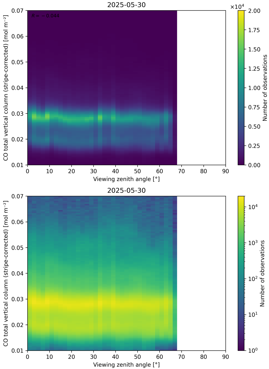
Figure 70: Scatter density plot of “Viewing zenith angle” against “CO total vertical column (stripe-corrected)” for 2025-05-29 to 2025-05-31.
