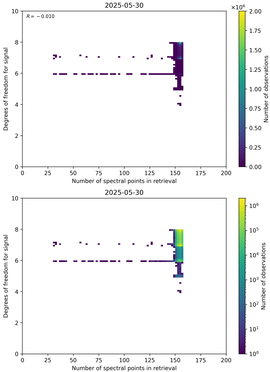
Figure 59: Scatter density plot of “Number of spectral points in retrieval” against “Degrees of freedom for signal” for 2025-05-29 to 2025-05-31.
