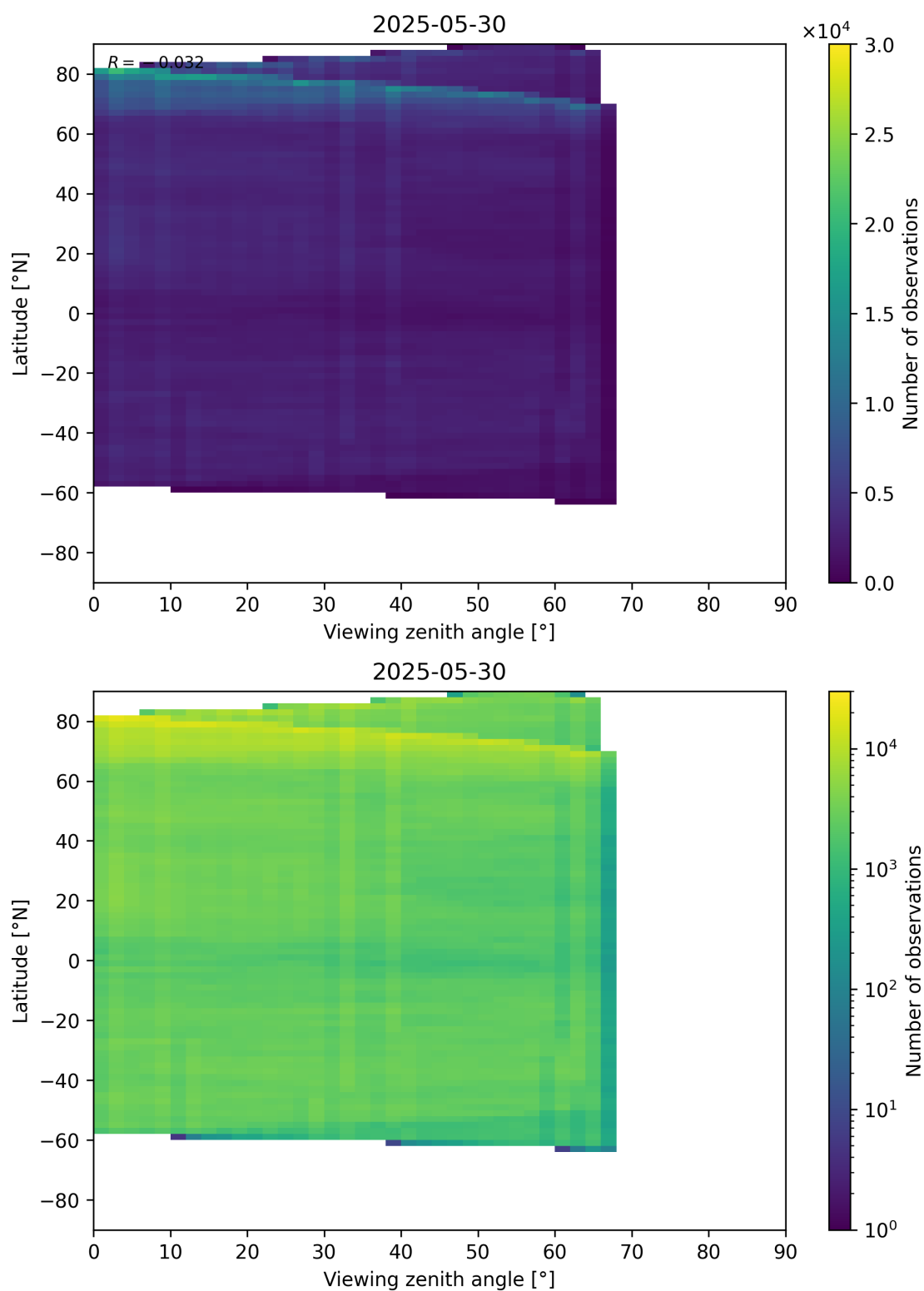
Figure 74: Scatter density plot of “Viewing zenith angle” against “Latitude” for 2025-05-29 to 2025-05-31.
