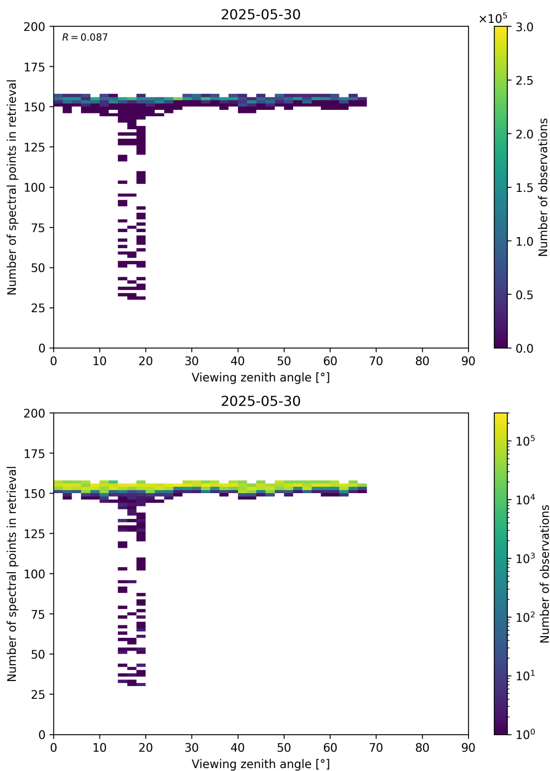
Figure 76: Scatter density plot of “Viewing zenith angle” against “Number of spectral points in retrieval” for 2025-05-29 to 2025-05-31.
