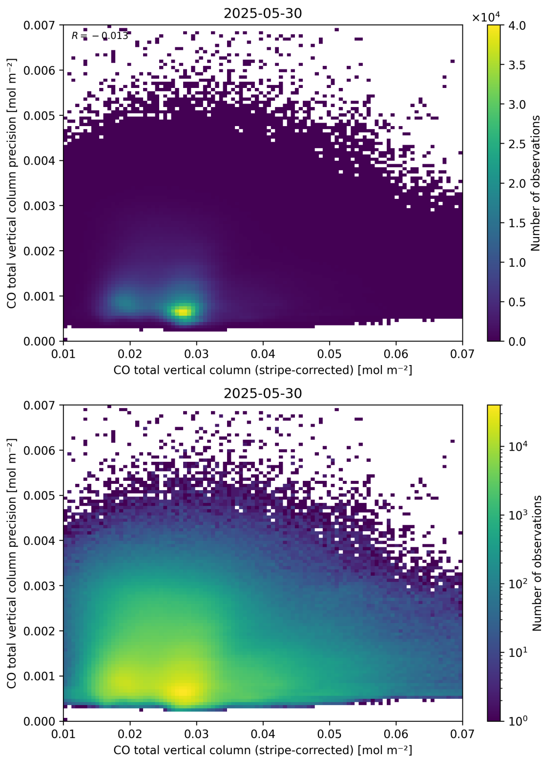
Figure 36: Scatter density plot of “CO total vertical column (stripe-corrected)” against “CO total vertical column precision” for 2025-05-29 to 2025-05-31.
