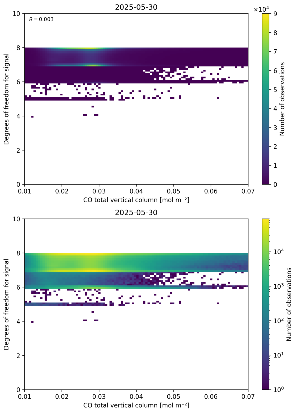
Figure 41: Scatter density plot of “CO total vertical column” against “Degrees of freedom for signal” for 2025-05-29 to 2025-05-31.
