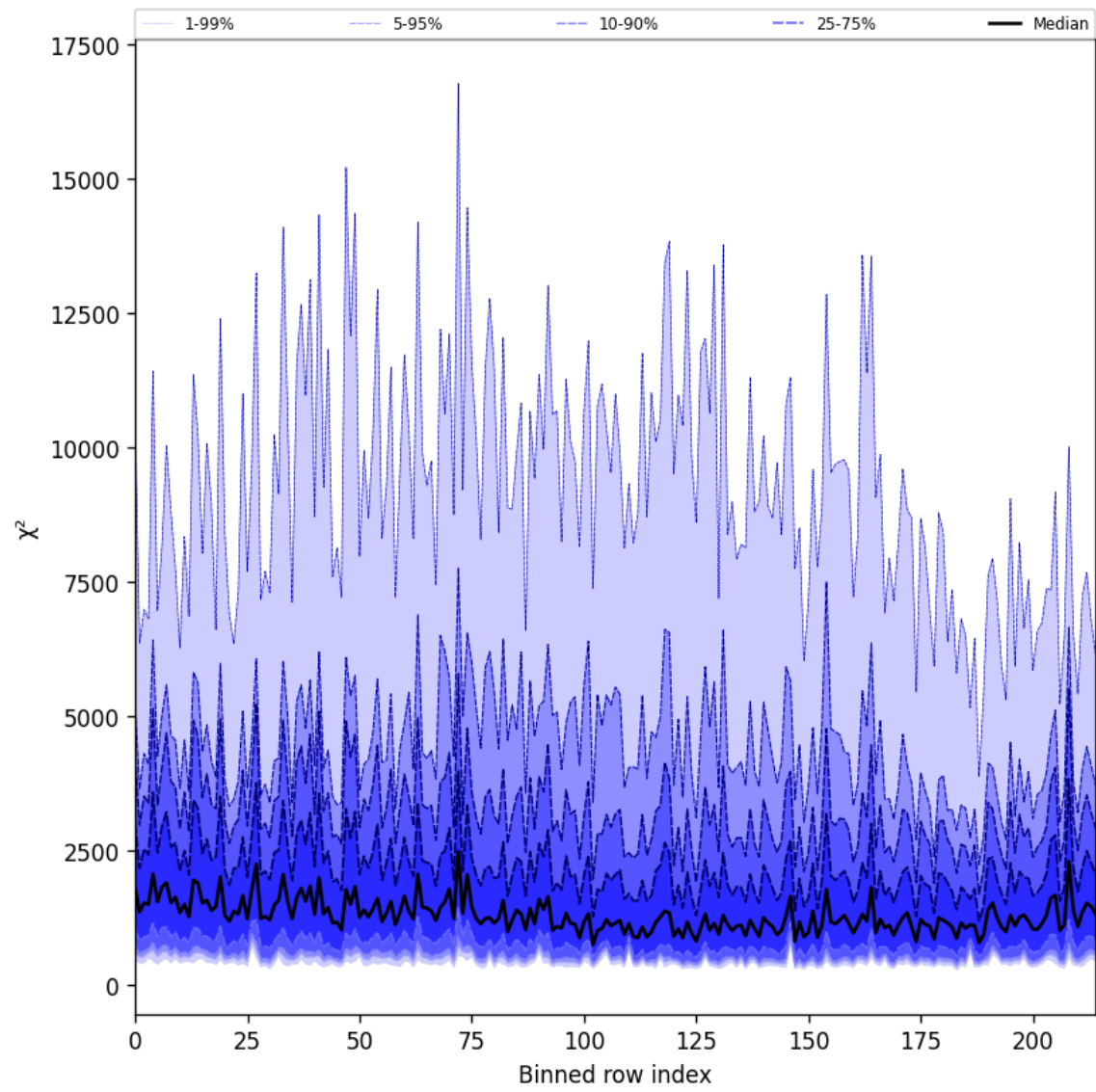
Figure 30: Along track statistics of “ \chi^2 ” for 2025-05-29 to 2025-05-31
