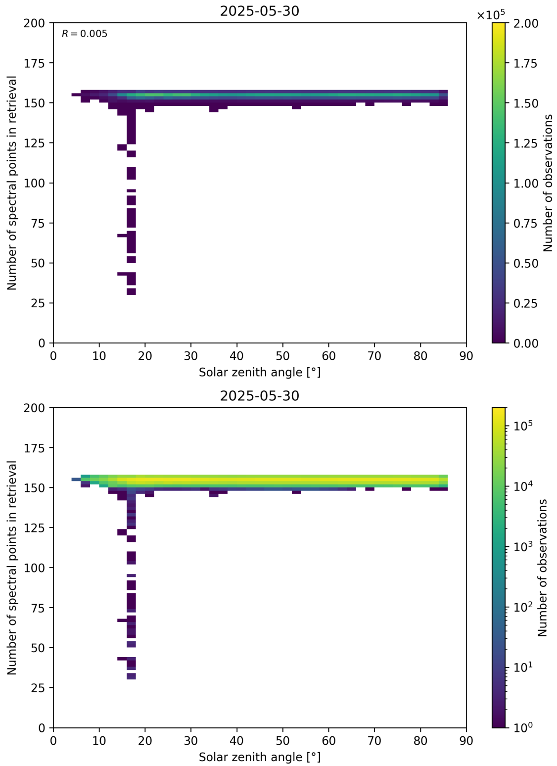
Figure 68: Scatter density plot of “Solar zenith angle” against “Number of spectral points in retrieval” for 2025-05-29 to 2025-05-31.
