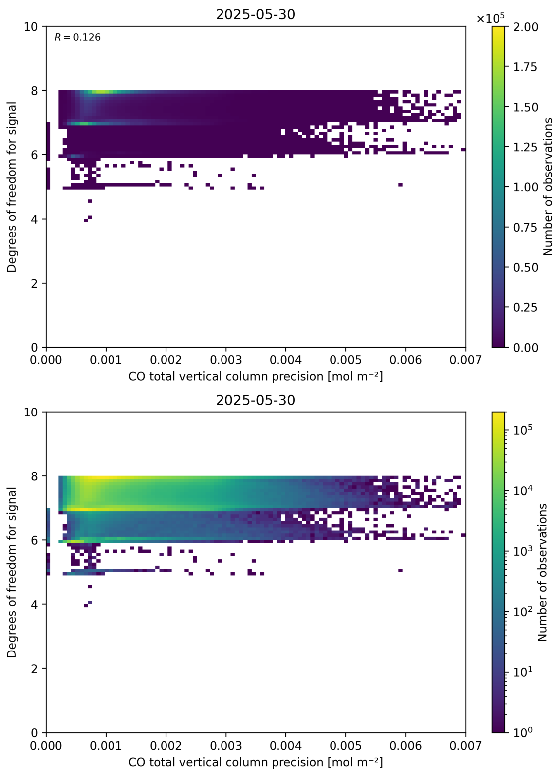
Figure 45: Scatter density plot of “CO total vertical column precision” against “Degrees of freedom for signal” for 2025-05-29 to 2025-05-31.
