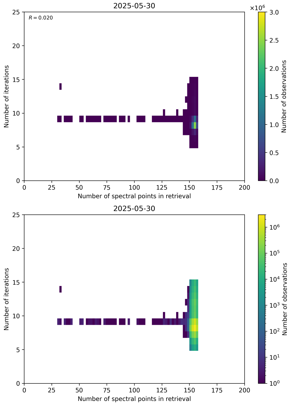
Figure 60: Scatter density plot of “Number of spectral points in retrieval” against “Number of iterations” for 2025-05-29 to 2025-05-31.
