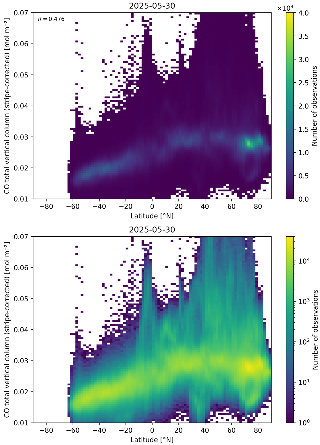
Figure 52: Scatter density plot of “Latitude” against “CO total vertical column (stripe-corrected)” for 2025-05-29 to 2025-05-31.
