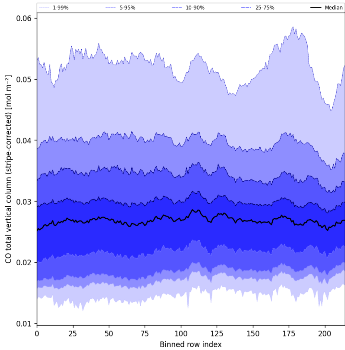
Figure 27: Along track statistics of “CO total vertical column (stripe-corrected)” for 2025-05-29 to 2025-05-31
