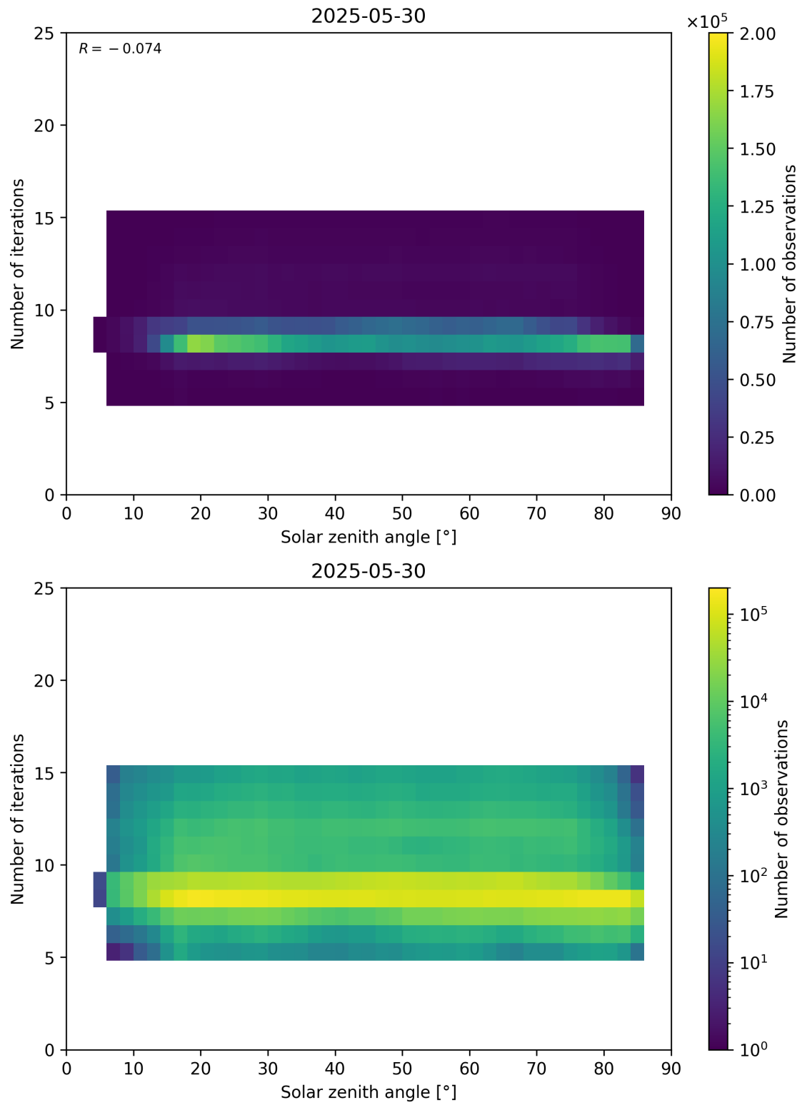
Figure 67: Scatter density plot of “Solar zenith angle” against “Number of iterations” for 2025-05-29 to 2025-05-31.
