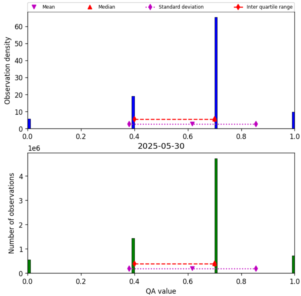
Figure 17: Histogram of “QA value” for 2025-05-29 to 2025-05-31
