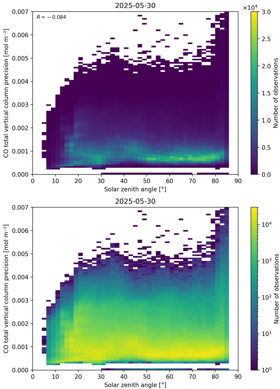
Figure 63: Scatter density plot of “Solar zenith angle” against “CO total vertical column precision” for 2025-05-29 to 2025-05-31.
