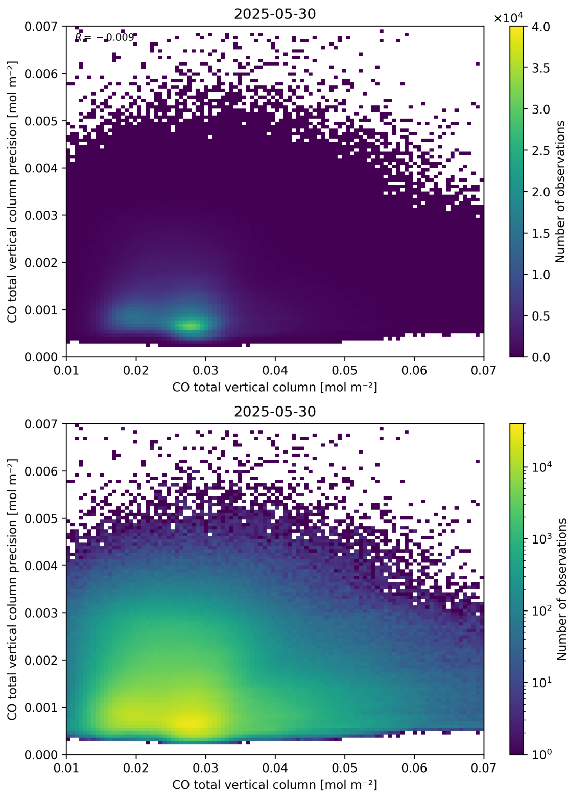
Figure 34: Scatter density plot of “CO total vertical column” against “CO total vertical column precision” for 2025-05-29 to 2025-05-31.
