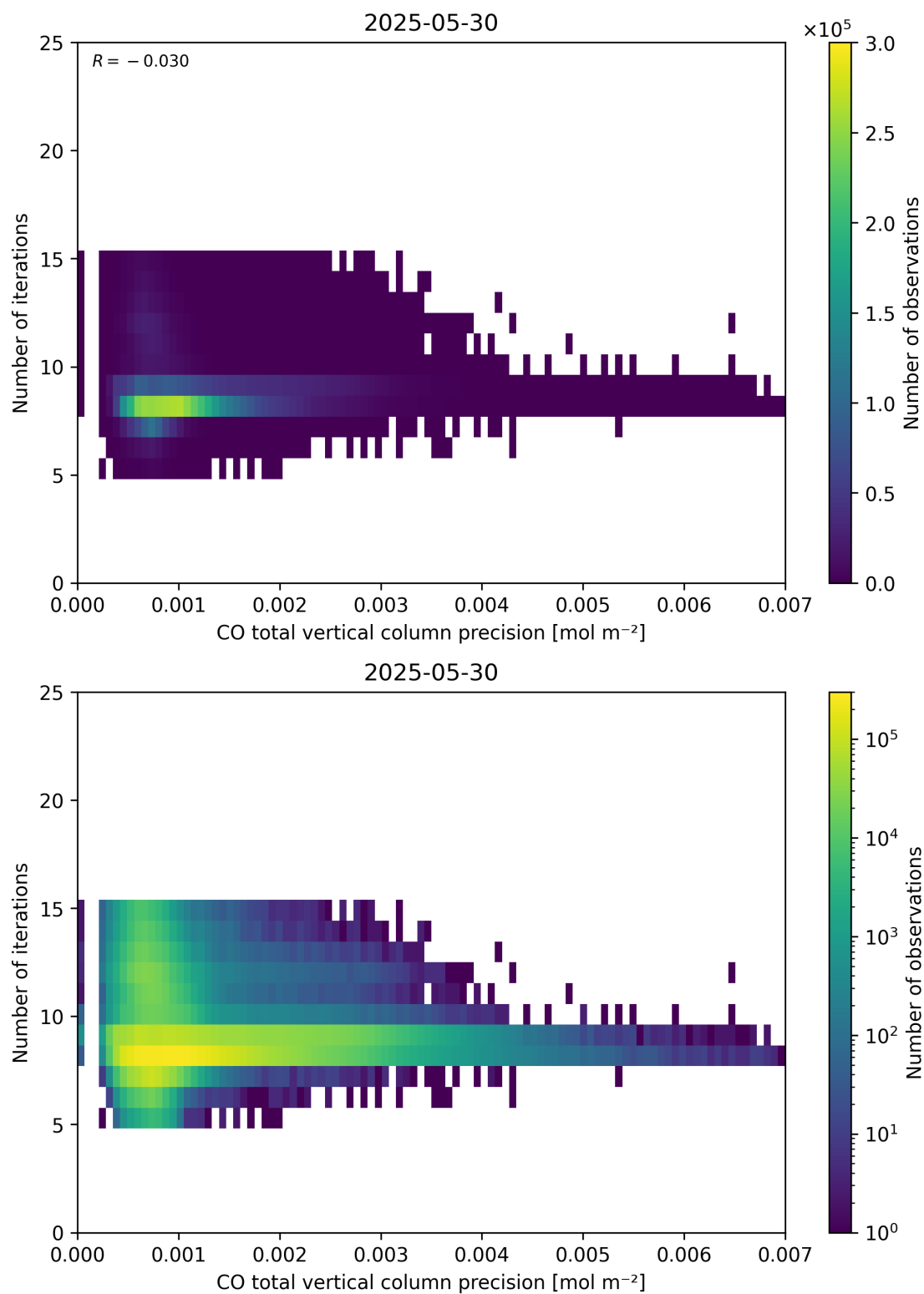
Figure 46: Scatter density plot of “CO total vertical column precision” against “Number of iterations” for 2025-05-29 to 2025-05-31.
