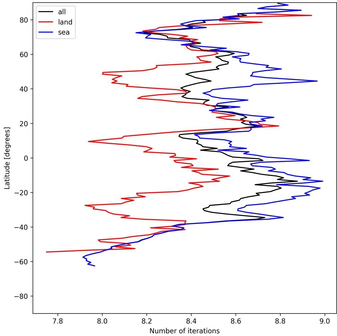
Figure 16: Zonal average of “Number of iterations” for 2025-05-29 to 2025-05-31.
