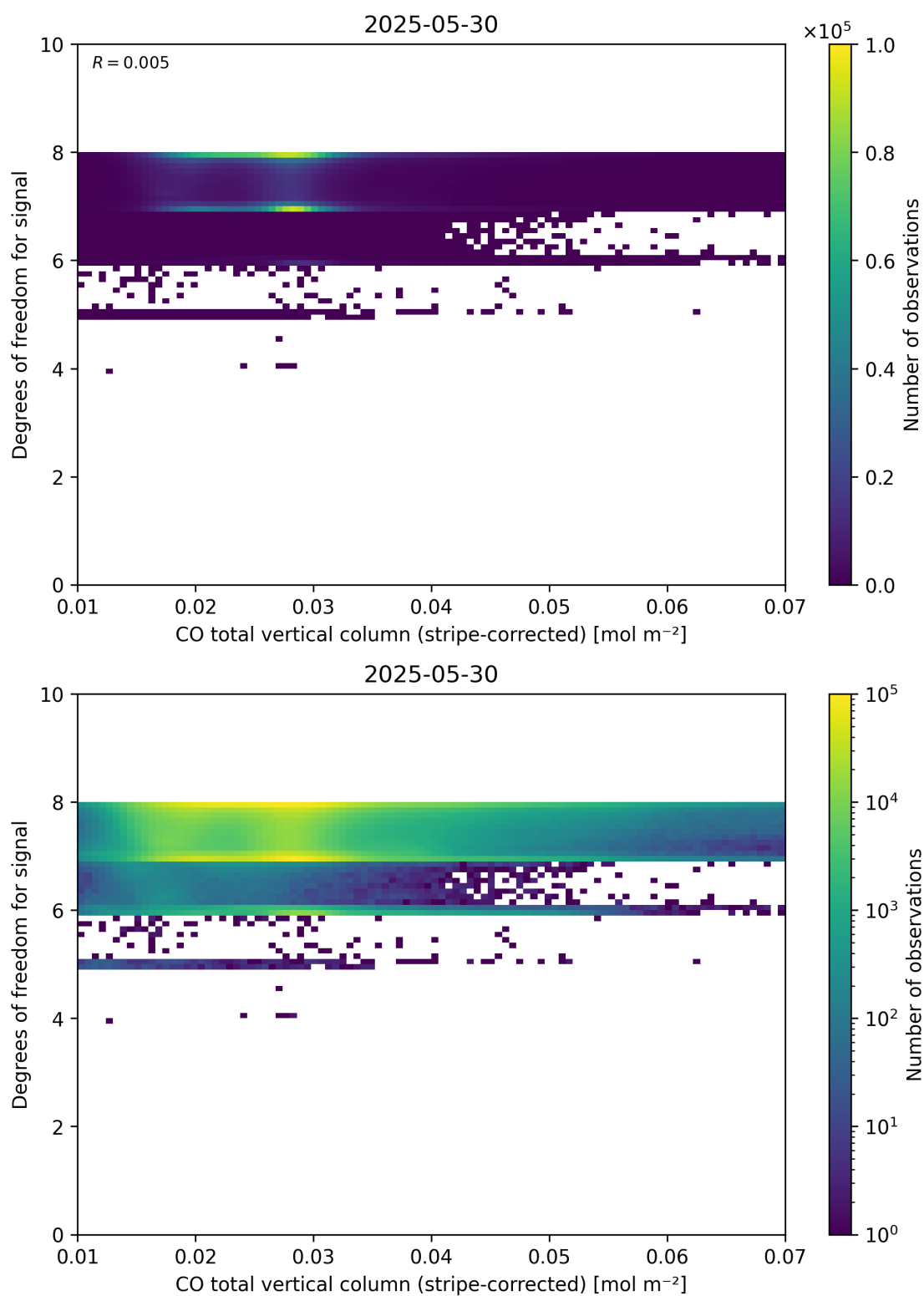
Figure 38: Scatter density plot of “CO total vertical column (stripe-corrected)” against “Degrees of freedom for signal” for 2025-05-29 to 2025-05-31.
