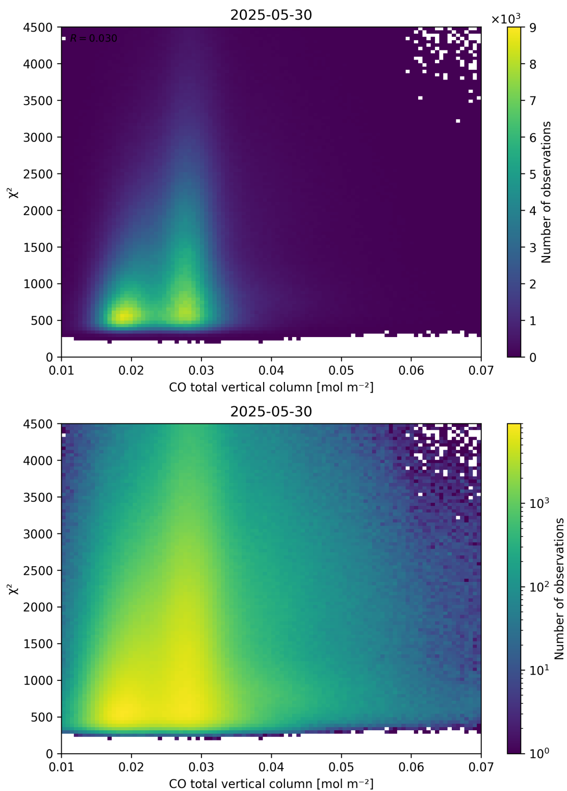
Figure 35: Scatter density plot of “CO total vertical column” against “ \chi^2 ” for 2025-05-29 to 2025-05-31.
