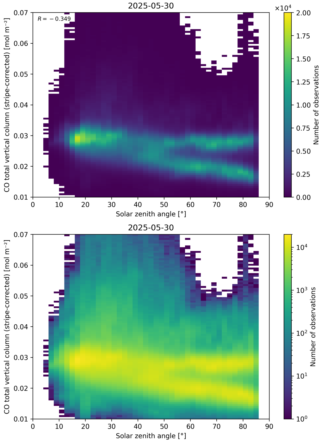
Figure 62: Scatter density plot of “Solar zenith angle” against “CO total vertical column (stripe-corrected)” for 2025-05-29 to 2025-05-31.
