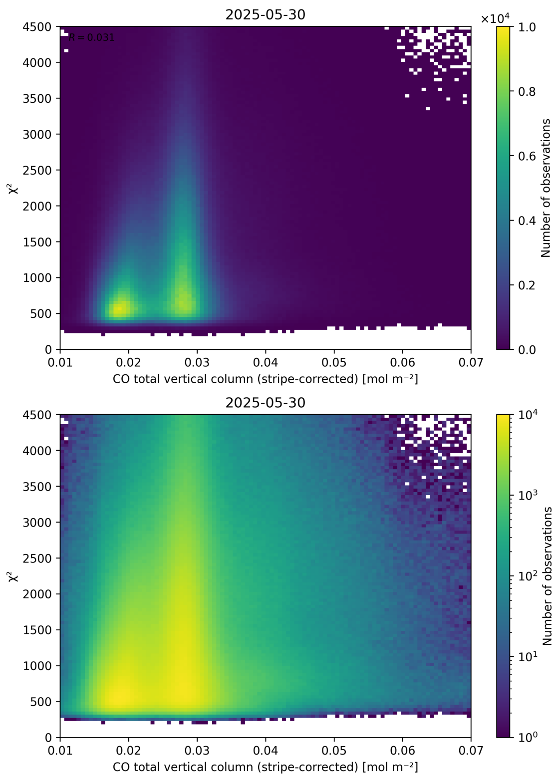
Figure 37: Scatter density plot of “CO total vertical column (stripe-corrected)” against “ \chi^2 ” for 2025-05-29 to 2025-05-31.
