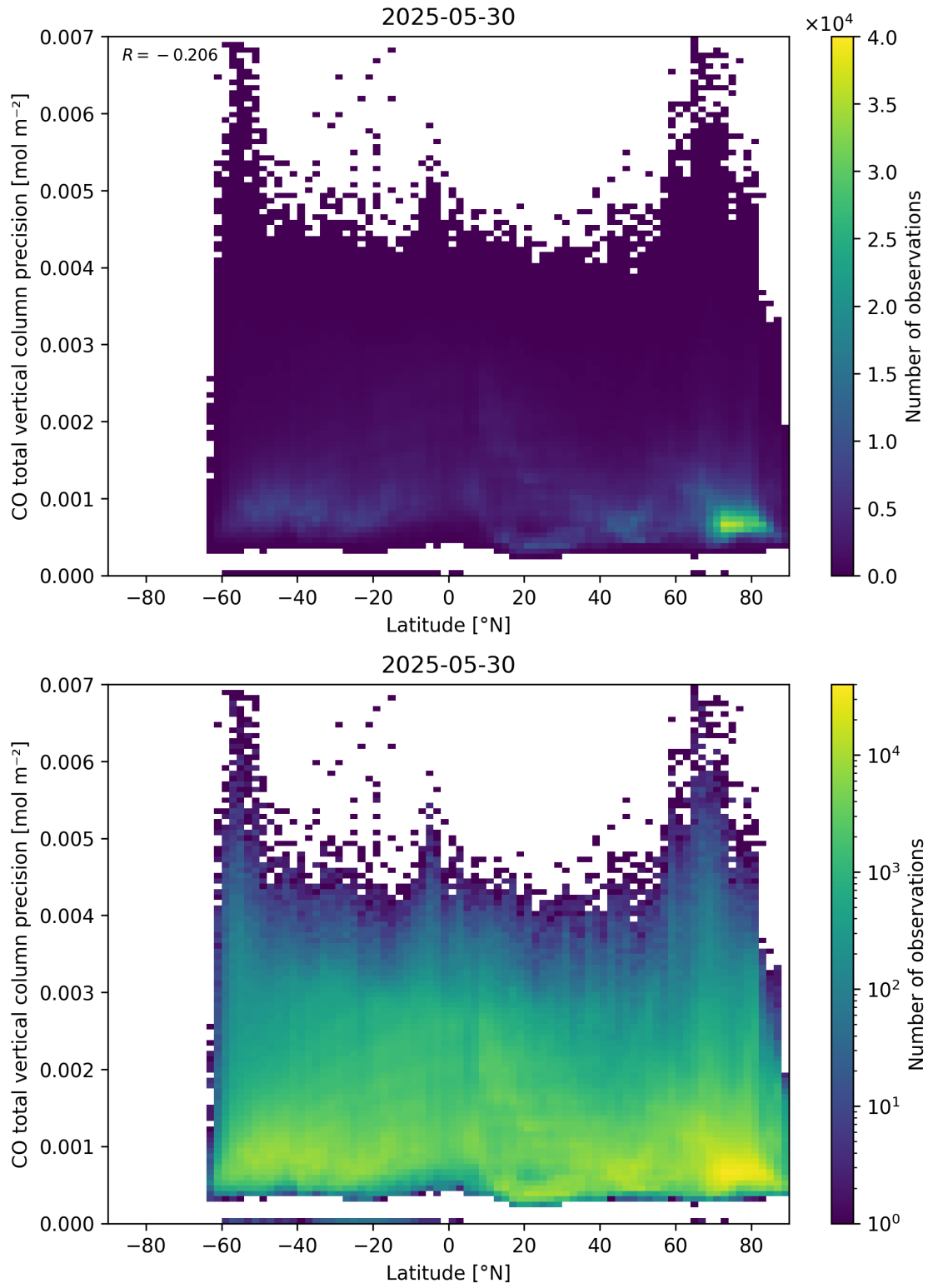
Figure 53: Scatter density plot of “Latitude” against “CO total vertical column precision” for 2025-05-29 to 2025-05-31.
