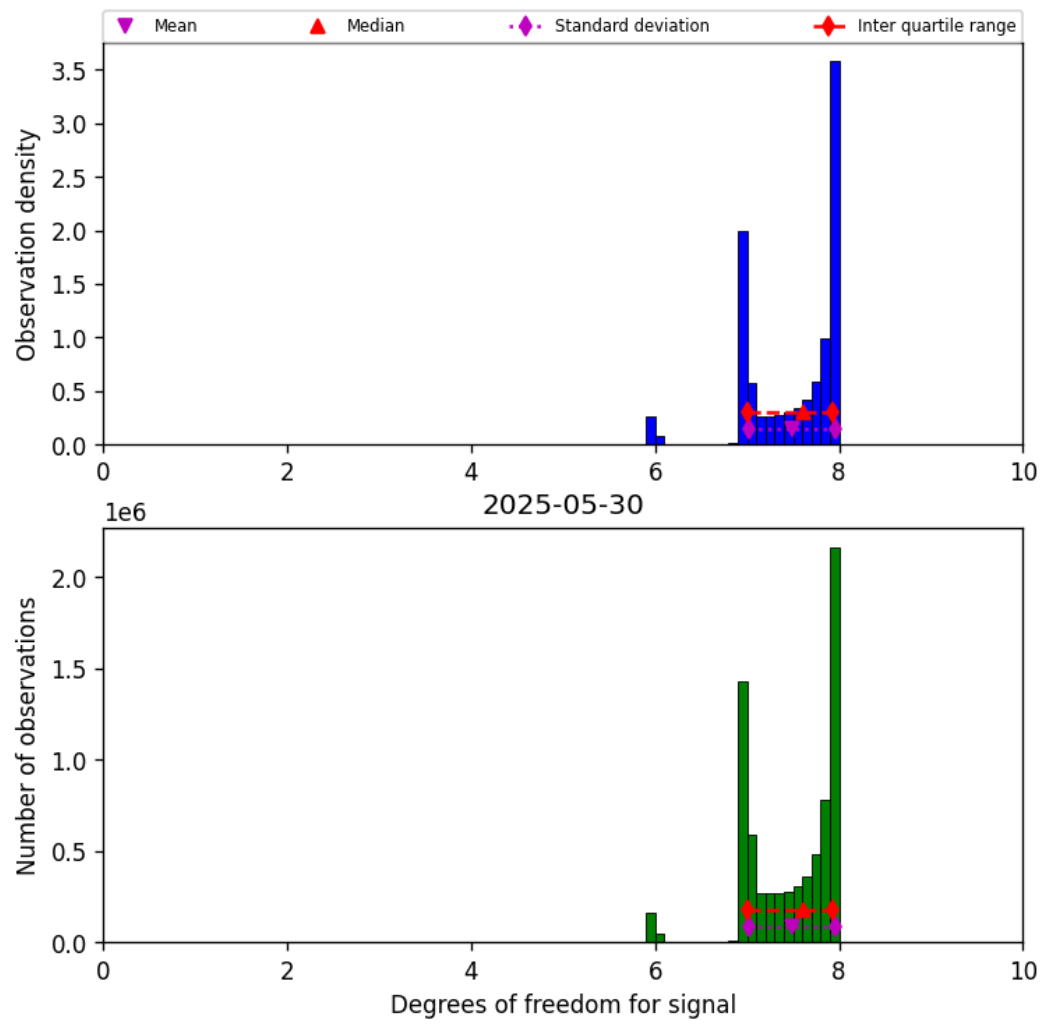
Figure 23: Histogram of “Degrees of freedom for signal” for 2025-05-29 to 2025-05-31
