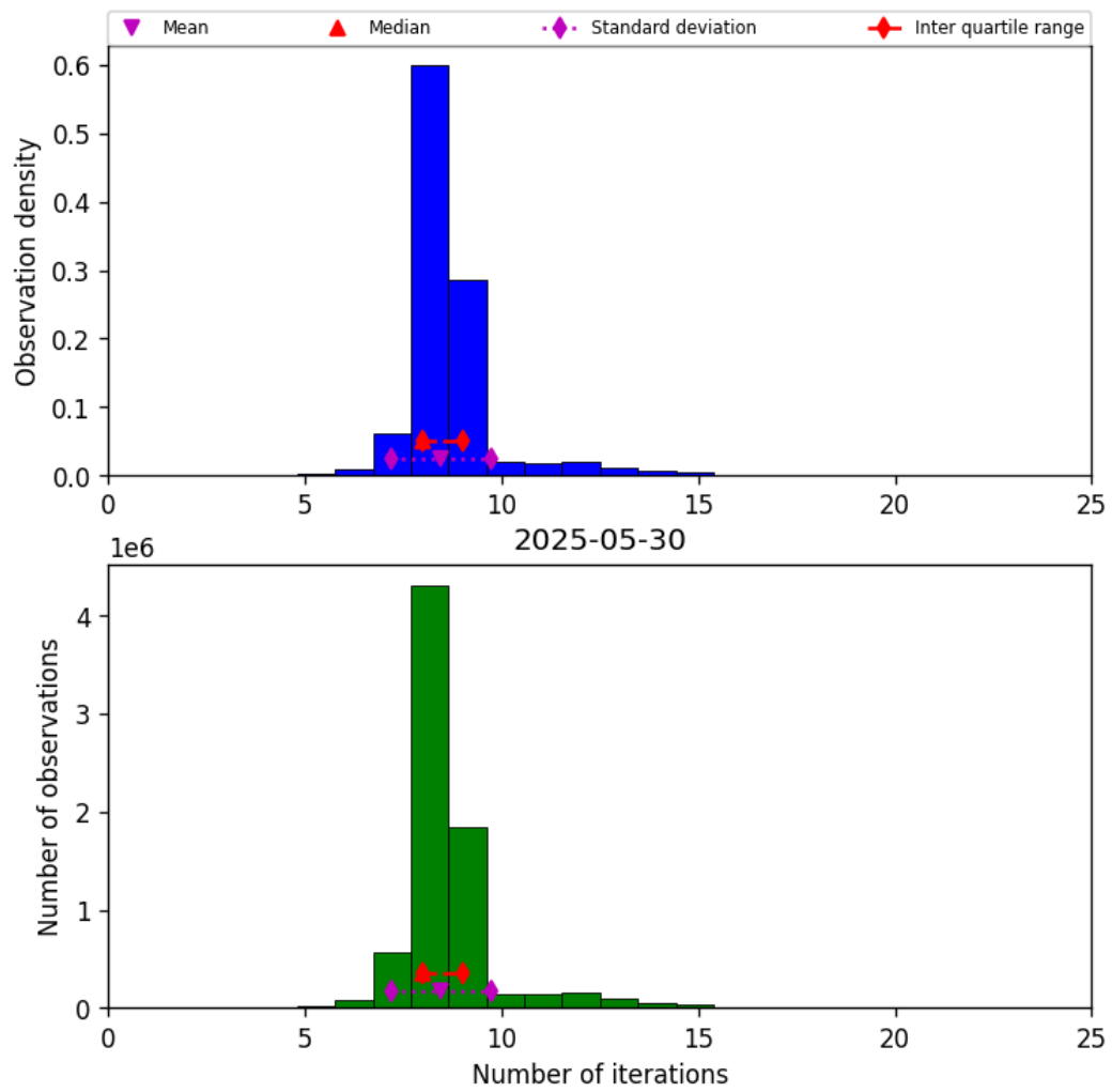
Figure 24: Histogram of “Number of iterations” for 2025-05-29 to 2025-05-31
