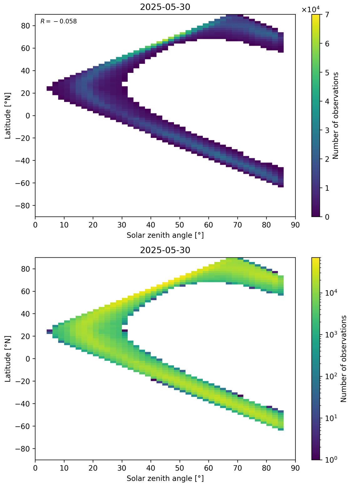
Figure 66: Scatter density plot of “Solar zenith angle” against “Latitude” for 2025-05-29 to 2025-05-31.
