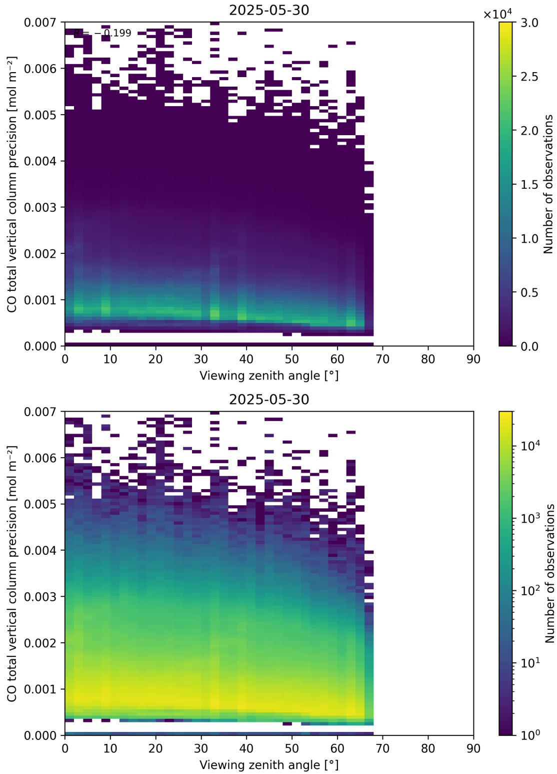
Figure 71: Scatter density plot of “Viewing zenith angle” against “CO total vertical column precision” for 2025-05-29 to 2025-05-31.
