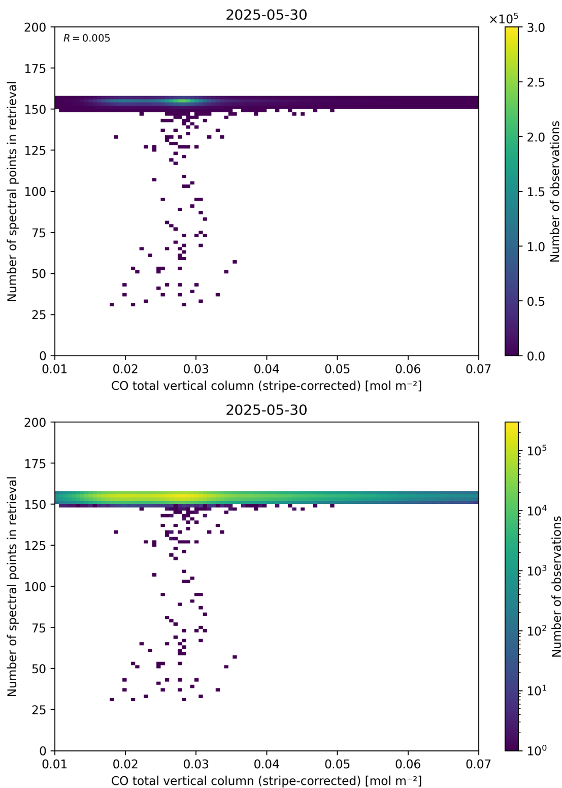
Figure 40: Scatter density plot of “CO total vertical column (stripe-corrected)” against “Number of spectral points in retrieval” for 2025-05-29 to 2025-05-31.
