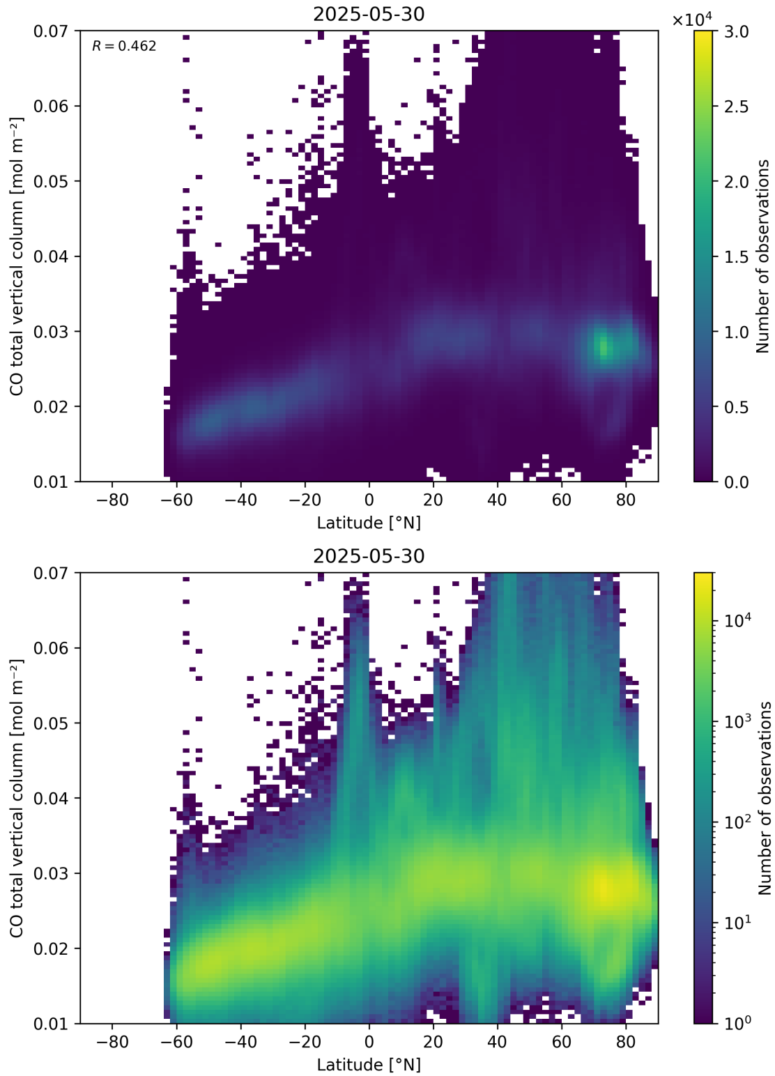
Figure 51: Scatter density plot of “Latitude” against “CO total vertical column” for 2025-05-29 to 2025-05-31.
