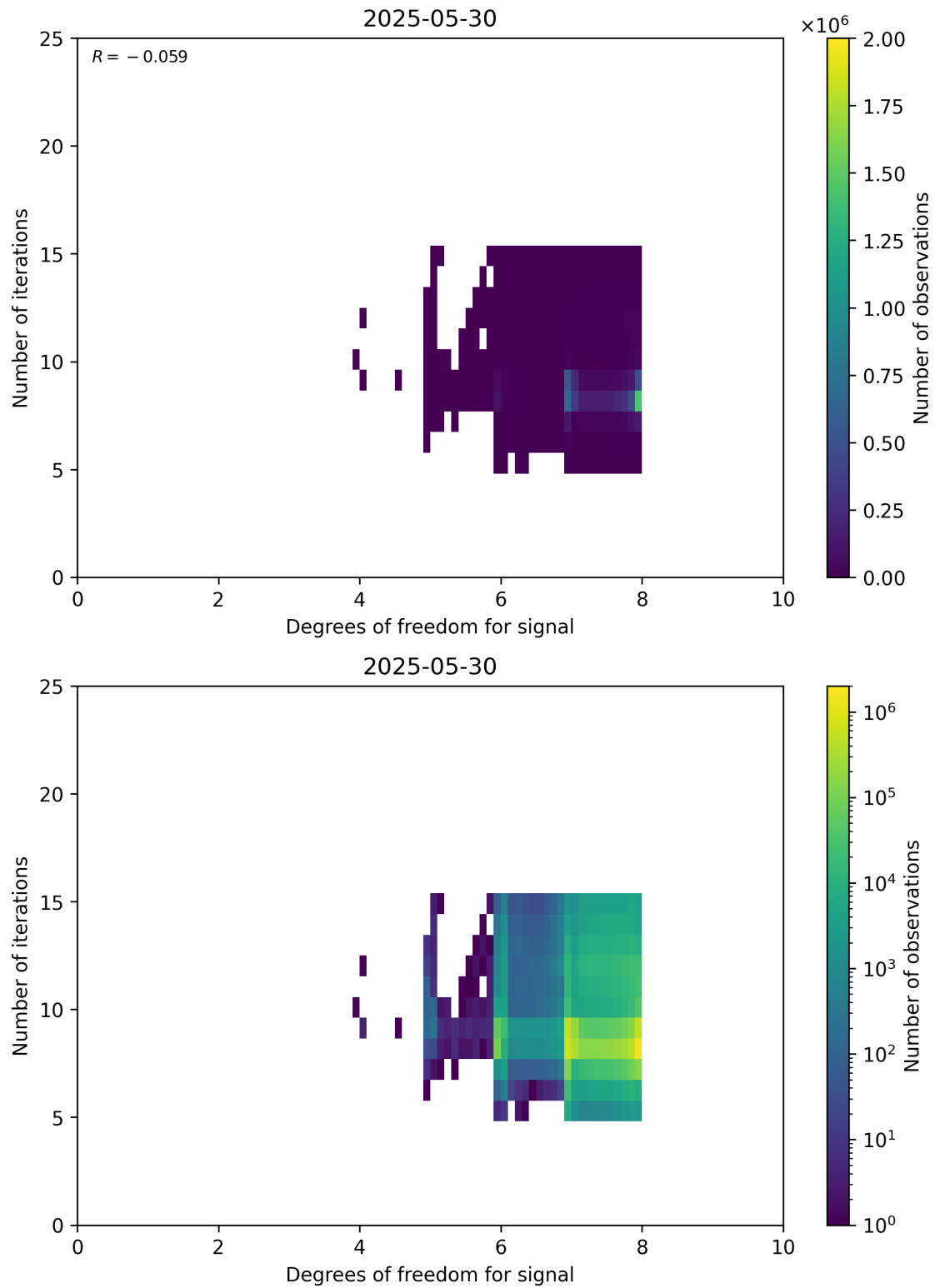
Figure 50: Scatter density plot of “Degrees of freedom for signal” against “Number of iterations” for 2025-05-29 to 2025-05-31.
