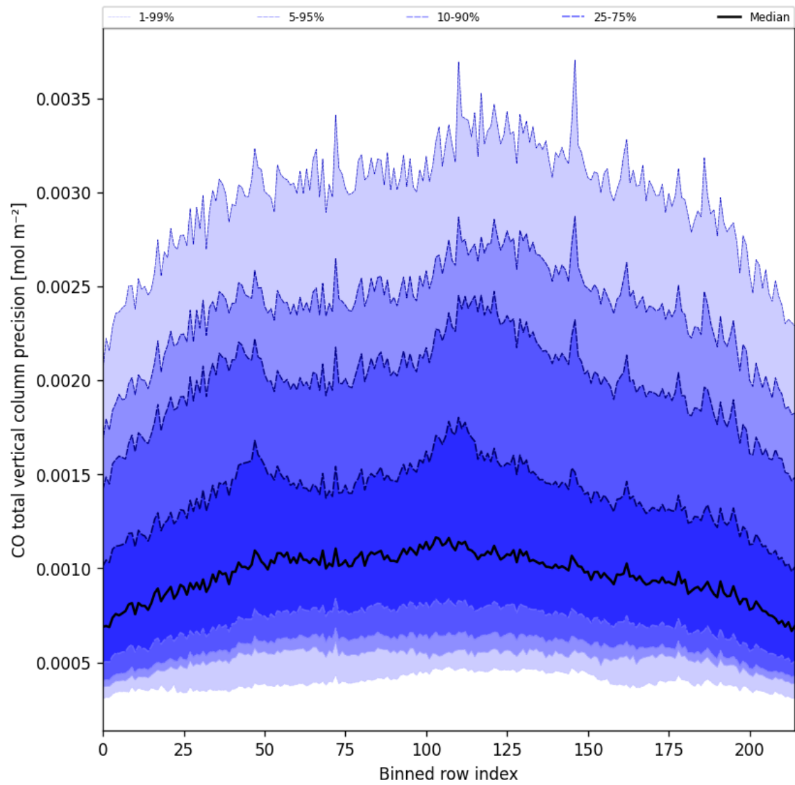
Figure 28: Along track statistics of “CO total vertical column precision” for 2025-05-29 to 2025-05-31
