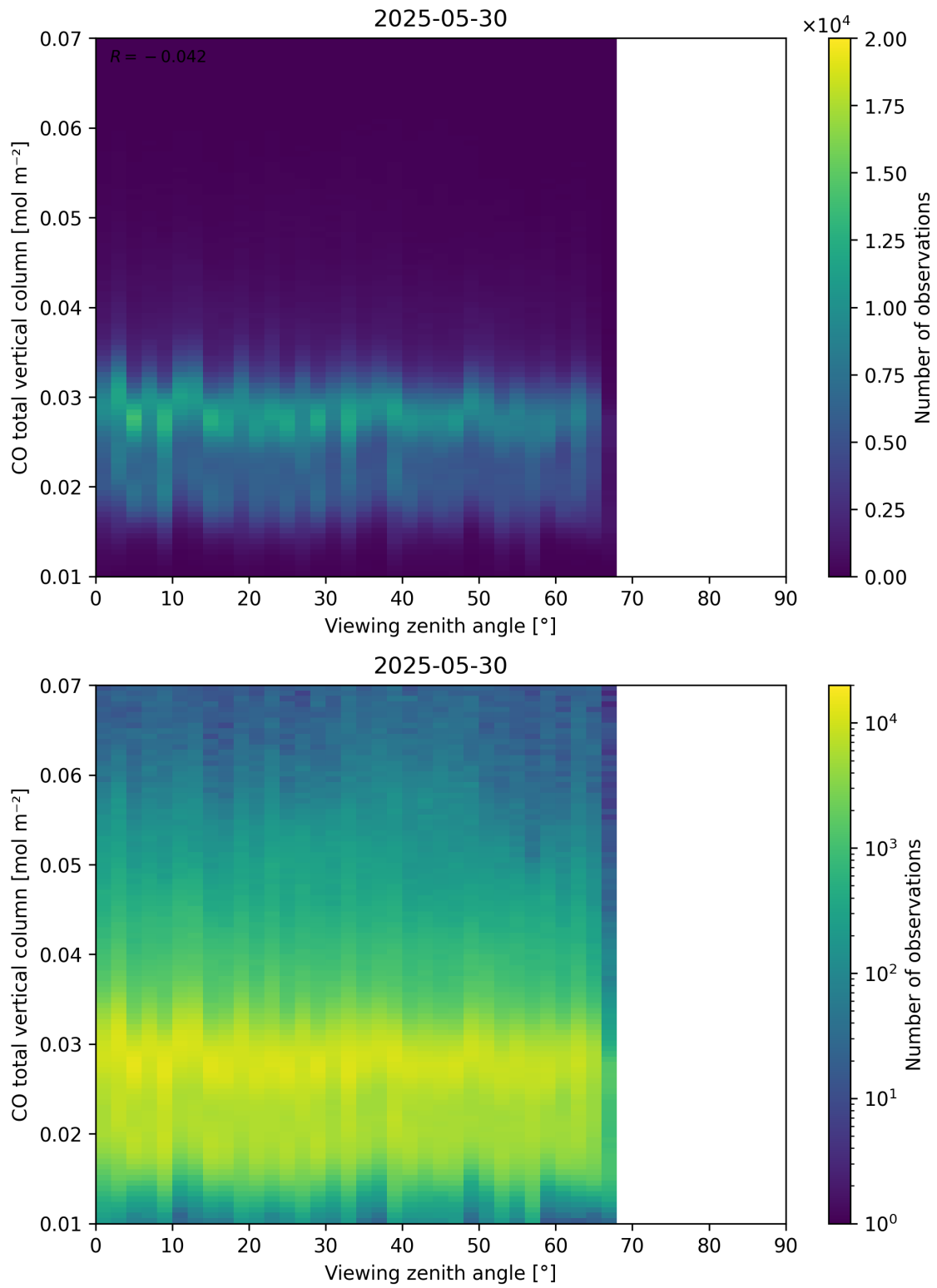
Figure 69: Scatter density plot of “Viewing zenith angle” against “CO total vertical column” for 2025-05-29 to 2025-05-31.
