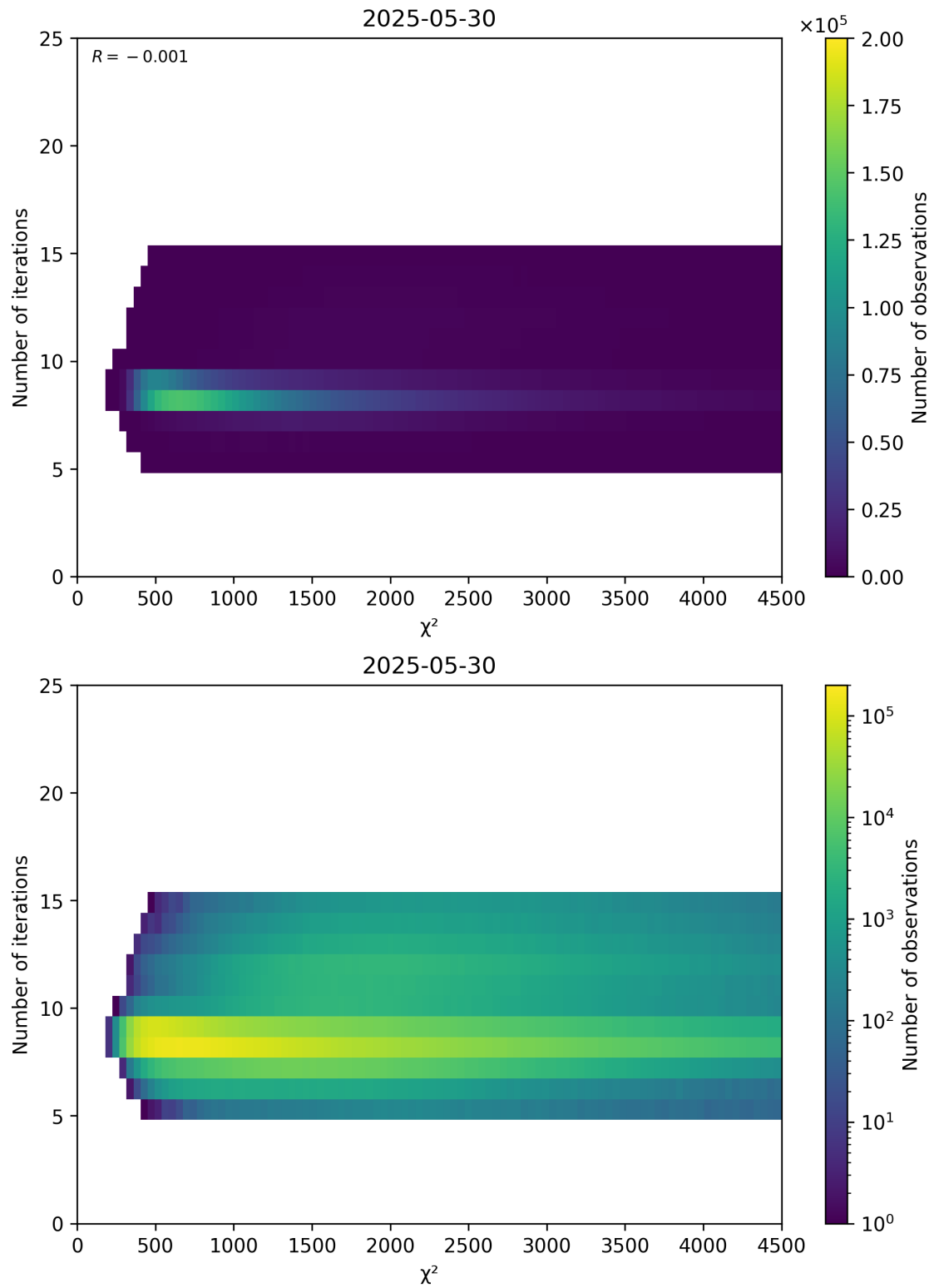
Figure 49: Scatter density plot of “ \chi^2 ” against “Number of iterations” for 2025-05-29 to 2025-05-31.
