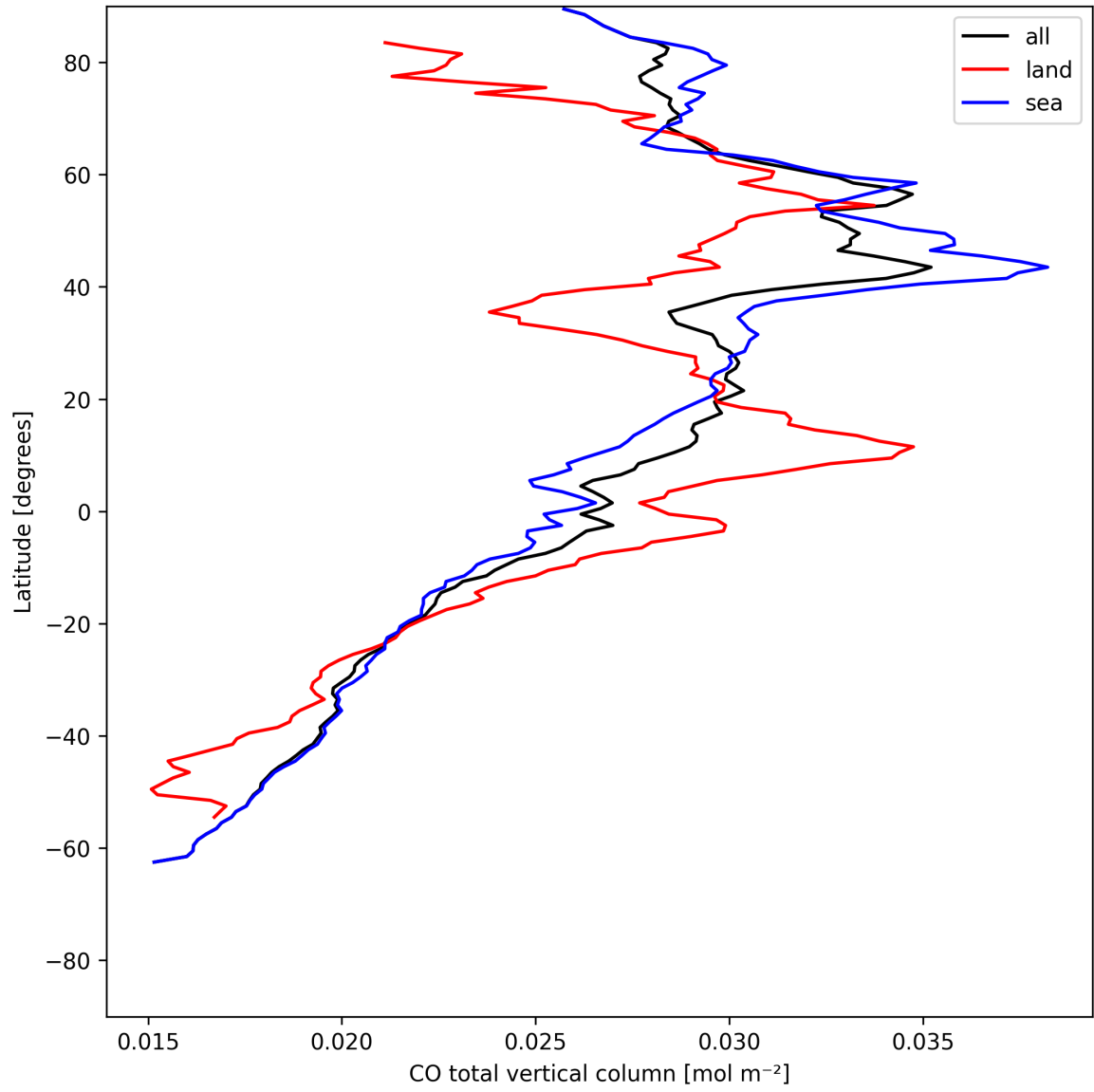
Figure 10: Zonal average of “CO total vertical column” for 2025-05-29 to 2025-05-31.
