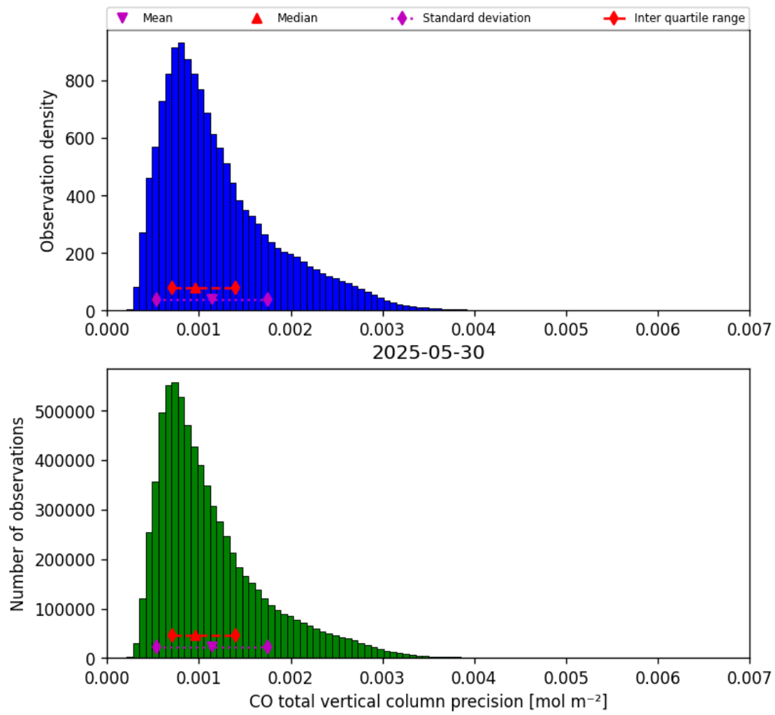
Figure 20: Histogram of “CO total vertical column precision” for 2025-05-29 to 2025-05-31
