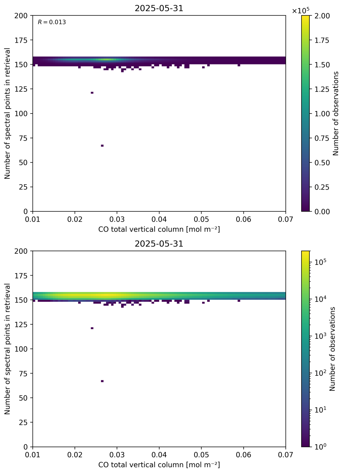
Figure 43: Scatter density plot of “CO total vertical column” against “Number of spectral points in retrieval” for 2025-05-31 to 2025-06-01.
