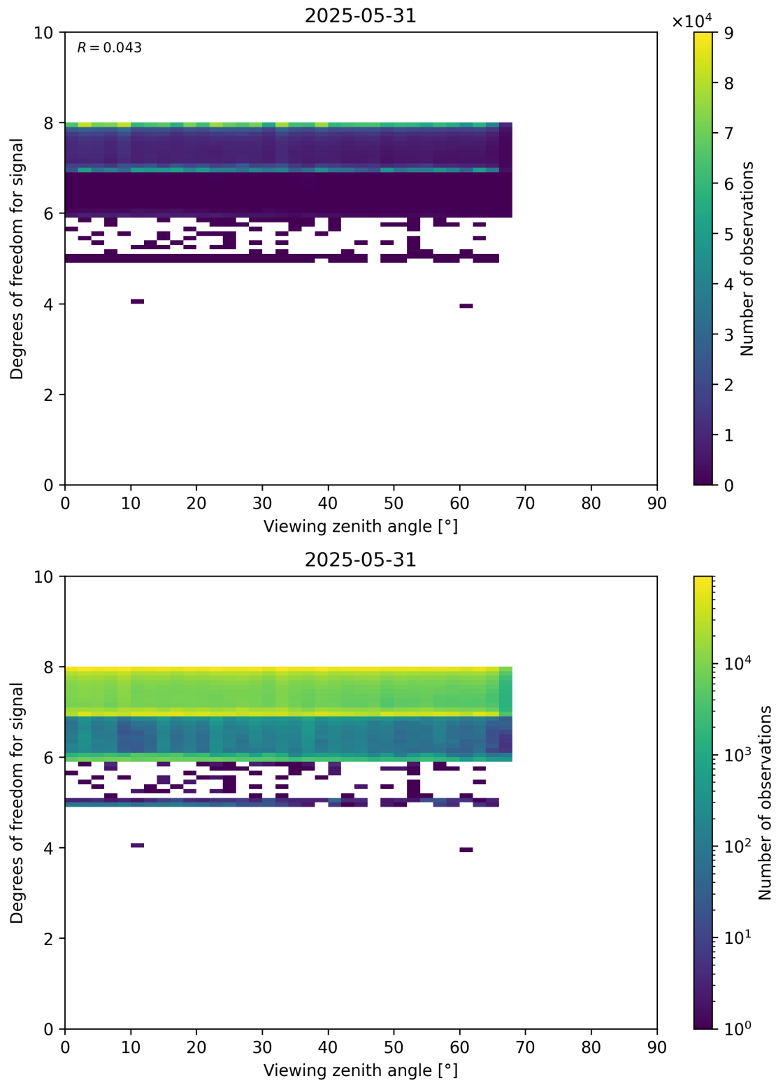
Figure 73: Scatter density plot of “Viewing zenith angle” against “Degrees of freedom for signal” for 2025-05-31 to 2025-06-01.
