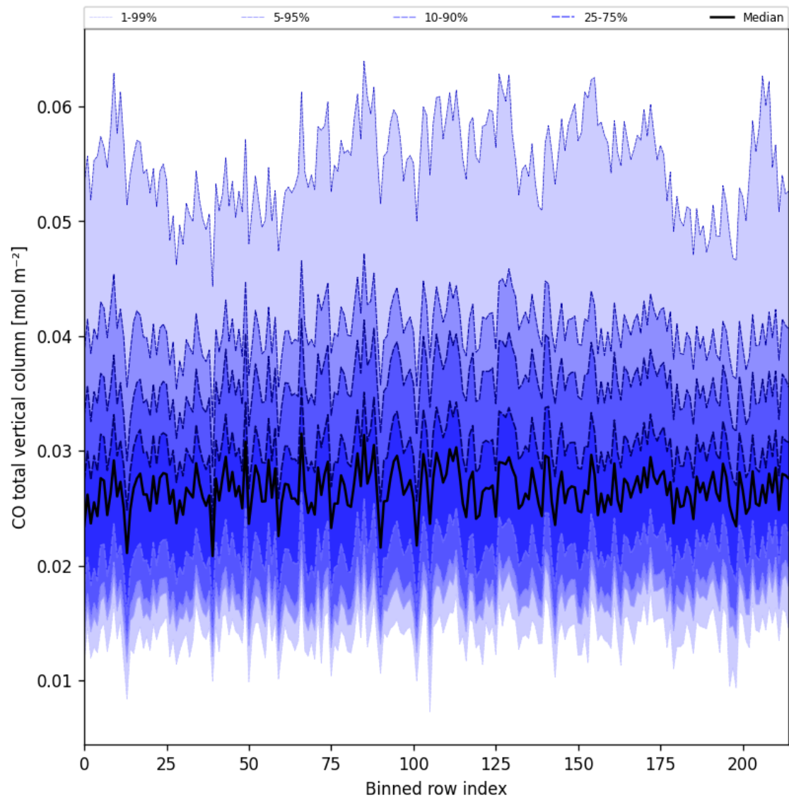
Figure 26: Along track statistics of “CO total vertical column” for 2025-05-31 to 2025-06-01
