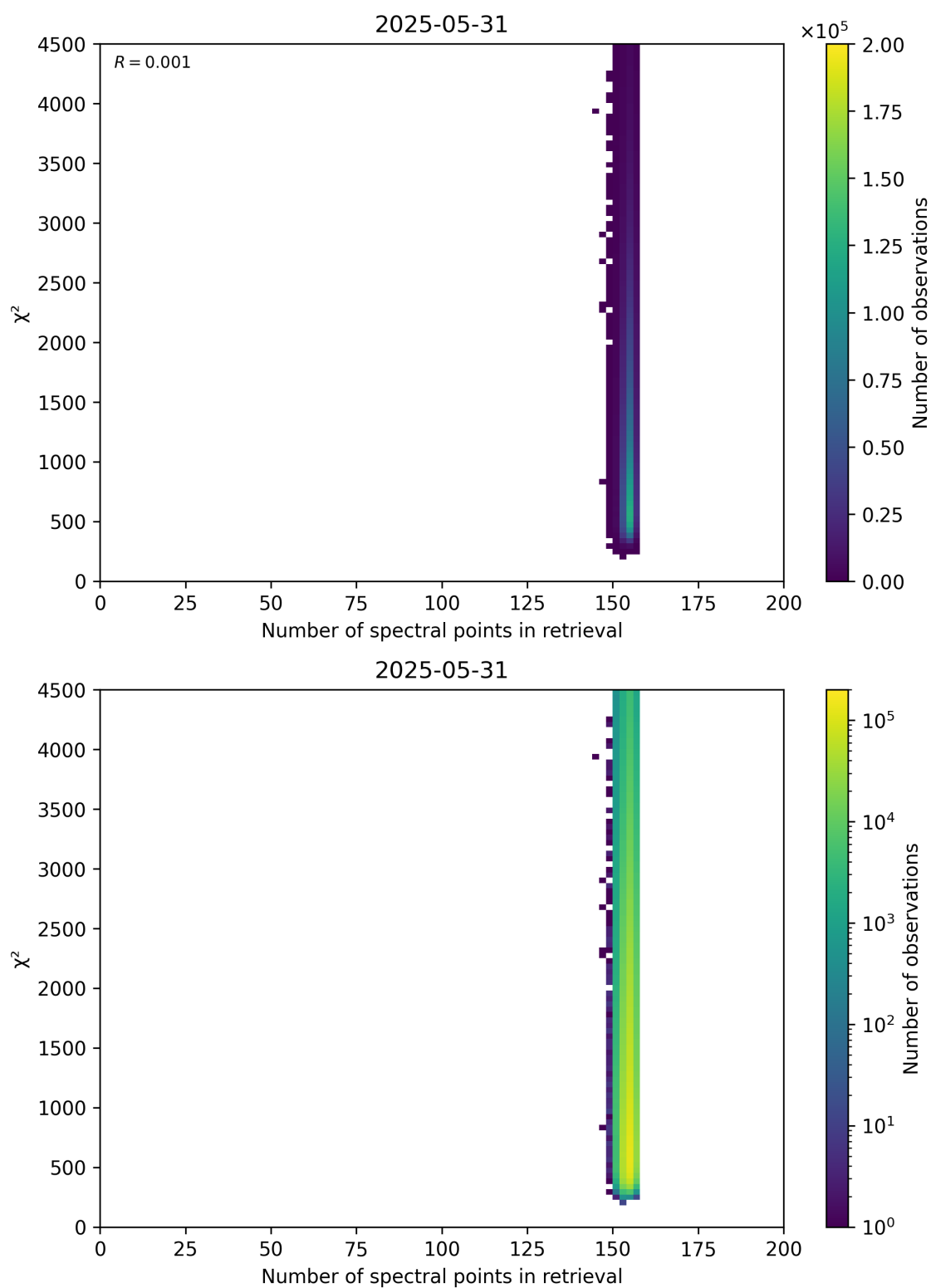
Figure 58: Scatter density plot of “Number of spectral points in retrieval” against “ \chi^2 ” for 2025-05-31 to 2025-06-01.
