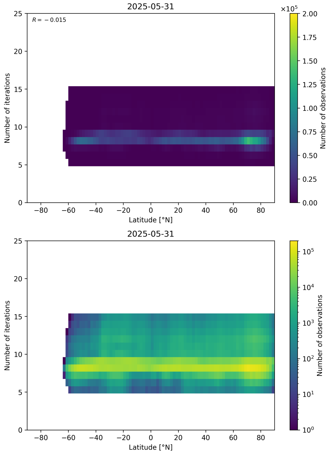
Figure 56: Scatter density plot of “Latitude” against “Number of iterations” for 2025-05-31 to 2025-06-01.
