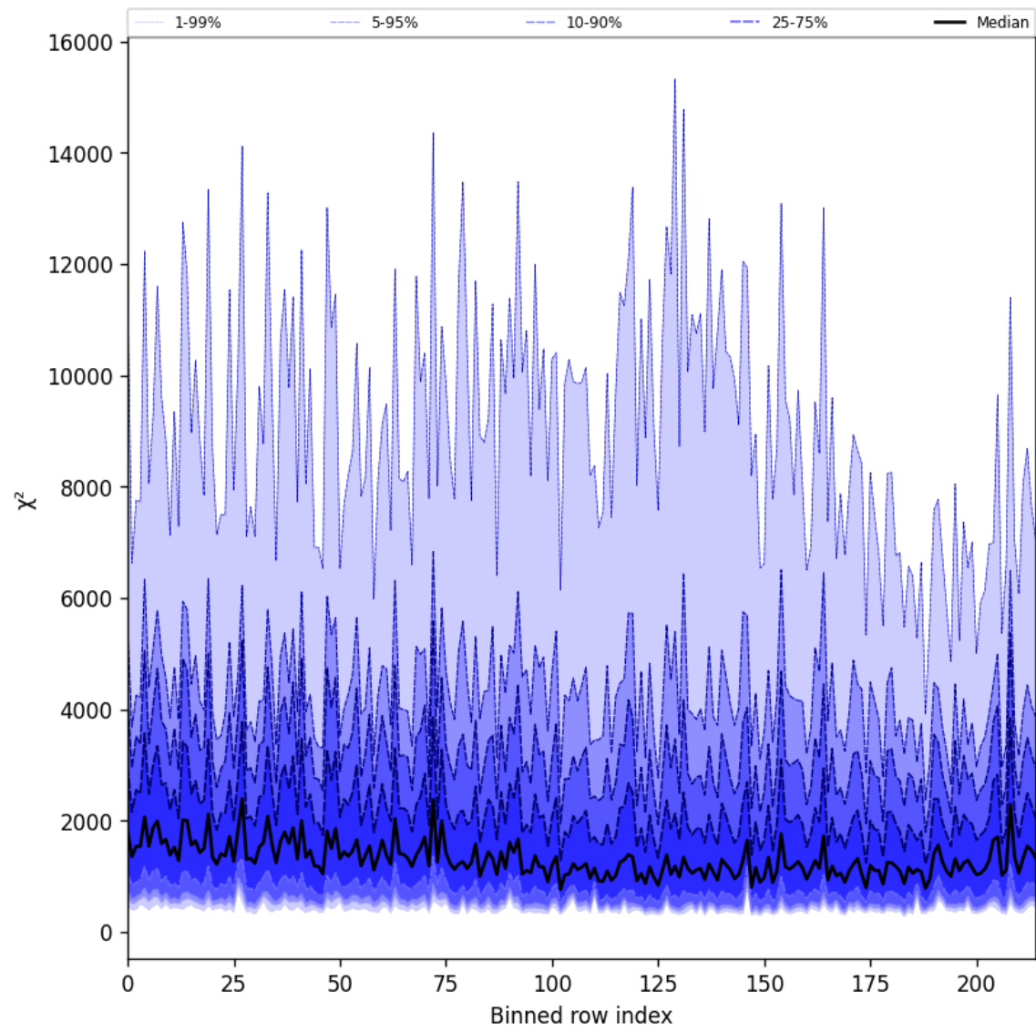
Figure 30: Along track statistics of “ \chi^2 ” for 2025-05-31 to 2025-06-01
