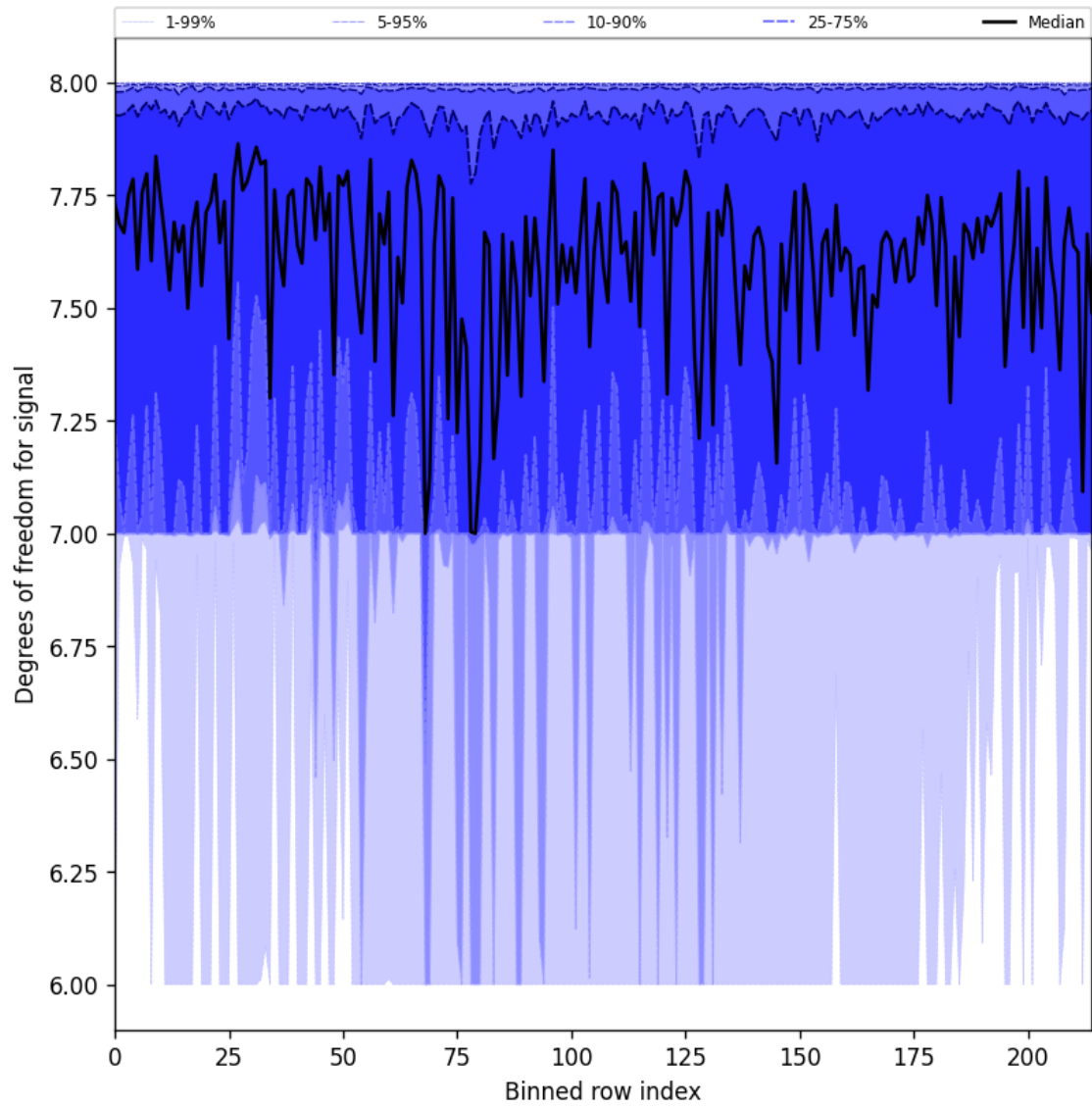
Figure 31: Along track statistics of “Degrees of freedom for signal” for 2025-05-31 to 2025-06-01
