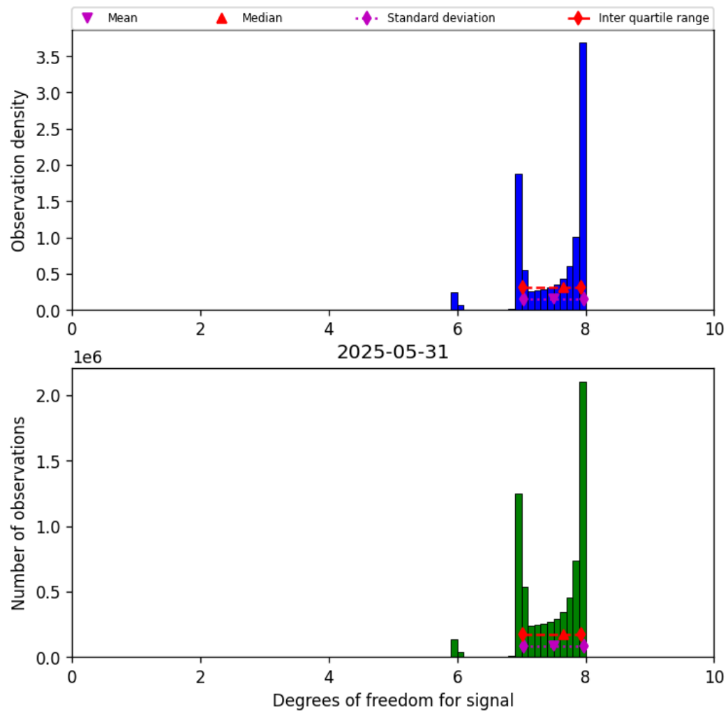
Figure 23: Histogram of “Degrees of freedom for signal” for 2025-05-31 to 2025-06-01
