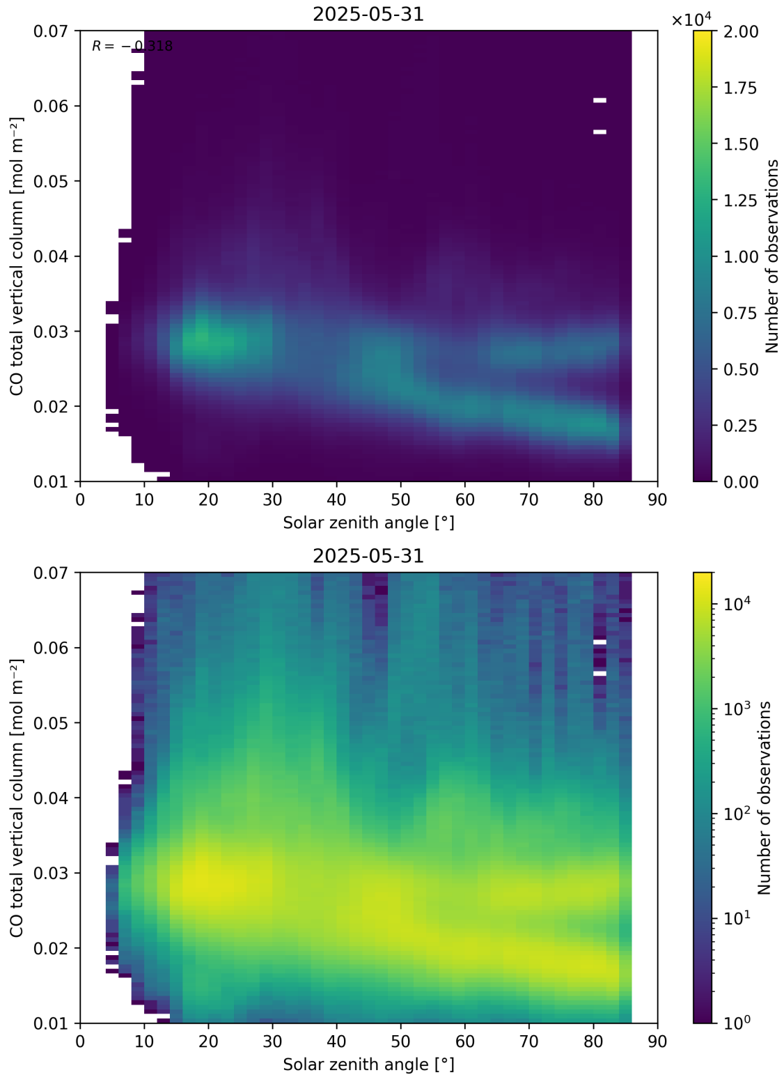
Figure 61: Scatter density plot of “Solar zenith angle” against “CO total vertical column” for 2025-05-31 to 2025-06-01.
