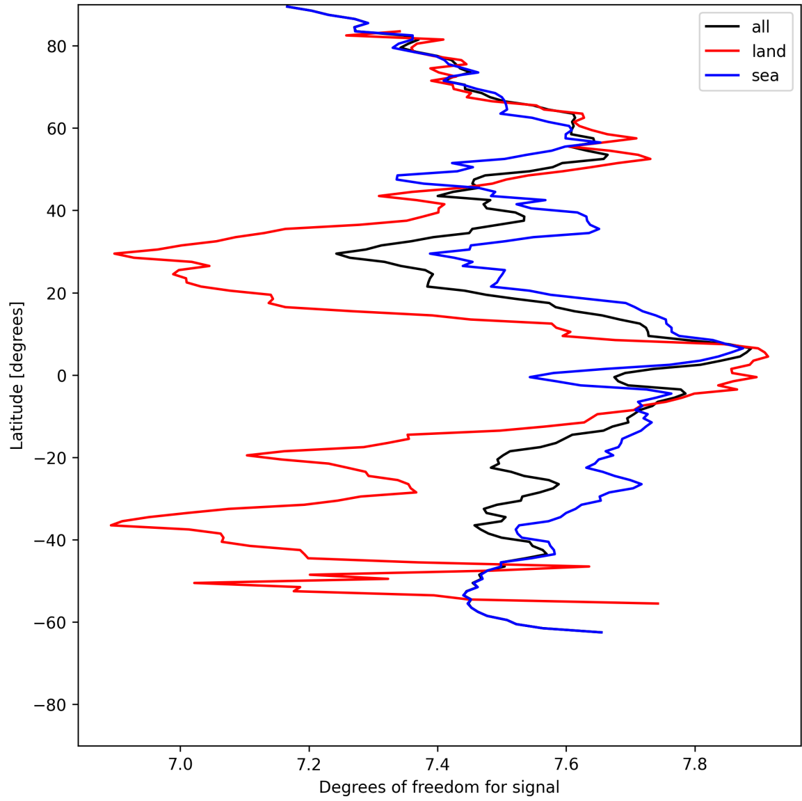
Figure 15: Zonal average of “Degrees of freedom for signal” for 2025-05-31 to 2025-06-01.
