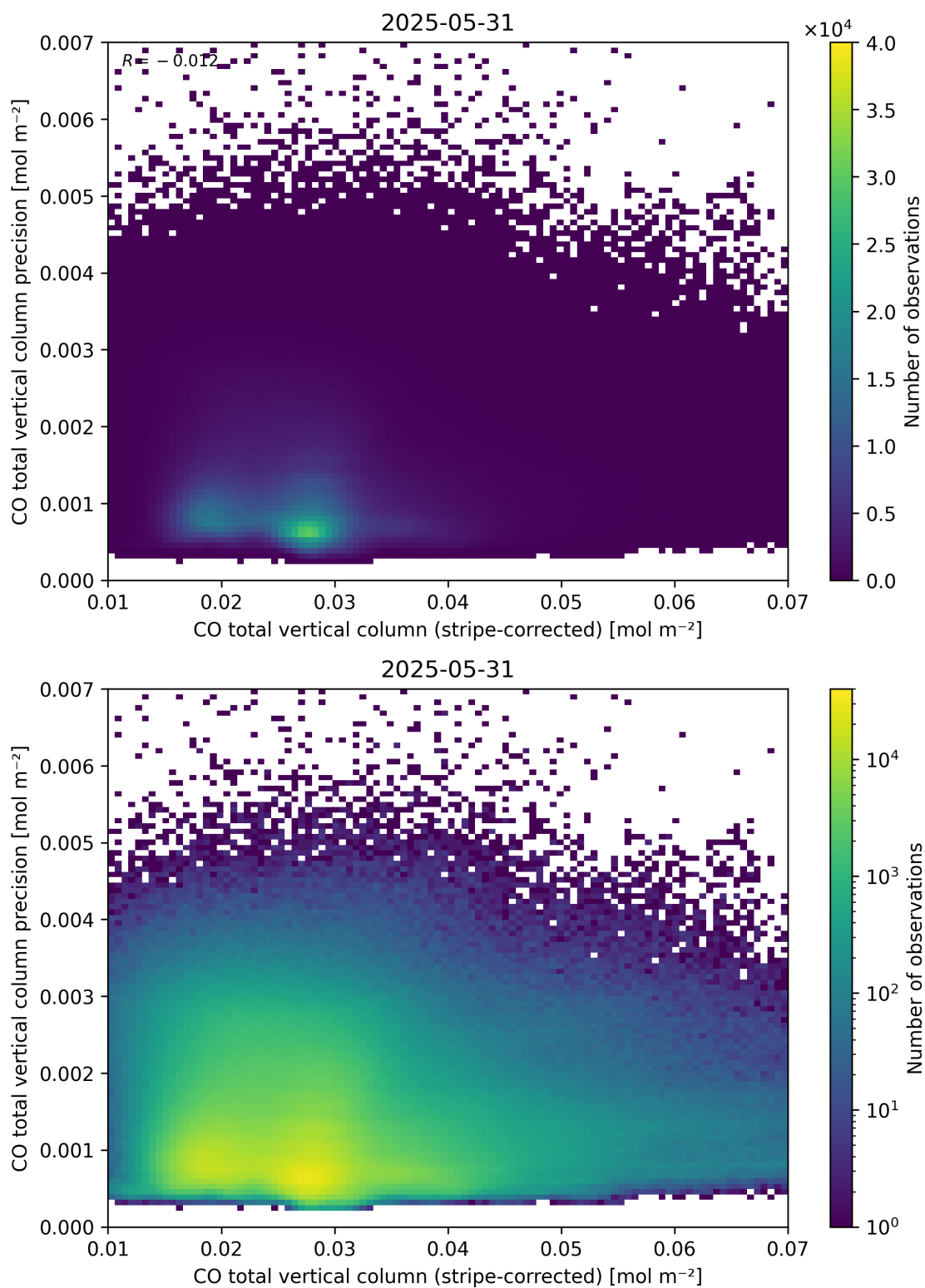
Figure 36: Scatter density plot of “CO total vertical column (stripe-corrected)” against “CO total vertical column precision” for 2025-05-31 to 2025-06-01.
