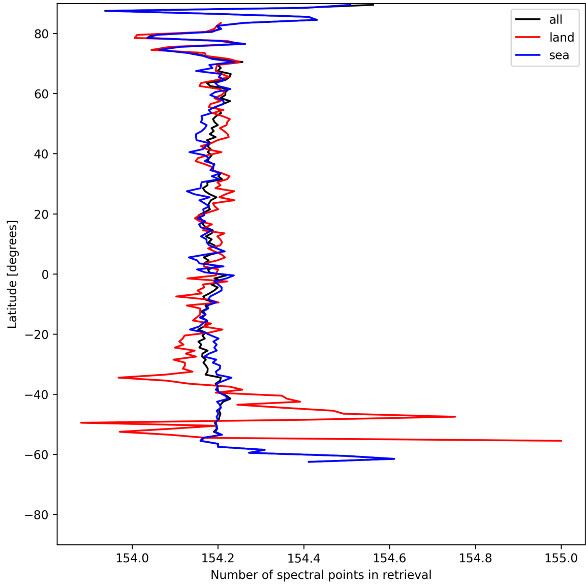
Figure 13: Zonal average of “Number of spectral points in retrieval” for 2025-05-31 to 2025-06-01.
