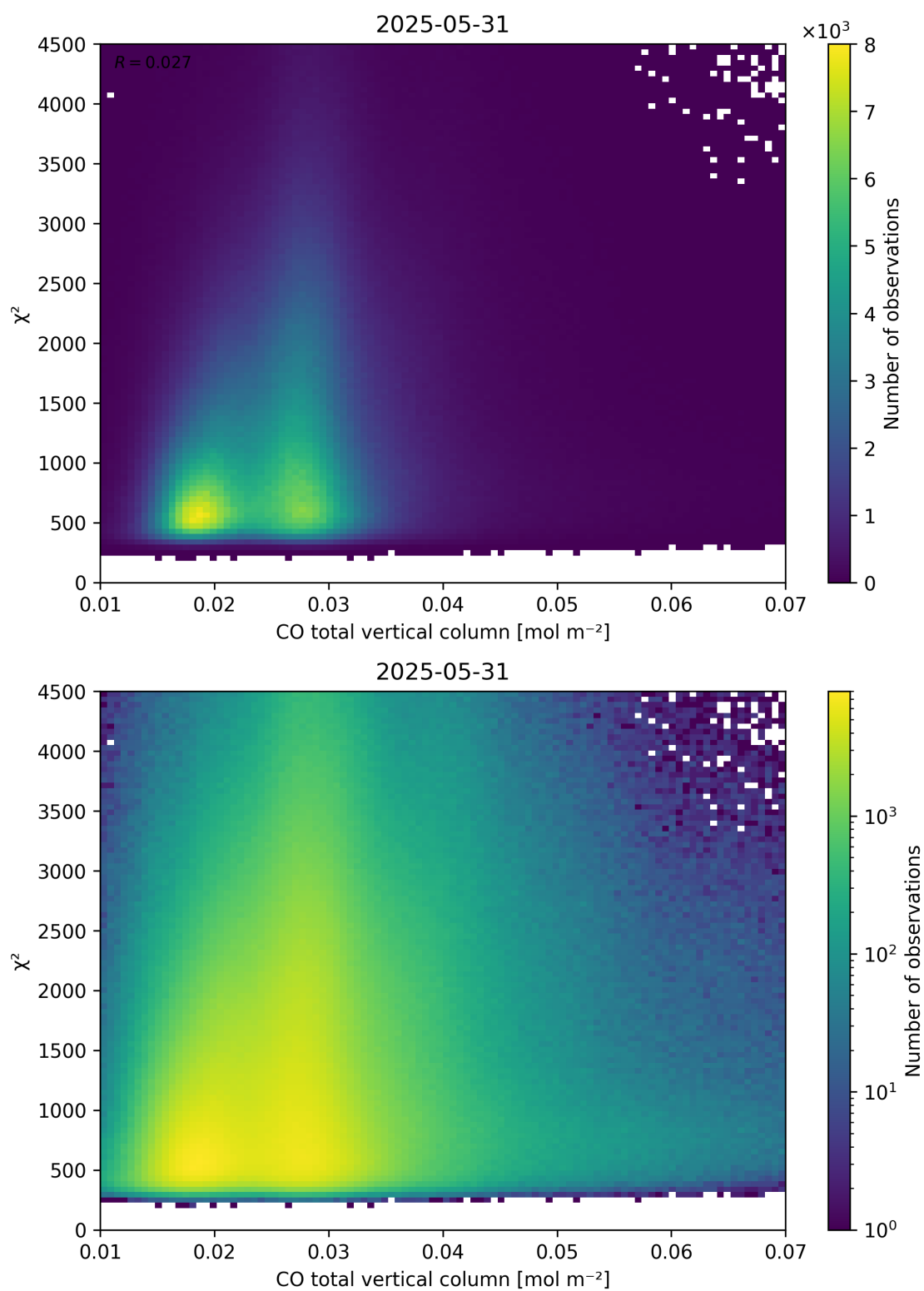
Figure 35: Scatter density plot of “CO total vertical column” against “ \chi^2 ” for 2025-05-31 to 2025-06-01.
