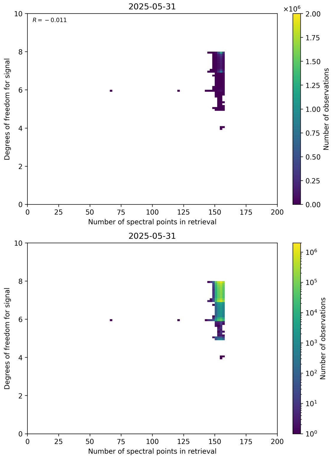
Figure 59: Scatter density plot of “Number of spectral points in retrieval” against “Degrees of freedom for signal” for 2025-05-31 to 2025-06-01.
