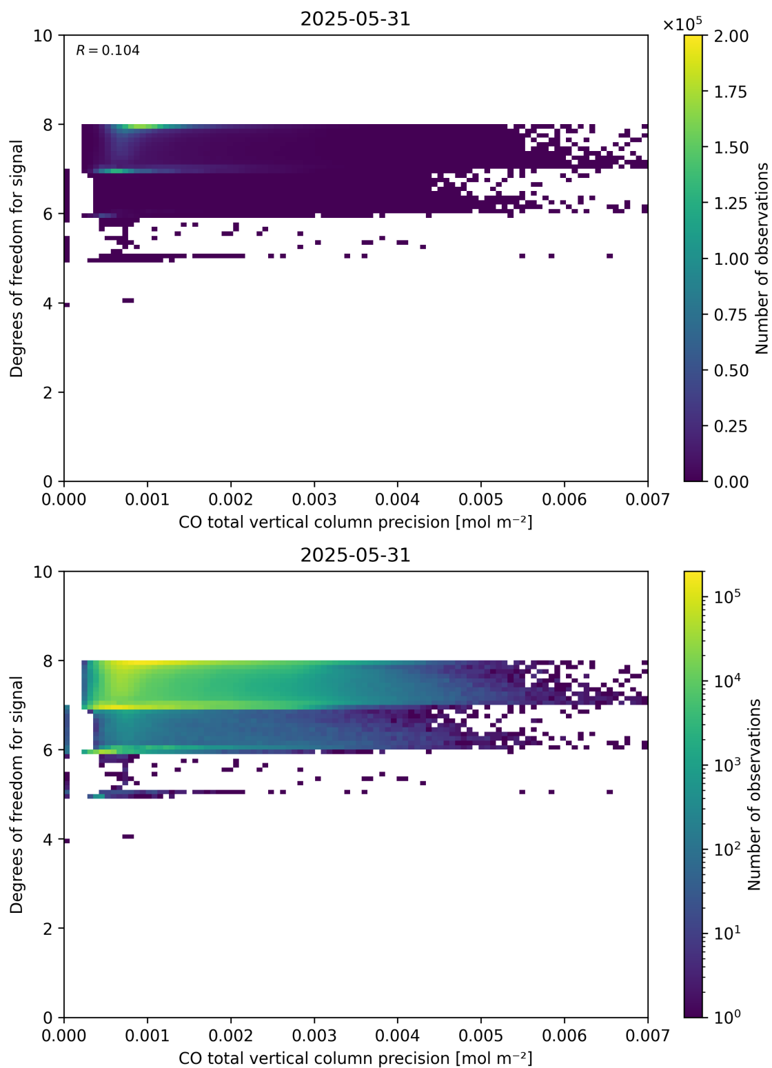
Figure 45: Scatter density plot of “CO total vertical column precision” against “Degrees of freedom for signal” for 2025-05-31 to 2025-06-01.
