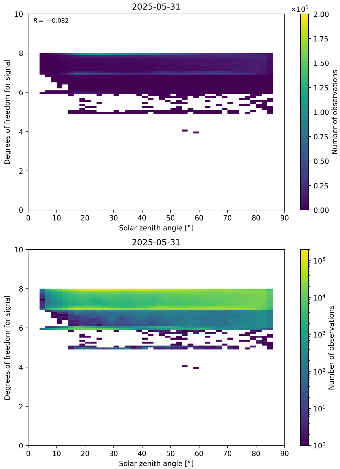
Figure 65: Scatter density plot of “Solar zenith angle” against “Degrees of freedom for signal” for 2025-05-31 to 2025-06-01.
