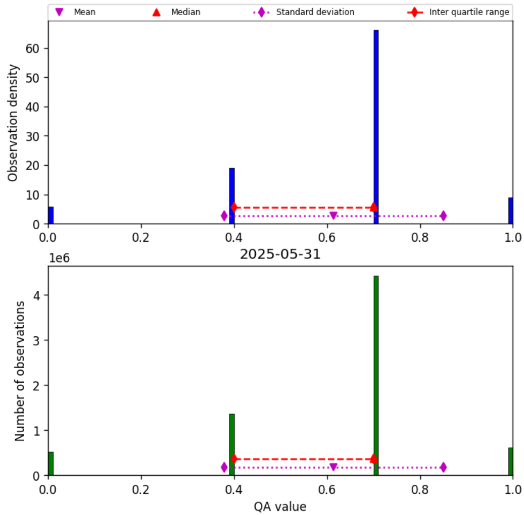
Figure 17: Histogram of “QA value” for 2025-05-31 to 2025-06-01
