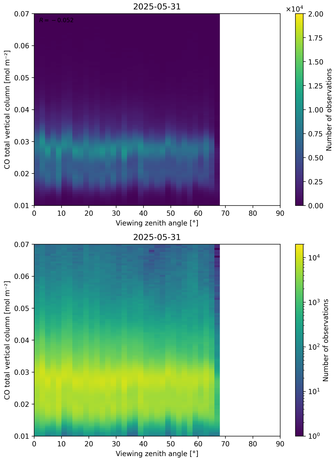
Figure 69: Scatter density plot of “Viewing zenith angle” against “CO total vertical column” for 2025-05-31 to 2025-06-01.
