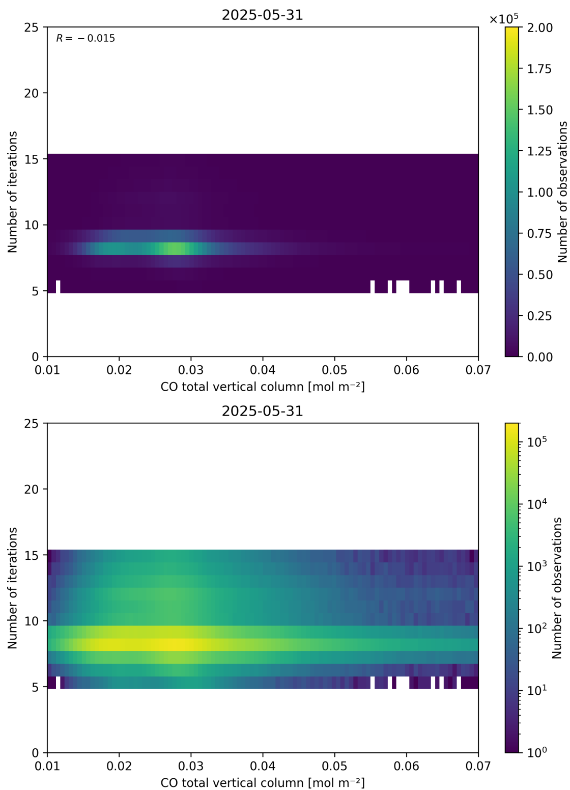
Figure 42: Scatter density plot of “CO total vertical column” against “Number of iterations” for 2025-05-31 to 2025-06-01.
