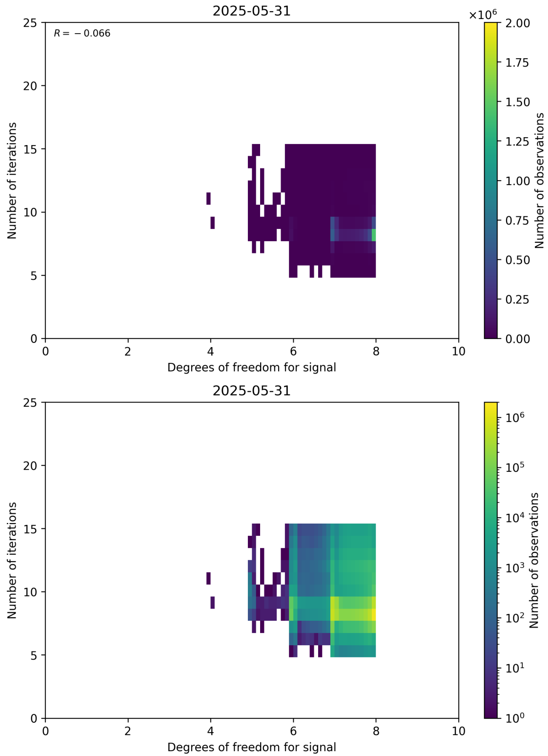
Figure 50: Scatter density plot of “Degrees of freedom for signal” against “Number of iterations” for 2025-05-31 to 2025-06-01.
