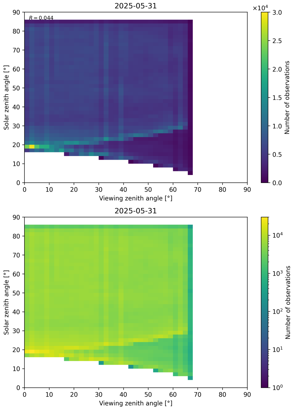
Figure 77: Scatter density plot of “Viewing zenith angle” against “Solar zenith angle” for 2025-05-31 to 2025-06-01.
