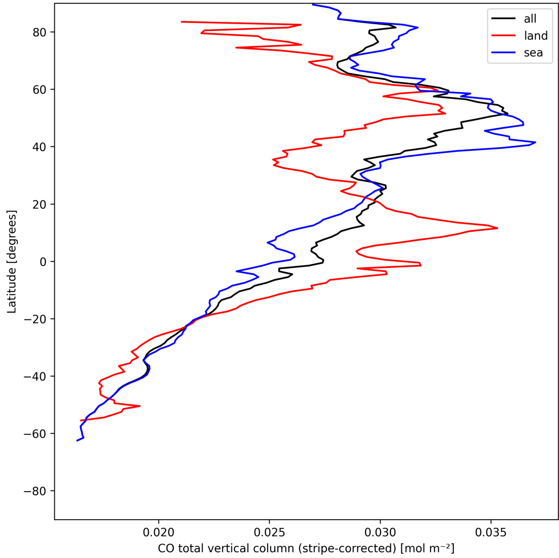
Figure 11: Zonal average of “CO total vertical column (stripe-corrected)” for 2025-05-31 to 2025-06-01.
