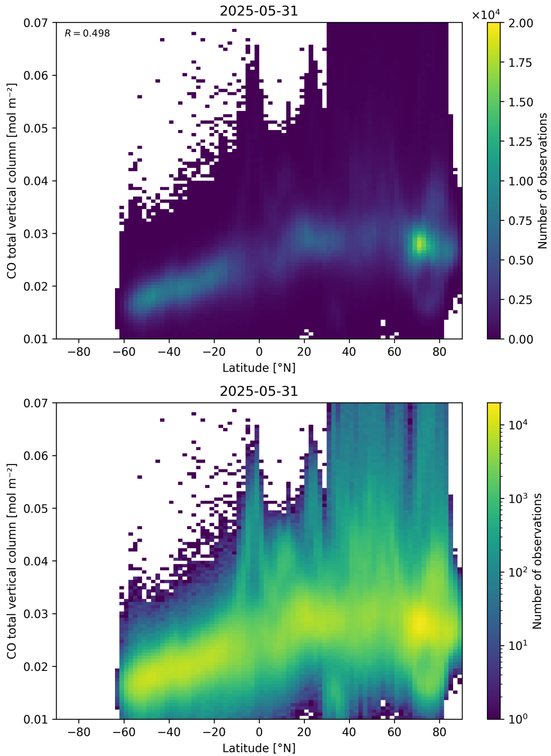
Figure 51: Scatter density plot of “Latitude” against “CO total vertical column” for 2025-05-31 to 2025-06-01.
