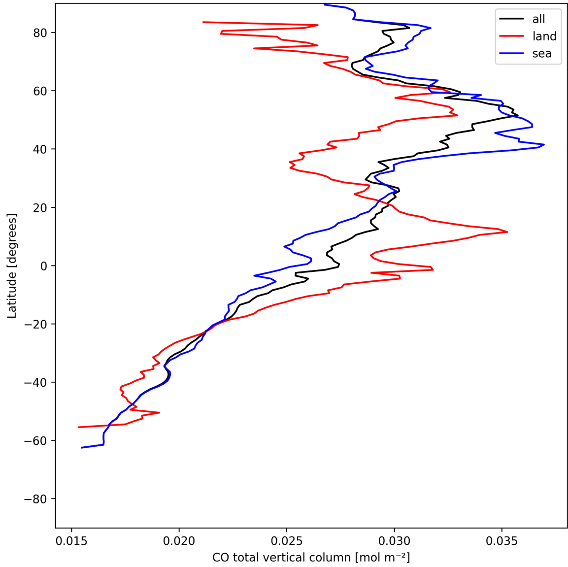
Figure 10: Zonal average of “CO total vertical column” for 2025-05-31 to 2025-06-01.
