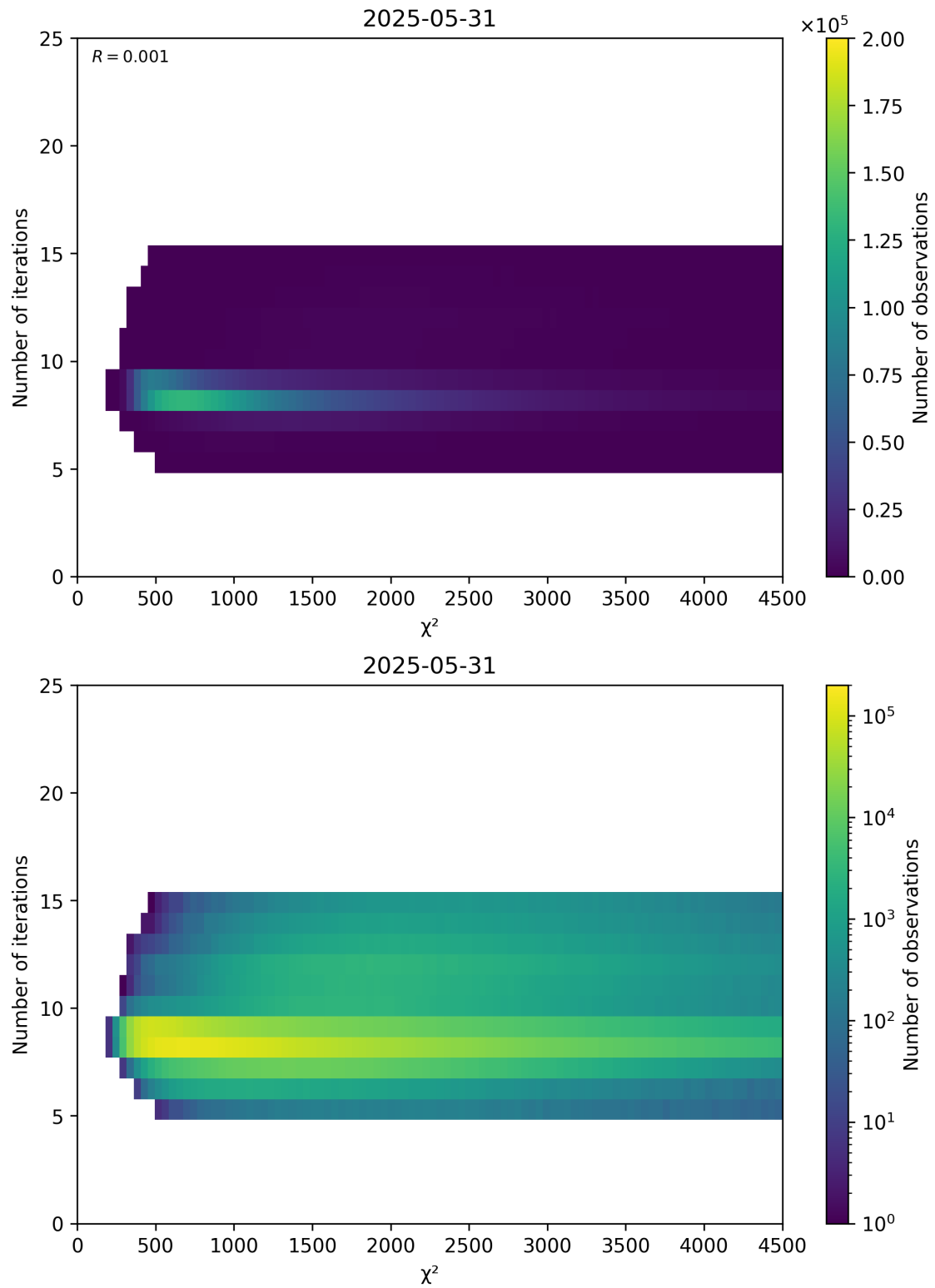
Figure 49: Scatter density plot of “ \chi^2 ” against “Number of iterations” for 2025-05-31 to 2025-06-01.
