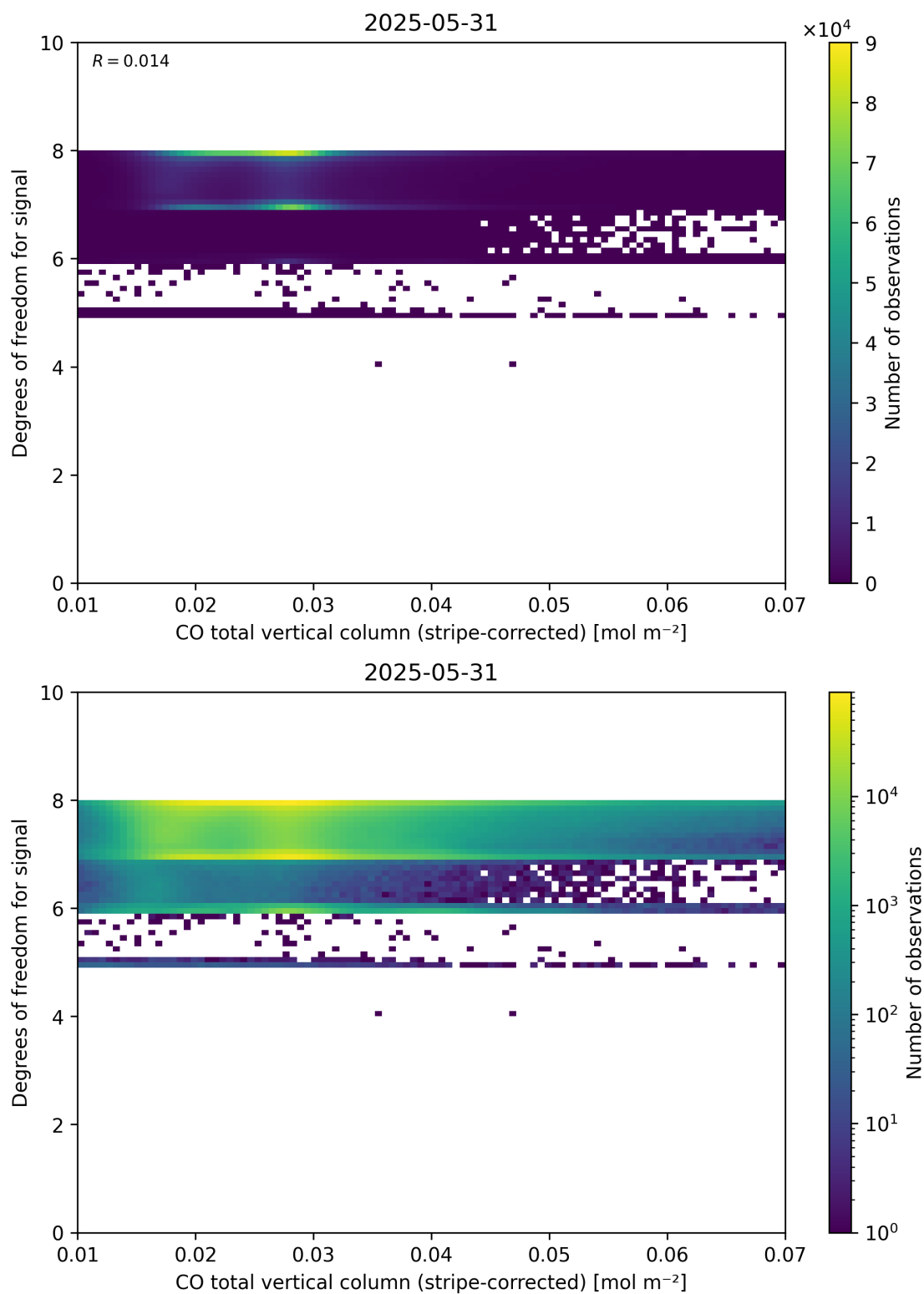
Figure 38: Scatter density plot of “CO total vertical column (stripe-corrected)” against “Degrees of freedom for signal” for 2025-05-31 to 2025-06-01.
