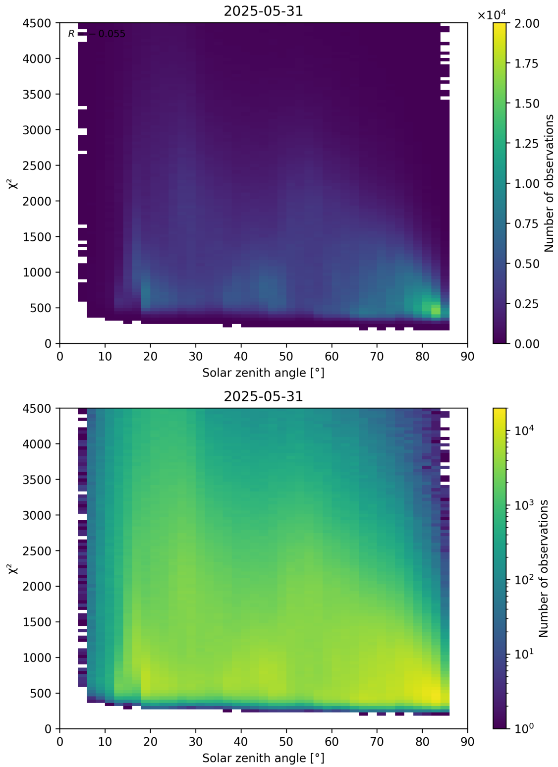
Figure 64: Scatter density plot of “Solar zenith angle” against “ \chi^2 ” for 2025-05-31 to 2025-06-01.
