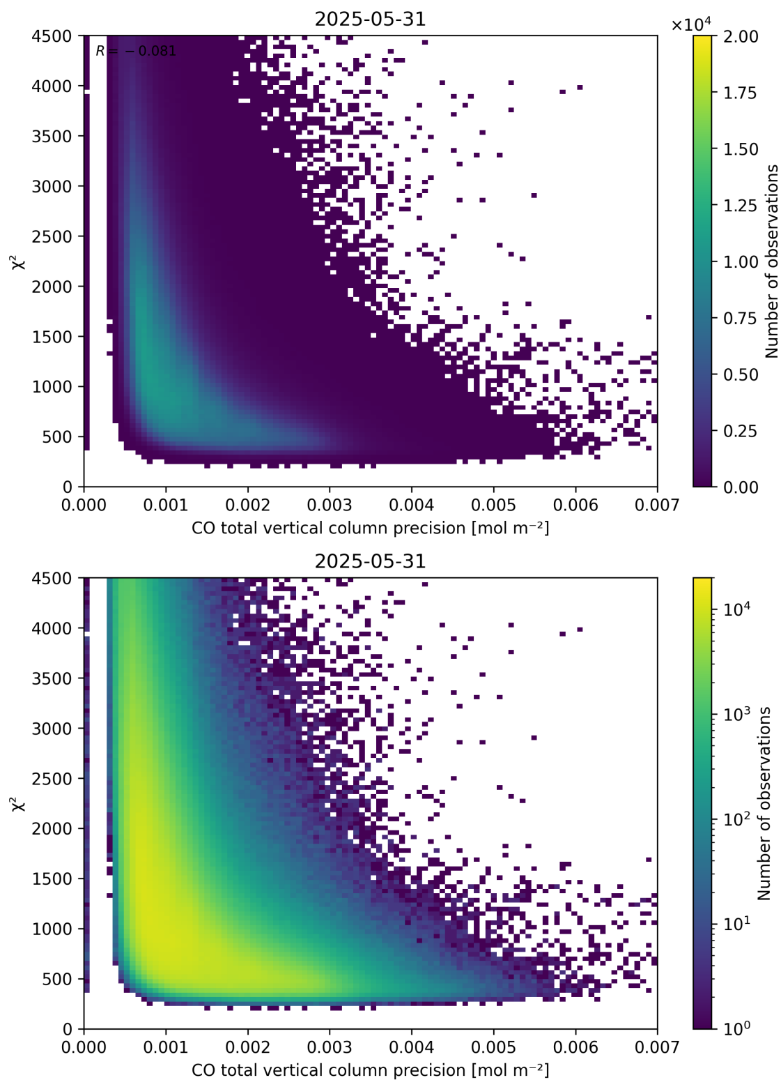
Figure 44: Scatter density plot of “CO total vertical column precision” against “ \chi^2 ” for 2025-05-31 to 2025-06-01.
