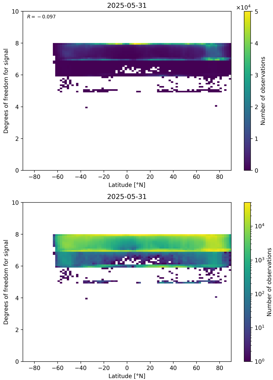
Figure 55: Scatter density plot of “Latitude” against “Degrees of freedom for signal” for 2025-05-31 to 2025-06-01.
