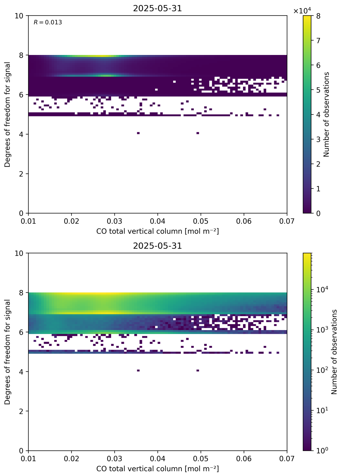
Figure 41: Scatter density plot of “CO total vertical column” against “Degrees of freedom for signal” for 2025-05-31 to 2025-06-01.
