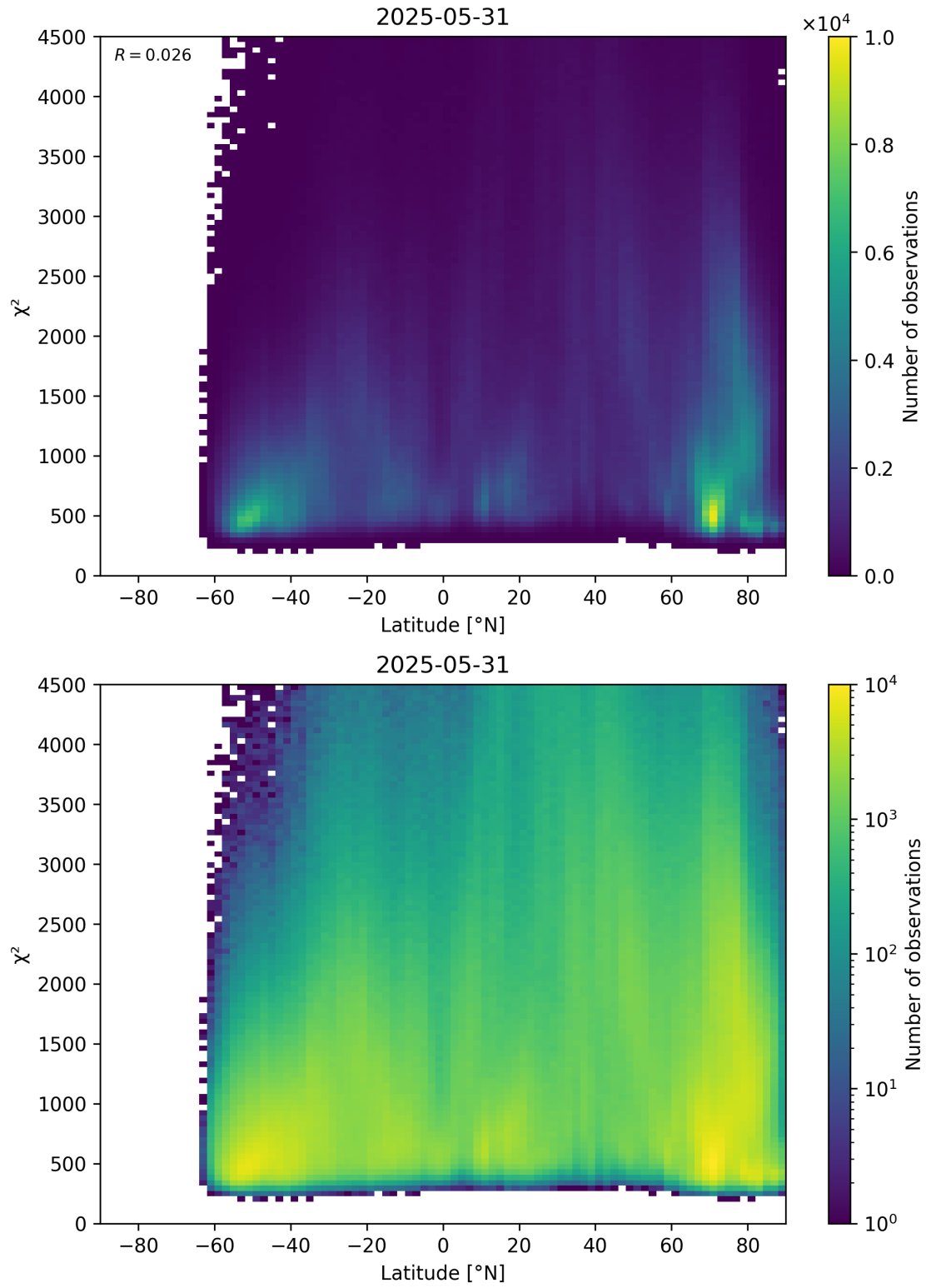
Figure 54: Scatter density plot of “Latitude” against “ \chi^2 ” for 2025-05-31 to 2025-06-01.
