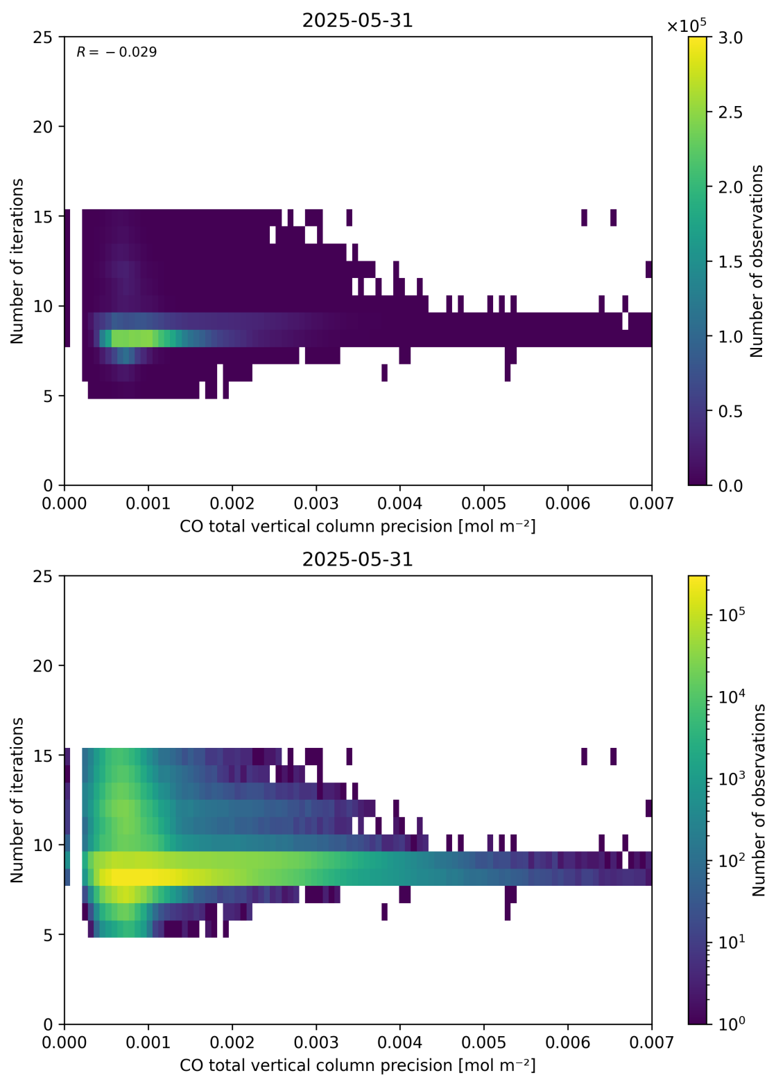
Figure 46: Scatter density plot of “CO total vertical column precision” against “Number of iterations” for 2025-05-31 to 2025-06-01.
