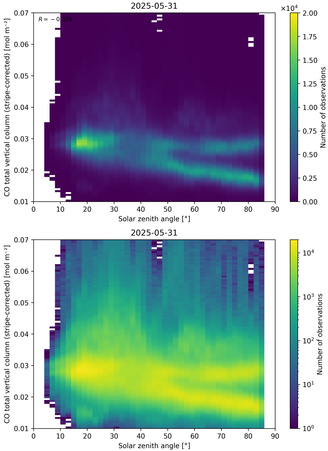
Figure 62: Scatter density plot of “Solar zenith angle” against “CO total vertical column (stripe-corrected)” for 2025-05-31 to 2025-06-01.
