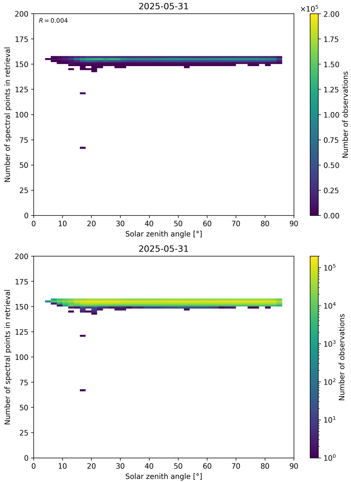
Figure 68: Scatter density plot of “Solar zenith angle” against “Number of spectral points in retrieval” for 2025-05-31 to 2025-06-01.
