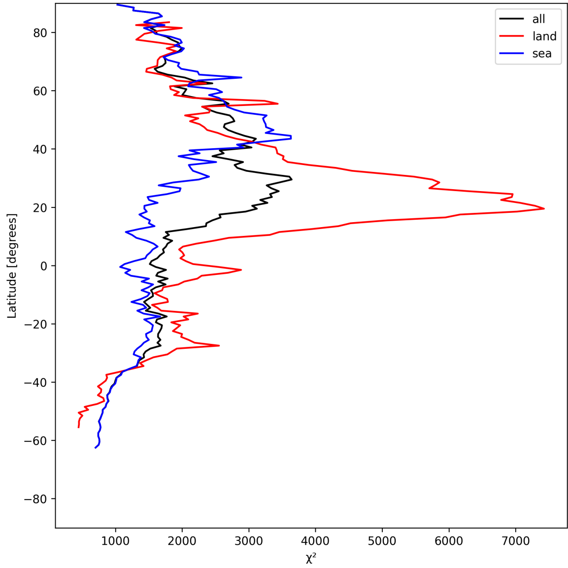
Figure 14: Zonal average of “ \chi^2 ” for 2025-05-31 to 2025-06-01.
