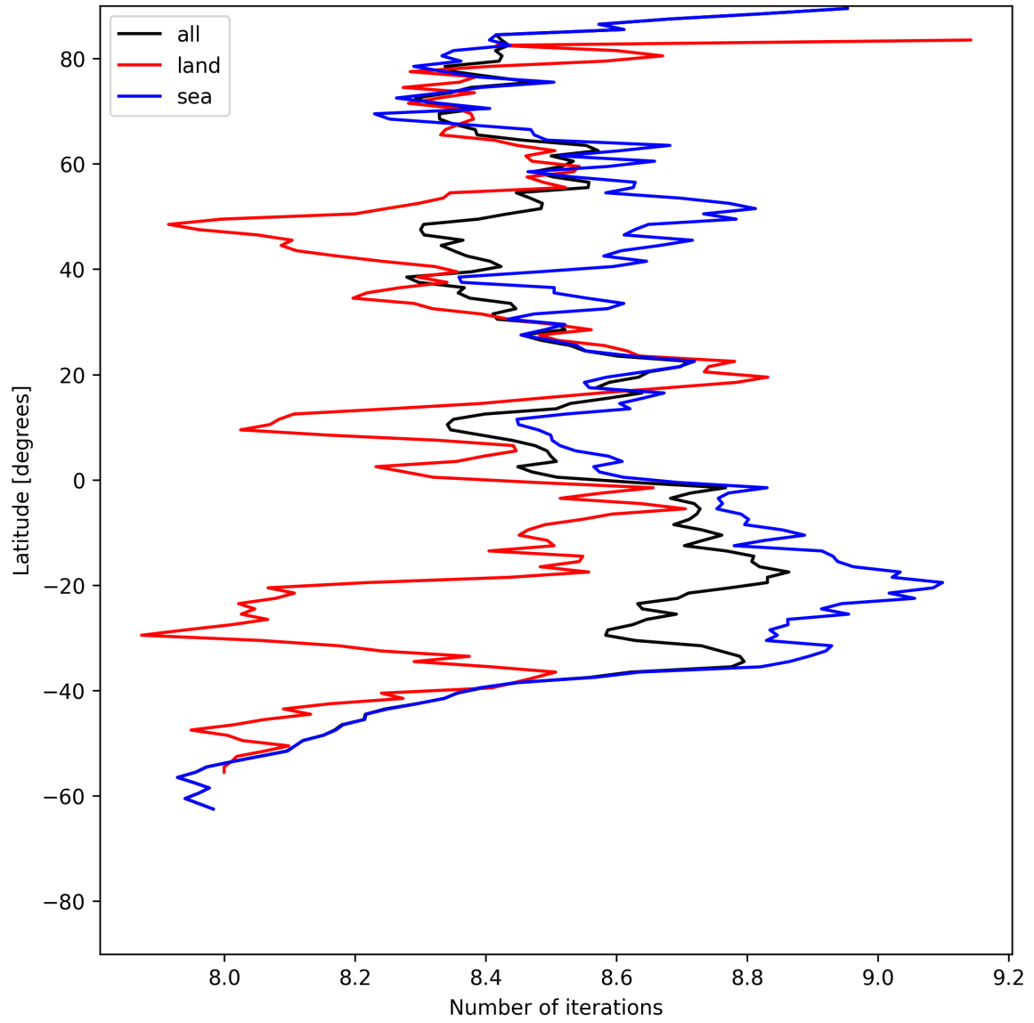
Figure 16: Zonal average of “Number of iterations” for 2025-05-31 to 2025-06-01.
