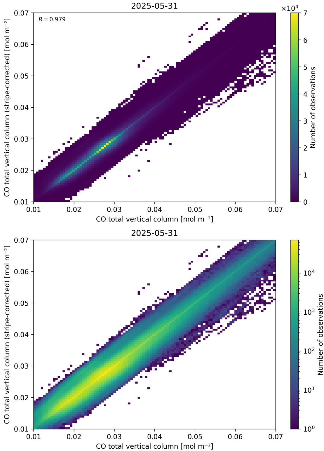
Figure 33: Scatter density plot of “CO total vertical column” against “CO total vertical column (stripe-corrected)” for 2025-05-31 to 2025-06-01.
