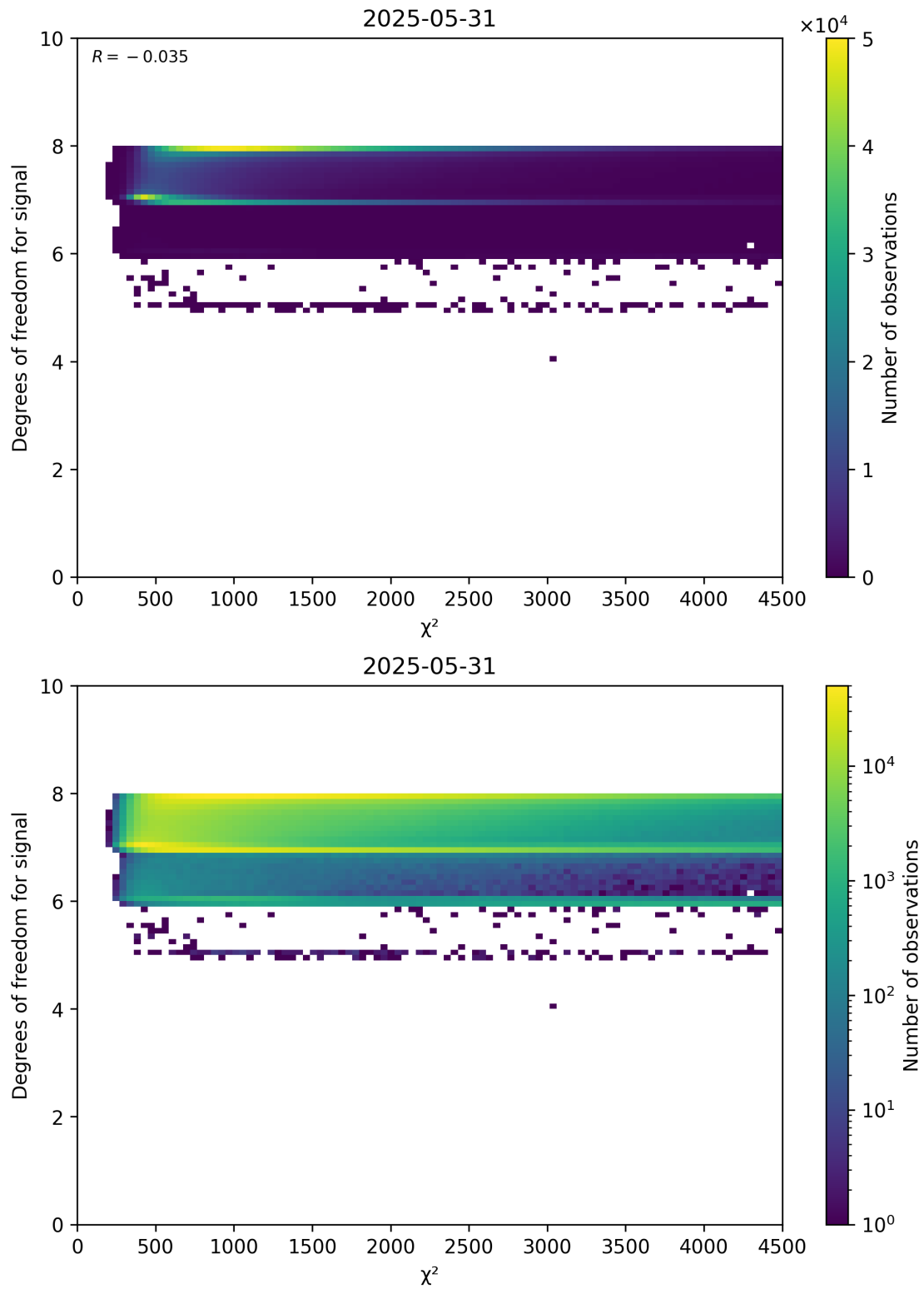
Figure 48: Scatter density plot of “ \chi^2 ” against “Degrees of freedom for signal” for 2025-05-31 to 2025-06-01.
