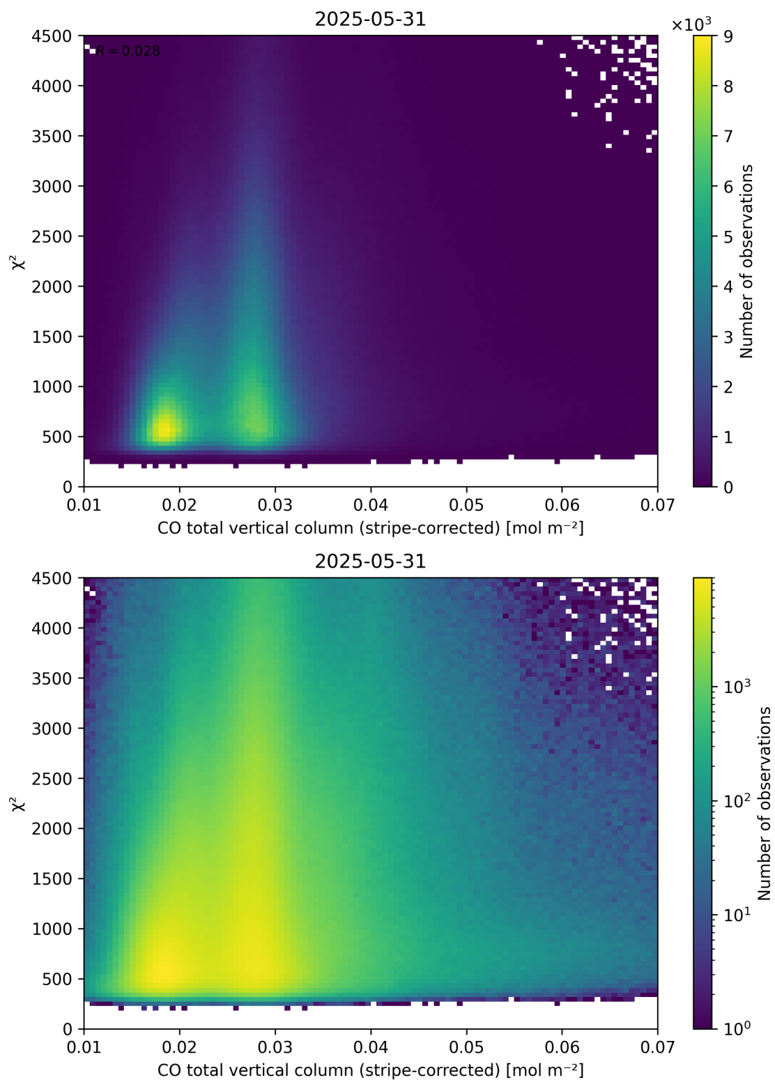
Figure 37: Scatter density plot of “CO total vertical column (stripe-corrected)” against “ \chi^2 ” for 2025-05-31 to 2025-06-01.
