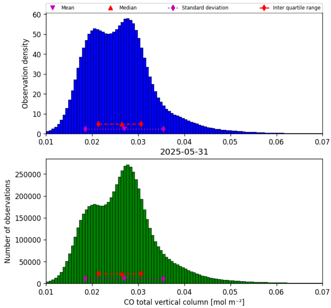
Figure 18: Histogram of “CO total vertical column” for 2025-05-31 to 2025-06-01
