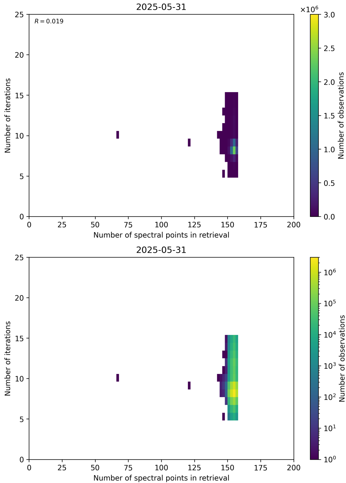
Figure 60: Scatter density plot of “Number of spectral points in retrieval” against “Number of iterations” for 2025-05-31 to 2025-06-01.
