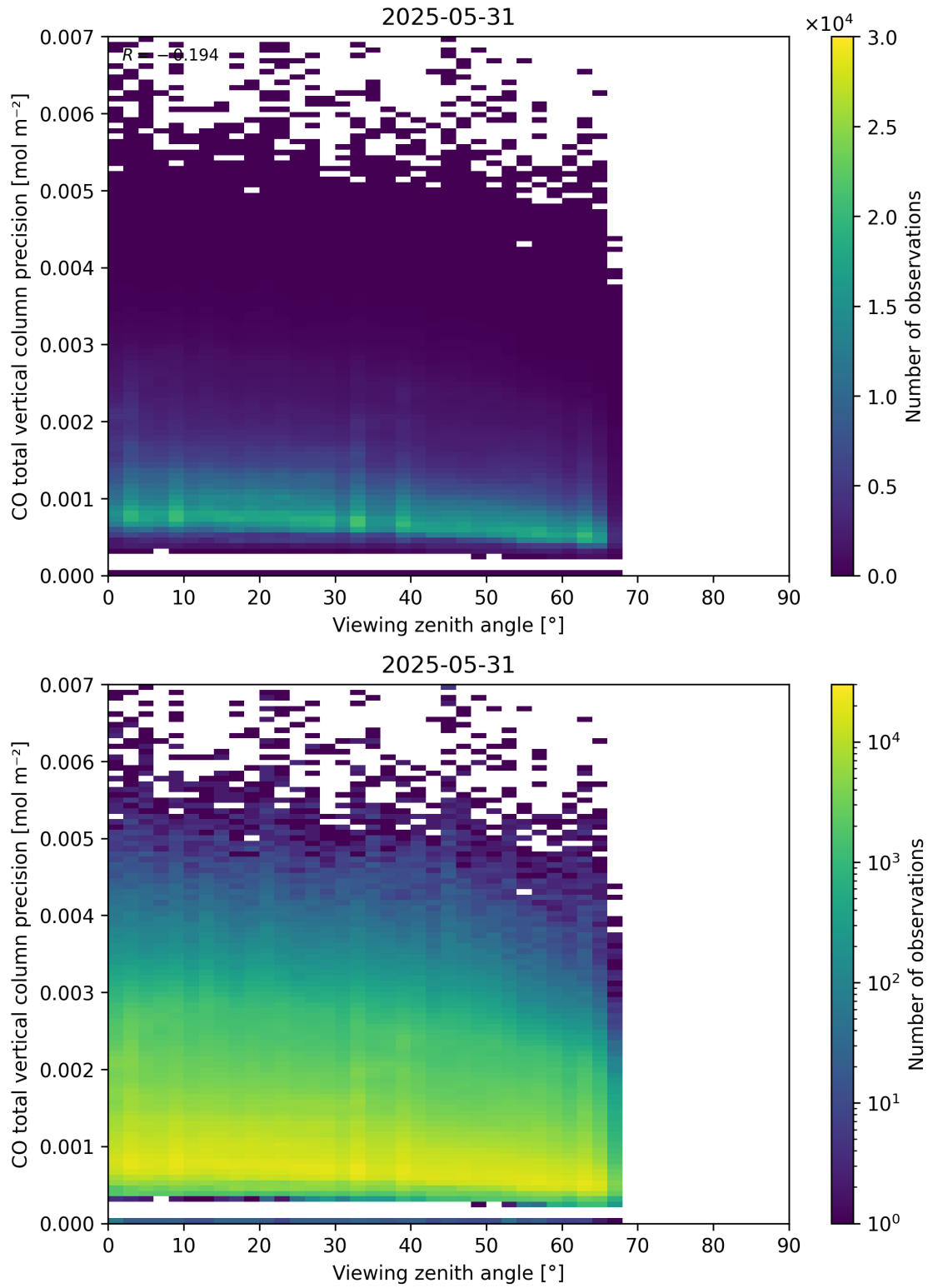
Figure 71: Scatter density plot of “Viewing zenith angle” against “CO total vertical column precision” for 2025-05-31 to 2025-06-01.
