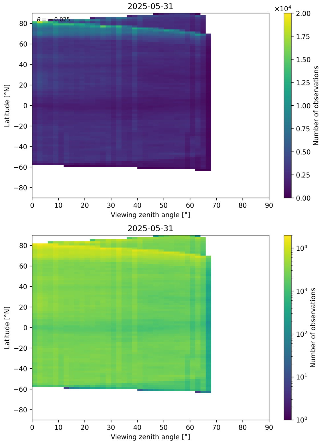
Figure 74: Scatter density plot of “Viewing zenith angle” against “Latitude” for 2025-05-31 to 2025-06-01.
