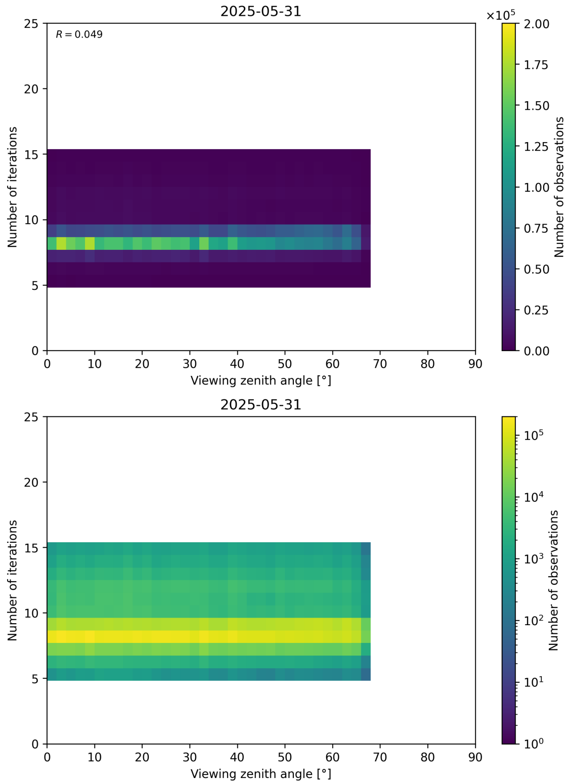
Figure 75: Scatter density plot of “Viewing zenith angle” against “Number of iterations” for 2025-05-31 to 2025-06-01.
