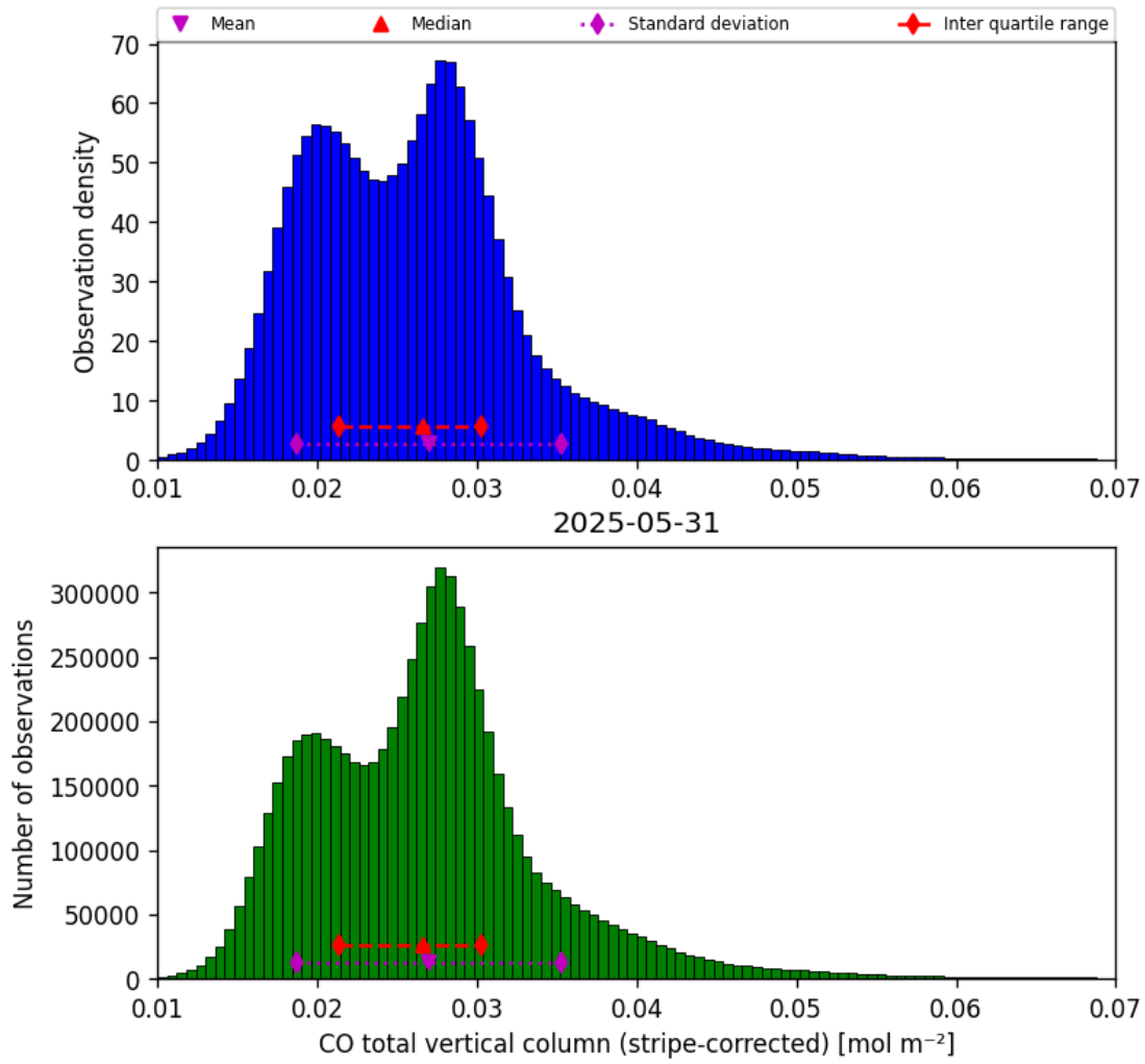
Figure 19: Histogram of “CO total vertical column (stripe-corrected)” for 2025-05-31 to 2025-06-01
