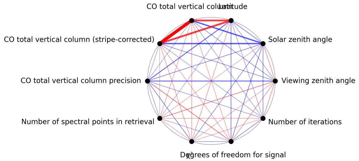
Figure 1: Map of correlation graph for 2025-05-31 to 2025-06-01.
