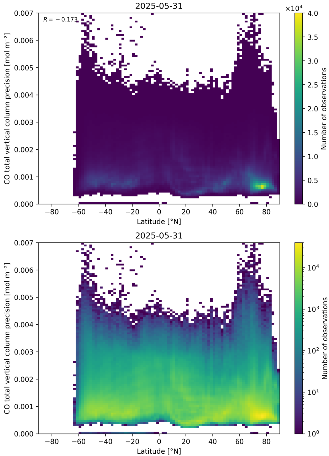
Figure 53: Scatter density plot of “Latitude” against “CO total vertical column precision” for 2025-05-31 to 2025-06-01.
