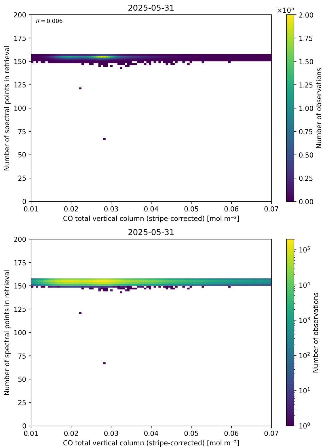
Figure 40: Scatter density plot of “CO total vertical column (stripe-corrected)” against “Number of spectral points in retrieval” for 2025-05-31 to 2025-06-01.
