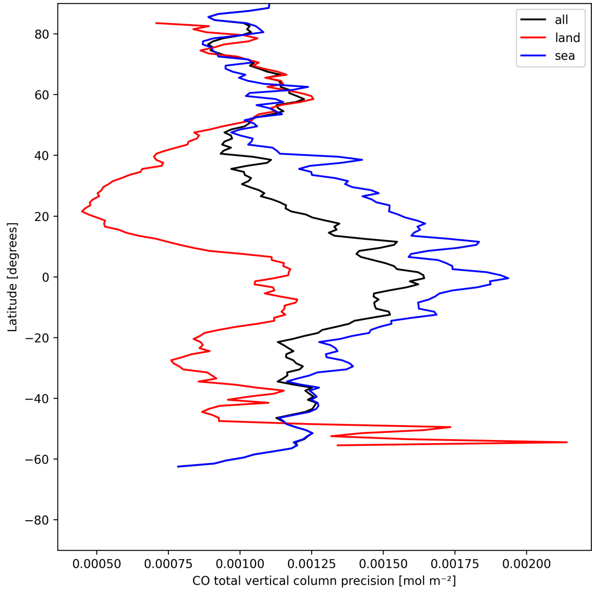
Figure 12: Zonal average of “CO total vertical column precision” for 2025-05-31 to 2025-06-01.
