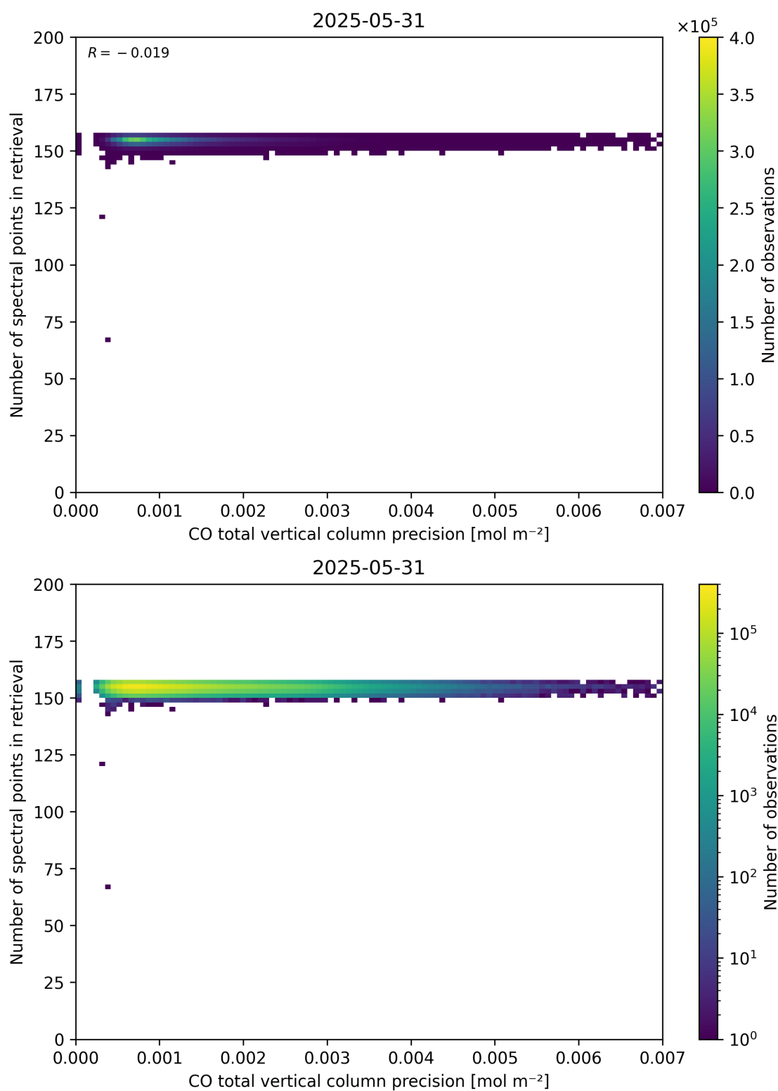
Figure 47: Scatter density plot of “CO total vertical column precision” against “Number of spectral points in retrieval” for 2025-05-31 to 2025-06-01.
