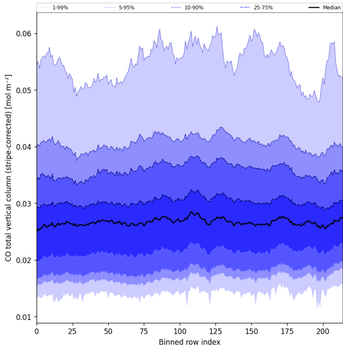
Figure 27: Along track statistics of “CO total vertical column (stripe-corrected)” for 2025-05-31 to 2025-06-01
