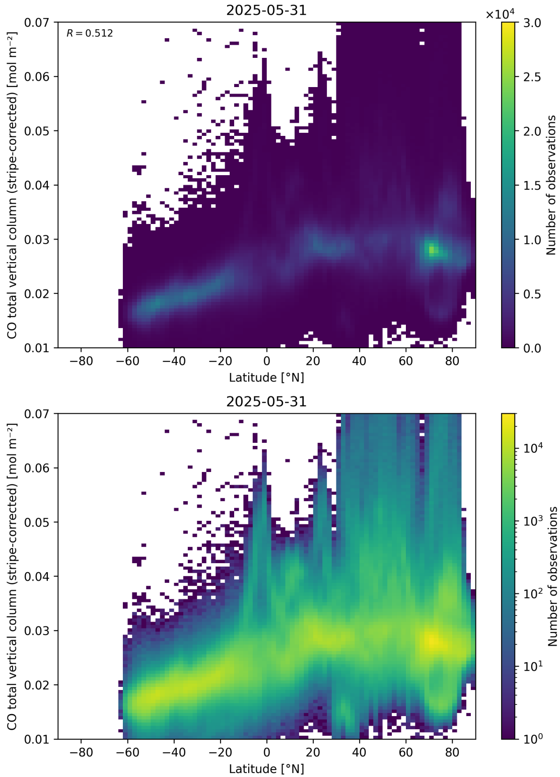
Figure 52: Scatter density plot of “Latitude” against “CO total vertical column (stripe-corrected)” for 2025-05-31 to 2025-06-01.
