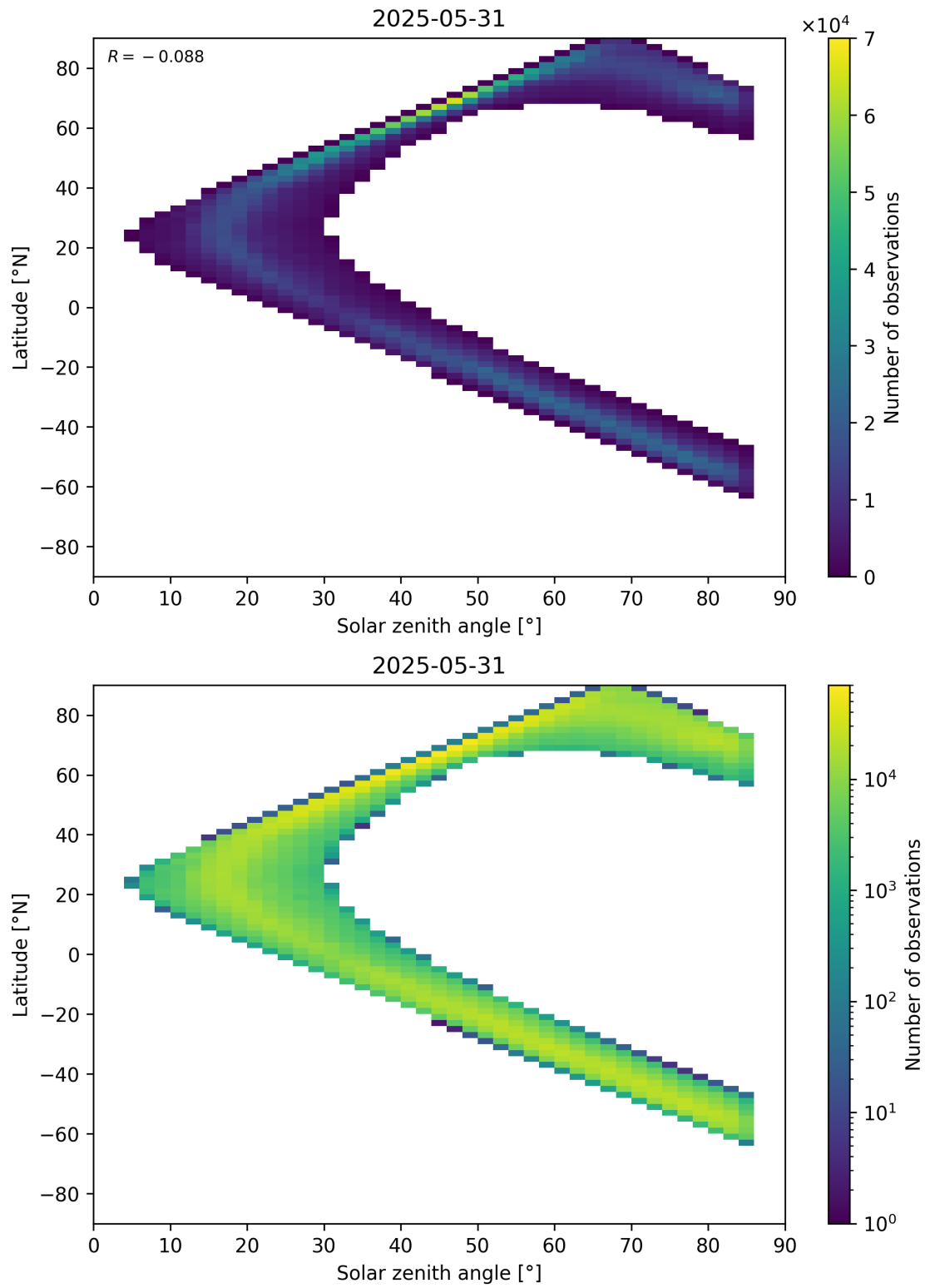
Figure 66: Scatter density plot of “Solar zenith angle” against “Latitude” for 2025-05-31 to 2025-06-01.
