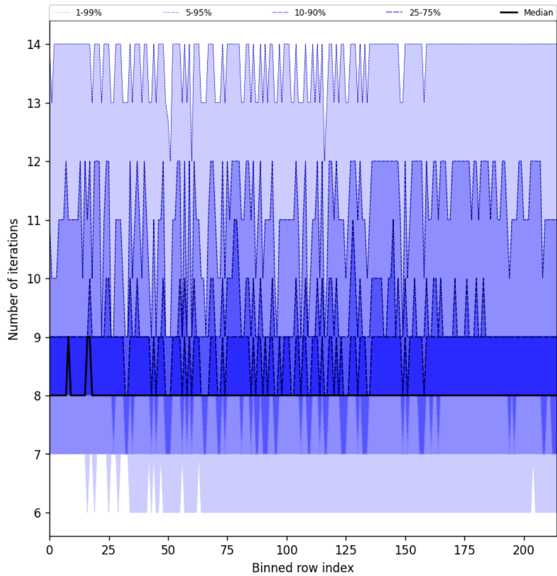
Figure 32: Along track statistics of “Number of iterations” for 2025-05-31 to 2025-06-01
