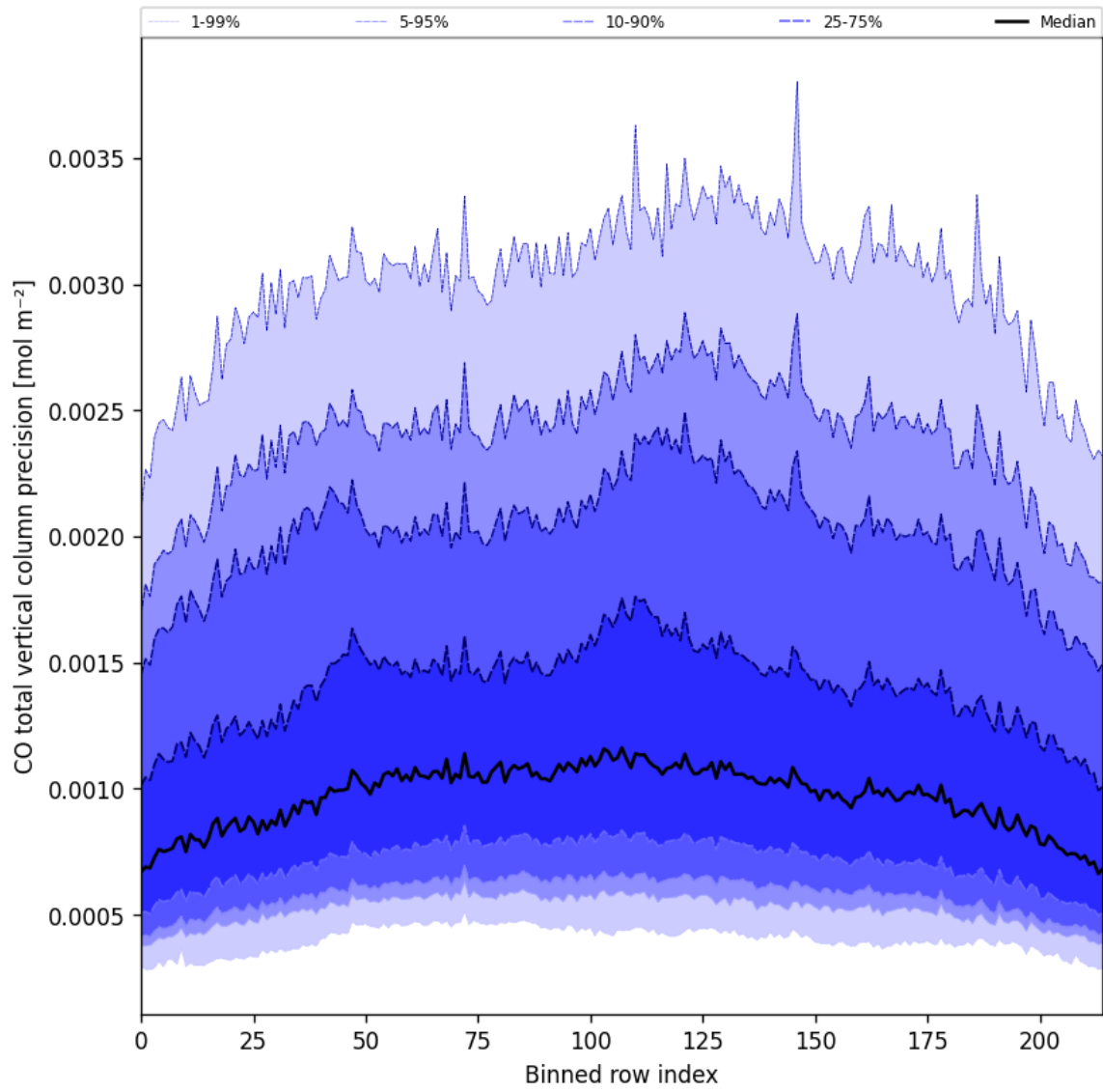
Figure 28: Along track statistics of “CO total vertical column precision” for 2025-05-31 to 2025-06-01
