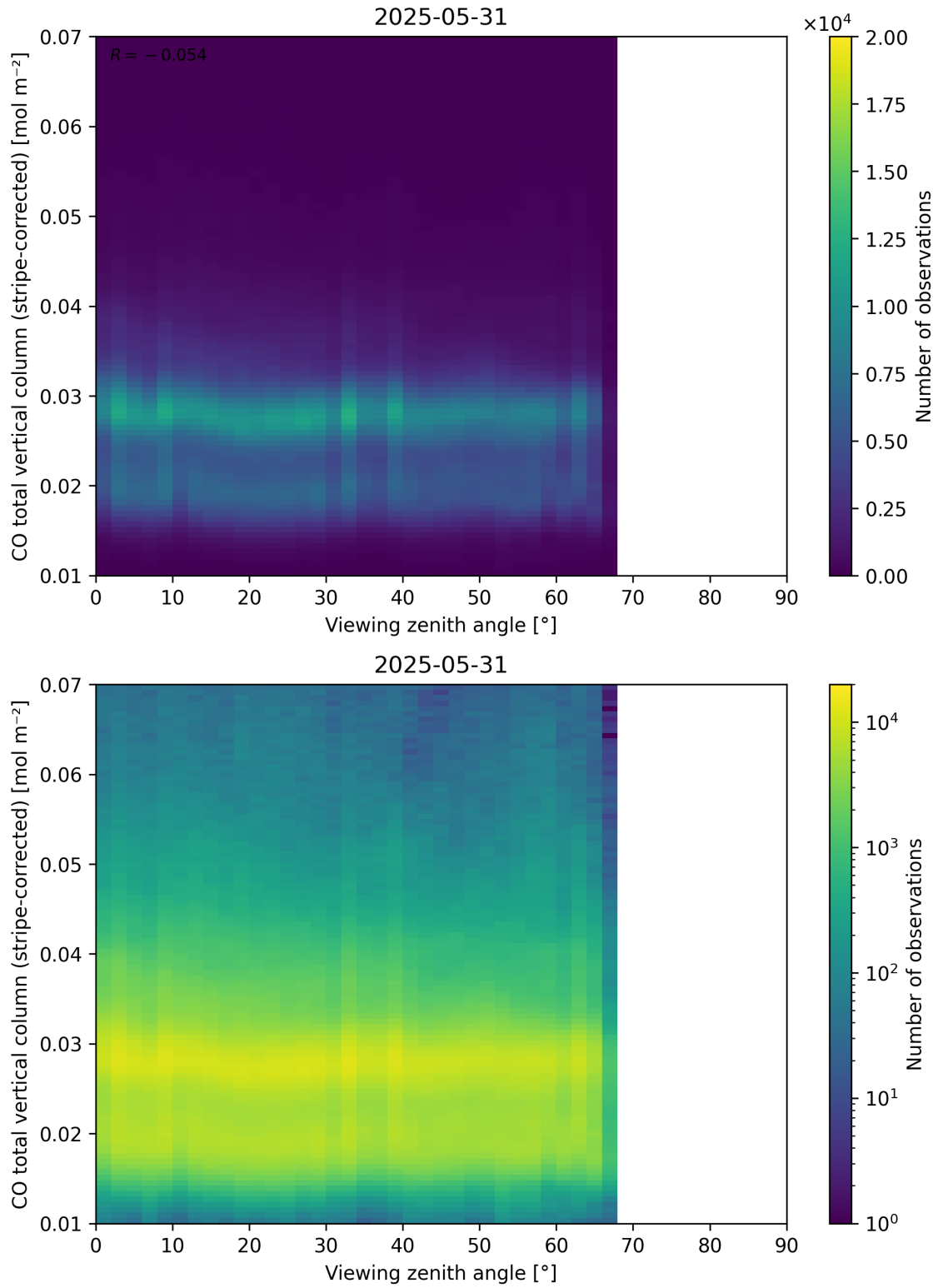
Figure 70: Scatter density plot of “Viewing zenith angle” against “CO total vertical column (stripe-corrected)” for 2025-05-31 to 2025-06-01.
