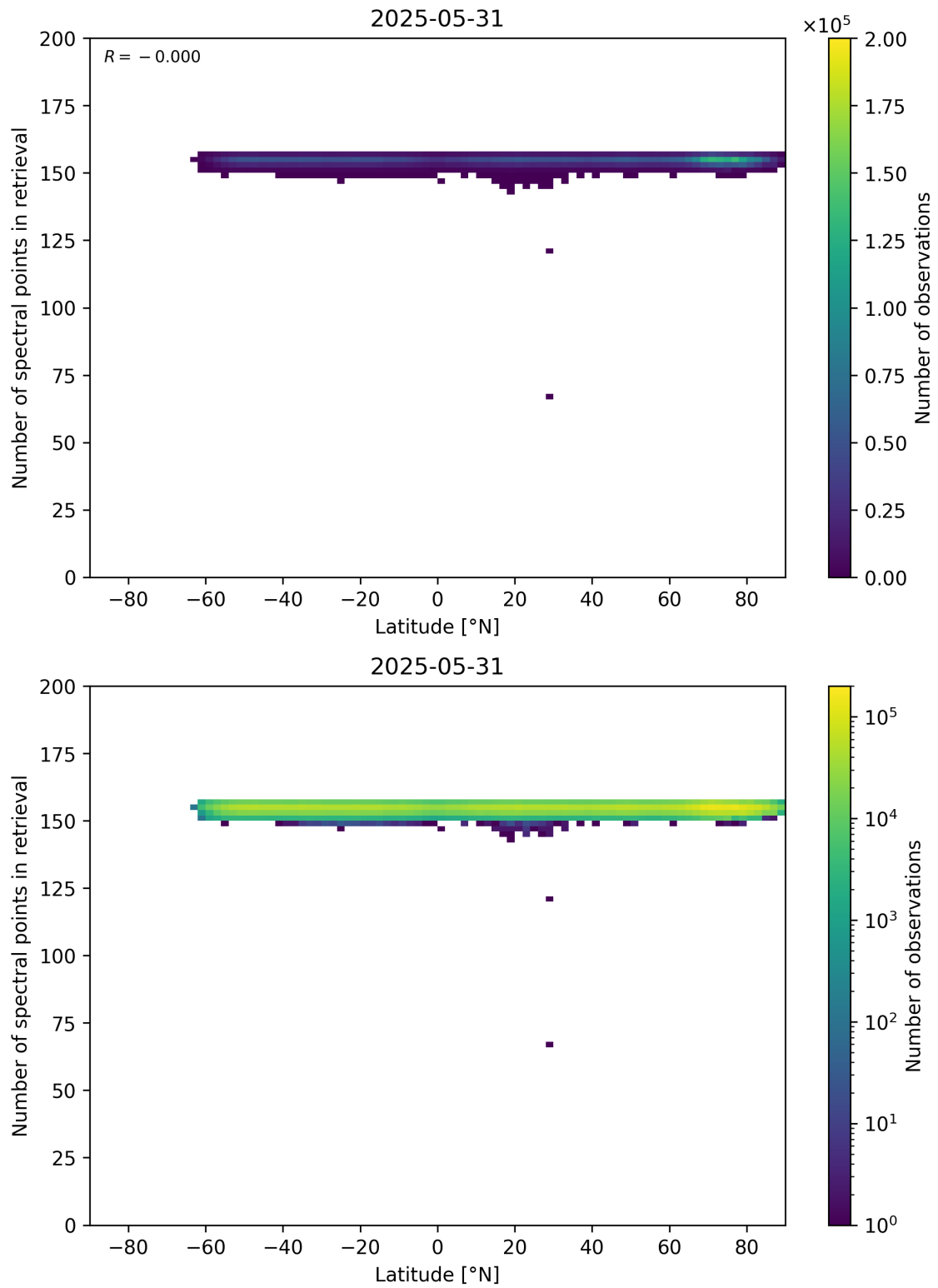
Figure 57: Scatter density plot of “Latitude” against “Number of spectral points in retrieval” for 2025-05-31 to 2025-06-01.
