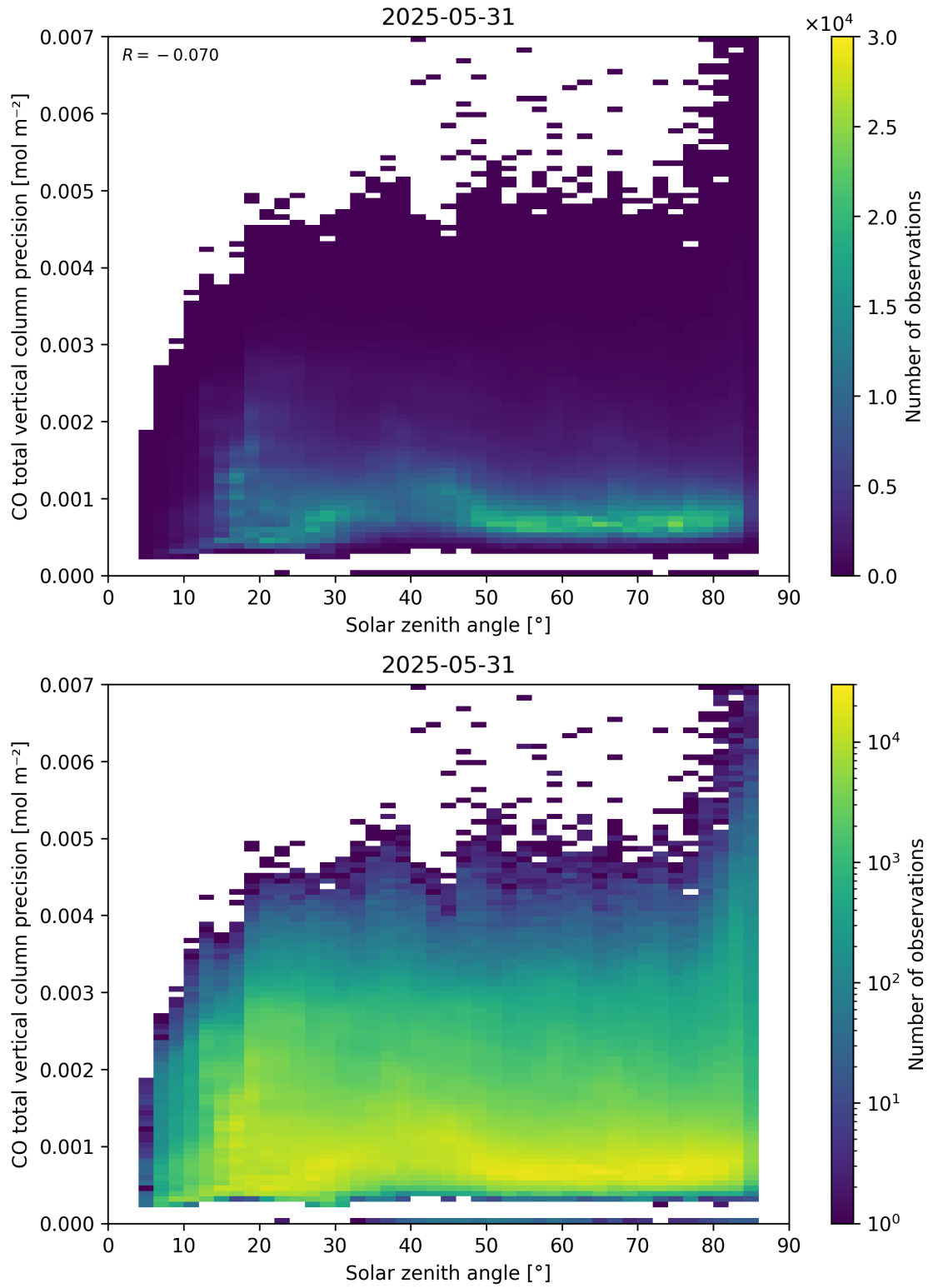
Figure 63: Scatter density plot of “Solar zenith angle” against “CO total vertical column precision” for 2025-05-31 to 2025-06-01.
