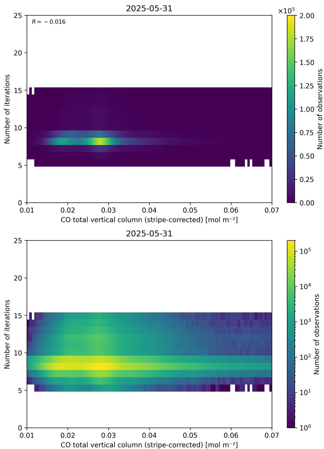
Figure 39: Scatter density plot of “CO total vertical column (stripe-corrected)” against “Number of iterations” for 2025-05-31 to 2025-06-01.
