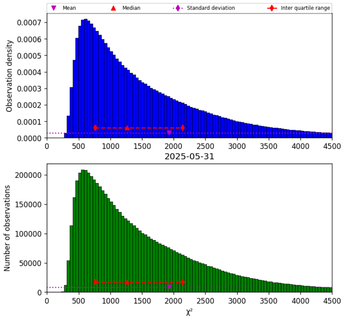
Figure 22: Histogram of " \chi^2 " for 2025-05-31 to 2025-06-01
