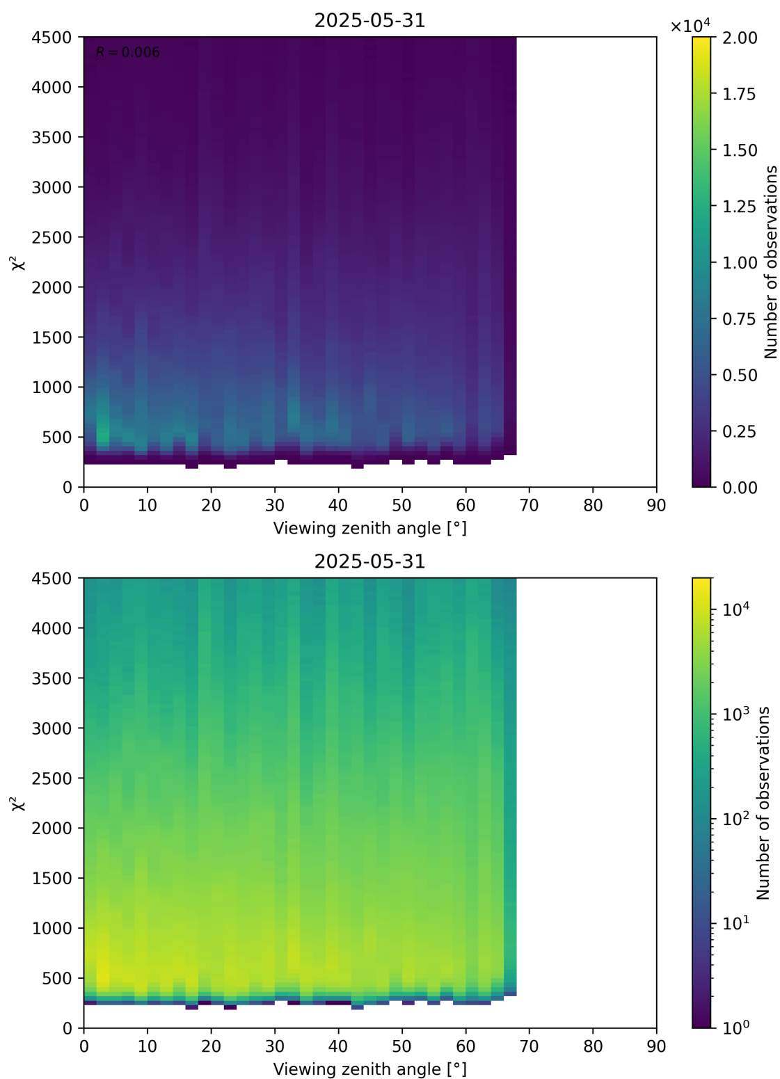
Figure 72: Scatter density plot of “Viewing zenith angle” against “ \chi^2 ” for 2025-05-31 to 2025-06-01.
