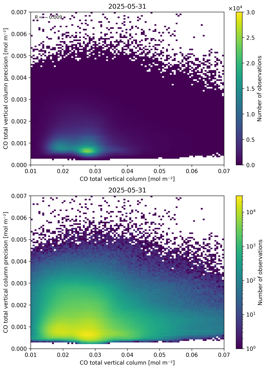
Figure 34: Scatter density plot of “CO total vertical column” against “CO total vertical column precision” for 2025-05-31 to 2025-06-01.
