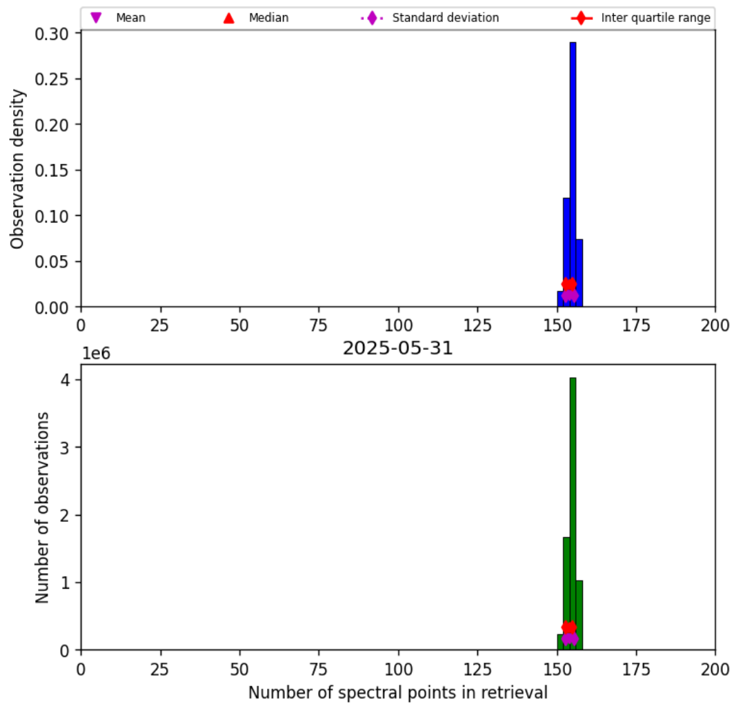
Figure 21: Histogram of “Number of spectral points in retrieval” for 2025-05-31 to 2025-06-01
