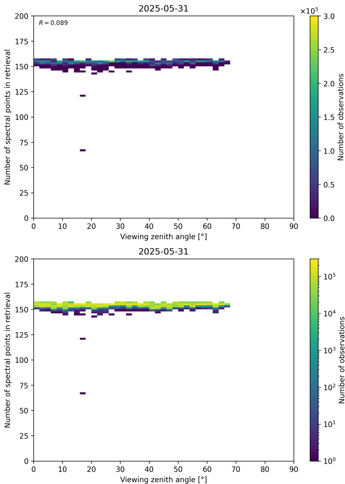
Figure 76: Scatter density plot of “Viewing zenith angle” against “Number of spectral points in retrieval” for 2025-05-31 to 2025-06-01.
