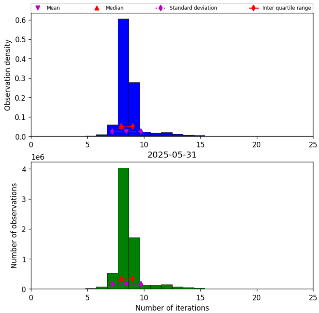
Figure 24: Histogram of “Number of iterations” for 2025-05-31 to 2025-06-01
