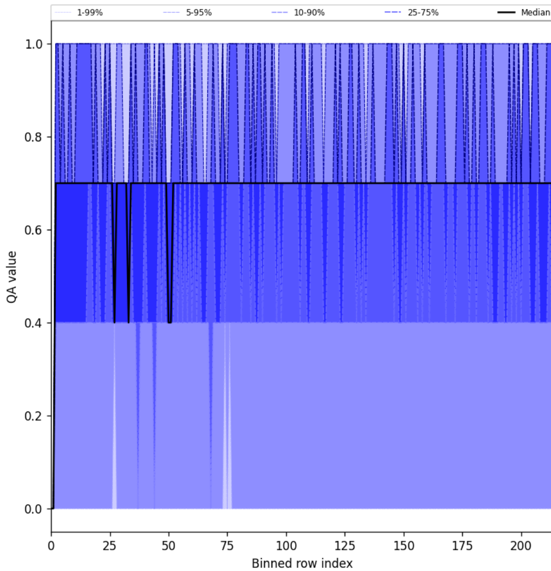
Figure 25: Along track statistics of “QA value” for 2025-05-31 to 2025-06-01
