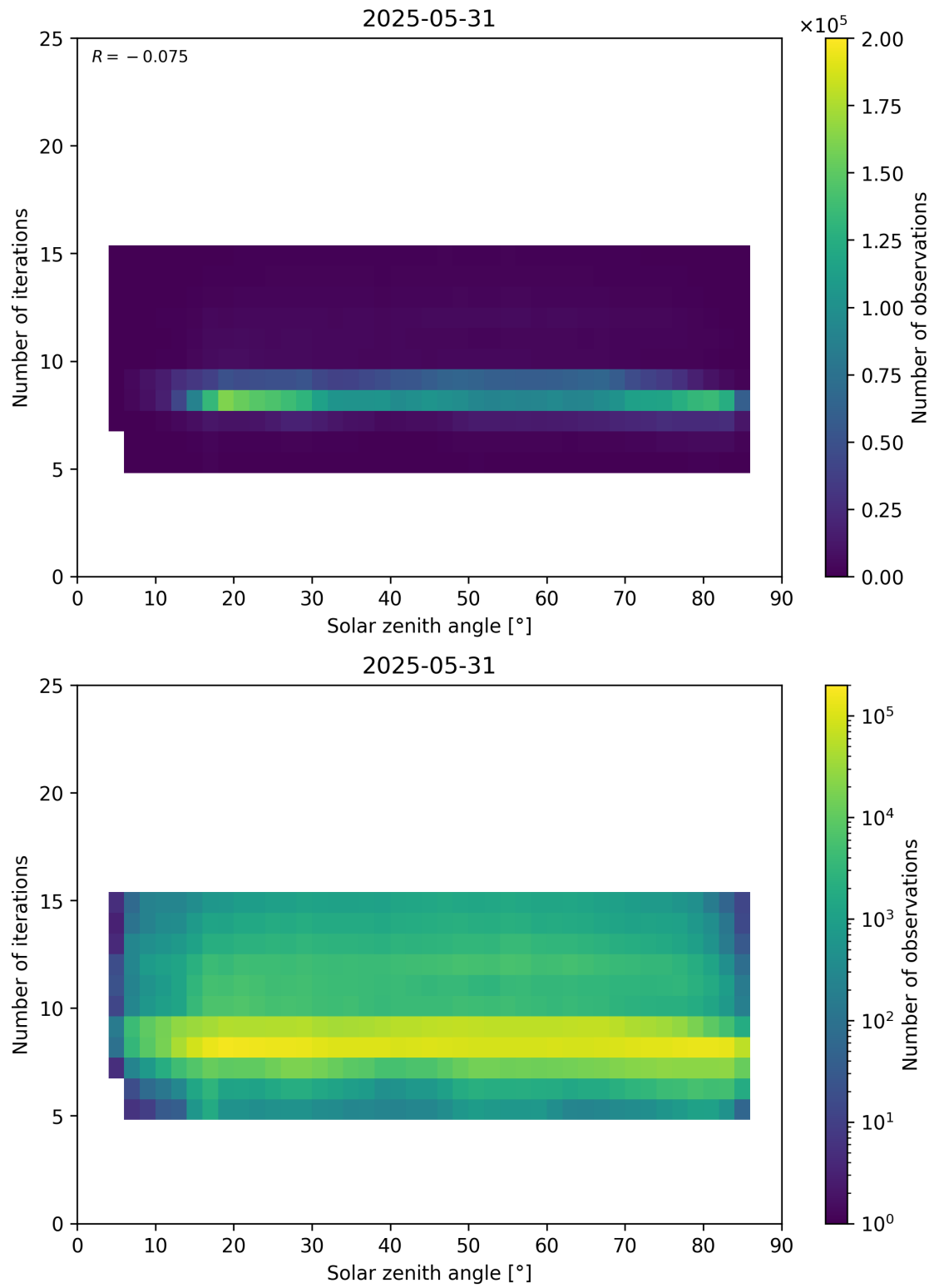
Figure 67: Scatter density plot of “Solar zenith angle” against “Number of iterations” for 2025-05-31 to 2025-06-01.
