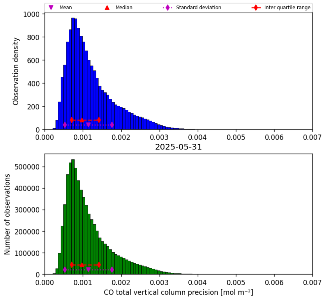
Figure 20: Histogram of “CO total vertical column precision” for 2025-05-31 to 2025-06-01
