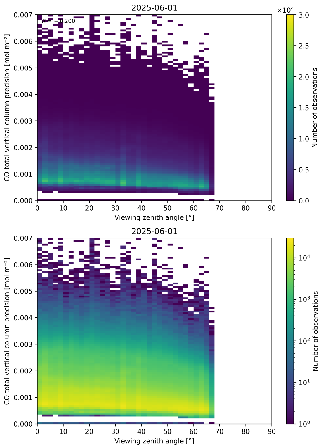
Figure 71: Scatter density plot of “Viewing zenith angle” against “CO total vertical column precision” for 2025-06-01 to 2025-06-02.
