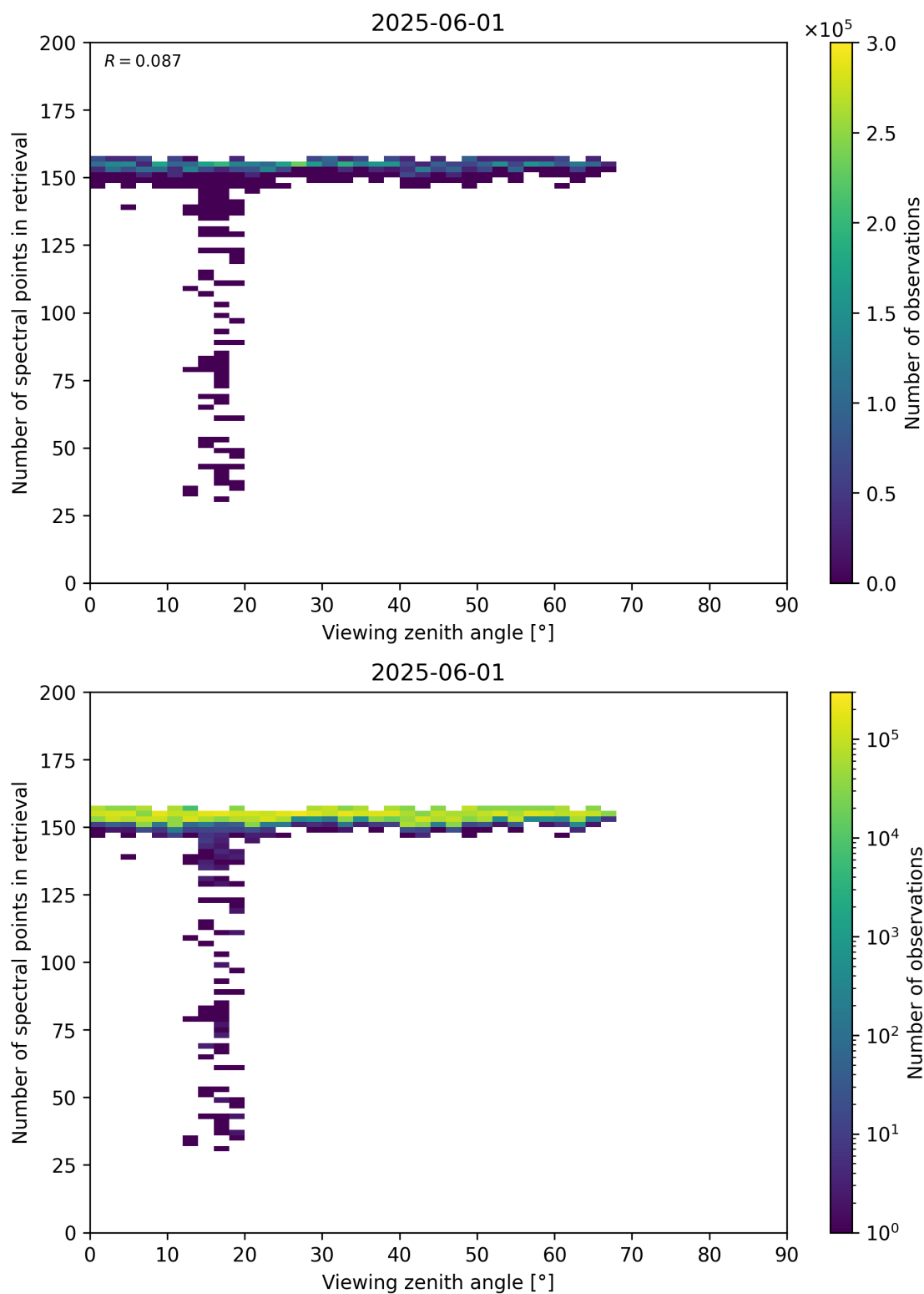
Figure 76: Scatter density plot of “Viewing zenith angle” against “Number of spectral points in retrieval” for 2025-06-01 to 2025-06-02.
