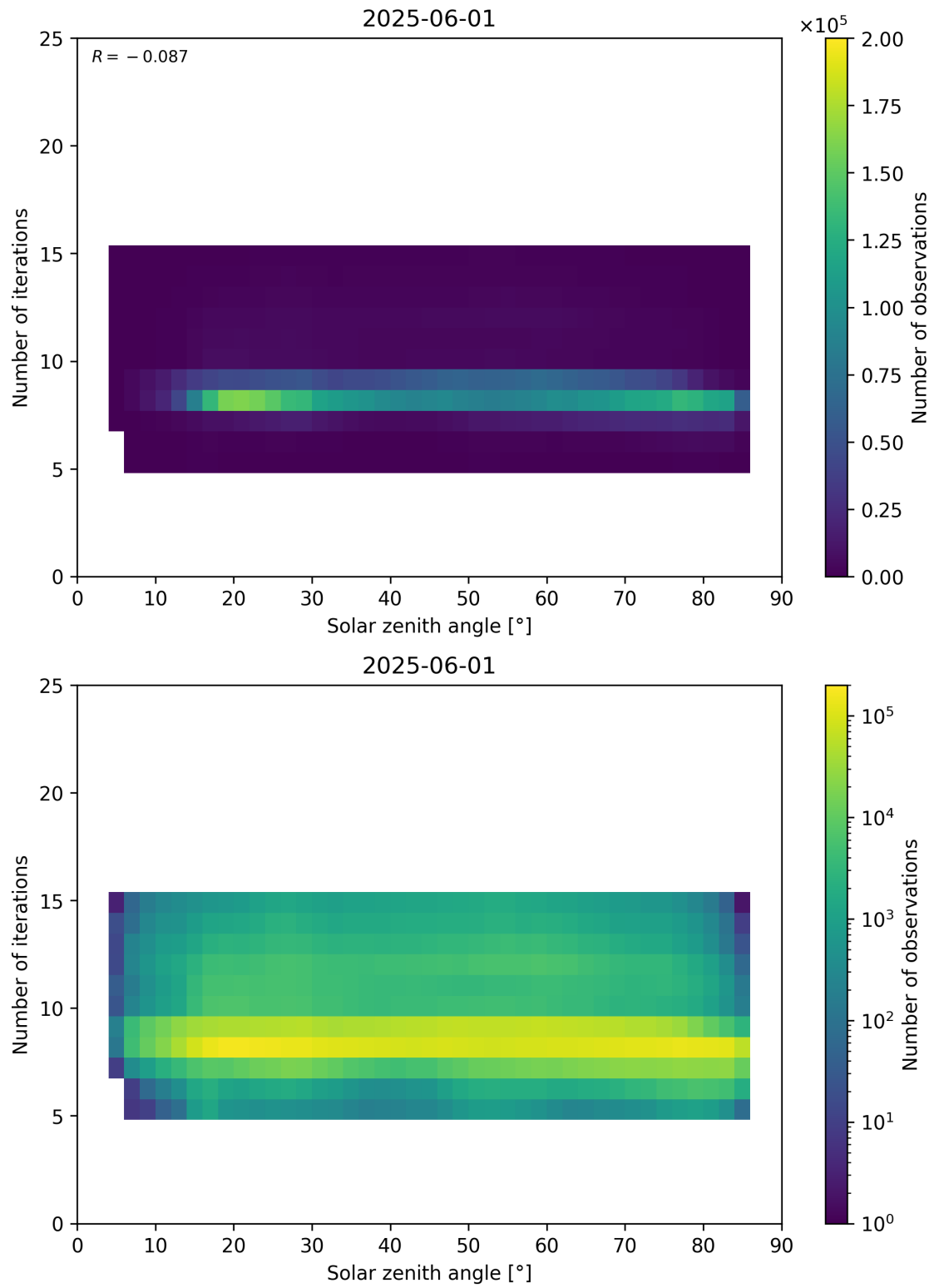
Figure 67: Scatter density plot of “Solar zenith angle” against “Number of iterations” for 2025-06-01 to 2025-06-02.
