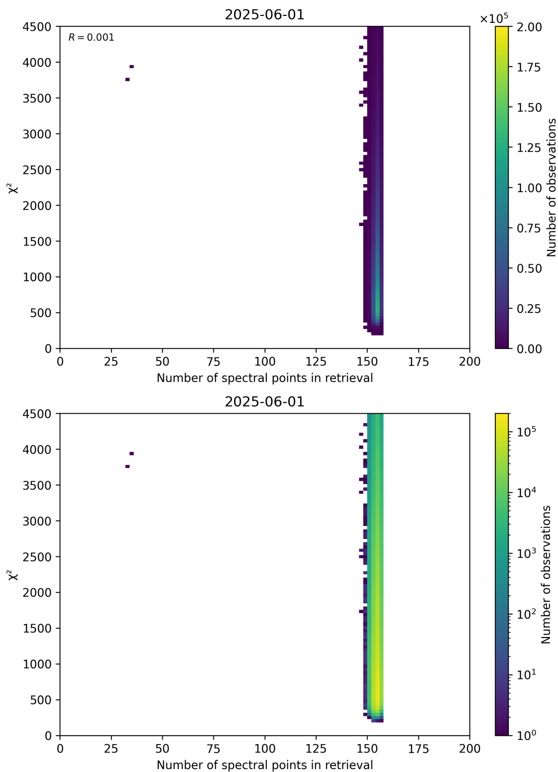
Figure 58: Scatter density plot of “Number of spectral points in retrieval” against “ \chi^2 ” for 2025-06-01 to 2025-06-02.
