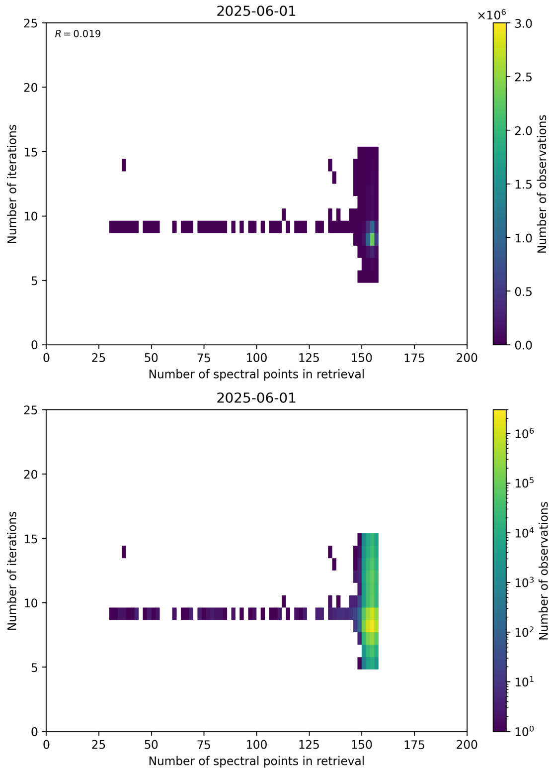
Figure 60: Scatter density plot of “Number of spectral points in retrieval” against “Number of iterations” for 2025-06-01 to 2025-06-02.
