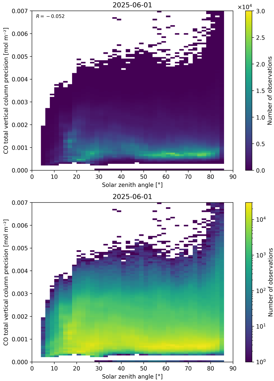
Figure 63: Scatter density plot of “Solar zenith angle” against “CO total vertical column precision” for 2025-06-01 to 2025-06-02.
