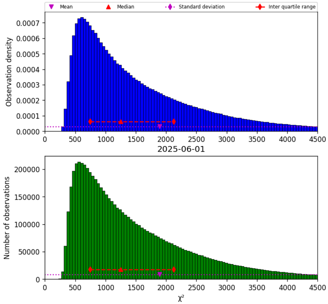
Figure 22: Histogram of “ \chi^2 ” for 2025-06-01 to 2025-06-02
