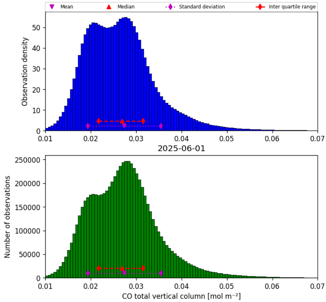
Figure 18: Histogram of “CO total vertical column” for 2025-06-01 to 2025-06-02
