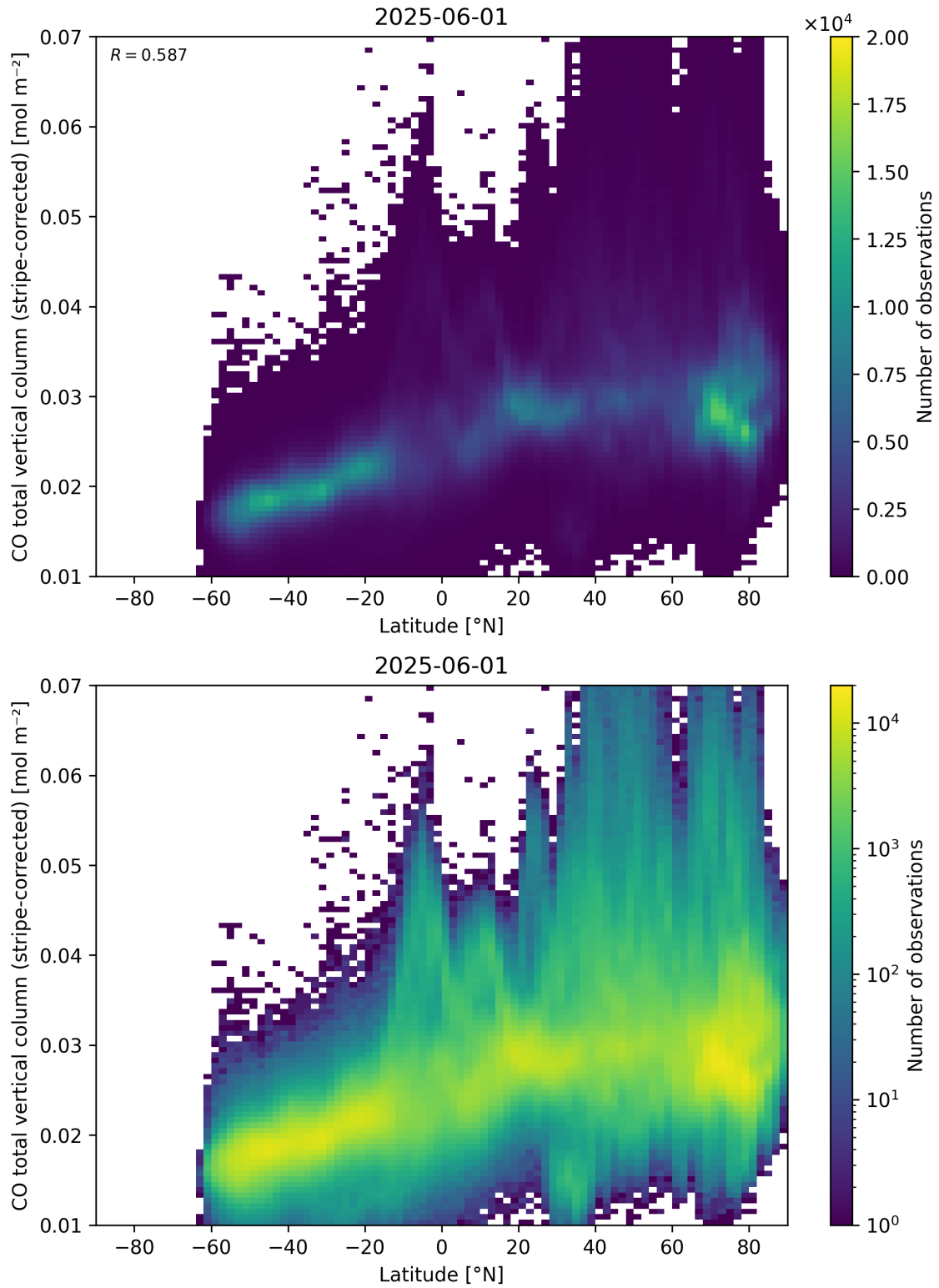
Figure 52: Scatter density plot of “Latitude” against “CO total vertical column (stripe-corrected)” for 2025-06-01 to 2025-06-02.
