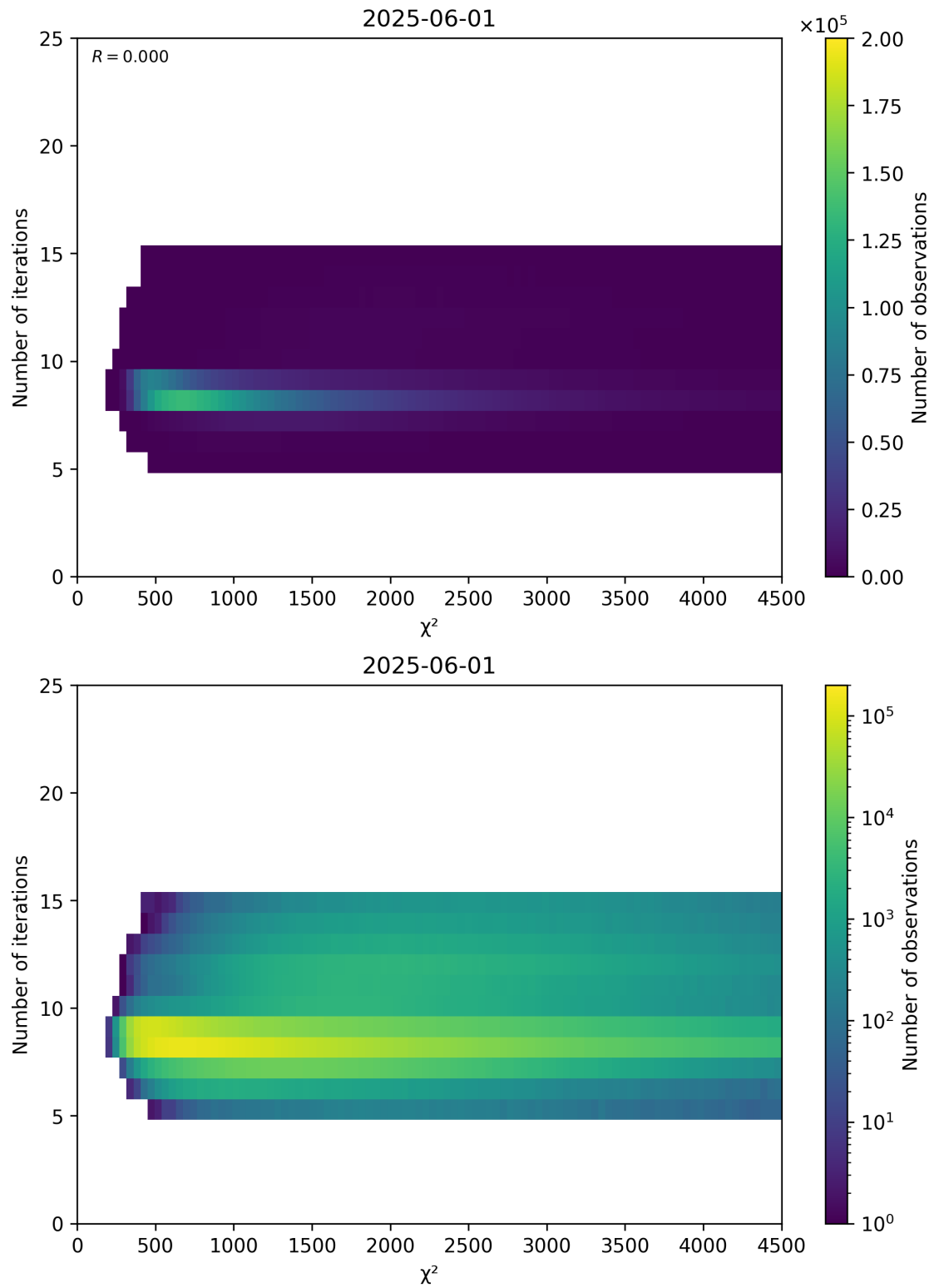
Figure 49: Scatter density plot of “ \chi^2 ” against “Number of iterations” for 2025-06-01 to 2025-06-02.
