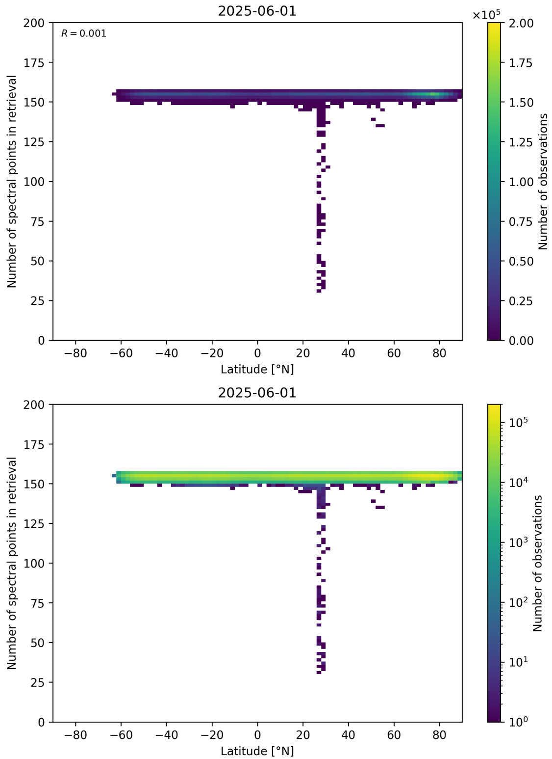
Figure 57: Scatter density plot of “Latitude” against “Number of spectral points in retrieval” for 2025-06-01 to 2025-06-02.
