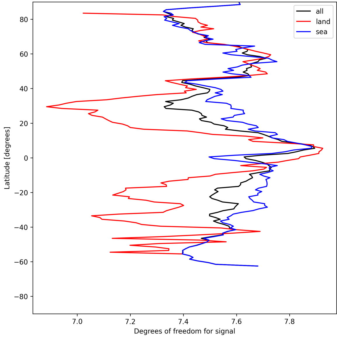
Figure 15: Zonal average of “Degrees of freedom for signal” for 2025-06-01 to 2025-06-02.
