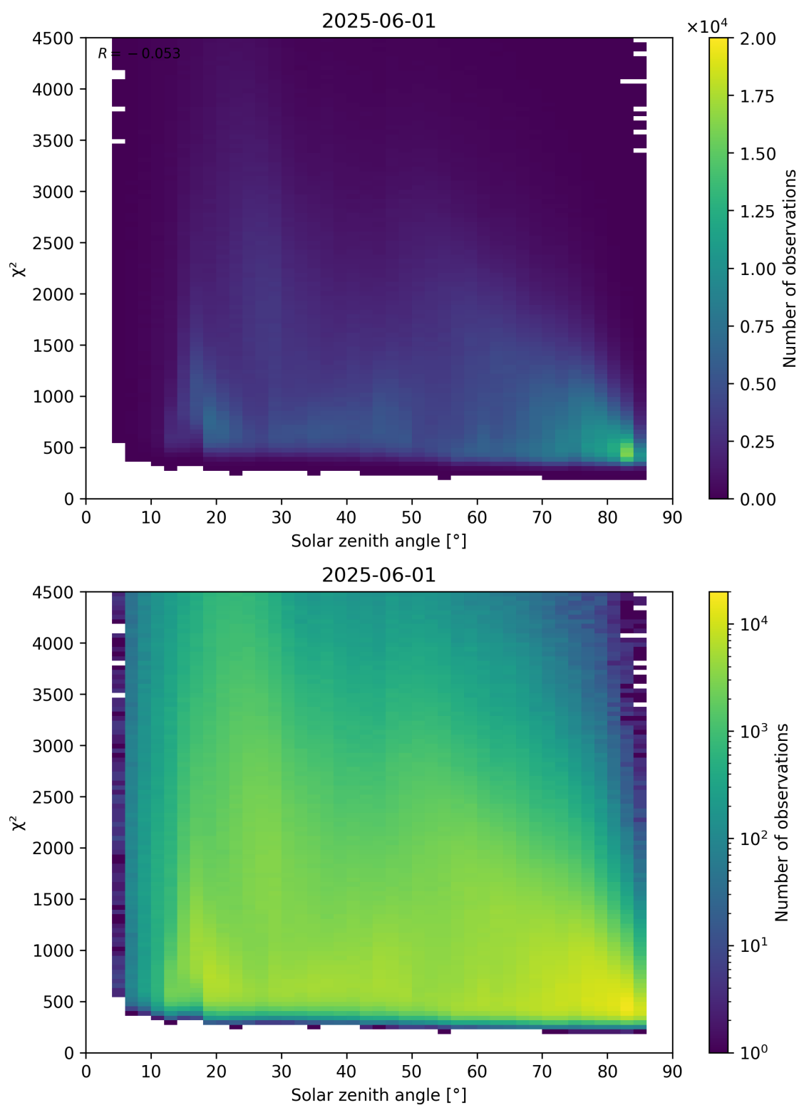
Figure 64: Scatter density plot of “Solar zenith angle” against “ \chi^2 ” for 2025-06-01 to 2025-06-02.
