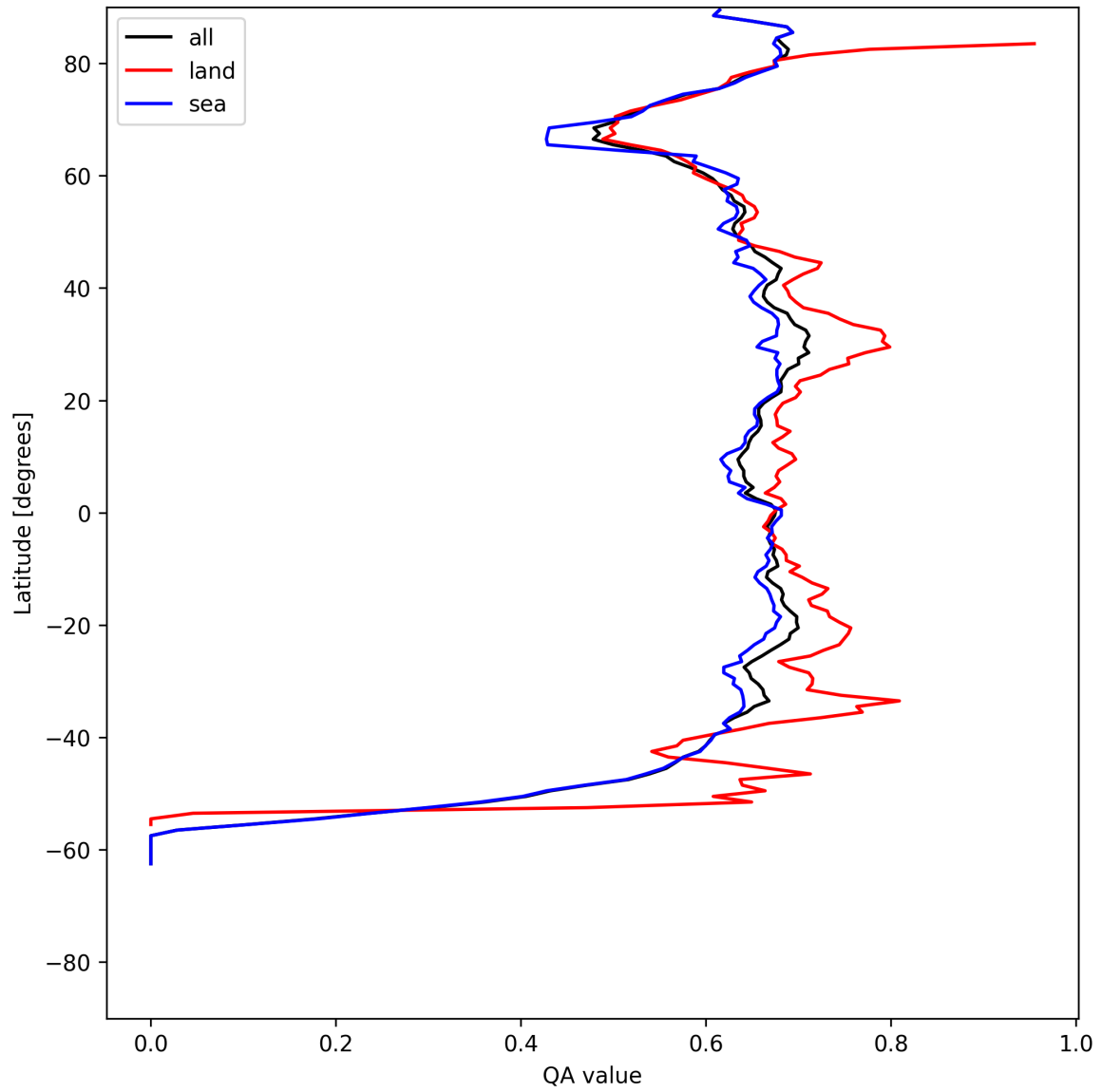
Figure 9: Zonal average of “QA value” for 2025-06-01 to 2025-06-02.
