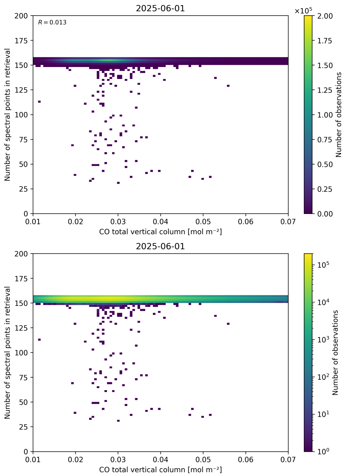
Figure 43: Scatter density plot of “CO total vertical column” against “Number of spectral points in retrieval” for 2025-06-01 to 2025-06-02.
