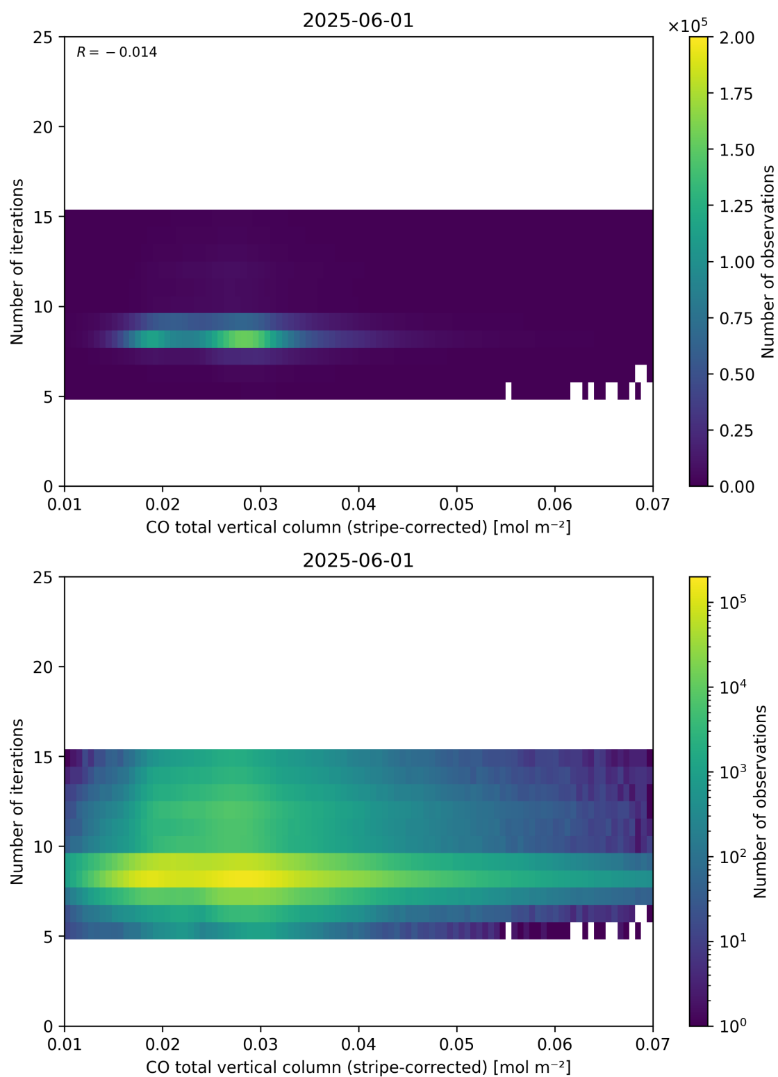
Figure 39: Scatter density plot of “CO total vertical column (stripe-corrected)” against “Number of iterations” for 2025-06-01 to 2025-06-02.
