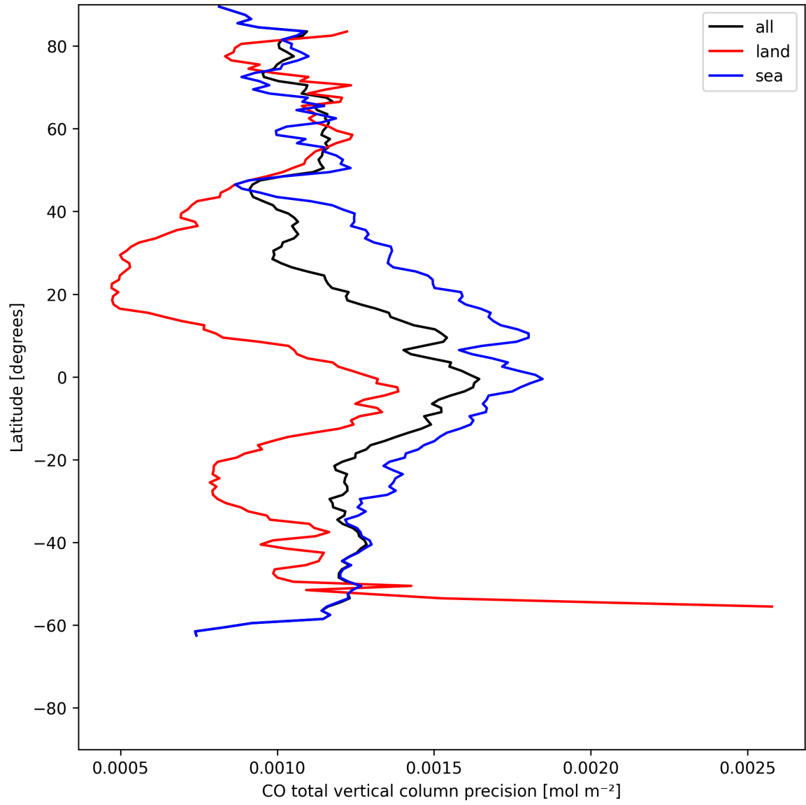
Figure 12: Zonal average of “CO total vertical column precision” for 2025-06-01 to 2025-06-02.
