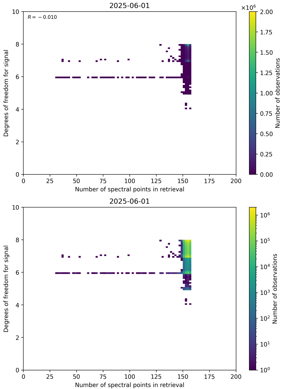
Figure 59: Scatter density plot of “Number of spectral points in retrieval” against “Degrees of freedom for signal” for 2025-06-01 to 2025-06-02.
