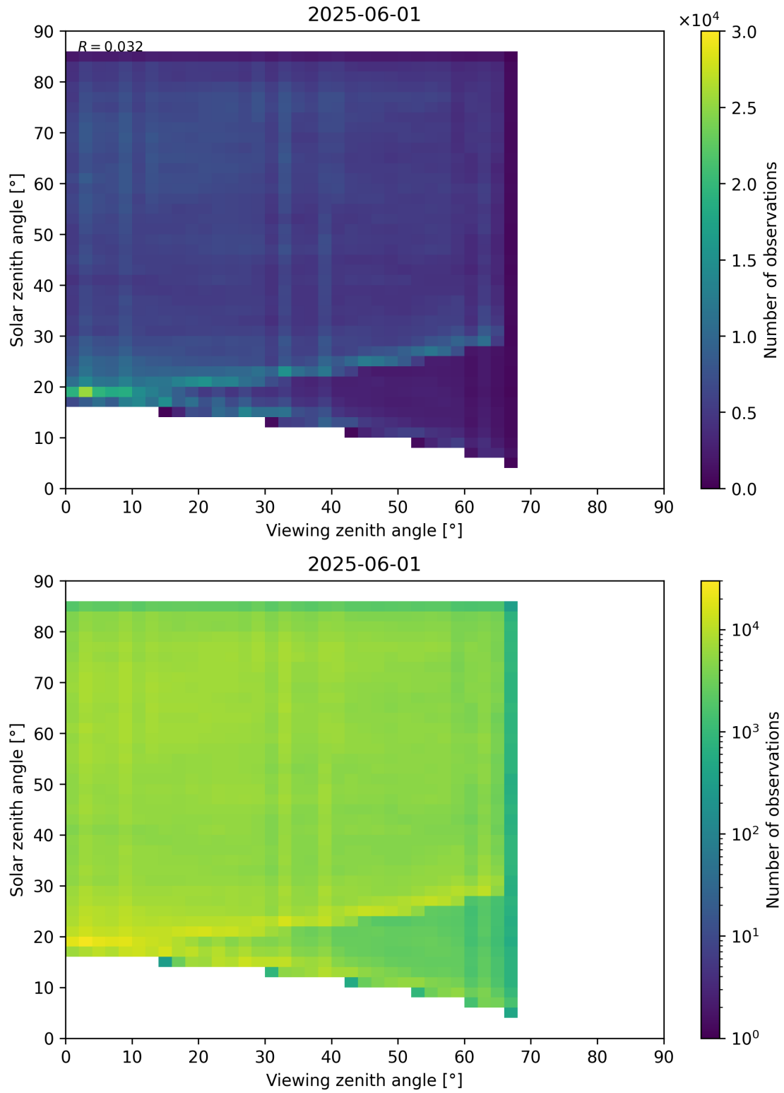
Figure 77: Scatter density plot of “Viewing zenith angle” against “Solar zenith angle” for 2025-06-01 to 2025-06-02.
