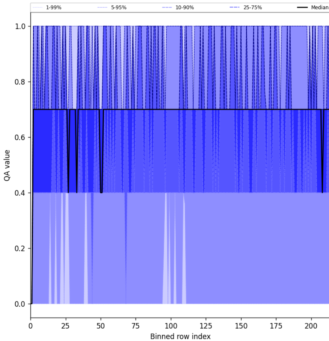
Figure 25: Along track statistics of “QA value” for 2025-06-01 to 2025-06-02
