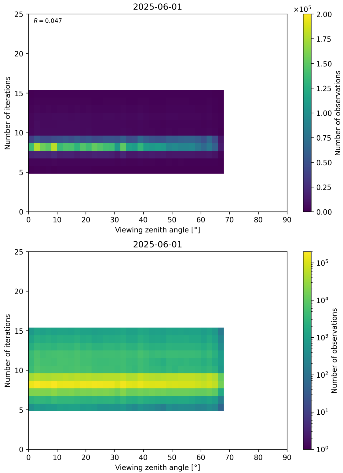
Figure 75: Scatter density plot of “Viewing zenith angle” against “Number of iterations” for 2025-06-01 to 2025-06-02.
