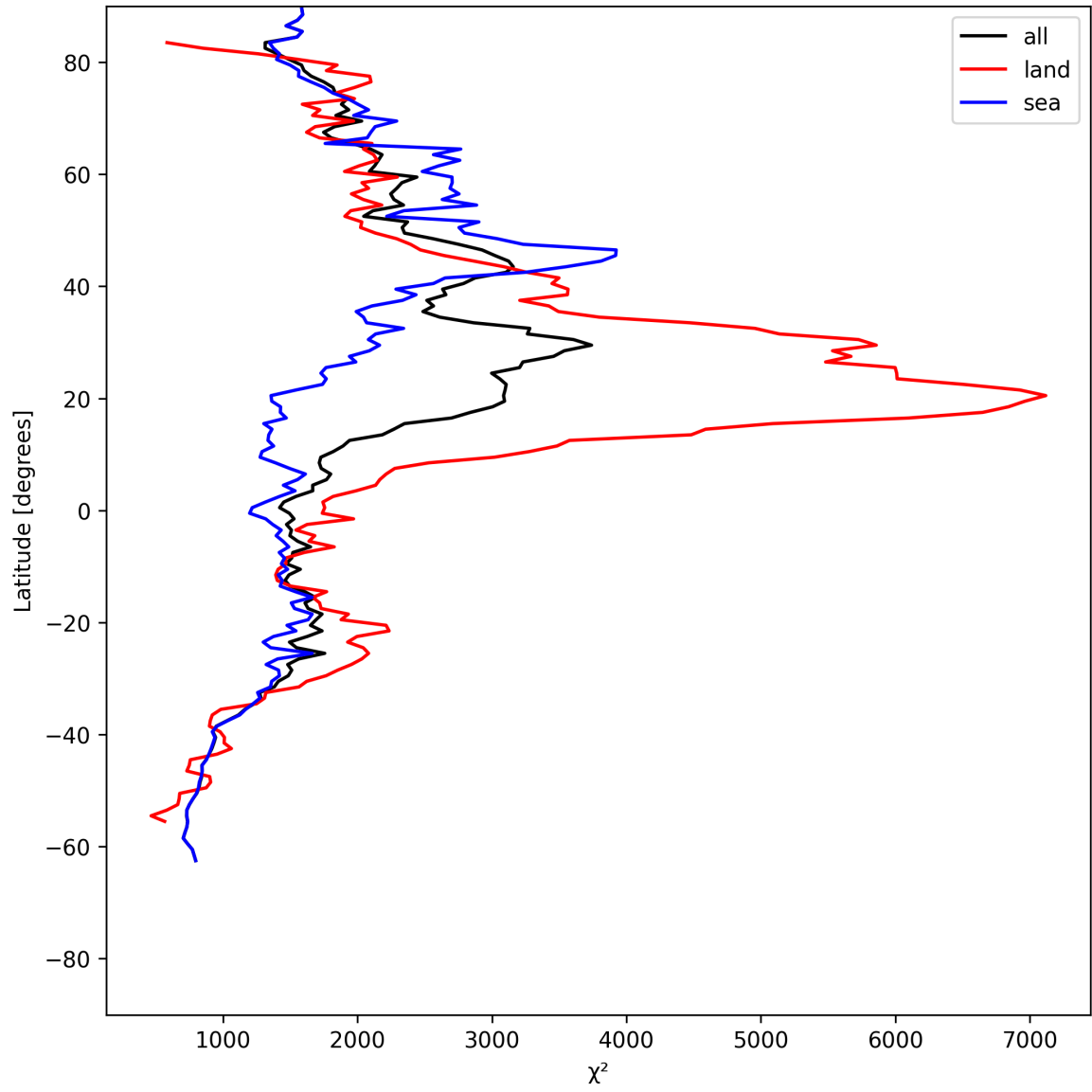
Figure 14: Zonal average of “ \chi^2 ” for 2025-06-01 to 2025-06-02.
