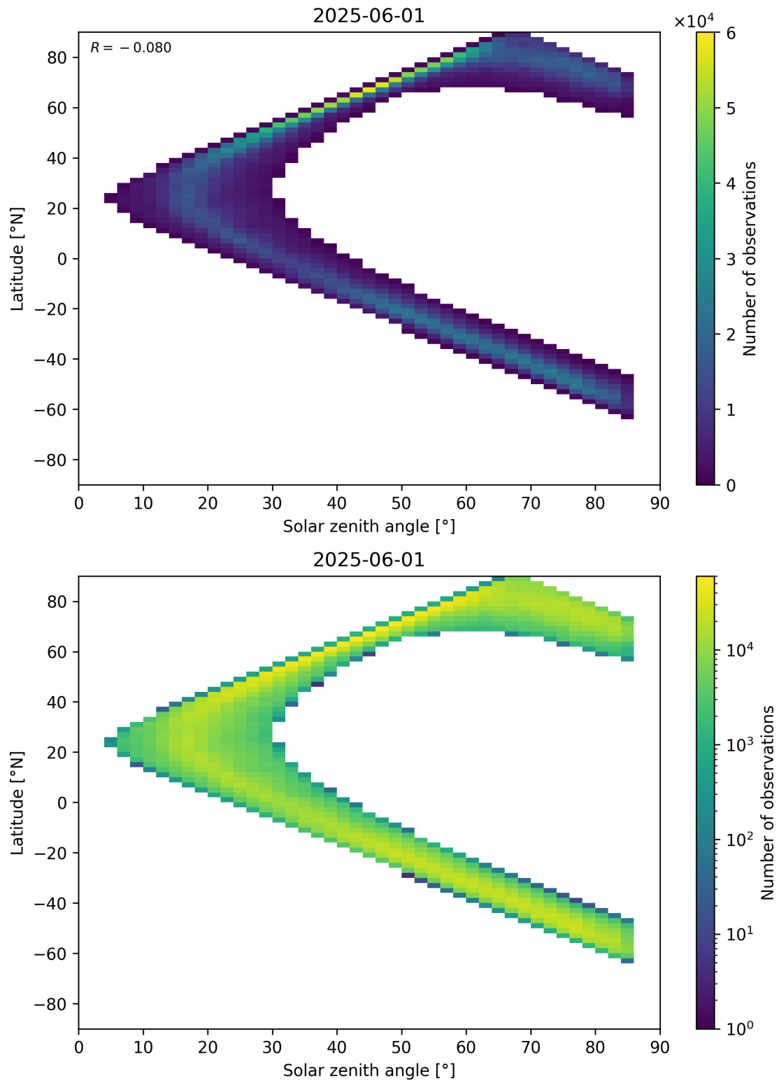
Figure 66: Scatter density plot of “Solar zenith angle” against “Latitude” for 2025-06-01 to 2025-06-02.
