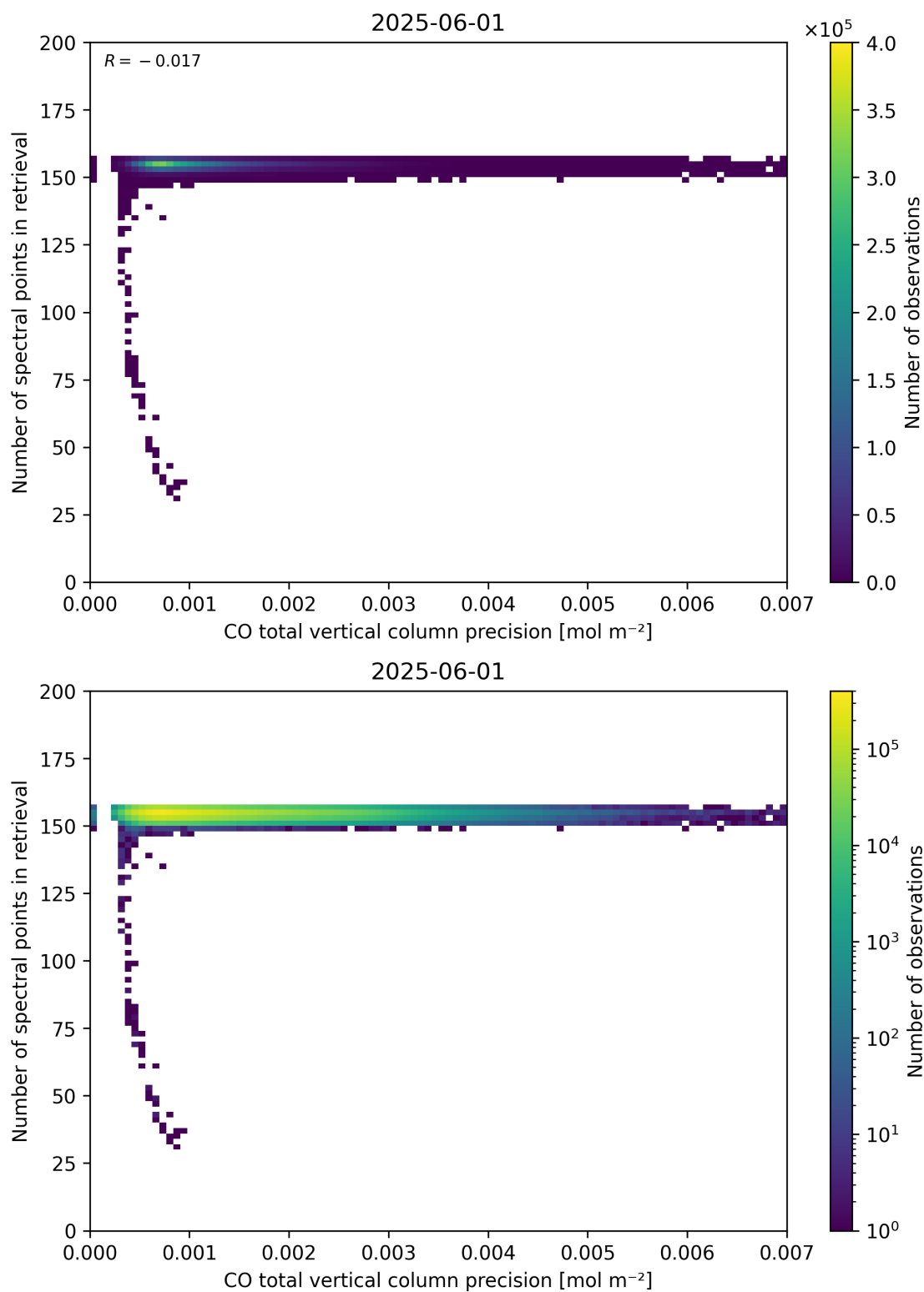
Figure 47: Scatter density plot of “CO total vertical column precision” against “Number of spectral points in retrieval” for 2025-06-01 to 2025-06-02.
