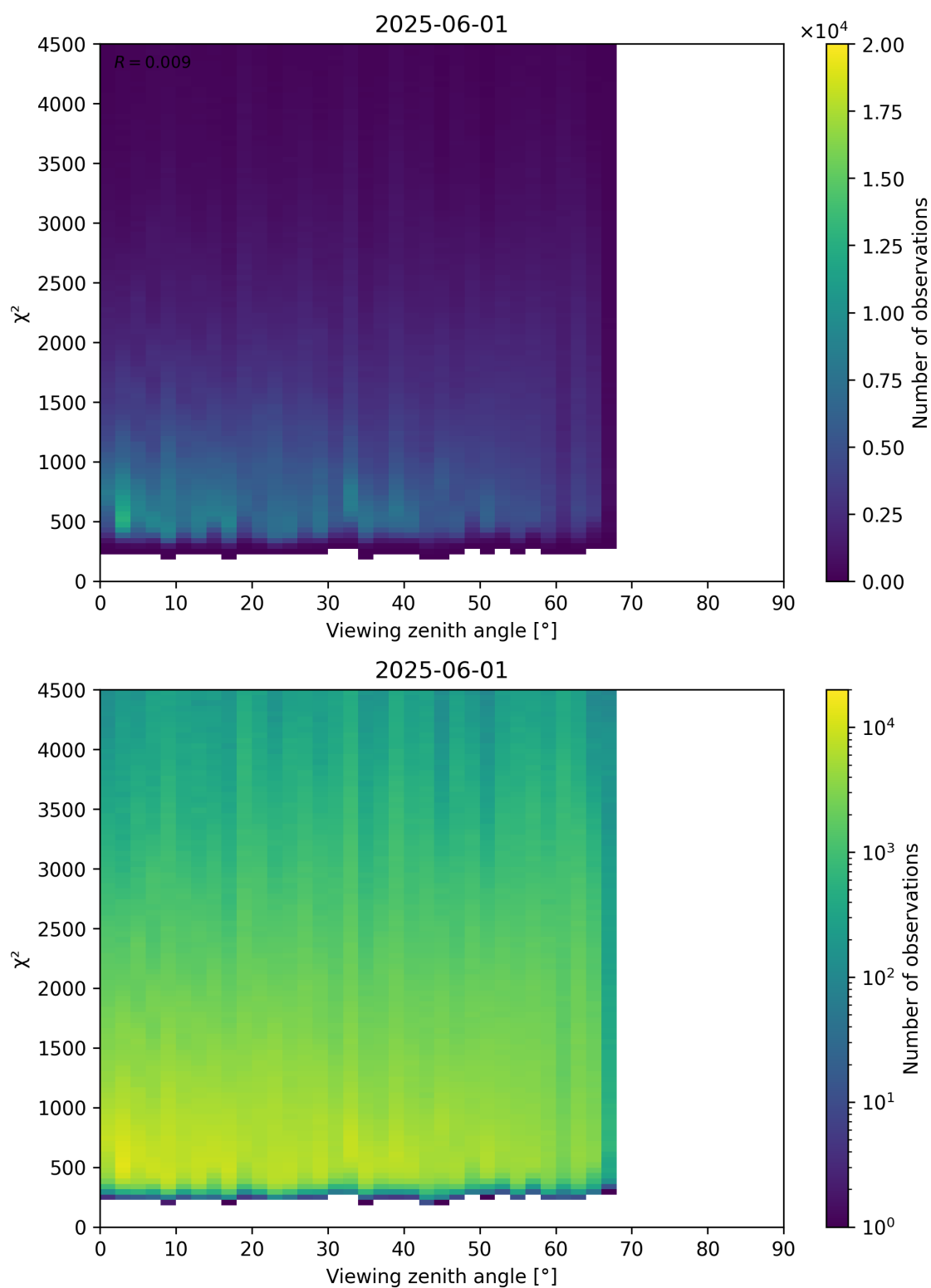
Figure 72: Scatter density plot of “Viewing zenith angle” against “ \chi^2 ” for 2025-06-01 to 2025-06-02.
