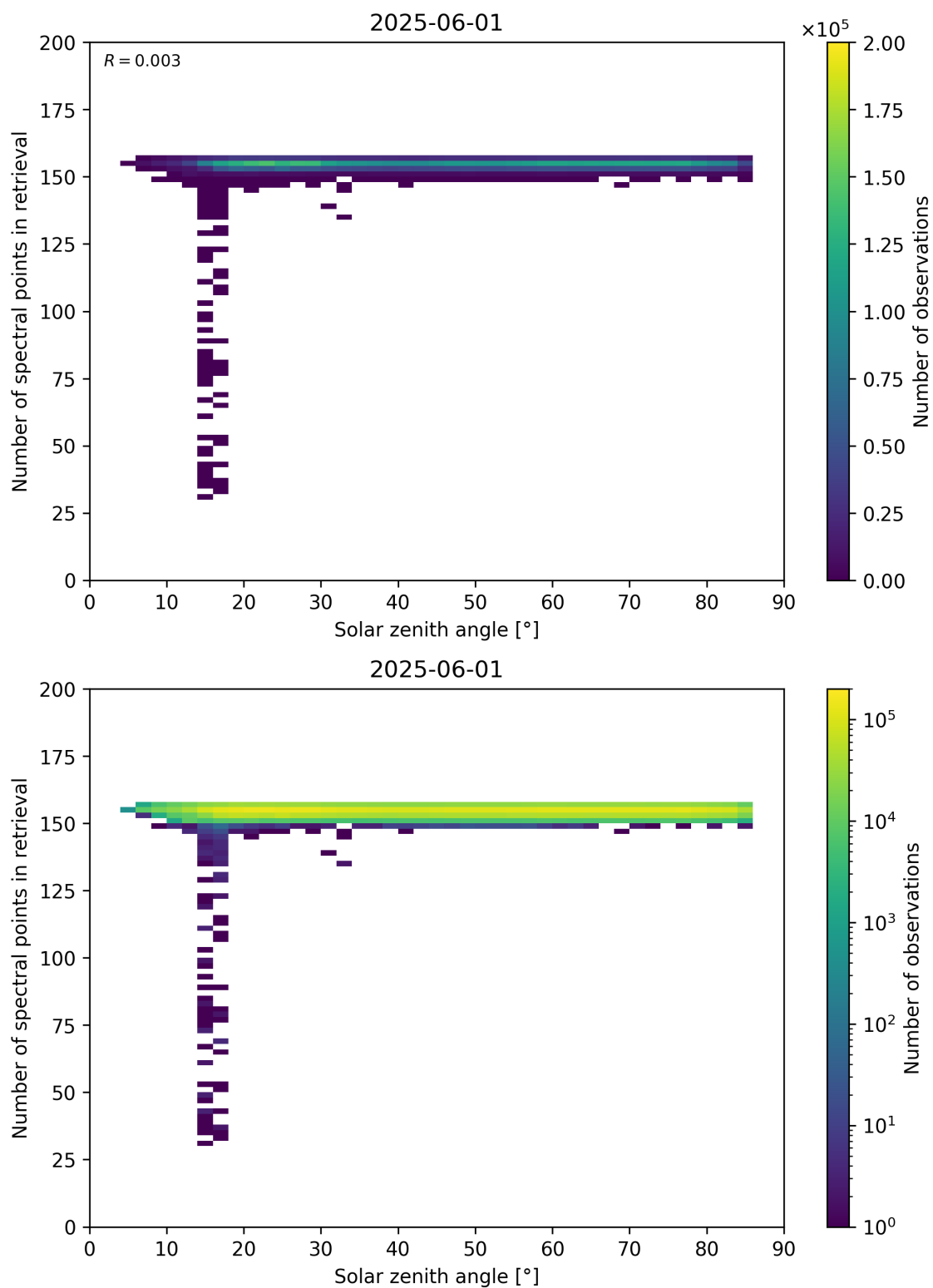
Figure 68: Scatter density plot of “Solar zenith angle” against “Number of spectral points in retrieval” for 2025-06-01 to 2025-06-02.
