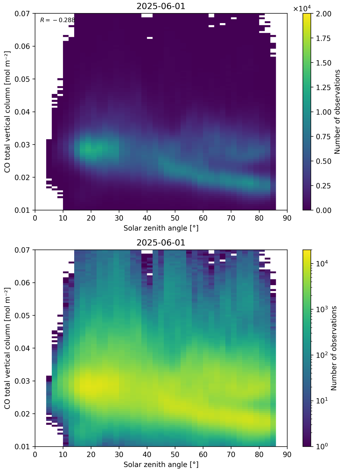
Figure 61: Scatter density plot of “Solar zenith angle” against “CO total vertical column” for 2025-06-01 to 2025-06-02.
