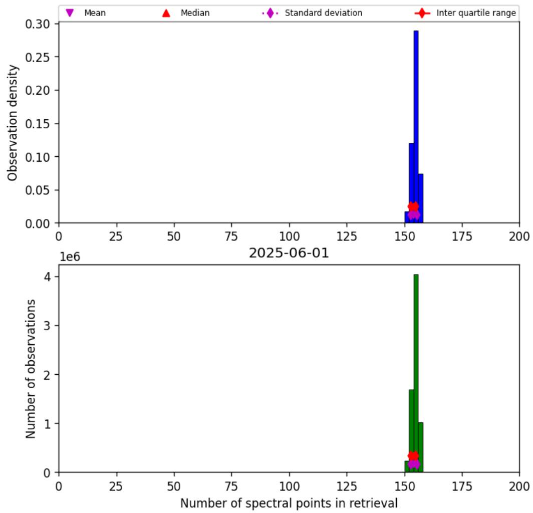
Figure 21: Histogram of “Number of spectral points in retrieval” for 2025-06-01 to 2025-06-02
