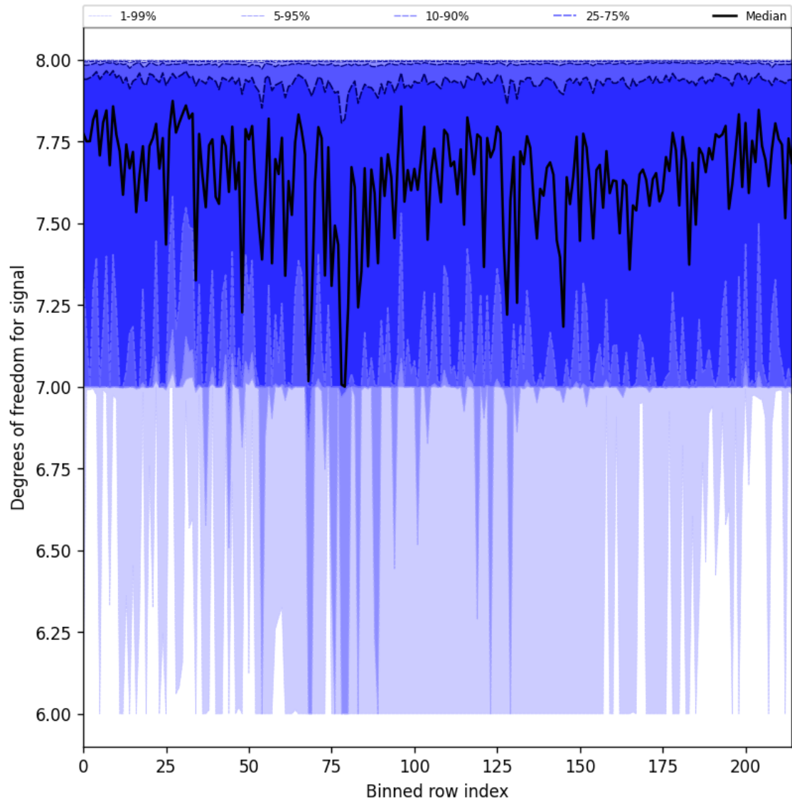
Figure 31: Along track statistics of “Degrees of freedom for signal” for 2025-06-01 to 2025-06-02
