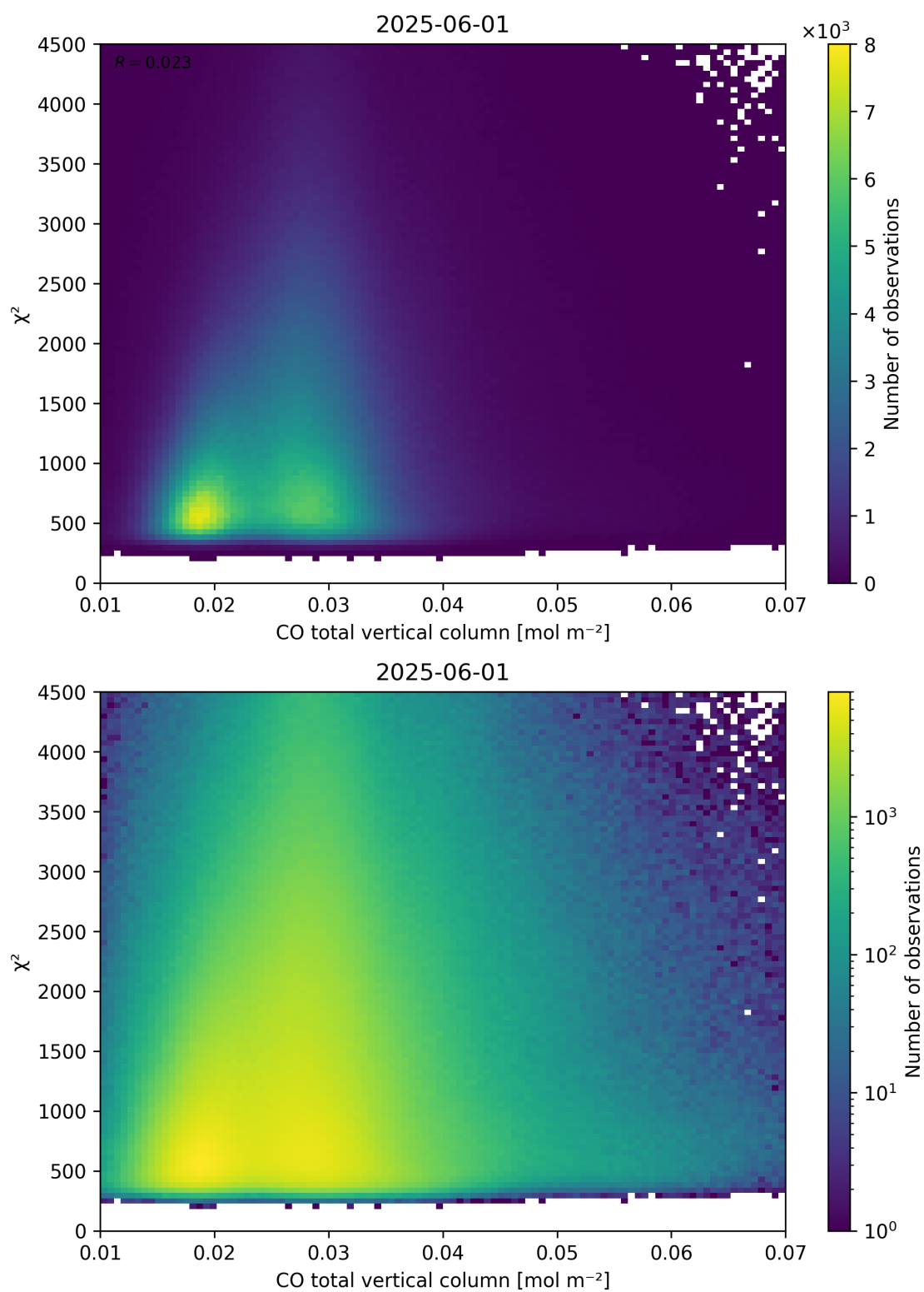
Figure 35: Scatter density plot of “CO total vertical column” against “ \chi^2 ” for 2025-06-01 to 2025-06-02.
