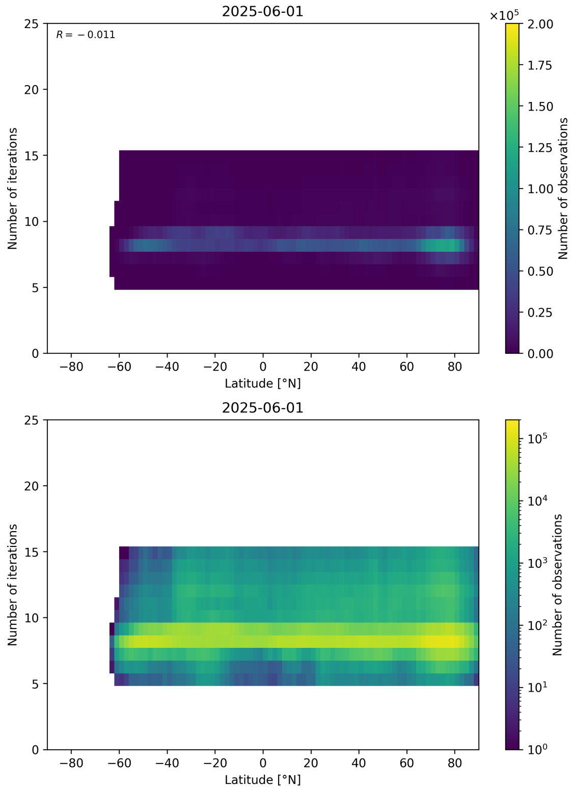
Figure 56: Scatter density plot of “Latitude” against “Number of iterations” for 2025-06-01 to 2025-06-02.
