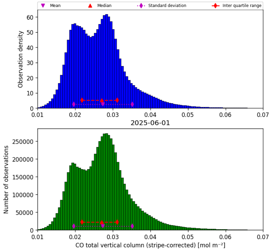
Figure 19: Histogram of “CO total vertical column (stripe-corrected)” for 2025-06-01 to 2025-06-02
