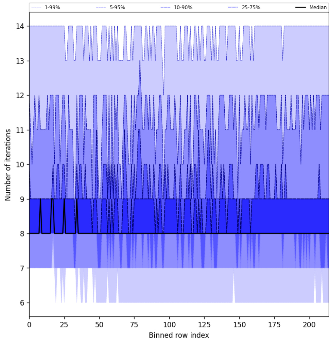
Figure 32: Along track statistics of “Number of iterations” for 2025-06-01 to 2025-06-02
