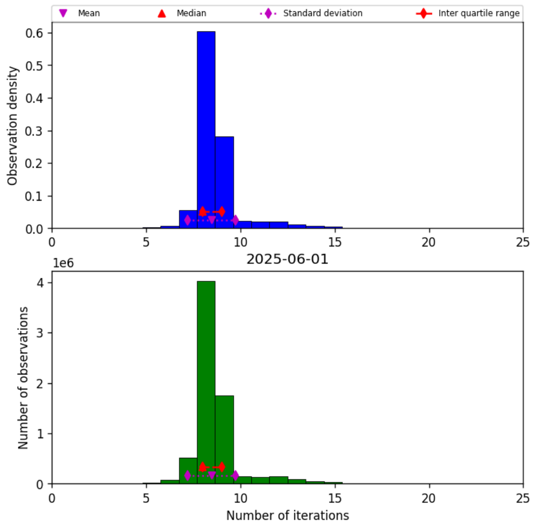
Figure 24: Histogram of “Number of iterations” for 2025-06-01 to 2025-06-02
