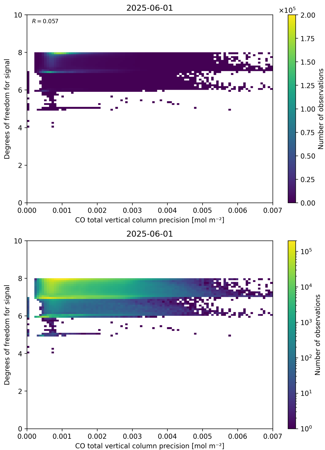
Figure 45: Scatter density plot of “CO total vertical column precision” against “Degrees of freedom for signal” for 2025-06-01 to 2025-06-02.
