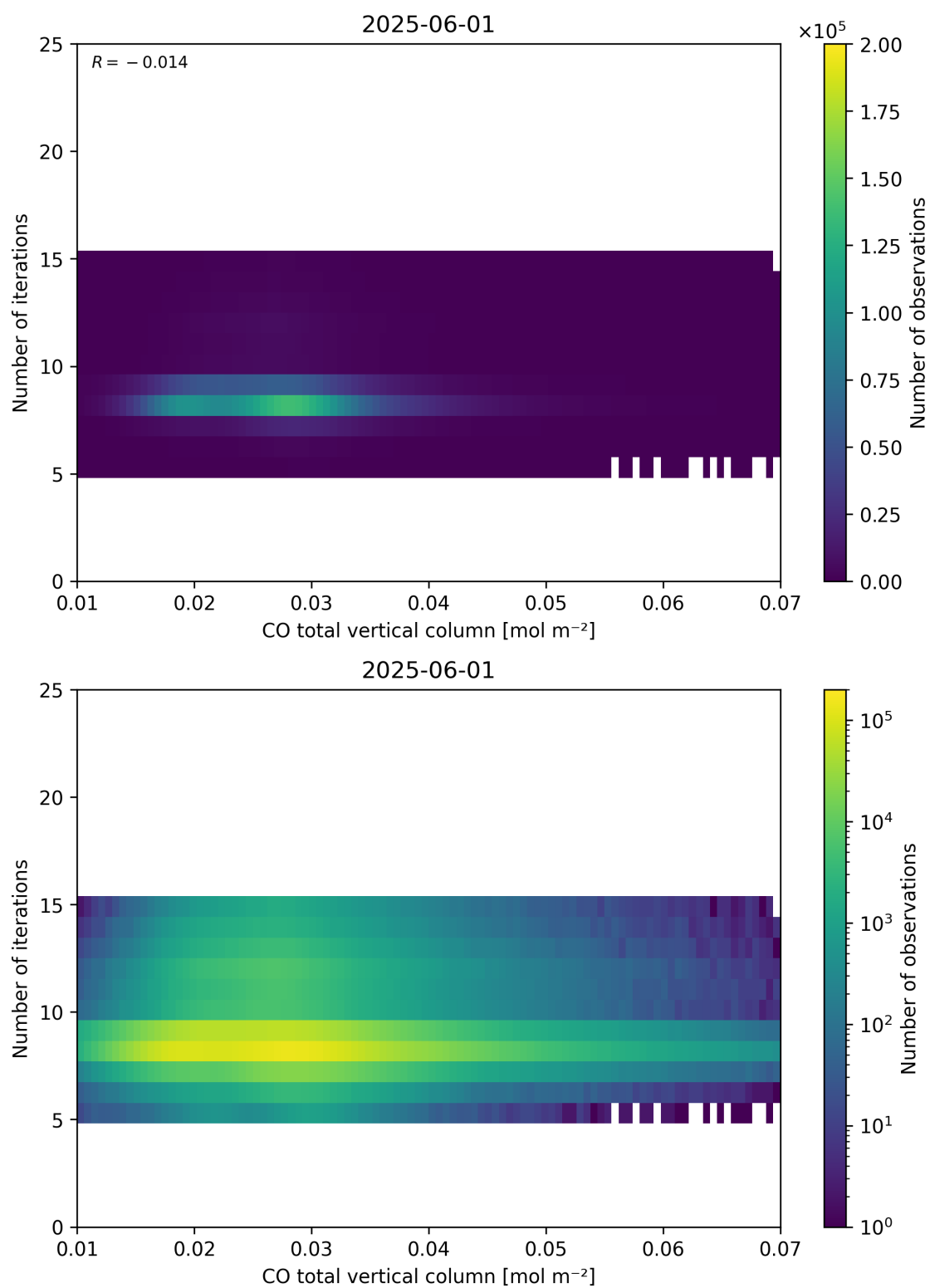
Figure 42: Scatter density plot of “CO total vertical column” against “Number of iterations” for 2025-06-01 to 2025-06-02.
