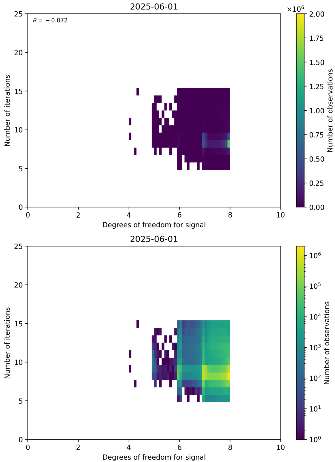
Figure 50: Scatter density plot of “Degrees of freedom for signal” against “Number of iterations” for 2025-06-01 to 2025-06-02.
