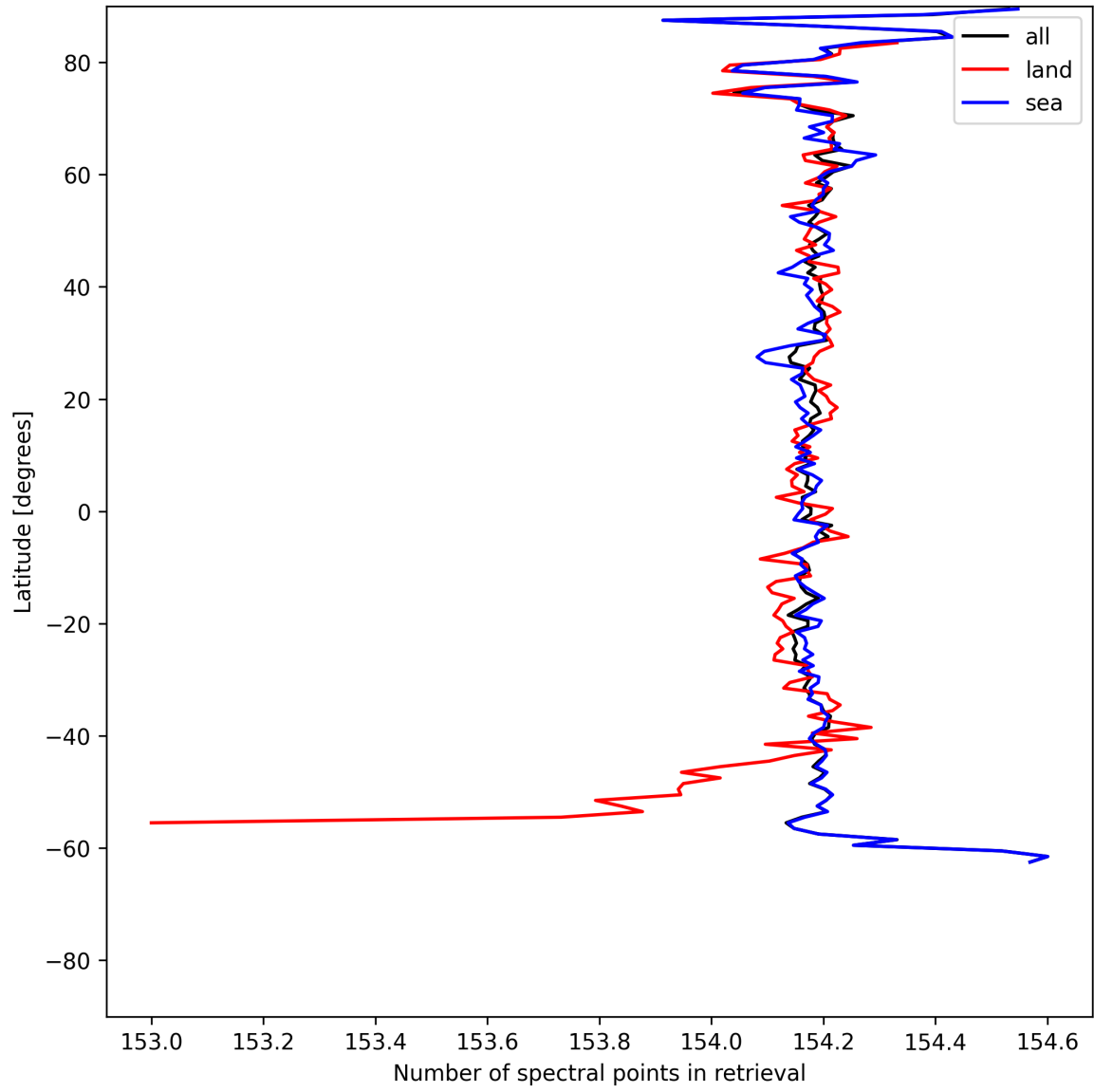
Figure 13: Zonal average of “Number of spectral points in retrieval” for 2025-06-01 to 2025-06-02.
