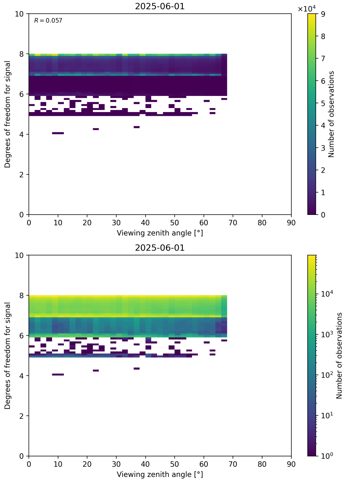
Figure 73: Scatter density plot of “Viewing zenith angle” against “Degrees of freedom for signal” for 2025-06-01 to 2025-06-02.
