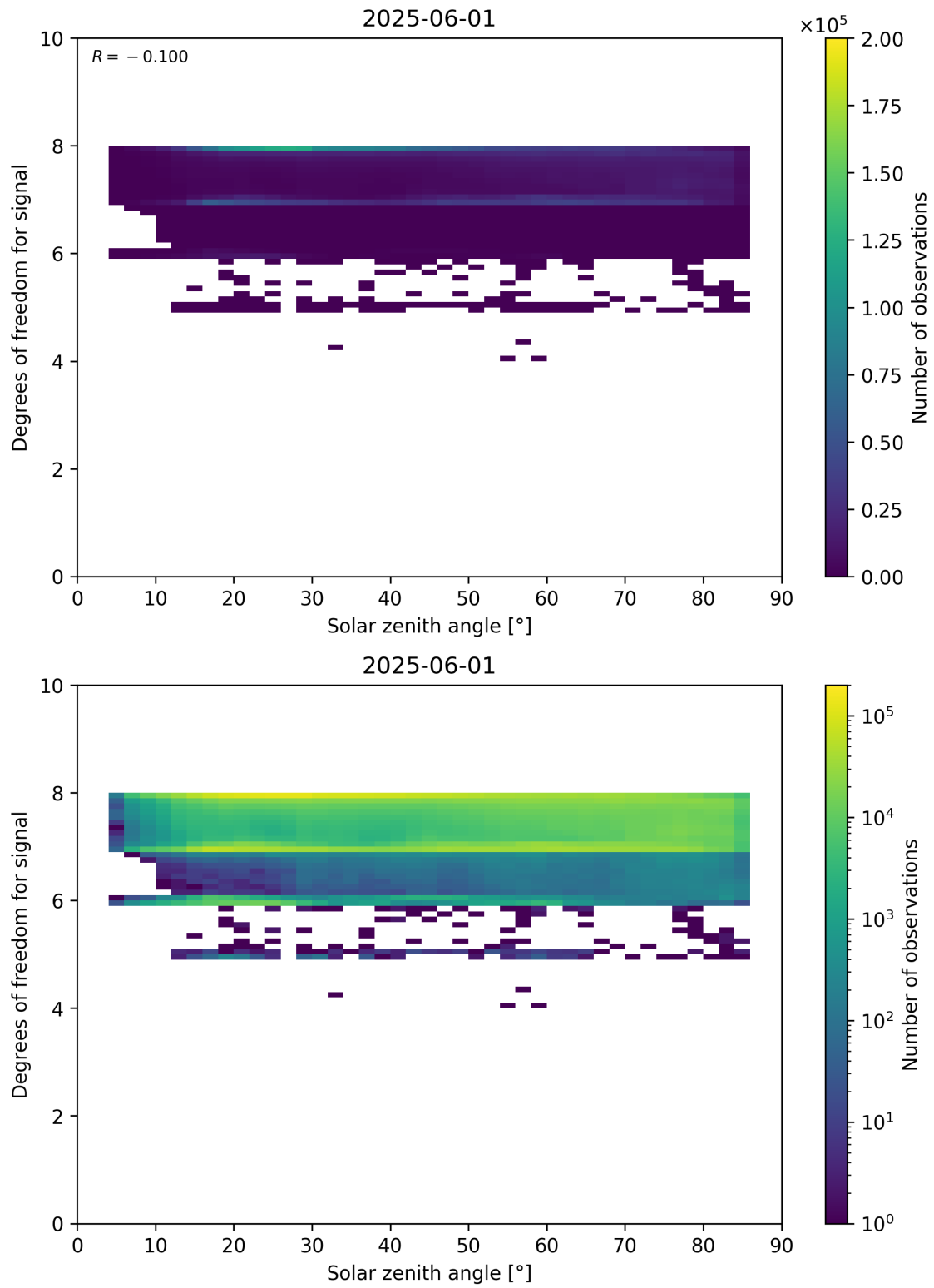
Figure 65: Scatter density plot of “Solar zenith angle” against “Degrees of freedom for signal” for 2025-06-01 to 2025-06-02.
