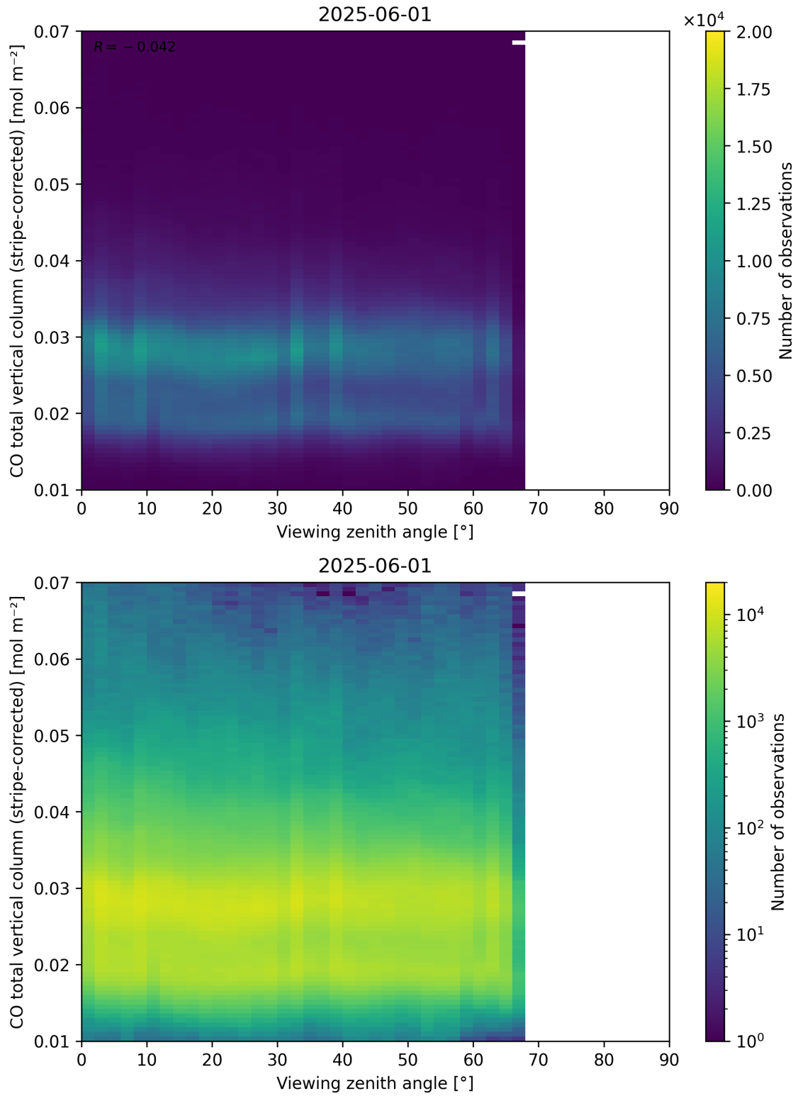
Figure 70: Scatter density plot of “Viewing zenith angle” against “CO total vertical column (stripe-corrected)” for 2025-06-01 to 2025-06-02.
