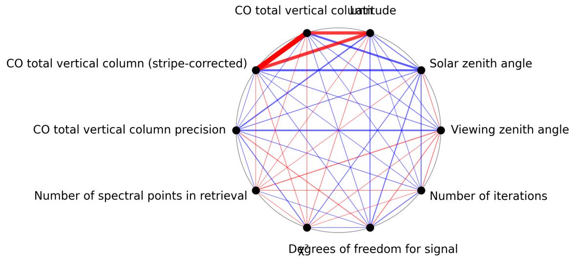
Figure 1: Map of correlation graph for 2025-06-01 to 2025-06-02.
