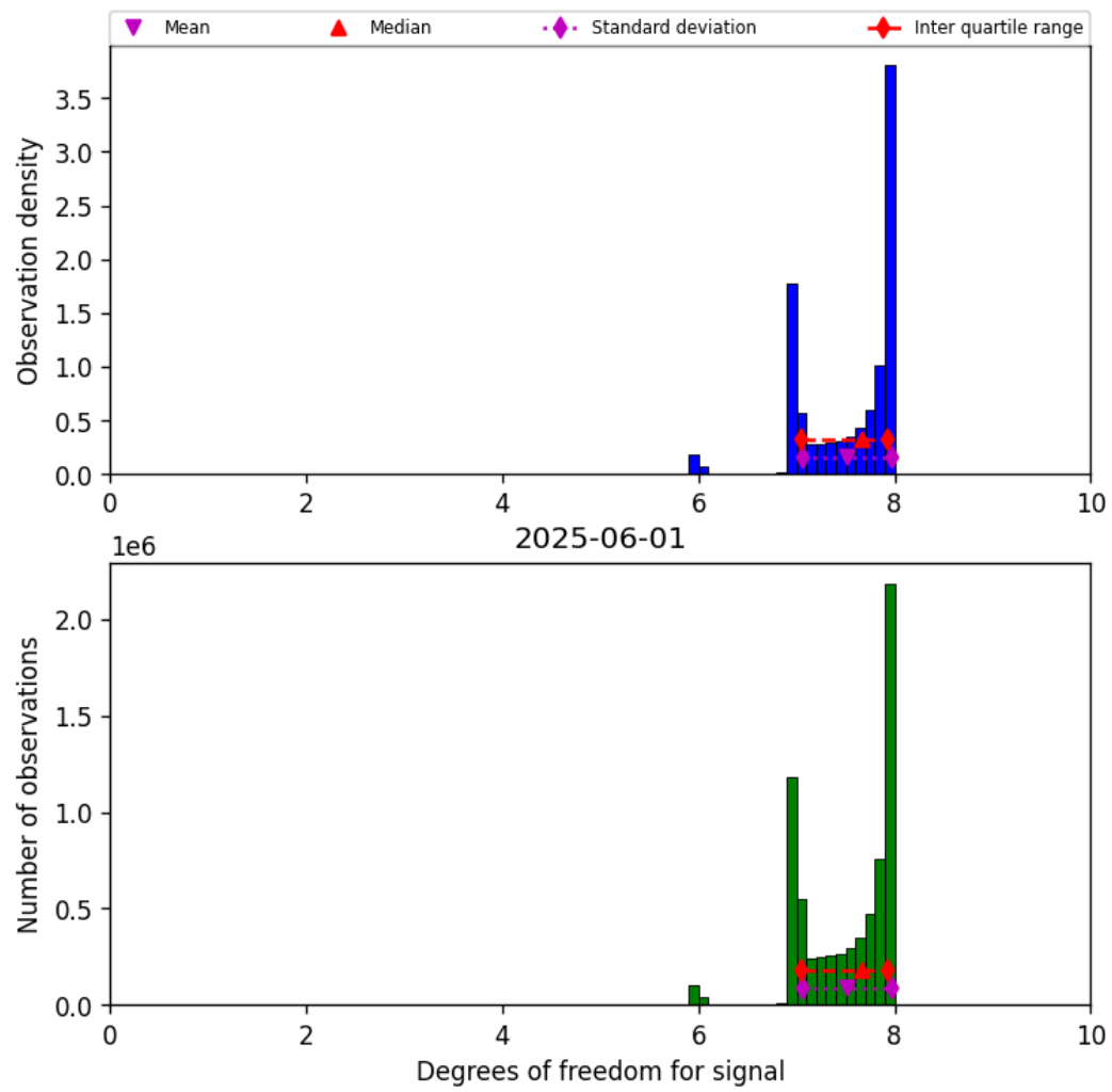
Figure 23: Histogram of “Degrees of freedom for signal” for 2025-06-01 to 2025-06-02
