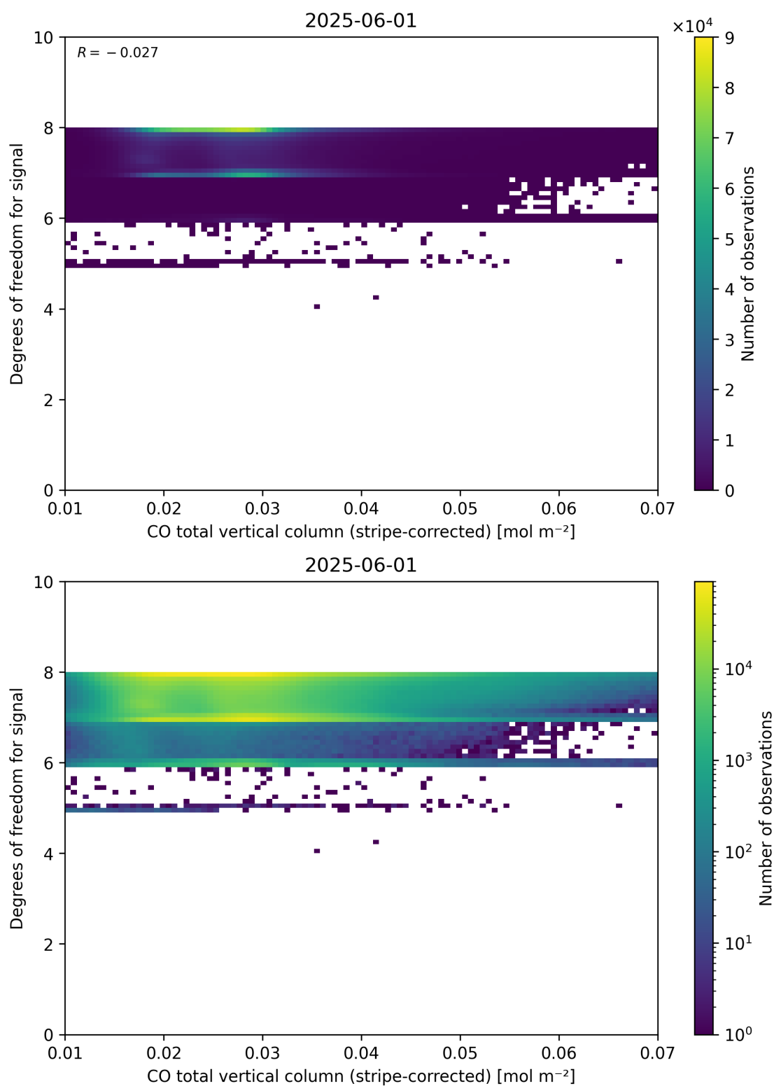
Figure 38: Scatter density plot of “CO total vertical column (stripe-corrected)” against “Degrees of freedom for signal” for 2025-06-01 to 2025-06-02.
