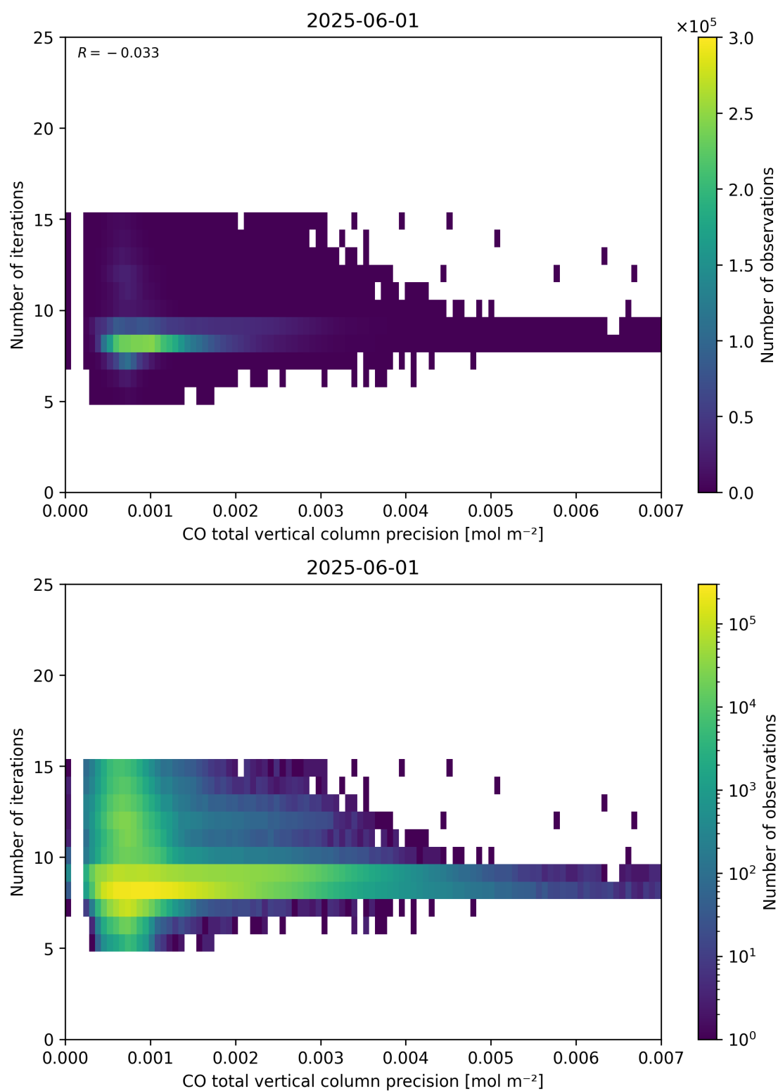
Figure 46: Scatter density plot of “CO total vertical column precision” against “Number of iterations” for 2025-06-01 to 2025-06-02.
