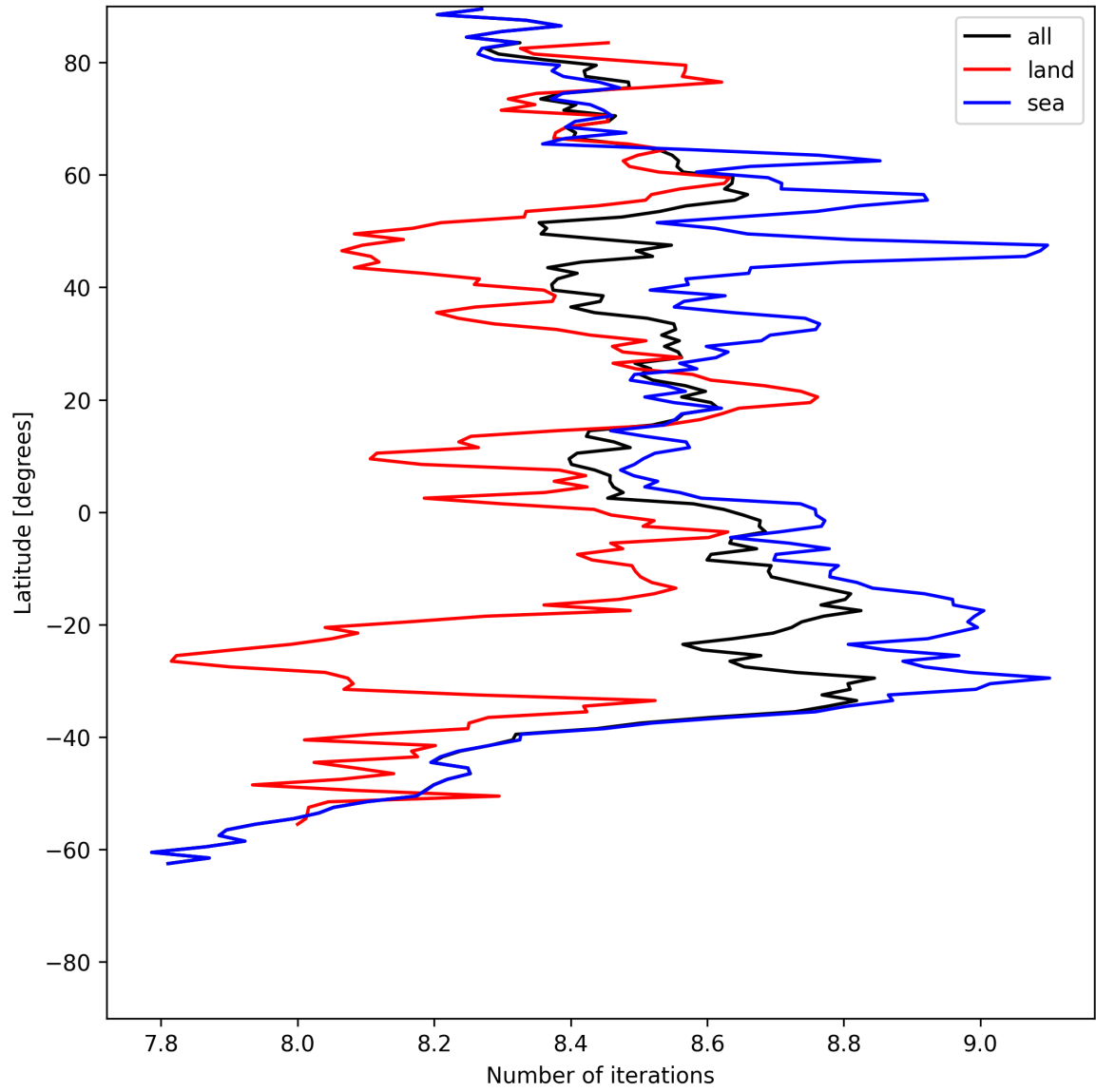
Figure 16: Zonal average of “Number of iterations” for 2025-06-01 to 2025-06-02.
