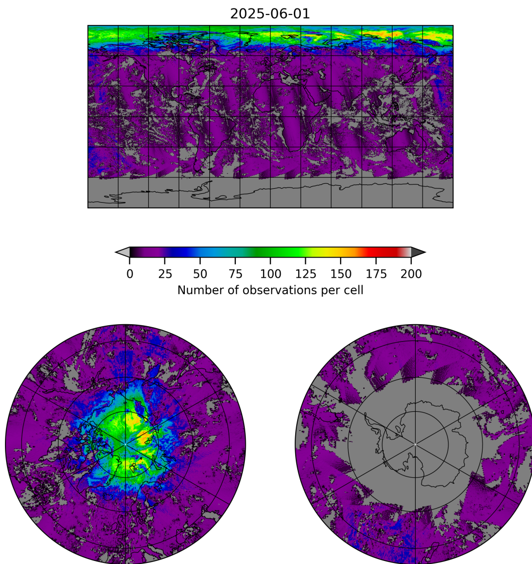
Figure 8: Map of the number of observations for 2025-06-01 to 2025-06-02
