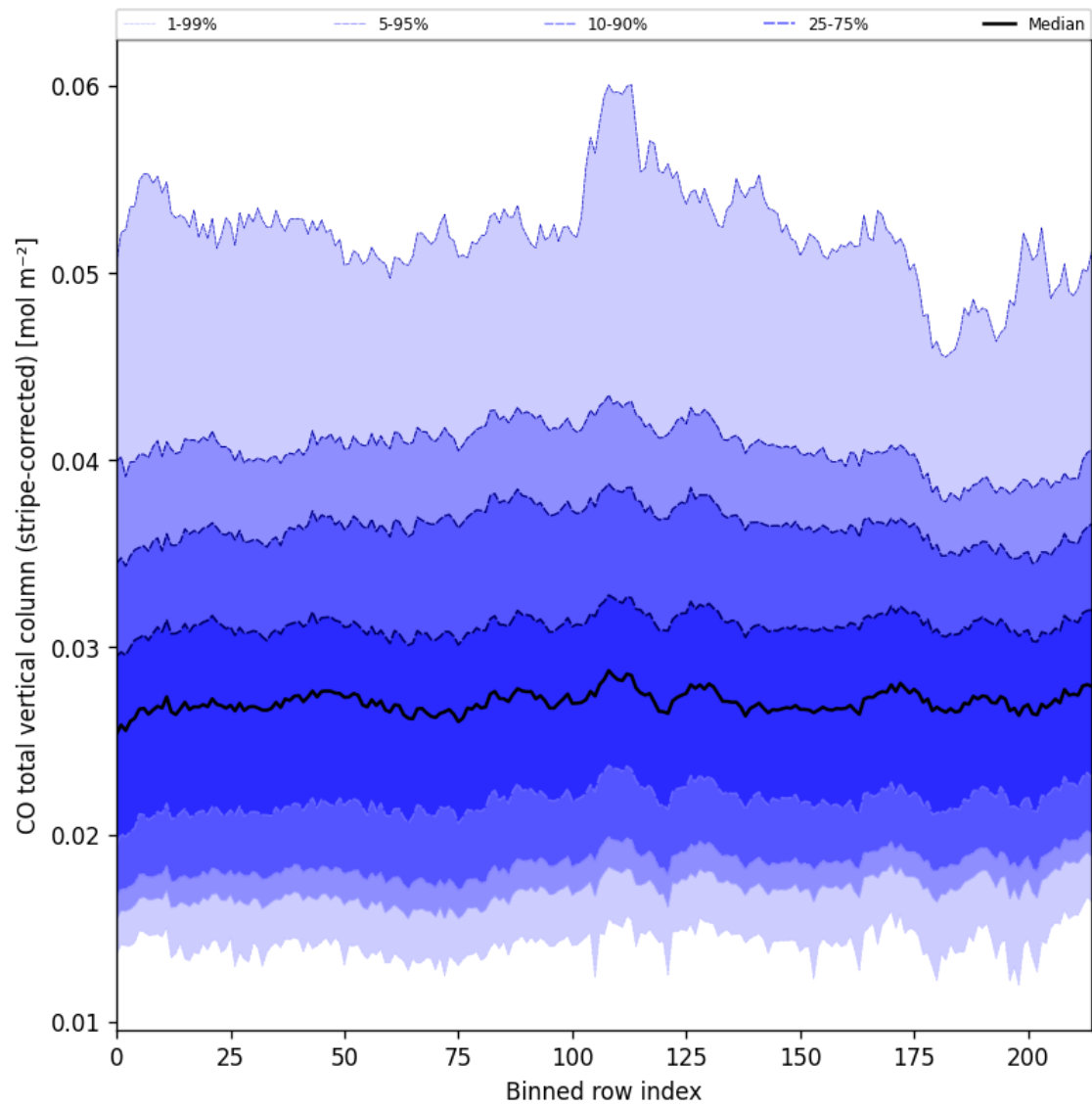
Figure 27: Along track statistics of “CO total vertical column (stripe-corrected)” for 2025-06-01 to 2025-06-02
