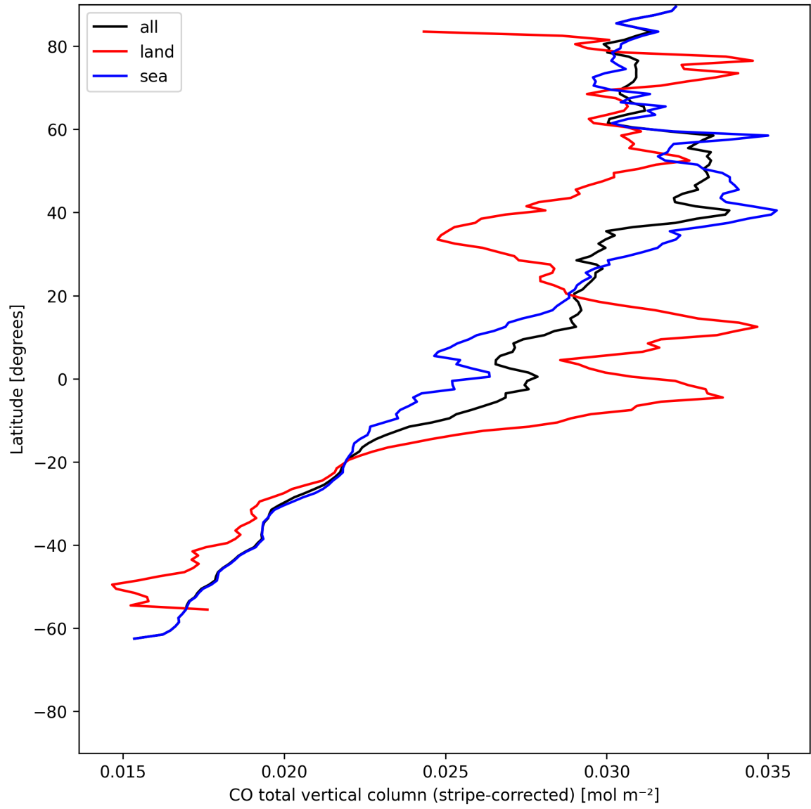
Figure 11: Zonal average of “CO total vertical column (stripe-corrected)” for 2025-06-01 to 2025-06-02.
