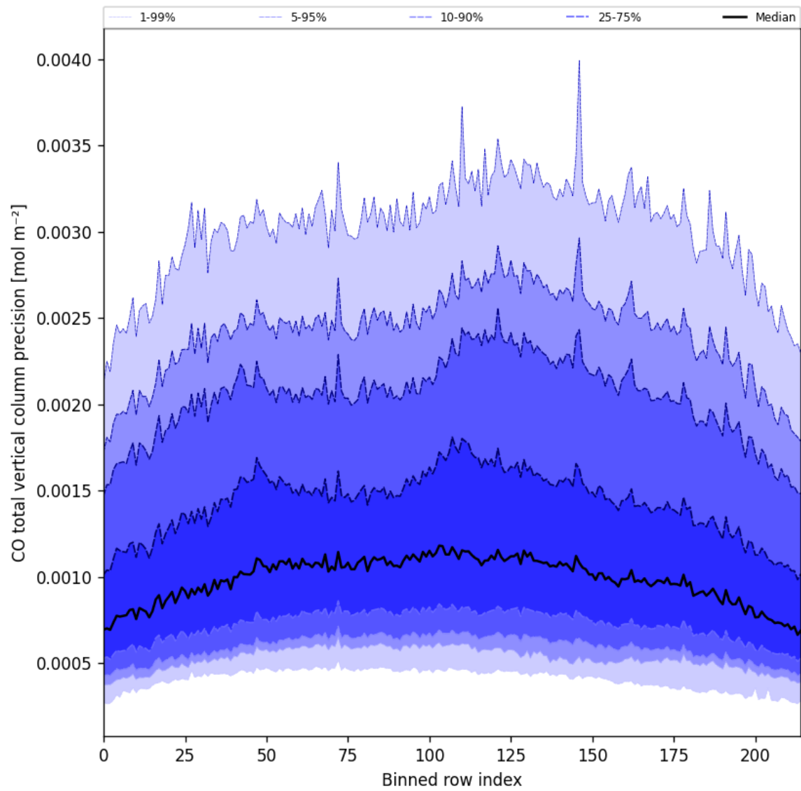
Figure 28: Along track statistics of “CO total vertical column precision” for 2025-06-01 to 2025-06-02
