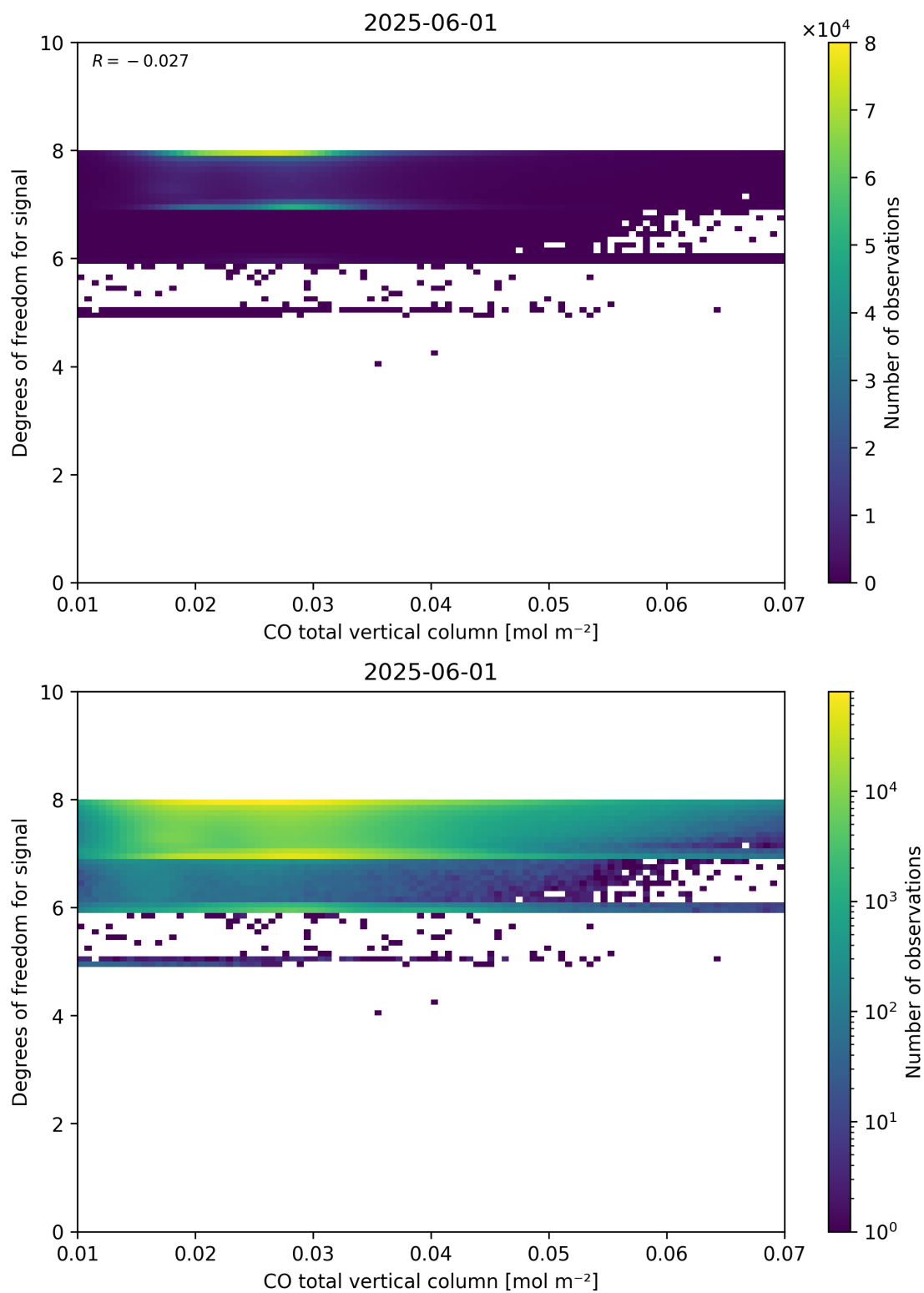
Figure 41: Scatter density plot of “CO total vertical column” against “Degrees of freedom for signal” for 2025-06-01 to 2025-06-02.
