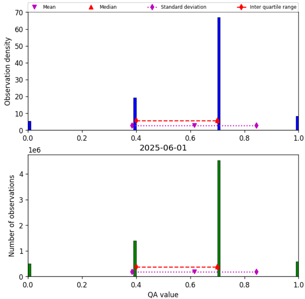
Figure 17: Histogram of “QA value” for 2025-06-01 to 2025-06-02
