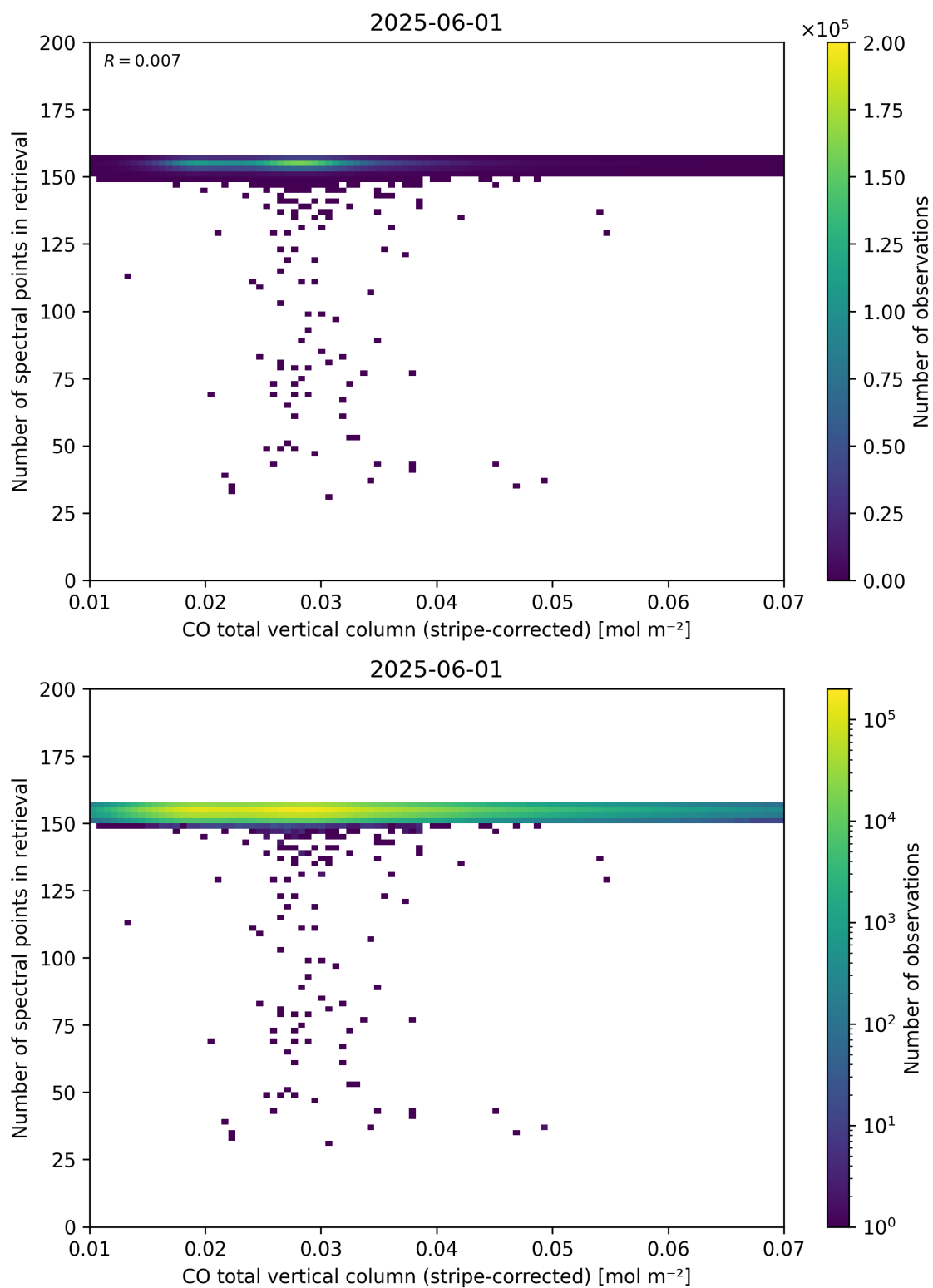
Figure 40: Scatter density plot of “CO total vertical column (stripe-corrected)” against “Number of spectral points in retrieval” for 2025-06-01 to 2025-06-02.
