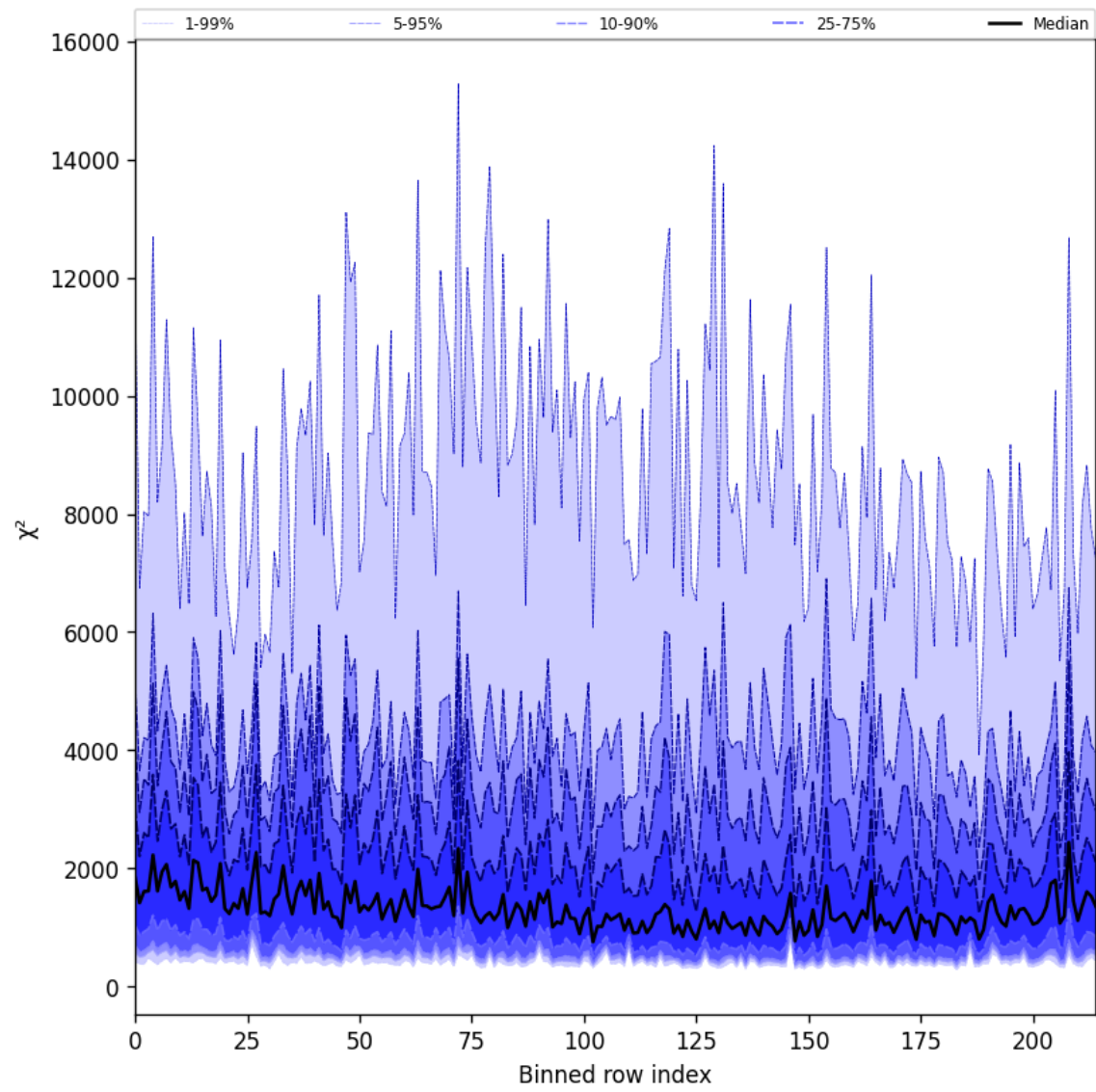
Figure 30: Along track statistics of “ \chi^2 ” for 2025-06-01 to 2025-06-02
