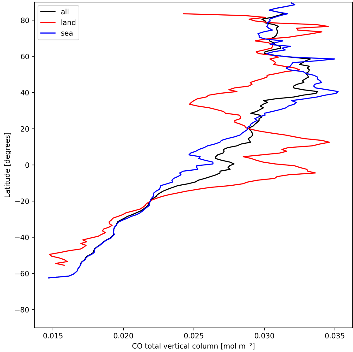
Figure 10: Zonal average of “CO total vertical column” for 2025-06-01 to 2025-06-02.
