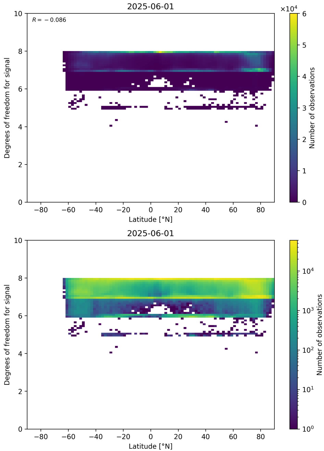
Figure 55: Scatter density plot of “Latitude” against “Degrees of freedom for signal” for 2025-06-01 to 2025-06-02.
