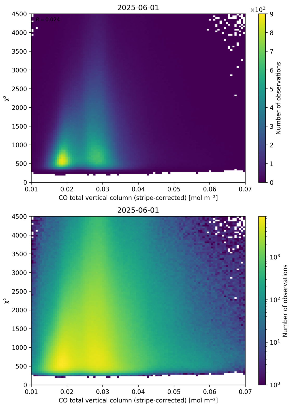
Figure 37: Scatter density plot of “CO total vertical column (stripe-corrected)” against “ \chi^2 ” for 2025-06-01 to 2025-06-02.
