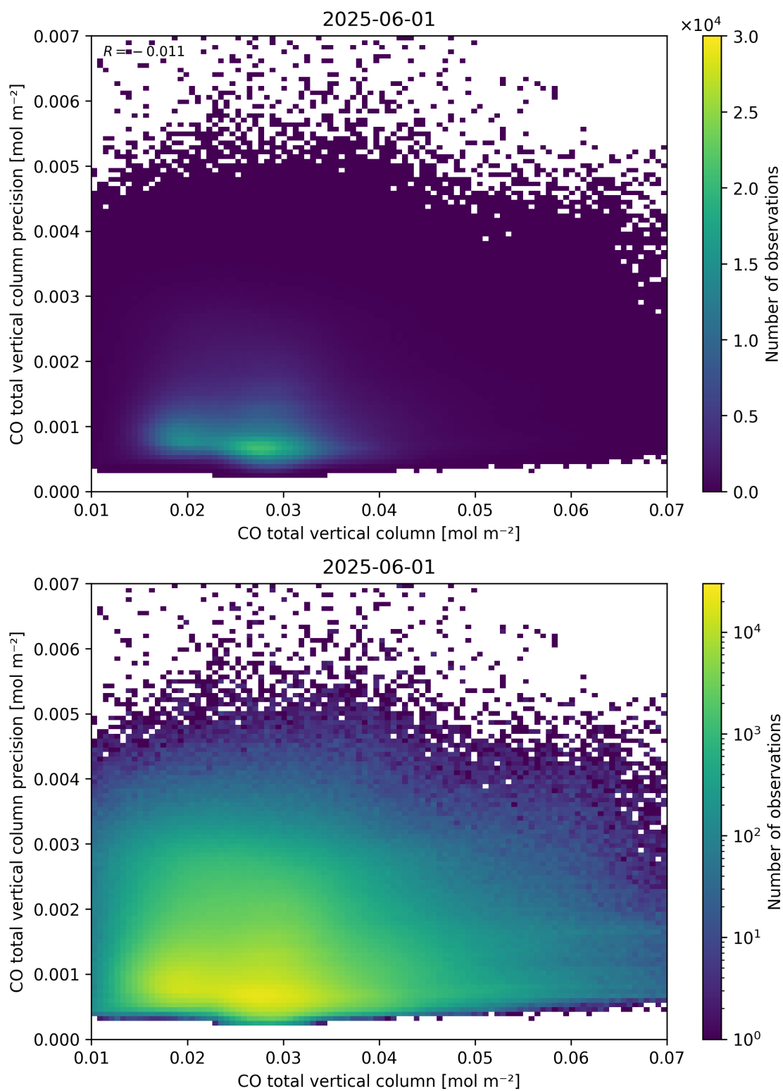
Figure 34: Scatter density plot of “CO total vertical column” against “CO total vertical column precision” for 2025-06-01 to 2025-06-02.
