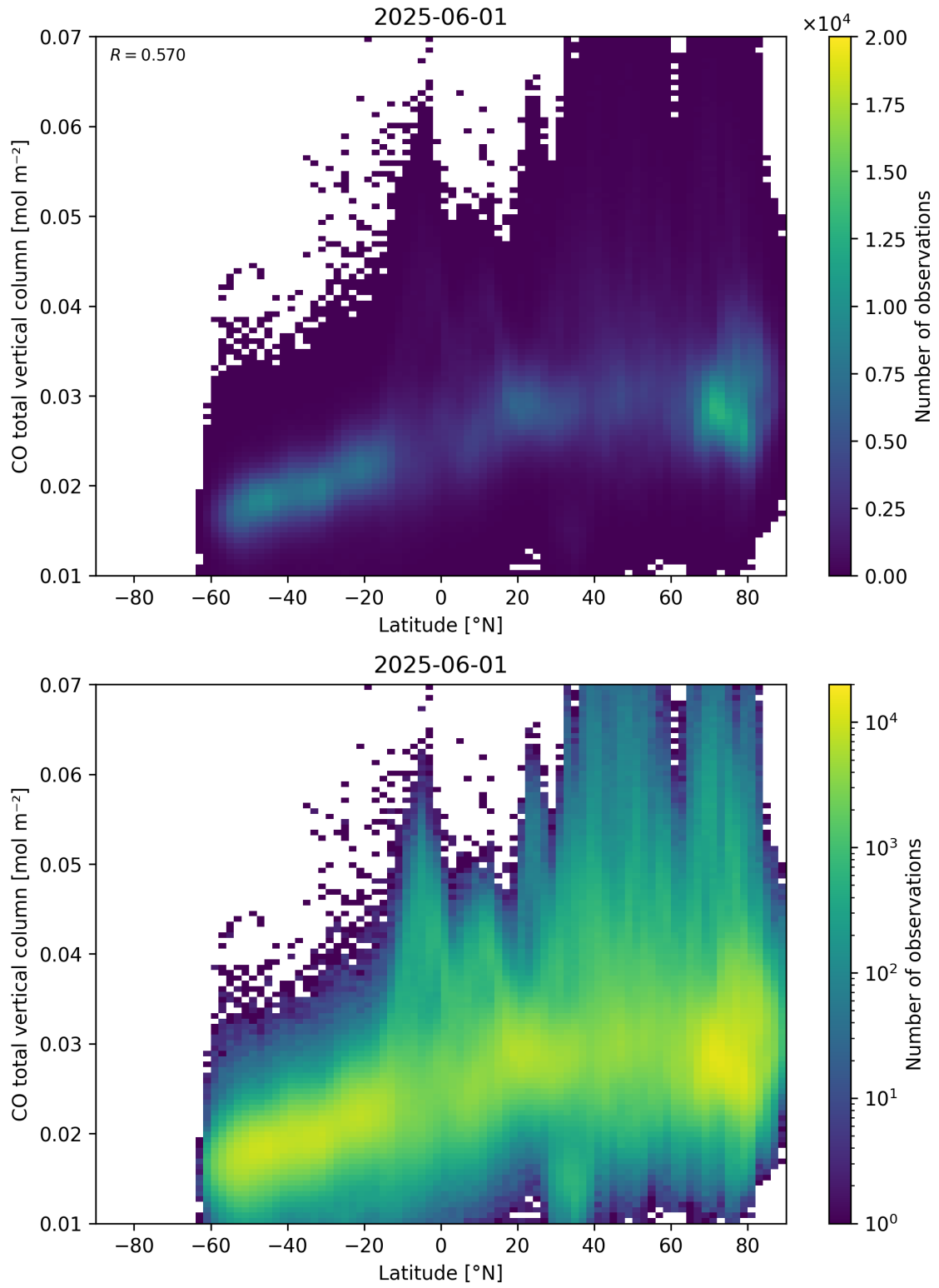
Figure 51: Scatter density plot of “Latitude” against “CO total vertical column” for 2025-06-01 to 2025-06-02.
