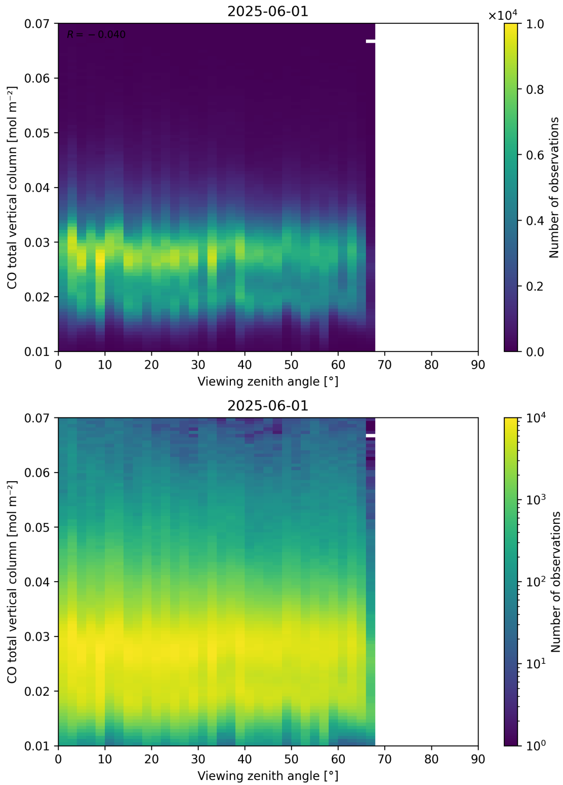
Figure 69: Scatter density plot of “Viewing zenith angle” against “CO total vertical column” for 2025-06-01 to 2025-06-02.
