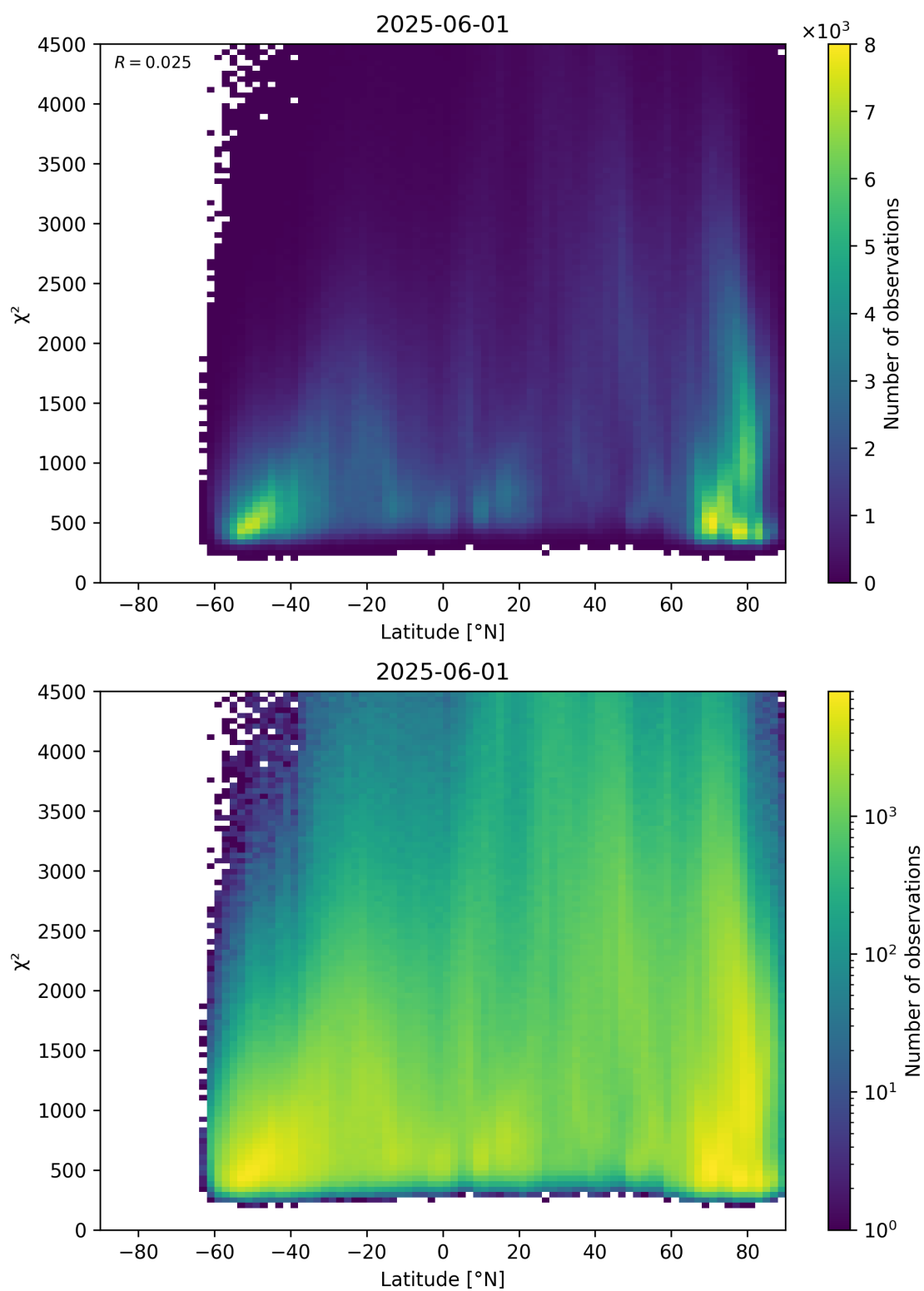
Figure 54: Scatter density plot of “Latitude” against “ \chi^2 ” for 2025-06-01 to 2025-06-02.
