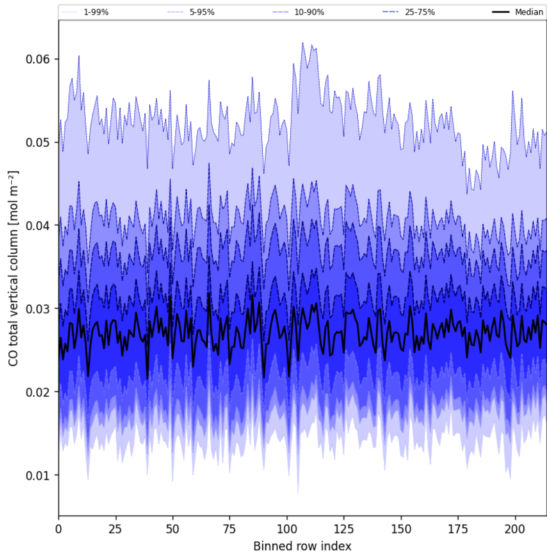
Figure 26: Along track statistics of “CO total vertical column” for 2025-06-01 to 2025-06-02
