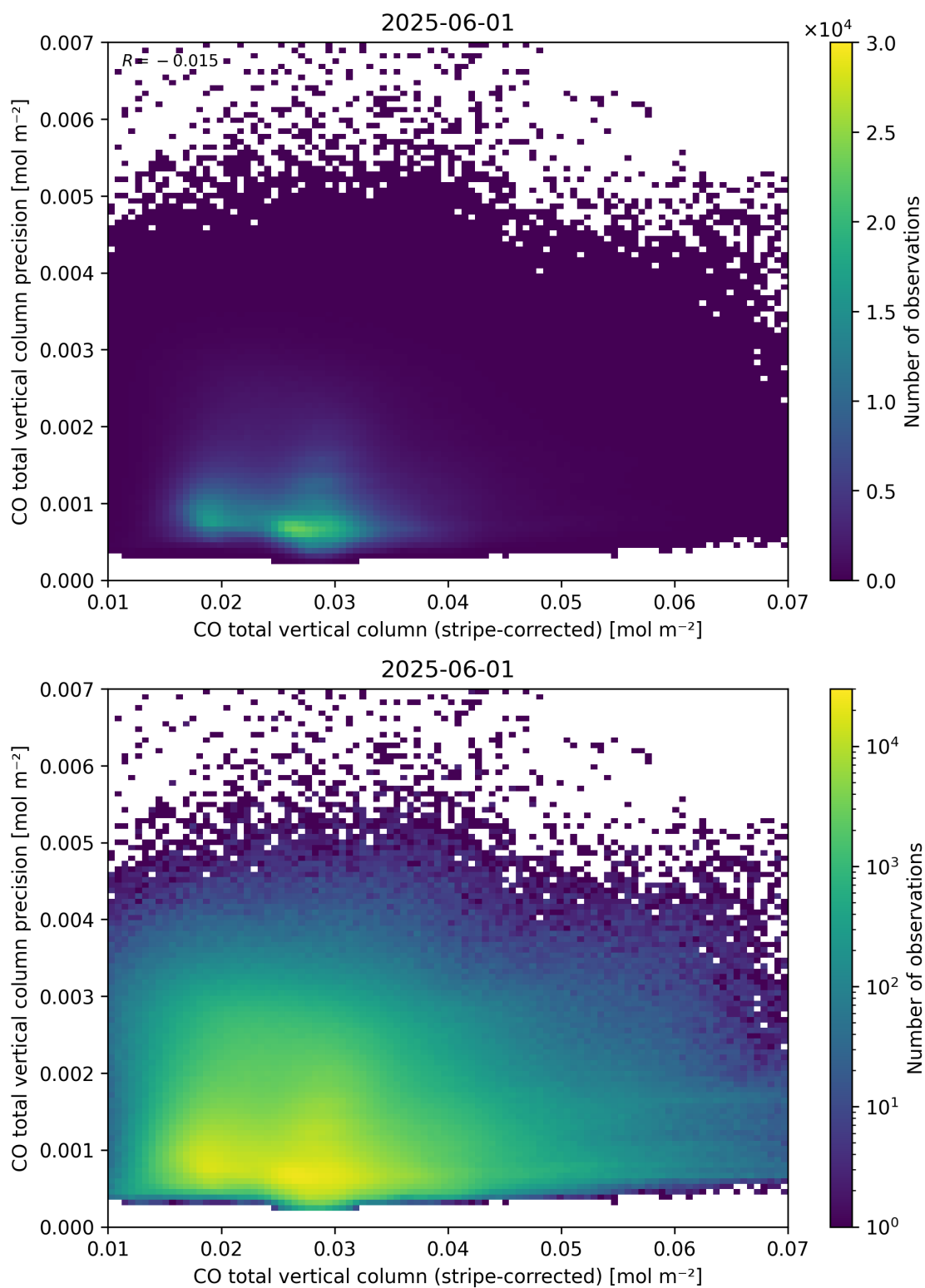
Figure 36: Scatter density plot of “CO total vertical column (stripe-corrected)” against “CO total vertical column precision” for 2025-06-01 to 2025-06-02.
