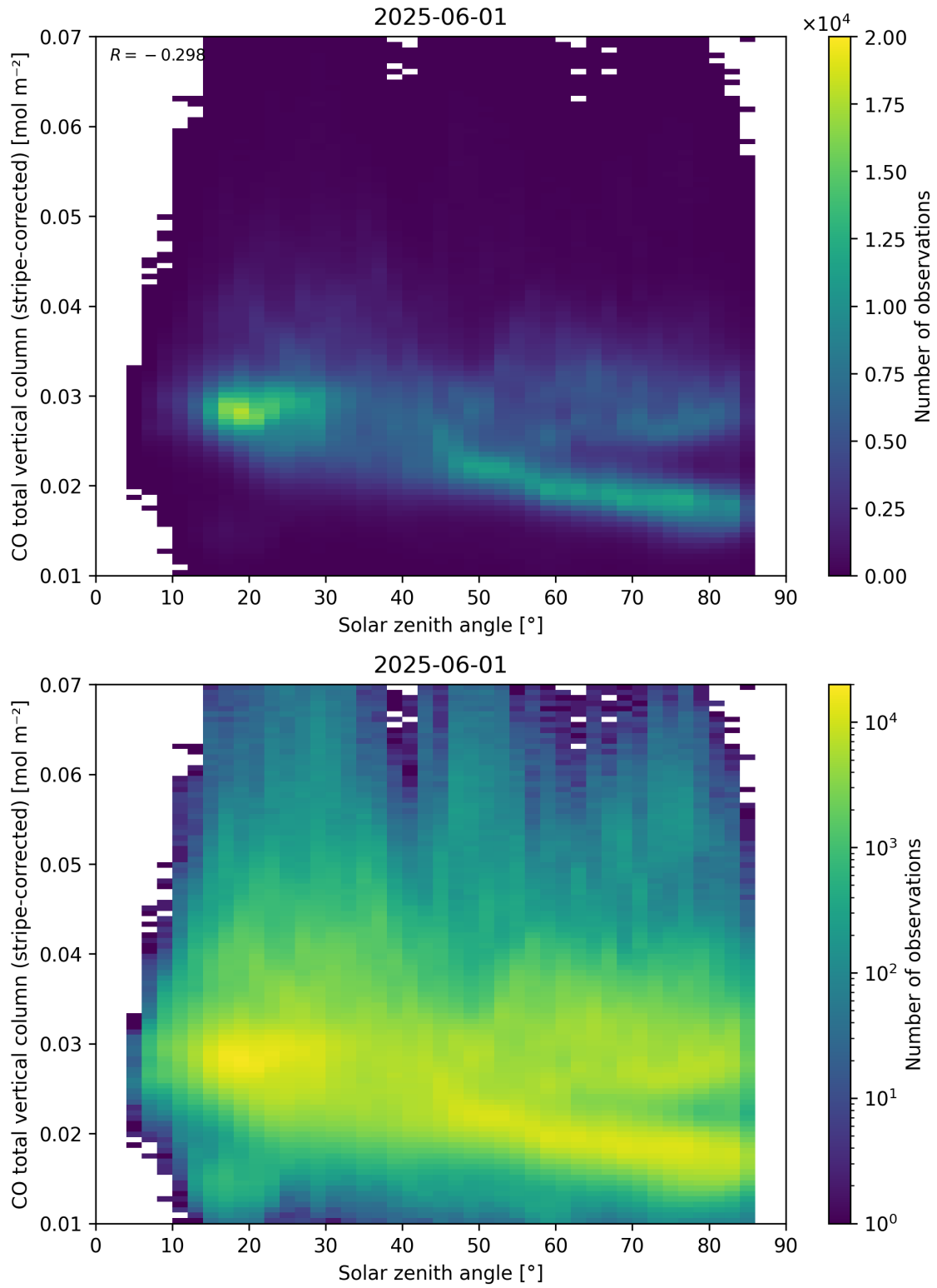
Figure 62: Scatter density plot of “Solar zenith angle” against “CO total vertical column (stripe-corrected)” for 2025-06-01 to 2025-06-02.
