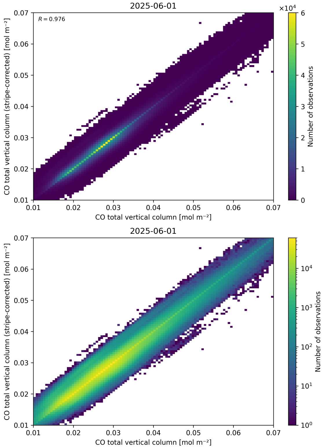
Figure 33: Scatter density plot of “CO total vertical column” against “CO total vertical column (stripe-corrected)” for 2025-06-01 to 2025-06-02.
