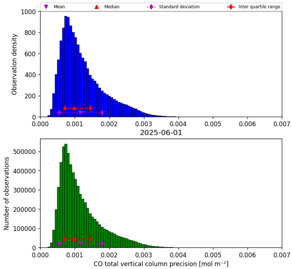
Figure 20: Histogram of “CO total vertical column precision” for 2025-06-01 to 2025-06-02
