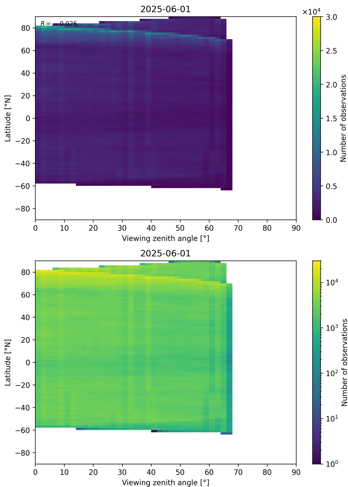
Figure 74: Scatter density plot of “Viewing zenith angle” against “Latitude” for 2025-06-01 to 2025-06-02.
