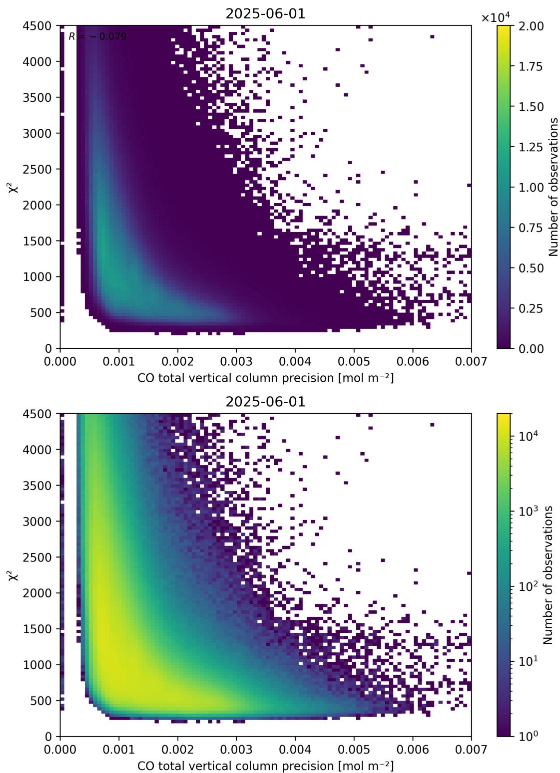
Figure 44: Scatter density plot of “CO total vertical column precision” against “ \chi^2 ” for 2025-06-01 to 2025-06-02.
