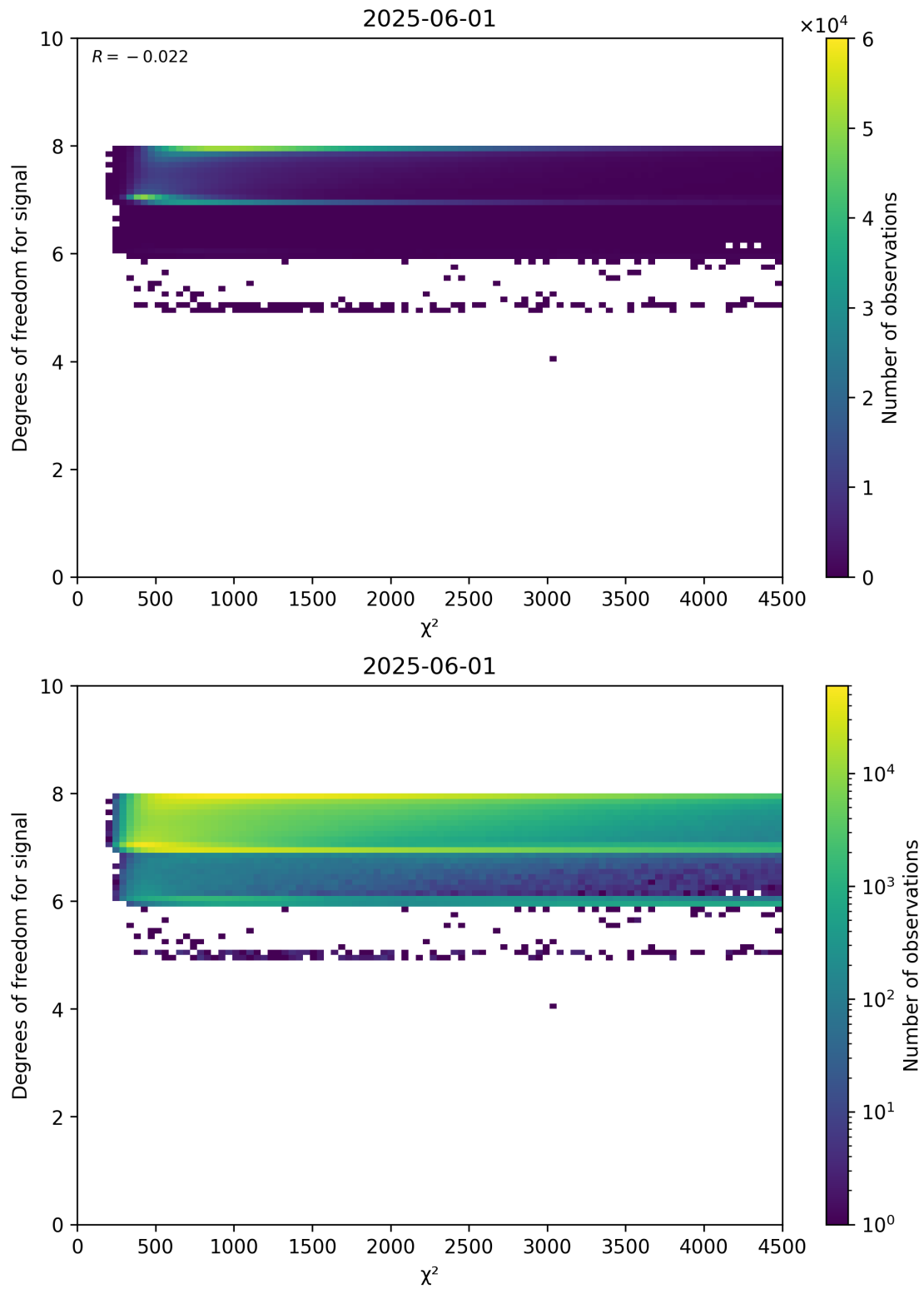
Figure 48: Scatter density plot of “ \chi^2 ” against “Degrees of freedom for signal” for 2025-06-01 to 2025-06-02.
