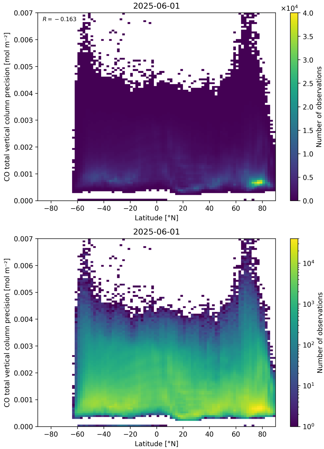
Figure 53: Scatter density plot of “Latitude” against “CO total vertical column precision” for 2025-06-01 to 2025-06-02.
