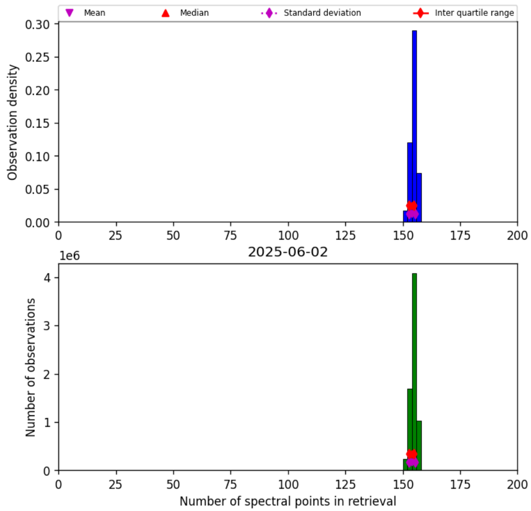
Figure 21: Histogram of “Number of spectral points in retrieval” for 2025-06-01 to 2025-06-03
