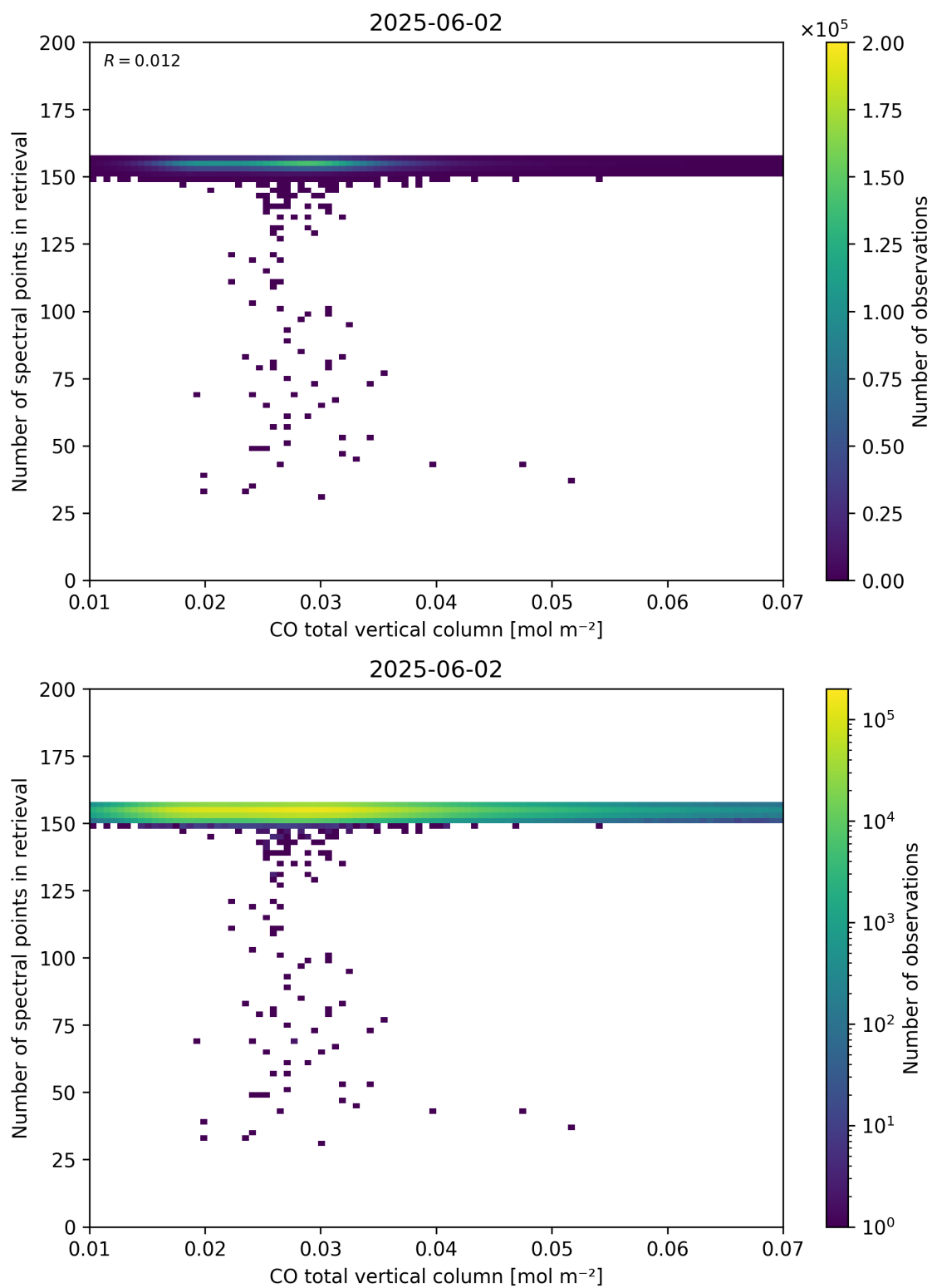
Figure 43: Scatter density plot of “CO total vertical column” against “Number of spectral points in retrieval” for 2025-06-01 to 2025-06-03.
