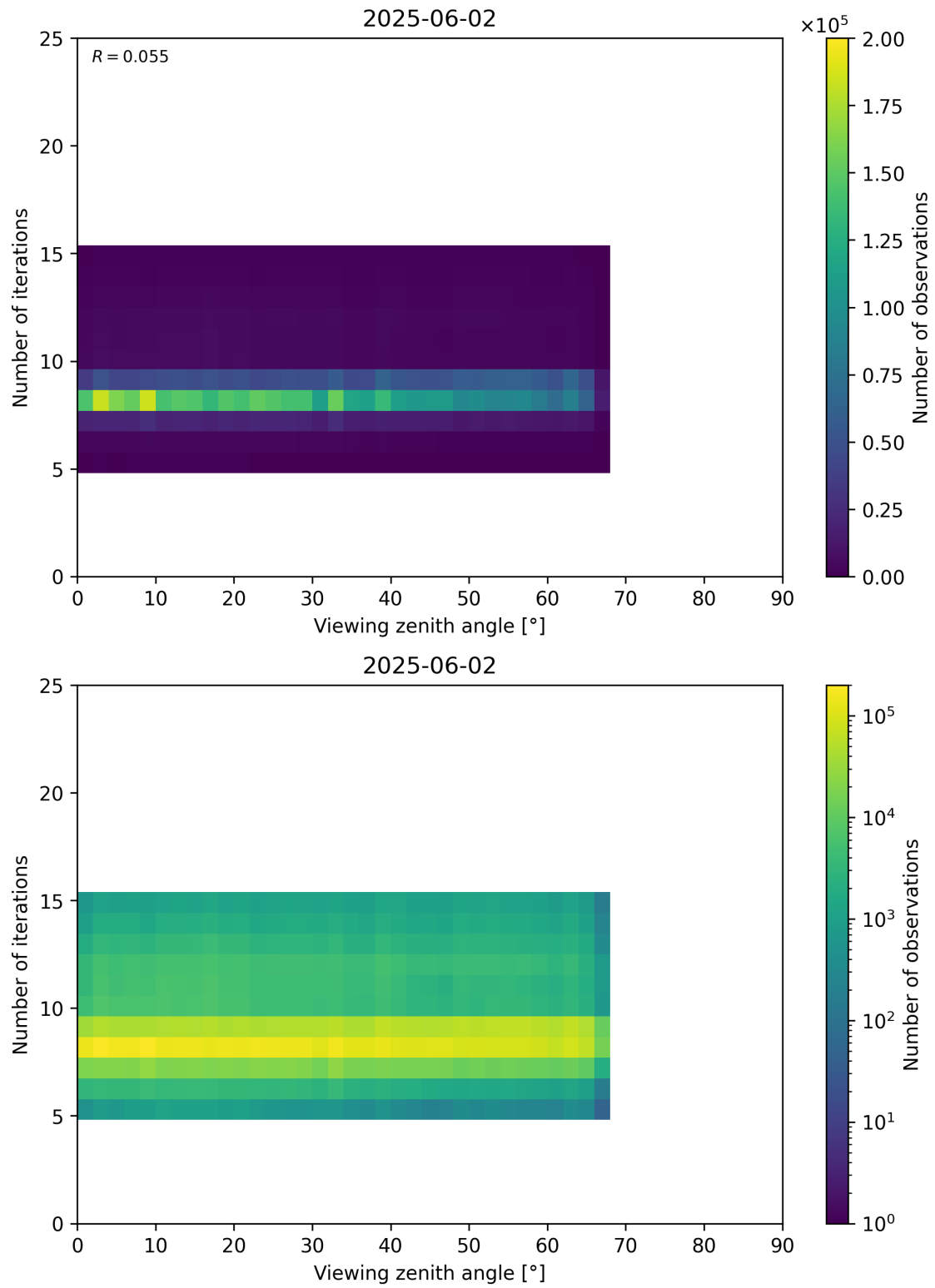
Figure 75: Scatter density plot of “Viewing zenith angle” against “Number of iterations” for 2025-06-01 to 2025-06-03.
