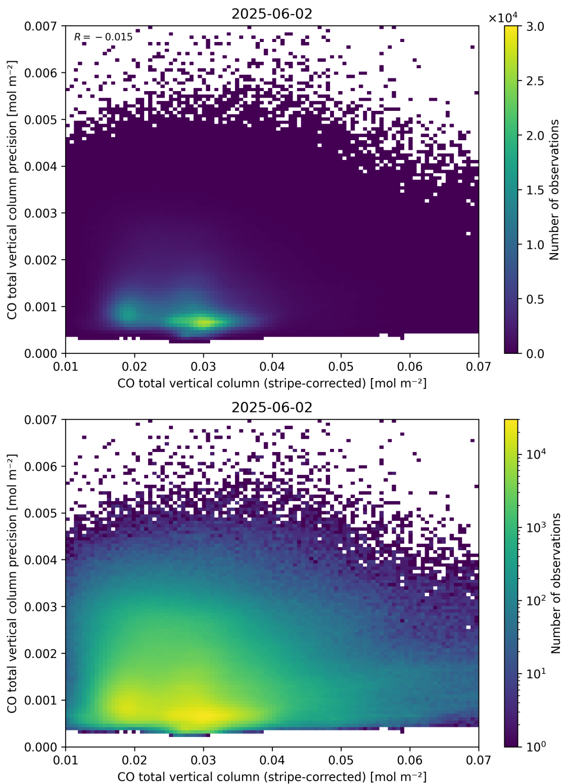
Figure 36: Scatter density plot of “CO total vertical column (stripe-corrected)” against “CO total vertical column precision” for 2025-06-01 to 2025-06-03.
