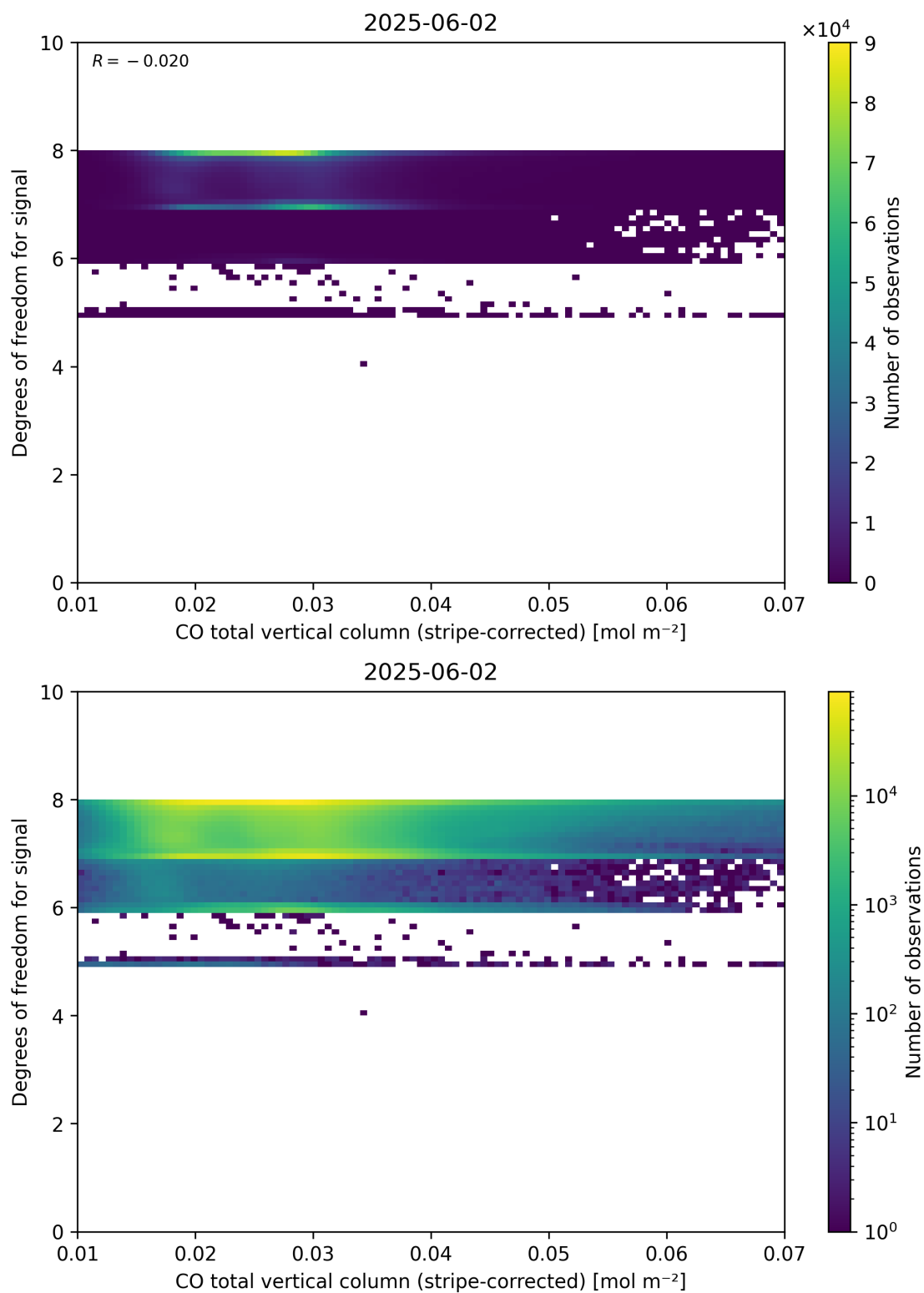
Figure 38: Scatter density plot of “CO total vertical column (stripe-corrected)” against “Degrees of freedom for signal” for 2025-06-01 to 2025-06-03.
