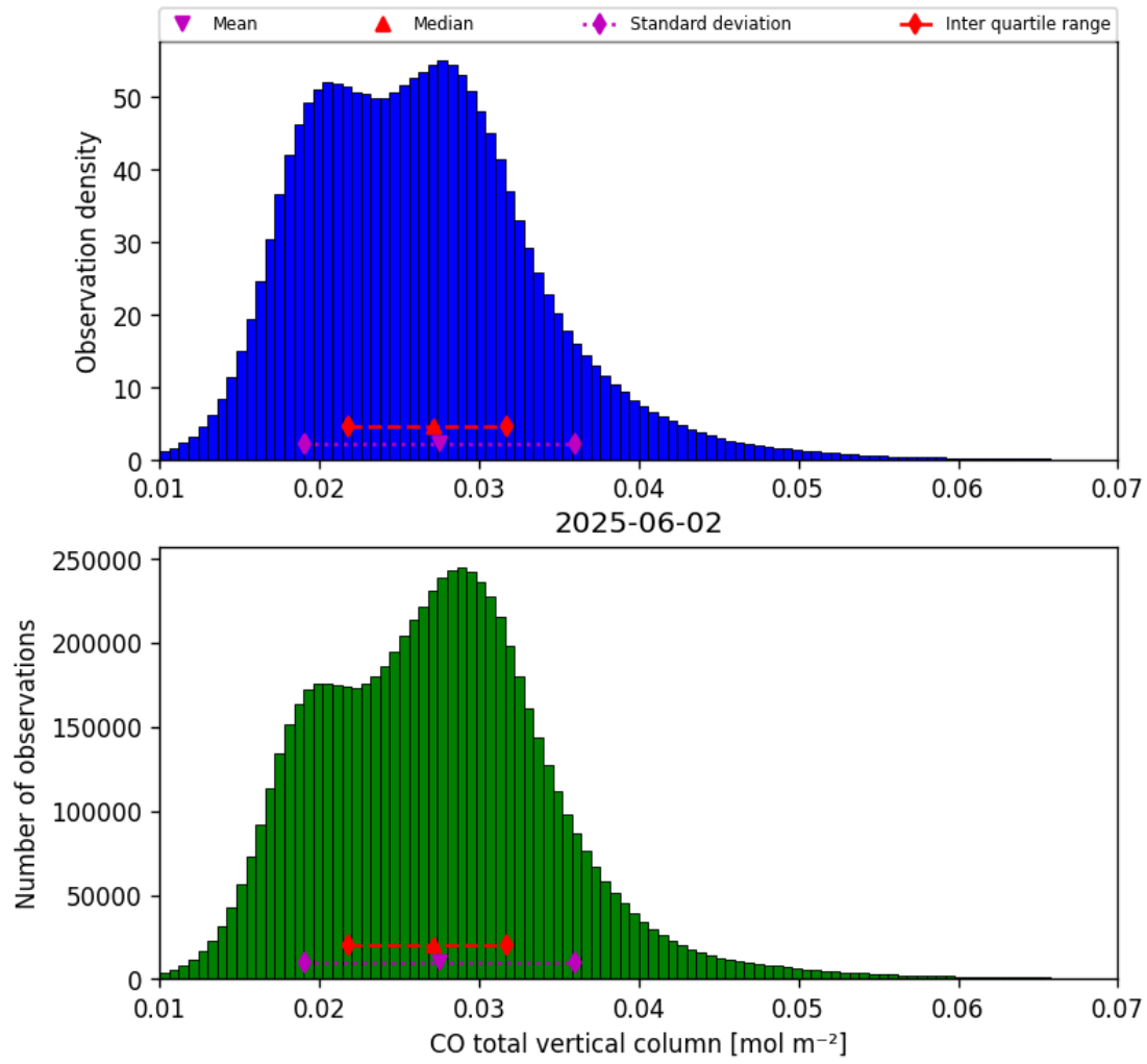
Figure 18: Histogram of “CO total vertical column” for 2025-06-01 to 2025-06-03
