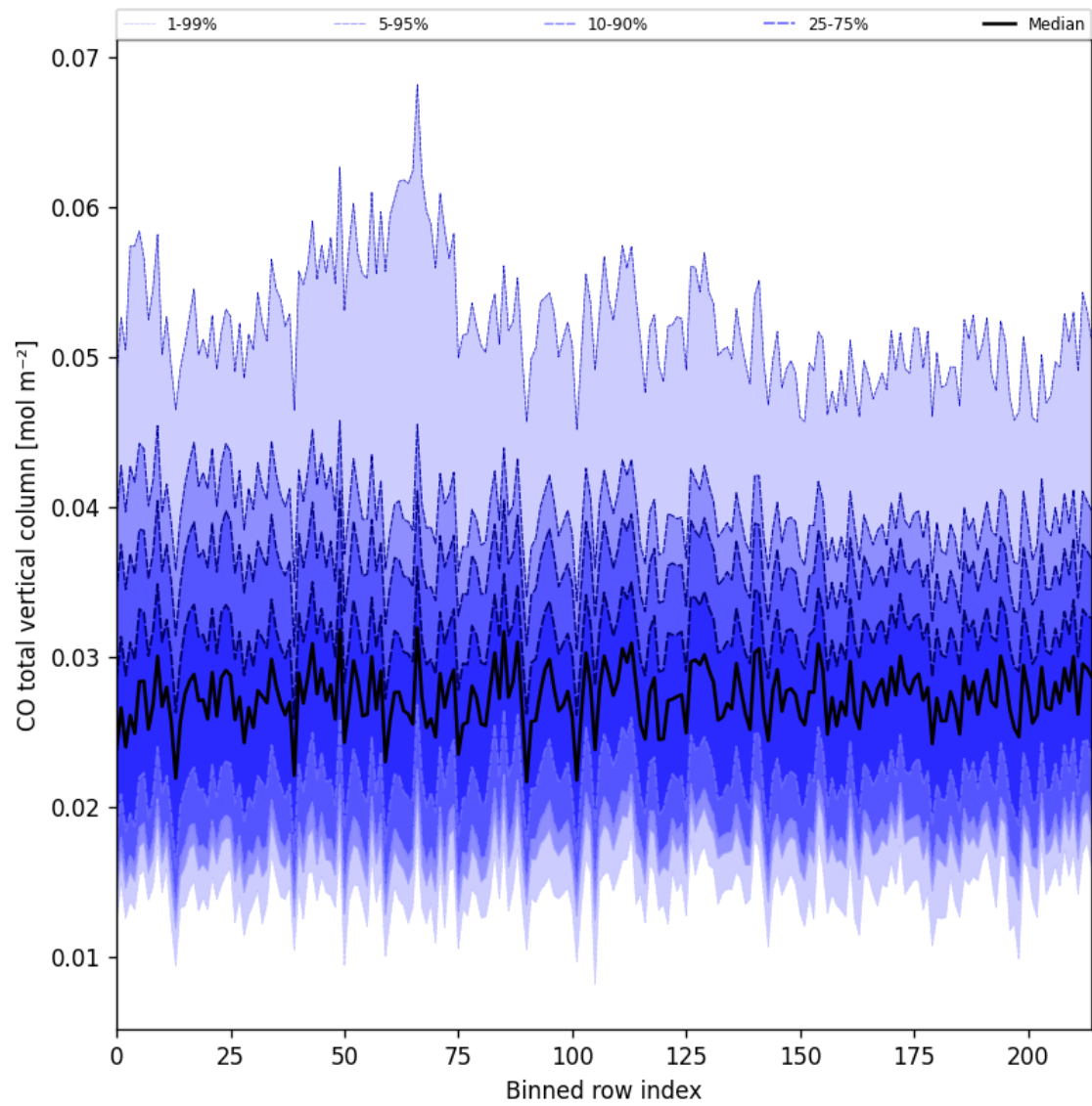
Figure 26: Along track statistics of “CO total vertical column” for 2025-06-01 to 2025-06-03
