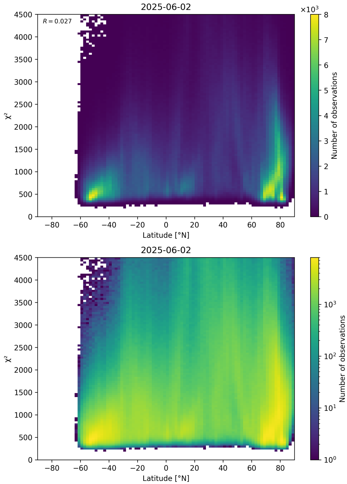
Figure 54: Scatter density plot of “Latitude” against “ \chi^2 ” for 2025-06-01 to 2025-06-03.
