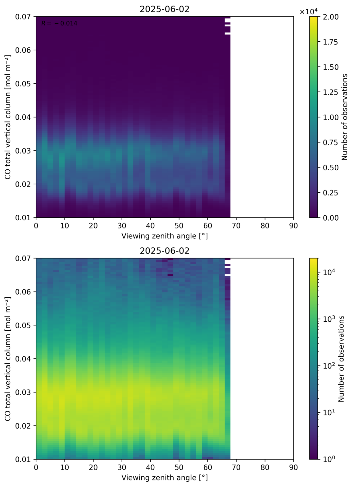
Figure 69: Scatter density plot of “Viewing zenith angle” against “CO total vertical column” for 2025-06-01 to 2025-06-03.
