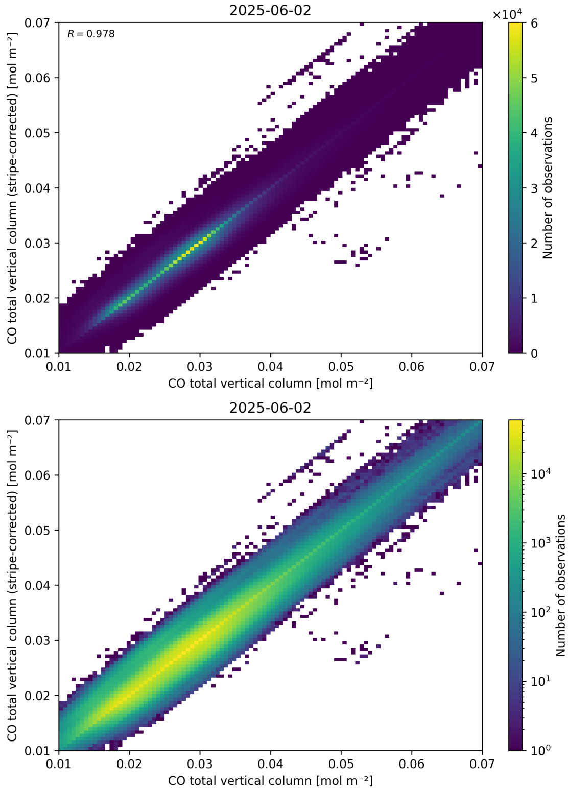
Figure 33: Scatter density plot of “CO total vertical column” against “CO total vertical column (stripe-corrected)” for 2025-06-01 to 2025-06-03.
