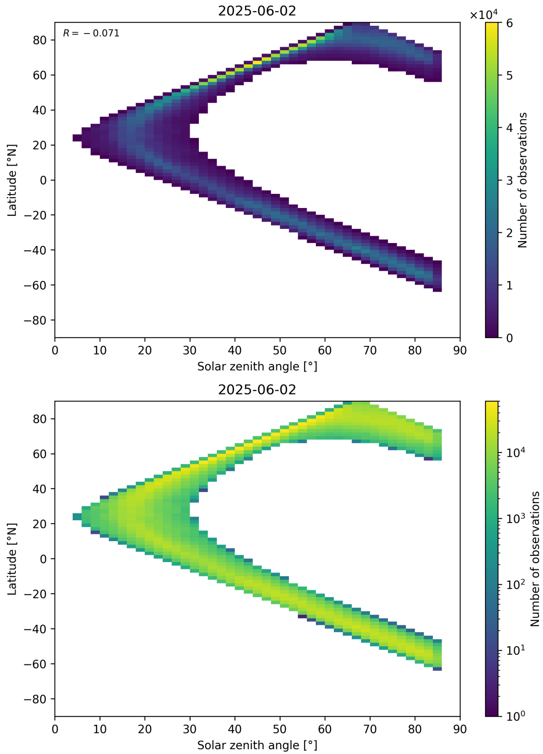
Figure 66: Scatter density plot of “Solar zenith angle” against “Latitude” for 2025-06-01 to 2025-06-03.
