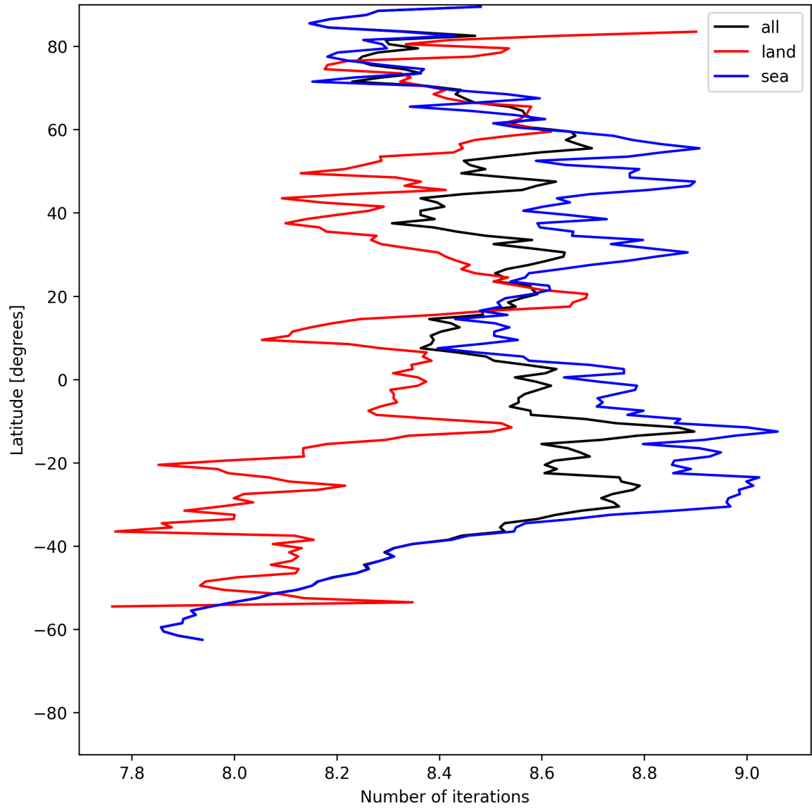
Figure 16: Zonal average of “Number of iterations” for 2025-06-01 to 2025-06-03.
