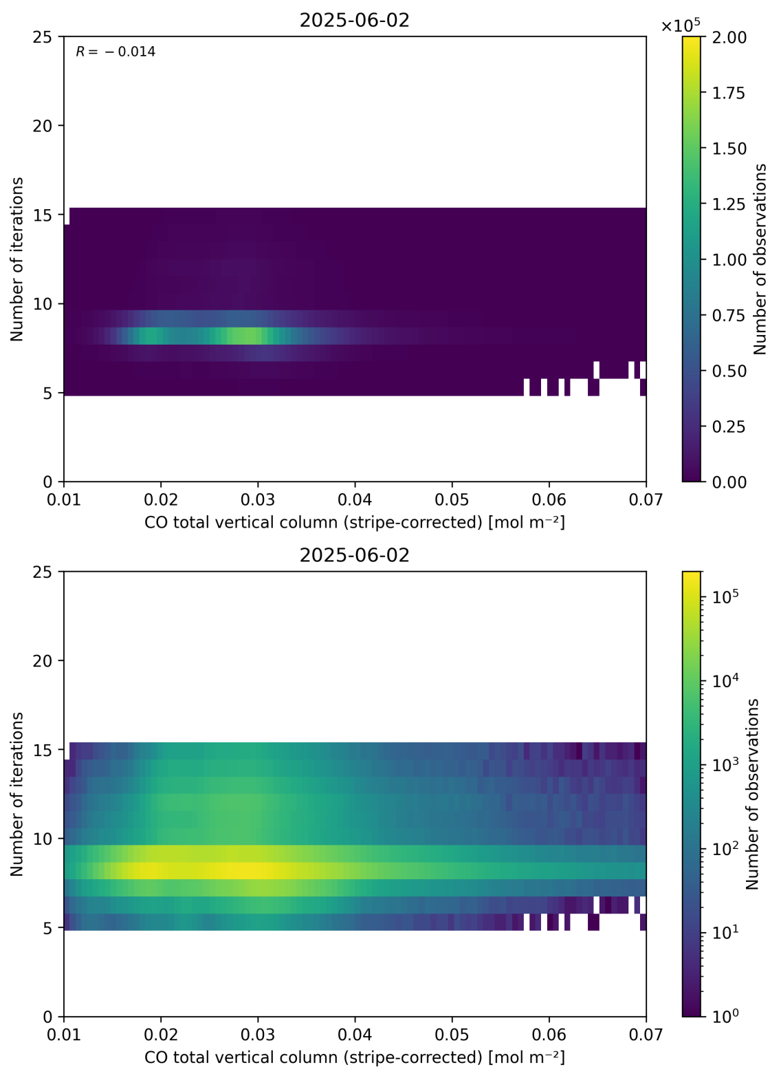
Figure 39: Scatter density plot of “CO total vertical column (stripe-corrected)” against “Number of iterations” for 2025-06-01 to 2025-06-03.
