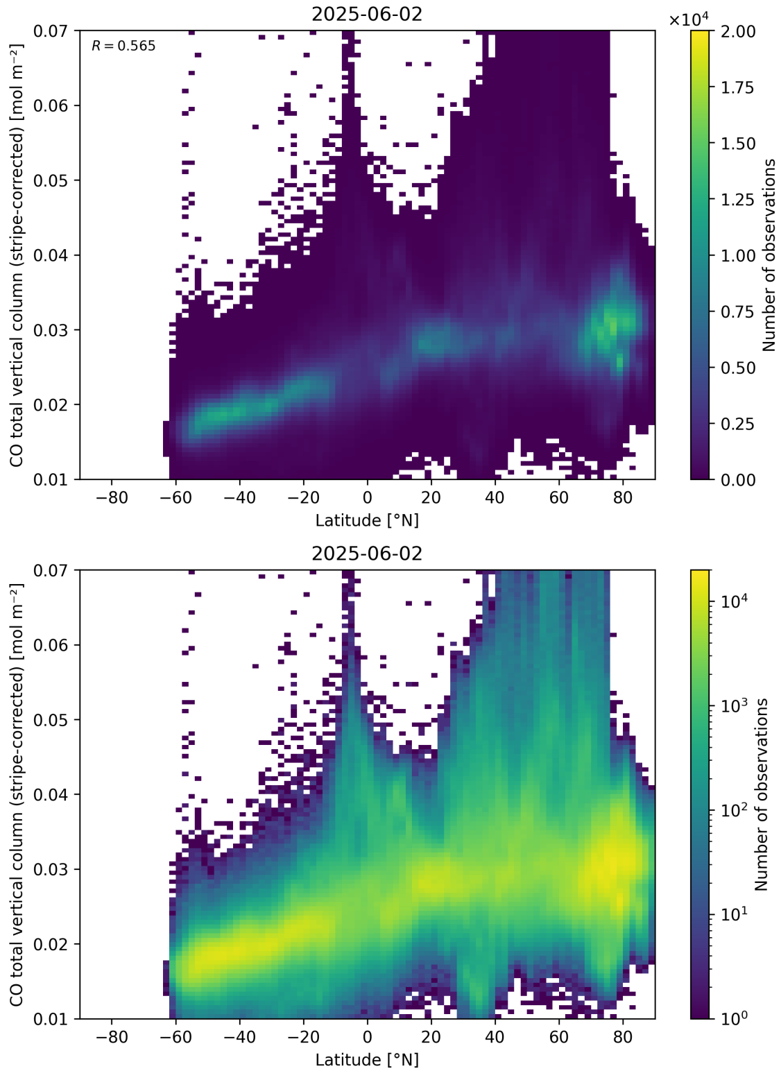
Figure 52: Scatter density plot of “Latitude” against “CO total vertical column (stripe-corrected)” for 2025-06-01 to 2025-06-03.
