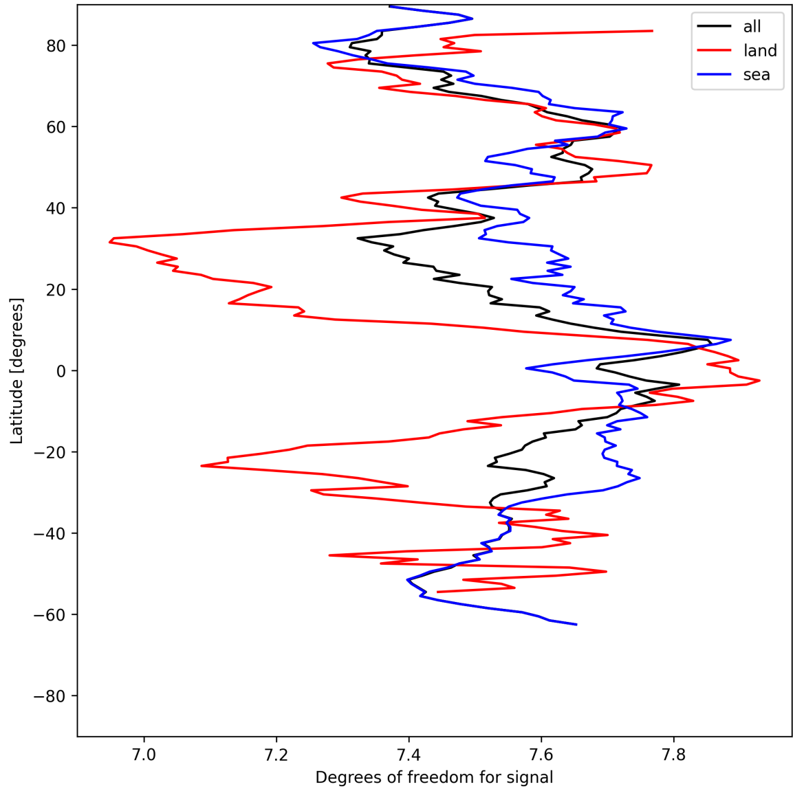
Figure 15: Zonal average of “Degrees of freedom for signal” for 2025-06-01 to 2025-06-03.
