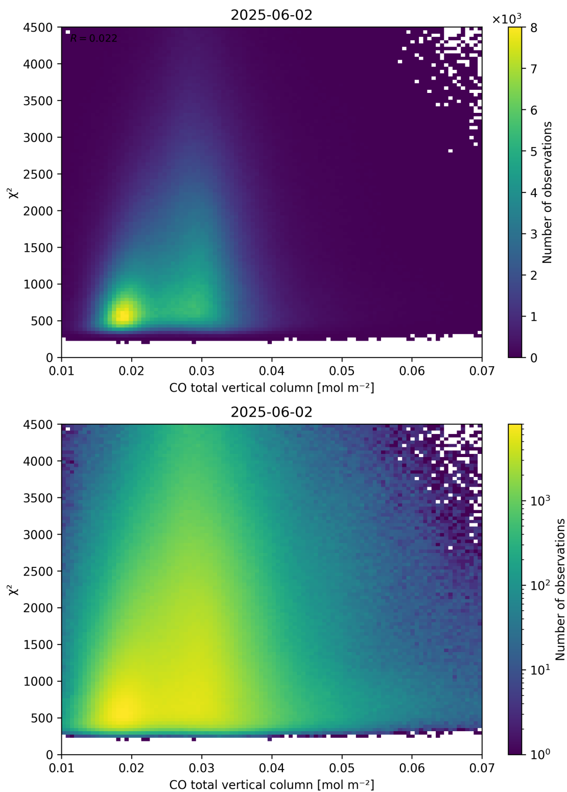
Figure 35: Scatter density plot of “CO total vertical column” against “ \chi^2 ” for 2025-06-01 to 2025-06-03.
