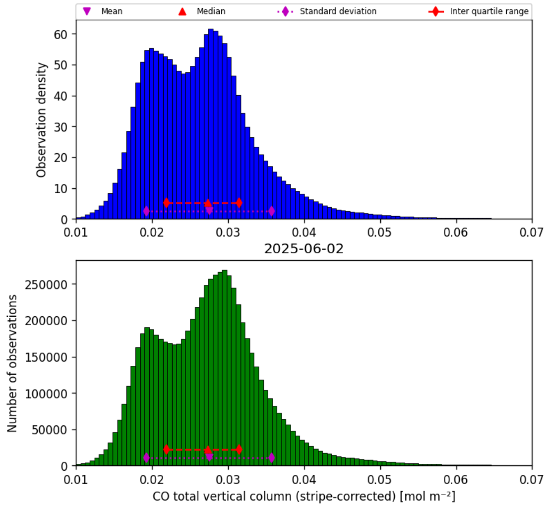
Figure 19: Histogram of “CO total vertical column (stripe-corrected)” for 2025-06-01 to 2025-06-03
