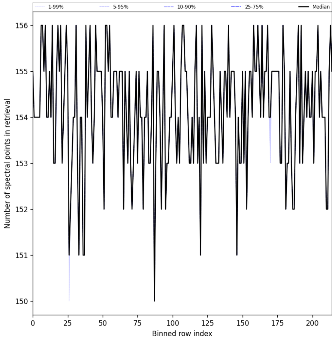
Figure 29: Along track statistics of “Number of spectral points in retrieval” for 2025-06-01 to 2025-06-03
