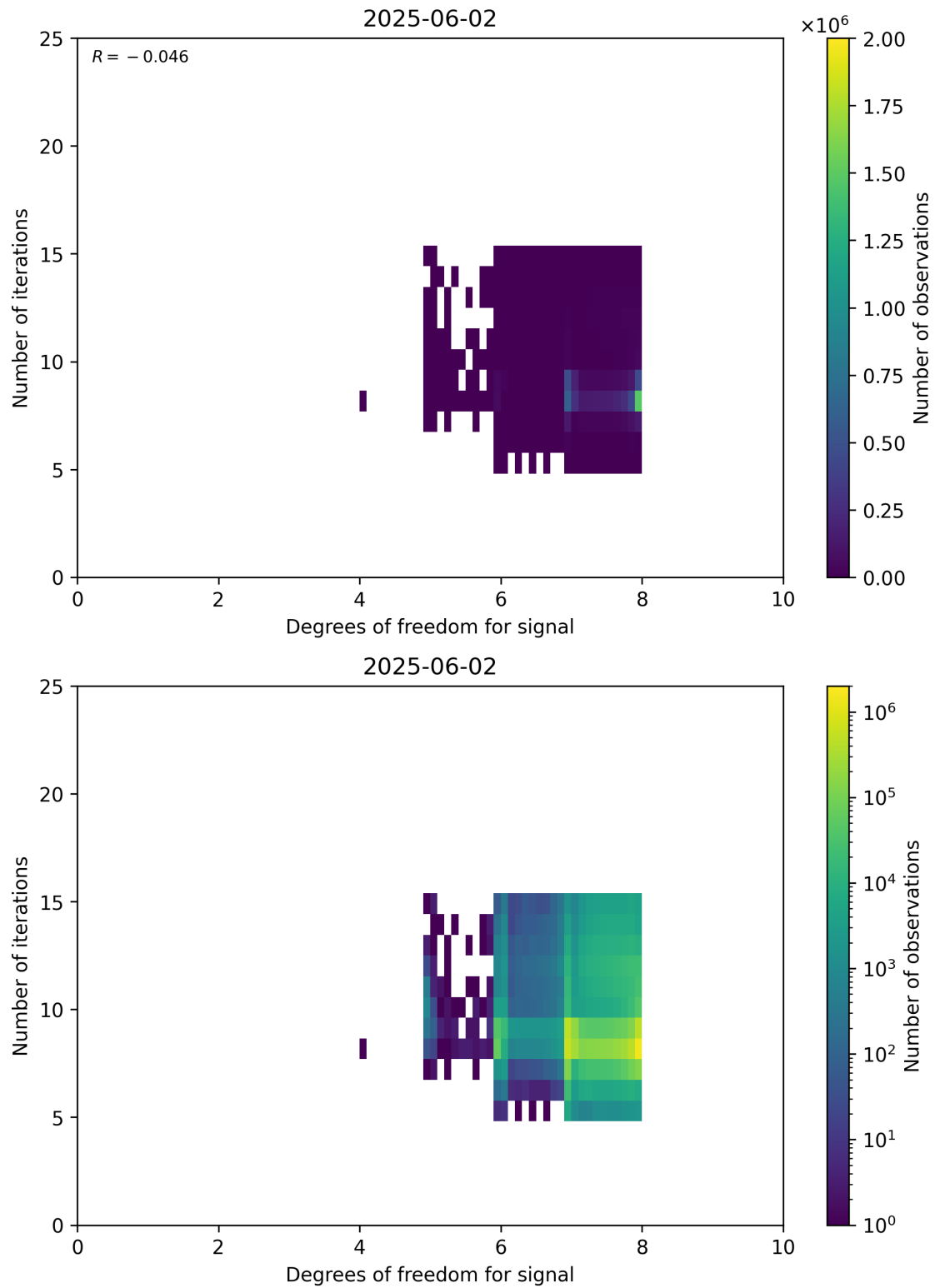
Figure 50: Scatter density plot of “Degrees of freedom for signal” against “Number of iterations” for 2025-06-01 to 2025-06-03.
