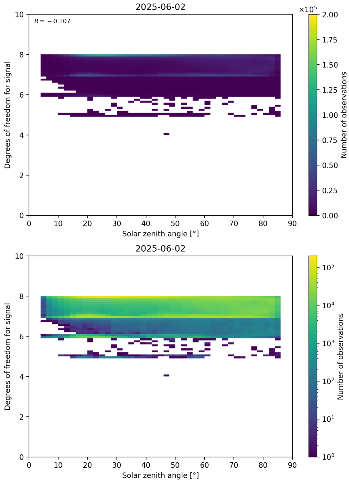
Figure 65: Scatter density plot of “Solar zenith angle” against “Degrees of freedom for signal” for 2025-06-01 to 2025-06-03.
