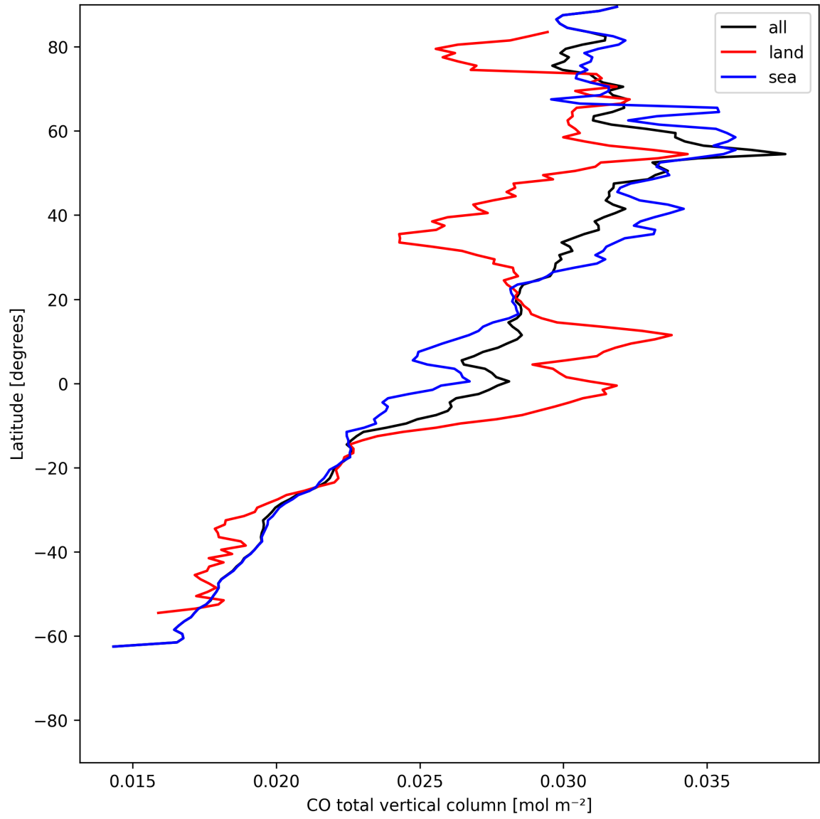
Figure 10: Zonal average of “CO total vertical column” for 2025-06-01 to 2025-06-03.
