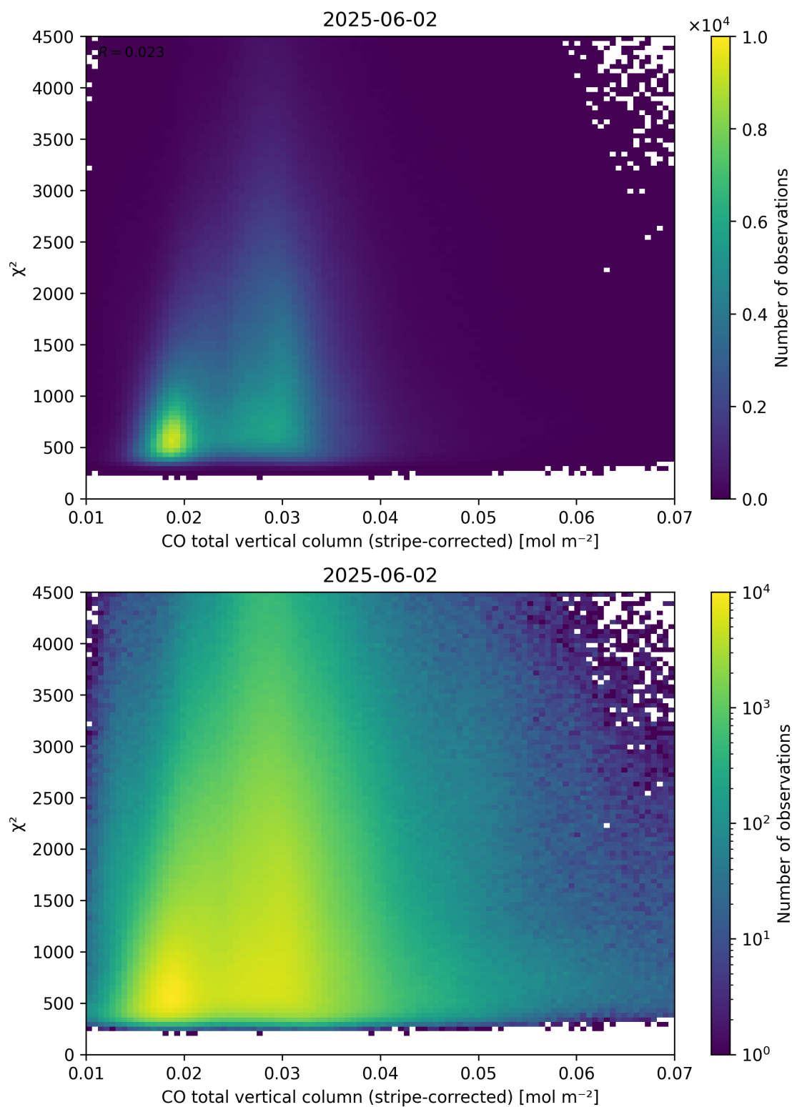
Figure 37: Scatter density plot of “CO total vertical column (stripe-corrected)” against “ \chi^2 ” for 2025-06-01 to 2025-06-03.
