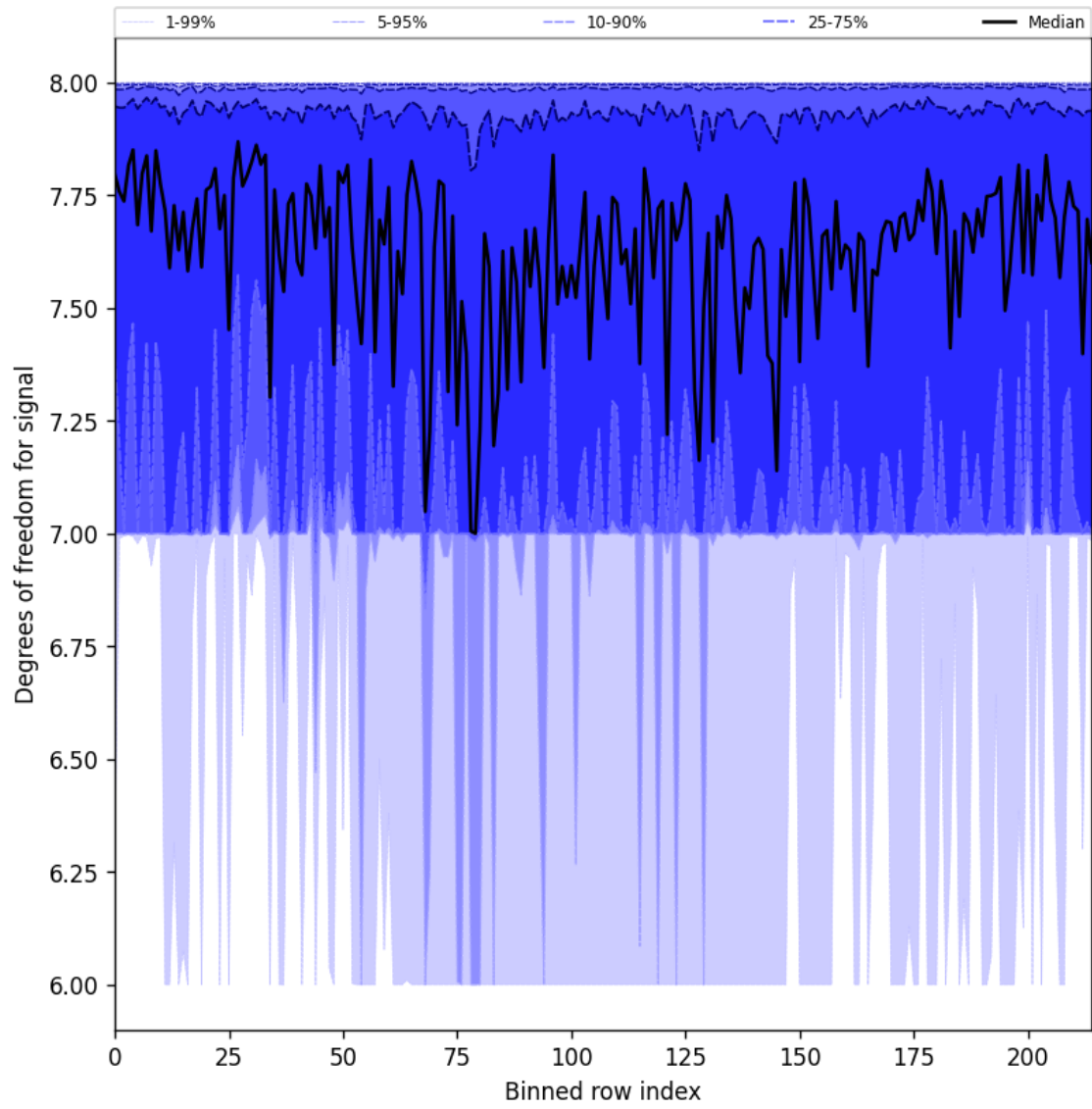
Figure 31: Along track statistics of “Degrees of freedom for signal” for 2025-06-01 to 2025-06-03
