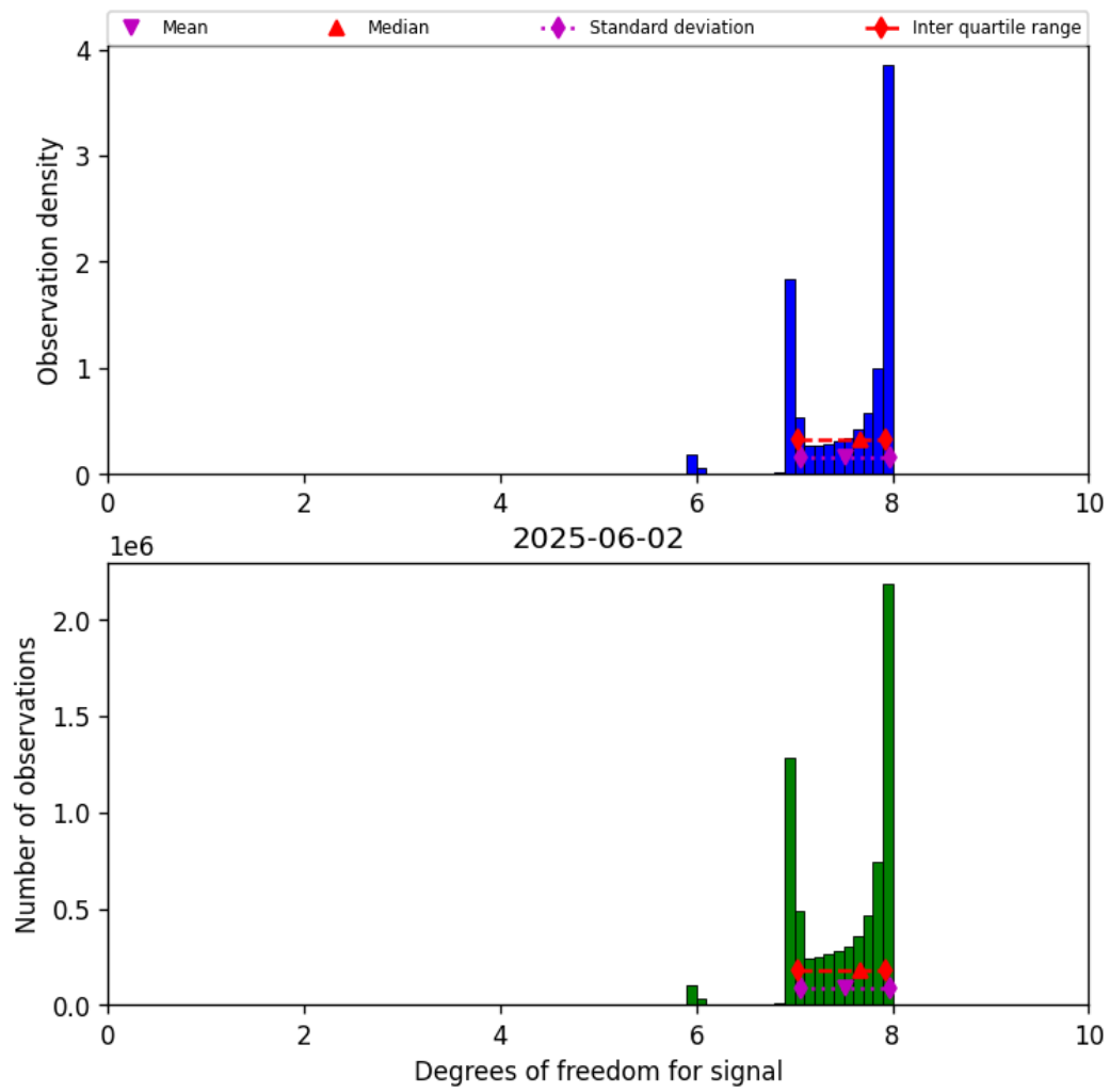
Figure 23: Histogram of “Degrees of freedom for signal” for 2025-06-01 to 2025-06-03
