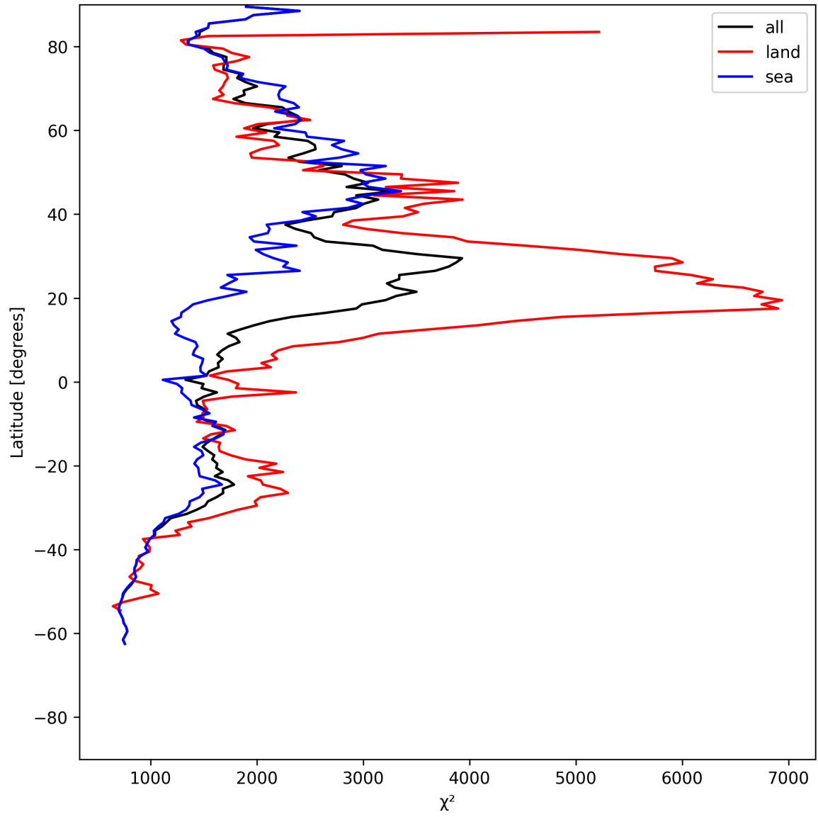
Figure 14: Zonal average of “ \chi^2 ” for 2025-06-01 to 2025-06-03.
