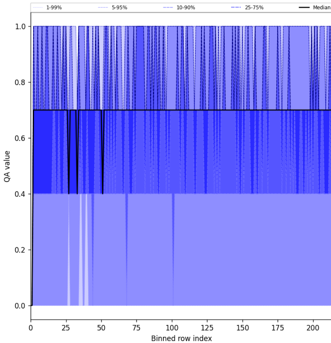
Figure 25: Along track statistics of “QA value” for 2025-06-01 to 2025-06-03
