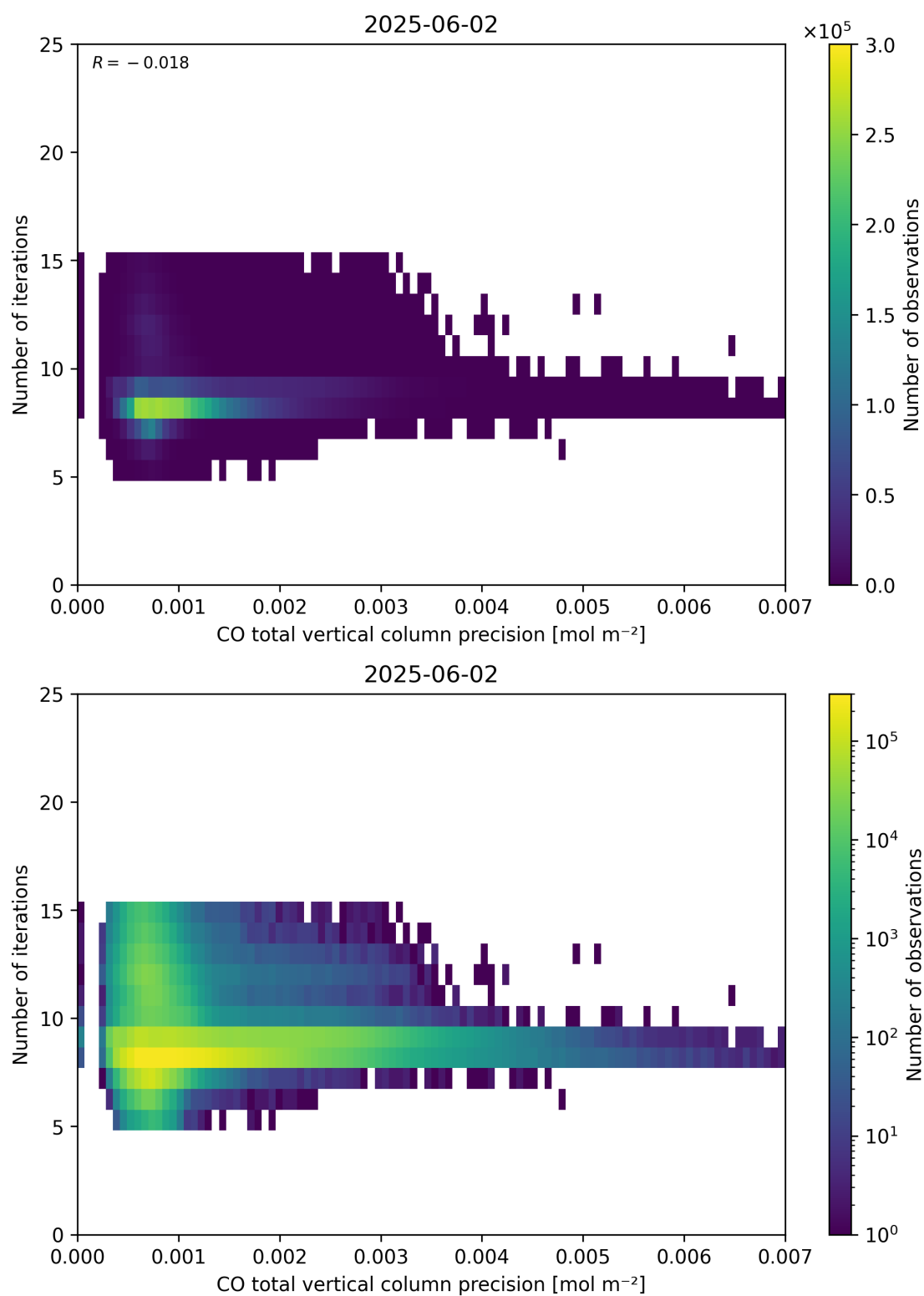
Figure 46: Scatter density plot of “CO total vertical column precision” against “Number of iterations” for 2025-06-01 to 2025-06-03.
