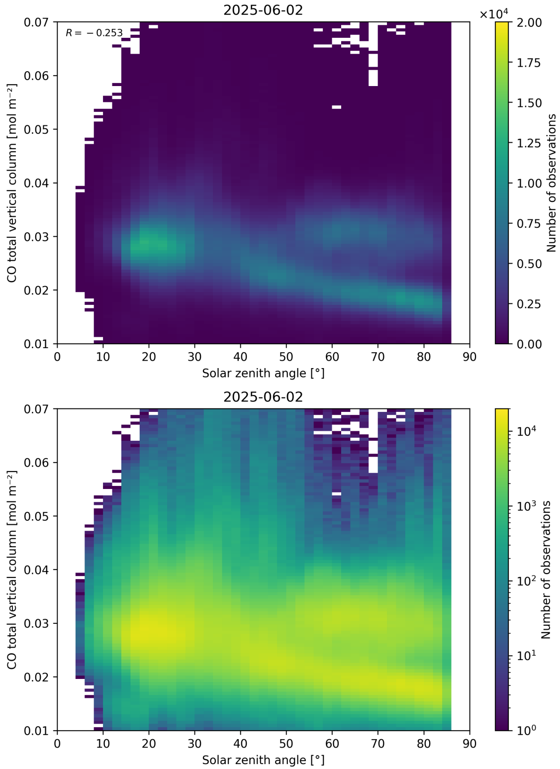
Figure 61: Scatter density plot of “Solar zenith angle” against “CO total vertical column” for 2025-06-01 to 2025-06-03.
