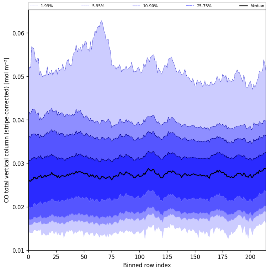
Figure 27: Along track statistics of “CO total vertical column (stripe-corrected)” for 2025-06-01 to 2025-06-03
