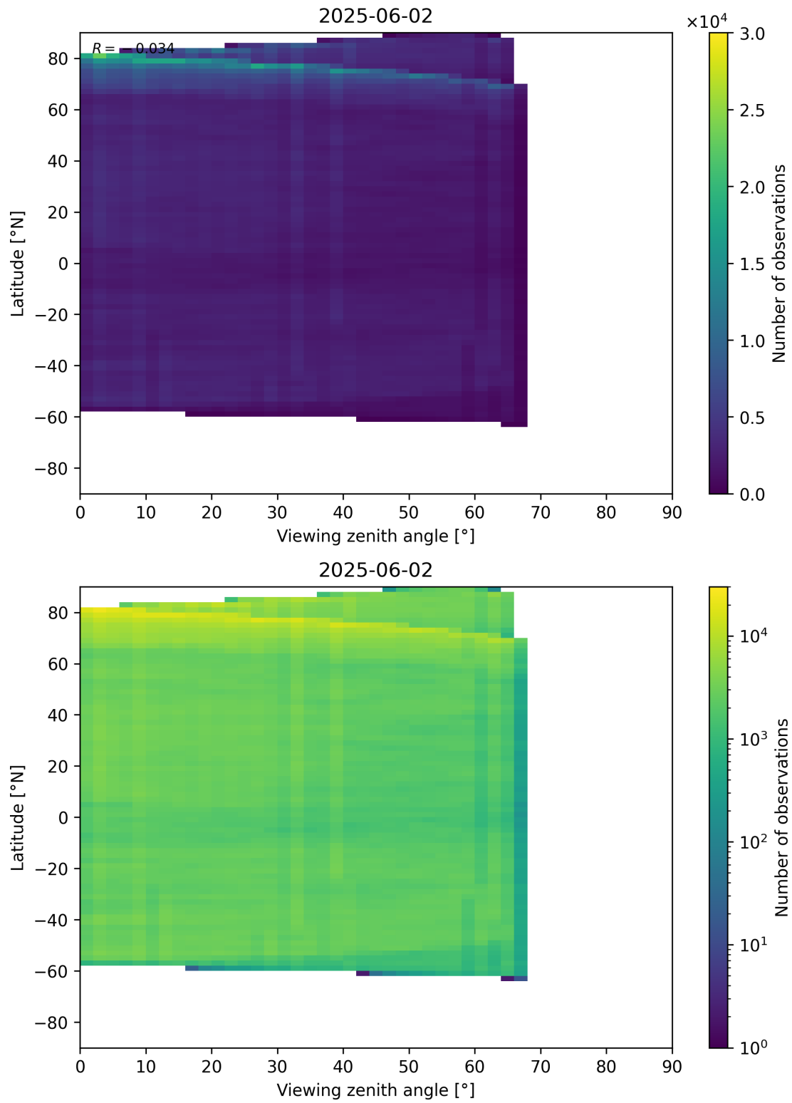
Figure 74: Scatter density plot of “Viewing zenith angle” against “Latitude” for 2025-06-01 to 2025-06-03.
