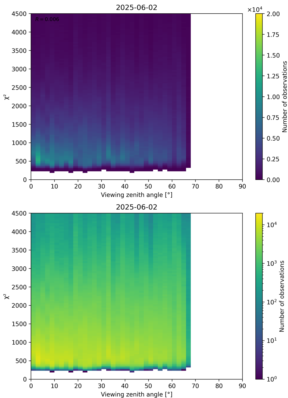
Figure 72: Scatter density plot of “Viewing zenith angle” against “ \chi^2 ” for 2025-06-01 to 2025-06-03.
