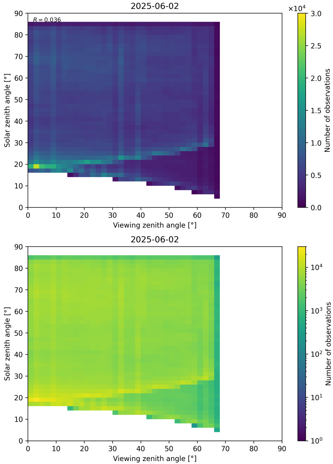
Figure 77: Scatter density plot of “Viewing zenith angle” against “Solar zenith angle” for 2025-06-01 to 2025-06-03.
