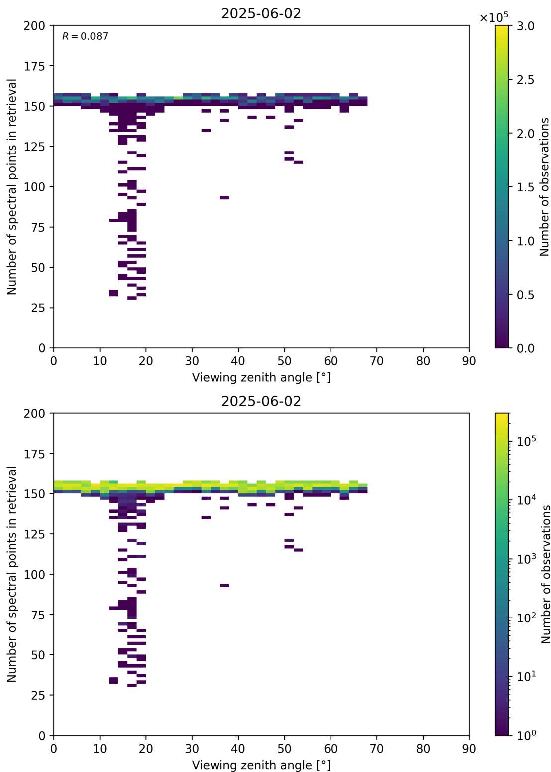
Figure 76: Scatter density plot of “Viewing zenith angle” against “Number of spectral points in retrieval” for 2025-06-01 to 2025-06-03.
