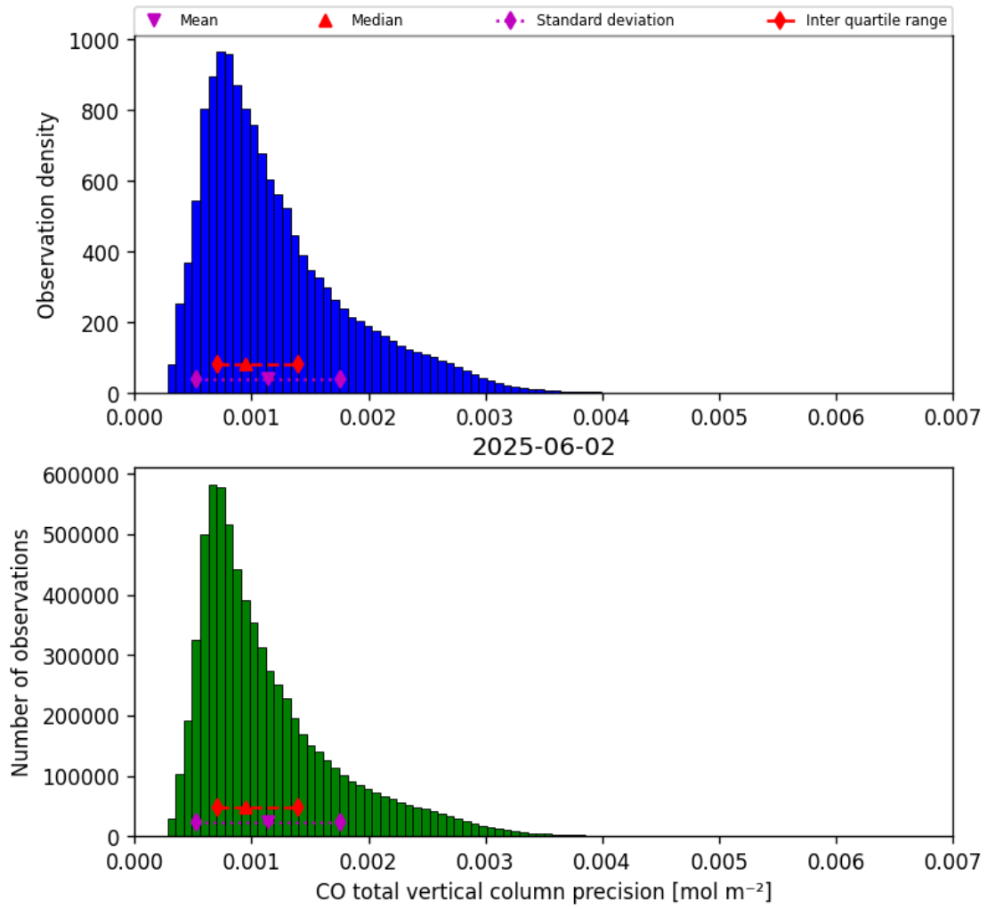
Figure 20: Histogram of “CO total vertical column precision” for 2025-06-01 to 2025-06-03
