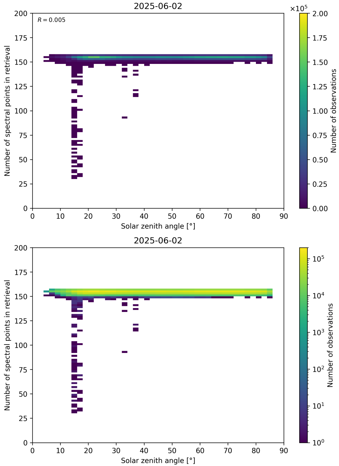
Figure 68: Scatter density plot of “Solar zenith angle” against “Number of spectral points in retrieval” for 2025-06-01 to 2025-06-03.
