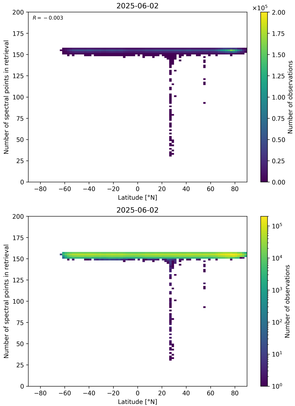
Figure 57: Scatter density plot of “Latitude” against “Number of spectral points in retrieval” for 2025-06-01 to 2025-06-03.
