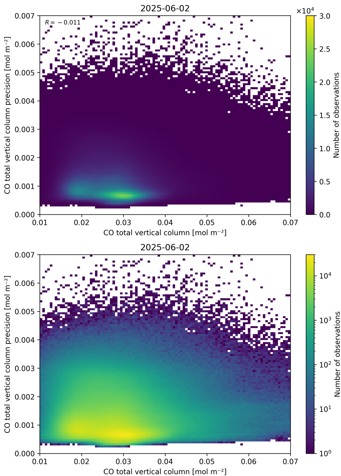
Figure 34: Scatter density plot of “CO total vertical column” against “CO total vertical column precision” for 2025-06-01 to 2025-06-03.
