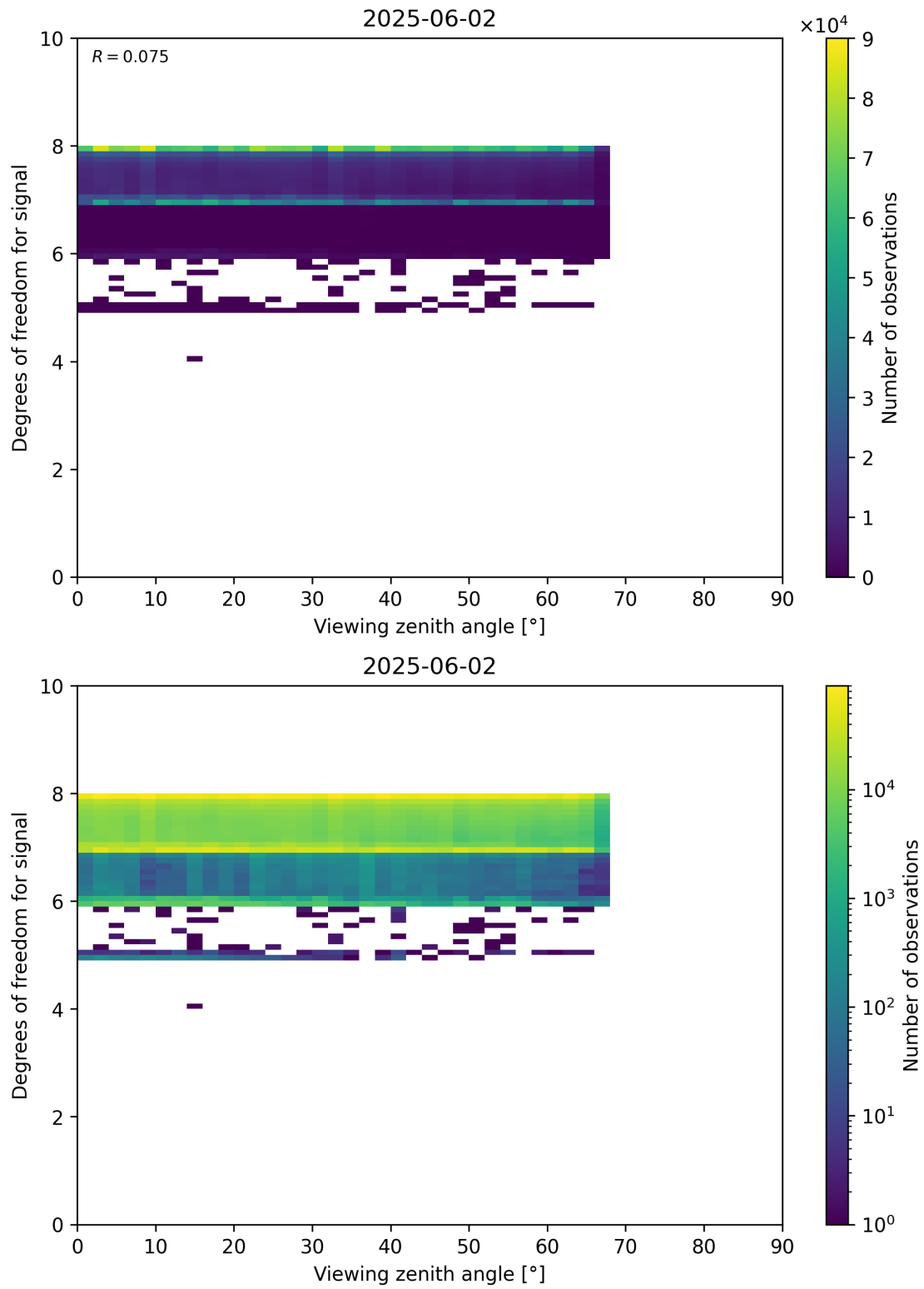
Figure 73: Scatter density plot of “Viewing zenith angle” against “Degrees of freedom for signal” for 2025-06-01 to 2025-06-03.
