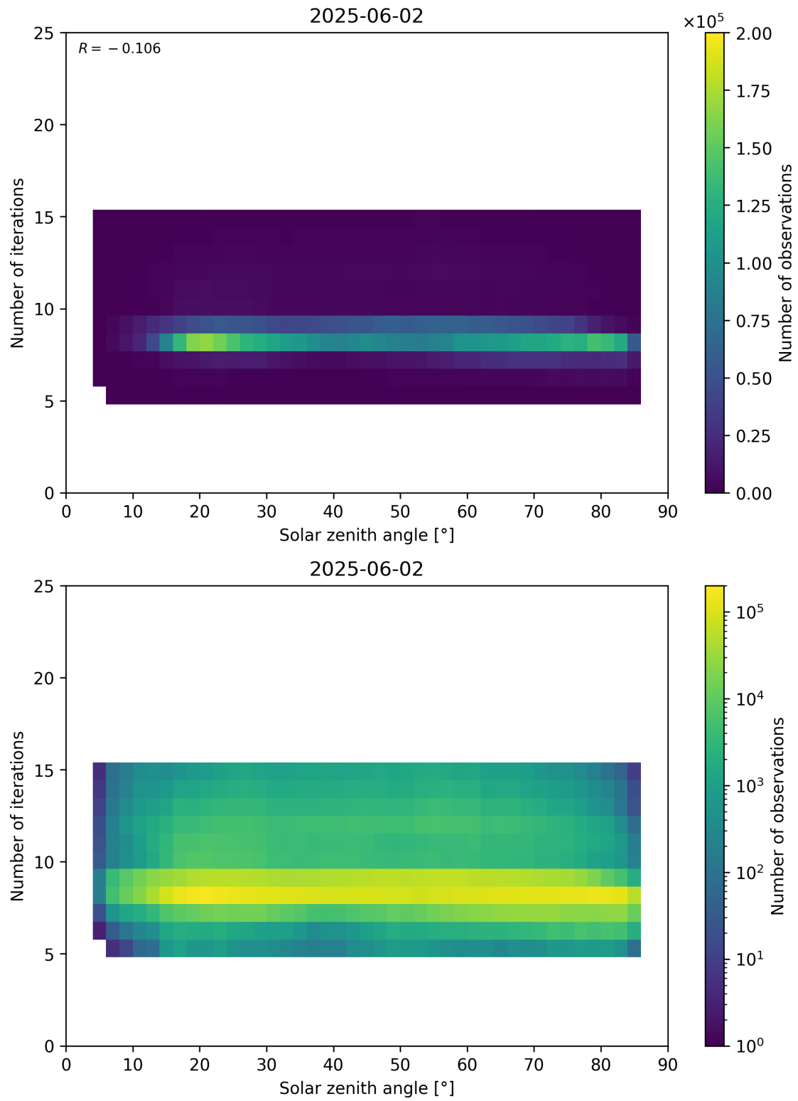
Figure 67: Scatter density plot of “Solar zenith angle” against “Number of iterations” for 2025-06-01 to 2025-06-03.
