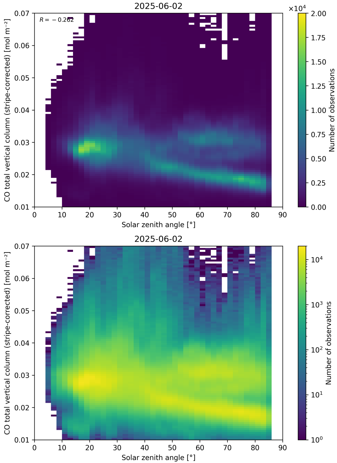
Figure 62: Scatter density plot of “Solar zenith angle” against “CO total vertical column (stripe-corrected)” for 2025-06-01 to 2025-06-03.
