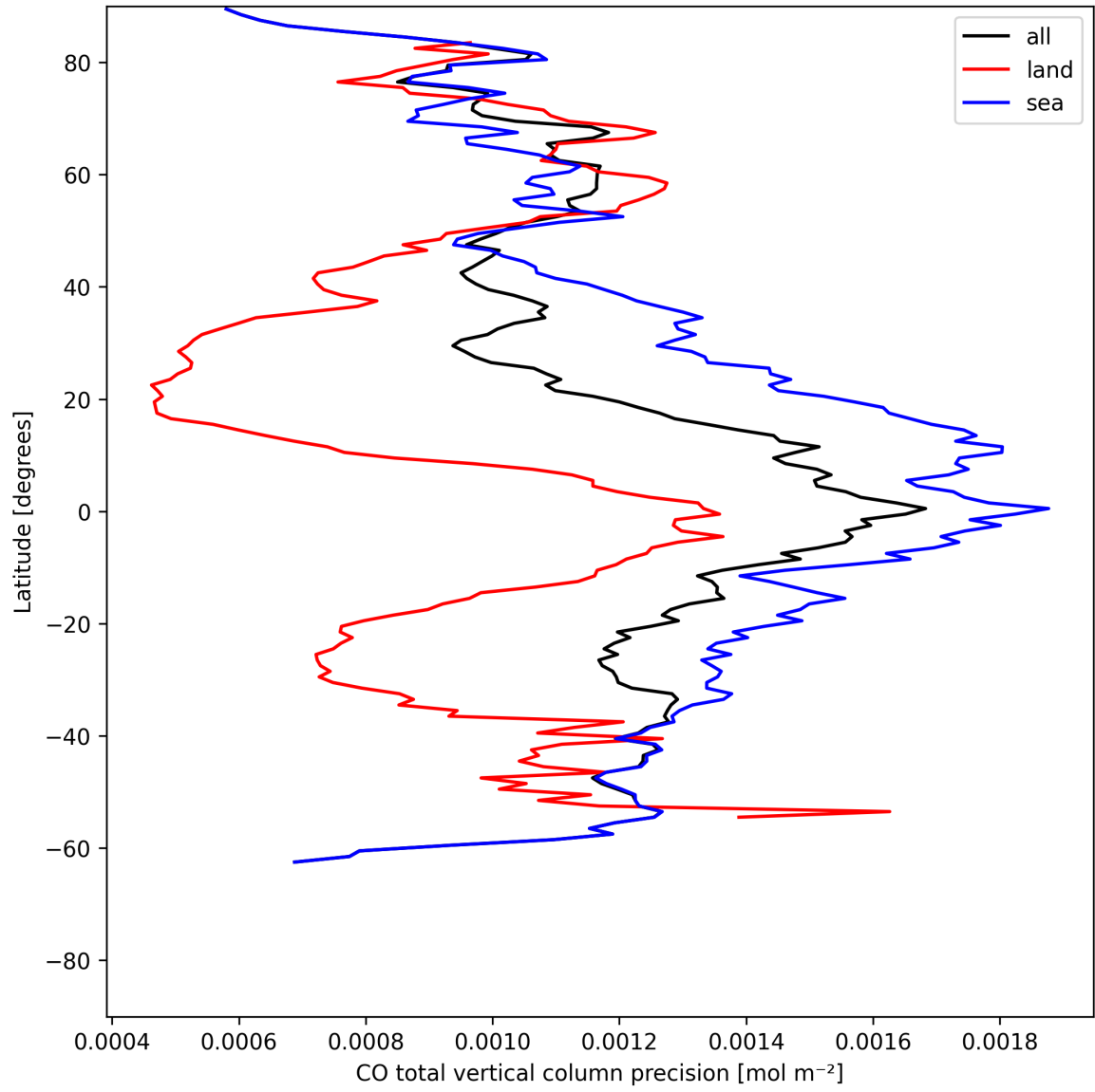
Figure 12: Zonal average of “CO total vertical column precision” for 2025-06-01 to 2025-06-03.
