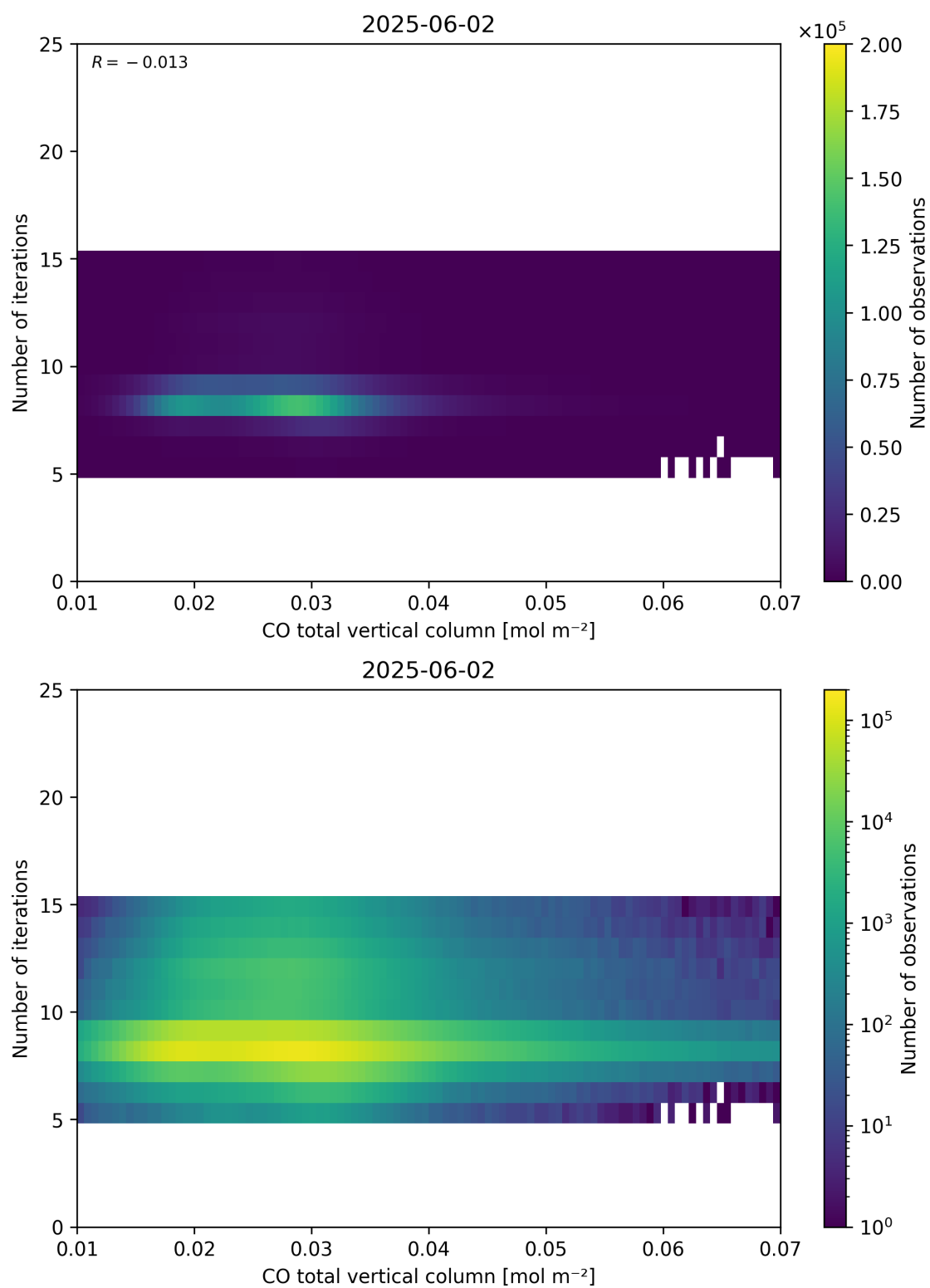
Figure 42: Scatter density plot of “CO total vertical column” against “Number of iterations” for 2025-06-01 to 2025-06-03.
