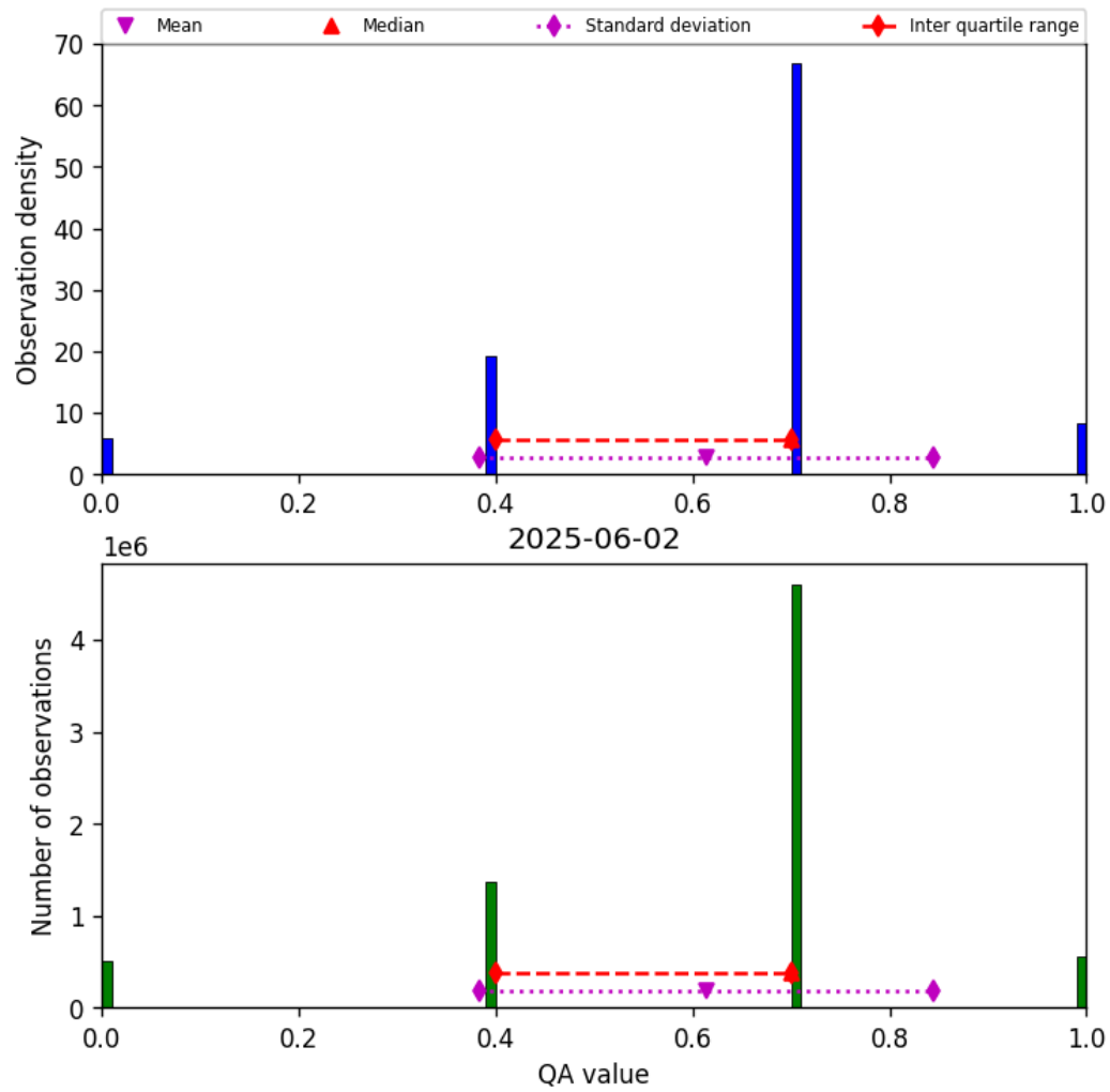
Figure 17: Histogram of “QA value” for 2025-06-01 to 2025-06-03
