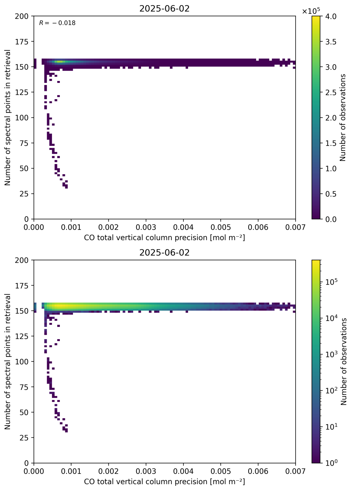
Figure 47: Scatter density plot of “CO total vertical column precision” against “Number of spectral points in retrieval” for 2025-06-01 to 2025-06-03.
