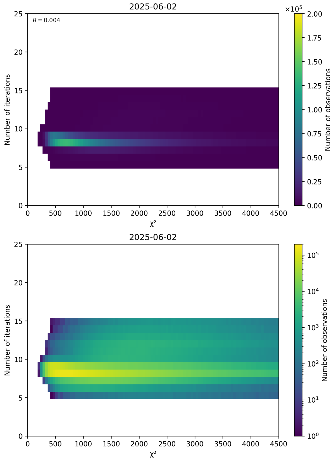
Figure 49: Scatter density plot of “ \chi^2 ” against “Number of iterations” for 2025-06-01 to 2025-06-03.
