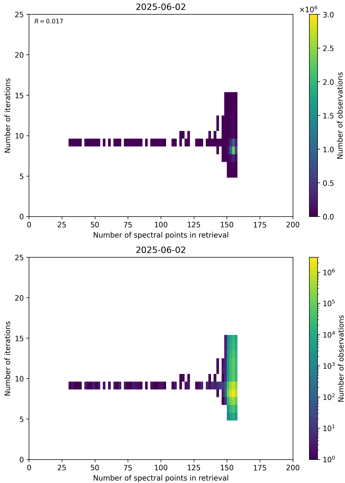
Figure 60: Scatter density plot of “Number of spectral points in retrieval” against “Number of iterations” for 2025-06-01 to 2025-06-03.
