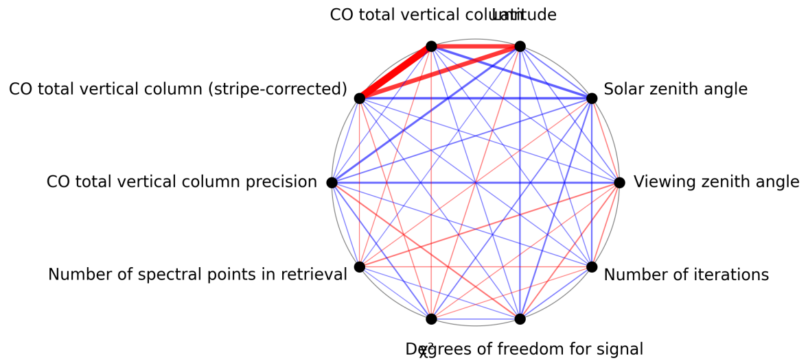
Figure 1: Map of correlation graph for 2025-06-01 to 2025-06-03.
