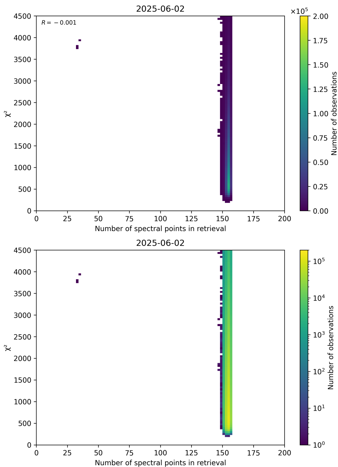
Figure 58: Scatter density plot of “Number of spectral points in retrieval” against “ \chi^2 ” for 2025-06-01 to 2025-06-03.
