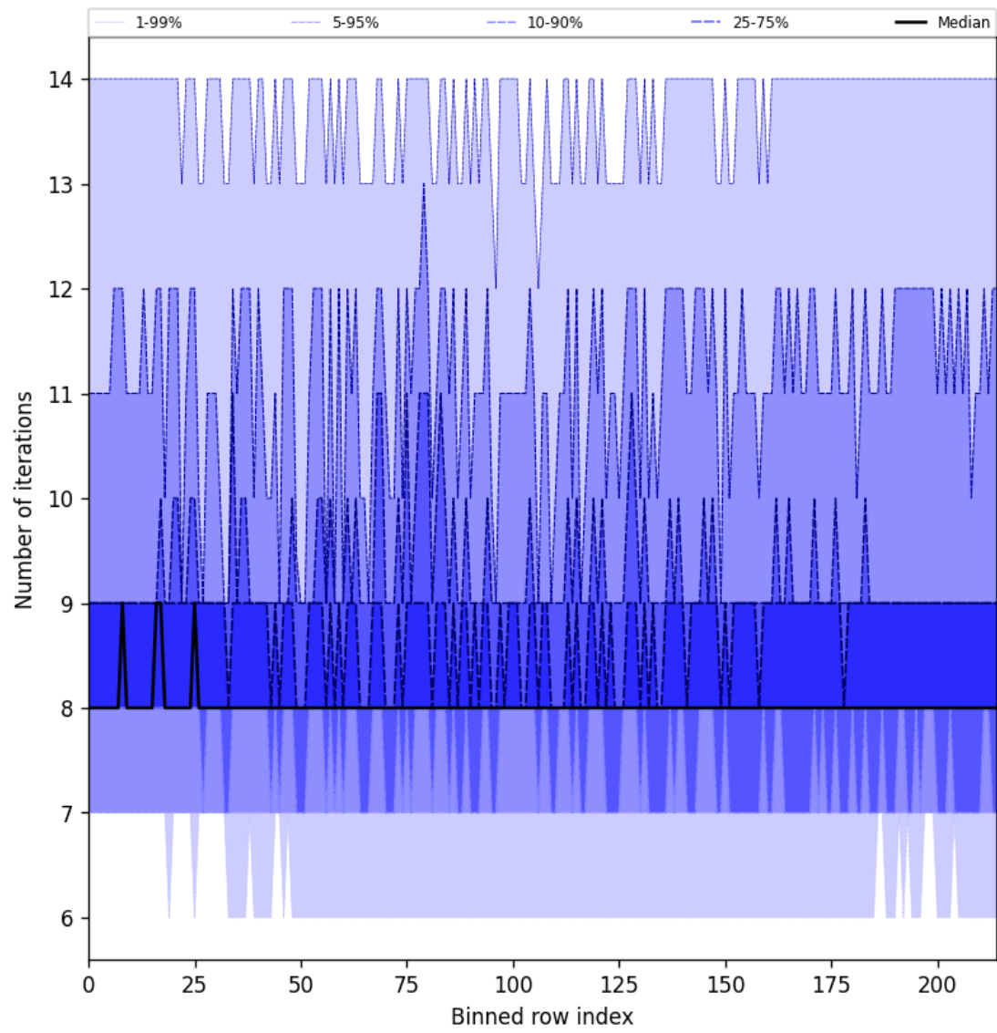
Figure 32: Along track statistics of “Number of iterations” for 2025-06-01 to 2025-06-03
