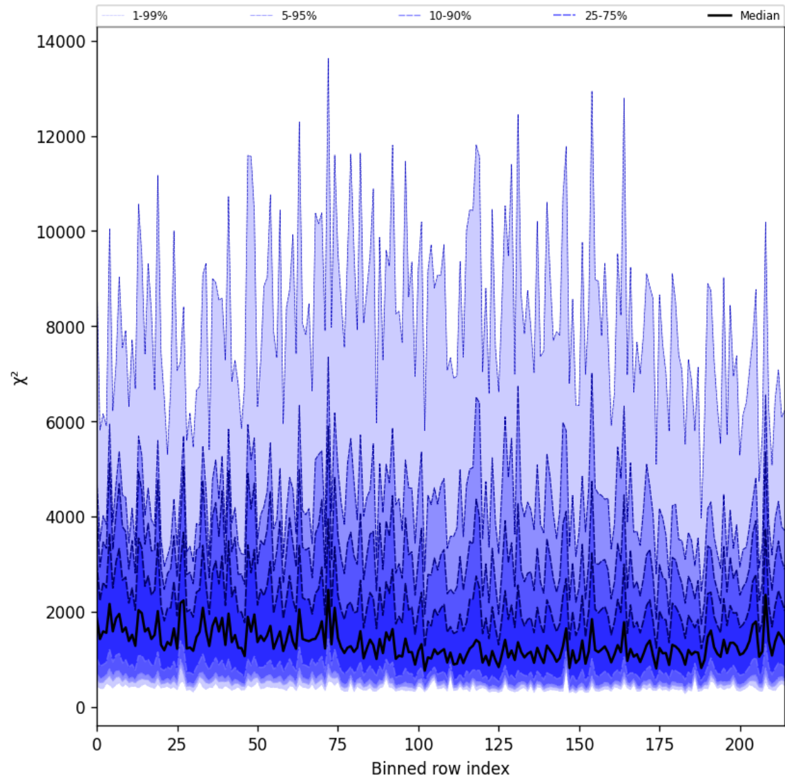
Figure 30: Along track statistics of “ \chi^2 ” for 2025-06-01 to 2025-06-03
