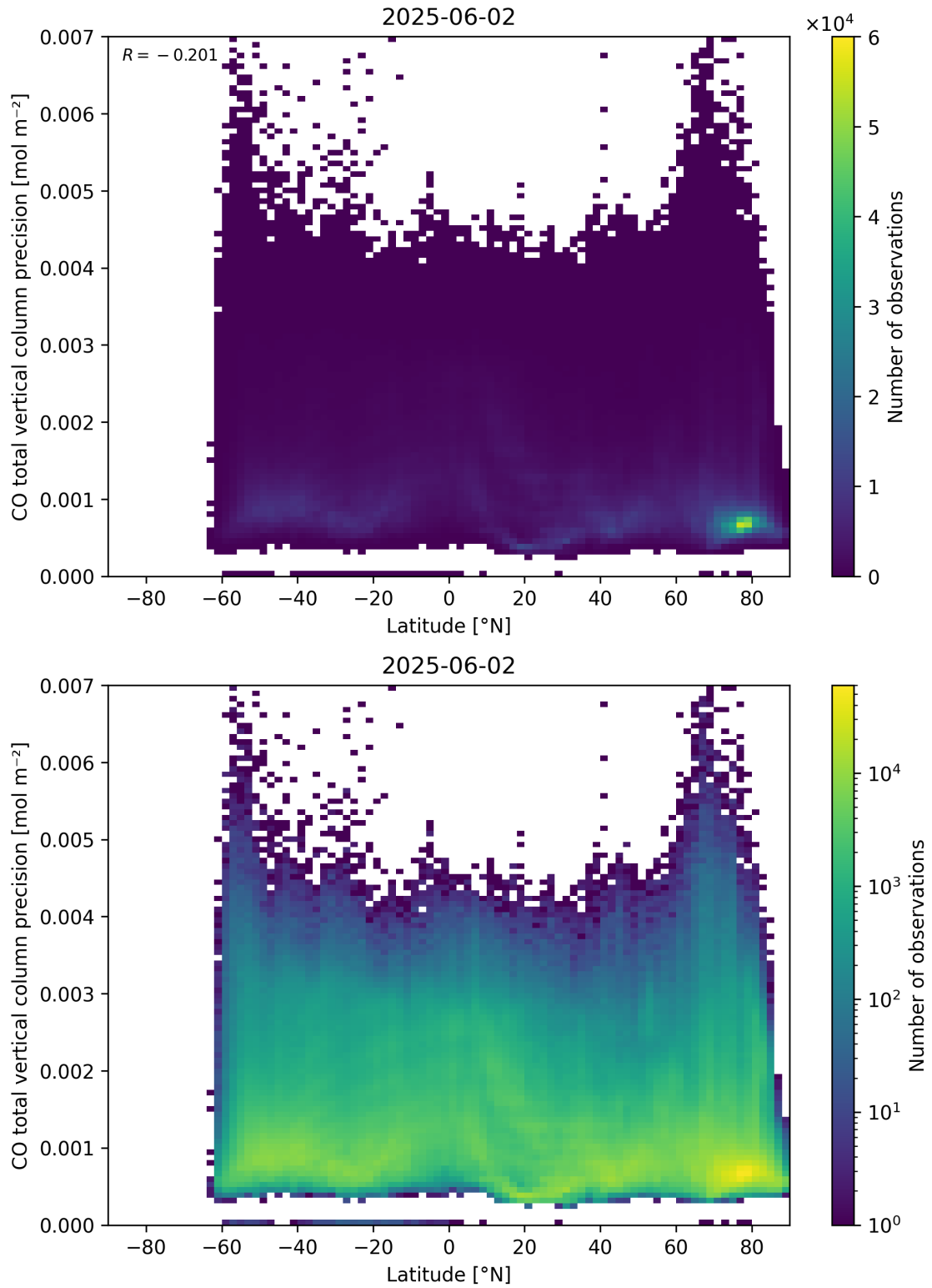
Figure 53: Scatter density plot of “Latitude” against “CO total vertical column precision” for 2025-06-01 to 2025-06-03.
