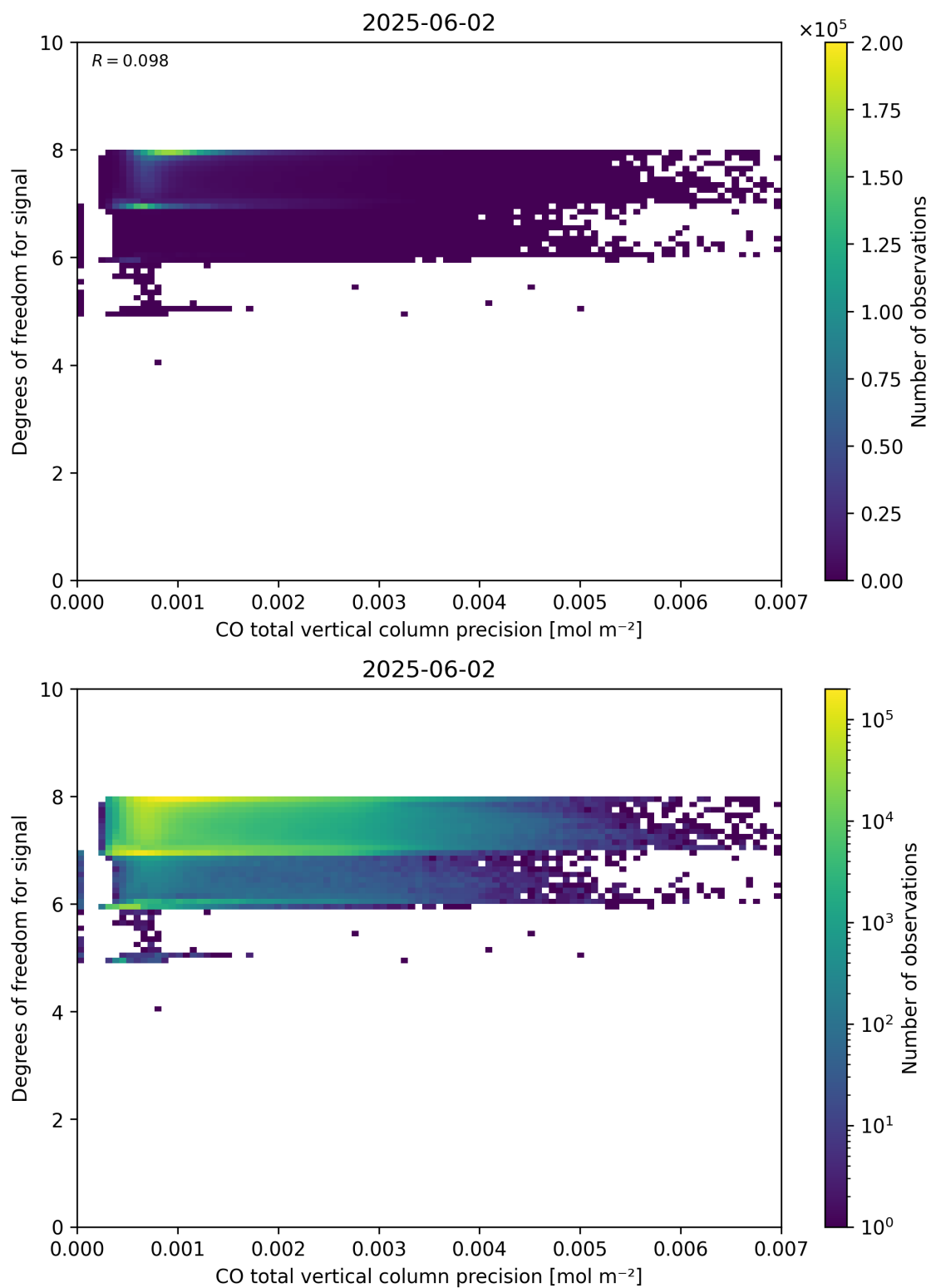
Figure 45: Scatter density plot of “CO total vertical column precision” against “Degrees of freedom for signal” for 2025-06-01 to 2025-06-03.
