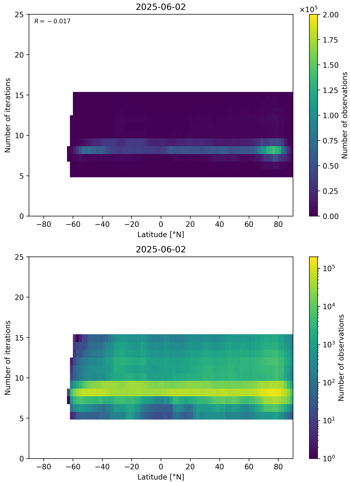
Figure 56: Scatter density plot of “Latitude” against “Number of iterations” for 2025-06-01 to 2025-06-03.
