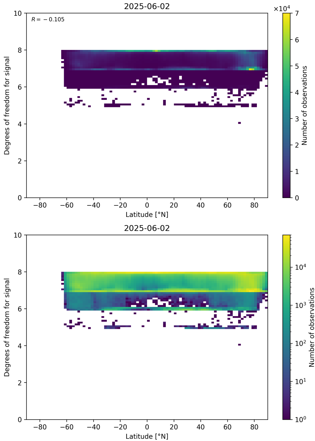
Figure 55: Scatter density plot of “Latitude” against “Degrees of freedom for signal” for 2025-06-01 to 2025-06-03.
