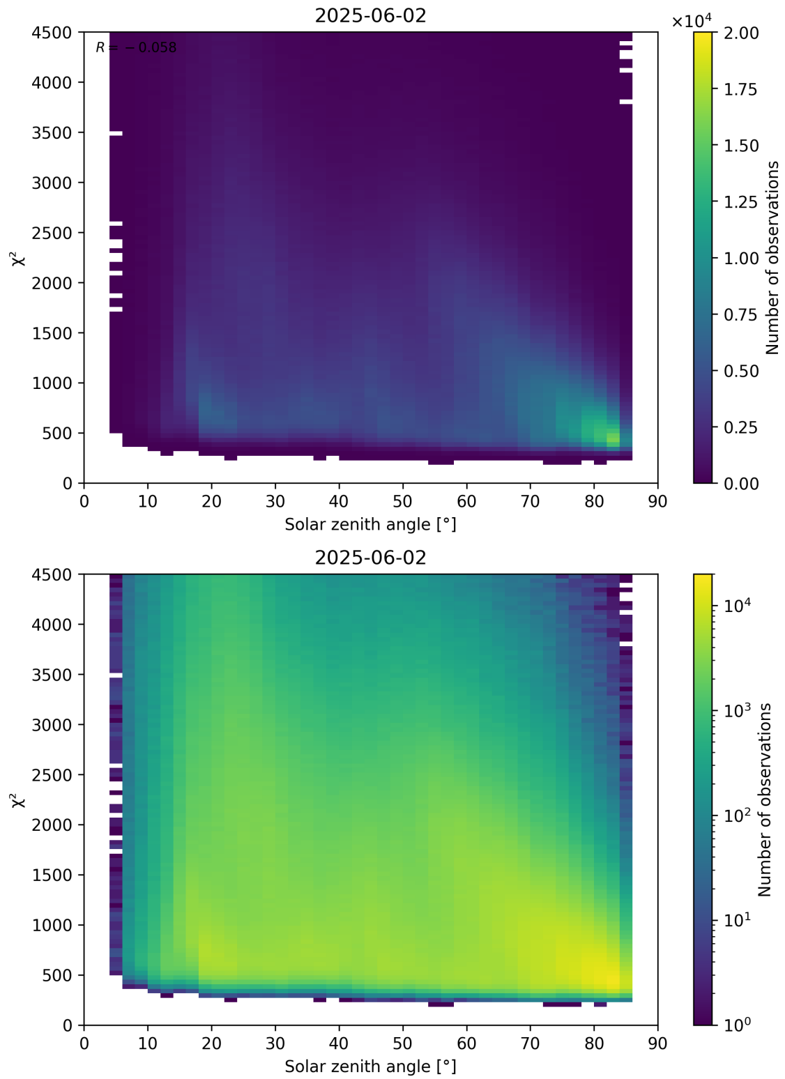
Figure 64: Scatter density plot of “Solar zenith angle” against “ \chi^2 ” for 2025-06-01 to 2025-06-03.
