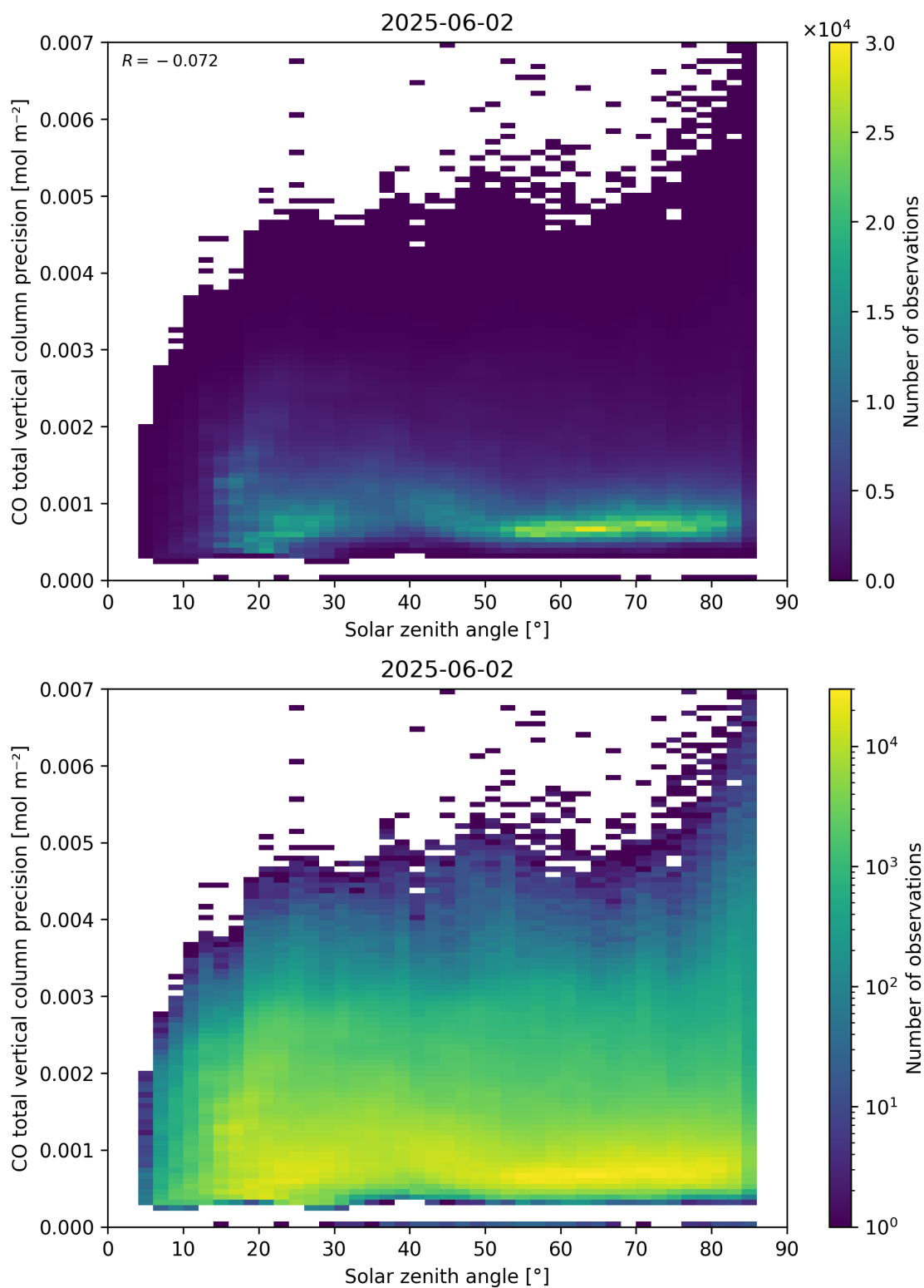
Figure 63: Scatter density plot of “Solar zenith angle” against “CO total vertical column precision” for 2025-06-01 to 2025-06-03.
