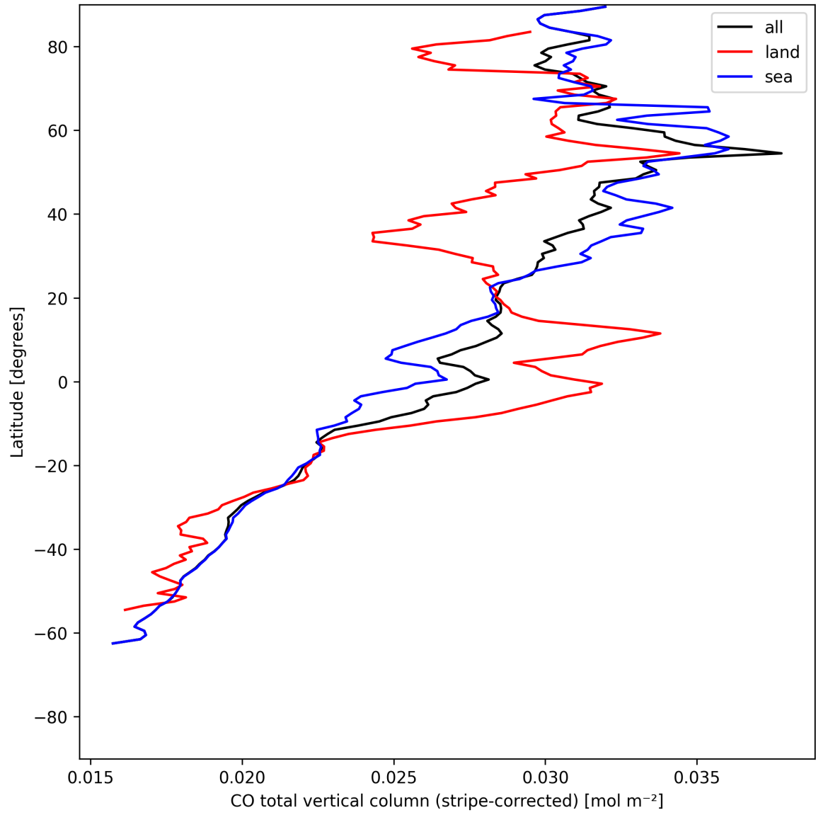
Figure 11: Zonal average of “CO total vertical column (stripe-corrected)” for 2025-06-01 to 2025-06-03.
