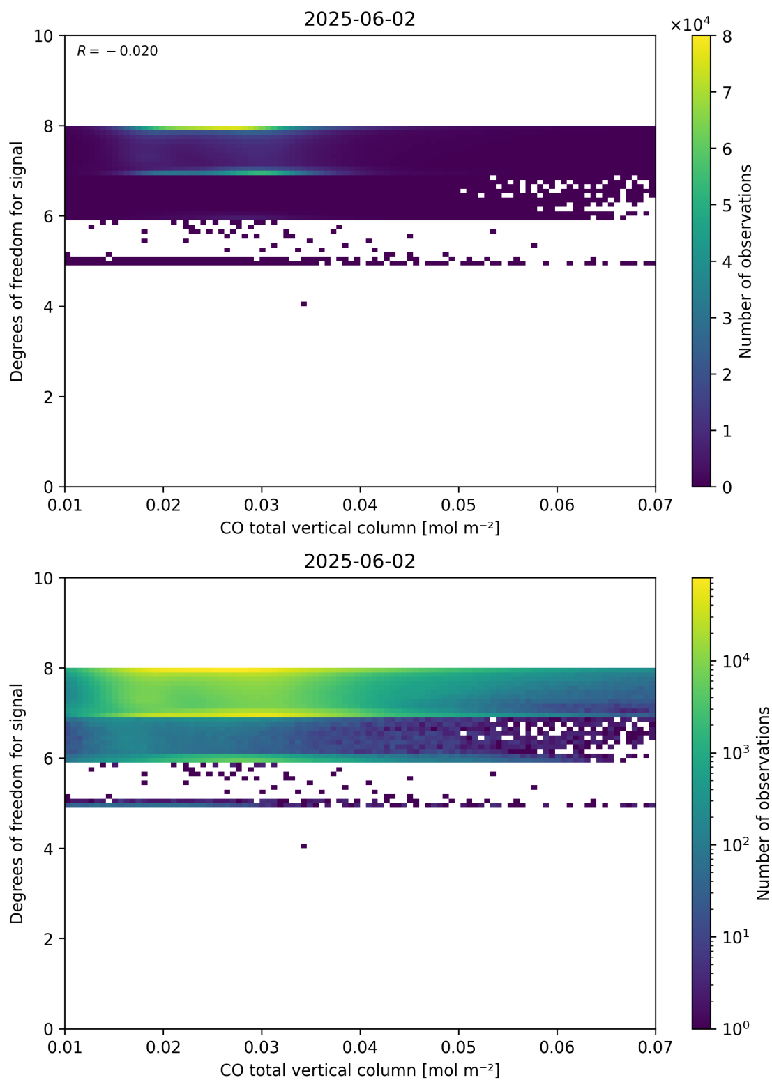
Figure 41: Scatter density plot of “CO total vertical column” against “Degrees of freedom for signal” for 2025-06-01 to 2025-06-03.
