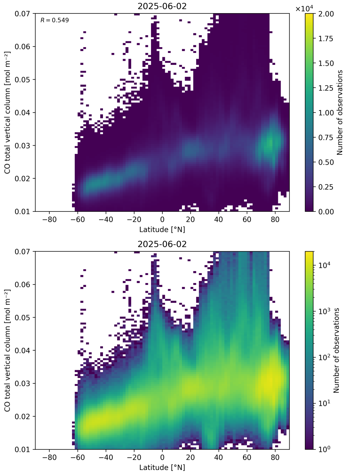
Figure 51: Scatter density plot of “Latitude” against “CO total vertical column” for 2025-06-01 to 2025-06-03.
