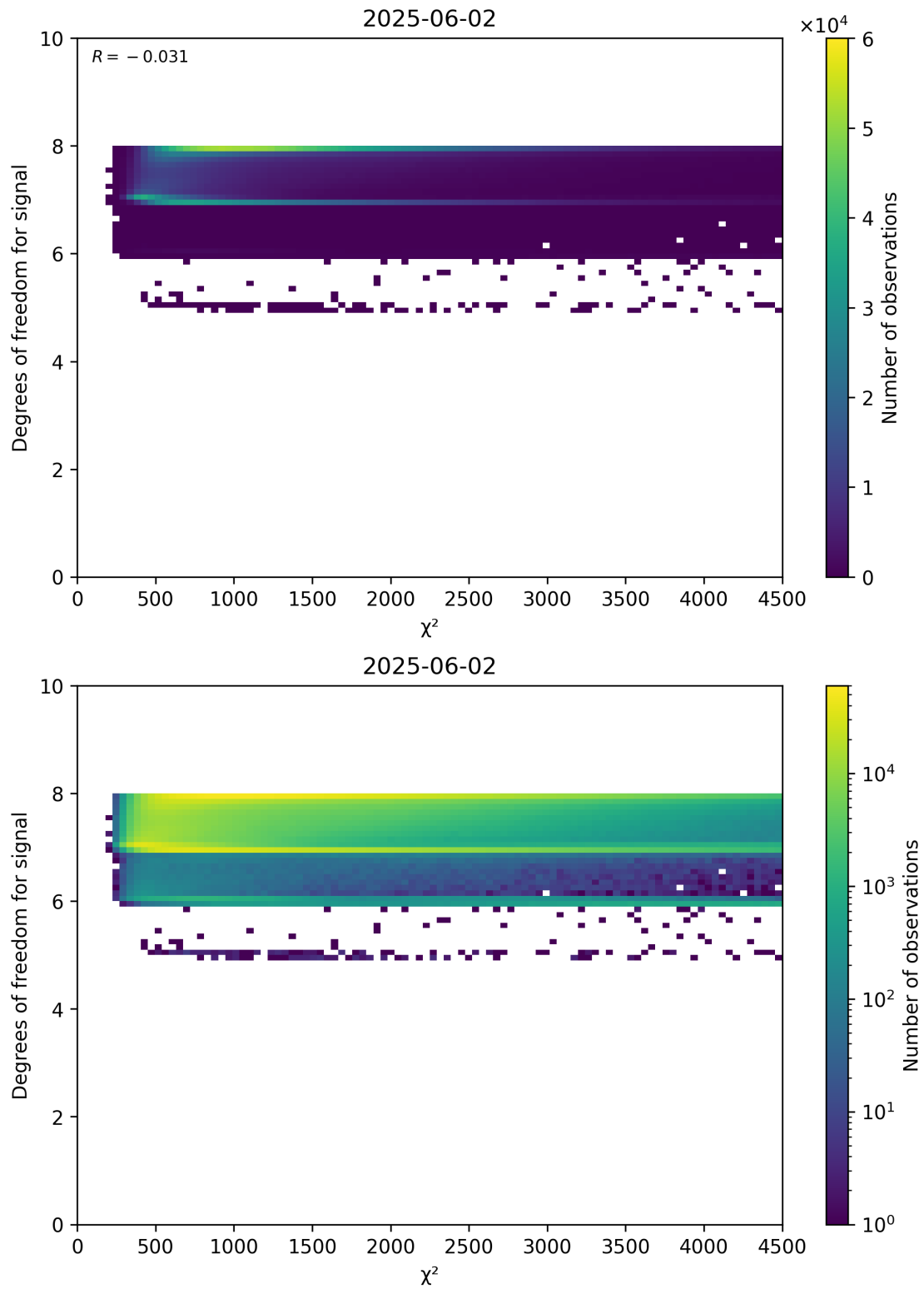
Figure 48: Scatter density plot of “ \chi^2 ” against “Degrees of freedom for signal” for 2025-06-01 to 2025-06-03.
