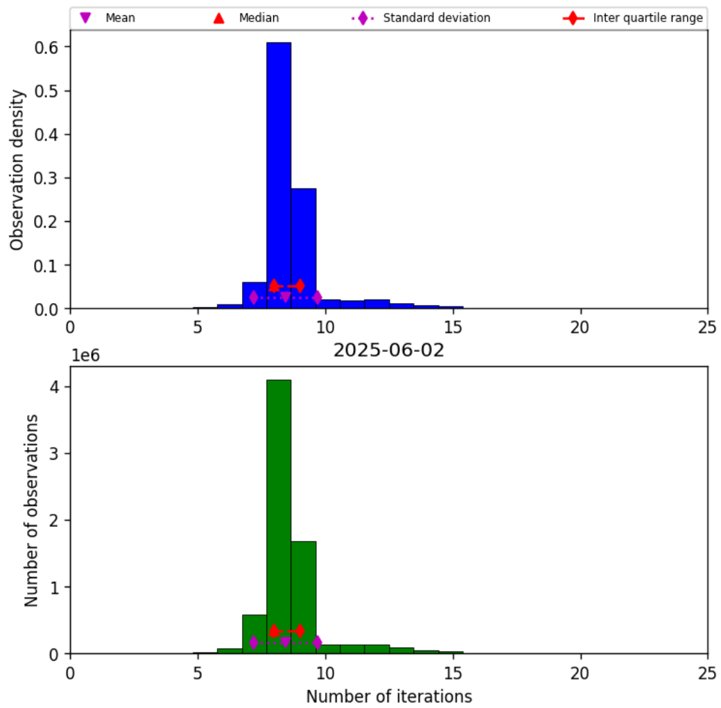
Figure 24: Histogram of “Number of iterations” for 2025-06-01 to 2025-06-03
