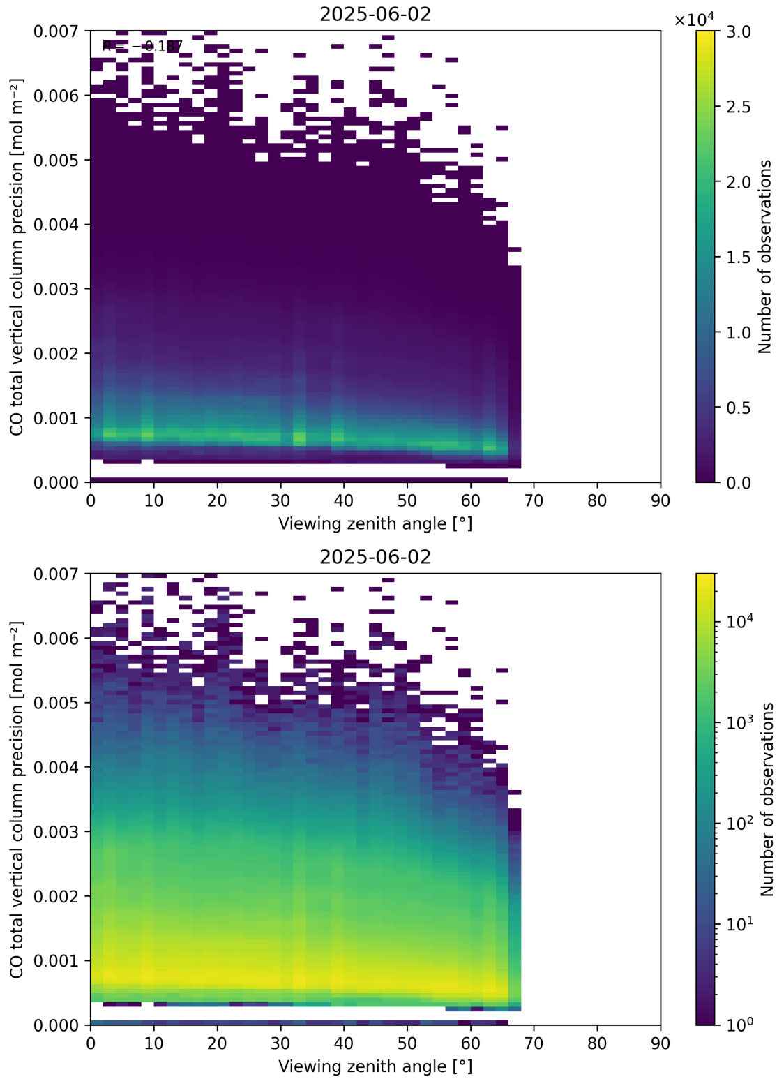
Figure 71: Scatter density plot of “Viewing zenith angle” against “CO total vertical column precision” for 2025-06-01 to 2025-06-03.
