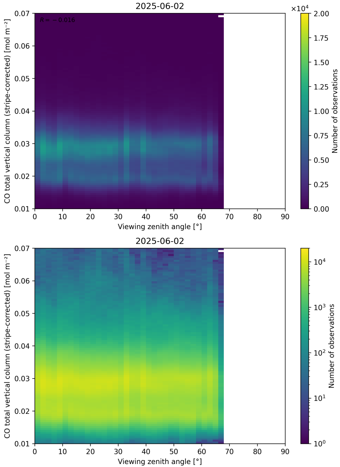
Figure 70: Scatter density plot of “Viewing zenith angle” against “CO total vertical column (stripe-corrected)” for 2025-06-01 to 2025-06-03.
