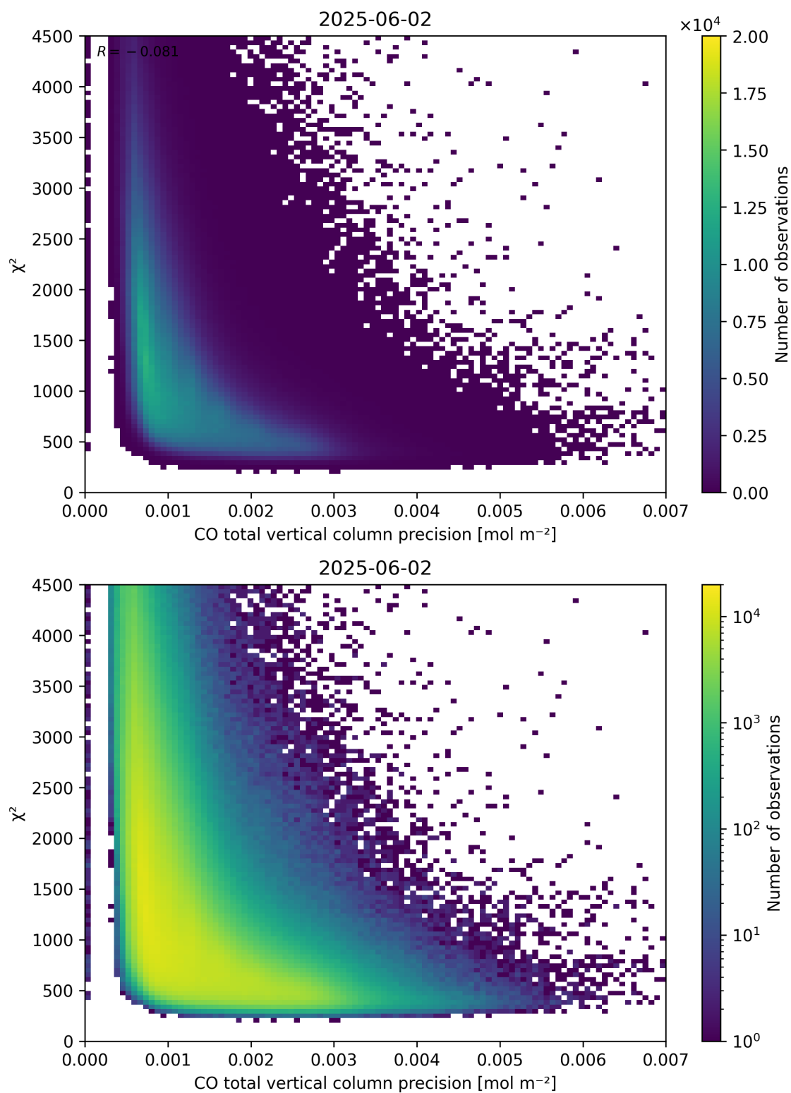
Figure 44: Scatter density plot of “CO total vertical column precision” against “ \chi^2 ” for 2025-06-01 to 2025-06-03.
