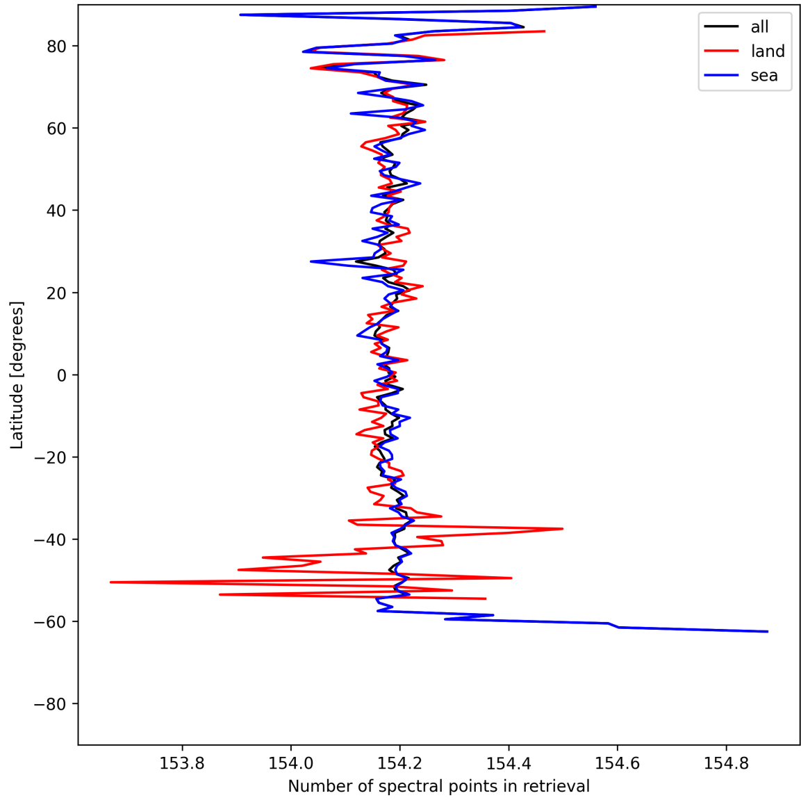
Figure 13: Zonal average of “Number of spectral points in retrieval” for 2025-06-01 to 2025-06-03.
