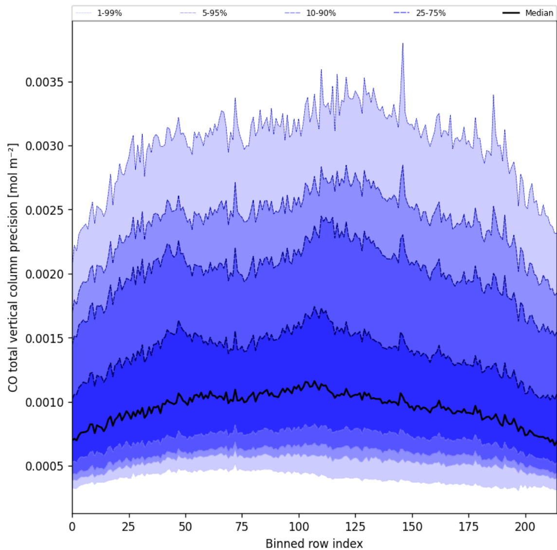
Figure 28: Along track statistics of “CO total vertical column precision” for 2025-06-01 to 2025-06-03
