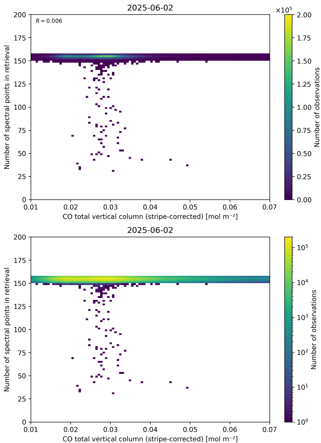
Figure 40: Scatter density plot of “CO total vertical column (stripe-corrected)” against “Number of spectral points in retrieval” for 2025-06-01 to 2025-06-03.
