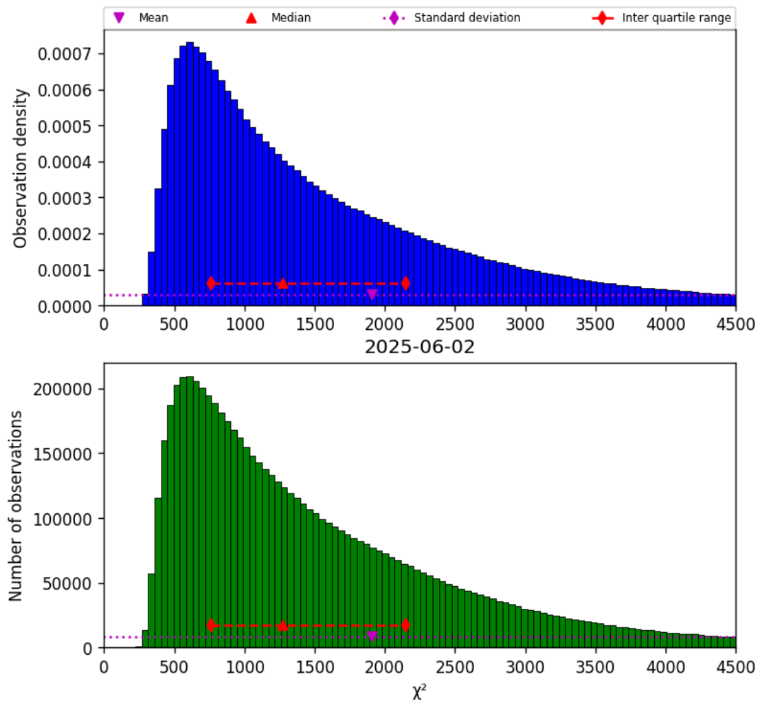
Figure 22: Histogram of “ \chi^2 ” for 2025-06-01 to 2025-06-03
