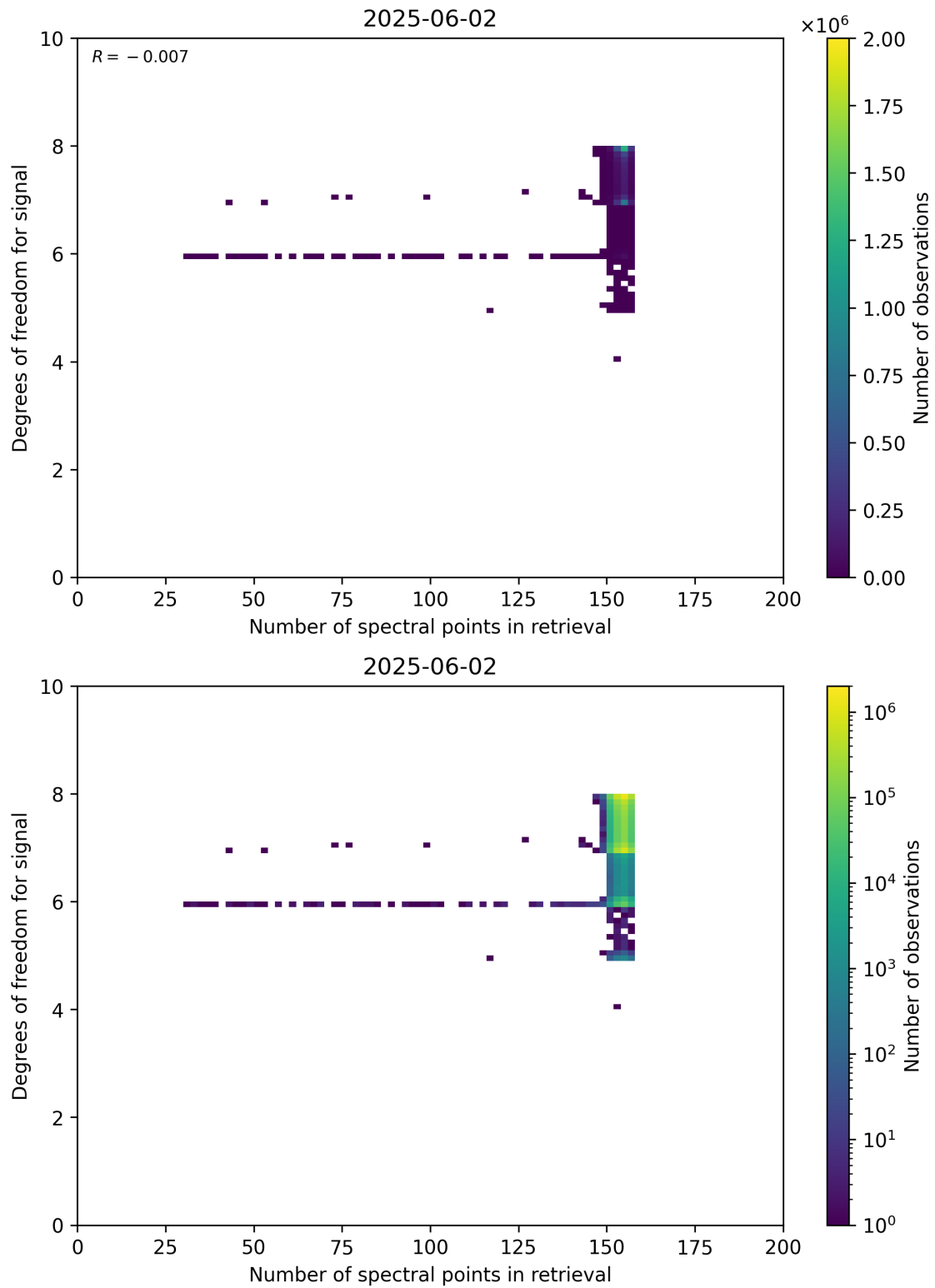
Figure 59: Scatter density plot of “Number of spectral points in retrieval” against “Degrees of freedom for signal” for 2025-06-01 to 2025-06-03.
