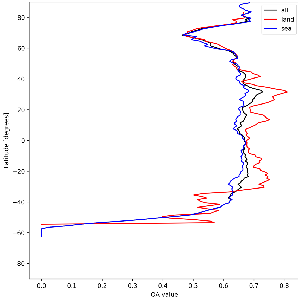
Figure 9: Zonal average of “QA value” for 2025-06-01 to 2025-06-03.
