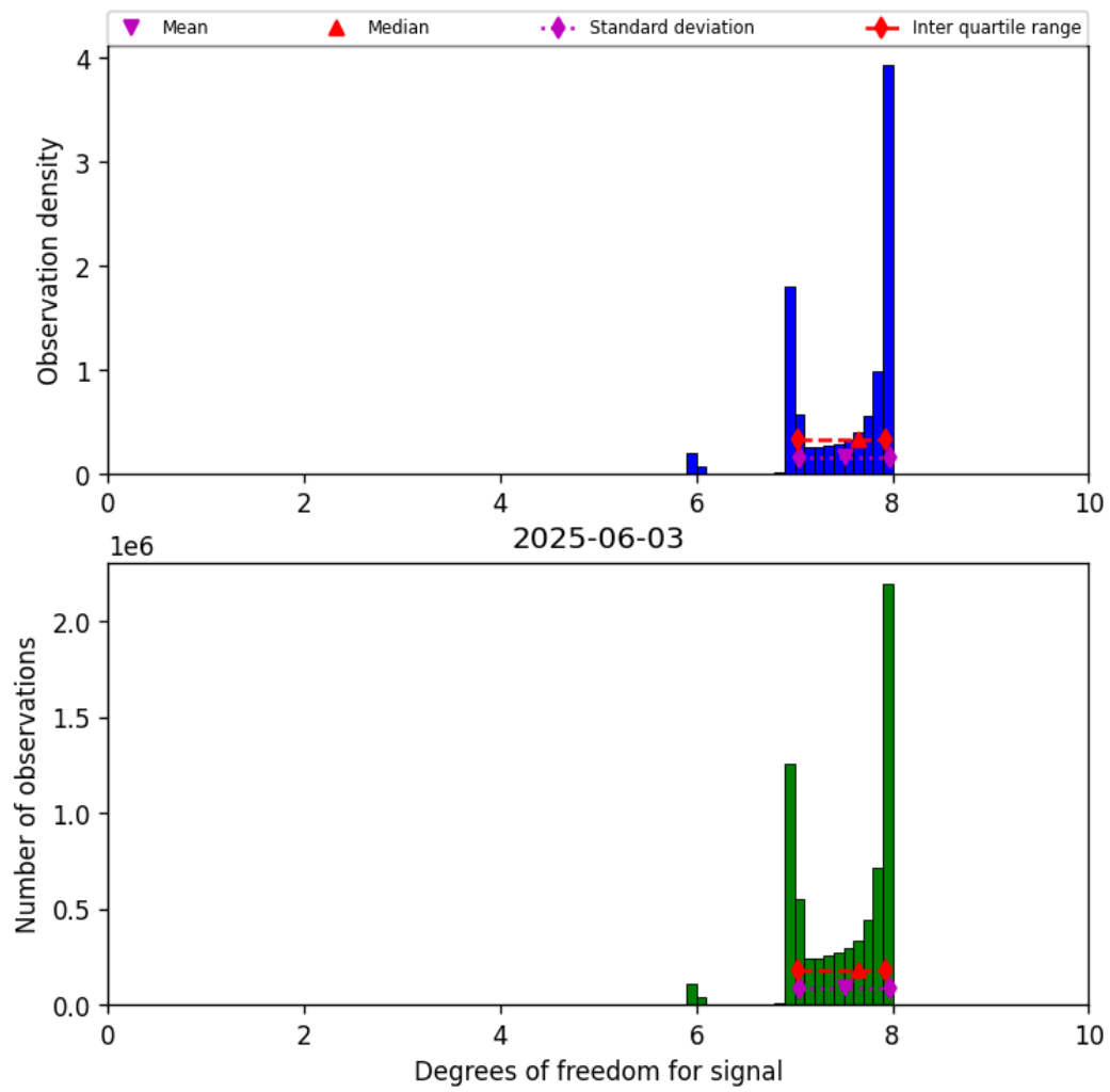
Figure 23: Histogram of “Degrees of freedom for signal” for 2025-06-02 to 2025-06-04
