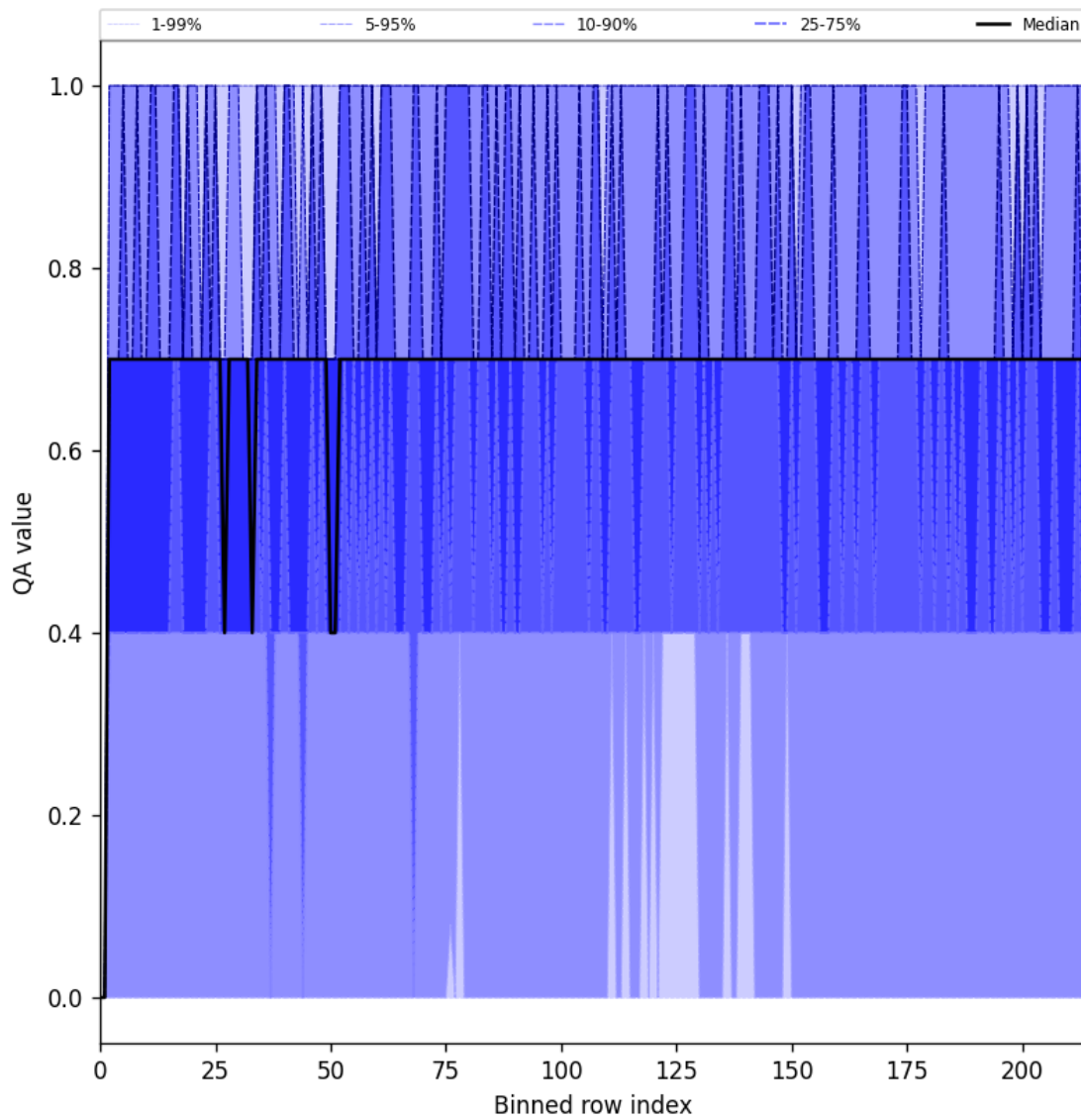
Figure 25: Along track statistics of “QA value” for 2025-06-02 to 2025-06-04
