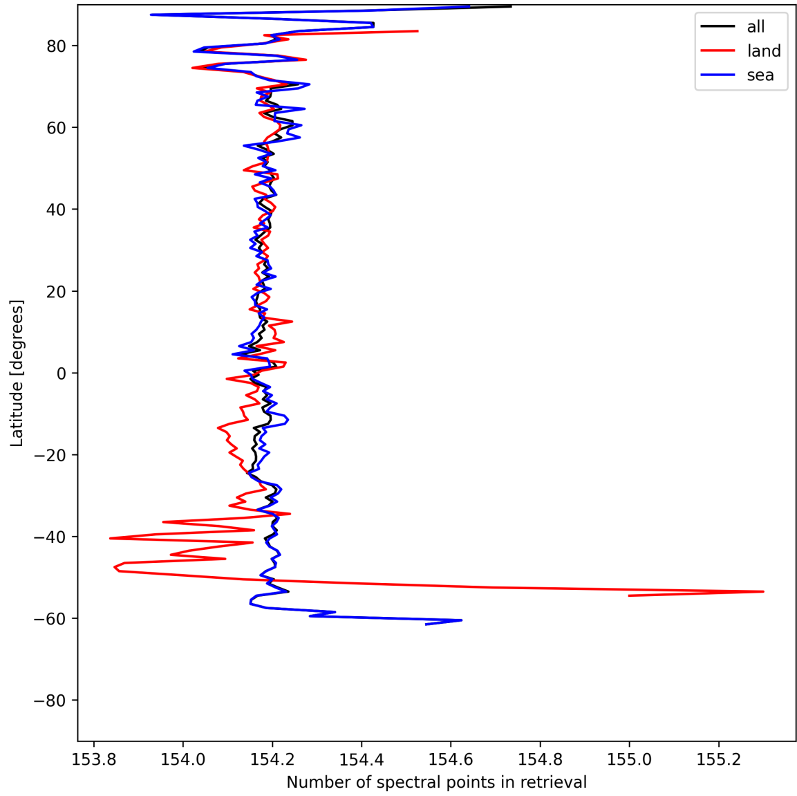
Figure 13: Zonal average of “Number of spectral points in retrieval” for 2025-06-02 to 2025-06-04.
