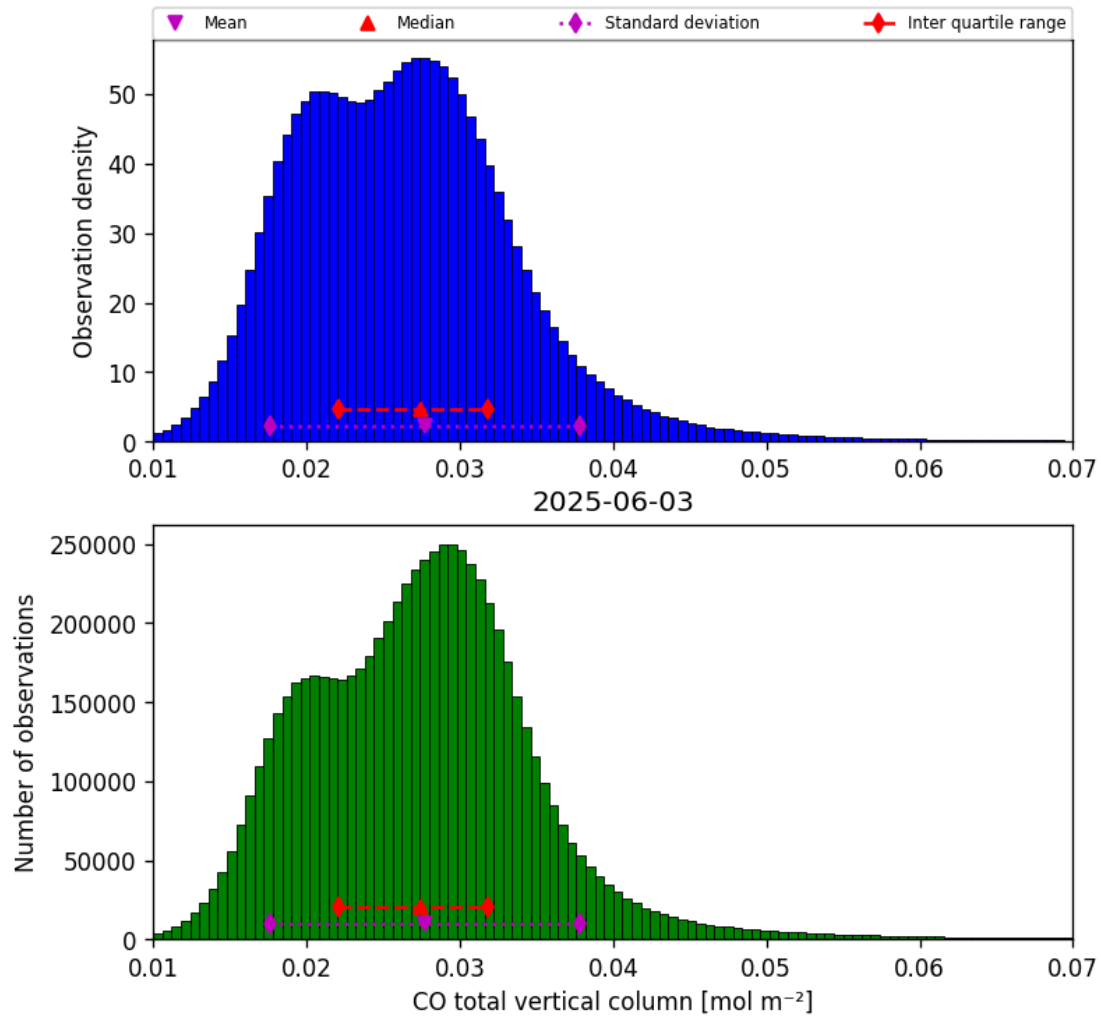
Figure 18: Histogram of “CO total vertical column” for 2025-06-02 to 2025-06-04
