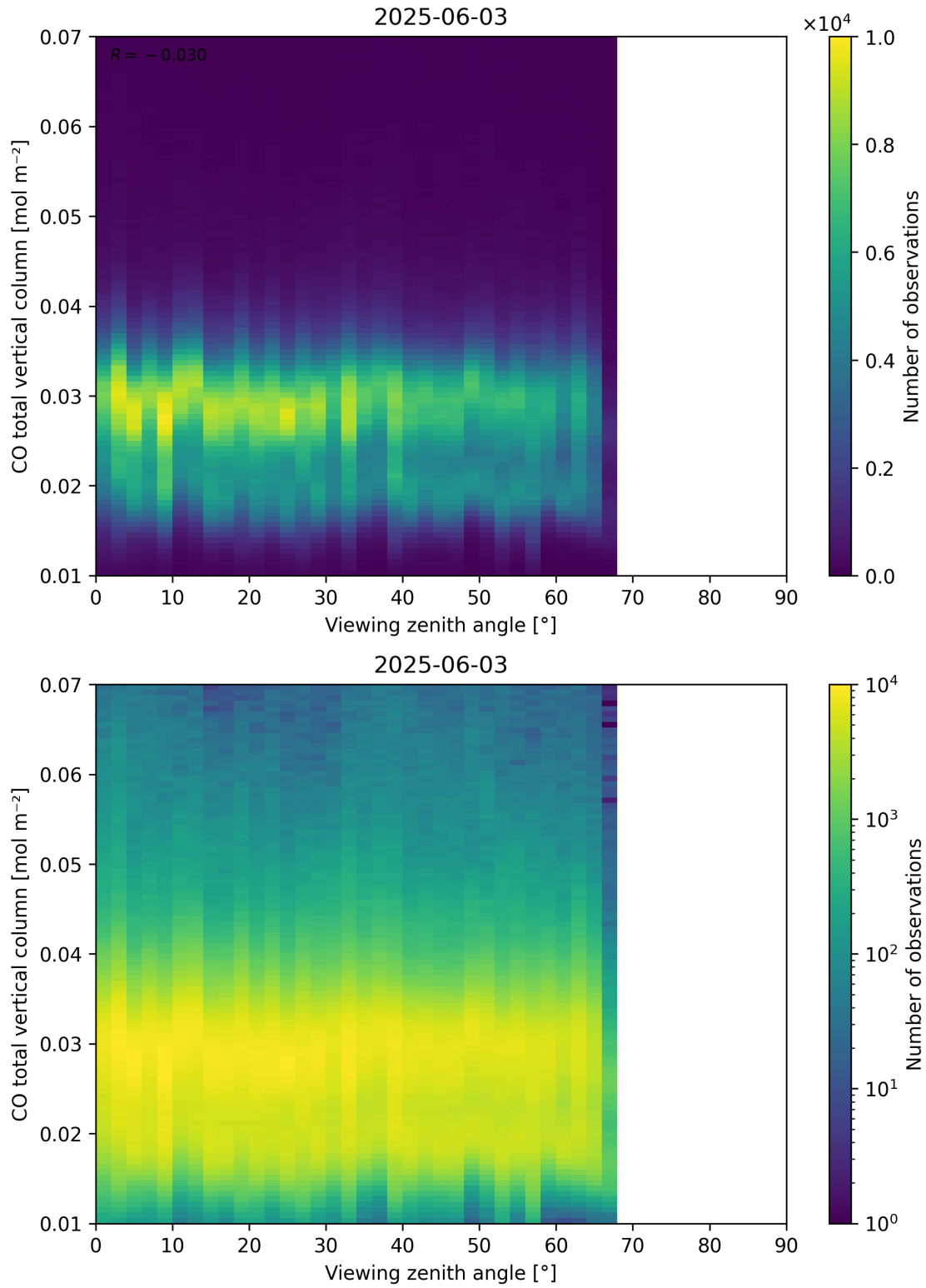
Figure 69: Scatter density plot of “Viewing zenith angle” against “CO total vertical column” for 2025-06-02 to 2025-06-04.
