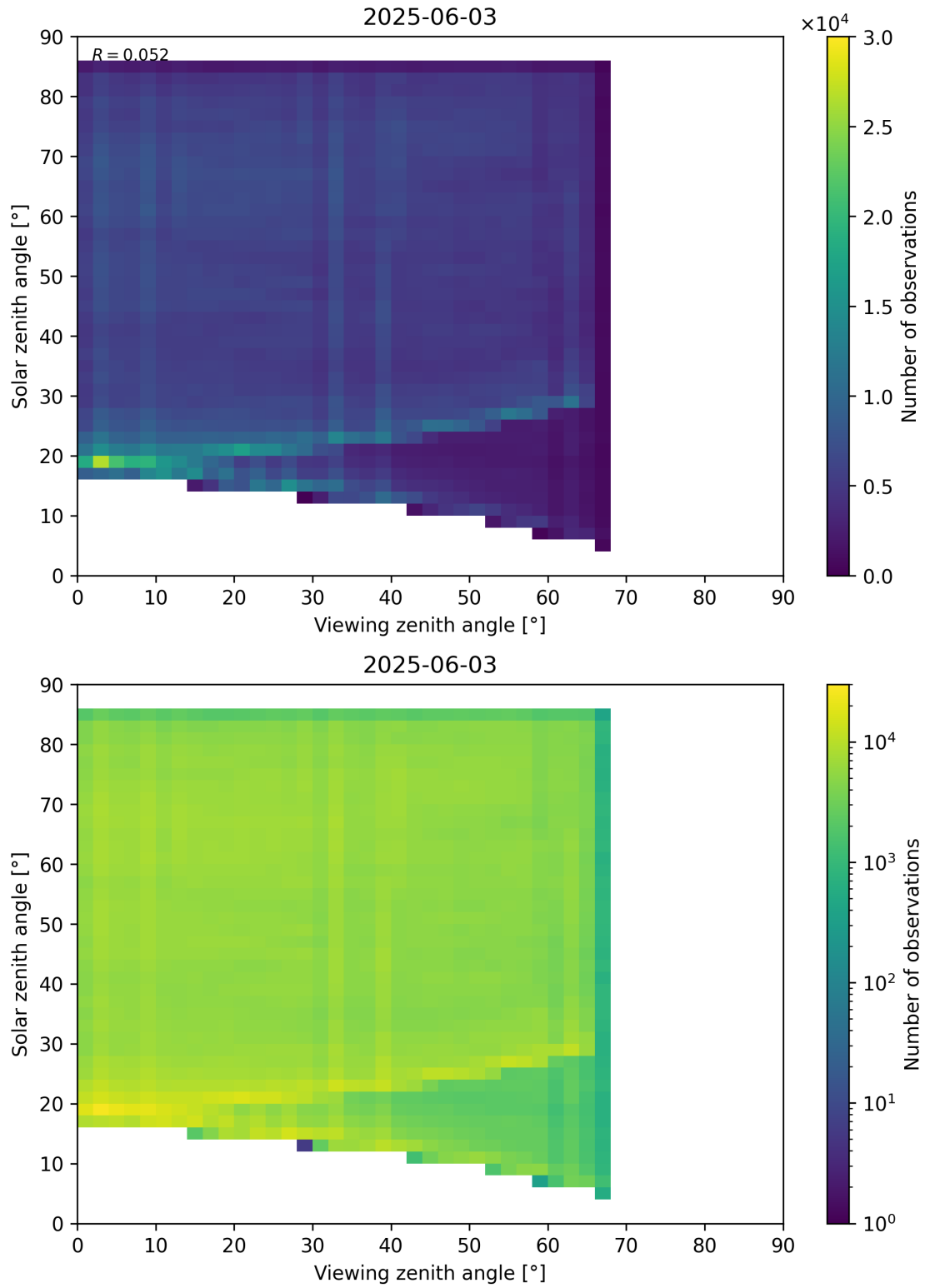
Figure 77: Scatter density plot of “Viewing zenith angle” against “Solar zenith angle” for 2025-06-02 to 2025-06-04.
