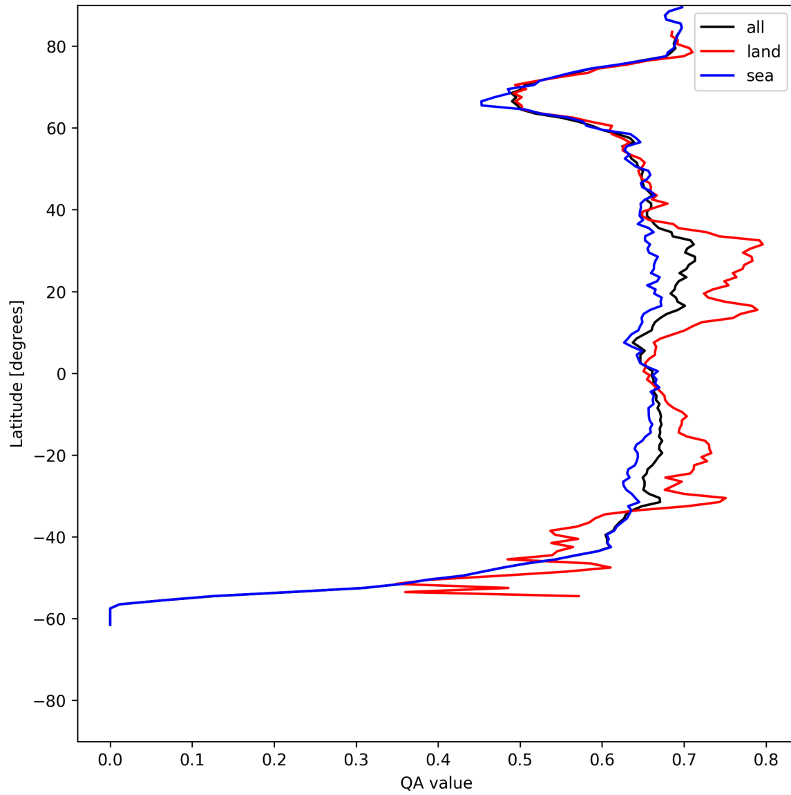
Figure 9: Zonal average of “QA value” for 2025-06-02 to 2025-06-04.
