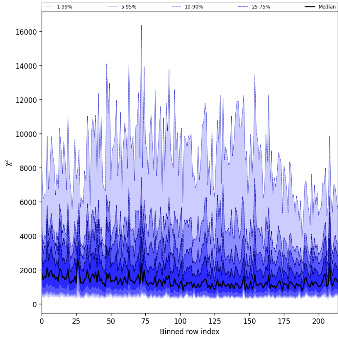
Figure 30: Along track statistics of “ \chi^2 ” for 2025-06-02 to 2025-06-04
