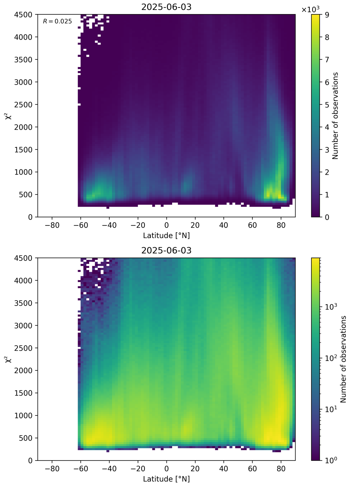
Figure 54: Scatter density plot of “Latitude” against “ \chi^2 ” for 2025-06-02 to 2025-06-04.
