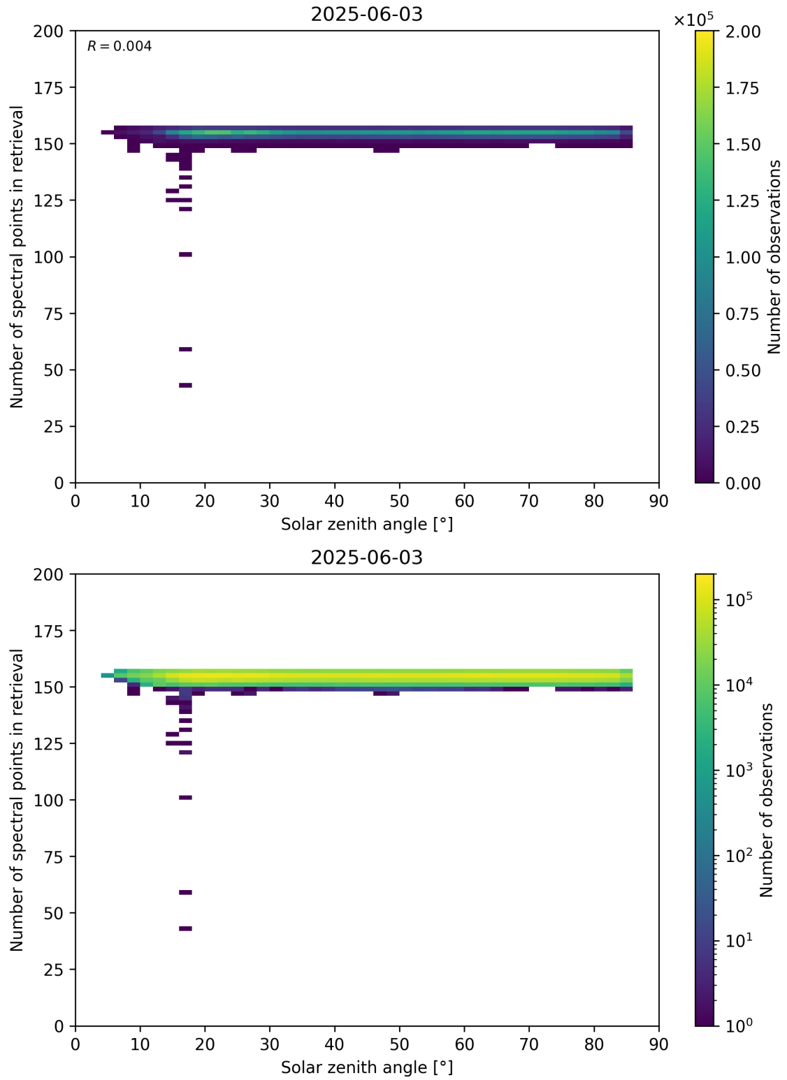
Figure 68: Scatter density plot of “Solar zenith angle” against “Number of spectral points in retrieval” for 2025-06-02 to 2025-06-04.
