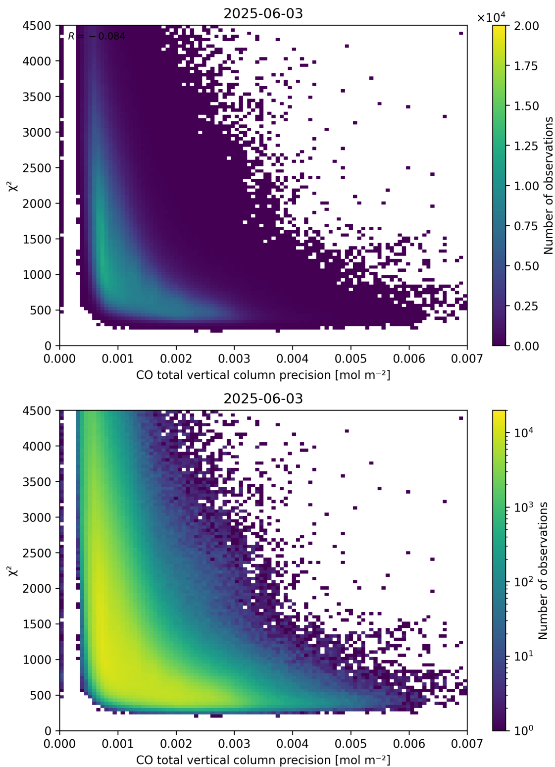
Figure 44: Scatter density plot of “CO total vertical column precision” against “ \chi^2 ” for 2025-06-02 to 2025-06-04.
