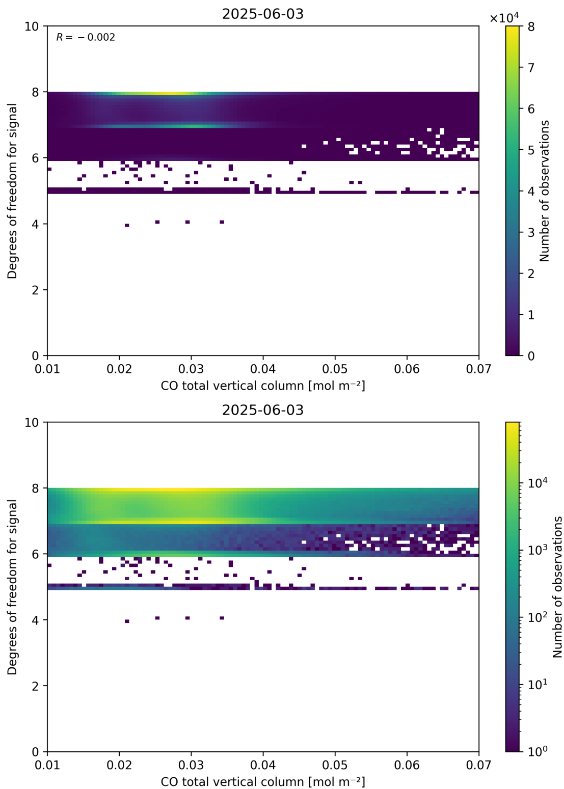
Figure 41: Scatter density plot of “CO total vertical column” against “Degrees of freedom for signal” for 2025-06-02 to 2025-06-04.
