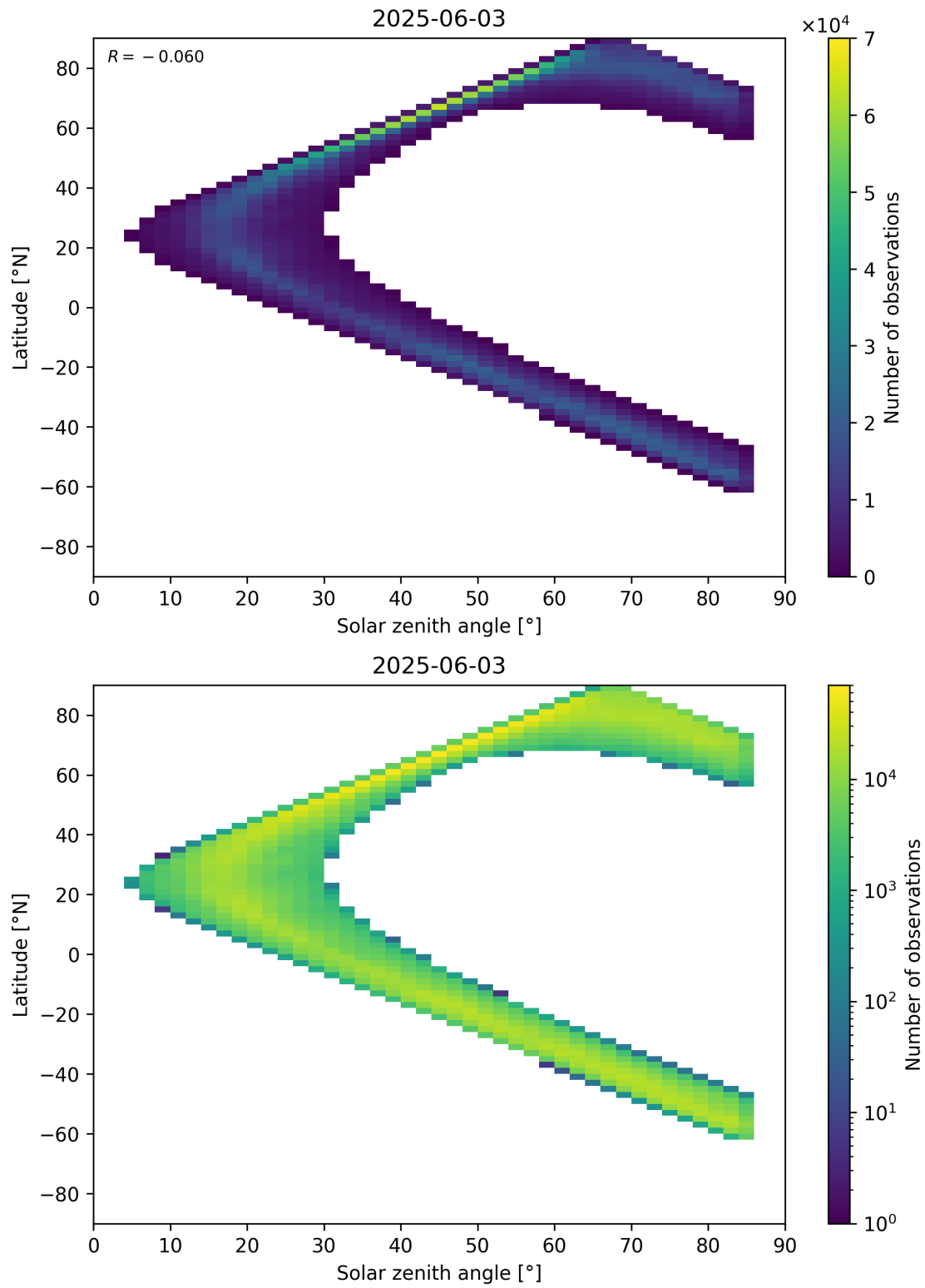
Figure 66: Scatter density plot of “Solar zenith angle” against “Latitude” for 2025-06-02 to 2025-06-04.
