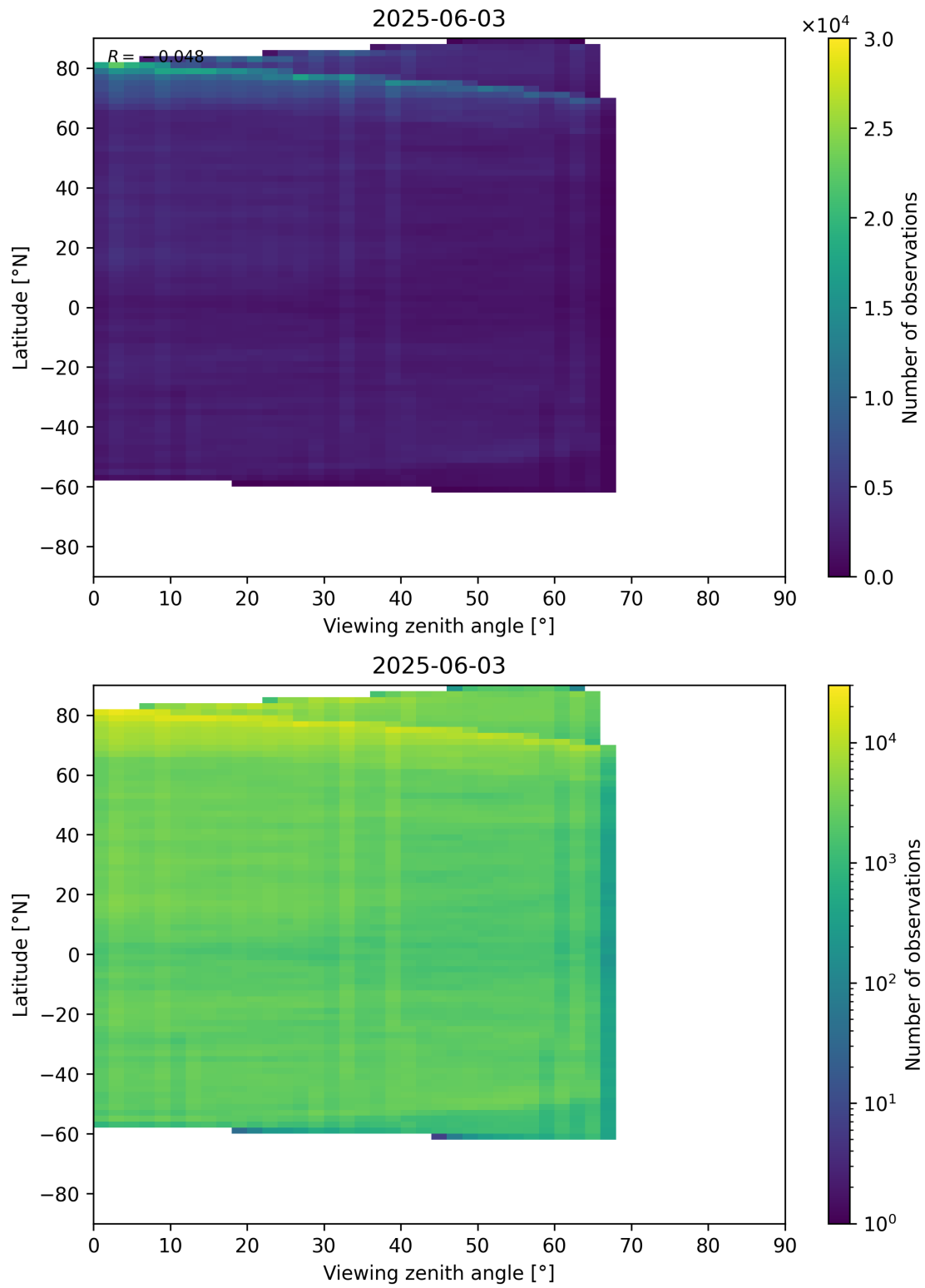
Figure 74: Scatter density plot of “Viewing zenith angle” against “Latitude” for 2025-06-02 to 2025-06-04.
