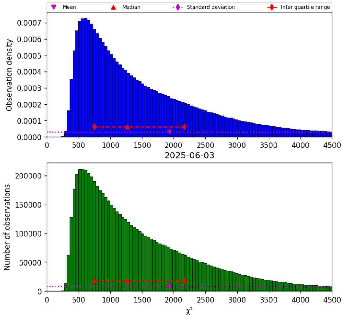
Figure 22: Histogram of “ \chi^2 ” for 2025-06-02 to 2025-06-04
