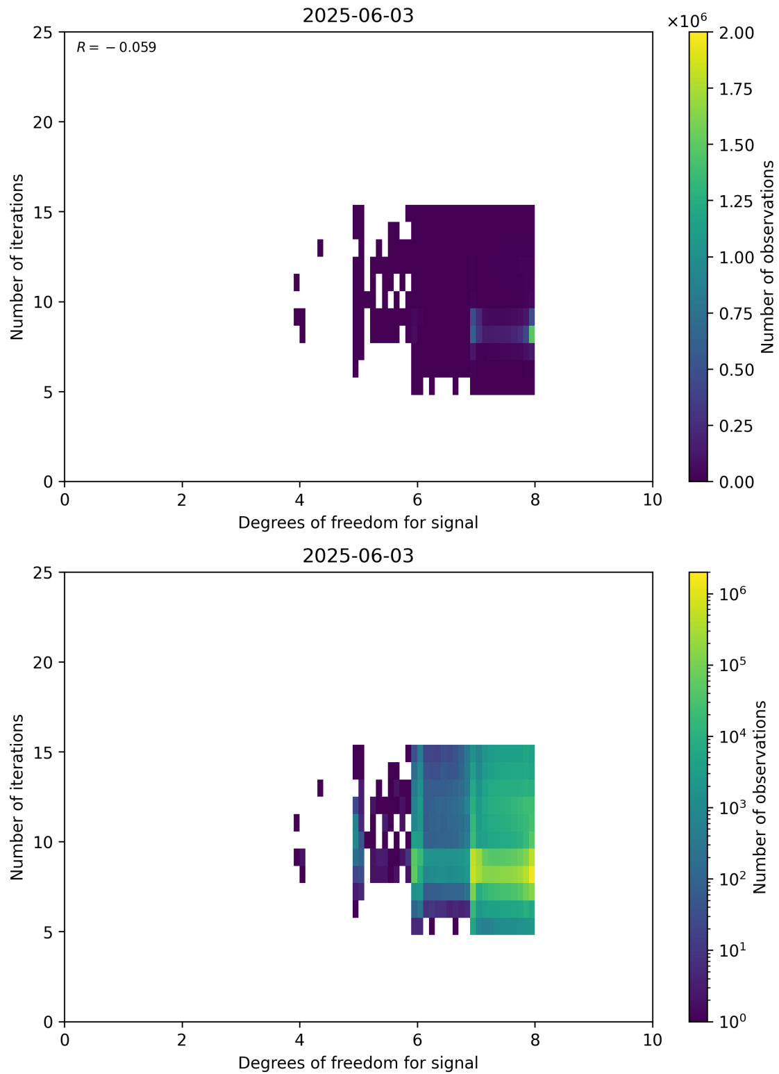
Figure 50: Scatter density plot of “Degrees of freedom for signal” against “Number of iterations” for 2025-06-02 to 2025-06-04.
