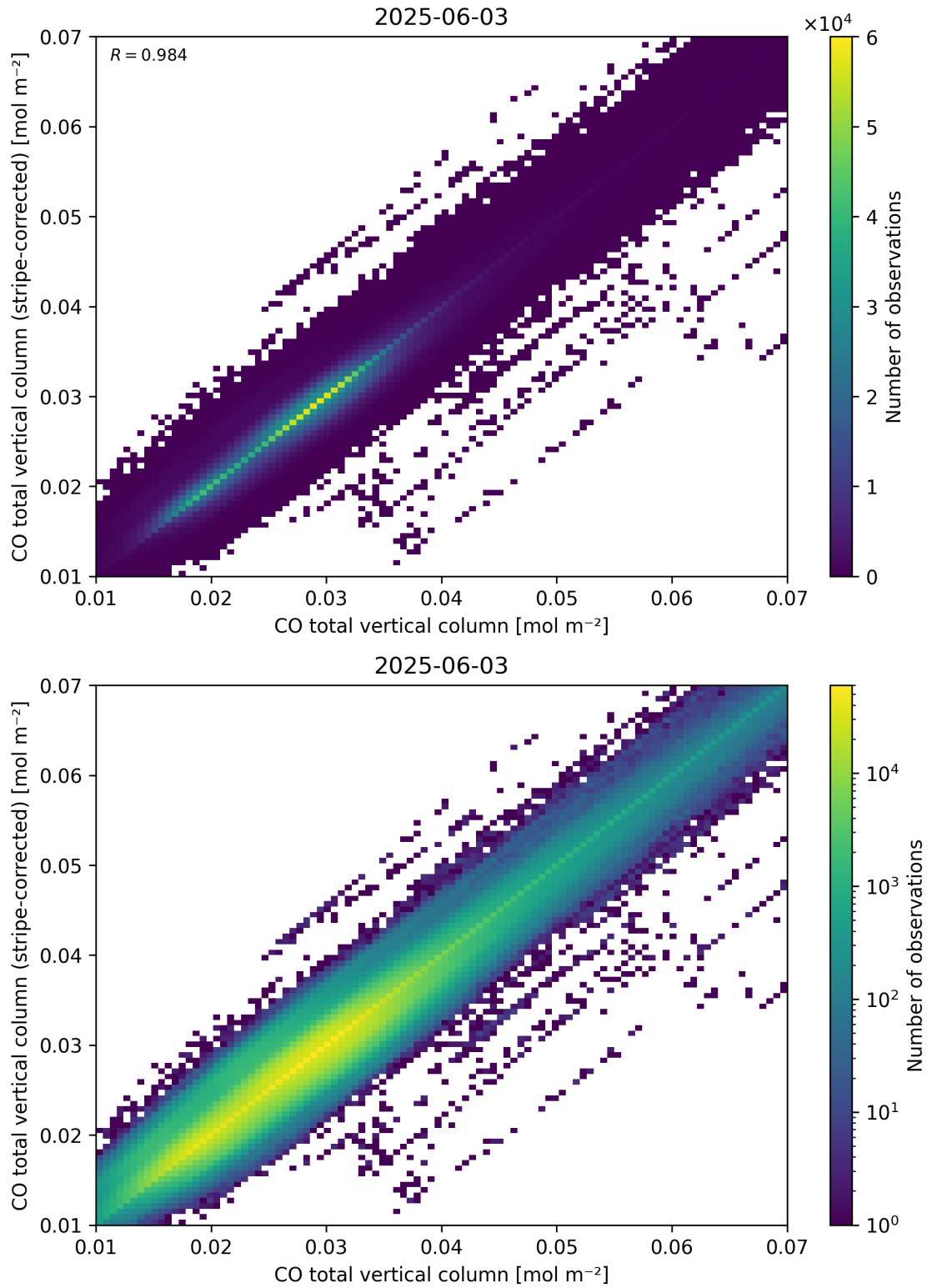
Figure 33: Scatter density plot of “CO total vertical column” against “CO total vertical column (stripe-corrected)” for 2025-06-02 to 2025-06-04.
