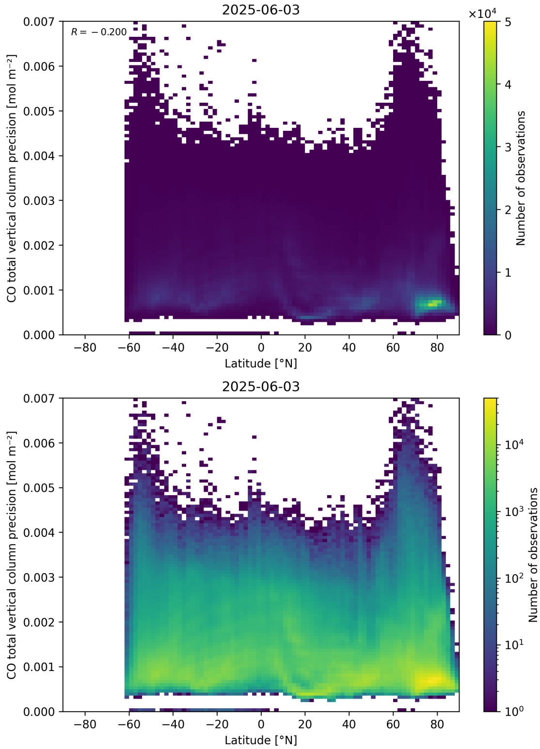
Figure 53: Scatter density plot of “Latitude” against “CO total vertical column precision” for 2025-06-02 to 2025-06-04.
