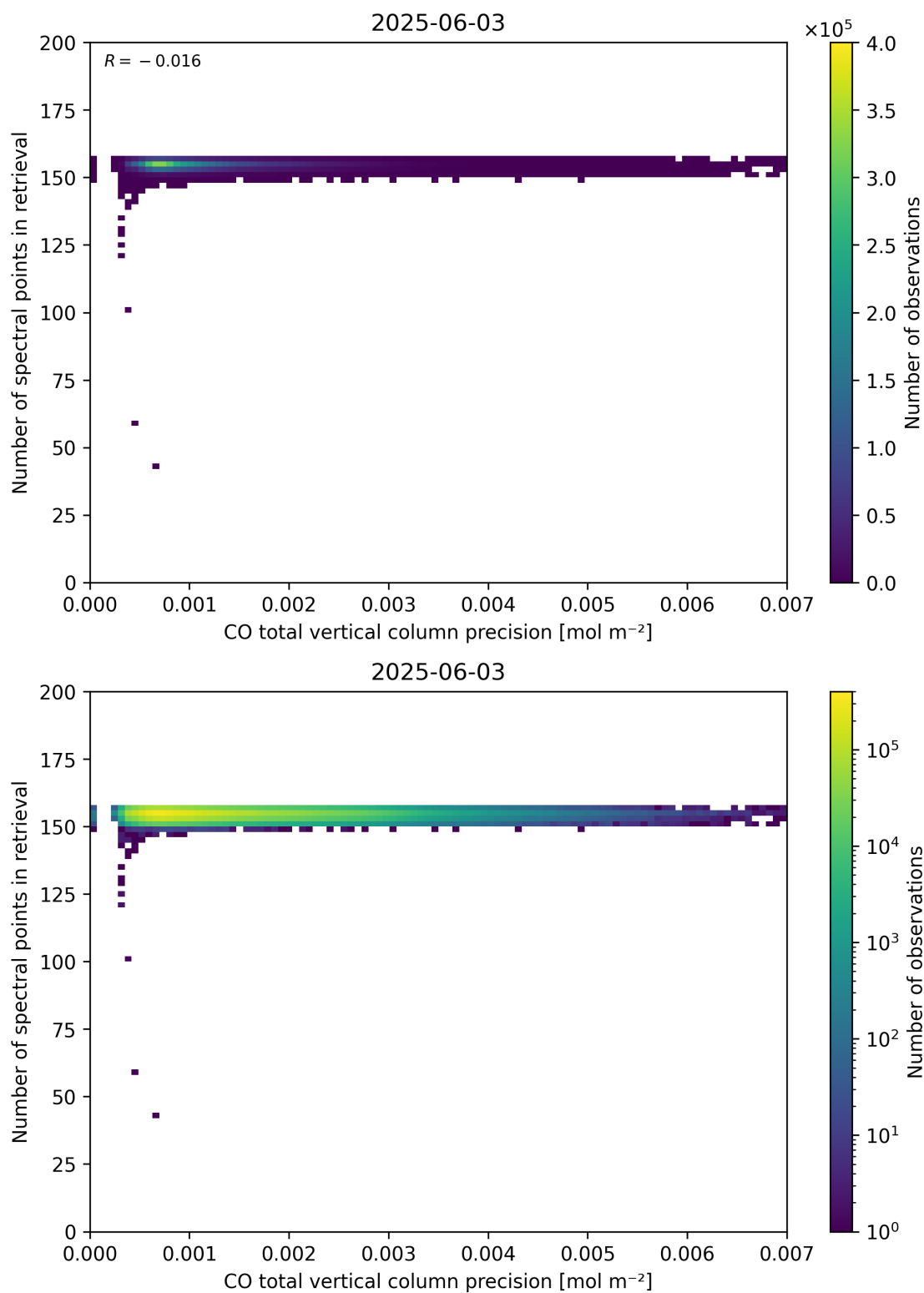
Figure 47: Scatter density plot of “CO total vertical column precision” against “Number of spectral points in retrieval” for 2025-06-02 to 2025-06-04.
