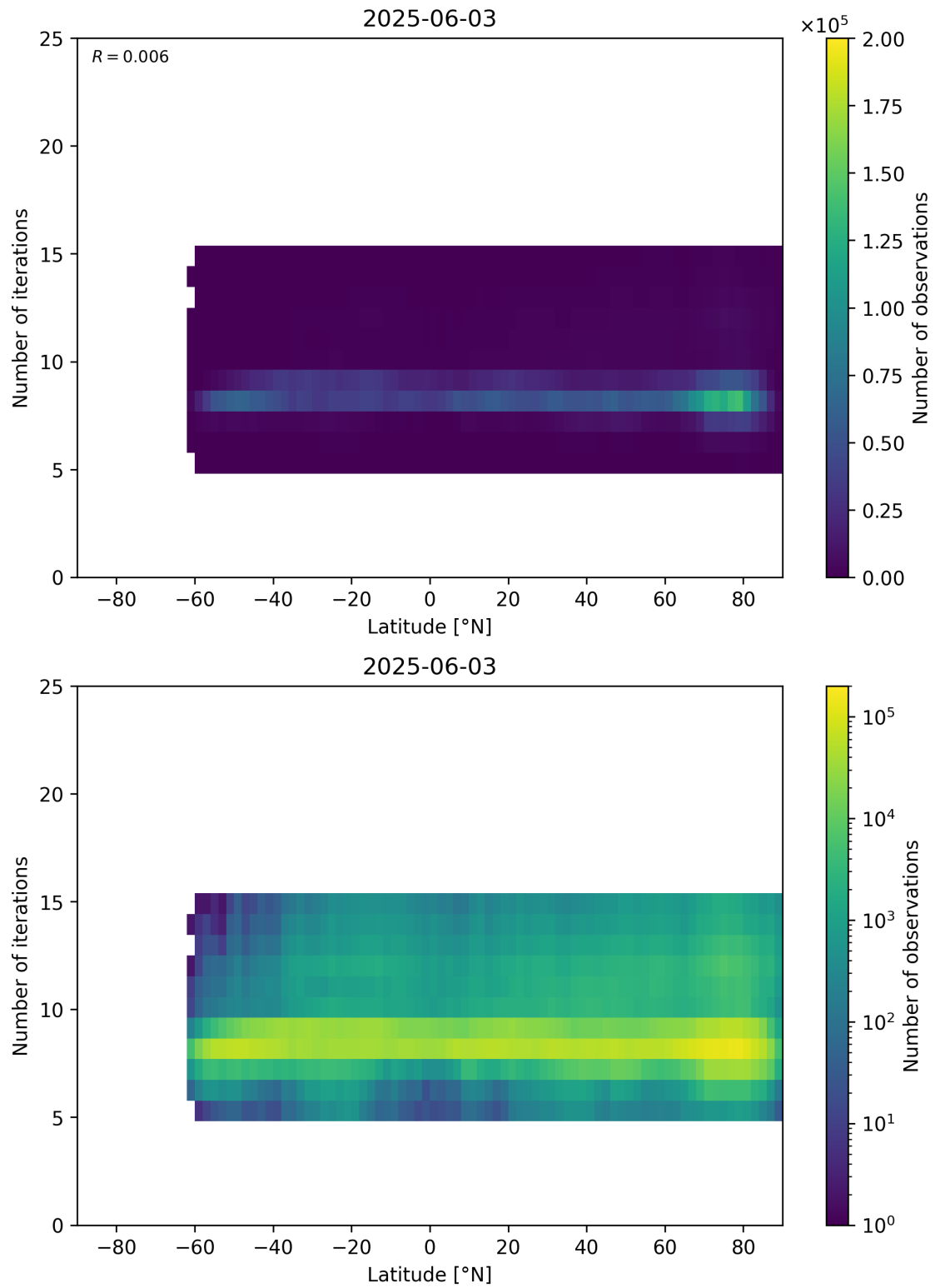
Figure 56: Scatter density plot of “Latitude” against “Number of iterations” for 2025-06-02 to 2025-06-04.
