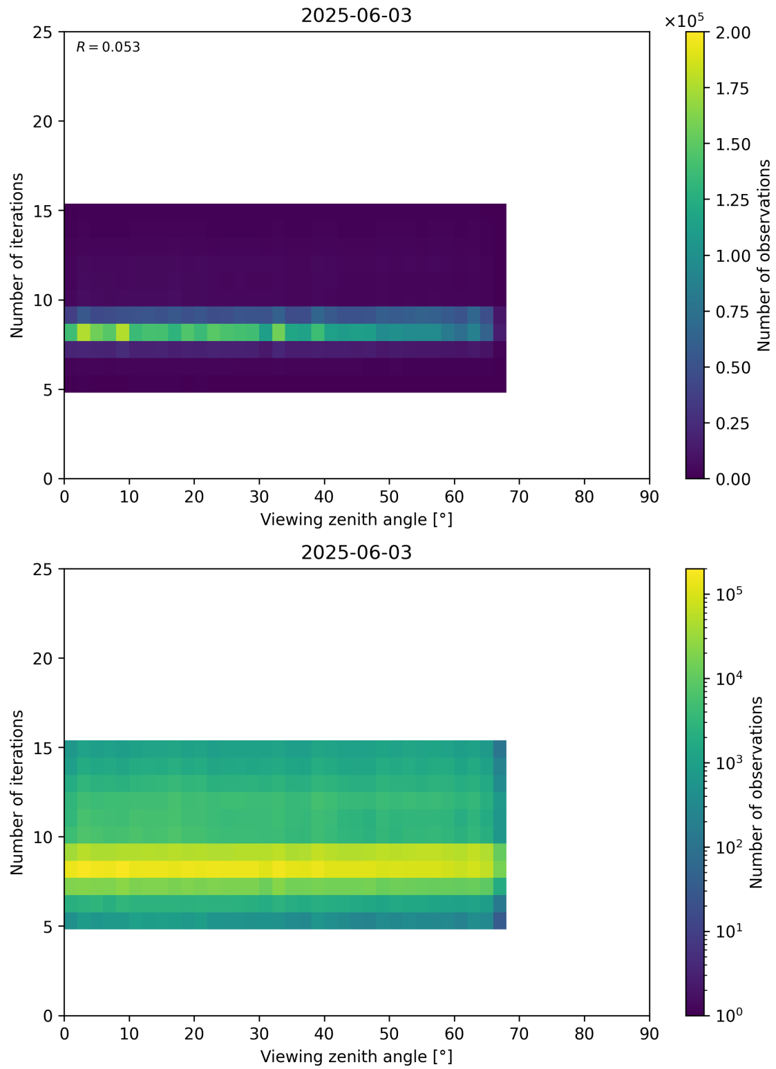
Figure 75: Scatter density plot of “Viewing zenith angle” against “Number of iterations” for 2025-06-02 to 2025-06-04.
