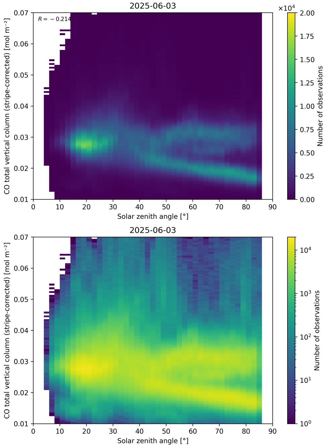
Figure 62: Scatter density plot of “Solar zenith angle” against “CO total vertical column (stripe-corrected)” for 2025-06-02 to 2025-06-04.
