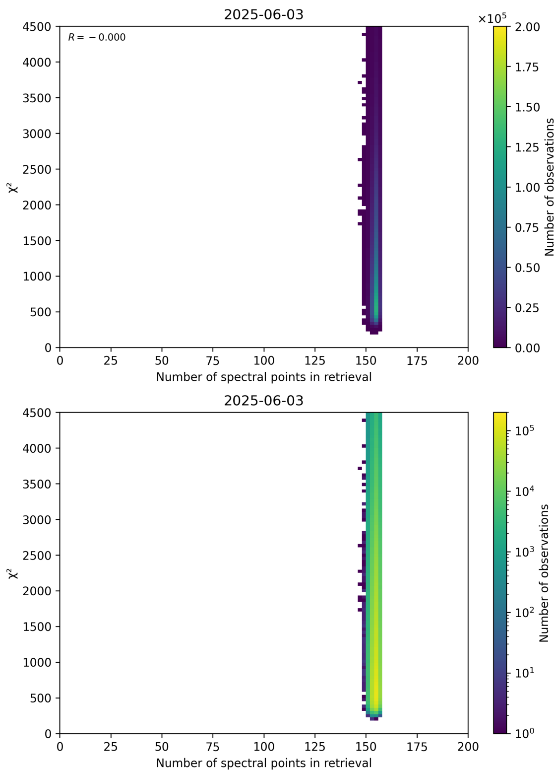
Figure 58: Scatter density plot of “Number of spectral points in retrieval” against “ \chi^2 ” for 2025-06-02 to 2025-06-04.
