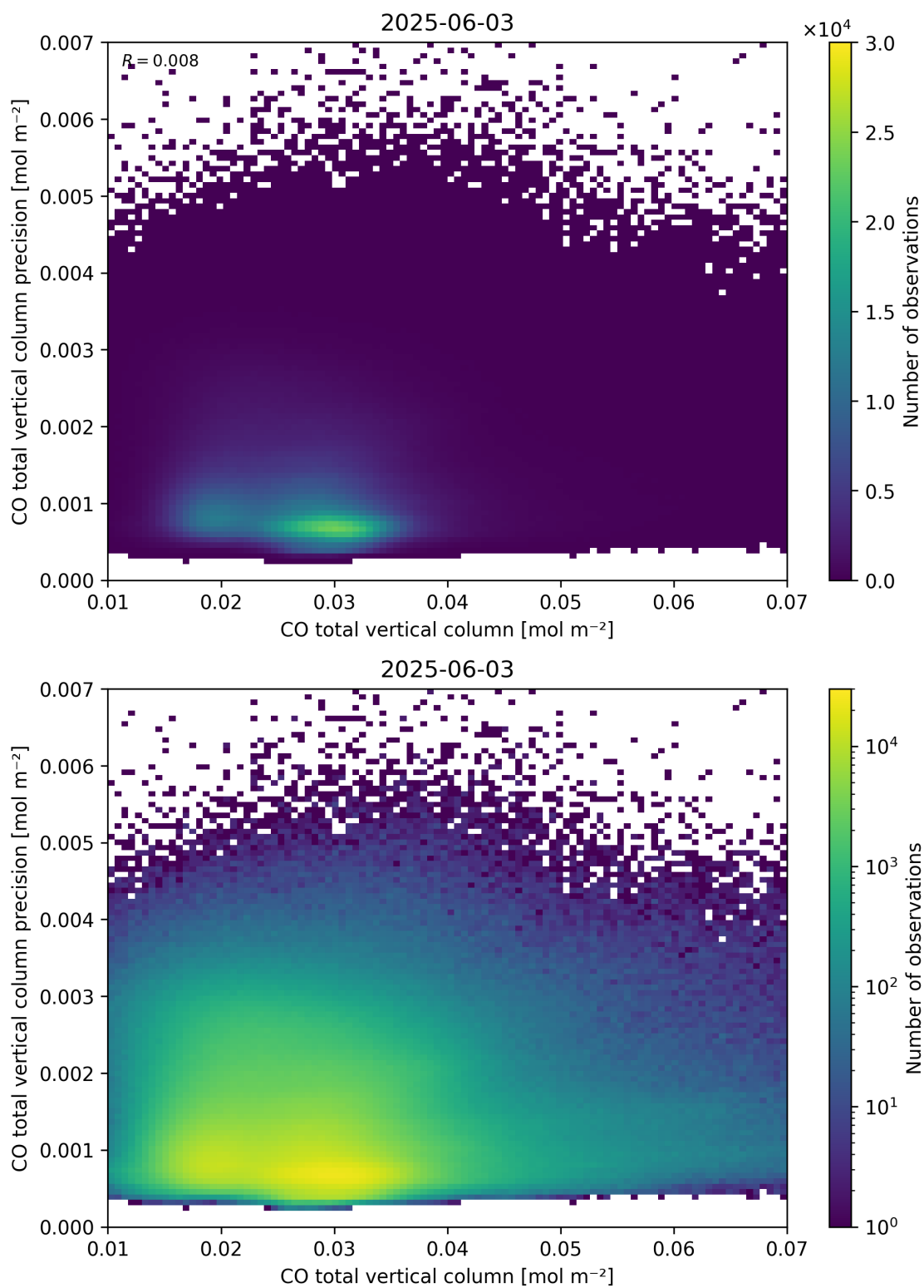
Figure 34: Scatter density plot of “CO total vertical column” against “CO total vertical column precision” for 2025-06-02 to 2025-06-04.
