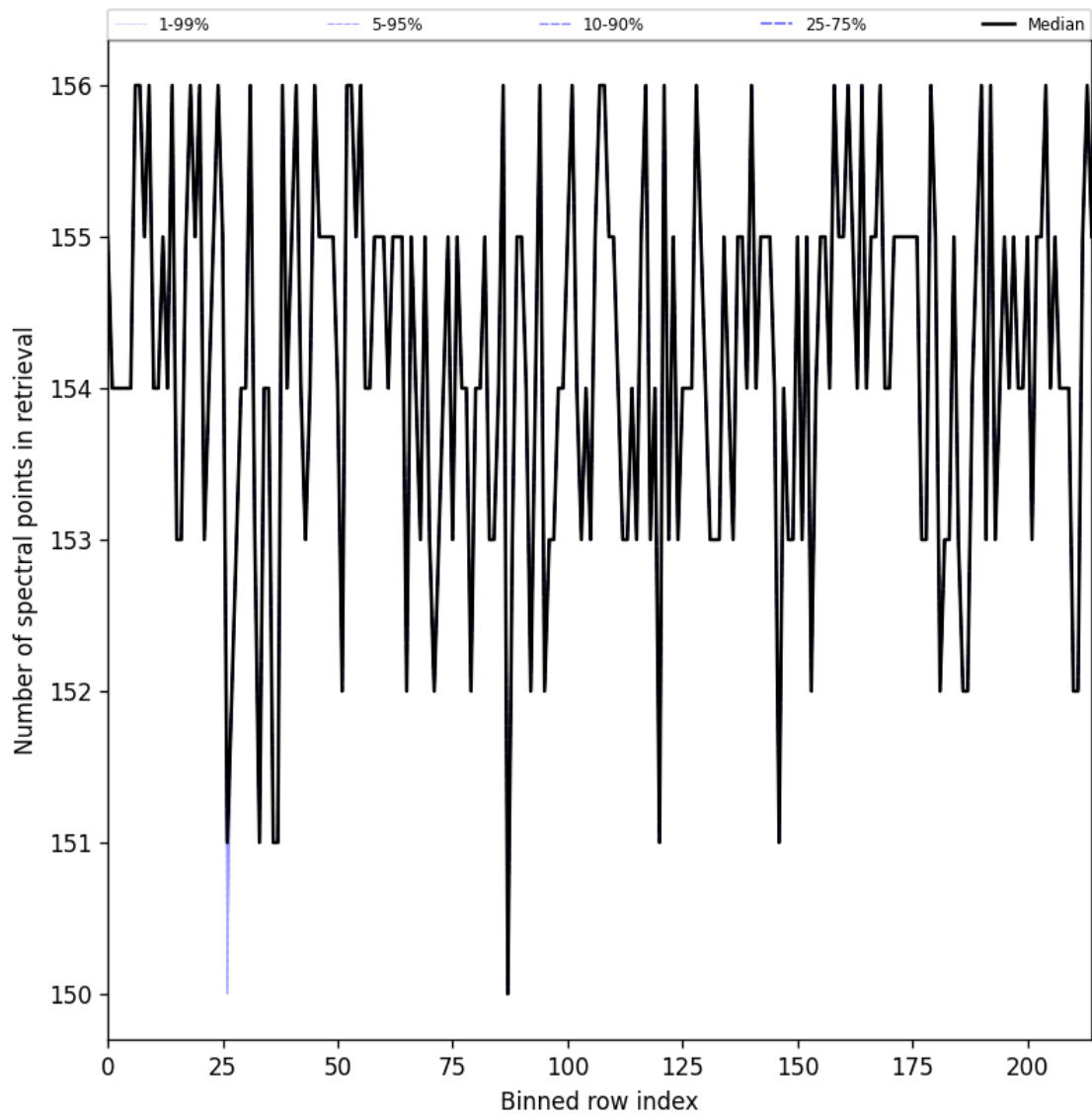
Figure 29: Along track statistics of “Number of spectral points in retrieval” for 2025-06-02 to 2025-06-04
