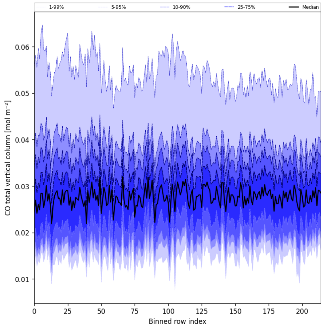
Figure 26: Along track statistics of “CO total vertical column” for 2025-06-02 to 2025-06-04
