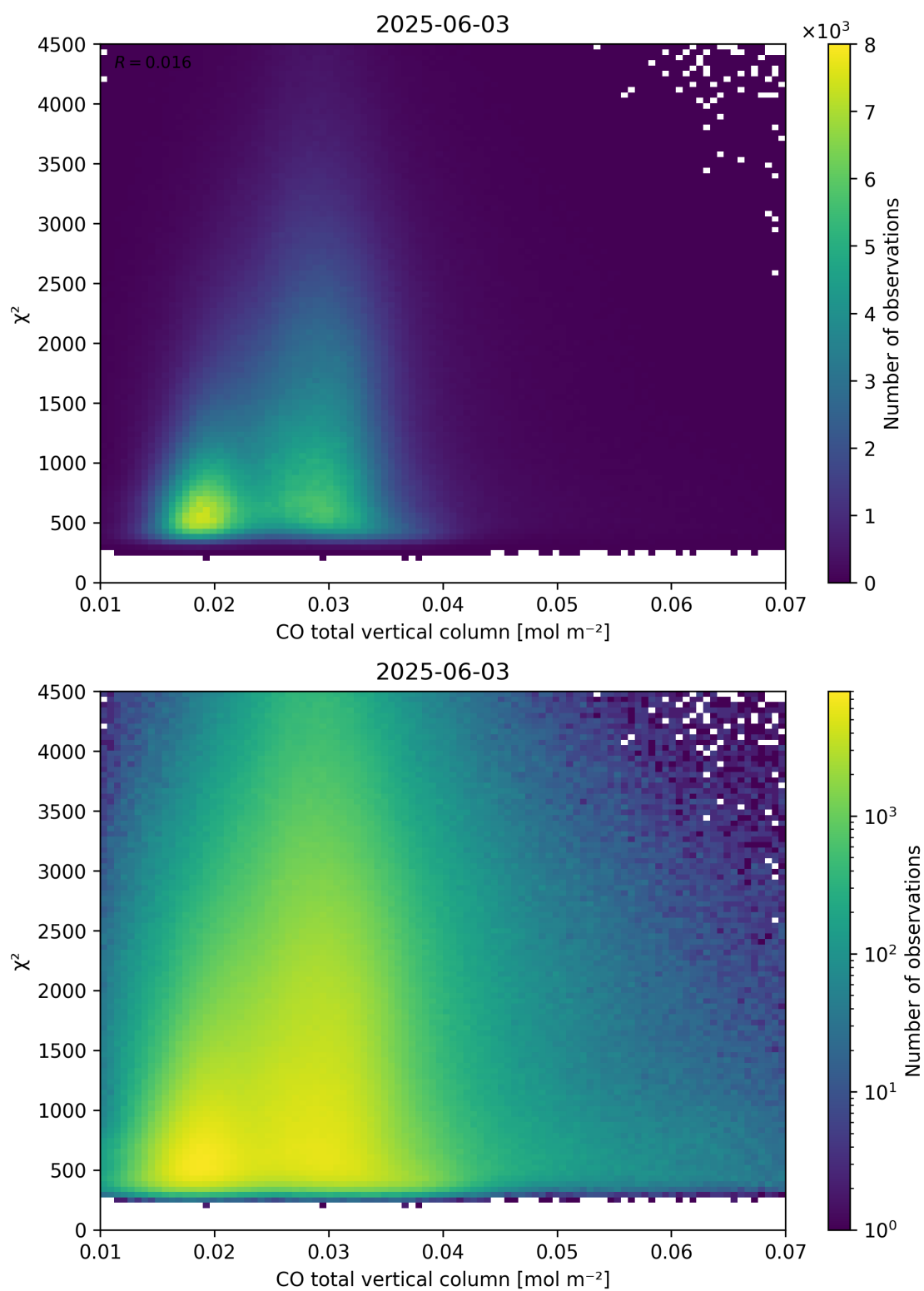
Figure 35: Scatter density plot of “CO total vertical column” against “ \chi^2 ” for 2025-06-02 to 2025-06-04.
