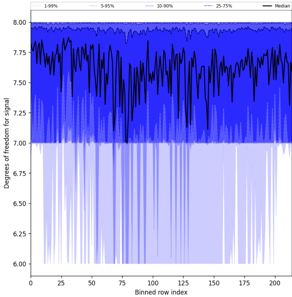
Figure 31: Along track statistics of “Degrees of freedom for signal” for 2025-06-02 to 2025-06-04
