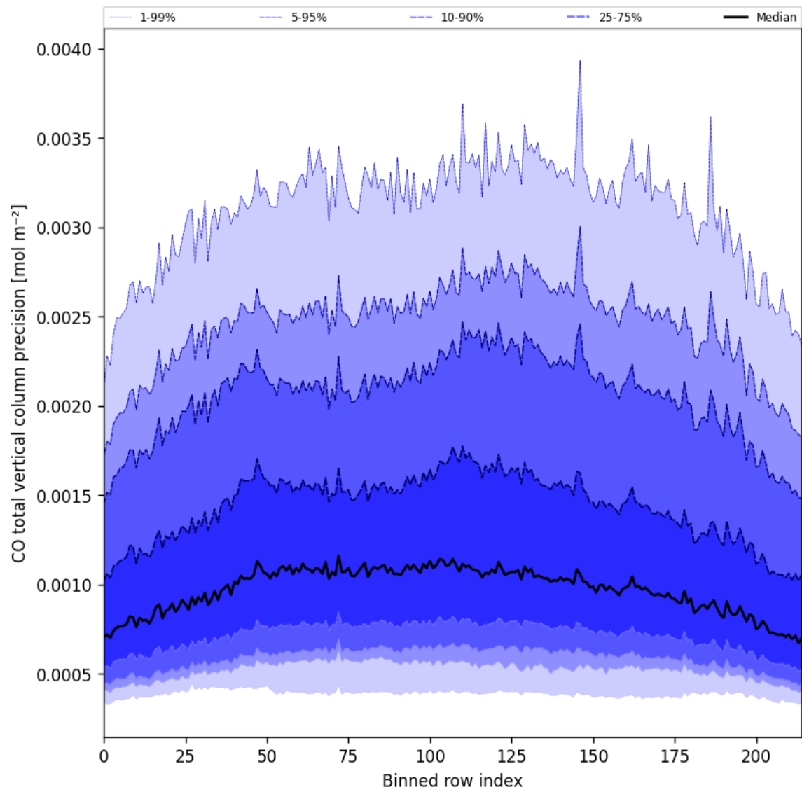
Figure 28: Along track statistics of “CO total vertical column precision” for 2025-06-02 to 2025-06-04
