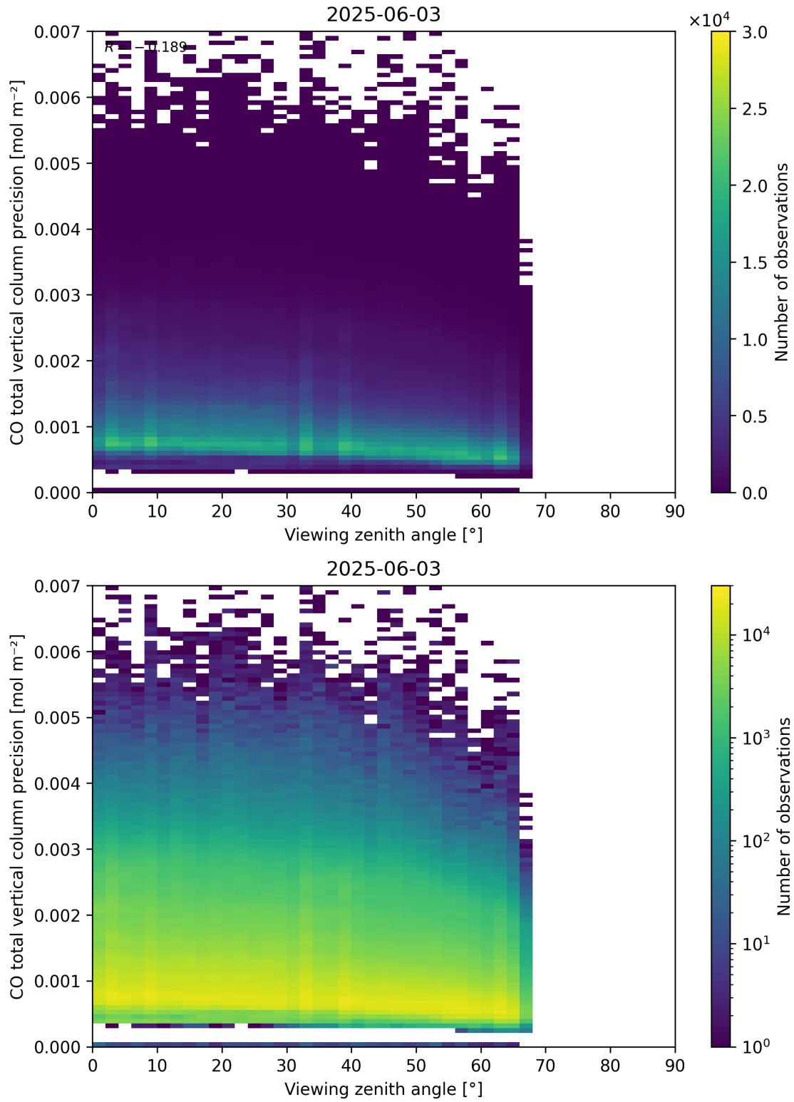
Figure 71: Scatter density plot of “Viewing zenith angle” against “CO total vertical column precision” for 2025-06-02 to 2025-06-04.
