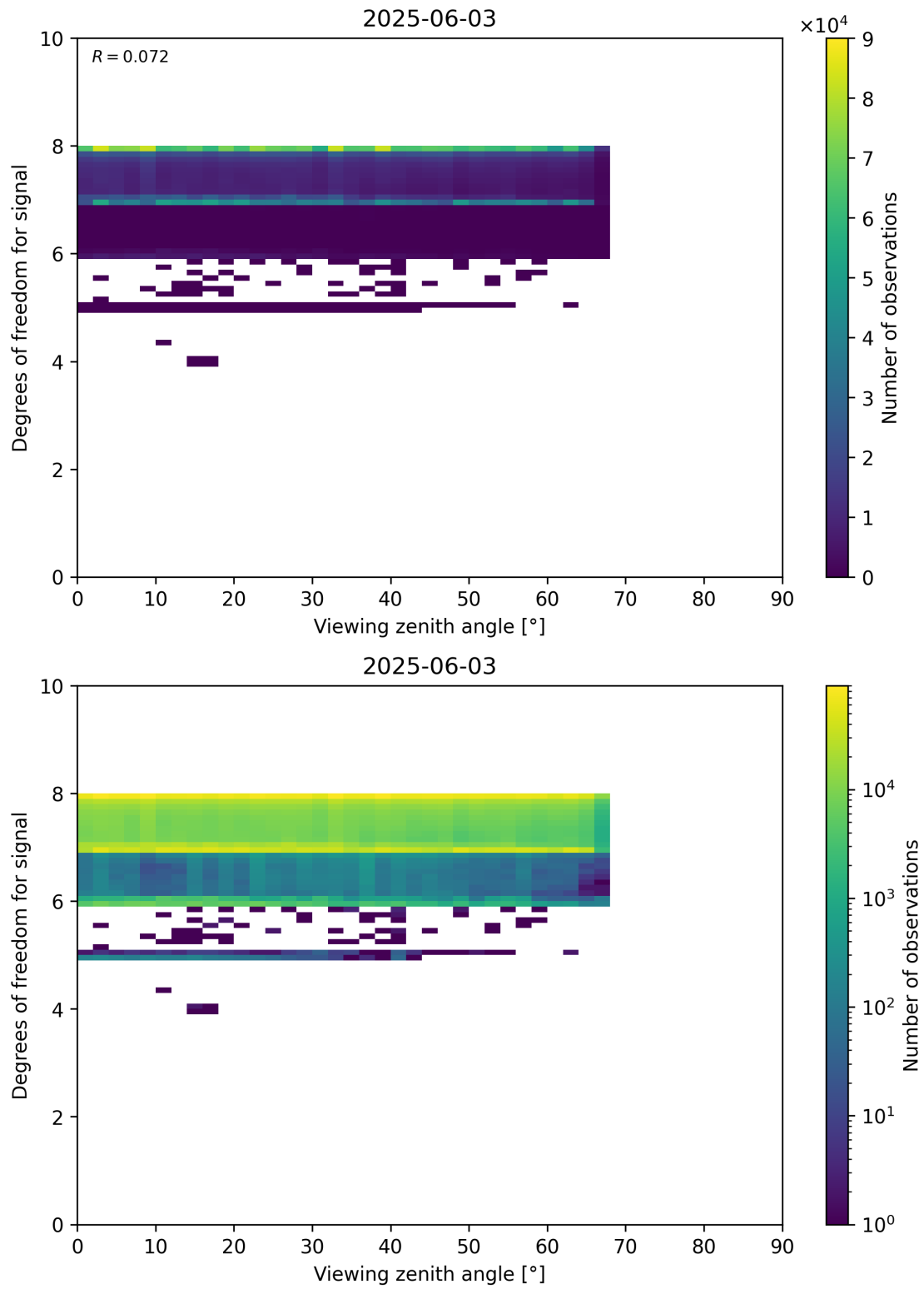
Figure 73: Scatter density plot of “Viewing zenith angle” against “Degrees of freedom for signal” for 2025-06-02 to 2025-06-04.
