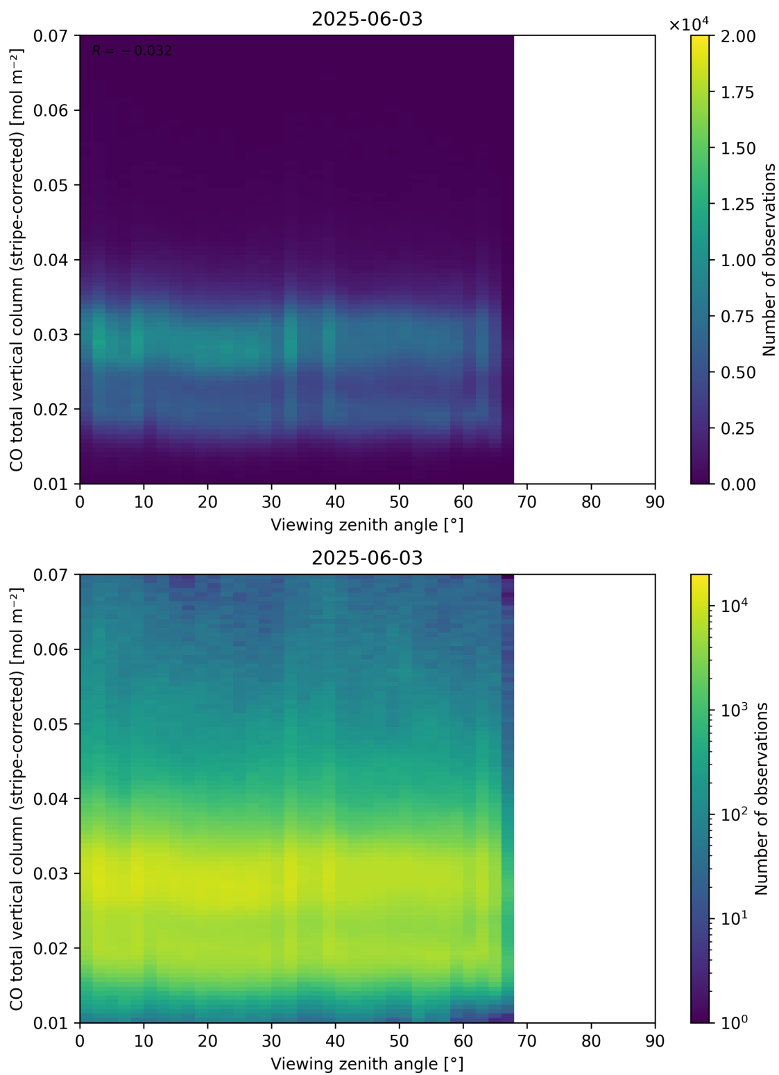
Figure 70: Scatter density plot of “Viewing zenith angle” against “CO total vertical column (stripe-corrected)” for 2025-06-02 to 2025-06-04.
