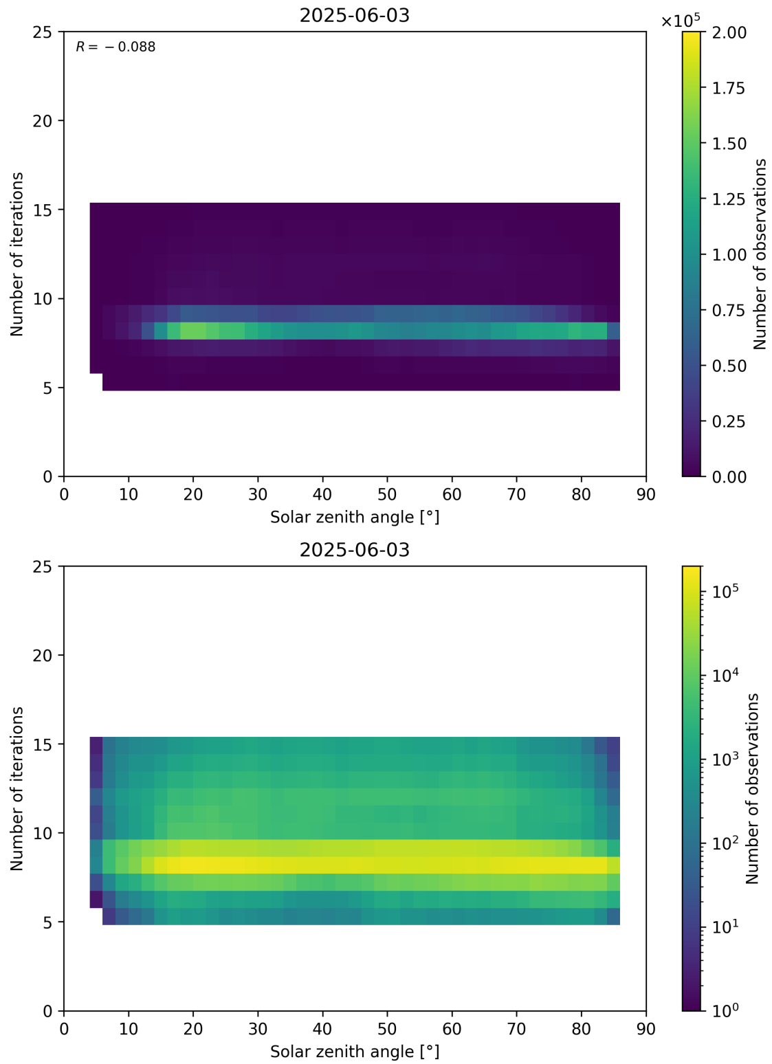
Figure 67: Scatter density plot of “Solar zenith angle” against “Number of iterations” for 2025-06-02 to 2025-06-04.
