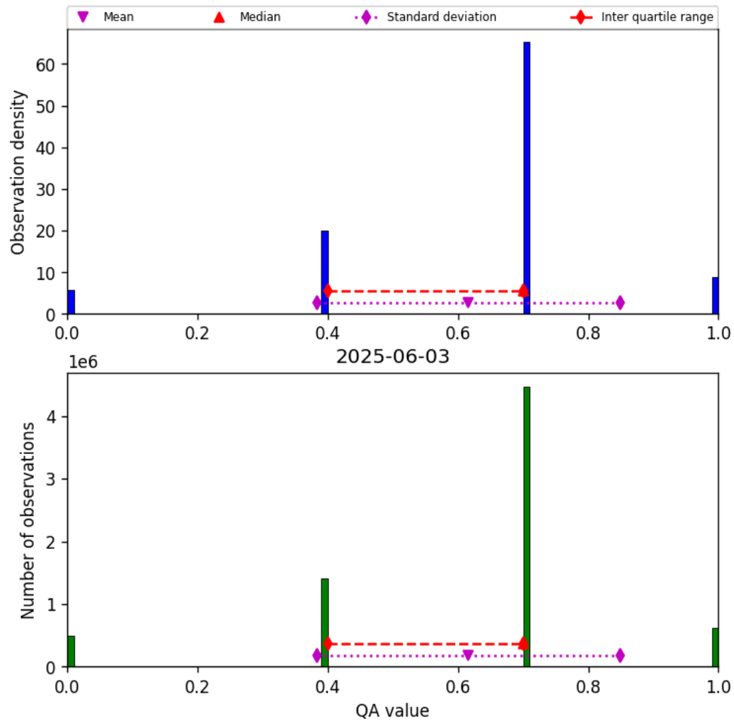
Figure 17: Histogram of “QA value” for 2025-06-02 to 2025-06-04
