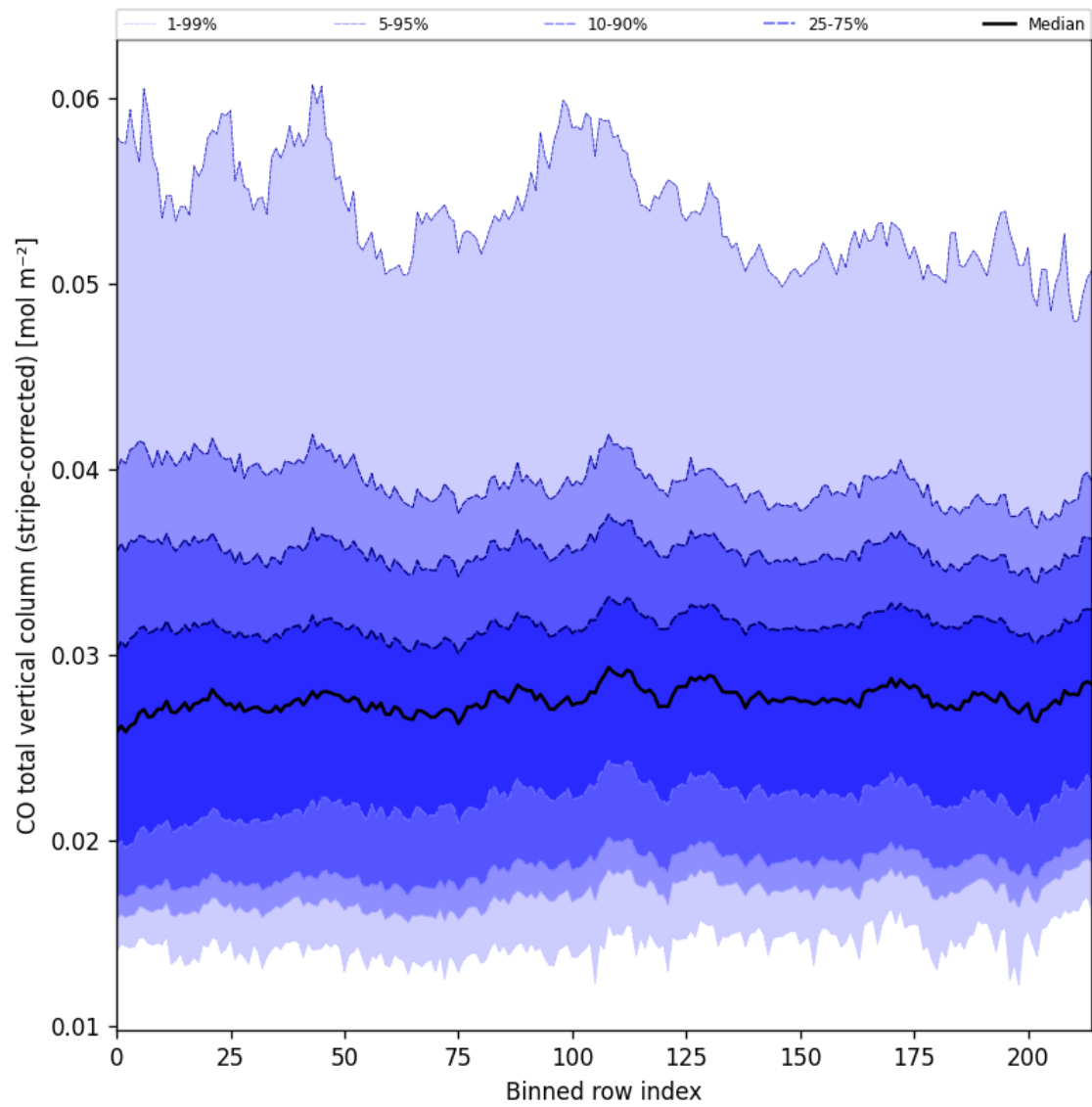
Figure 27: Along track statistics of “CO total vertical column (stripe-corrected)” for 2025-06-02 to 2025-06-04
