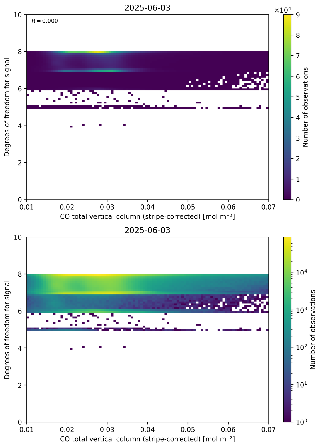
Figure 38: Scatter density plot of “CO total vertical column (stripe-corrected)” against “Degrees of freedom for signal” for 2025-06-02 to 2025-06-04.
