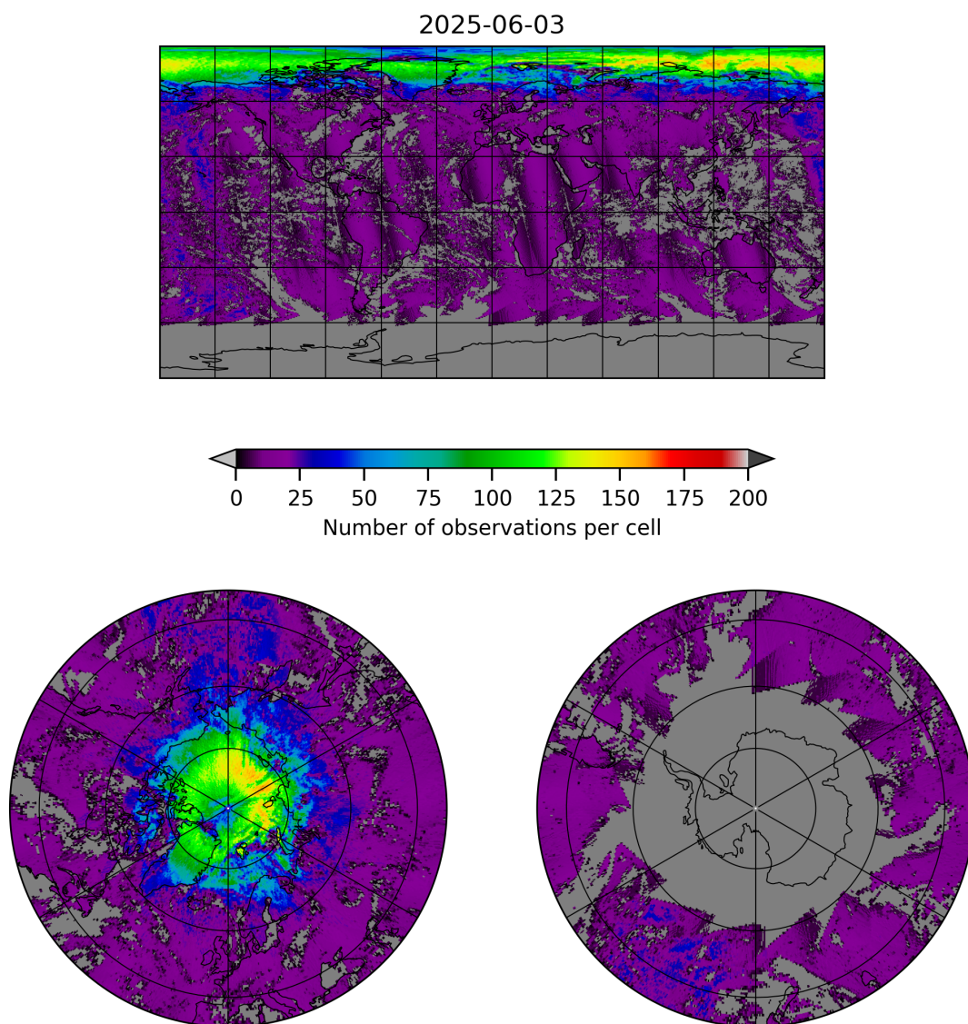
Figure 8: Map of the number of observations for 2025-06-02 to 2025-06-04
