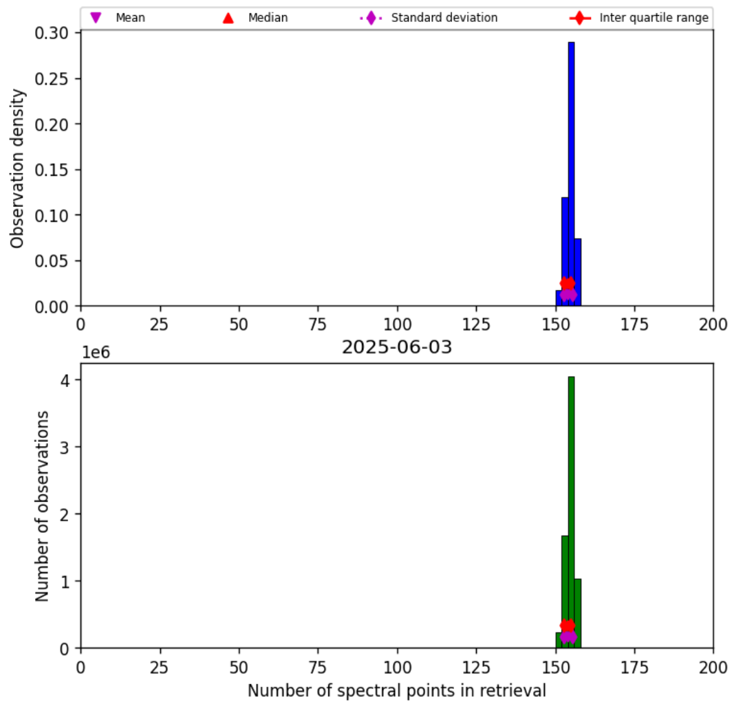
Figure 21: Histogram of “Number of spectral points in retrieval” for 2025-06-02 to 2025-06-04
