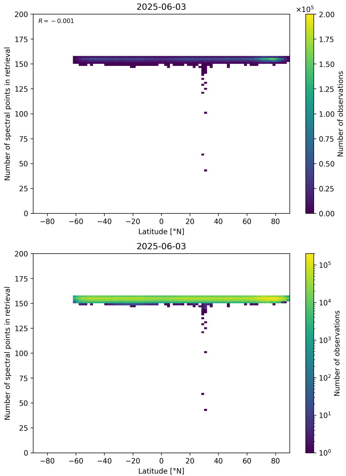
Figure 57: Scatter density plot of “Latitude” against “Number of spectral points in retrieval” for 2025-06-02 to 2025-06-04.
