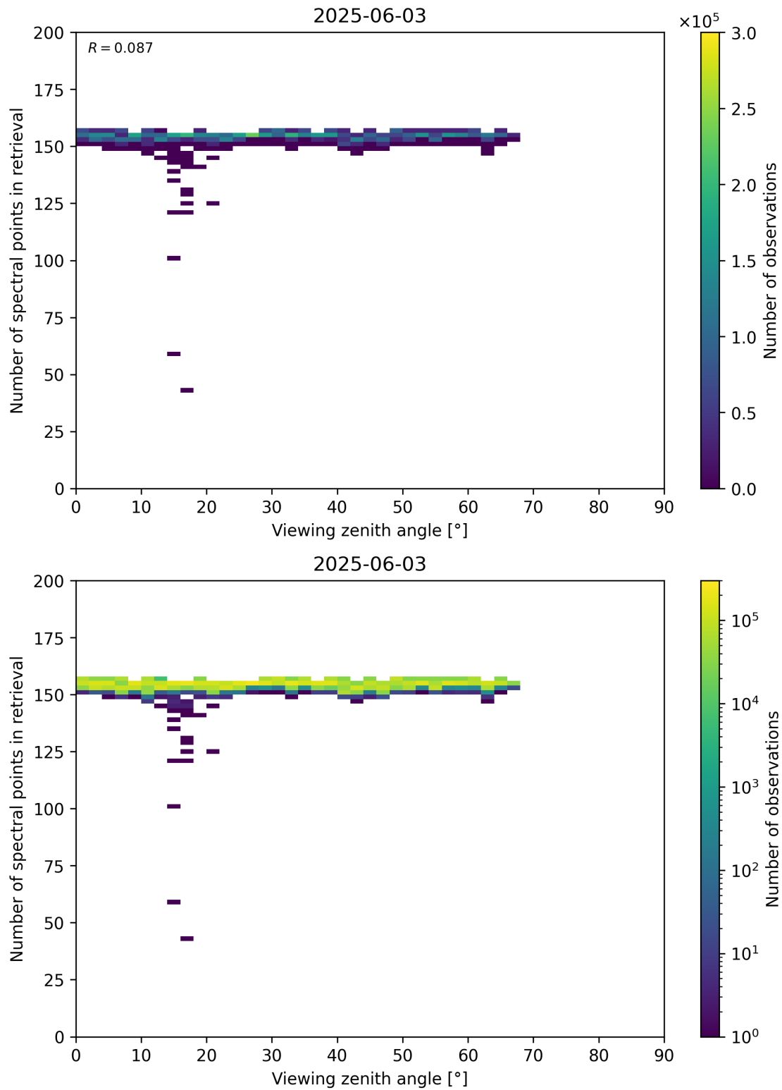
Figure 76: Scatter density plot of “Viewing zenith angle” against “Number of spectral points in retrieval” for 2025-06-02 to 2025-06-04.
