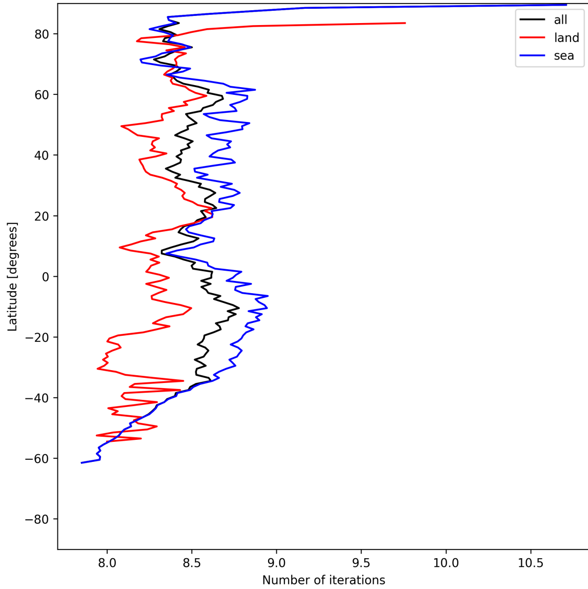
Figure 16: Zonal average of “Number of iterations” for 2025-06-02 to 2025-06-04.
