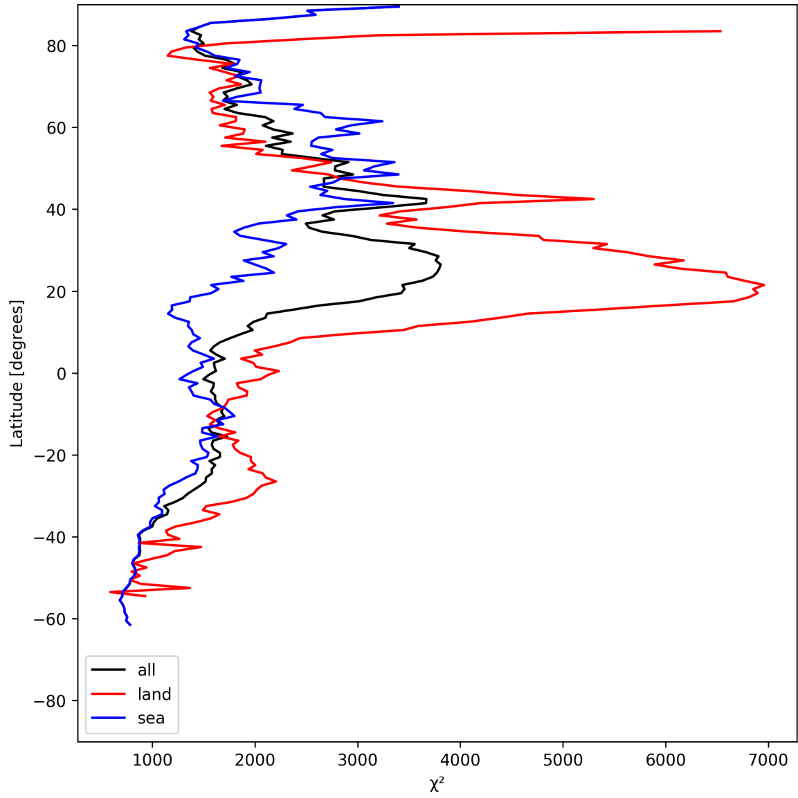
Figure 14: Zonal average of “ \chi^2 ” for 2025-06-02 to 2025-06-04.
