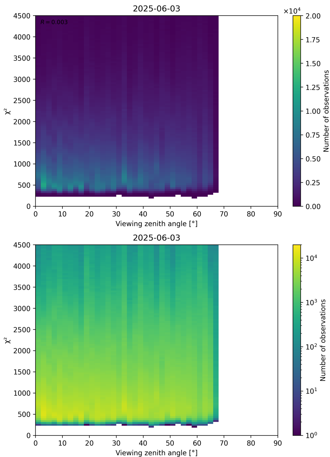
Figure 72: Scatter density plot of “Viewing zenith angle” against “ \chi^2 ” for 2025-06-02 to 2025-06-04.
