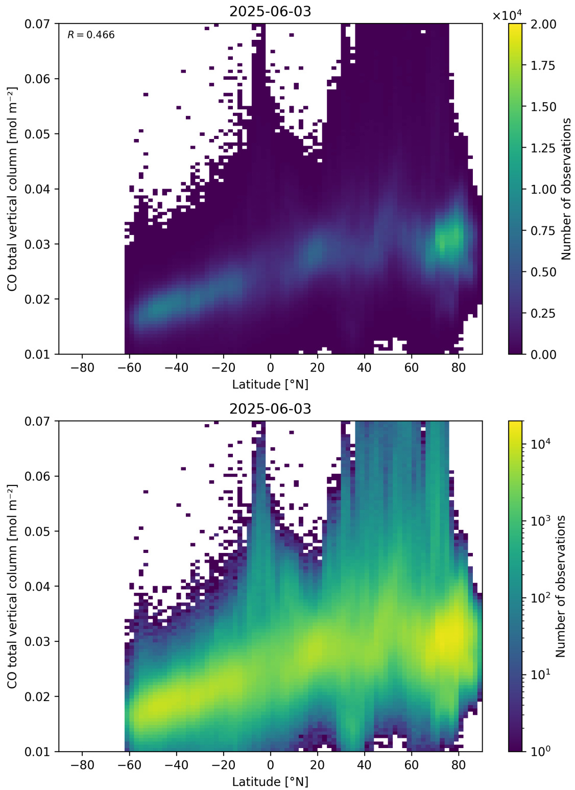
Figure 51: Scatter density plot of “Latitude” against “CO total vertical column” for 2025-06-02 to 2025-06-04.
