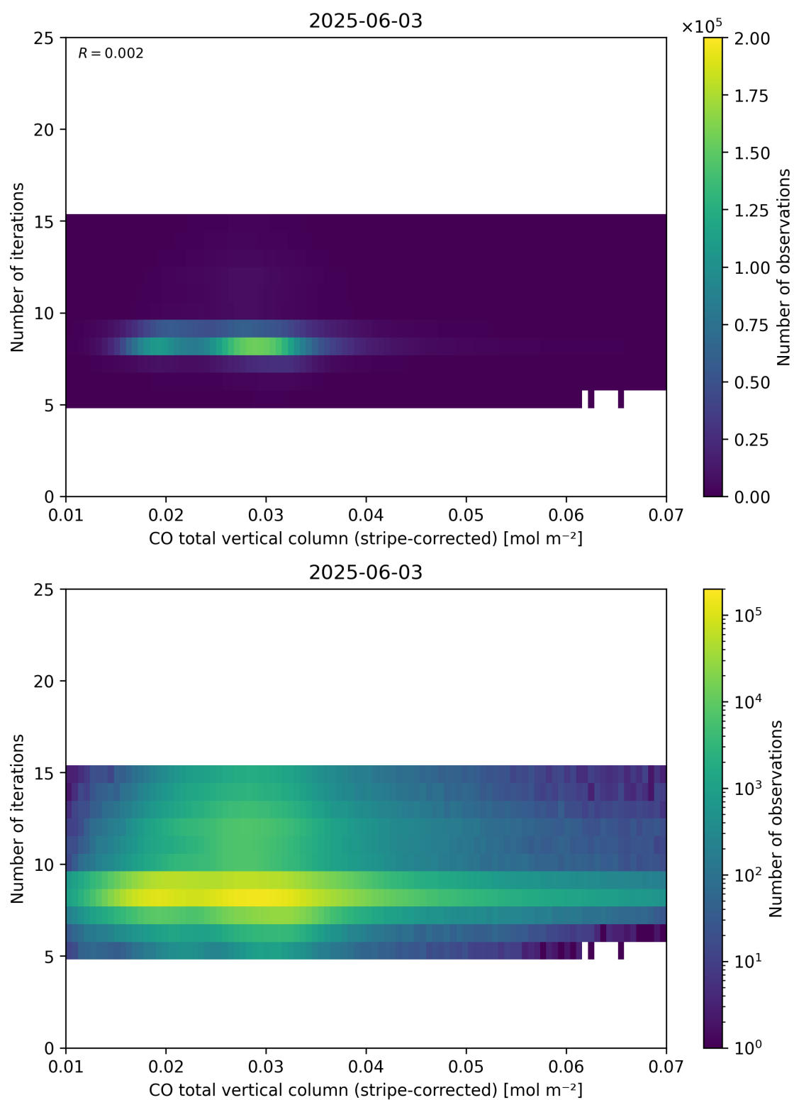
Figure 39: Scatter density plot of “CO total vertical column (stripe-corrected)” against “Number of iterations” for 2025-06-02 to 2025-06-04.
