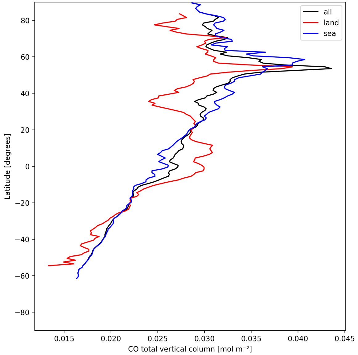
Figure 10: Zonal average of “CO total vertical column” for 2025-06-02 to 2025-06-04.
