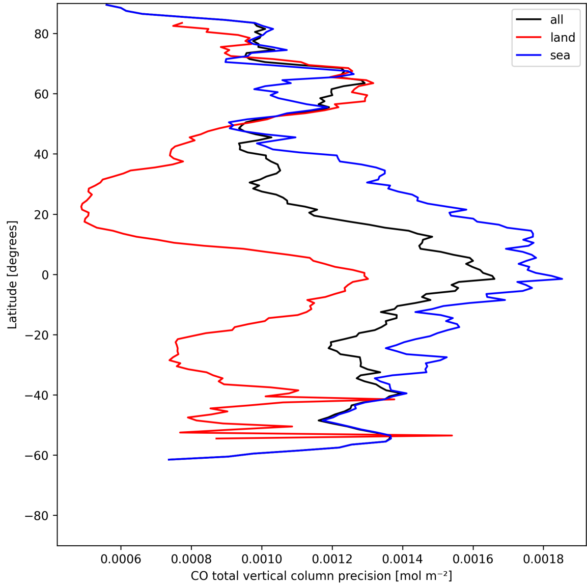
Figure 12: Zonal average of “CO total vertical column precision” for 2025-06-02 to 2025-06-04.
