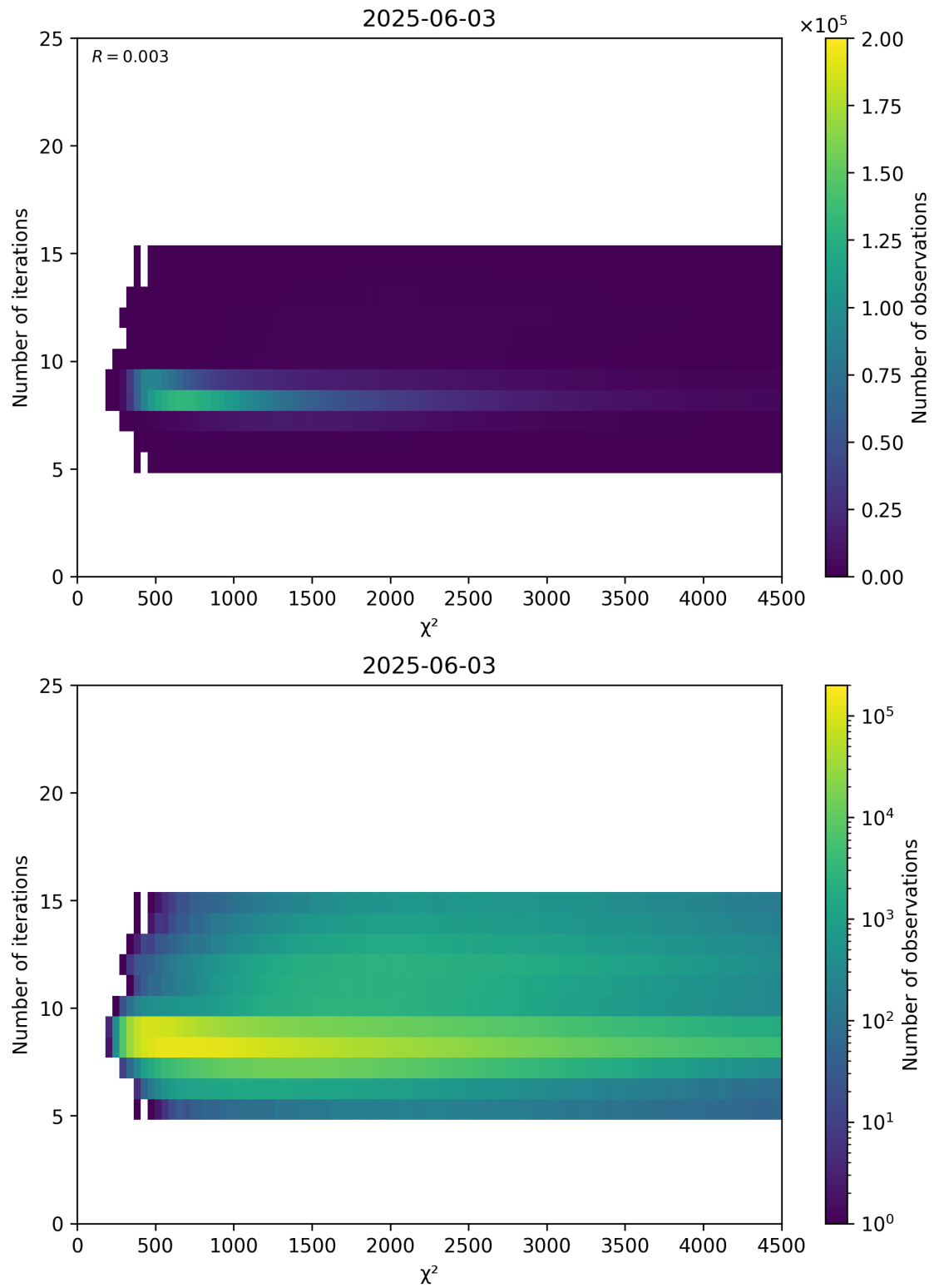
Figure 49: Scatter density plot of “ \chi^2 ” against “Number of iterations” for 2025-06-02 to 2025-06-04.
