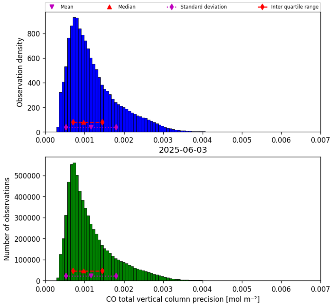
Figure 20: Histogram of “CO total vertical column precision” for 2025-06-02 to 2025-06-04
