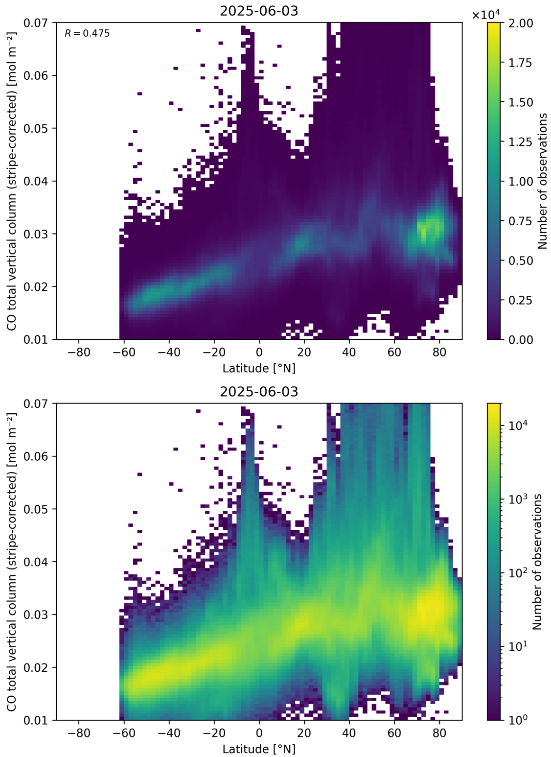
Figure 52: Scatter density plot of “Latitude” against “CO total vertical column (stripe-corrected)” for 2025-06-02 to 2025-06-04.
