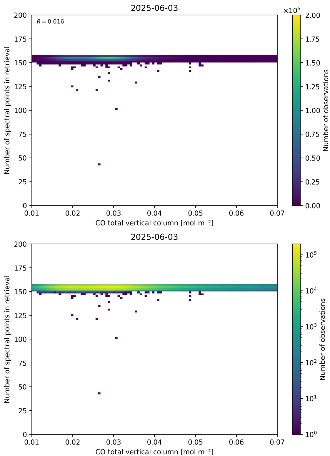
Figure 43: Scatter density plot of “CO total vertical column” against “Number of spectral points in retrieval” for 2025-06-02 to 2025-06-04.
