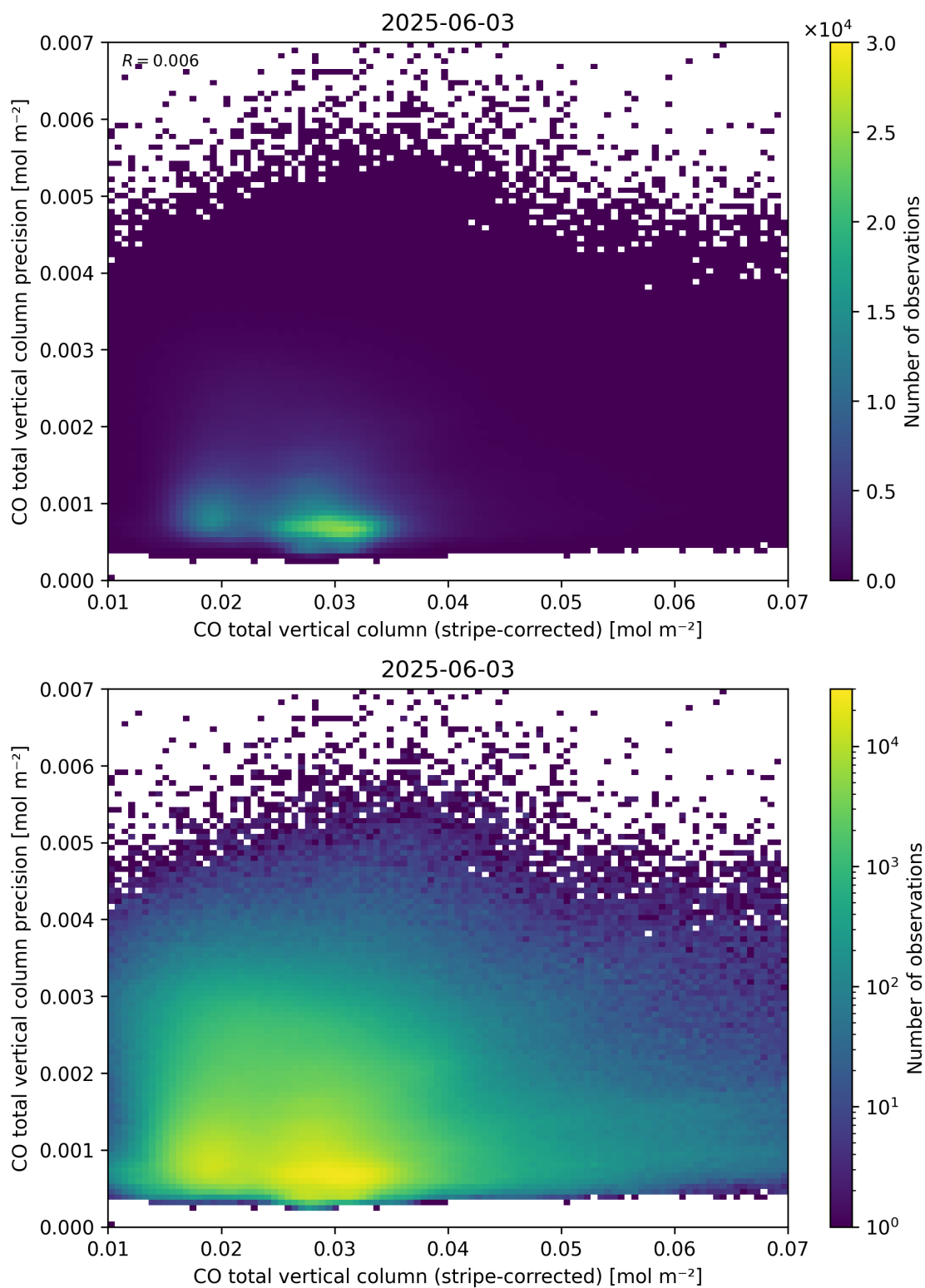
Figure 36: Scatter density plot of “CO total vertical column (stripe-corrected)” against “CO total vertical column precision” for 2025-06-02 to 2025-06-04.
