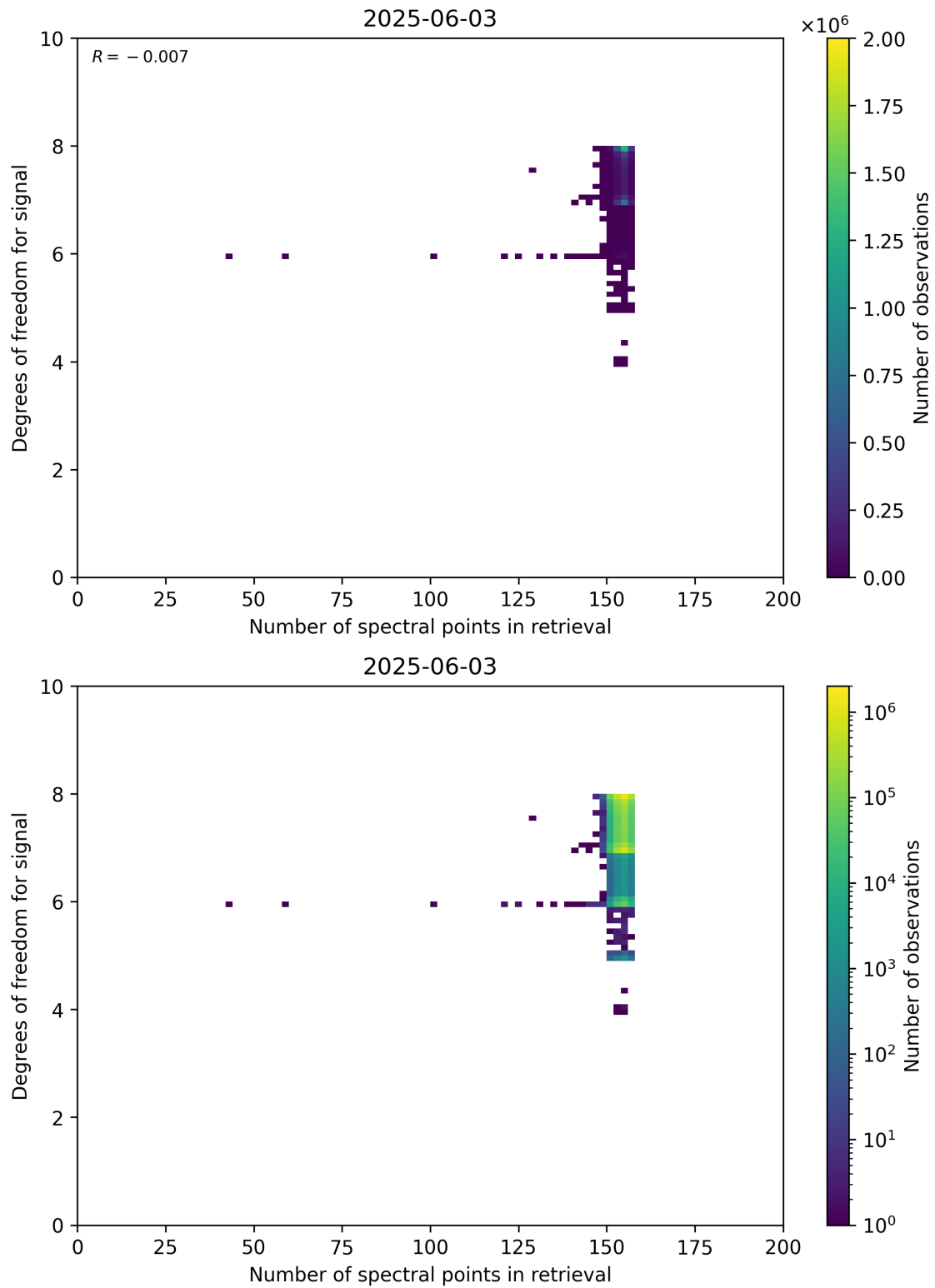
Figure 59: Scatter density plot of “Number of spectral points in retrieval” against “Degrees of freedom for signal” for 2025-06-02 to 2025-06-04.
