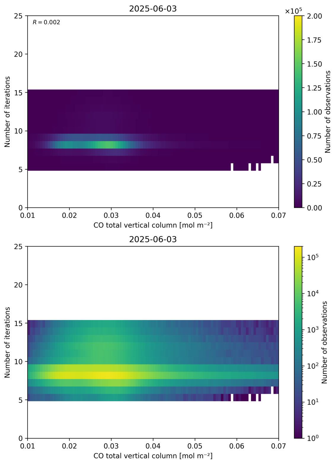
Figure 42: Scatter density plot of “CO total vertical column” against “Number of iterations” for 2025-06-02 to 2025-06-04.
