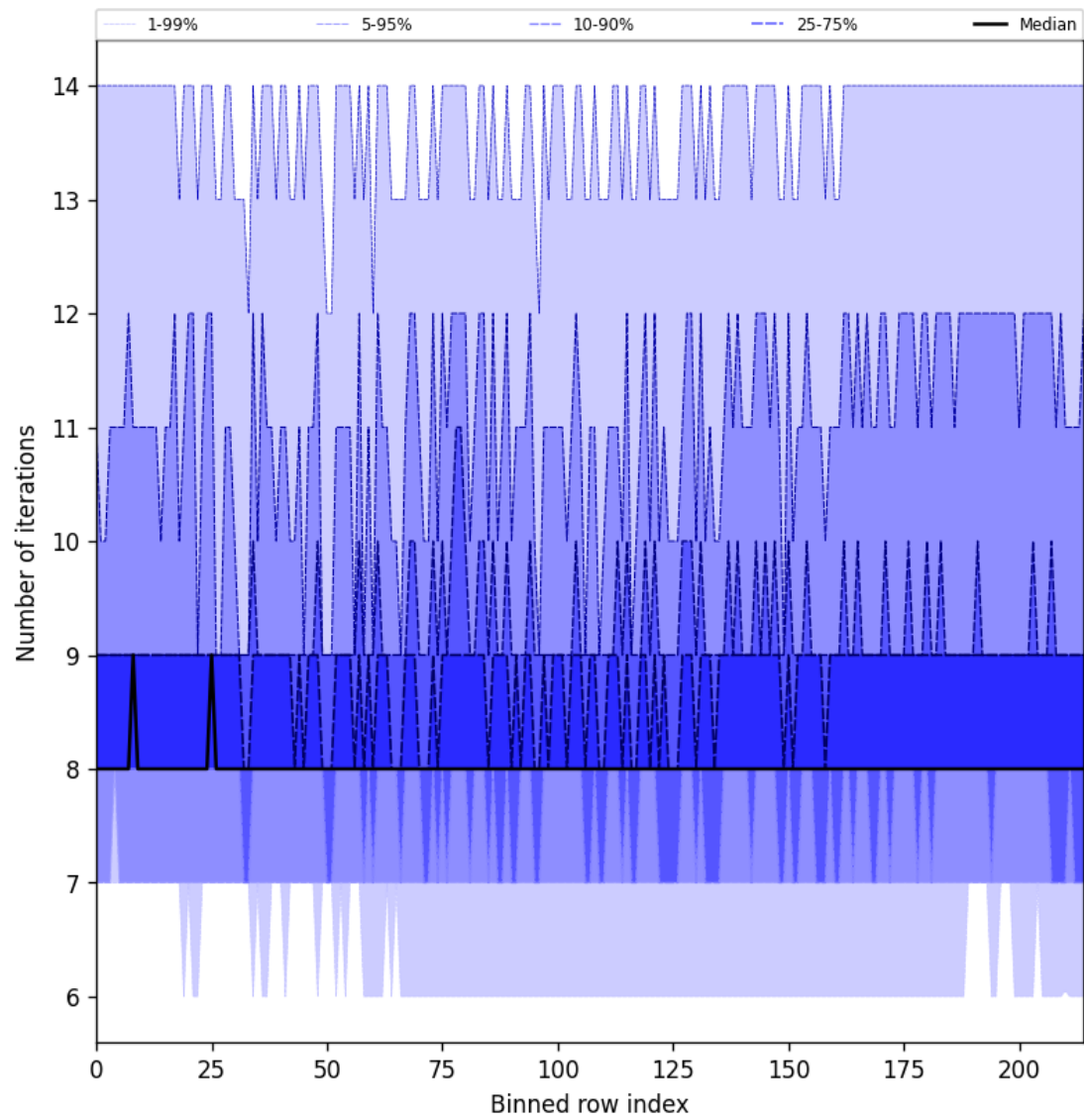
Figure 32: Along track statistics of “Number of iterations” for 2025-06-02 to 2025-06-04
