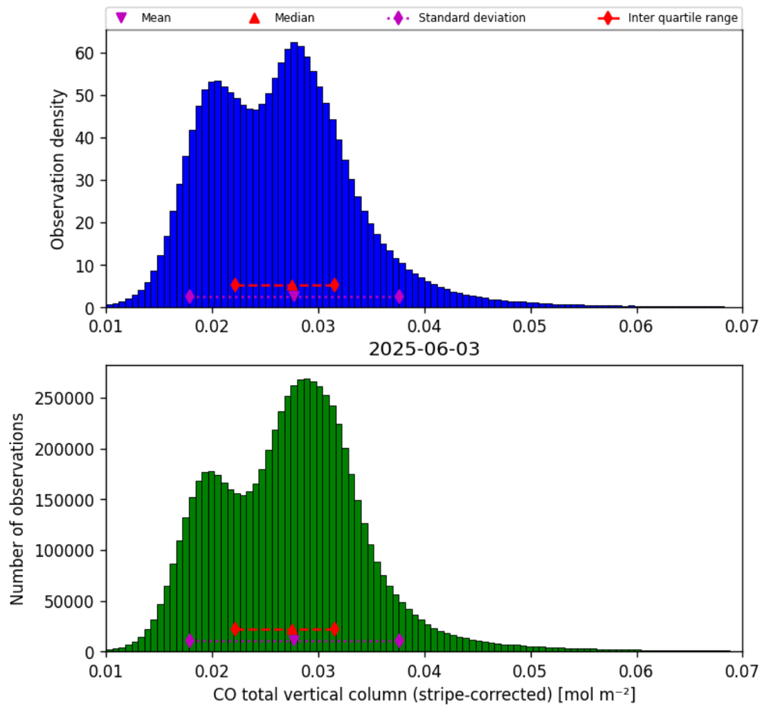
Figure 19: Histogram of “CO total vertical column (stripe-corrected)” for 2025-06-02 to 2025-06-04
