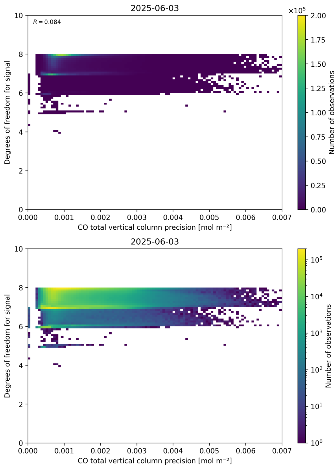
Figure 45: Scatter density plot of “CO total vertical column precision” against “Degrees of freedom for signal” for 2025-06-02 to 2025-06-04.
