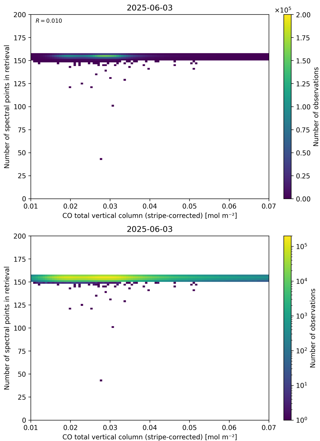
Figure 40: Scatter density plot of “CO total vertical column (stripe-corrected)” against “Number of spectral points in retrieval” for 2025-06-02 to 2025-06-04.
