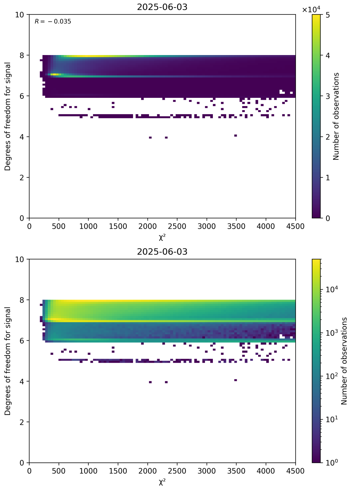
Figure 48: Scatter density plot of “ \chi^2 ” against “Degrees of freedom for signal” for 2025-06-02 to 2025-06-04.
