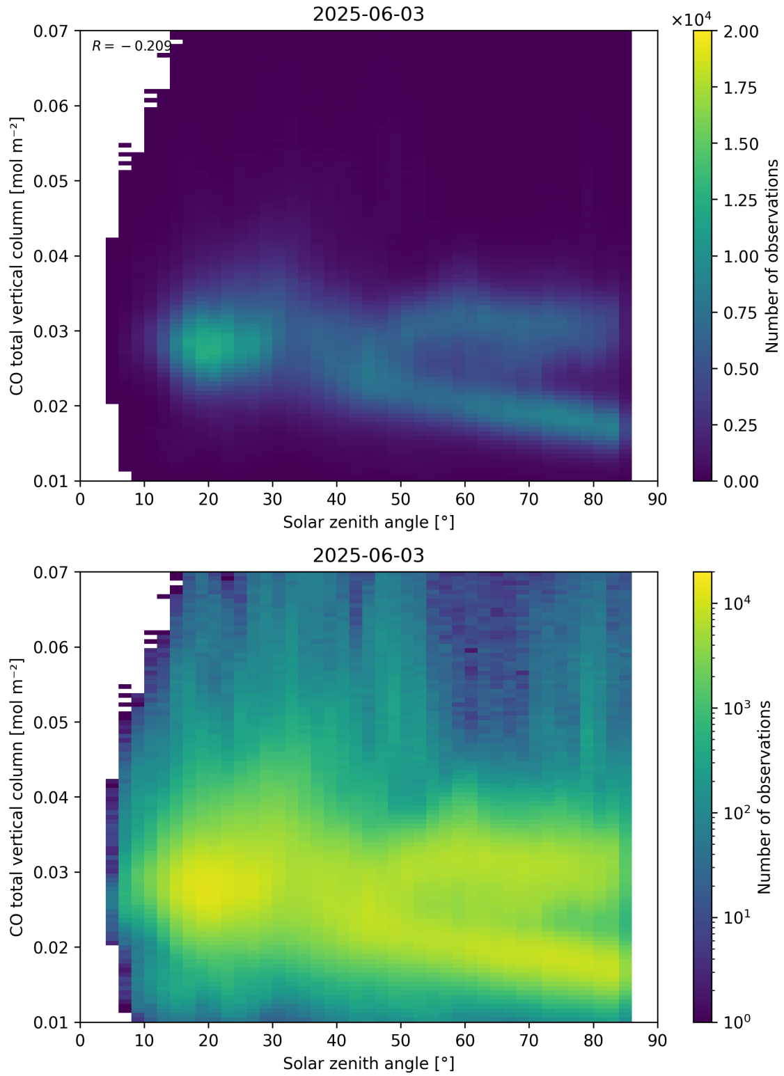
Figure 61: Scatter density plot of “Solar zenith angle” against “CO total vertical column” for 2025-06-02 to 2025-06-04.
