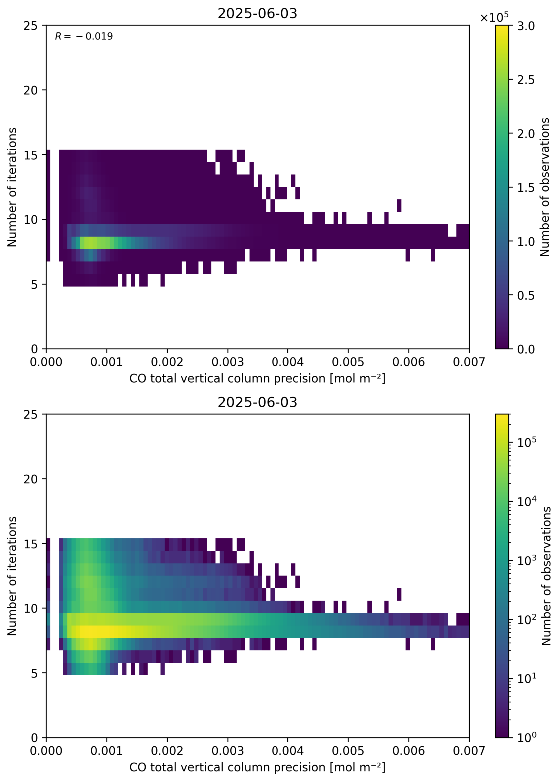
Figure 46: Scatter density plot of “CO total vertical column precision” against “Number of iterations” for 2025-06-02 to 2025-06-04.
