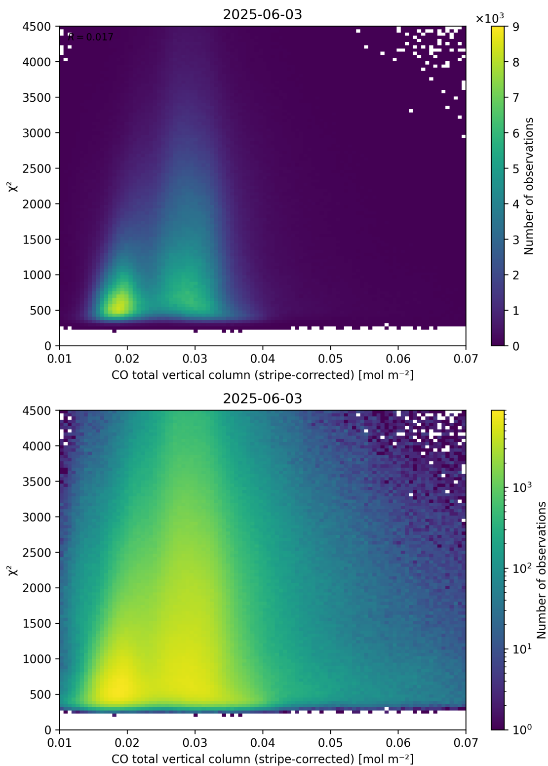
Figure 37: Scatter density plot of “CO total vertical column (stripe-corrected)” against “ \chi^2 ” for 2025-06-02 to 2025-06-04.
