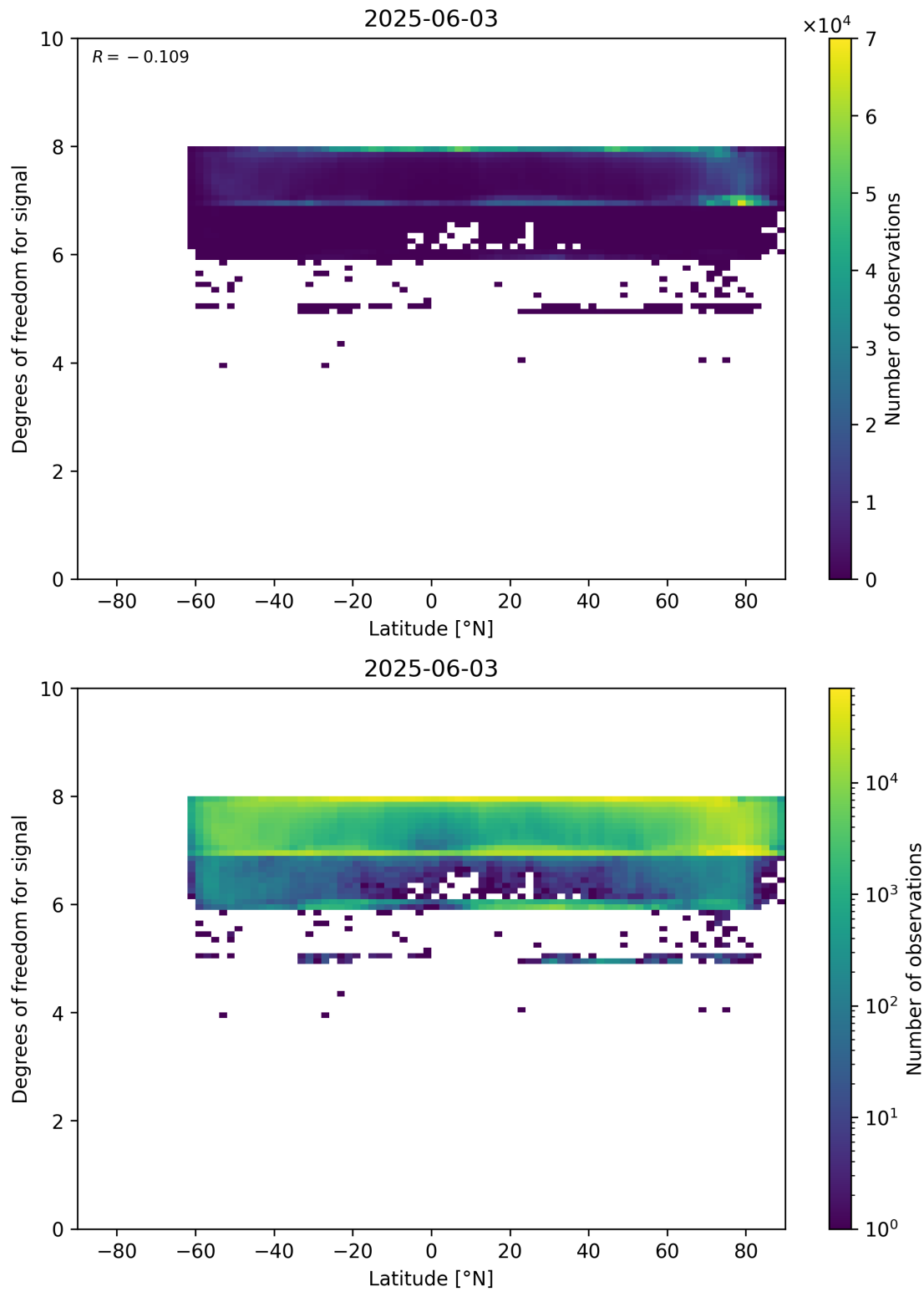
Figure 55: Scatter density plot of “Latitude” against “Degrees of freedom for signal” for 2025-06-02 to 2025-06-04.
