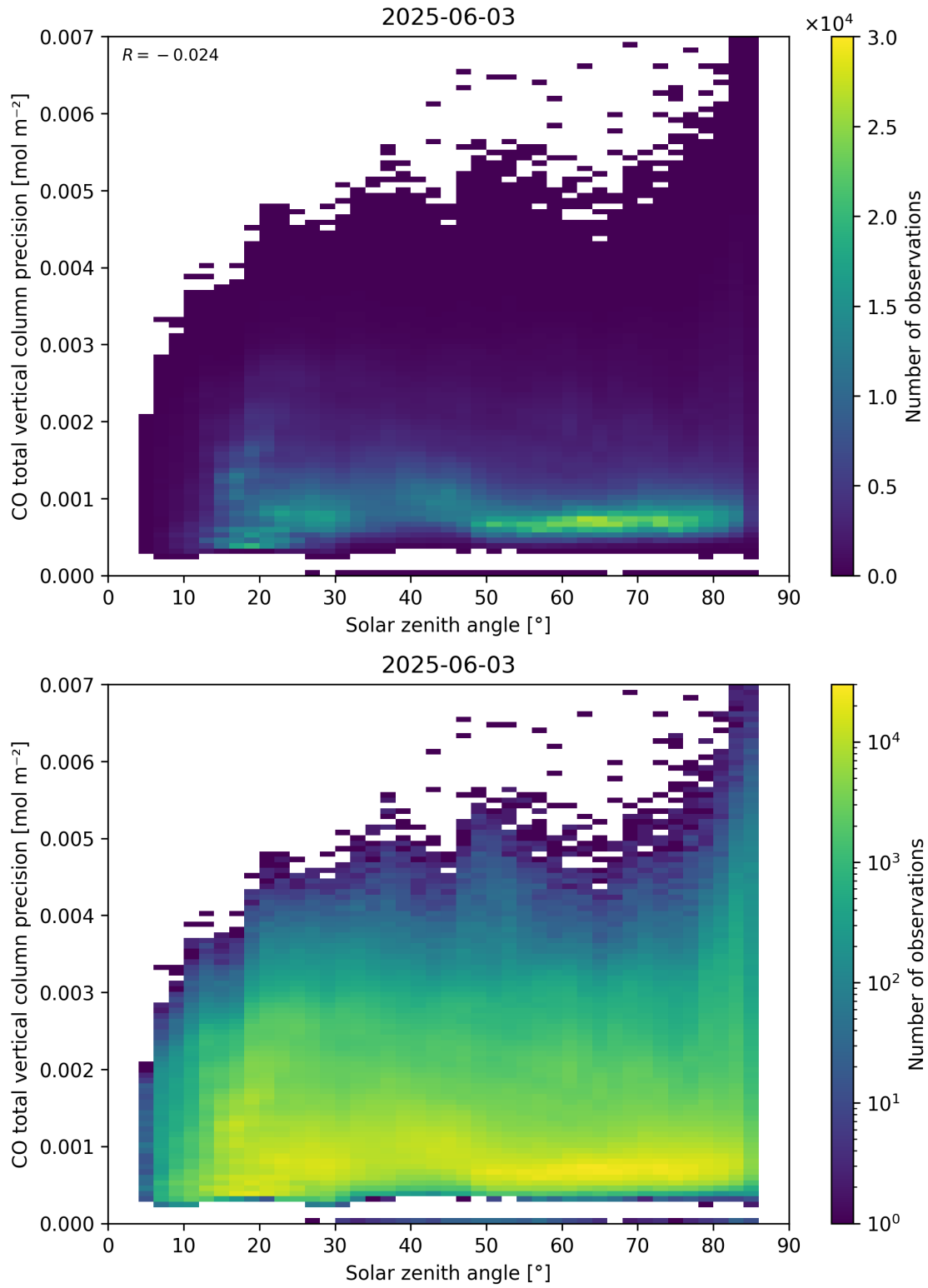
Figure 63: Scatter density plot of “Solar zenith angle” against “CO total vertical column precision” for 2025-06-02 to 2025-06-04.
