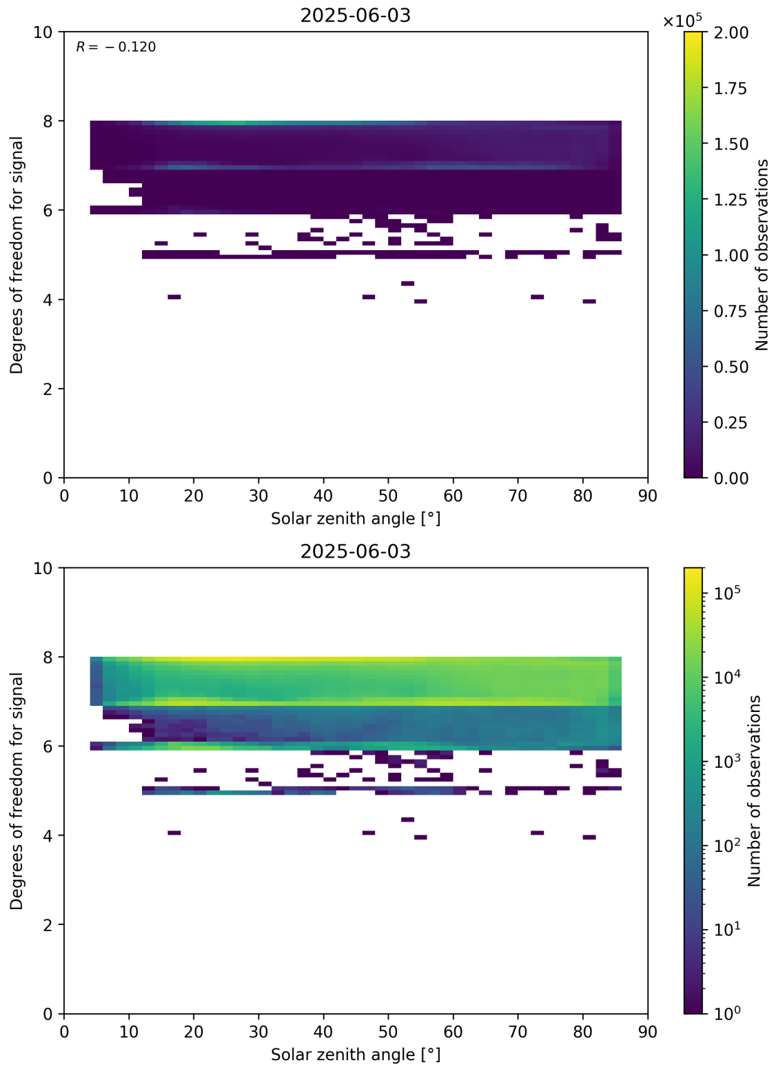
Figure 65: Scatter density plot of “Solar zenith angle” against “Degrees of freedom for signal” for 2025-06-02 to 2025-06-04.
