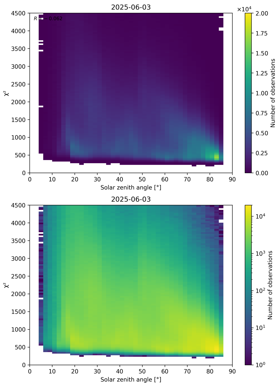
Figure 64: Scatter density plot of “Solar zenith angle” against “ \chi^2 ” for 2025-06-02 to 2025-06-04.
