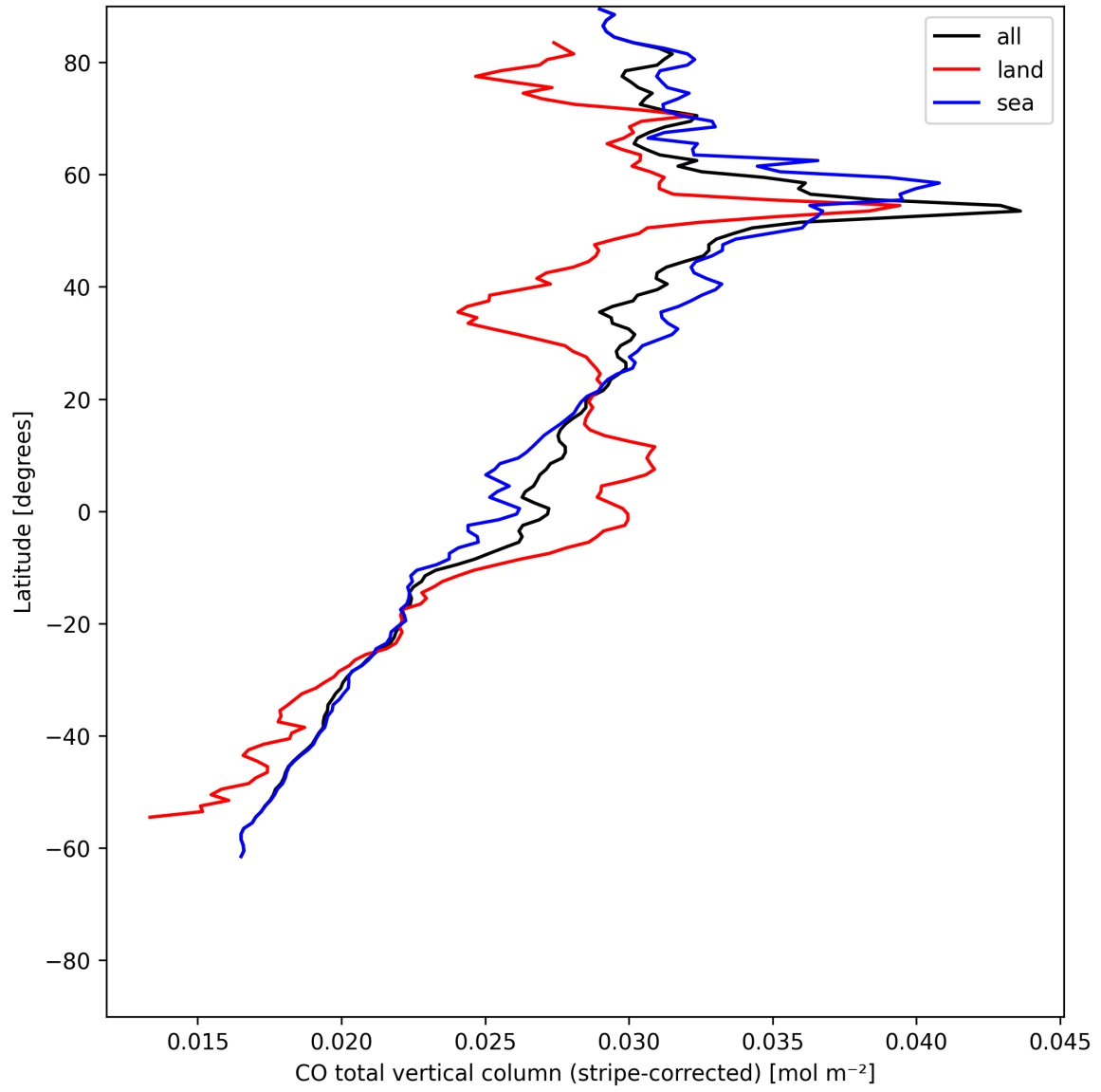
Figure 11: Zonal average of “CO total vertical column (stripe-corrected)” for 2025-06-02 to 2025-06-04.
