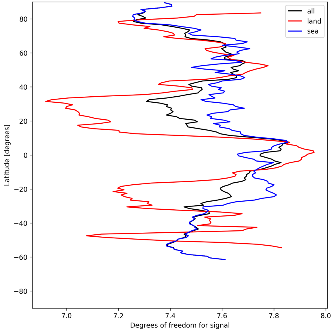
Figure 15: Zonal average of “Degrees of freedom for signal” for 2025-06-02 to 2025-06-04.
