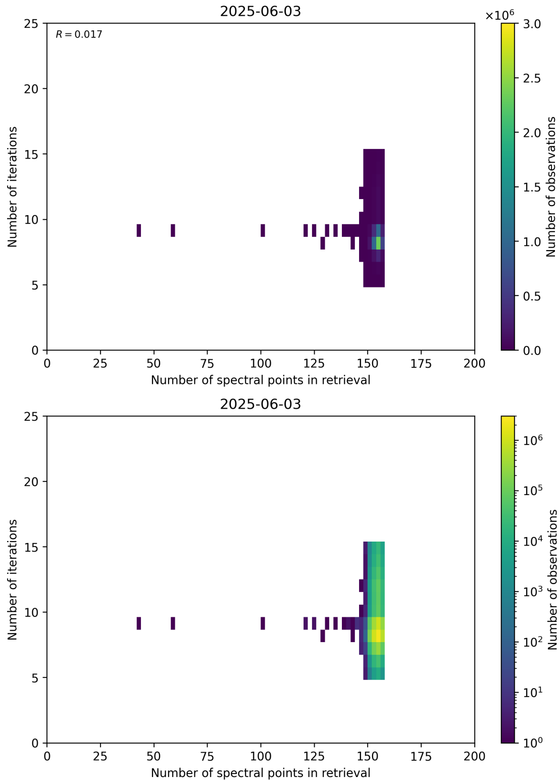
Figure 60: Scatter density plot of “Number of spectral points in retrieval” against “Number of iterations” for 2025-06-02 to 2025-06-04.
