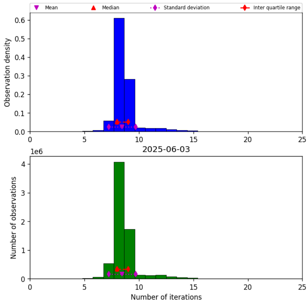
Figure 24: Histogram of “Number of iterations” for 2025-06-02 to 2025-06-04
