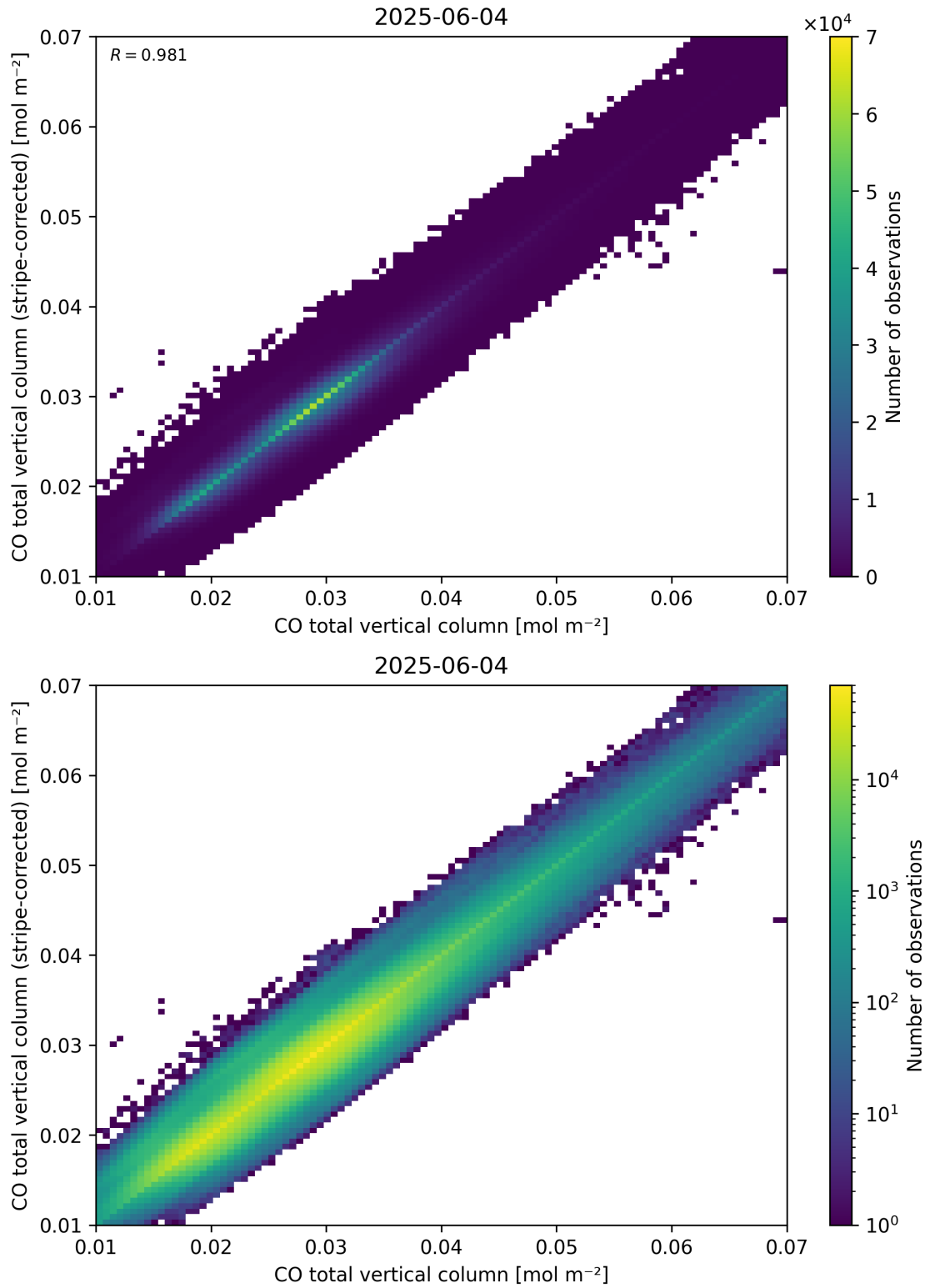
Figure 33: Scatter density plot of “CO total vertical column” against “CO total vertical column (stripe-corrected)” for 2025-06-03 to 2025-06-05.
