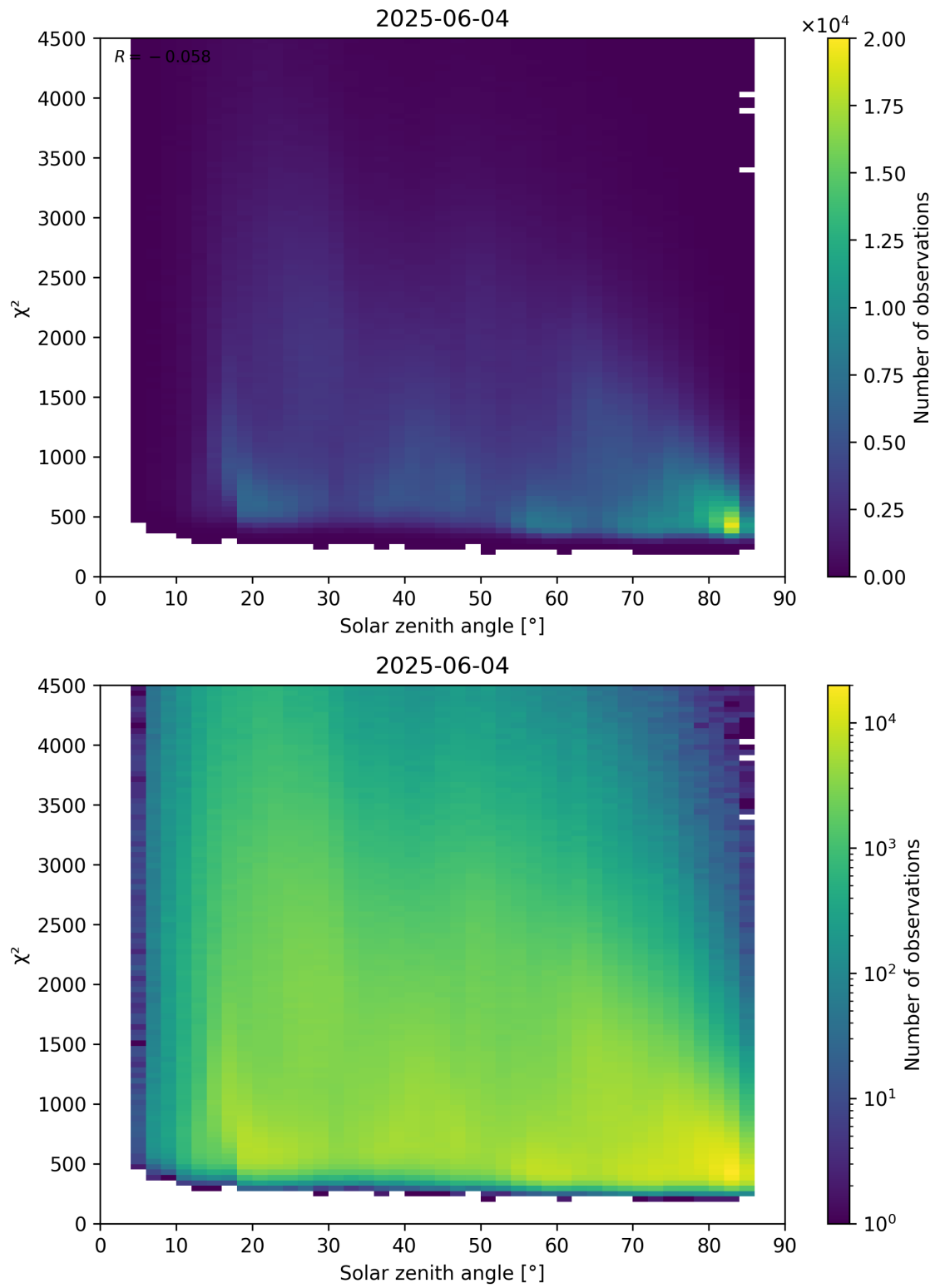
Figure 64: Scatter density plot of “Solar zenith angle” against “ \chi^2 ” for 2025-06-03 to 2025-06-05.
