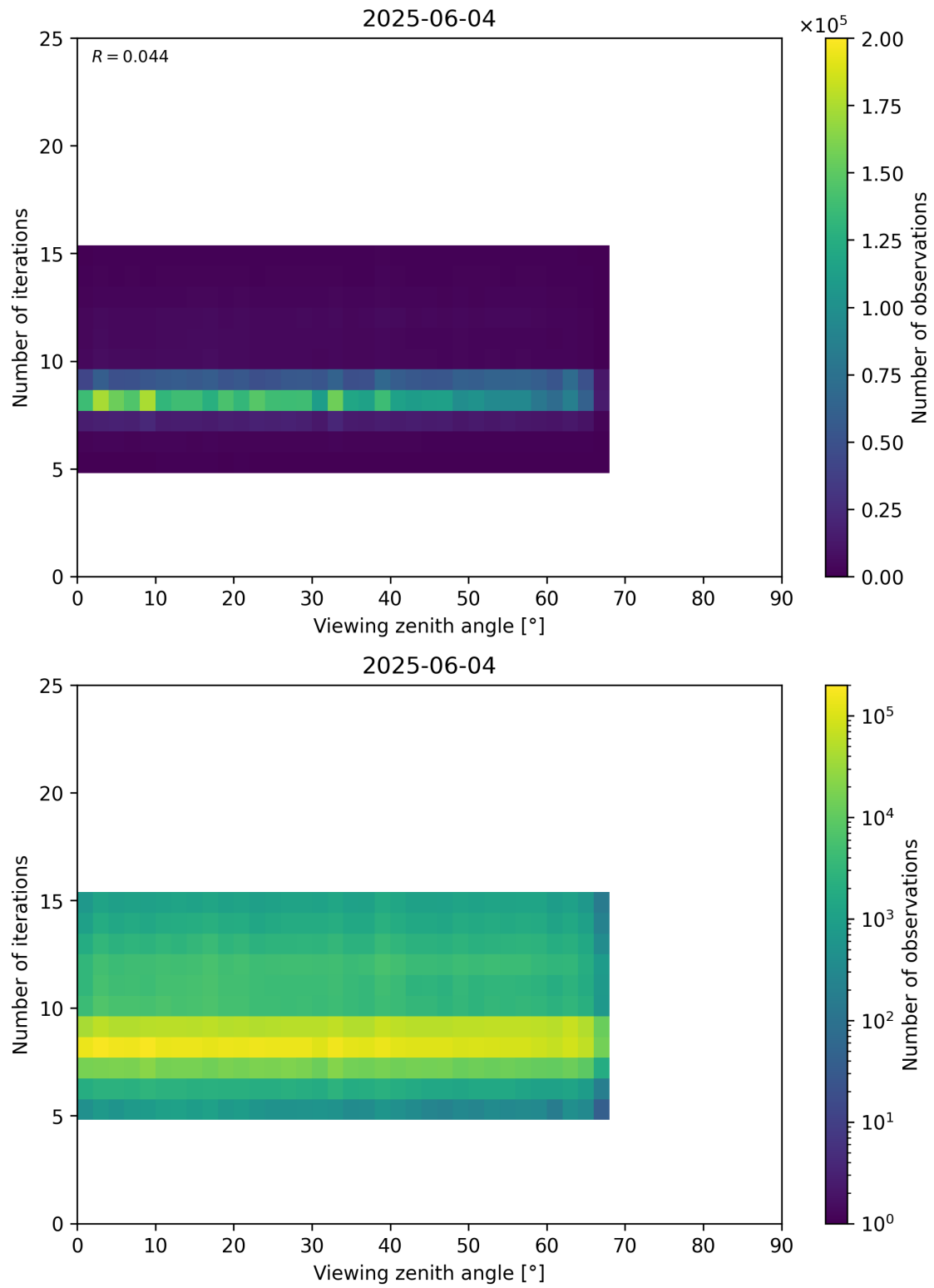
Figure 75: Scatter density plot of “Viewing zenith angle” against “Number of iterations” for 2025-06-03 to 2025-06-05.
