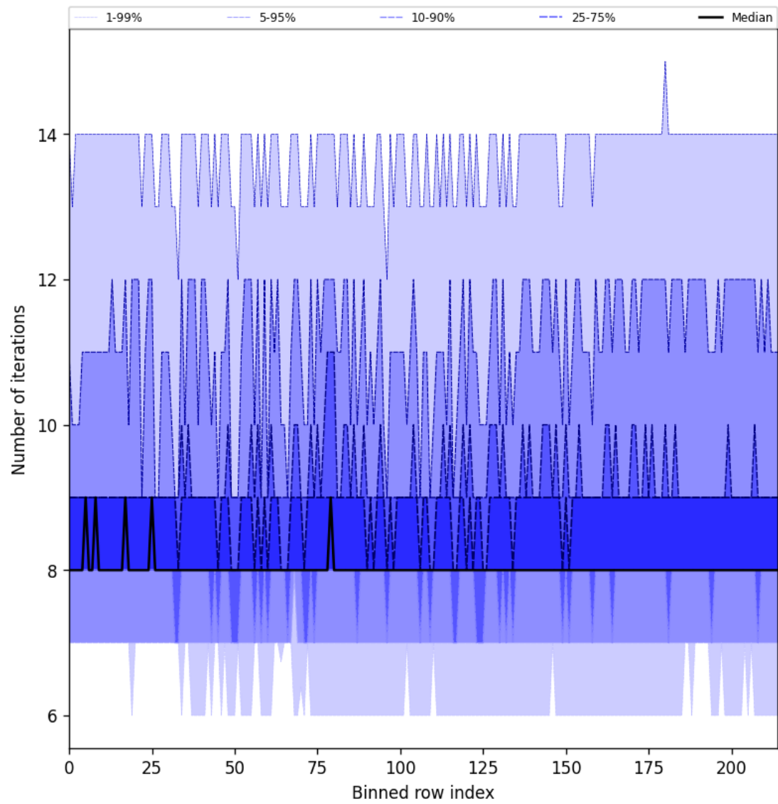
Figure 32: Along track statistics of “Number of iterations” for 2025-06-03 to 2025-06-05
