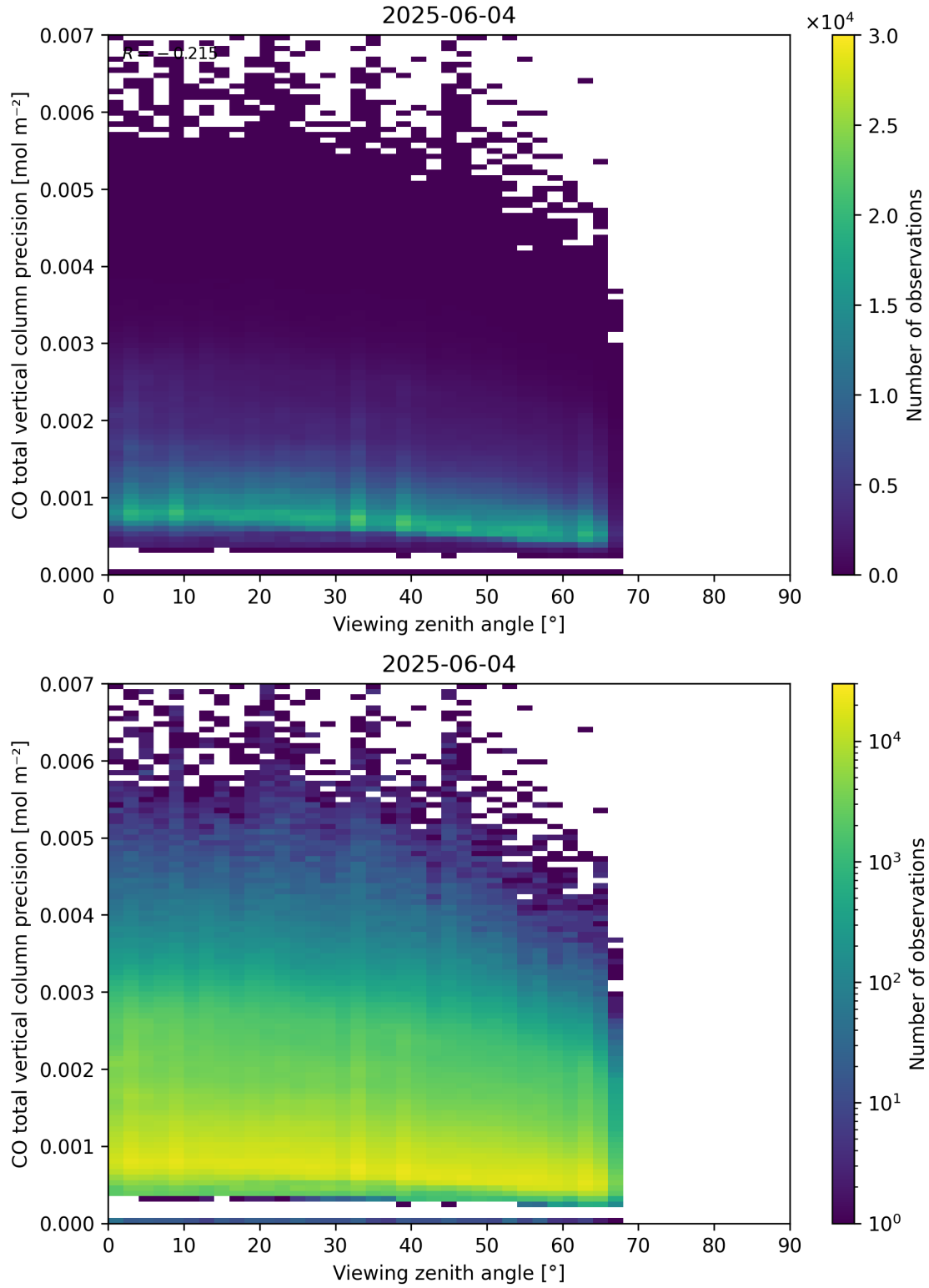
Figure 71: Scatter density plot of “Viewing zenith angle” against “CO total vertical column precision” for 2025-06-03 to 2025-06-05.
