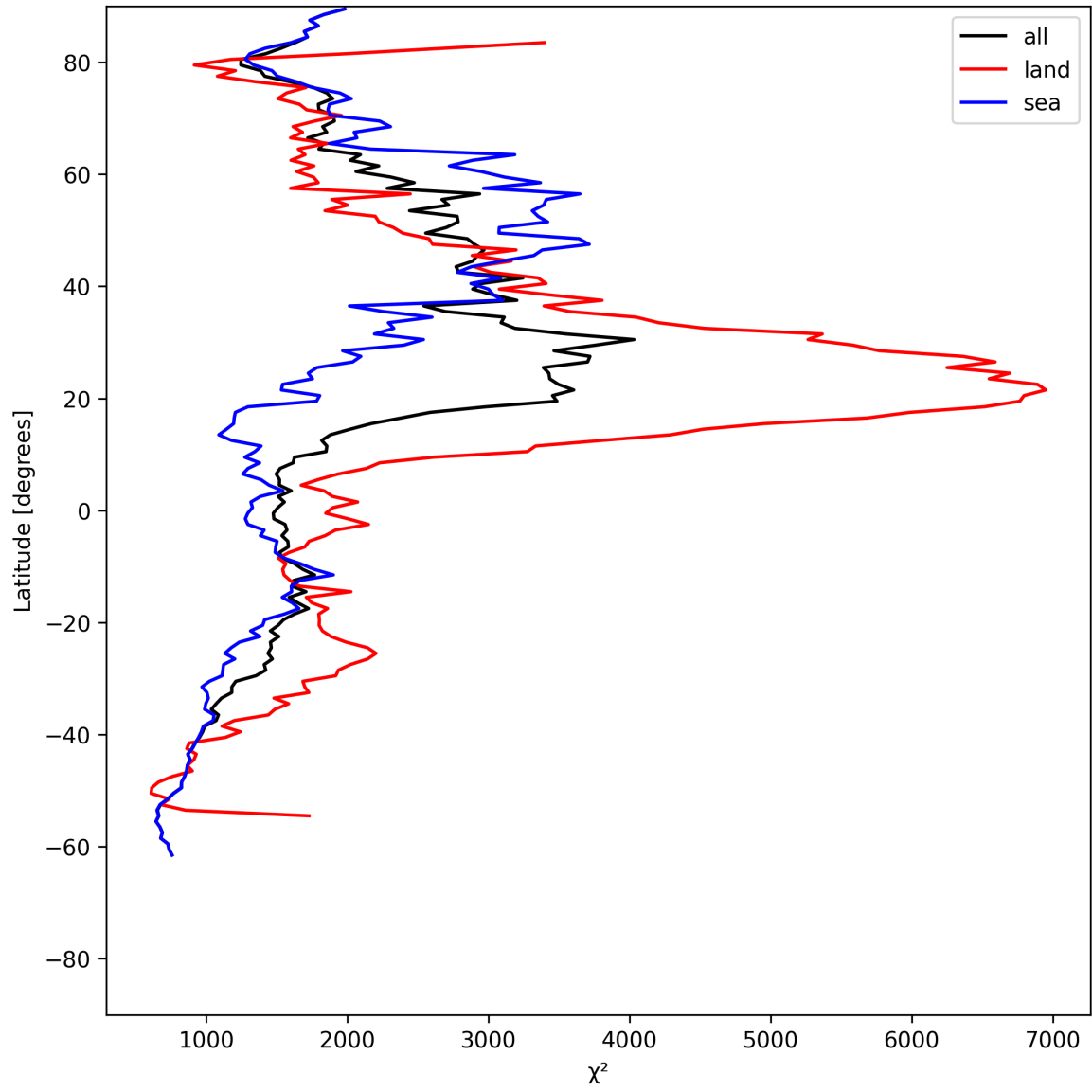
Figure 14: Zonal average of “ \chi^2 ” for 2025-06-03 to 2025-06-05.
