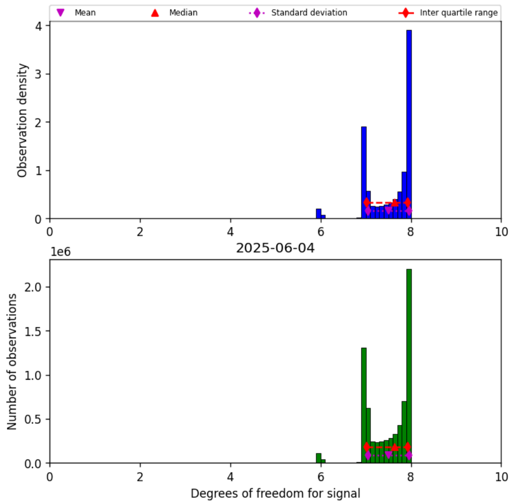
Figure 23: Histogram of “Degrees of freedom for signal” for 2025-06-03 to 2025-06-05
