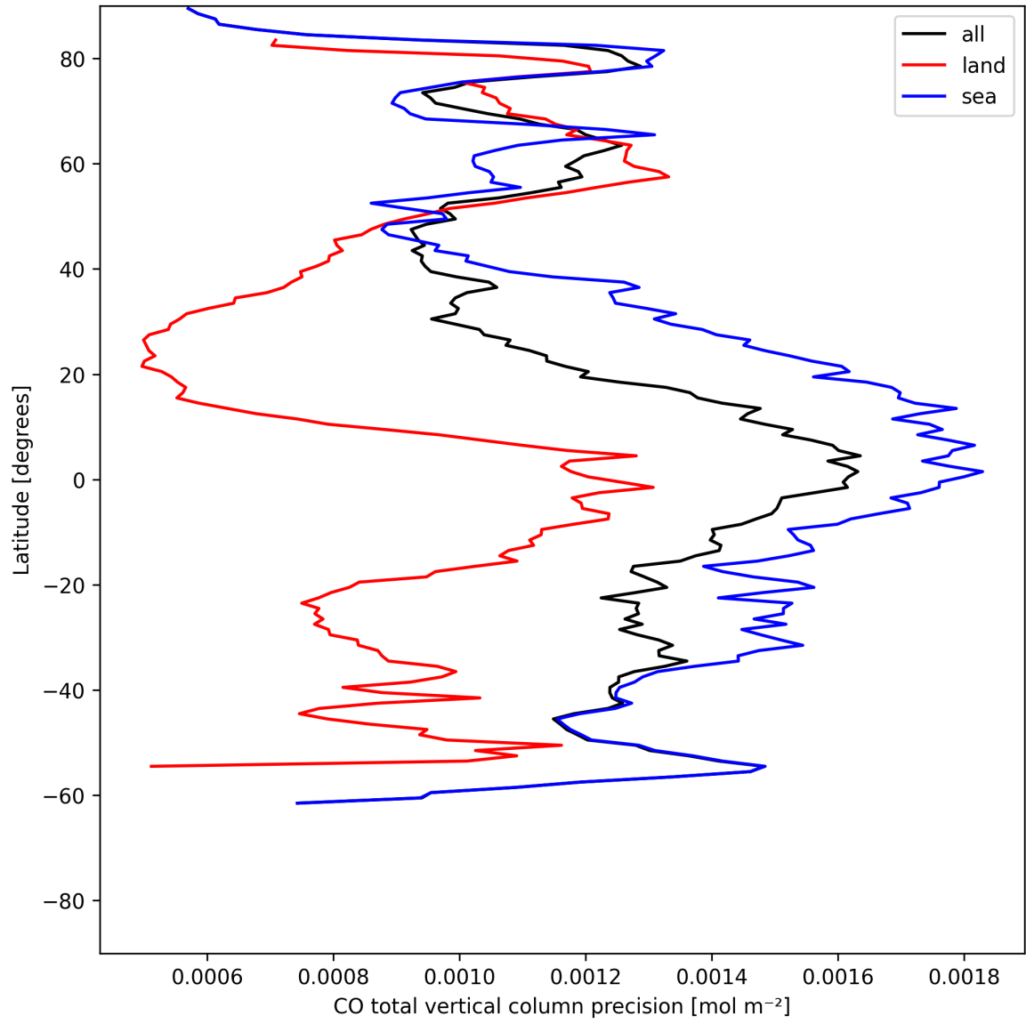
Figure 12: Zonal average of “CO total vertical column precision” for 2025-06-03 to 2025-06-05.
