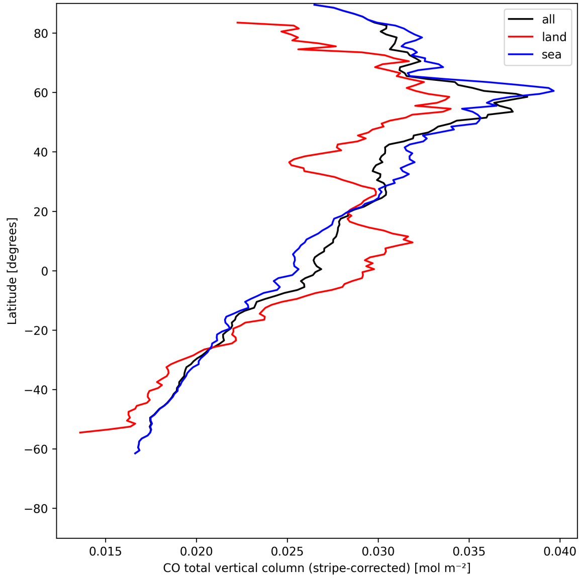
Figure 11: Zonal average of “CO total vertical column (stripe-corrected)” for 2025-06-03 to 2025-06-05.
