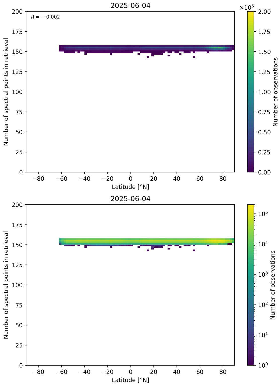
Figure 57: Scatter density plot of “Latitude” against “Number of spectral points in retrieval” for 2025-06-03 to 2025-06-05.
