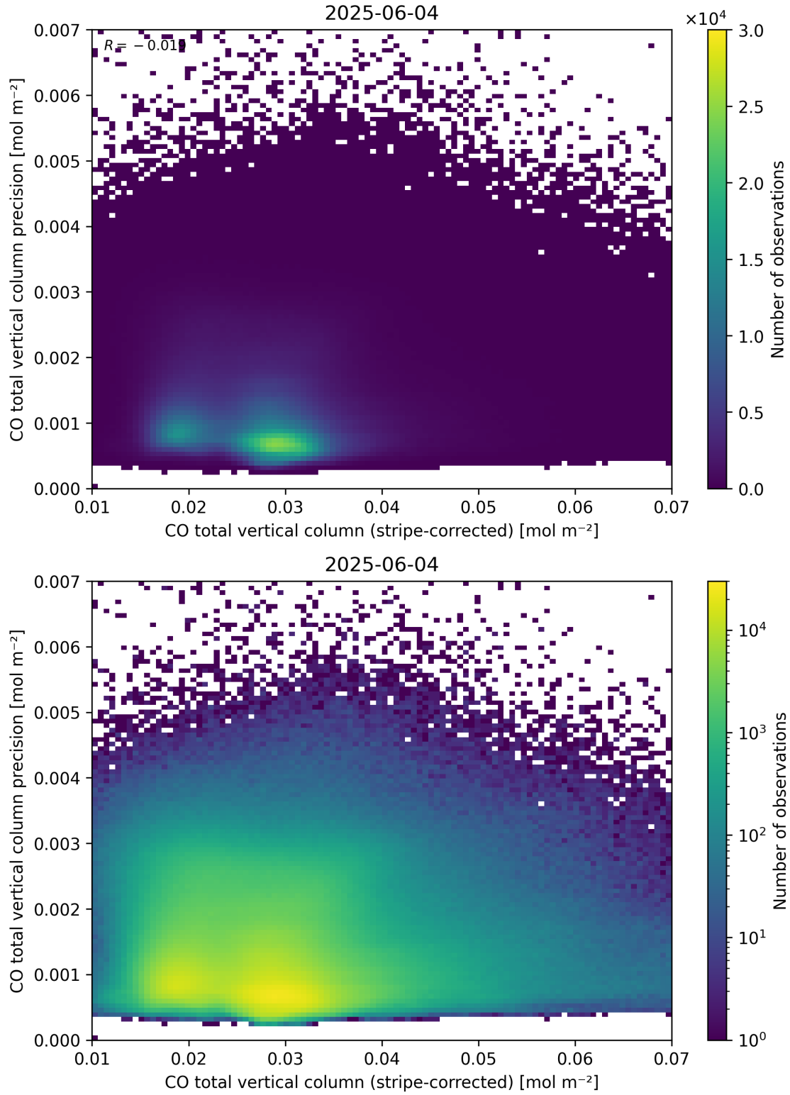
Figure 36: Scatter density plot of “CO total vertical column (stripe-corrected)” against “CO total vertical column precision” for 2025-06-03 to 2025-06-05.
