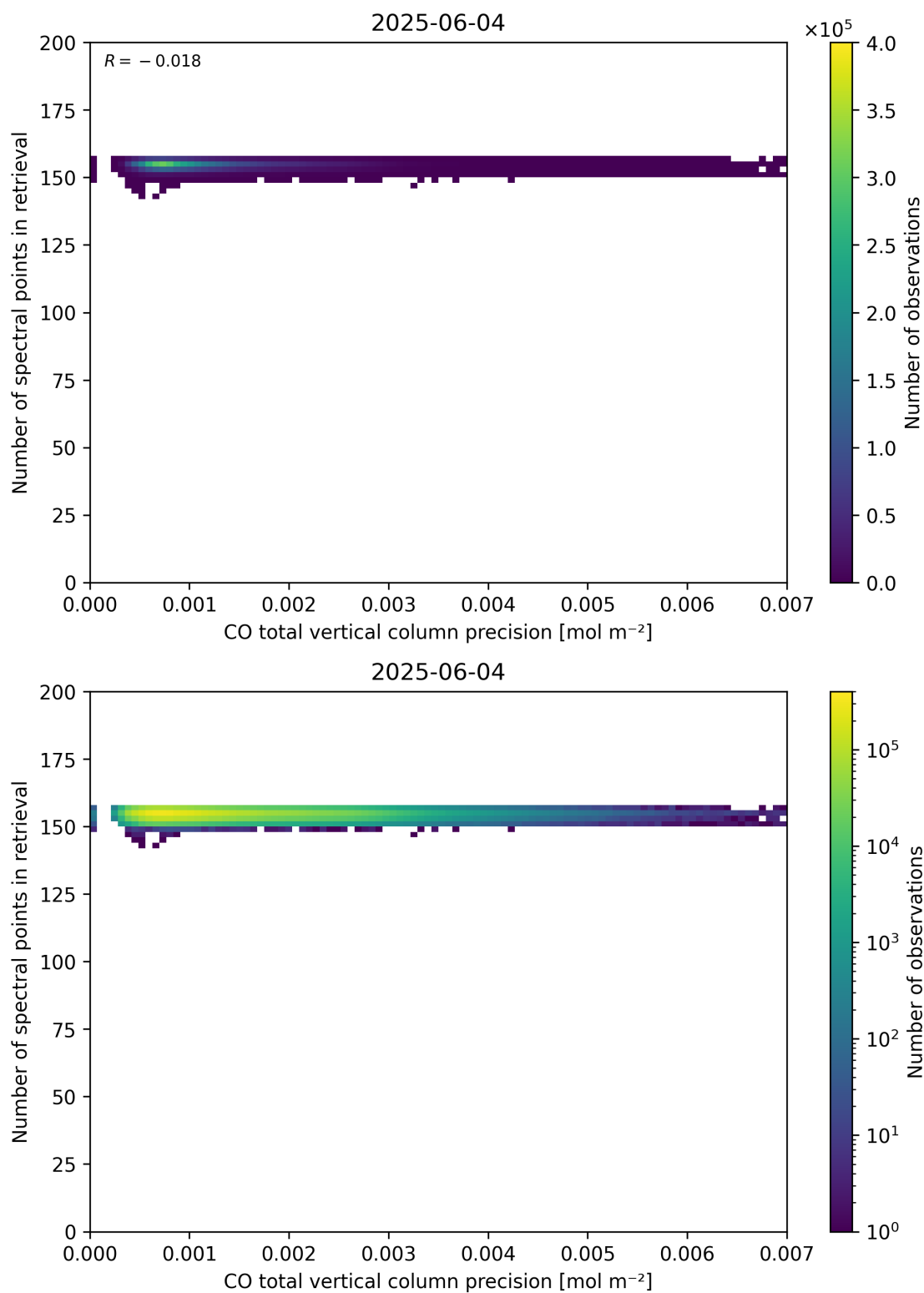
Figure 47: Scatter density plot of “CO total vertical column precision” against “Number of spectral points in retrieval” for 2025-06-03 to 2025-06-05.
