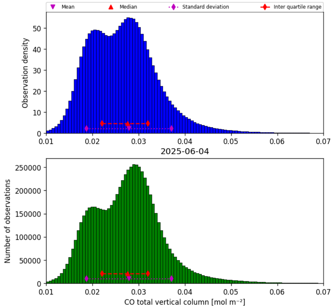
Figure 18: Histogram of “CO total vertical column” for 2025-06-03 to 2025-06-05
