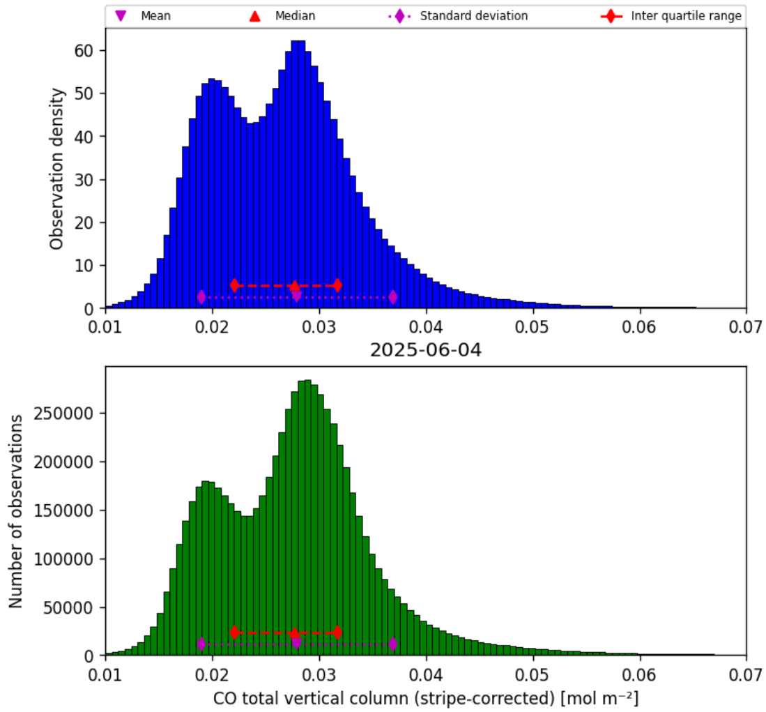
Figure 19: Histogram of “CO total vertical column (stripe-corrected)” for 2025-06-03 to 2025-06-05
