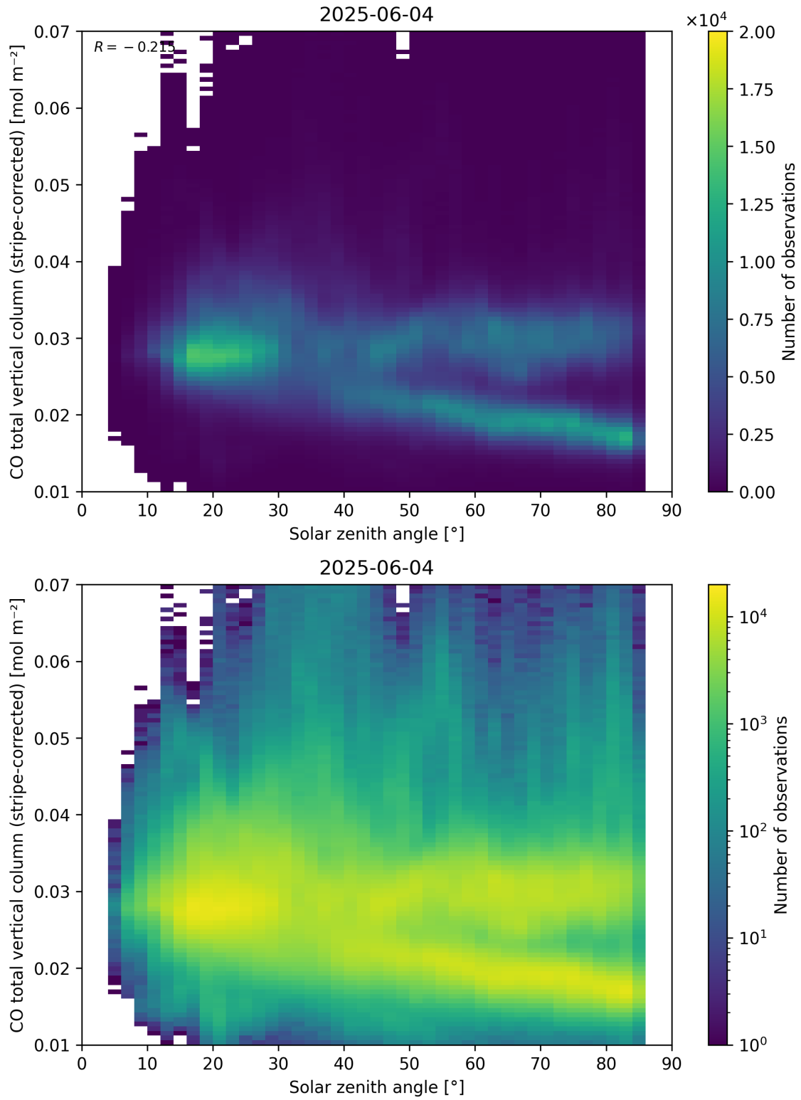
Figure 62: Scatter density plot of “Solar zenith angle” against “CO total vertical column (stripe-corrected)” for 2025-06-03 to 2025-06-05.
