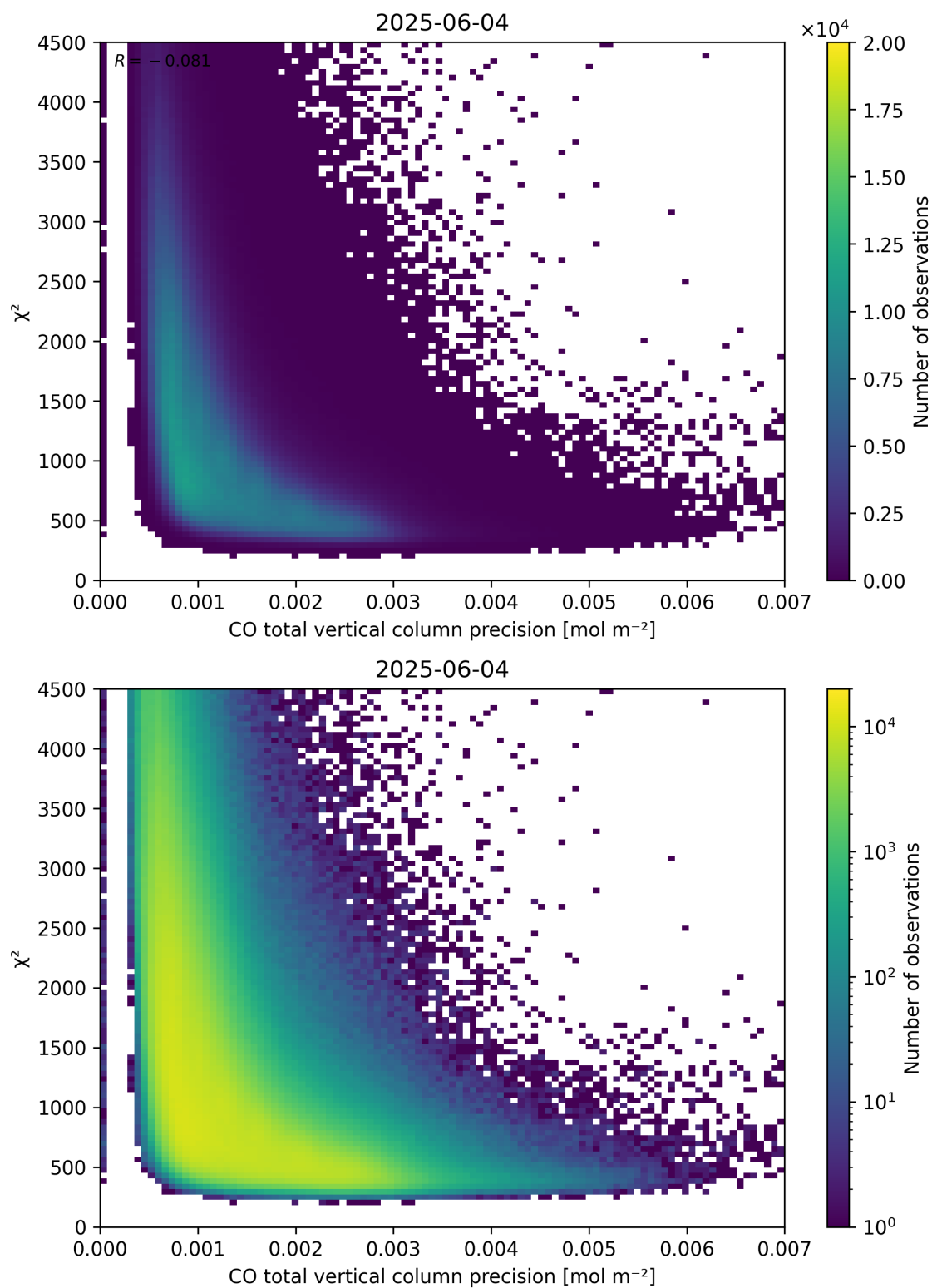
Figure 44: Scatter density plot of “CO total vertical column precision” against “ \chi^2 ” for 2025-06-03 to 2025-06-05.
