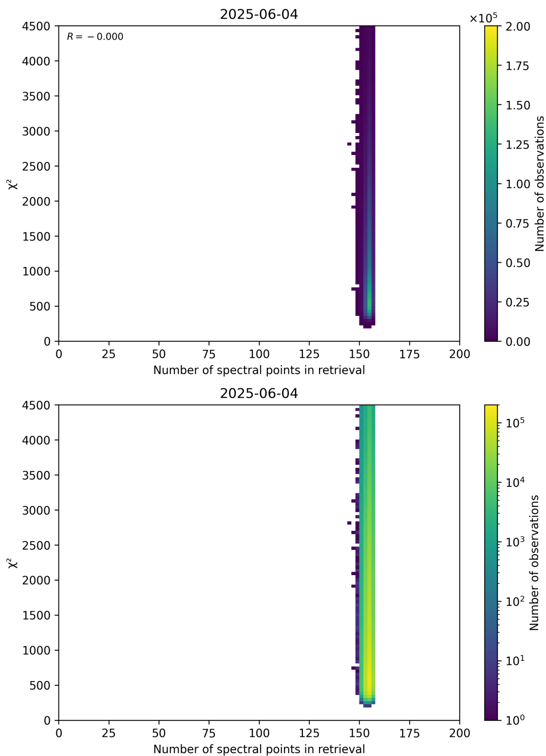
Figure 58: Scatter density plot of “Number of spectral points in retrieval” against “ \chi^2 ” for 2025-06-03 to 2025-06-05.
