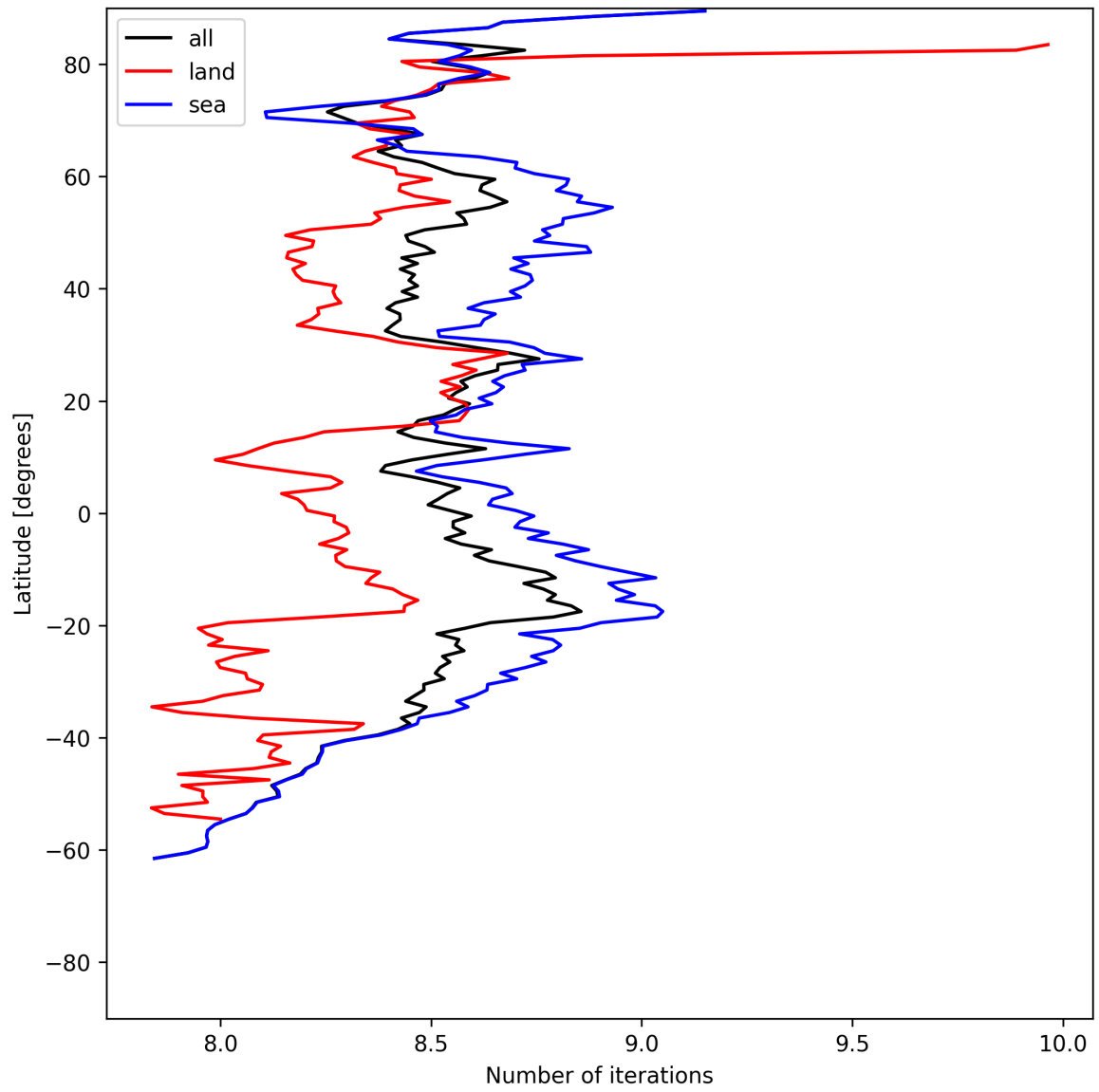
Figure 16: Zonal average of “Number of iterations” for 2025-06-03 to 2025-06-05.
