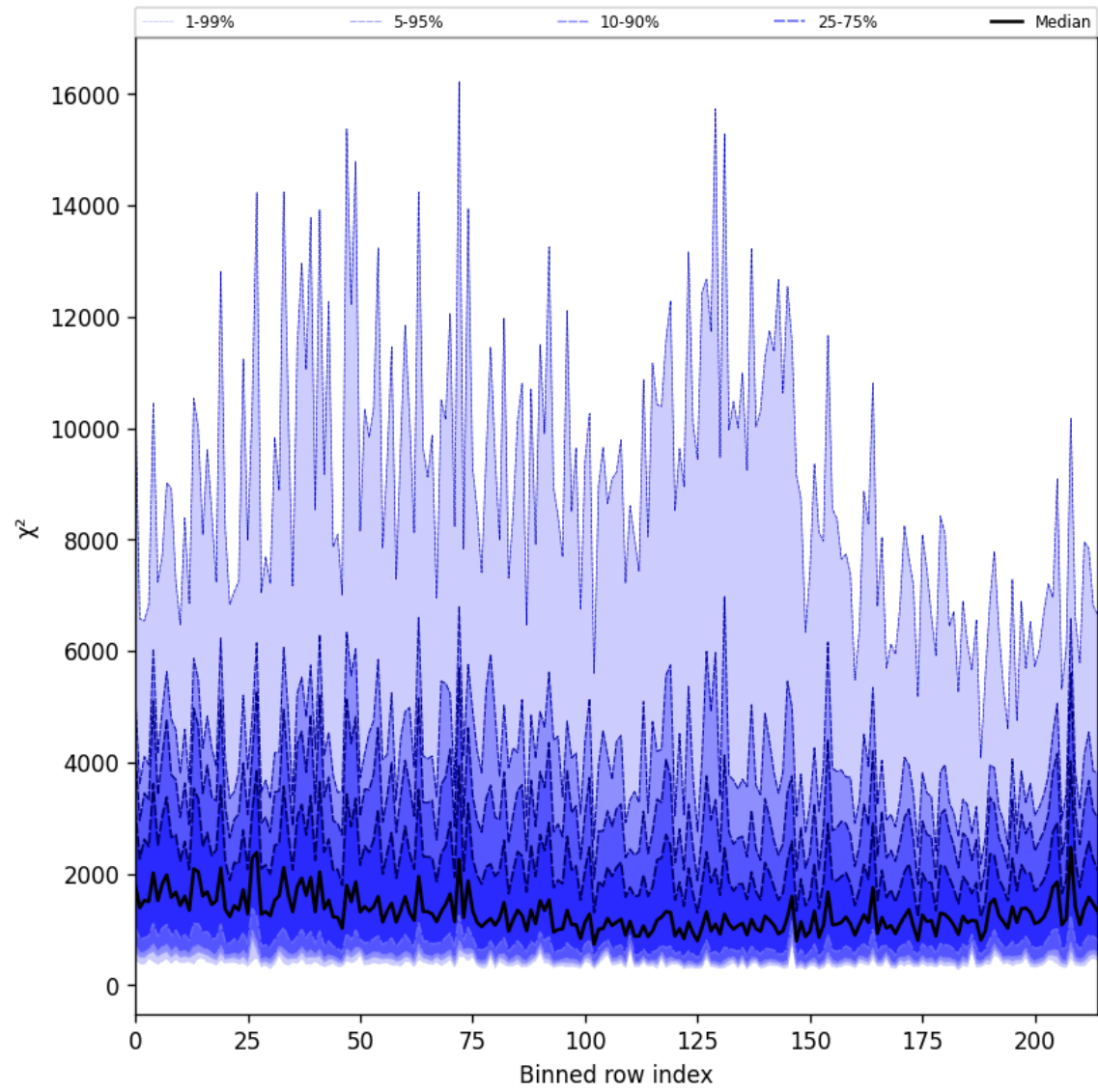
Figure 30: Along track statistics of “ \chi^2 ” for 2025-06-03 to 2025-06-05
