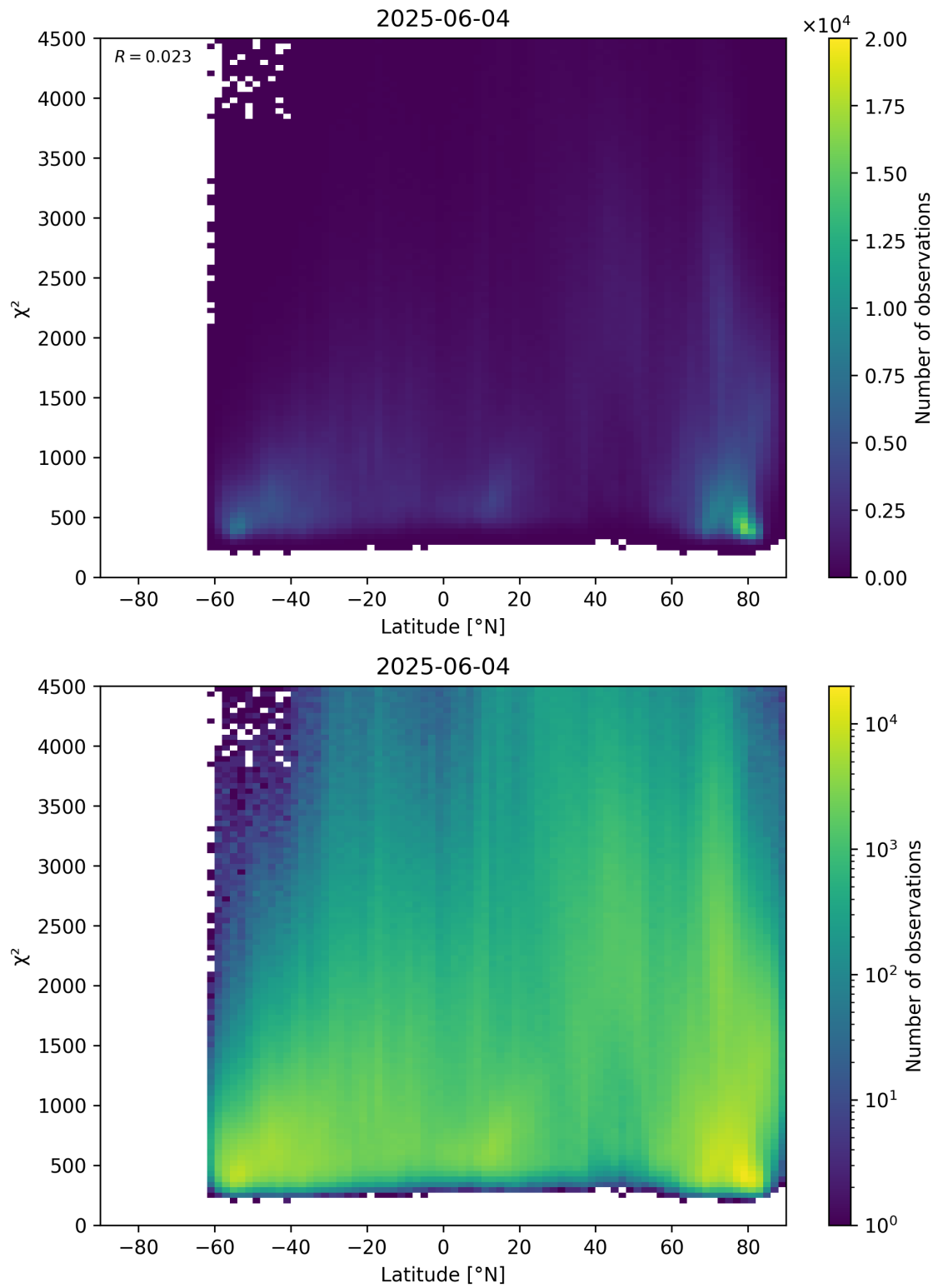
Figure 54: Scatter density plot of “Latitude” against “ \chi^2 ” for 2025-06-03 to 2025-06-05.
