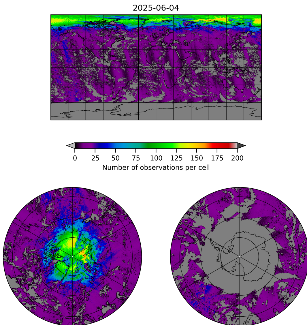
Figure 8: Map of the number of observations for 2025-06-03 to 2025-06-05
