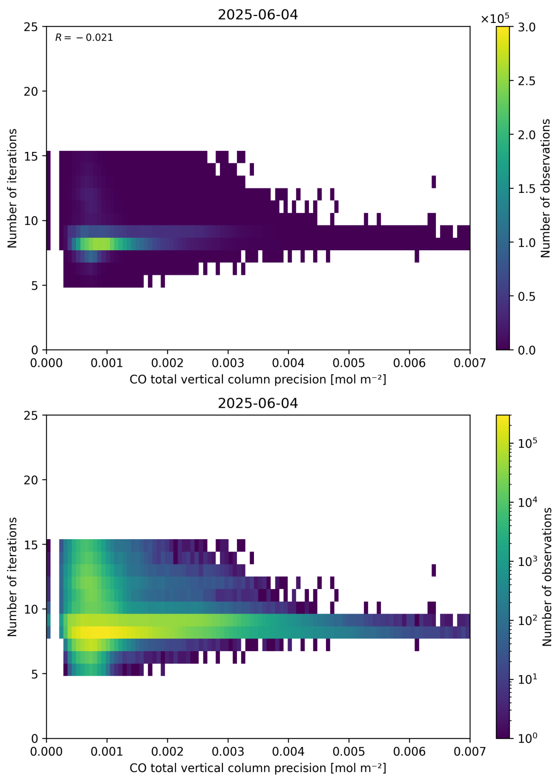
Figure 46: Scatter density plot of “CO total vertical column precision” against “Number of iterations” for 2025-06-03 to 2025-06-05.
