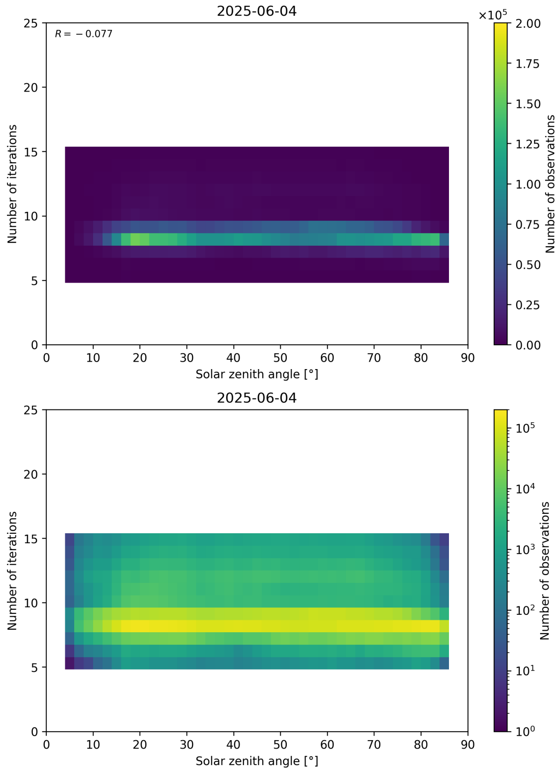
Figure 67: Scatter density plot of “Solar zenith angle” against “Number of iterations” for 2025-06-03 to 2025-06-05.
