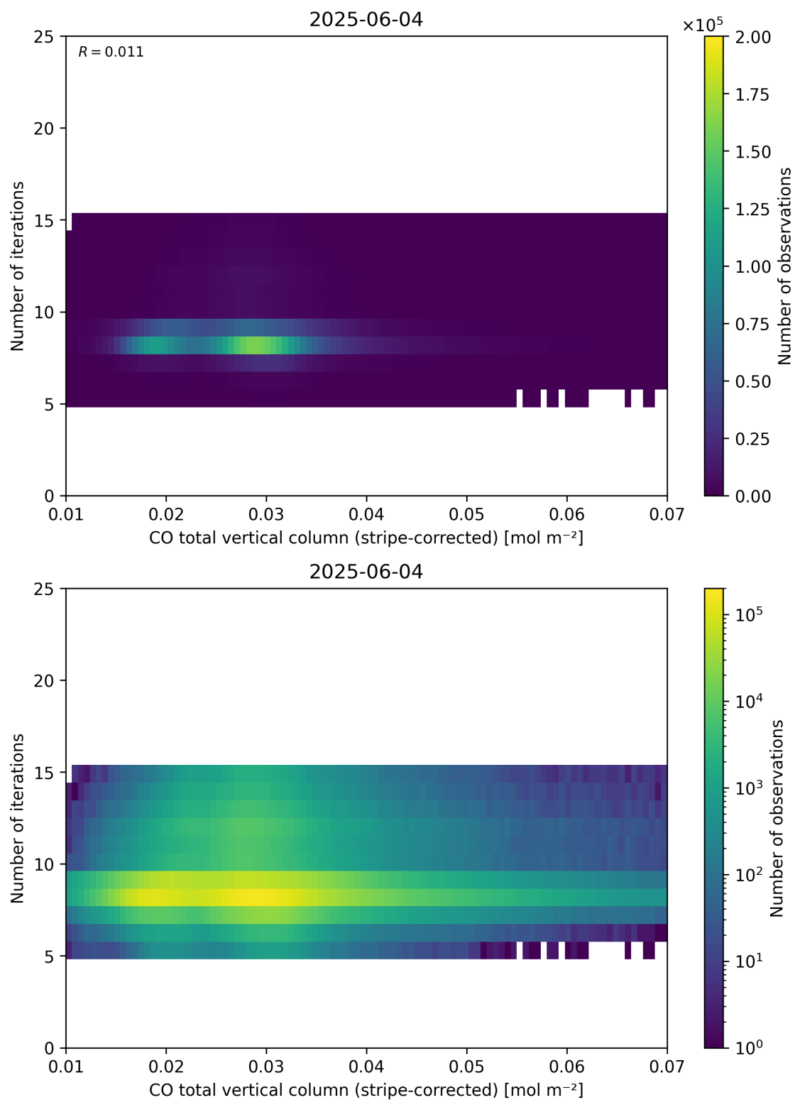
Figure 39: Scatter density plot of “CO total vertical column (stripe-corrected)” against “Number of iterations” for 2025-06-03 to 2025-06-05.
