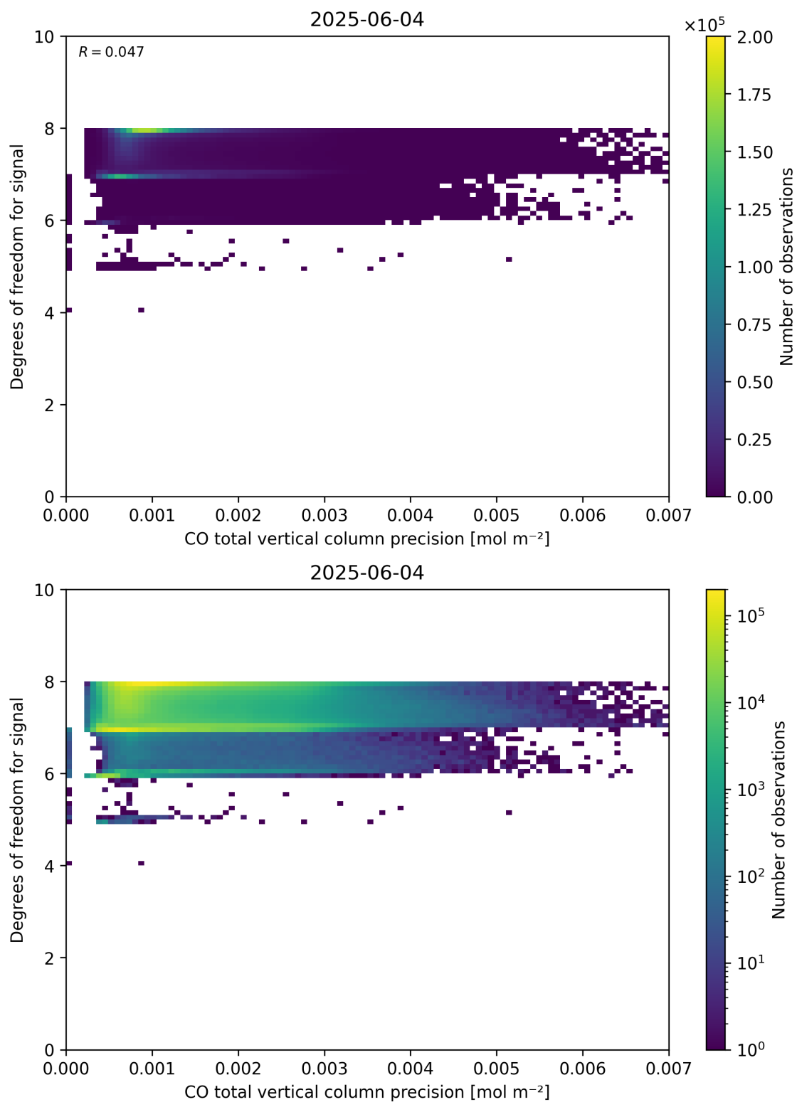
Figure 45: Scatter density plot of “CO total vertical column precision” against “Degrees of freedom for signal” for 2025-06-03 to 2025-06-05.
