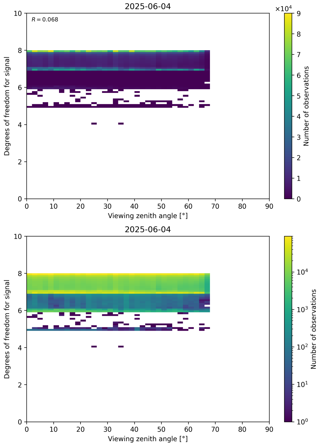
Figure 73: Scatter density plot of “Viewing zenith angle” against “Degrees of freedom for signal” for 2025-06-03 to 2025-06-05.
