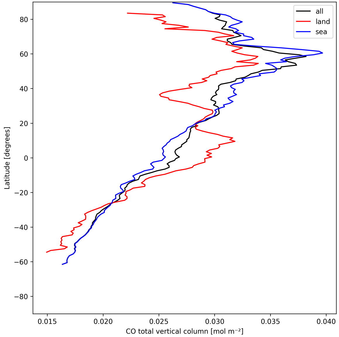
Figure 10: Zonal average of “CO total vertical column” for 2025-06-03 to 2025-06-05.
