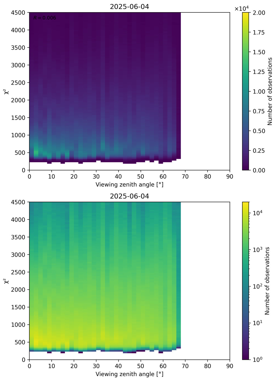
Figure 72: Scatter density plot of “Viewing zenith angle” against “ \chi^2 ” for 2025-06-03 to 2025-06-05.
