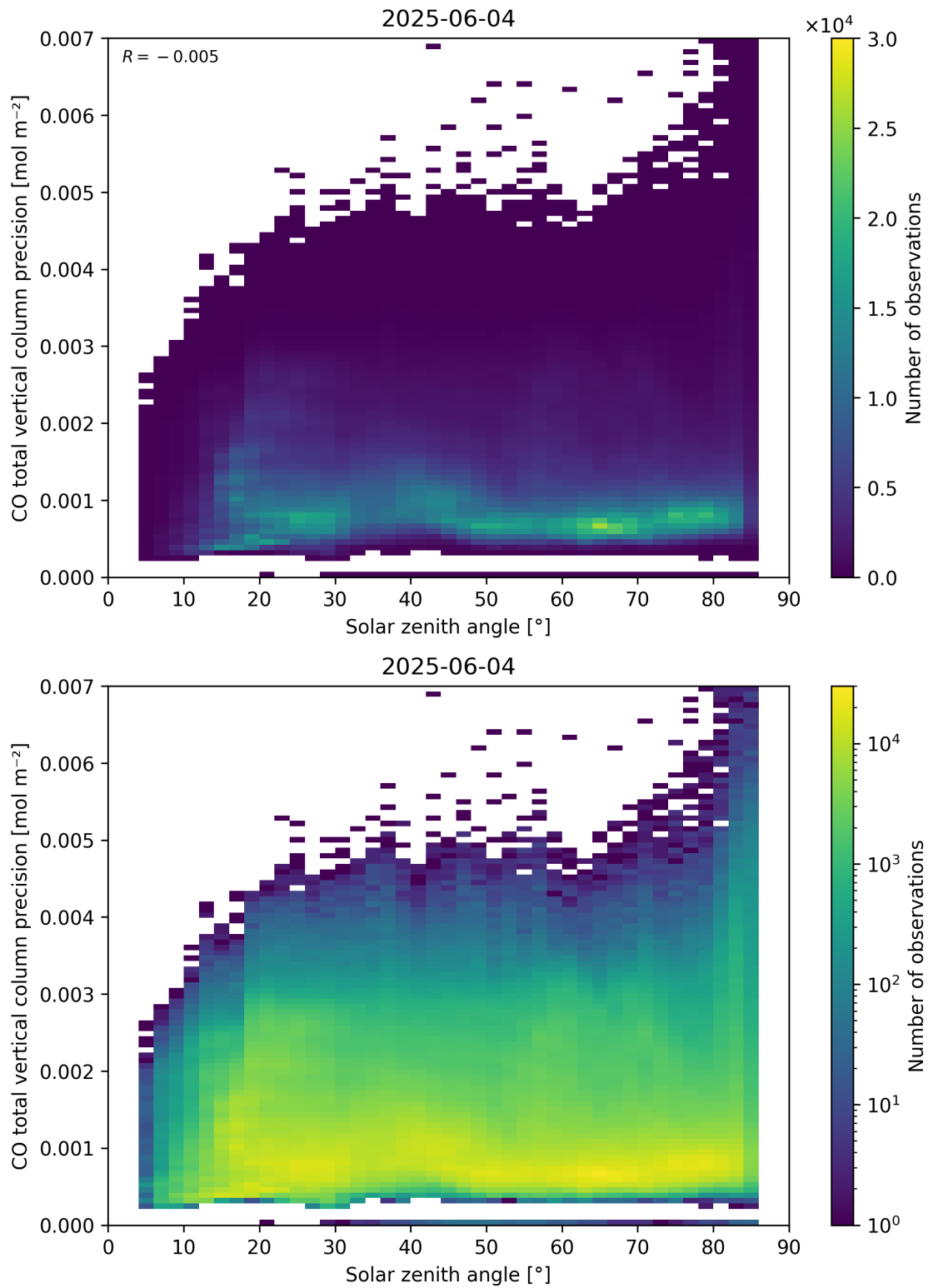
Figure 63: Scatter density plot of “Solar zenith angle” against “CO total vertical column precision” for 2025-06-03 to 2025-06-05.
