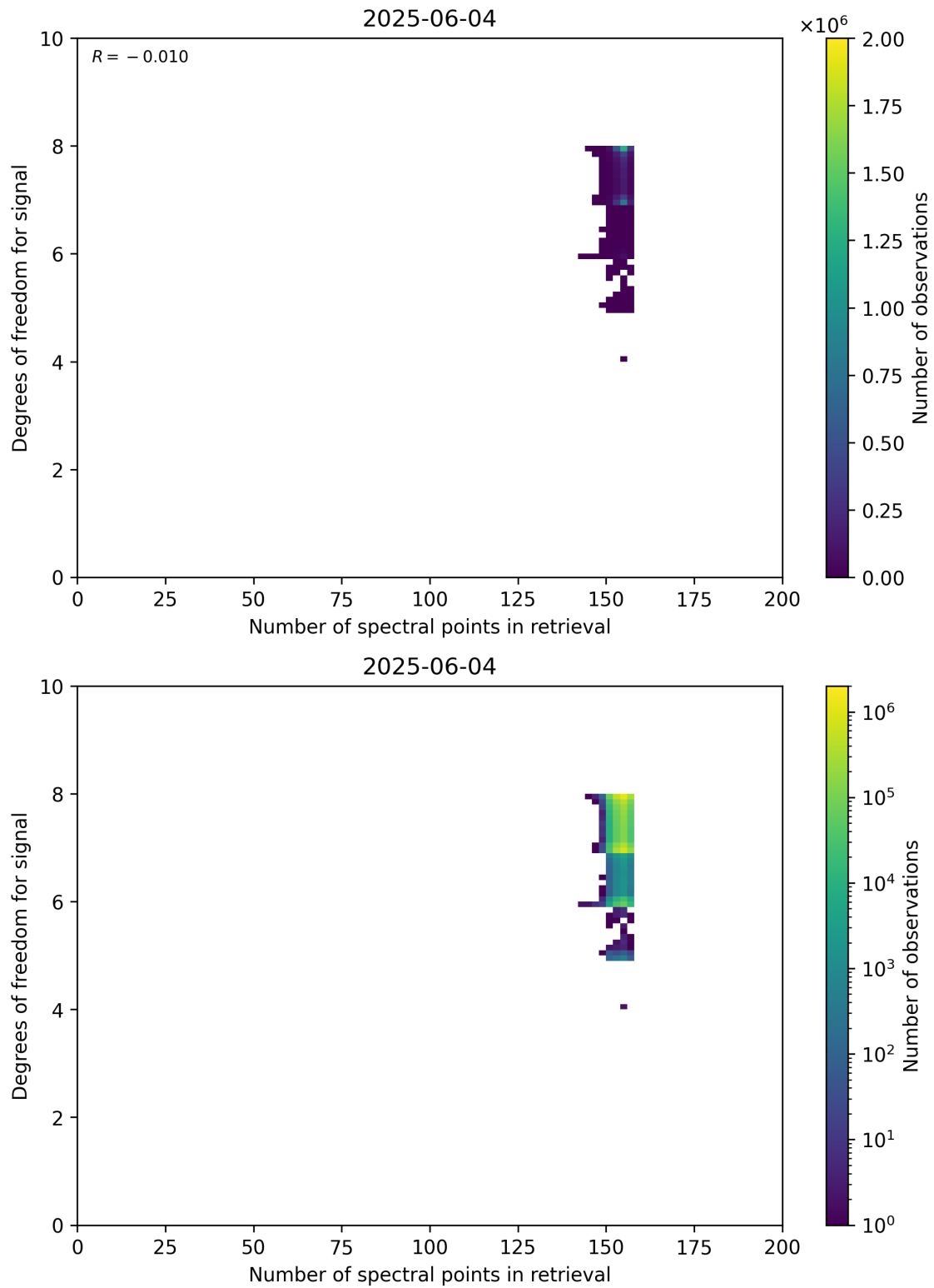
Figure 59: Scatter density plot of “Number of spectral points in retrieval” against “Degrees of freedom for signal” for 2025-06-03 to 2025-06-05.
