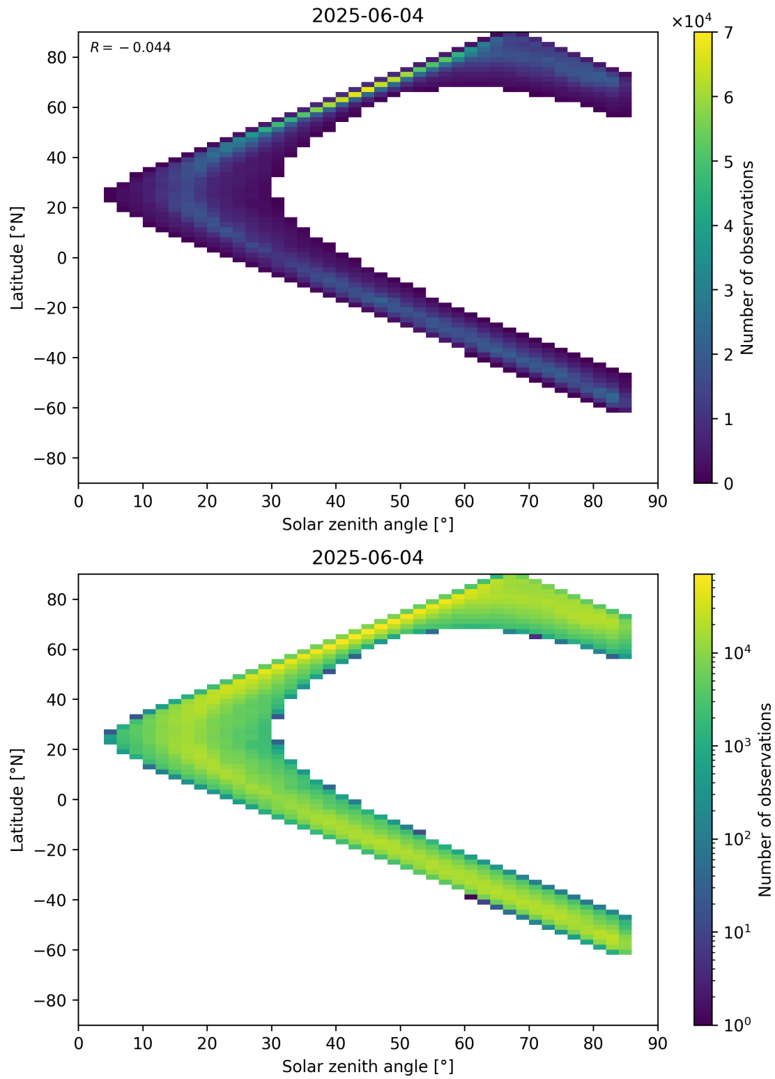
Figure 66: Scatter density plot of “Solar zenith angle” against “Latitude” for 2025-06-03 to 2025-06-05.
