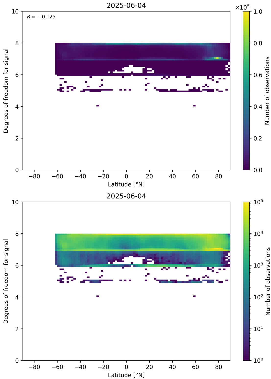
Figure 55: Scatter density plot of “Latitude” against “Degrees of freedom for signal” for 2025-06-03 to 2025-06-05.
