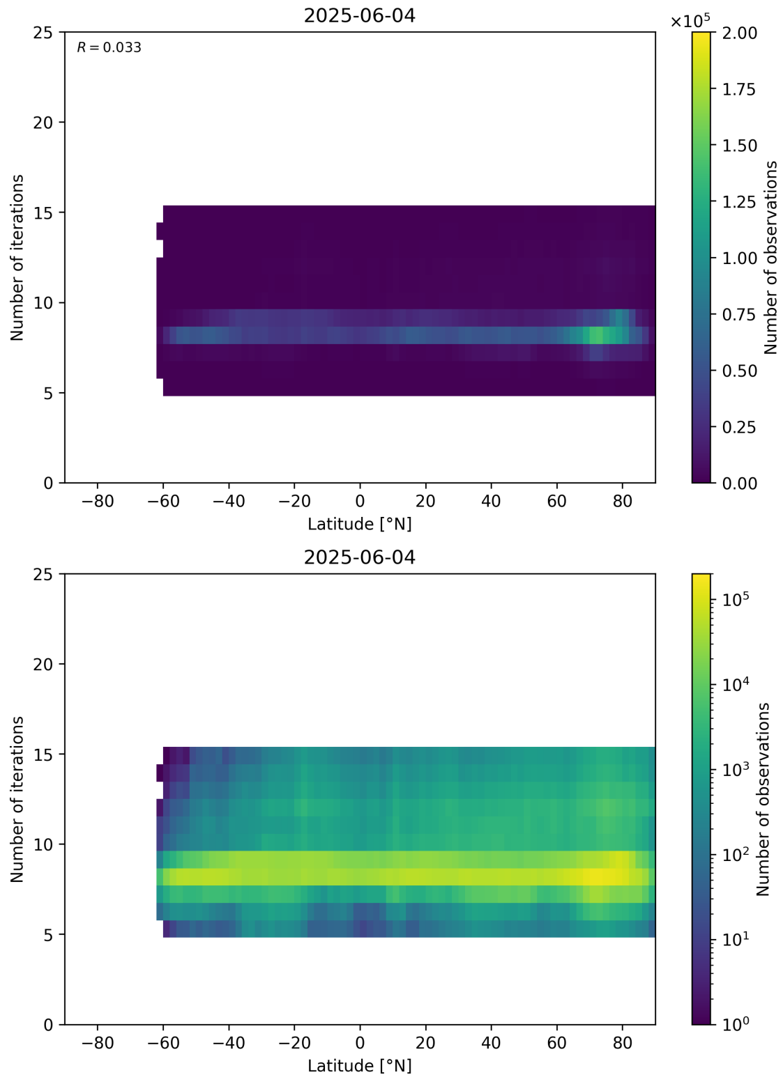
Figure 56: Scatter density plot of “Latitude” against “Number of iterations” for 2025-06-03 to 2025-06-05.
