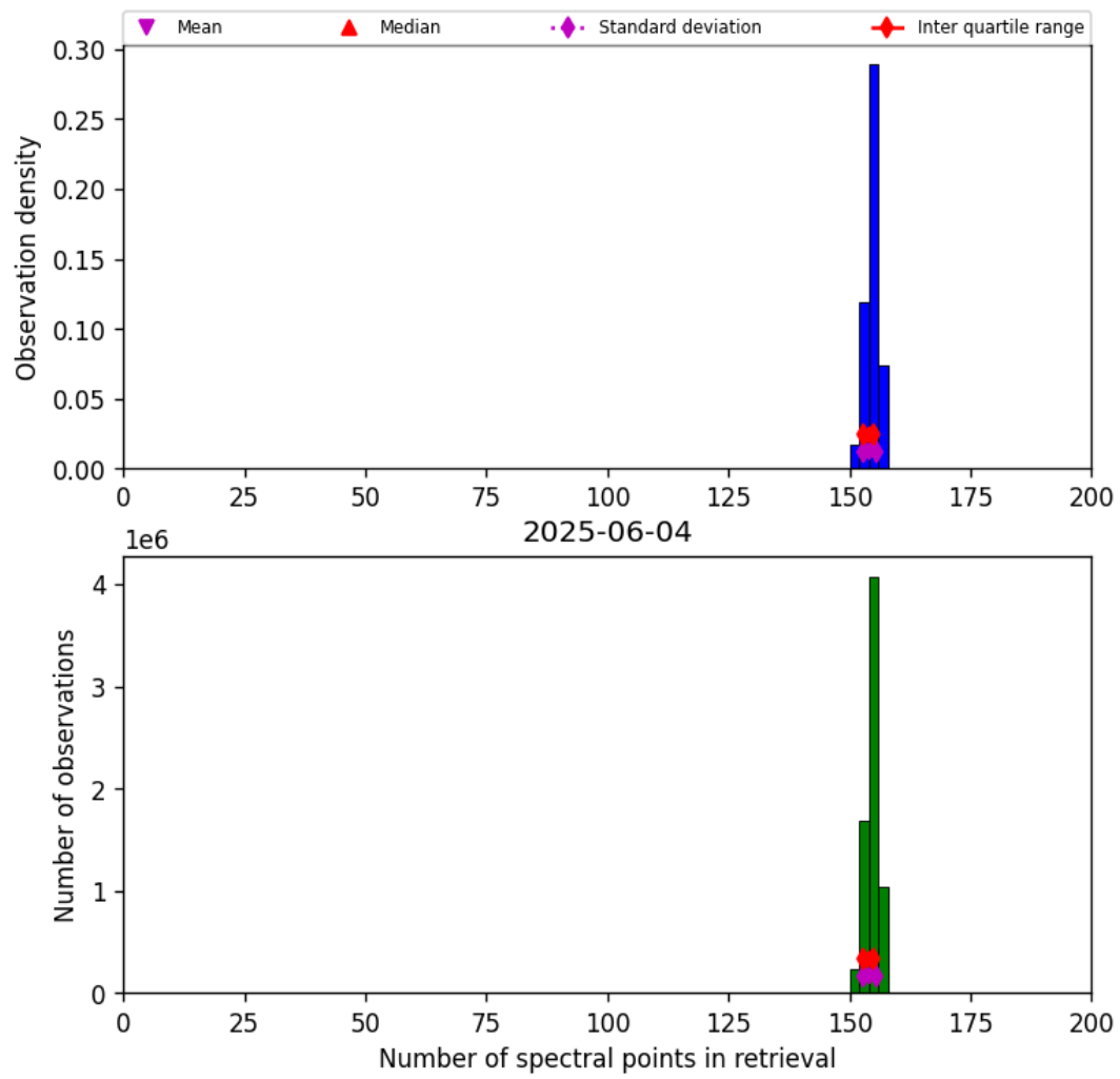
Figure 21: Histogram of “Number of spectral points in retrieval” for 2025-06-03 to 2025-06-05
