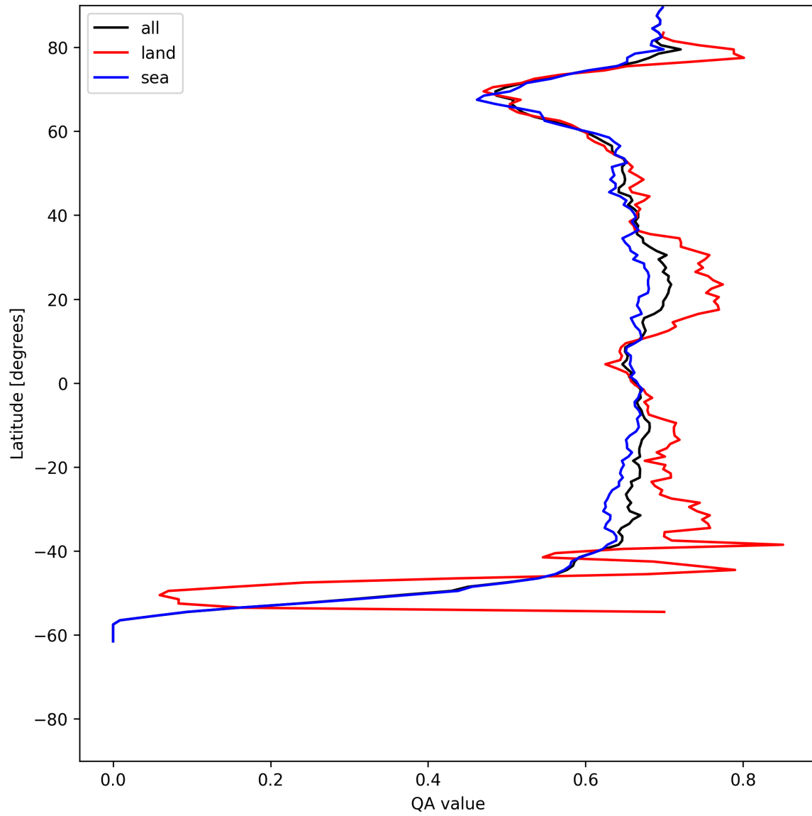
Figure 9: Zonal average of “QA value” for 2025-06-03 to 2025-06-05.
