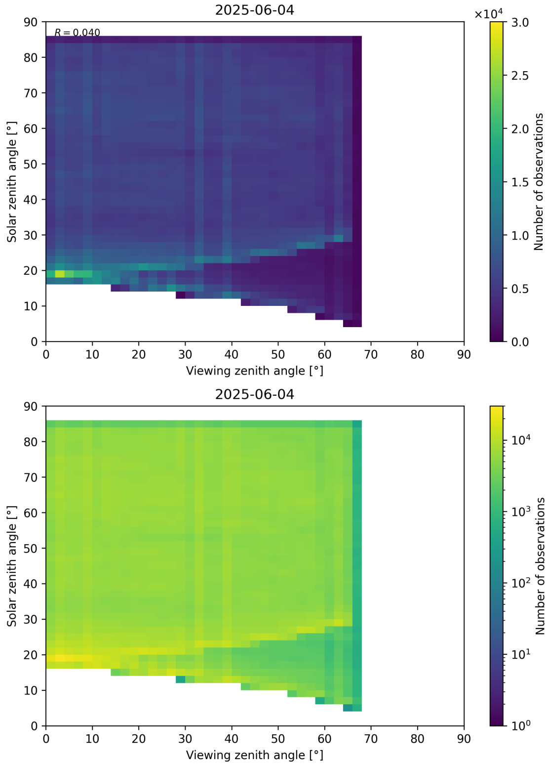
Figure 77: Scatter density plot of “Viewing zenith angle” against “Solar zenith angle” for 2025-06-03 to 2025-06-05.
