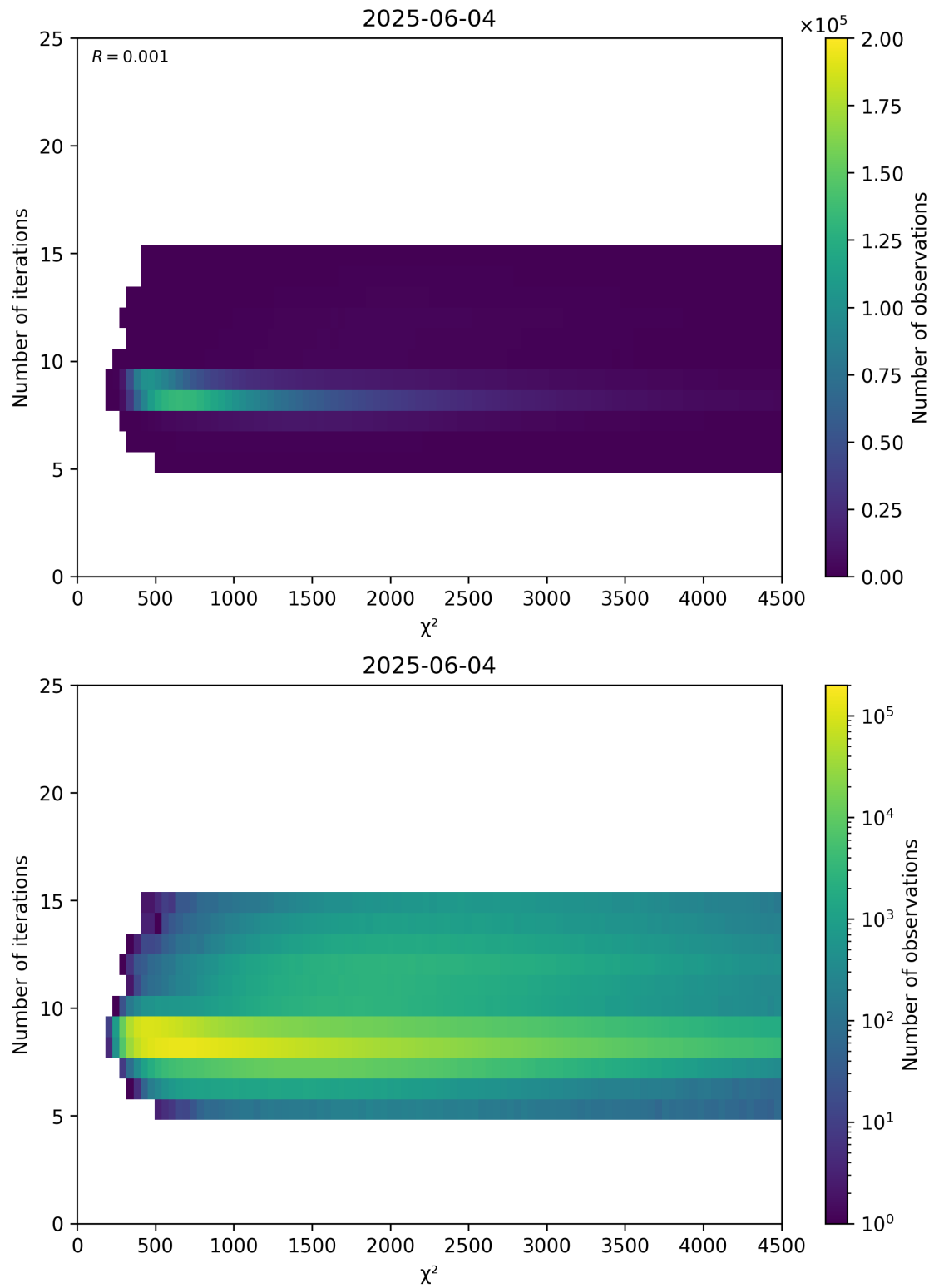
Figure 49: Scatter density plot of “ \chi^2 ” against “Number of iterations” for 2025-06-03 to 2025-06-05.
