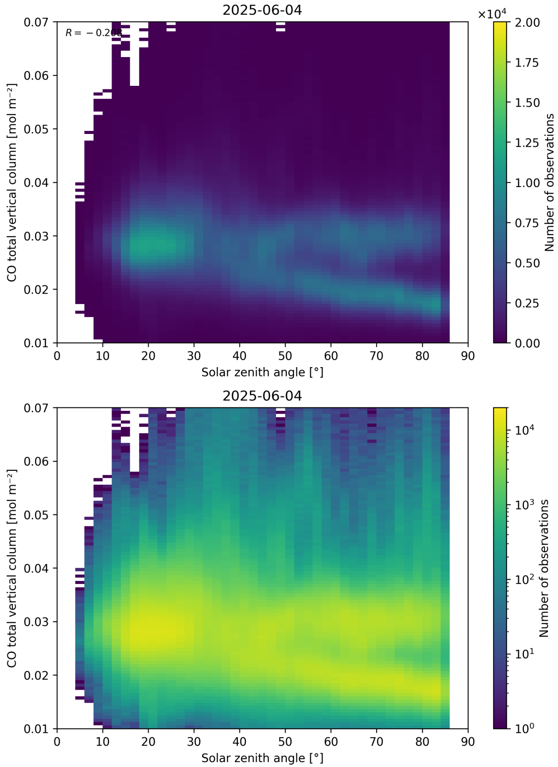
Figure 61: Scatter density plot of “Solar zenith angle” against “CO total vertical column” for 2025-06-03 to 2025-06-05.
