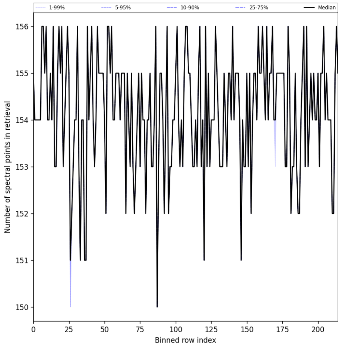
Figure 29: Along track statistics of “Number of spectral points in retrieval” for 2025-06-03 to 2025-06-05
