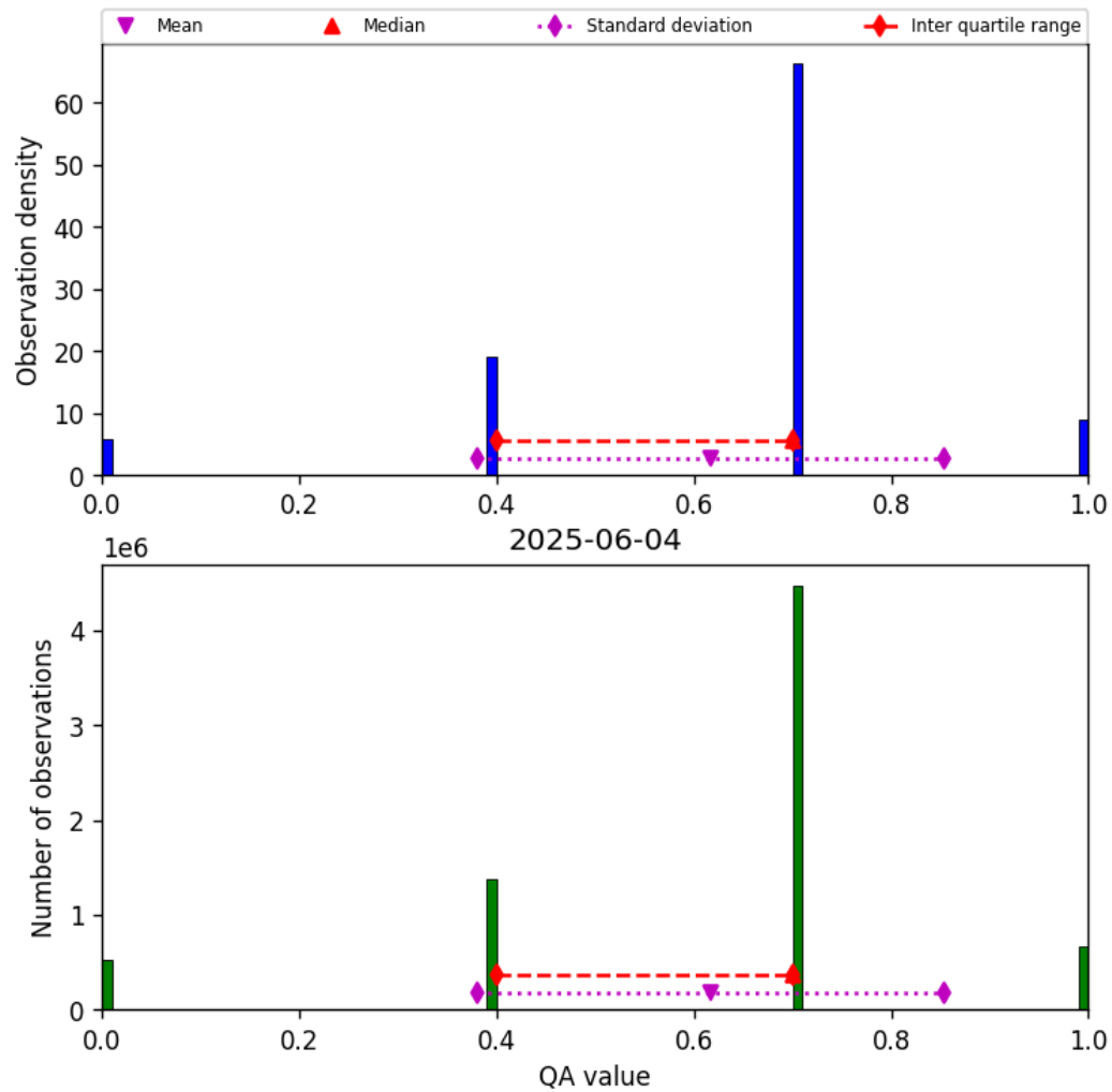
Figure 17: Histogram of “QA value” for 2025-06-03 to 2025-06-05
