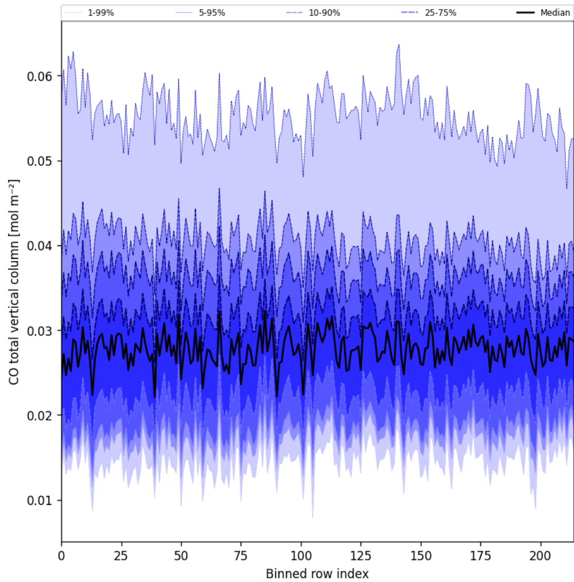
Figure 26: Along track statistics of “CO total vertical column” for 2025-06-03 to 2025-06-05
