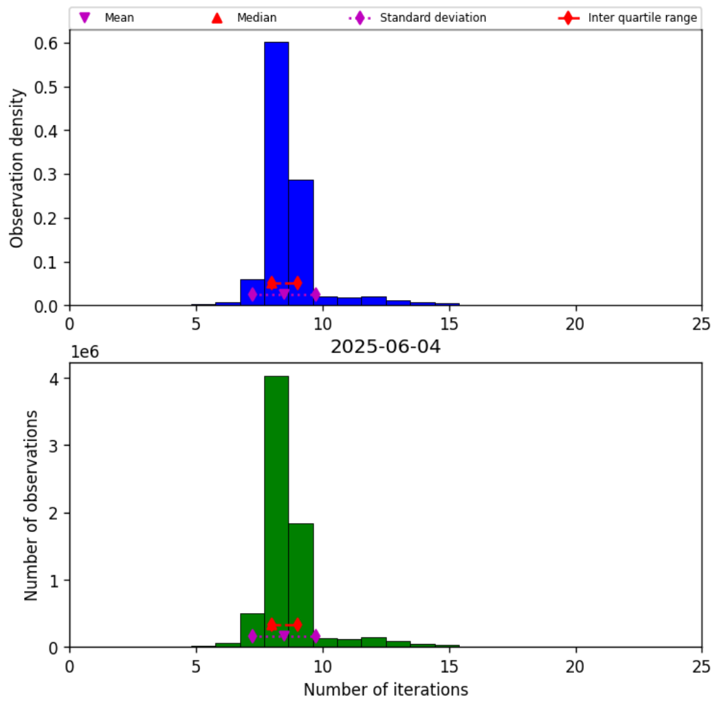
Figure 24: Histogram of “Number of iterations” for 2025-06-03 to 2025-06-05
