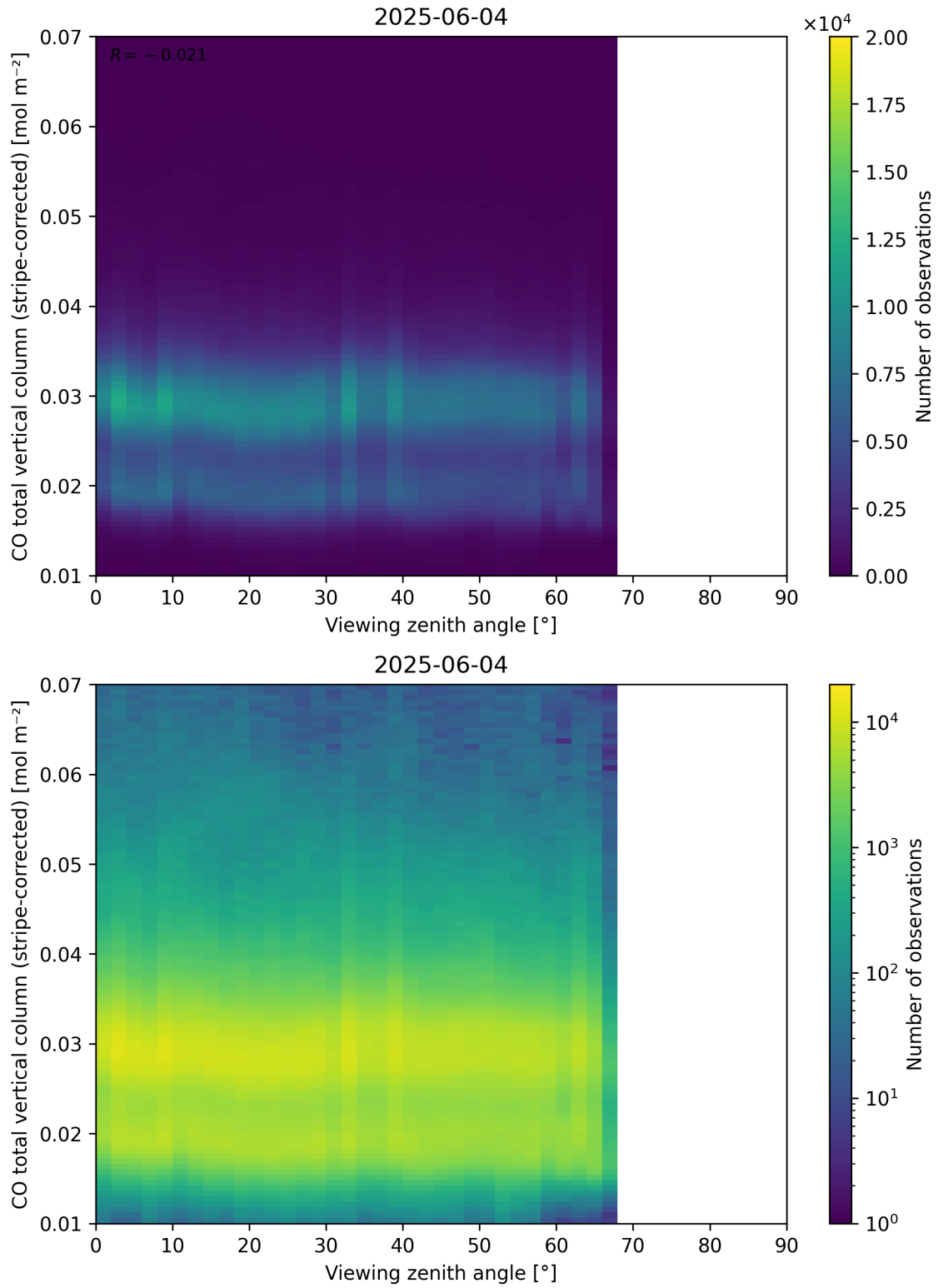
Figure 70: Scatter density plot of “Viewing zenith angle” against “CO total vertical column (stripe-corrected)” for 2025-06-03 to 2025-06-05.
