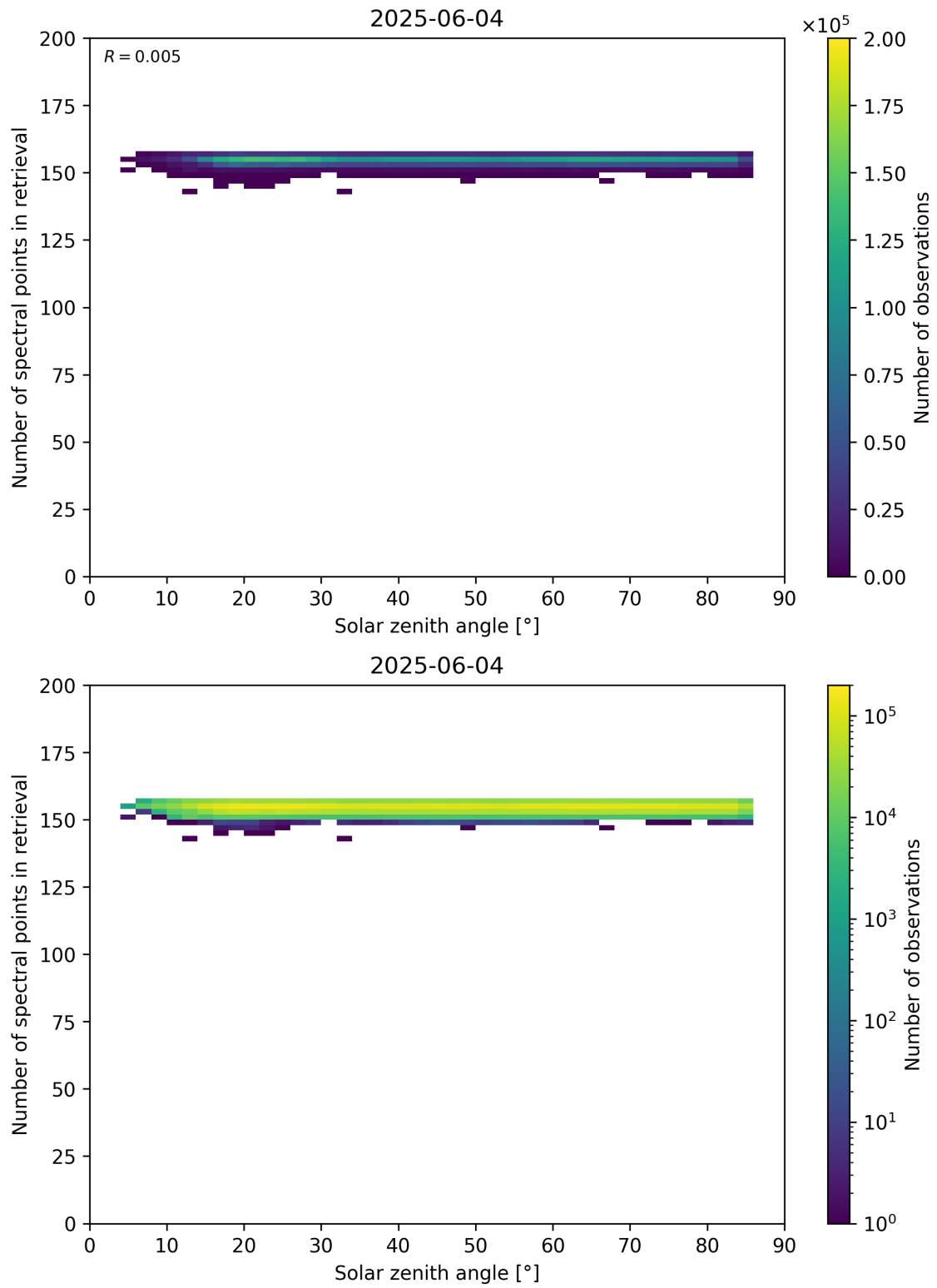
Figure 68: Scatter density plot of “Solar zenith angle” against “Number of spectral points in retrieval” for 2025-06-03 to 2025-06-05.
