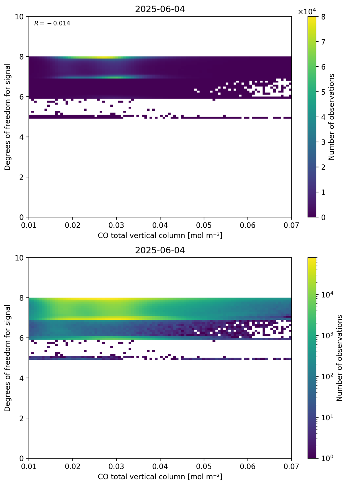
Figure 41: Scatter density plot of “CO total vertical column” against “Degrees of freedom for signal” for 2025-06-03 to 2025-06-05.
