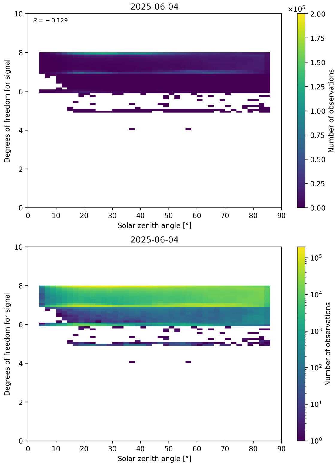
Figure 65: Scatter density plot of “Solar zenith angle” against “Degrees of freedom for signal” for 2025-06-03 to 2025-06-05.
