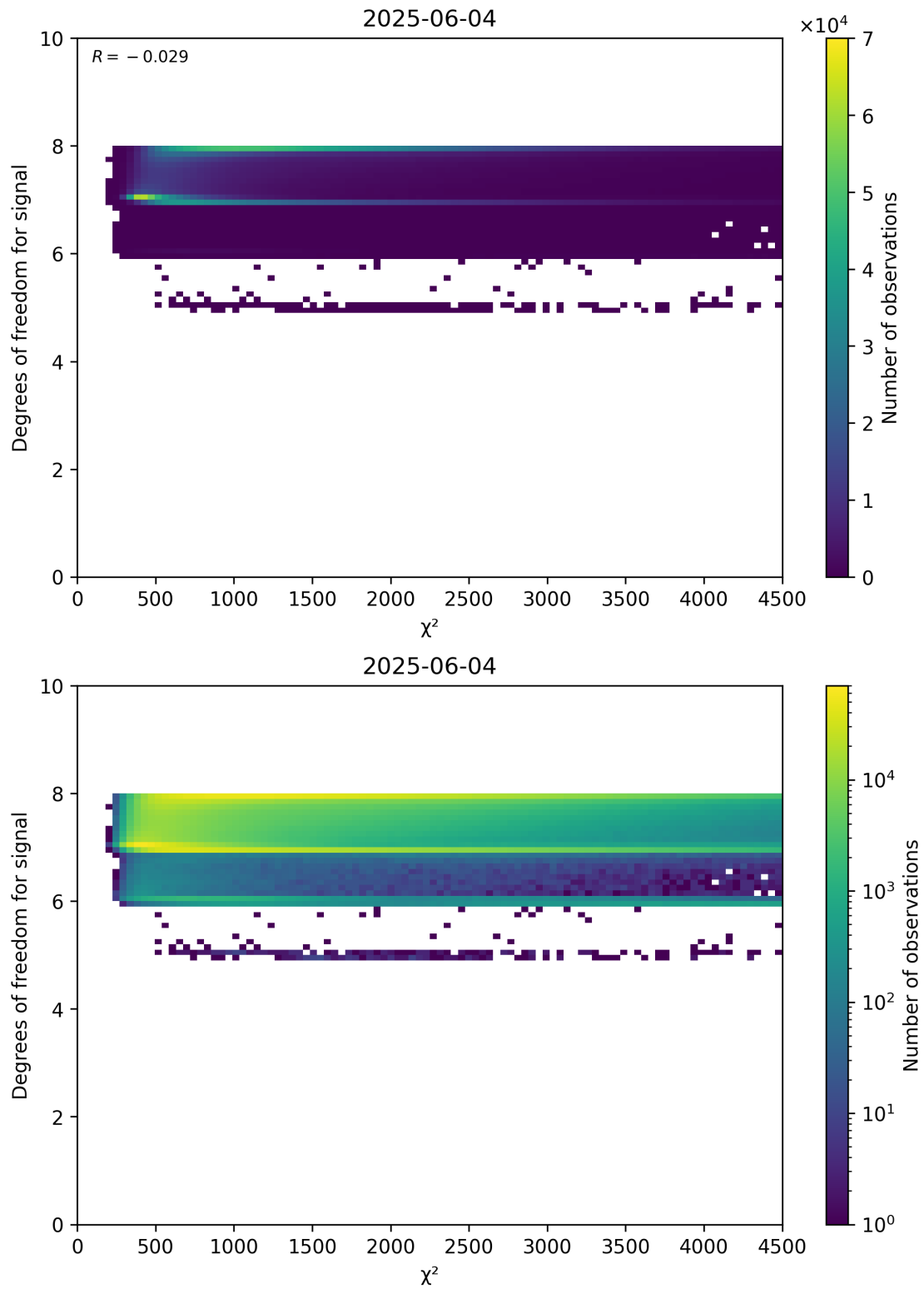
Figure 48: Scatter density plot of “ \chi^2 ” against “Degrees of freedom for signal” for 2025-06-03 to 2025-06-05.
