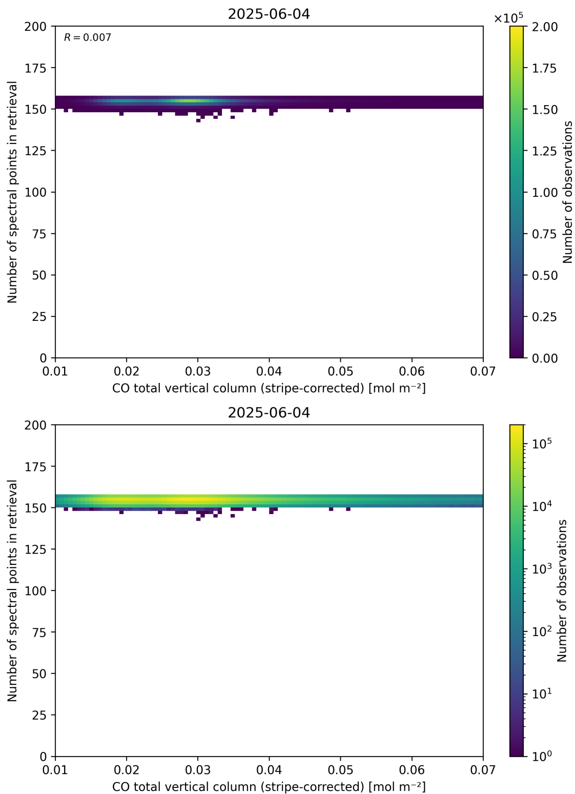
Figure 40: Scatter density plot of “CO total vertical column (stripe-corrected)” against “Number of spectral points in retrieval” for 2025-06-03 to 2025-06-05.
