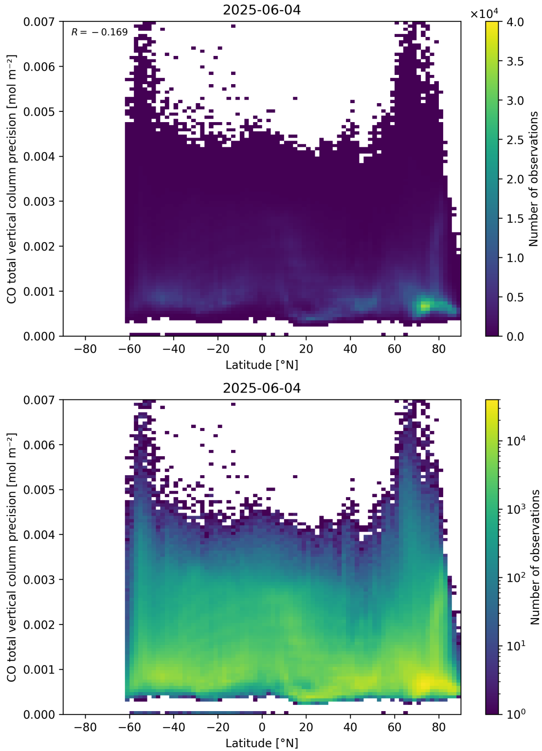
Figure 53: Scatter density plot of “Latitude” against “CO total vertical column precision” for 2025-06-03 to 2025-06-05.
