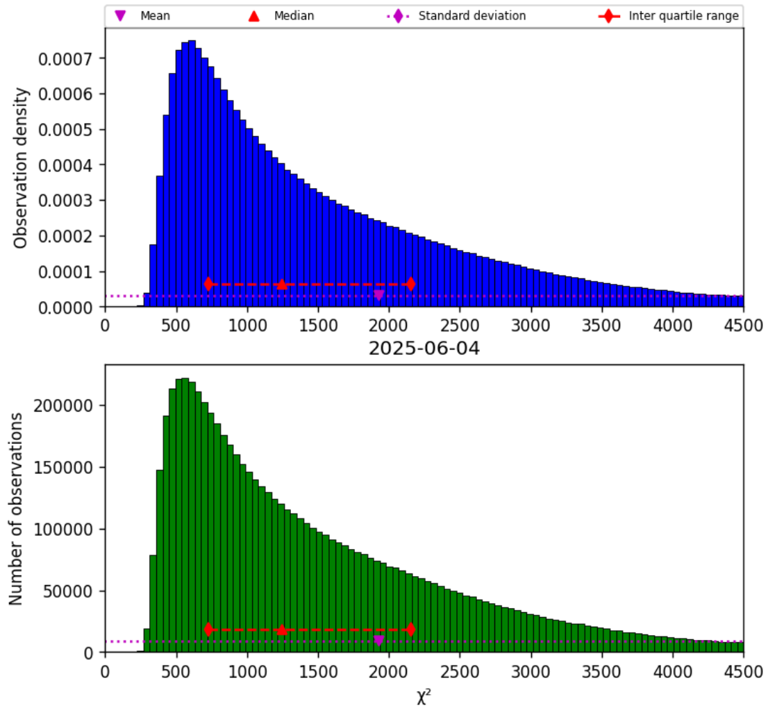
Figure 22: Histogram of " \chi^2 " for 2025-06-03 to 2025-06-05
