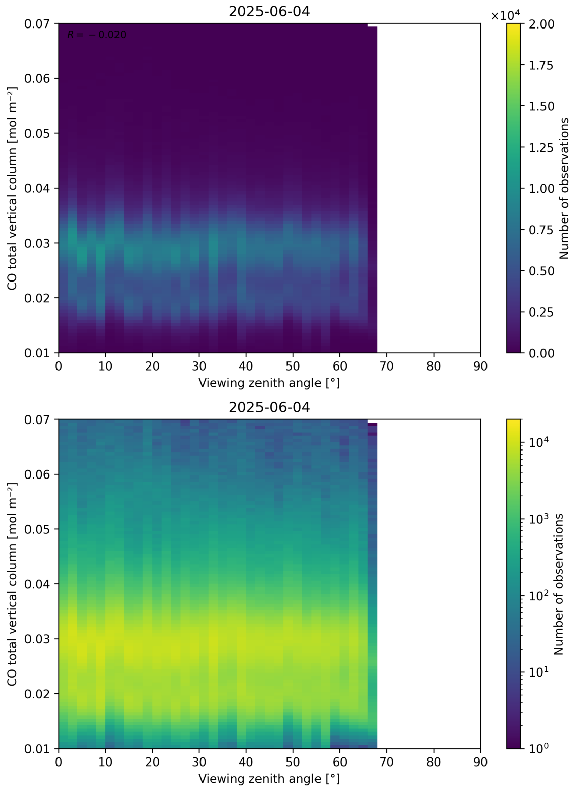
Figure 69: Scatter density plot of “Viewing zenith angle” against “CO total vertical column” for 2025-06-03 to 2025-06-05.
