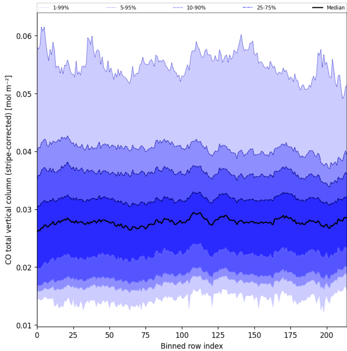
Figure 27: Along track statistics of “CO total vertical column (stripe-corrected)” for 2025-06-03 to 2025-06-05
