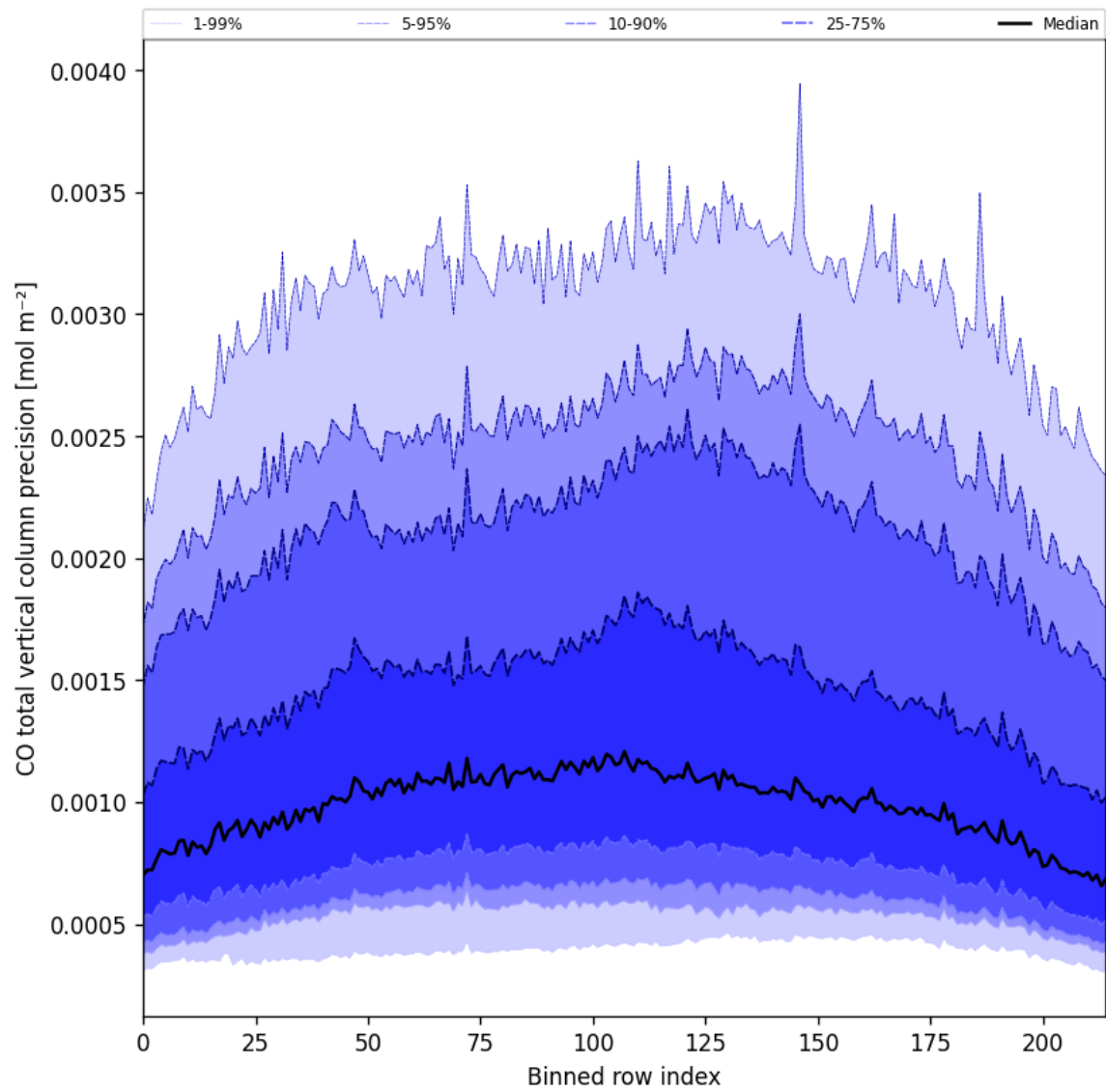
Figure 28: Along track statistics of “CO total vertical column precision” for 2025-06-03 to 2025-06-05
