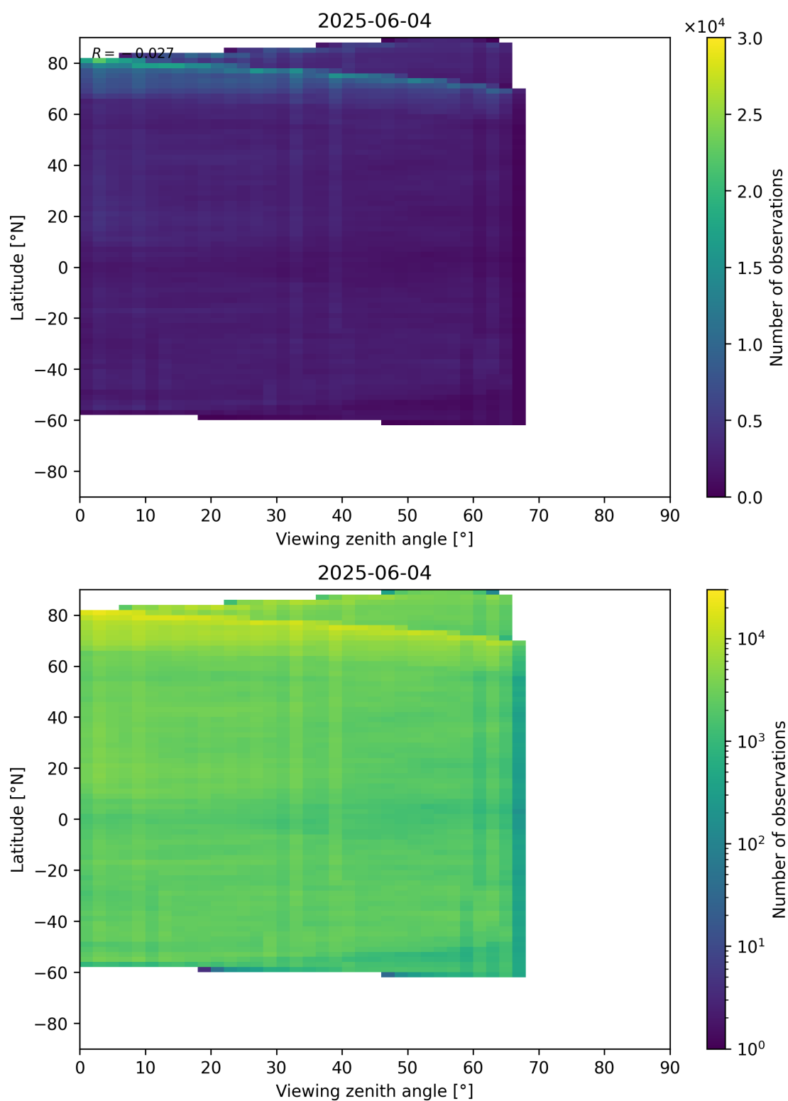
Figure 74: Scatter density plot of “Viewing zenith angle” against “Latitude” for 2025-06-03 to 2025-06-05.
