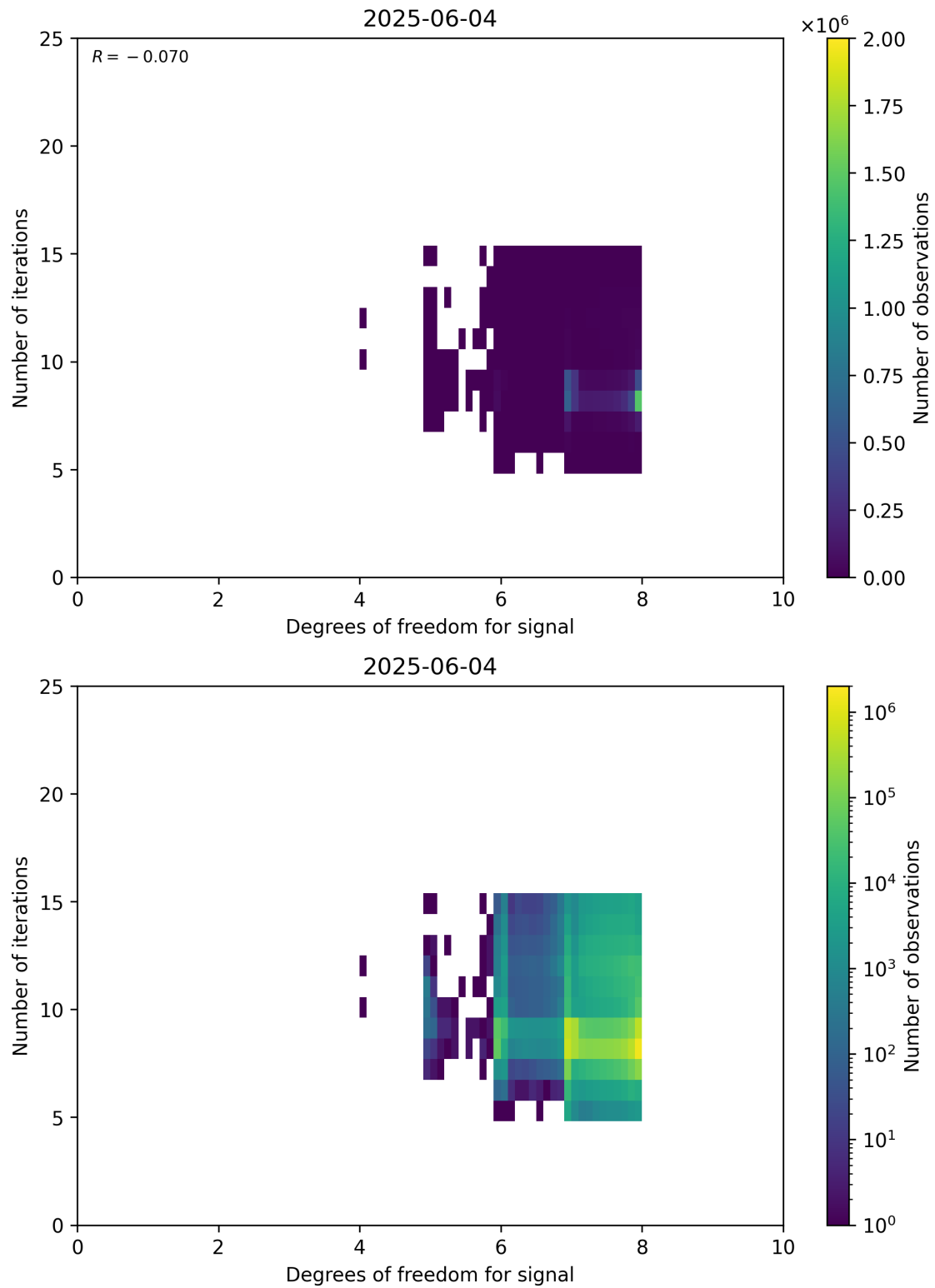
Figure 50: Scatter density plot of “Degrees of freedom for signal” against “Number of iterations” for 2025-06-03 to 2025-06-05.
