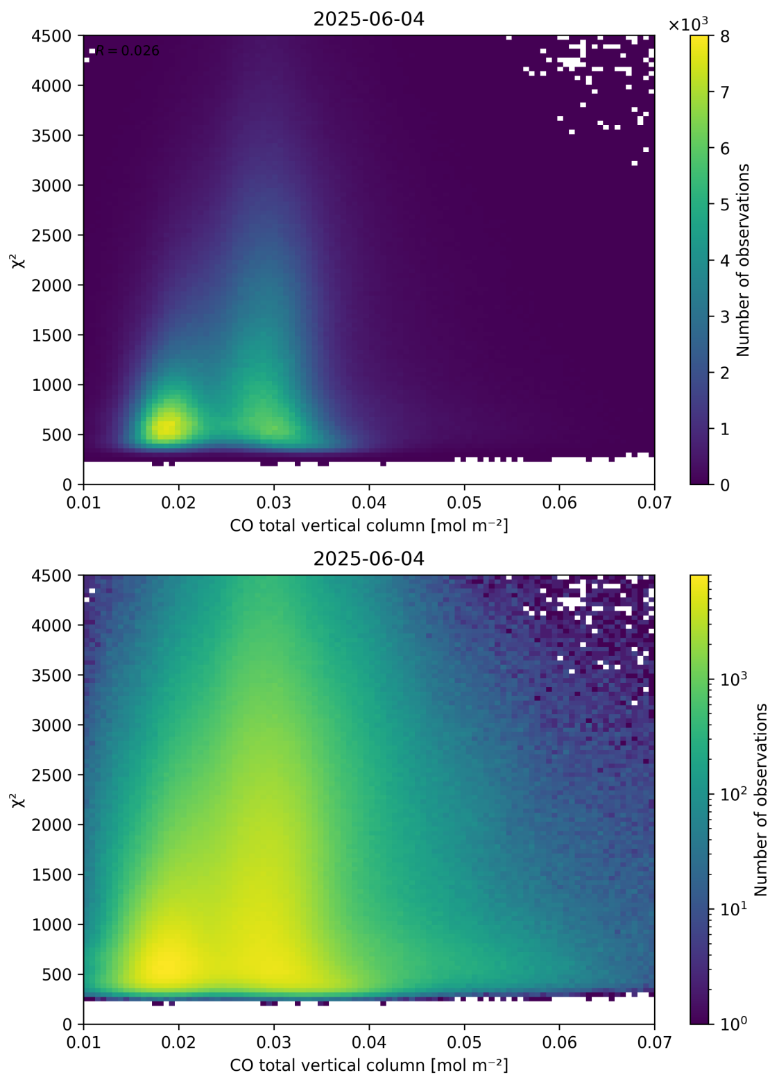
Figure 35: Scatter density plot of “CO total vertical column” against “ \chi^2 ” for 2025-06-03 to 2025-06-05.
