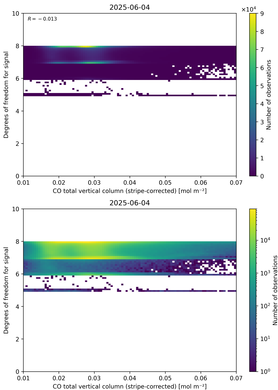
Figure 38: Scatter density plot of “CO total vertical column (stripe-corrected)” against “Degrees of freedom for signal” for 2025-06-03 to 2025-06-05.
