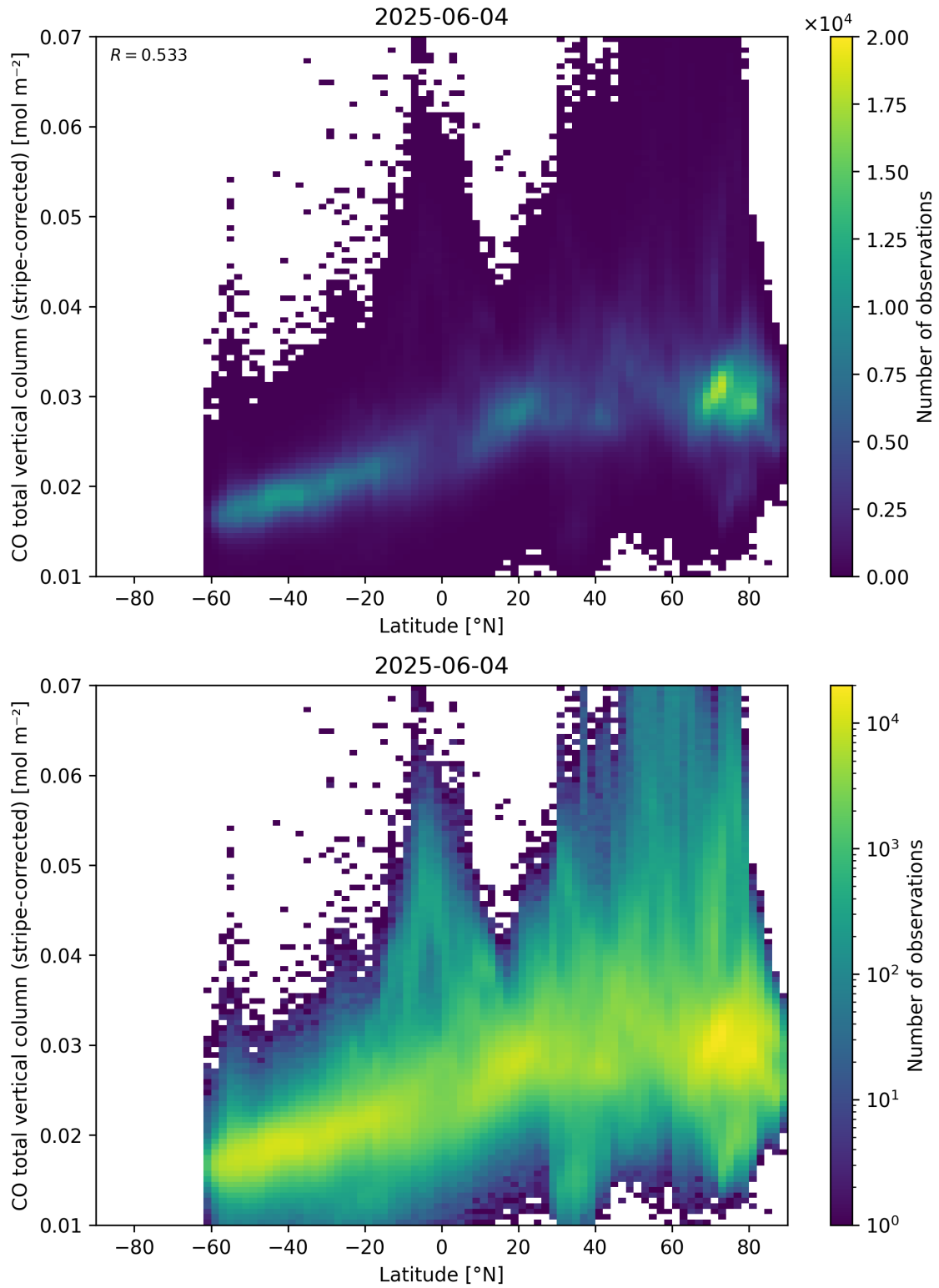
Figure 52: Scatter density plot of “Latitude” against “CO total vertical column (stripe-corrected)” for 2025-06-03 to 2025-06-05.
