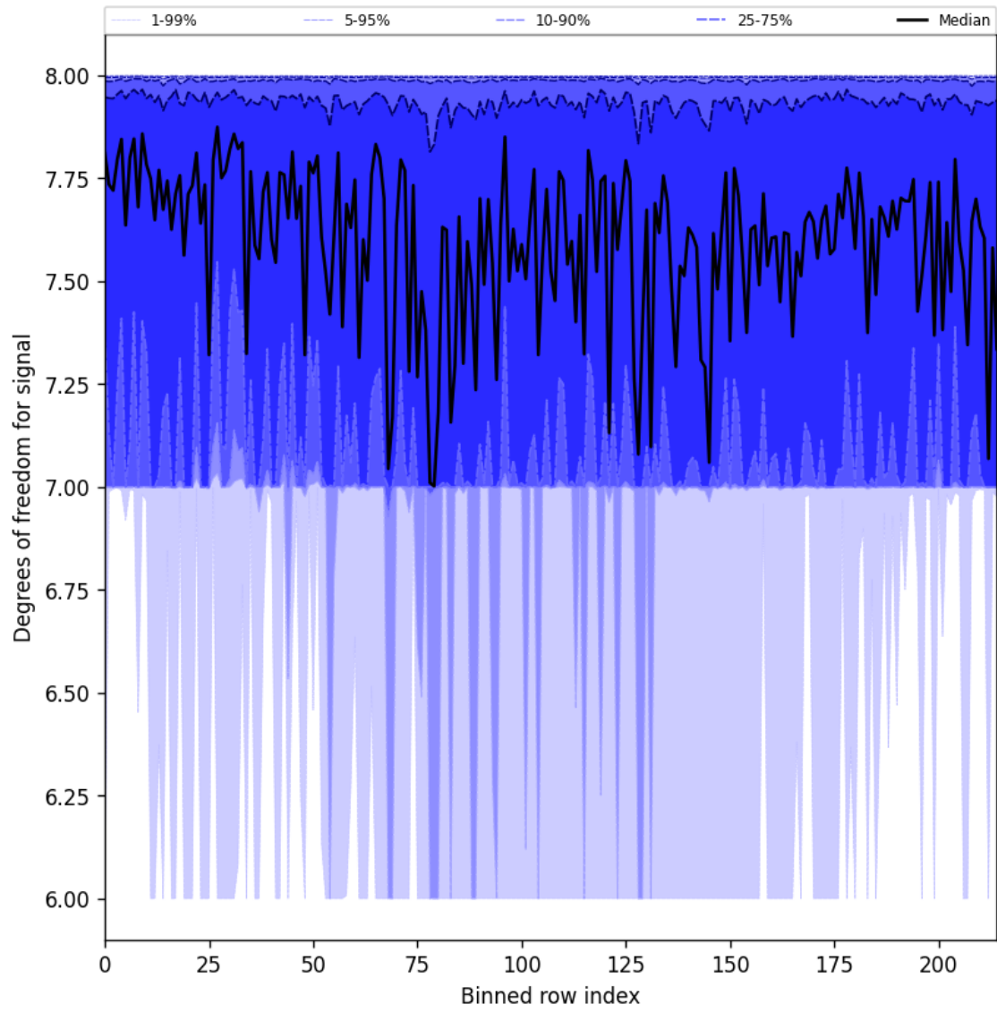
Figure 31: Along track statistics of “Degrees of freedom for signal” for 2025-06-03 to 2025-06-05
