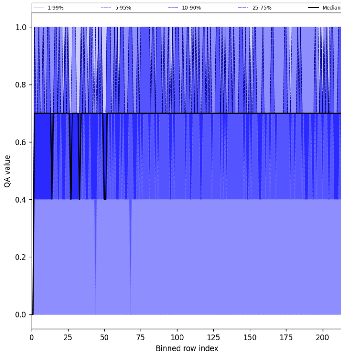
Figure 25: Along track statistics of “QA value” for 2025-06-03 to 2025-06-05
