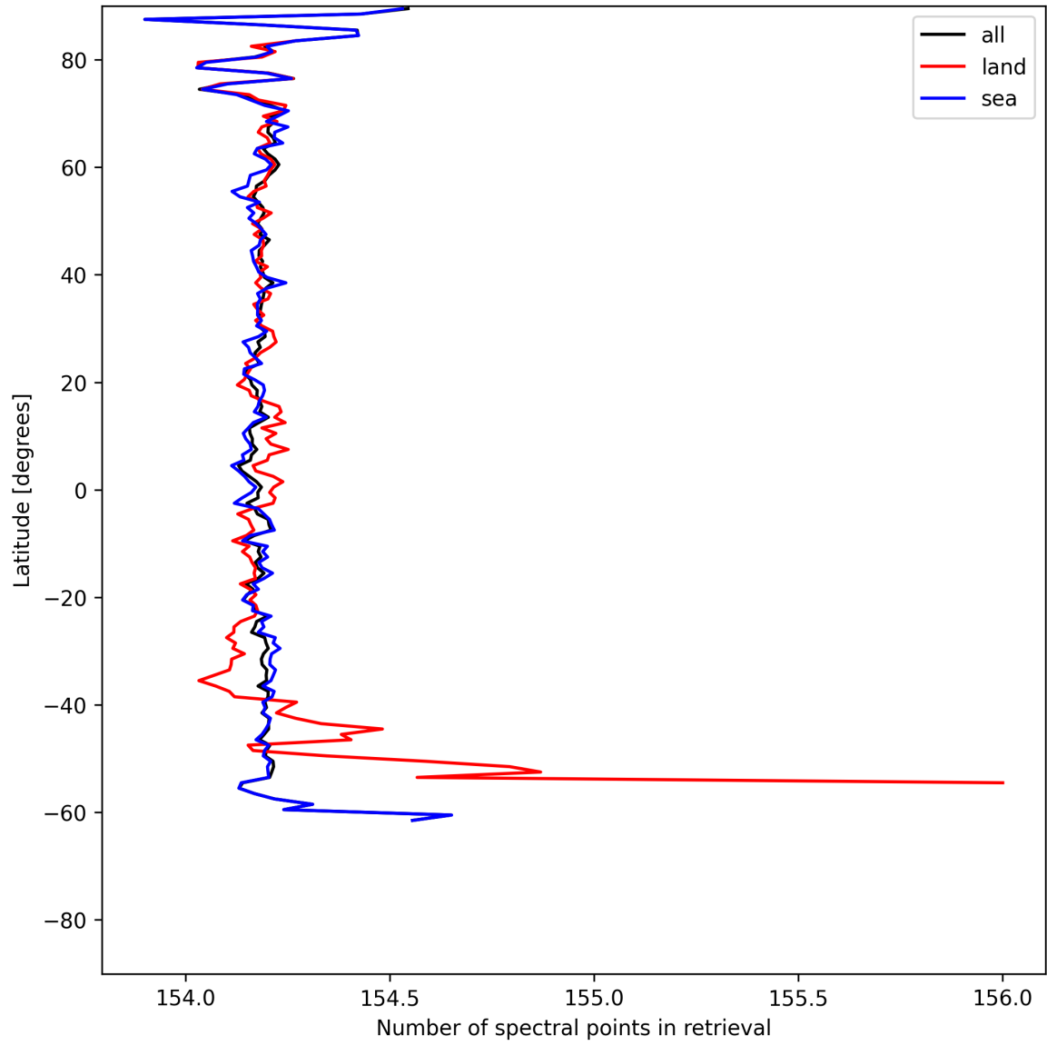
Figure 13: Zonal average of “Number of spectral points in retrieval” for 2025-06-03 to 2025-06-05.
