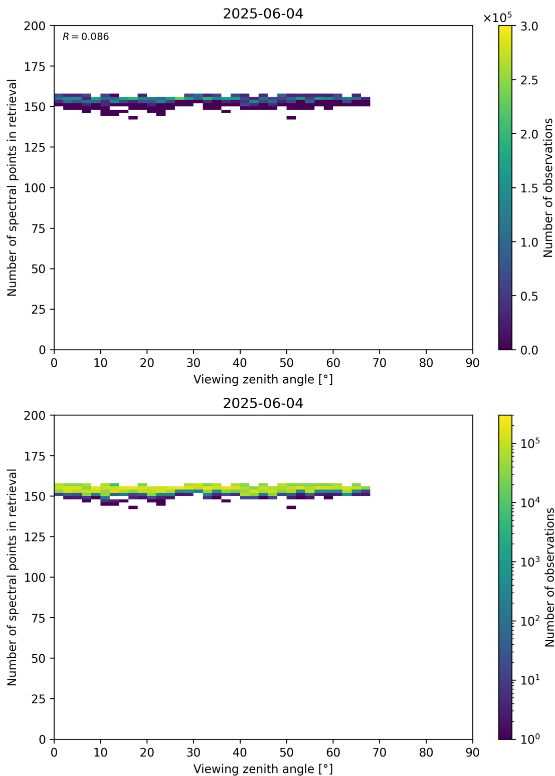
Figure 76: Scatter density plot of “Viewing zenith angle” against “Number of spectral points in retrieval” for 2025-06-03 to 2025-06-05.
