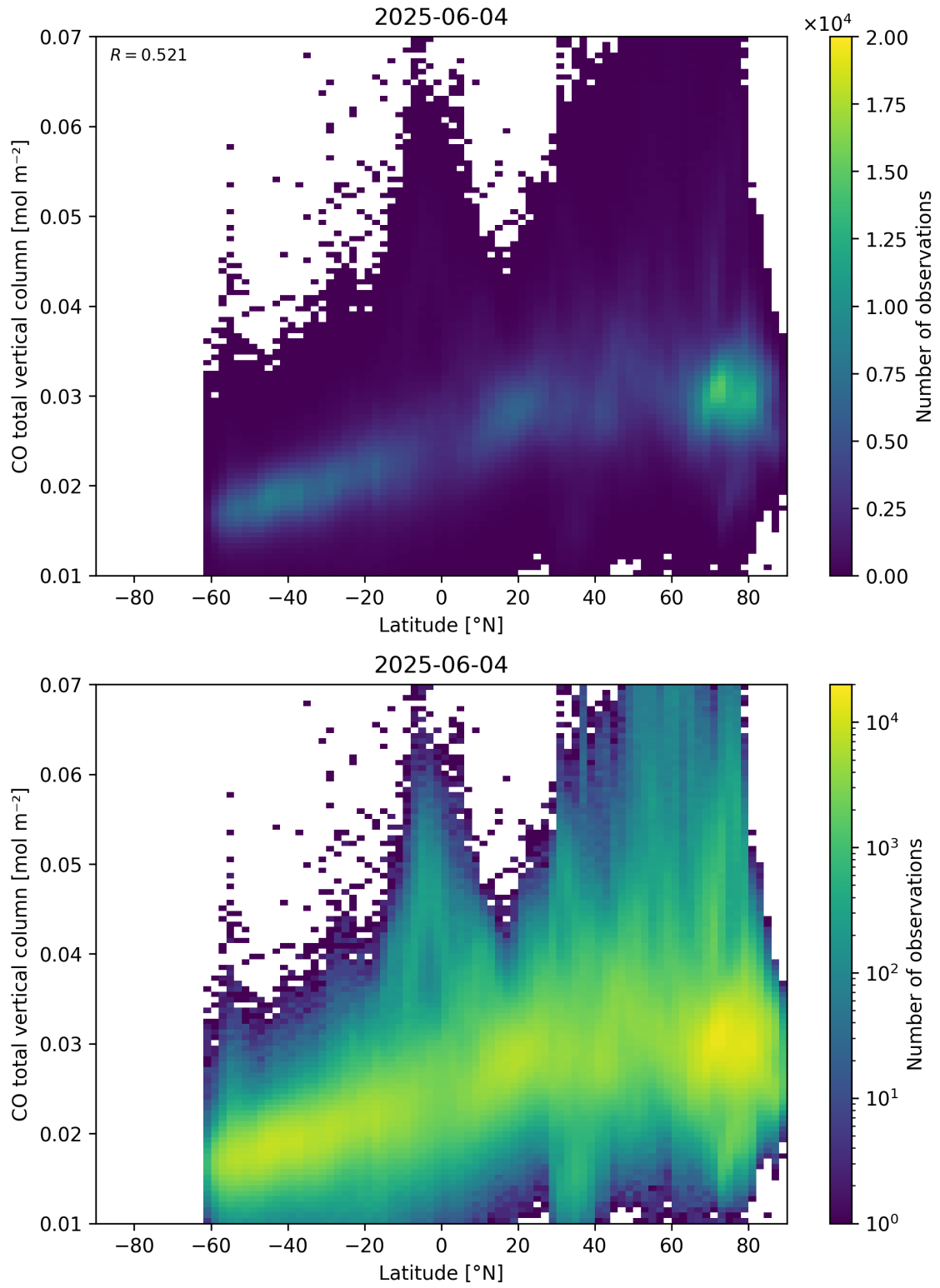
Figure 51: Scatter density plot of “Latitude” against “CO total vertical column” for 2025-06-03 to 2025-06-05.
