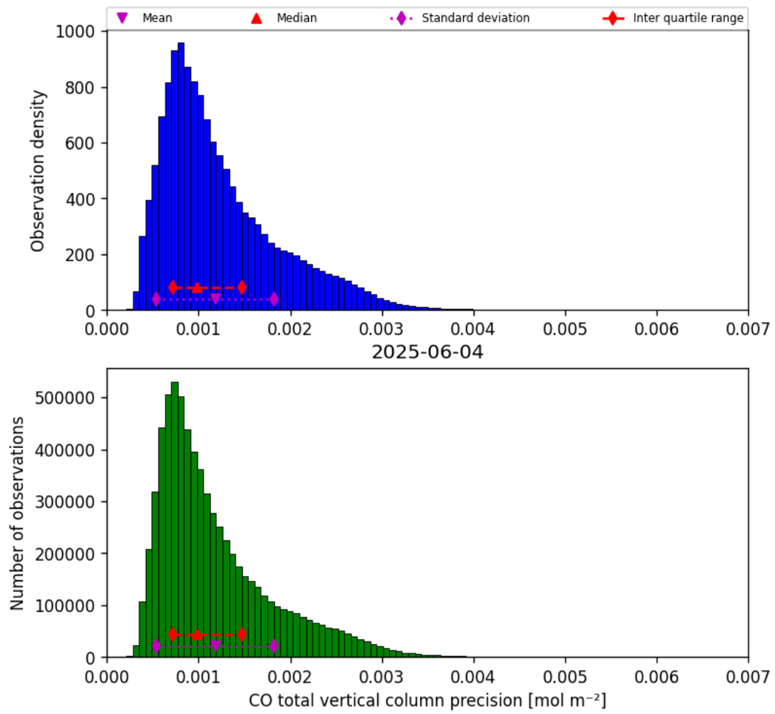
Figure 20: Histogram of “CO total vertical column precision” for 2025-06-03 to 2025-06-05
