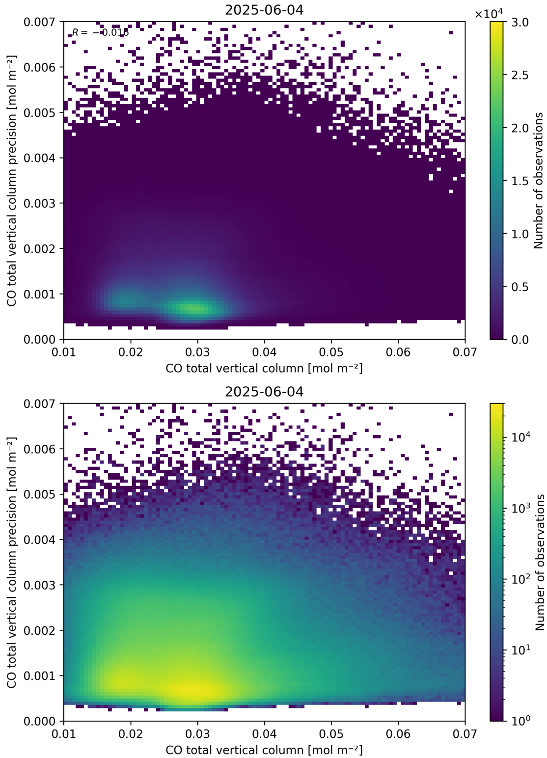
Figure 34: Scatter density plot of “CO total vertical column” against “CO total vertical column precision” for 2025-06-03 to 2025-06-05.
