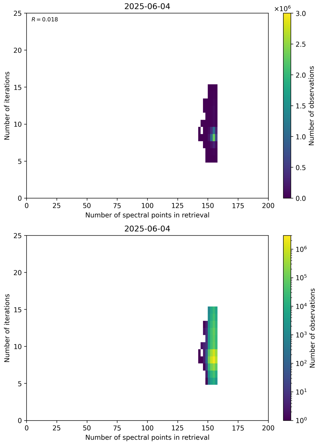
Figure 60: Scatter density plot of “Number of spectral points in retrieval” against “Number of iterations” for 2025-06-03 to 2025-06-05.
