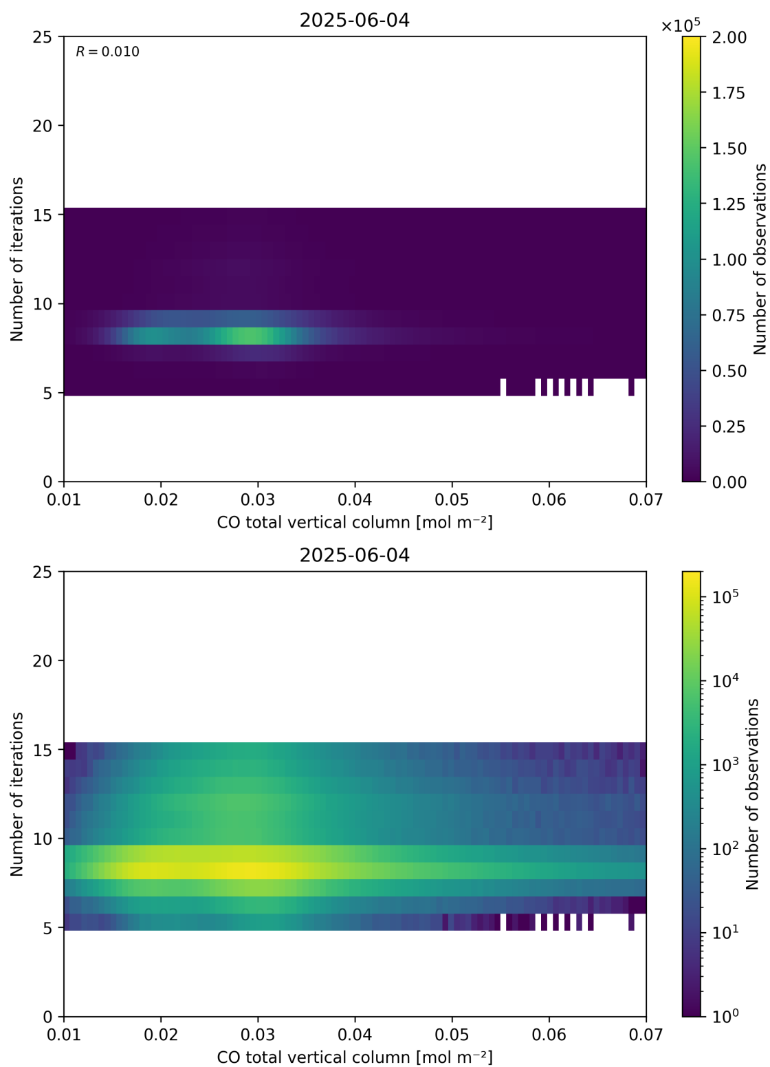
Figure 42: Scatter density plot of “CO total vertical column” against “Number of iterations” for 2025-06-03 to 2025-06-05.
