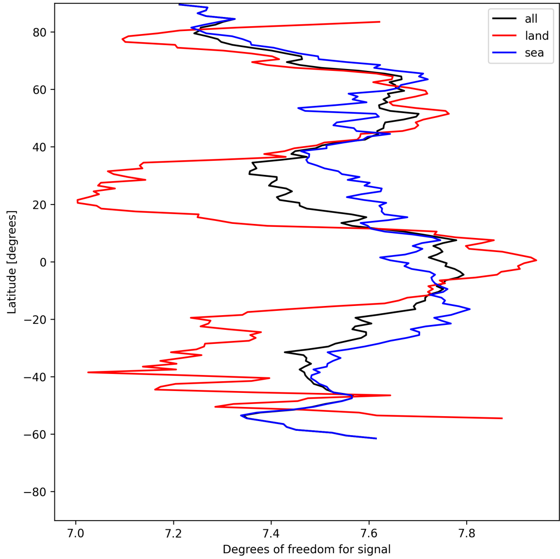
Figure 15: Zonal average of “Degrees of freedom for signal” for 2025-06-03 to 2025-06-05.
