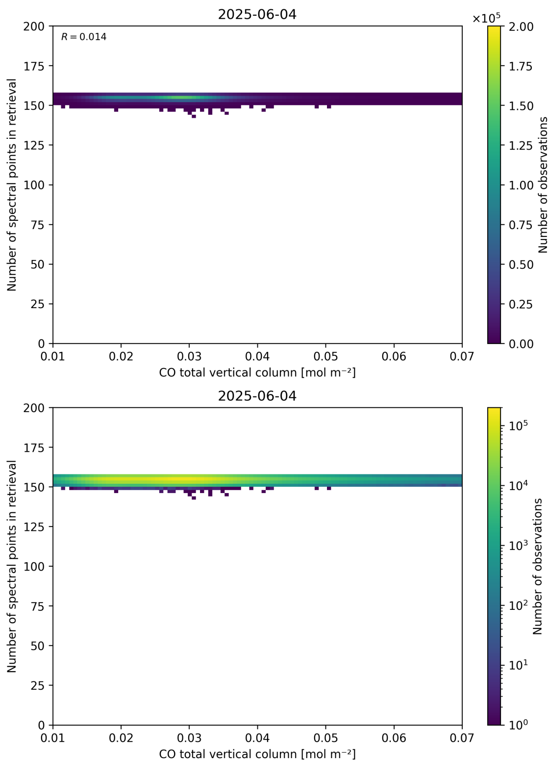
Figure 43: Scatter density plot of “CO total vertical column” against “Number of spectral points in retrieval” for 2025-06-03 to 2025-06-05.
