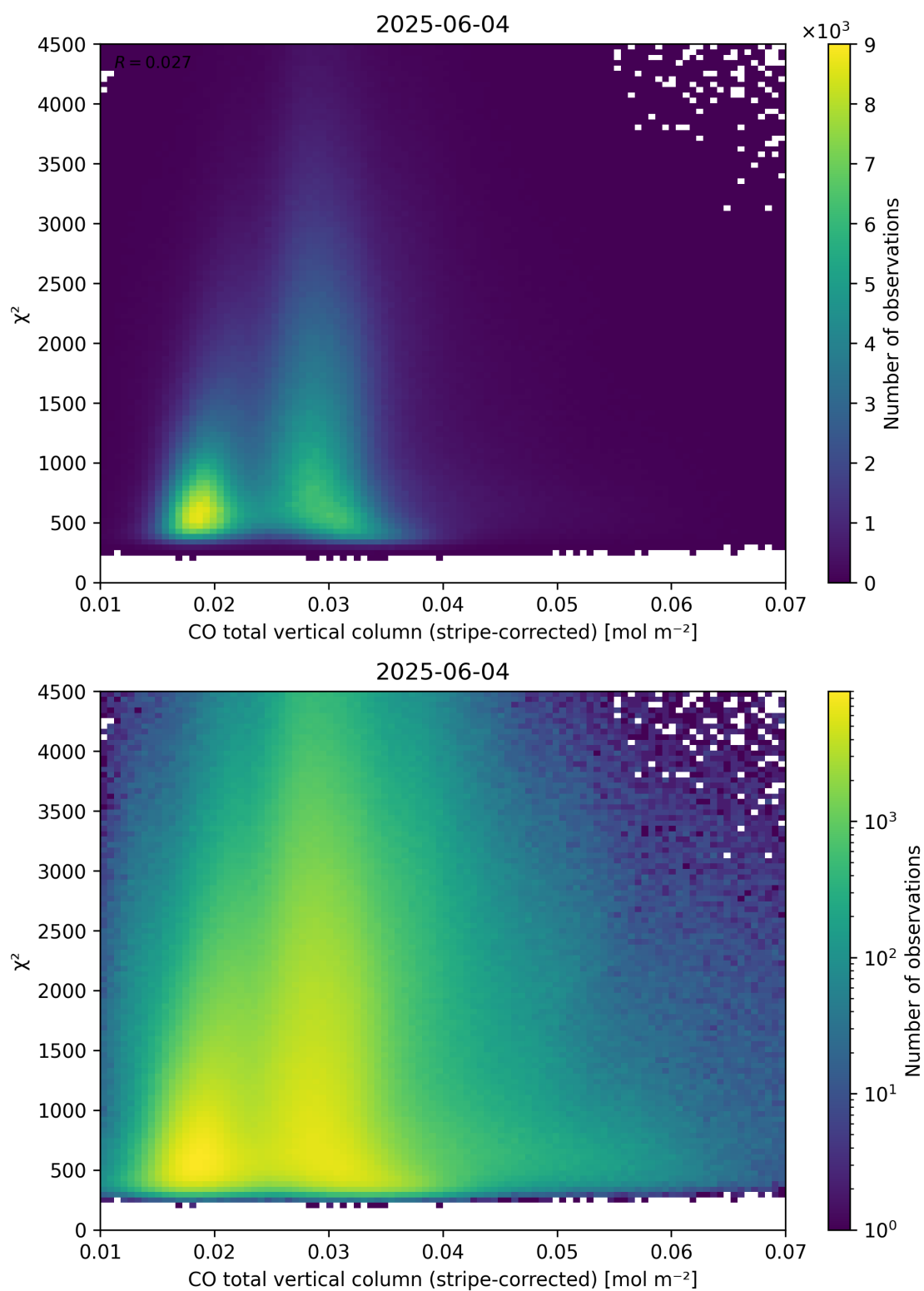
Figure 37: Scatter density plot of “CO total vertical column (stripe-corrected)” against “ \chi^2 ” for 2025-06-03 to 2025-06-05.
