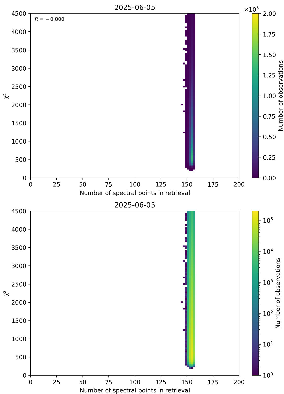
Figure 58: Scatter density plot of “Number of spectral points in retrieval” against “ \chi^2 ” for 2025-06-04 to 2025-06-06.
