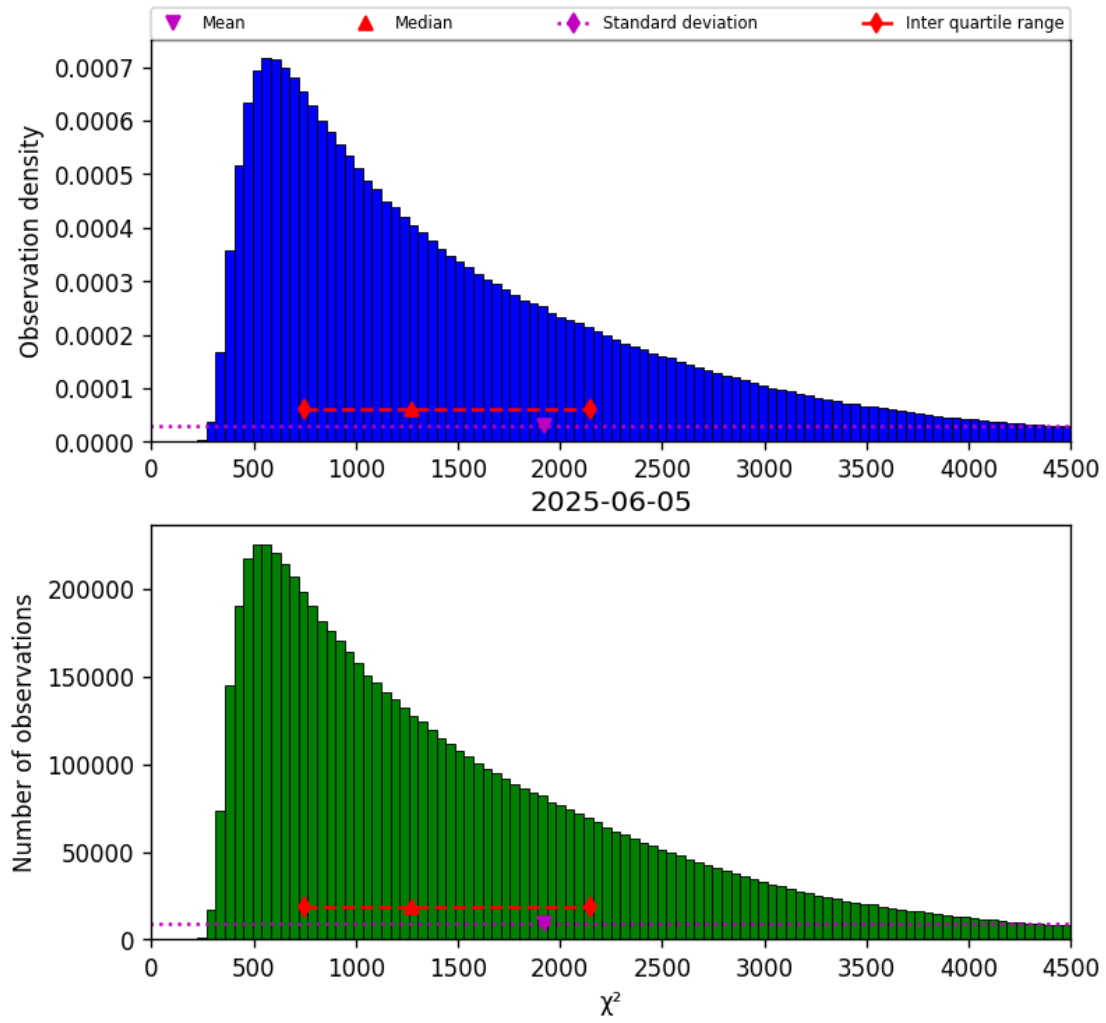
Figure 22: Histogram of “ \chi^2 ” for 2025-06-04 to 2025-06-06
