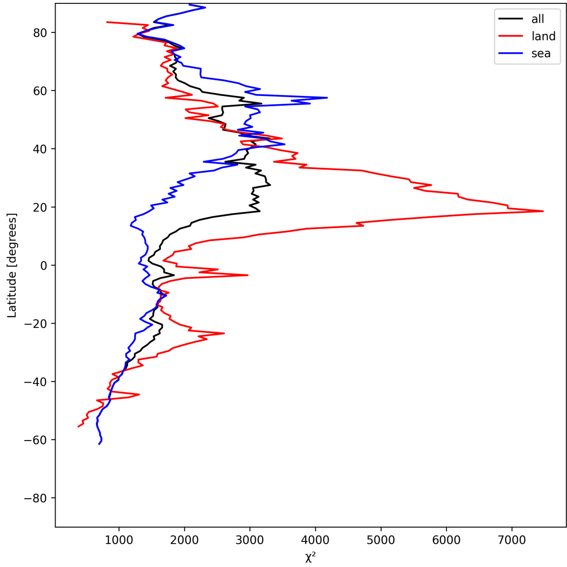
Figure 14: Zonal average of “ \chi^2 ” for 2025-06-04 to 2025-06-06.
