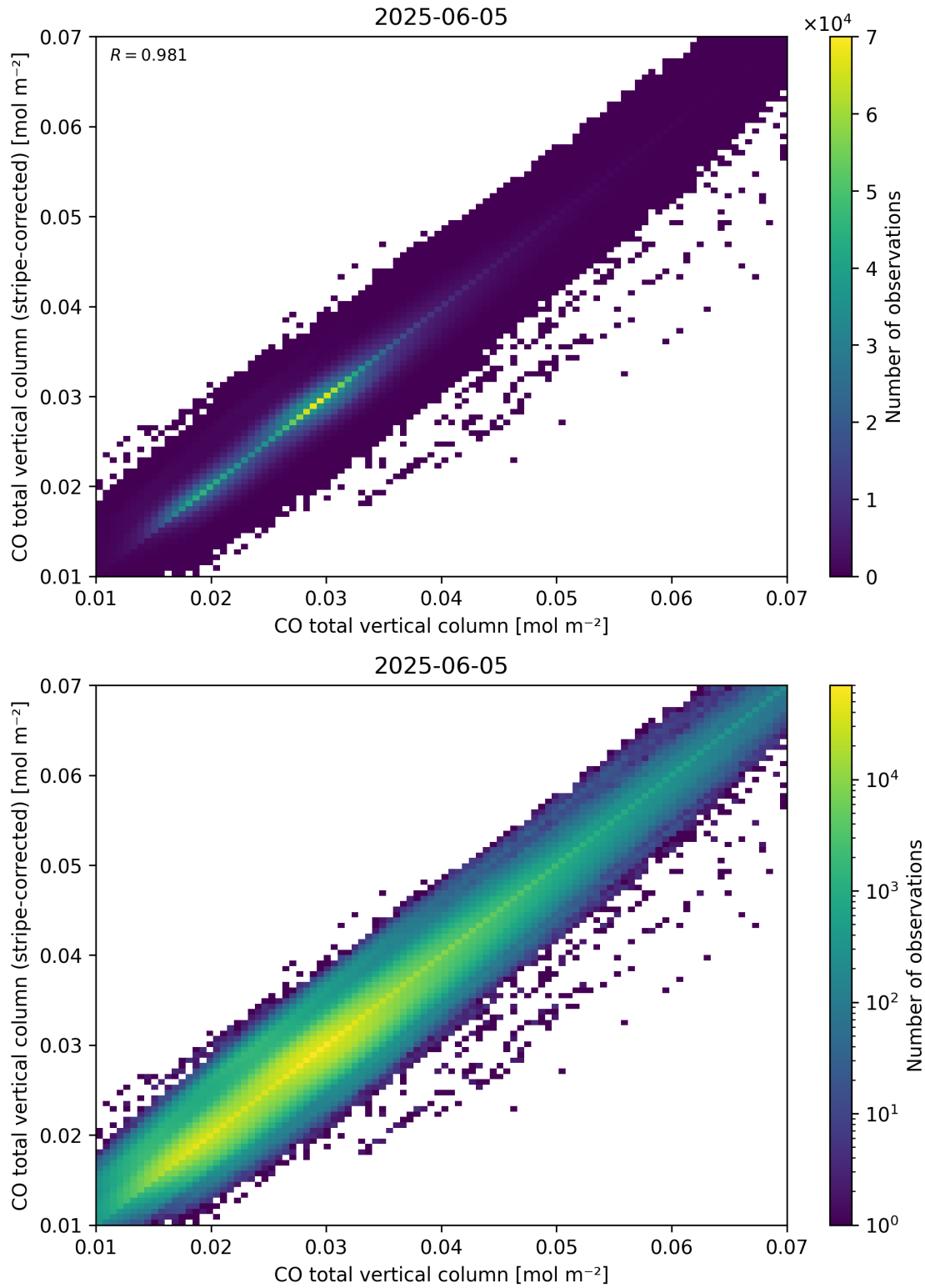
Figure 33: Scatter density plot of “CO total vertical column” against “CO total vertical column (stripe-corrected)” for 2025-06-04 to 2025-06-06.
