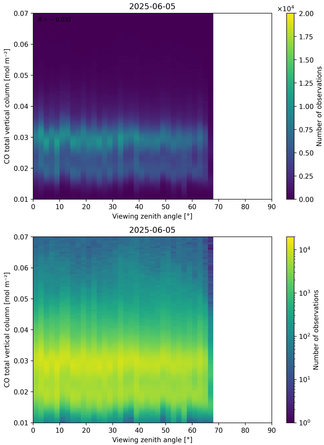
Figure 69: Scatter density plot of “Viewing zenith angle” against “CO total vertical column” for 2025-06-04 to 2025-06-06.
