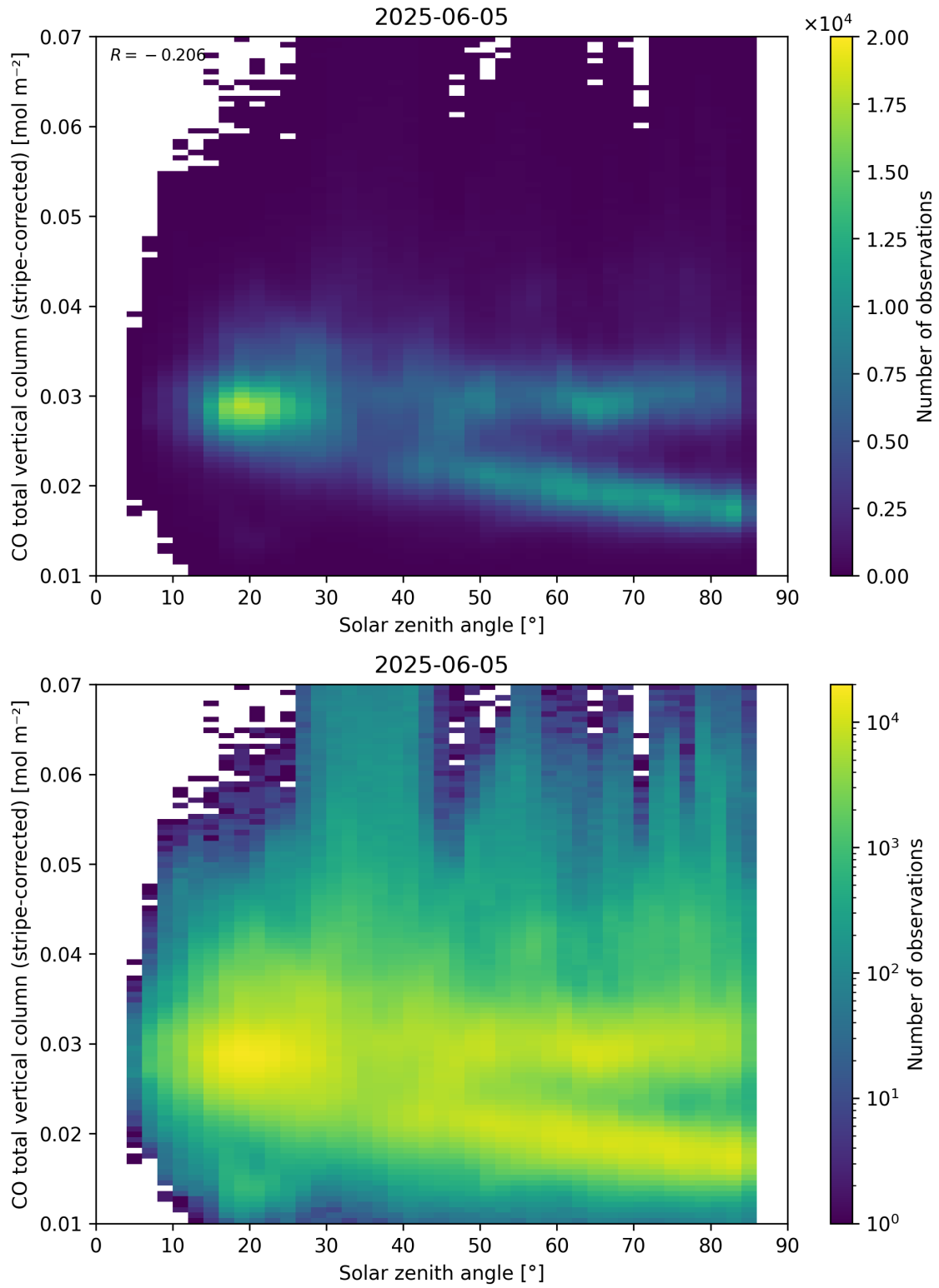
Figure 62: Scatter density plot of “Solar zenith angle” against “CO total vertical column (stripe-corrected)” for 2025-06-04 to 2025-06-06.
