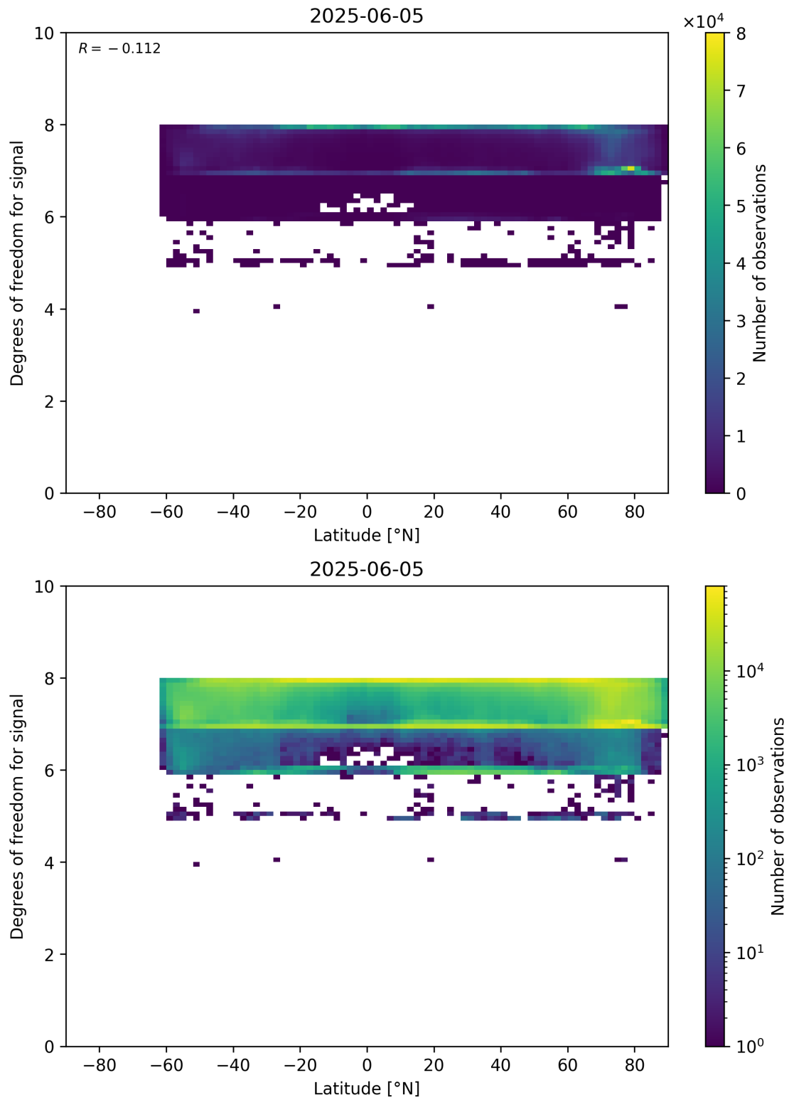
Figure 55: Scatter density plot of “Latitude” against “Degrees of freedom for signal” for 2025-06-04 to 2025-06-06.
