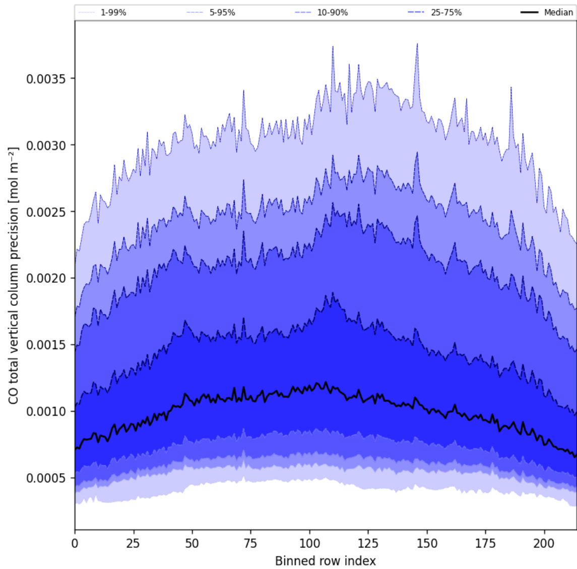
Figure 28: Along track statistics of “CO total vertical column precision” for 2025-06-04 to 2025-06-06
