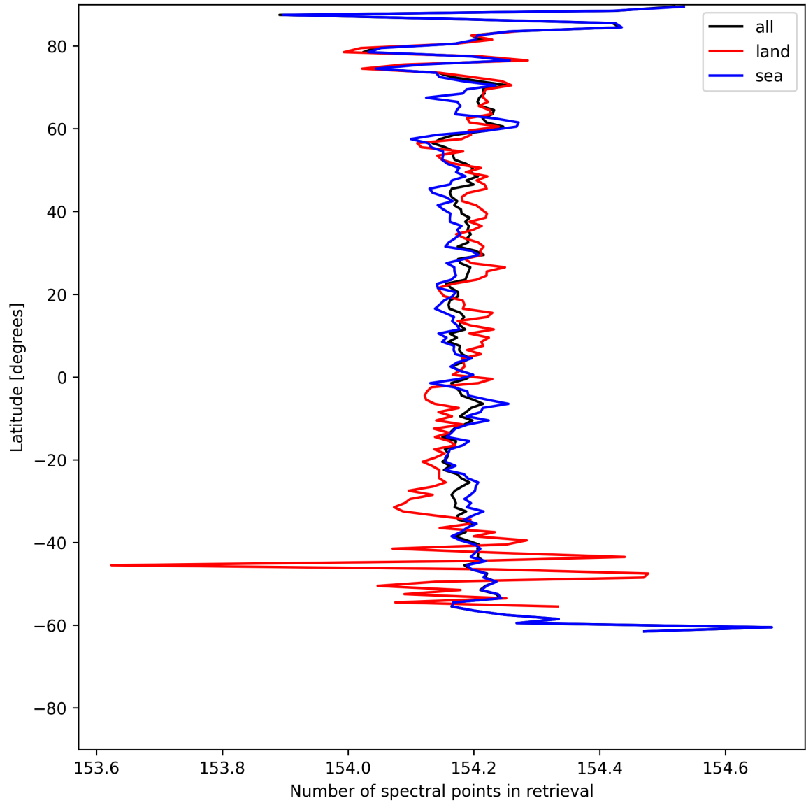
Figure 13: Zonal average of “Number of spectral points in retrieval” for 2025-06-04 to 2025-06-06.
