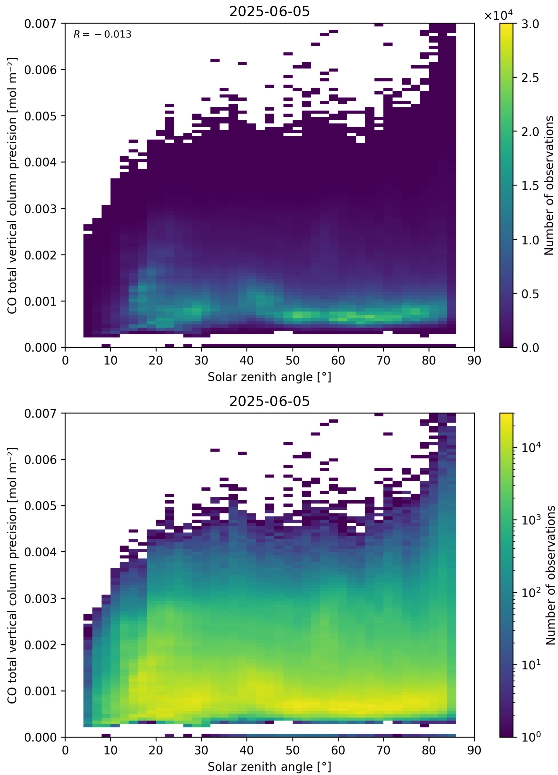
Figure 63: Scatter density plot of “Solar zenith angle” against “CO total vertical column precision” for 2025-06-04 to 2025-06-06.
