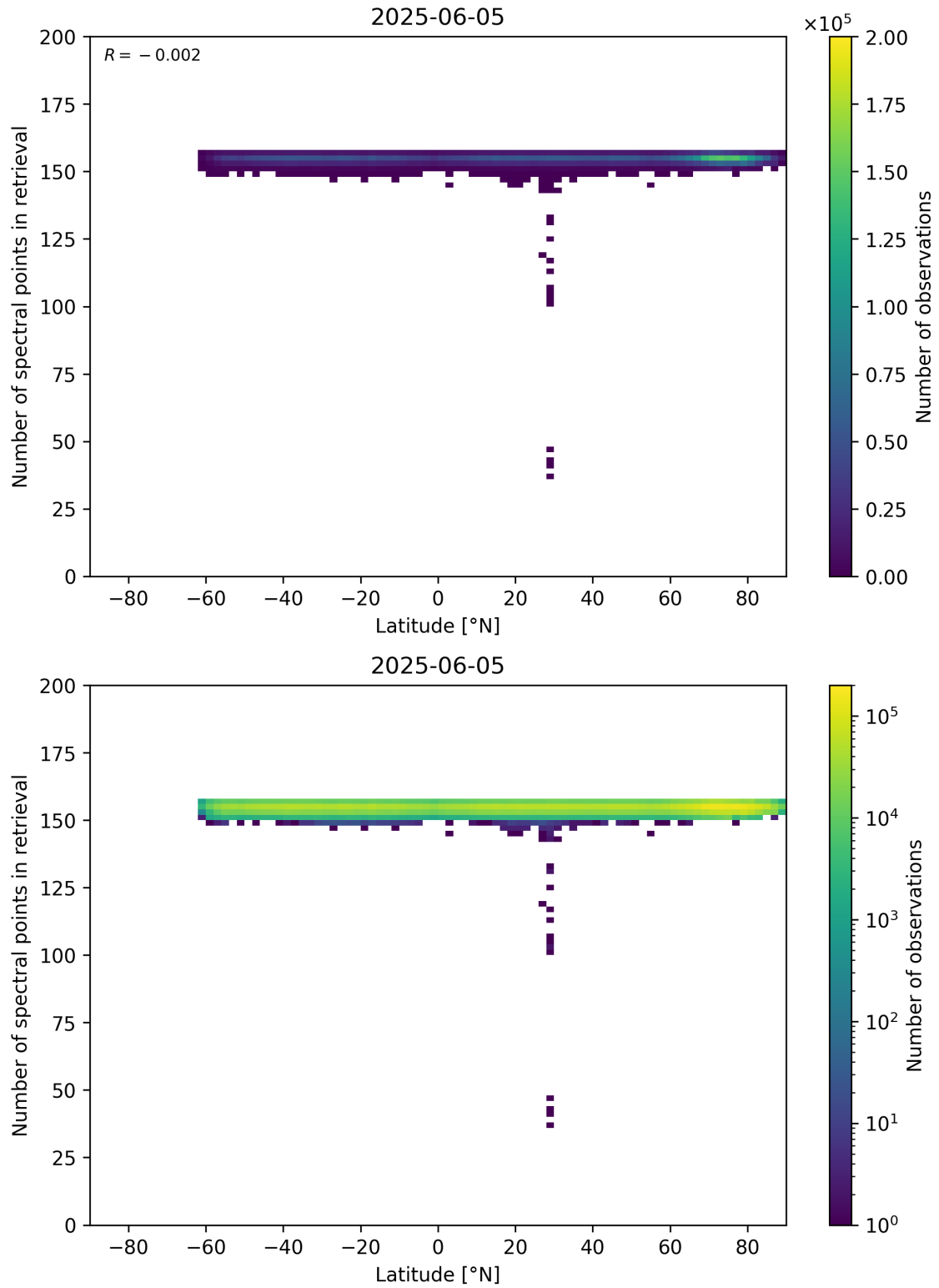
Figure 57: Scatter density plot of “Latitude” against “Number of spectral points in retrieval” for 2025-06-04 to 2025-06-06.
