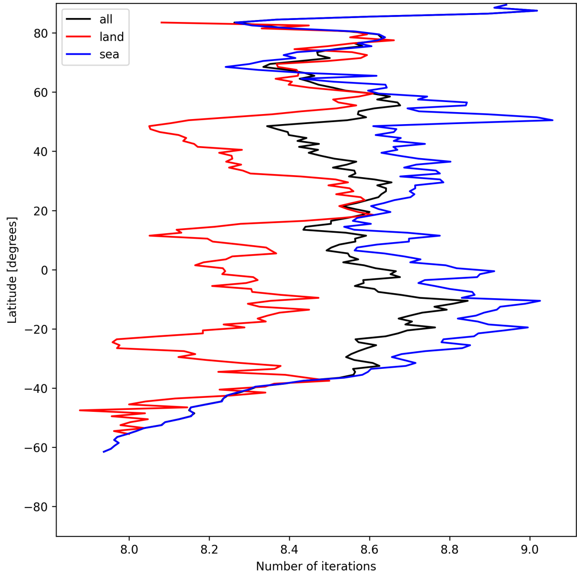
Figure 16: Zonal average of “Number of iterations” for 2025-06-04 to 2025-06-06.
