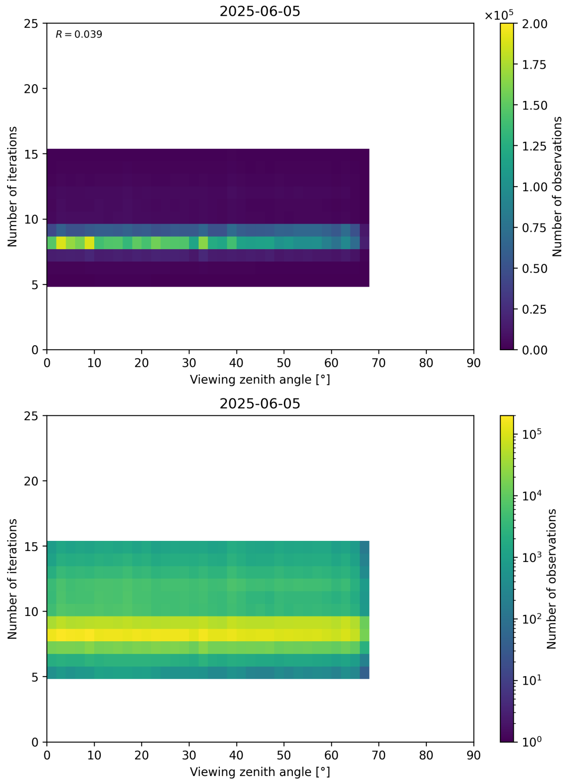
Figure 75: Scatter density plot of “Viewing zenith angle” against “Number of iterations” for 2025-06-04 to 2025-06-06.
