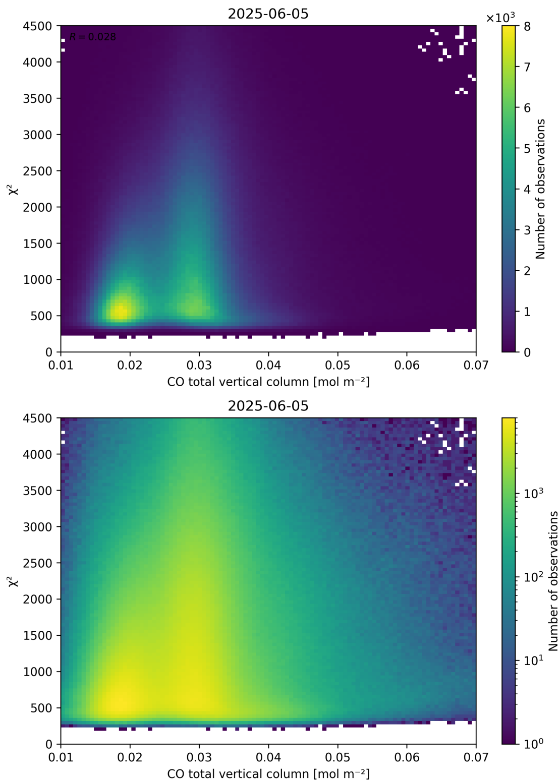
Figure 35: Scatter density plot of “CO total vertical column” against “ \chi^2 ” for 2025-06-04 to 2025-06-06.
