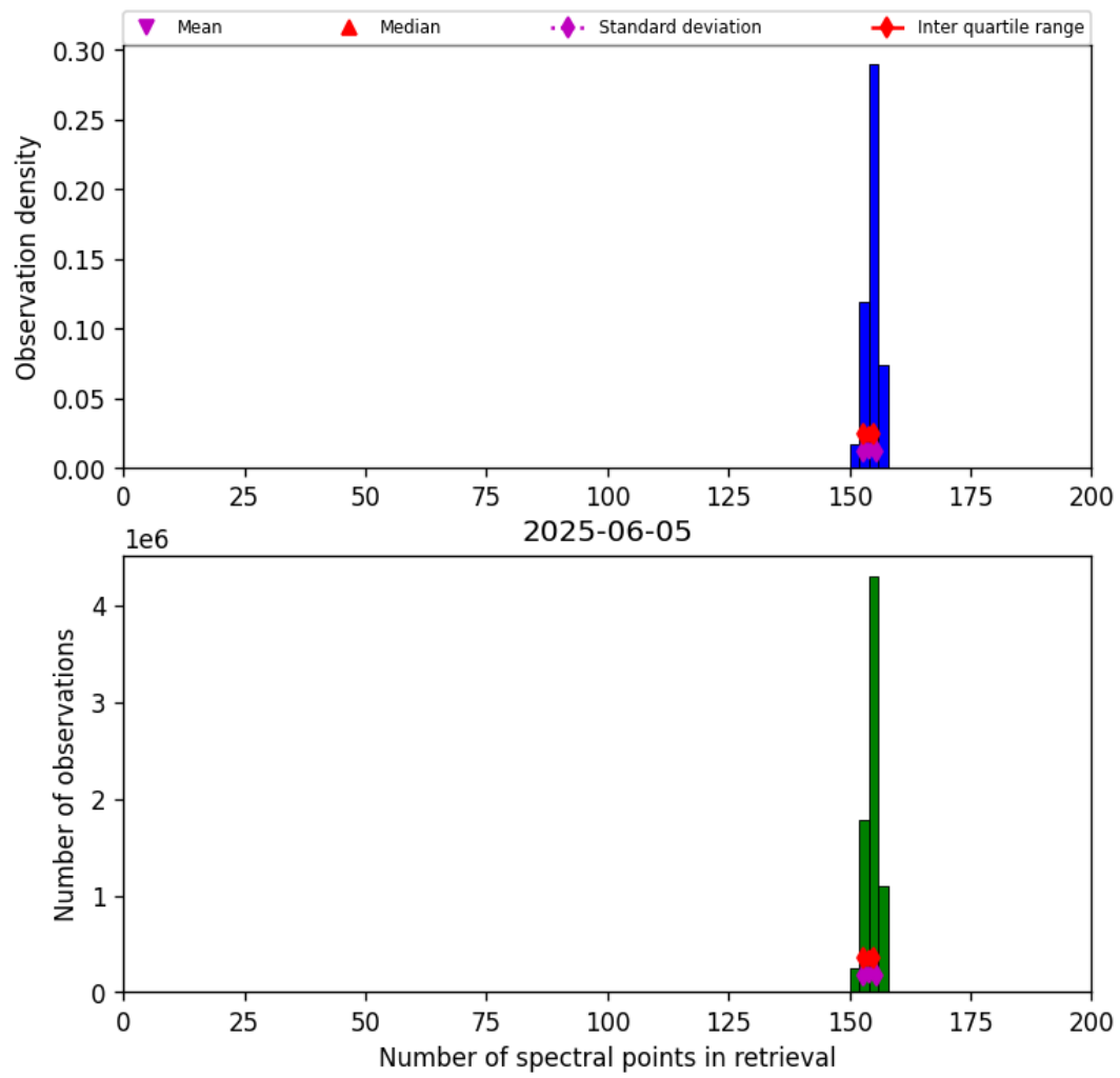
Figure 21: Histogram of “Number of spectral points in retrieval” for 2025-06-04 to 2025-06-06
