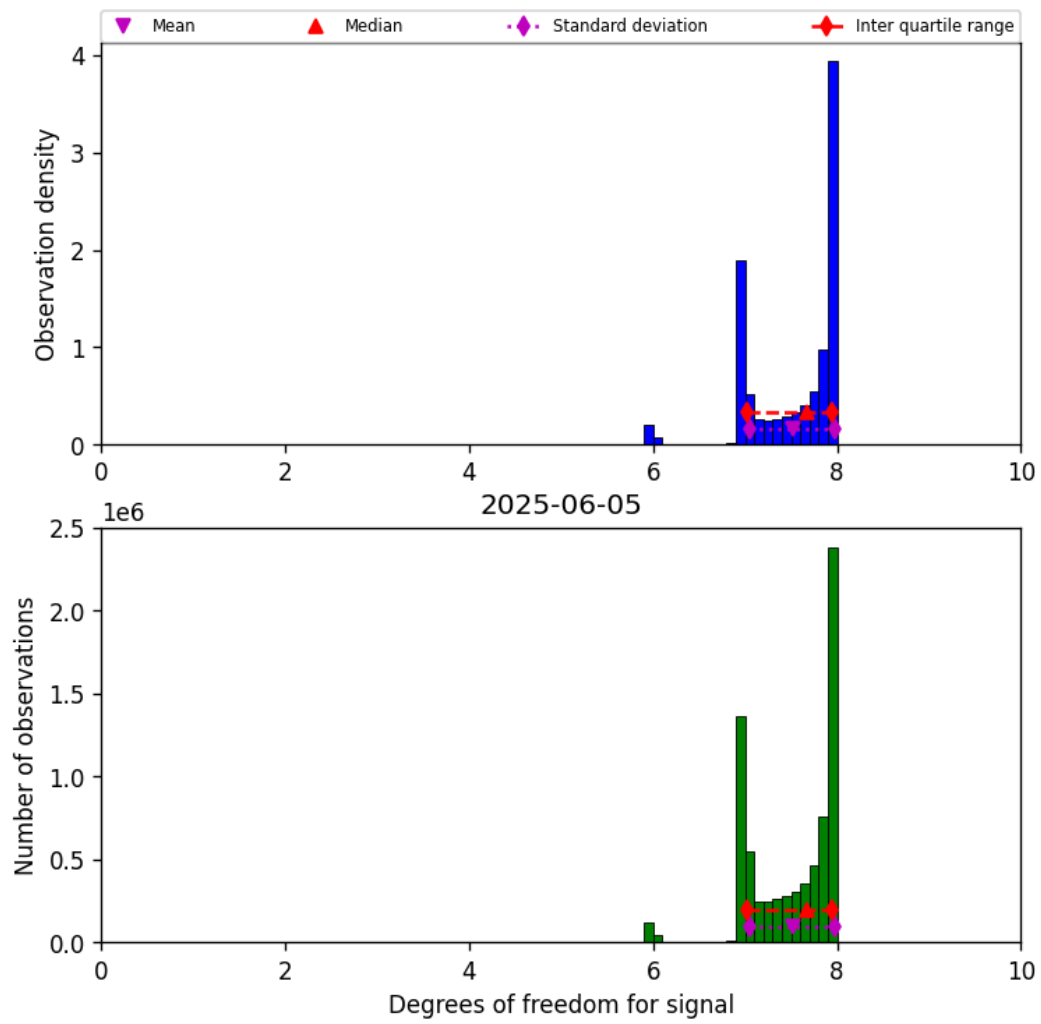
Figure 23: Histogram of “Degrees of freedom for signal” for 2025-06-04 to 2025-06-06
