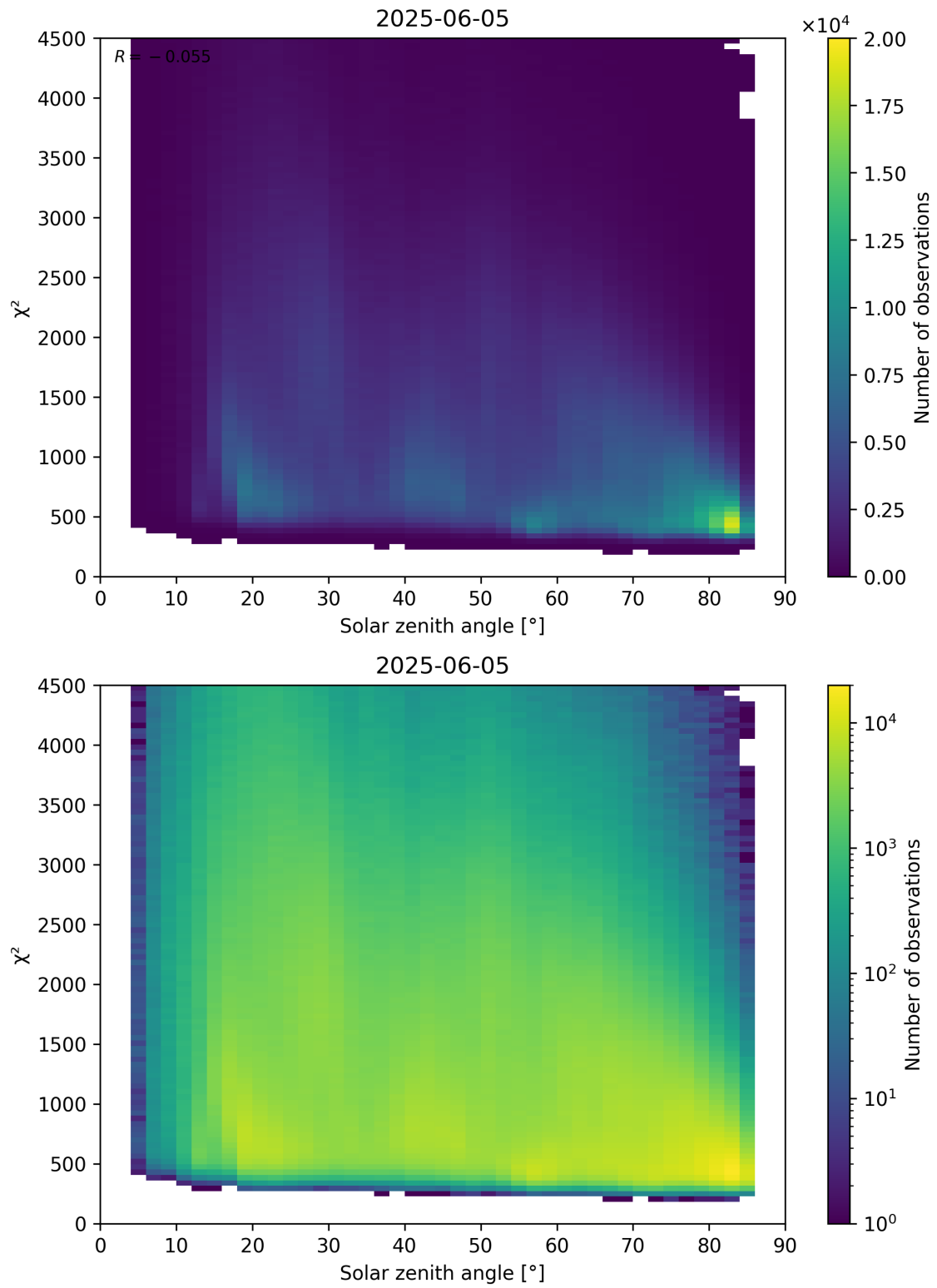
Figure 64: Scatter density plot of “Solar zenith angle” against “ \chi^2 ” for 2025-06-04 to 2025-06-06.
