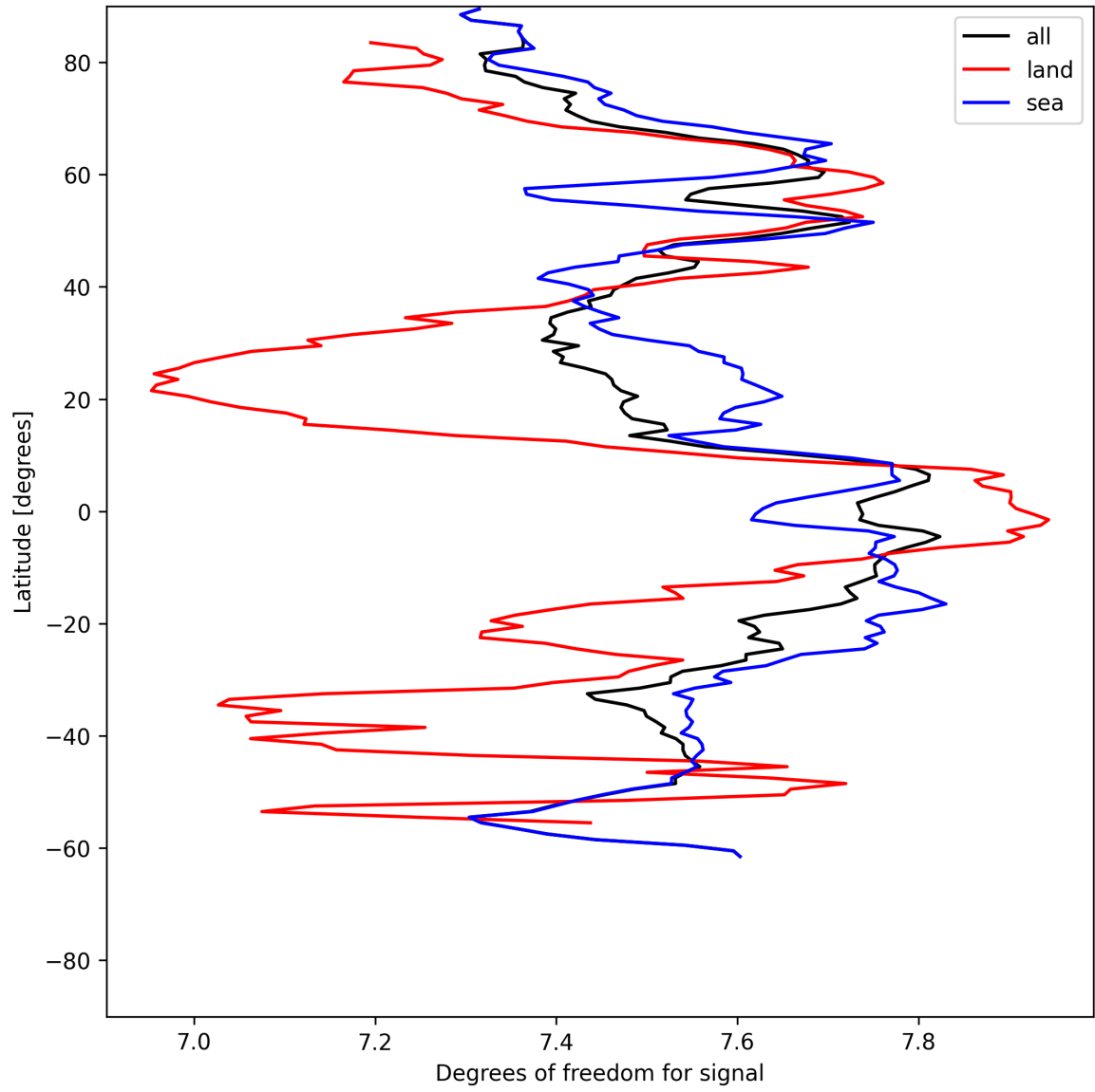
Figure 15: Zonal average of “Degrees of freedom for signal” for 2025-06-04 to 2025-06-06.
