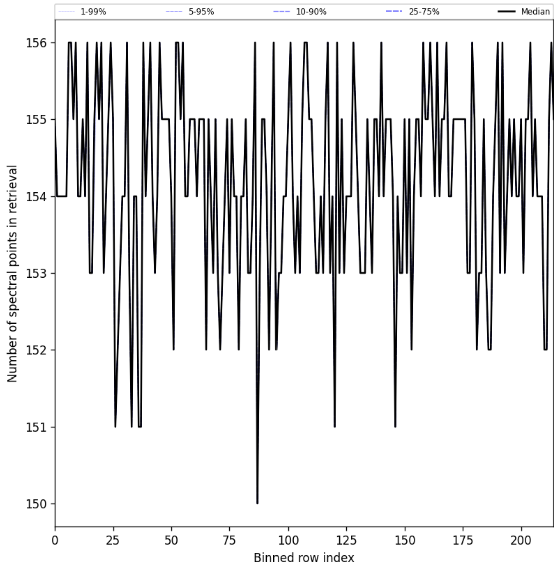
Figure 29: Along track statistics of “Number of spectral points in retrieval” for 2025-06-04 to 2025-06-06
