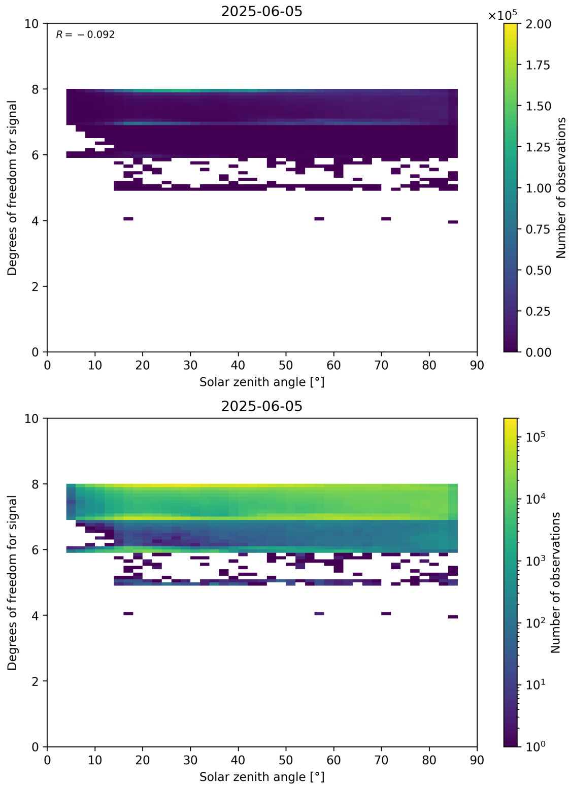
Figure 65: Scatter density plot of “Solar zenith angle” against “Degrees of freedom for signal” for 2025-06-04 to 2025-06-06.
