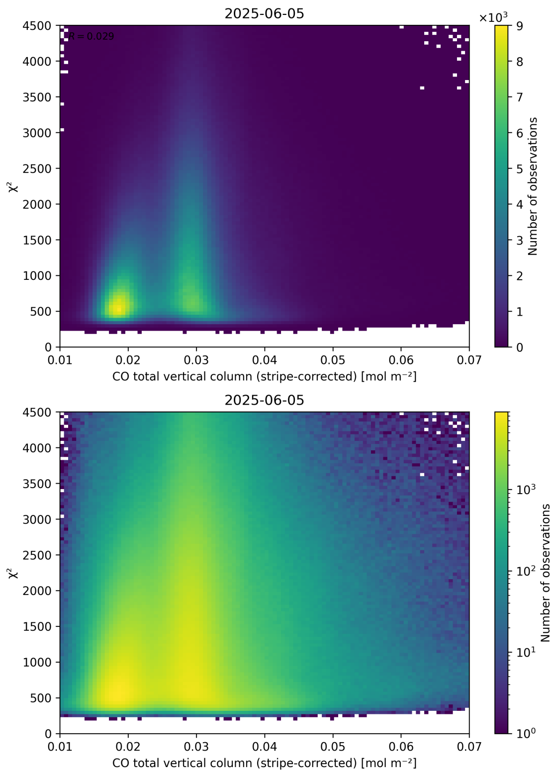
Figure 37: Scatter density plot of “CO total vertical column (stripe-corrected)” against “ \chi^2 ” for 2025-06-04 to 2025-06-06.
