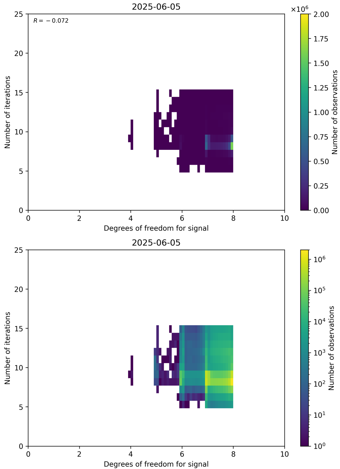
Figure 50: Scatter density plot of “Degrees of freedom for signal” against “Number of iterations” for 2025-06-04 to 2025-06-06.
