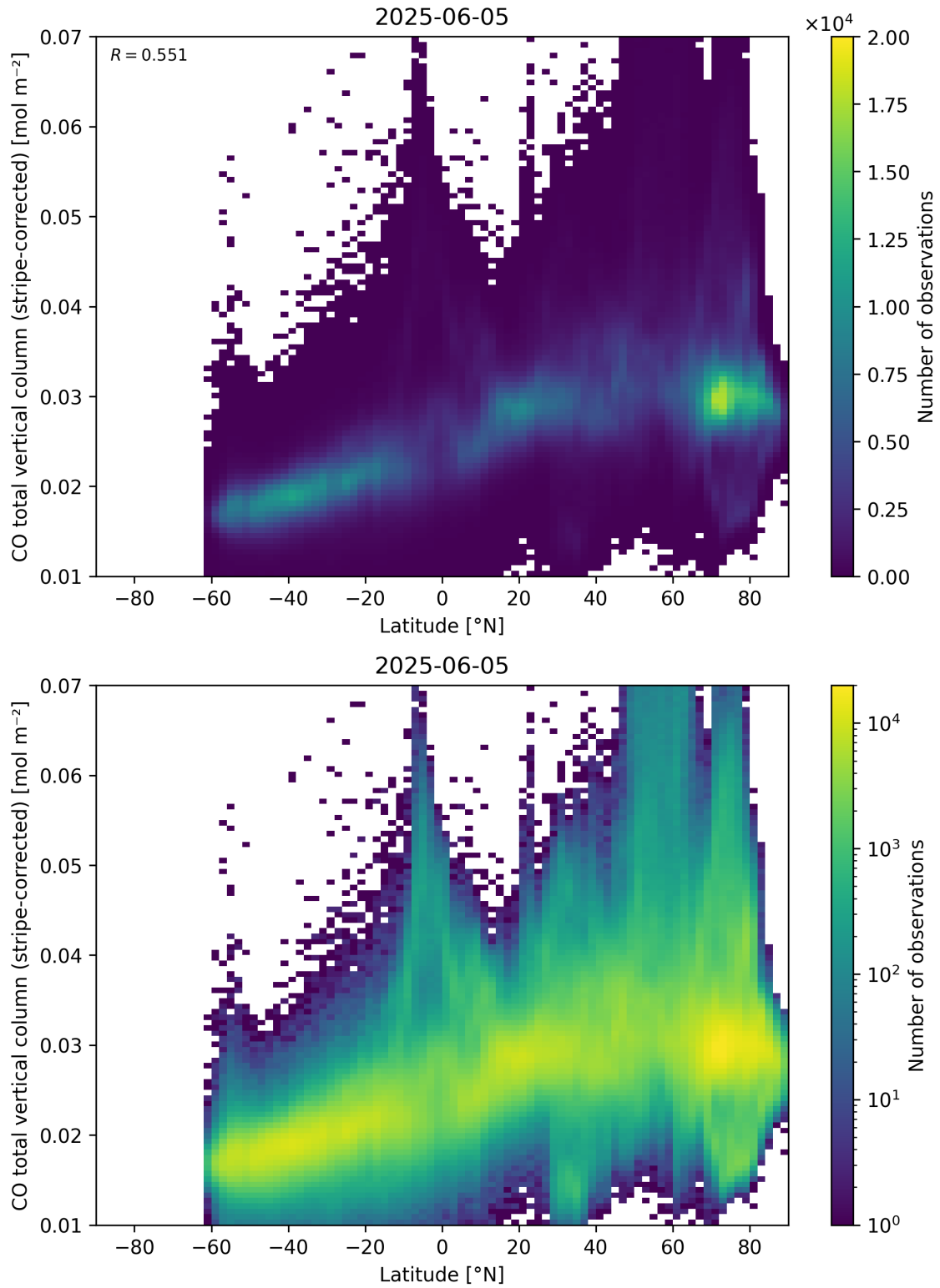
Figure 52: Scatter density plot of “Latitude” against “CO total vertical column (stripe-corrected)” for 2025-06-04 to 2025-06-06.
