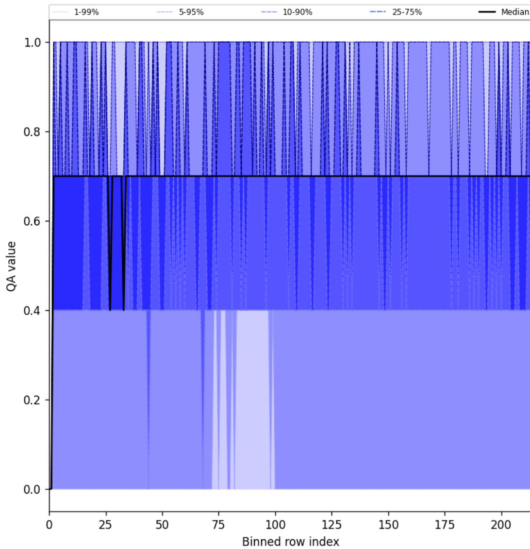
Figure 25: Along track statistics of “QA value” for 2025-06-04 to 2025-06-06
