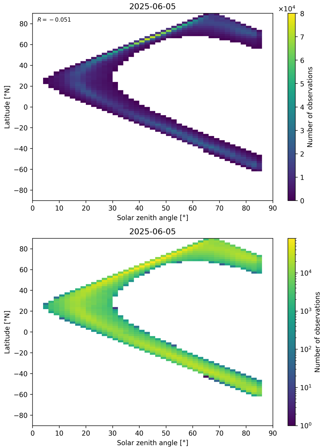
Figure 66: Scatter density plot of “Solar zenith angle” against “Latitude” for 2025-06-04 to 2025-06-06.
