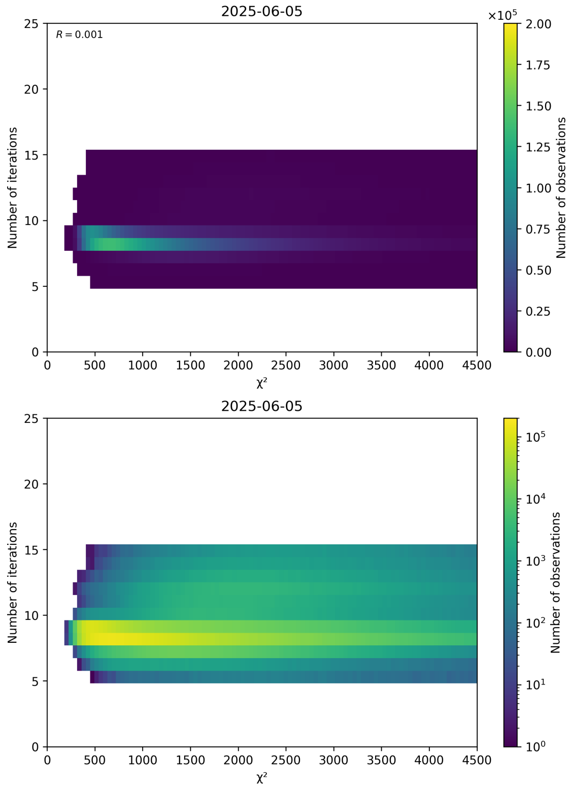
Figure 49: Scatter density plot of “ \chi^2 ” against “Number of iterations” for 2025-06-04 to 2025-06-06.
