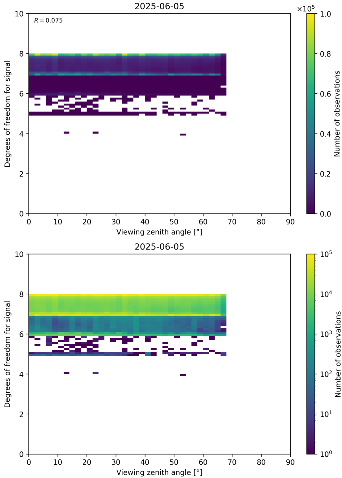
Figure 73: Scatter density plot of “Viewing zenith angle” against “Degrees of freedom for signal” for 2025-06-04 to 2025-06-06.
