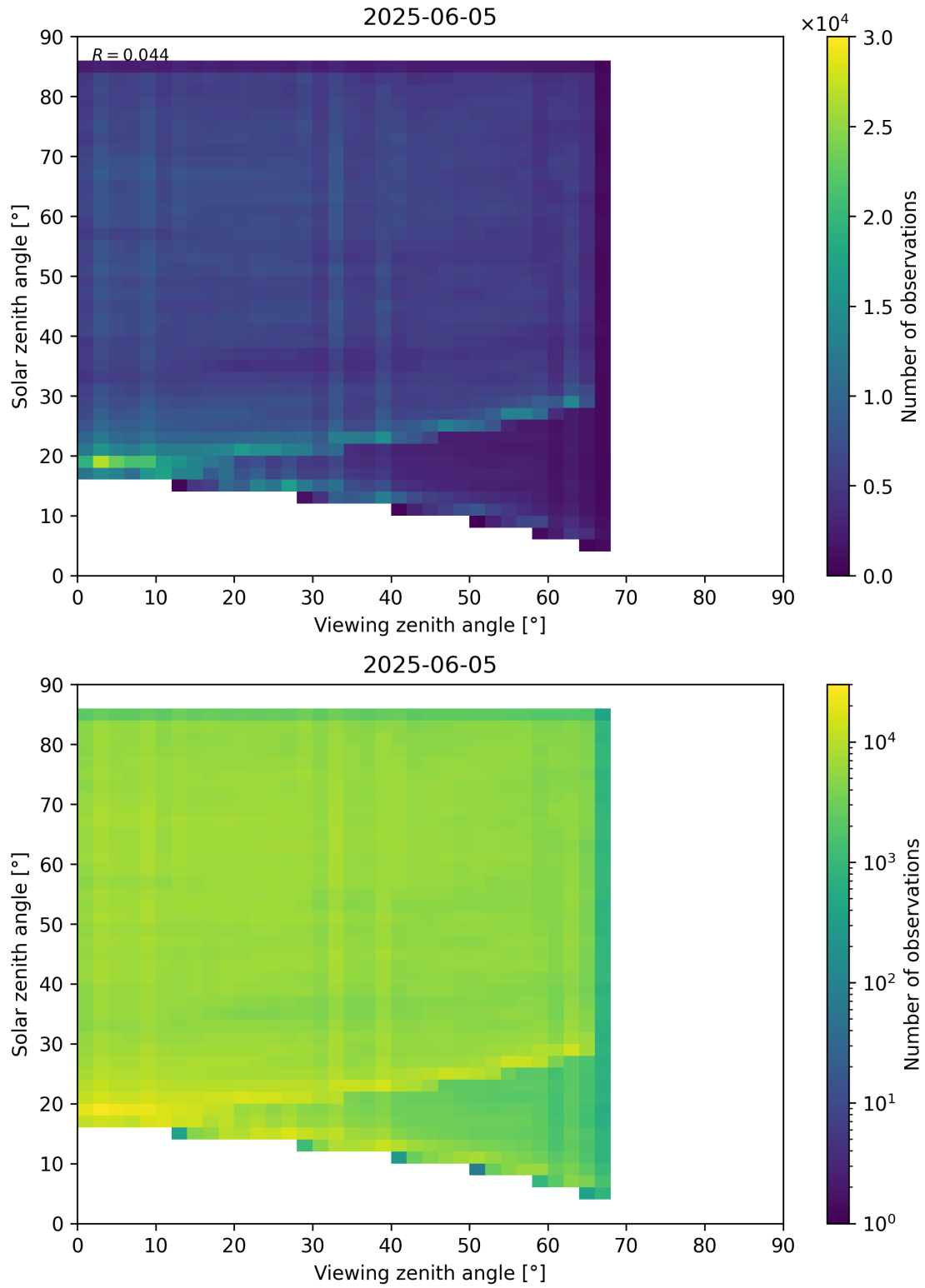
Figure 77: Scatter density plot of “Viewing zenith angle” against “Solar zenith angle” for 2025-06-04 to 2025-06-06.
