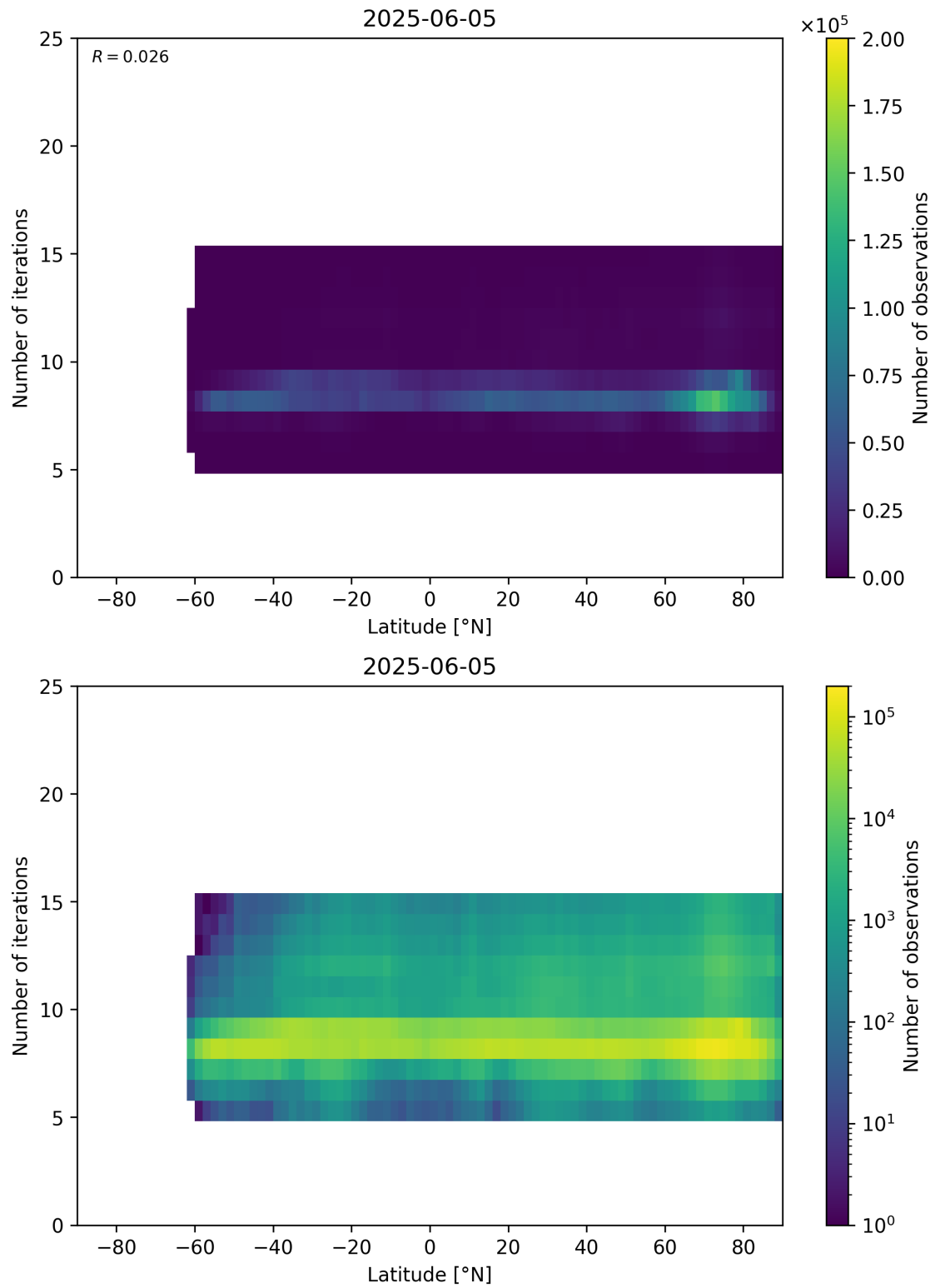
Figure 56: Scatter density plot of “Latitude” against “Number of iterations” for 2025-06-04 to 2025-06-06.
