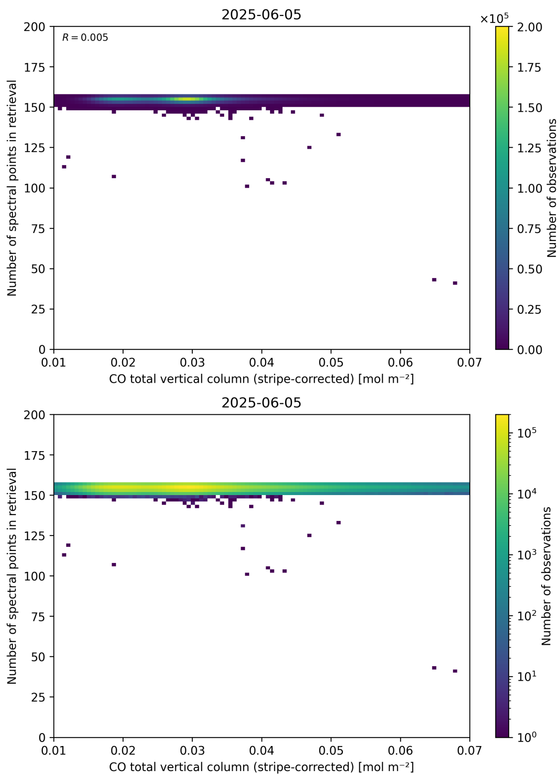
Figure 40: Scatter density plot of “CO total vertical column (stripe-corrected)” against “Number of spectral points in retrieval” for 2025-06-04 to 2025-06-06.
