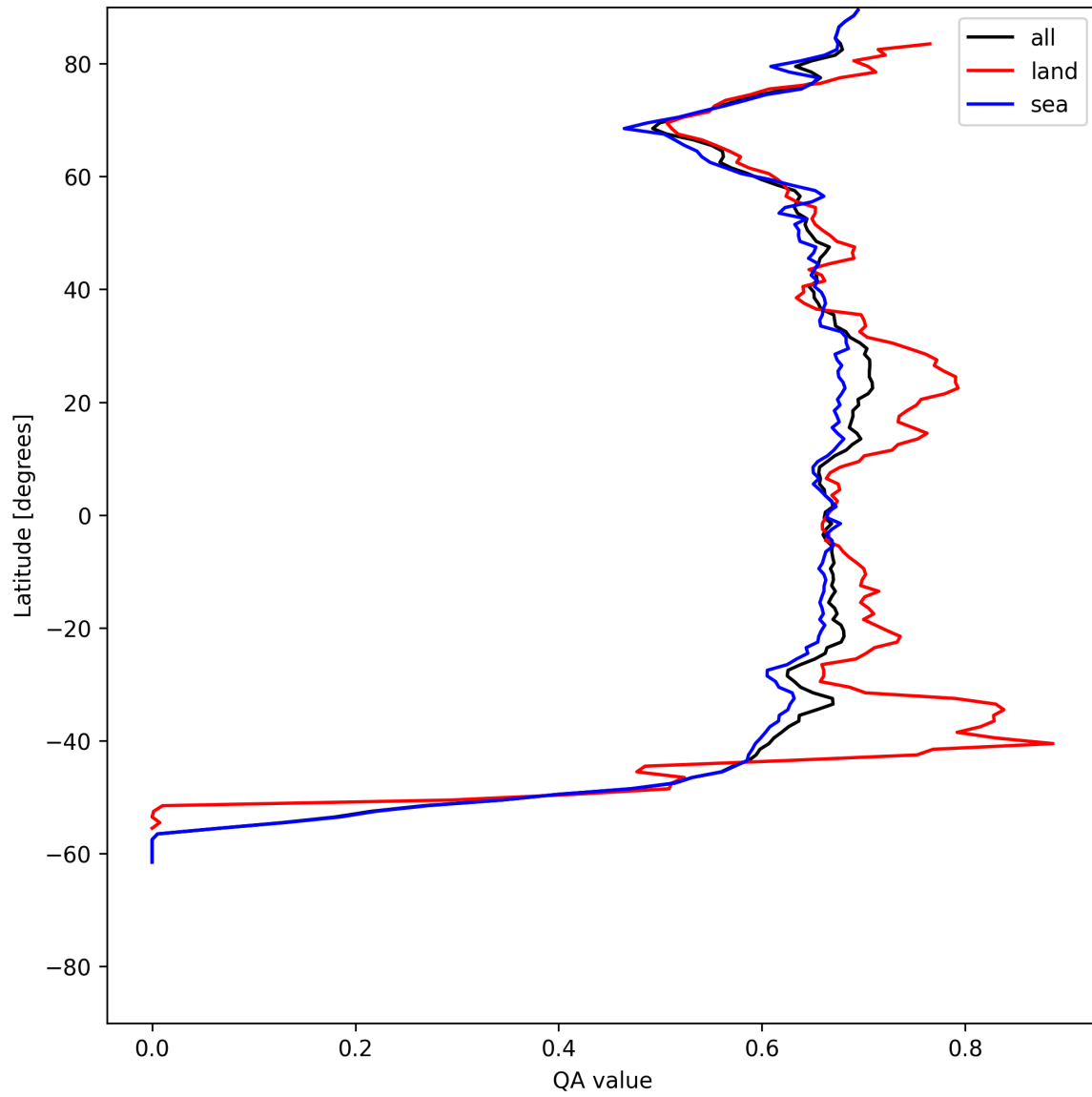
Figure 9: Zonal average of “QA value” for 2025-06-04 to 2025-06-06.
