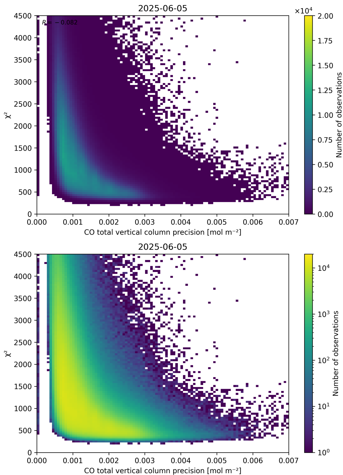
Figure 44: Scatter density plot of “CO total vertical column precision” against “ \chi^2 ” for 2025-06-04 to 2025-06-06.
