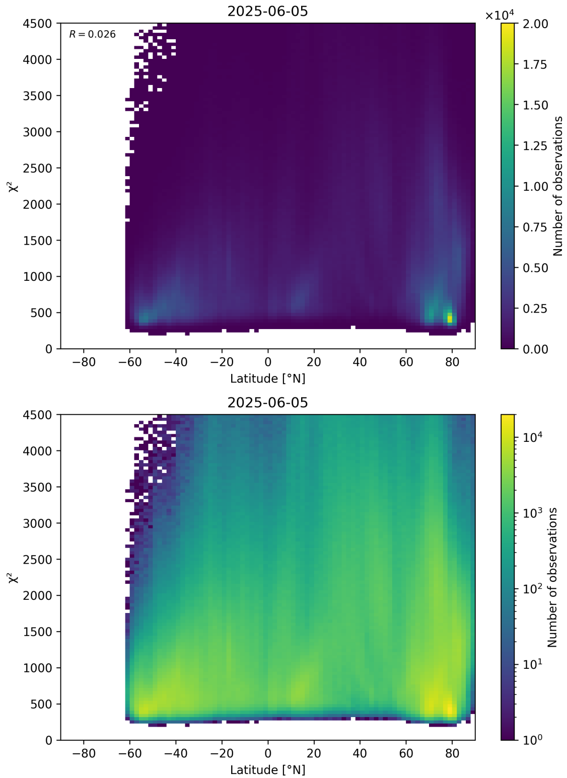
Figure 54: Scatter density plot of “Latitude” against “ \chi^2 ” for 2025-06-04 to 2025-06-06.
