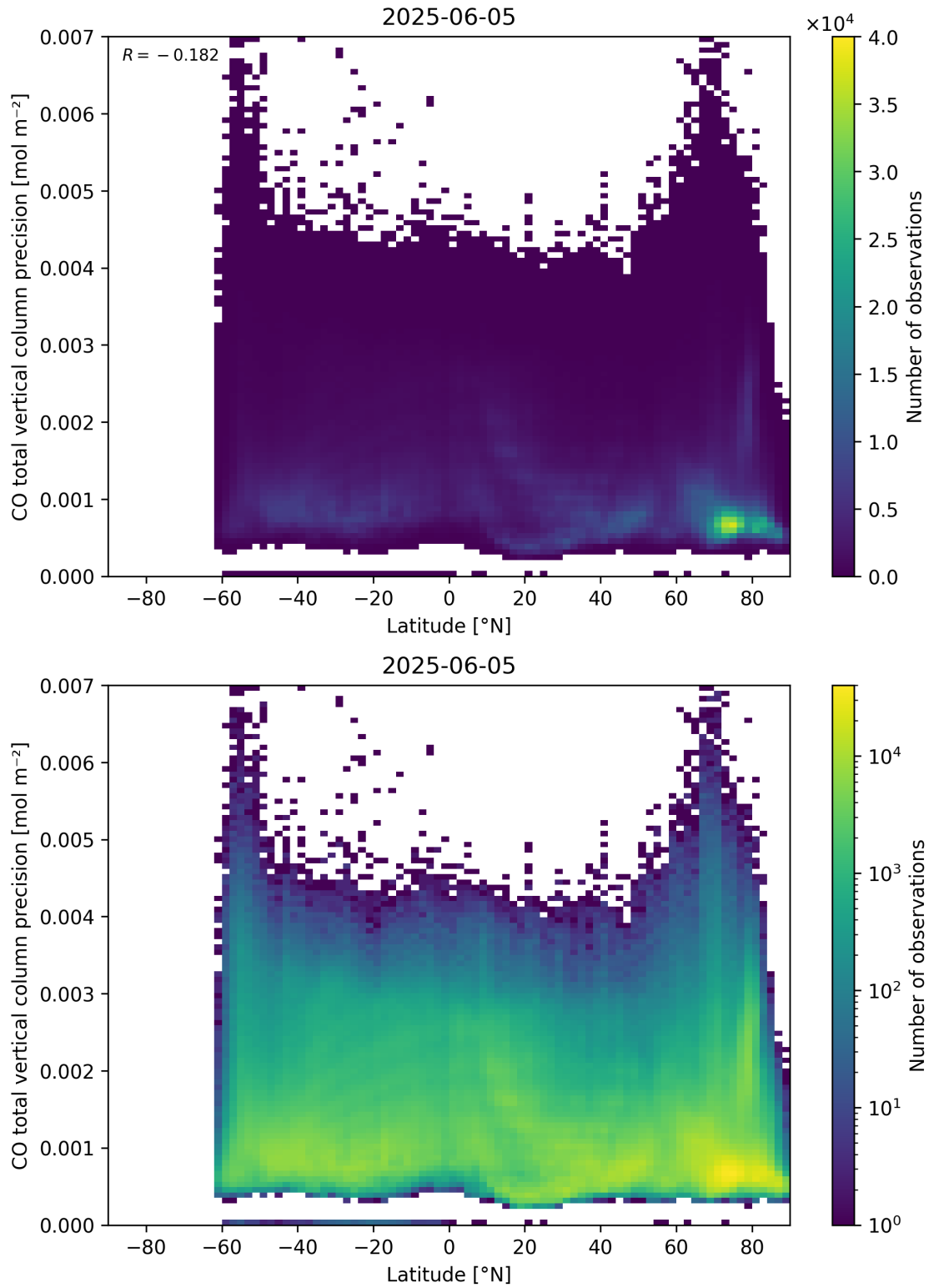
Figure 53: Scatter density plot of “Latitude” against “CO total vertical column precision” for 2025-06-04 to 2025-06-06.
