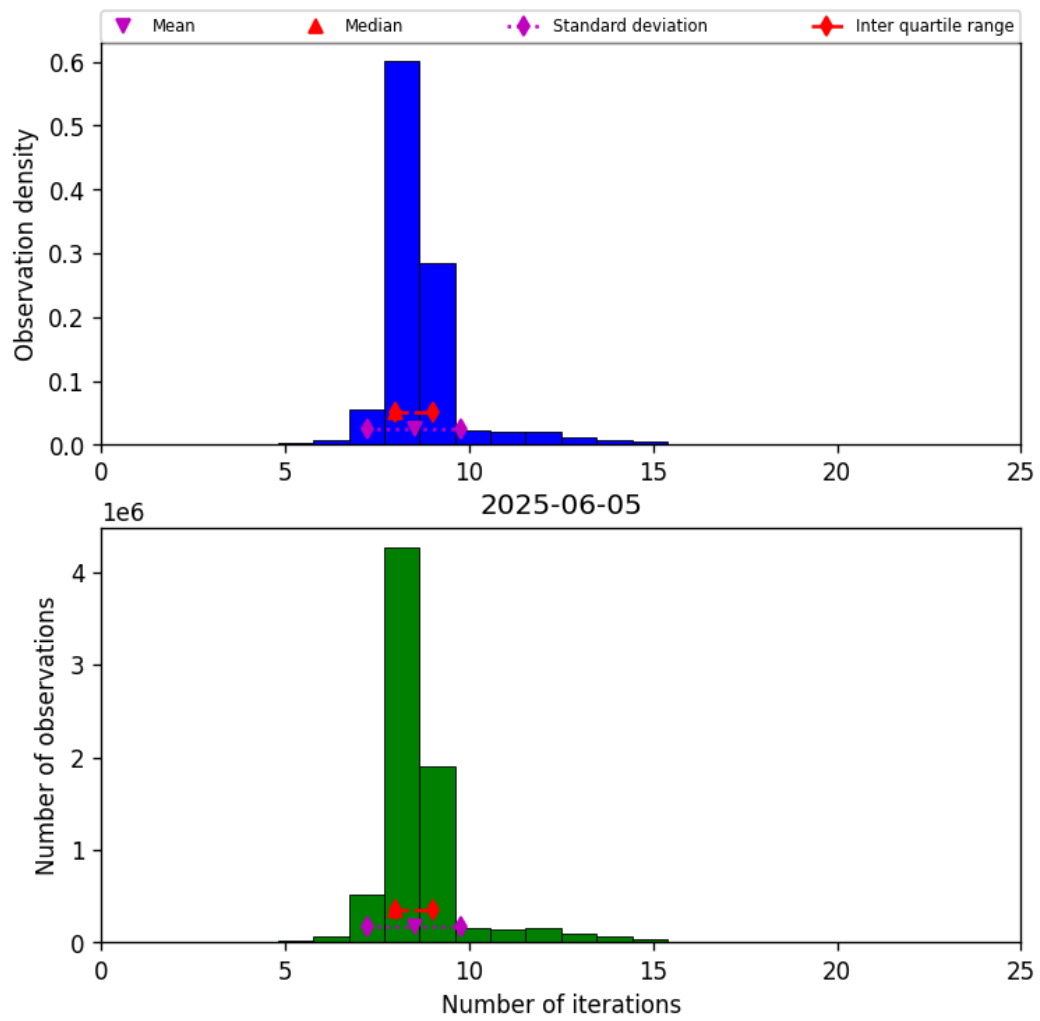
Figure 24: Histogram of “Number of iterations” for 2025-06-04 to 2025-06-06
