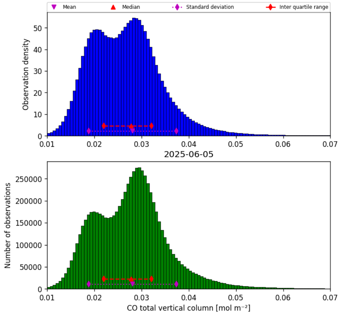
Figure 18: Histogram of “CO total vertical column” for 2025-06-04 to 2025-06-06
