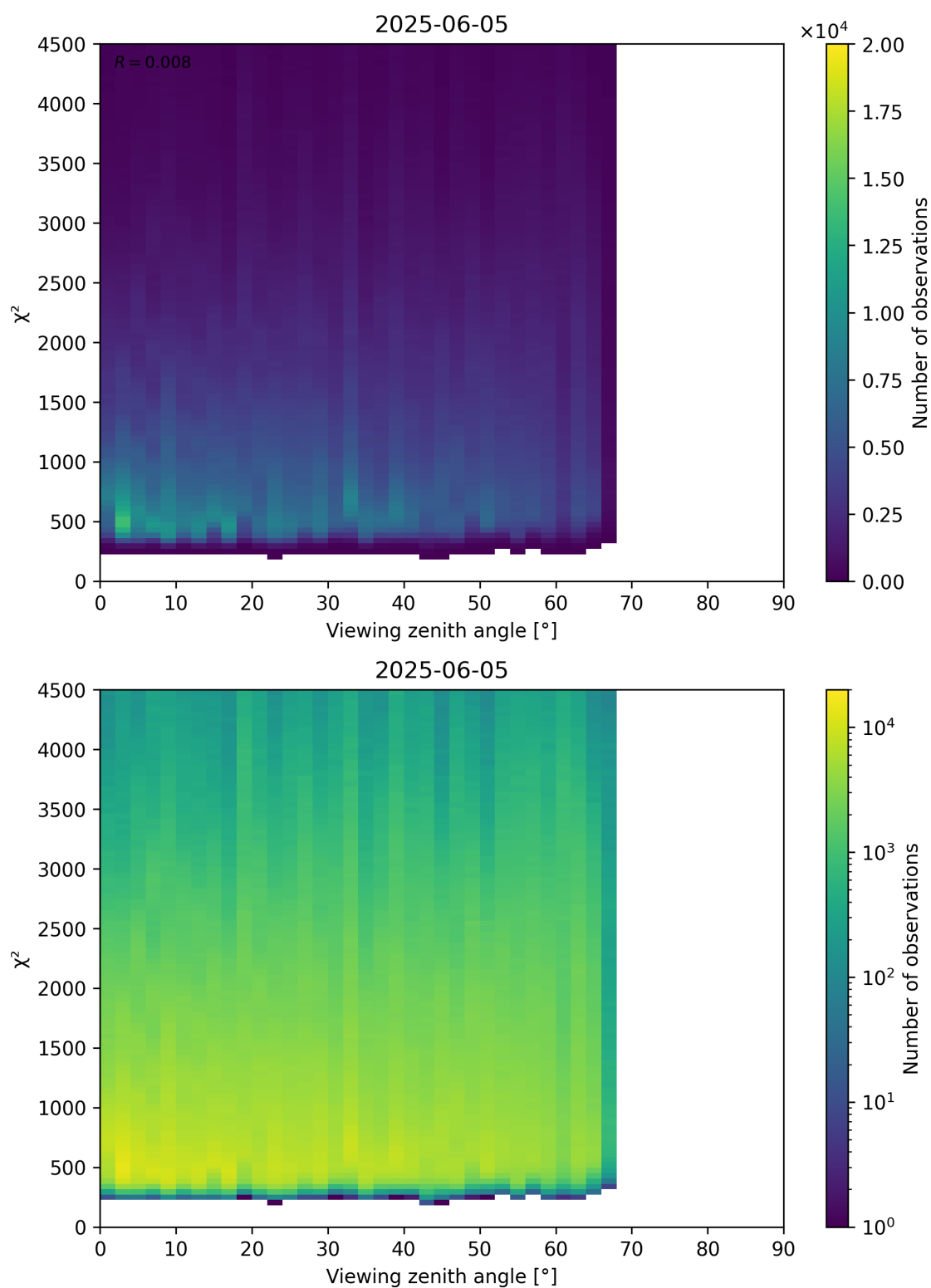
Figure 72: Scatter density plot of “Viewing zenith angle” against “ \chi^2 ” for 2025-06-04 to 2025-06-06.
