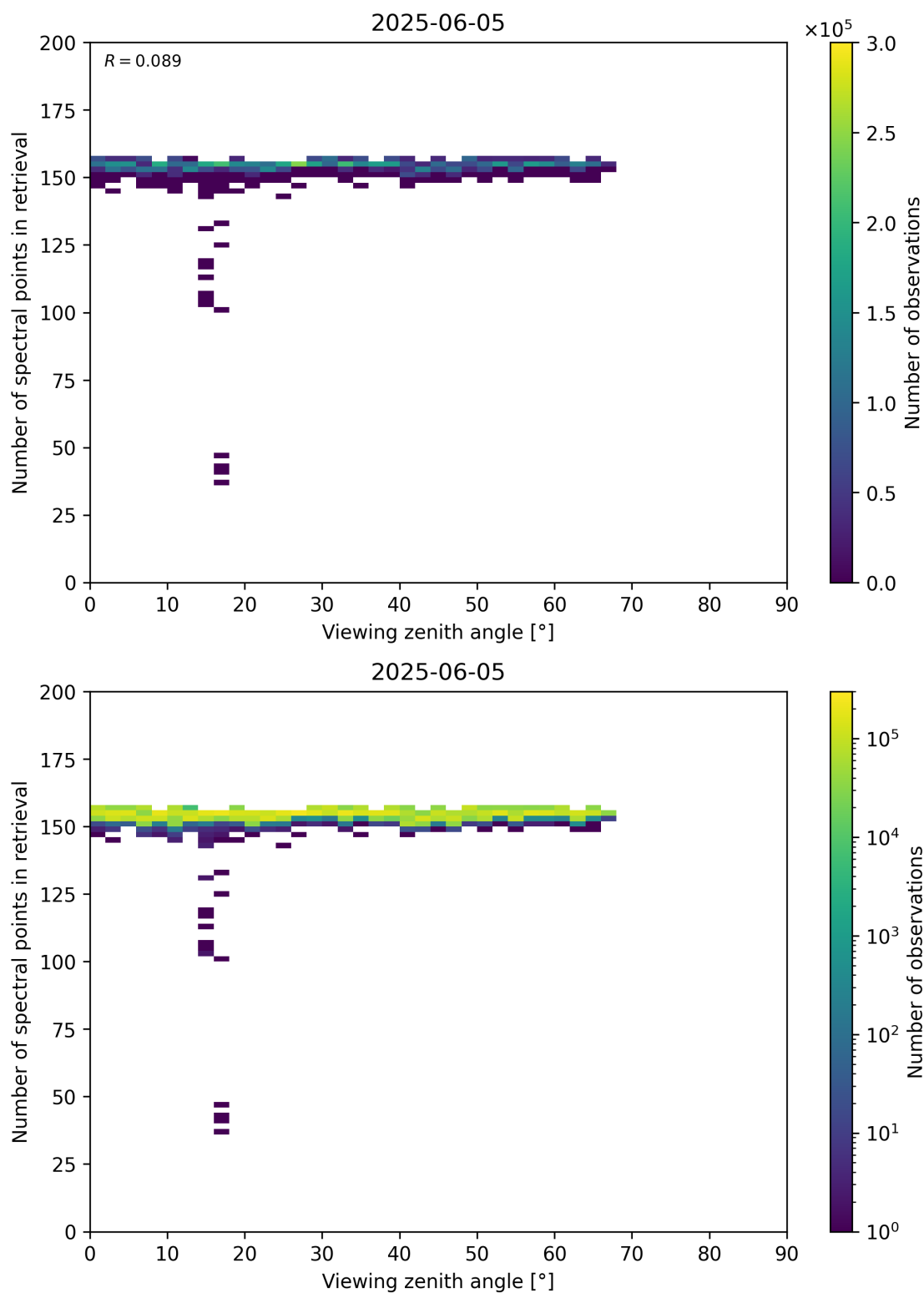
Figure 76: Scatter density plot of “Viewing zenith angle” against “Number of spectral points in retrieval” for 2025-06-04 to 2025-06-06.
