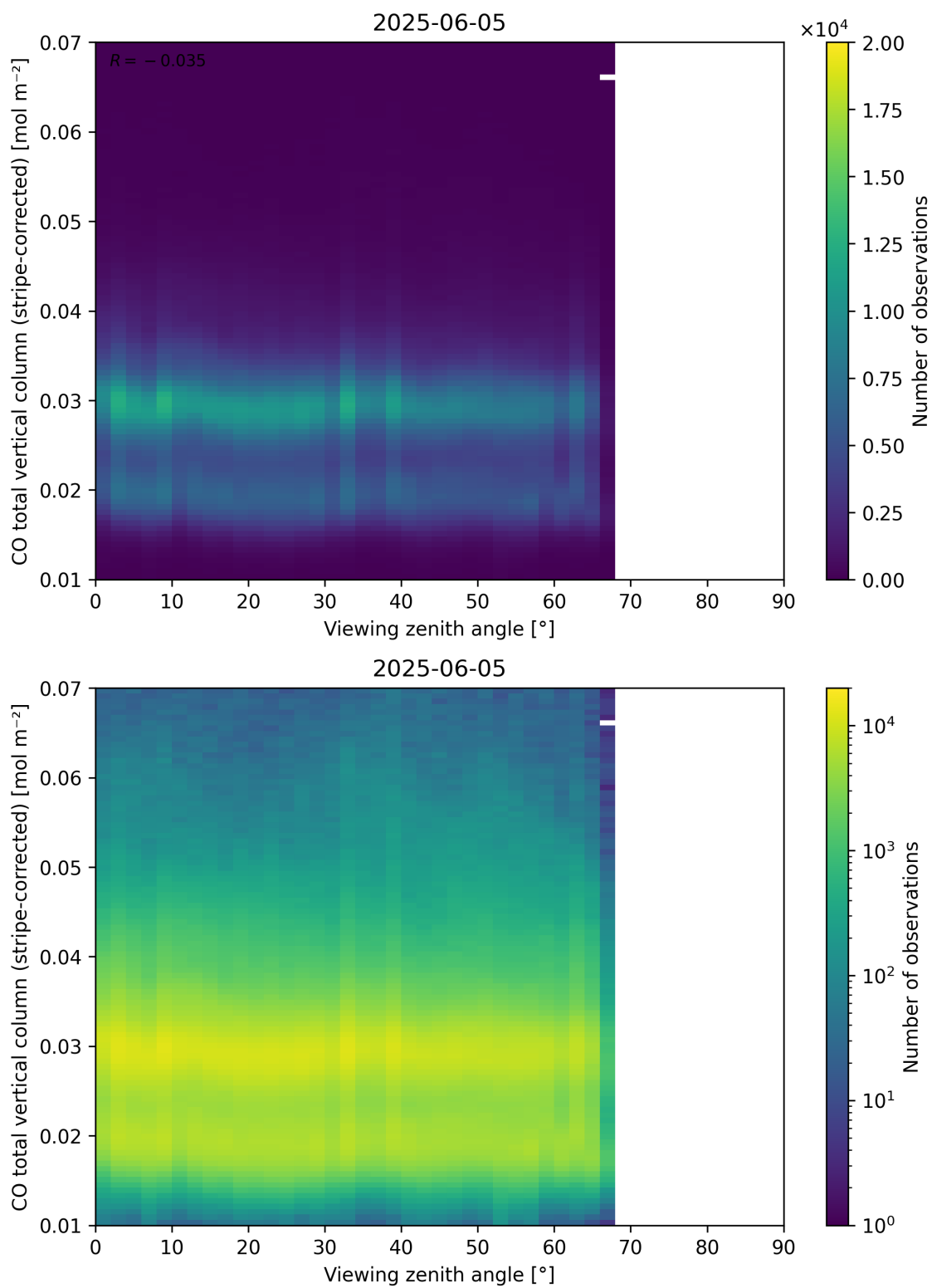
Figure 70: Scatter density plot of “Viewing zenith angle” against “CO total vertical column (stripe-corrected)” for 2025-06-04 to 2025-06-06.
