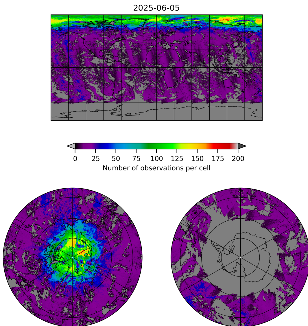
Figure 8: Map of the number of observations for 2025-06-04 to 2025-06-06
