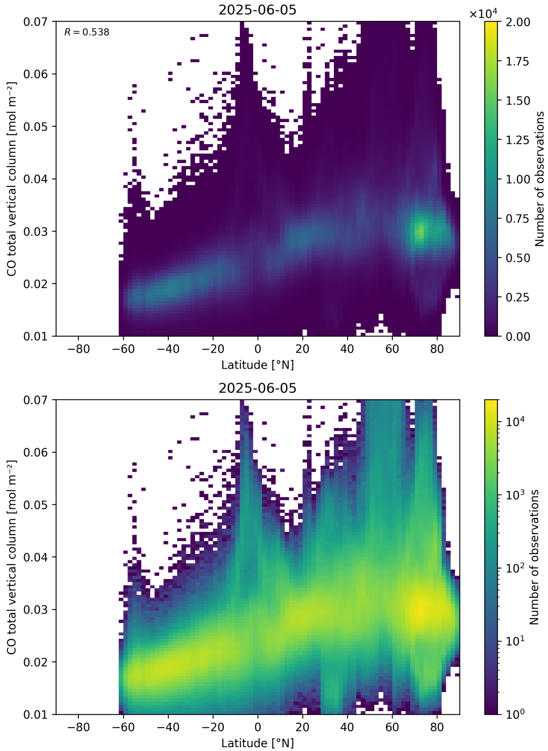
Figure 51: Scatter density plot of “Latitude” against “CO total vertical column” for 2025-06-04 to 2025-06-06.
