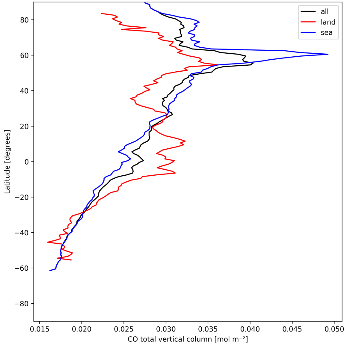
Figure 10: Zonal average of “CO total vertical column” for 2025-06-04 to 2025-06-06.
