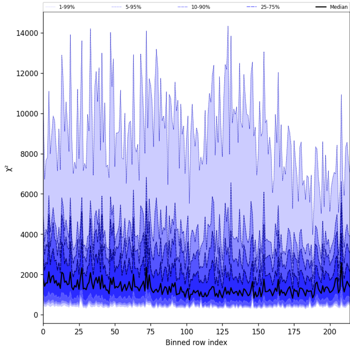
Figure 30: Along track statistics of “ \chi^2 ” for 2025-06-04 to 2025-06-06
