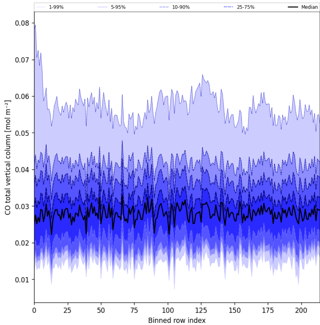
Figure 26: Along track statistics of “CO total vertical column” for 2025-06-04 to 2025-06-06
