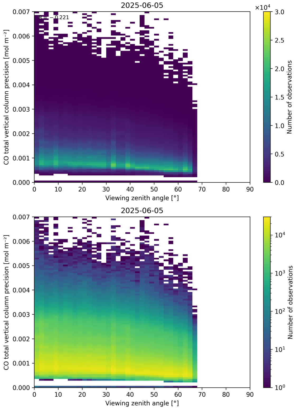
Figure 71: Scatter density plot of “Viewing zenith angle” against “CO total vertical column precision” for 2025-06-04 to 2025-06-06.
