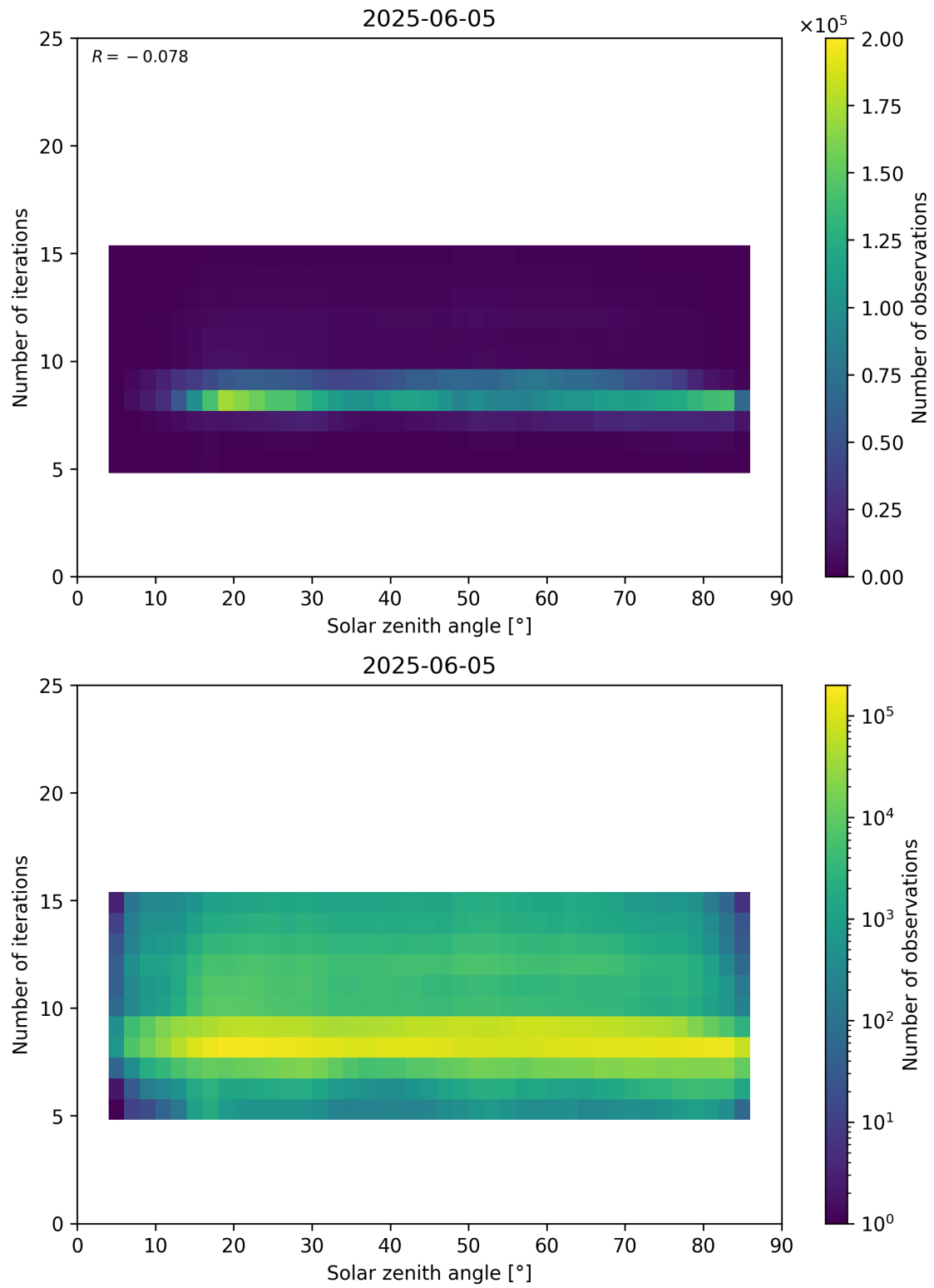
Figure 67: Scatter density plot of “Solar zenith angle” against “Number of iterations” for 2025-06-04 to 2025-06-06.
