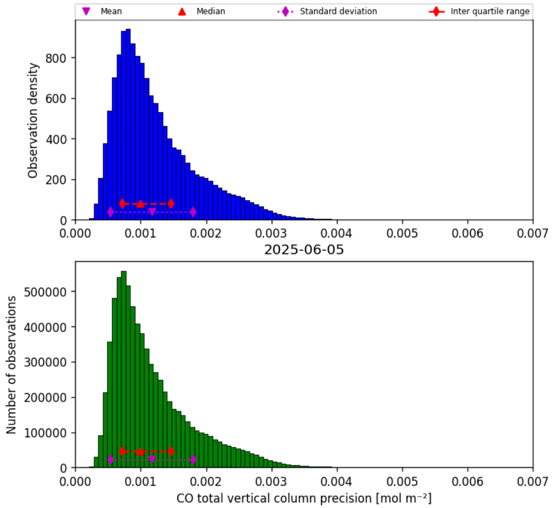
Figure 20: Histogram of “CO total vertical column precision” for 2025-06-04 to 2025-06-06
