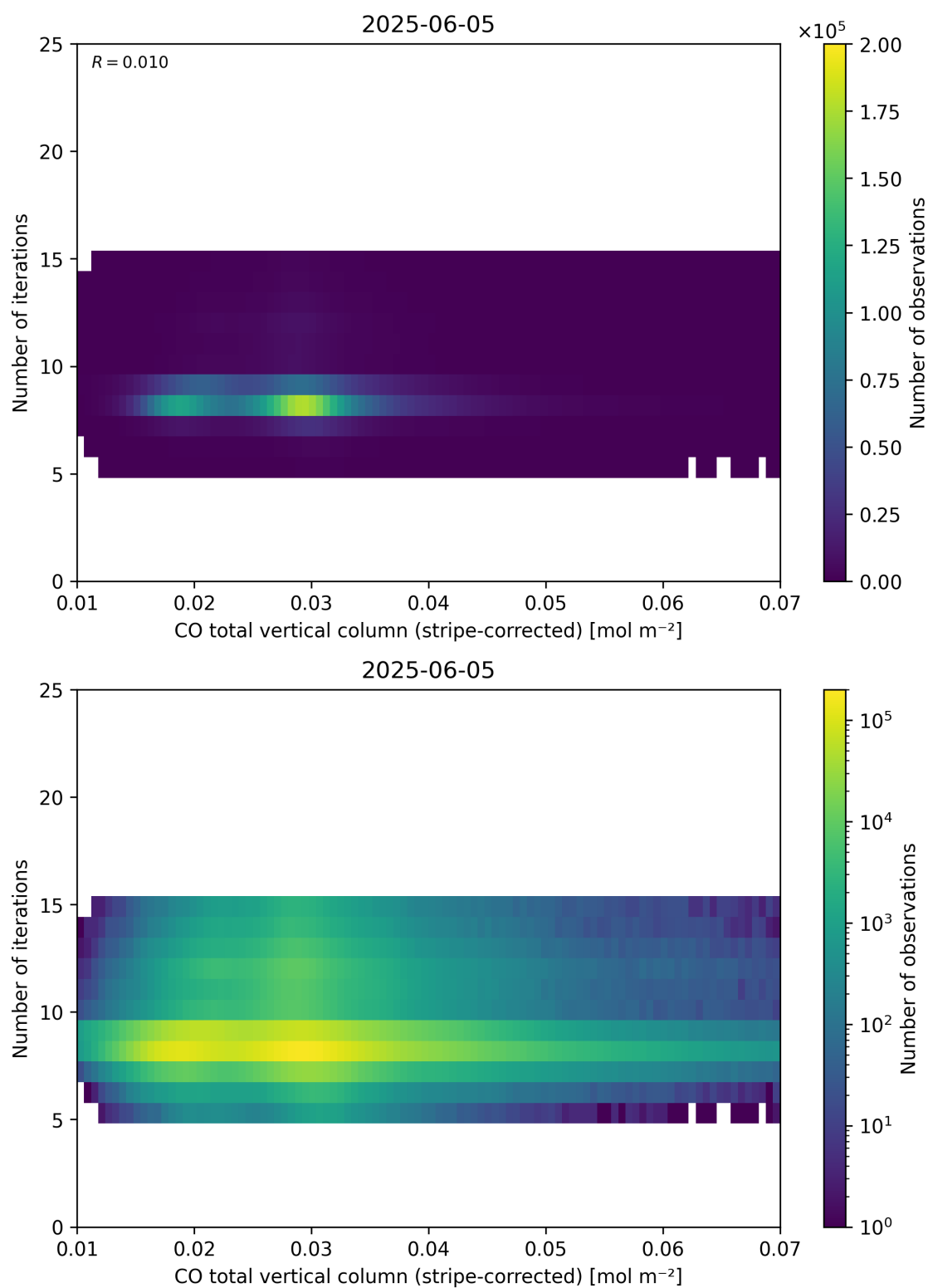
Figure 39: Scatter density plot of “CO total vertical column (stripe-corrected)” against “Number of iterations” for 2025-06-04 to 2025-06-06.
