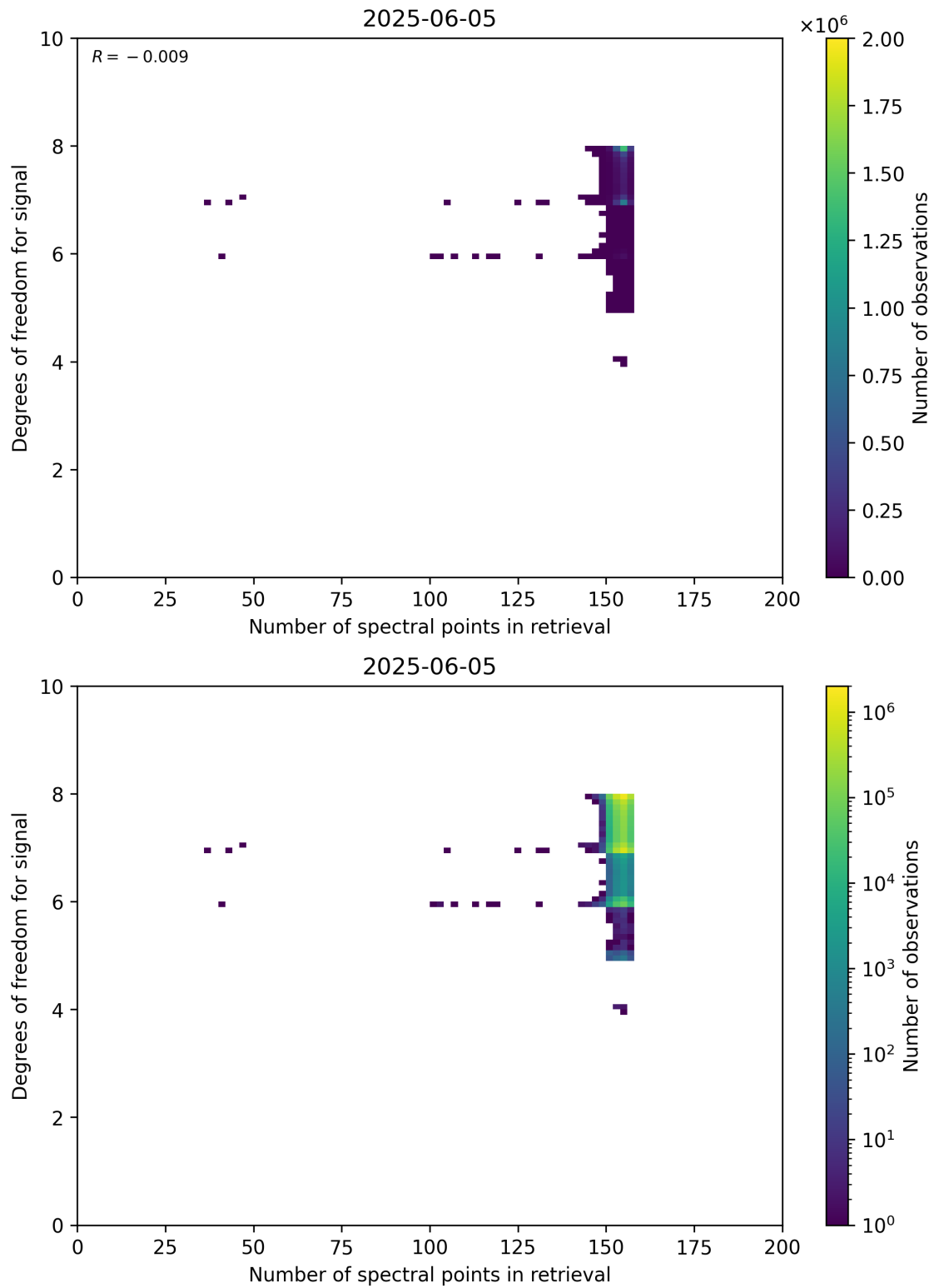
Figure 59: Scatter density plot of “Number of spectral points in retrieval” against “Degrees of freedom for signal” for 2025-06-04 to 2025-06-06.
