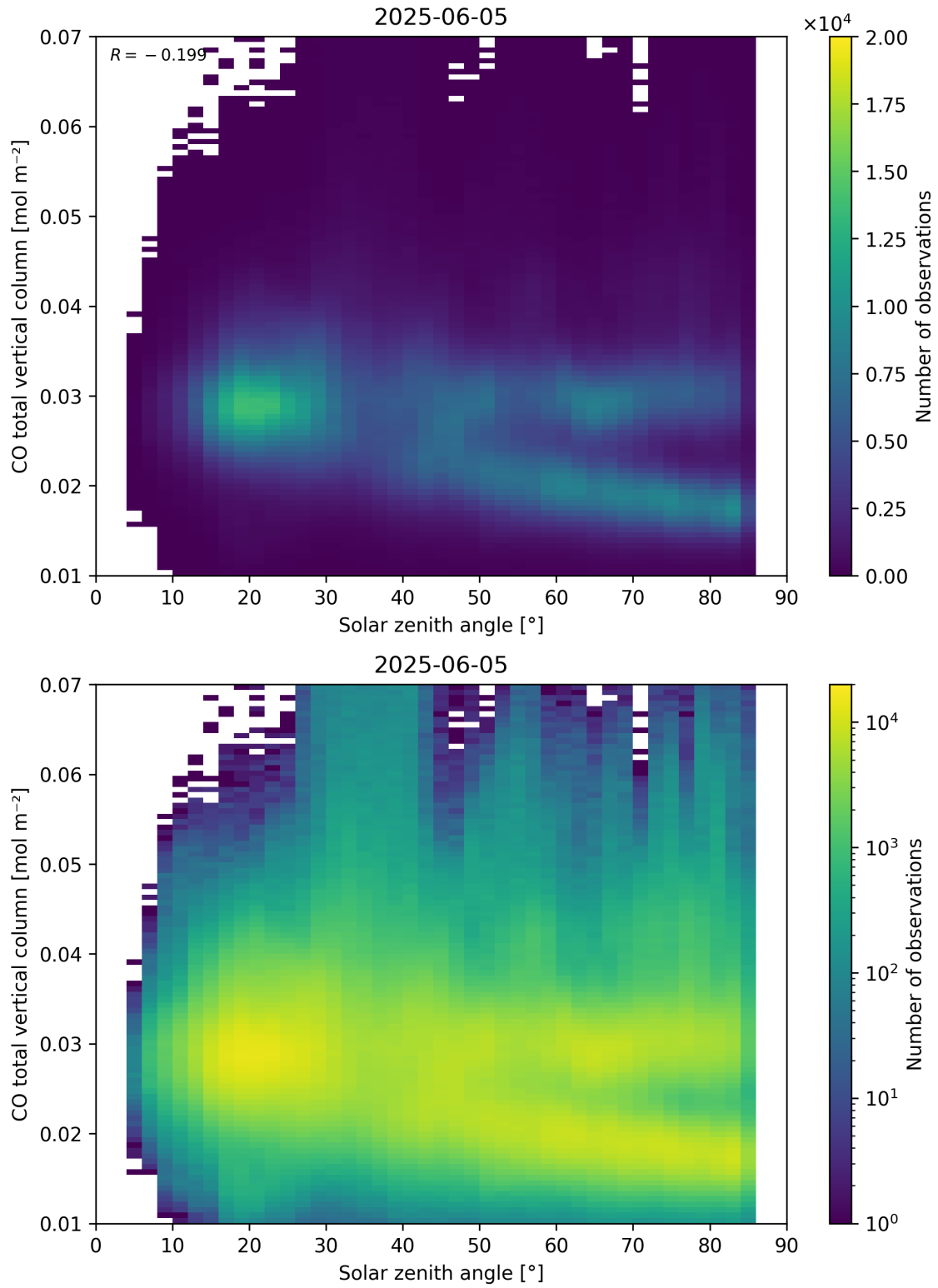
Figure 61: Scatter density plot of “Solar zenith angle” against “CO total vertical column” for 2025-06-04 to 2025-06-06.
