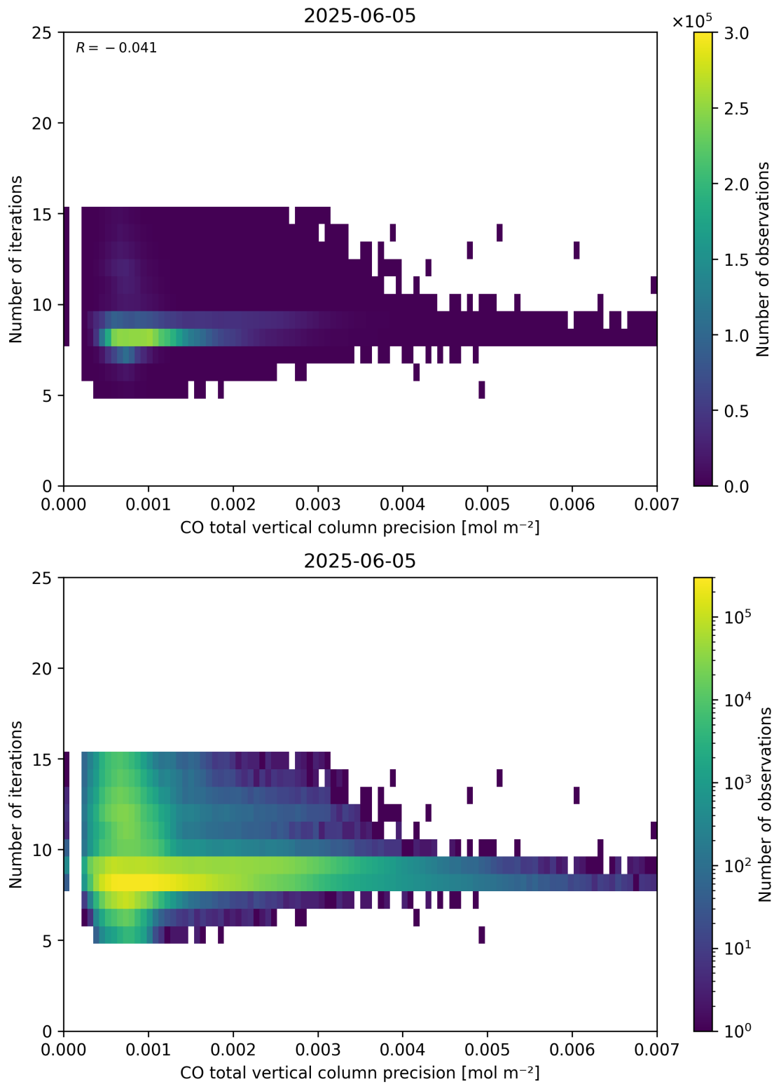
Figure 46: Scatter density plot of “CO total vertical column precision” against “Number of iterations” for 2025-06-04 to 2025-06-06.
