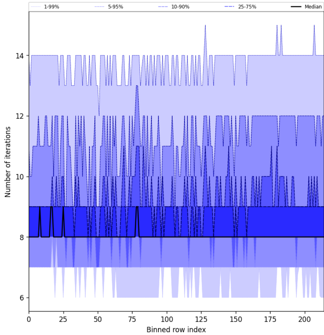
Figure 32: Along track statistics of “Number of iterations” for 2025-06-04 to 2025-06-06
