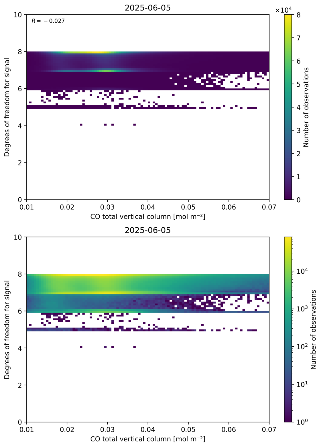
Figure 41: Scatter density plot of “CO total vertical column” against “Degrees of freedom for signal” for 2025-06-04 to 2025-06-06.
