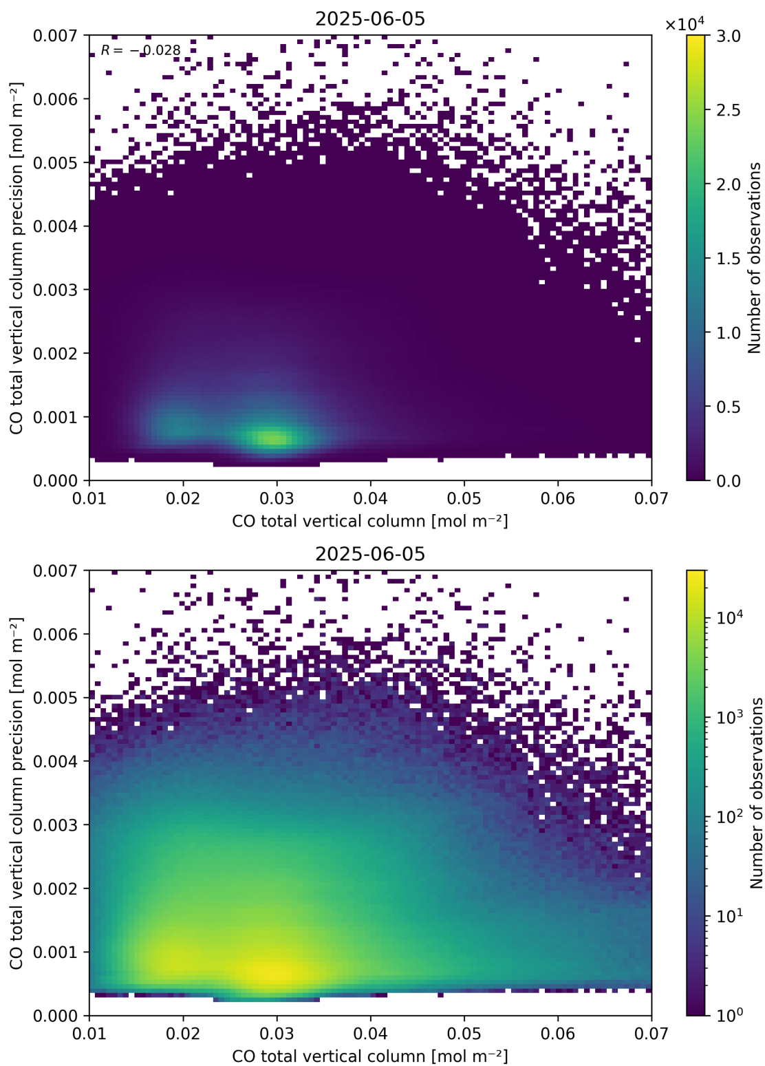
Figure 34: Scatter density plot of “CO total vertical column” against “CO total vertical column precision” for 2025-06-04 to 2025-06-06.
