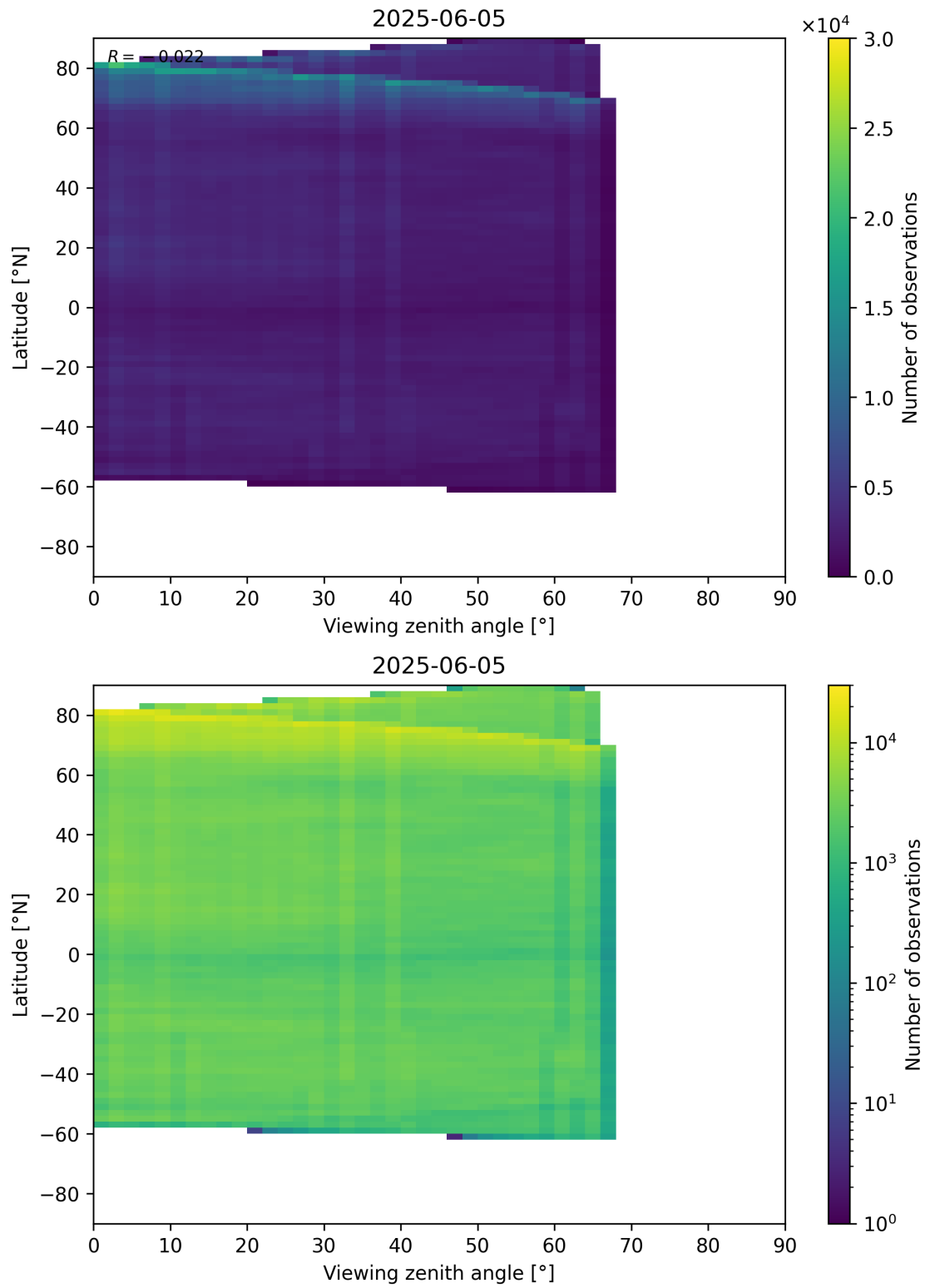
Figure 74: Scatter density plot of “Viewing zenith angle” against “Latitude” for 2025-06-04 to 2025-06-06.
