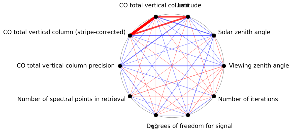
Figure 1: Map of correlation graph for 2025-06-04 to 2025-06-06.
