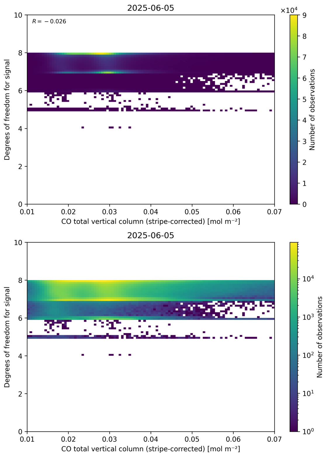
Figure 38: Scatter density plot of “CO total vertical column (stripe-corrected)” against “Degrees of freedom for signal” for 2025-06-04 to 2025-06-06.
