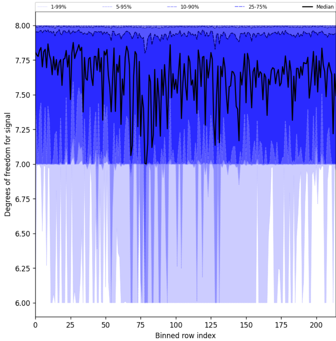
Figure 31: Along track statistics of “Degrees of freedom for signal” for 2025-06-04 to 2025-06-06
