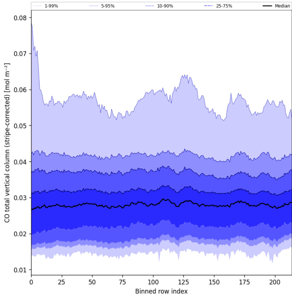
Figure 27: Along track statistics of “CO total vertical column (stripe-corrected)” for 2025-06-04 to 2025-06-06
