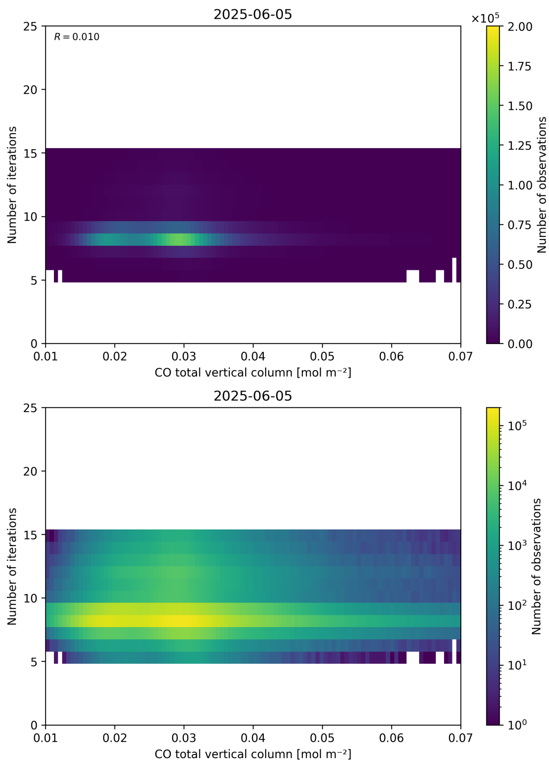
Figure 42: Scatter density plot of “CO total vertical column” against “Number of iterations” for 2025-06-04 to 2025-06-06.
