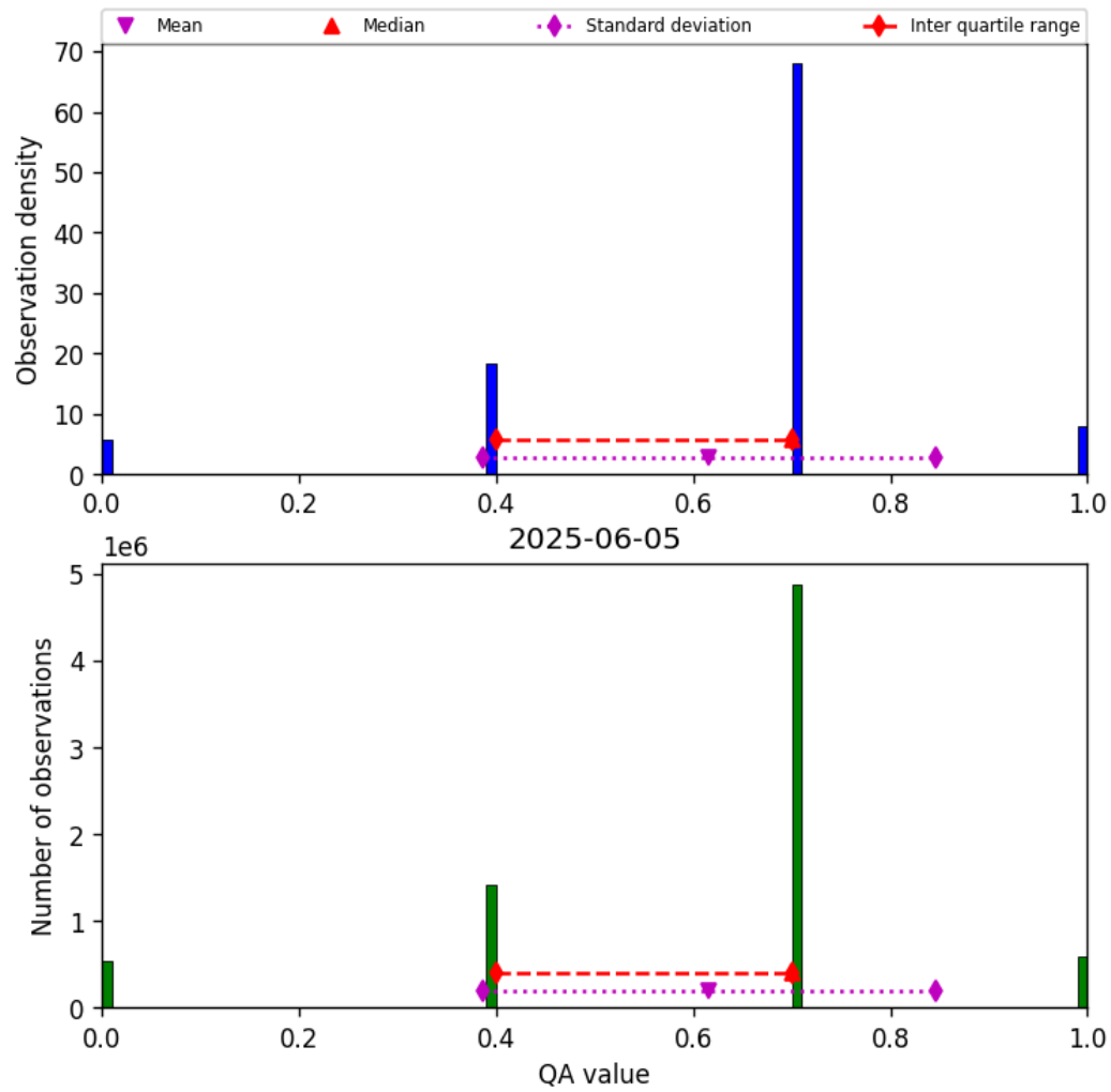
Figure 17: Histogram of “QA value” for 2025-06-04 to 2025-06-06
