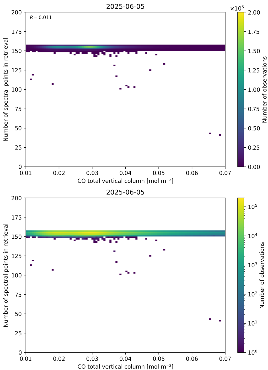
Figure 43: Scatter density plot of “CO total vertical column” against “Number of spectral points in retrieval” for 2025-06-04 to 2025-06-06.
