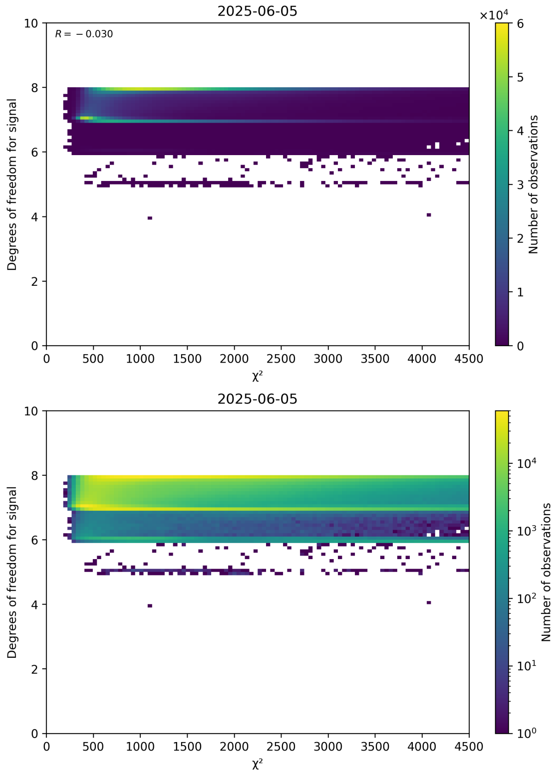
Figure 48: Scatter density plot of “ \chi^2 ” against “Degrees of freedom for signal” for 2025-06-04 to 2025-06-06.
