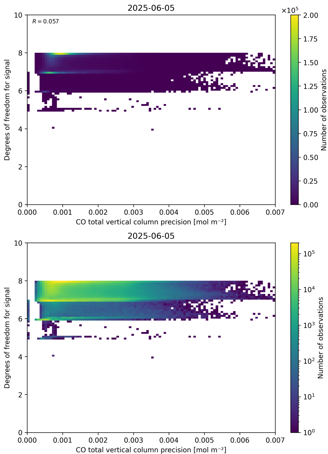
Figure 45: Scatter density plot of “CO total vertical column precision” against “Degrees of freedom for signal” for 2025-06-04 to 2025-06-06.
