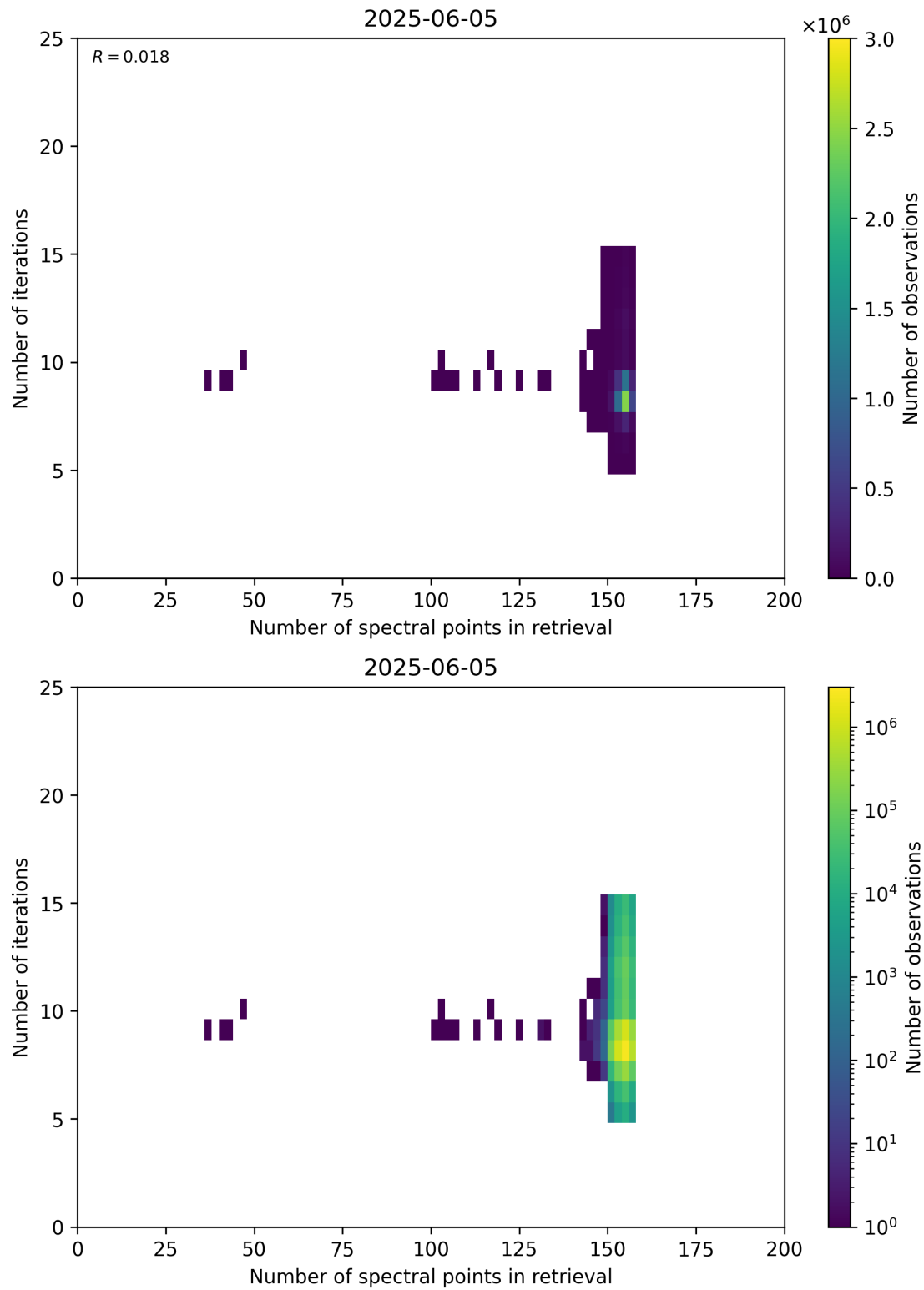
Figure 60: Scatter density plot of “Number of spectral points in retrieval” against “Number of iterations” for 2025-06-04 to 2025-06-06.
