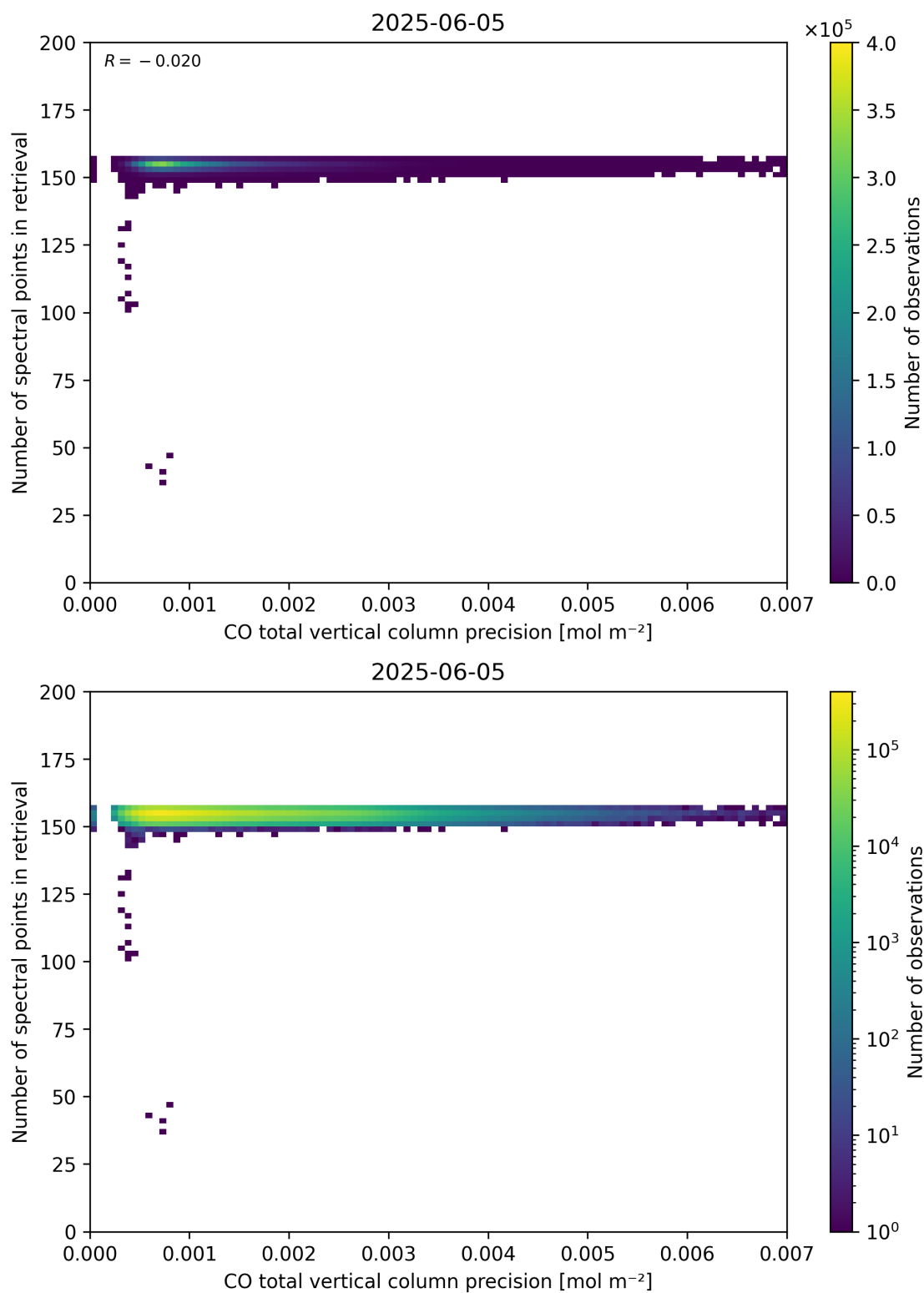
Figure 47: Scatter density plot of “CO total vertical column precision” against “Number of spectral points in retrieval” for 2025-06-04 to 2025-06-06.
