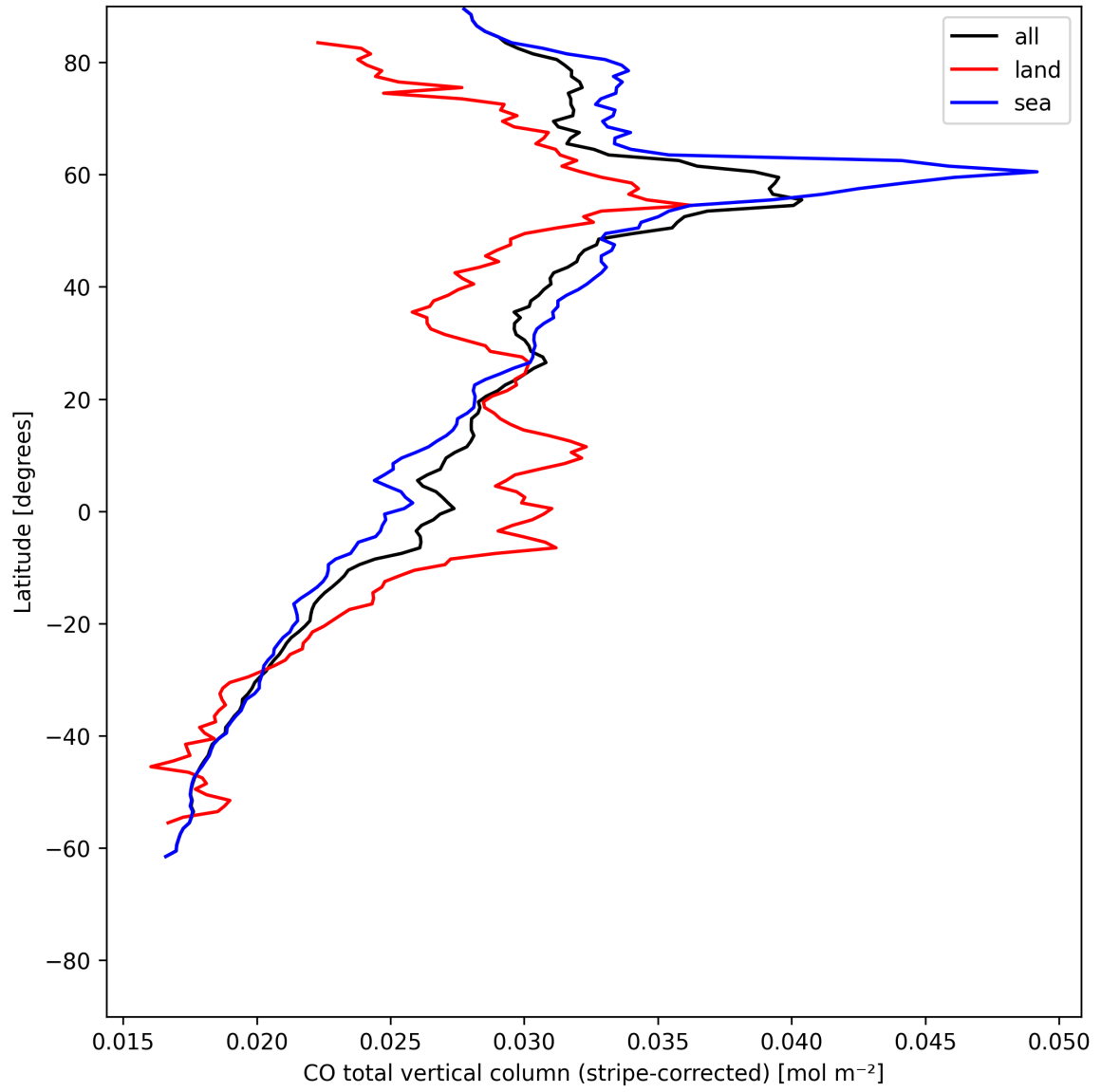
Figure 11: Zonal average of “CO total vertical column (stripe-corrected)” for 2025-06-04 to 2025-06-06.
