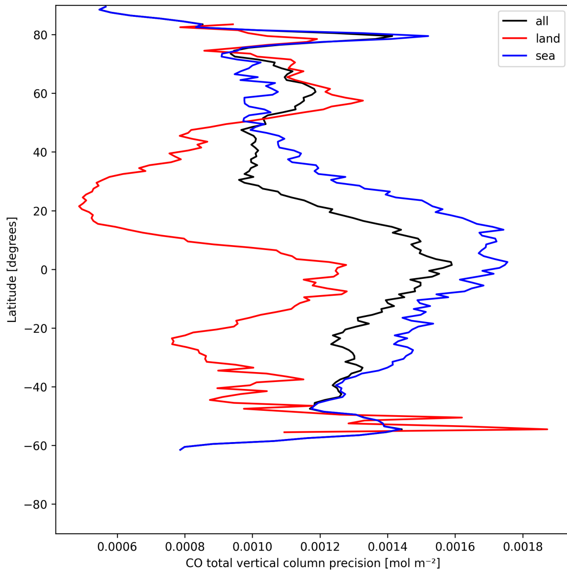
Figure 12: Zonal average of “CO total vertical column precision” for 2025-06-04 to 2025-06-06.
