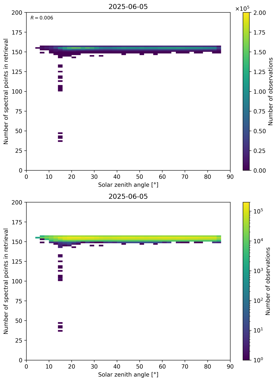
Figure 68: Scatter density plot of “Solar zenith angle” against “Number of spectral points in retrieval” for 2025-06-04 to 2025-06-06.
