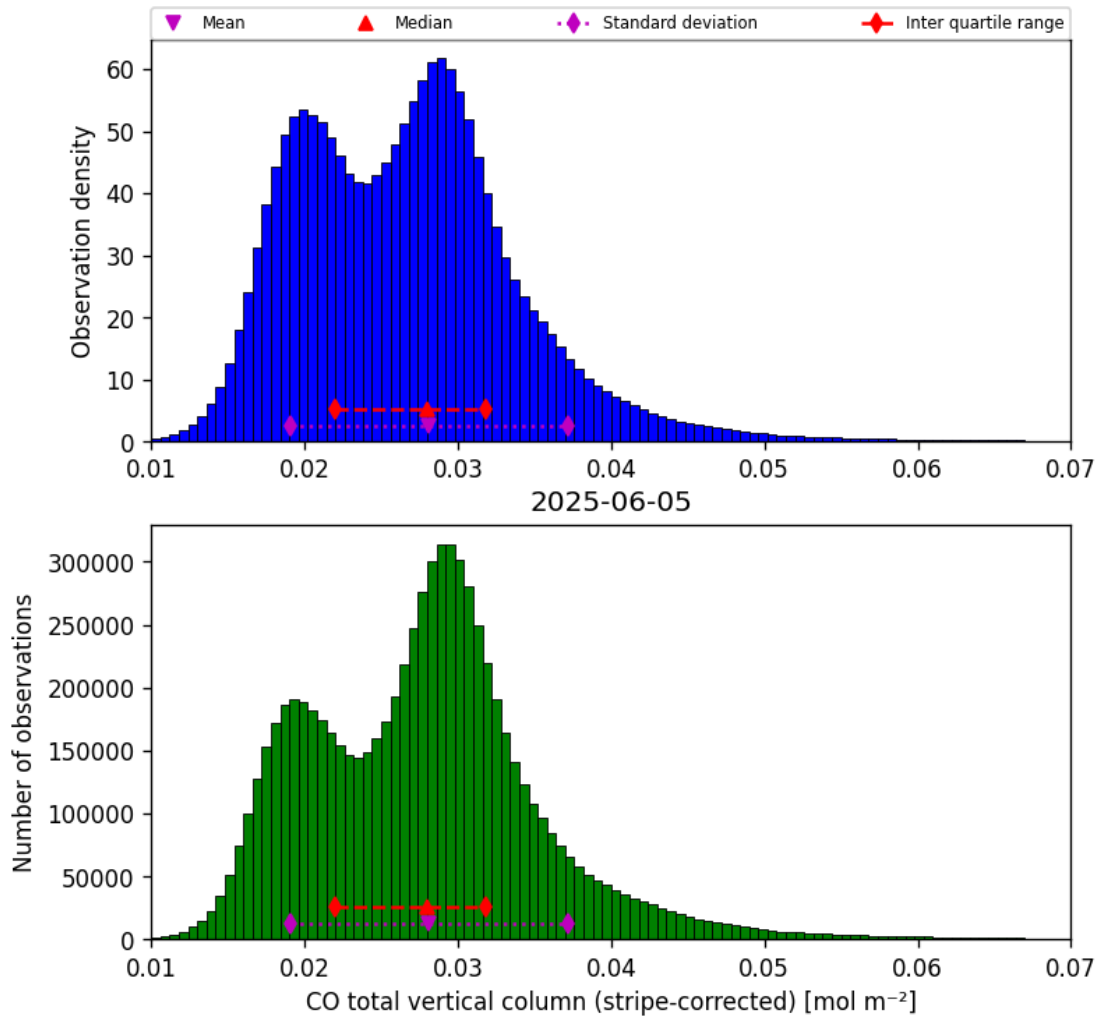
Figure 19: Histogram of “CO total vertical column (stripe-corrected)” for 2025-06-04 to 2025-06-06
