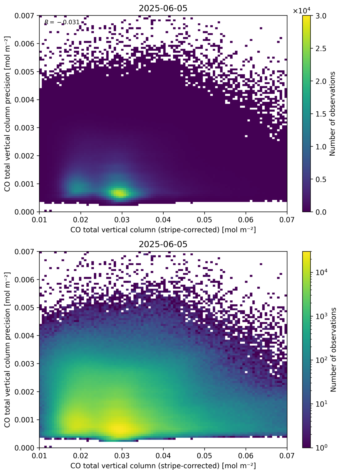
Figure 36: Scatter density plot of “CO total vertical column (stripe-corrected)” against “CO total vertical column precision” for 2025-06-04 to 2025-06-06.
