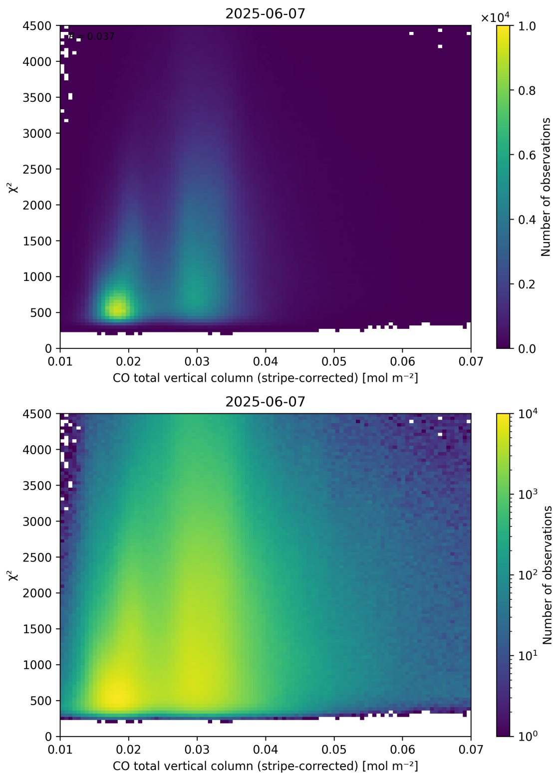
Figure 37: Scatter density plot of “CO total vertical column (stripe-corrected)” against “ \chi^2 ” for 2025-06-06 to 2025-06-08.
