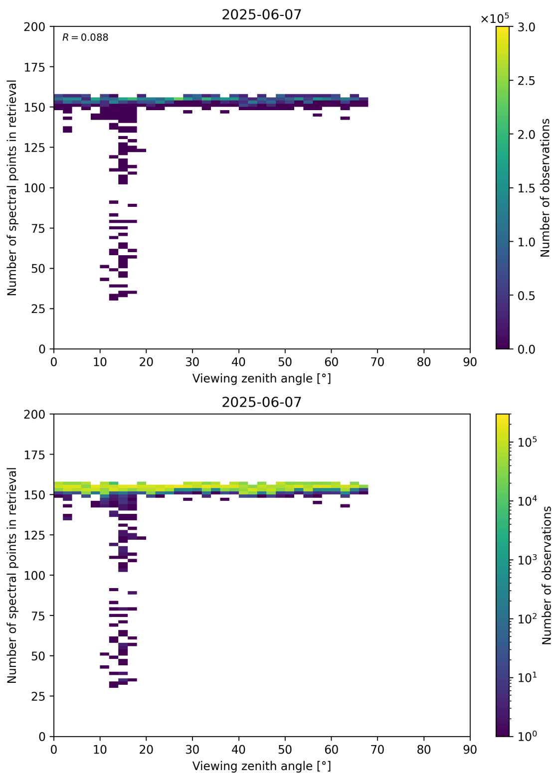
Figure 76: Scatter density plot of “Viewing zenith angle” against “Number of spectral points in retrieval” for 2025-06-06 to 2025-06-08.
