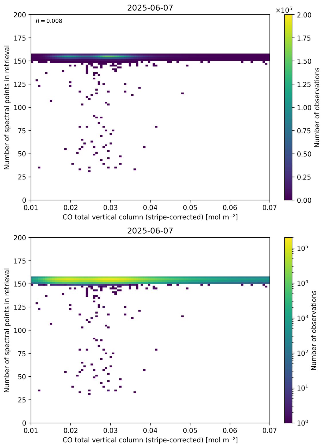
Figure 40: Scatter density plot of “CO total vertical column (stripe-corrected)” against “Number of spectral points in retrieval” for 2025-06-06 to 2025-06-08.
