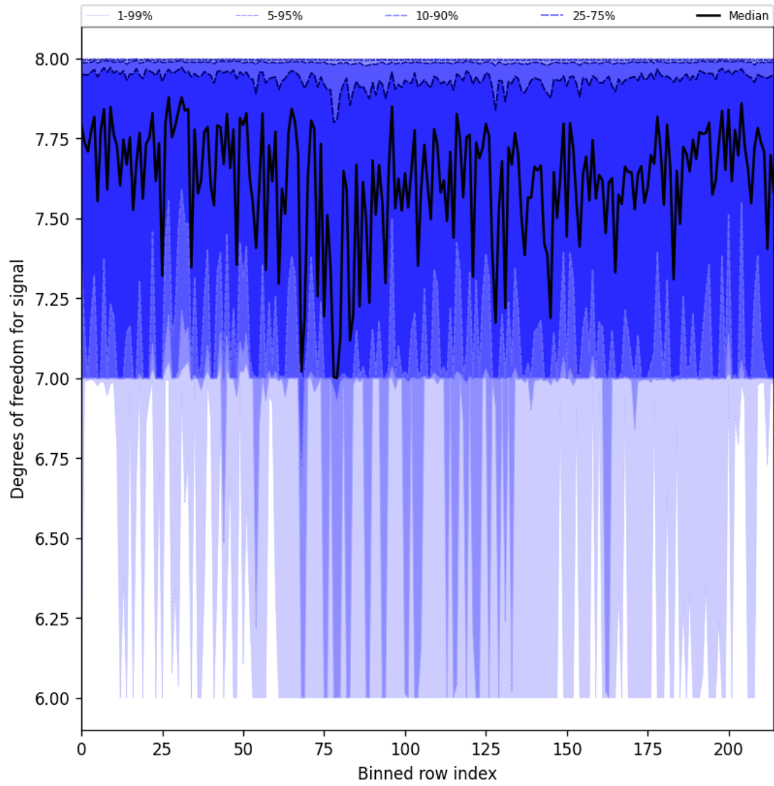
Figure 31: Along track statistics of “Degrees of freedom for signal” for 2025-06-06 to 2025-06-08
