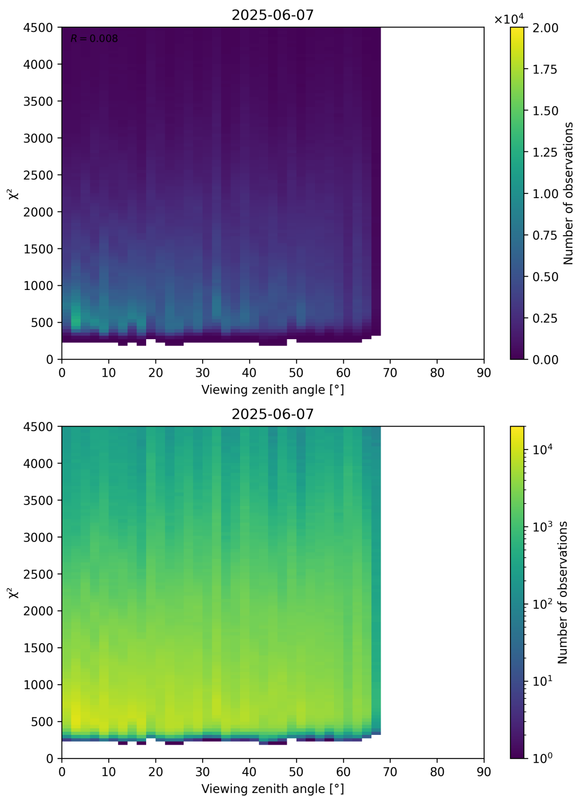
Figure 72: Scatter density plot of “Viewing zenith angle” against “ \chi^2 ” for 2025-06-06 to 2025-06-08.
