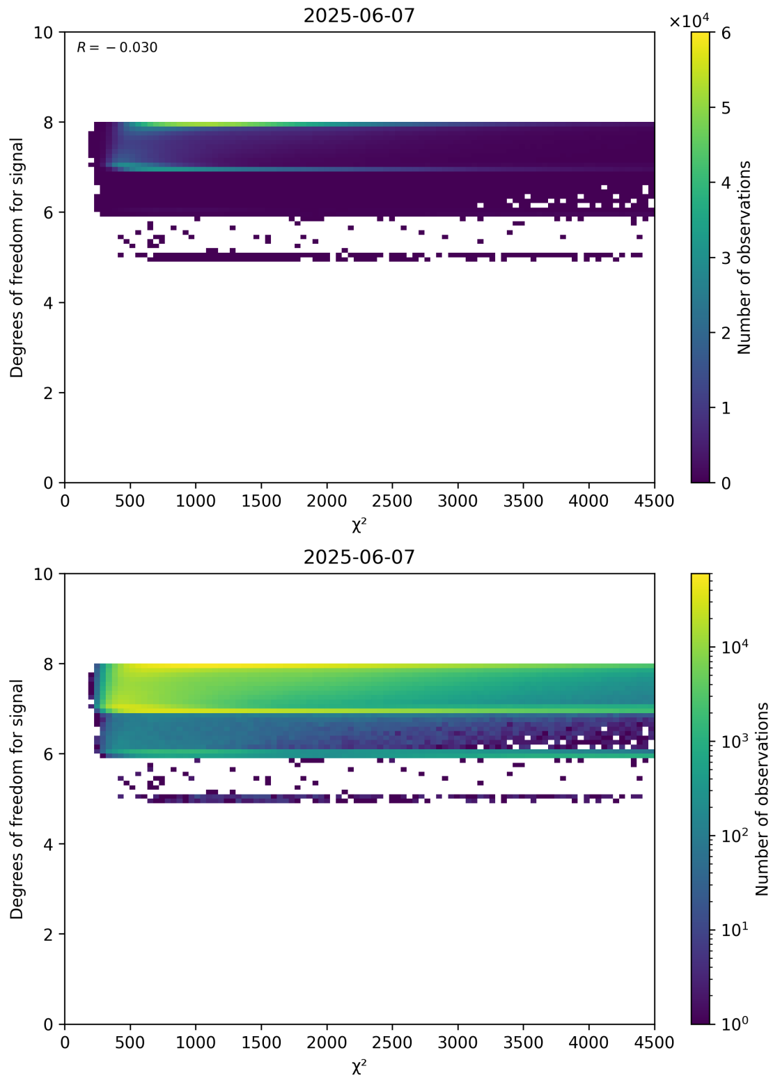
Figure 48: Scatter density plot of “ \chi^2 ” against “Degrees of freedom for signal” for 2025-06-06 to 2025-06-08.
