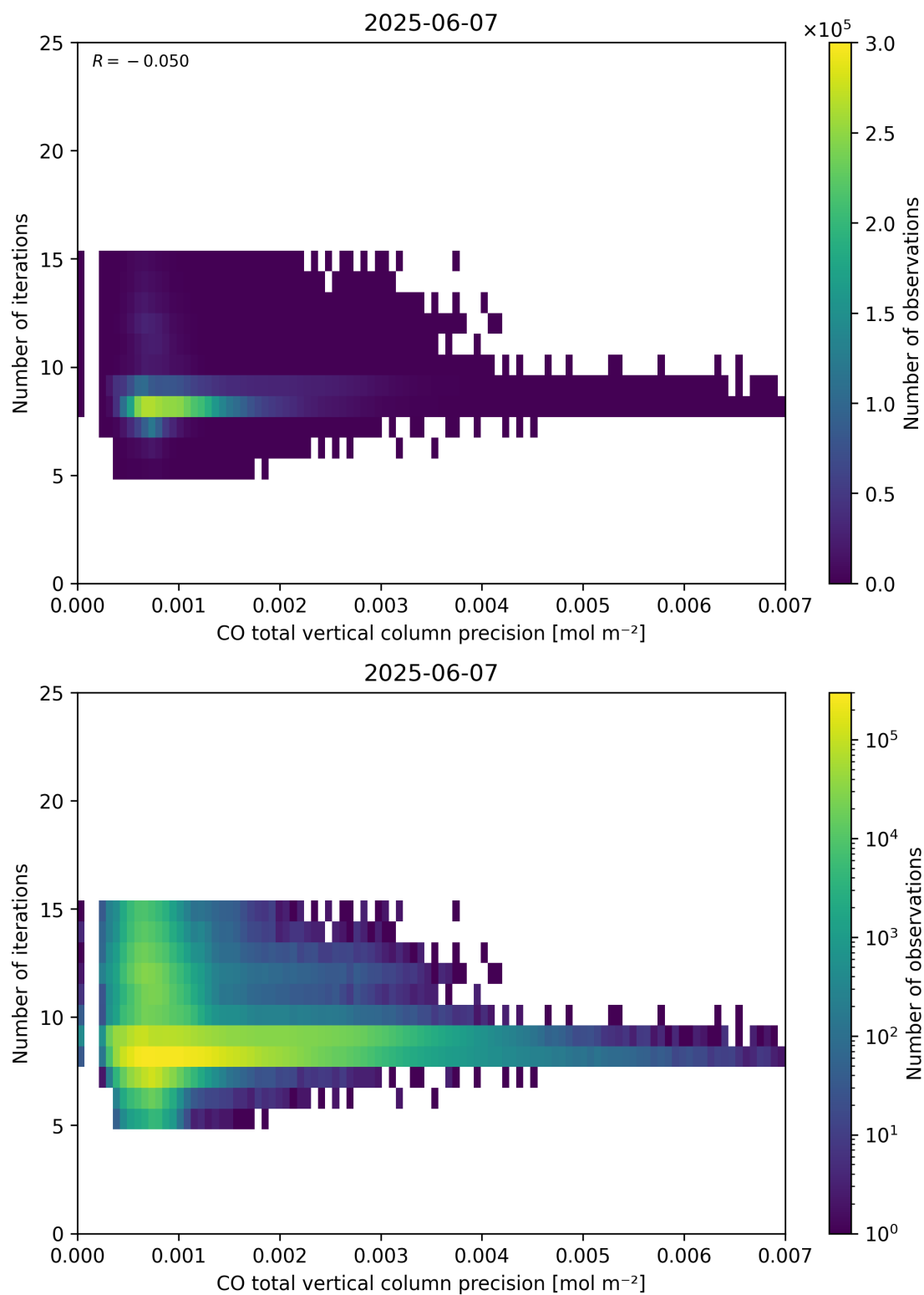
Figure 46: Scatter density plot of “CO total vertical column precision” against “Number of iterations” for 2025-06-06 to 2025-06-08.
