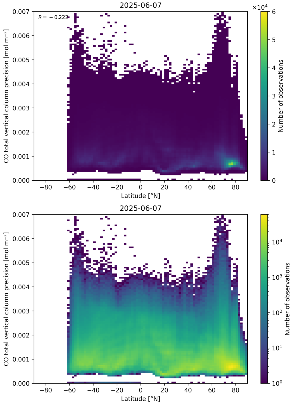
Figure 53: Scatter density plot of “Latitude” against “CO total vertical column precision” for 2025-06-06 to 2025-06-08.
