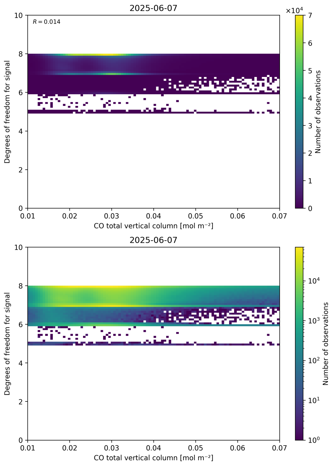
Figure 41: Scatter density plot of “CO total vertical column” against “Degrees of freedom for signal” for 2025-06-06 to 2025-06-08.
