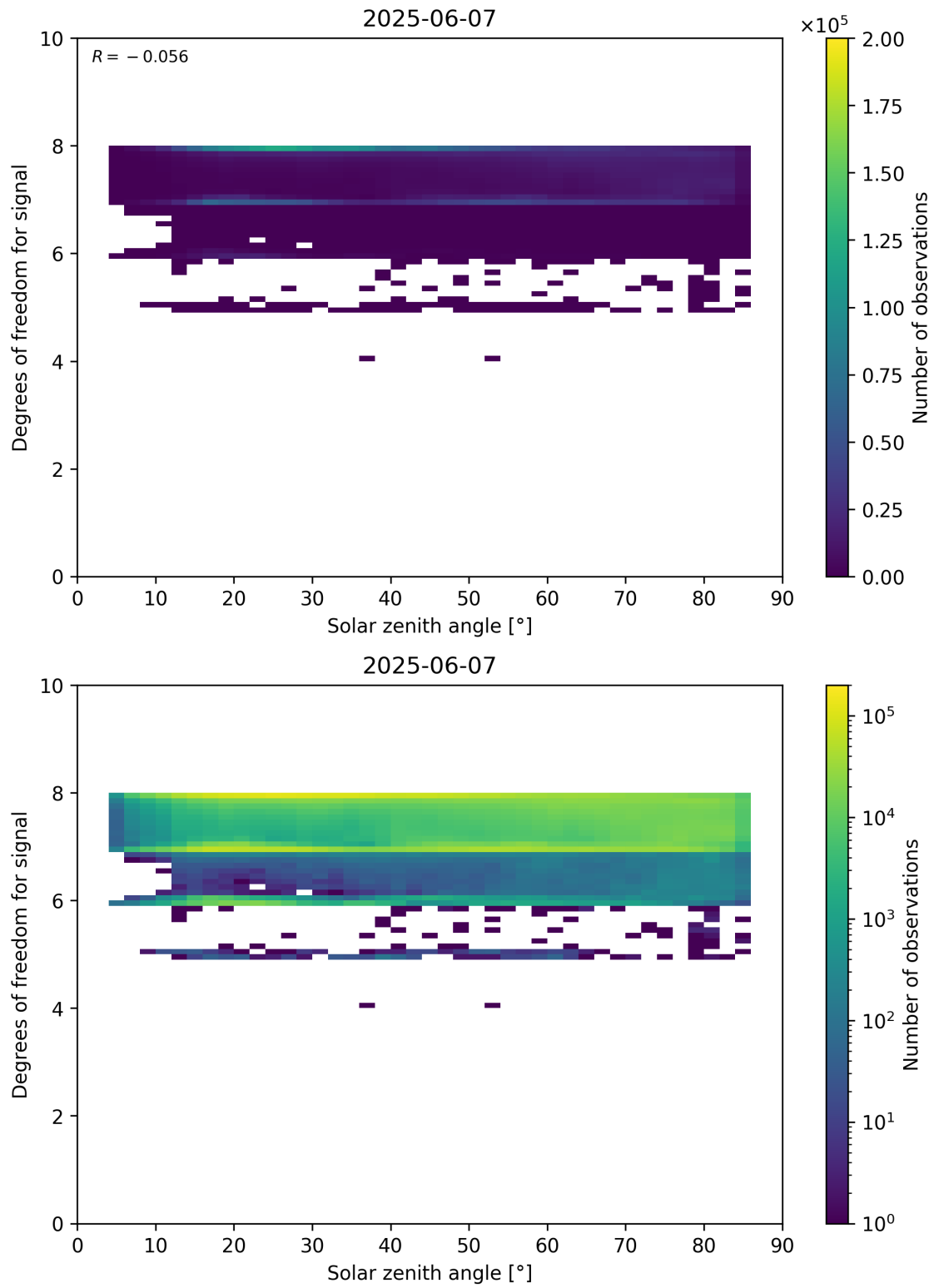
Figure 65: Scatter density plot of “Solar zenith angle” against “Degrees of freedom for signal” for 2025-06-06 to 2025-06-08.
