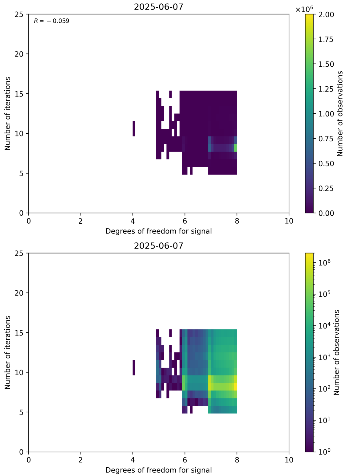
Figure 50: Scatter density plot of “Degrees of freedom for signal” against “Number of iterations” for 2025-06-06 to 2025-06-08.
