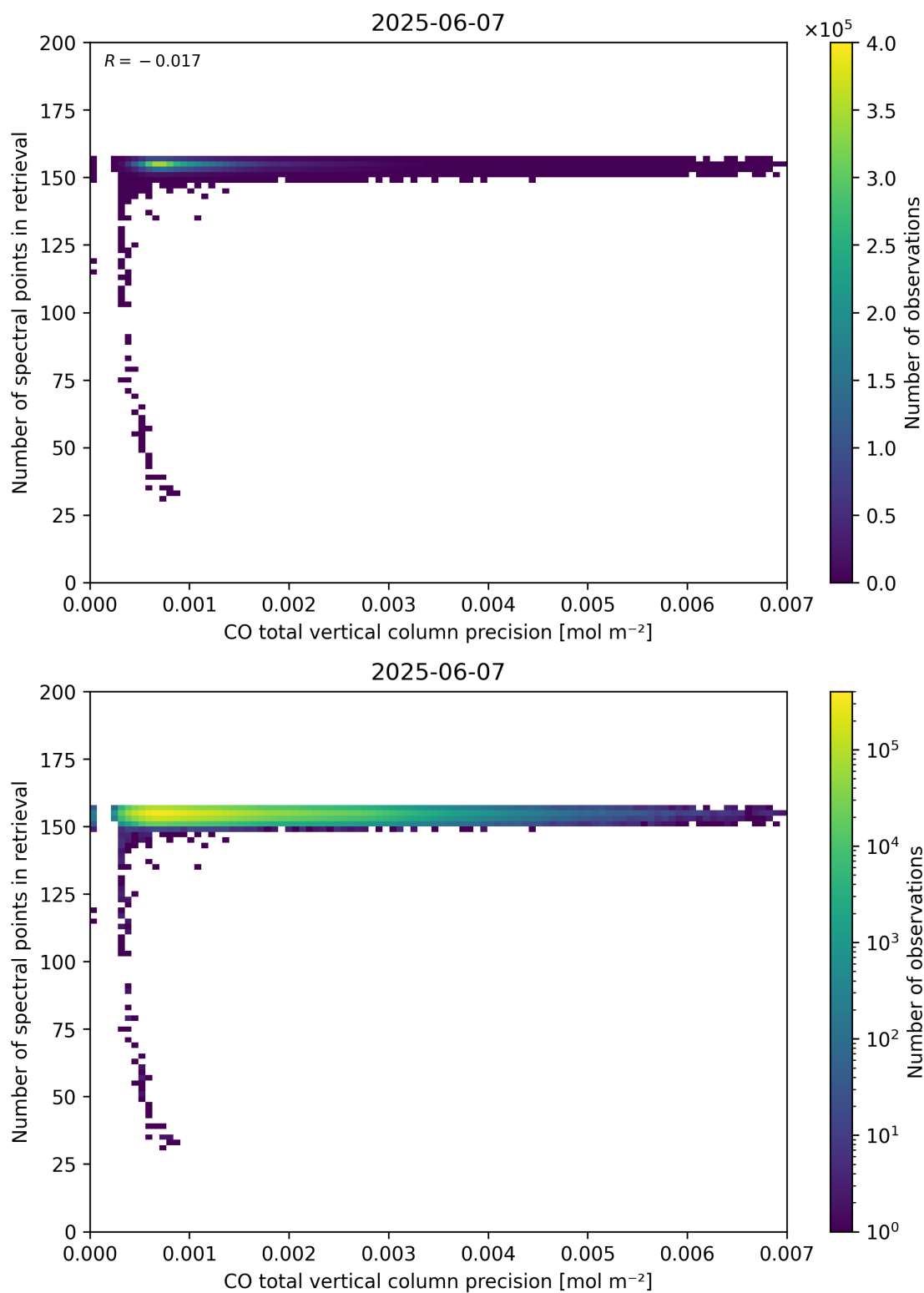
Figure 47: Scatter density plot of “CO total vertical column precision” against “Number of spectral points in retrieval” for 2025-06-06 to 2025-06-08.
