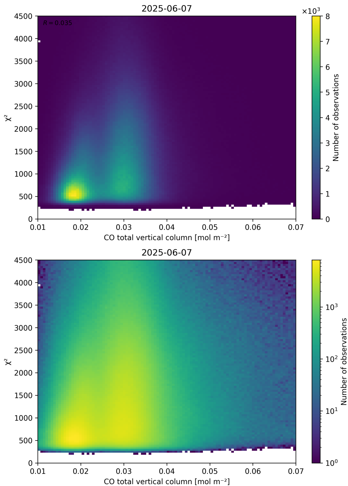
Figure 35: Scatter density plot of “CO total vertical column” against “ \chi^2 ” for 2025-06-06 to 2025-06-08.
