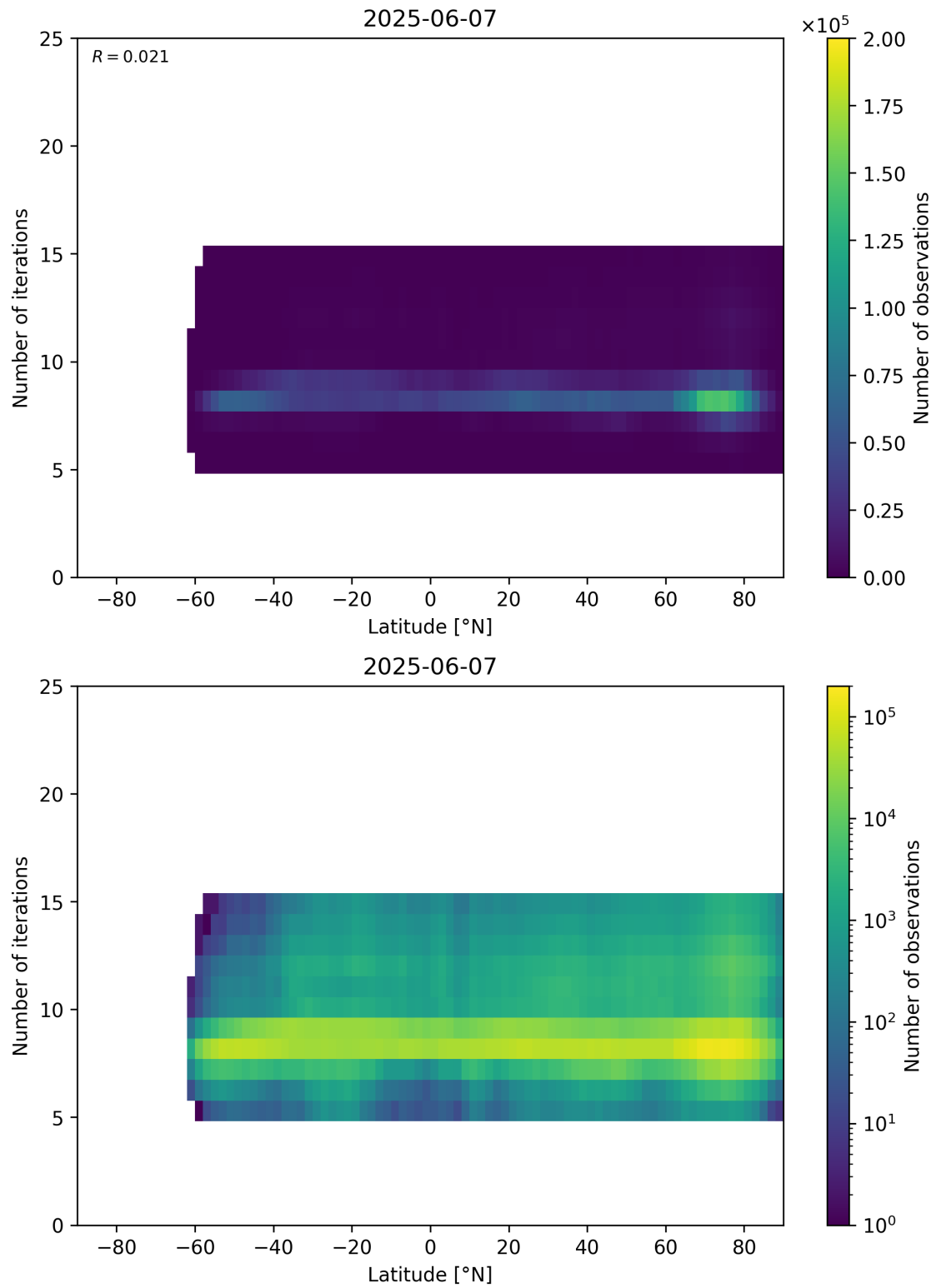
Figure 56: Scatter density plot of “Latitude” against “Number of iterations” for 2025-06-06 to 2025-06-08.
