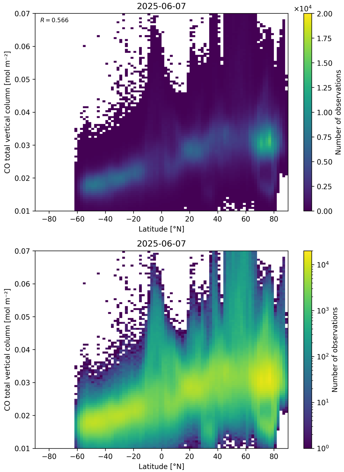
Figure 51: Scatter density plot of “Latitude” against “CO total vertical column” for 2025-06-06 to 2025-06-08.
