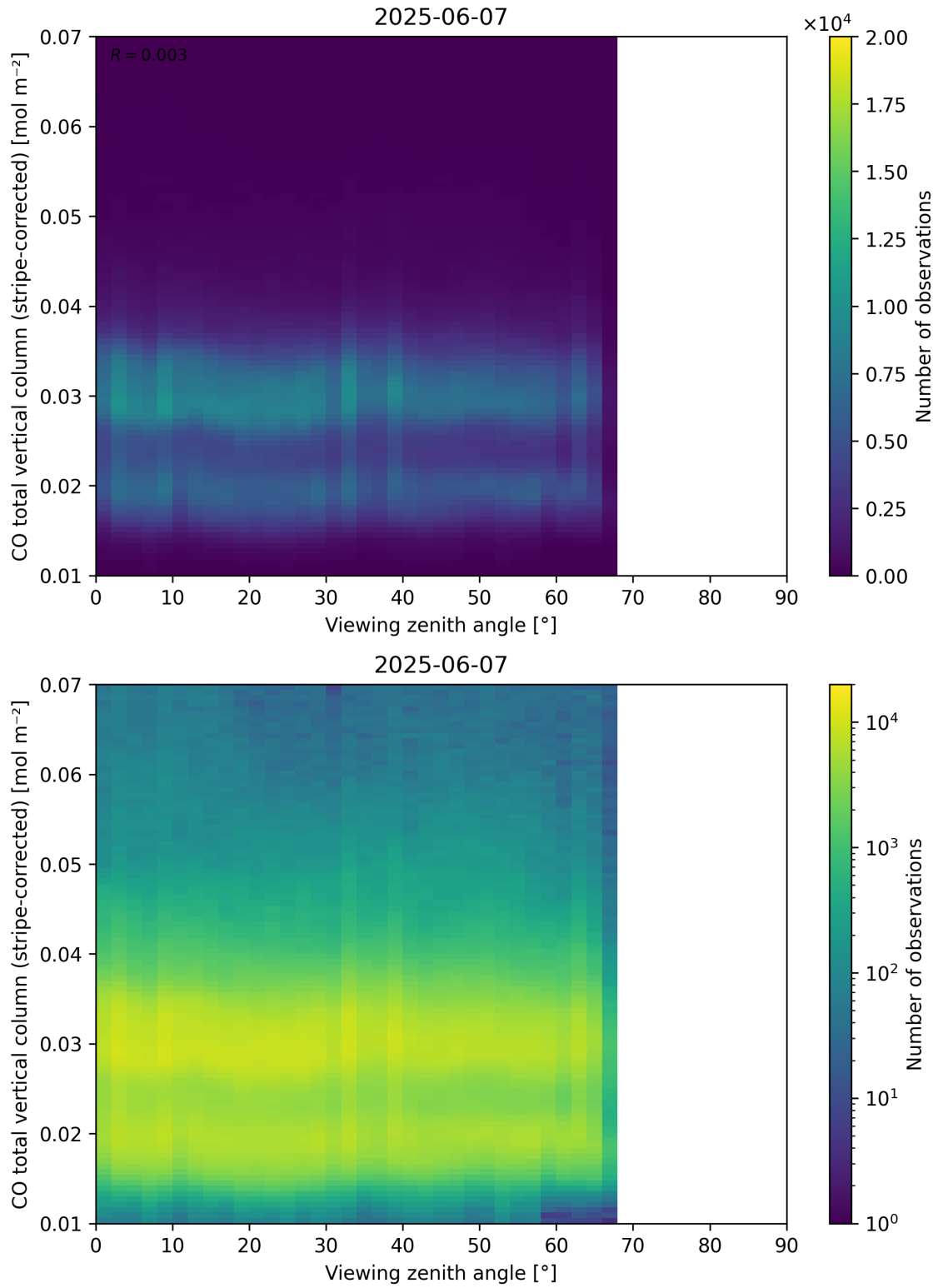
Figure 70: Scatter density plot of “Viewing zenith angle” against “CO total vertical column (stripe-corrected)” for 2025-06-06 to 2025-06-08.
