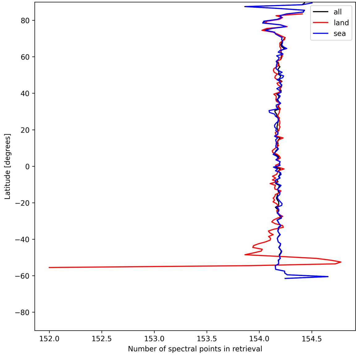
Figure 13: Zonal average of “Number of spectral points in retrieval” for 2025-06-06 to 2025-06-08.
