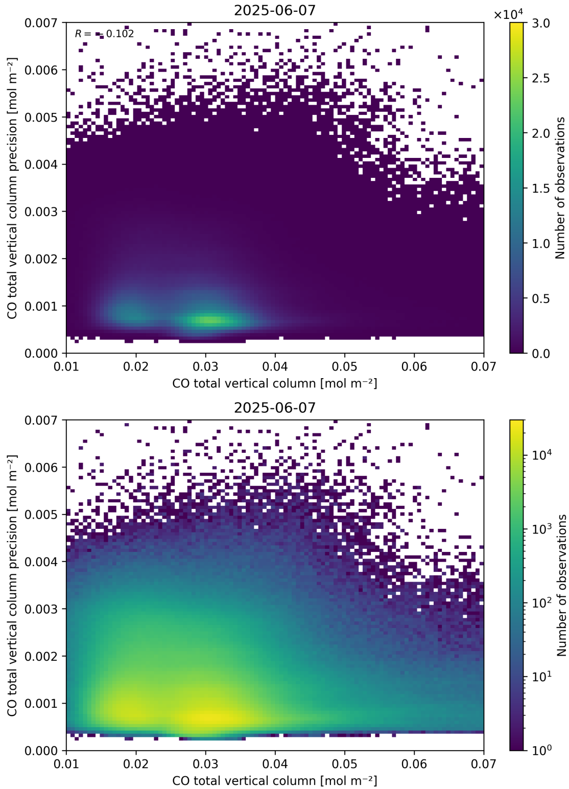
Figure 34: Scatter density plot of “CO total vertical column” against “CO total vertical column precision” for 2025-06-06 to 2025-06-08.
