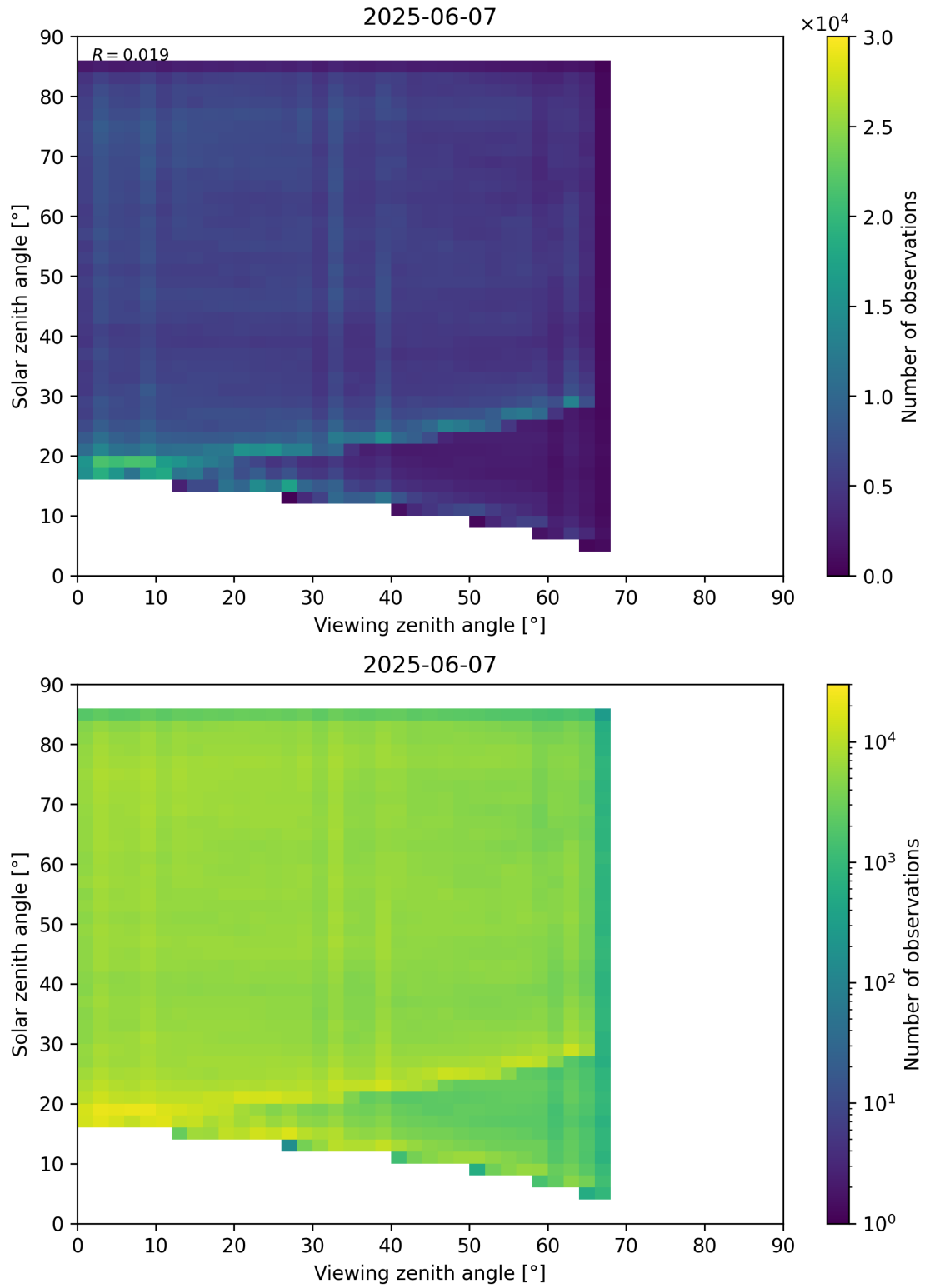
Figure 77: Scatter density plot of “Viewing zenith angle” against “Solar zenith angle” for 2025-06-06 to 2025-06-08.
