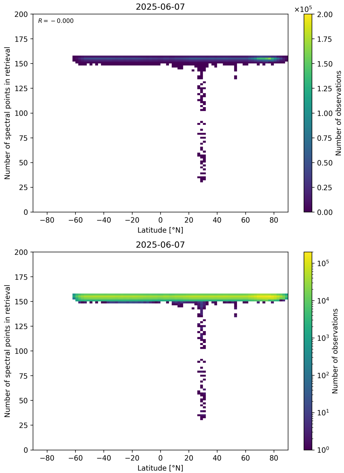
Figure 57: Scatter density plot of “Latitude” against “Number of spectral points in retrieval” for 2025-06-06 to 2025-06-08.
