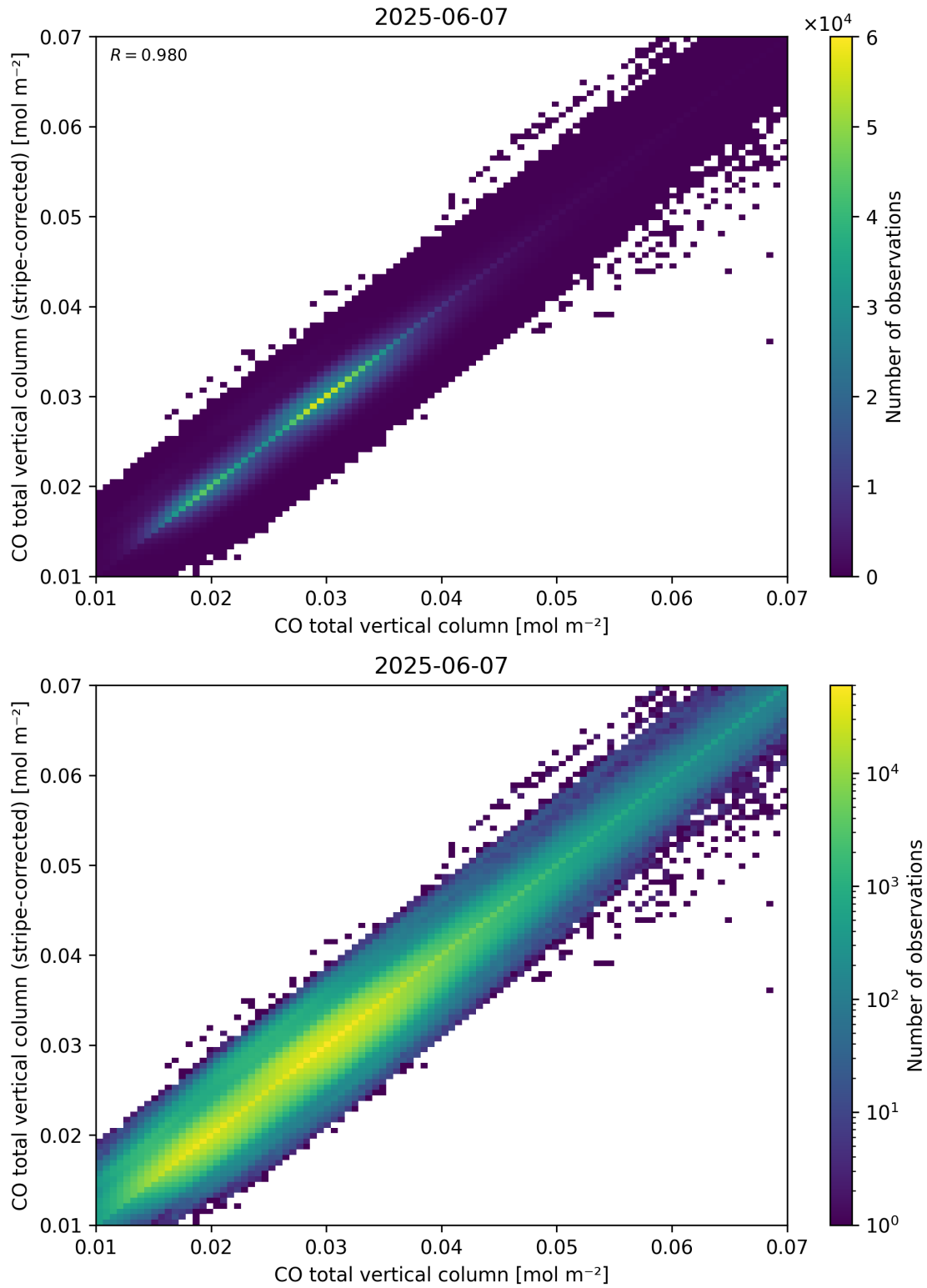
Figure 33: Scatter density plot of “CO total vertical column” against “CO total vertical column (stripe-corrected)” for 2025-06-06 to 2025-06-08.
