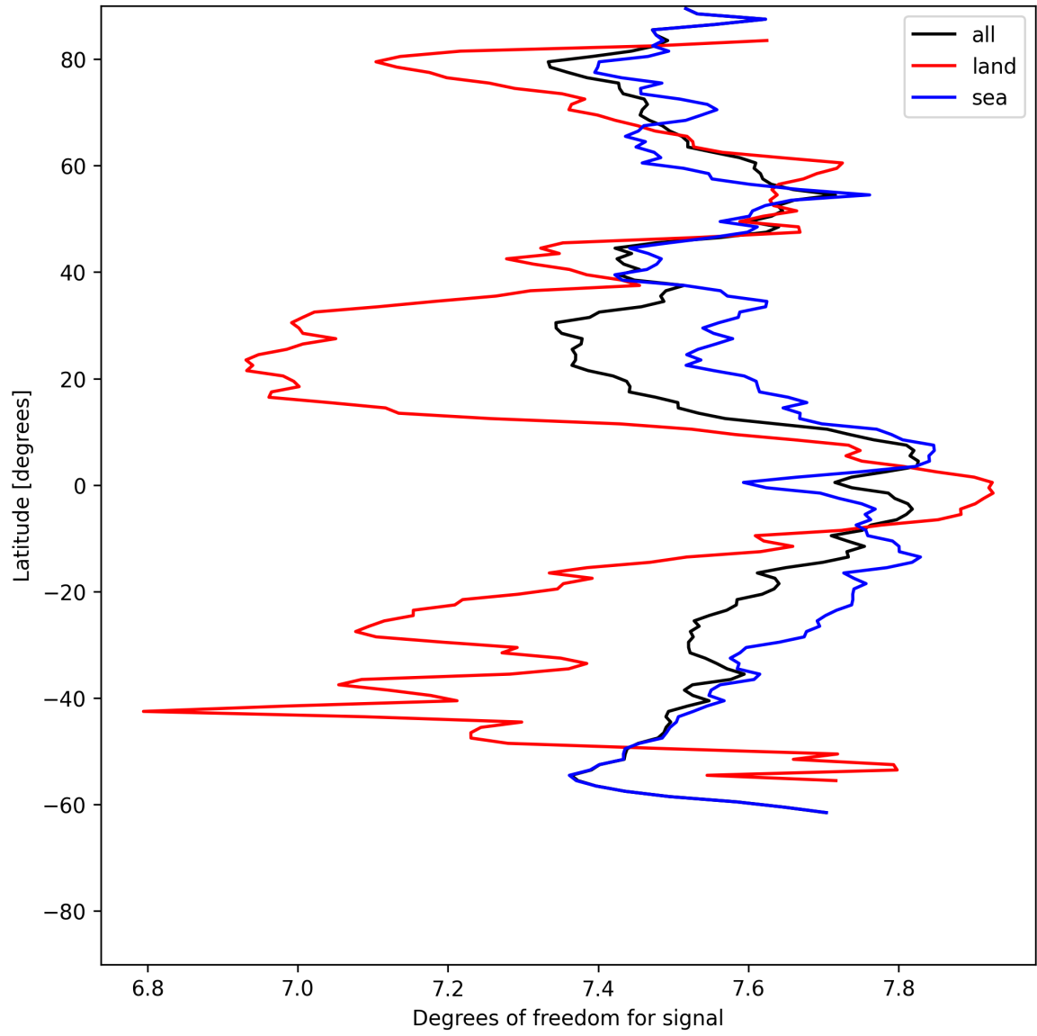
Figure 15: Zonal average of “Degrees of freedom for signal” for 2025-06-06 to 2025-06-08.
