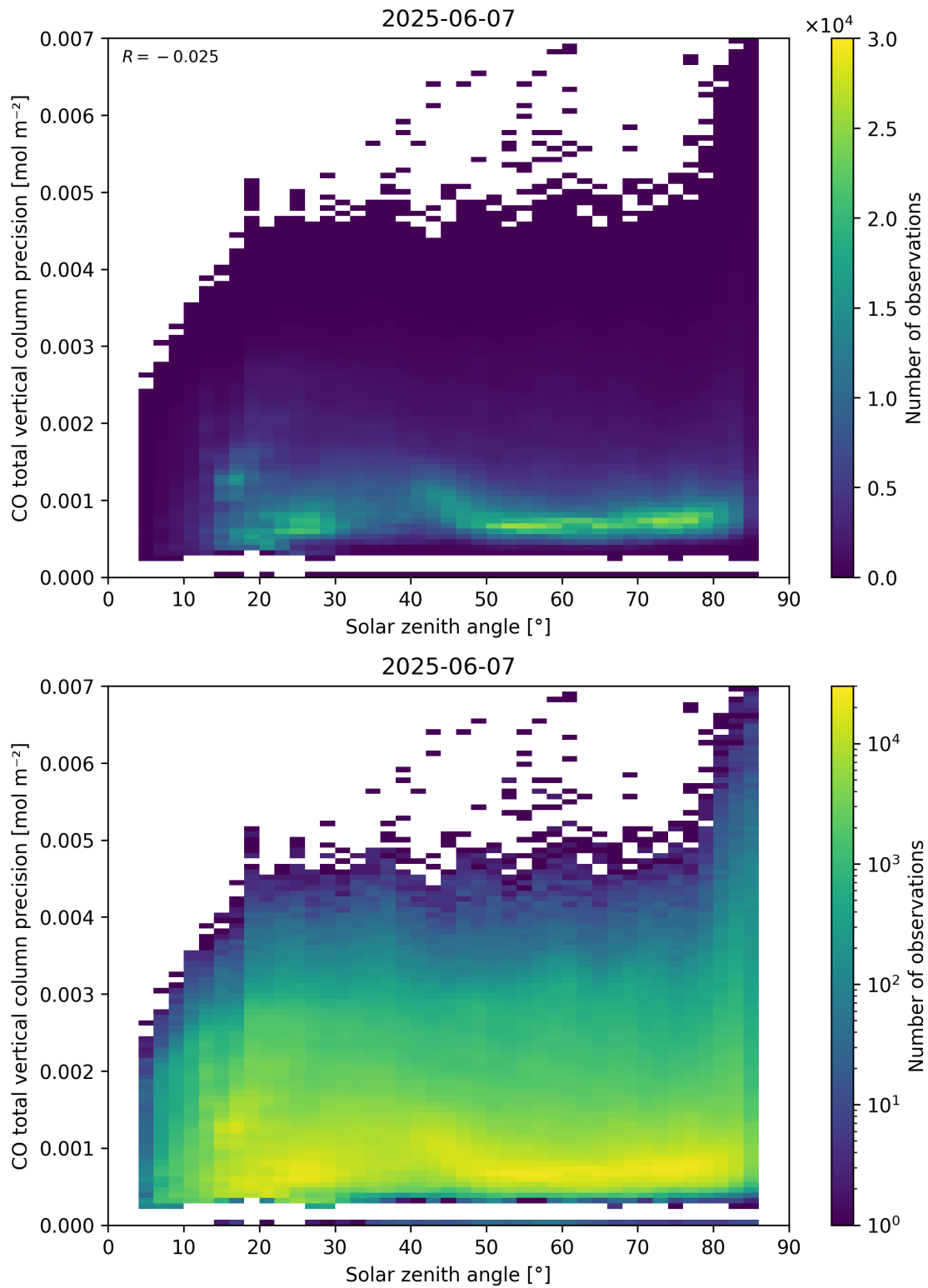
Figure 63: Scatter density plot of “Solar zenith angle” against “CO total vertical column precision” for 2025-06-06 to 2025-06-08.
