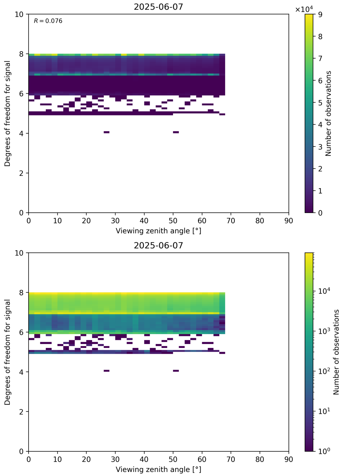
Figure 73: Scatter density plot of “Viewing zenith angle” against “Degrees of freedom for signal” for 2025-06-06 to 2025-06-08.
