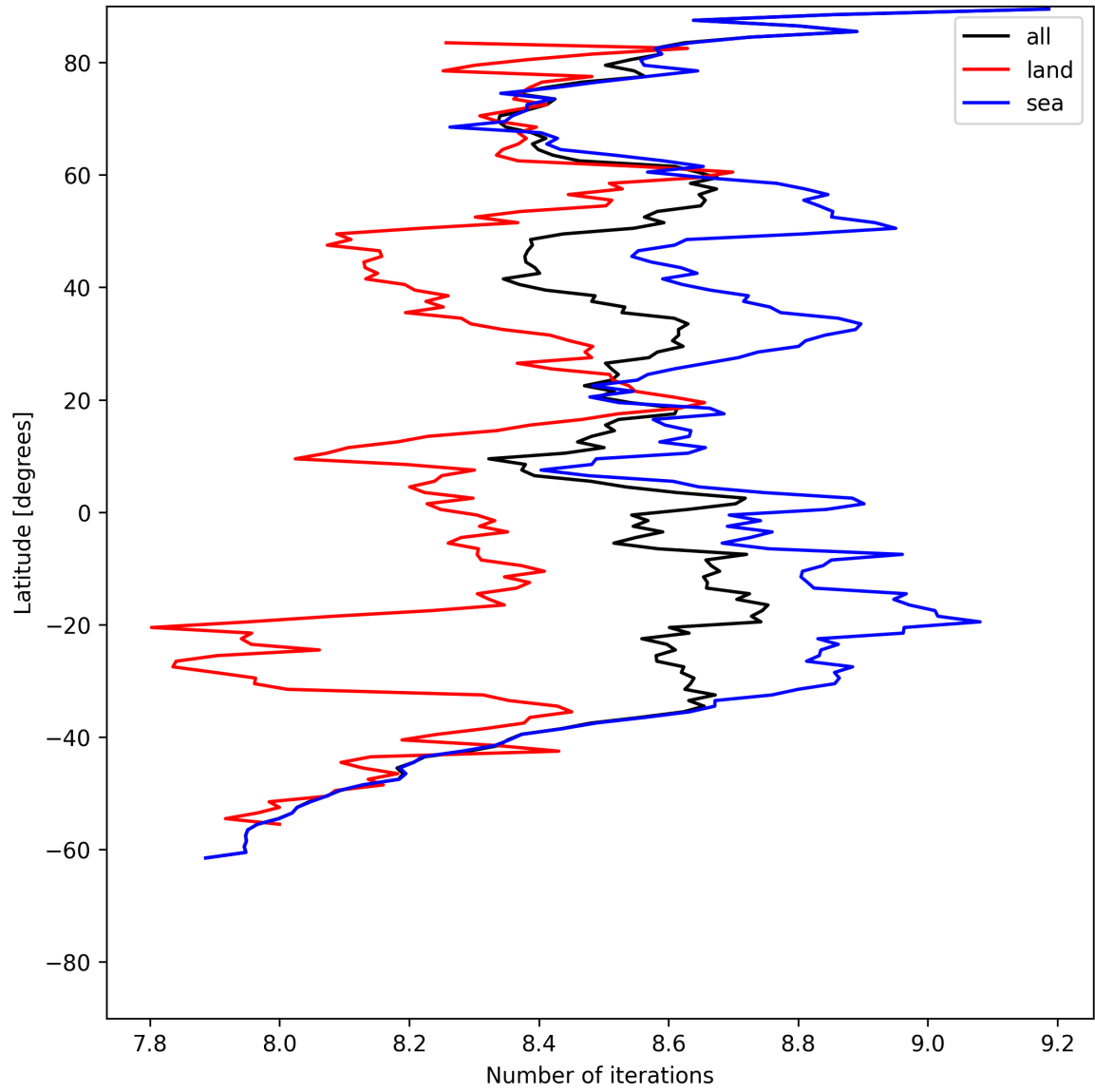
Figure 16: Zonal average of “Number of iterations” for 2025-06-06 to 2025-06-08.
