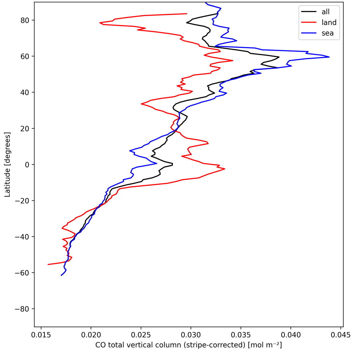
Figure 11: Zonal average of “CO total vertical column (stripe-corrected)” for 2025-06-06 to 2025-06-08.
