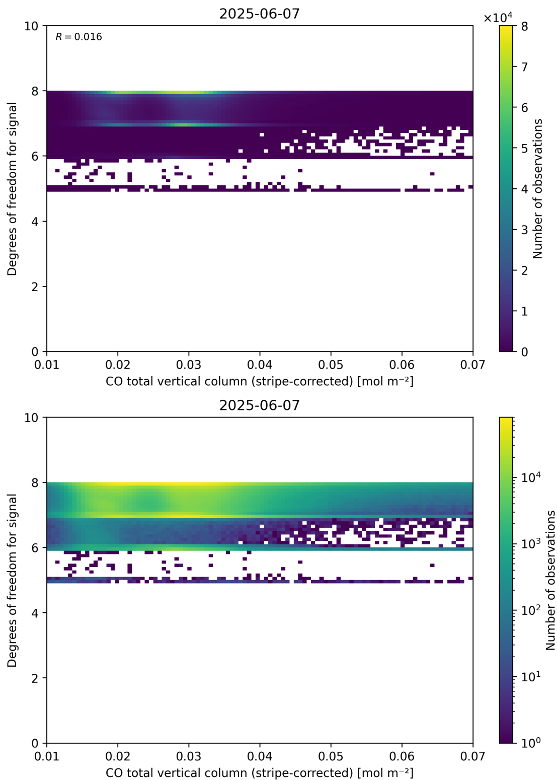
Figure 38: Scatter density plot of “CO total vertical column (stripe-corrected)” against “Degrees of freedom for signal” for 2025-06-06 to 2025-06-08.
