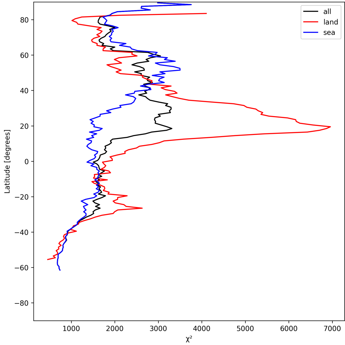
Figure 14: Zonal average of “ \chi^2 ” for 2025-06-06 to 2025-06-08.
