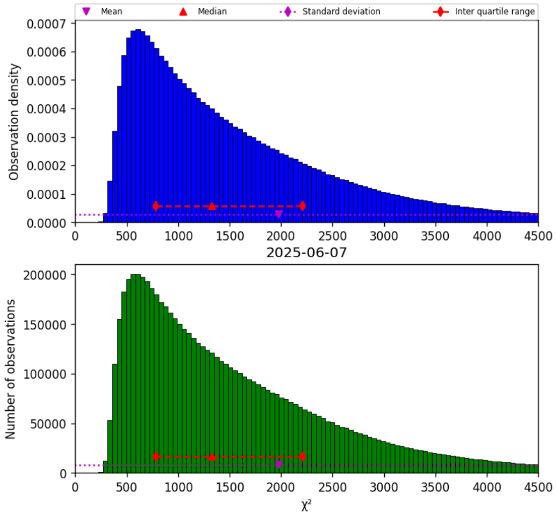
Figure 22: Histogram of “ \chi^2 ” for 2025-06-06 to 2025-06-08
