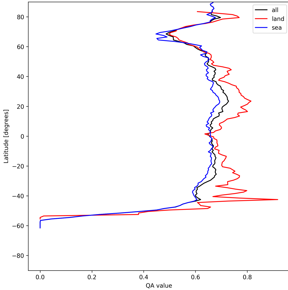
Figure 9: Zonal average of “QA value” for 2025-06-06 to 2025-06-08.
