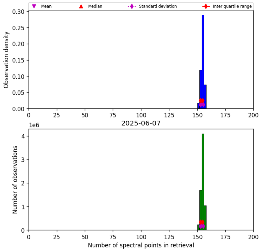
Figure 21: Histogram of “Number of spectral points in retrieval” for 2025-06-06 to 2025-06-08
