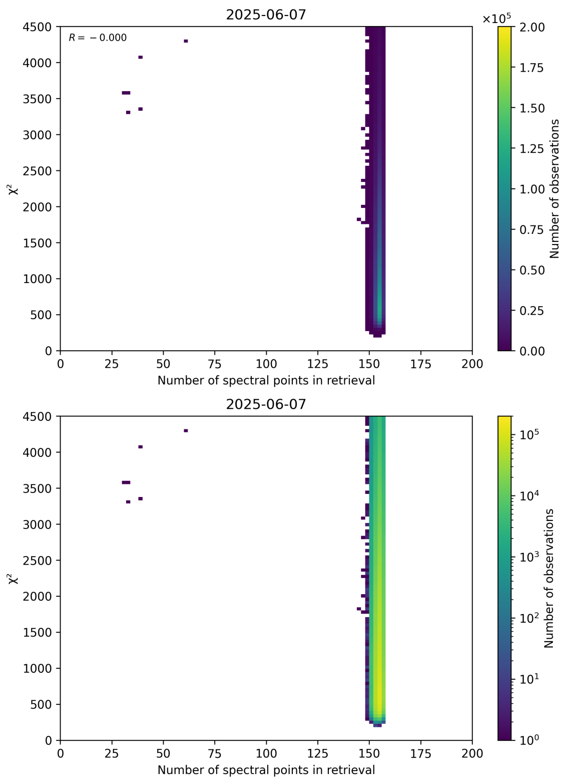
Figure 58: Scatter density plot of “Number of spectral points in retrieval” against “ \chi^2 ” for 2025-06-06 to 2025-06-08.
