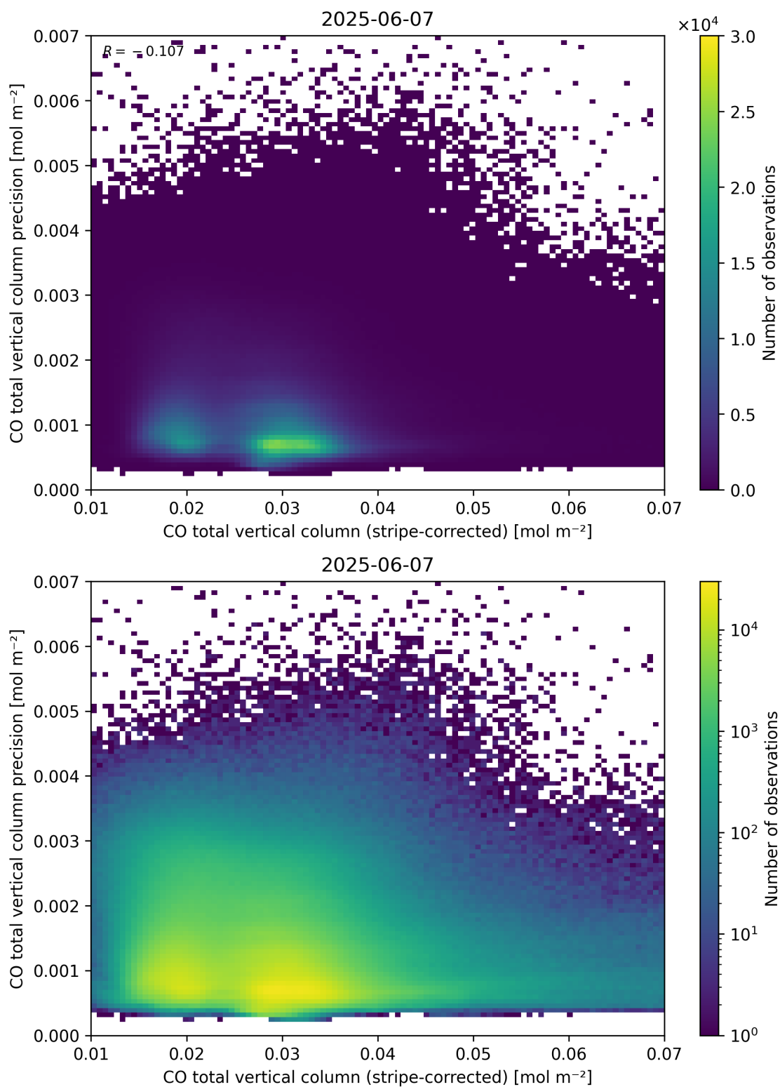
Figure 36: Scatter density plot of “CO total vertical column (stripe-corrected)” against “CO total vertical column precision” for 2025-06-06 to 2025-06-08.
