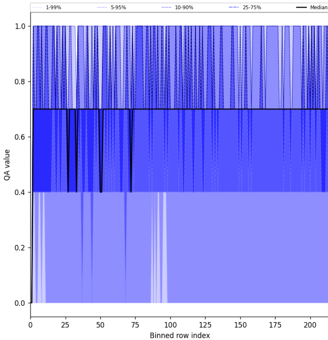
Figure 25: Along track statistics of “QA value” for 2025-06-06 to 2025-06-08
