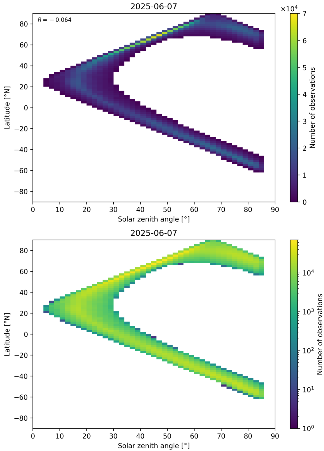
Figure 66: Scatter density plot of “Solar zenith angle” against “Latitude” for 2025-06-06 to 2025-06-08.
