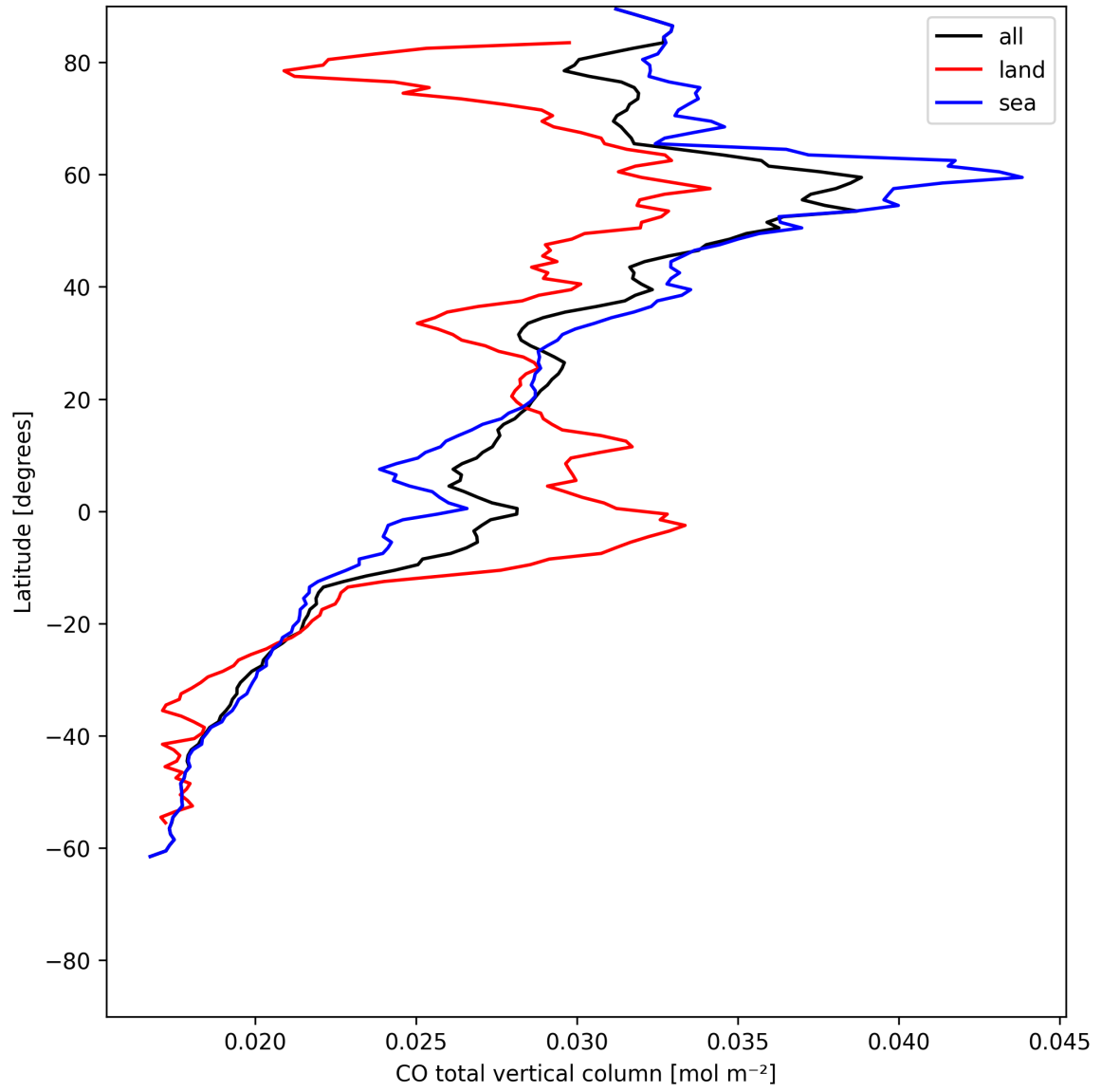
Figure 10: Zonal average of “CO total vertical column” for 2025-06-06 to 2025-06-08.
