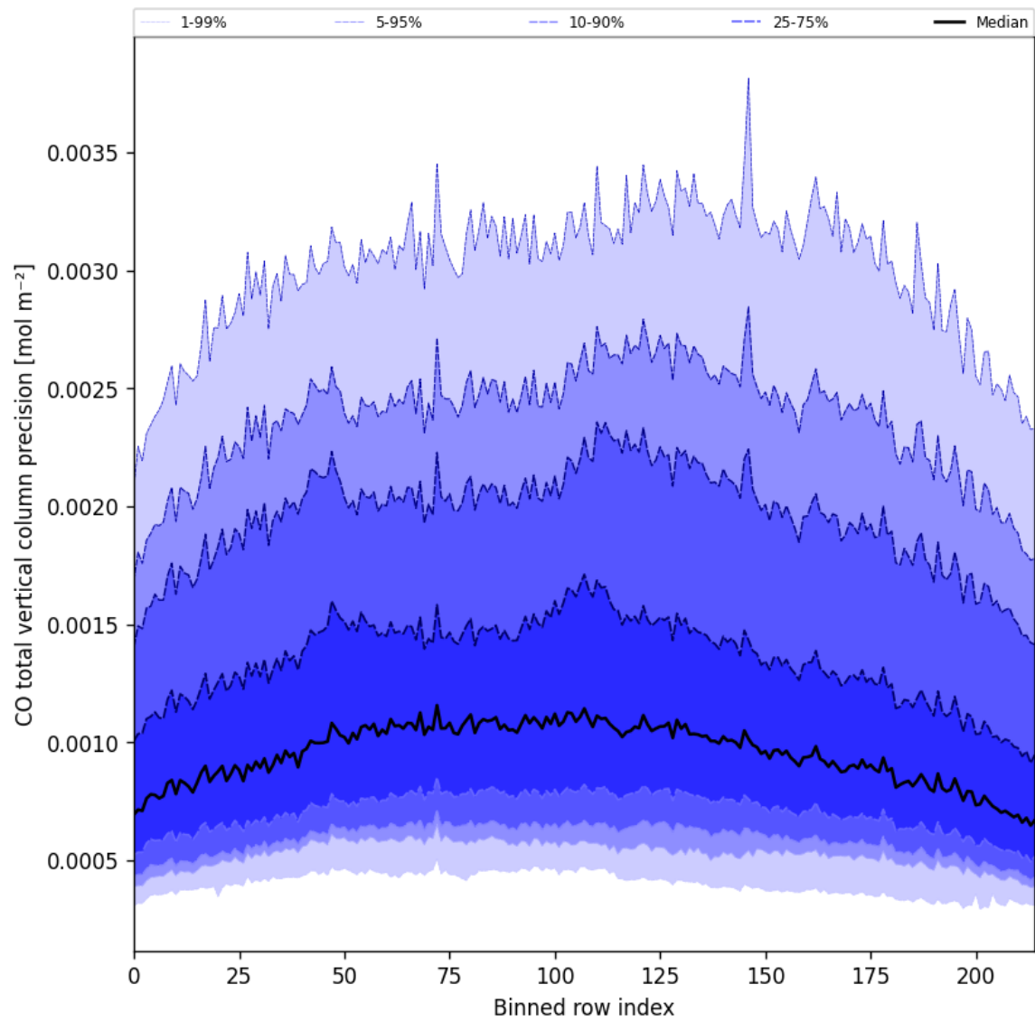
Figure 28: Along track statistics of “CO total vertical column precision” for 2025-06-06 to 2025-06-08
