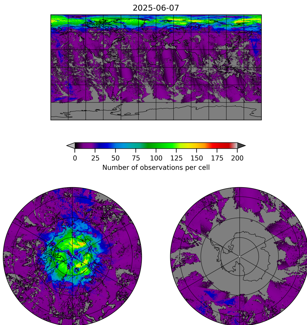
Figure 8: Map of the number of observations for 2025-06-06 to 2025-06-08
