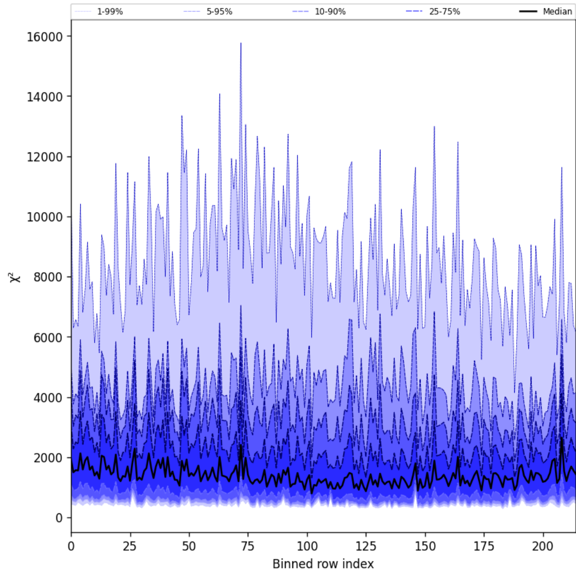
Figure 30: Along track statistics of “ \chi^2 ” for 2025-06-06 to 2025-06-08
