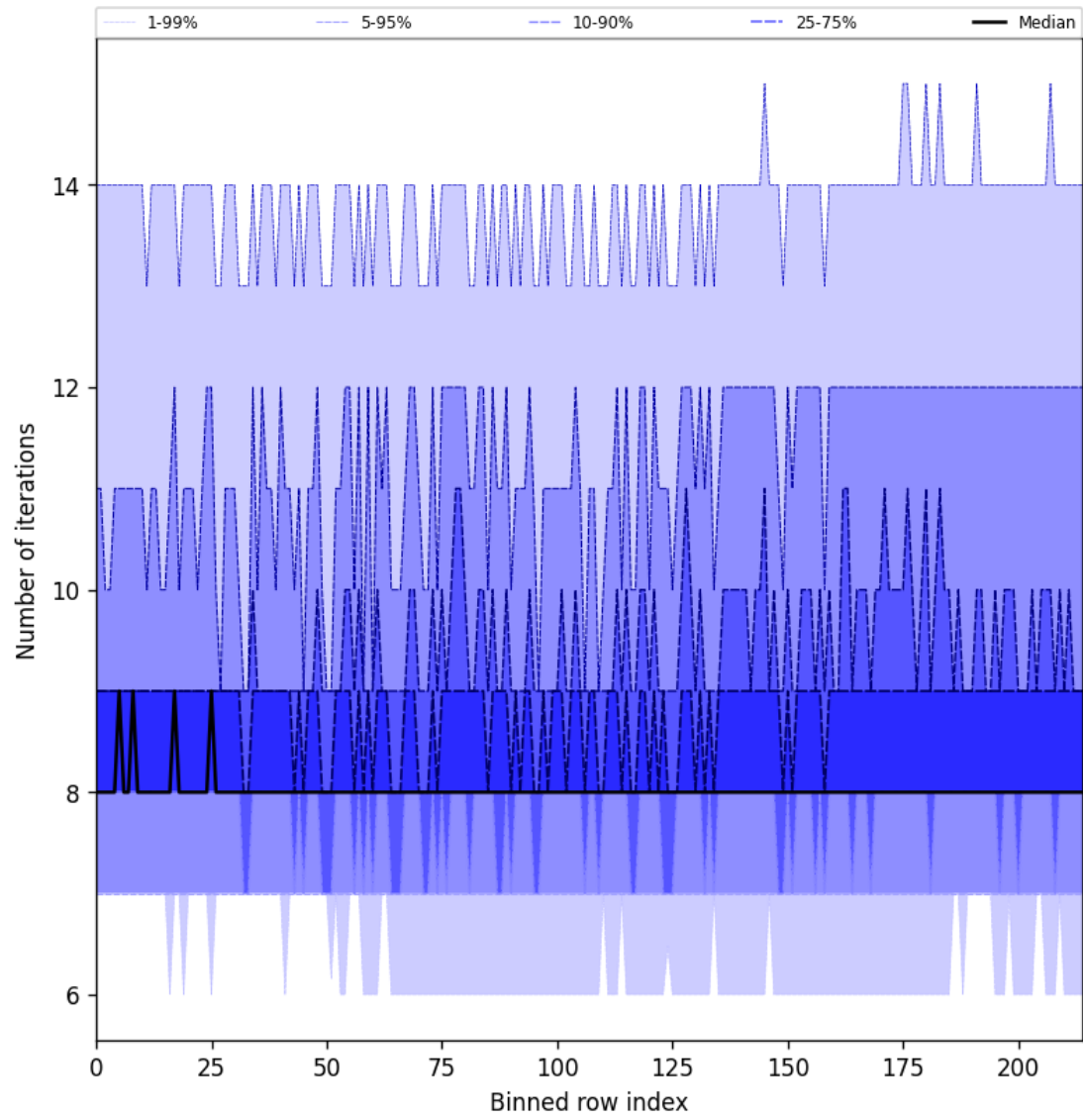
Figure 32: Along track statistics of “Number of iterations” for 2025-06-06 to 2025-06-08
