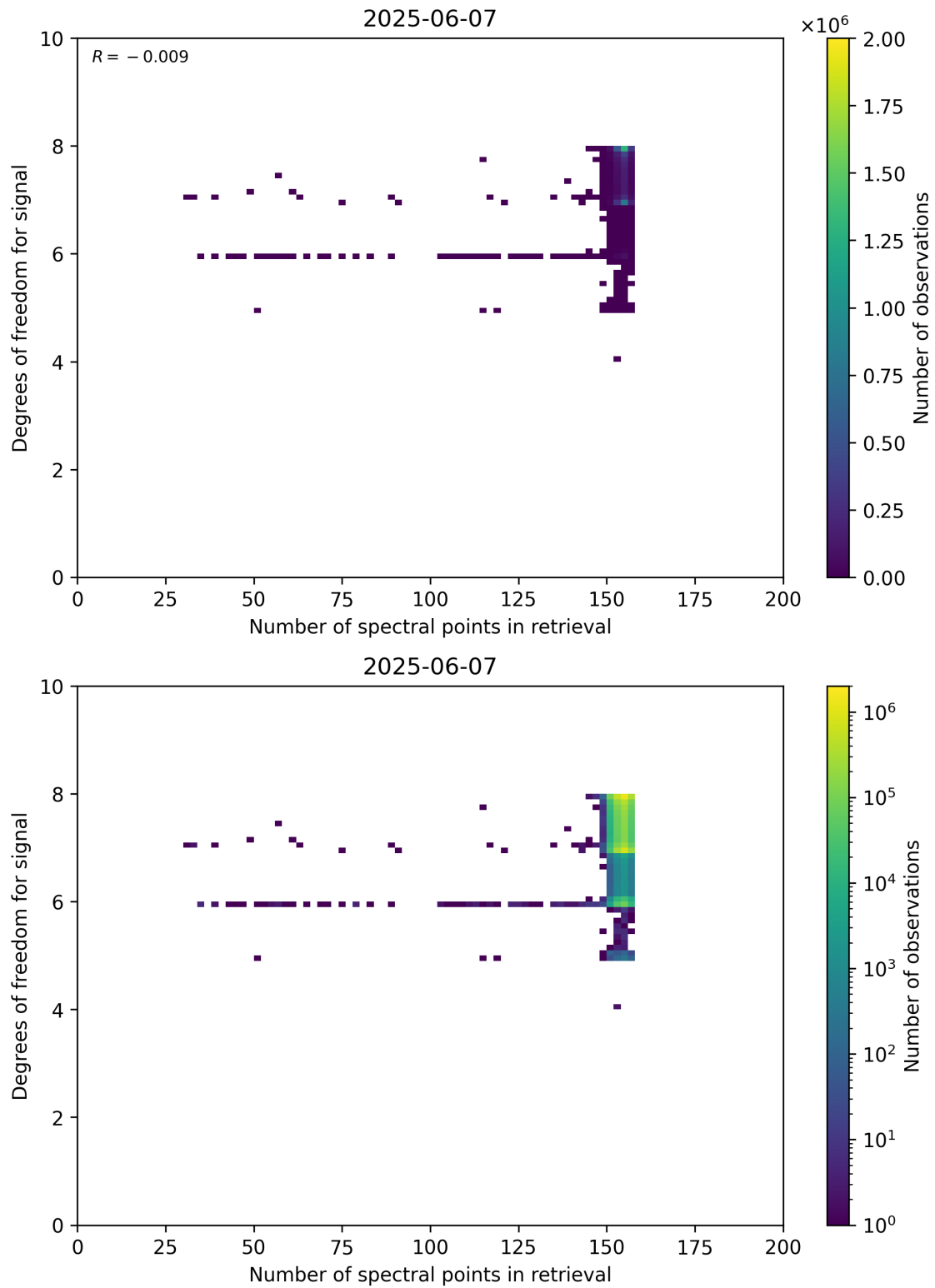
Figure 59: Scatter density plot of “Number of spectral points in retrieval” against “Degrees of freedom for signal” for 2025-06-06 to 2025-06-08.
