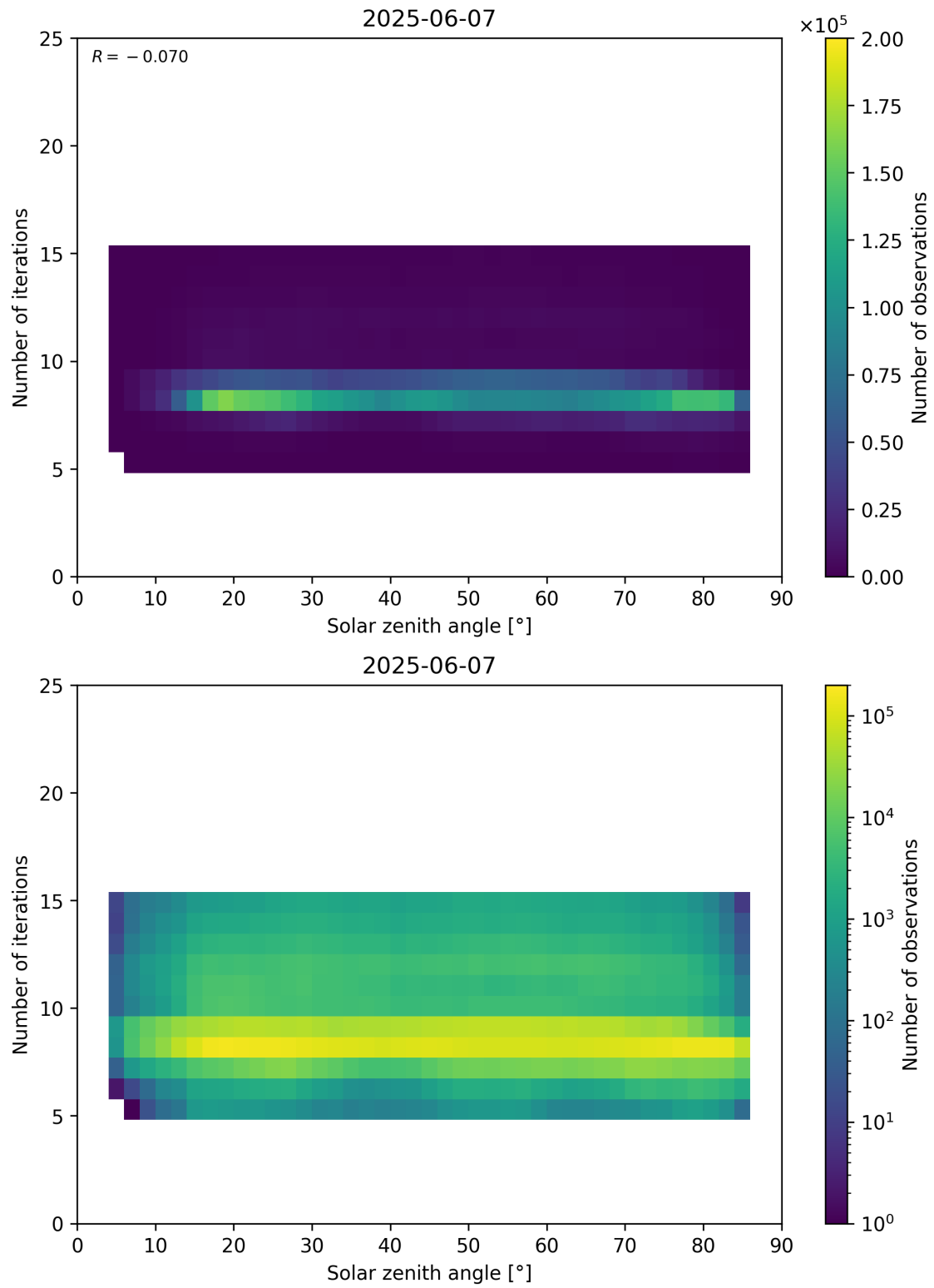
Figure 67: Scatter density plot of “Solar zenith angle” against “Number of iterations” for 2025-06-06 to 2025-06-08.
