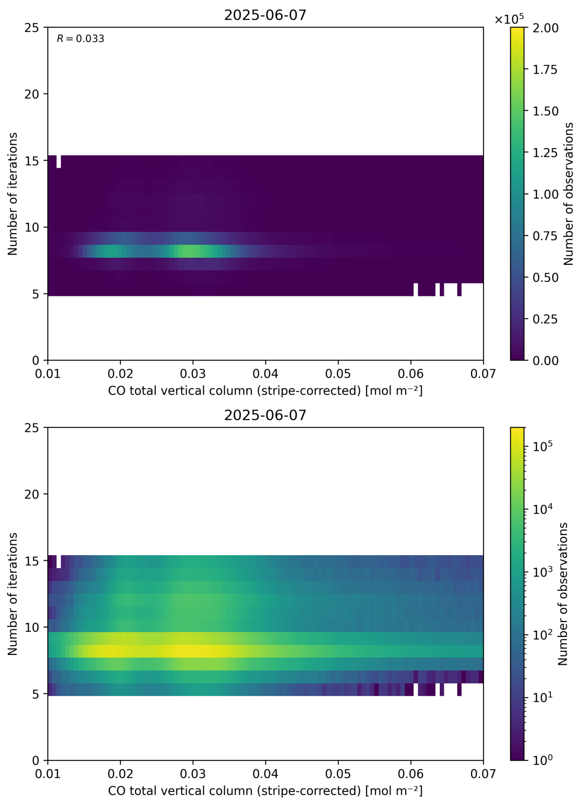
Figure 39: Scatter density plot of “CO total vertical column (stripe-corrected)” against “Number of iterations” for 2025-06-06 to 2025-06-08.
