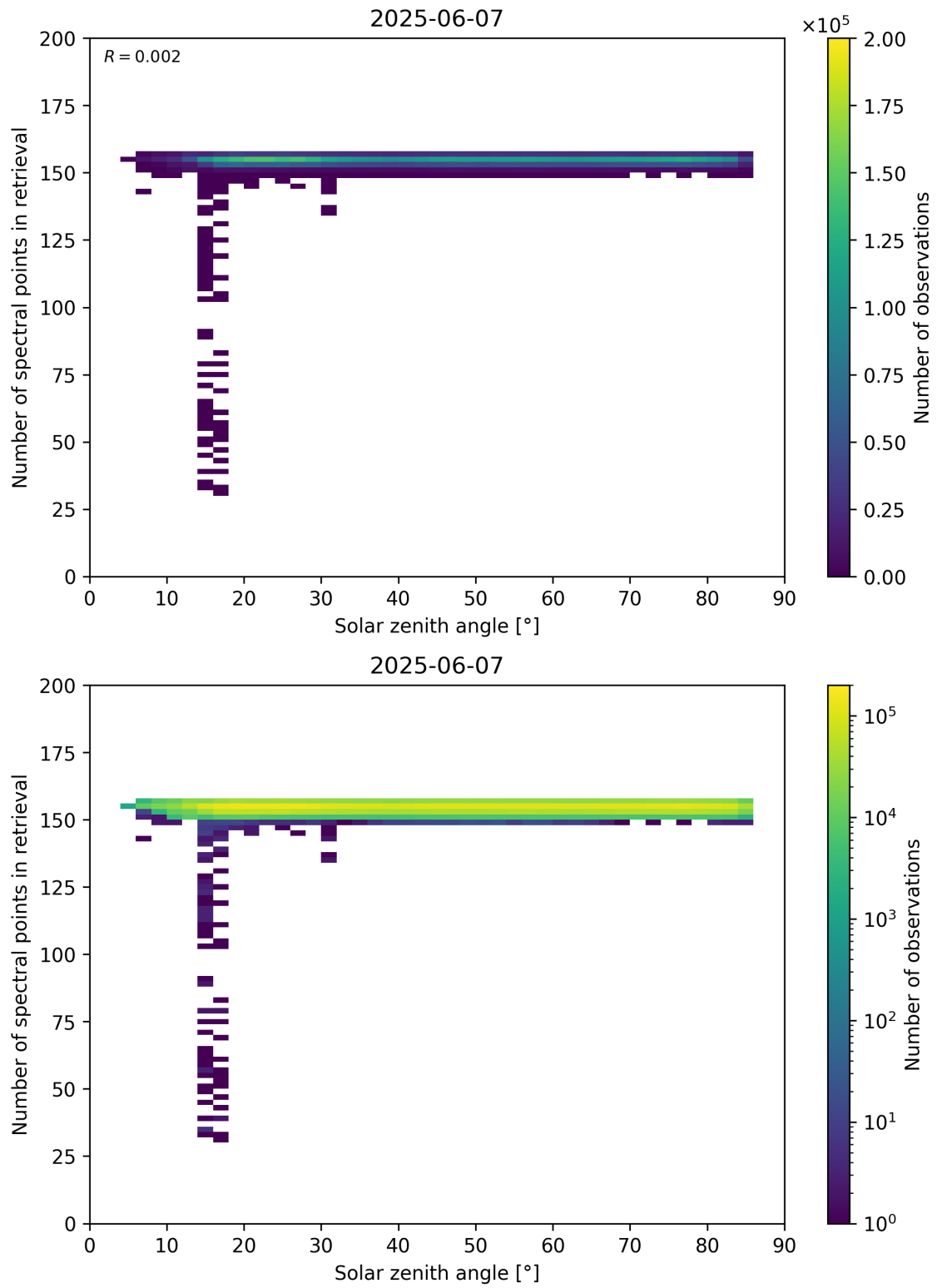
Figure 68: Scatter density plot of “Solar zenith angle” against “Number of spectral points in retrieval” for 2025-06-06 to 2025-06-08.
