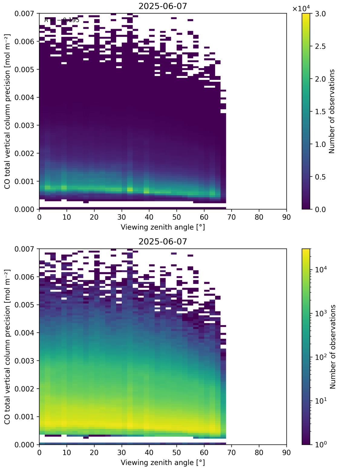
Figure 71: Scatter density plot of “Viewing zenith angle” against “CO total vertical column precision” for 2025-06-06 to 2025-06-08.
