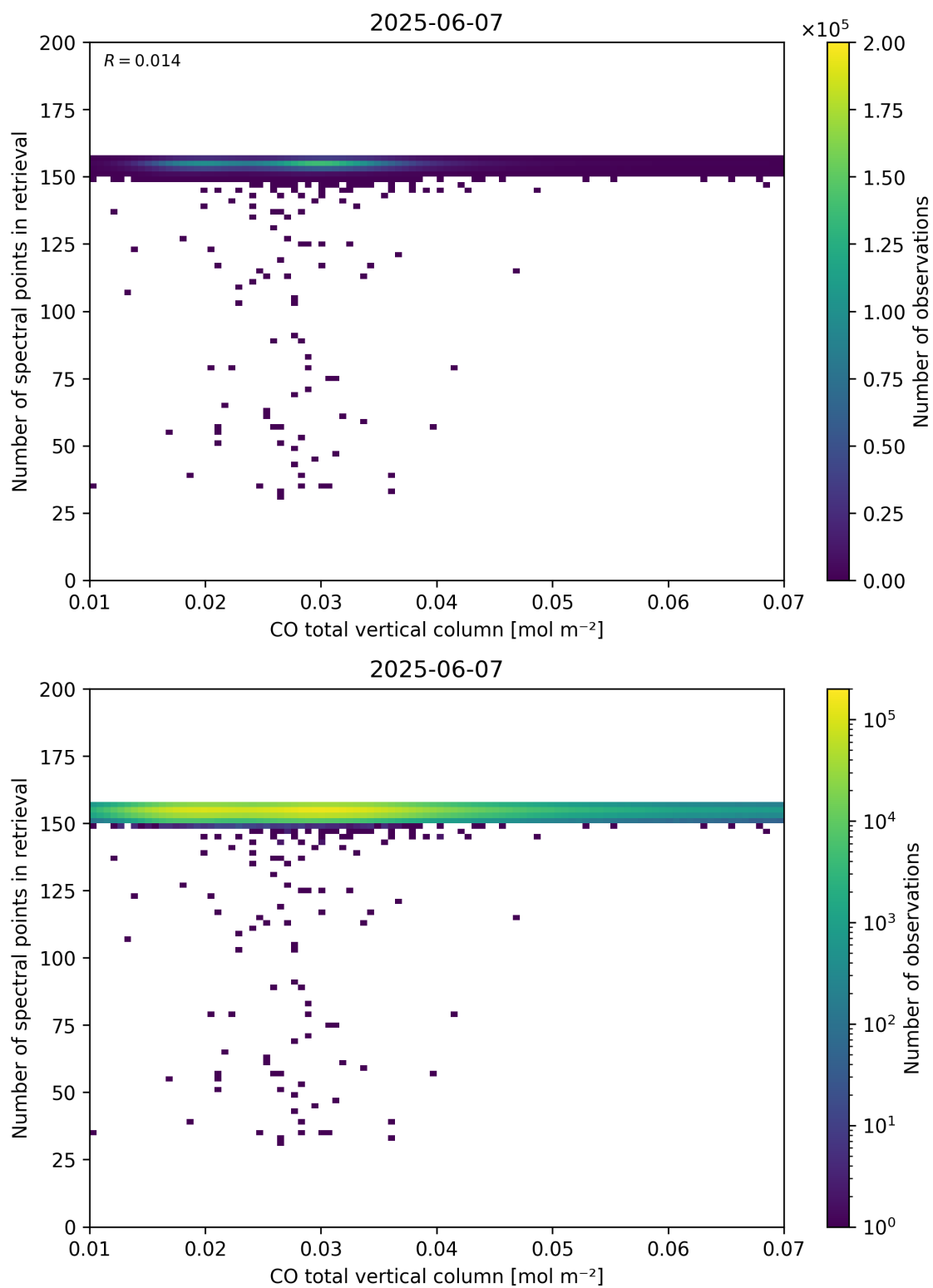
Figure 43: Scatter density plot of “CO total vertical column” against “Number of spectral points in retrieval” for 2025-06-06 to 2025-06-08.
