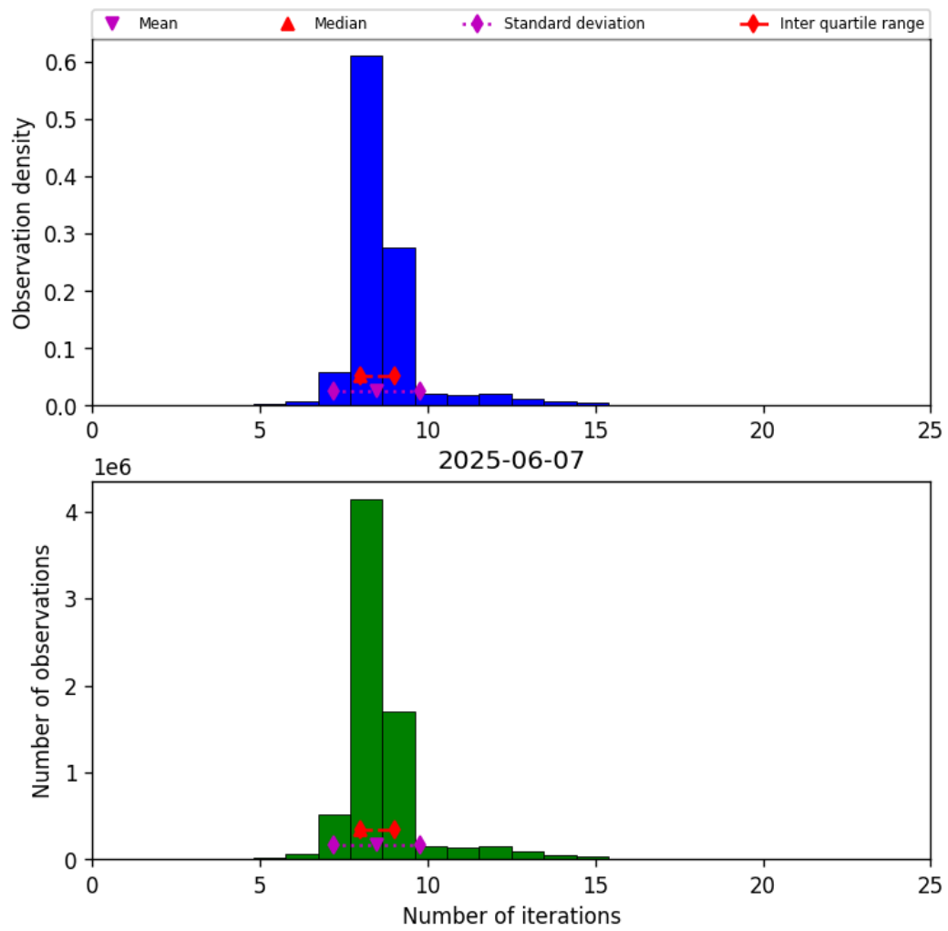
Figure 24: Histogram of “Number of iterations” for 2025-06-06 to 2025-06-08
