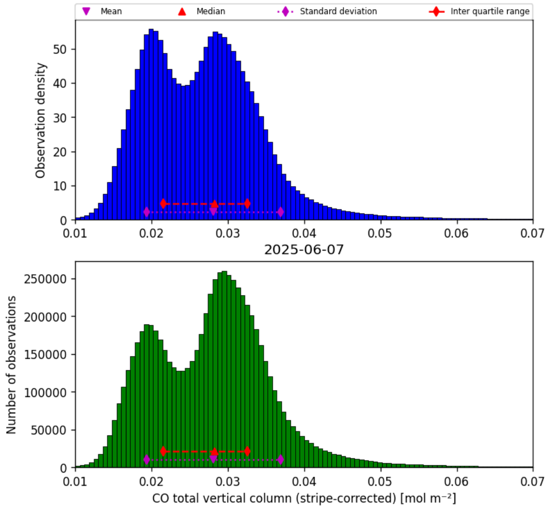
Figure 19: Histogram of “CO total vertical column (stripe-corrected)” for 2025-06-06 to 2025-06-08
