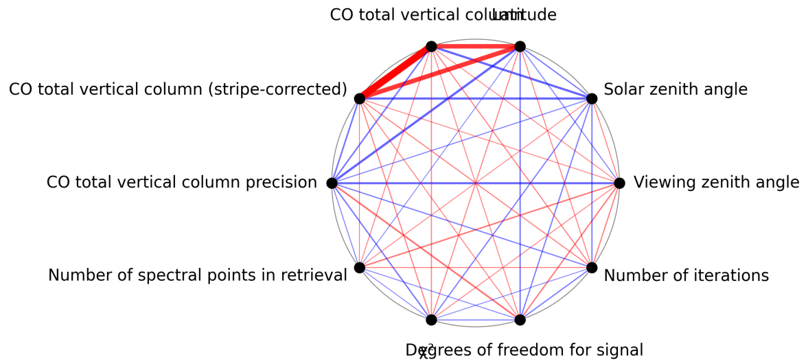
Figure 1: Map of correlation graph for 2025-06-06 to 2025-06-08.
