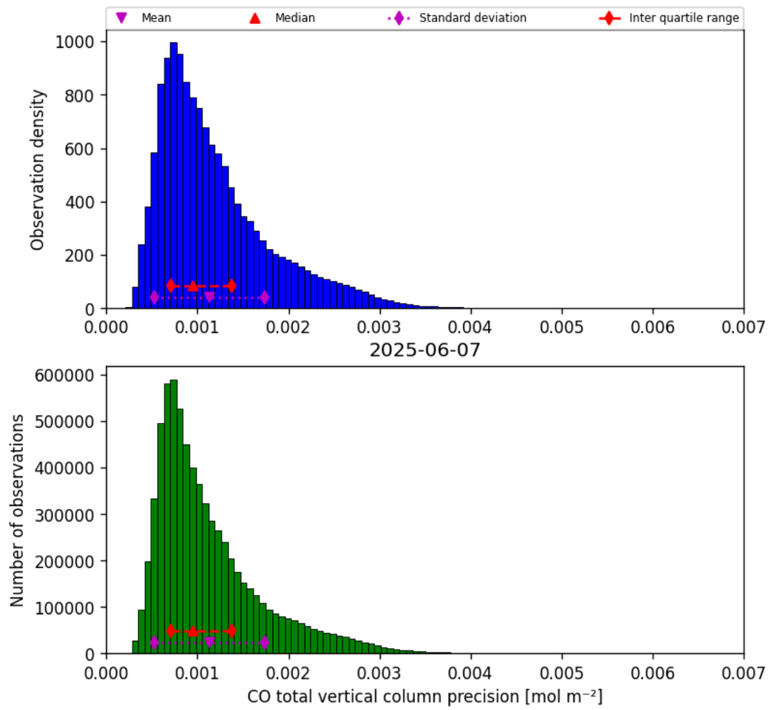
Figure 20: Histogram of “CO total vertical column precision” for 2025-06-06 to 2025-06-08
