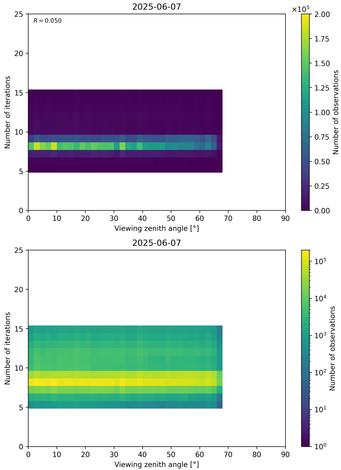
Figure 75: Scatter density plot of “Viewing zenith angle” against “Number of iterations” for 2025-06-06 to 2025-06-08.
