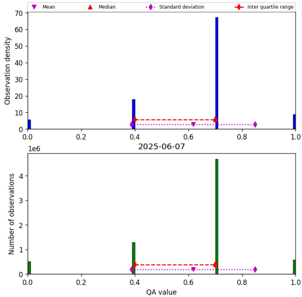
Figure 17: Histogram of “QA value” for 2025-06-06 to 2025-06-08
