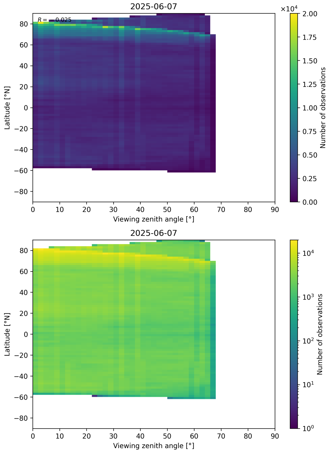
Figure 74: Scatter density plot of “Viewing zenith angle” against “Latitude” for 2025-06-06 to 2025-06-08.
