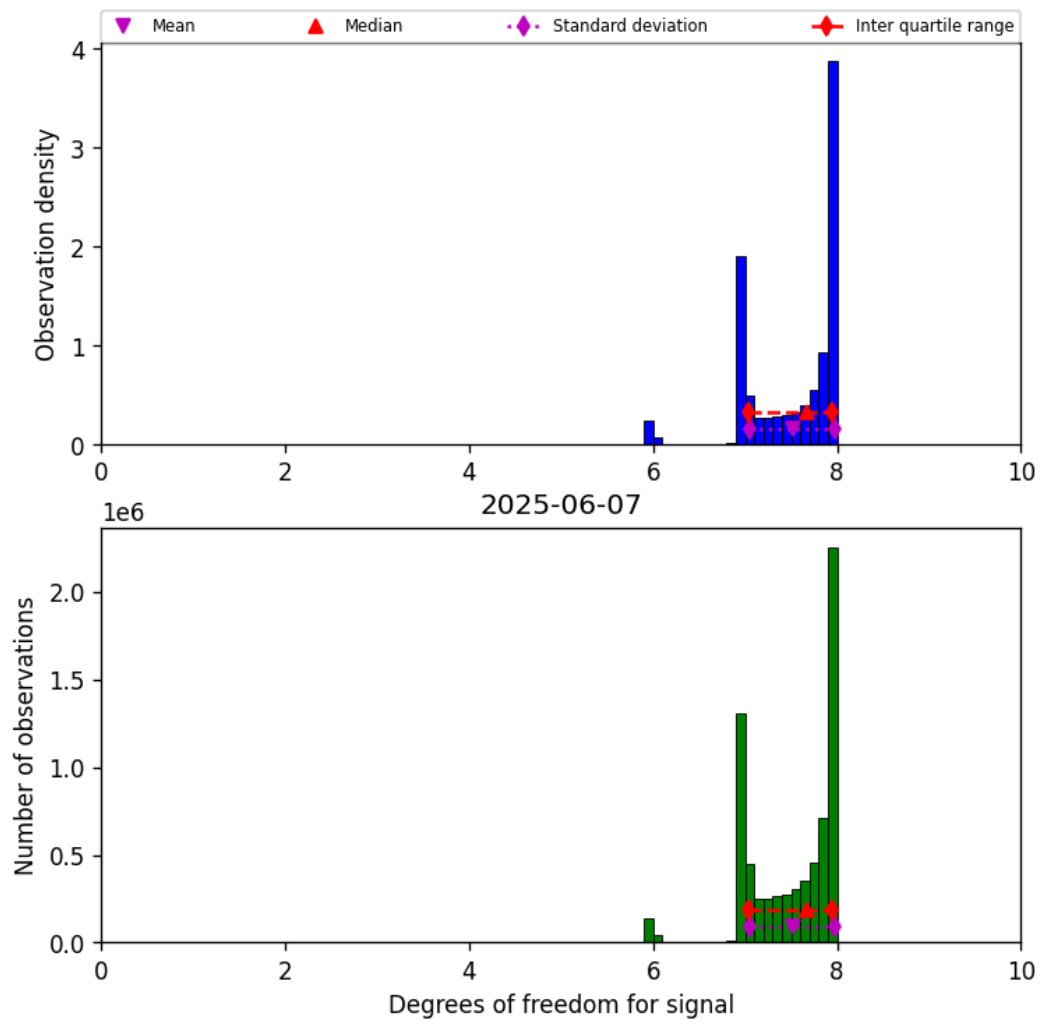
Figure 23: Histogram of “Degrees of freedom for signal” for 2025-06-06 to 2025-06-08
