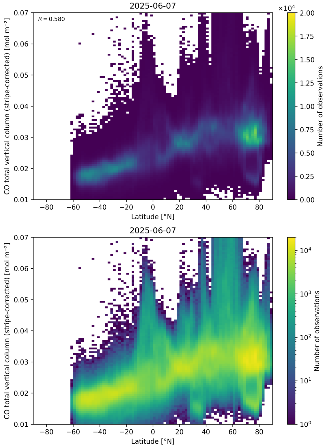
Figure 52: Scatter density plot of “Latitude” against “CO total vertical column (stripe-corrected)” for 2025-06-06 to 2025-06-08.
