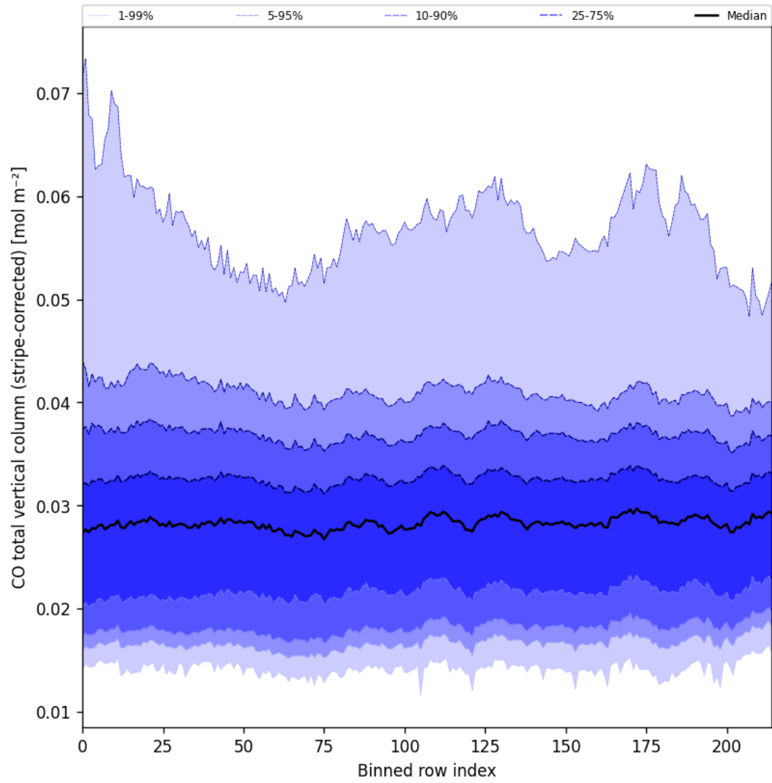
Figure 27: Along track statistics of “CO total vertical column (stripe-corrected)” for 2025-06-06 to 2025-06-08
