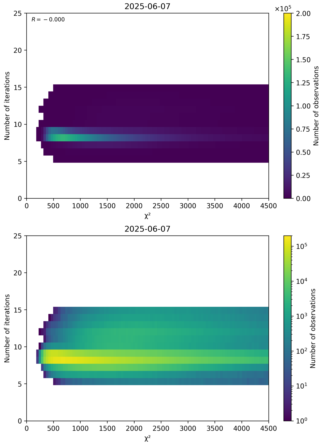
Figure 49: Scatter density plot of “ \chi^2 ” against “Number of iterations” for 2025-06-06 to 2025-06-08.
