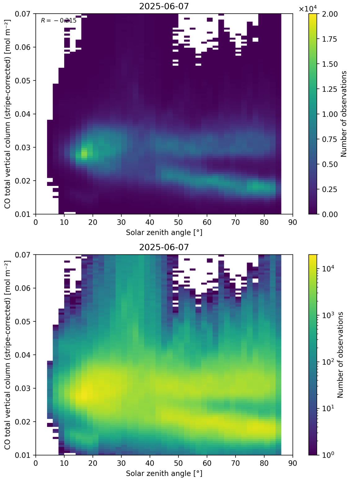
Figure 62: Scatter density plot of “Solar zenith angle” against “CO total vertical column (stripe-corrected)” for 2025-06-06 to 2025-06-08.
