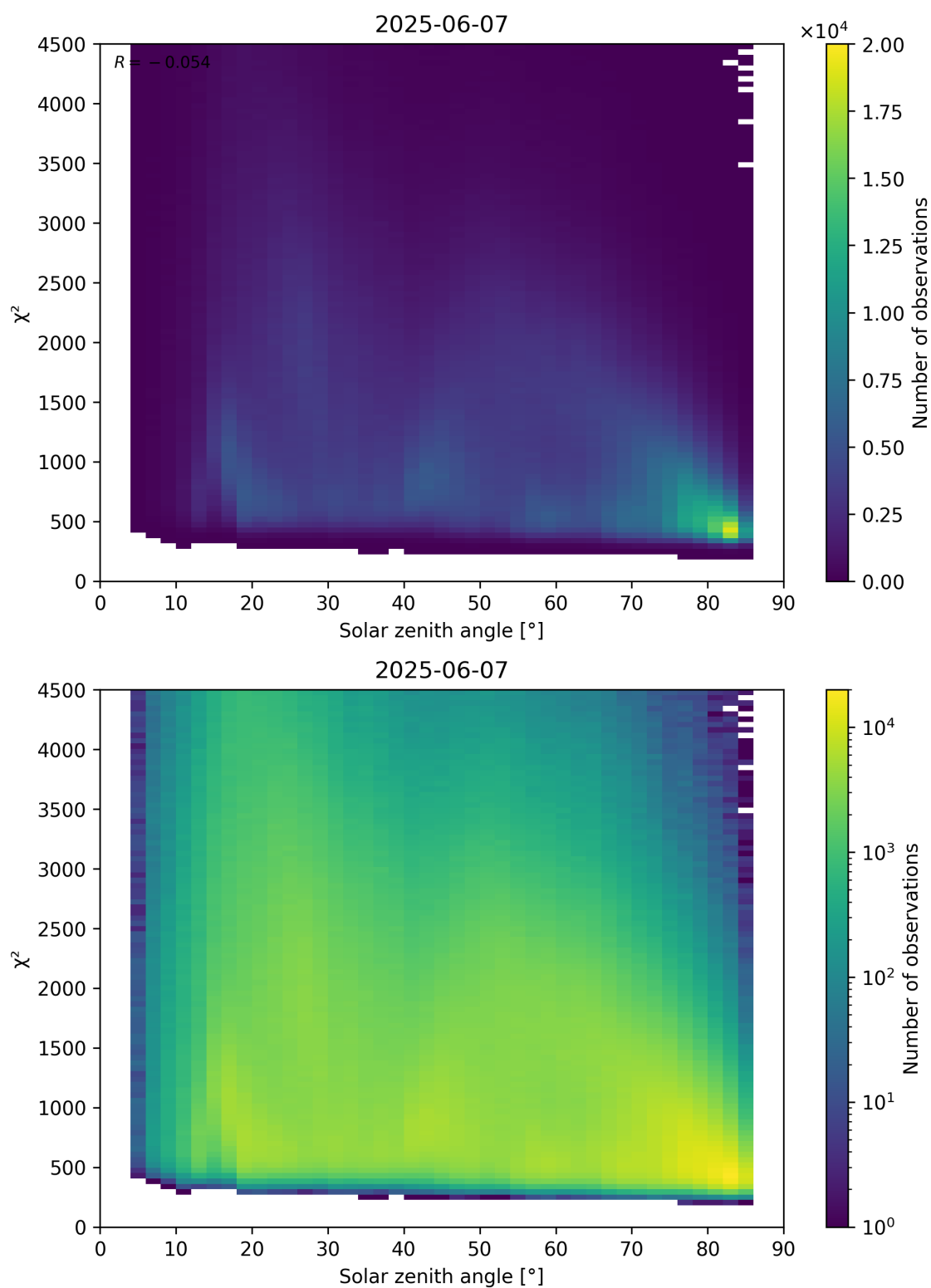
Figure 64: Scatter density plot of “Solar zenith angle” against “ \chi^2 ” for 2025-06-06 to 2025-06-08.
