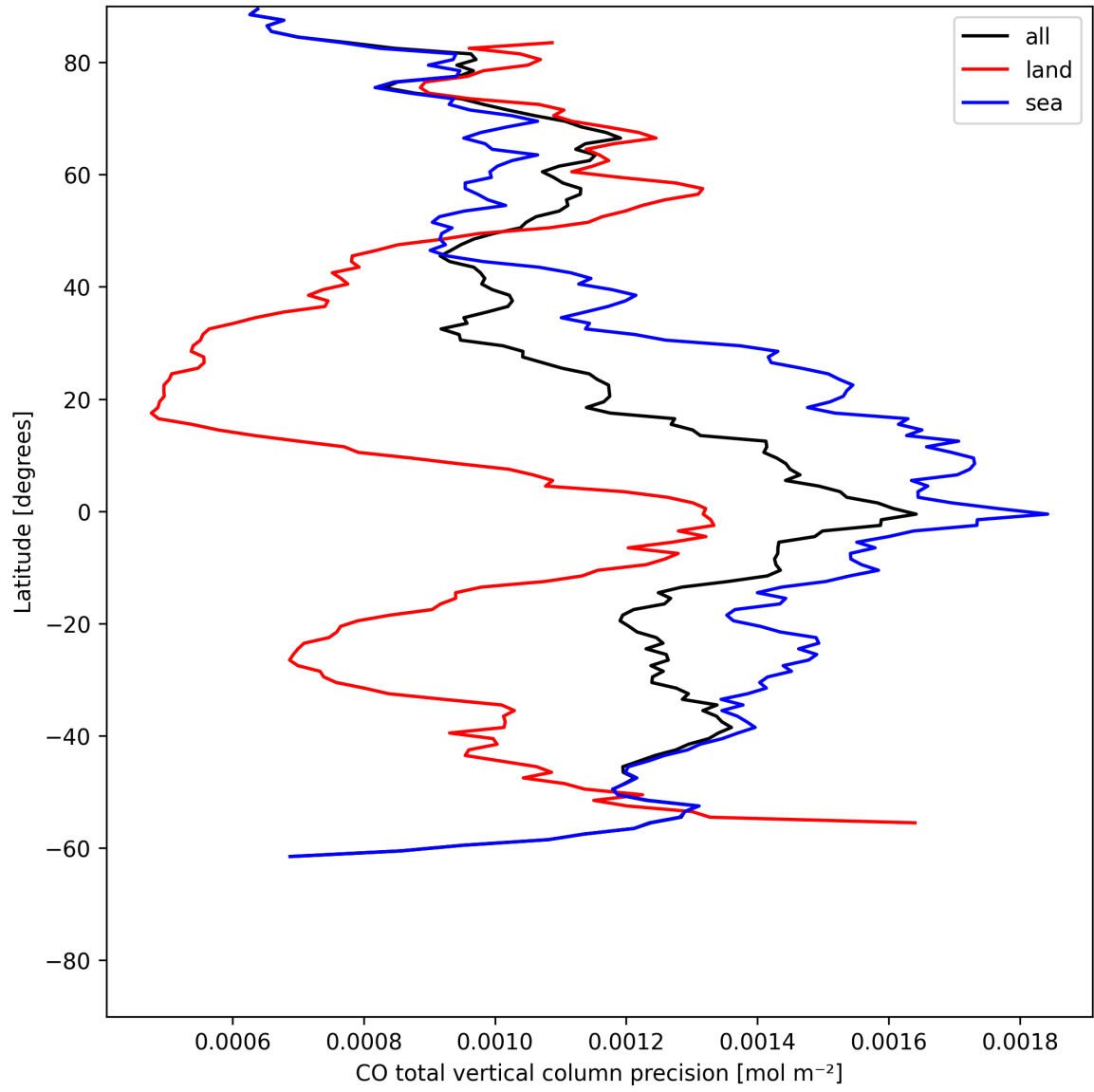
Figure 12: Zonal average of “CO total vertical column precision” for 2025-06-06 to 2025-06-08.
