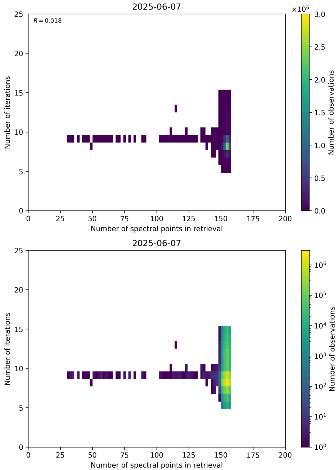
Figure 60: Scatter density plot of “Number of spectral points in retrieval” against “Number of iterations” for 2025-06-06 to 2025-06-08.
