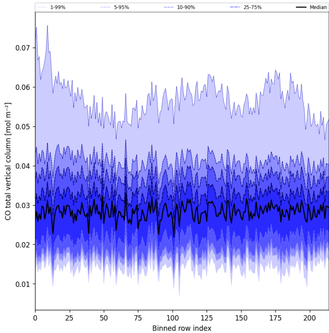
Figure 26: Along track statistics of “CO total vertical column” for 2025-06-06 to 2025-06-08
