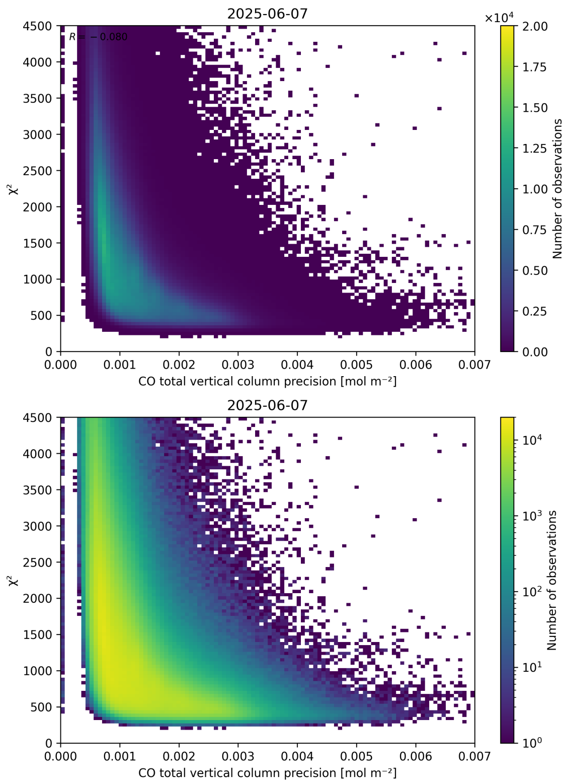
Figure 44: Scatter density plot of “CO total vertical column precision” against “ \chi^2 ” for 2025-06-06 to 2025-06-08.
