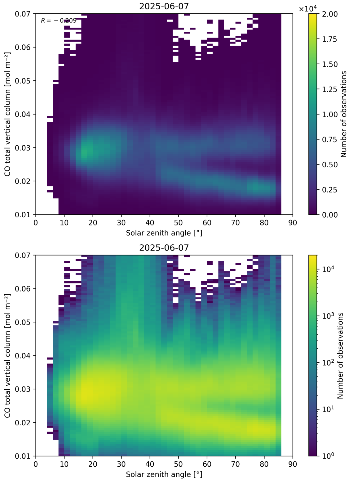
Figure 61: Scatter density plot of “Solar zenith angle” against “CO total vertical column” for 2025-06-06 to 2025-06-08.
