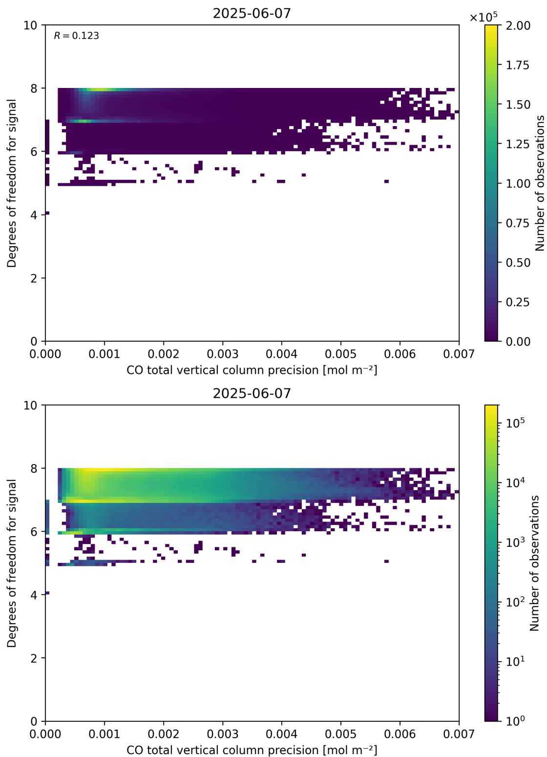
Figure 45: Scatter density plot of “CO total vertical column precision” against “Degrees of freedom for signal” for 2025-06-06 to 2025-06-08.
