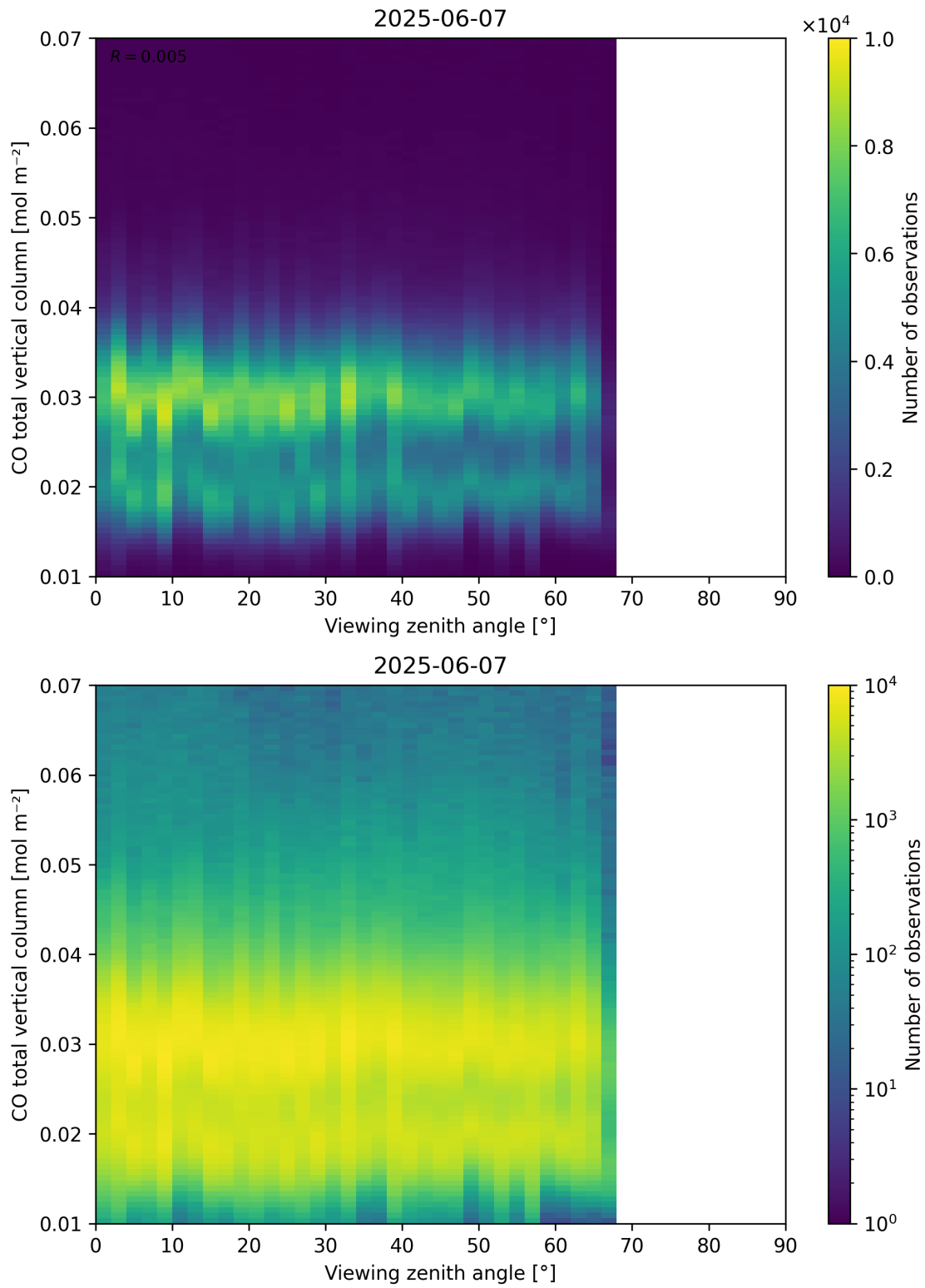
Figure 69: Scatter density plot of “Viewing zenith angle” against “CO total vertical column” for 2025-06-06 to 2025-06-08.
