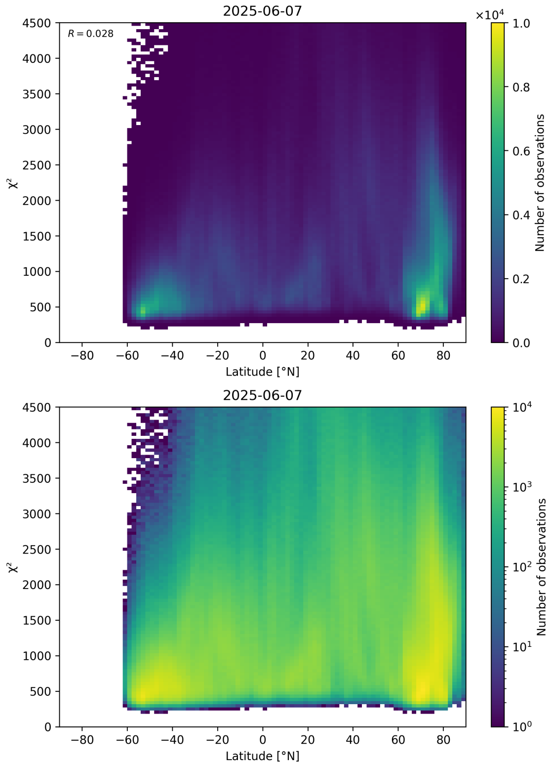
Figure 54: Scatter density plot of “Latitude” against “ \chi^2 ” for 2025-06-06 to 2025-06-08.
