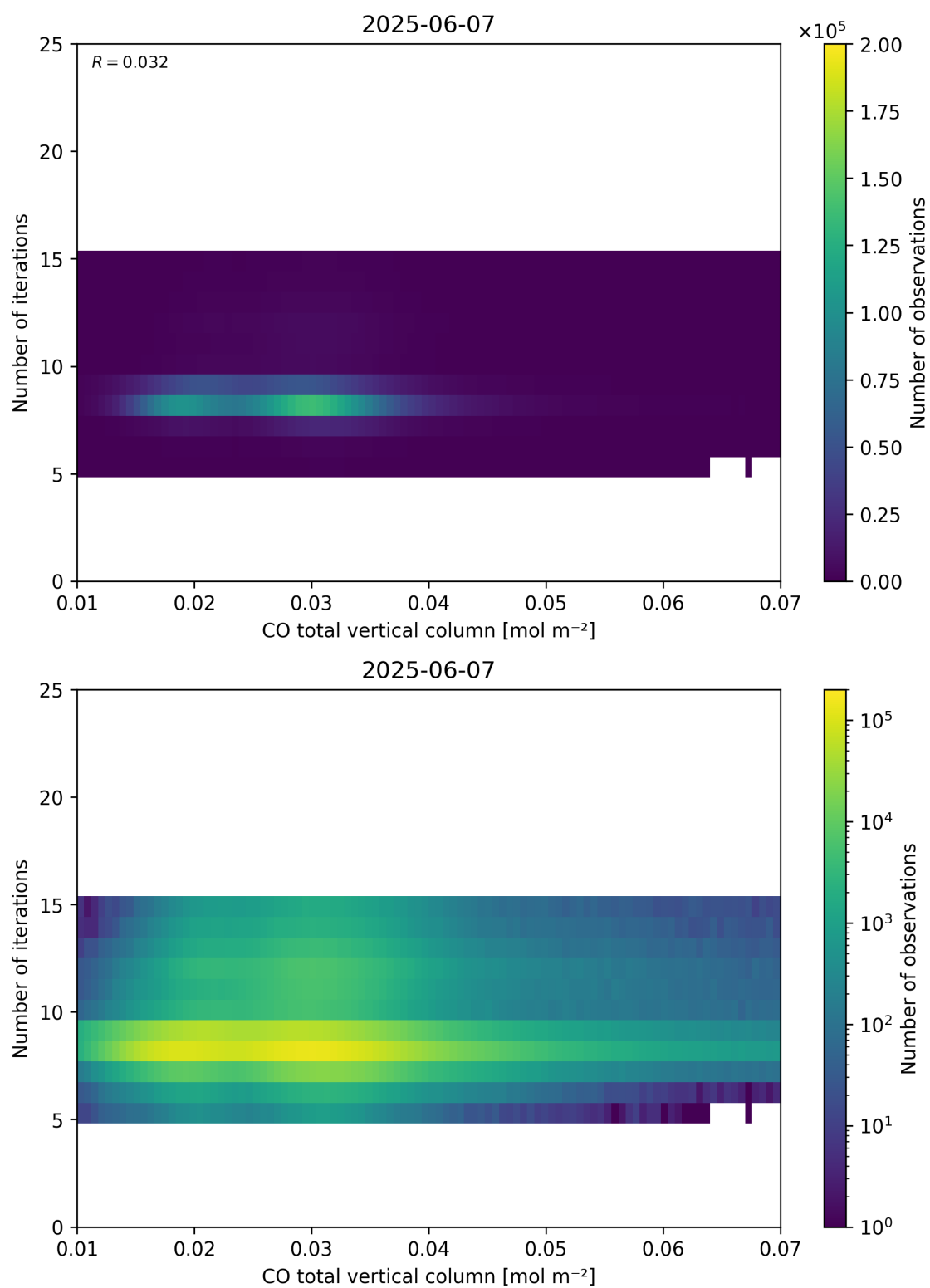
Figure 42: Scatter density plot of “CO total vertical column” against “Number of iterations” for 2025-06-06 to 2025-06-08.
