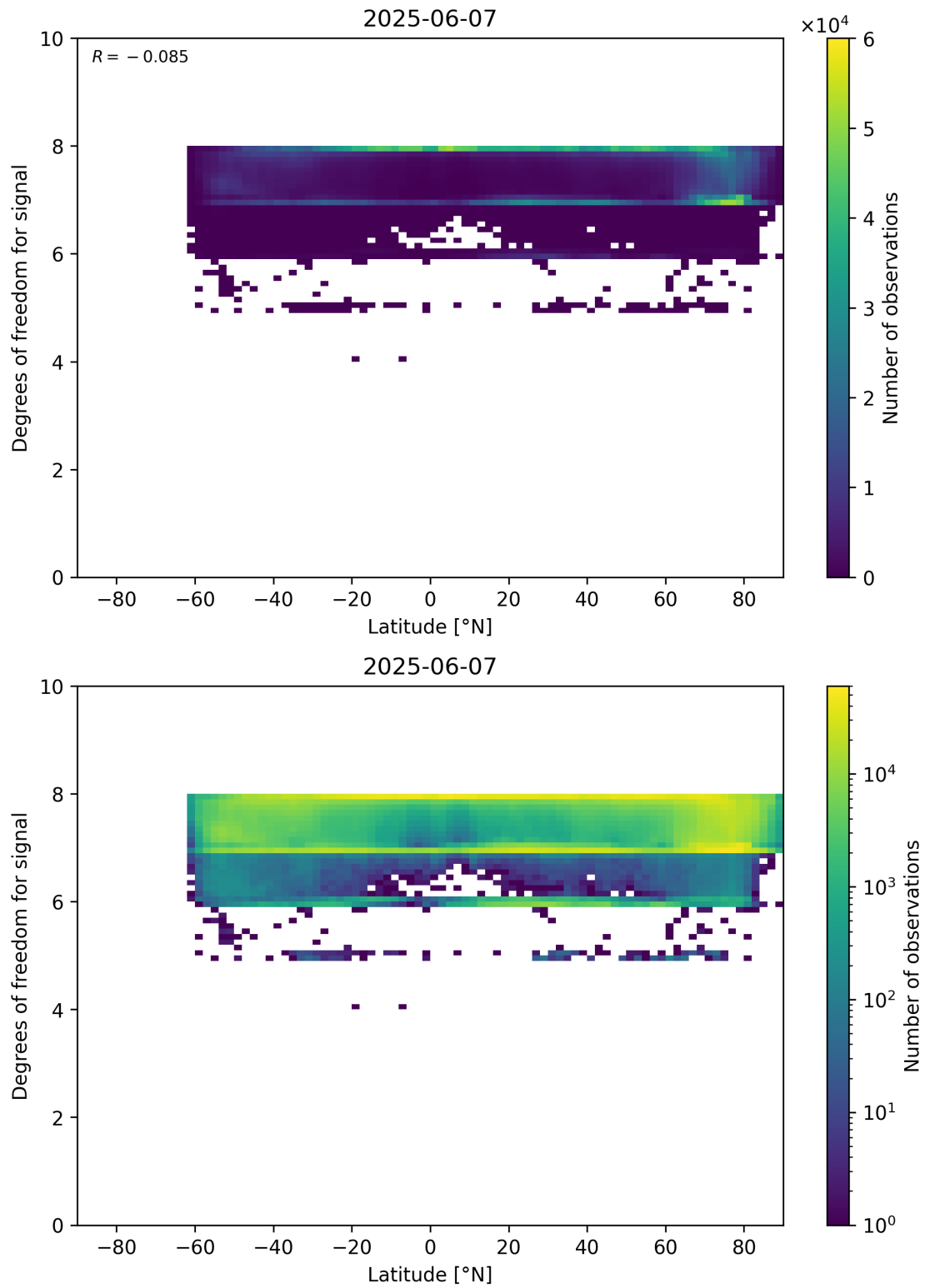
Figure 55: Scatter density plot of “Latitude” against “Degrees of freedom for signal” for 2025-06-06 to 2025-06-08.
