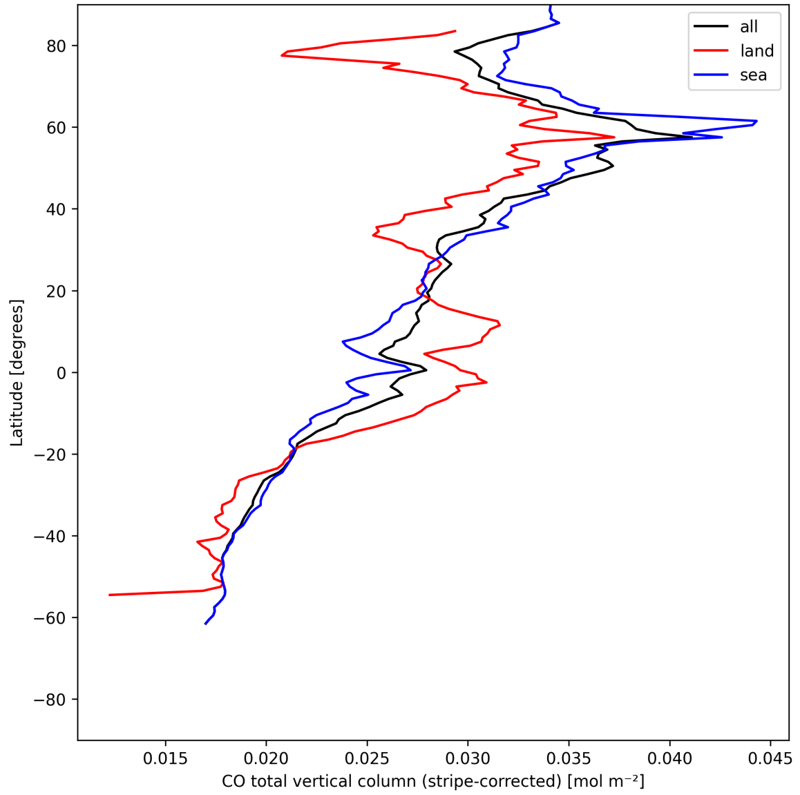
Figure 11: Zonal average of “CO total vertical column (stripe-corrected)” for 2025-06-07 to 2025-06-09.
