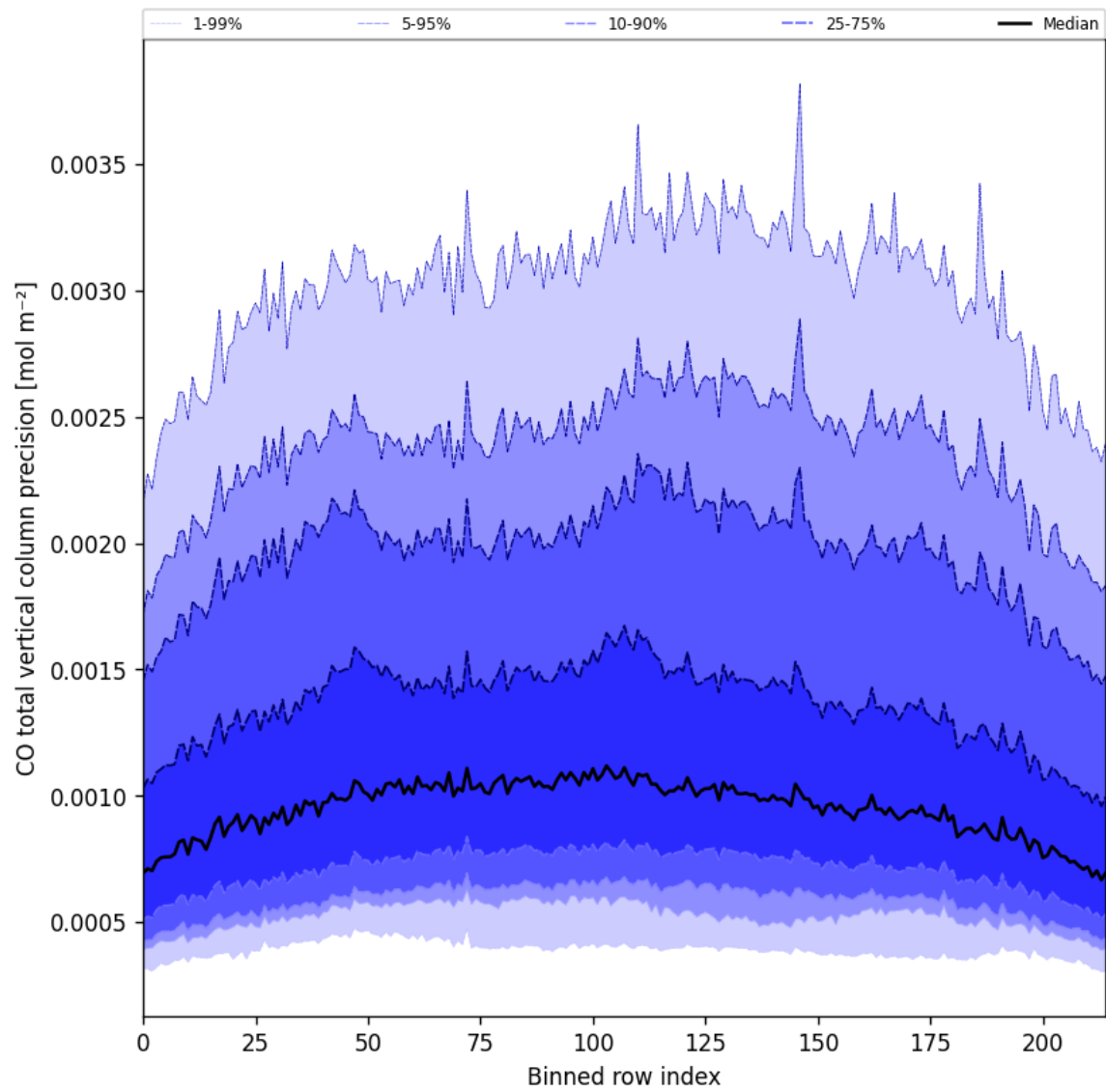
Figure 28: Along track statistics of "CO total vertical column precision" for 2025-06-07 to 2025-06-09
