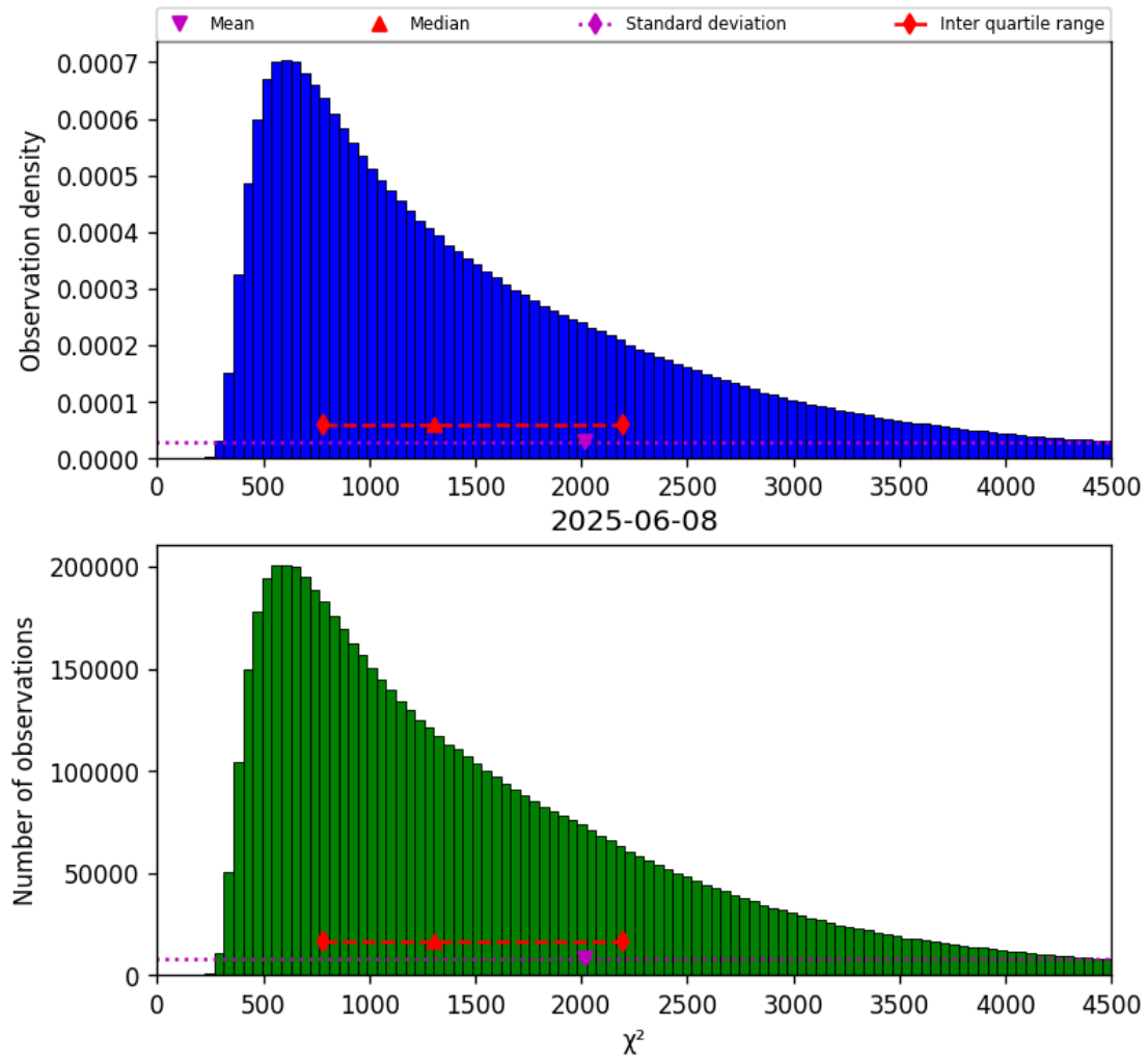
Figure 22: Histogram of “ \chi^2 ” for 2025-06-07 to 2025-06-09
