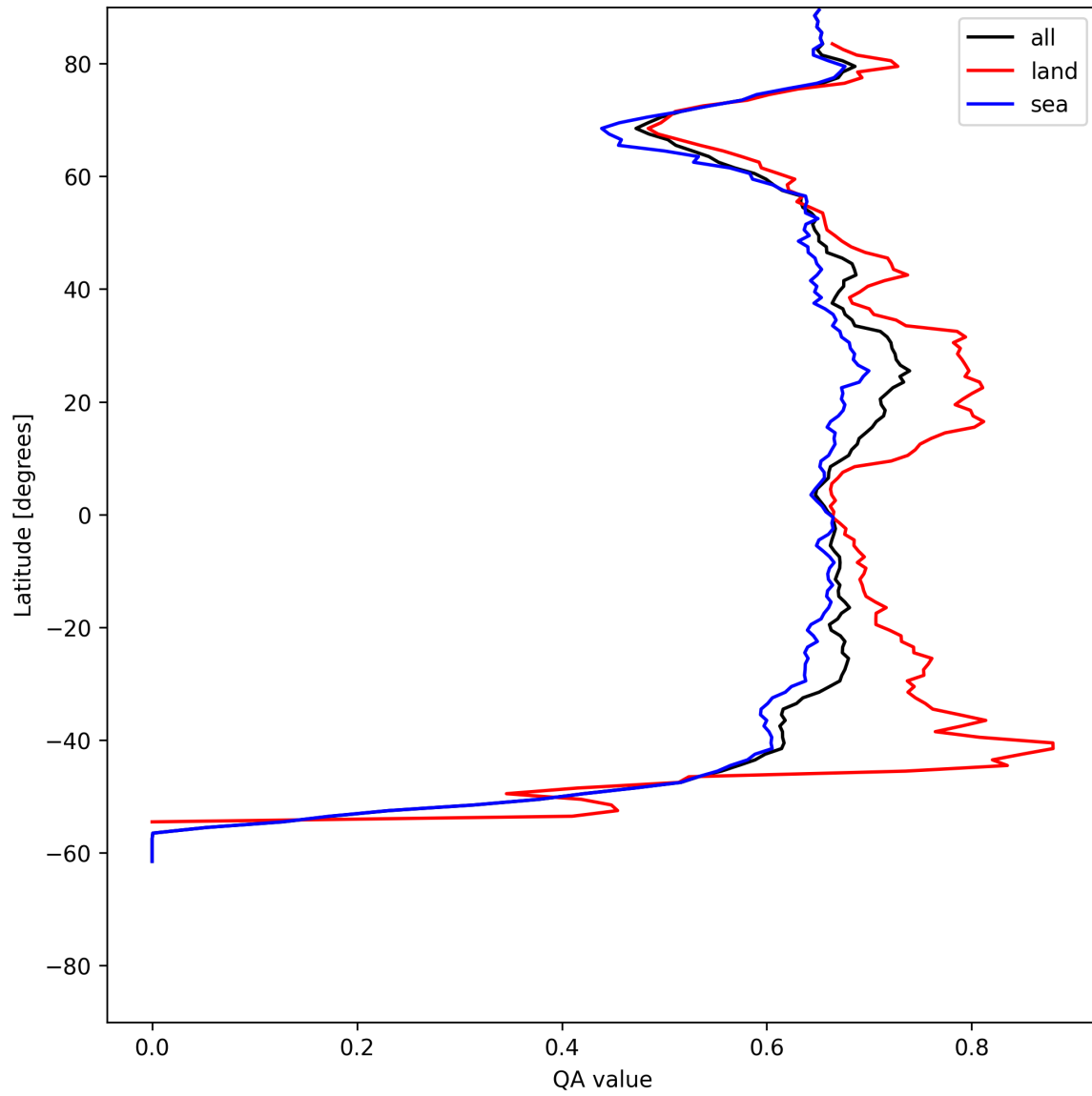
Figure 9: Zonal average of “QA value” for 2025-06-07 to 2025-06-09.
