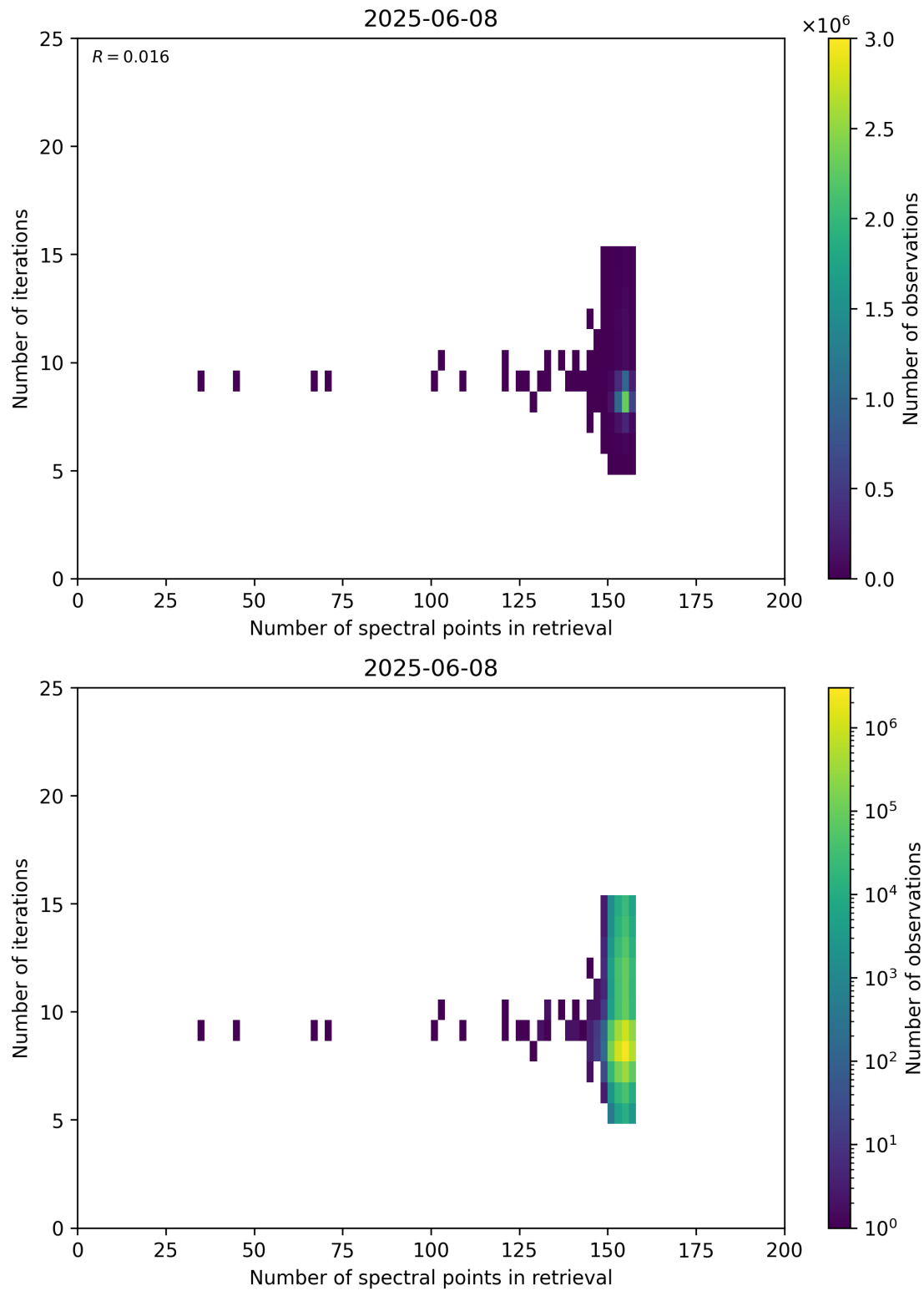
Figure 60: Scatter density plot of “Number of spectral points in retrieval” against “Number of iterations” for 2025-06-07 to 2025-06-09.
