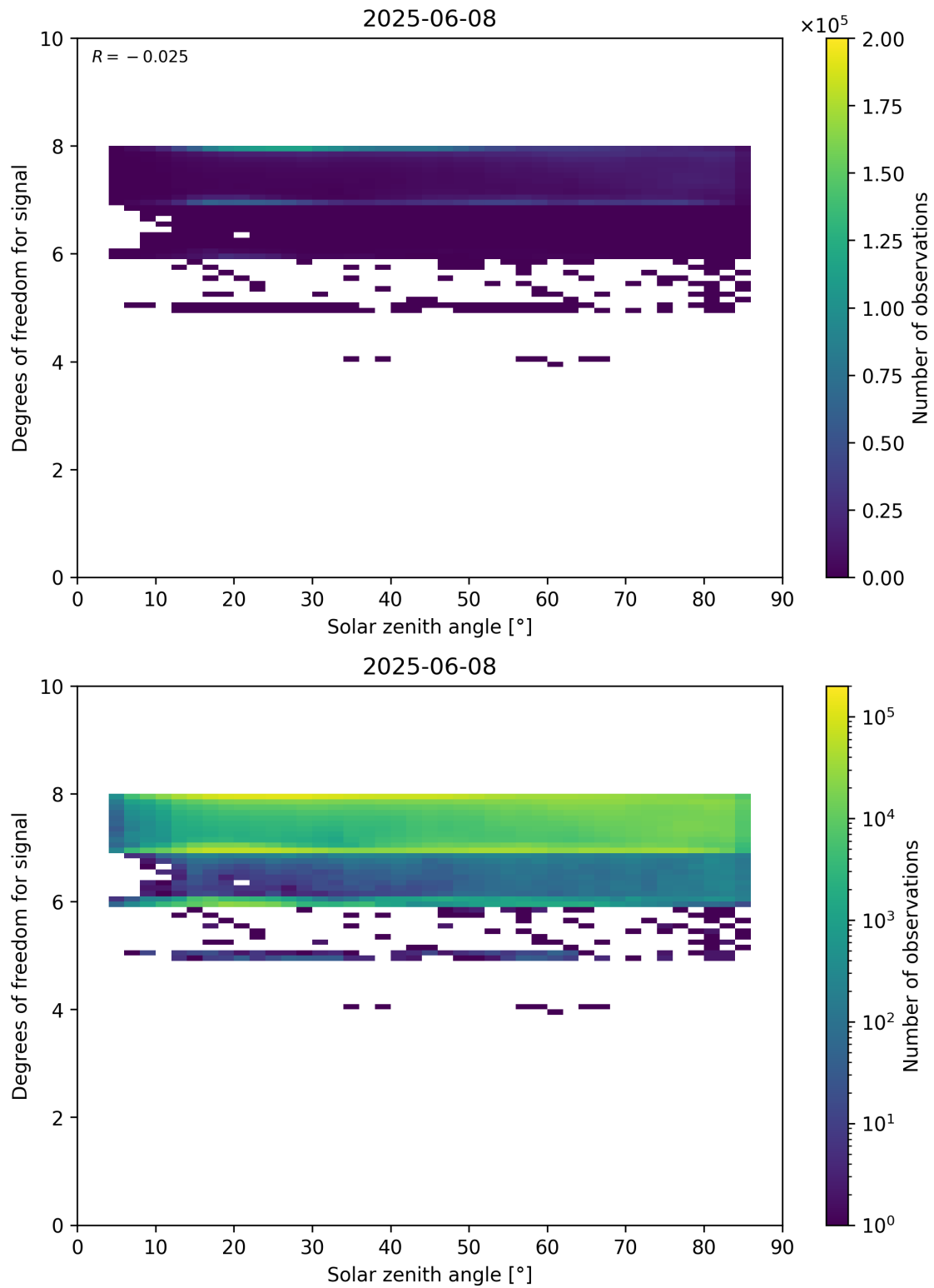
Figure 65: Scatter density plot of “Solar zenith angle” against “Degrees of freedom for signal” for 2025-06-07 to 2025-06-09.
