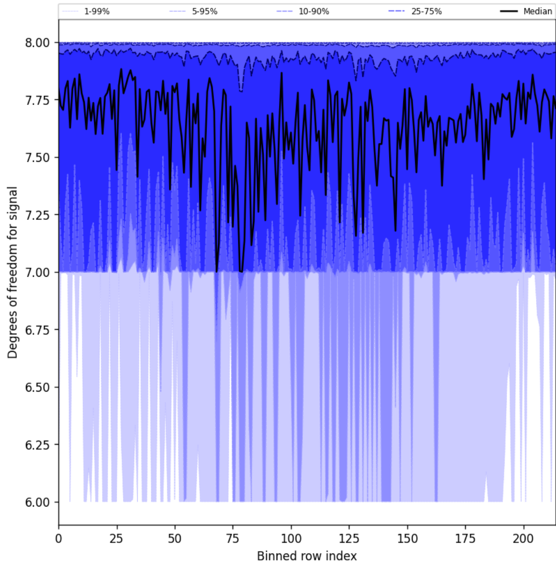
Figure 31: Along track statistics of “Degrees of freedom for signal” for 2025-06-07 to 2025-06-09
