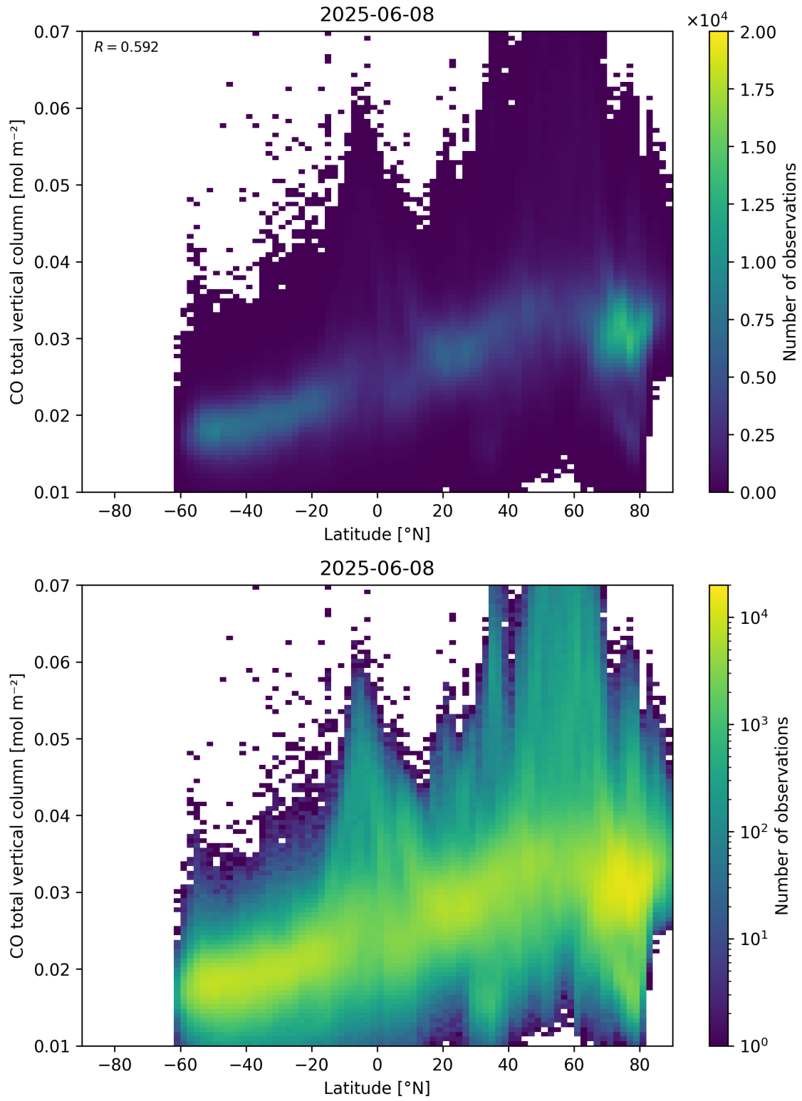
Figure 51: Scatter density plot of “Latitude” against “CO total vertical column” for 2025-06-07 to 2025-06-09.
