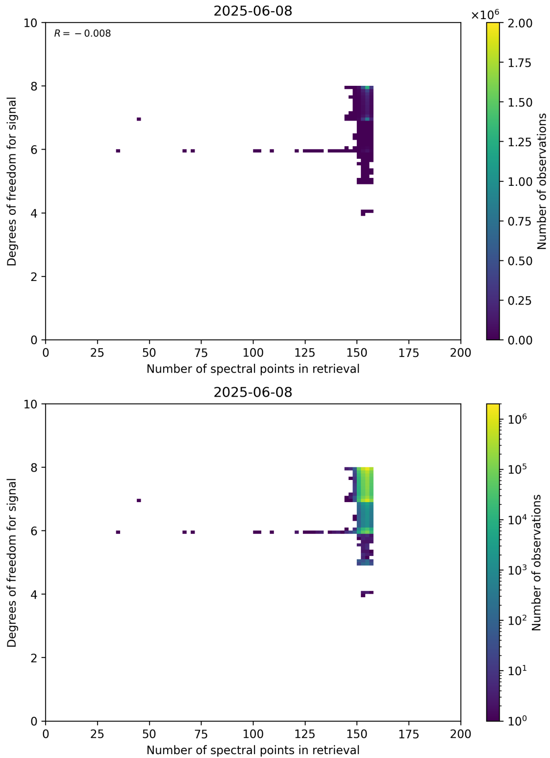
Figure 59: Scatter density plot of “Number of spectral points in retrieval” against “Degrees of freedom for signal” for 2025-06-07 to 2025-06-09.
