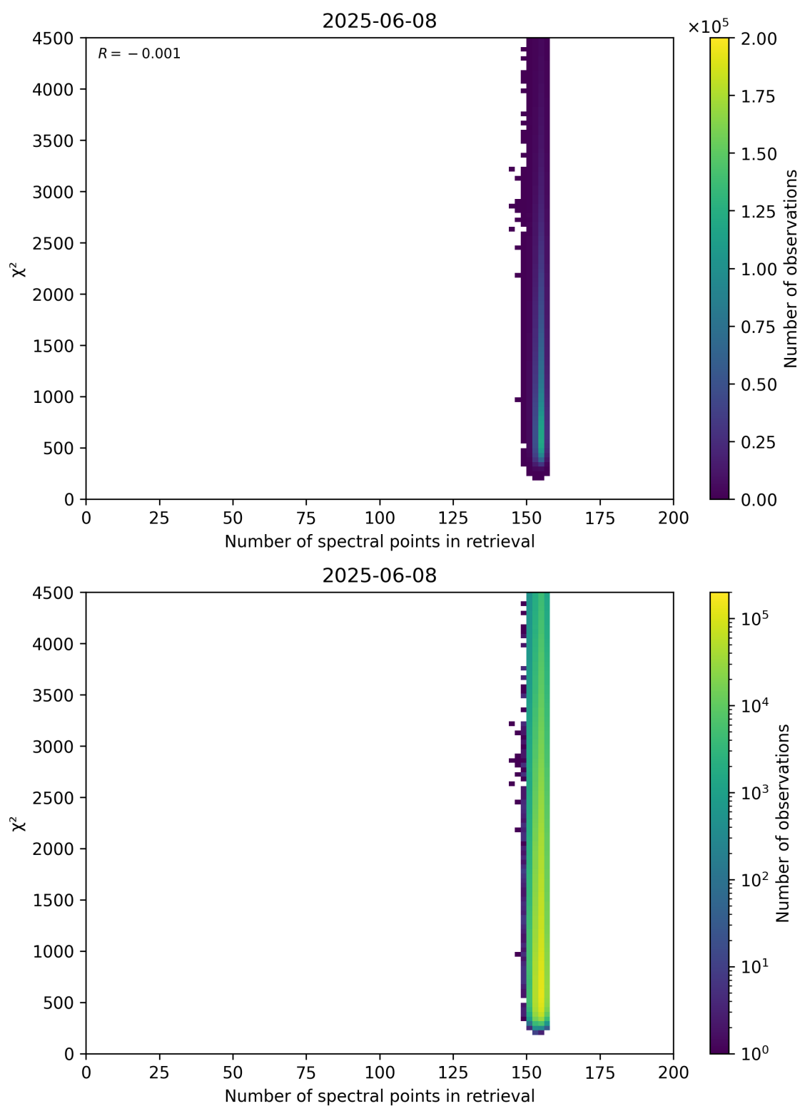
Figure 58: Scatter density plot of “Number of spectral points in retrieval” against “ \chi^2 ” for 2025-06-07 to 2025-06-09.
