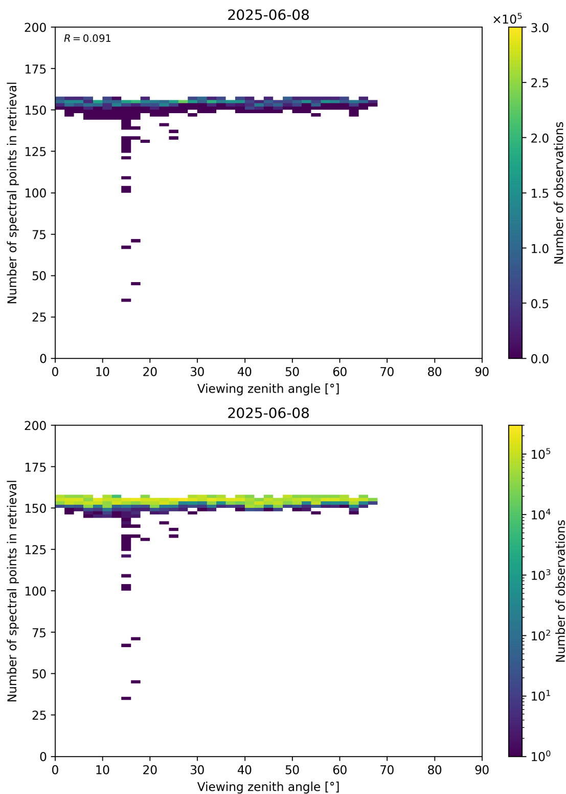
Figure 76: Scatter density plot of “Viewing zenith angle” against “Number of spectral points in retrieval” for 2025-06-07 to 2025-06-09.
