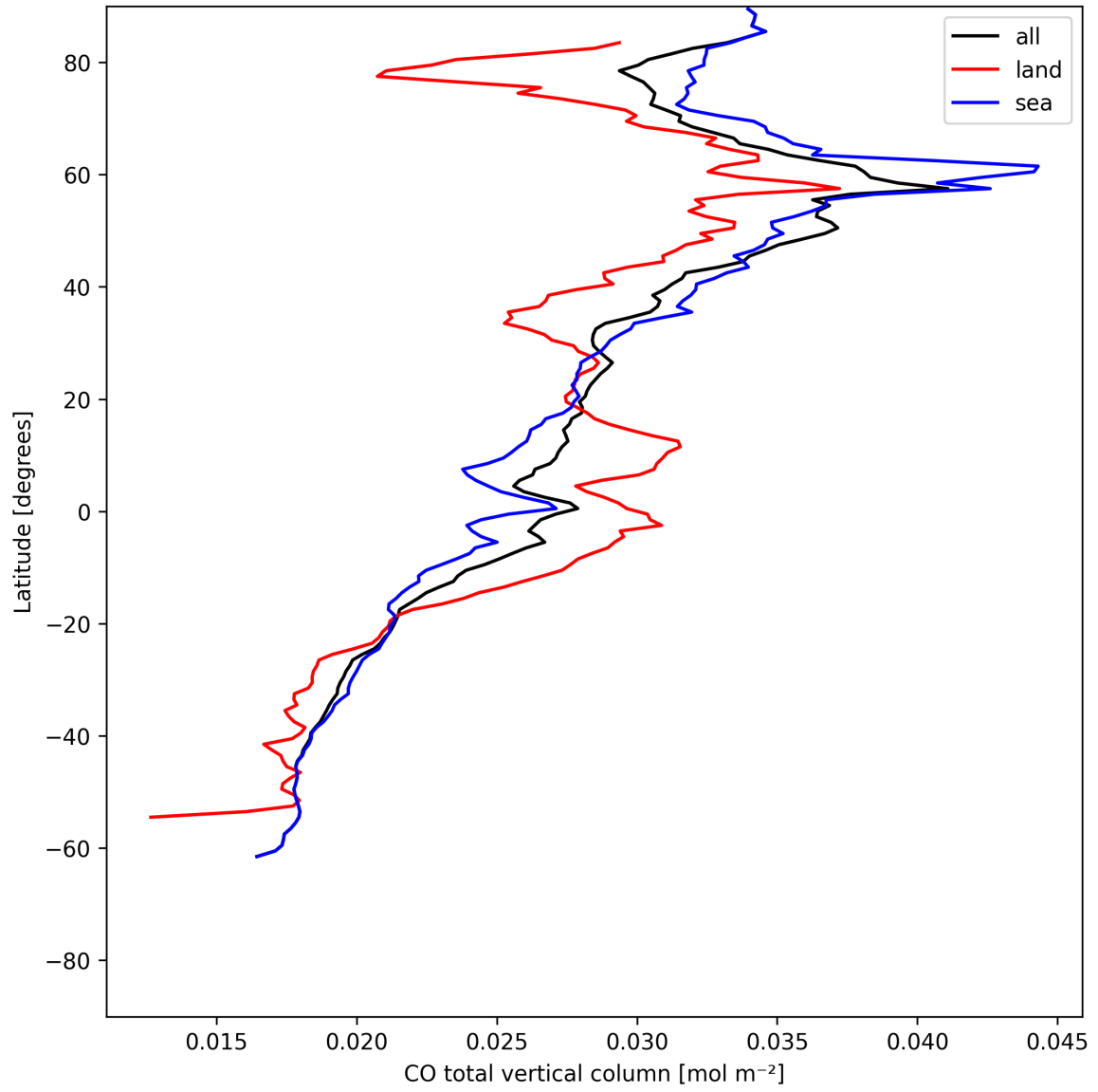
Figure 10: Zonal average of “CO total vertical column” for 2025-06-07 to 2025-06-09.
