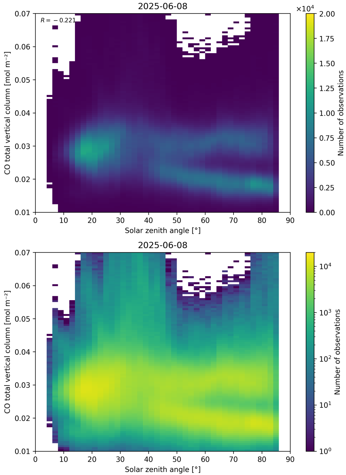
Figure 61: Scatter density plot of “Solar zenith angle” against “CO total vertical column” for 2025-06-07 to 2025-06-09.
