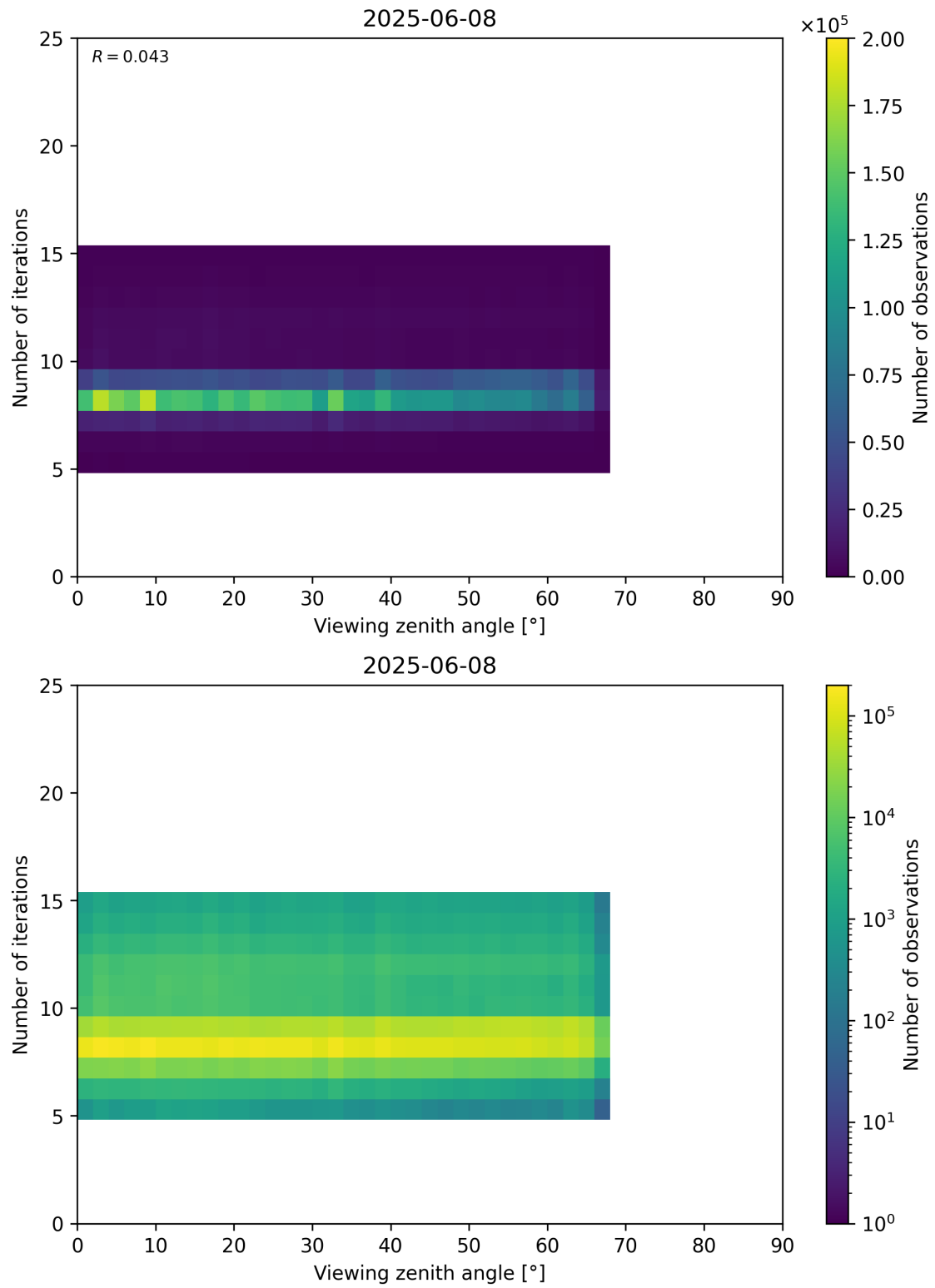
Figure 75: Scatter density plot of “Viewing zenith angle” against “Number of iterations” for 2025-06-07 to 2025-06-09.
