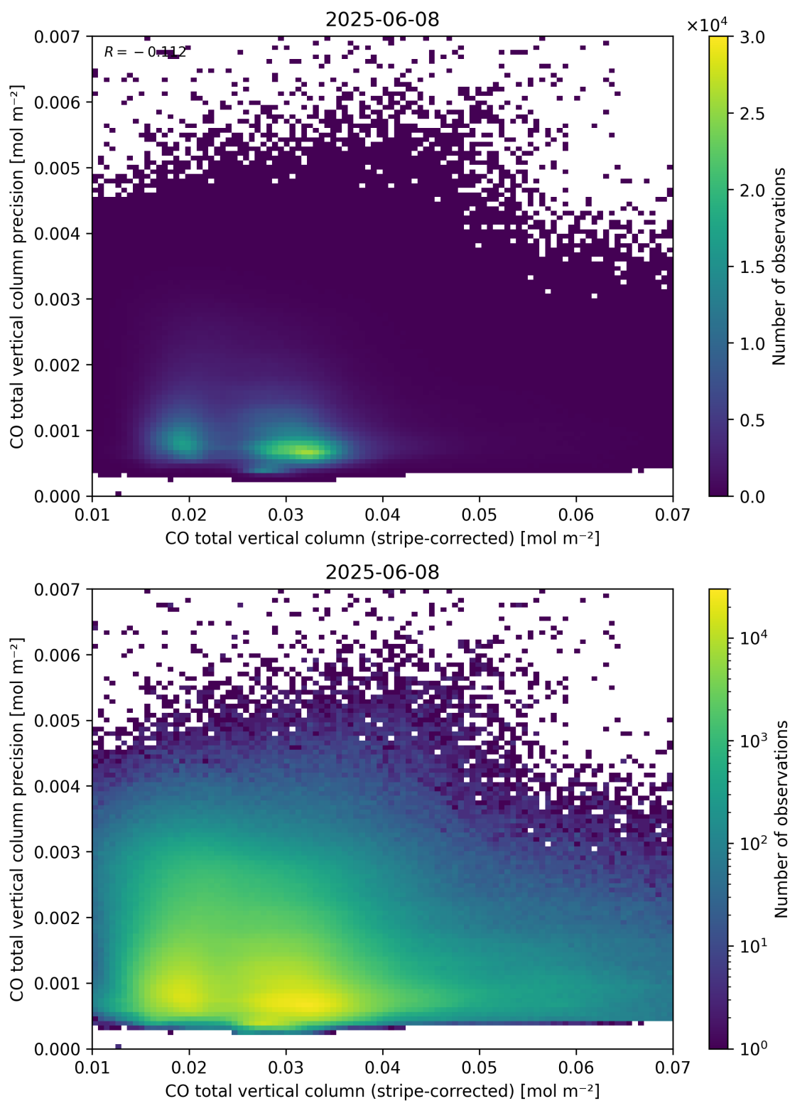
Figure 36: Scatter density plot of “CO total vertical column (stripe-corrected)” against “CO total vertical column precision” for 2025-06-07 to 2025-06-09.
