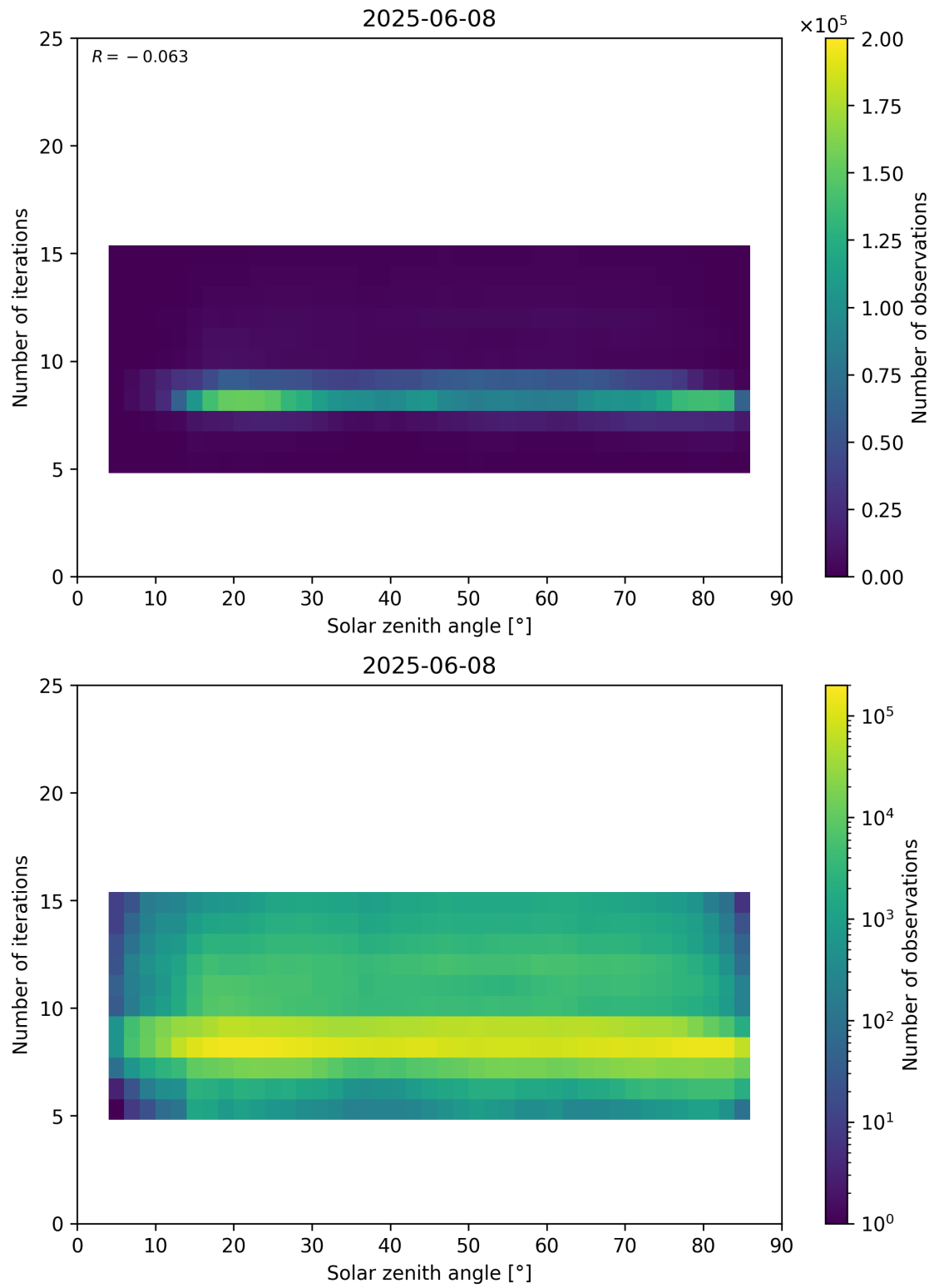
Figure 67: Scatter density plot of “Solar zenith angle” against “Number of iterations” for 2025-06-07 to 2025-06-09.
