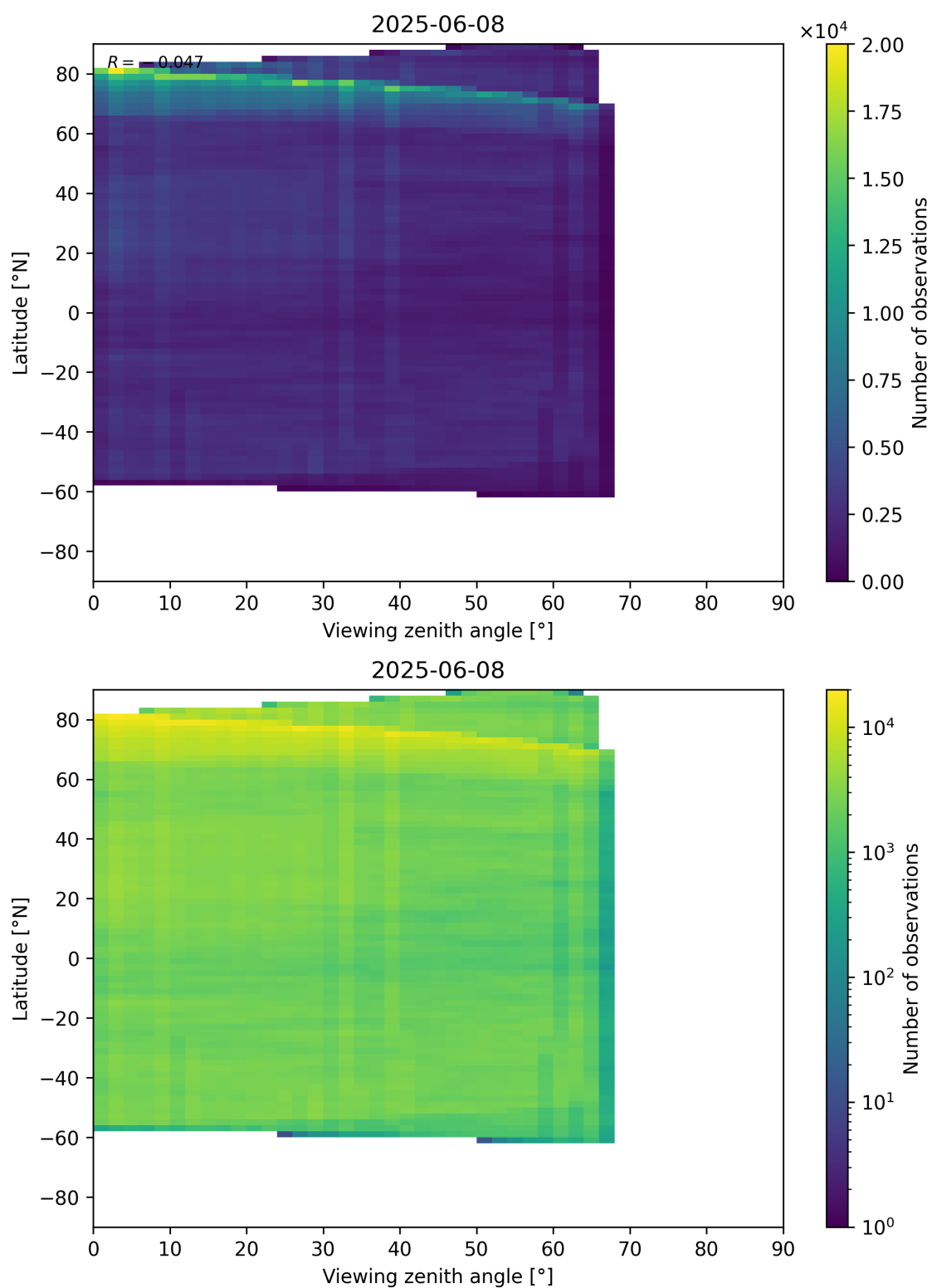
Figure 74: Scatter density plot of “Viewing zenith angle” against “Latitude” for 2025-06-07 to 2025-06-09.
