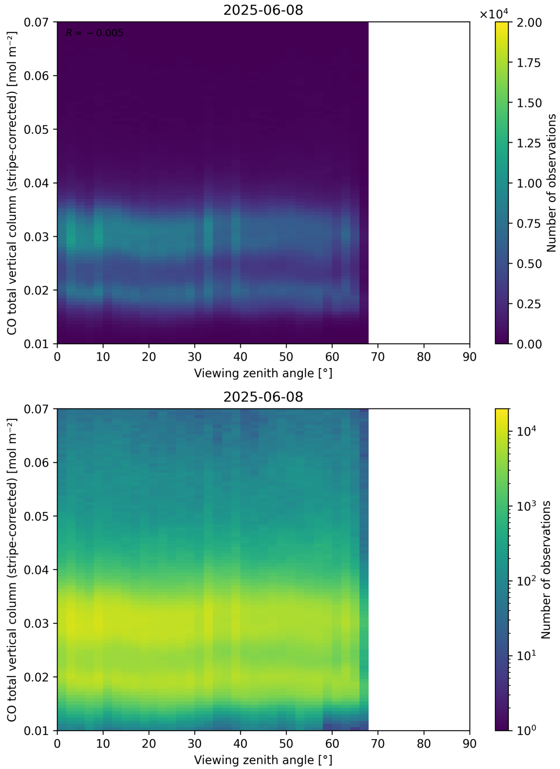
Figure 70: Scatter density plot of “Viewing zenith angle” against “CO total vertical column (stripe-corrected)” for 2025-06-07 to 2025-06-09.
