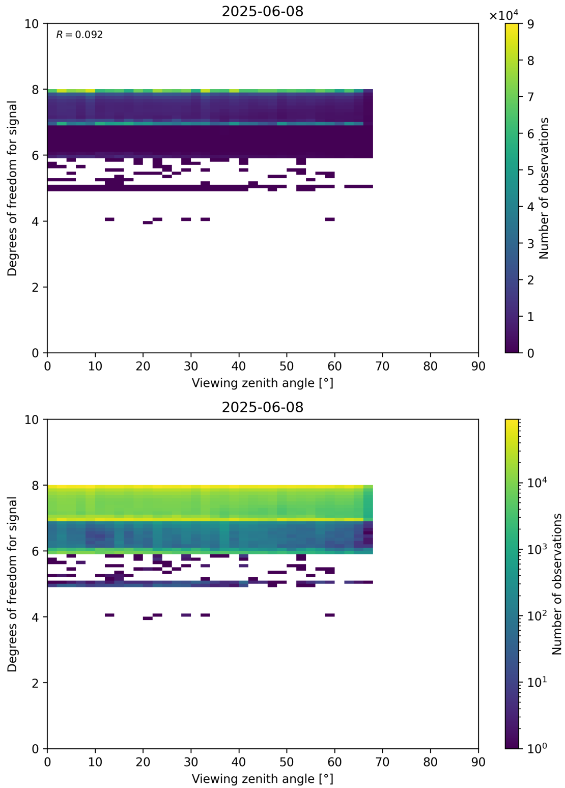
Figure 73: Scatter density plot of “Viewing zenith angle” against “Degrees of freedom for signal” for 2025-06-07 to 2025-06-09.
