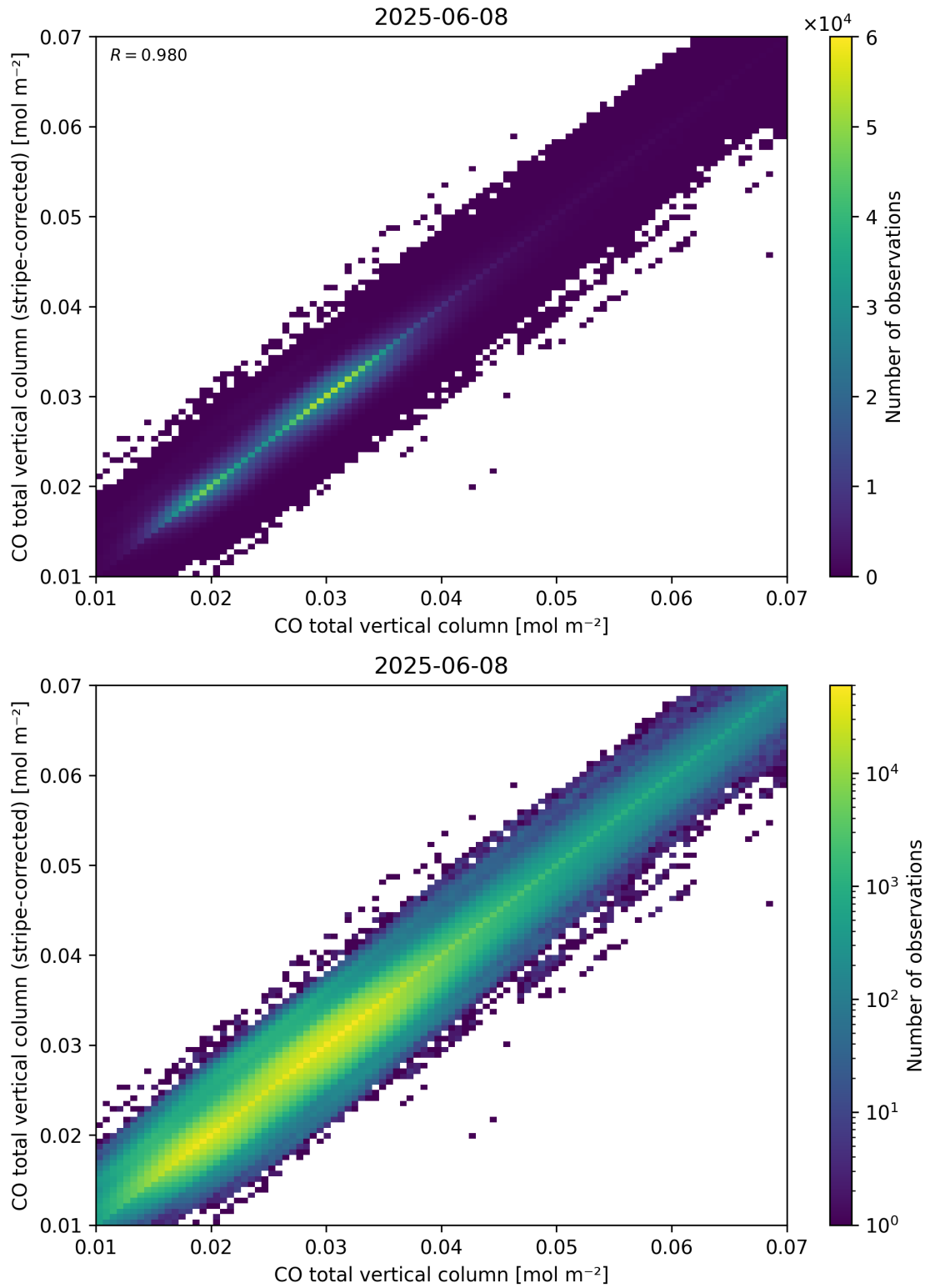
Figure 33: Scatter density plot of “CO total vertical column” against “CO total vertical column (stripe-corrected)” for 2025-06-07 to 2025-06-09.
