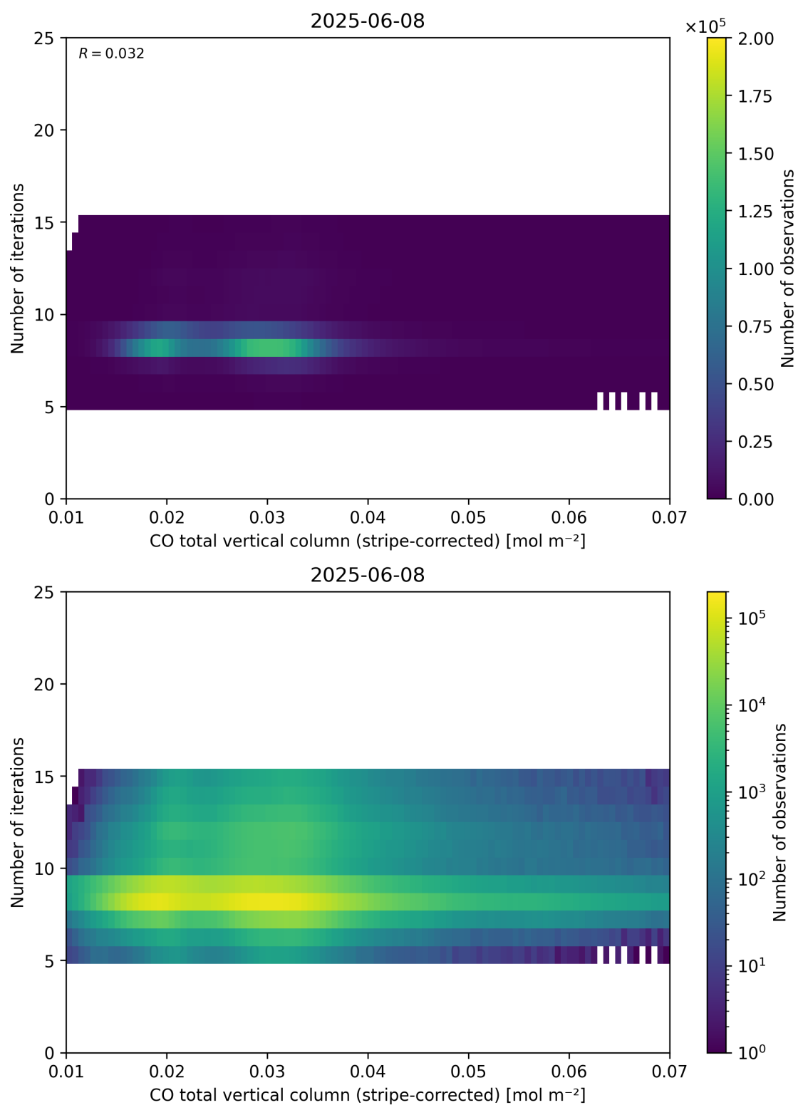
Figure 39: Scatter density plot of “CO total vertical column (stripe-corrected)” against “Number of iterations” for 2025-06-07 to 2025-06-09.
