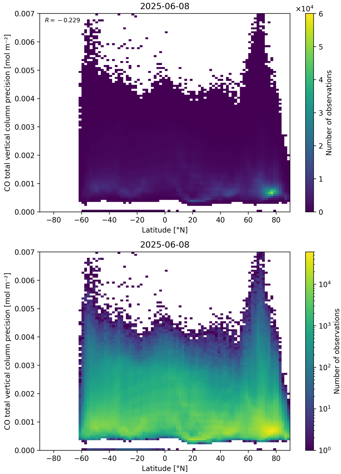
Figure 53: Scatter density plot of “Latitude” against “CO total vertical column precision” for 2025-06-07 to 2025-06-09.
