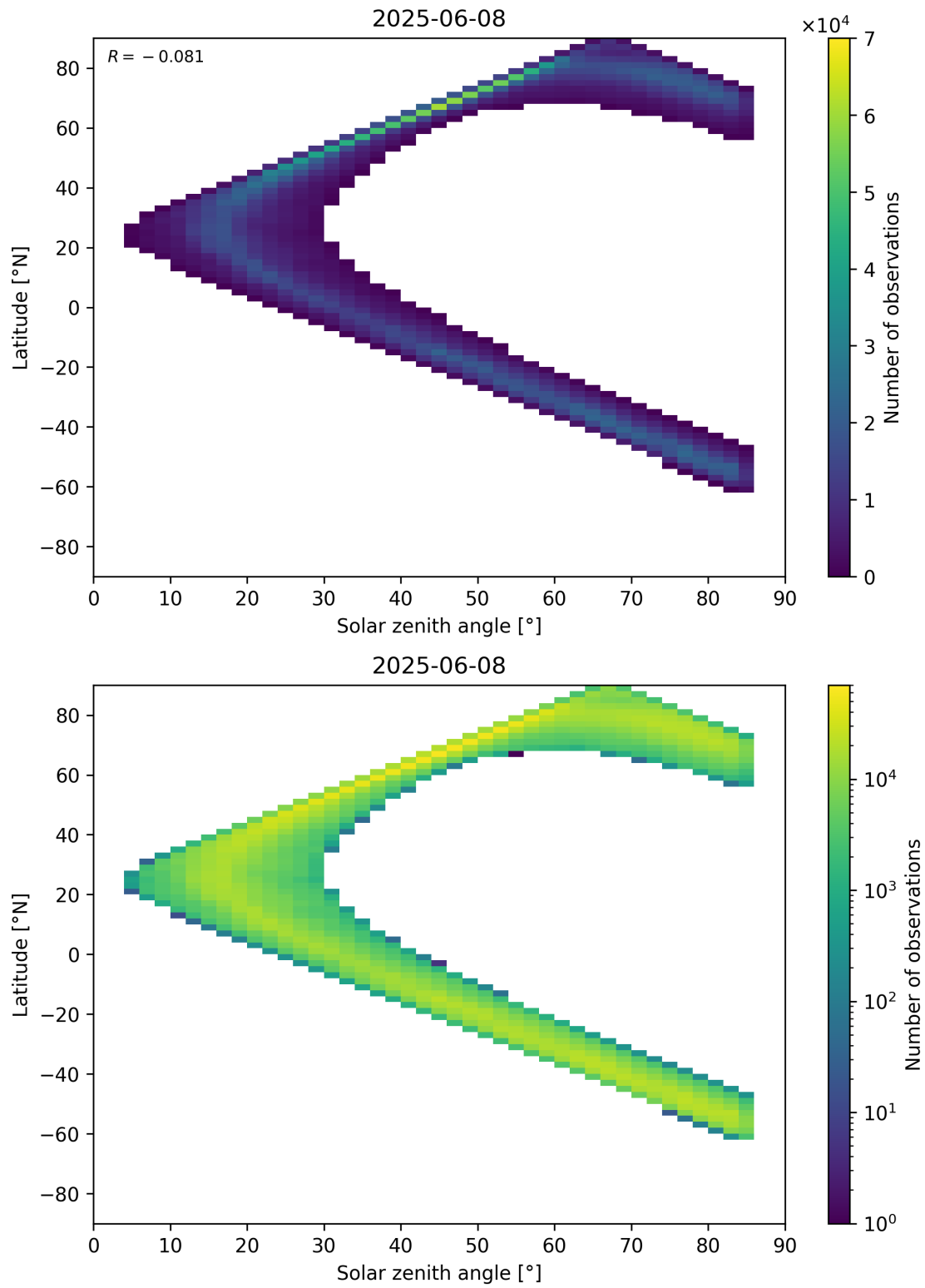
Figure 66: Scatter density plot of “Solar zenith angle” against “Latitude” for 2025-06-07 to 2025-06-09.
