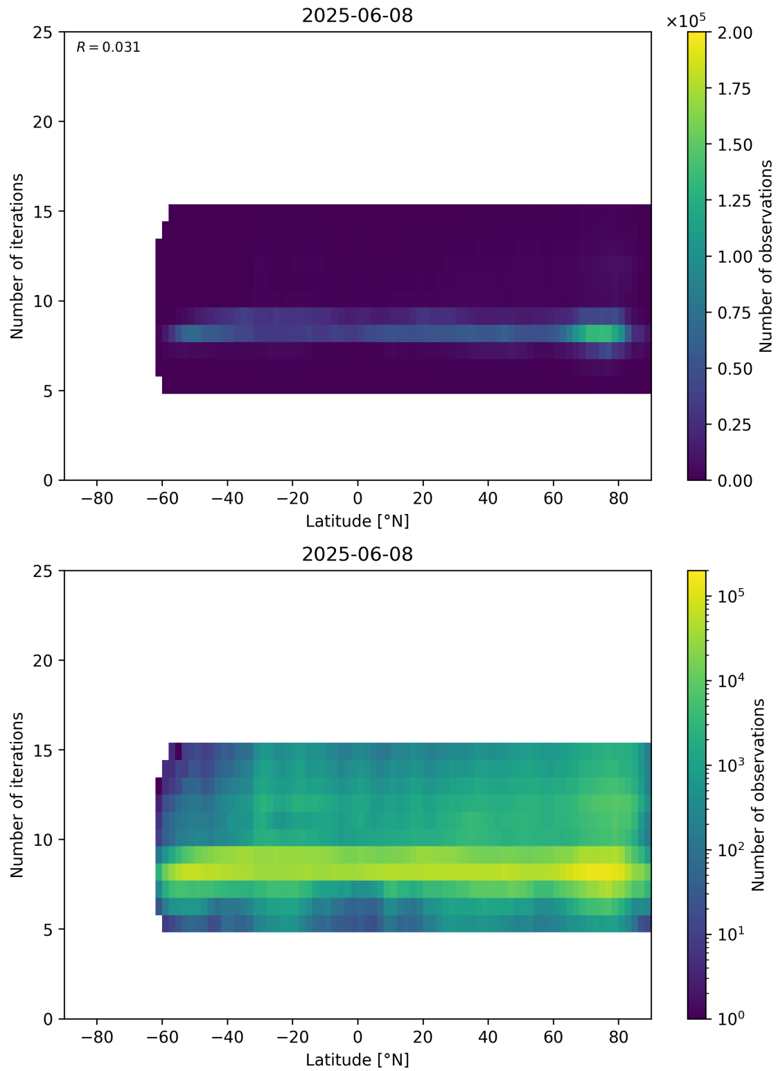
Figure 56: Scatter density plot of “Latitude” against “Number of iterations” for 2025-06-07 to 2025-06-09.
