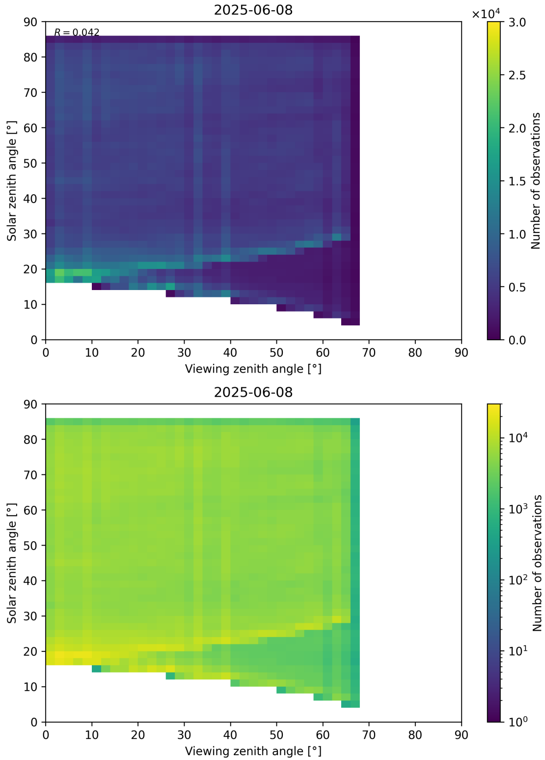
Figure 77: Scatter density plot of “Viewing zenith angle” against “Solar zenith angle” for 2025-06-07 to 2025-06-09.
