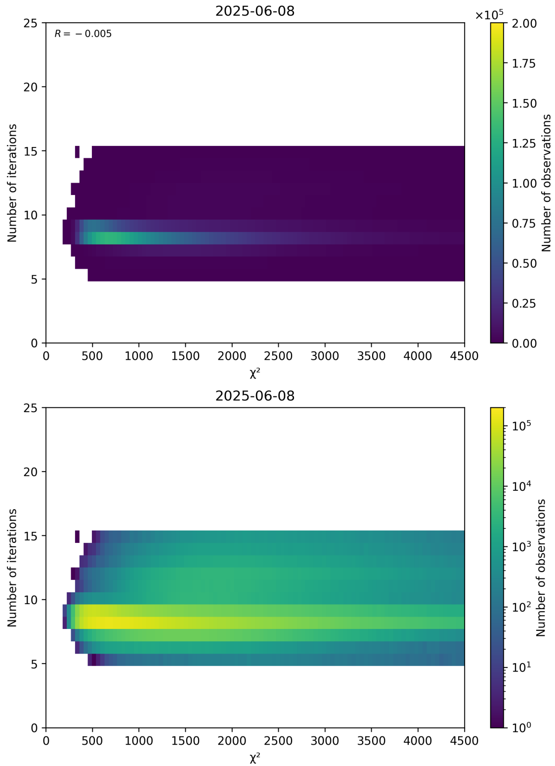
Figure 49: Scatter density plot of “ \chi^2 ” against “Number of iterations” for 2025-06-07 to 2025-06-09.
