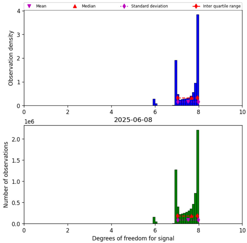
Figure 23: Histogram of “Degrees of freedom for signal” for 2025-06-07 to 2025-06-09
