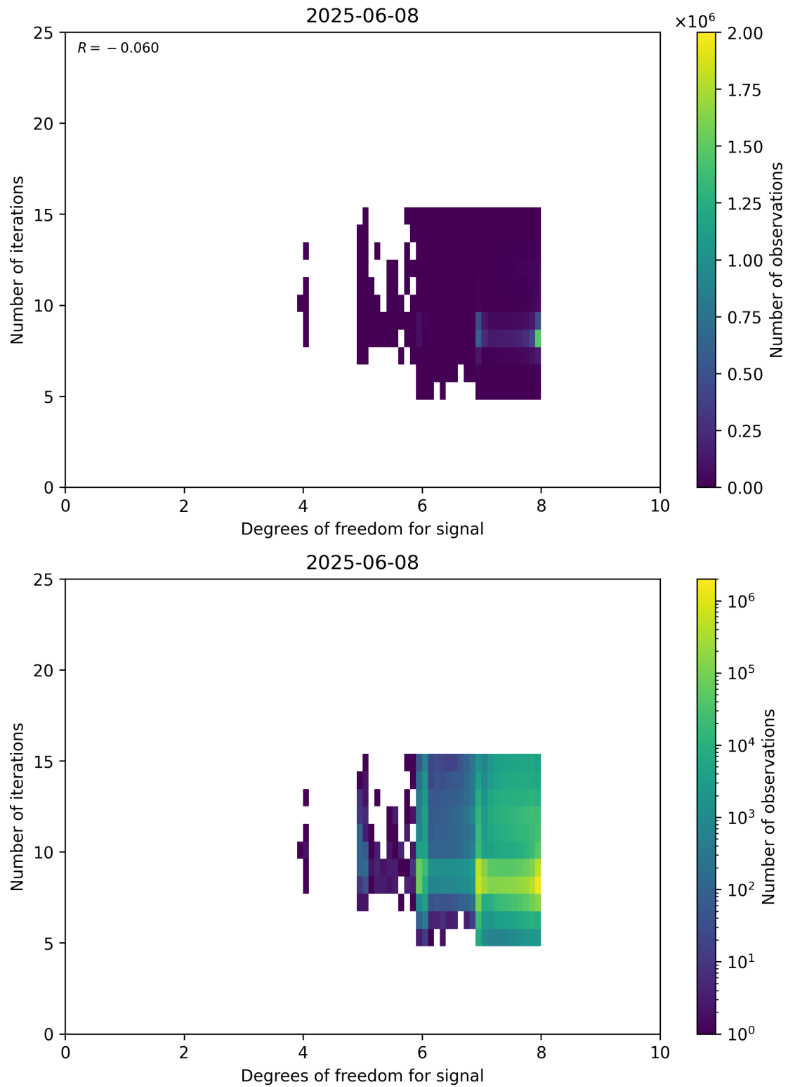
Figure 50: Scatter density plot of “Degrees of freedom for signal” against “Number of iterations” for 2025-06-07 to 2025-06-09.
