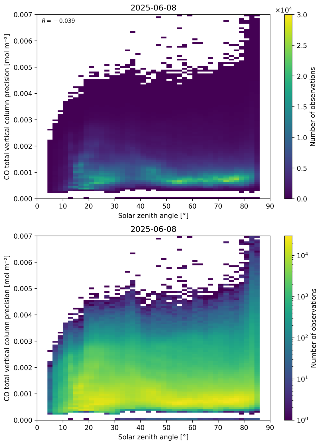
Figure 63: Scatter density plot of “Solar zenith angle” against “CO total vertical column precision” for 2025-06-07 to 2025-06-09.
