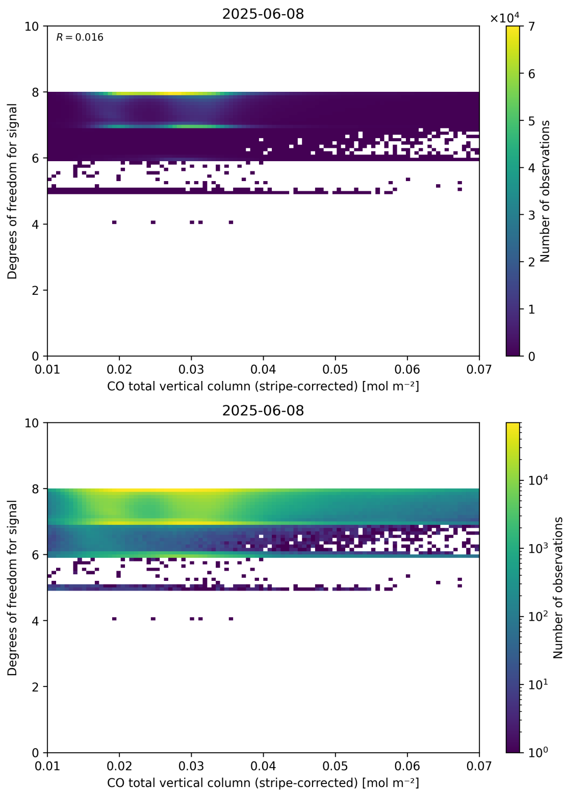
Figure 38: Scatter density plot of “CO total vertical column (stripe-corrected)” against “Degrees of freedom for signal” for 2025-06-07 to 2025-06-09.
