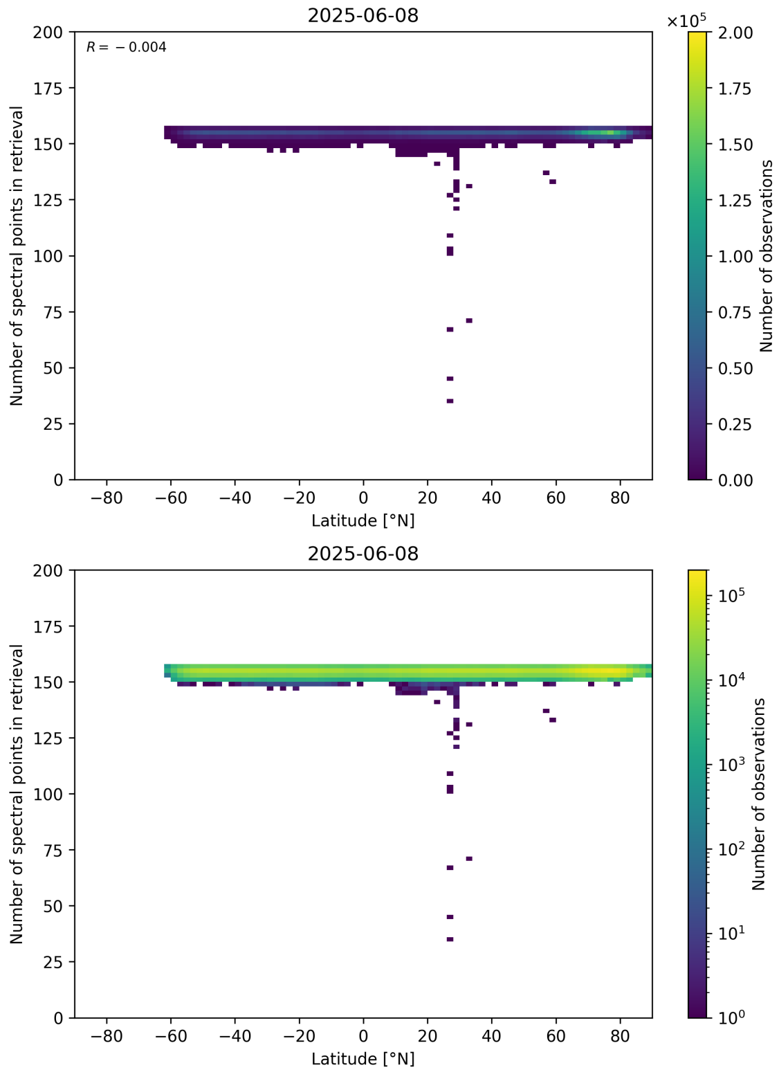
Figure 57: Scatter density plot of “Latitude” against “Number of spectral points in retrieval” for 2025-06-07 to 2025-06-09.
