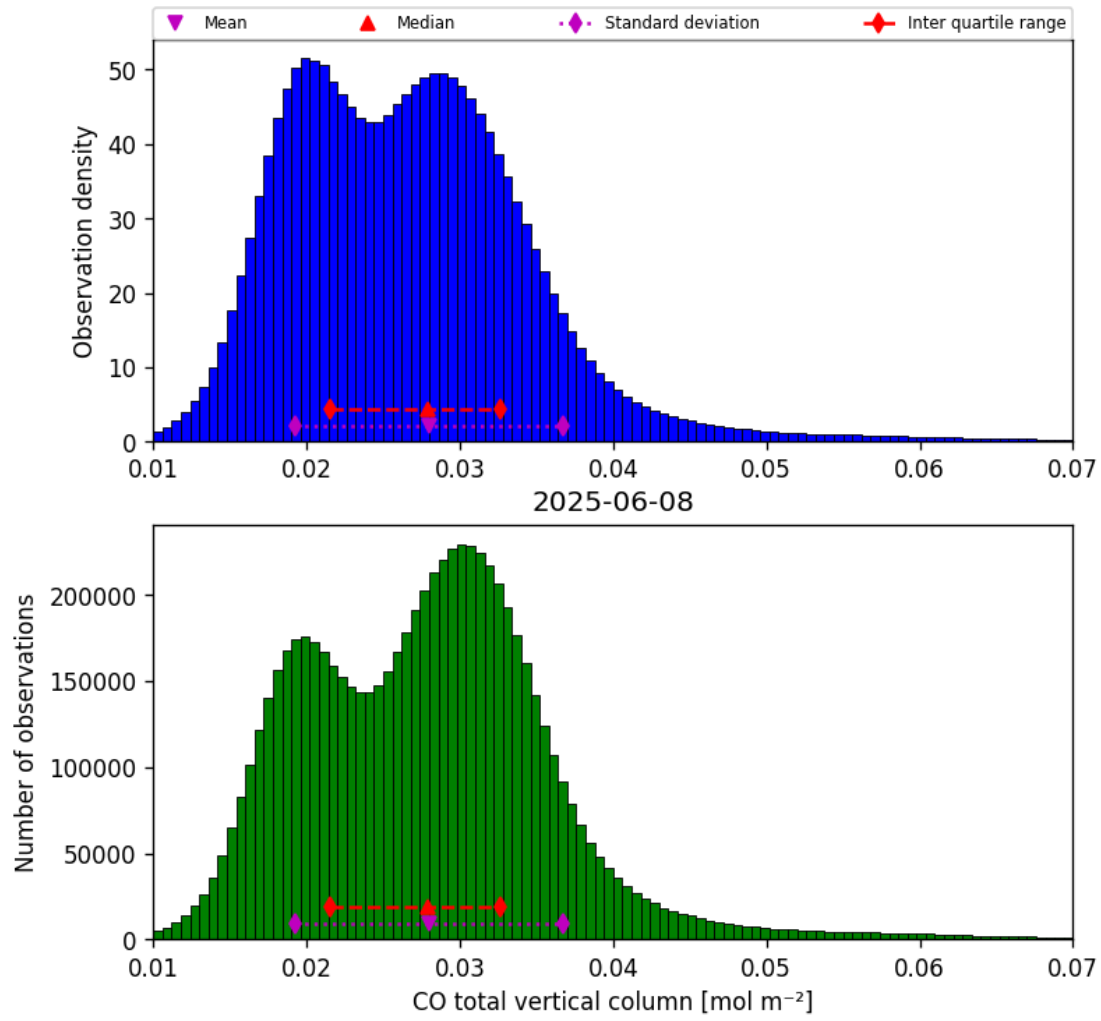
Figure 18: Histogram of “CO total vertical column” for 2025-06-07 to 2025-06-09
