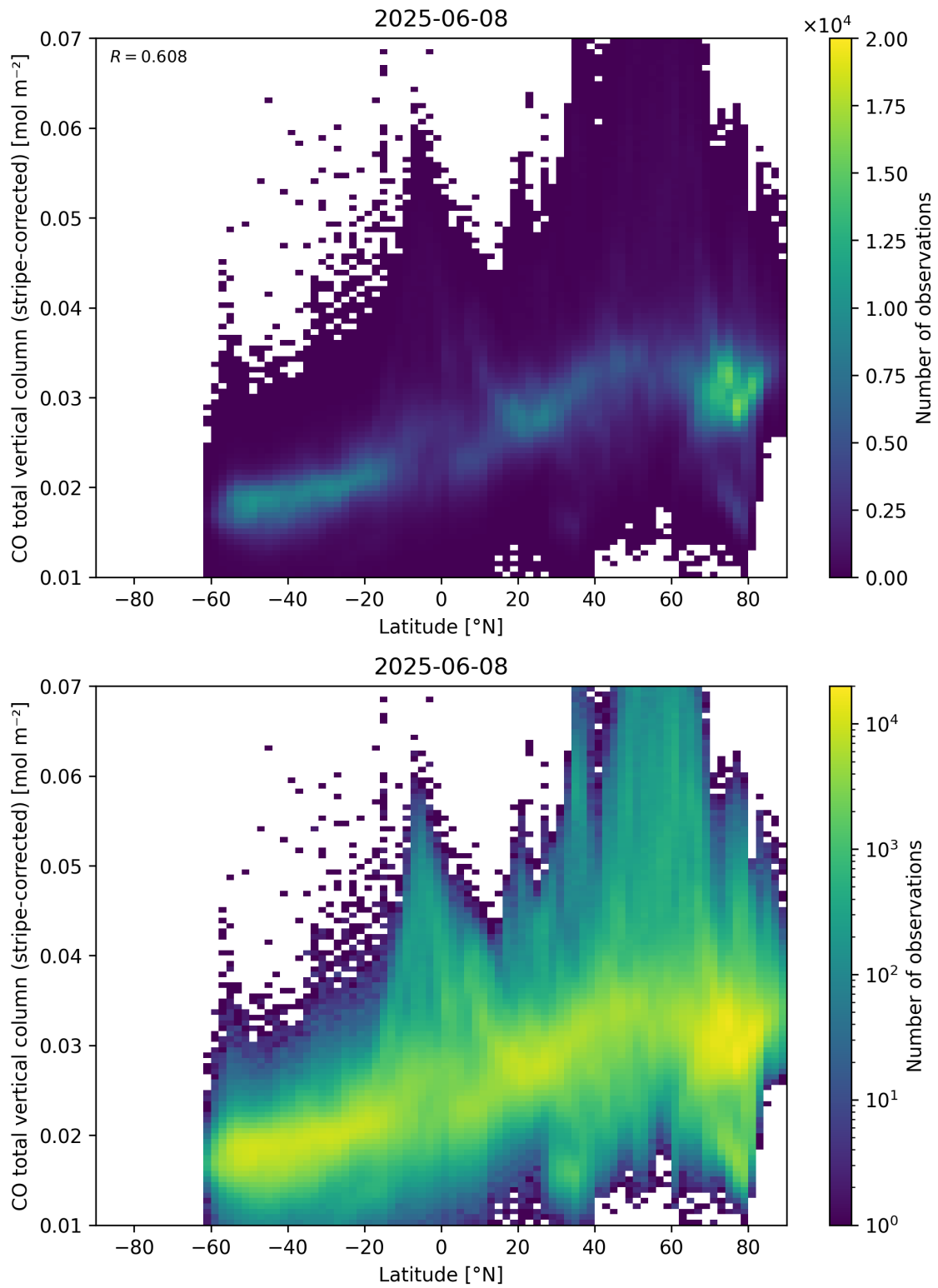
Figure 52: Scatter density plot of “Latitude” against “CO total vertical column (stripe-corrected)” for 2025-06-07 to 2025-06-09.
