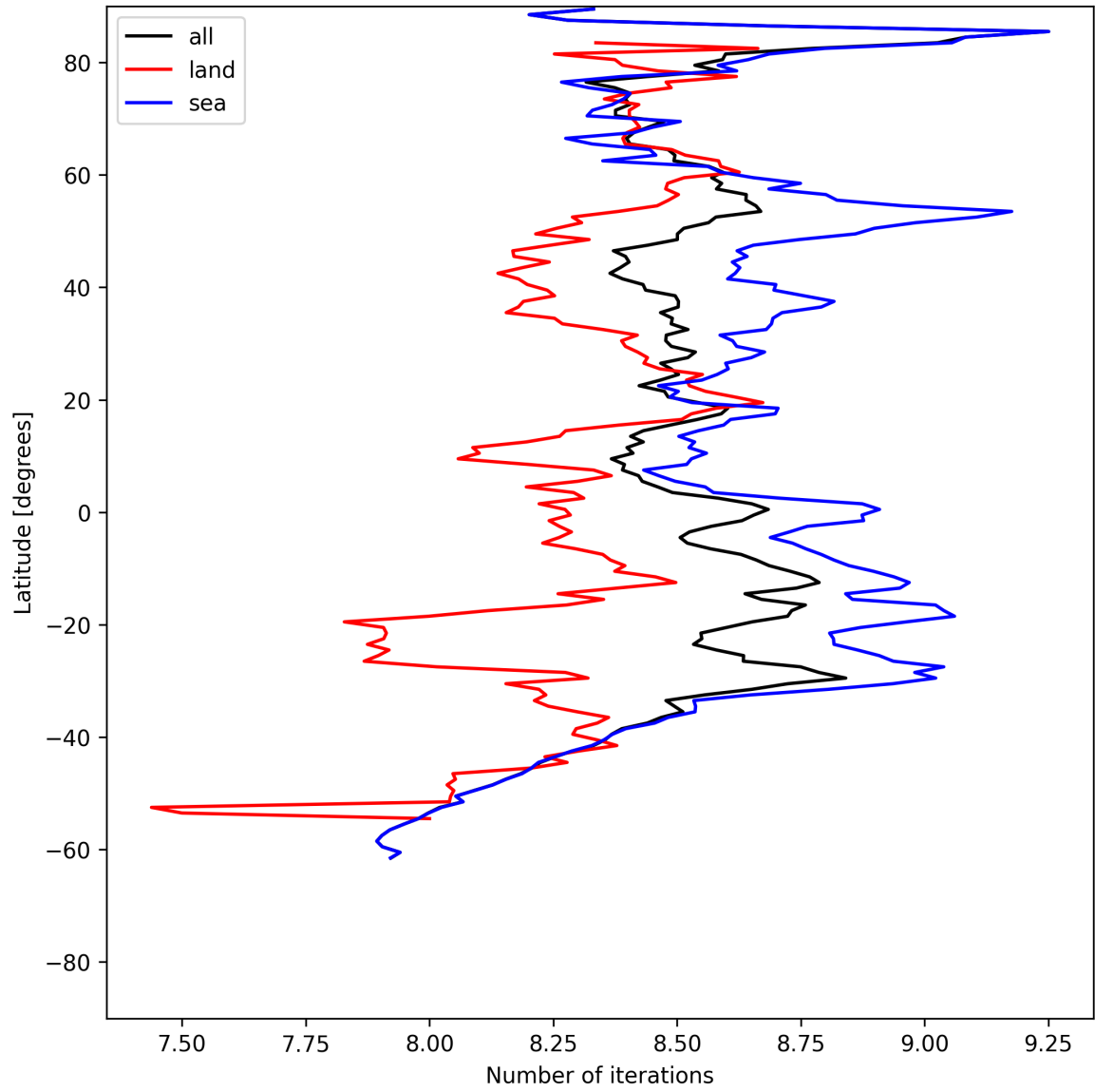
Figure 16: Zonal average of “Number of iterations” for 2025-06-07 to 2025-06-09.
