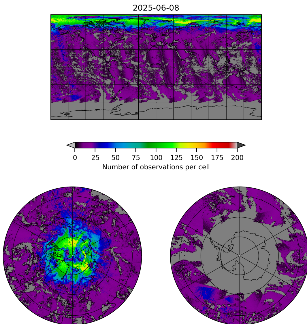
Figure 8: Map of the number of observations for 2025-06-07 to 2025-06-09
