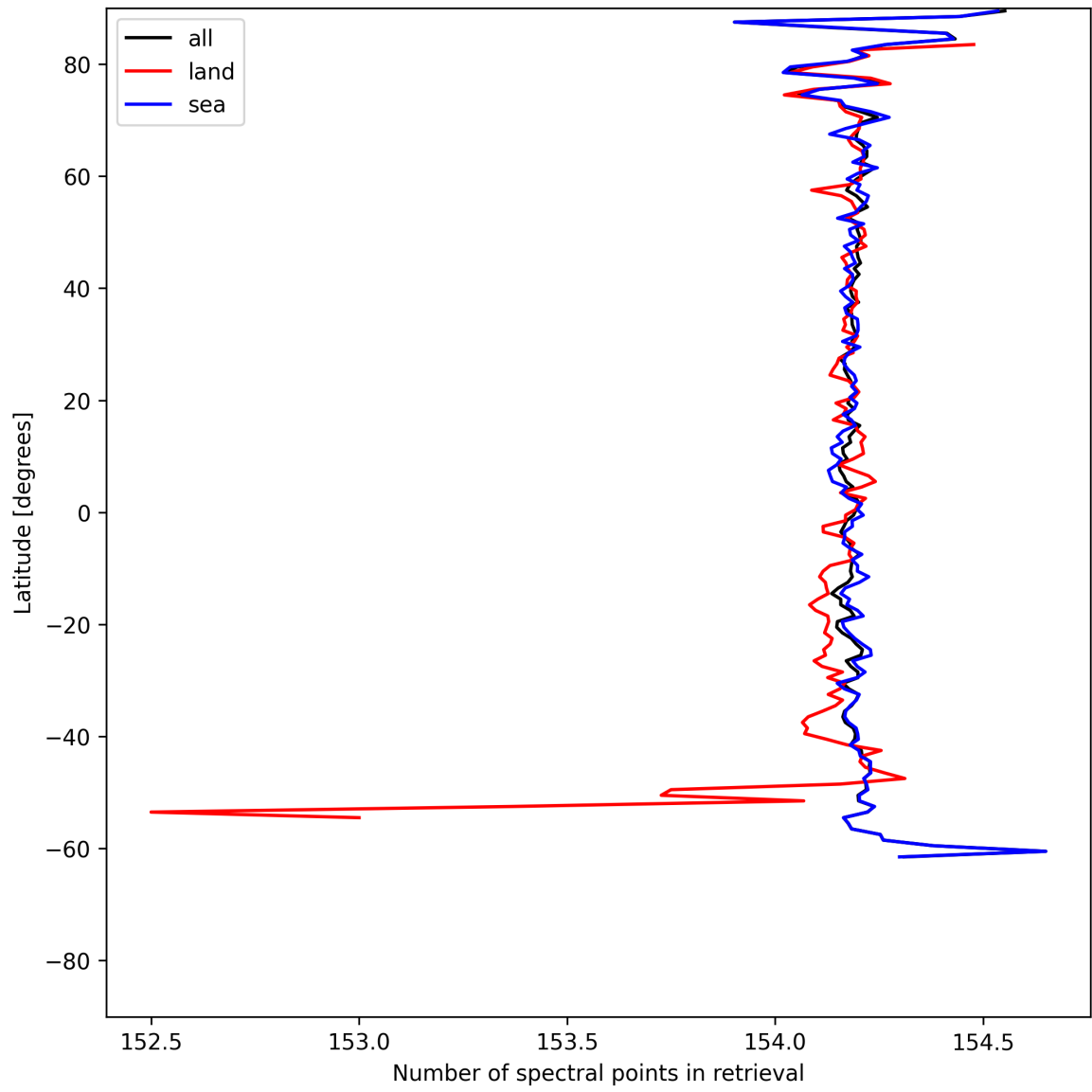
Figure 13: Zonal average of “Number of spectral points in retrieval” for 2025-06-07 to 2025-06-09.
