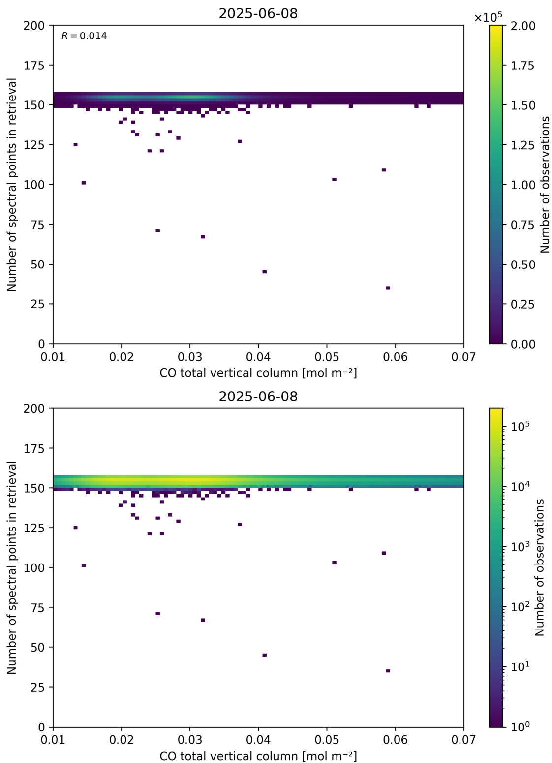
Figure 43: Scatter density plot of “CO total vertical column” against “Number of spectral points in retrieval” for 2025-06-07 to 2025-06-09.
