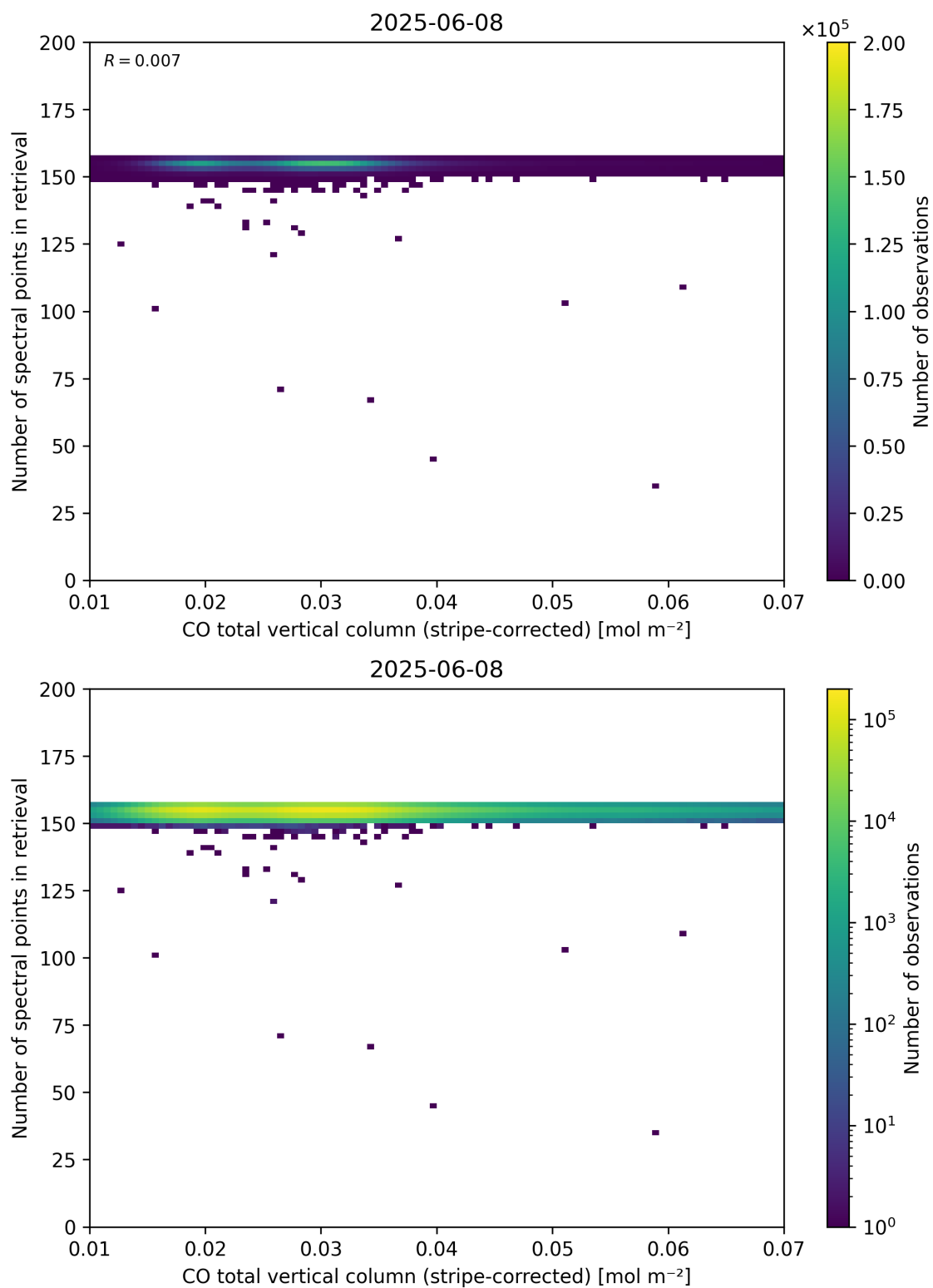
Figure 40: Scatter density plot of “CO total vertical column (stripe-corrected)” against “Number of spectral points in retrieval” for 2025-06-07 to 2025-06-09.
