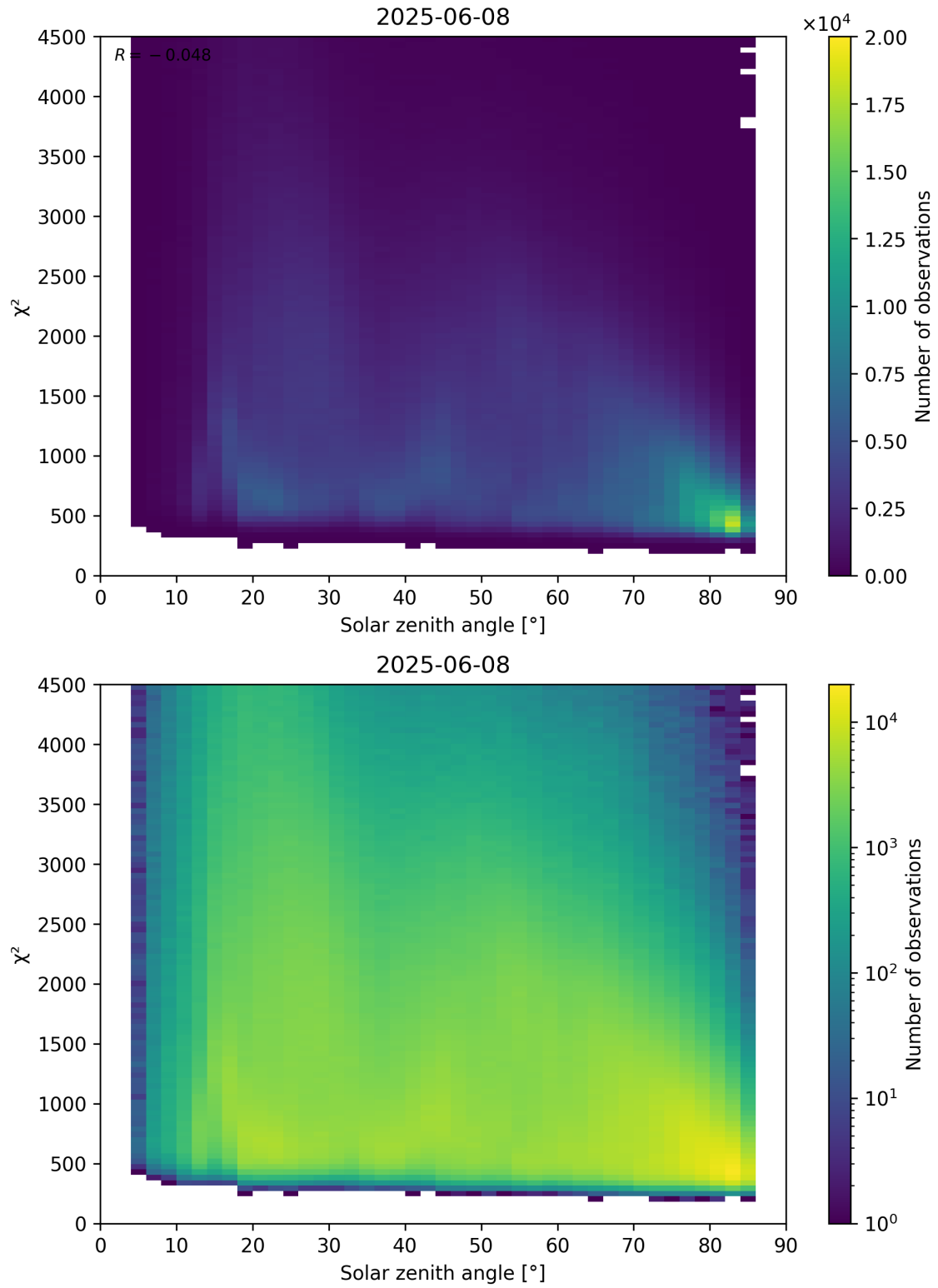
Figure 64: Scatter density plot of “Solar zenith angle” against “ \chi^2 ” for 2025-06-07 to 2025-06-09.
