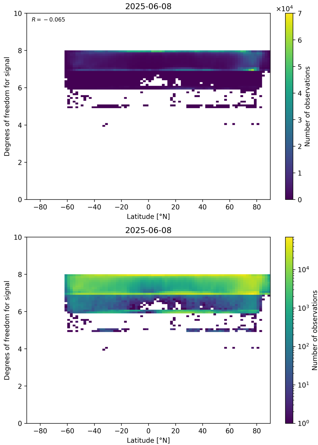
Figure 55: Scatter density plot of “Latitude” against “Degrees of freedom for signal” for 2025-06-07 to 2025-06-09.
