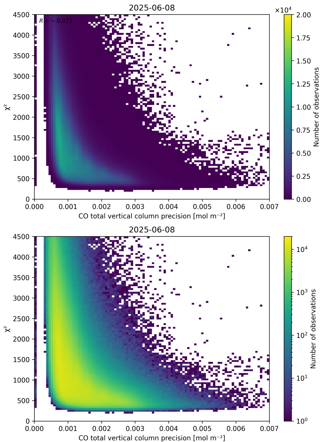
Figure 44: Scatter density plot of “CO total vertical column precision” against “ \chi^2 ” for 2025-06-07 to 2025-06-09.
