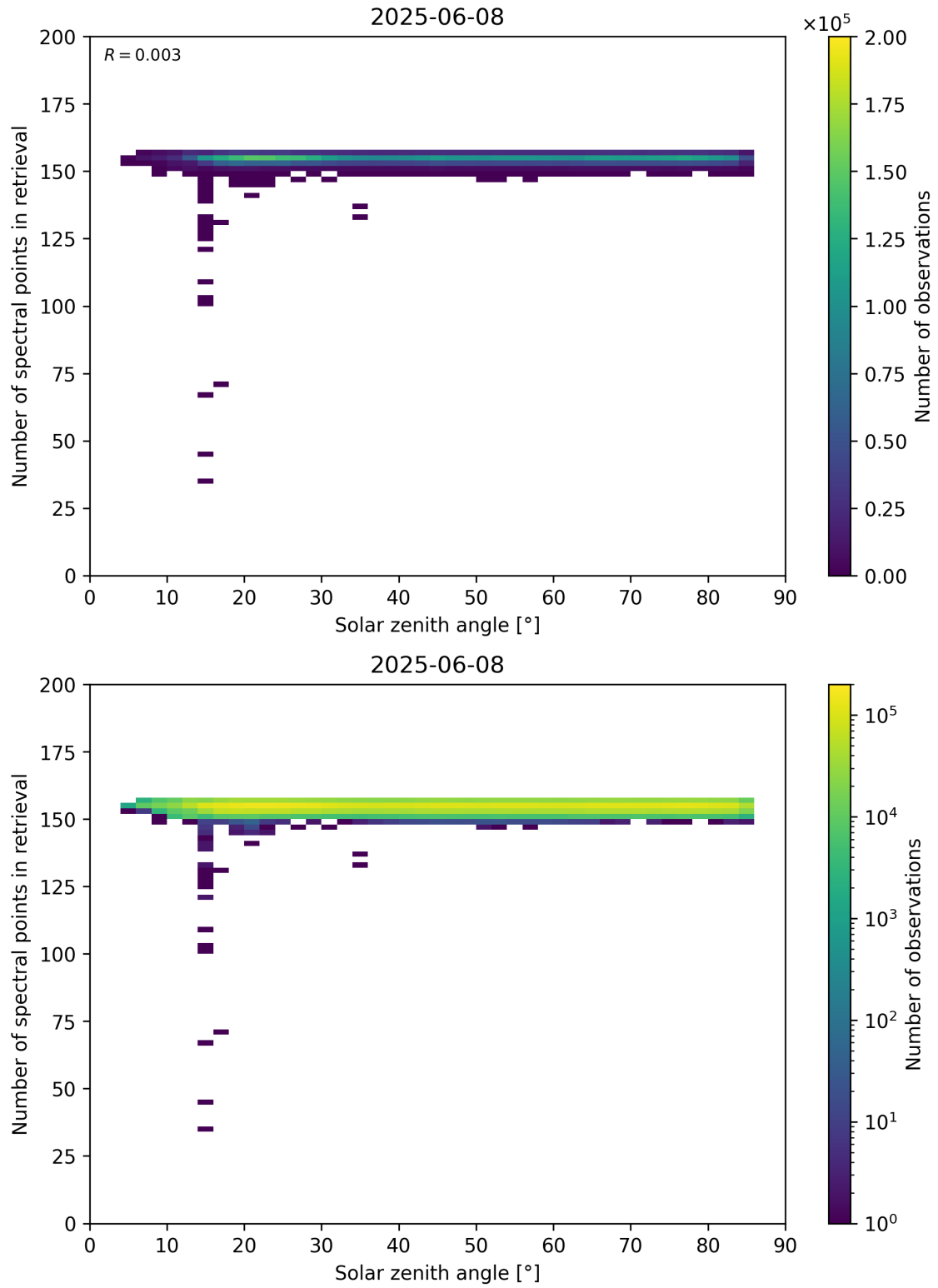
Figure 68: Scatter density plot of “Solar zenith angle” against “Number of spectral points in retrieval” for 2025-06-07 to 2025-06-09.
