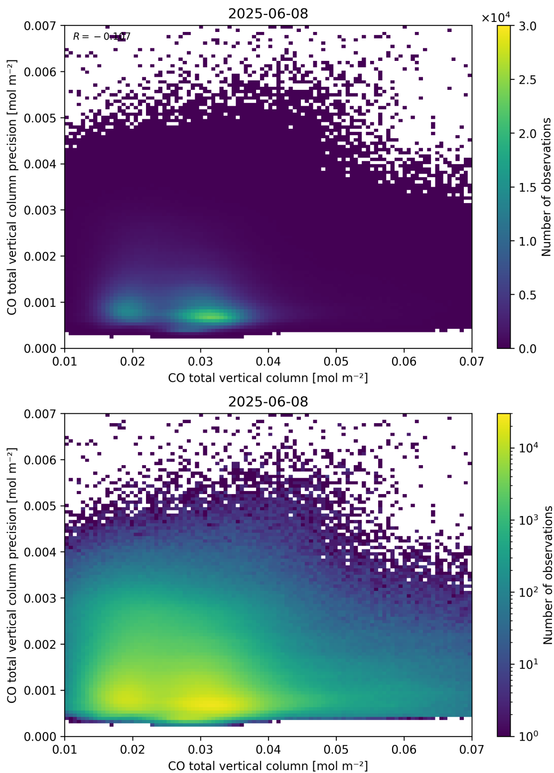
Figure 34: Scatter density plot of “CO total vertical column” against “CO total vertical column precision” for 2025-06-07 to 2025-06-09.
