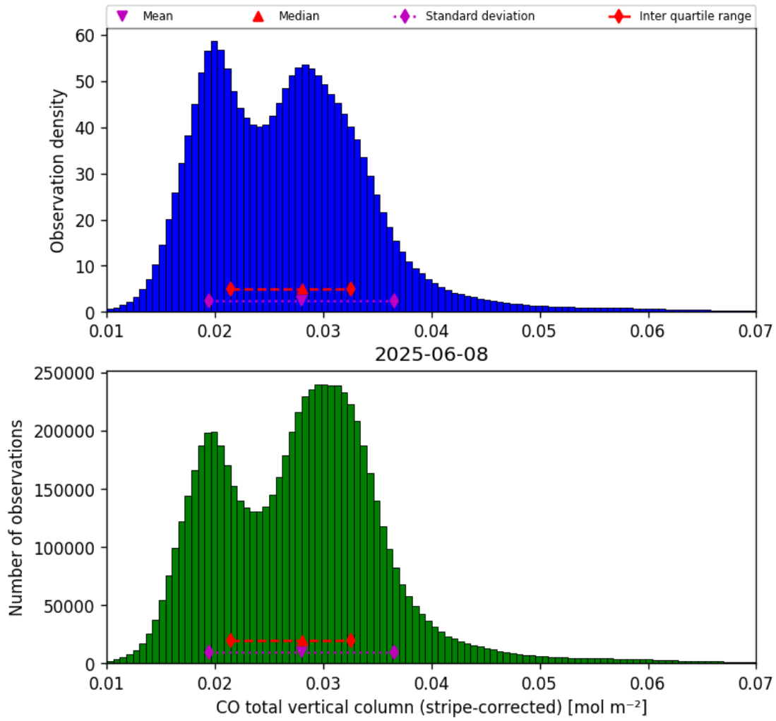
Figure 19: Histogram of “CO total vertical column (stripe-corrected)” for 2025-06-07 to 2025-06-09
