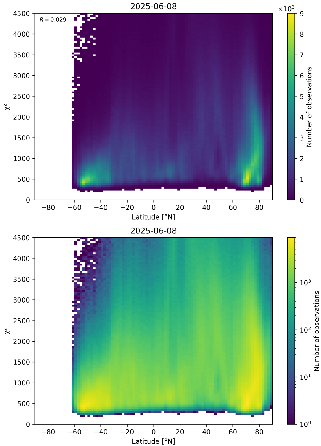
Figure 54: Scatter density plot of “Latitude” against “ \chi^2 ” for 2025-06-07 to 2025-06-09.
