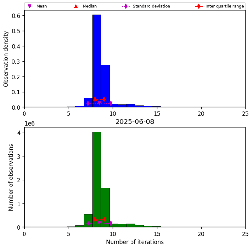
Figure 24: Histogram of “Number of iterations” for 2025-06-07 to 2025-06-09
