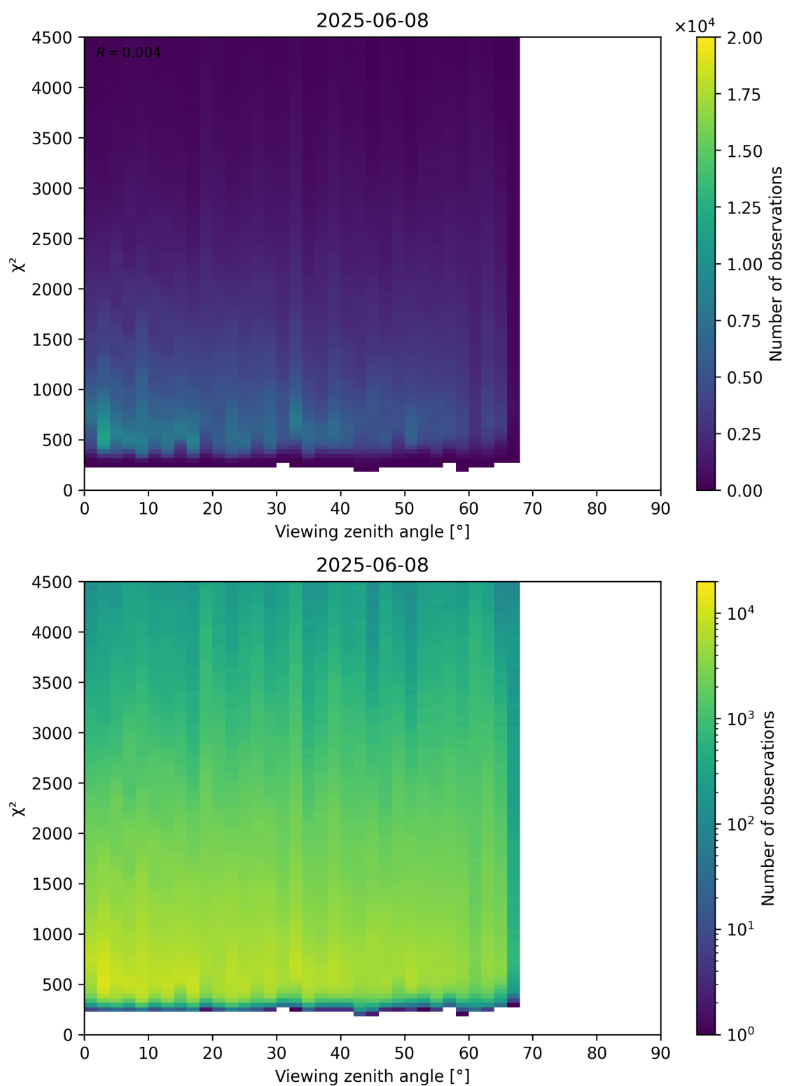
Figure 72: Scatter density plot of “Viewing zenith angle” against “ \chi^2 ” for 2025-06-07 to 2025-06-09.
