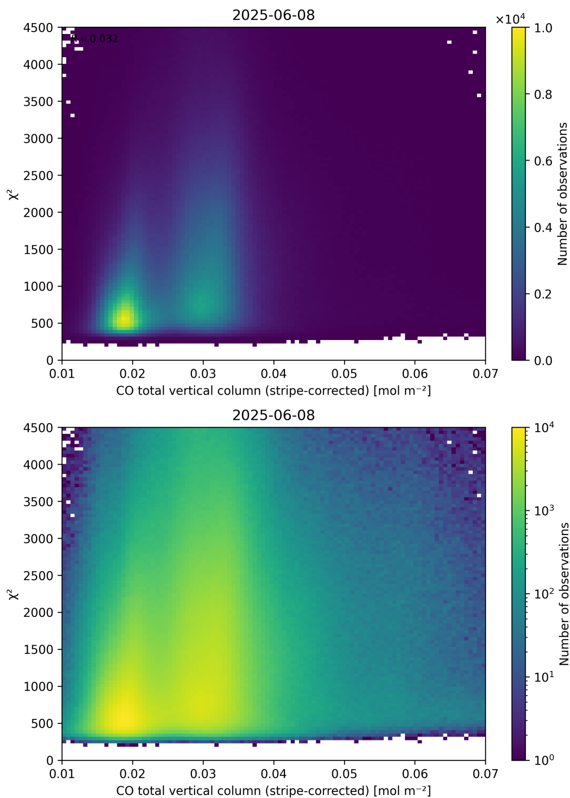
Figure 37: Scatter density plot of “CO total vertical column (stripe-corrected)” against “ \chi^2 ” for 2025-06-07 to 2025-06-09.
