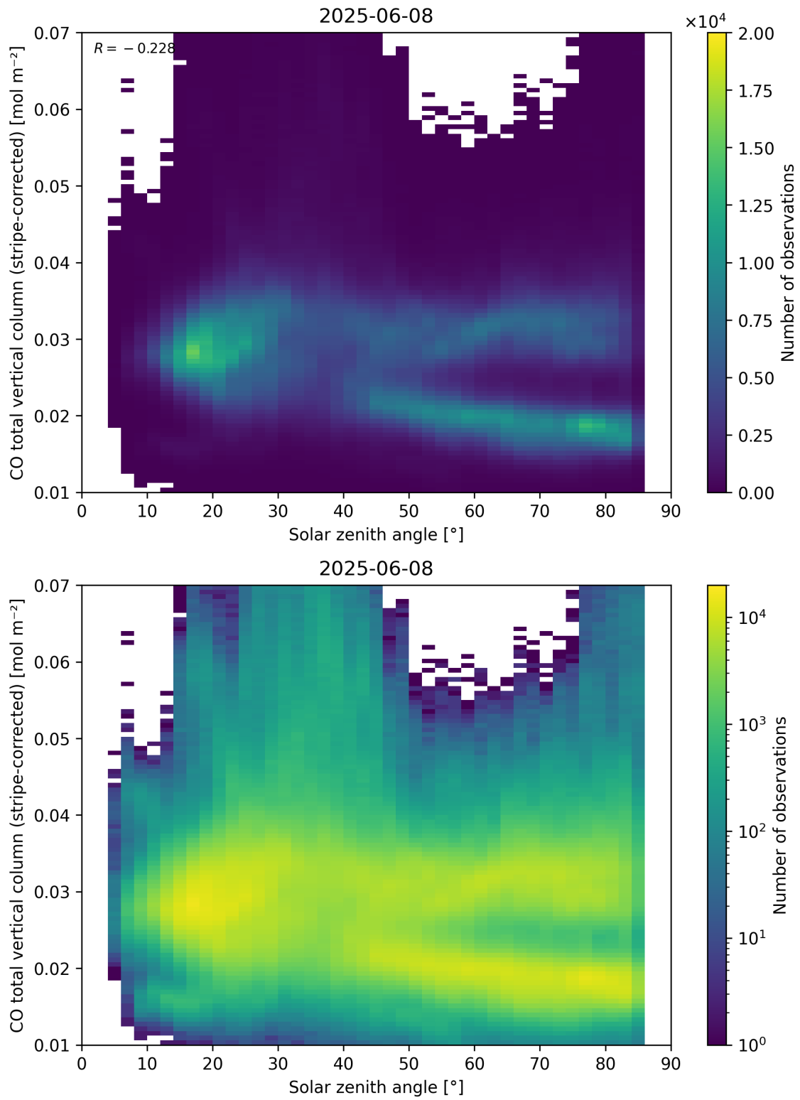
Figure 62: Scatter density plot of “Solar zenith angle” against “CO total vertical column (stripe-corrected)” for 2025-06-07 to 2025-06-09.
