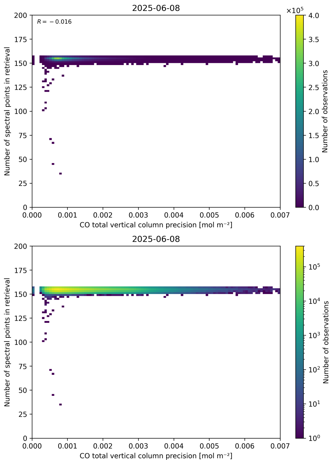
Figure 47: Scatter density plot of “CO total vertical column precision” against “Number of spectral points in retrieval” for 2025-06-07 to 2025-06-09.
