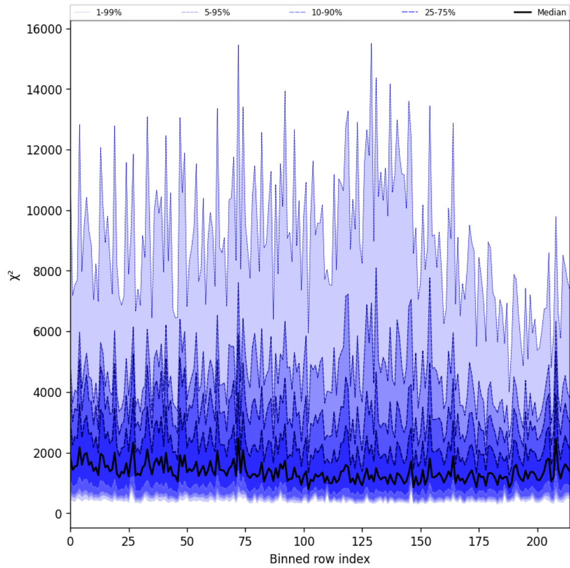
Figure 30: Along track statistics of “ \chi^2 ” for 2025-06-07 to 2025-06-09
