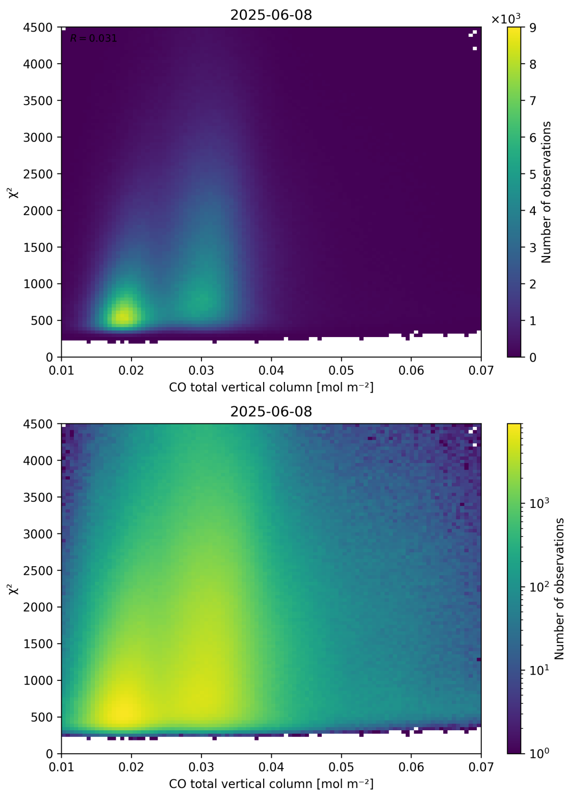
Figure 35: Scatter density plot of “CO total vertical column” against “ \chi^2 ” for 2025-06-07 to 2025-06-09.
