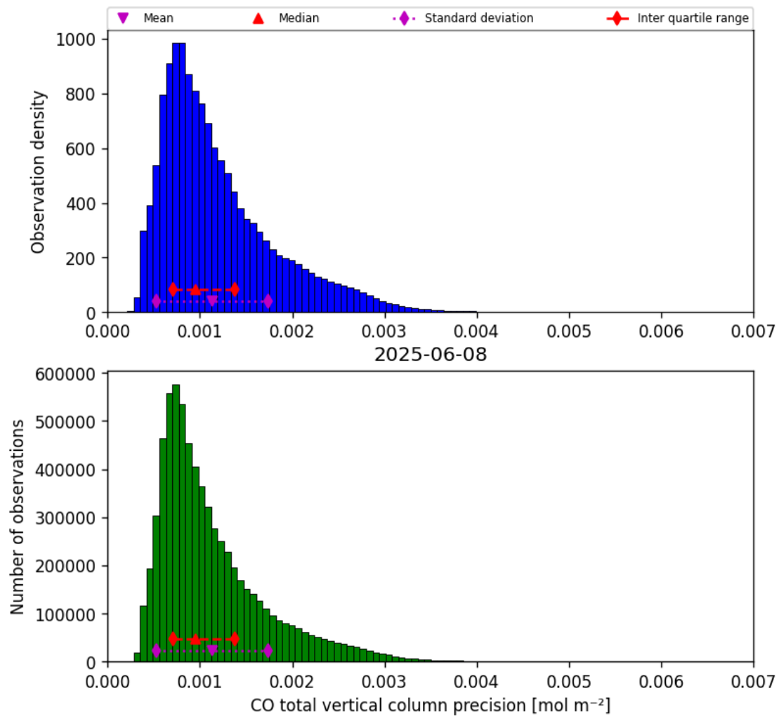
Figure 20: Histogram of “CO total vertical column precision” for 2025-06-07 to 2025-06-09
