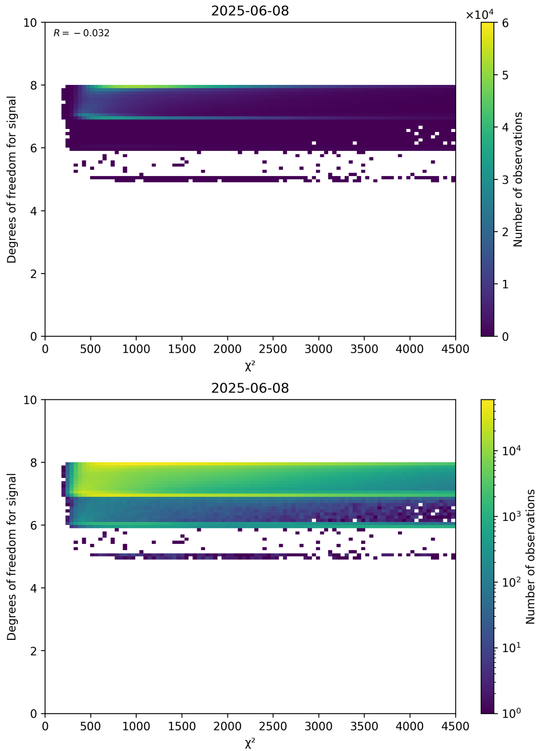
Figure 48: Scatter density plot of “ \chi^2 ” against “Degrees of freedom for signal” for 2025-06-07 to 2025-06-09.
