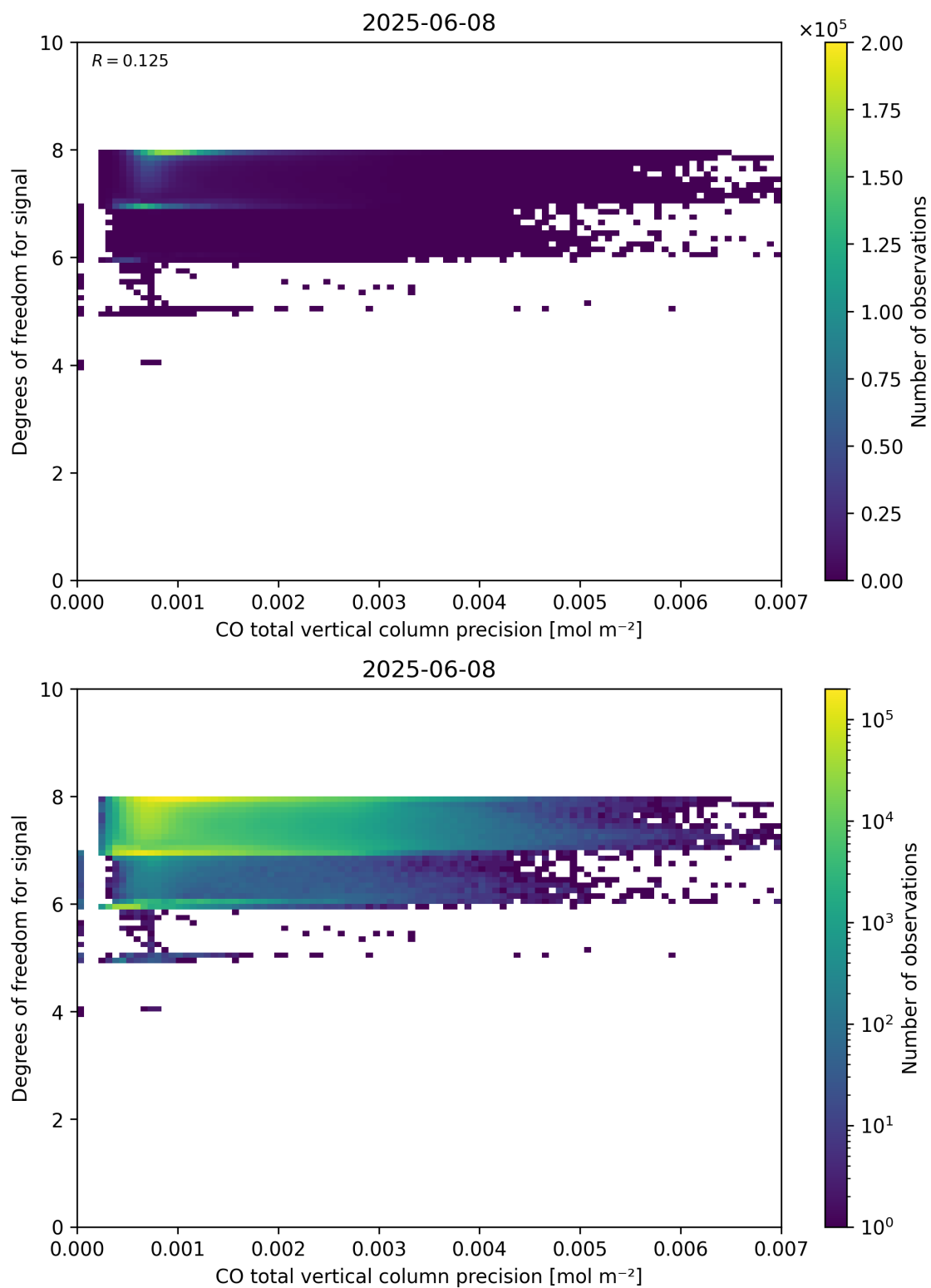
Figure 45: Scatter density plot of “CO total vertical column precision” against “Degrees of freedom for signal” for 2025-06-07 to 2025-06-09.
