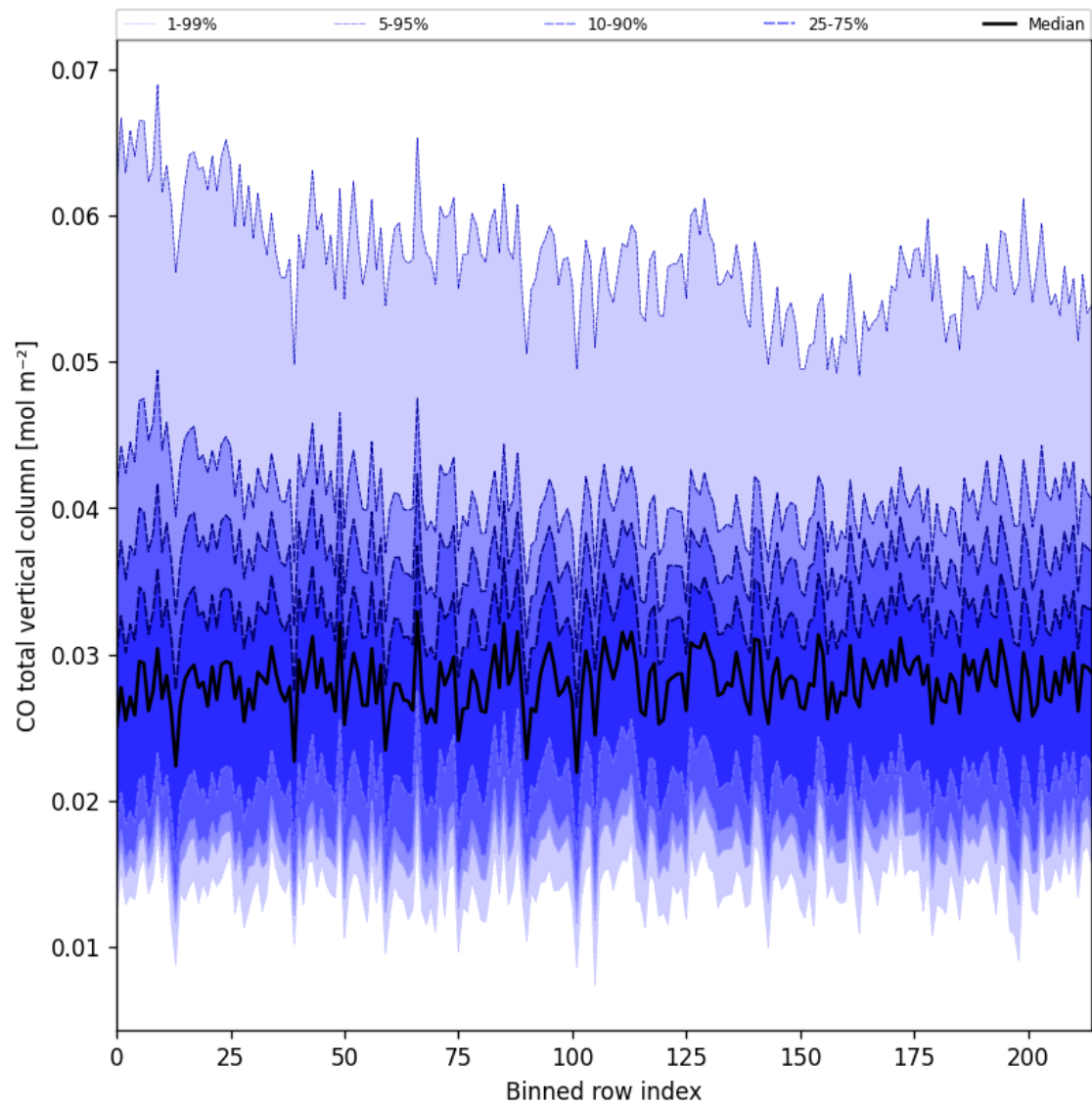
Figure 26: Along track statistics of “CO total vertical column” for 2025-06-07 to 2025-06-09
