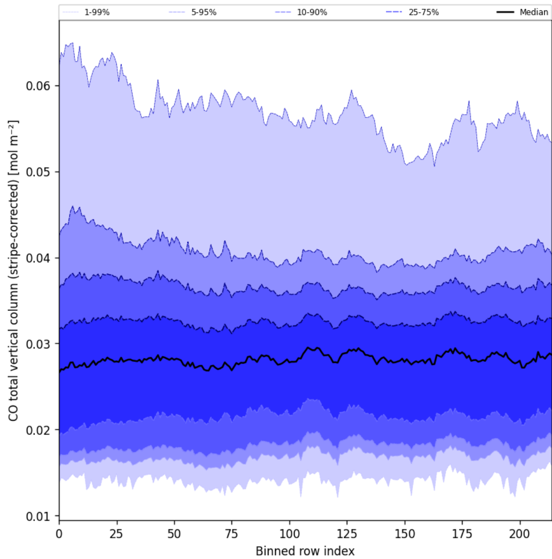
Figure 27: Along track statistics of “CO total vertical column (stripe-corrected)” for 2025-06-07 to 2025-06-09
