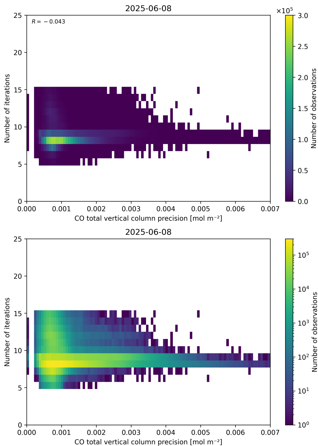
Figure 46: Scatter density plot of “CO total vertical column precision” against “Number of iterations” for 2025-06-07 to 2025-06-09.
