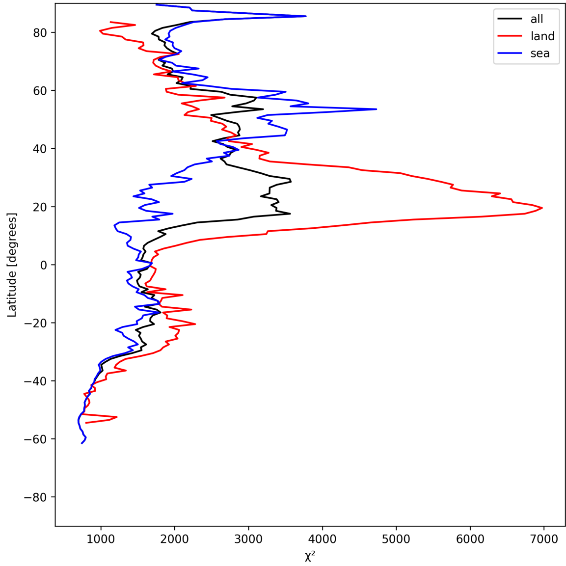
Figure 14: Zonal average of “ \chi^2 ” for 2025-06-07 to 2025-06-09.
