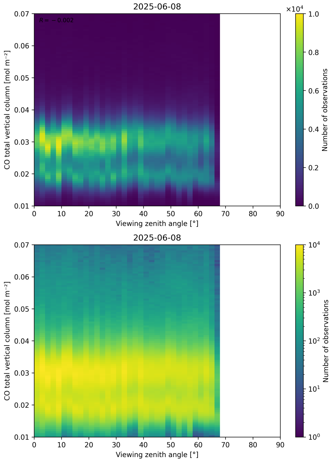
Figure 69: Scatter density plot of “Viewing zenith angle” against “CO total vertical column” for 2025-06-07 to 2025-06-09.
