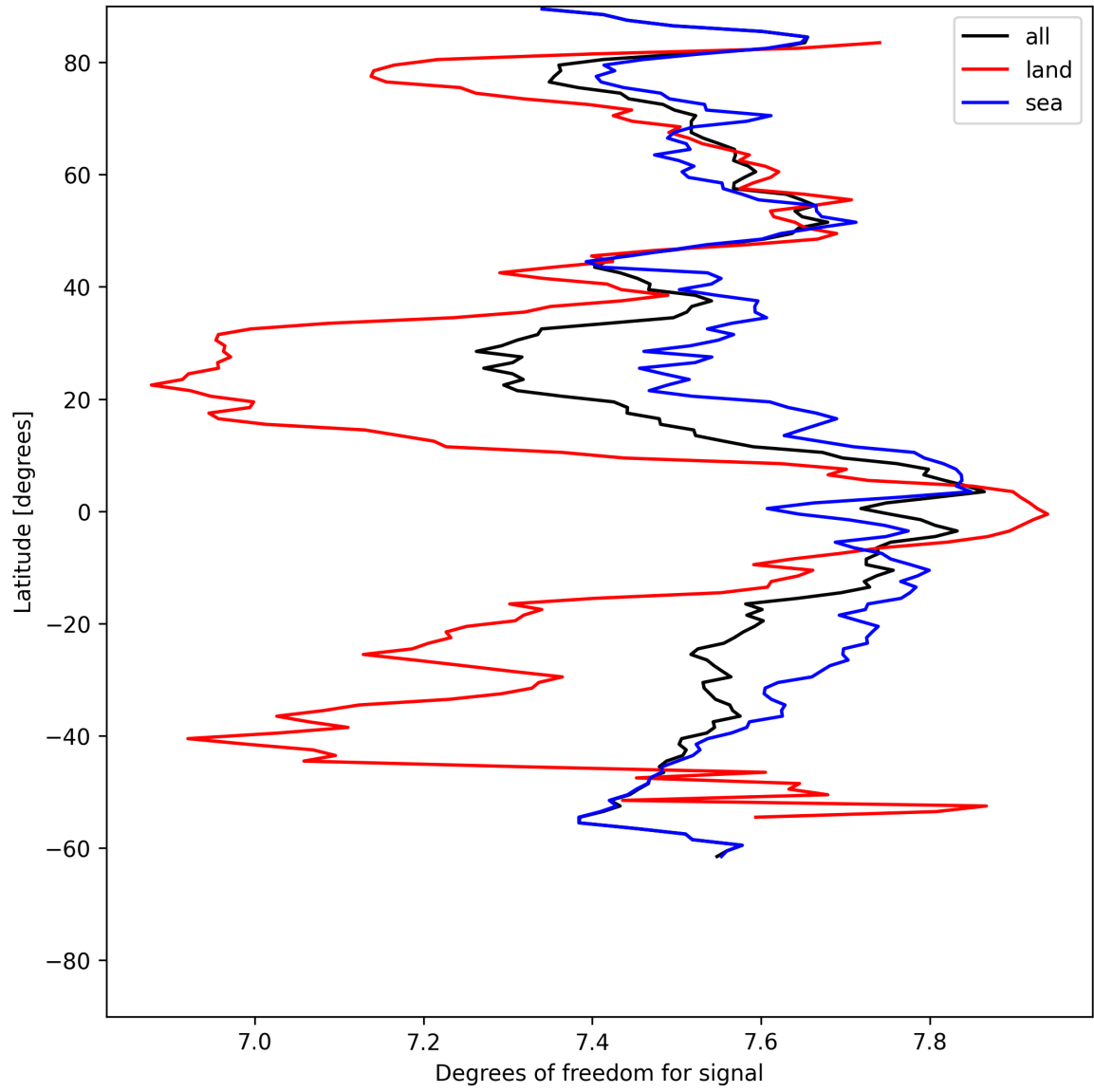
Figure 15: Zonal average of “Degrees of freedom for signal” for 2025-06-07 to 2025-06-09.
