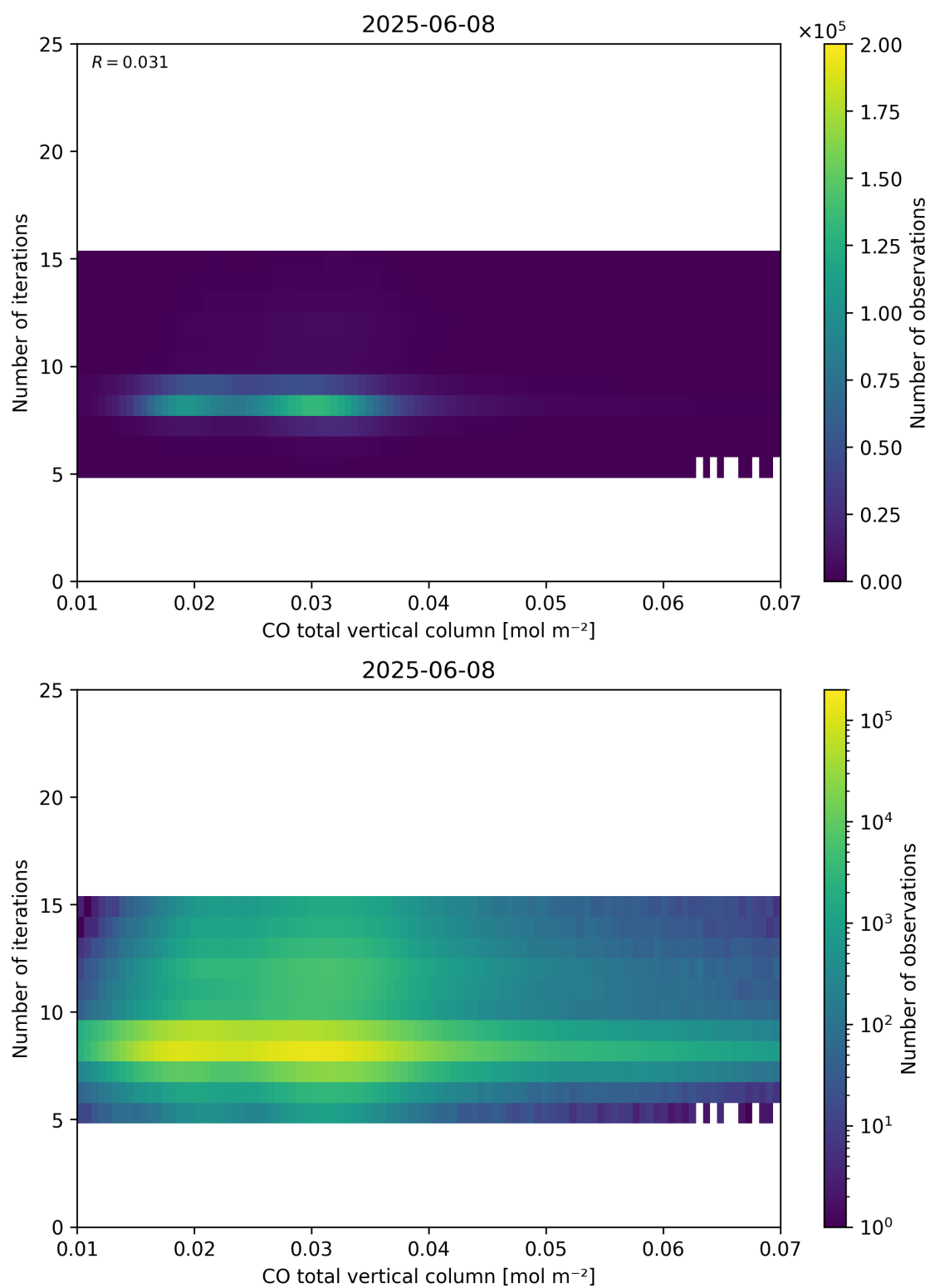
Figure 42: Scatter density plot of “CO total vertical column” against “Number of iterations” for 2025-06-07 to 2025-06-09.
