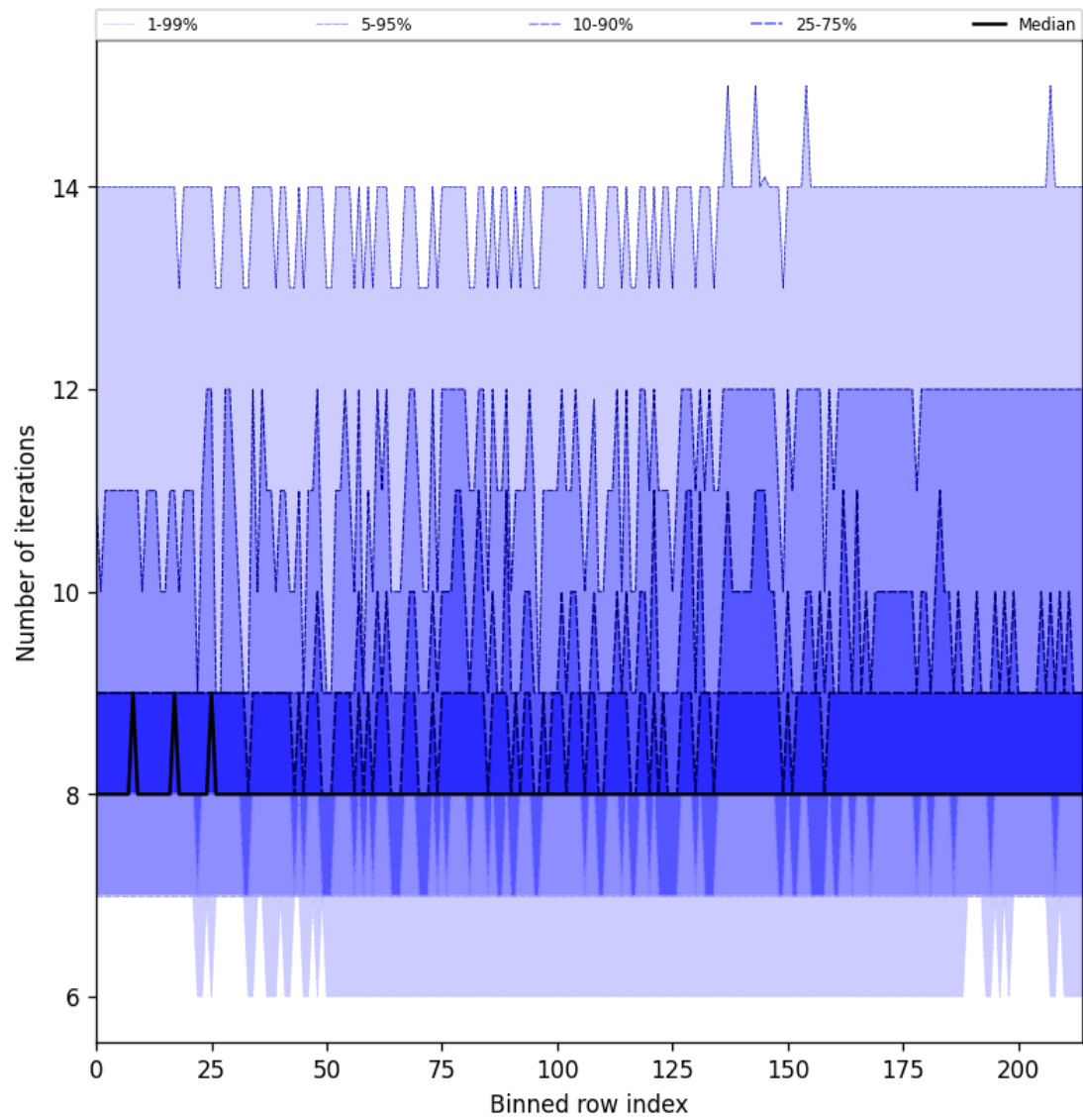
Figure 32: Along track statistics of “Number of iterations” for 2025-06-07 to 2025-06-09
