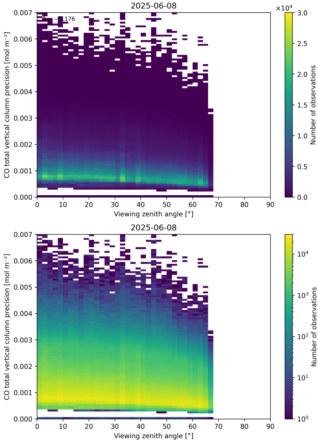
Figure 71: Scatter density plot of “Viewing zenith angle” against “CO total vertical column precision” for 2025-06-07 to 2025-06-09.
