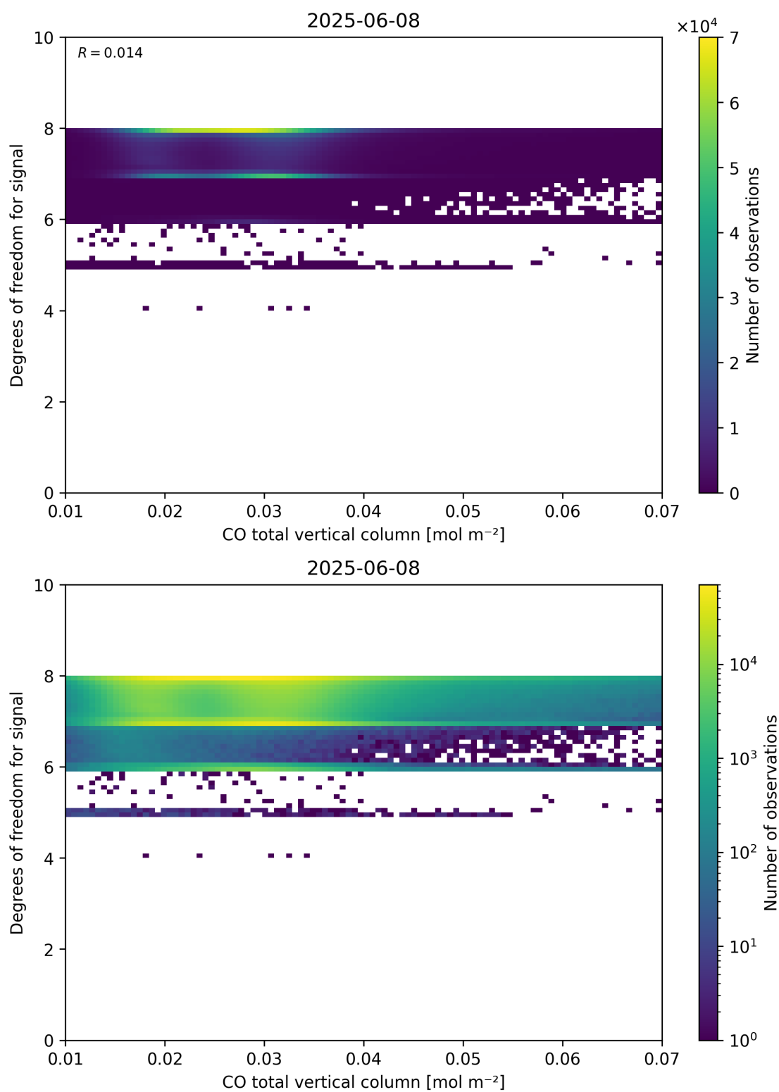
Figure 41: Scatter density plot of “CO total vertical column” against “Degrees of freedom for signal” for 2025-06-07 to 2025-06-09.
