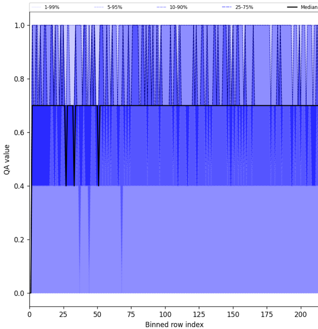
Figure 25: Along track statistics of “QA value” for 2025-06-07 to 2025-06-09
