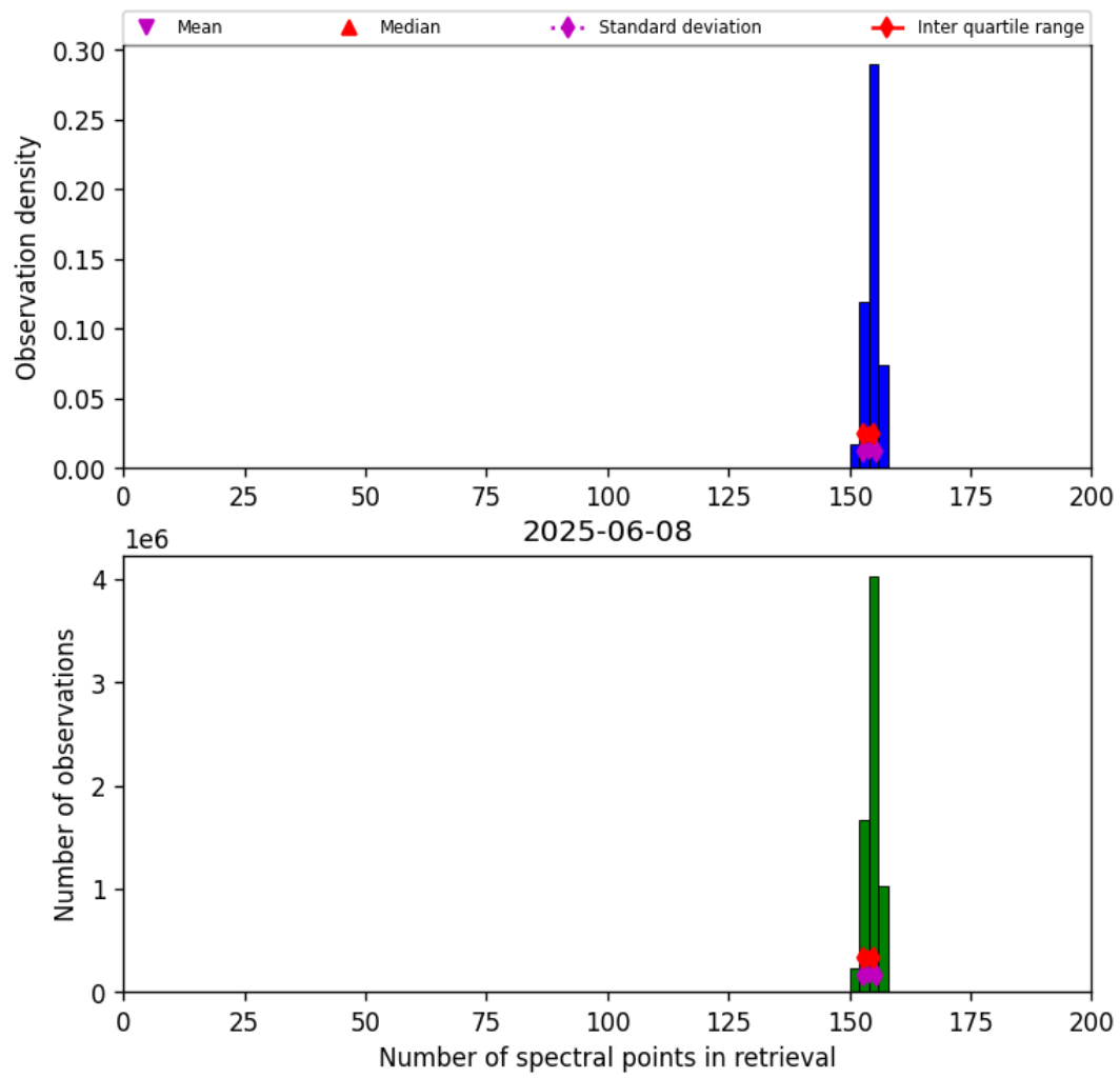
Figure 21: Histogram of “Number of spectral points in retrieval” for 2025-06-07 to 2025-06-09
