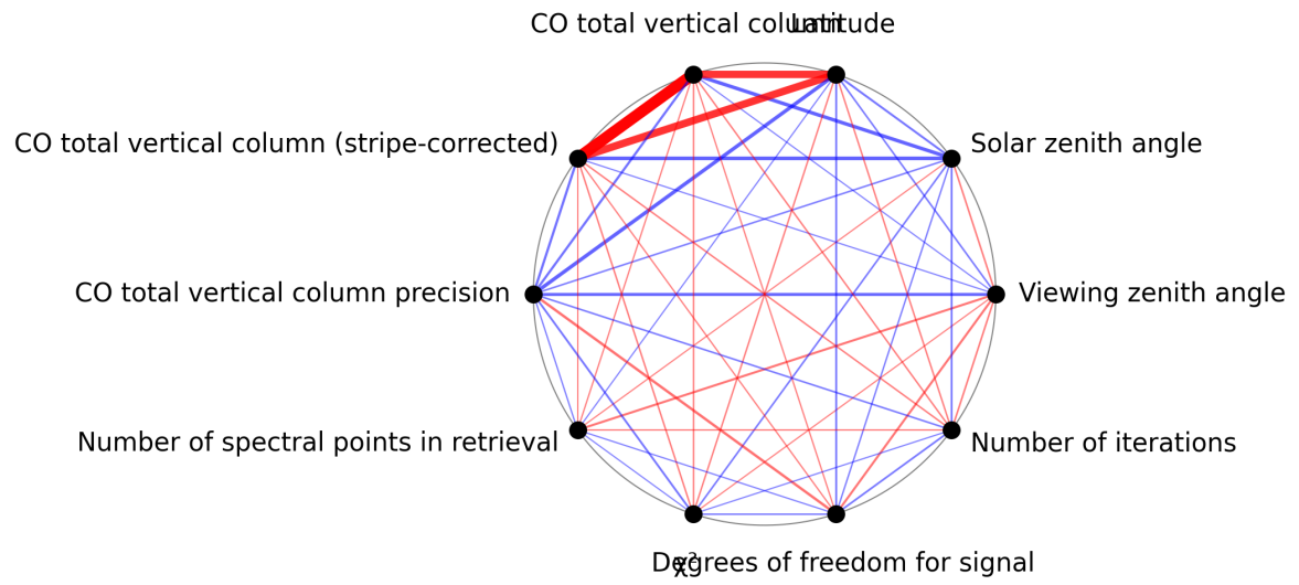
Figure 1: Map of correlation graph for 2025-06-07 to 2025-06-09.
