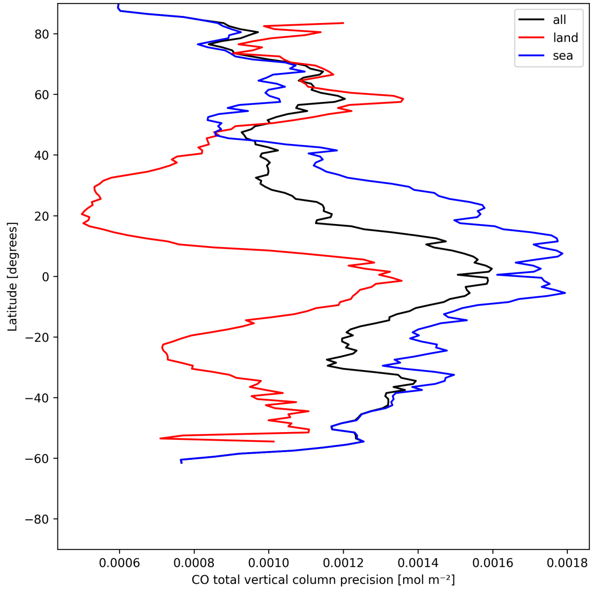
Figure 12: Zonal average of "CO total vertical column precision" for 2025-06-07 to 2025-06-09.
