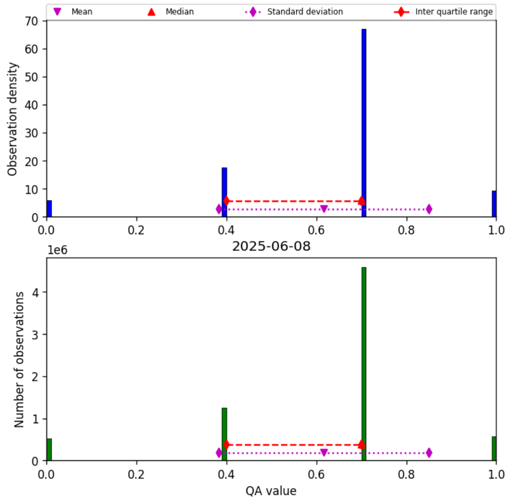
Figure 17: Histogram of “QA value” for 2025-06-07 to 2025-06-09
