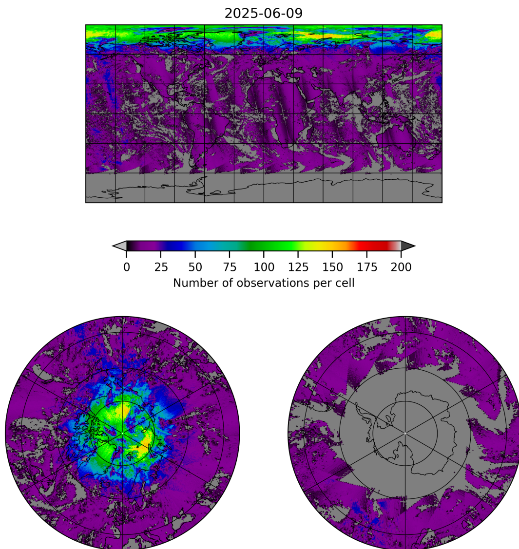
Figure 8: Map of the number of observations for 2025-06-08 to 2025-06-10
