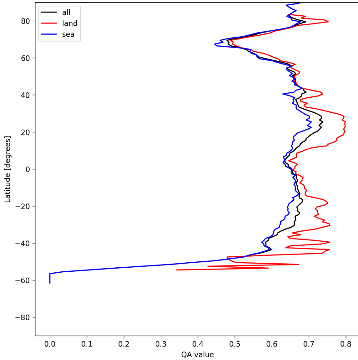
Figure 9: Zonal average of “QA value” for 2025-06-08 to 2025-06-10.
