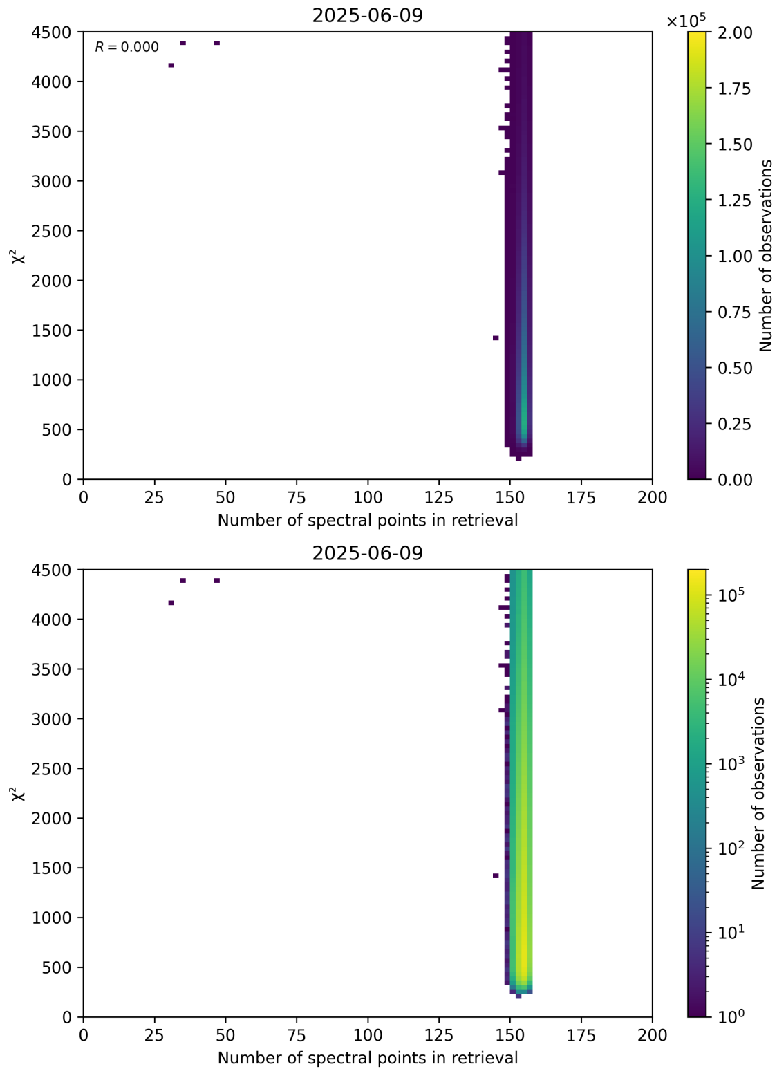
Figure 58: Scatter density plot of “Number of spectral points in retrieval” against “ \chi^2 ” for 2025-06-08 to 2025-06-10.
