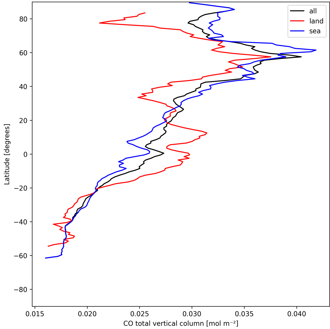
Figure 10: Zonal average of “CO total vertical column” for 2025-06-08 to 2025-06-10.
