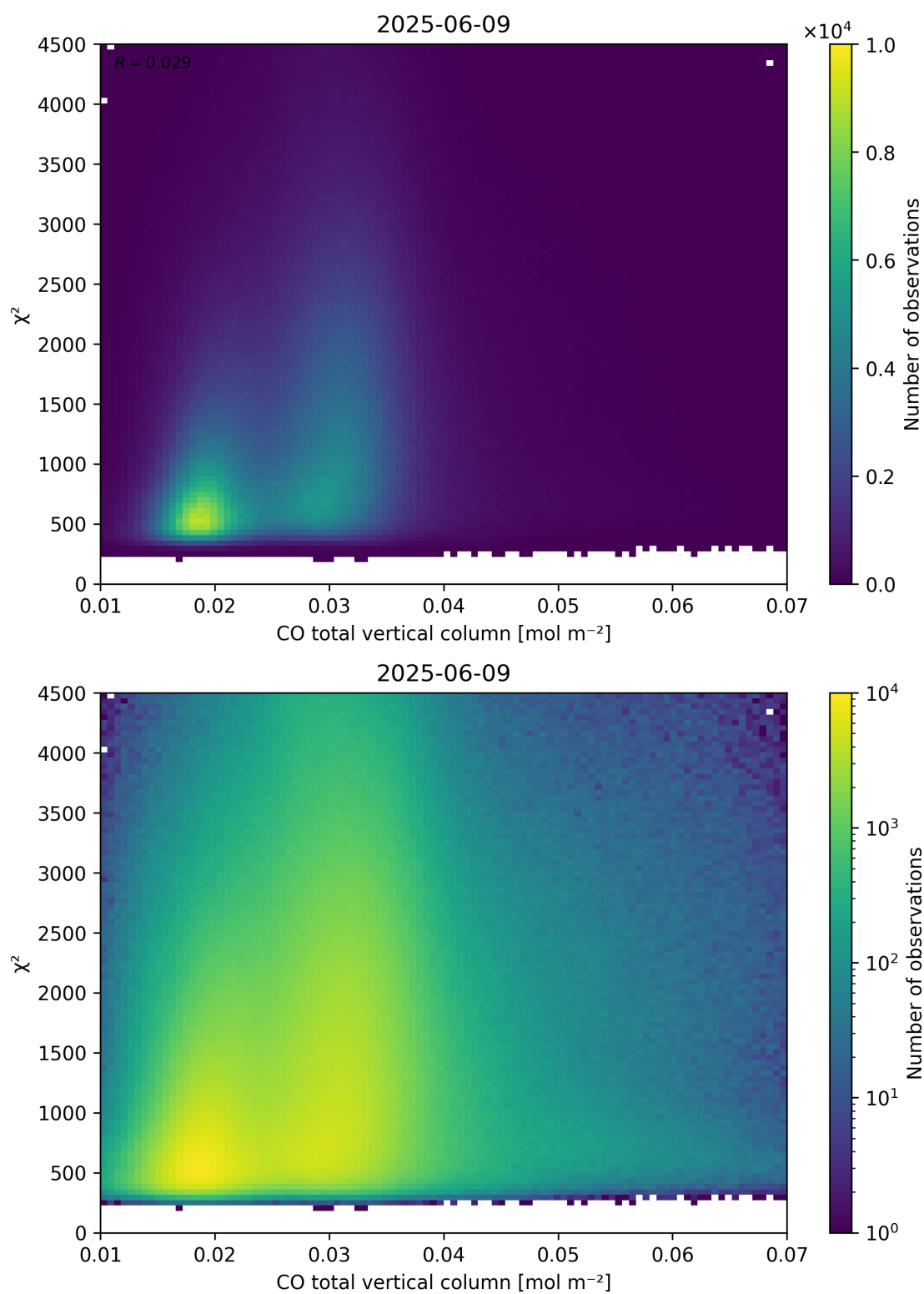
Figure 35: Scatter density plot of “CO total vertical column” against “ \chi^2 ” for 2025-06-08 to 2025-06-10.
