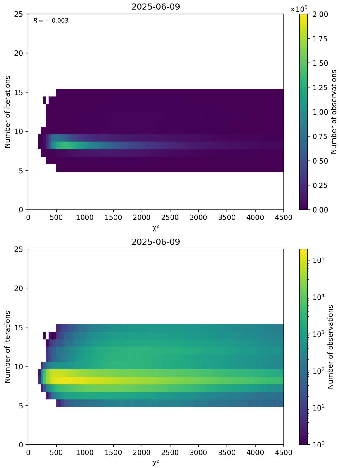
Figure 49: Scatter density plot of “ \chi^2 ” against “Number of iterations” for 2025-06-08 to 2025-06-10.
