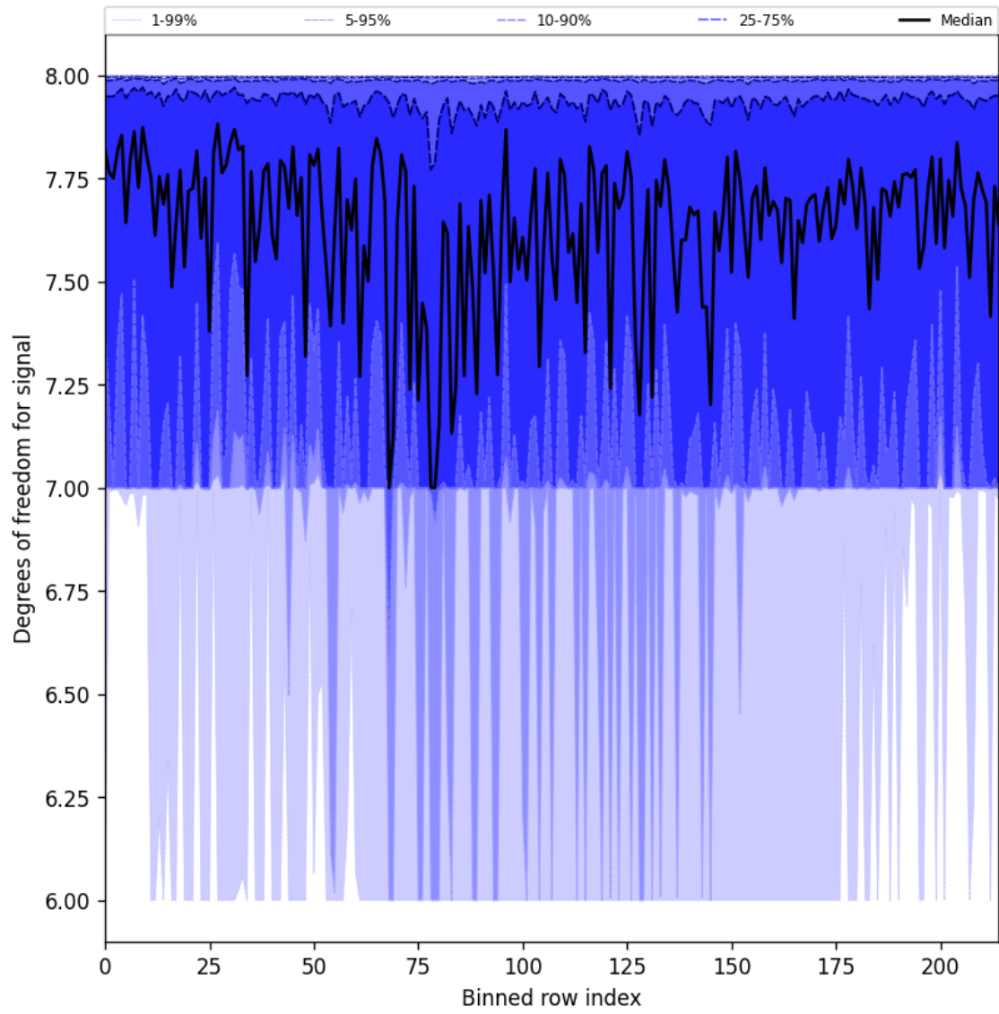
Figure 31: Along track statistics of “Degrees of freedom for signal” for 2025-06-08 to 2025-06-10
