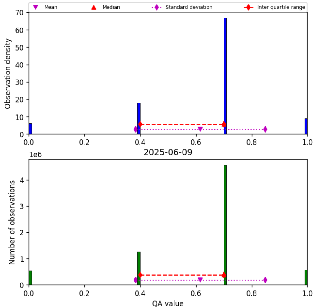
Figure 17: Histogram of “QA value” for 2025-06-08 to 2025-06-10
