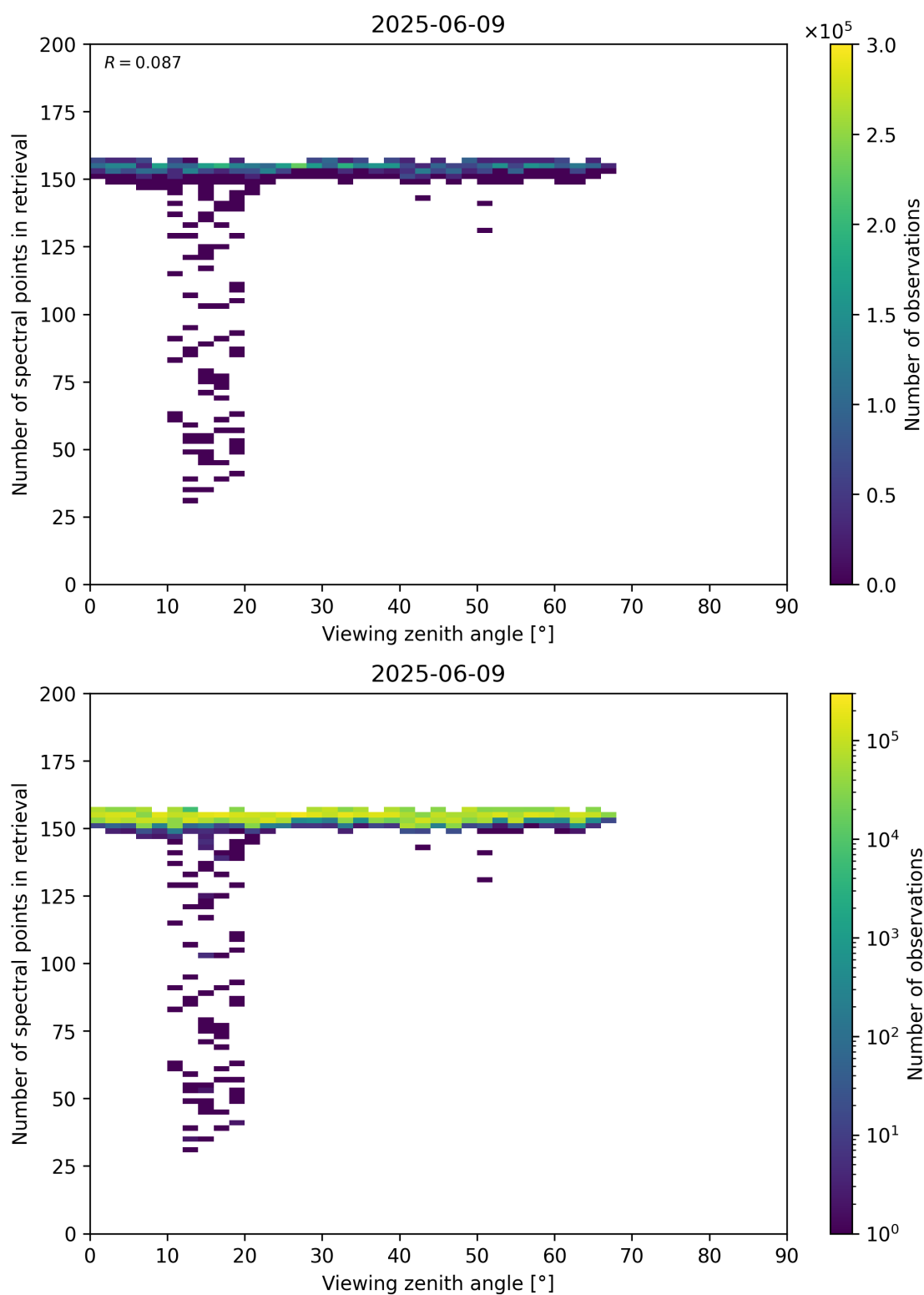
Figure 76: Scatter density plot of “Viewing zenith angle” against “Number of spectral points in retrieval” for 2025-06-08 to 2025-06-10.
