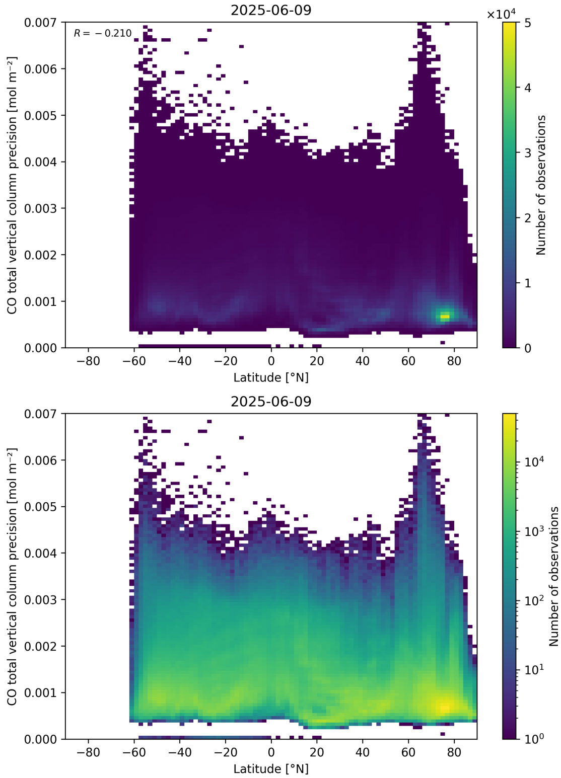
Figure 53: Scatter density plot of “Latitude” against “CO total vertical column precision” for 2025-06-08 to 2025-06-10.
