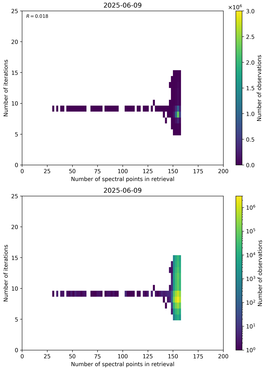
Figure 60: Scatter density plot of “Number of spectral points in retrieval” against “Number of iterations” for 2025-06-08 to 2025-06-10.
