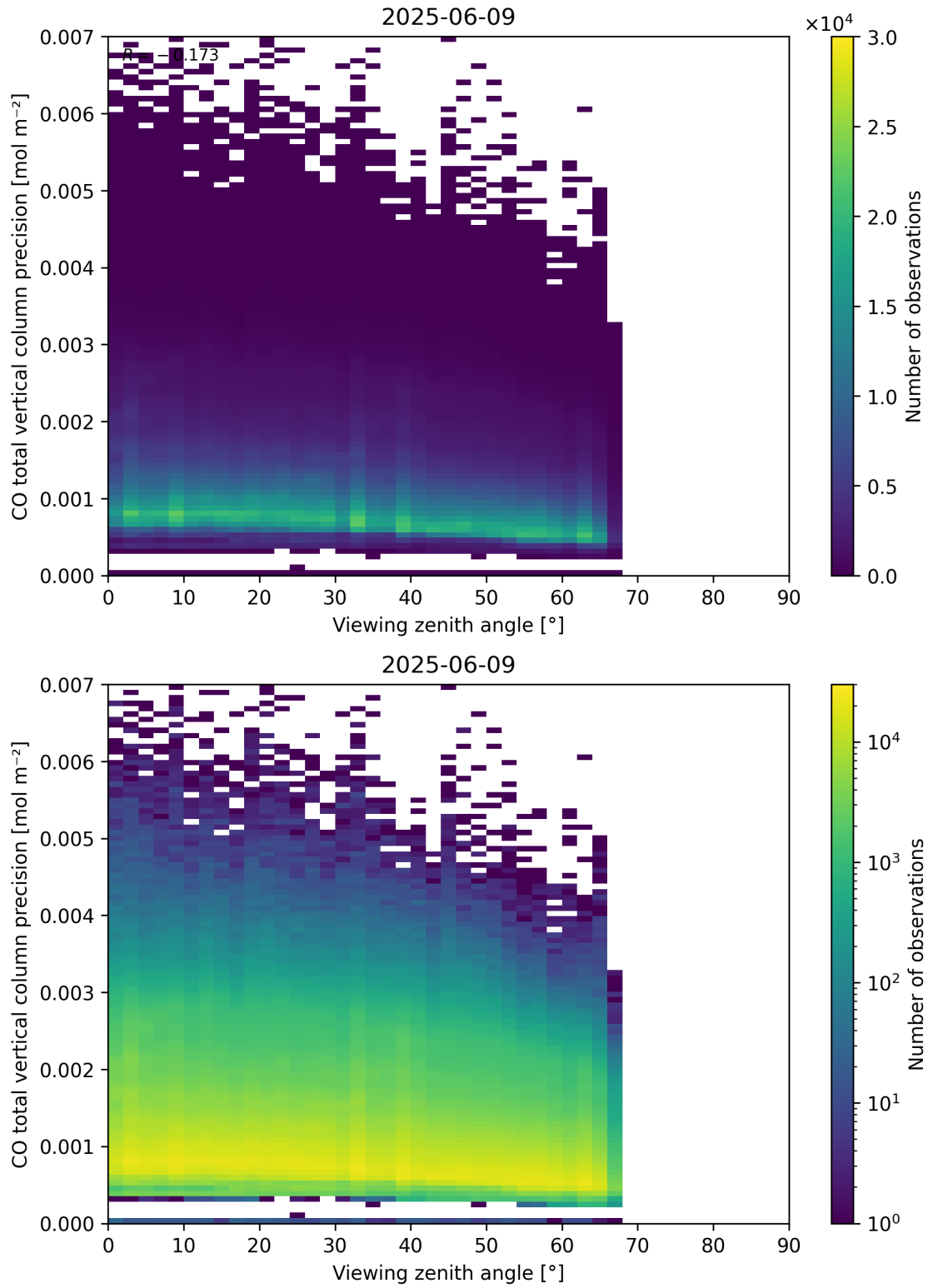
Figure 71: Scatter density plot of “Viewing zenith angle” against “CO total vertical column precision” for 2025-06-08 to 2025-06-10.
