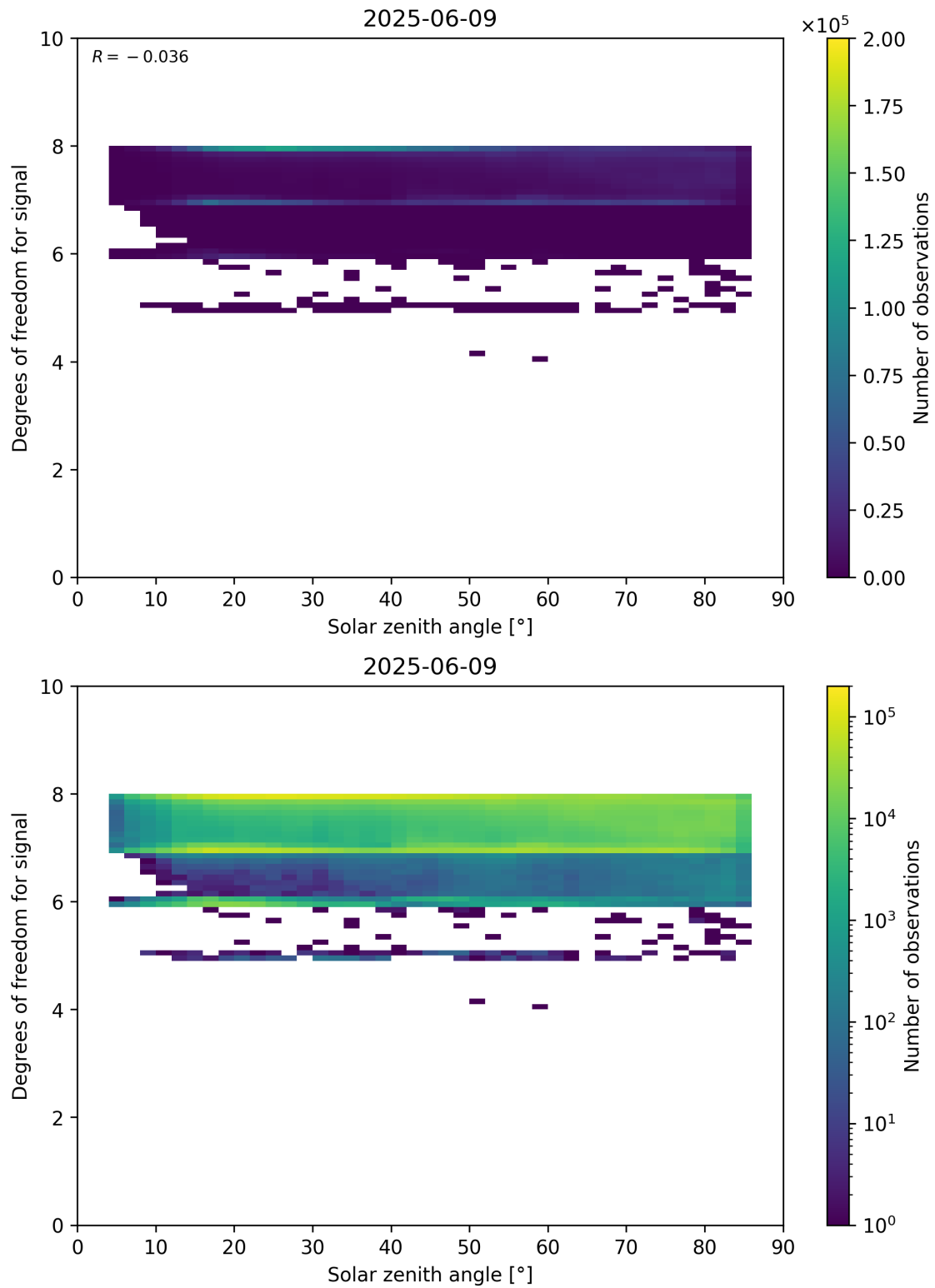
Figure 65: Scatter density plot of “Solar zenith angle” against “Degrees of freedom for signal” for 2025-06-08 to 2025-06-10.
