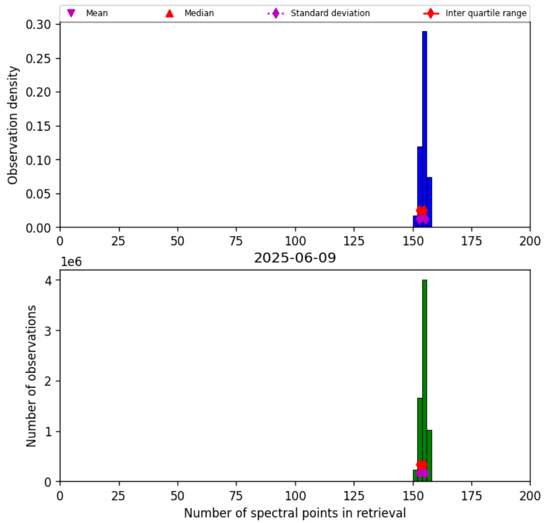
Figure 21: Histogram of “Number of spectral points in retrieval” for 2025-06-08 to 2025-06-10
