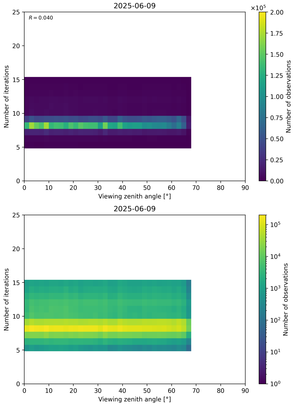
Figure 75: Scatter density plot of “Viewing zenith angle” against “Number of iterations” for 2025-06-08 to 2025-06-10.
