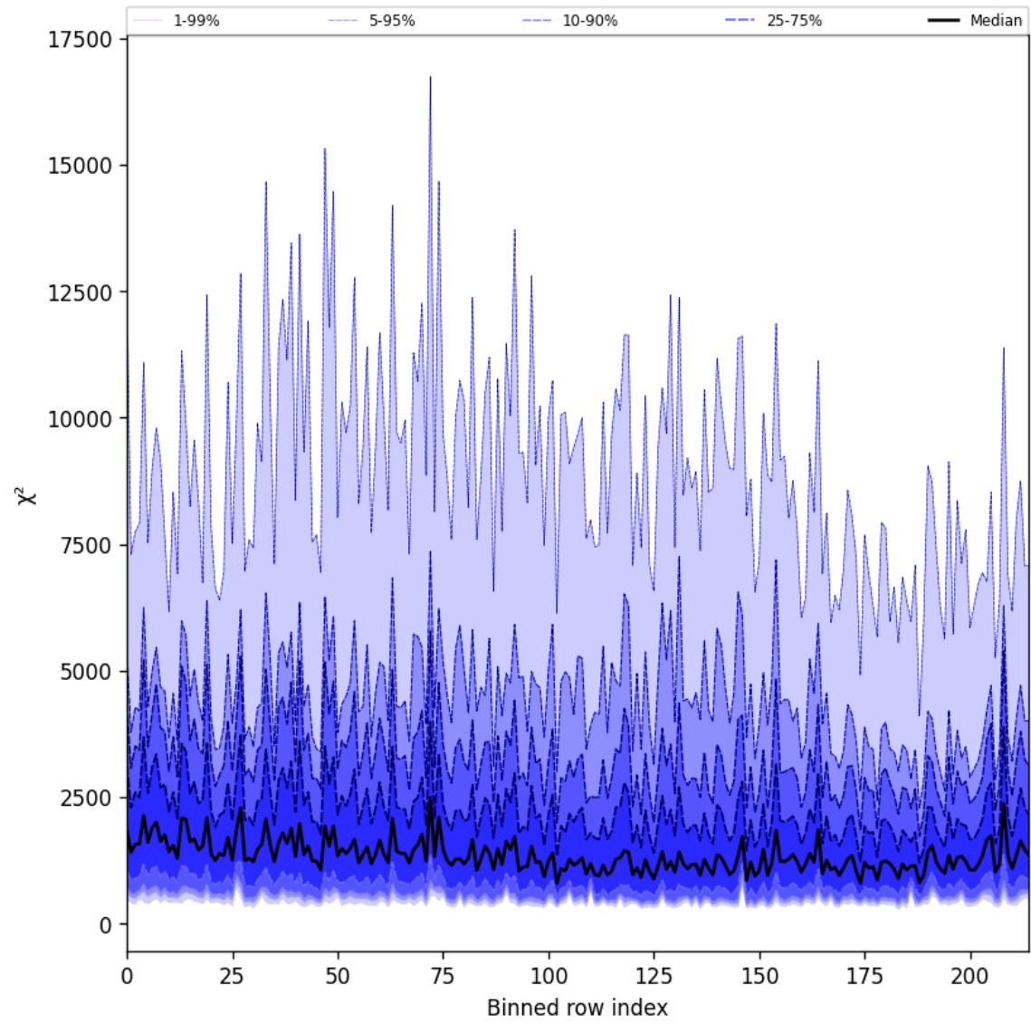
Figure 30: Along track statistics of “ \chi^2 ” for 2025-06-08 to 2025-06-10
