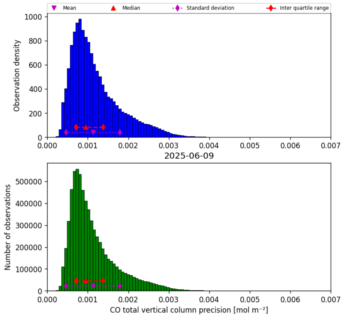
Figure 20: Histogram of “CO total vertical column precision” for 2025-06-08 to 2025-06-10
