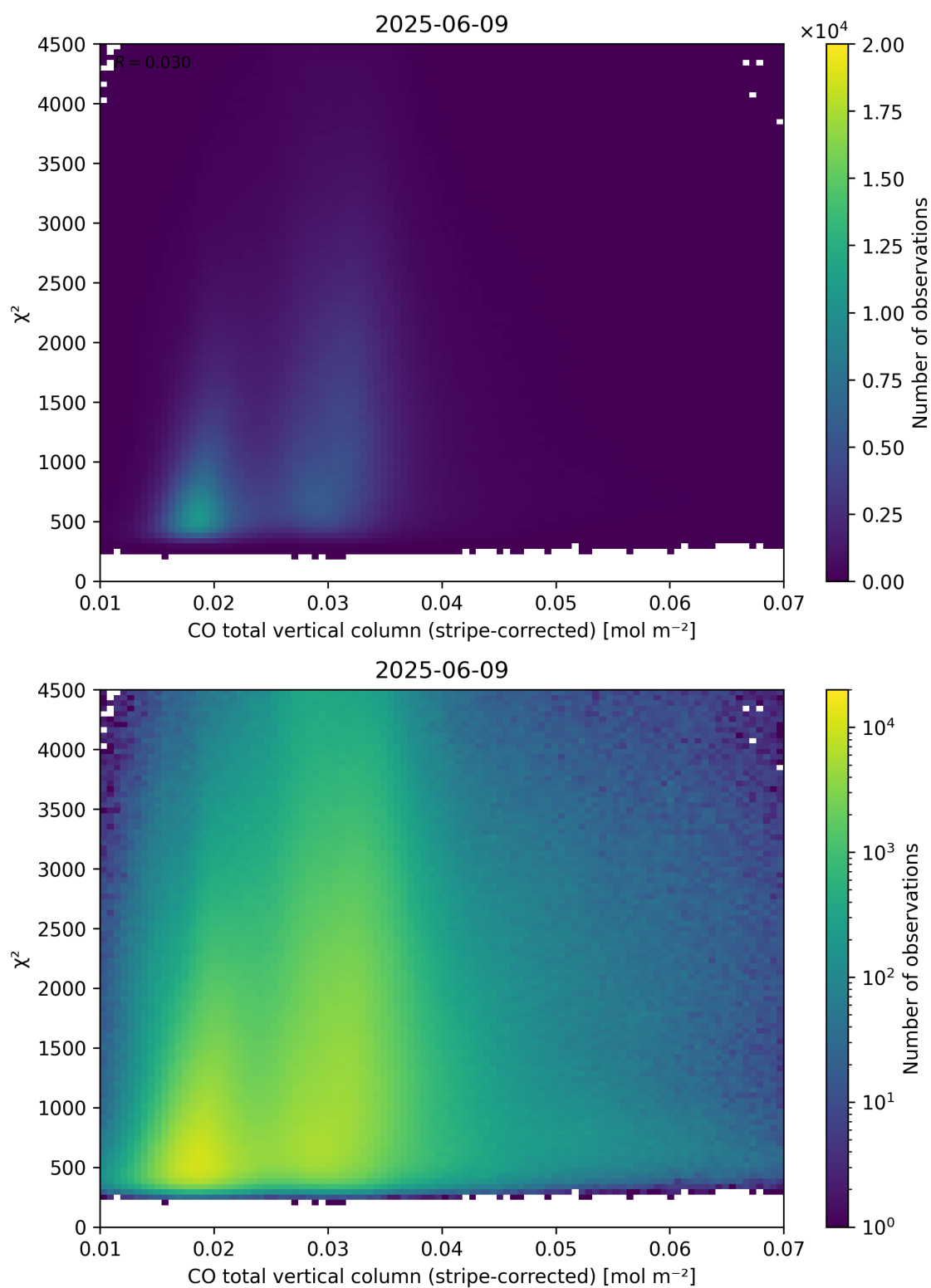
Figure 37: Scatter density plot of “CO total vertical column (stripe-corrected)” against “ \chi^2 ” for 2025-06-08 to 2025-06-10.
