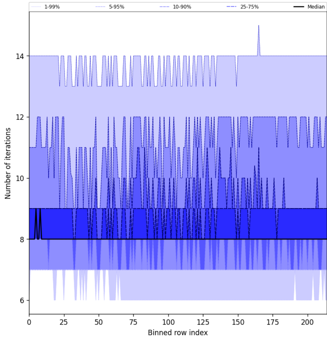
Figure 32: Along track statistics of “Number of iterations” for 2025-06-08 to 2025-06-10
