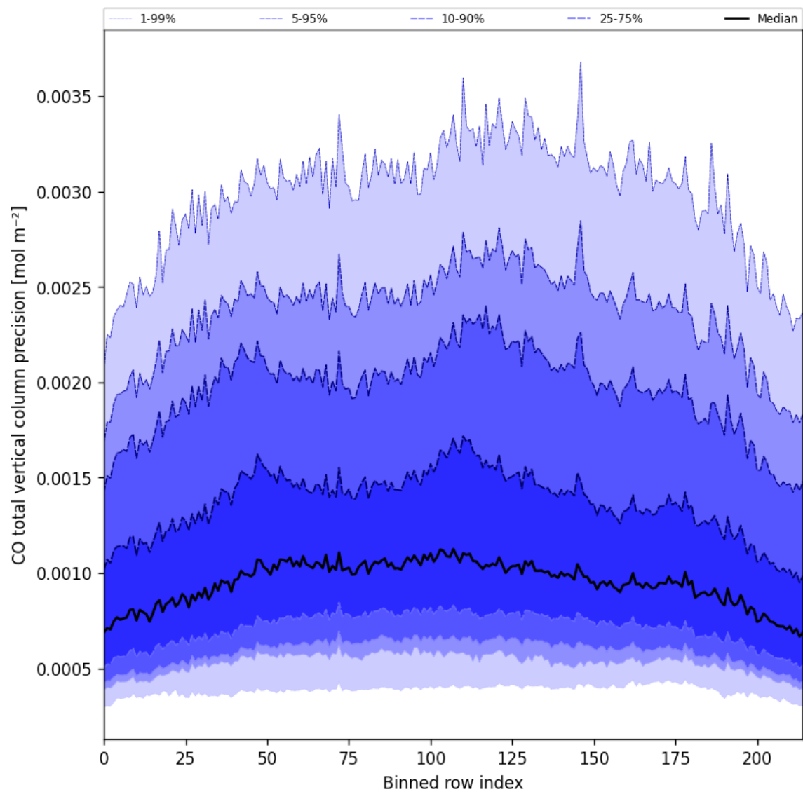
Figure 28: Along track statistics of “CO total vertical column precision” for 2025-06-08 to 2025-06-10
