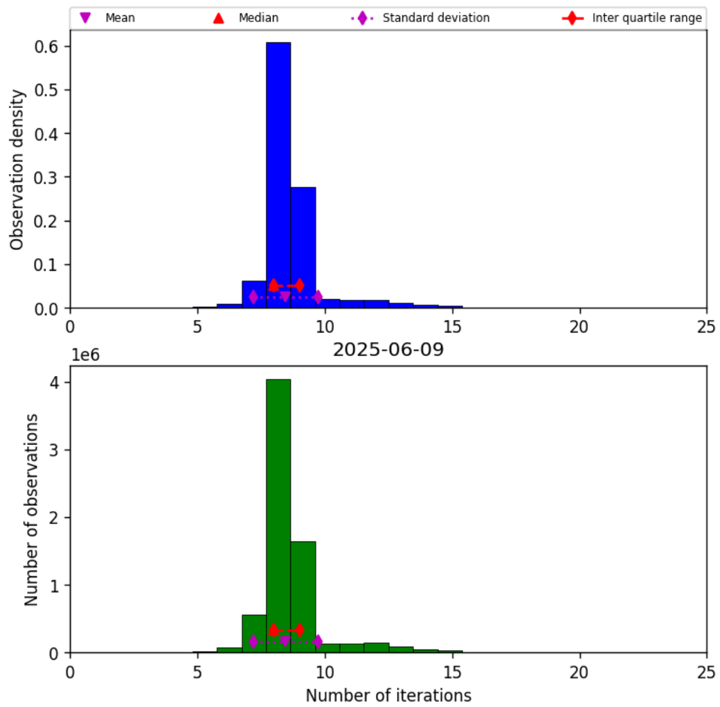
Figure 24: Histogram of “Number of iterations” for 2025-06-08 to 2025-06-10
