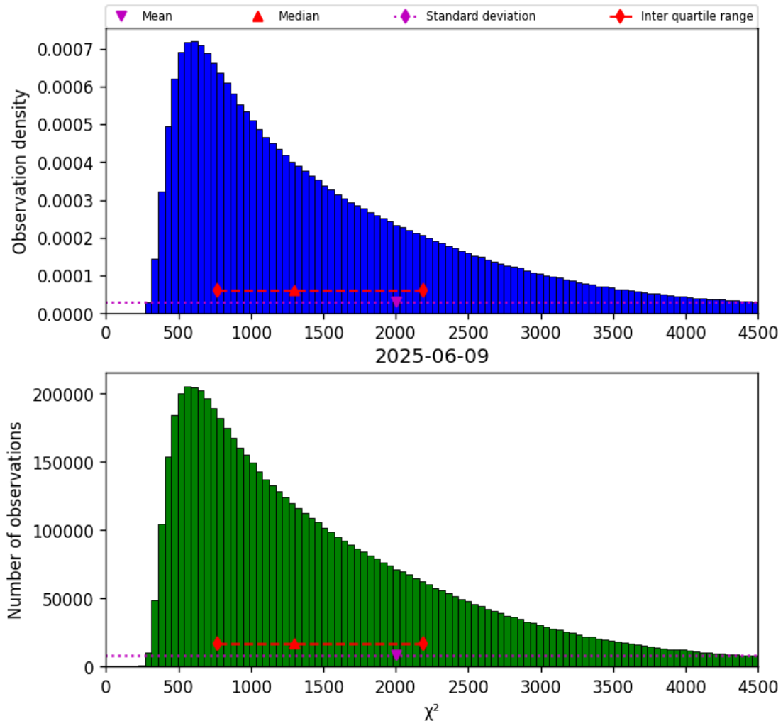
Figure 22: Histogram of “ \chi^2 ” for 2025-06-08 to 2025-06-10
