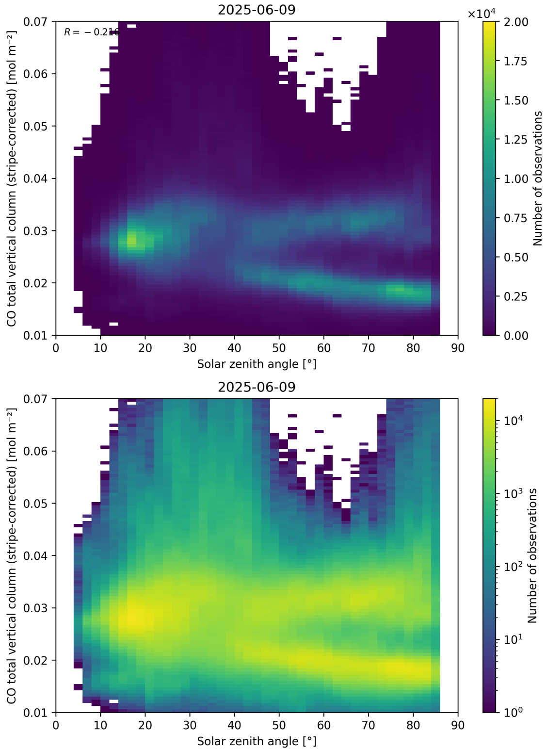
Figure 62: Scatter density plot of “Solar zenith angle” against “CO total vertical column (stripe-corrected)” for 2025-06-08 to 2025-06-10.
