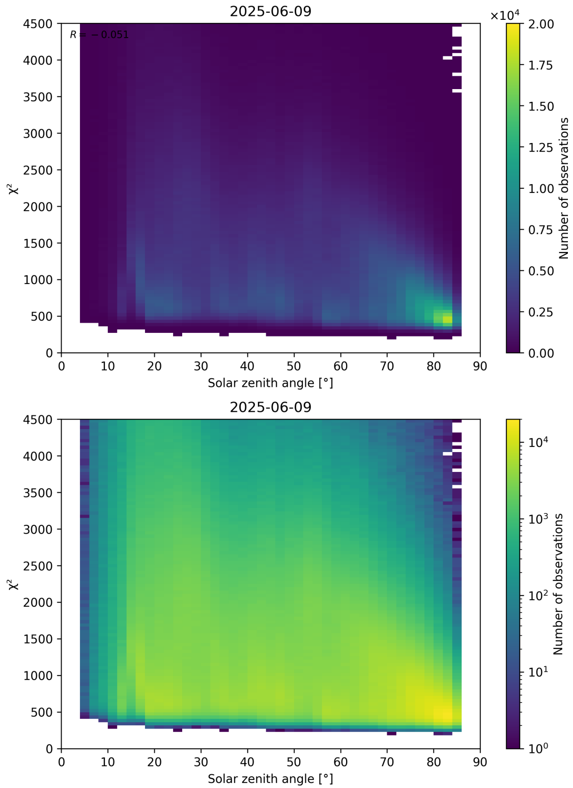
Figure 64: Scatter density plot of “Solar zenith angle” against “ \chi^2 ” for 2025-06-08 to 2025-06-10.
