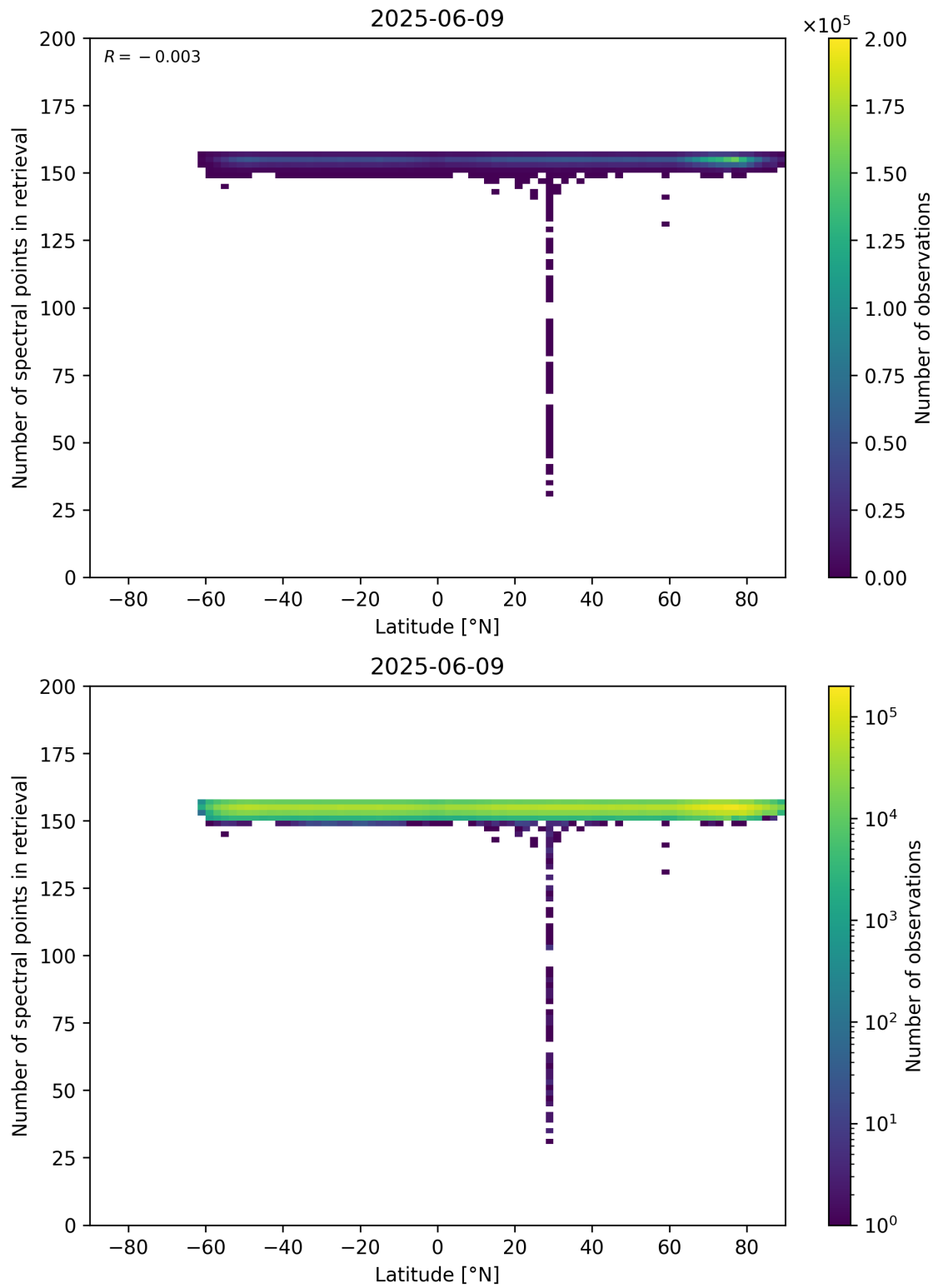
Figure 57: Scatter density plot of “Latitude” against “Number of spectral points in retrieval” for 2025-06-08 to 2025-06-10.
