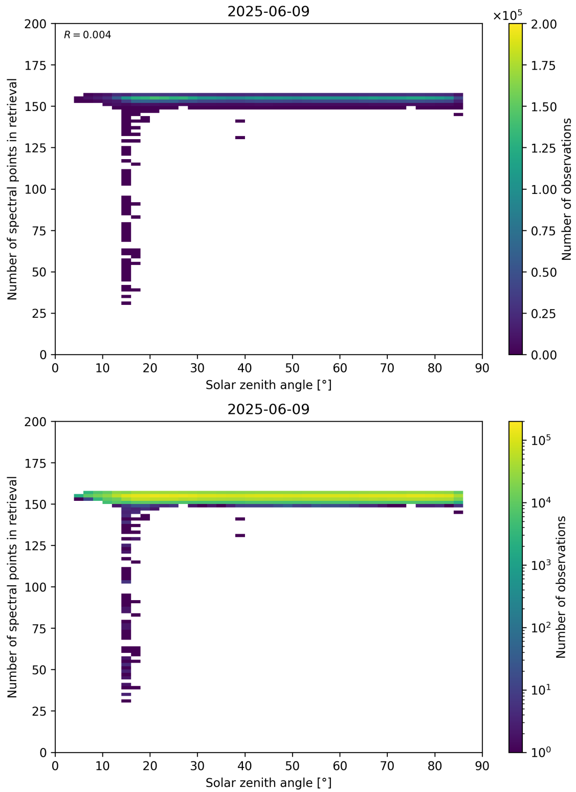
Figure 68: Scatter density plot of “Solar zenith angle” against “Number of spectral points in retrieval” for 2025-06-08 to 2025-06-10.
