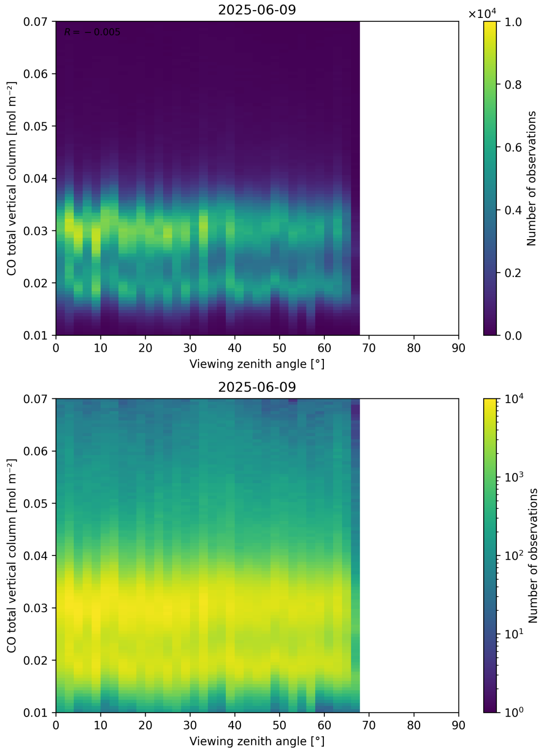
Figure 69: Scatter density plot of “Viewing zenith angle” against “CO total vertical column” for 2025-06-08 to 2025-06-10.
