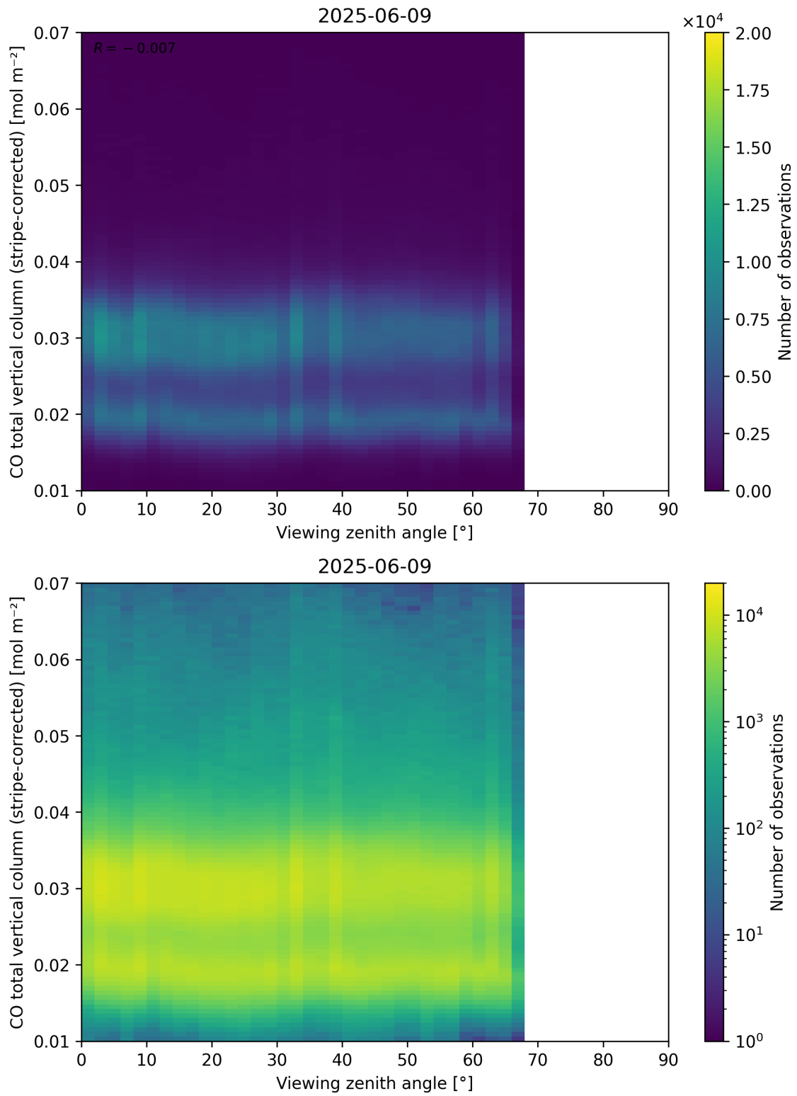
Figure 70: Scatter density plot of “Viewing zenith angle” against “CO total vertical column (stripe-corrected)” for 2025-06-08 to 2025-06-10.
