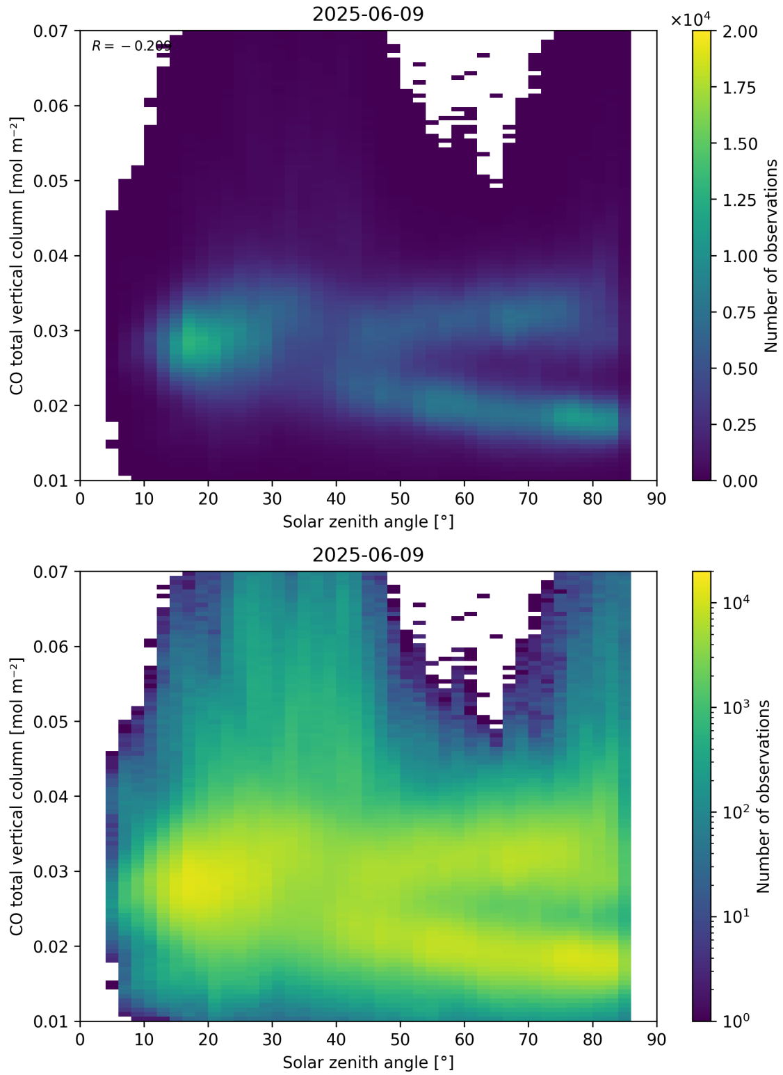
Figure 61: Scatter density plot of “Solar zenith angle” against “CO total vertical column” for 2025-06-08 to 2025-06-10.
