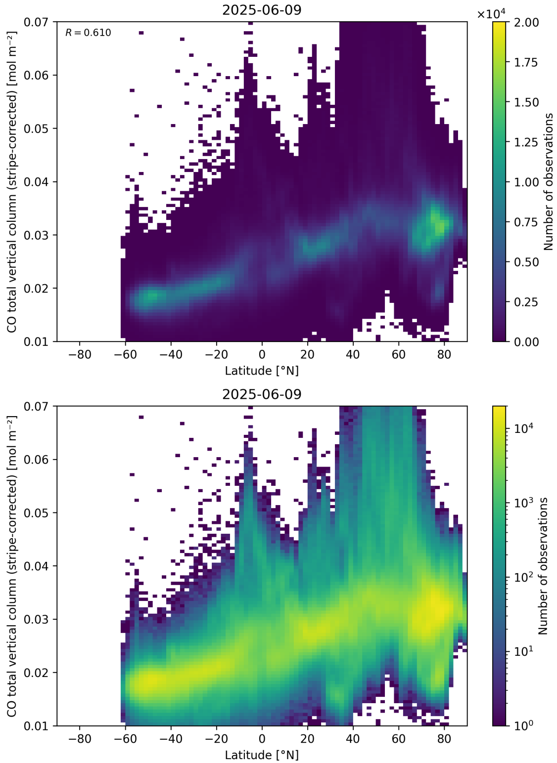
Figure 52: Scatter density plot of “Latitude” against “CO total vertical column (stripe-corrected)” for 2025-06-08 to 2025-06-10.
