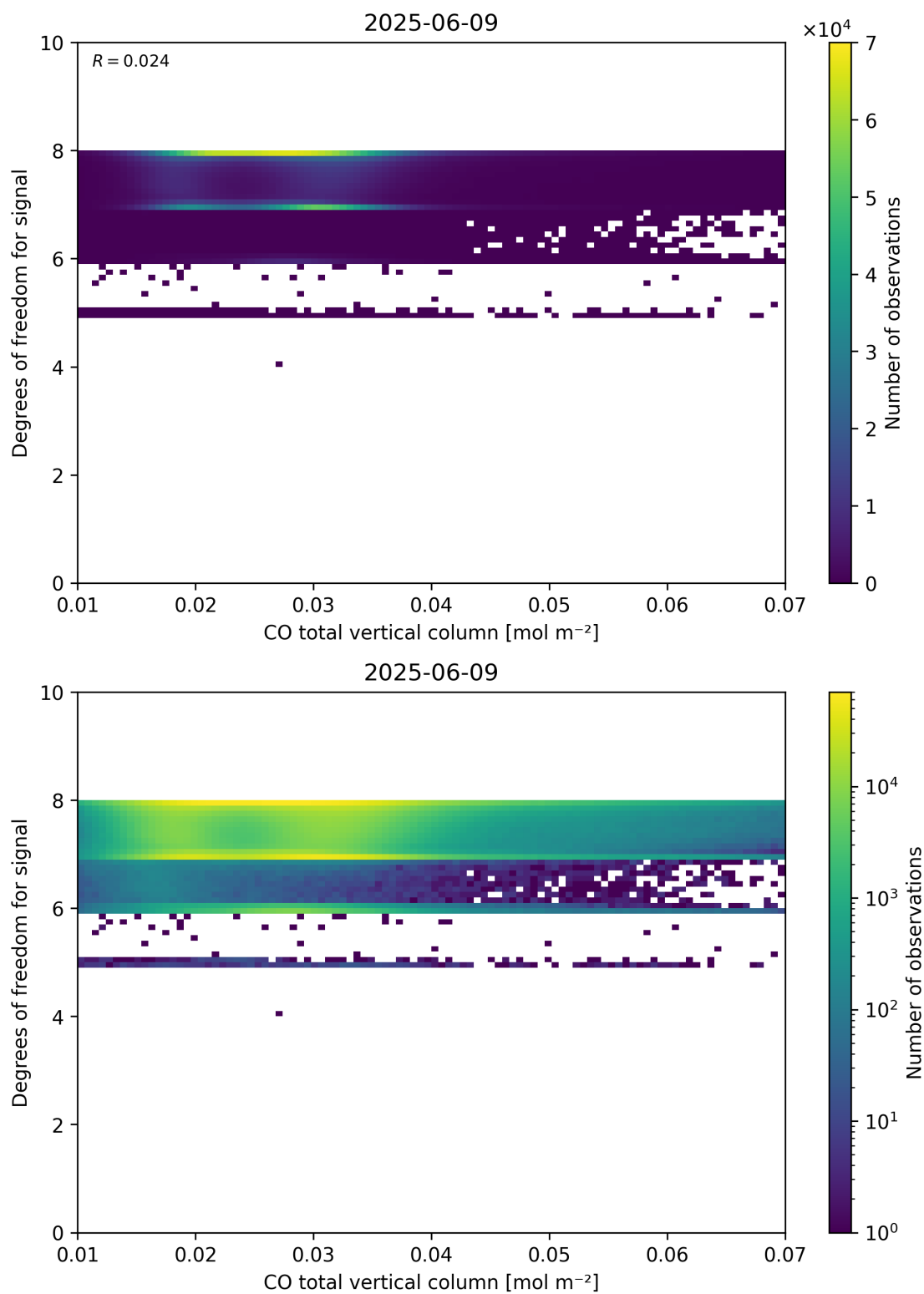
Figure 41: Scatter density plot of “CO total vertical column” against “Degrees of freedom for signal” for 2025-06-08 to 2025-06-10.
