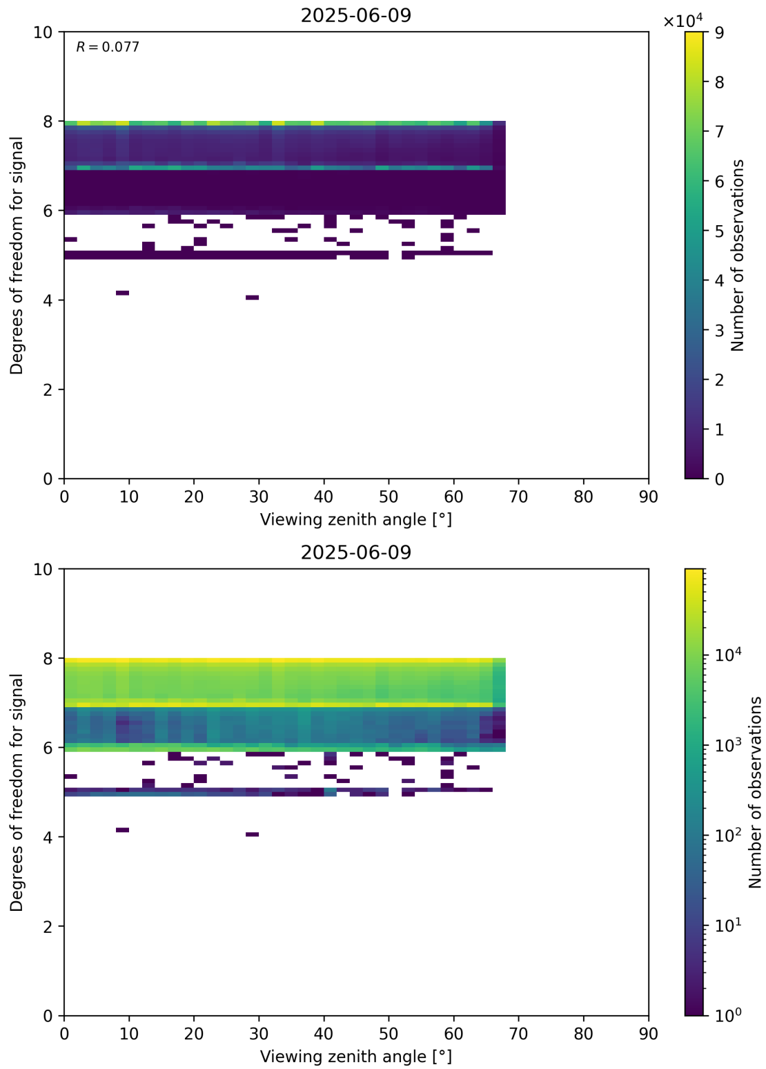
Figure 73: Scatter density plot of “Viewing zenith angle” against “Degrees of freedom for signal” for 2025-06-08 to 2025-06-10.
