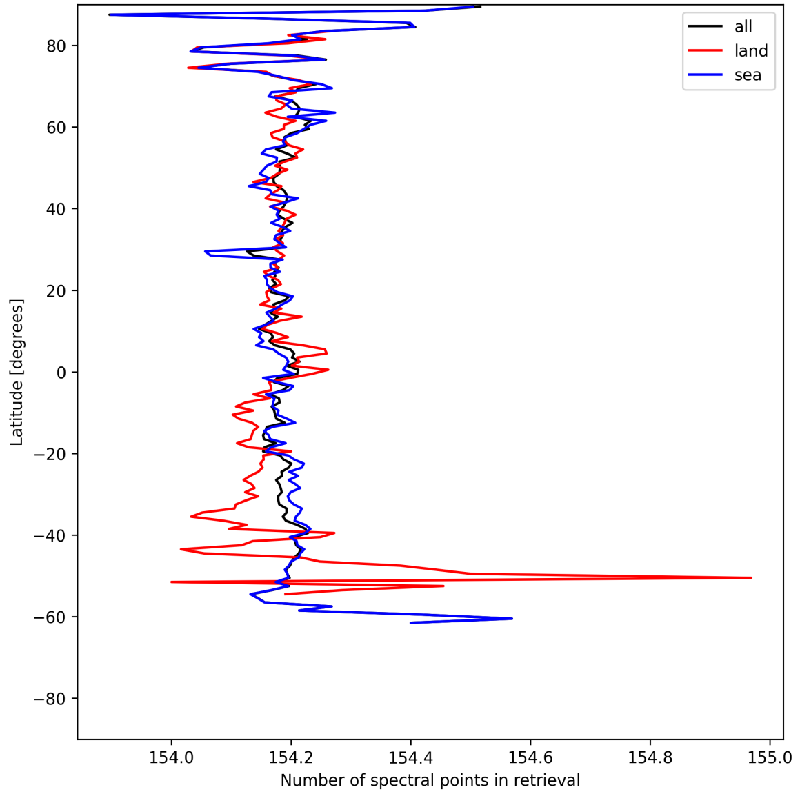
Figure 13: Zonal average of “Number of spectral points in retrieval” for 2025-06-08 to 2025-06-10.
