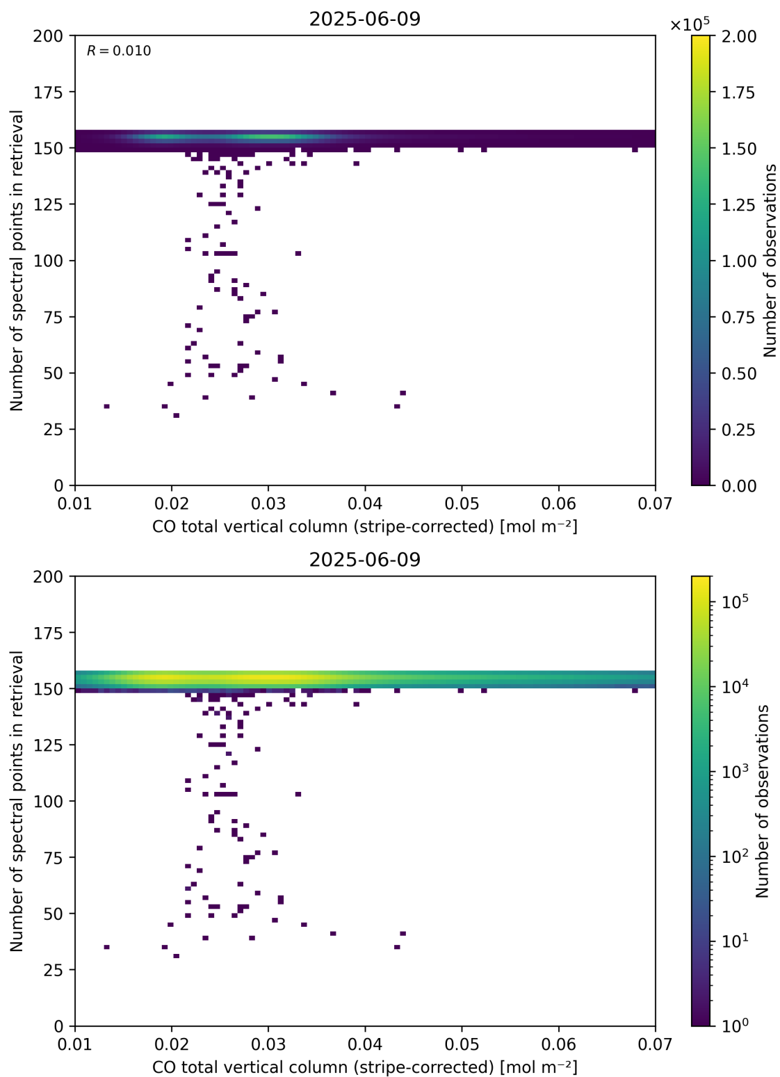
Figure 40: Scatter density plot of “CO total vertical column (stripe-corrected)” against “Number of spectral points in retrieval” for 2025-06-08 to 2025-06-10.
