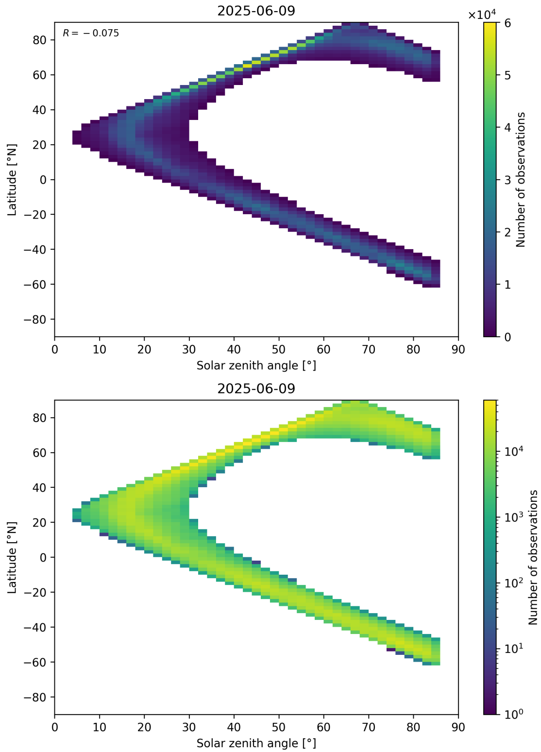
Figure 66: Scatter density plot of “Solar zenith angle” against “Latitude” for 2025-06-08 to 2025-06-10.
