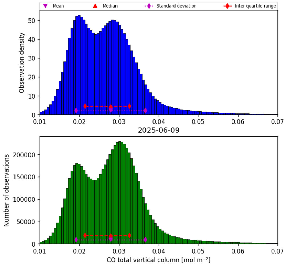
Figure 18: Histogram of “CO total vertical column” for 2025-06-08 to 2025-06-10
