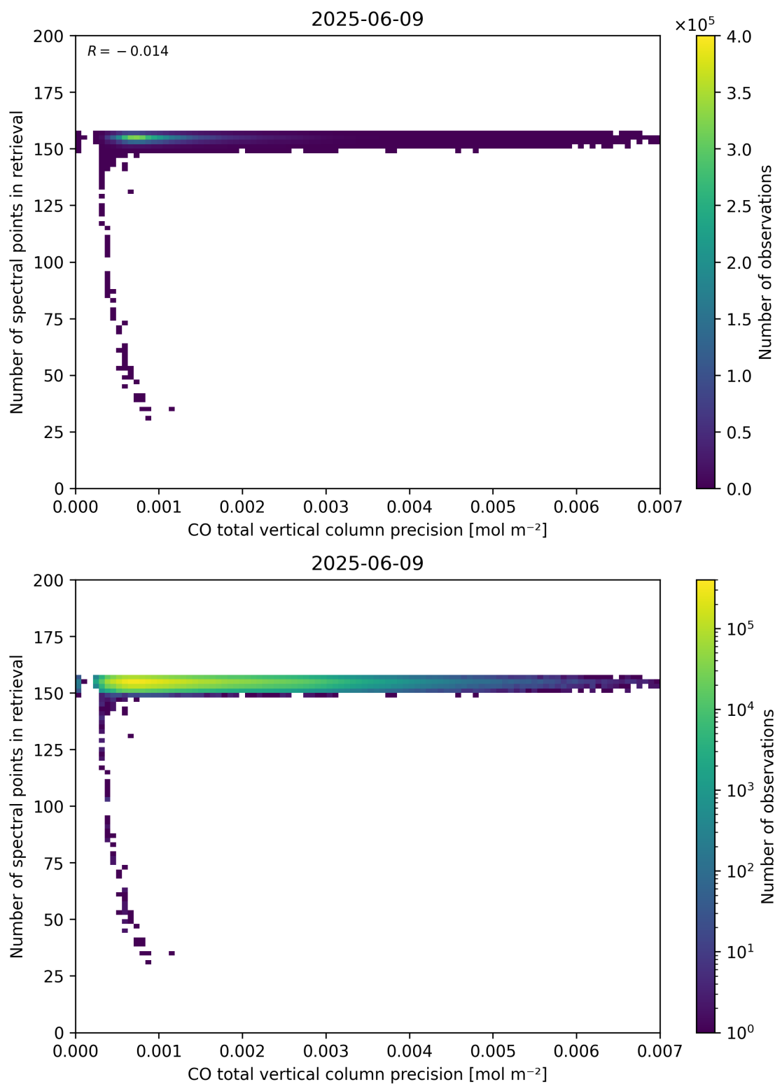
Figure 47: Scatter density plot of “CO total vertical column precision” against “Number of spectral points in retrieval” for 2025-06-08 to 2025-06-10.
