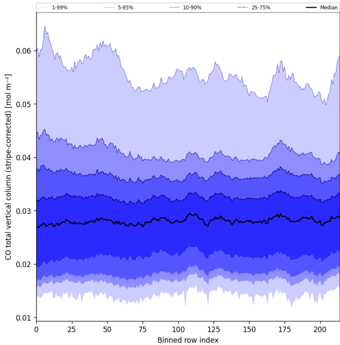
Figure 27: Along track statistics of “CO total vertical column (stripe-corrected)” for 2025-06-08 to 2025-06-10
