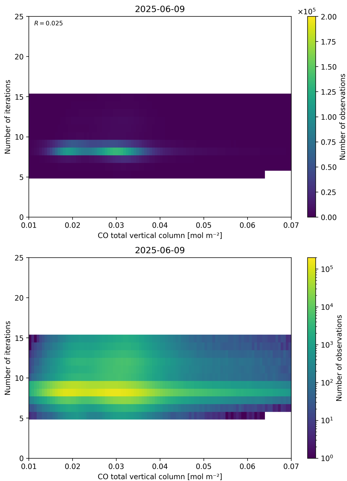
Figure 42: Scatter density plot of “CO total vertical column” against “Number of iterations” for 2025-06-08 to 2025-06-10.
