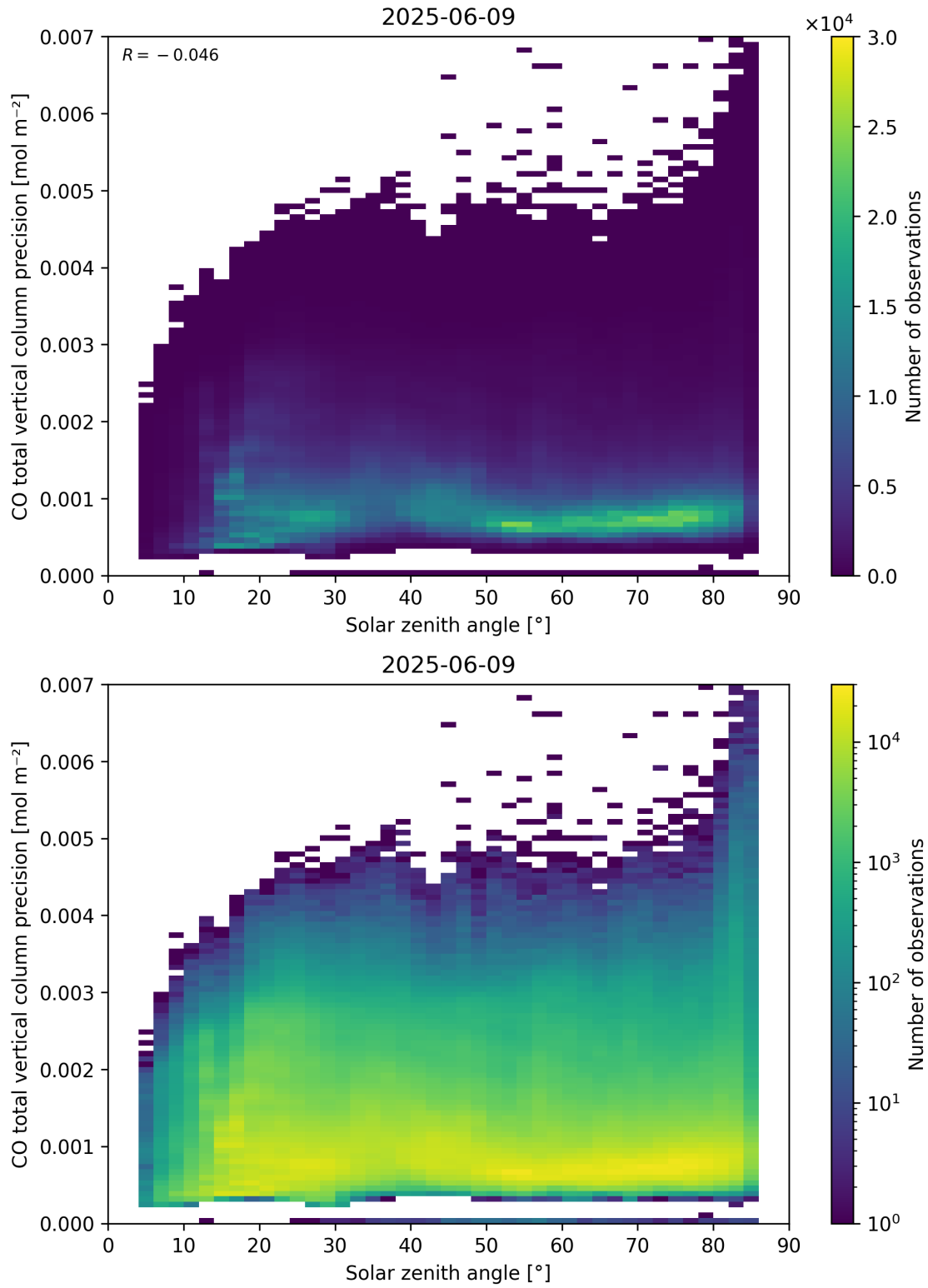
Figure 63: Scatter density plot of “Solar zenith angle” against “CO total vertical column precision” for 2025-06-08 to 2025-06-10.
