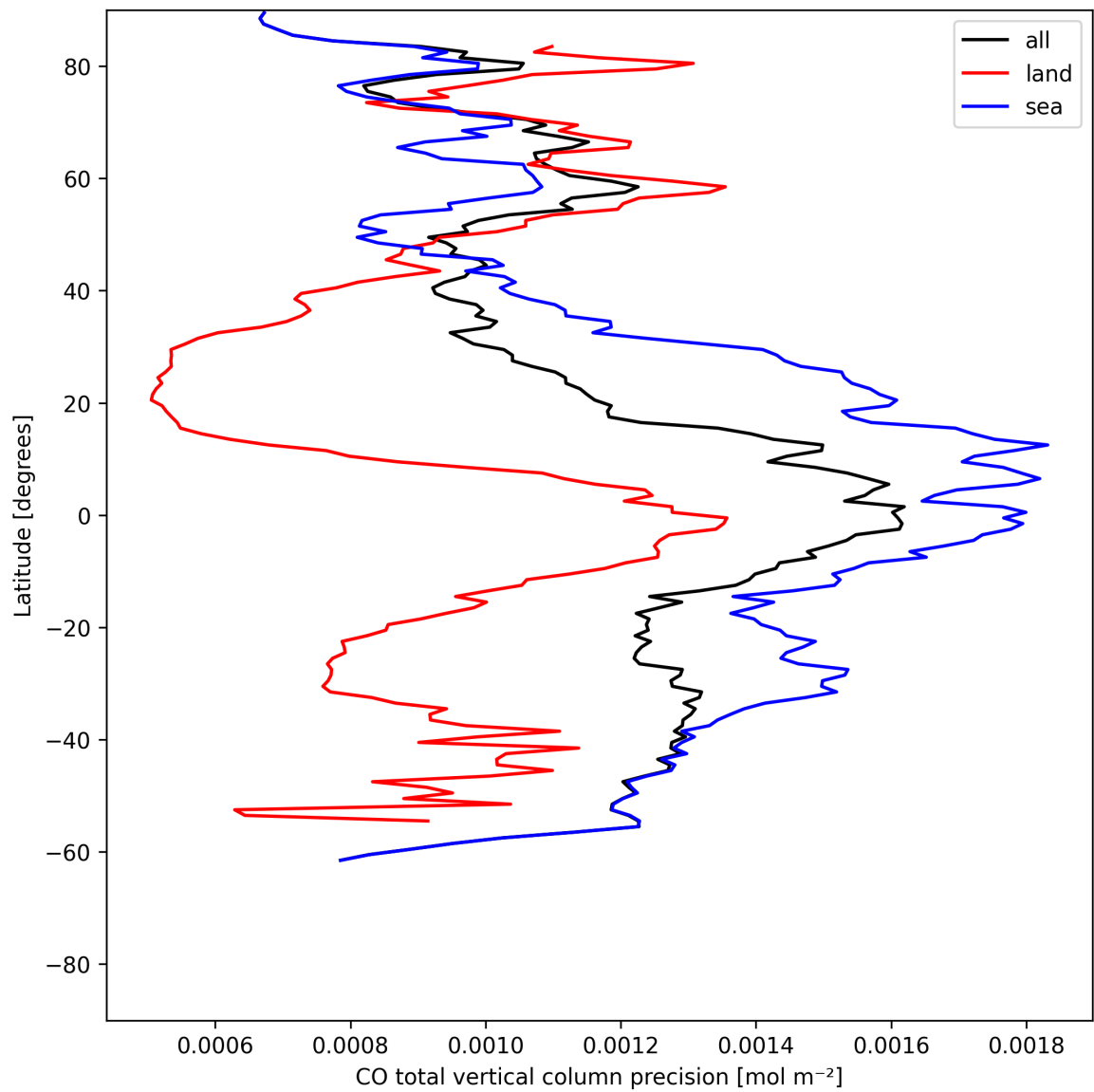
Figure 12: Zonal average of “CO total vertical column precision” for 2025-06-08 to 2025-06-10.
