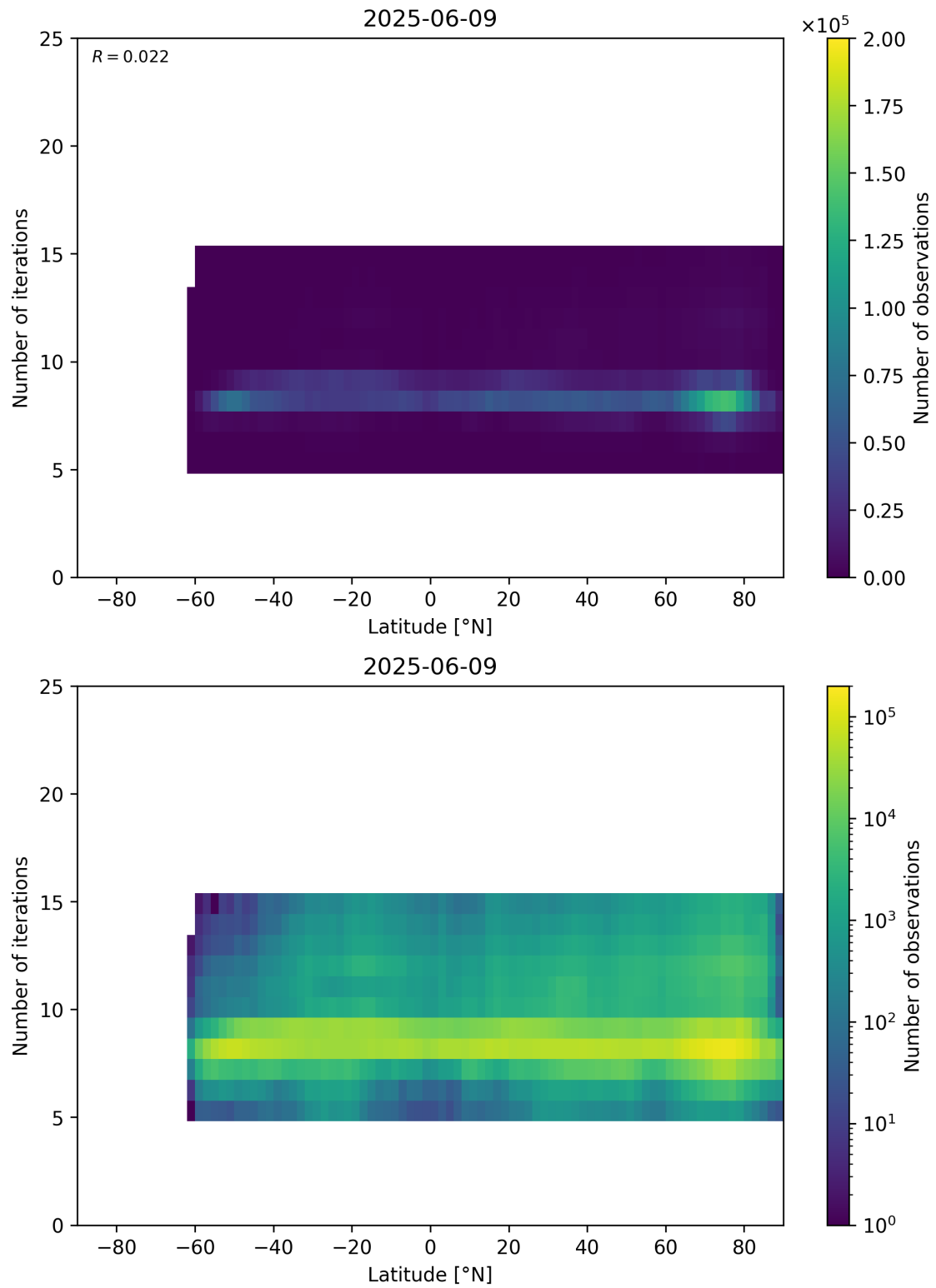
Figure 56: Scatter density plot of “Latitude” against “Number of iterations” for 2025-06-08 to 2025-06-10.
