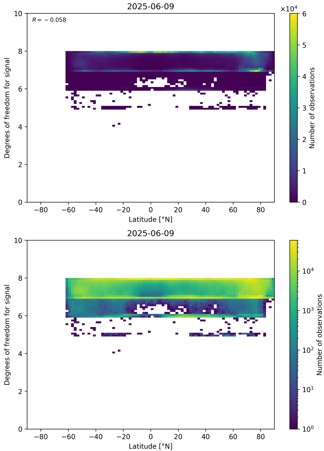
Figure 55: Scatter density plot of “Latitude” against “Degrees of freedom for signal” for 2025-06-08 to 2025-06-10.
