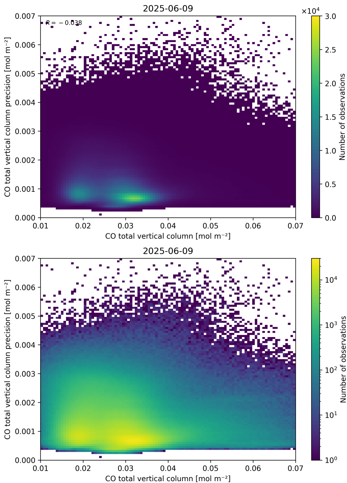
Figure 34: Scatter density plot of “CO total vertical column” against “CO total vertical column precision” for 2025-06-08 to 2025-06-10.
