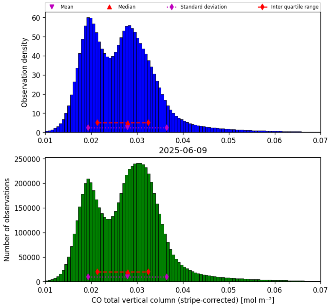
Figure 19: Histogram of “CO total vertical column (stripe-corrected)” for 2025-06-08 to 2025-06-10
