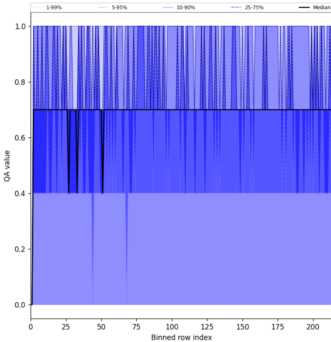
Figure 25: Along track statistics of “QA value” for 2025-06-08 to 2025-06-10
