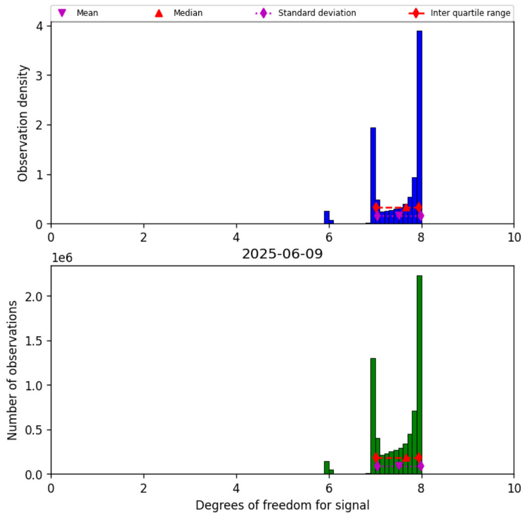
Figure 23: Histogram of “Degrees of freedom for signal” for 2025-06-08 to 2025-06-10
