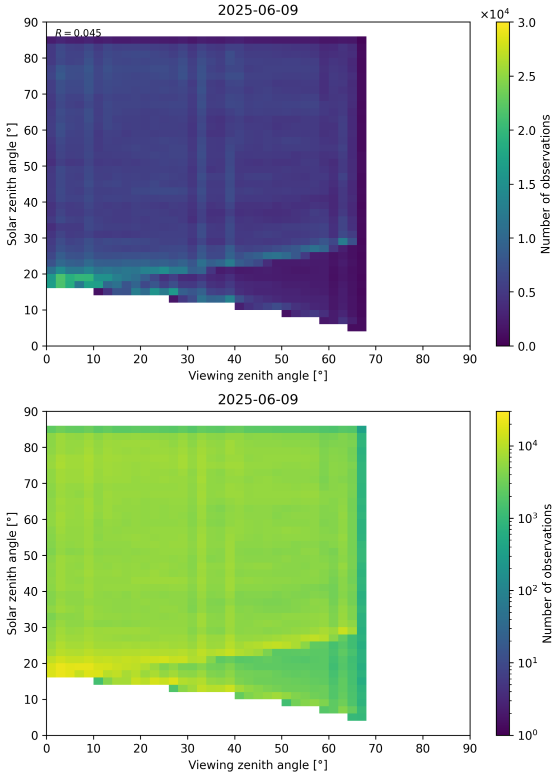
Figure 77: Scatter density plot of “Viewing zenith angle” against “Solar zenith angle” for 2025-06-08 to 2025-06-10.
