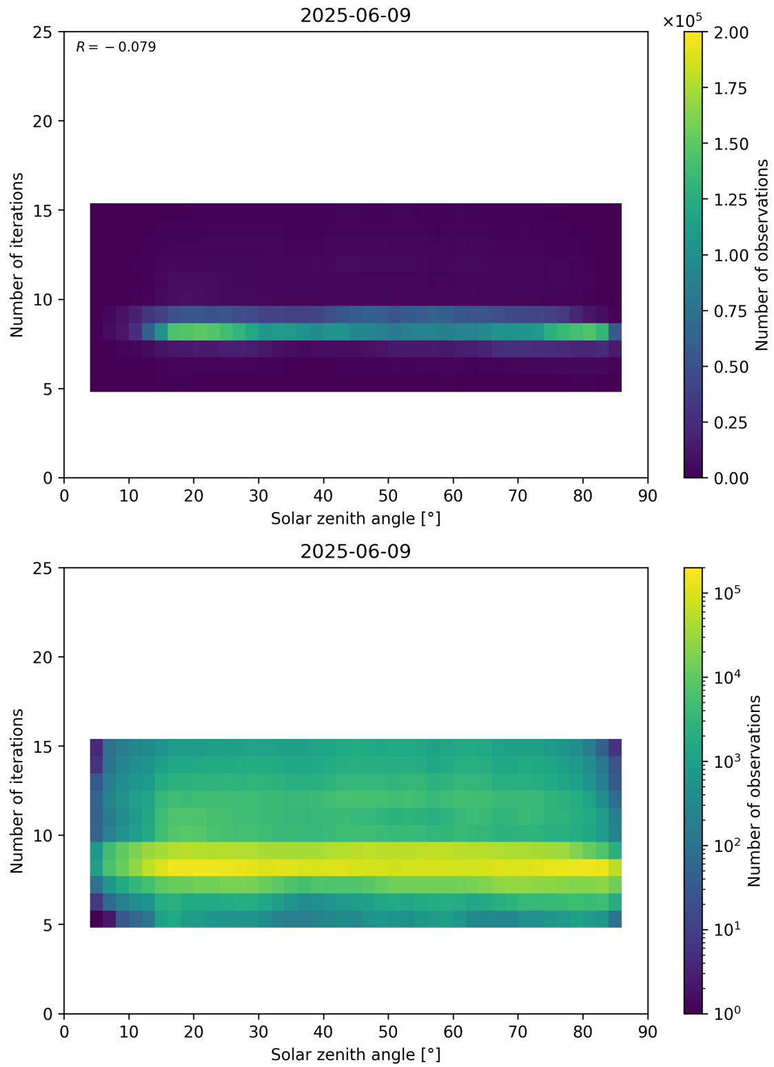
Figure 67: Scatter density plot of “Solar zenith angle” against “Number of iterations” for 2025-06-08 to 2025-06-10.
