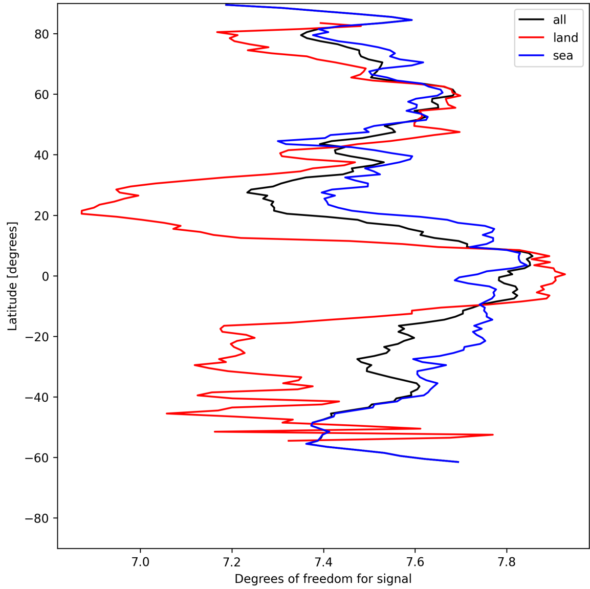
Figure 15: Zonal average of “Degrees of freedom for signal” for 2025-06-08 to 2025-06-10.
