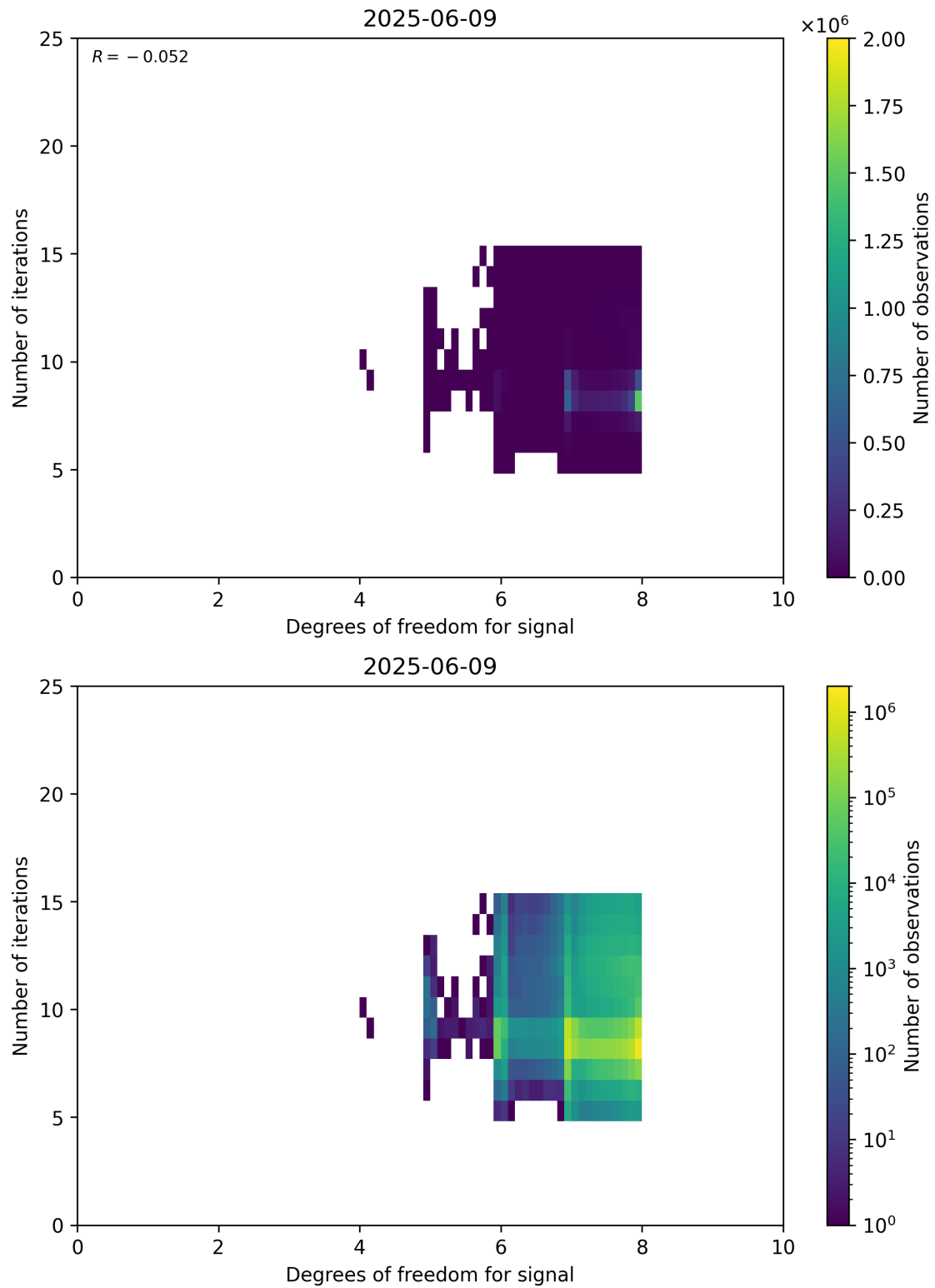
Figure 50: Scatter density plot of “Degrees of freedom for signal” against “Number of iterations” for 2025-06-08 to 2025-06-10.
