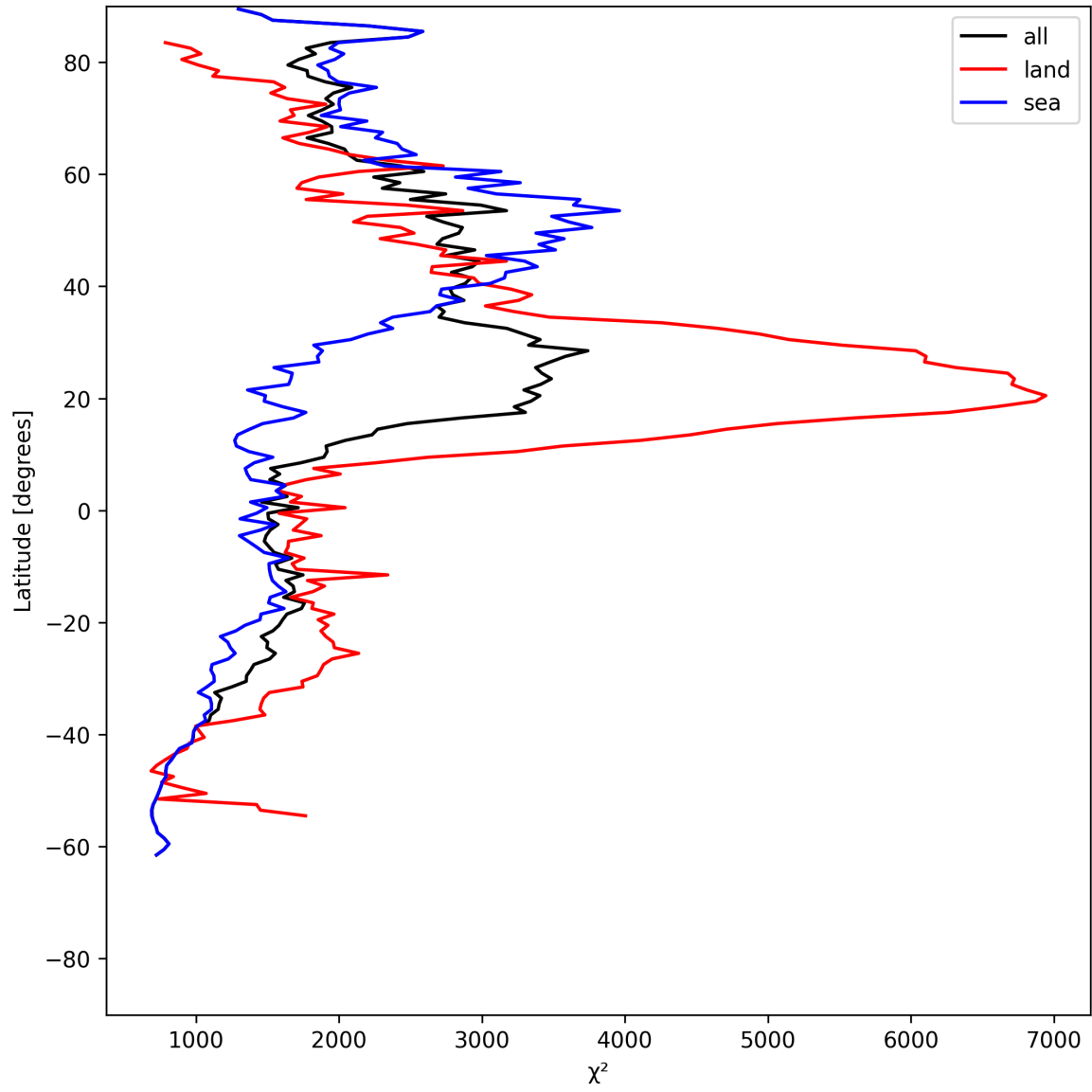
Figure 14: Zonal average of “ \chi^2 ” for 2025-06-08 to 2025-06-10.
