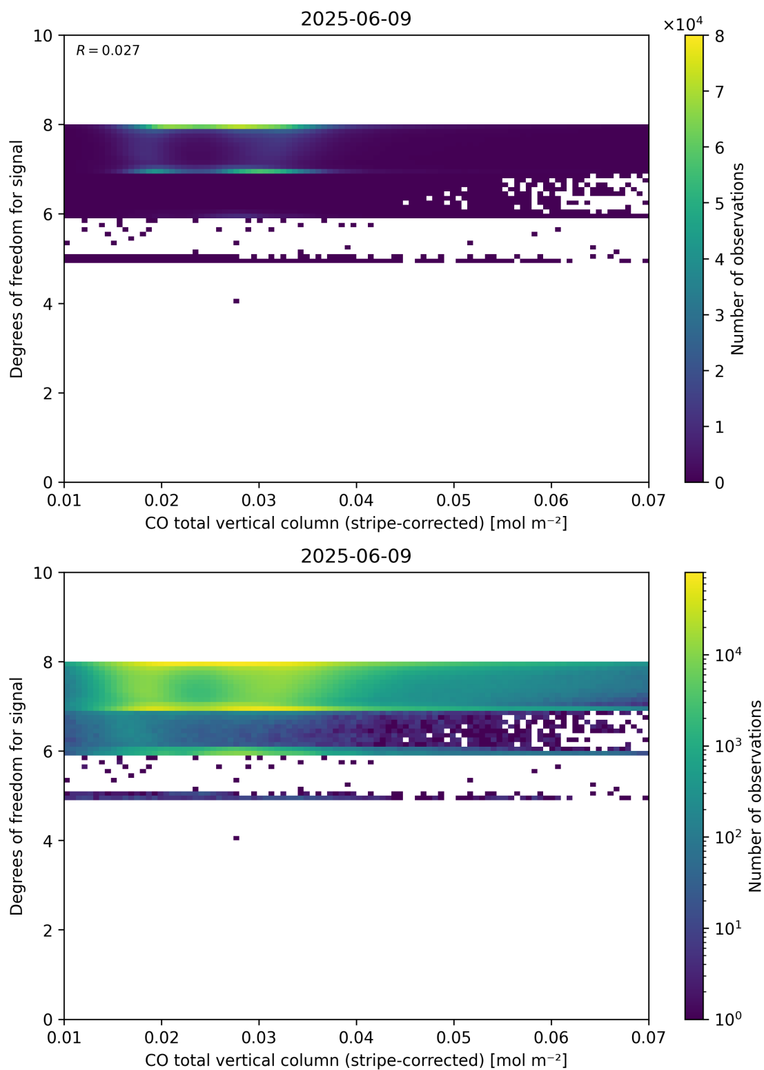
Figure 38: Scatter density plot of “CO total vertical column (stripe-corrected)” against “Degrees of freedom for signal” for 2025-06-08 to 2025-06-10.
