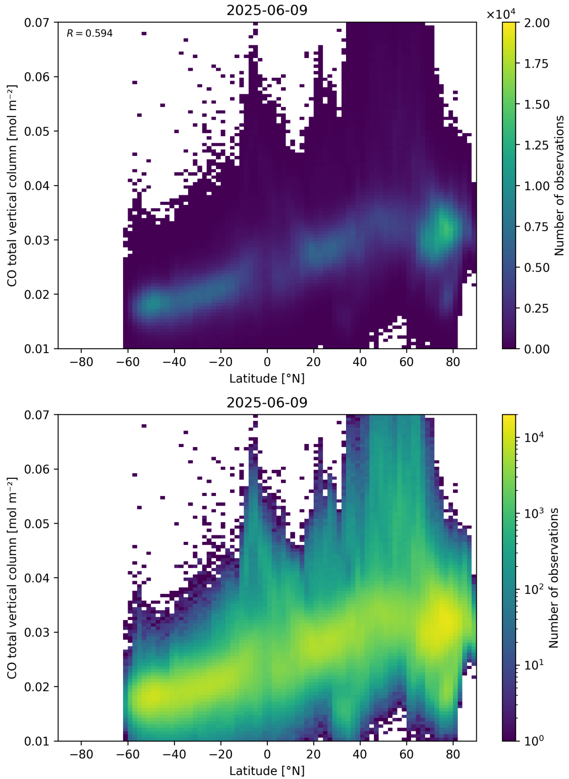
Figure 51: Scatter density plot of “Latitude” against “CO total vertical column” for 2025-06-08 to 2025-06-10.
