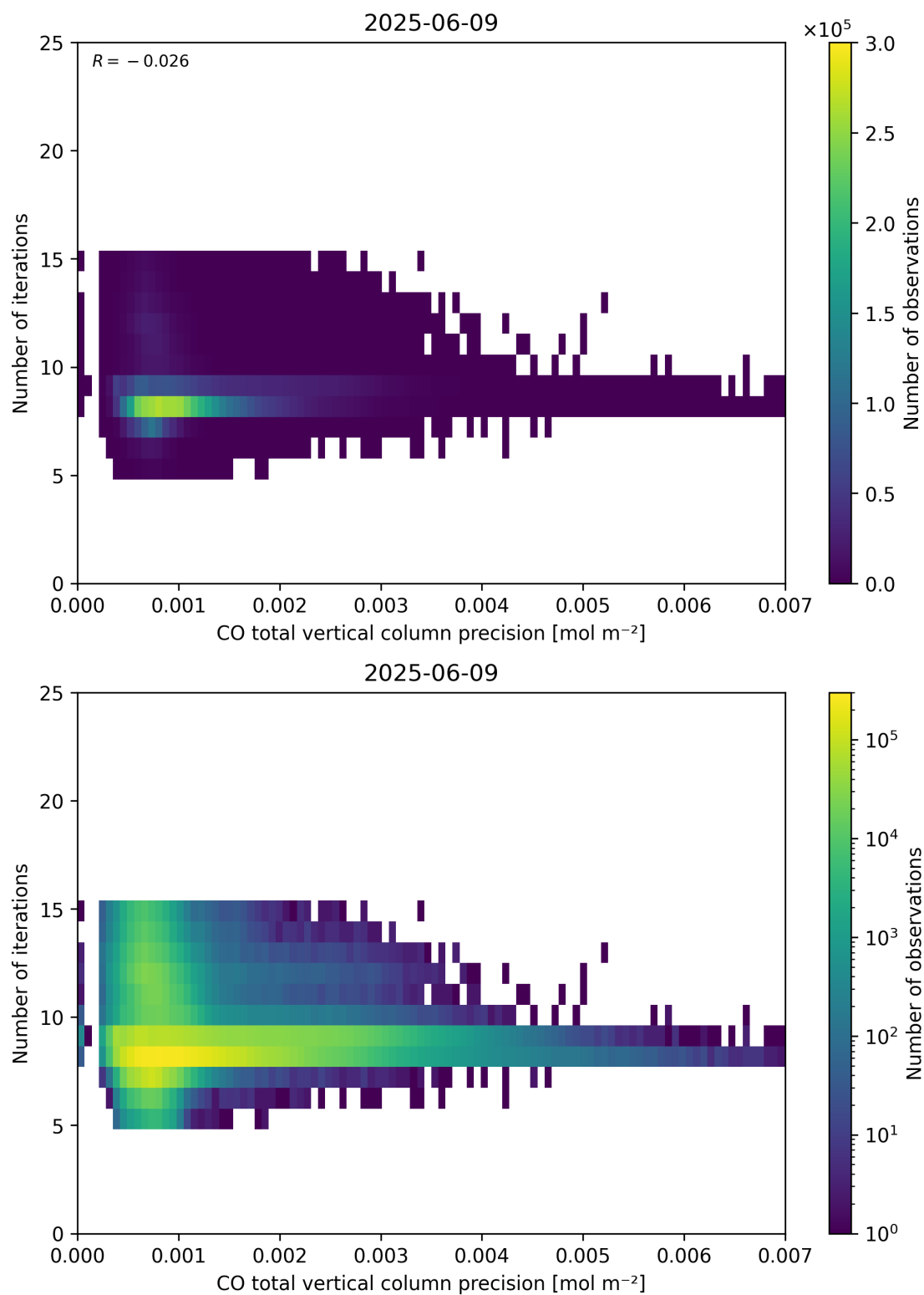
Figure 46: Scatter density plot of “CO total vertical column precision” against “Number of iterations” for 2025-06-08 to 2025-06-10.
