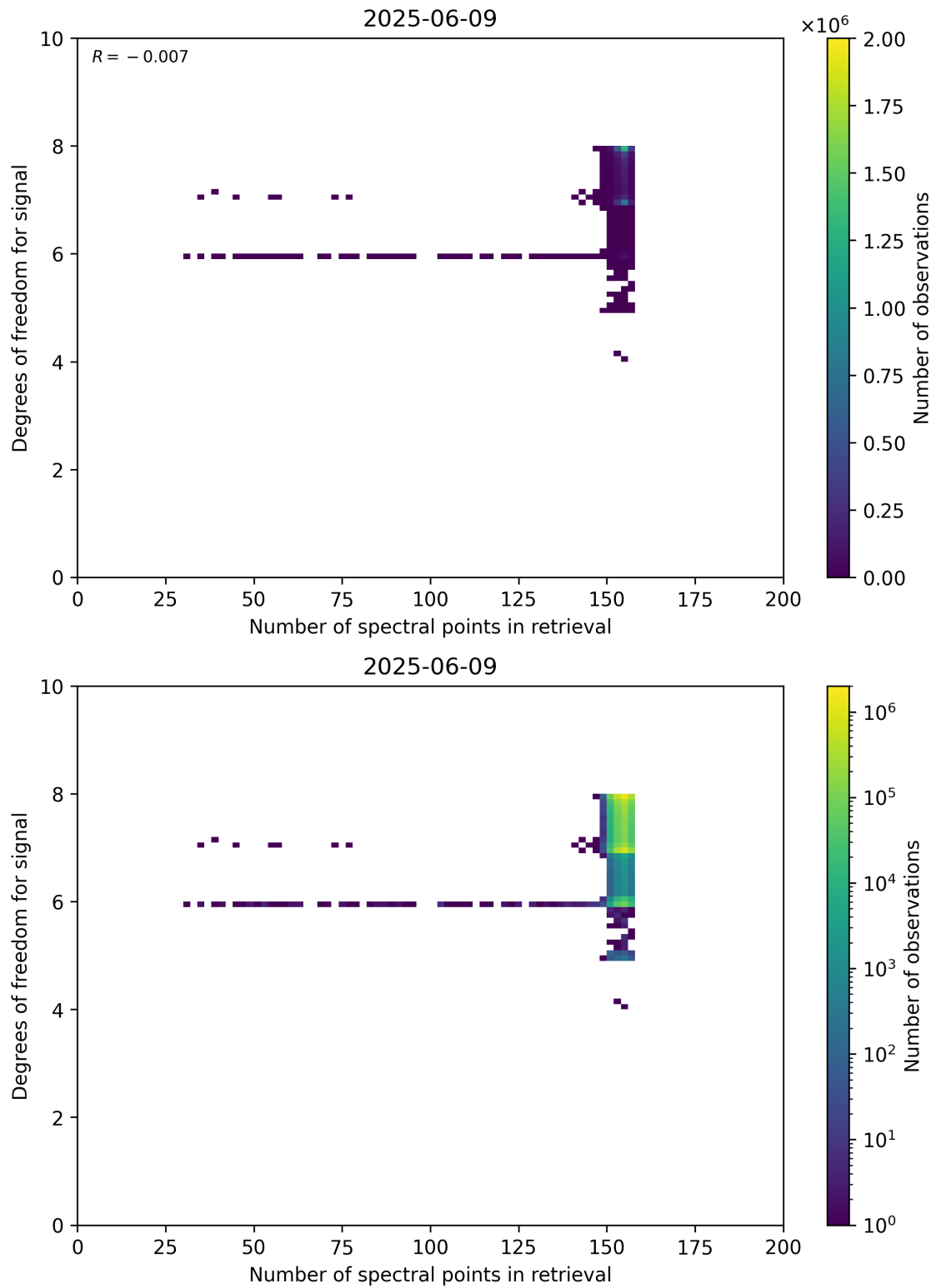
Figure 59: Scatter density plot of “Number of spectral points in retrieval” against “Degrees of freedom for signal” for 2025-06-08 to 2025-06-10.
