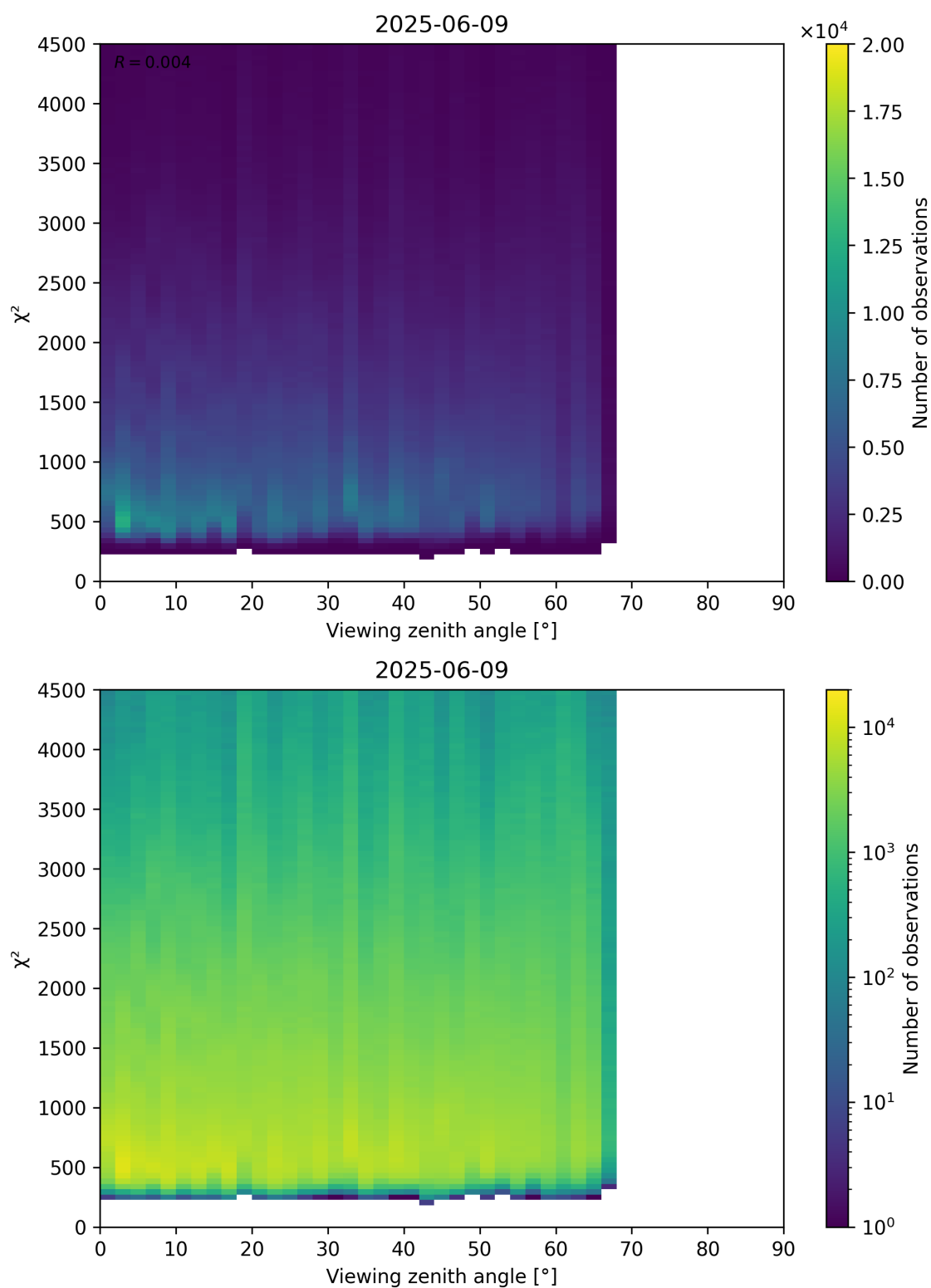
Figure 72: Scatter density plot of “Viewing zenith angle” against “ \chi^2 ” for 2025-06-08 to 2025-06-10.
