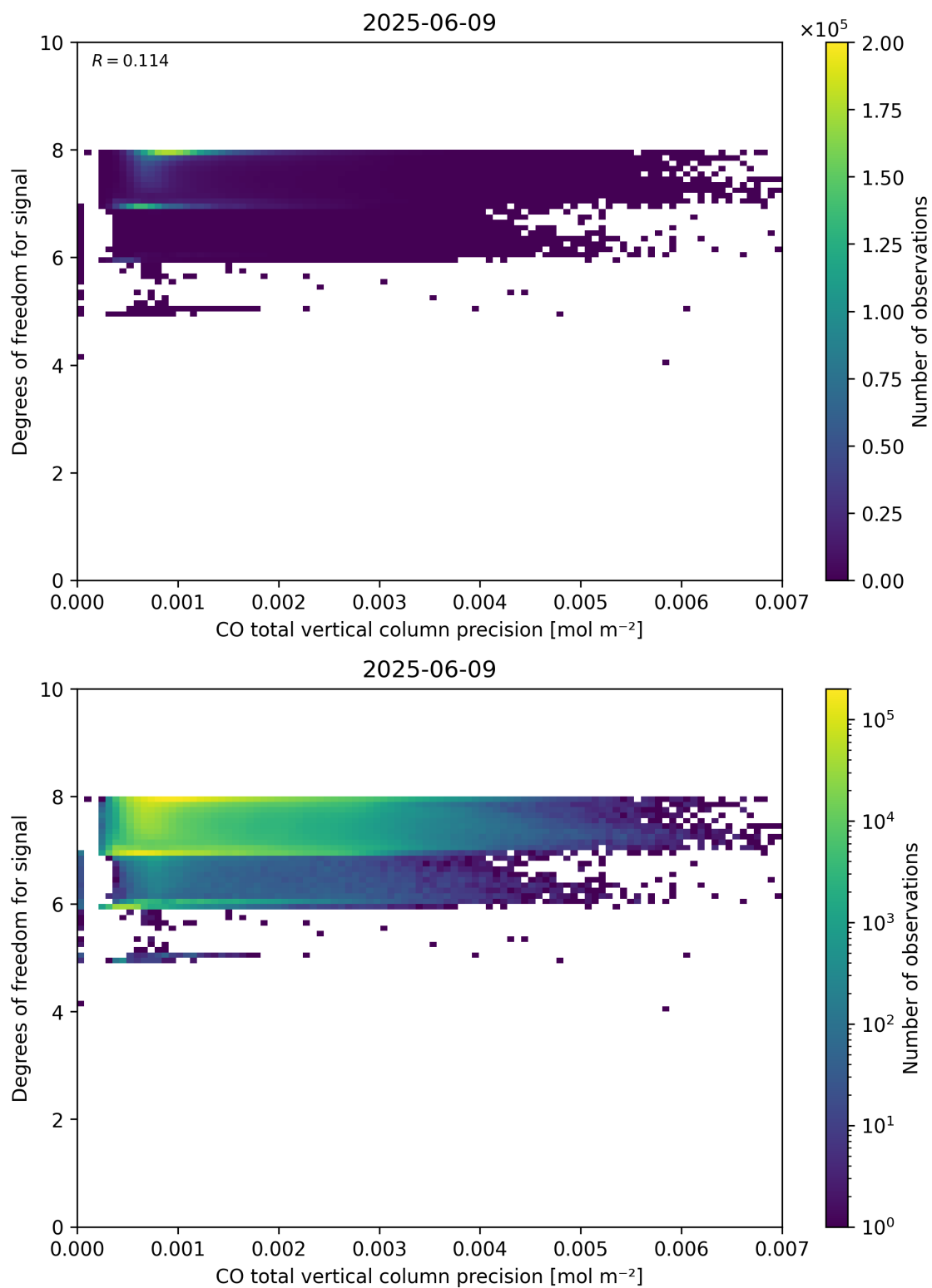
Figure 45: Scatter density plot of “CO total vertical column precision” against “Degrees of freedom for signal” for 2025-06-08 to 2025-06-10.
