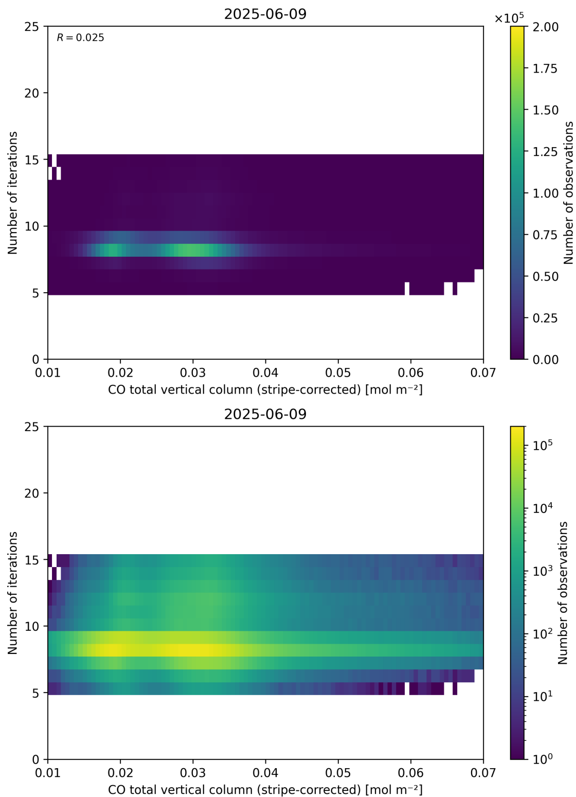
Figure 39: Scatter density plot of “CO total vertical column (stripe-corrected)” against “Number of iterations” for 2025-06-08 to 2025-06-10.
