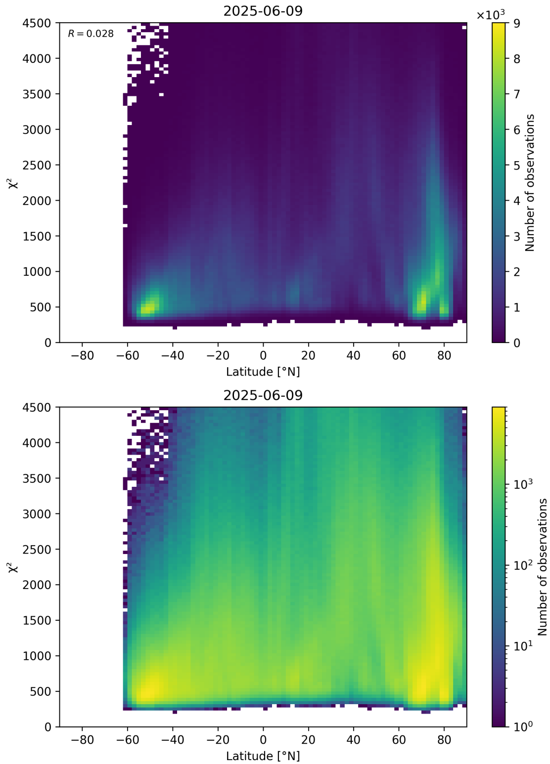
Figure 54: Scatter density plot of “Latitude” against “ \chi^2 ” for 2025-06-08 to 2025-06-10.
