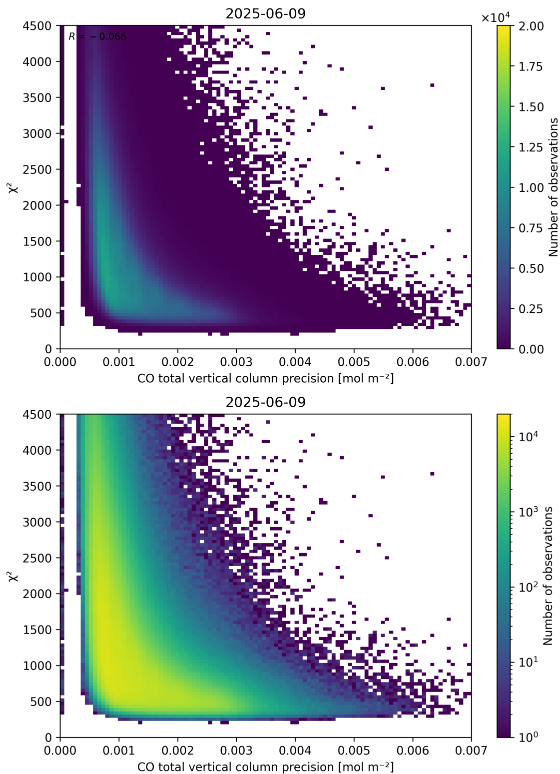
Figure 44: Scatter density plot of “CO total vertical column precision” against “ \chi^2 ” for 2025-06-08 to 2025-06-10.
