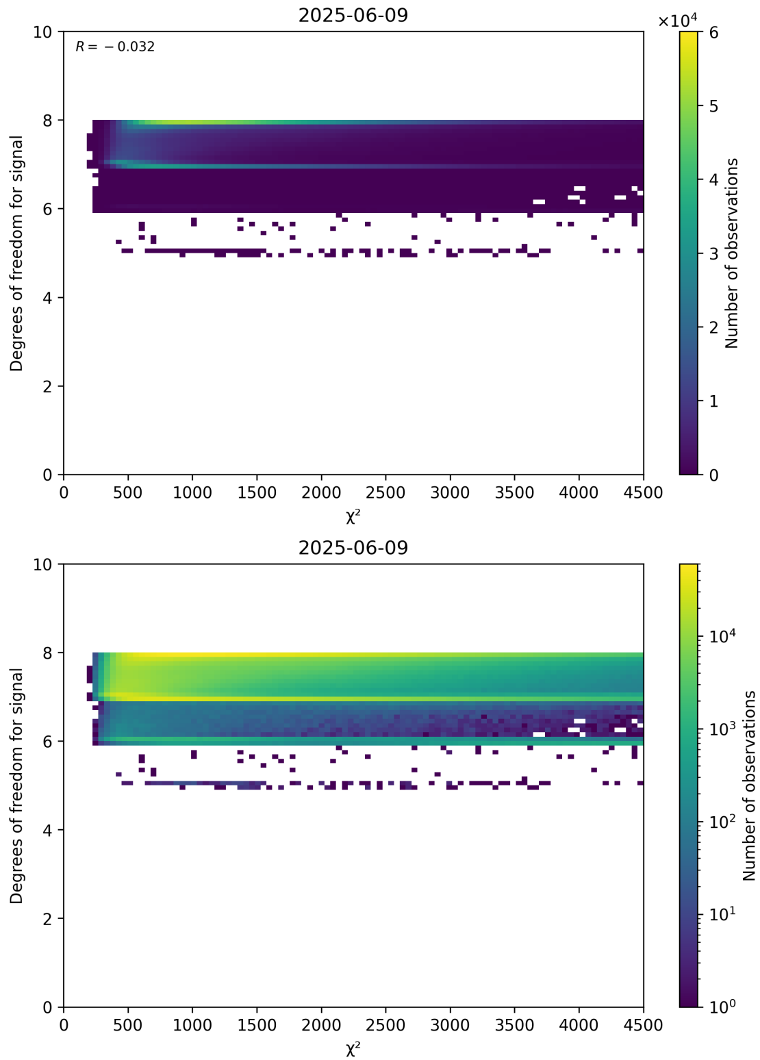
Figure 48: Scatter density plot of “ \chi^2 ” against “Degrees of freedom for signal” for 2025-06-08 to 2025-06-10.
