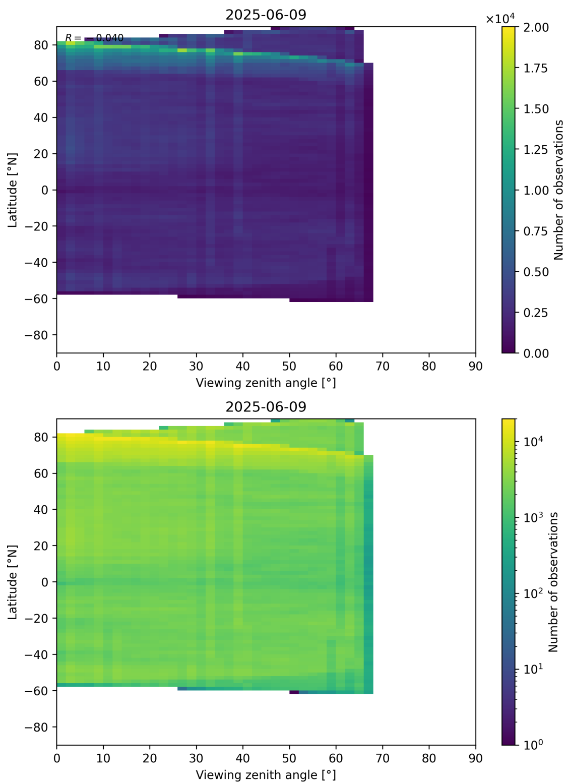
Figure 74: Scatter density plot of “Viewing zenith angle” against “Latitude” for 2025-06-08 to 2025-06-10.
