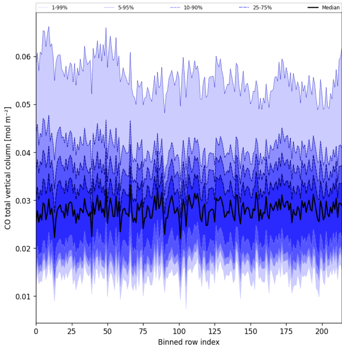
Figure 26: Along track statistics of “CO total vertical column” for 2025-06-08 to 2025-06-10
