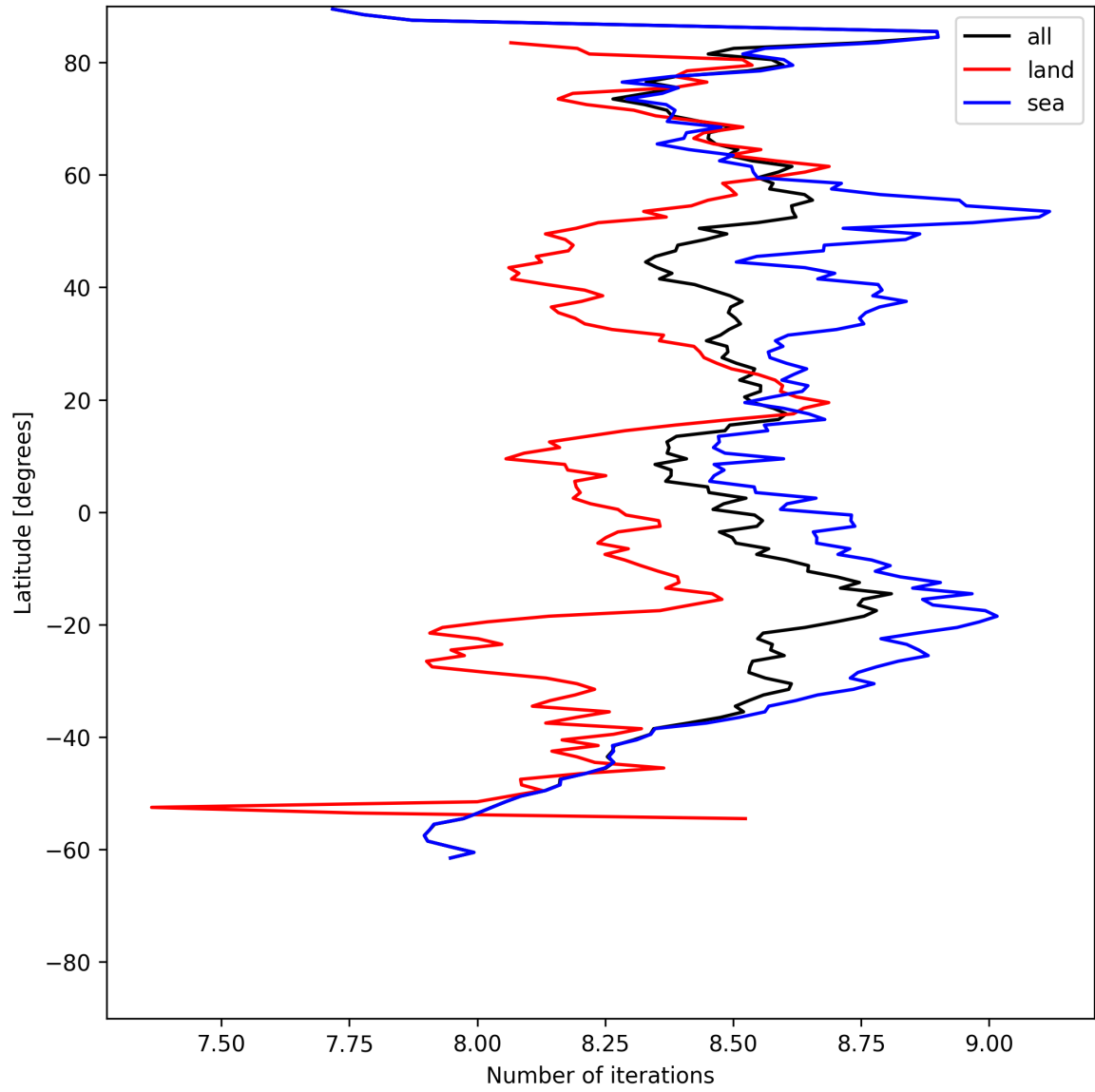
Figure 16: Zonal average of “Number of iterations” for 2025-06-08 to 2025-06-10.
