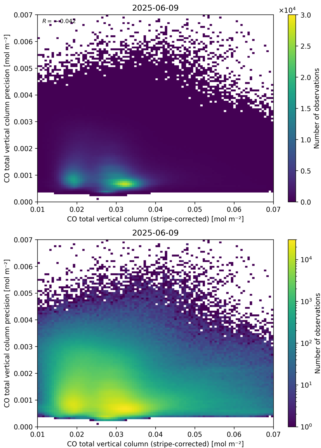
Figure 36: Scatter density plot of “CO total vertical column (stripe-corrected)” against “CO total vertical column precision” for 2025-06-08 to 2025-06-10.
