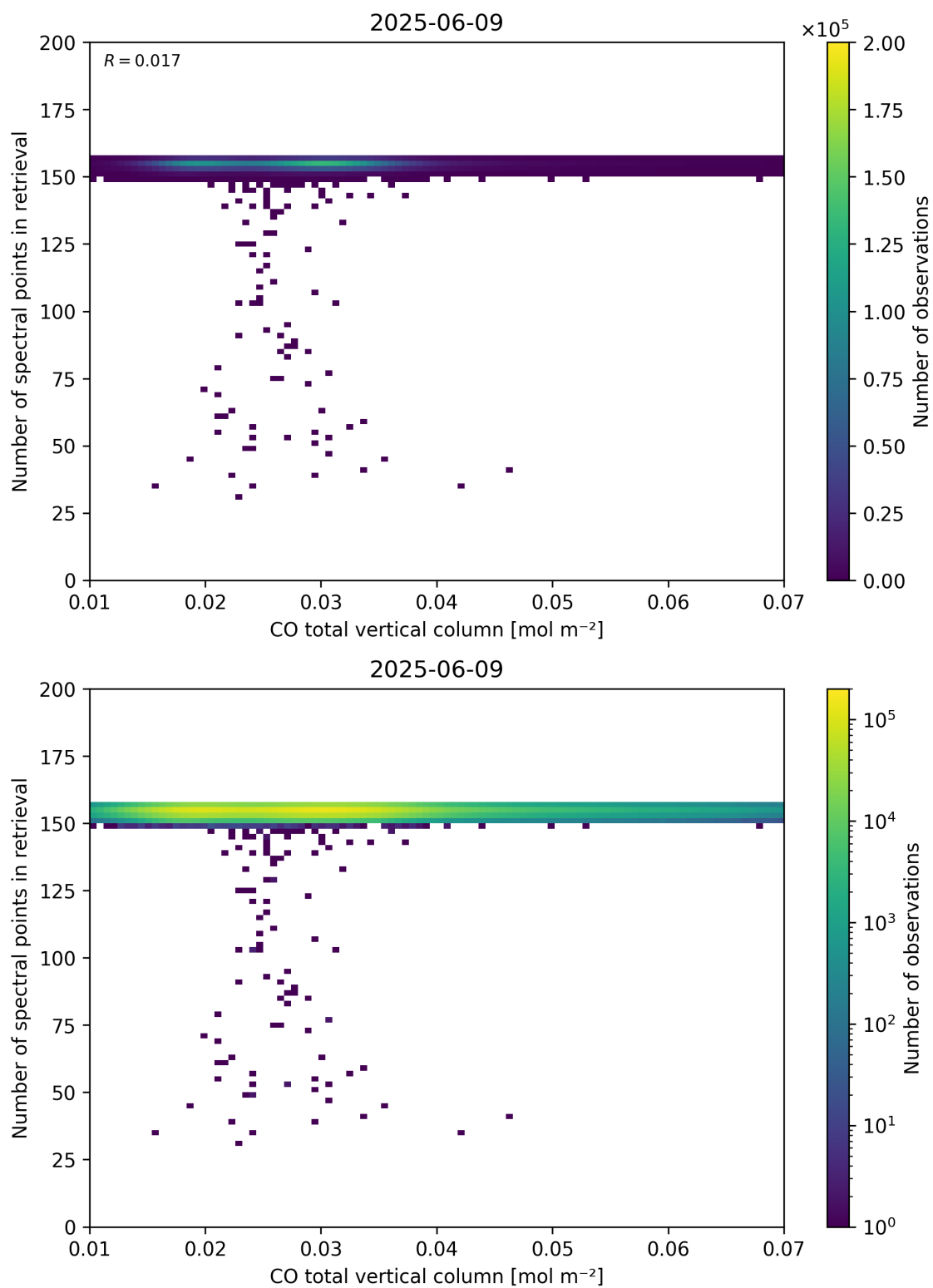
Figure 43: Scatter density plot of “CO total vertical column” against “Number of spectral points in retrieval” for 2025-06-08 to 2025-06-10.
