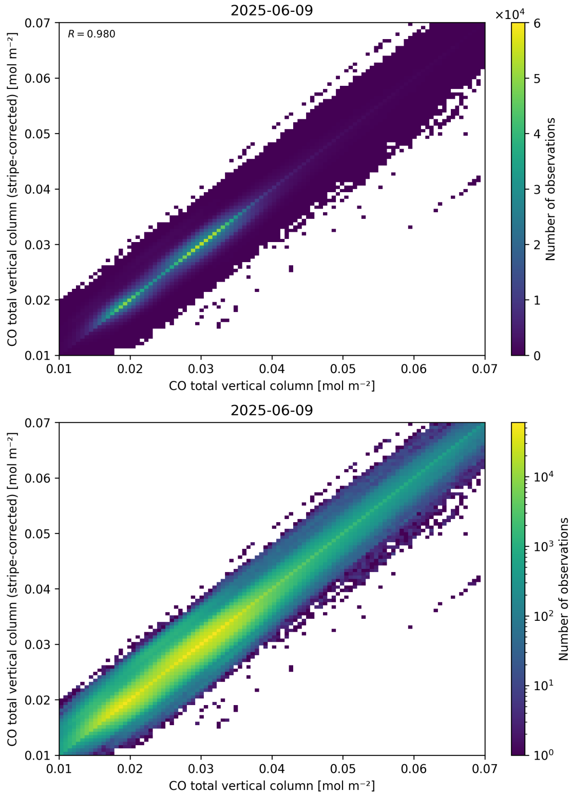
Figure 33: Scatter density plot of “CO total vertical column” against “CO total vertical column (stripe-corrected)” for 2025-06-08 to 2025-06-10.
