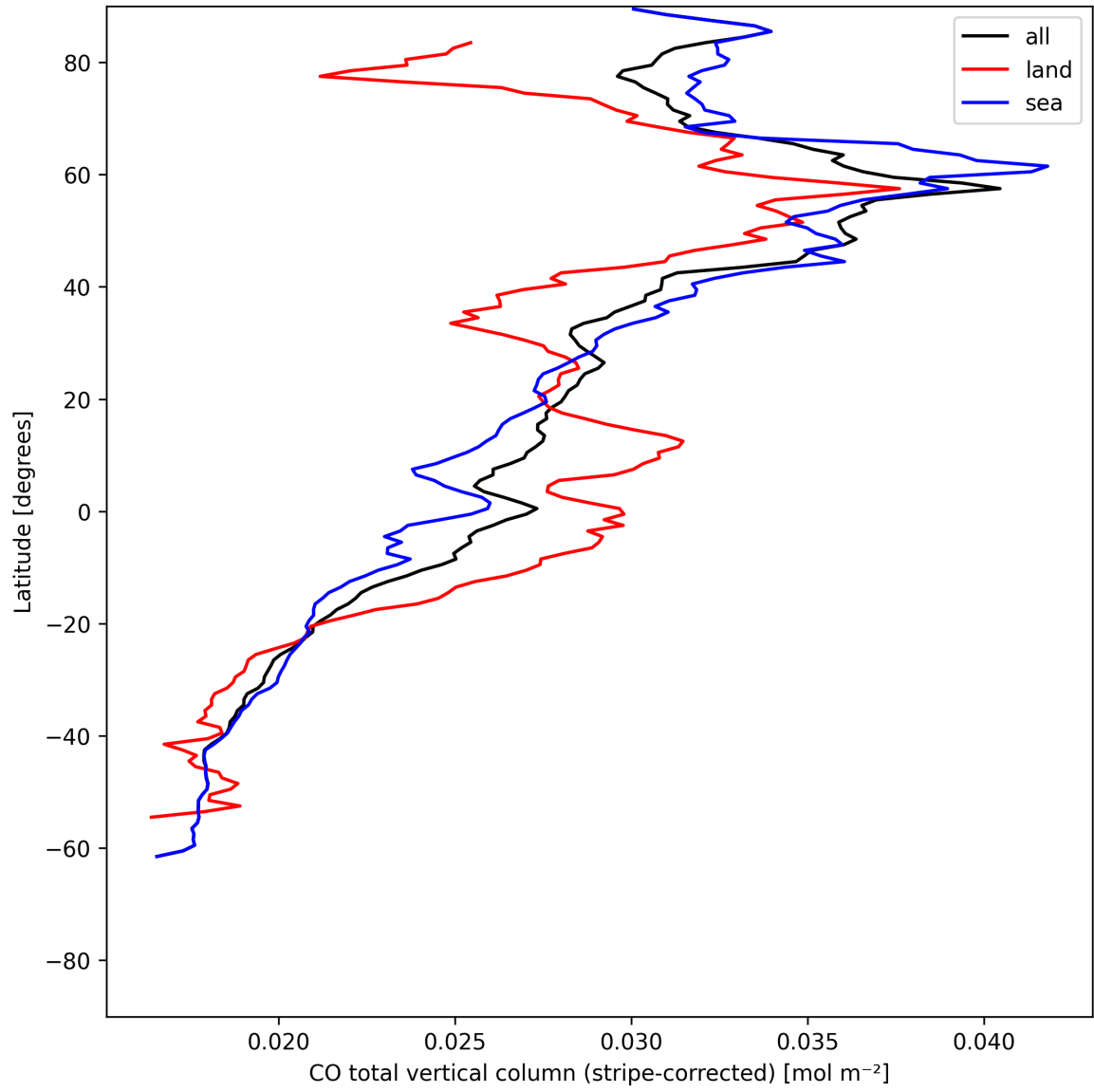
Figure 11: Zonal average of “CO total vertical column (stripe-corrected)” for 2025-06-08 to 2025-06-10.
