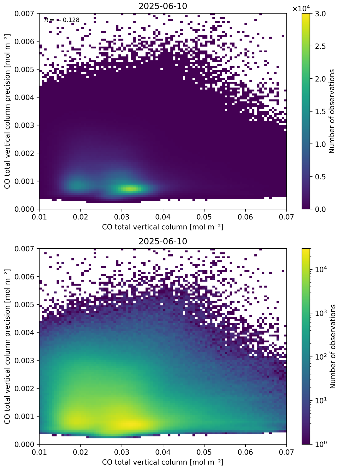
Figure 34: Scatter density plot of “CO total vertical column” against “CO total vertical column precision” for 2025-06-09 to 2025-06-11.
