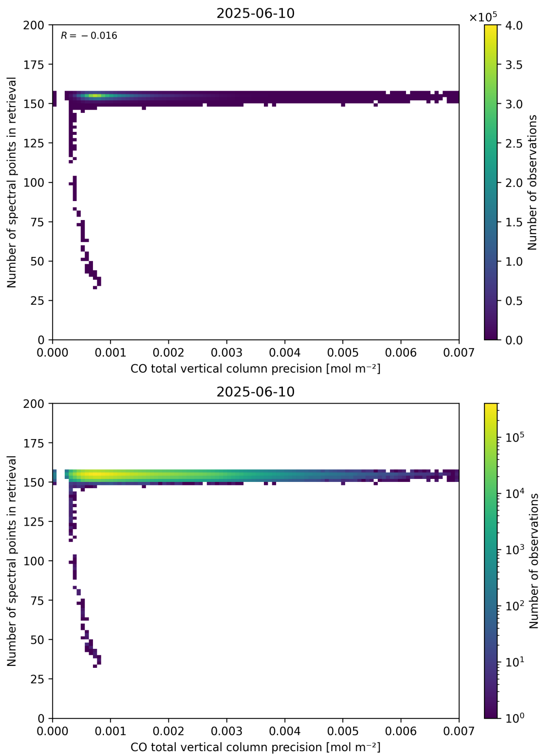
Figure 47: Scatter density plot of “CO total vertical column precision” against “Number of spectral points in retrieval” for 2025-06-09 to 2025-06-11.
