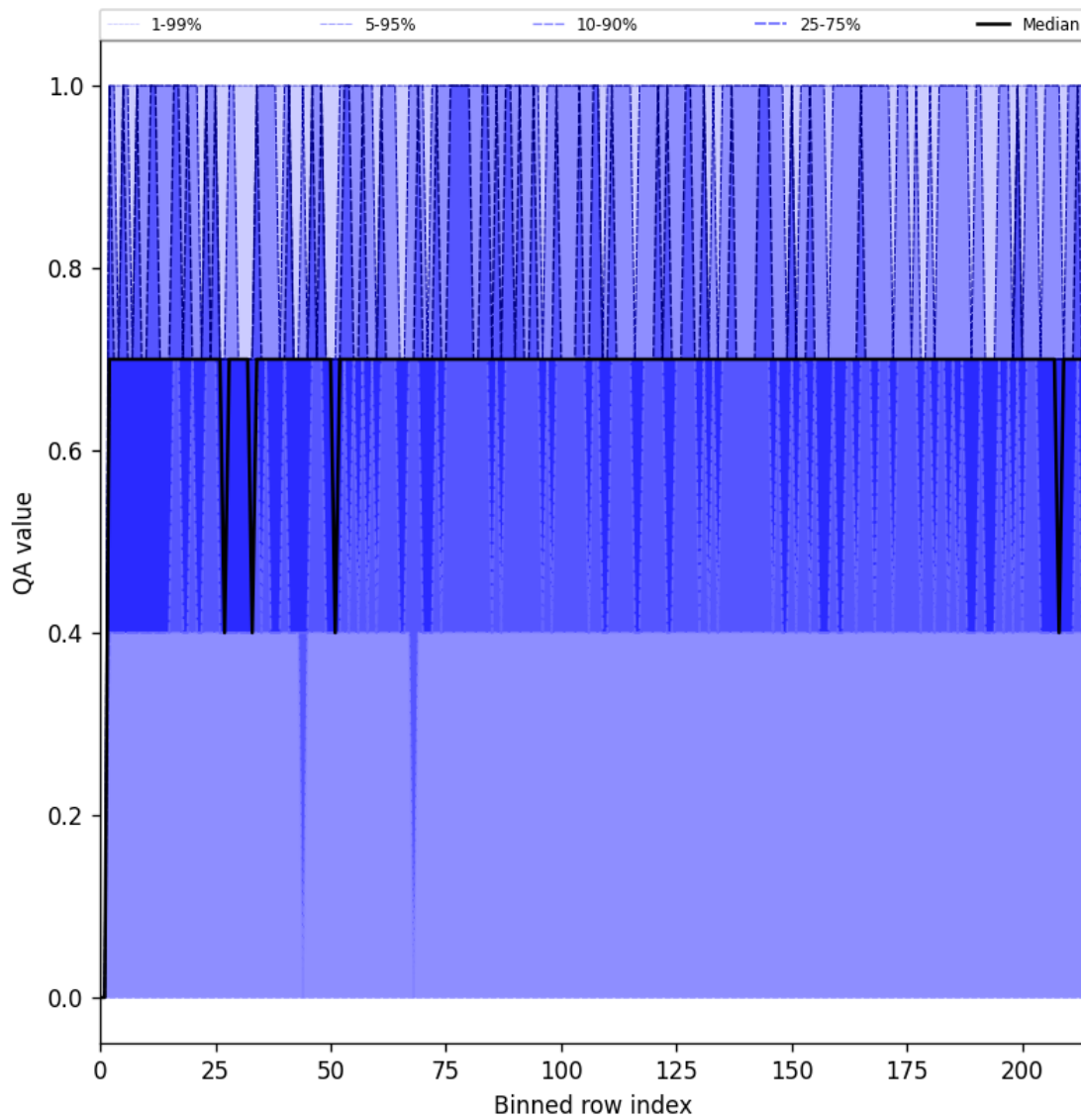
Figure 25: Along track statistics of “QA value” for 2025-06-09 to 2025-06-11
