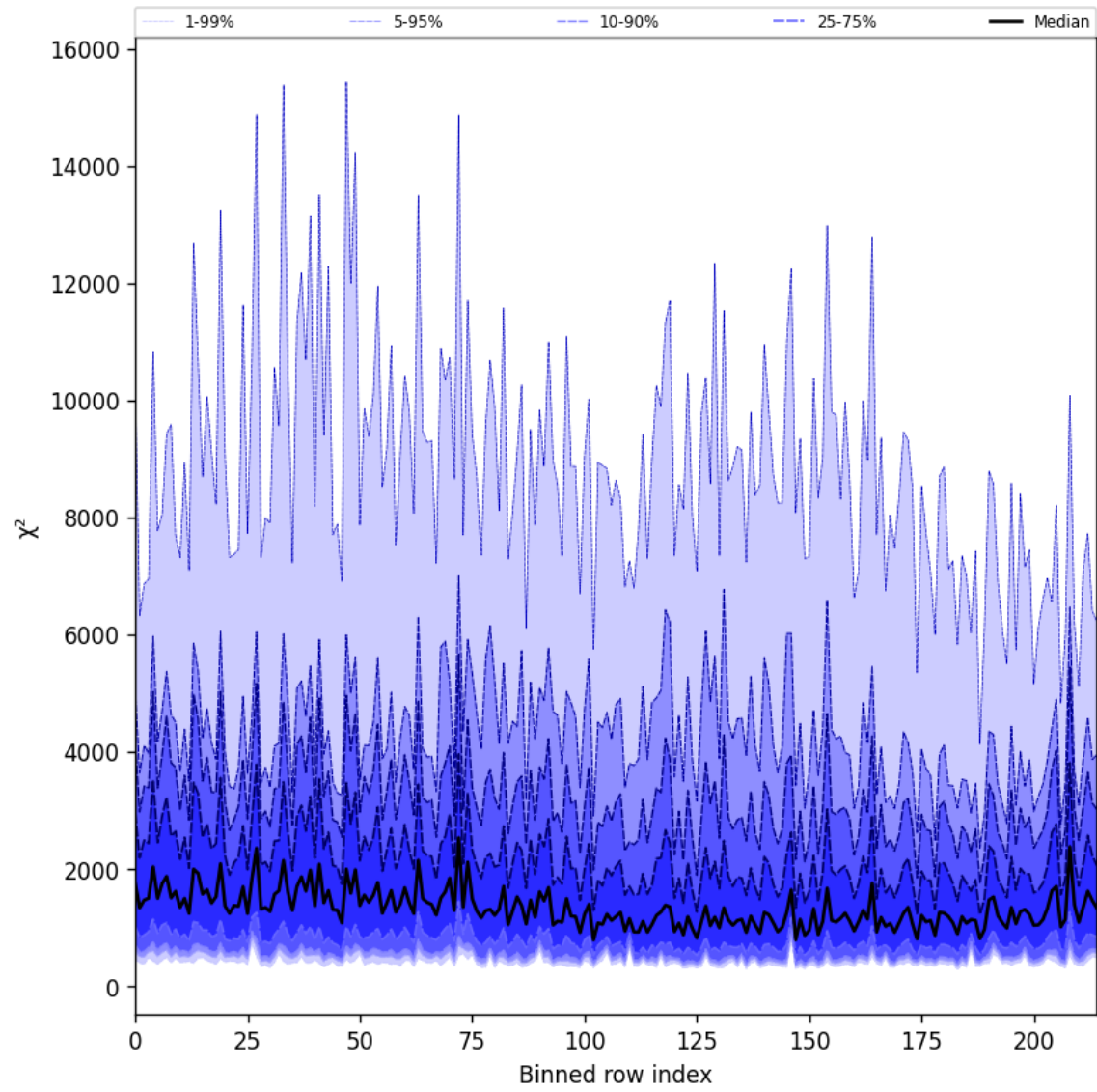
Figure 30: Along track statistics of “ \chi^2 ” for 2025-06-09 to 2025-06-11
