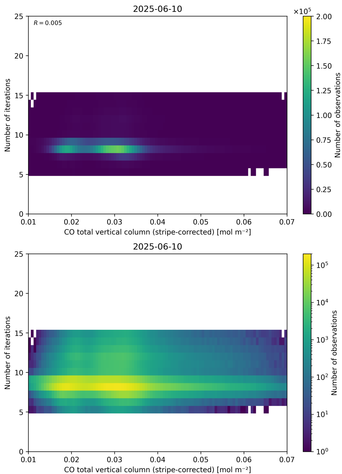
Figure 39: Scatter density plot of “CO total vertical column (stripe-corrected)” against “Number of iterations” for 2025-06-09 to 2025-06-11.
