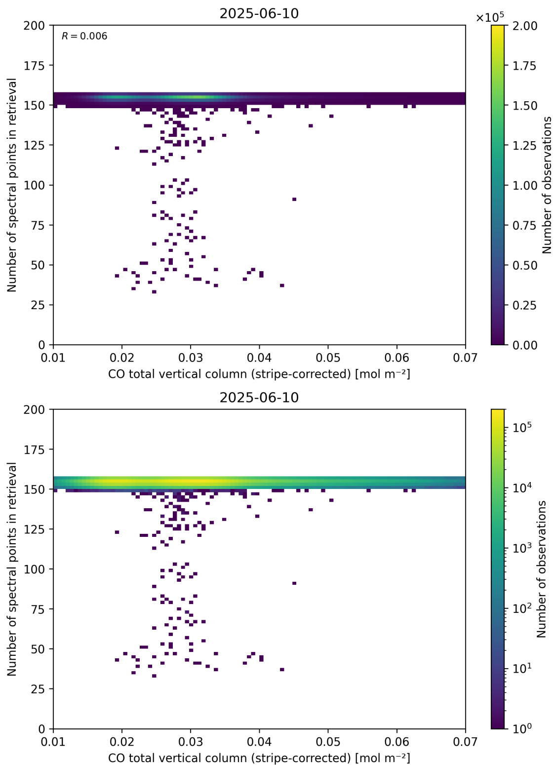
Figure 40: Scatter density plot of “CO total vertical column (stripe-corrected)” against “Number of spectral points in retrieval” for 2025-06-09 to 2025-06-11.
