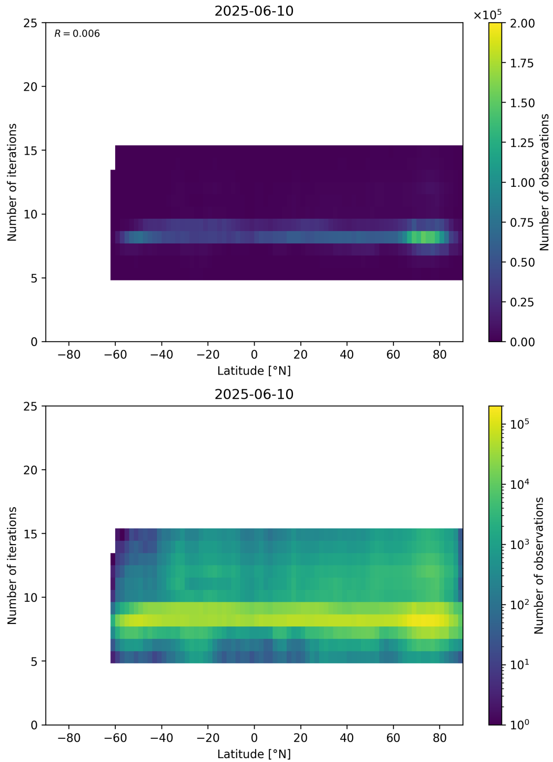
Figure 56: Scatter density plot of “Latitude” against “Number of iterations” for 2025-06-09 to 2025-06-11.
