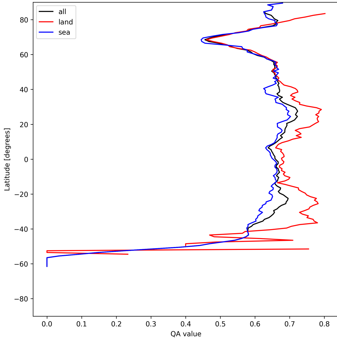
Figure 9: Zonal average of “QA value” for 2025-06-09 to 2025-06-11.
