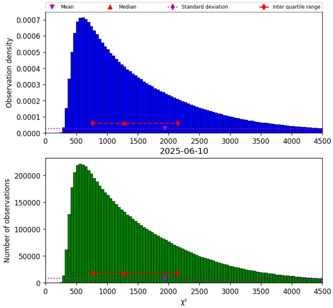
Figure 22: Histogram of “ \chi^2 ” for 2025-06-09 to 2025-06-11
