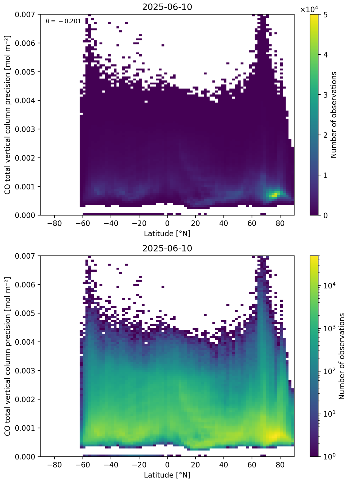
Figure 53: Scatter density plot of “Latitude” against “CO total vertical column precision” for 2025-06-09 to 2025-06-11.
