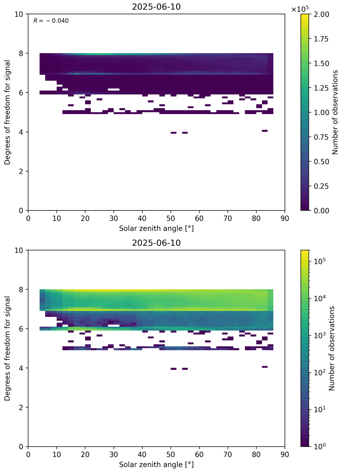
Figure 65: Scatter density plot of “Solar zenith angle” against “Degrees of freedom for signal” for 2025-06-09 to 2025-06-11.
