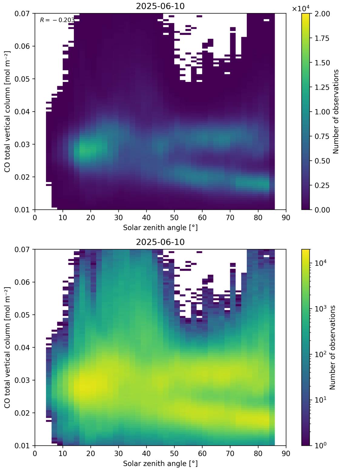
Figure 61: Scatter density plot of “Solar zenith angle” against “CO total vertical column” for 2025-06-09 to 2025-06-11.
