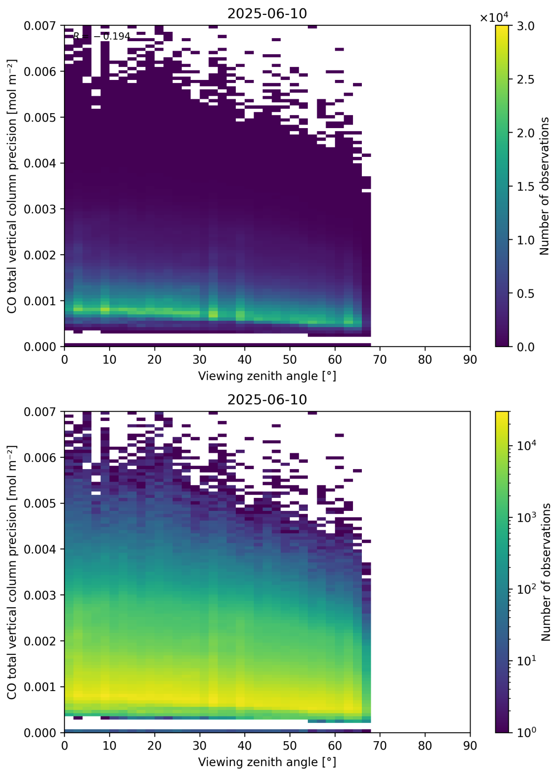
Figure 71: Scatter density plot of “Viewing zenith angle” against “CO total vertical column precision” for 2025-06-09 to 2025-06-11.
