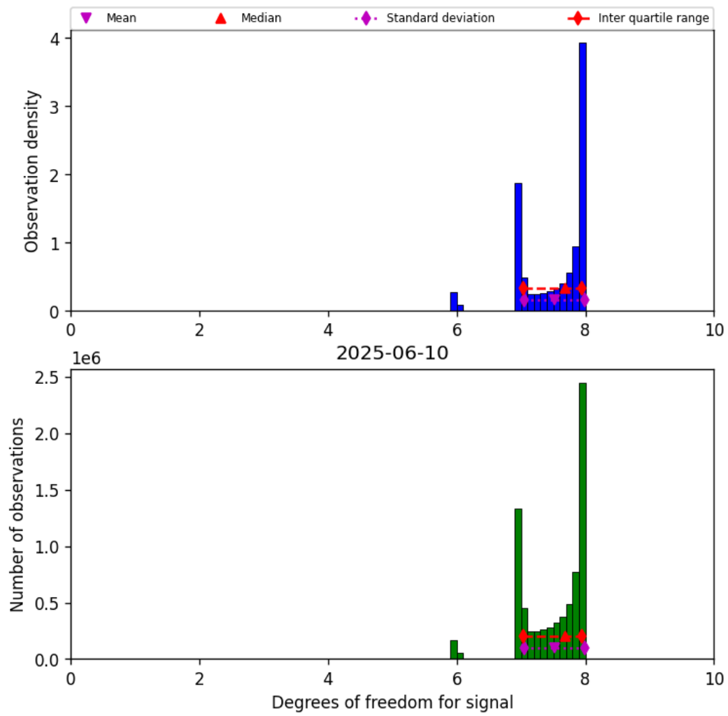
Figure 23: Histogram of “Degrees of freedom for signal” for 2025-06-09 to 2025-06-11
