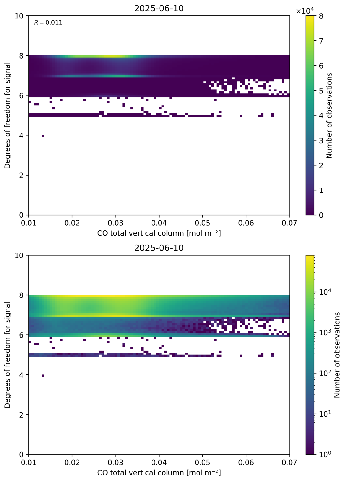
Figure 41: Scatter density plot of “CO total vertical column” against “Degrees of freedom for signal” for 2025-06-09 to 2025-06-11.
