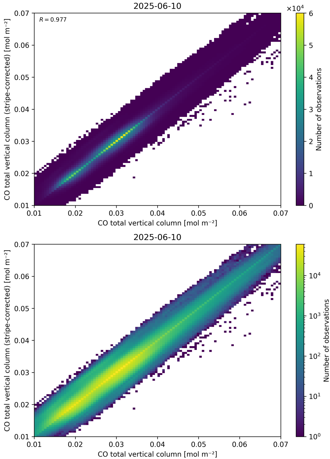
Figure 33: Scatter density plot of “CO total vertical column” against “CO total vertical column (stripe-corrected)” for 2025-06-09 to 2025-06-11.
