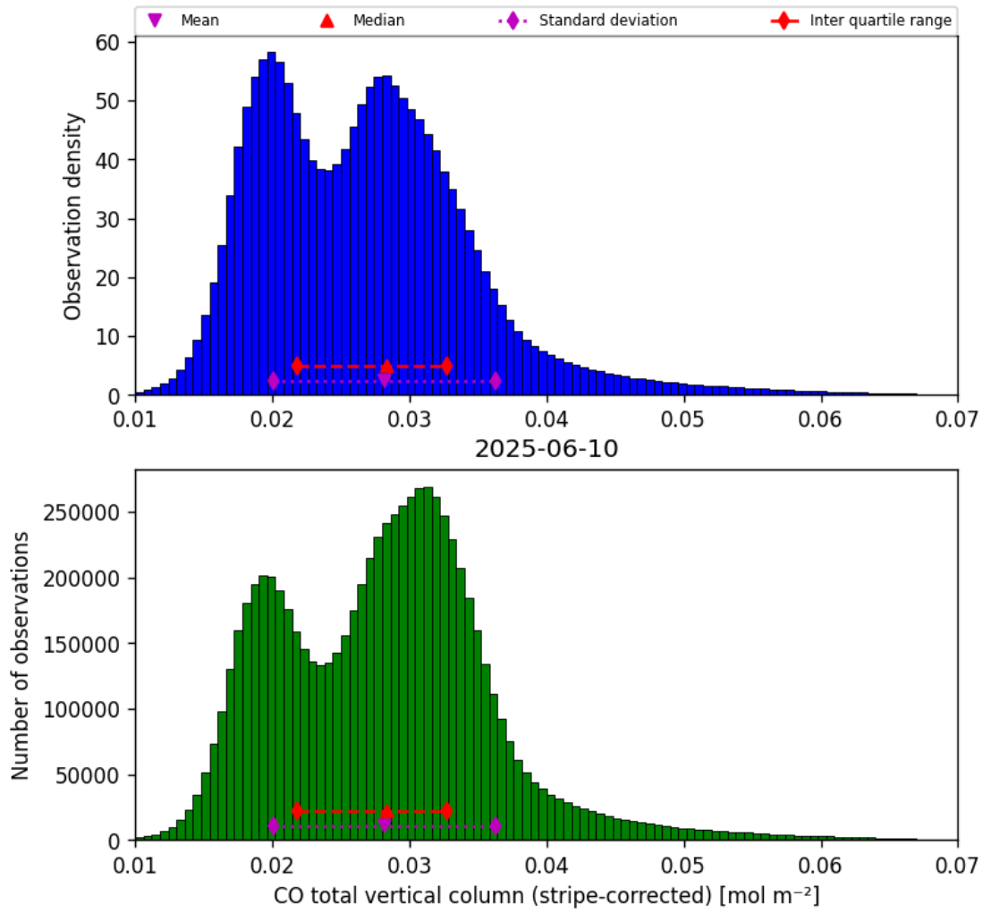
Figure 19: Histogram of “CO total vertical column (stripe-corrected)” for 2025-06-09 to 2025-06-11
