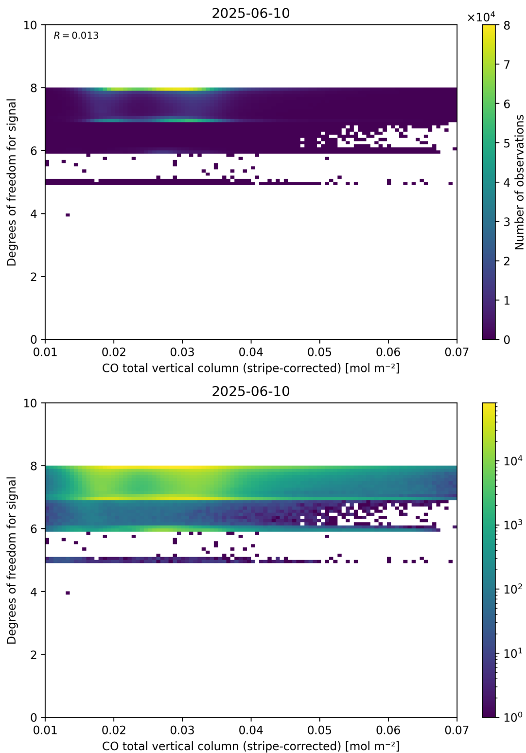
Figure 38: Scatter density plot of “CO total vertical column (stripe-corrected)” against “Degrees of freedom for signal” for 2025-06-09 to 2025-06-11.
