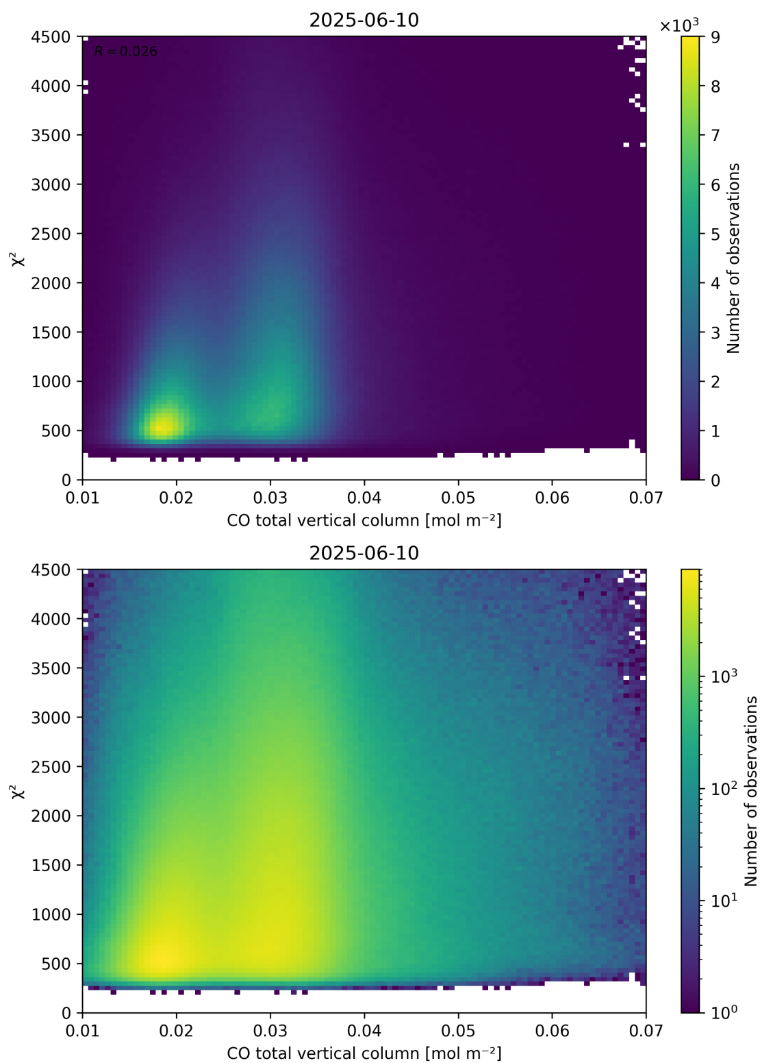
Figure 35: Scatter density plot of “CO total vertical column” against “ \chi^2 ” for 2025-06-09 to 2025-06-11.
