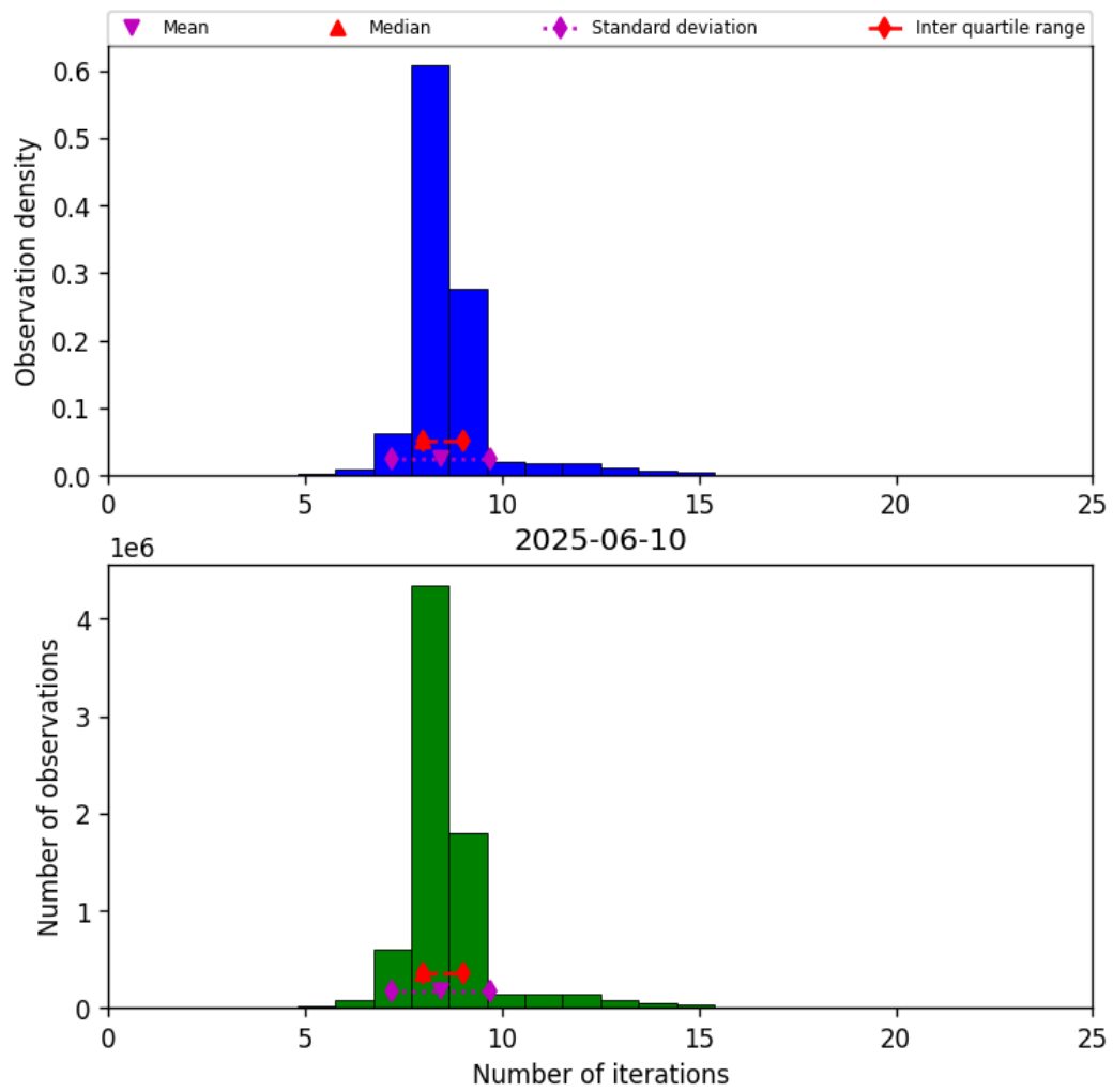
Figure 24: Histogram of “Number of iterations” for 2025-06-09 to 2025-06-11
