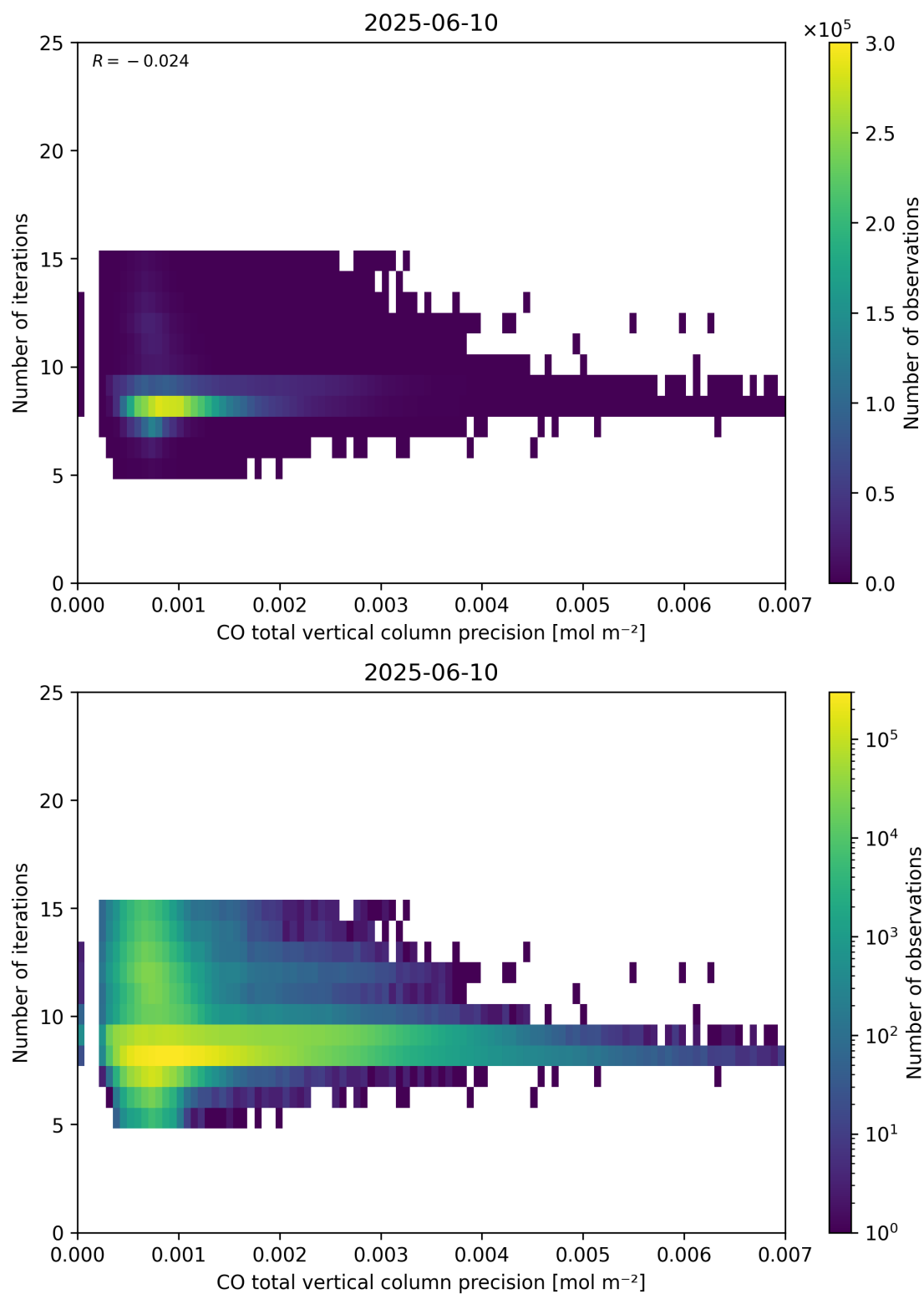
Figure 46: Scatter density plot of “CO total vertical column precision” against “Number of iterations” for 2025-06-09 to 2025-06-11.
