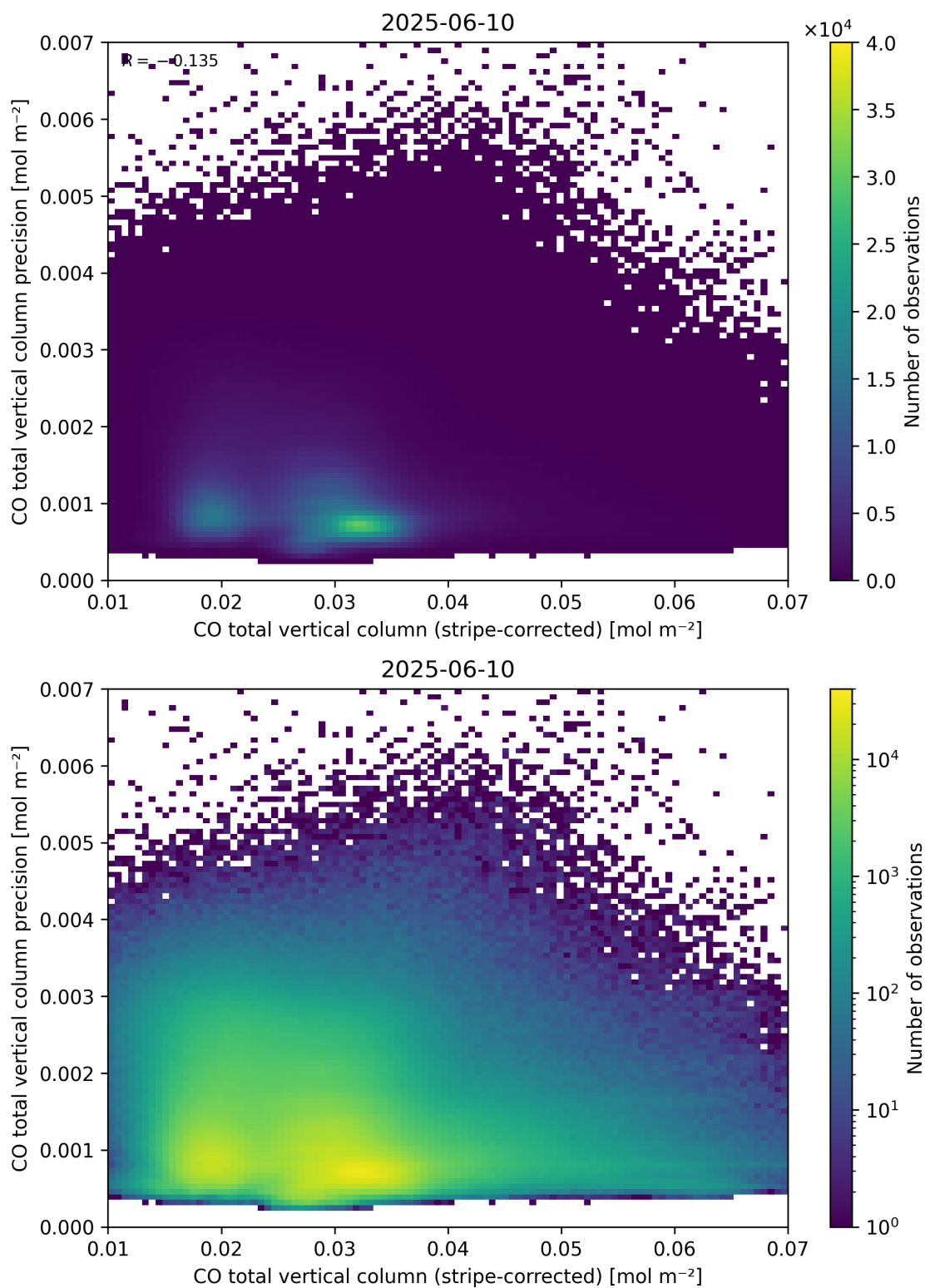
Figure 36: Scatter density plot of “CO total vertical column (stripe-corrected)” against “CO total vertical column precision” for 2025-06-09 to 2025-06-11.
