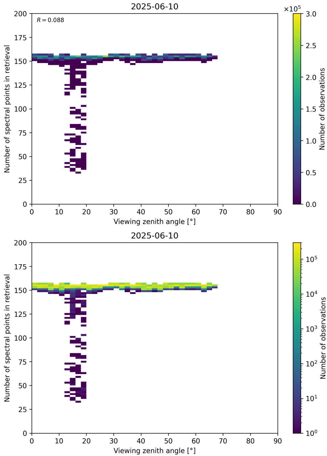
Figure 76: Scatter density plot of “Viewing zenith angle” against “Number of spectral points in retrieval” for 2025-06-09 to 2025-06-11.
