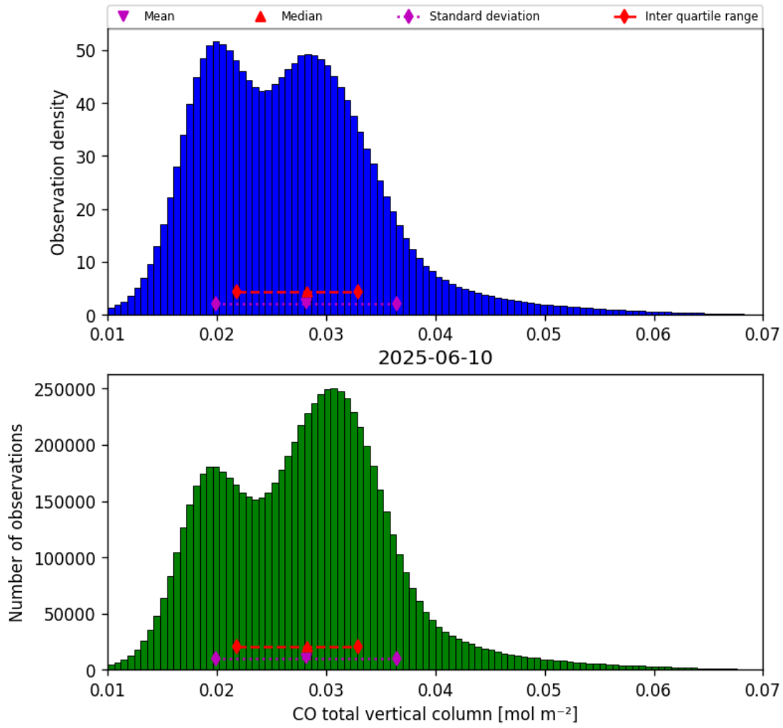
Figure 18: Histogram of “CO total vertical column” for 2025-06-09 to 2025-06-11
