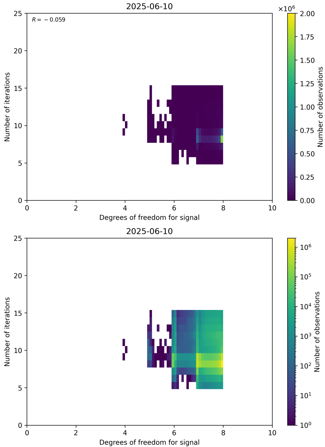
Figure 50: Scatter density plot of “Degrees of freedom for signal” against “Number of iterations” for 2025-06-09 to 2025-06-11.
