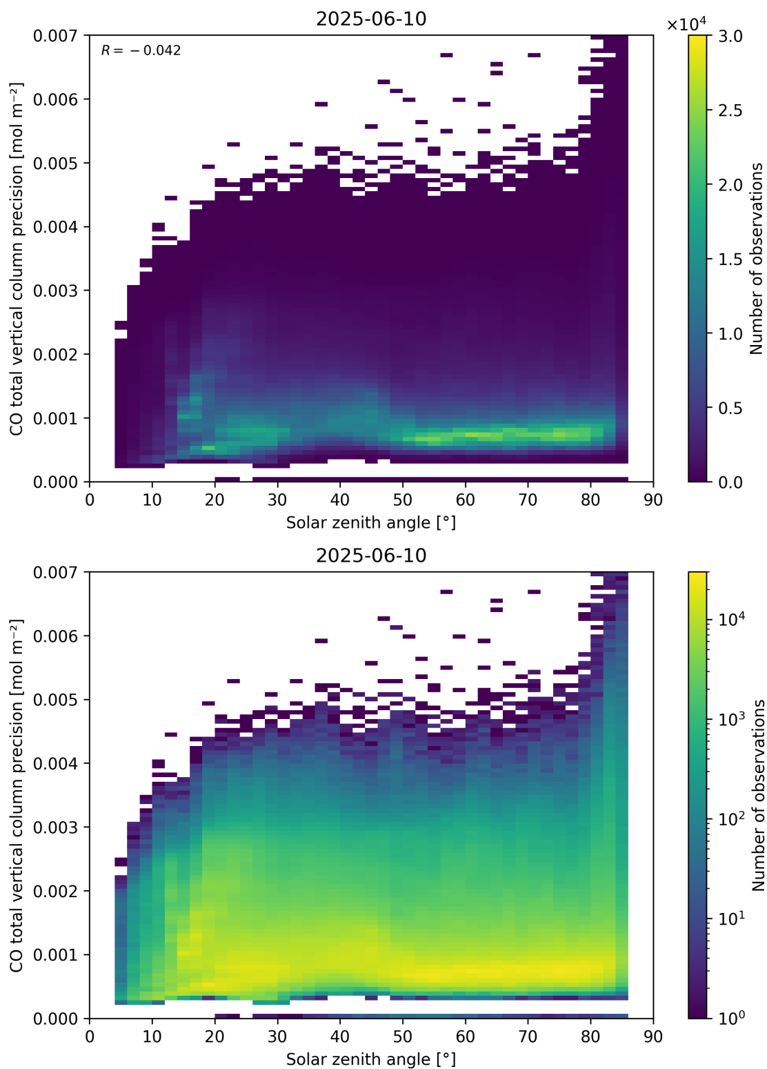
Figure 63: Scatter density plot of “Solar zenith angle” against “CO total vertical column precision” for 2025-06-09 to 2025-06-11.
