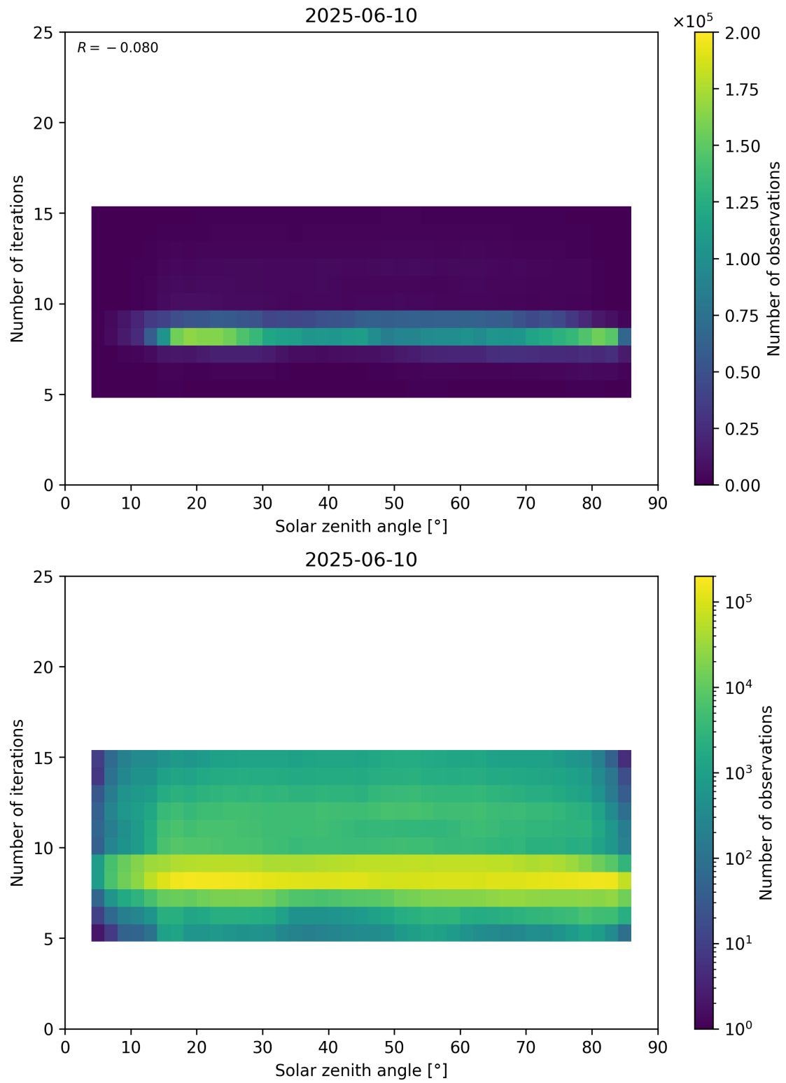
Figure 67: Scatter density plot of “Solar zenith angle” against “Number of iterations” for 2025-06-09 to 2025-06-11.
