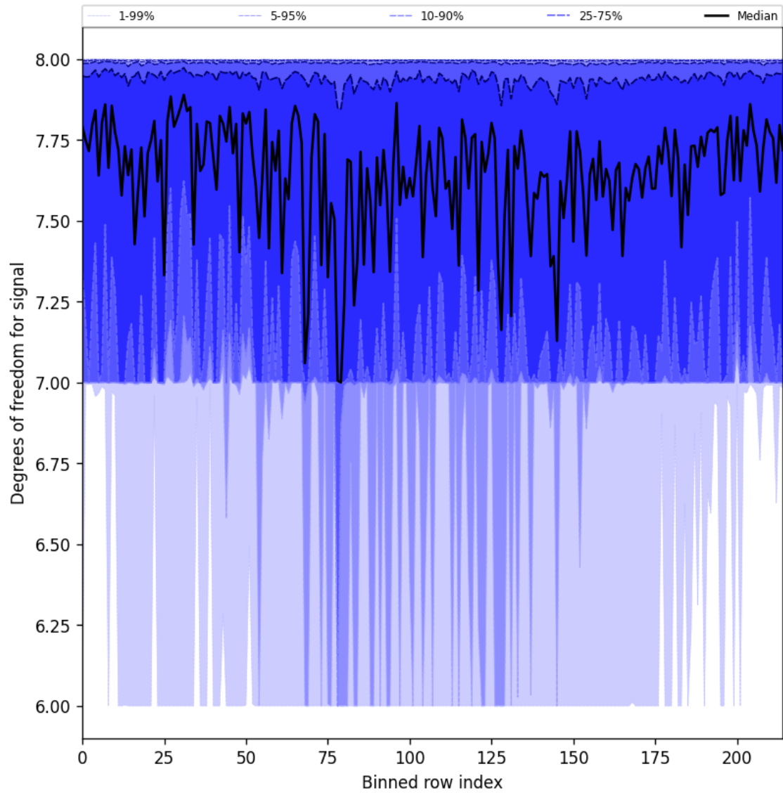
Figure 31: Along track statistics of “Degrees of freedom for signal” for 2025-06-09 to 2025-06-11
