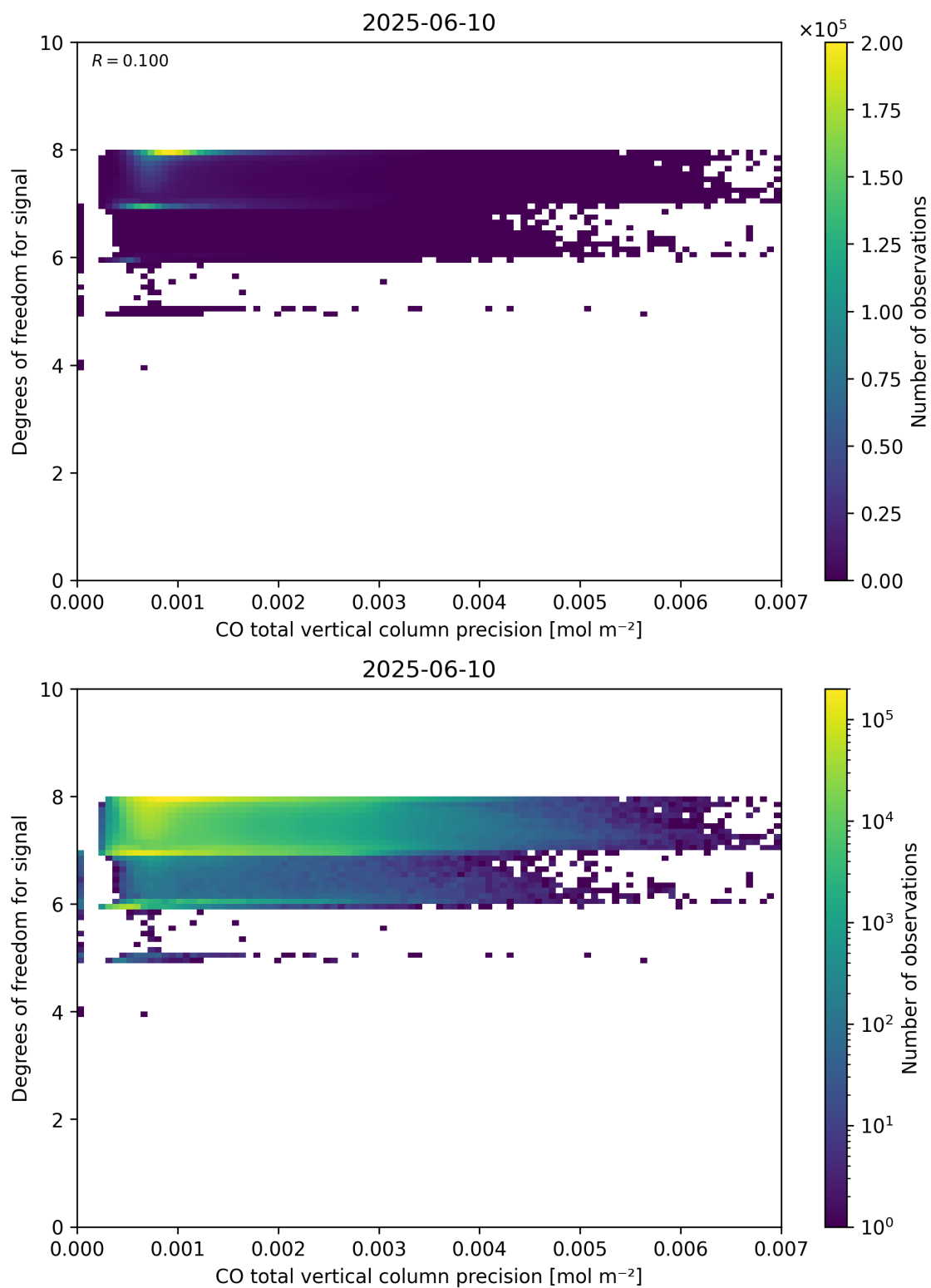
Figure 45: Scatter density plot of “CO total vertical column precision” against “Degrees of freedom for signal” for 2025-06-09 to 2025-06-11.
