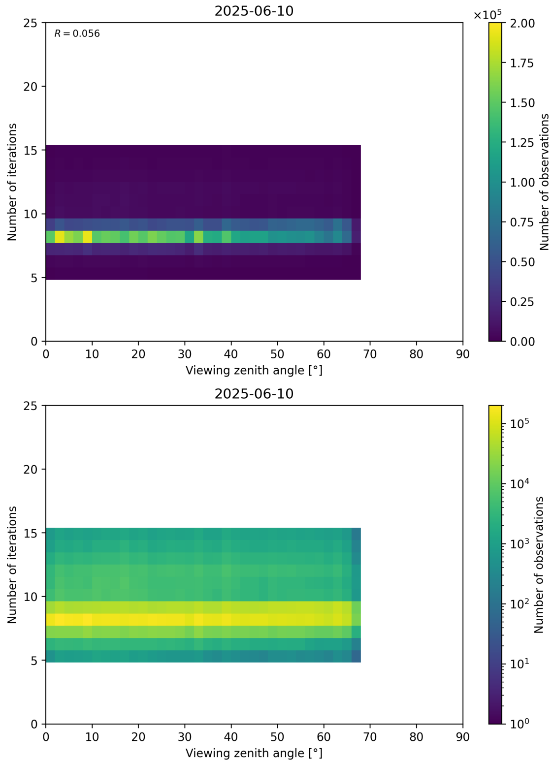
Figure 75: Scatter density plot of “Viewing zenith angle” against “Number of iterations” for 2025-06-09 to 2025-06-11.
