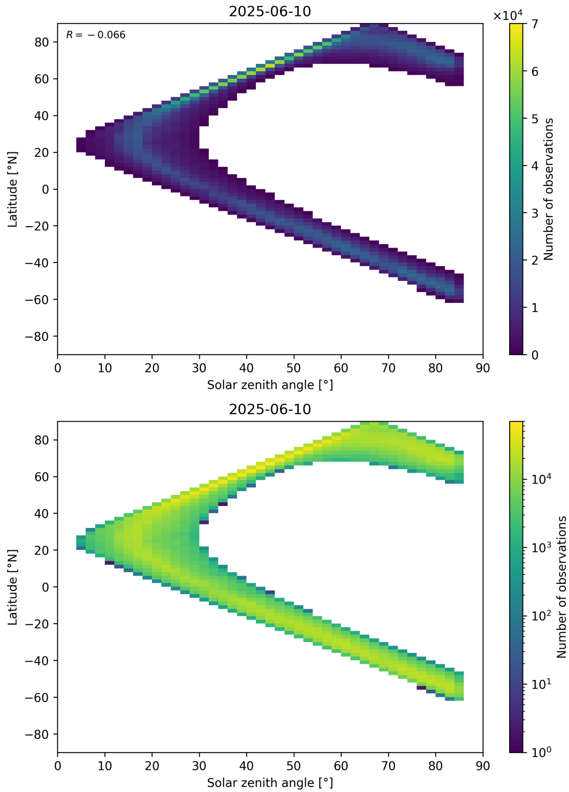
Figure 66: Scatter density plot of “Solar zenith angle” against “Latitude” for 2025-06-09 to 2025-06-11.
