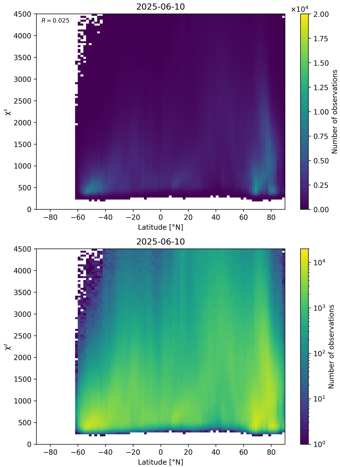
Figure 54: Scatter density plot of “Latitude” against “ \chi^2 ” for 2025-06-09 to 2025-06-11.
