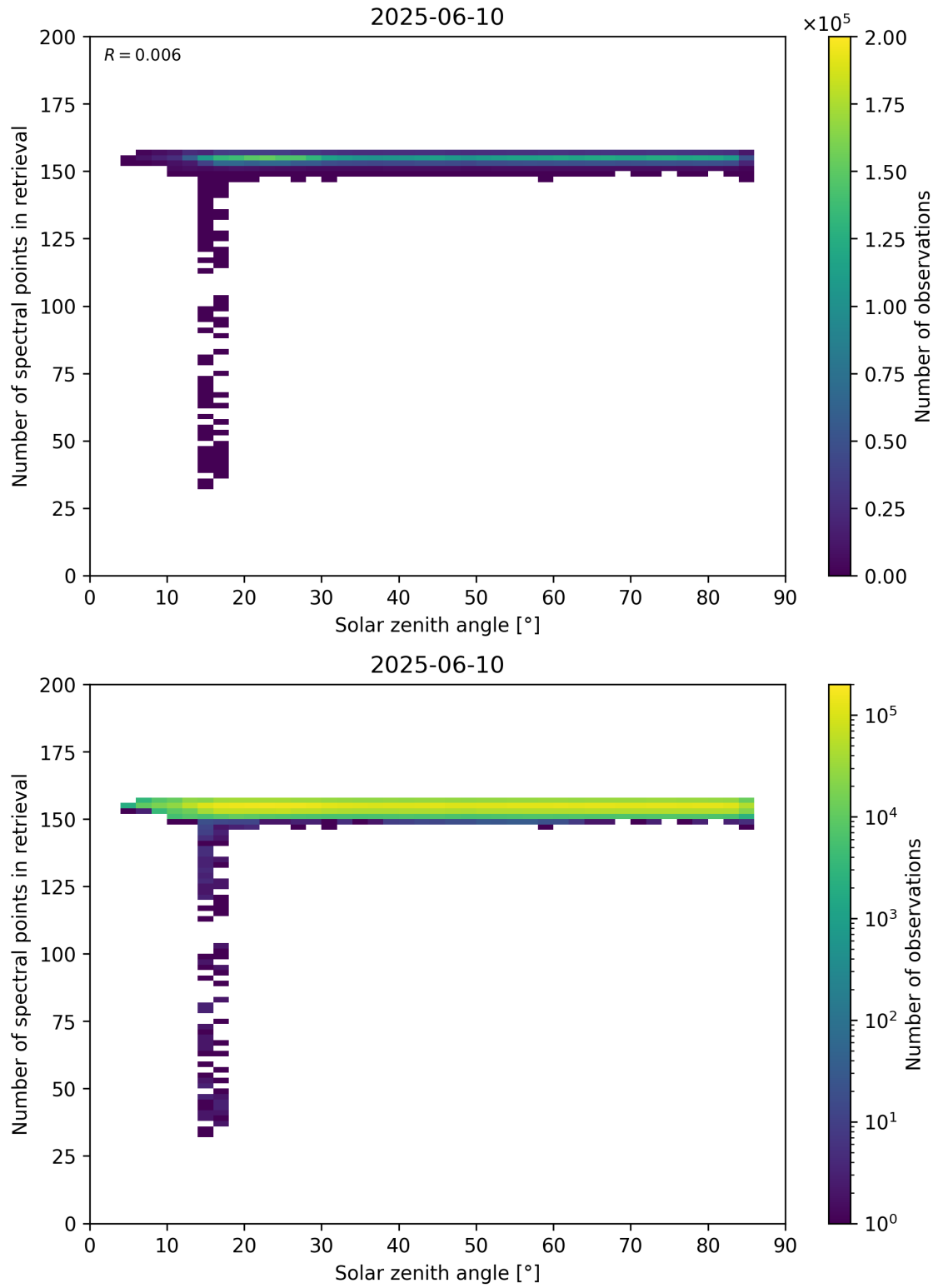
Figure 68: Scatter density plot of “Solar zenith angle” against “Number of spectral points in retrieval” for 2025-06-09 to 2025-06-11.
