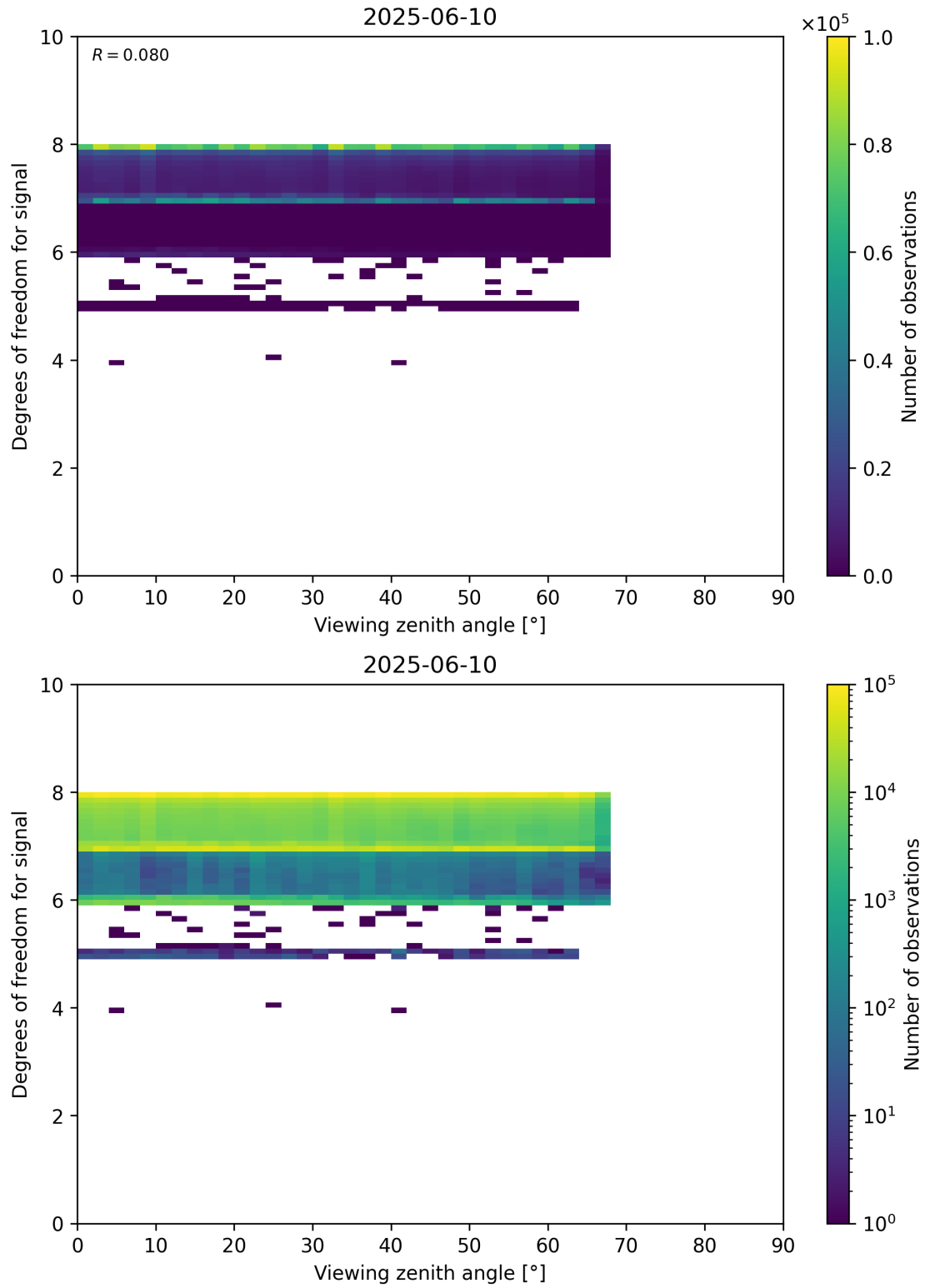
Figure 73: Scatter density plot of “Viewing zenith angle” against “Degrees of freedom for signal” for 2025-06-09 to 2025-06-11.
