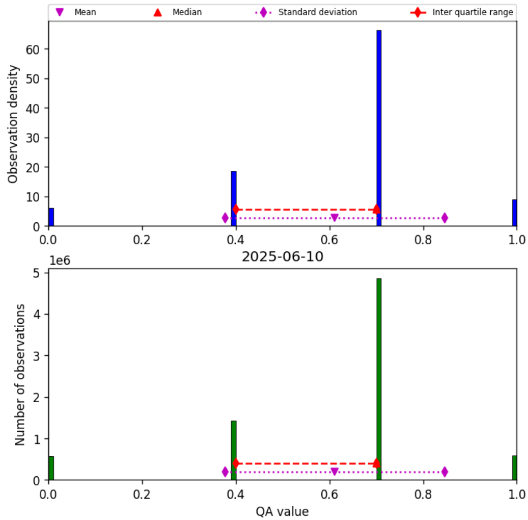
Figure 17: Histogram of “QA value” for 2025-06-09 to 2025-06-11
