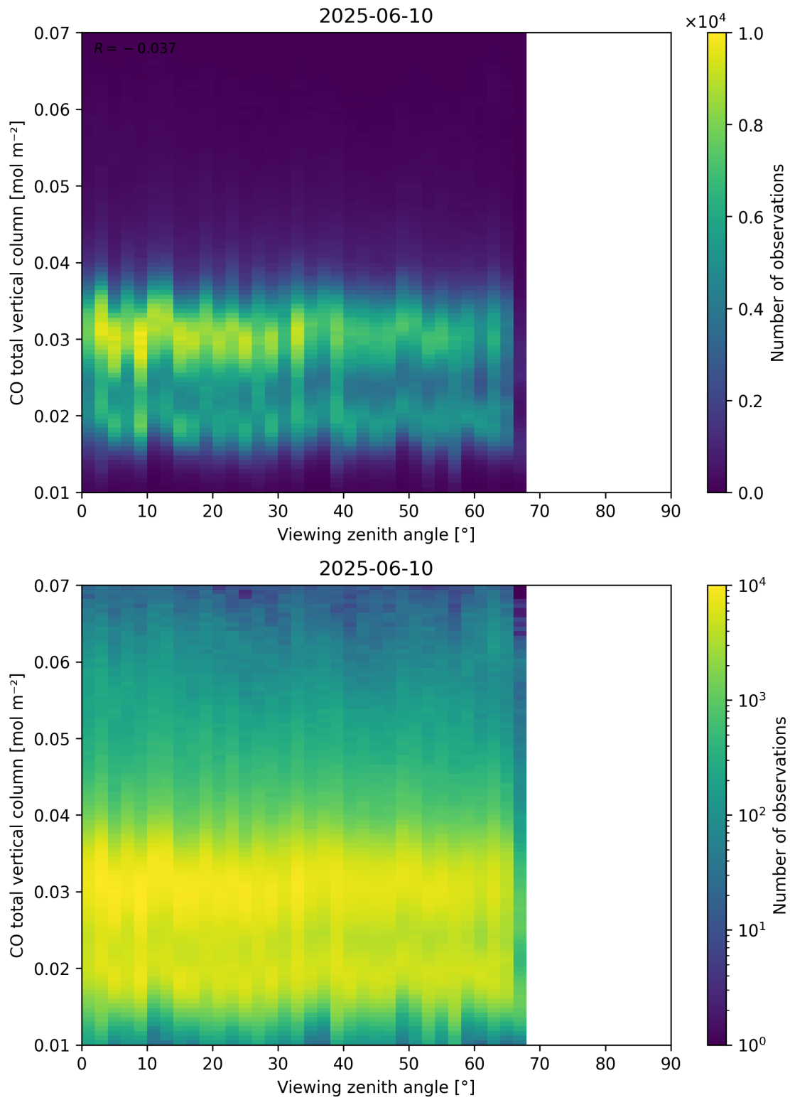
Figure 69: Scatter density plot of “Viewing zenith angle” against “CO total vertical column” for 2025-06-09 to 2025-06-11.
