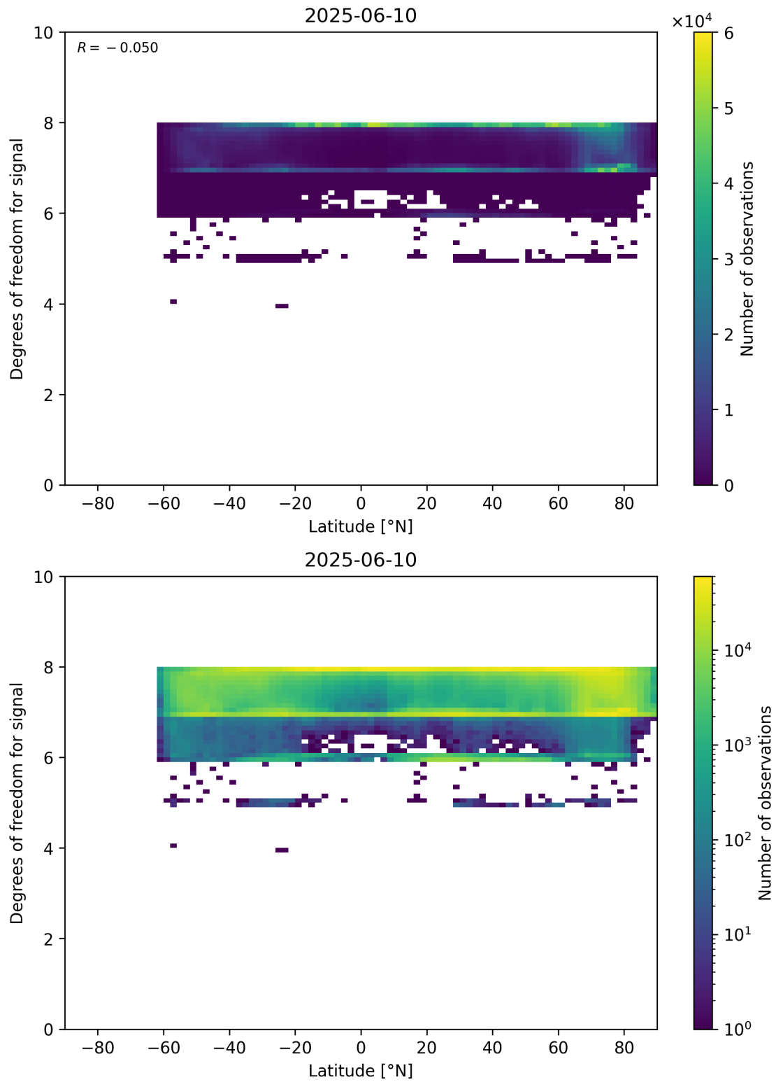
Figure 55: Scatter density plot of “Latitude” against “Degrees of freedom for signal” for 2025-06-09 to 2025-06-11.
