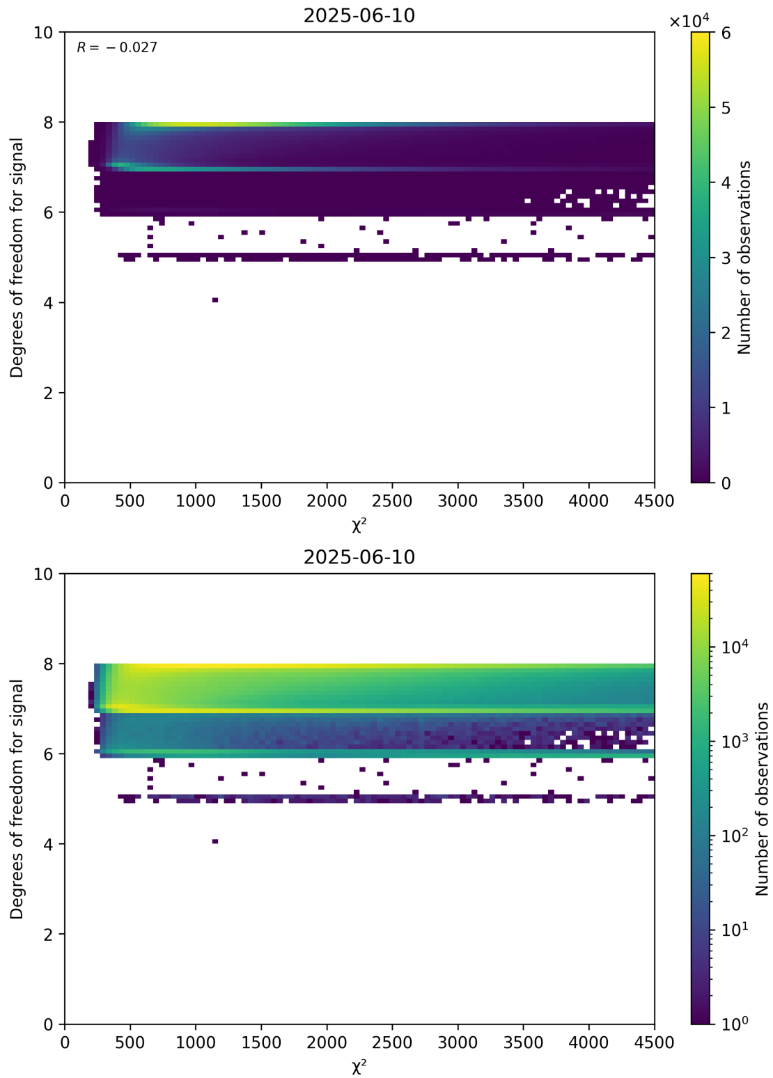
Figure 48: Scatter density plot of “ \chi^2 ” against “Degrees of freedom for signal” for 2025-06-09 to 2025-06-11.
