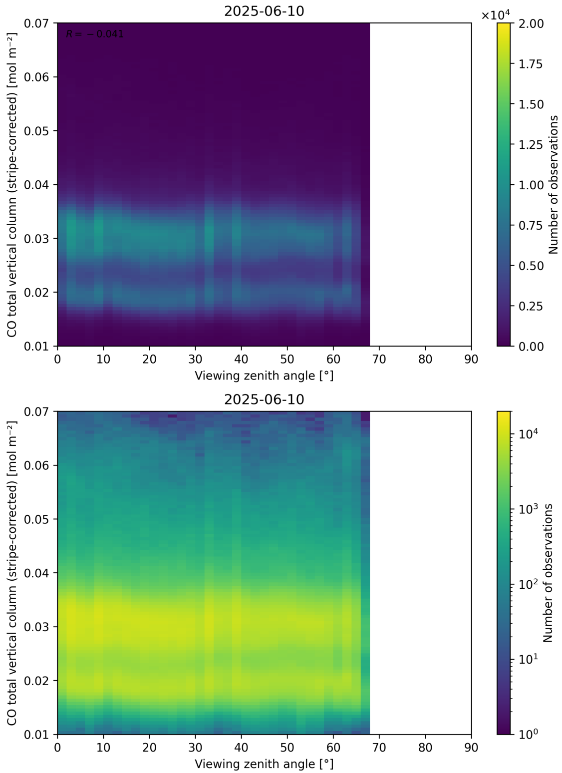
Figure 70: Scatter density plot of “Viewing zenith angle” against “CO total vertical column (stripe-corrected)” for 2025-06-09 to 2025-06-11.
