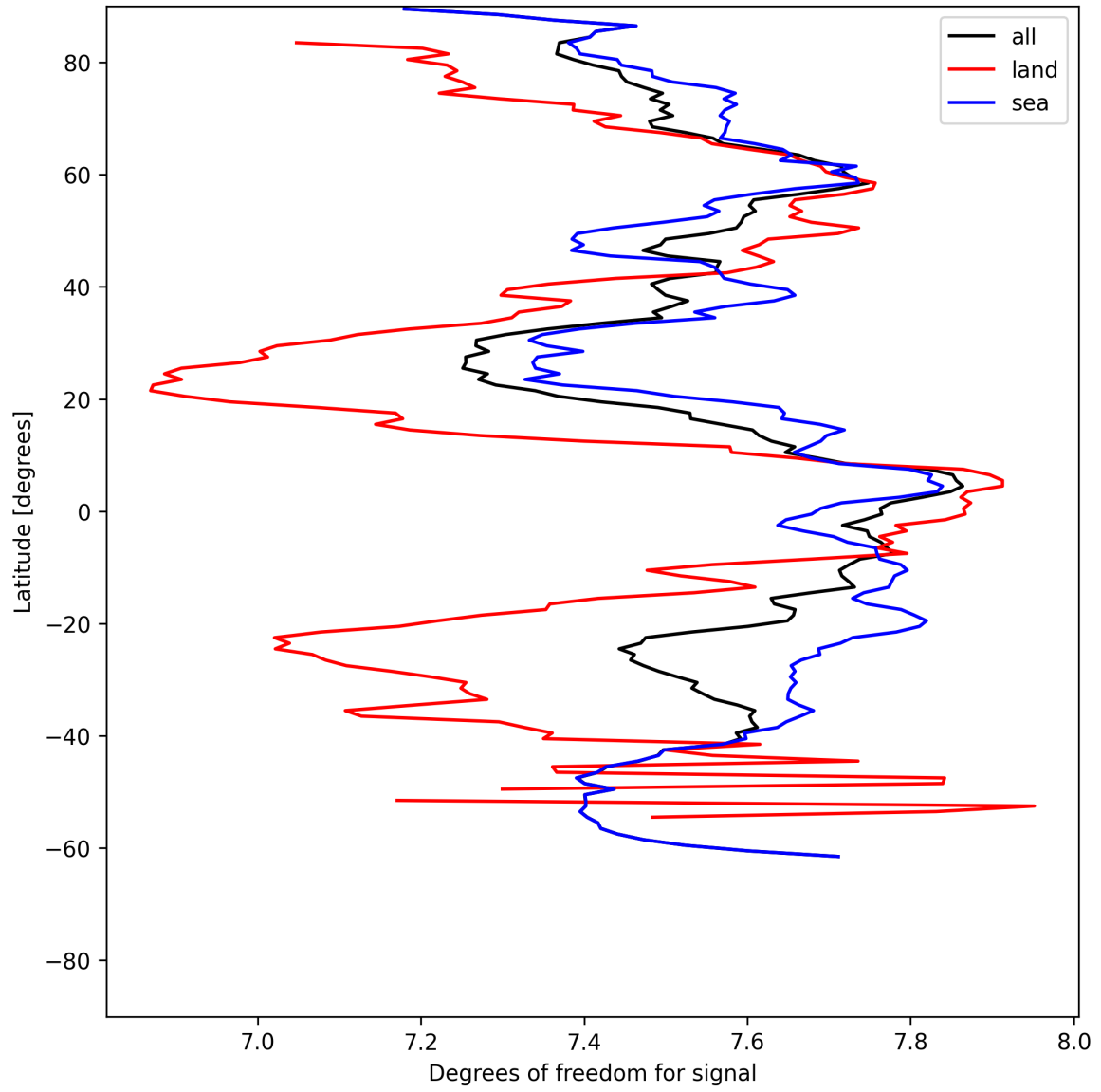
Figure 15: Zonal average of “Degrees of freedom for signal” for 2025-06-09 to 2025-06-11.
