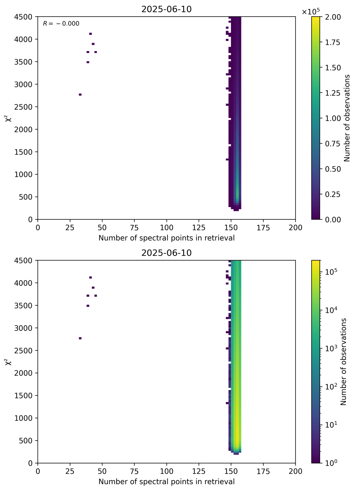
Figure 58: Scatter density plot of “Number of spectral points in retrieval” against “ \chi^2 ” for 2025-06-09 to 2025-06-11.
