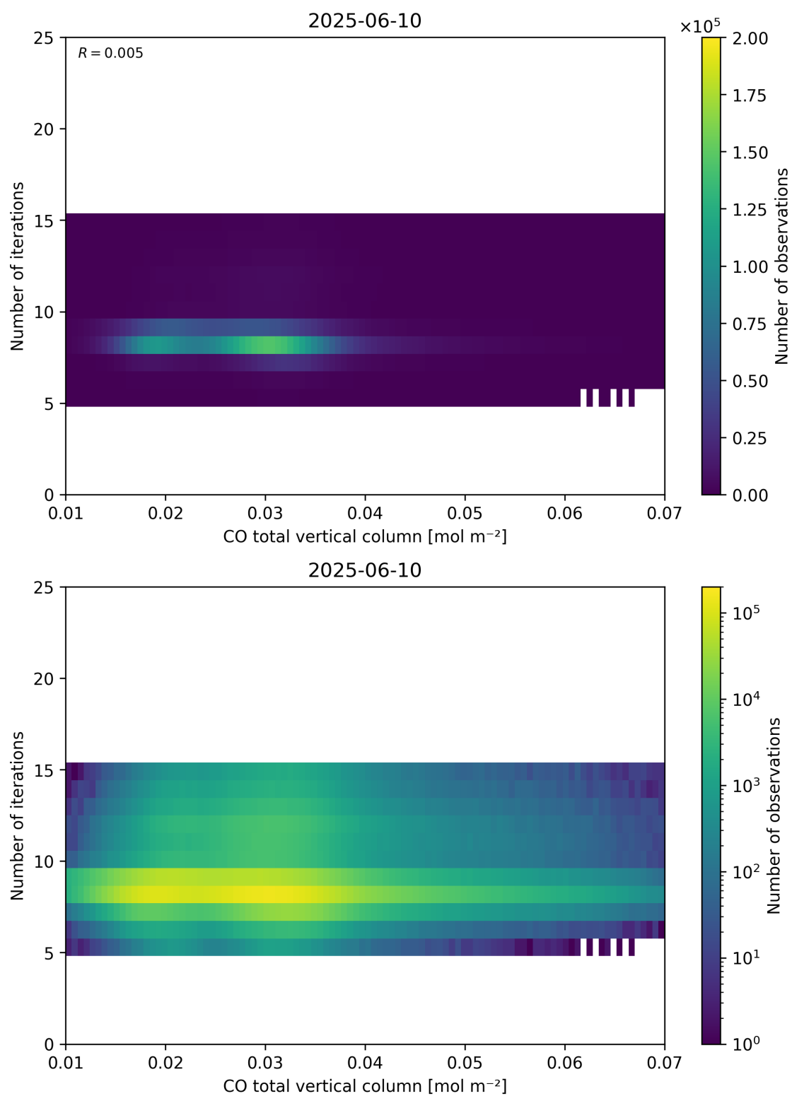
Figure 42: Scatter density plot of “CO total vertical column” against “Number of iterations” for 2025-06-09 to 2025-06-11.
