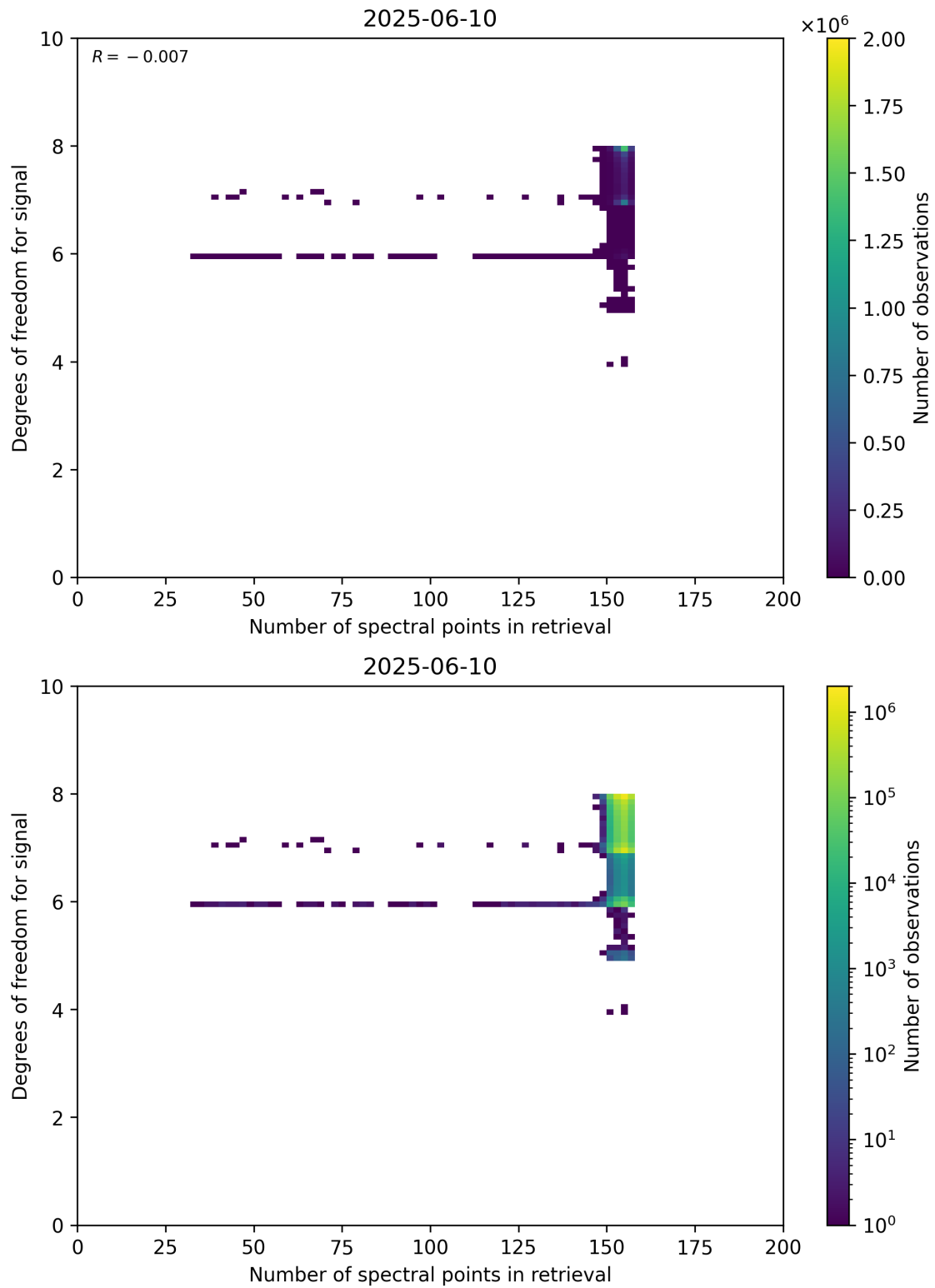
Figure 59: Scatter density plot of “Number of spectral points in retrieval” against “Degrees of freedom for signal” for 2025-06-09 to 2025-06-11.
