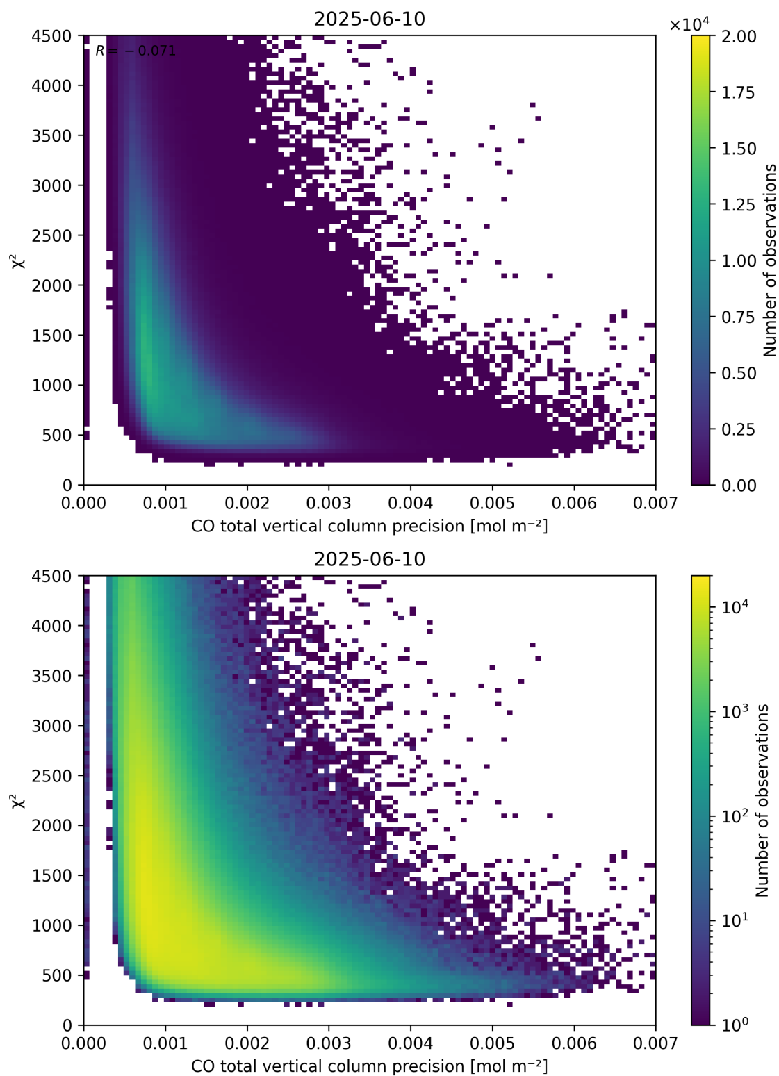
Figure 44: Scatter density plot of “CO total vertical column precision” against “ \chi^2 ” for 2025-06-09 to 2025-06-11.
