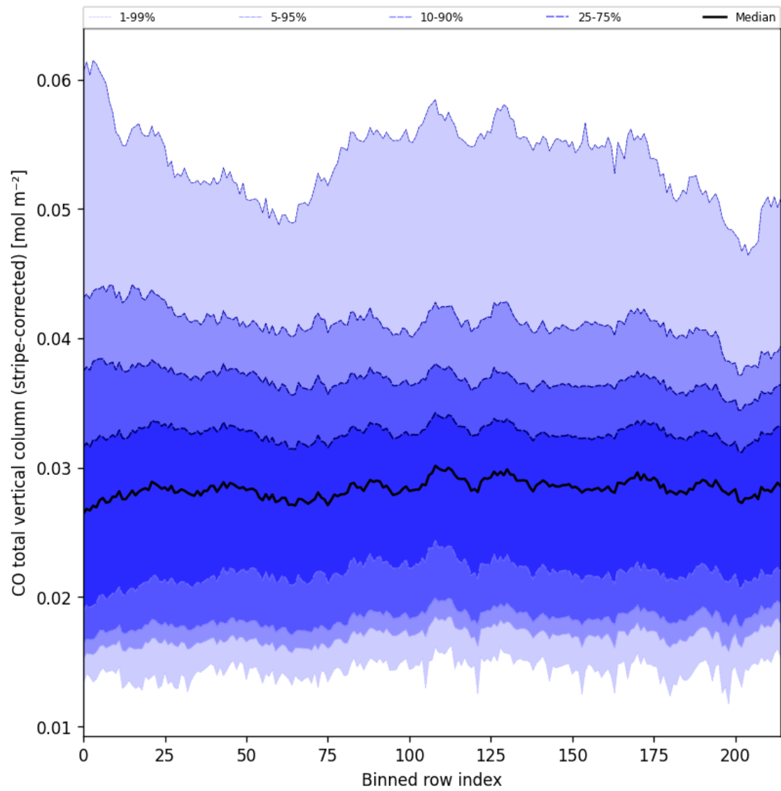
Figure 27: Along track statistics of “CO total vertical column (stripe-corrected)” for 2025-06-09 to 2025-06-11
