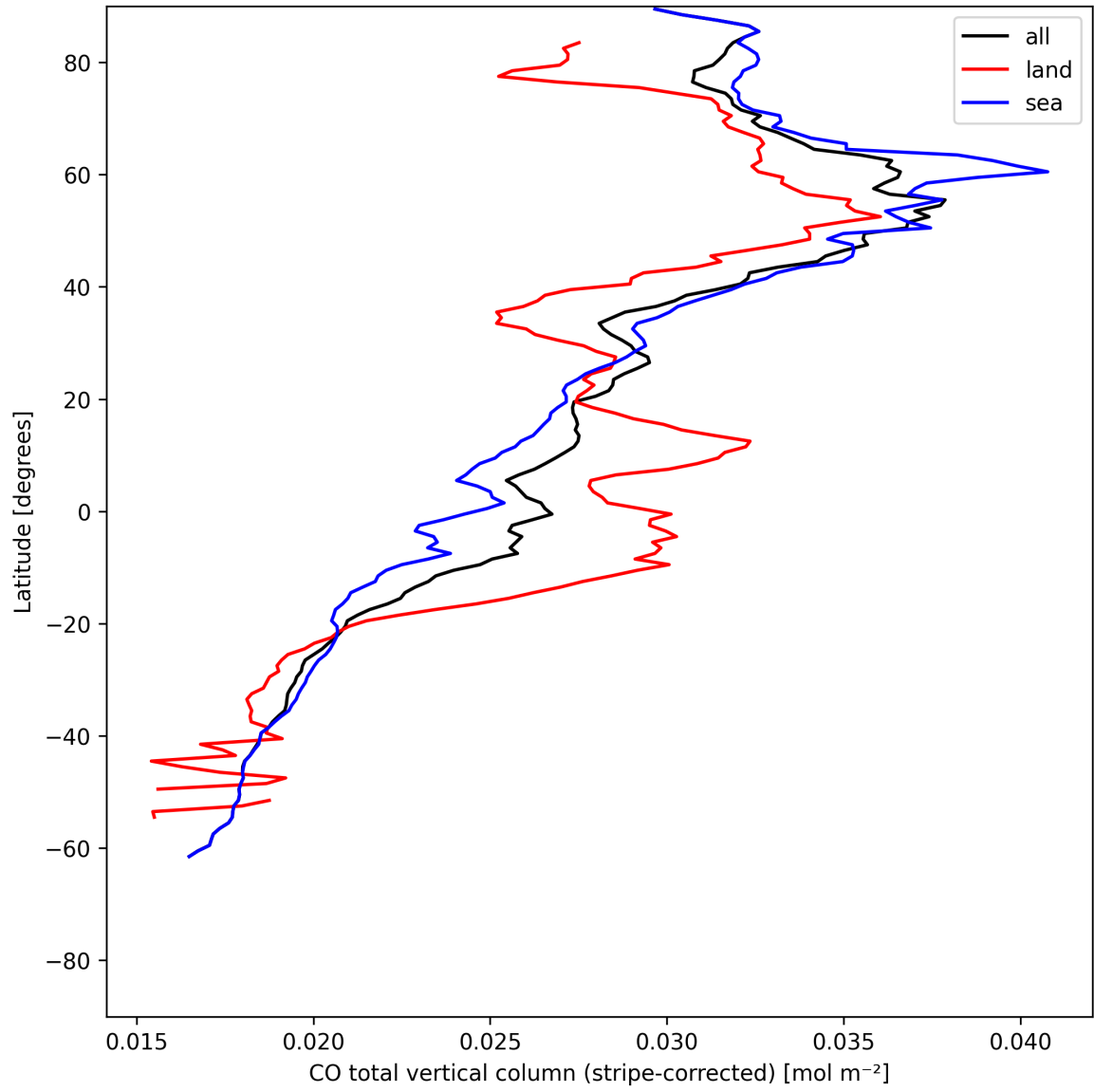
Figure 11: Zonal average of “CO total vertical column (stripe-corrected)” for 2025-06-09 to 2025-06-11.
