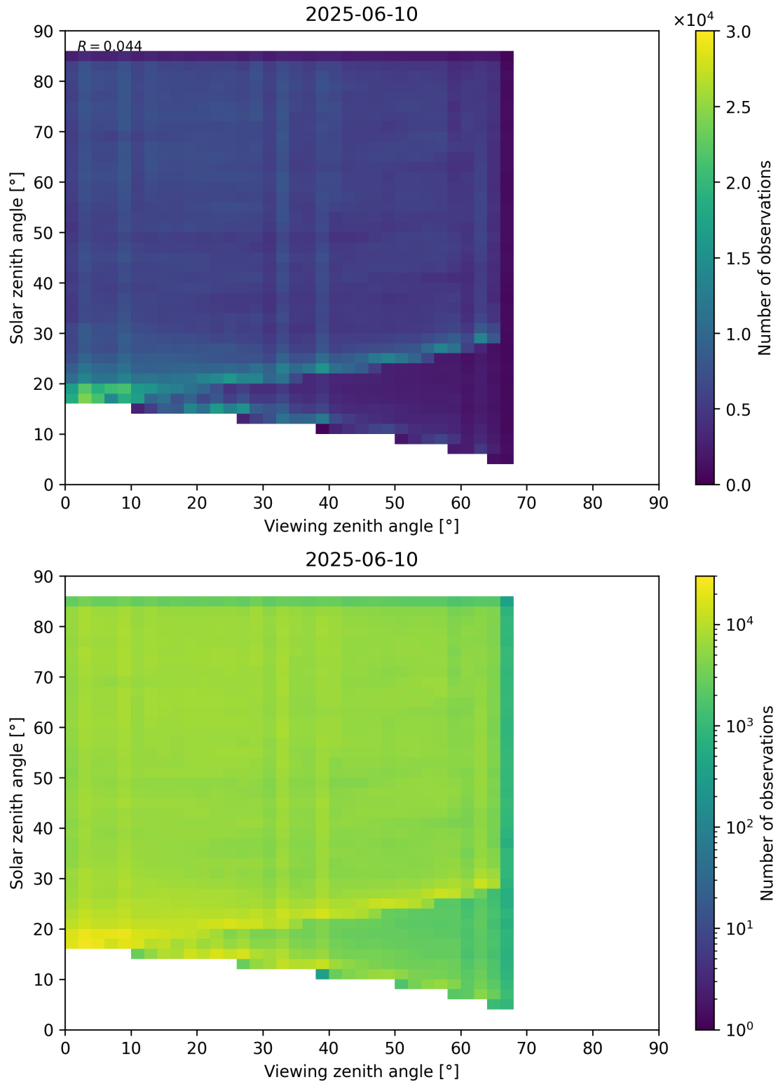
Figure 77: Scatter density plot of “Viewing zenith angle” against “Solar zenith angle” for 2025-06-09 to 2025-06-11.
