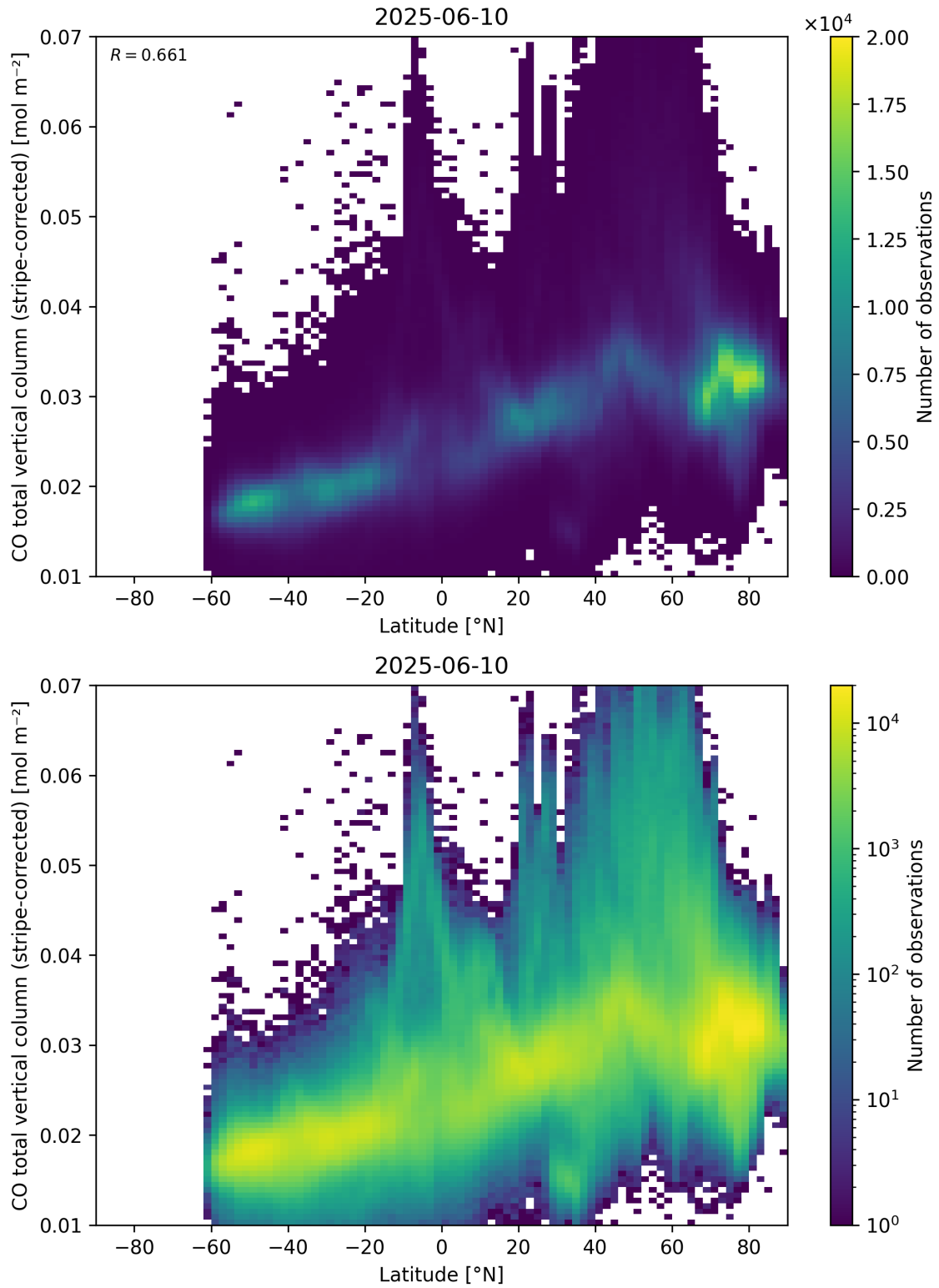
Figure 52: Scatter density plot of “Latitude” against “CO total vertical column (stripe-corrected)” for 2025-06-09 to 2025-06-11.
