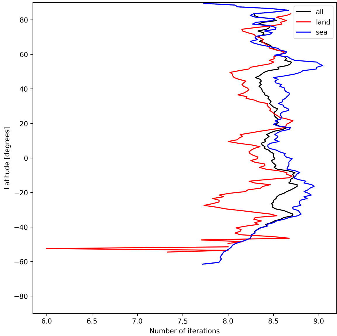
Figure 16: Zonal average of “Number of iterations” for 2025-06-09 to 2025-06-11.
