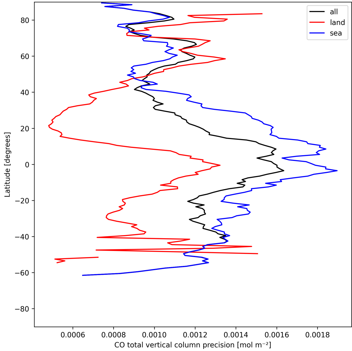
Figure 12: Zonal average of “CO total vertical column precision” for 2025-06-09 to 2025-06-11.
