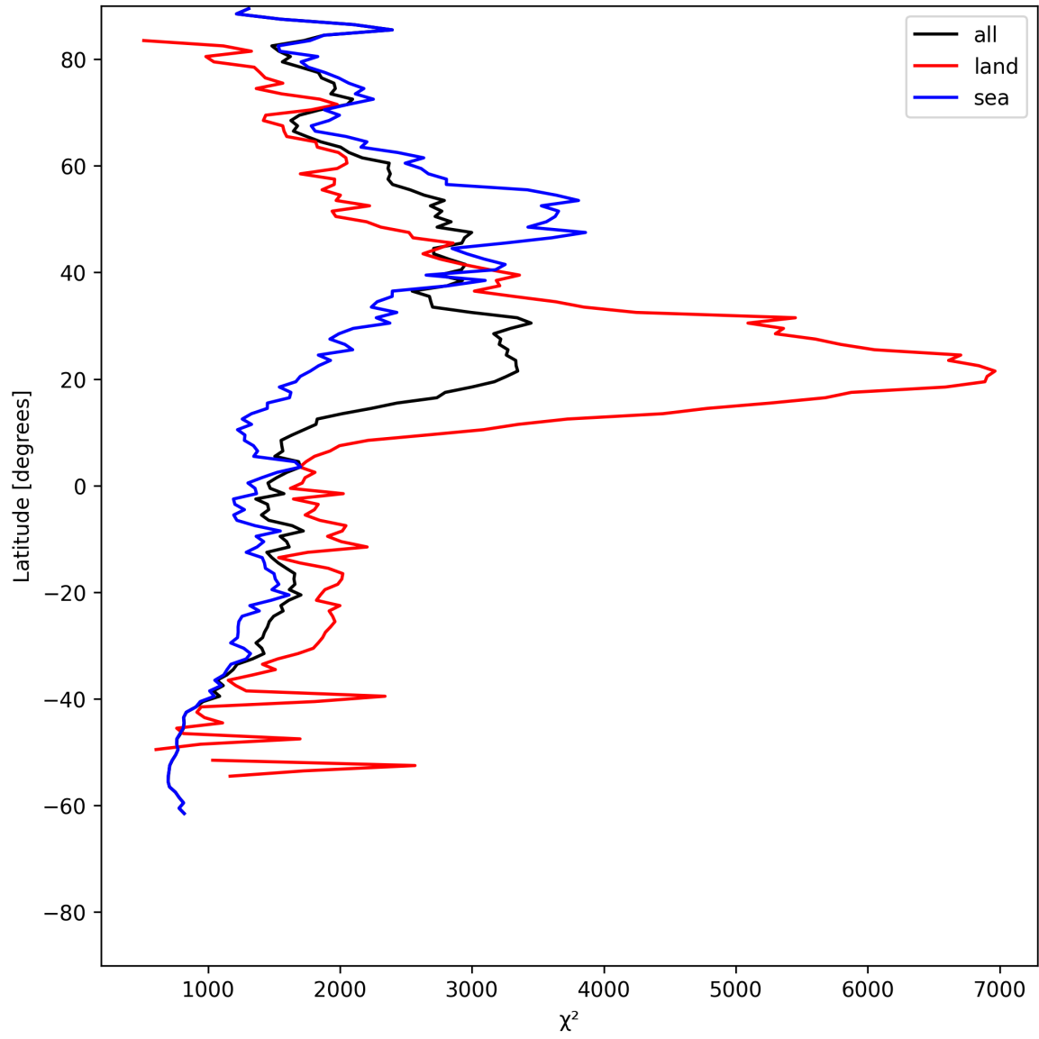
Figure 14: Zonal average of “ \chi^2 ” for 2025-06-09 to 2025-06-11.
