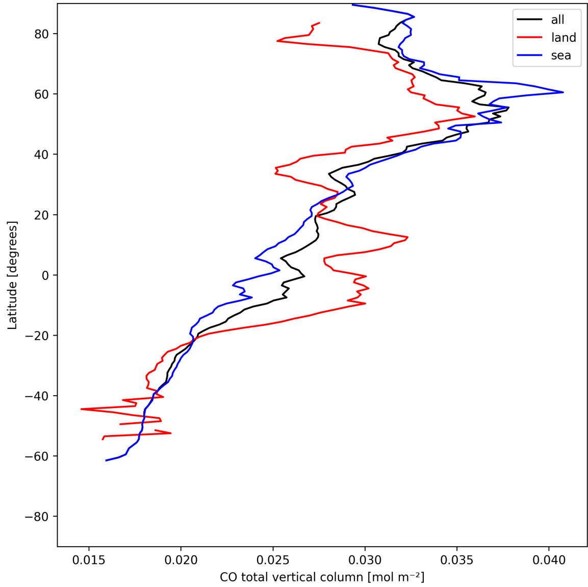
Figure 10: Zonal average of “CO total vertical column” for 2025-06-09 to 2025-06-11.
