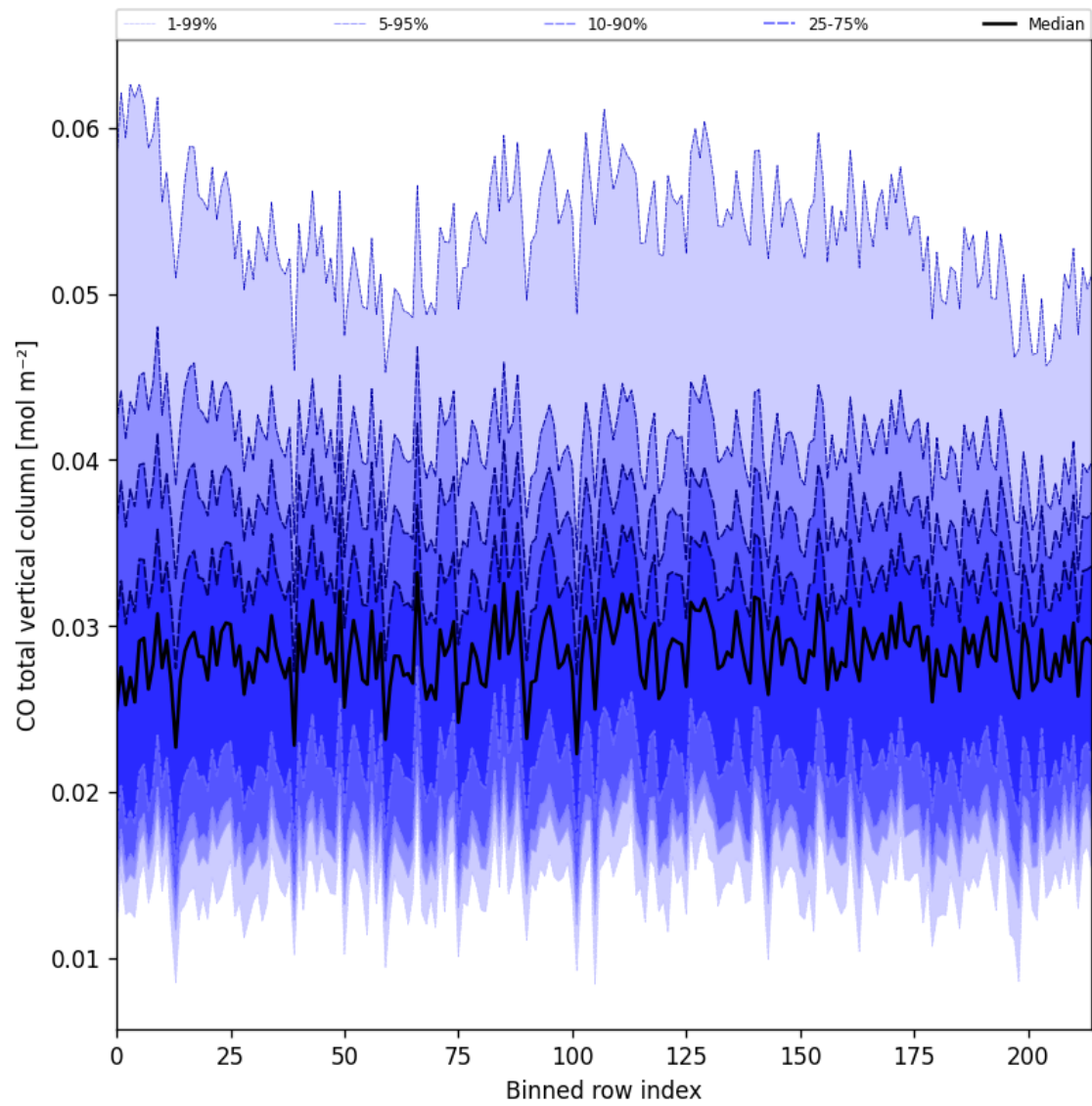
Figure 26: Along track statistics of "CO total vertical column" for 2025-06-09 to 2025-06-11
