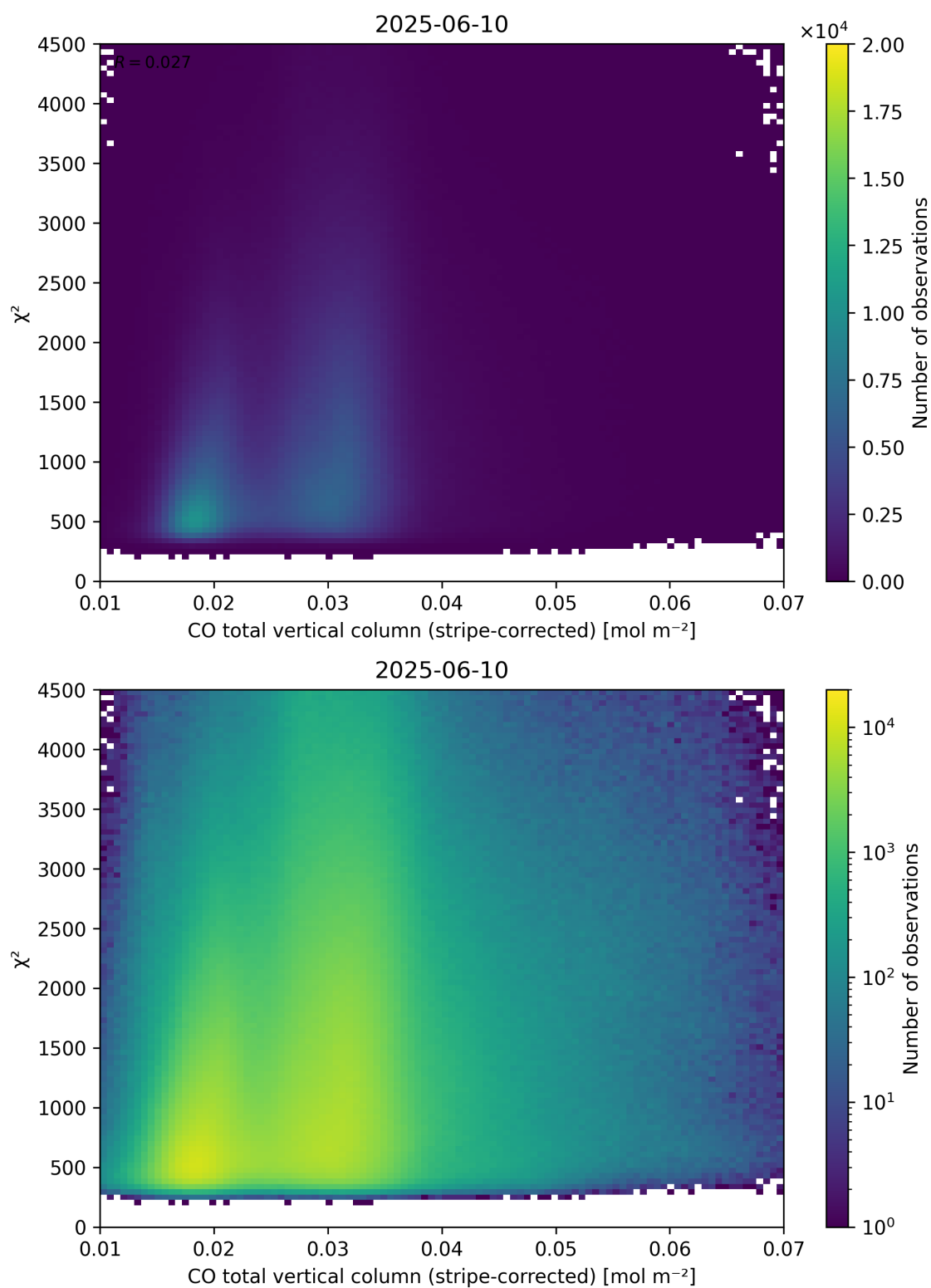
Figure 37: Scatter density plot of “CO total vertical column (stripe-corrected)” against “ \chi^2 ” for 2025-06-09 to 2025-06-11.
