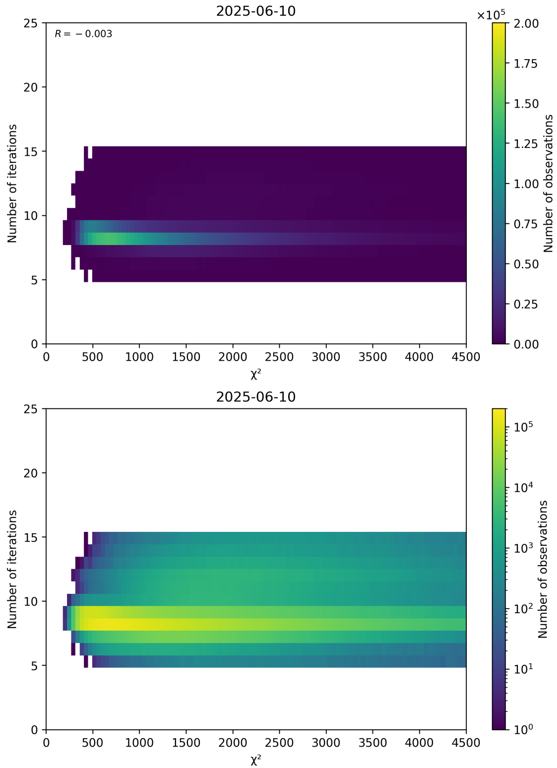
Figure 49: Scatter density plot of “ \chi^2 ” against “Number of iterations” for 2025-06-09 to 2025-06-11.
