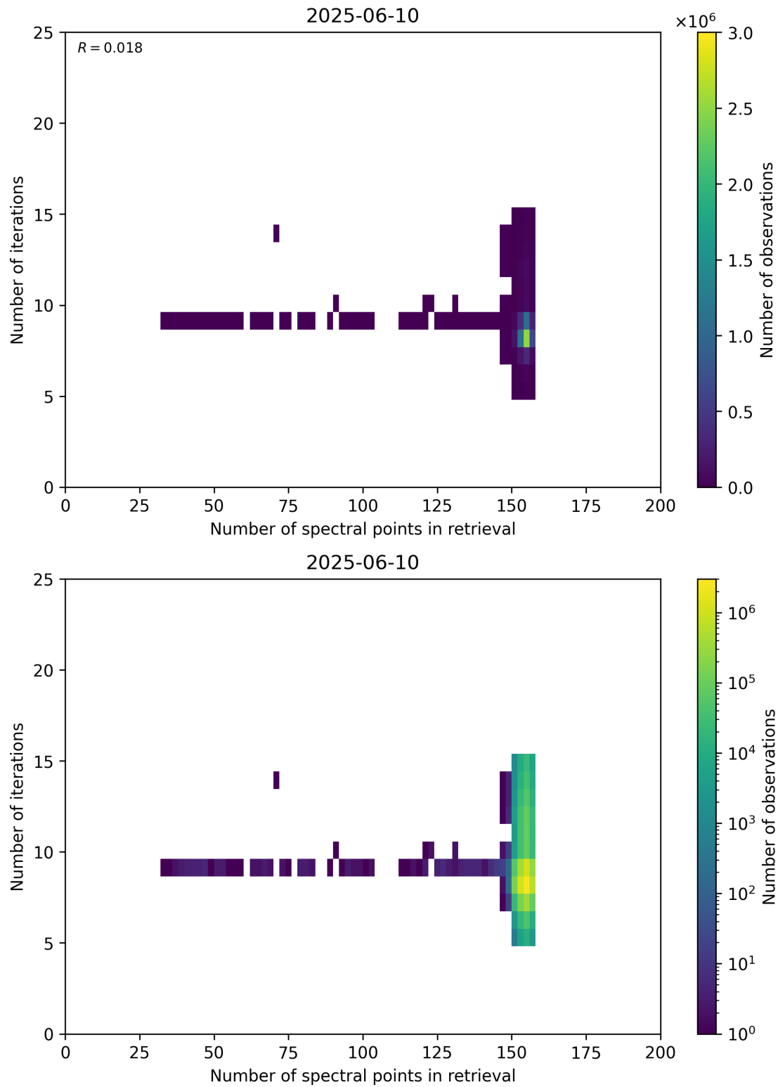
Figure 60: Scatter density plot of “Number of spectral points in retrieval” against “Number of iterations” for 2025-06-09 to 2025-06-11.
