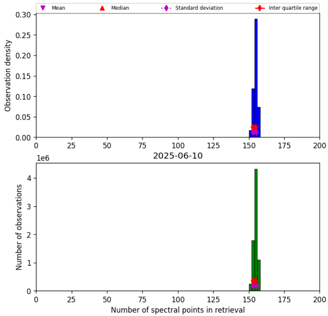
Figure 21: Histogram of “Number of spectral points in retrieval” for 2025-06-09 to 2025-06-11
