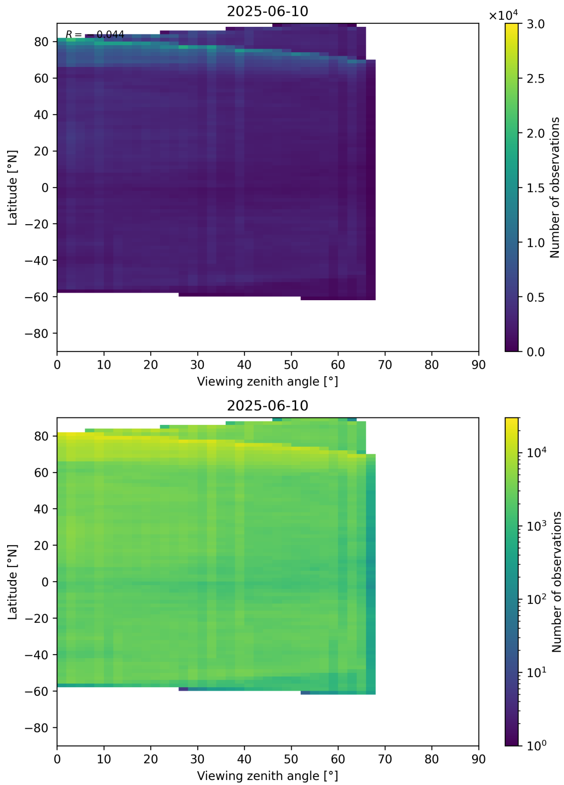
Figure 74: Scatter density plot of “Viewing zenith angle” against “Latitude” for 2025-06-09 to 2025-06-11.
