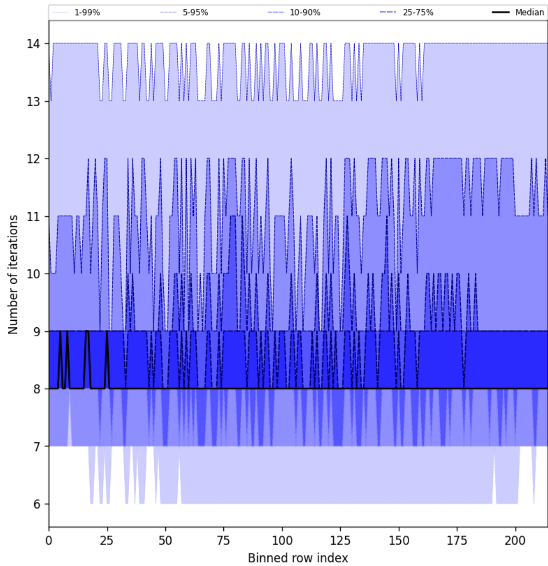
Figure 32: Along track statistics of “Number of iterations” for 2025-06-09 to 2025-06-11
