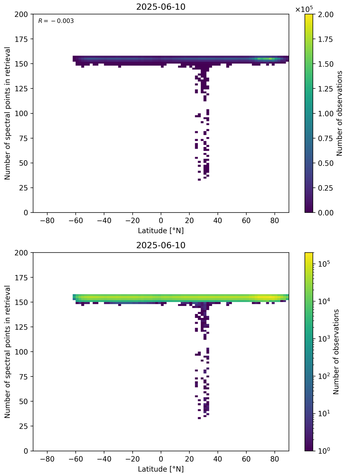
Figure 57: Scatter density plot of “Latitude” against “Number of spectral points in retrieval” for 2025-06-09 to 2025-06-11.
