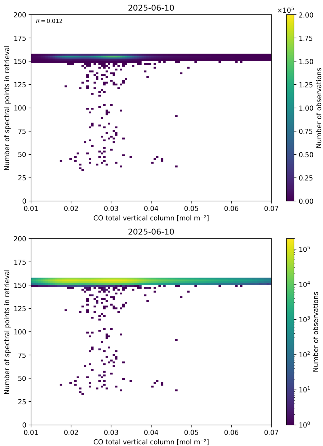
Figure 43: Scatter density plot of “CO total vertical column” against “Number of spectral points in retrieval” for 2025-06-09 to 2025-06-11.
