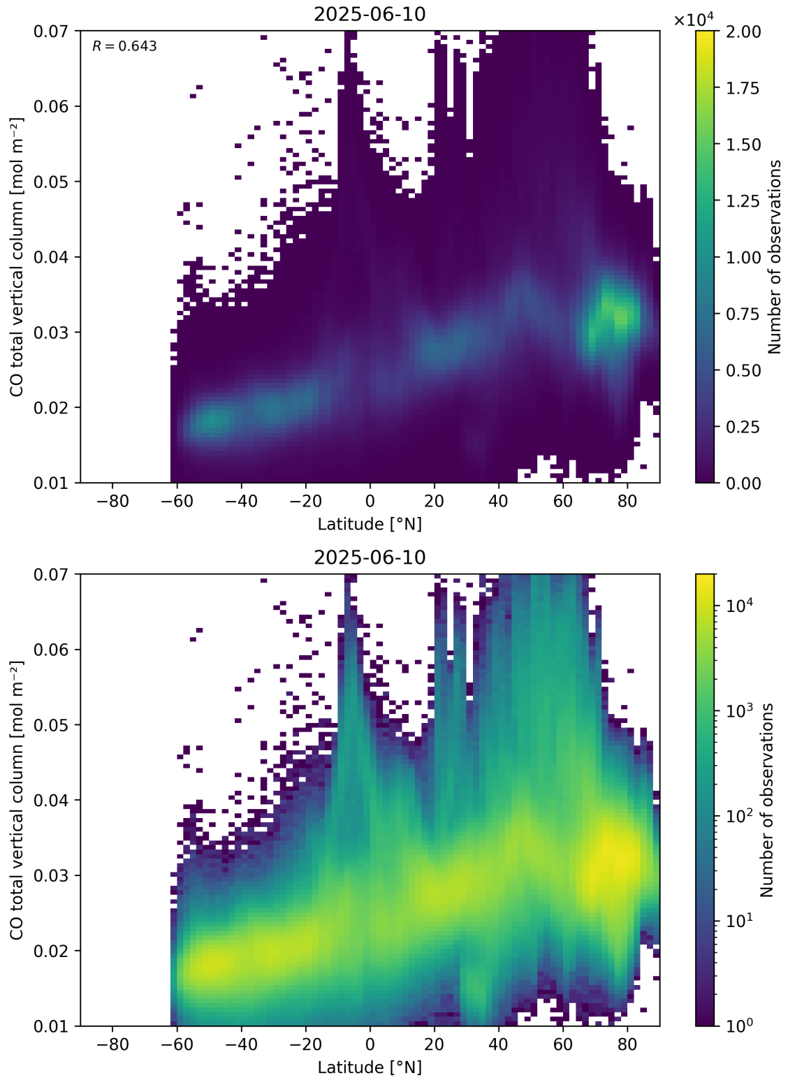
Figure 51: Scatter density plot of “Latitude” against “CO total vertical column” for 2025-06-09 to 2025-06-11.
