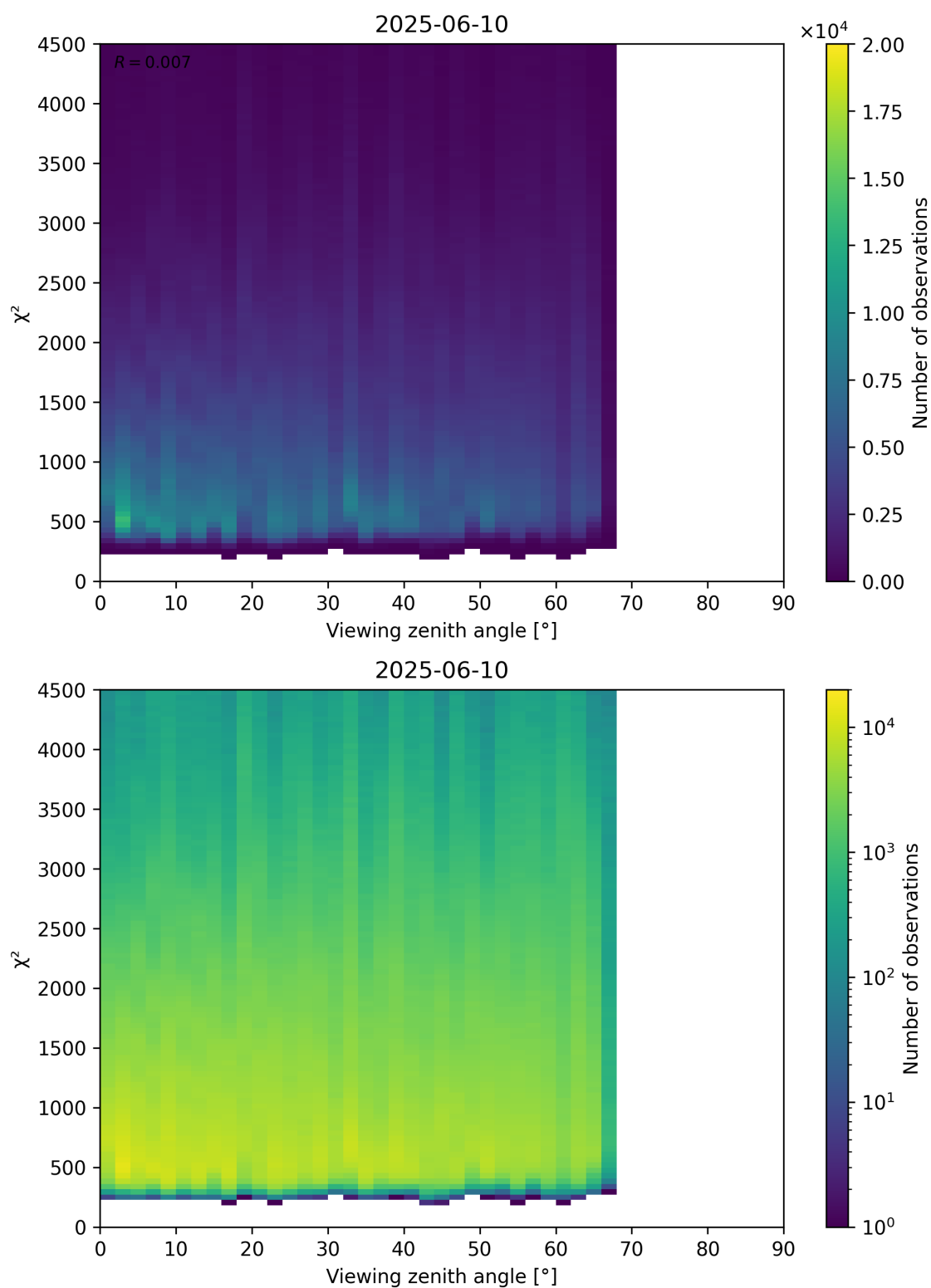
Figure 72: Scatter density plot of “Viewing zenith angle” against “ \chi^2 ” for 2025-06-09 to 2025-06-11.
