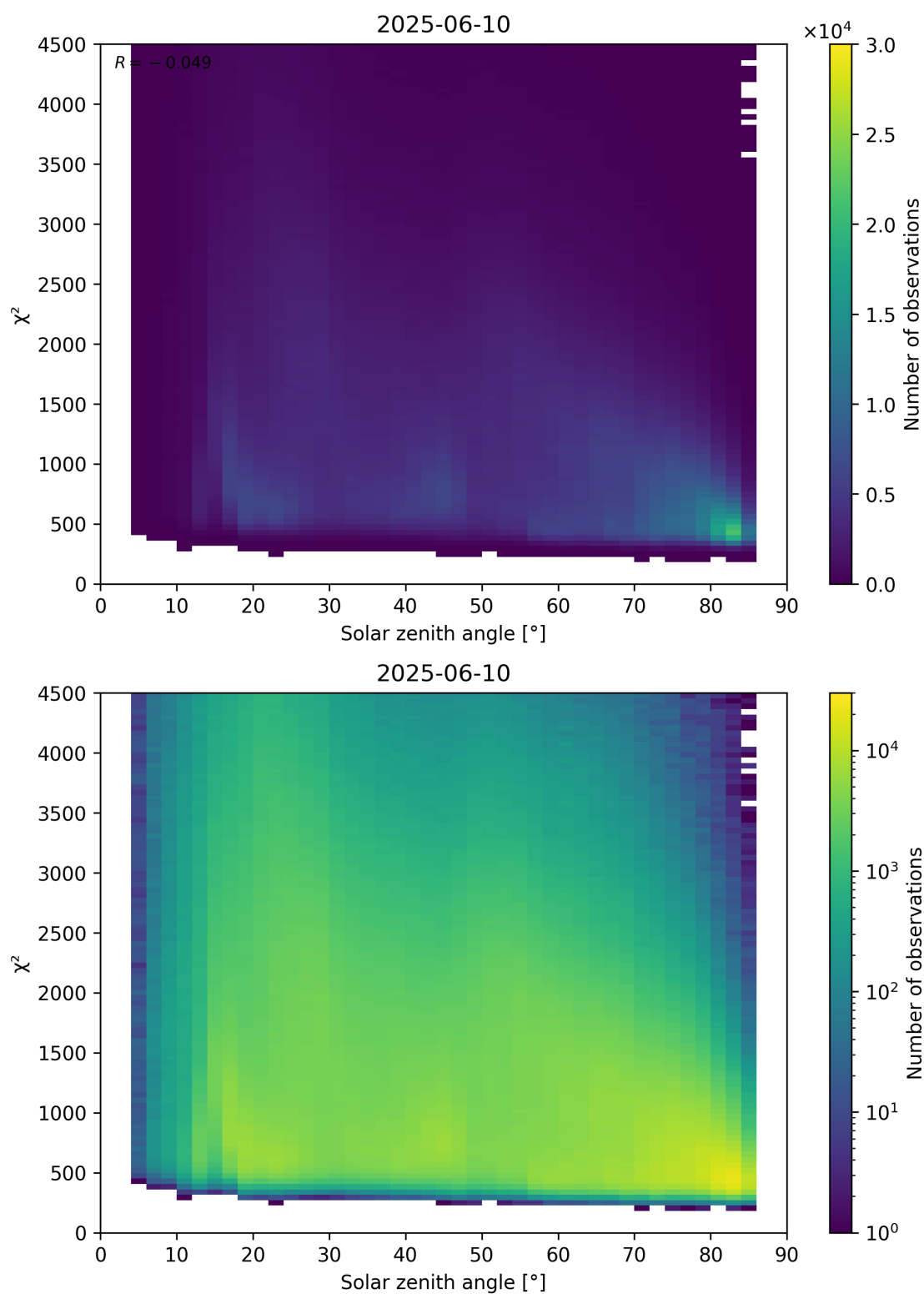
Figure 64: Scatter density plot of “Solar zenith angle” against “ \chi^2 ” for 2025-06-09 to 2025-06-11.
