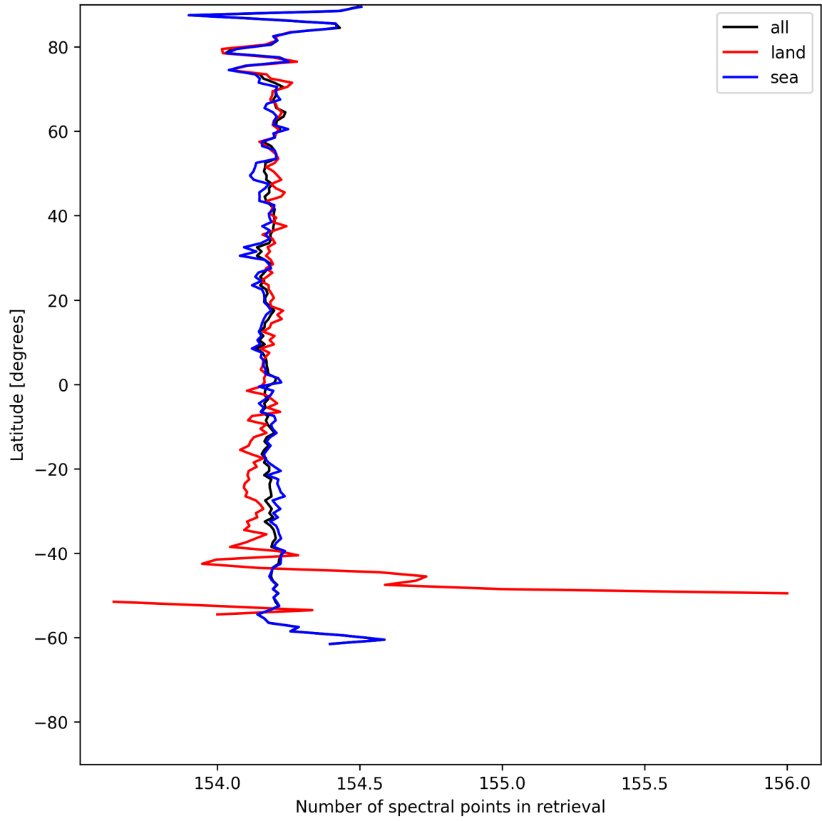
Figure 13: Zonal average of “Number of spectral points in retrieval” for 2025-06-09 to 2025-06-11.
