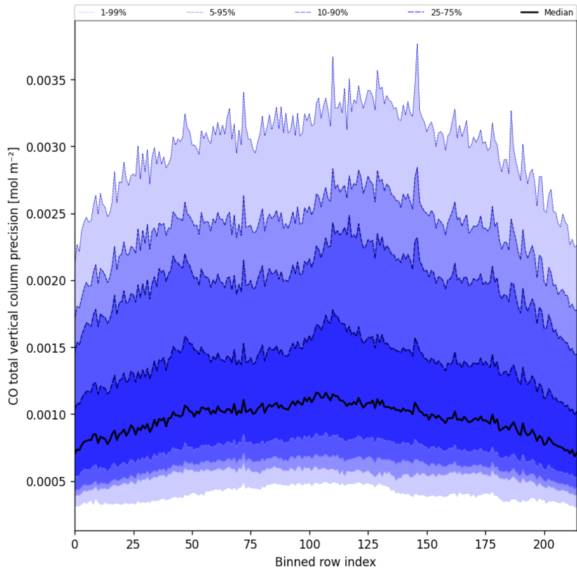
Figure 28: Along track statistics of “CO total vertical column precision” for 2025-06-09 to 2025-06-11
