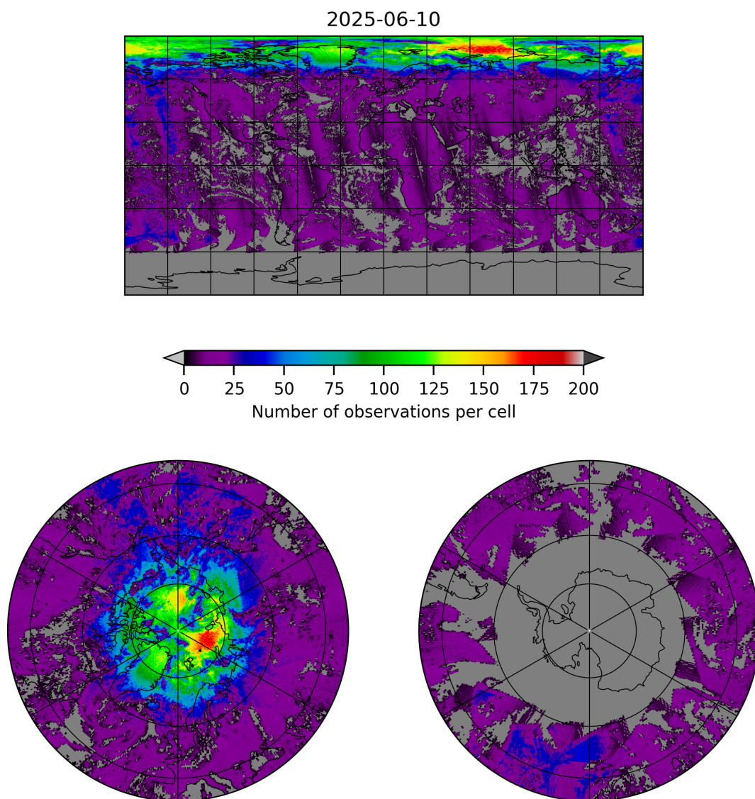
Figure 8: Map of the number of observations for 2025-06-09 to 2025-06-11
