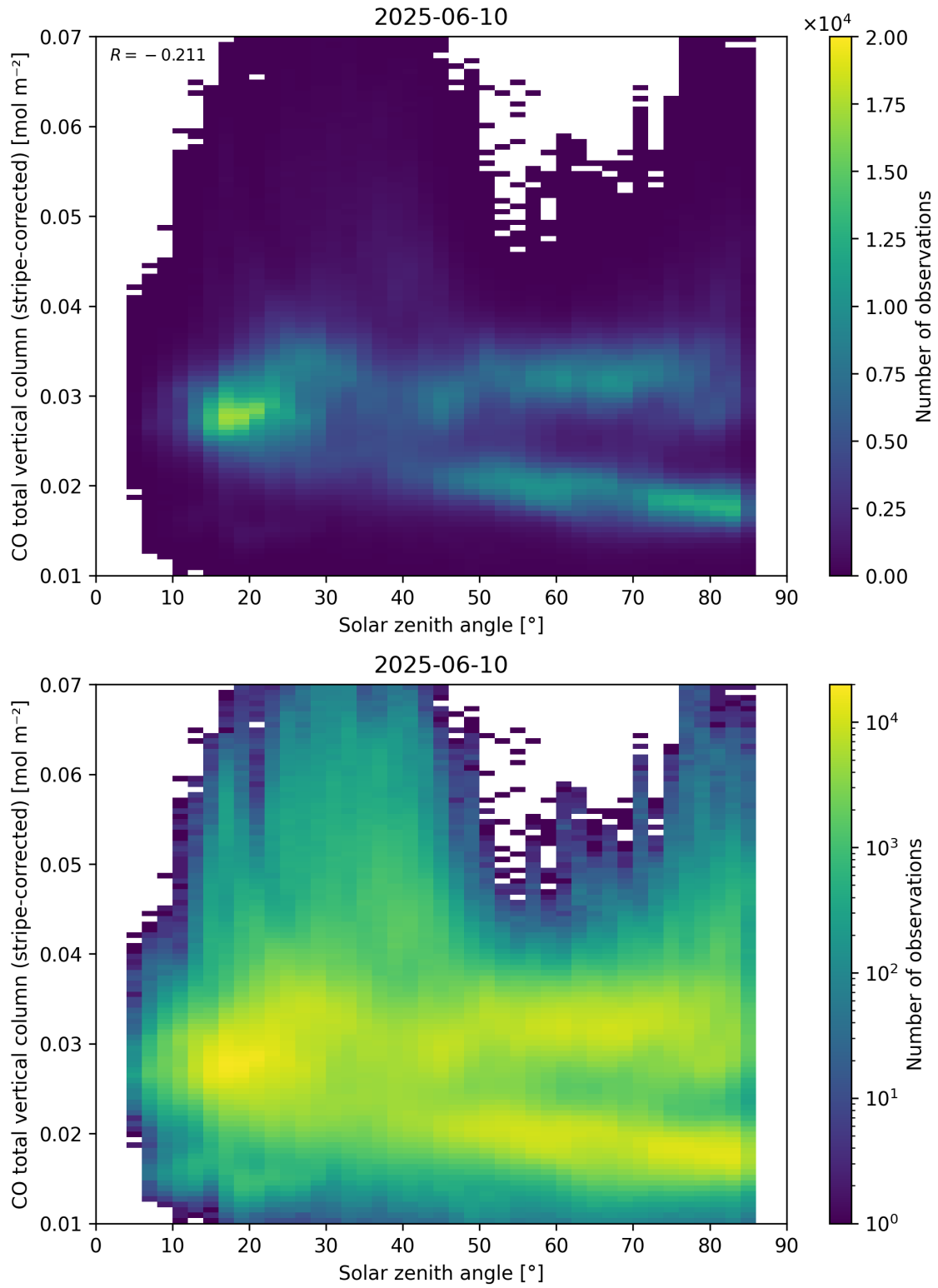
Figure 62: Scatter density plot of “Solar zenith angle” against “CO total vertical column (stripe-corrected)” for 2025-06-09 to 2025-06-11.
