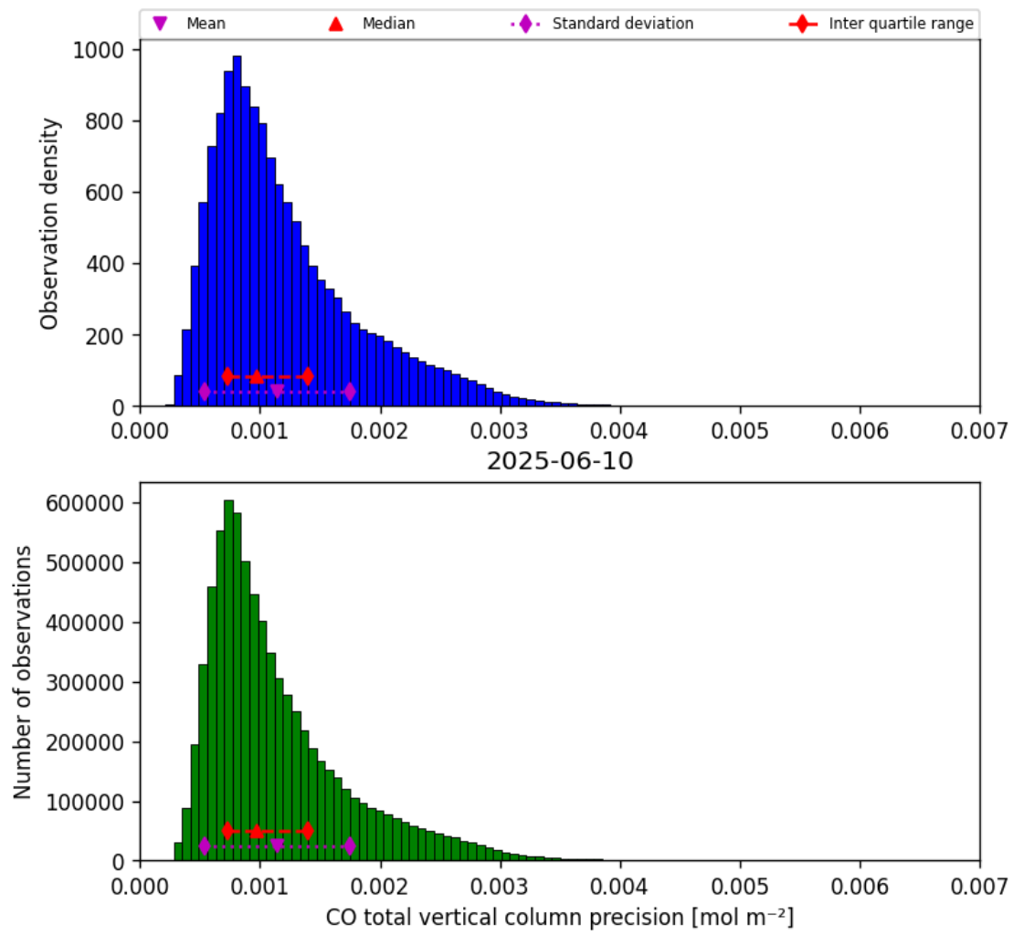
Figure 20: Histogram of “CO total vertical column precision” for 2025-06-09 to 2025-06-11
