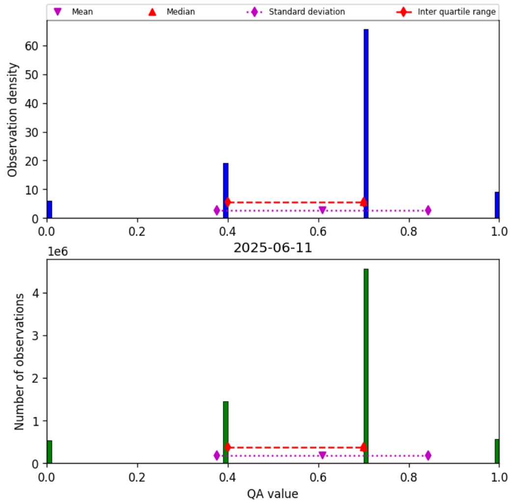
Figure 17: Histogram of “QA value” for 2025-06-11 to 2025-06-12
