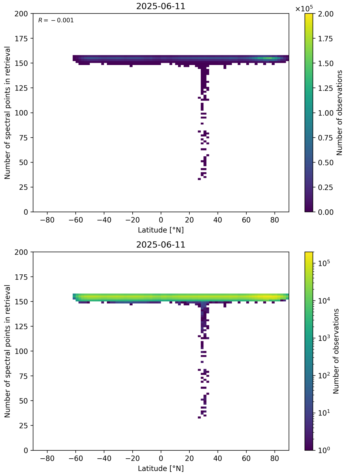
Figure 57: Scatter density plot of “Latitude” against “Number of spectral points in retrieval” for 2025-06-11 to 2025-06-12.
