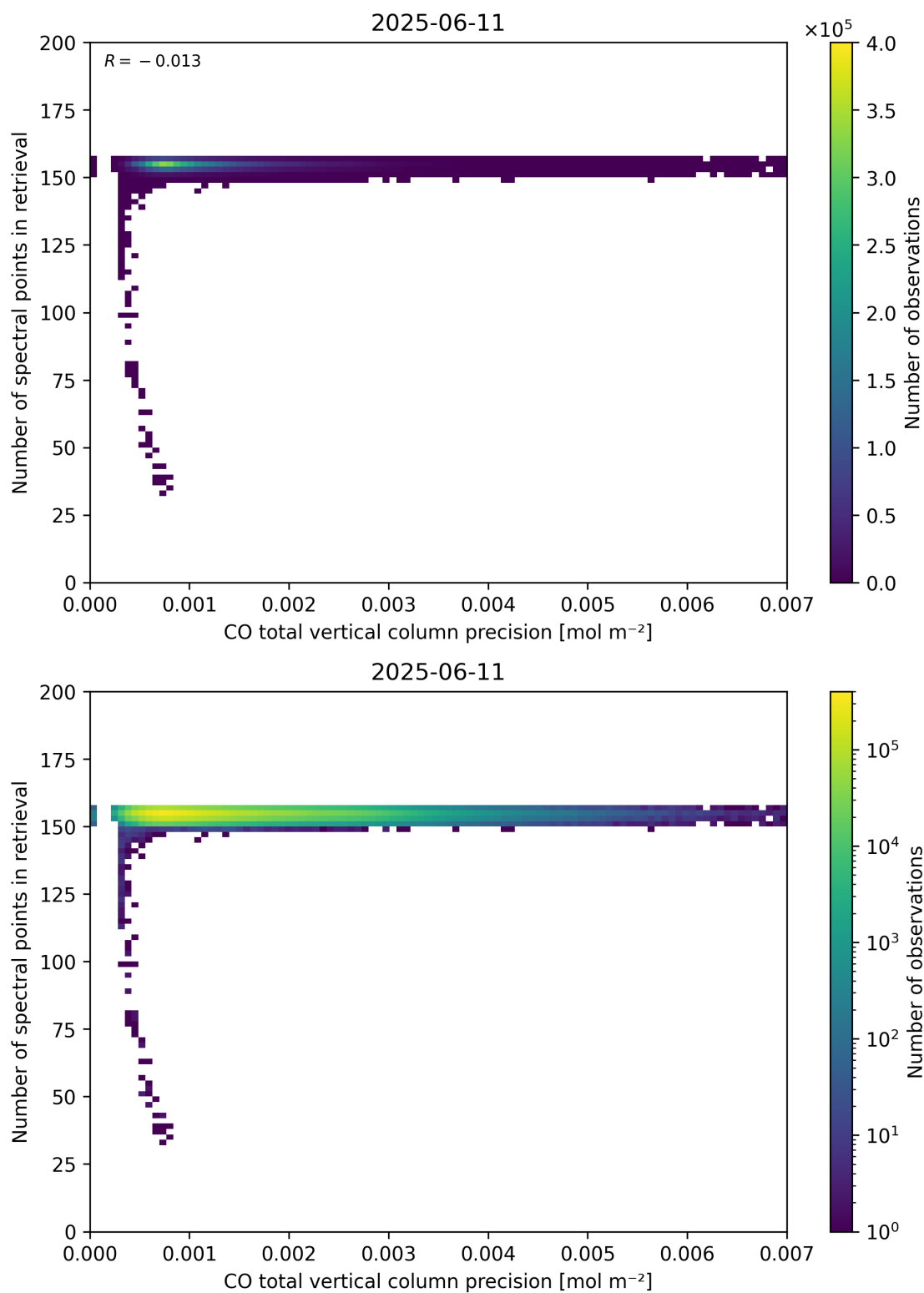
Figure 47: Scatter density plot of “CO total vertical column precision” against “Number of spectral points in retrieval” for 2025-06-11 to 2025-06-12.
