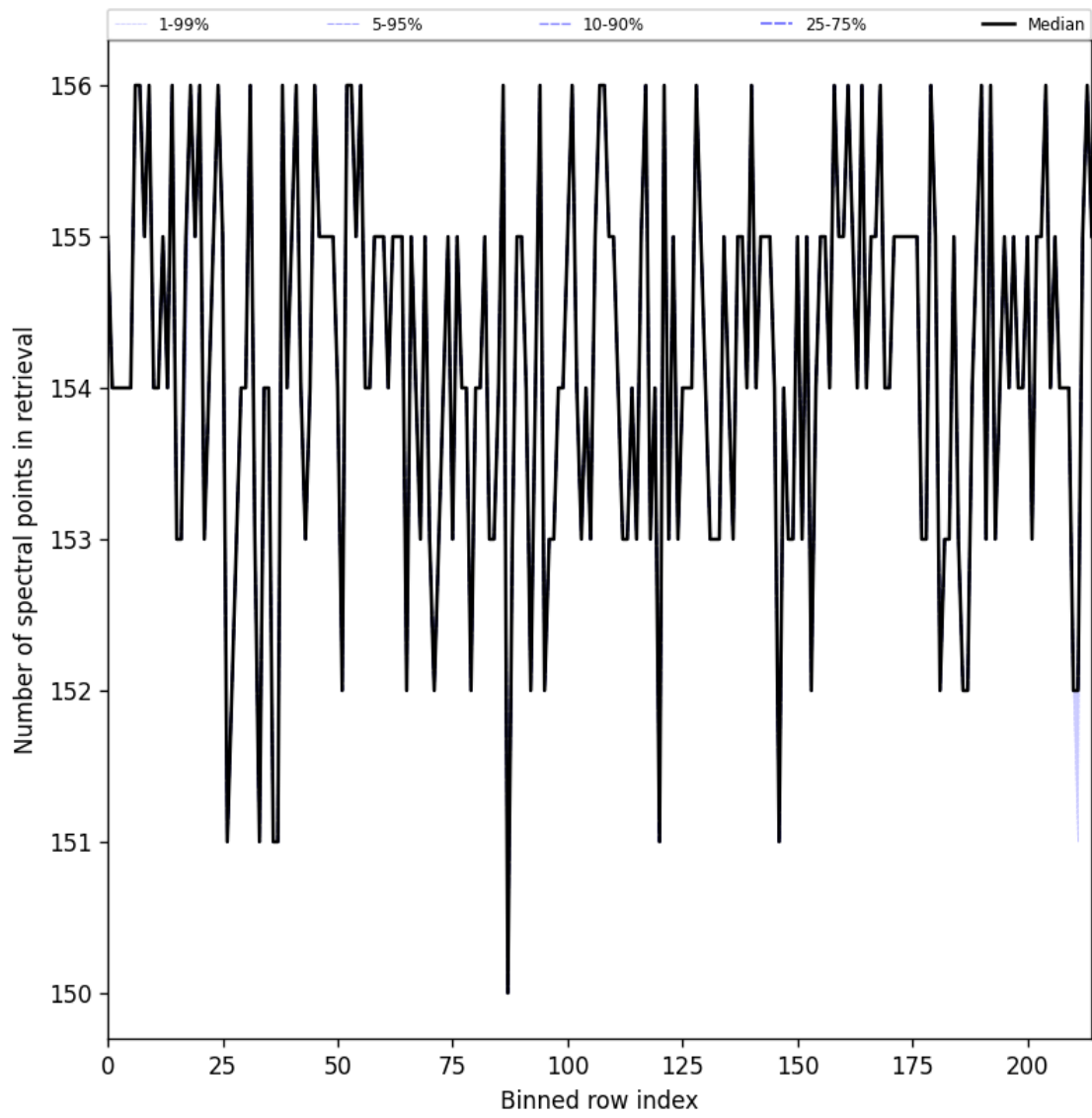
Figure 29: Along track statistics of “Number of spectral points in retrieval” for 2025-06-11 to 2025-06-12
