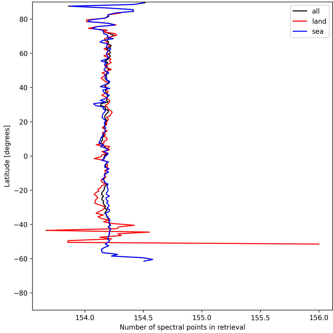
Figure 13: Zonal average of “Number of spectral points in retrieval” for 2025-06-11 to 2025-06-12.
