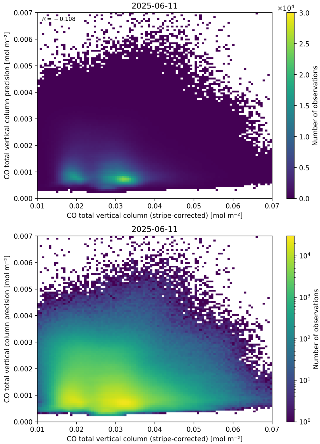
Figure 36: Scatter density plot of “CO total vertical column (stripe-corrected)” against “CO total vertical column precision” for 2025-06-11 to 2025-06-12.
