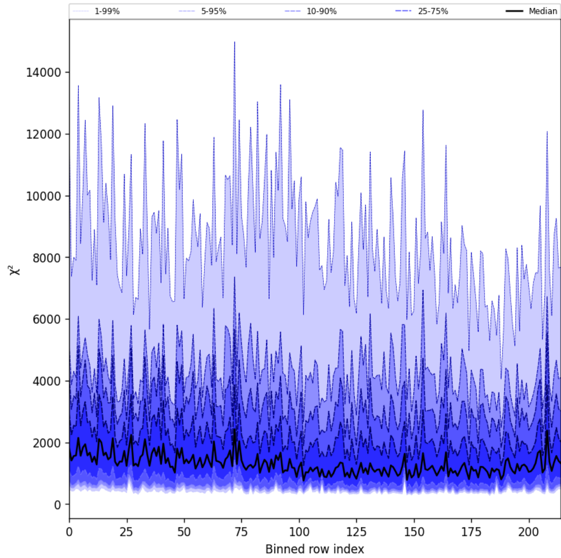
Figure 30: Along track statistics of “ \chi^2 ” for 2025-06-11 to 2025-06-12
