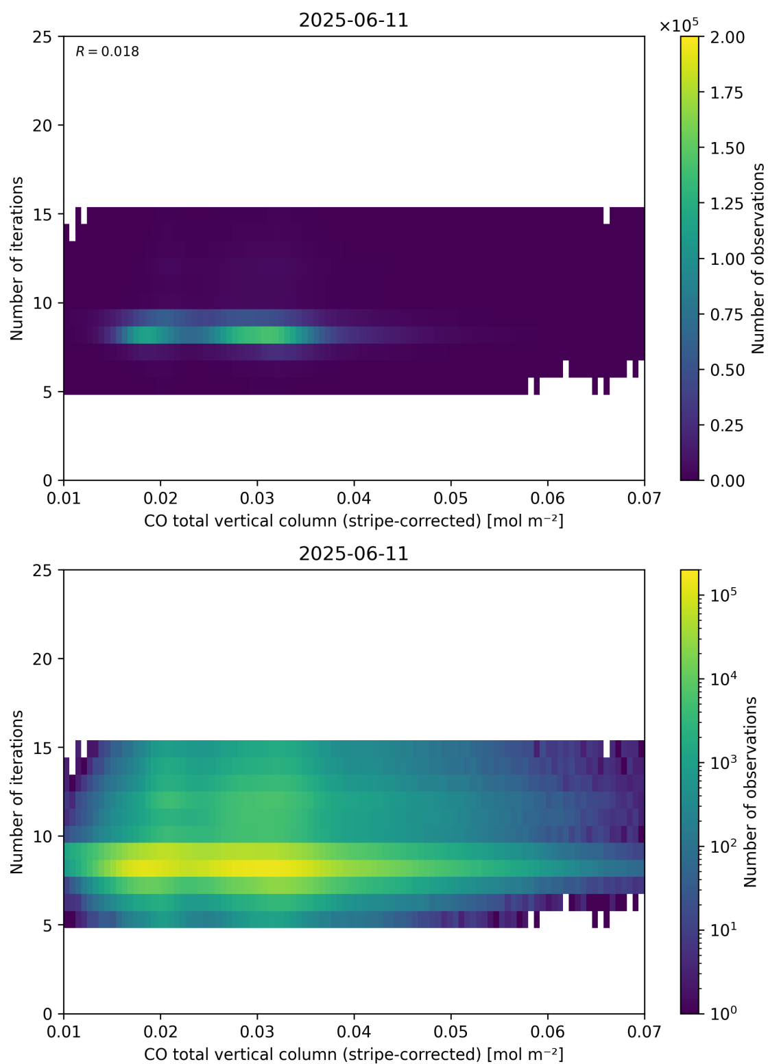
Figure 39: Scatter density plot of “CO total vertical column (stripe-corrected)” against “Number of iterations” for 2025-06-11 to 2025-06-12.
