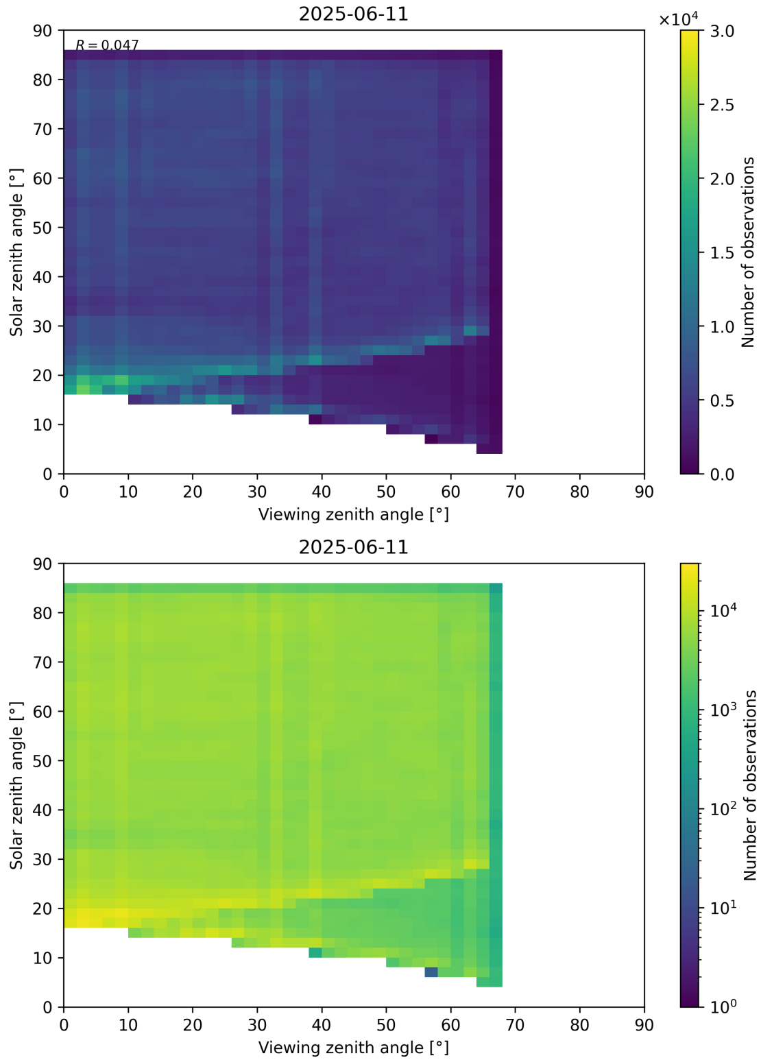
Figure 77: Scatter density plot of “Viewing zenith angle” against “Solar zenith angle” for 2025-06-11 to 2025-06-12.
