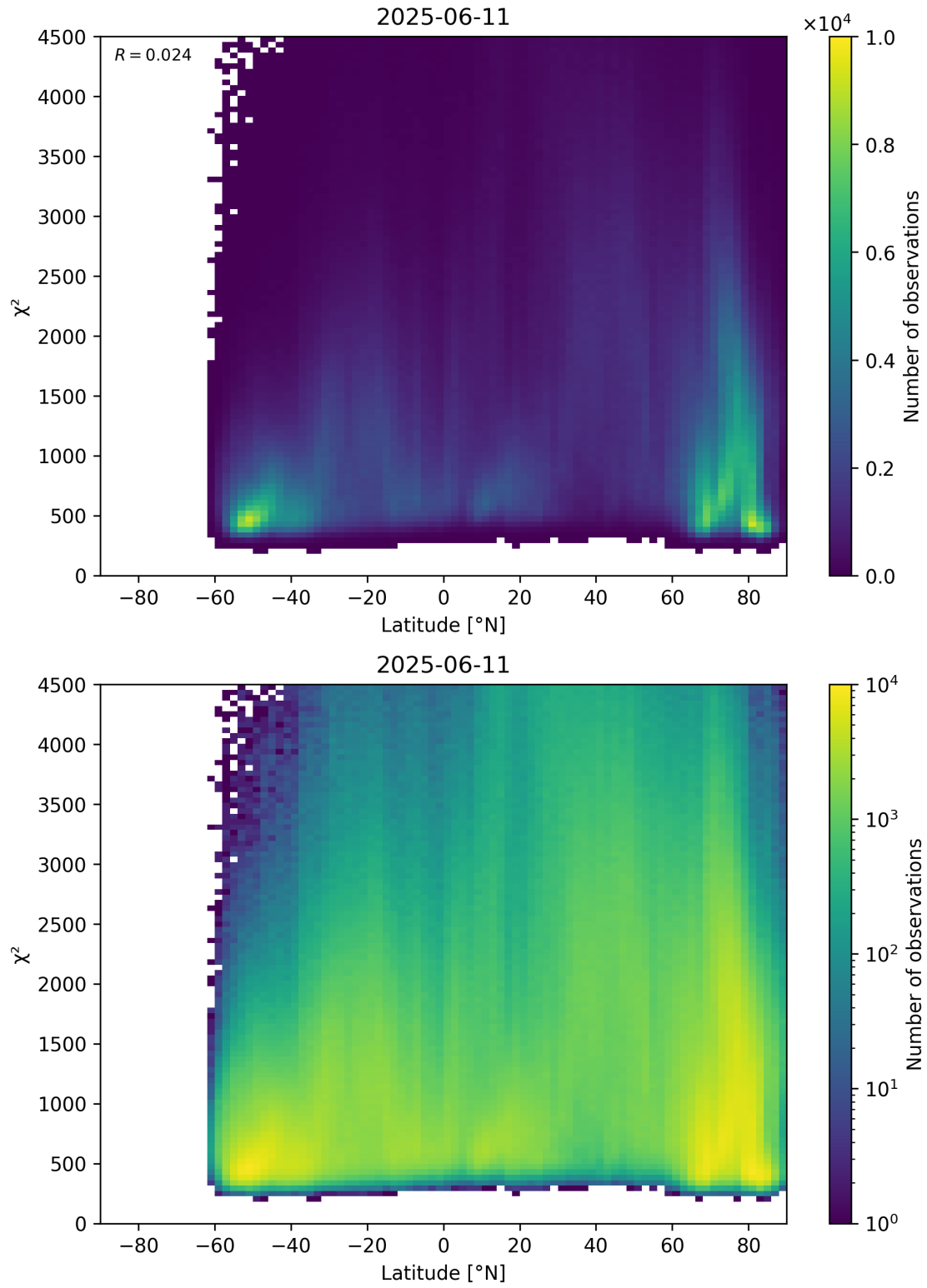
Figure 54: Scatter density plot of “Latitude” against “ \chi^2 ” for 2025-06-11 to 2025-06-12.
