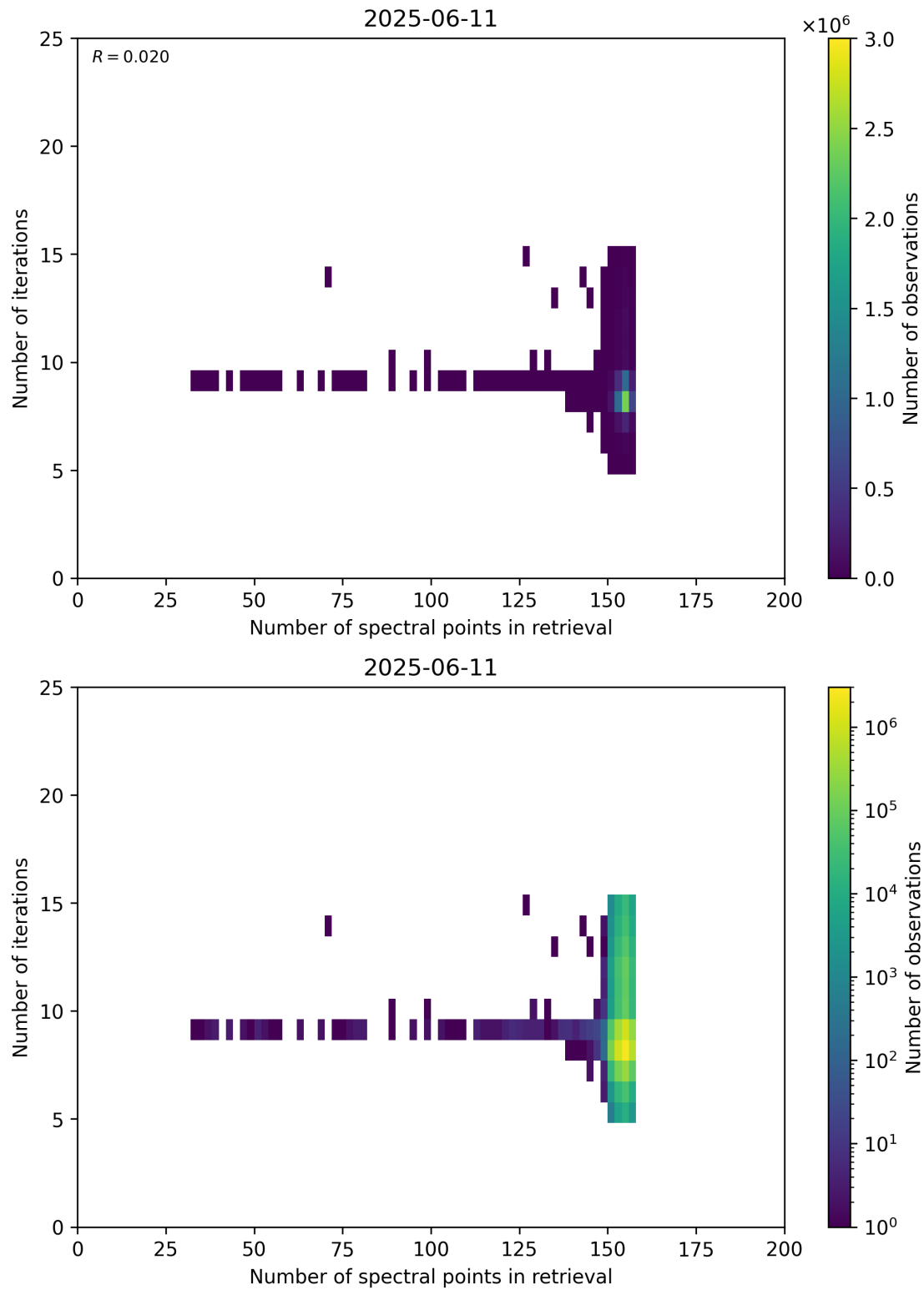
Figure 60: Scatter density plot of “Number of spectral points in retrieval” against “Number of iterations” for 2025-06-11 to 2025-06-12.
