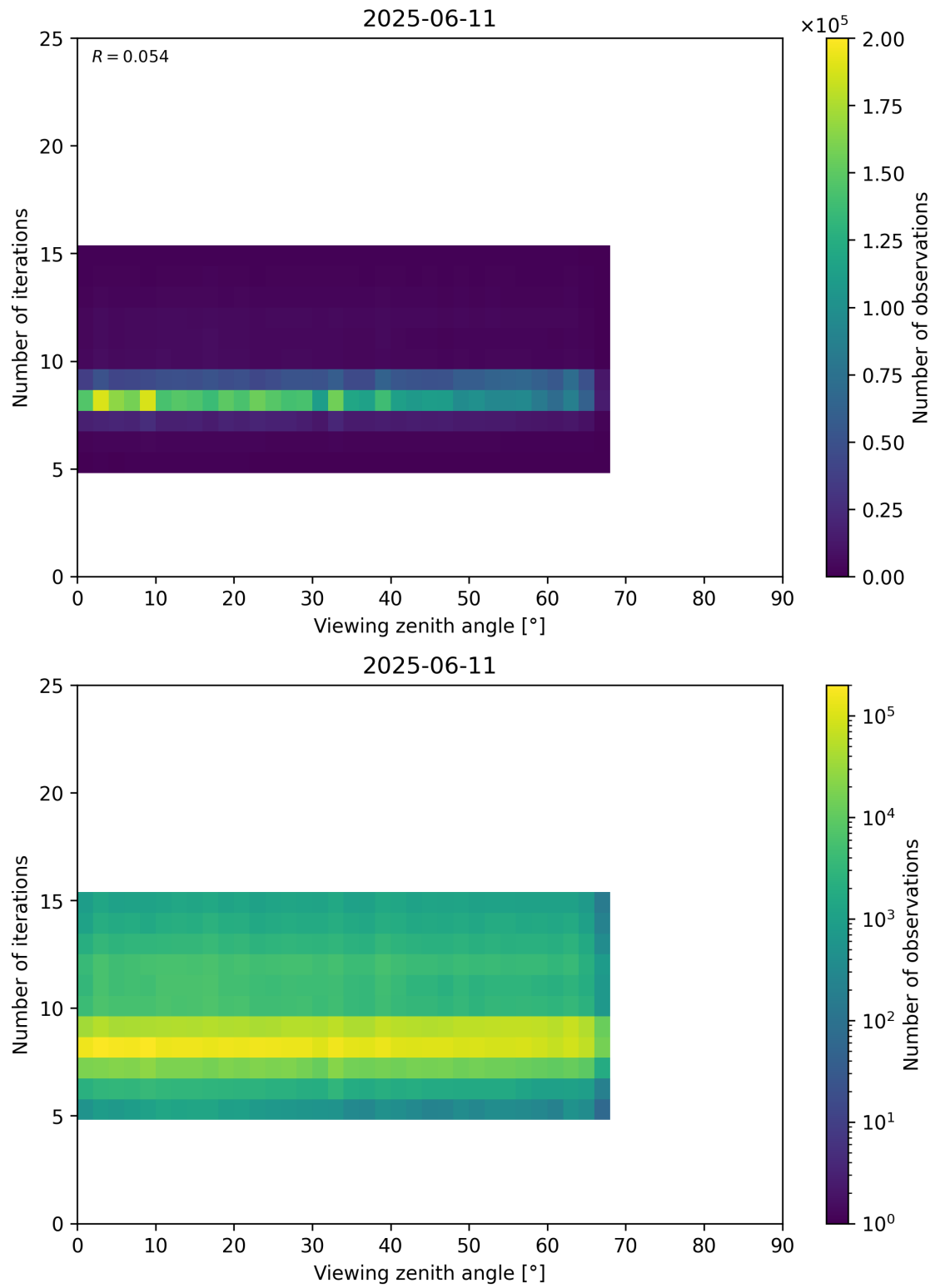
Figure 75: Scatter density plot of “Viewing zenith angle” against “Number of iterations” for 2025-06-11 to 2025-06-12.
