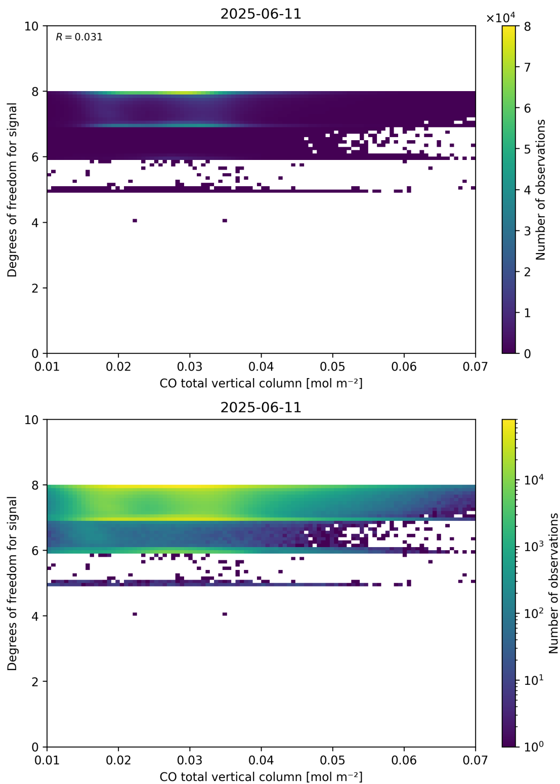
Figure 41: Scatter density plot of “CO total vertical column” against “Degrees of freedom for signal” for 2025-06-11 to 2025-06-12.
