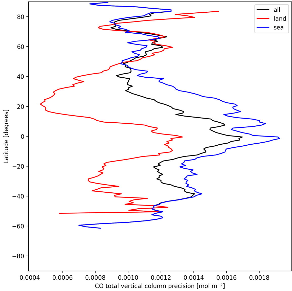
Figure 12: Zonal average of “CO total vertical column precision” for 2025-06-11 to 2025-06-12.
