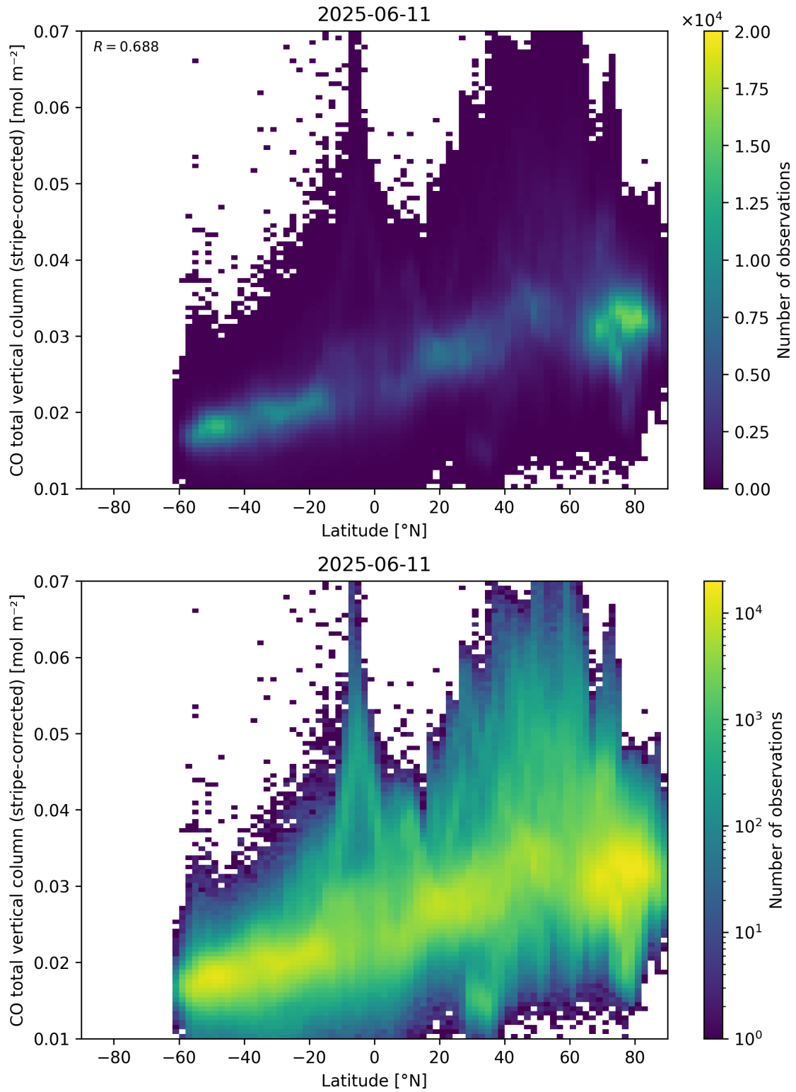
Figure 52: Scatter density plot of “Latitude” against “CO total vertical column (stripe-corrected)” for 2025-06-11 to 2025-06-12.
