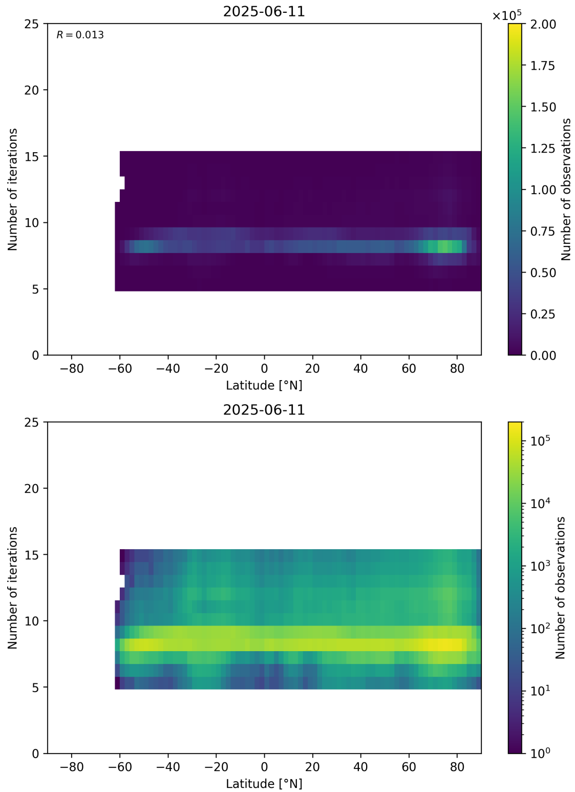
Figure 56: Scatter density plot of “Latitude” against “Number of iterations” for 2025-06-11 to 2025-06-12.
