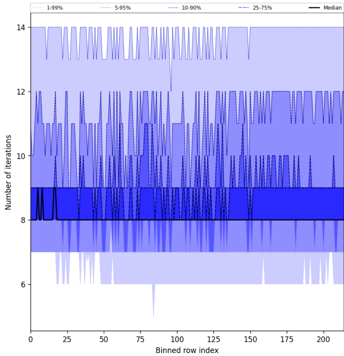
Figure 32: Along track statistics of “Number of iterations” for 2025-06-11 to 2025-06-12
