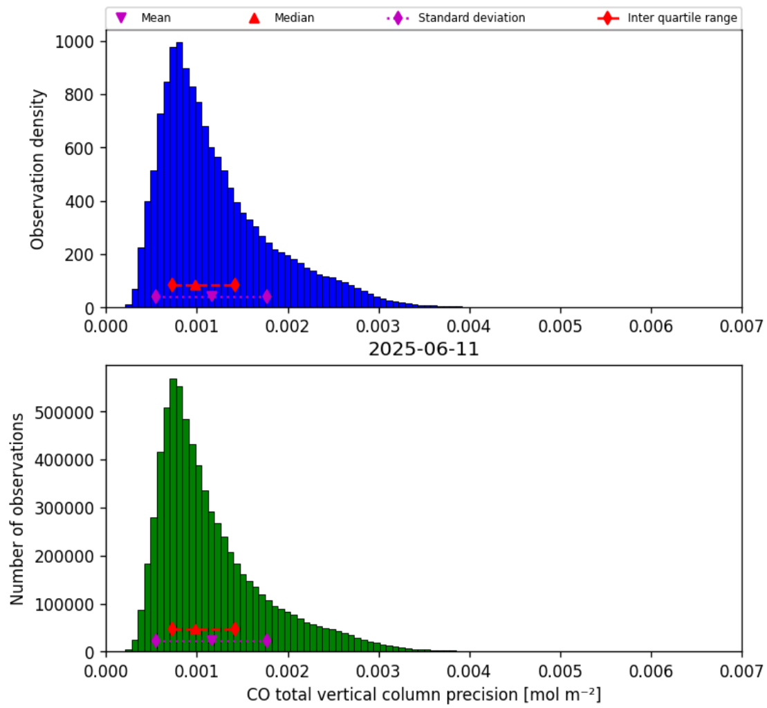
Figure 20: Histogram of “CO total vertical column precision” for 2025-06-11 to 2025-06-12
