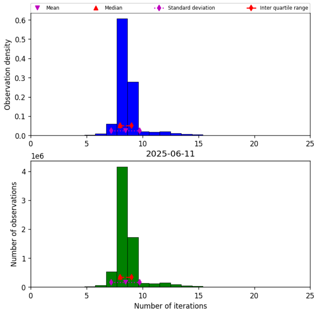
Figure 24: Histogram of “Number of iterations” for 2025-06-11 to 2025-06-12
