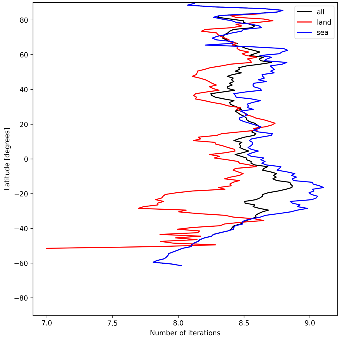
Figure 16: Zonal average of “Number of iterations” for 2025-06-11 to 2025-06-12.
