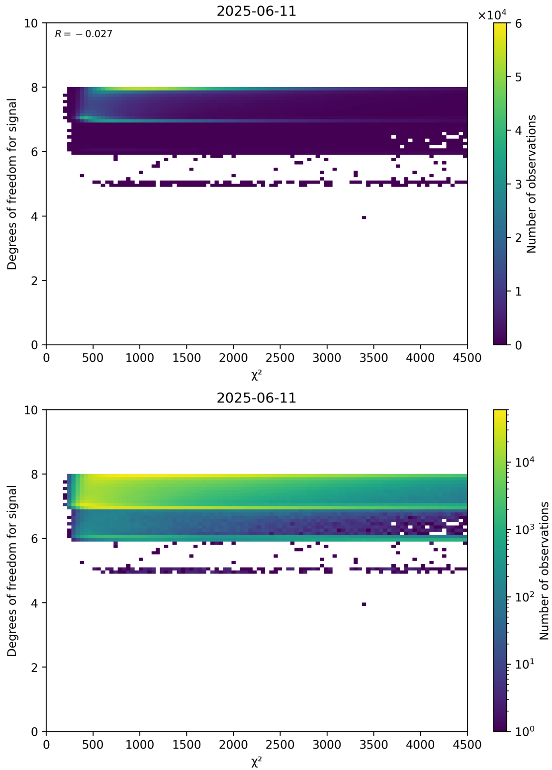
Figure 48: Scatter density plot of “ \chi^2 ” against “Degrees of freedom for signal” for 2025-06-11 to 2025-06-12.
