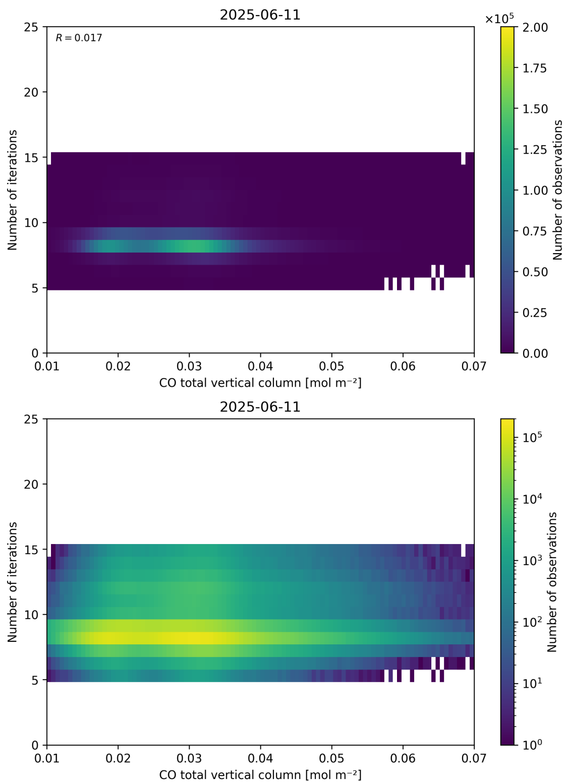
Figure 42: Scatter density plot of “CO total vertical column” against “Number of iterations” for 2025-06-11 to 2025-06-12.
