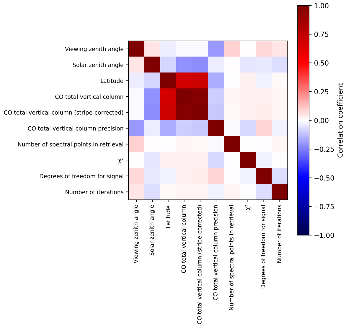
Figure 2: Map of correlation matrix for 2025-06-11 to 2025-06-12.
