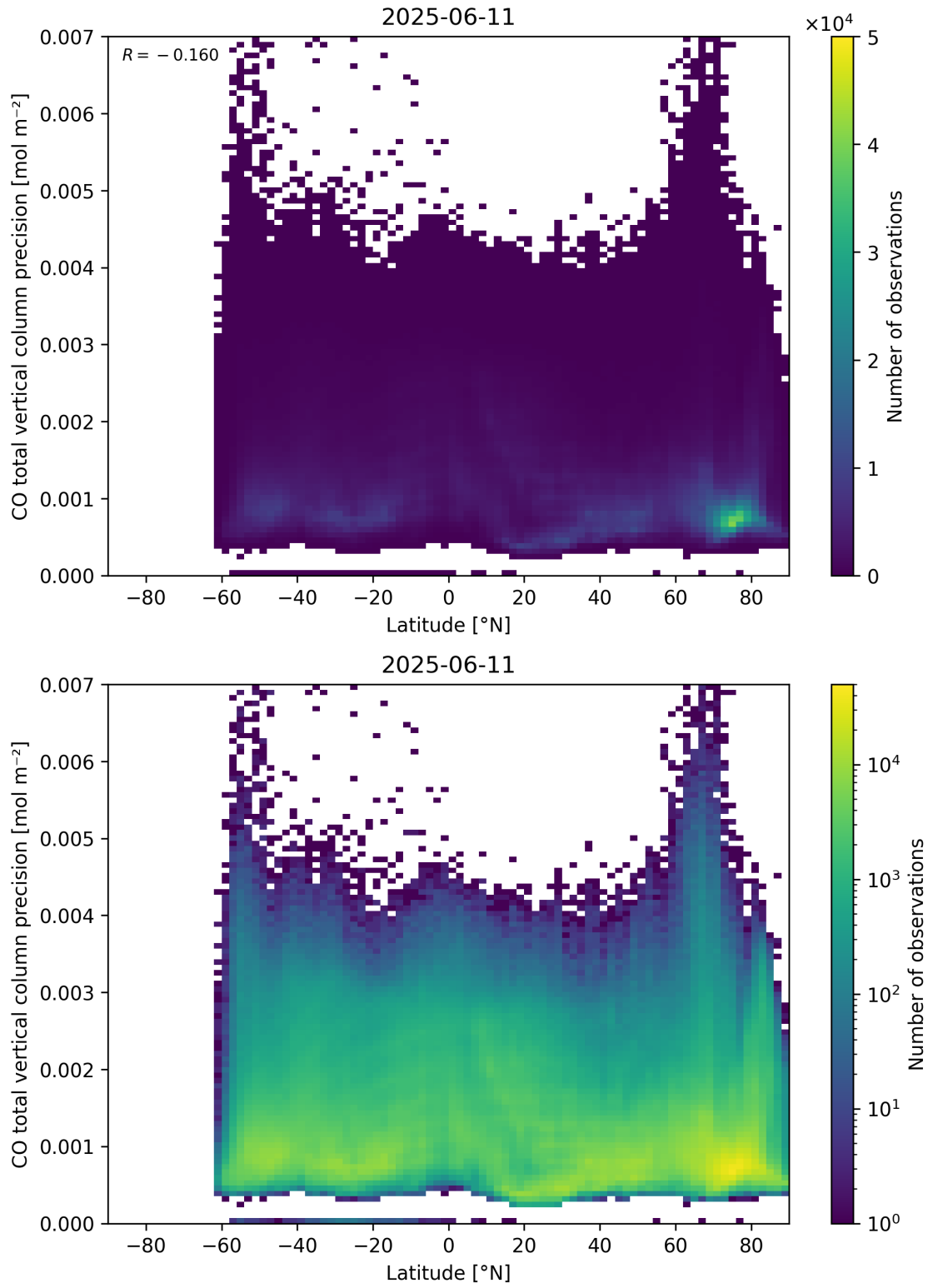
Figure 53: Scatter density plot of “Latitude” against “CO total vertical column precision” for 2025-06-11 to 2025-06-12.
