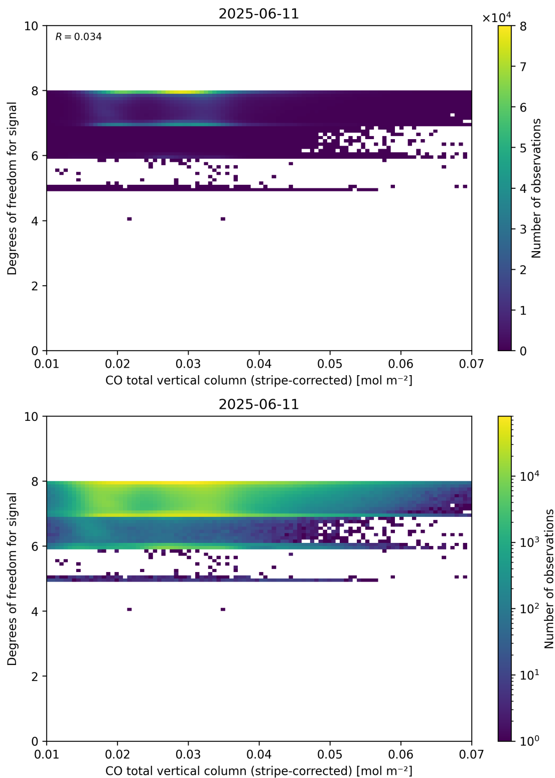
Figure 38: Scatter density plot of “CO total vertical column (stripe-corrected)” against “Degrees of freedom for signal” for 2025-06-11 to 2025-06-12.
