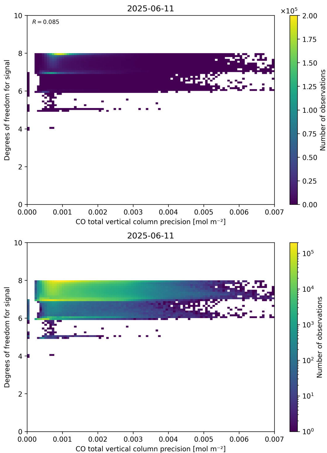
Figure 45: Scatter density plot of “CO total vertical column precision” against “Degrees of freedom for signal” for 2025-06-11 to 2025-06-12.
