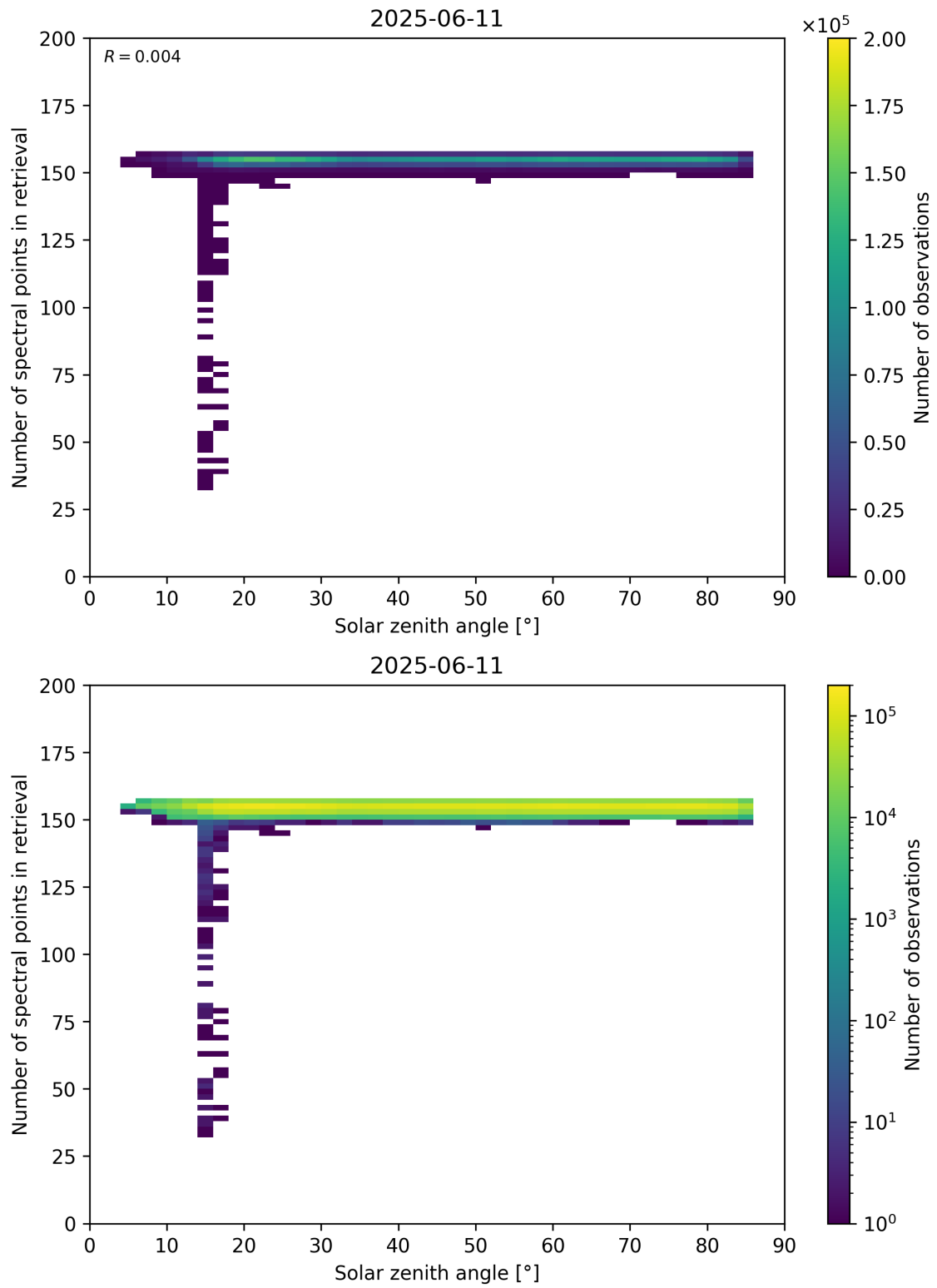
Figure 68: Scatter density plot of “Solar zenith angle” against “Number of spectral points in retrieval” for 2025-06-11 to 2025-06-12.
