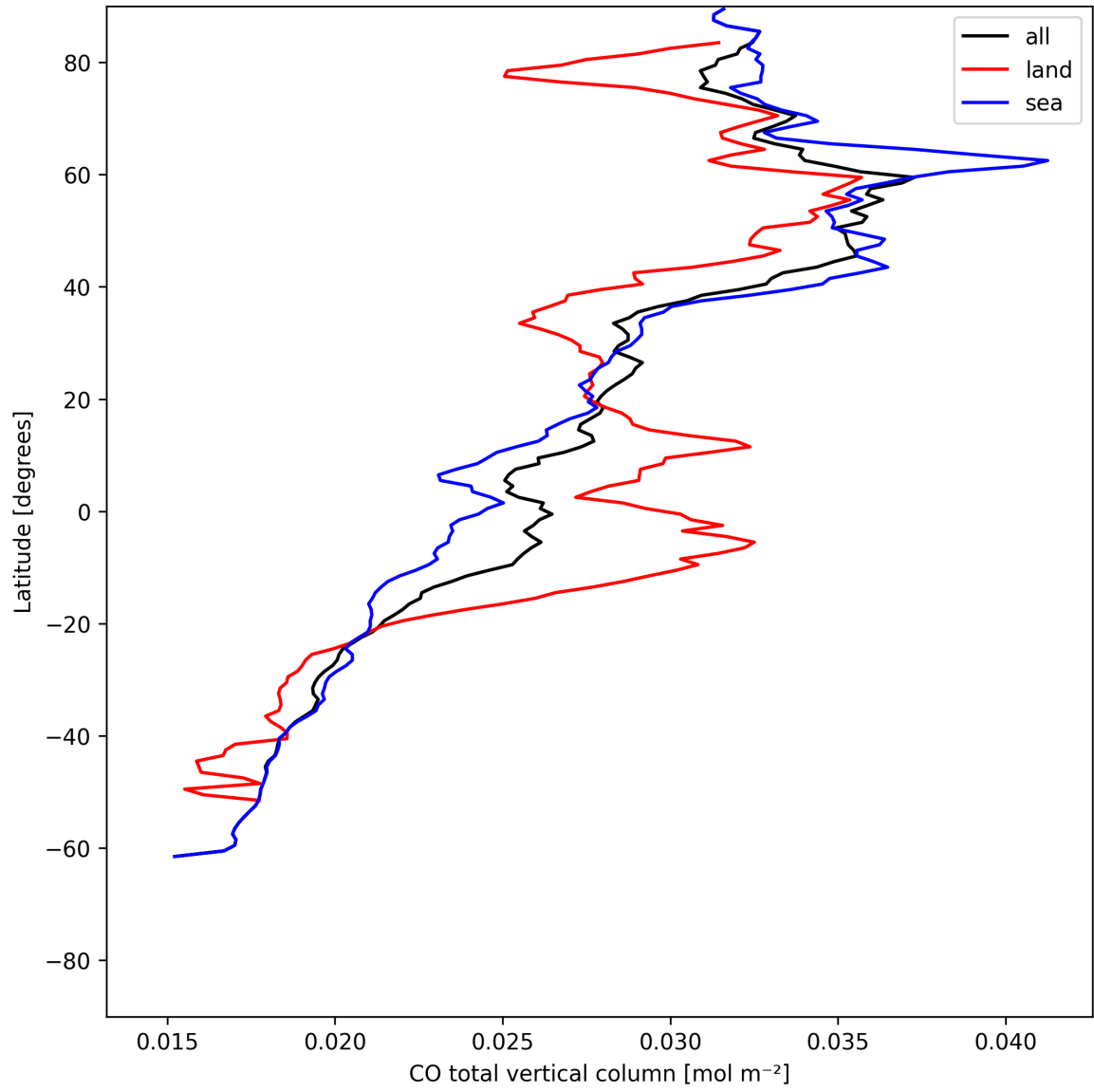
Figure 10: Zonal average of “CO total vertical column” for 2025-06-11 to 2025-06-12.
