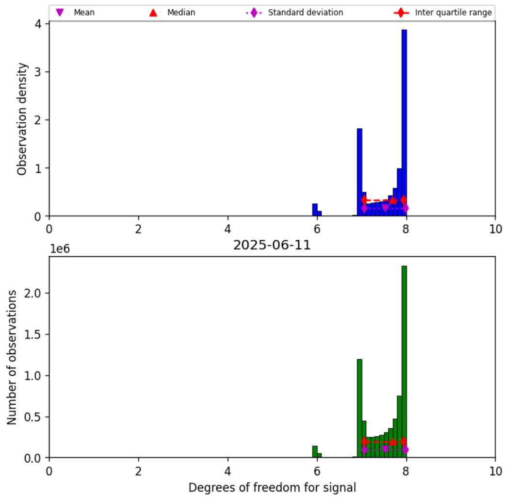
Figure 23: Histogram of “Degrees of freedom for signal” for 2025-06-11 to 2025-06-12
