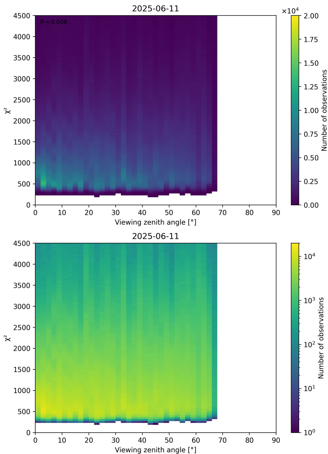
Figure 72: Scatter density plot of “Viewing zenith angle” against “ \chi^2 ” for 2025-06-11 to 2025-06-12.
