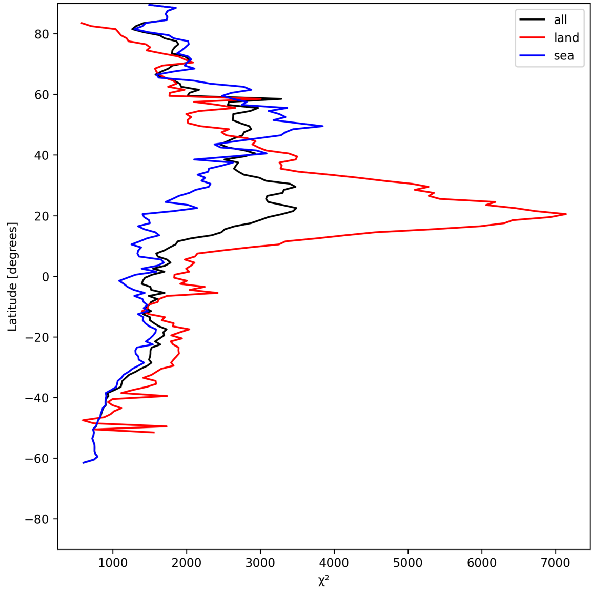
Figure 14: Zonal average of “ \chi^2 ” for 2025-06-11 to 2025-06-12.
