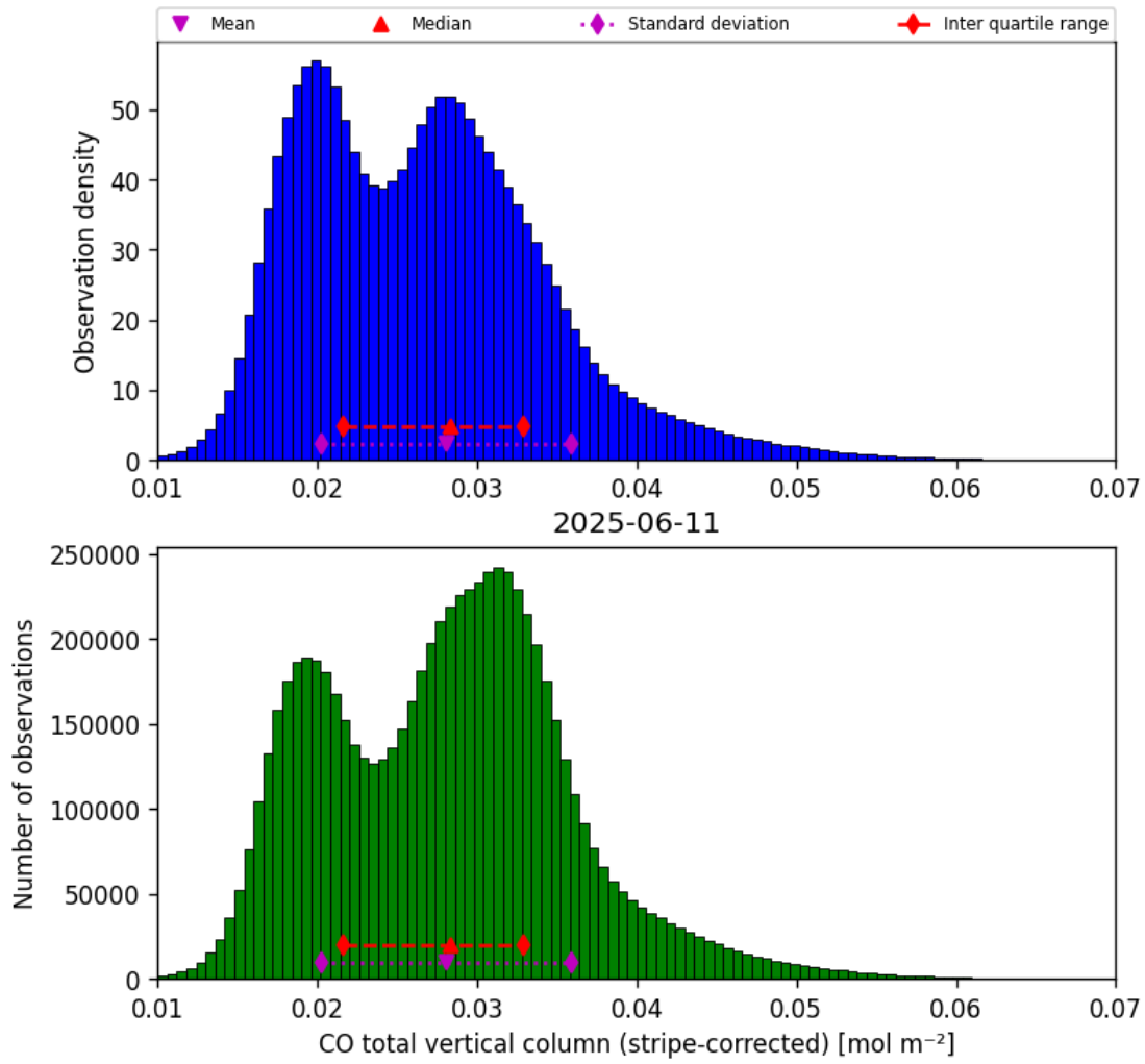
Figure 19: Histogram of “CO total vertical column (stripe-corrected)” for 2025-06-11 to 2025-06-12
