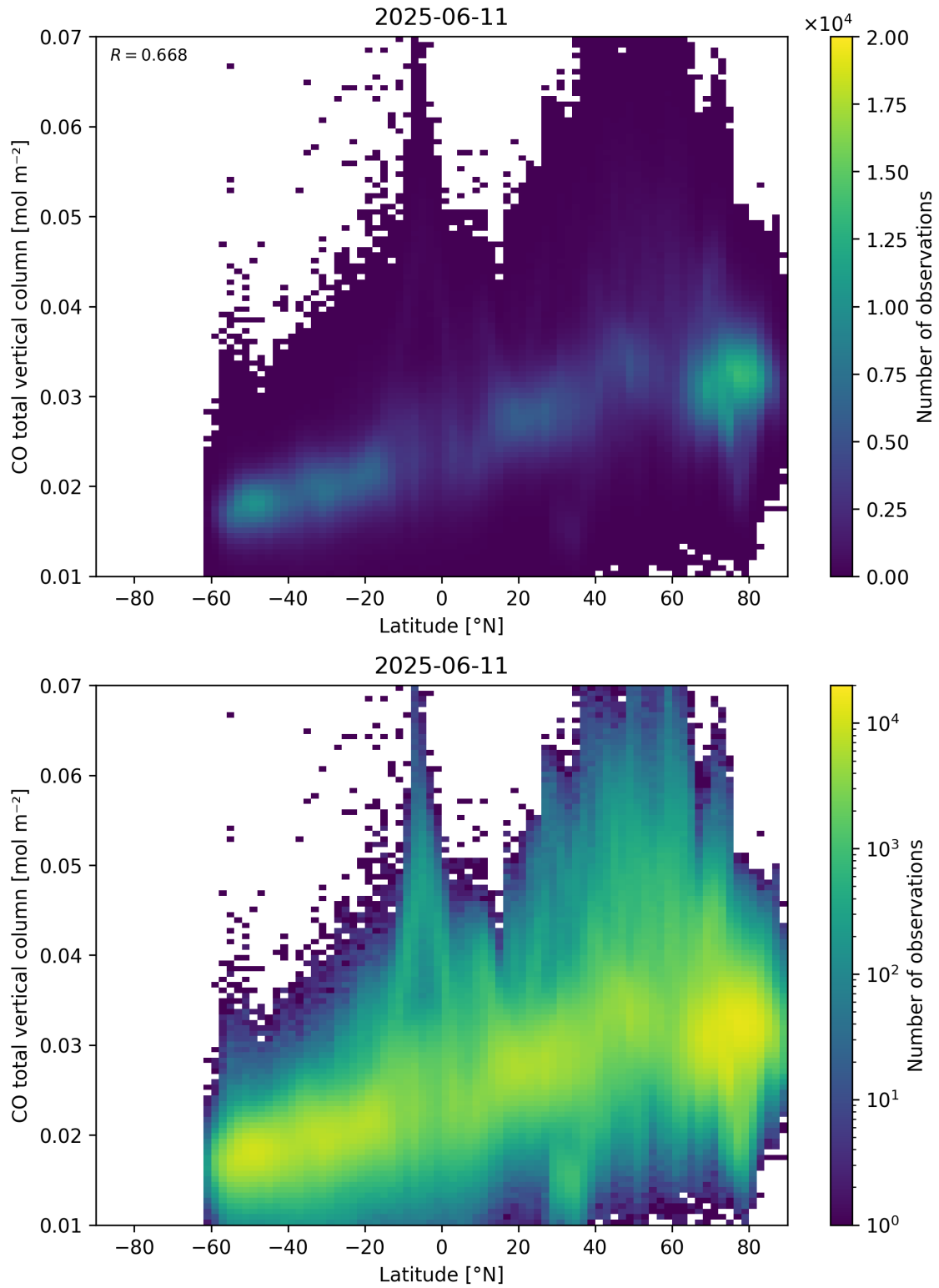
Figure 51: Scatter density plot of “Latitude” against “CO total vertical column” for 2025-06-11 to 2025-06-12.
