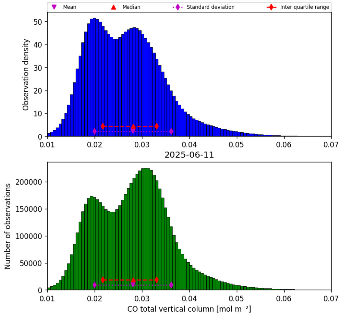
Figure 18: Histogram of “CO total vertical column” for 2025-06-11 to 2025-06-12
