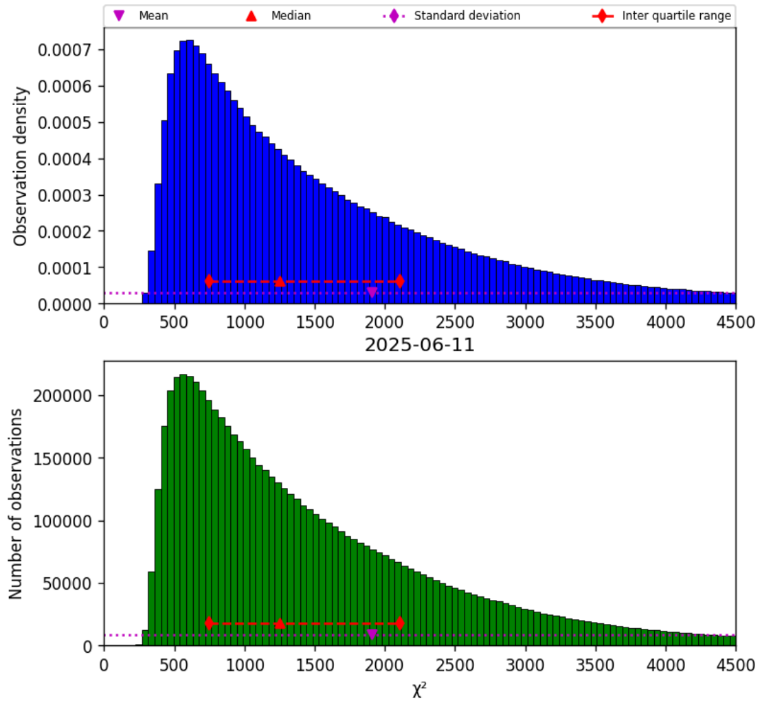
Figure 22: Histogram of “ \chi^2 ” for 2025-06-11 to 2025-06-12
