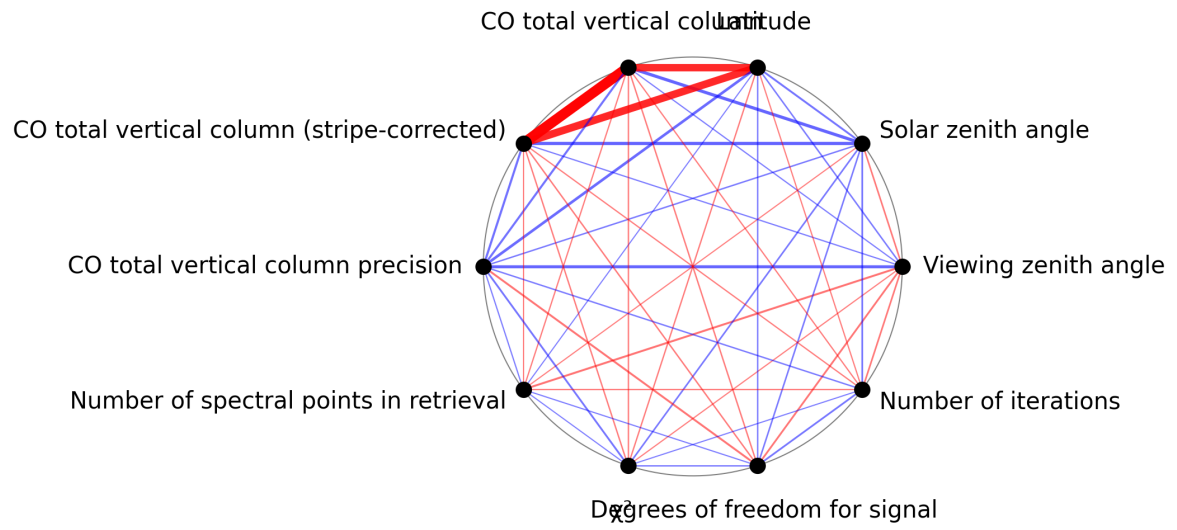
Figure 1: Map of correlation graph for 2025-06-11 to 2025-06-12.
