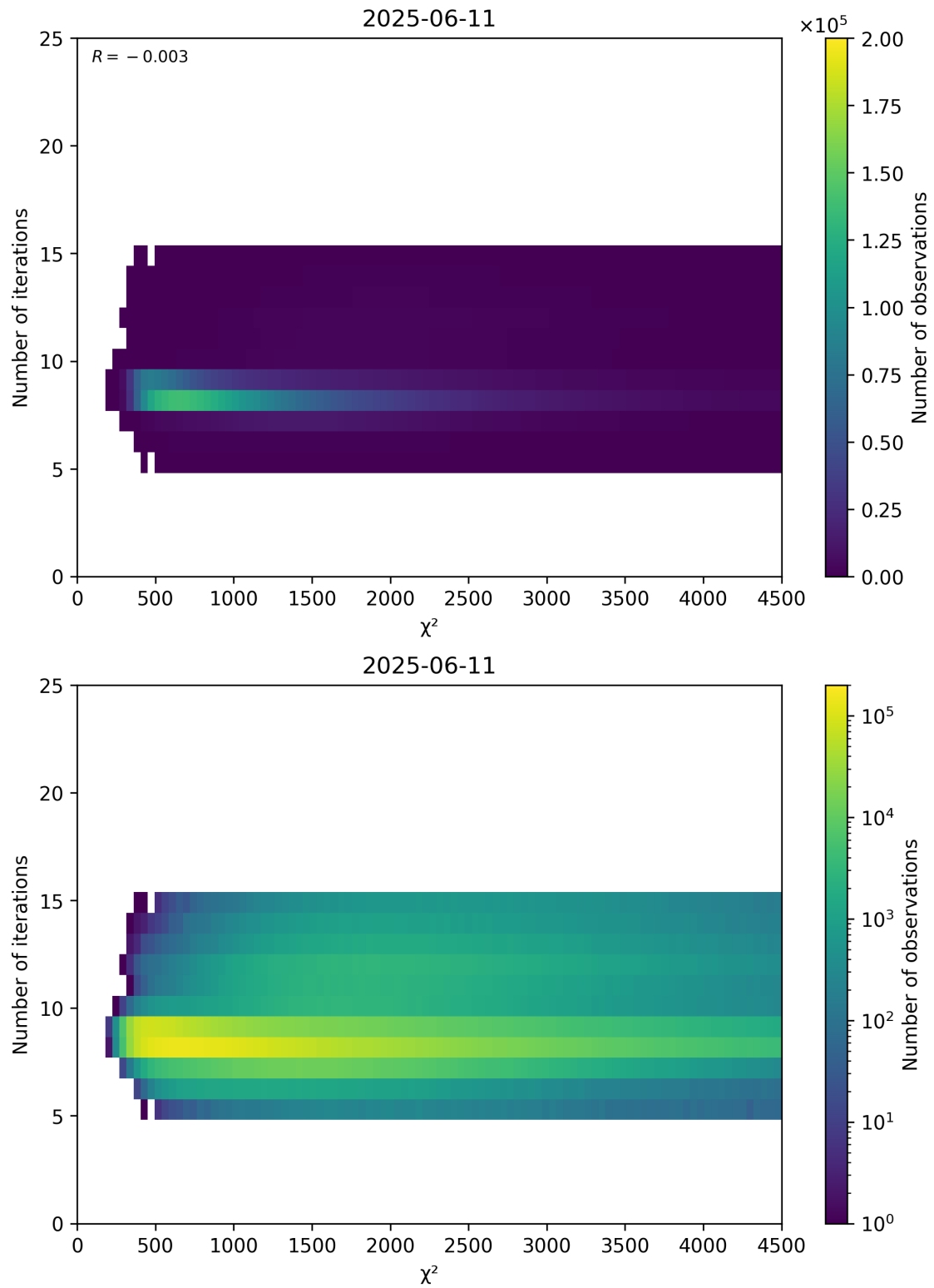
Figure 49: Scatter density plot of “ \chi^2 ” against “Number of iterations” for 2025-06-11 to 2025-06-12.
