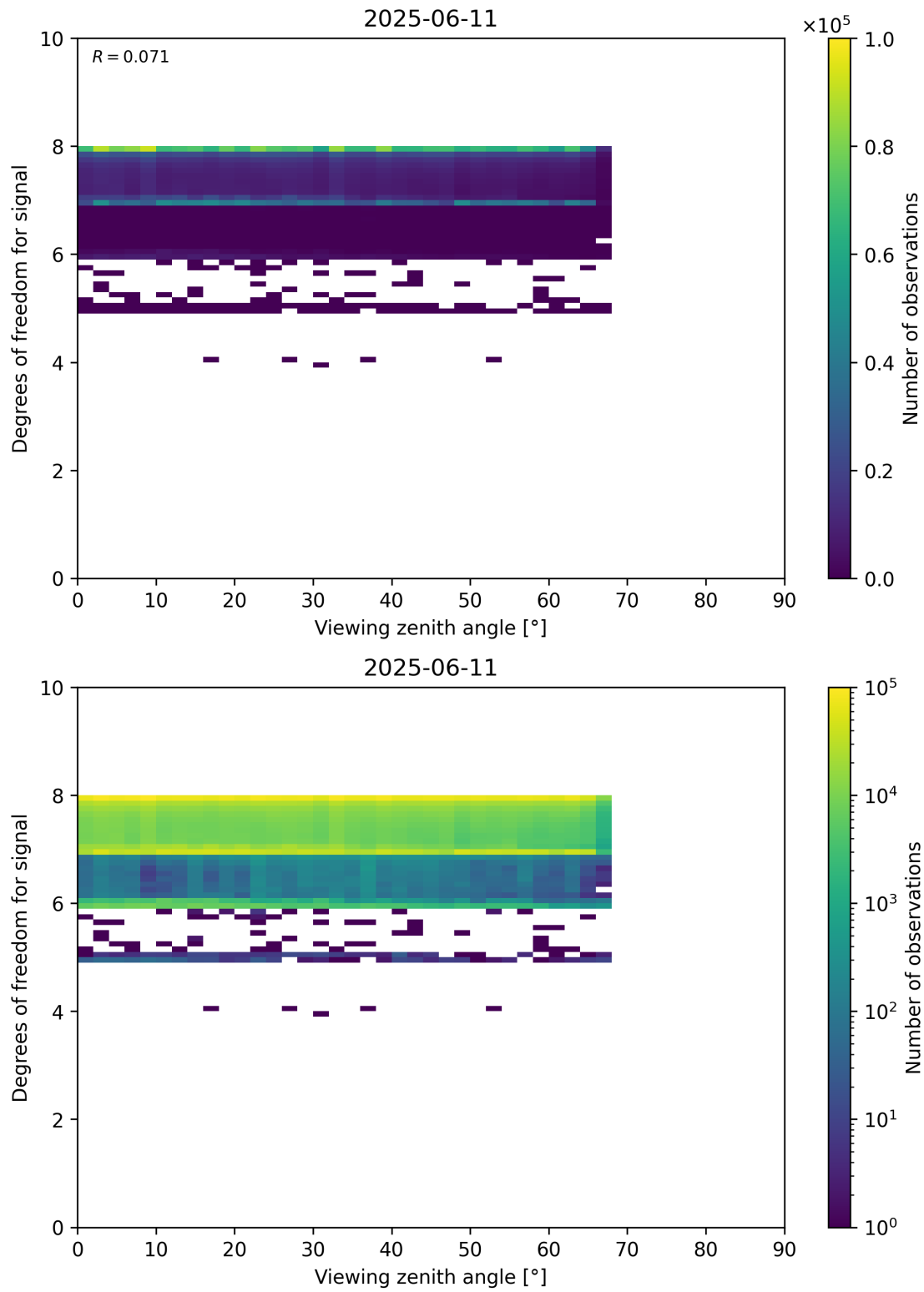
Figure 73: Scatter density plot of “Viewing zenith angle” against “Degrees of freedom for signal” for 2025-06-11 to 2025-06-12.
