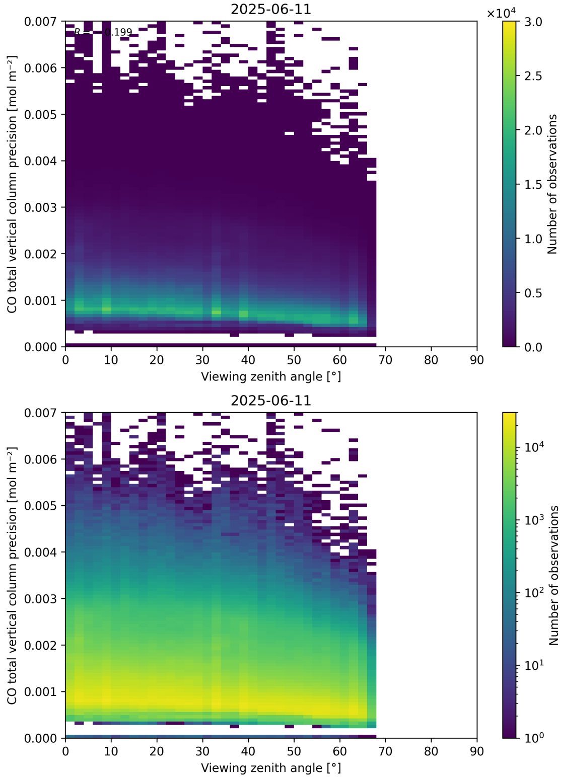
Figure 71: Scatter density plot of “Viewing zenith angle” against “CO total vertical column precision” for 2025-06-11 to 2025-06-12.
