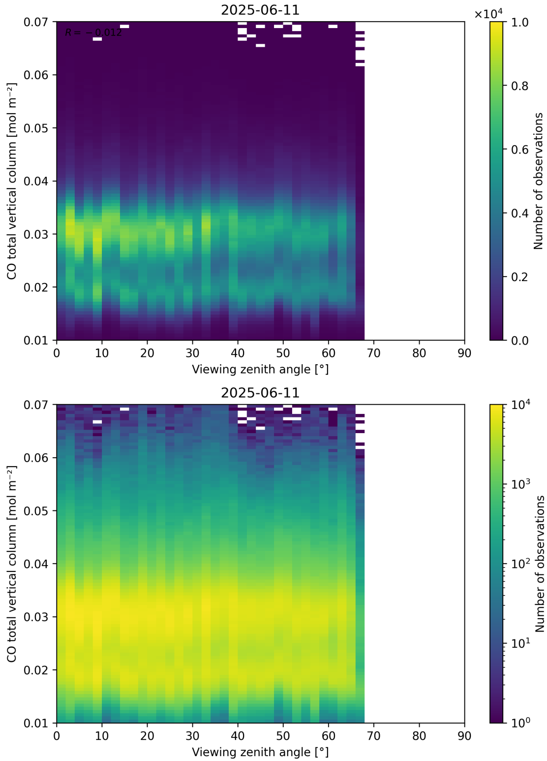
Figure 69: Scatter density plot of “Viewing zenith angle” against “CO total vertical column” for 2025-06-11 to 2025-06-12.
