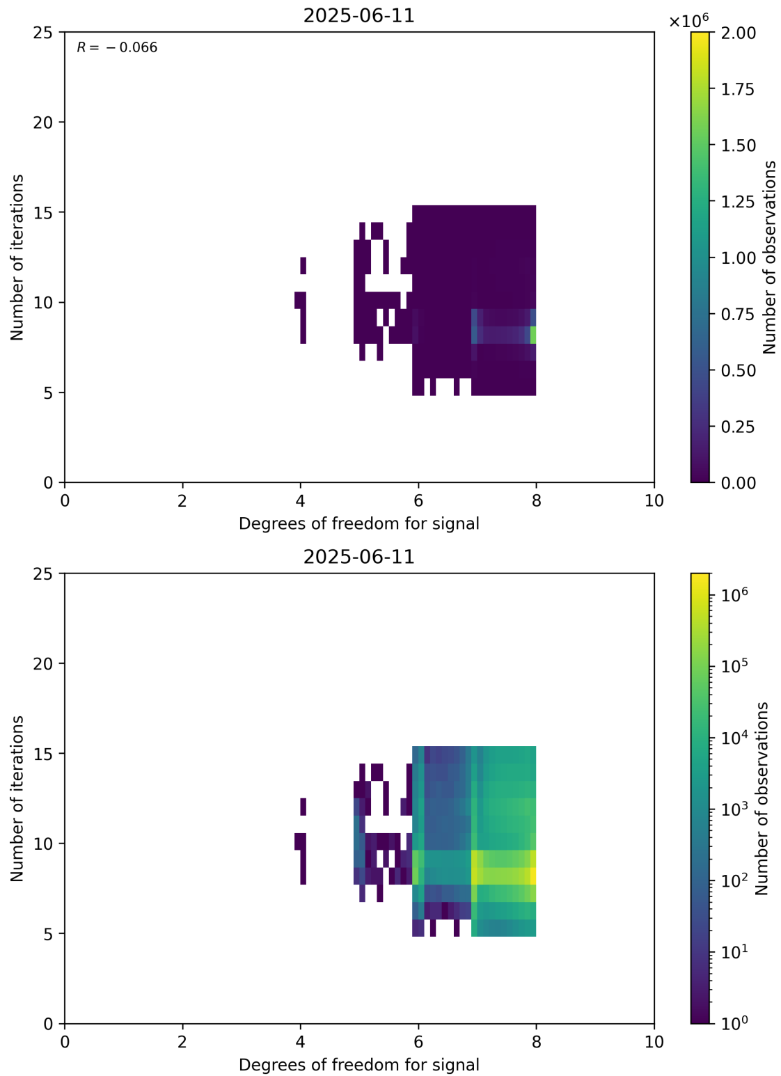
Figure 50: Scatter density plot of “Degrees of freedom for signal” against “Number of iterations” for 2025-06-11 to 2025-06-12.
