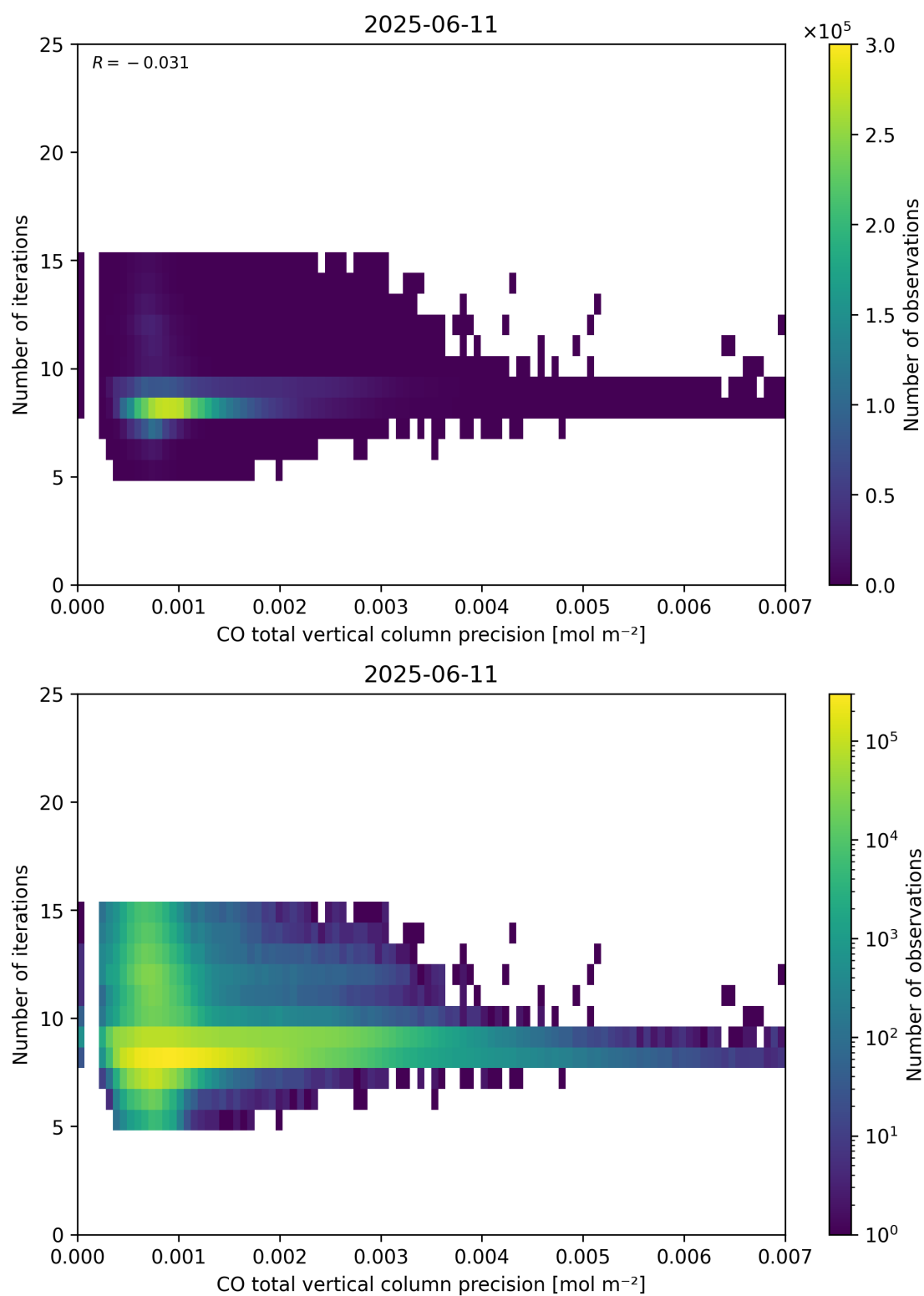
Figure 46: Scatter density plot of “CO total vertical column precision” against “Number of iterations” for 2025-06-11 to 2025-06-12.
