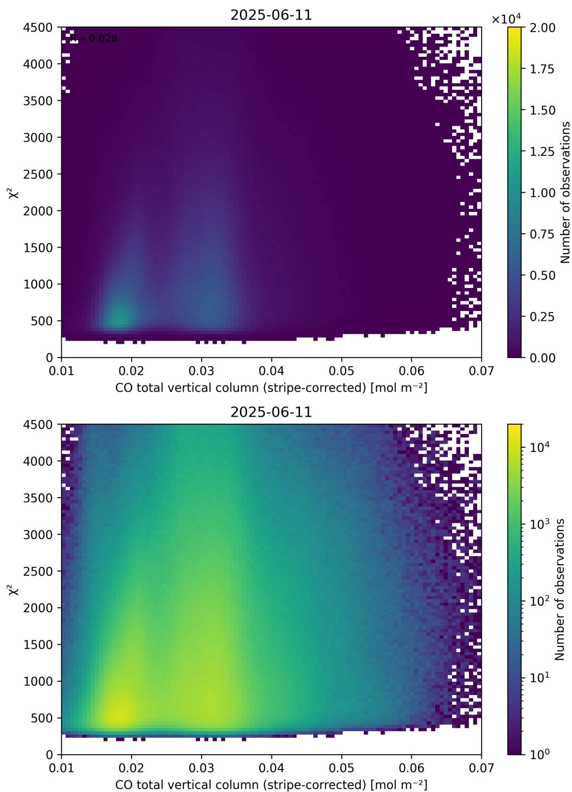
Figure 37: Scatter density plot of “CO total vertical column (stripe-corrected)” against “ \chi^2 ” for 2025-06-11 to 2025-06-12.
