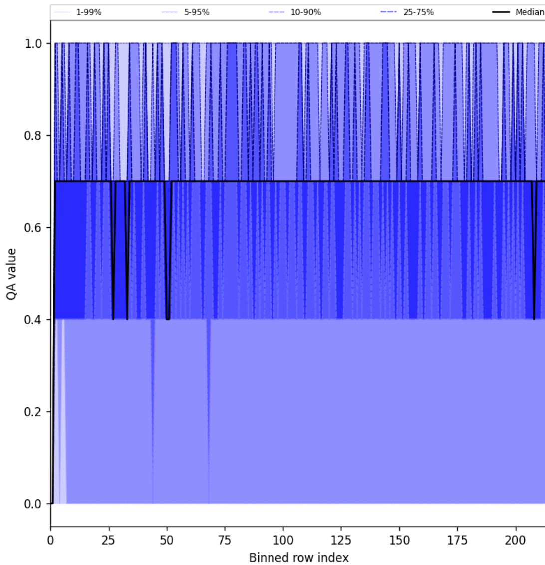
Figure 25: Along track statistics of “QA value” for 2025-06-11 to 2025-06-12
