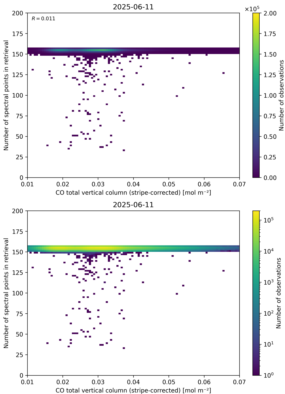
Figure 40: Scatter density plot of “CO total vertical column (stripe-corrected)” against “Number of spectral points in retrieval” for 2025-06-11 to 2025-06-12.
