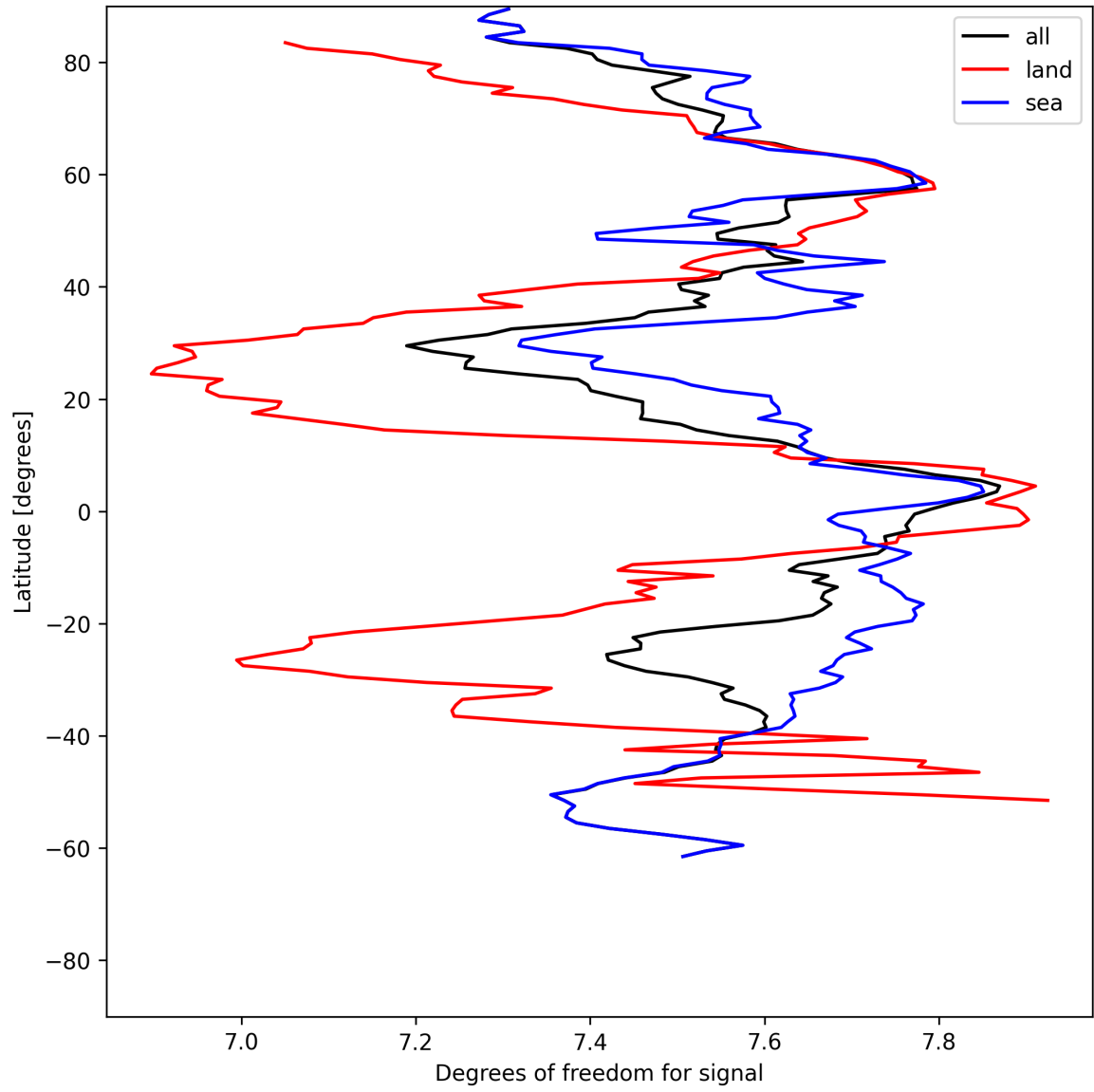
Figure 15: Zonal average of “Degrees of freedom for signal” for 2025-06-11 to 2025-06-12.
