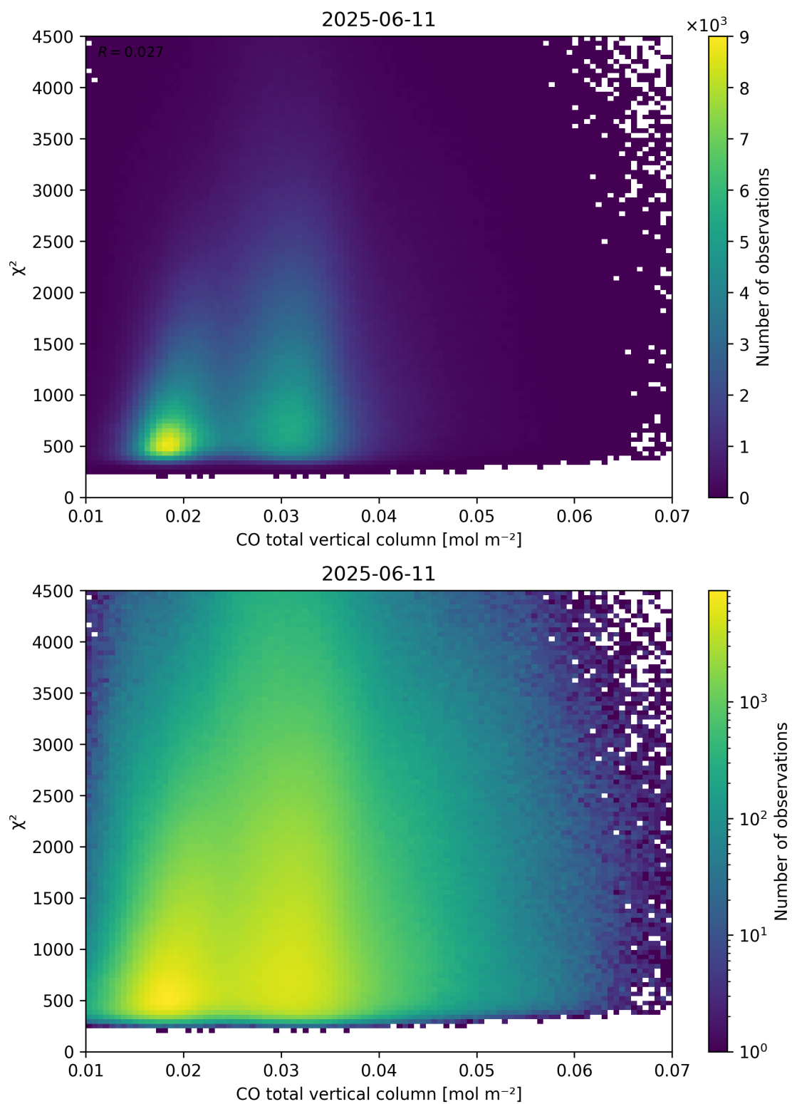
Figure 35: Scatter density plot of “CO total vertical column” against “ \chi^2 ” for 2025-06-11 to 2025-06-12.
