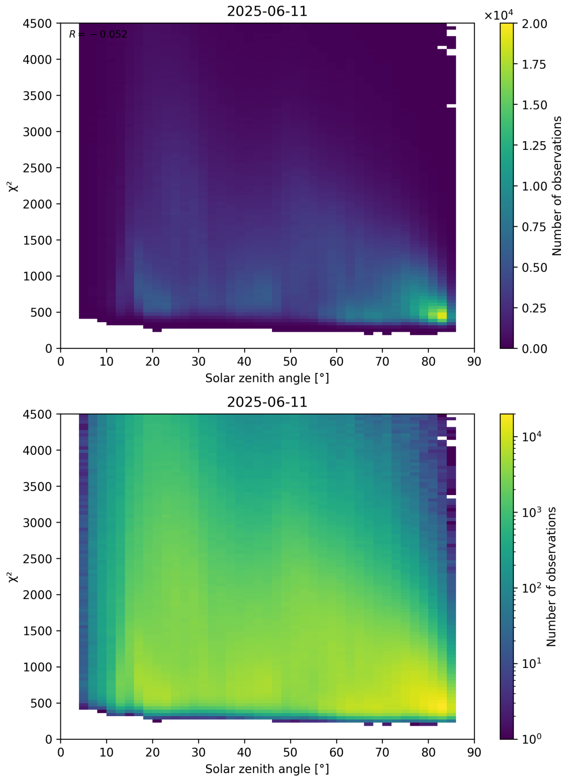
Figure 64: Scatter density plot of “Solar zenith angle” against “ \chi^2 ” for 2025-06-11 to 2025-06-12.
