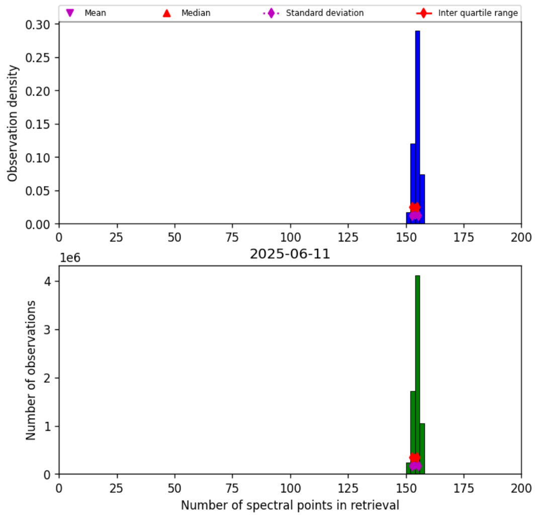
Figure 21: Histogram of “Number of spectral points in retrieval” for 2025-06-11 to 2025-06-12
