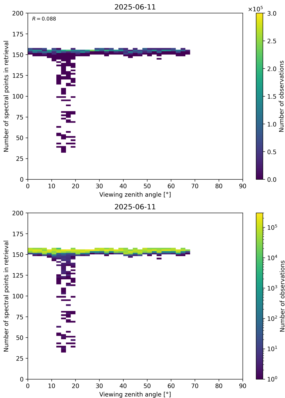
Figure 76: Scatter density plot of “Viewing zenith angle” against “Number of spectral points in retrieval” for 2025-06-11 to 2025-06-12.
