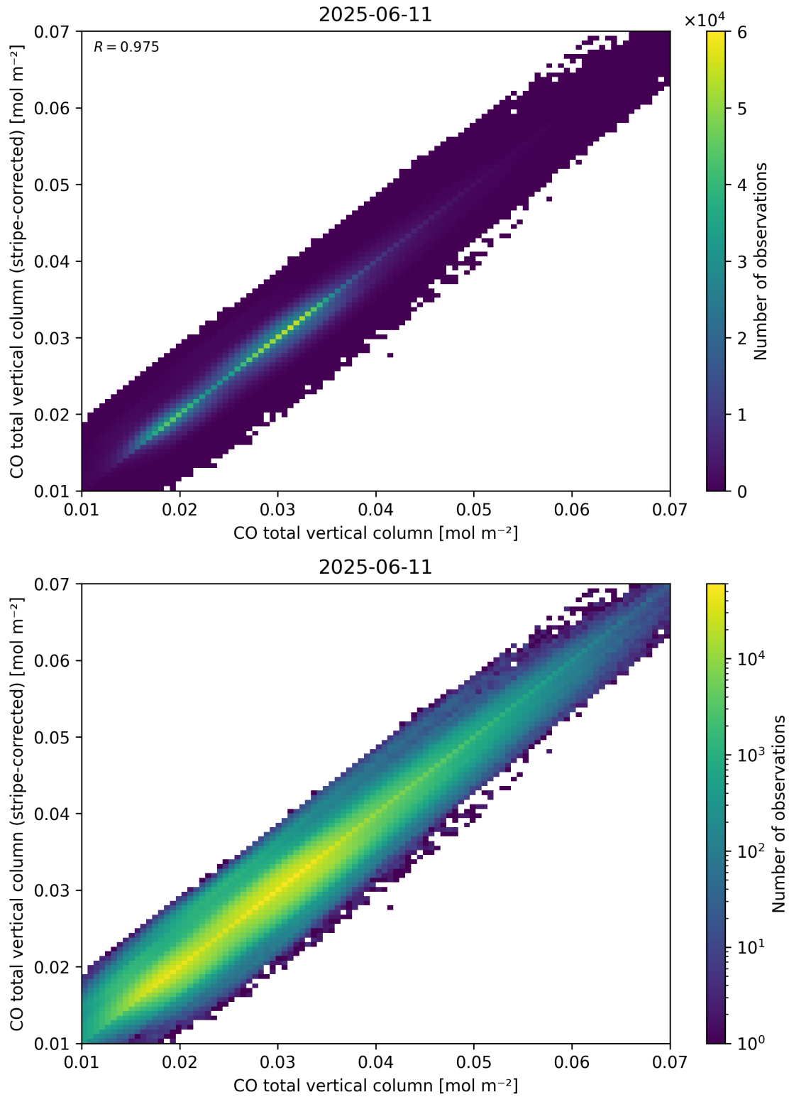
Figure 33: Scatter density plot of “CO total vertical column” against “CO total vertical column (stripe-corrected)” for 2025-06-11 to 2025-06-12.
