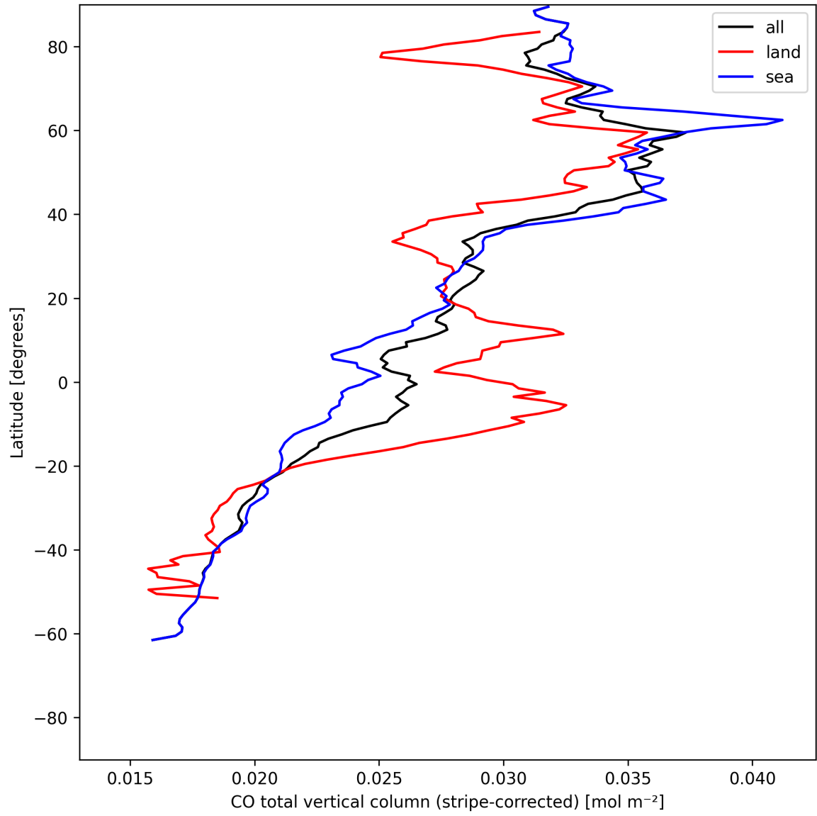
Figure 11: Zonal average of “CO total vertical column (stripe-corrected)” for 2025-06-11 to 2025-06-12.
