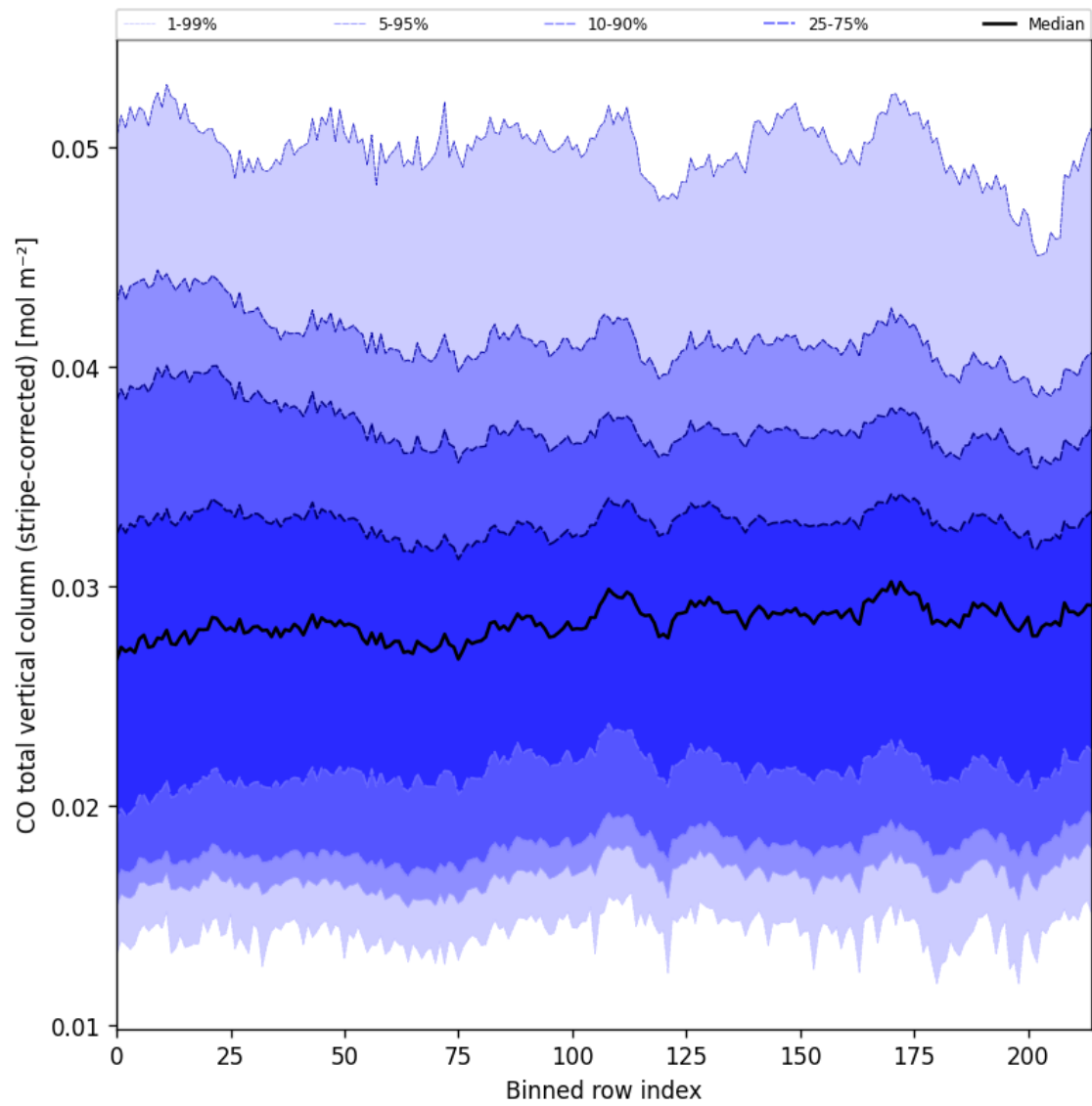
Figure 27: Along track statistics of “CO total vertical column (stripe-corrected)” for 2025-06-11 to 2025-06-12
