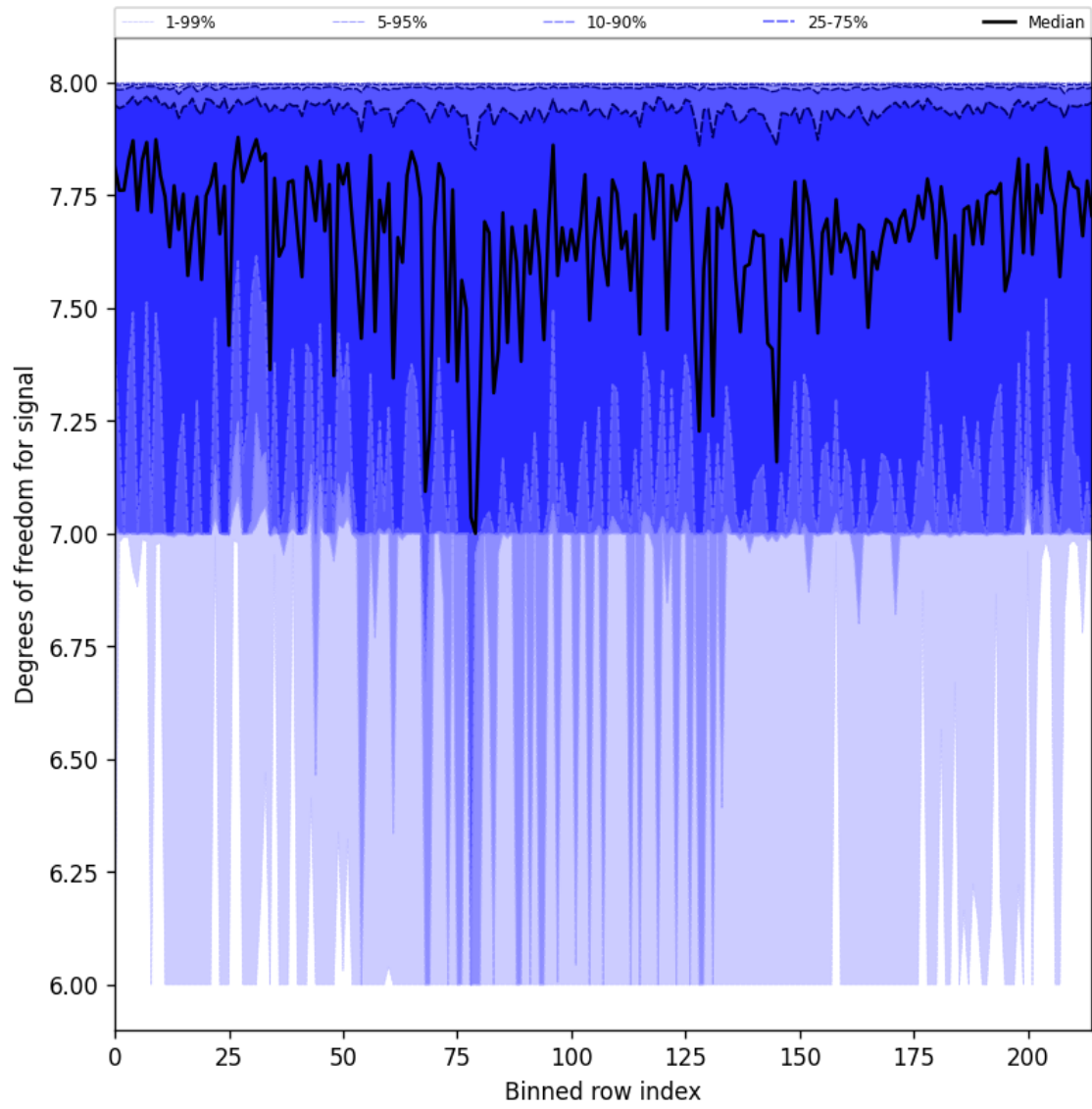
Figure 31: Along track statistics of “Degrees of freedom for signal” for 2025-06-11 to 2025-06-12
