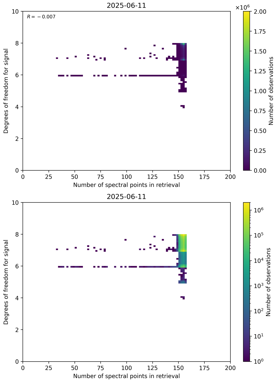
Figure 59: Scatter density plot of “Number of spectral points in retrieval” against “Degrees of freedom for signal” for 2025-06-11 to 2025-06-12.
