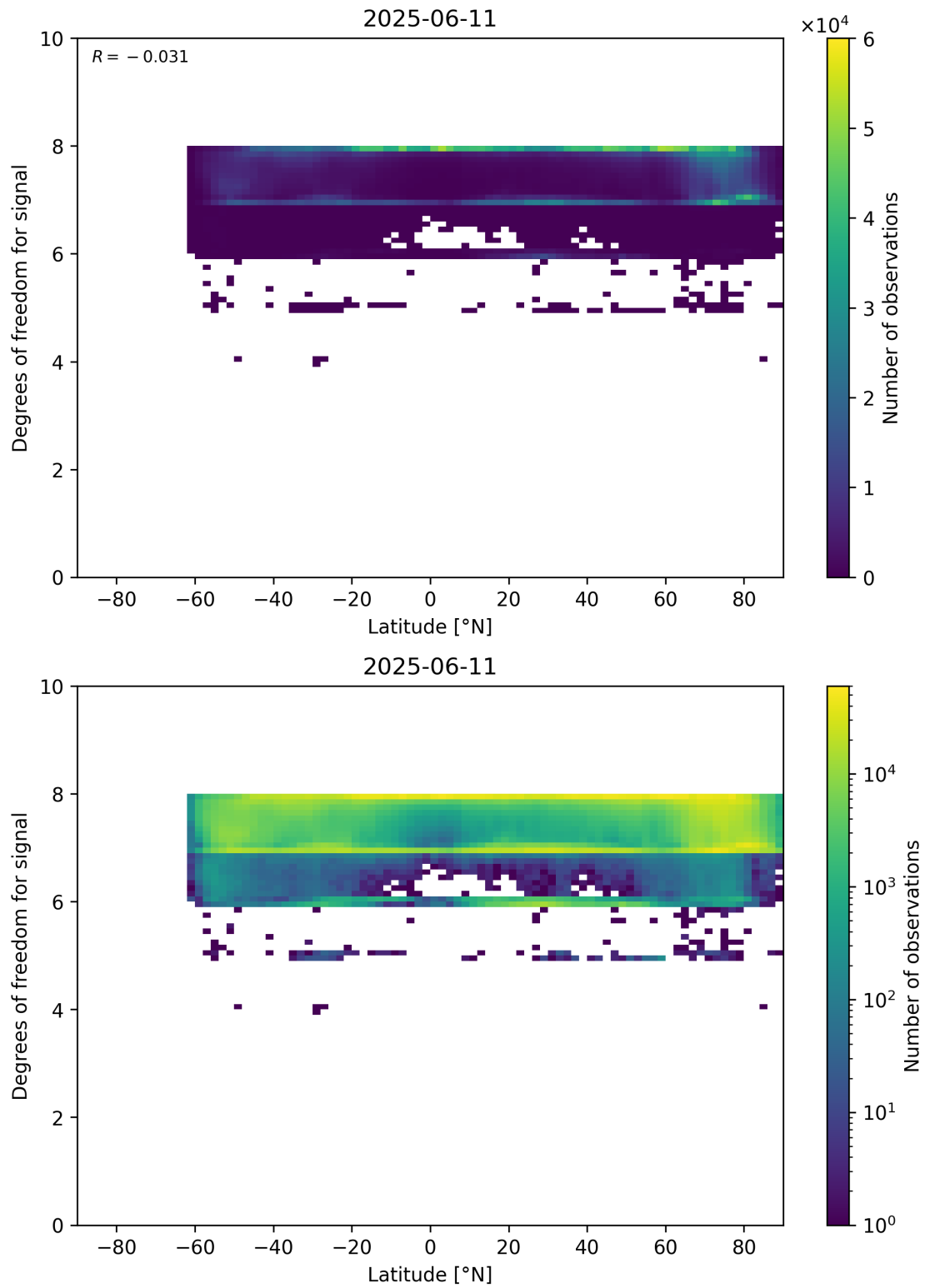
Figure 55: Scatter density plot of “Latitude” against “Degrees of freedom for signal” for 2025-06-11 to 2025-06-12.
