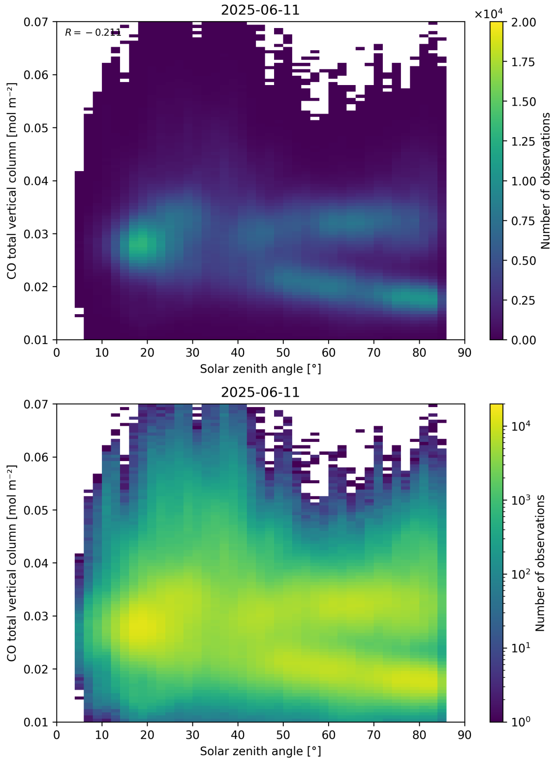
Figure 61: Scatter density plot of “Solar zenith angle” against “CO total vertical column” for 2025-06-11 to 2025-06-12.
