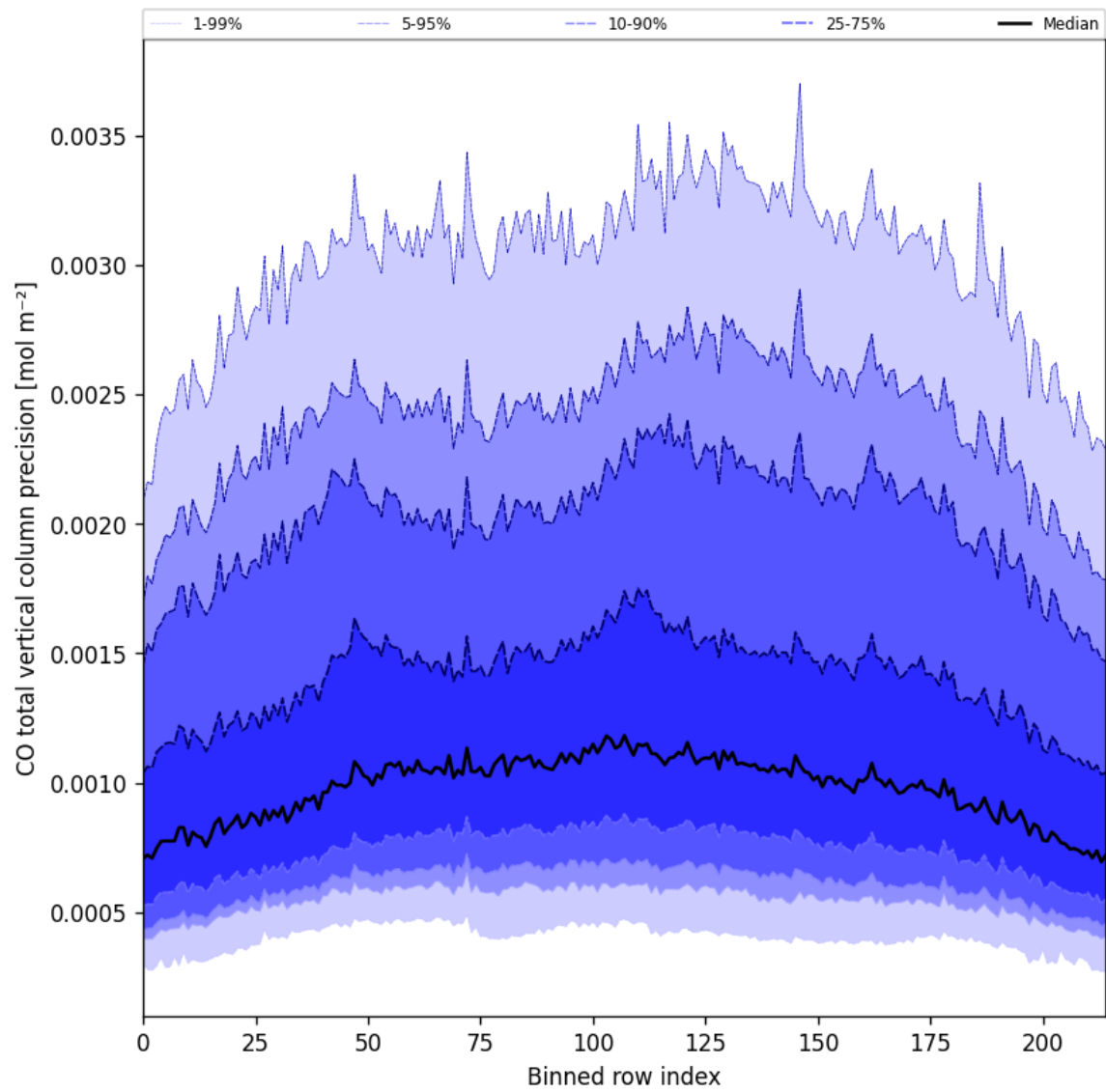
Figure 28: Along track statistics of "CO total vertical column precision" for 2025-06-11 to 2025-06-12
