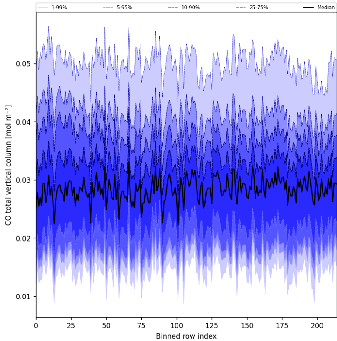
Figure 26: Along track statistics of “CO total vertical column” for 2025-06-11 to 2025-06-12
