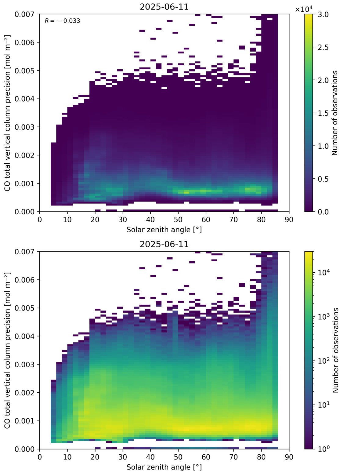
Figure 63: Scatter density plot of “Solar zenith angle” against “CO total vertical column precision” for 2025-06-11 to 2025-06-12.
