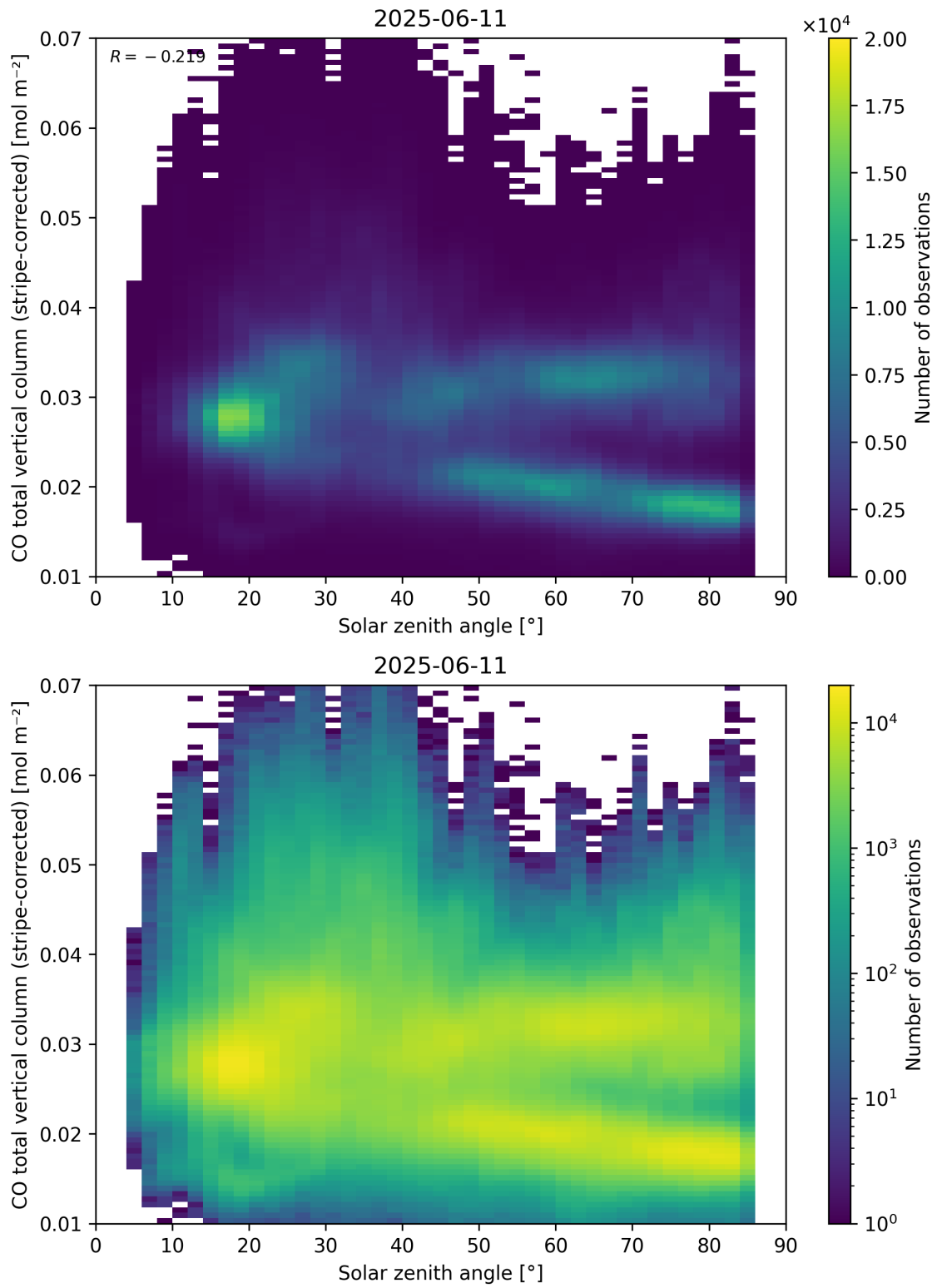
Figure 62: Scatter density plot of “Solar zenith angle” against “CO total vertical column (stripe-corrected)” for 2025-06-11 to 2025-06-12.
