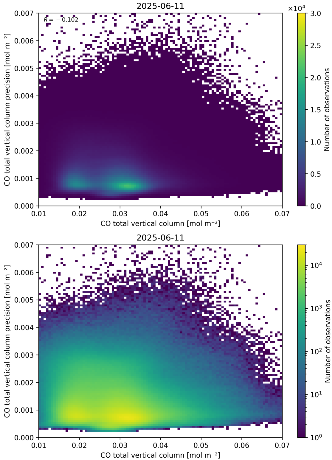
Figure 34: Scatter density plot of “CO total vertical column” against “CO total vertical column precision” for 2025-06-11 to 2025-06-12.
