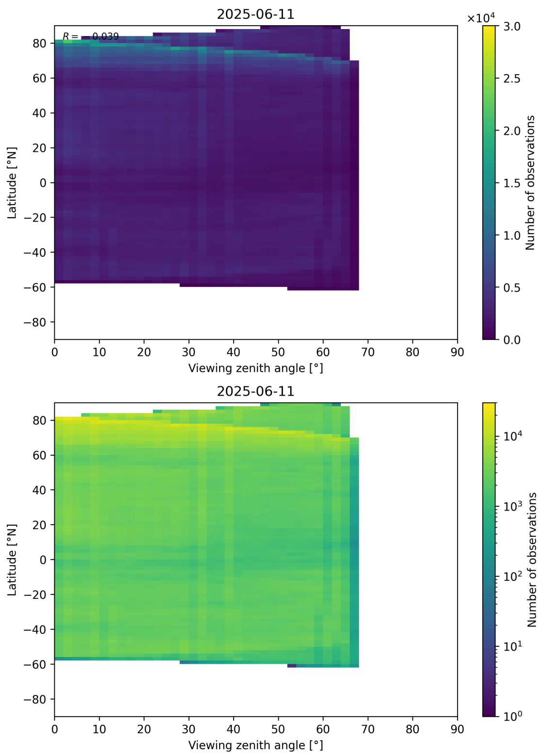
Figure 74: Scatter density plot of “Viewing zenith angle” against “Latitude” for 2025-06-11 to 2025-06-12.
