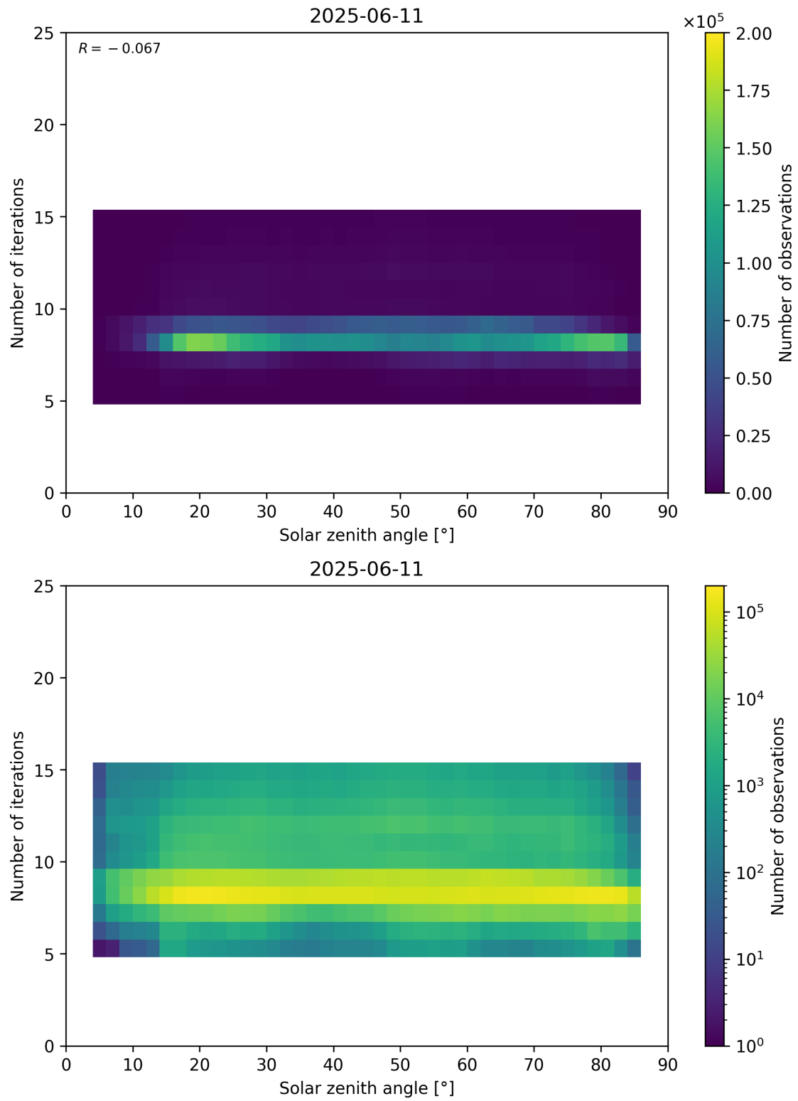
Figure 67: Scatter density plot of “Solar zenith angle” against “Number of iterations” for 2025-06-11 to 2025-06-12.
