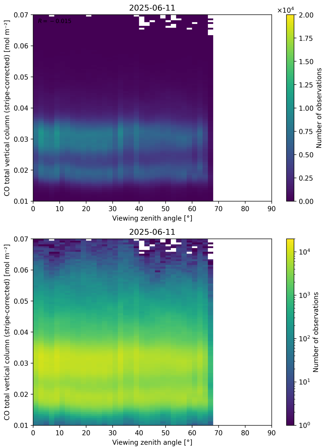
Figure 70: Scatter density plot of “Viewing zenith angle” against “CO total vertical column (stripe-corrected)” for 2025-06-11 to 2025-06-12.
