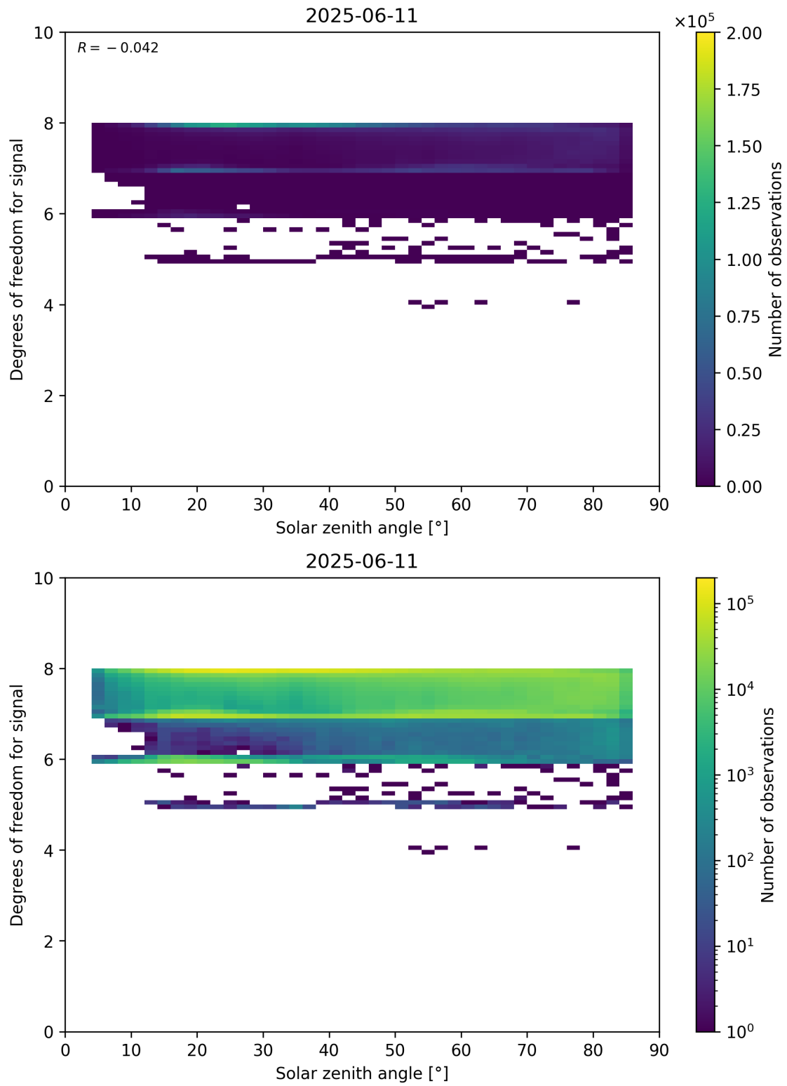
Figure 65: Scatter density plot of “Solar zenith angle” against “Degrees of freedom for signal” for 2025-06-11 to 2025-06-12.
