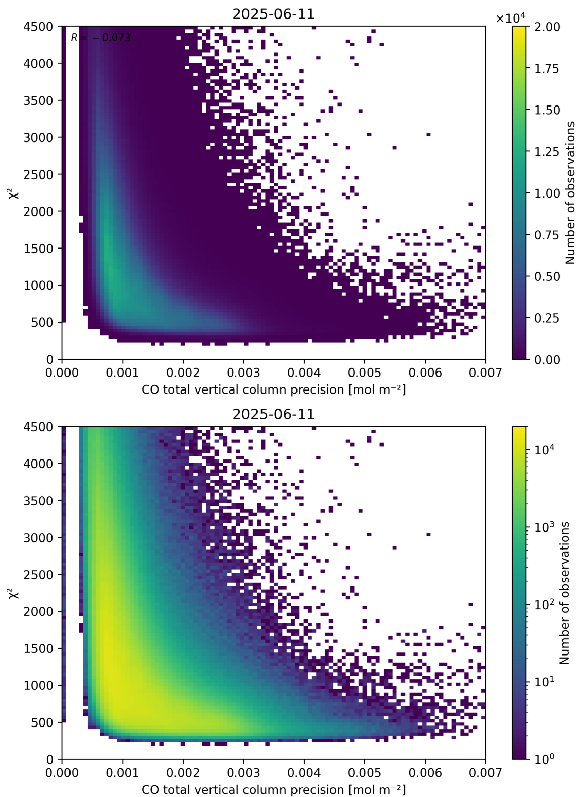
Figure 44: Scatter density plot of “CO total vertical column precision” against “ \chi^2 ” for 2025-06-11 to 2025-06-12.
