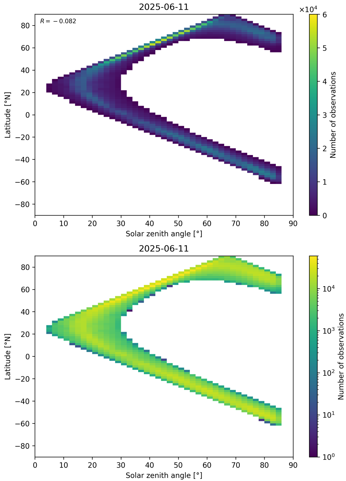
Figure 66: Scatter density plot of “Solar zenith angle” against “Latitude” for 2025-06-11 to 2025-06-12.
