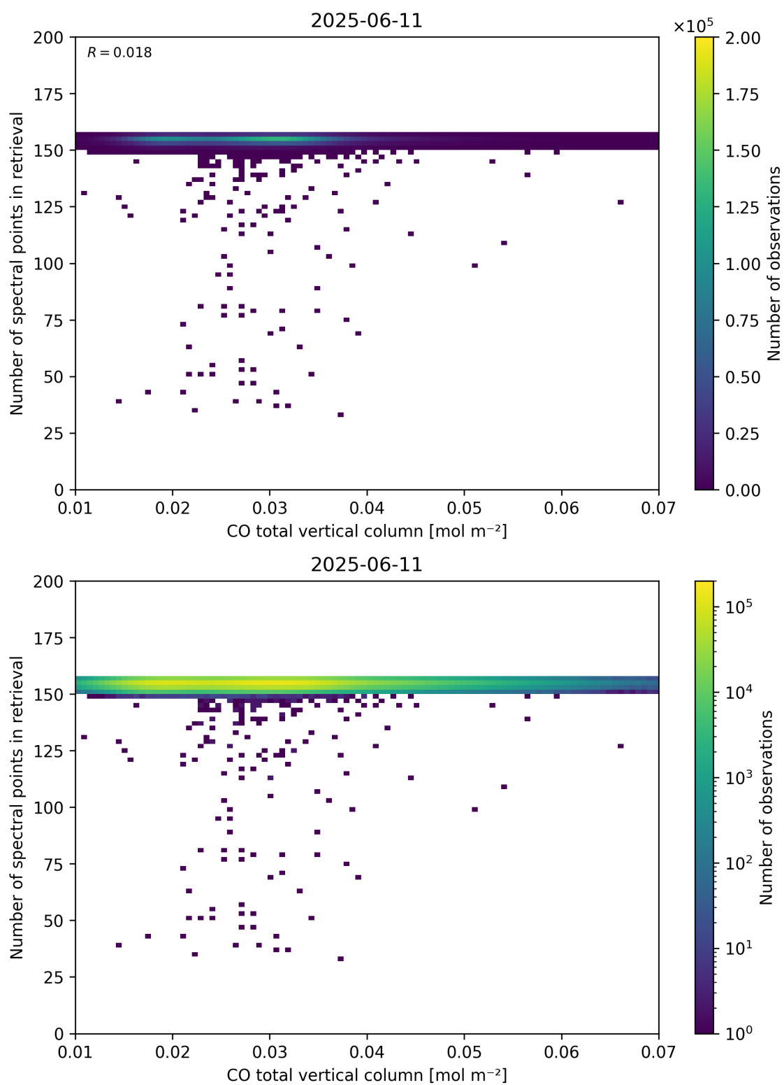
Figure 43: Scatter density plot of “CO total vertical column” against “Number of spectral points in retrieval” for 2025-06-11 to 2025-06-12.
