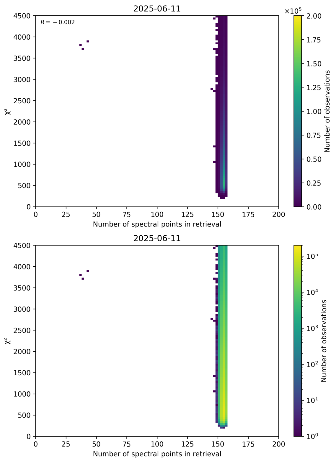
Figure 58: Scatter density plot of “Number of spectral points in retrieval” against “ \chi^2 ” for 2025-06-11 to 2025-06-12.
