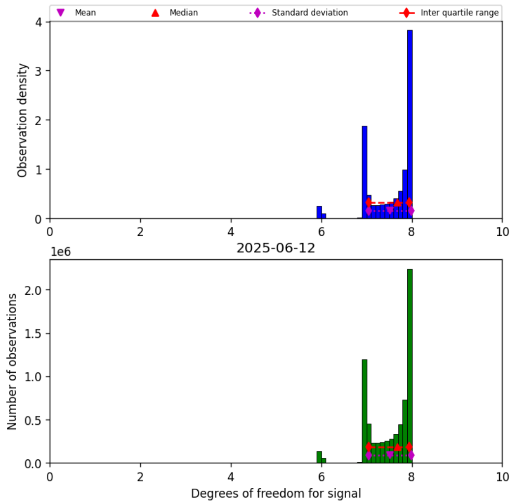
Figure 23: Histogram of “Degrees of freedom for signal” for 2025-06-11 to 2025-06-13
