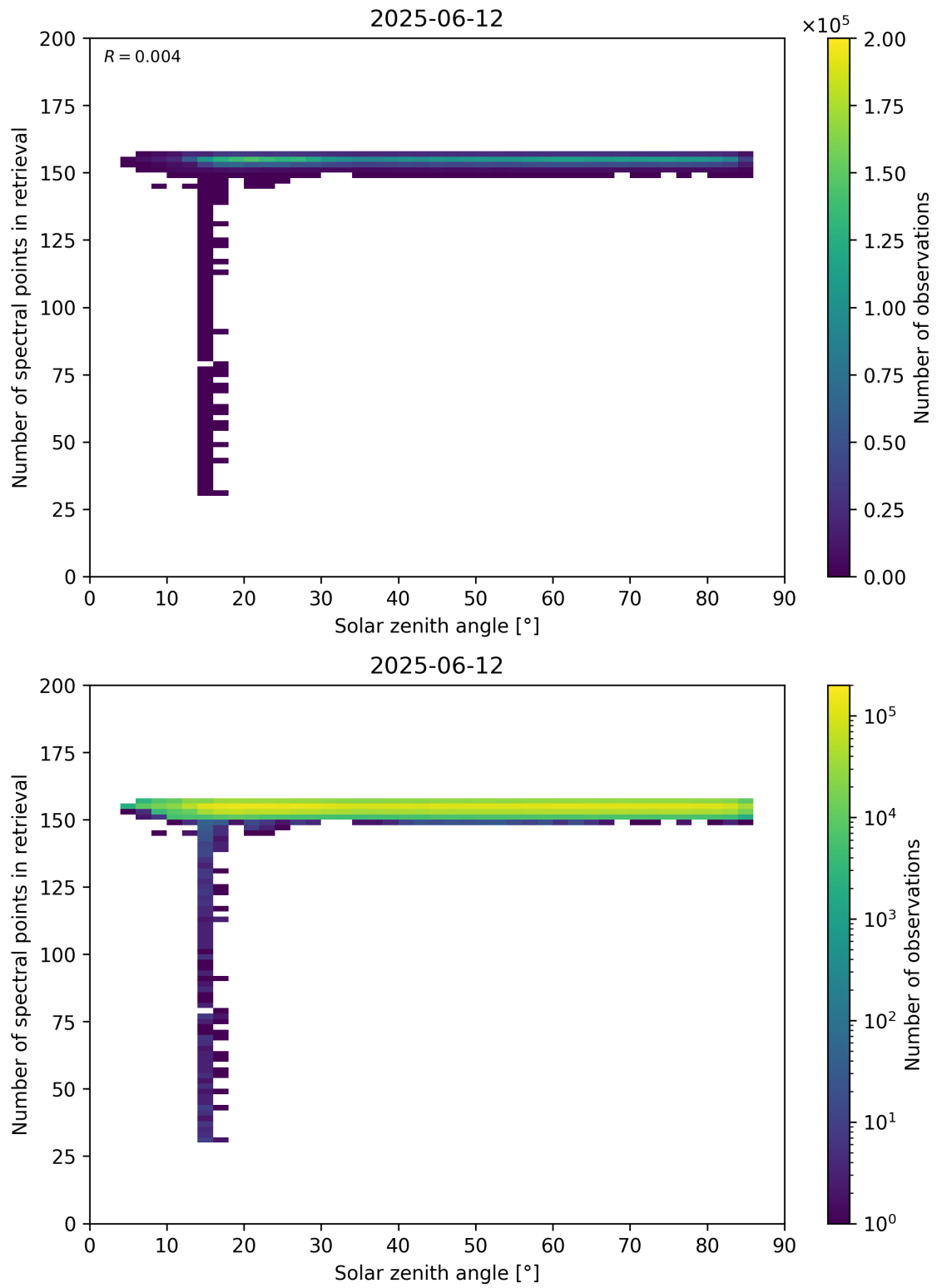
Figure 68: Scatter density plot of “Solar zenith angle” against “Number of spectral points in retrieval” for 2025-06-11 to 2025-06-13.
