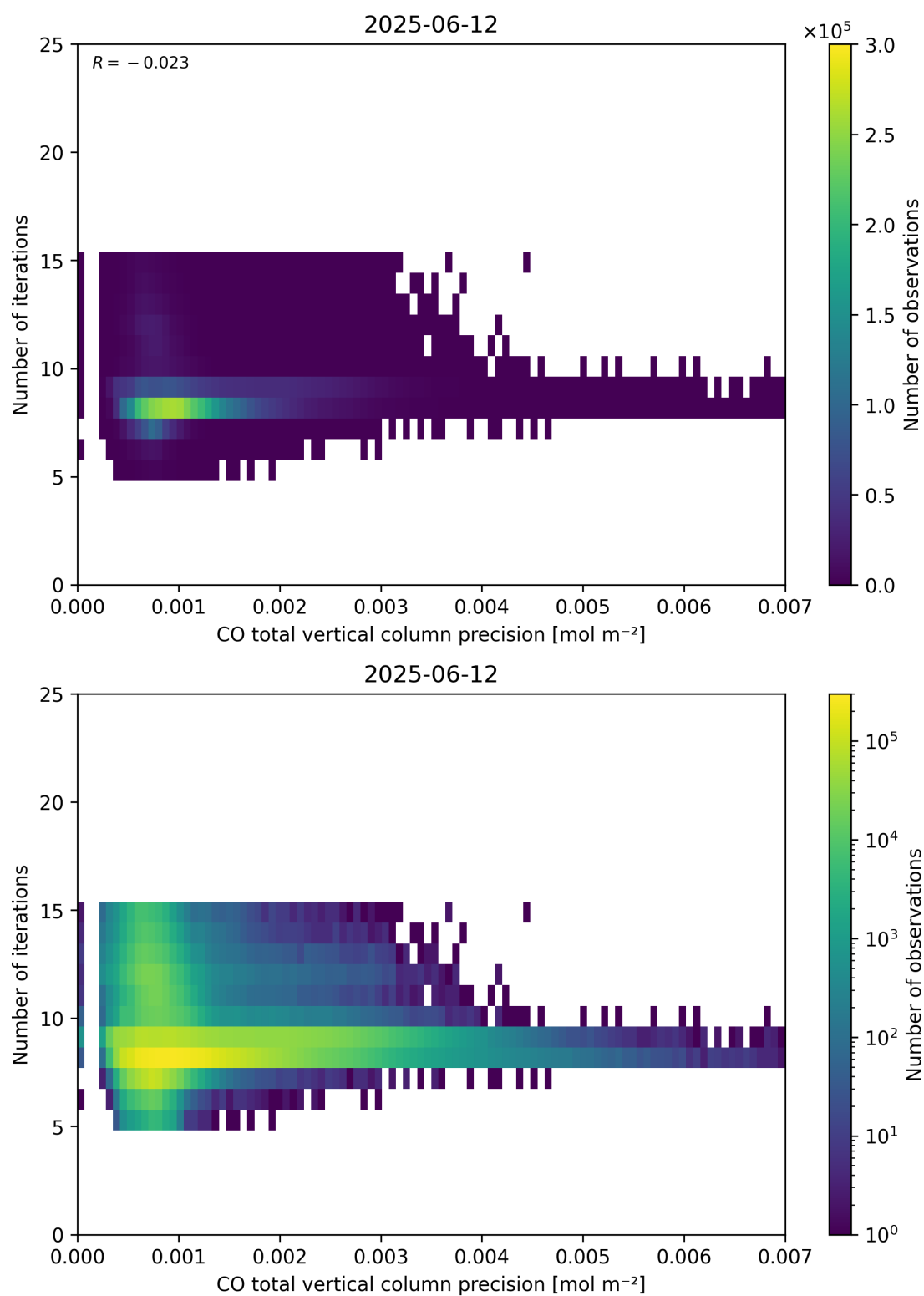
Figure 46: Scatter density plot of “CO total vertical column precision” against “Number of iterations” for 2025-06-11 to 2025-06-13.
