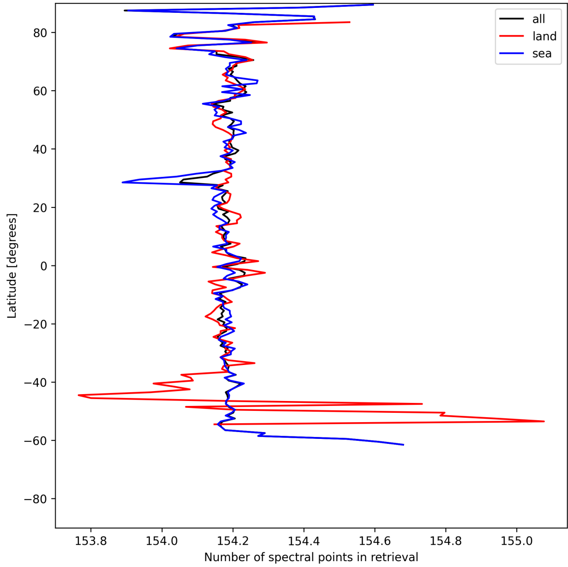
Figure 13: Zonal average of “Number of spectral points in retrieval” for 2025-06-11 to 2025-06-13.
