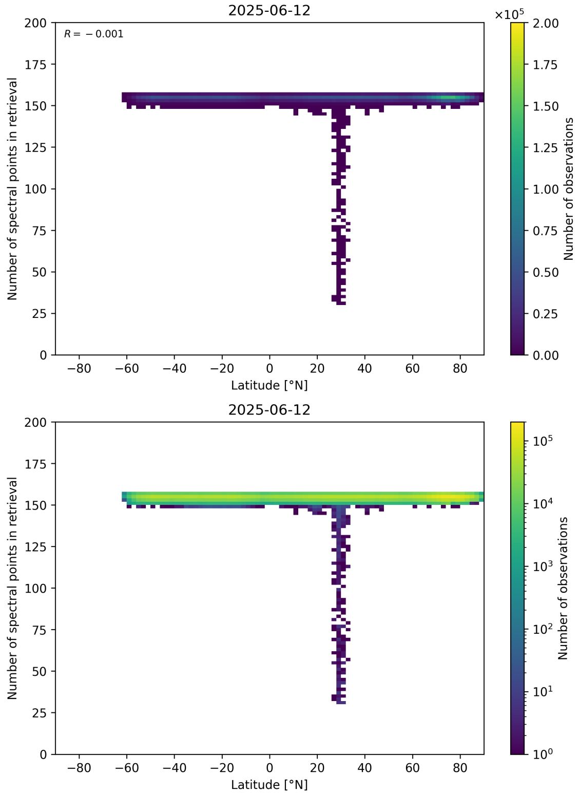
Figure 57: Scatter density plot of “Latitude” against “Number of spectral points in retrieval” for 2025-06-11 to 2025-06-13.
