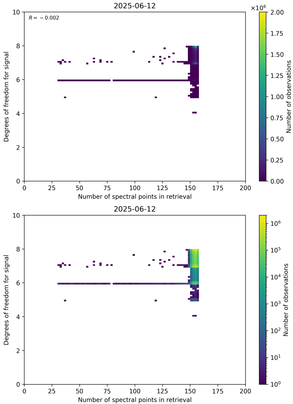
Figure 59: Scatter density plot of “Number of spectral points in retrieval” against “Degrees of freedom for signal” for 2025-06-11 to 2025-06-13.
