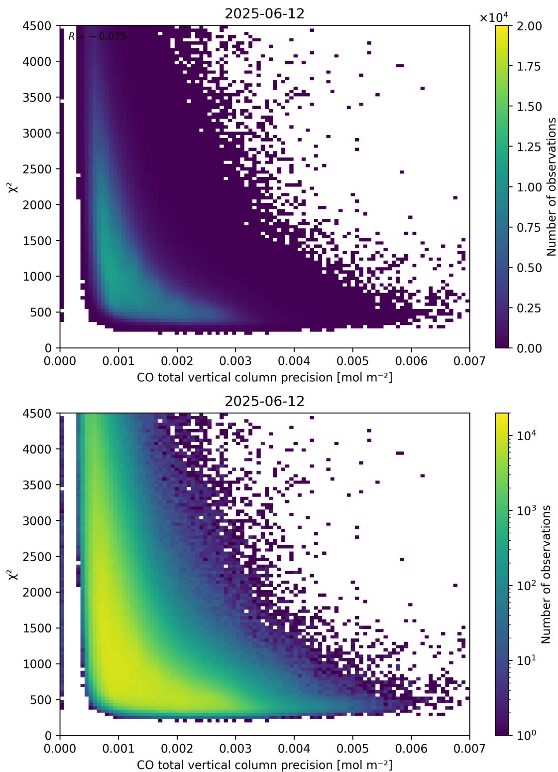
Figure 44: Scatter density plot of “CO total vertical column precision” against “ \chi^2 ” for 2025-06-11 to 2025-06-13.
