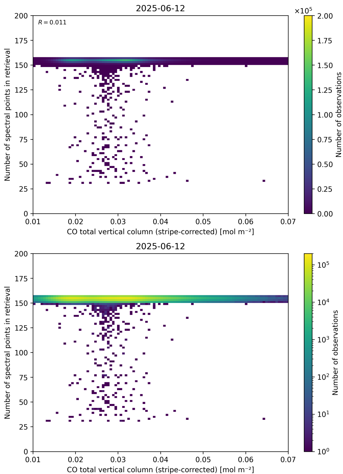
Figure 40: Scatter density plot of “CO total vertical column (stripe-corrected)” against “Number of spectral points in retrieval” for 2025-06-11 to 2025-06-13.
