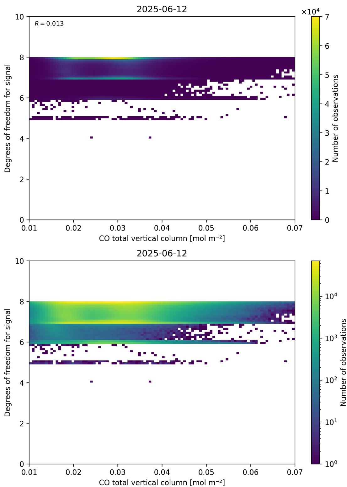
Figure 41: Scatter density plot of “CO total vertical column” against “Degrees of freedom for signal” for 2025-06-11 to 2025-06-13.
