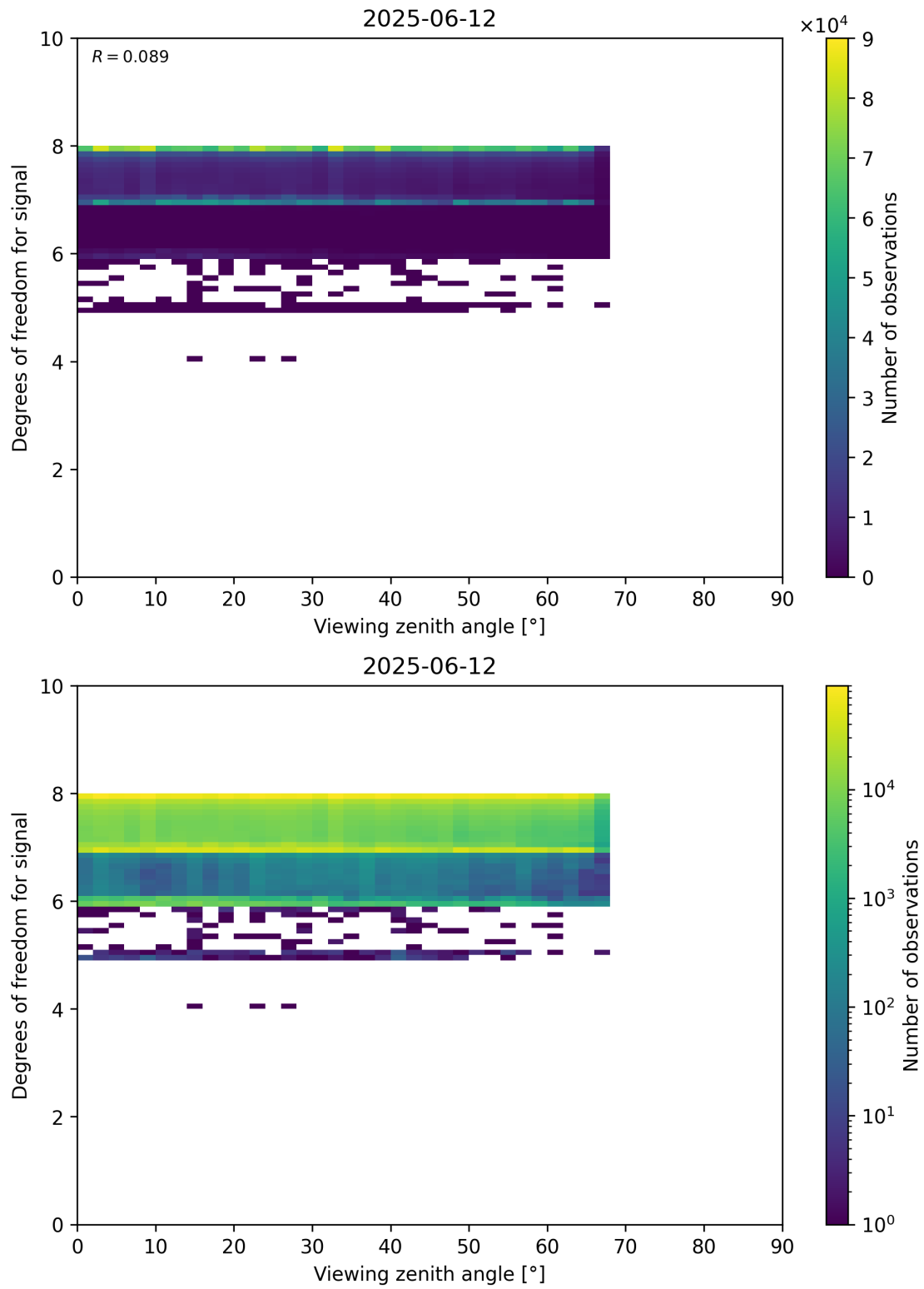
Figure 73: Scatter density plot of “Viewing zenith angle” against “Degrees of freedom for signal” for 2025-06-11 to 2025-06-13.
