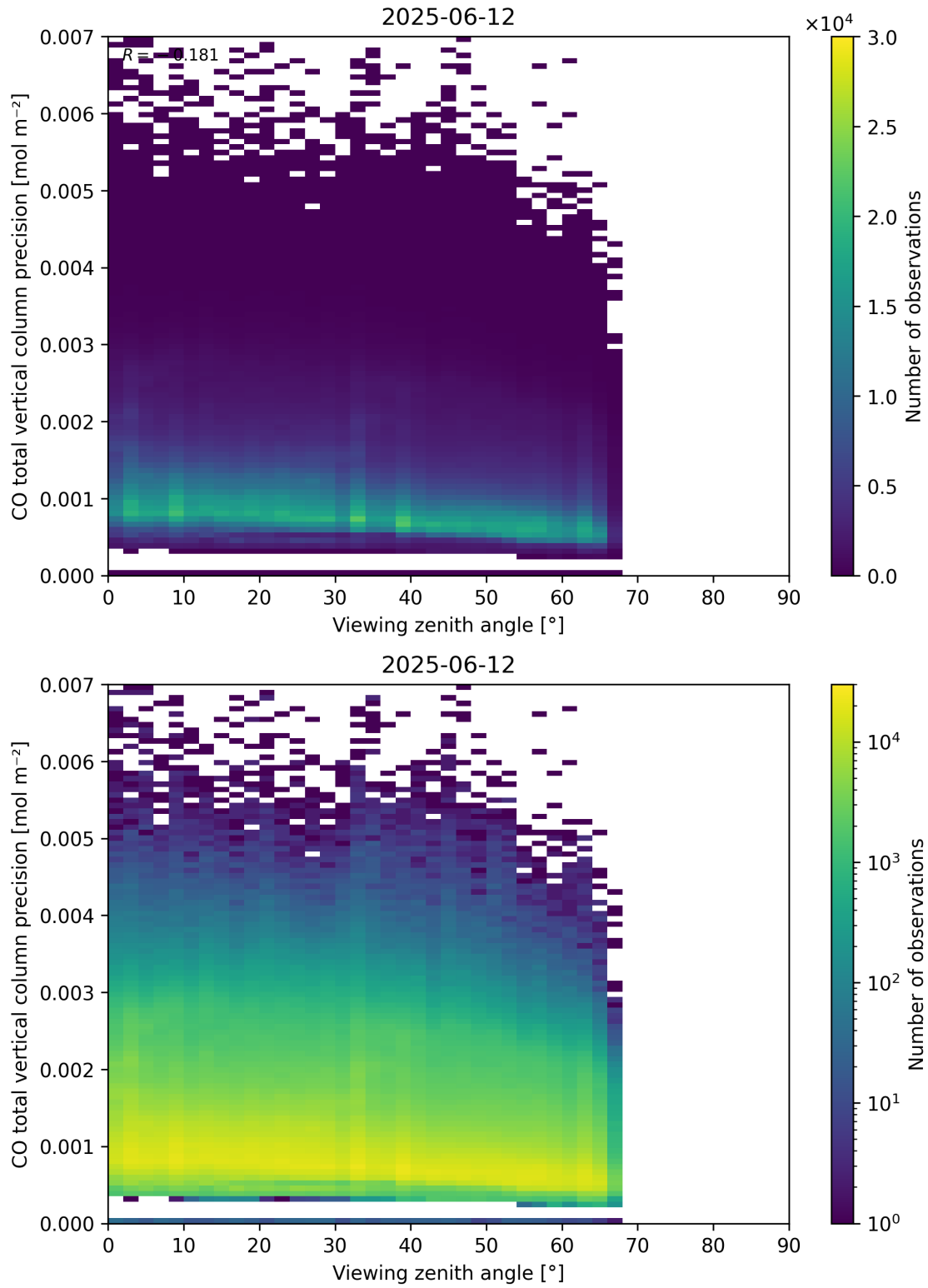
Figure 71: Scatter density plot of “Viewing zenith angle” against “CO total vertical column precision” for 2025-06-11 to 2025-06-13.
