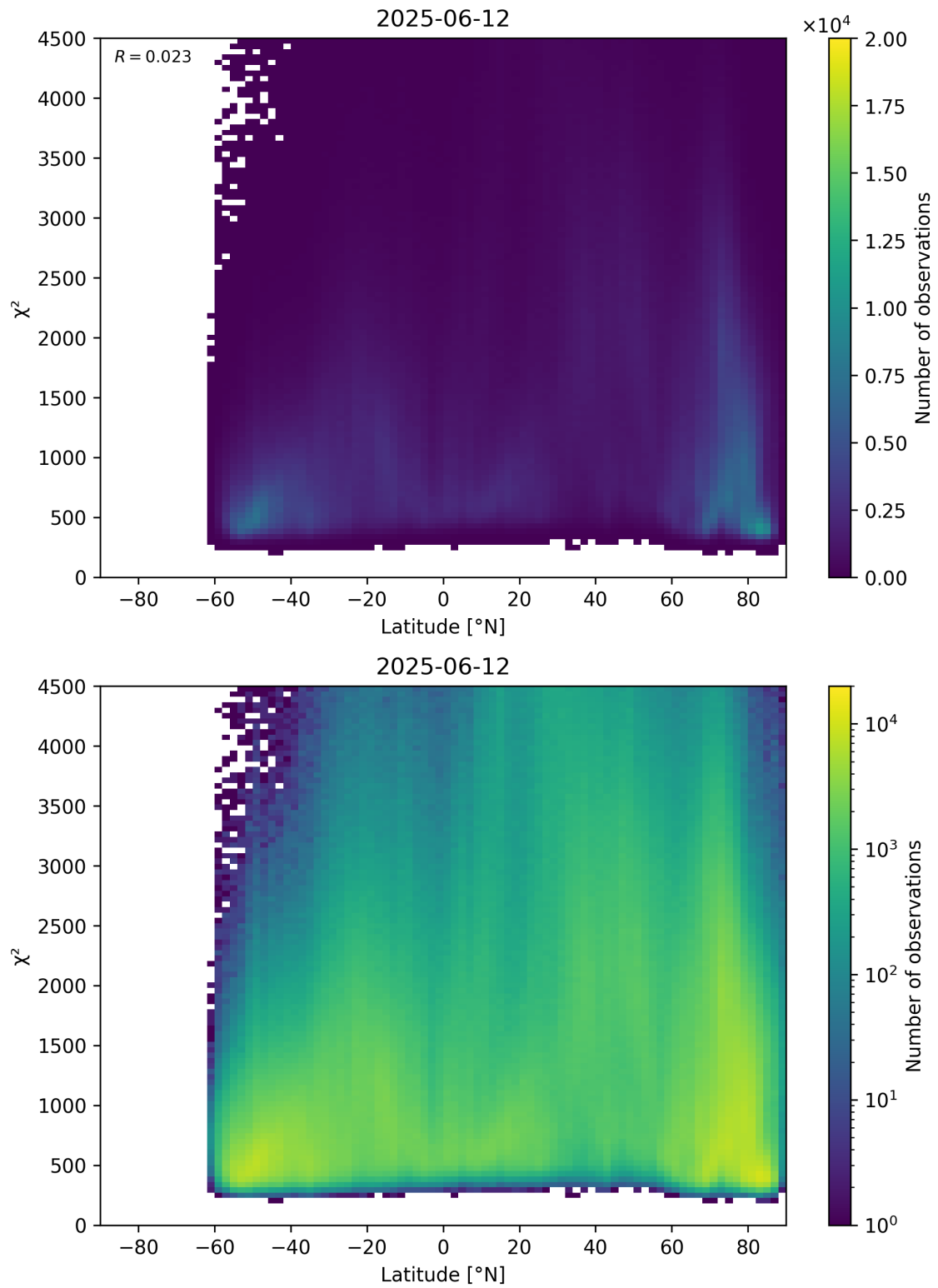
Figure 54: Scatter density plot of “Latitude” against “ \chi^2 ” for 2025-06-11 to 2025-06-13.
