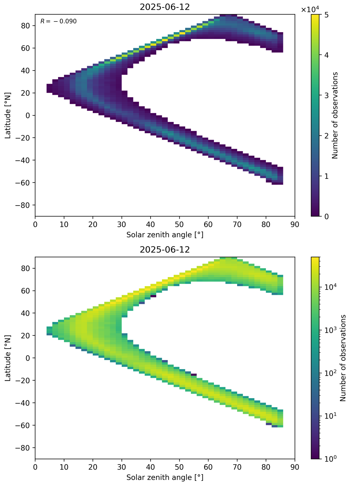
Figure 66: Scatter density plot of “Solar zenith angle” against “Latitude” for 2025-06-11 to 2025-06-13.
