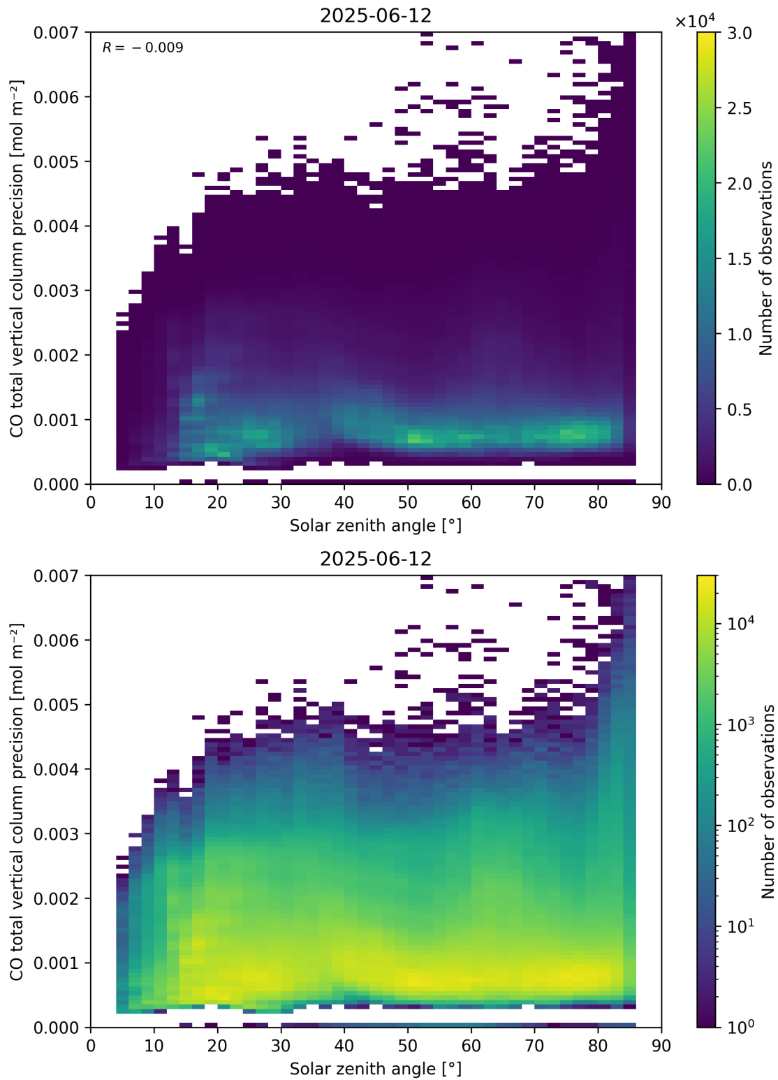
Figure 63: Scatter density plot of “Solar zenith angle” against “CO total vertical column precision” for 2025-06-11 to 2025-06-13.
