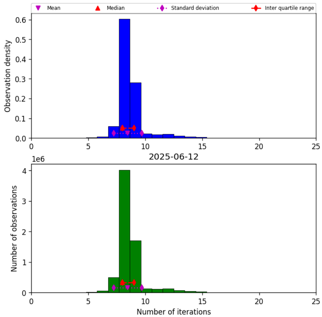
Figure 24: Histogram of “Number of iterations” for 2025-06-11 to 2025-06-13
