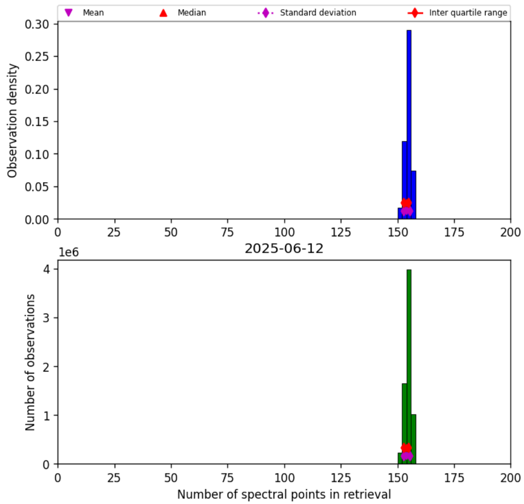
Figure 21: Histogram of “Number of spectral points in retrieval” for 2025-06-11 to 2025-06-13
