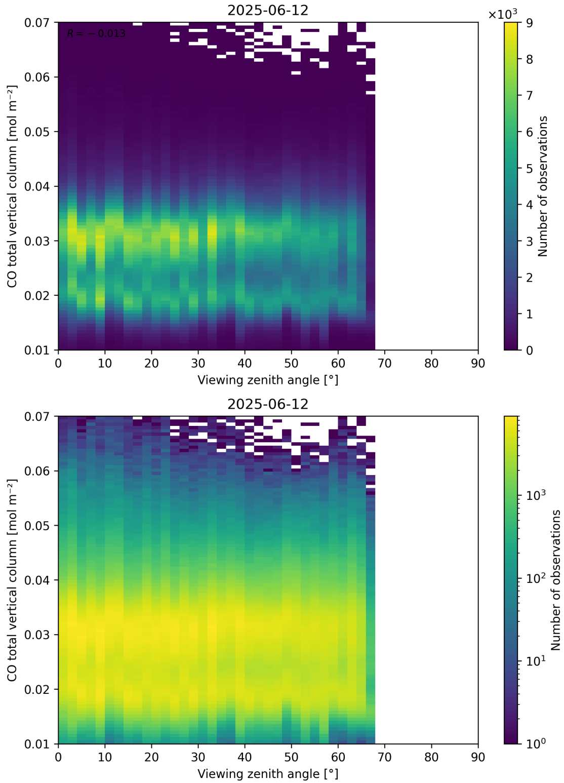
Figure 69: Scatter density plot of “Viewing zenith angle” against “CO total vertical column” for 2025-06-11 to 2025-06-13.
