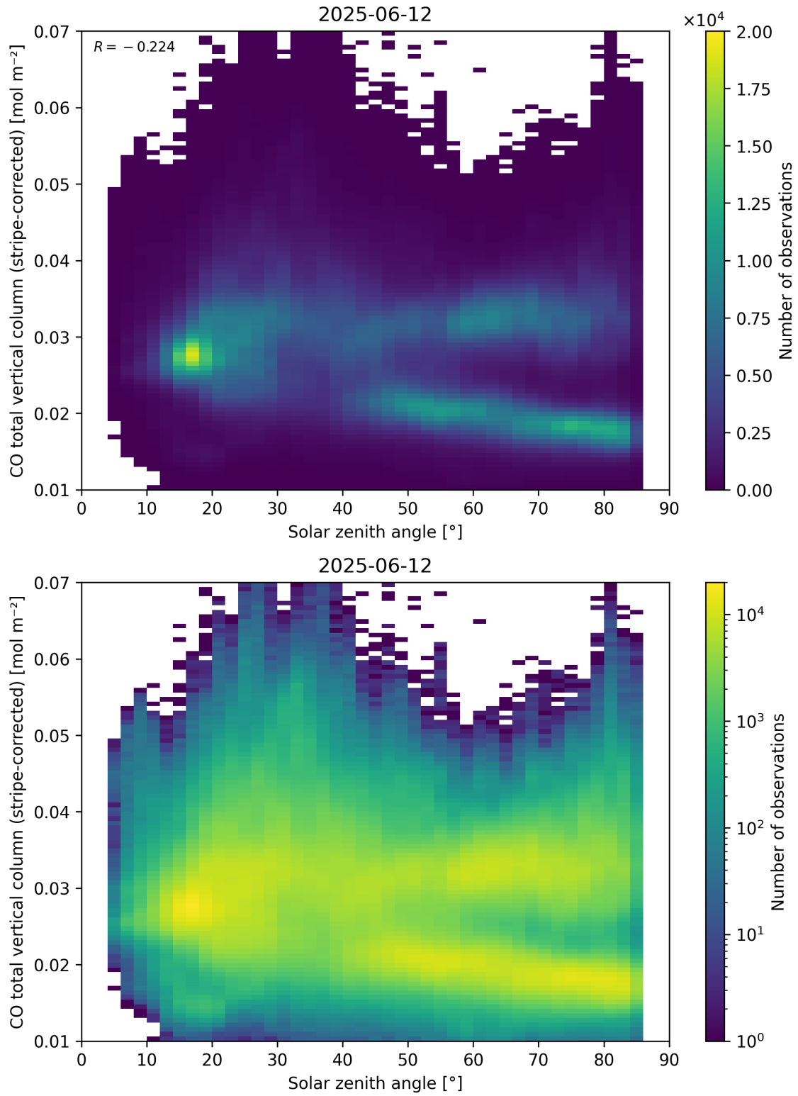
Figure 62: Scatter density plot of “Solar zenith angle” against “CO total vertical column (stripe-corrected)” for 2025-06-11 to 2025-06-13.
