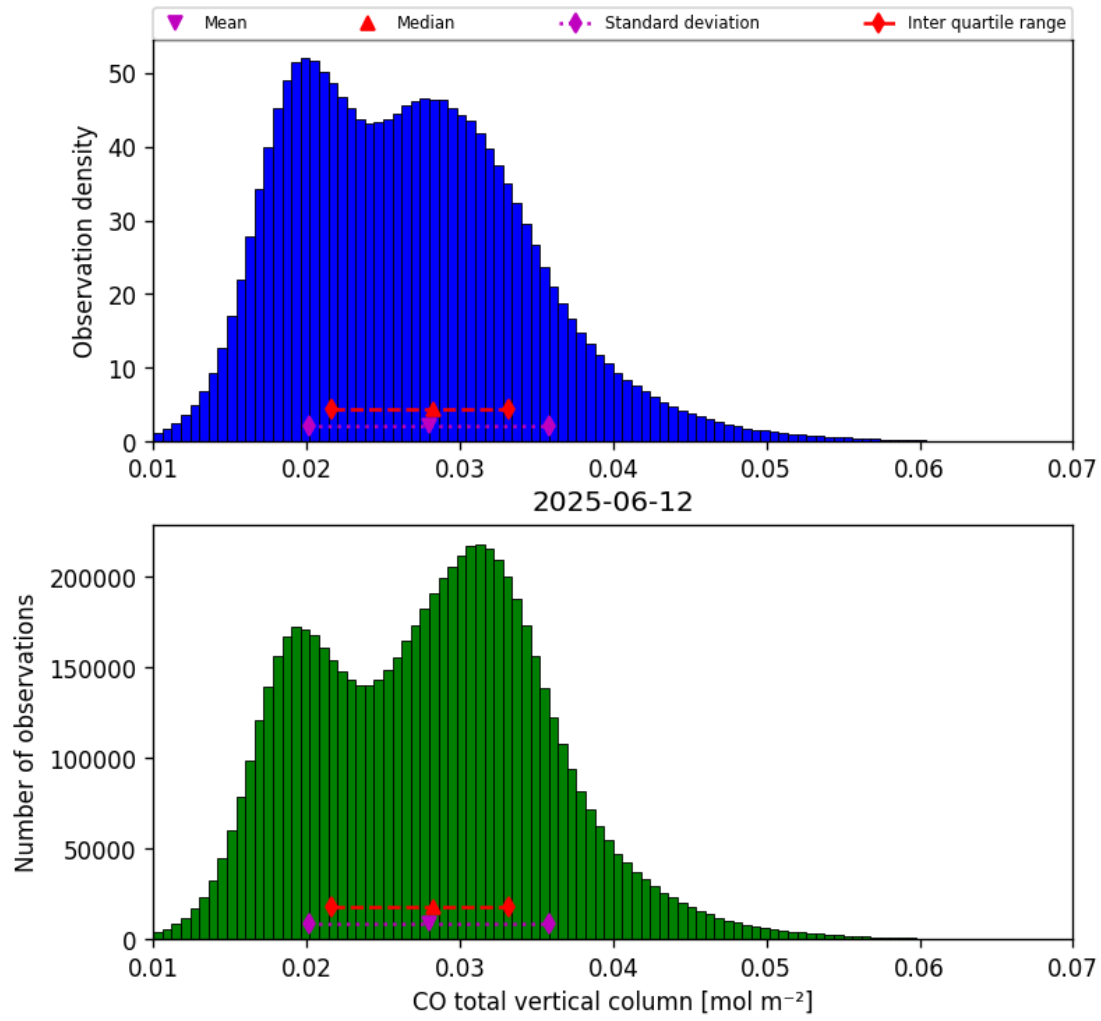
Figure 18: Histogram of “CO total vertical column” for 2025-06-11 to 2025-06-13
