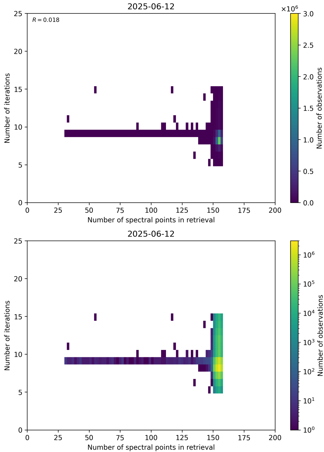
Figure 60: Scatter density plot of “Number of spectral points in retrieval” against “Number of iterations” for 2025-06-11 to 2025-06-13.
