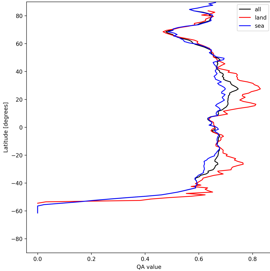
Figure 9: Zonal average of “QA value” for 2025-06-11 to 2025-06-13.
