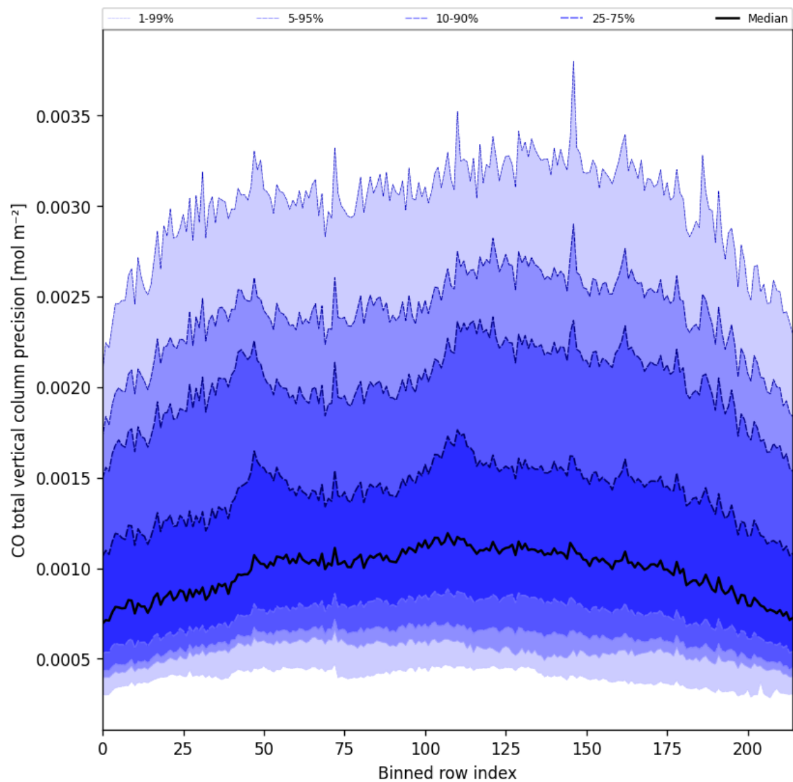
Figure 28: Along track statistics of “CO total vertical column precision” for 2025-06-11 to 2025-06-13
