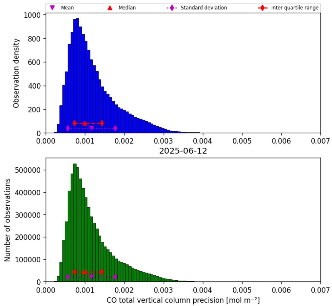
Figure 20: Histogram of “CO total vertical column precision” for 2025-06-11 to 2025-06-13
