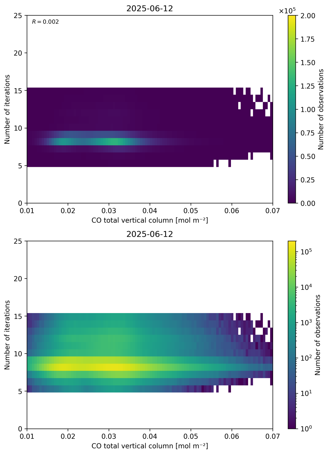
Figure 42: Scatter density plot of “CO total vertical column” against “Number of iterations” for 2025-06-11 to 2025-06-13.
