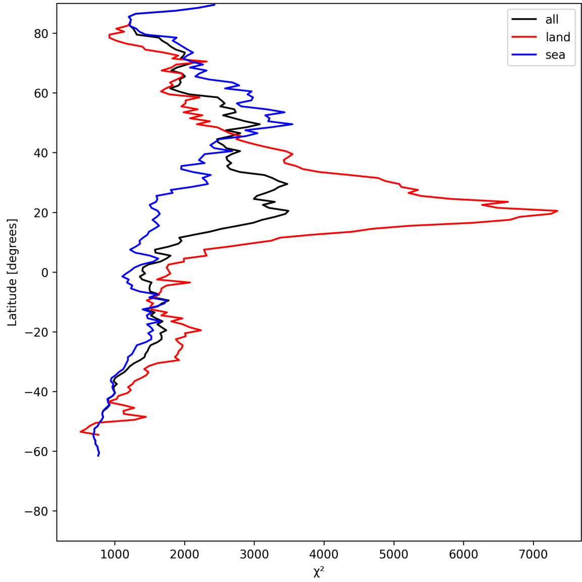
Figure 14: Zonal average of “ \chi^2 ” for 2025-06-11 to 2025-06-13.
