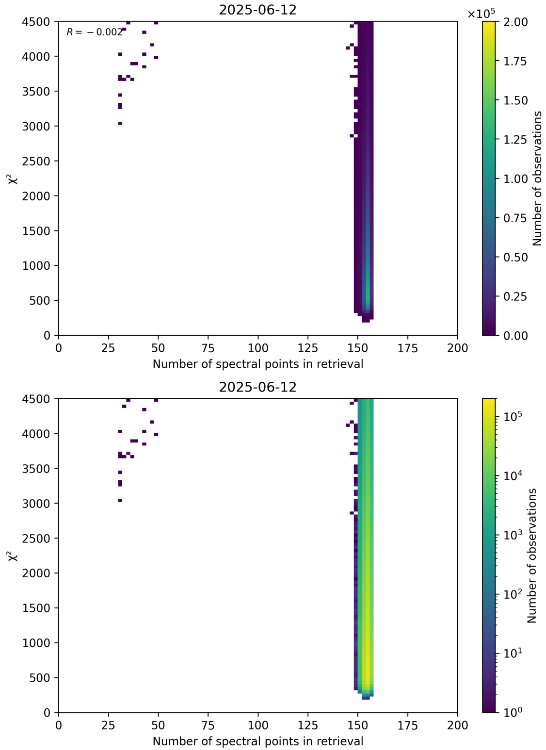
Figure 58: Scatter density plot of “Number of spectral points in retrieval” against “ \chi^2 ” for 2025-06-11 to 2025-06-13.
