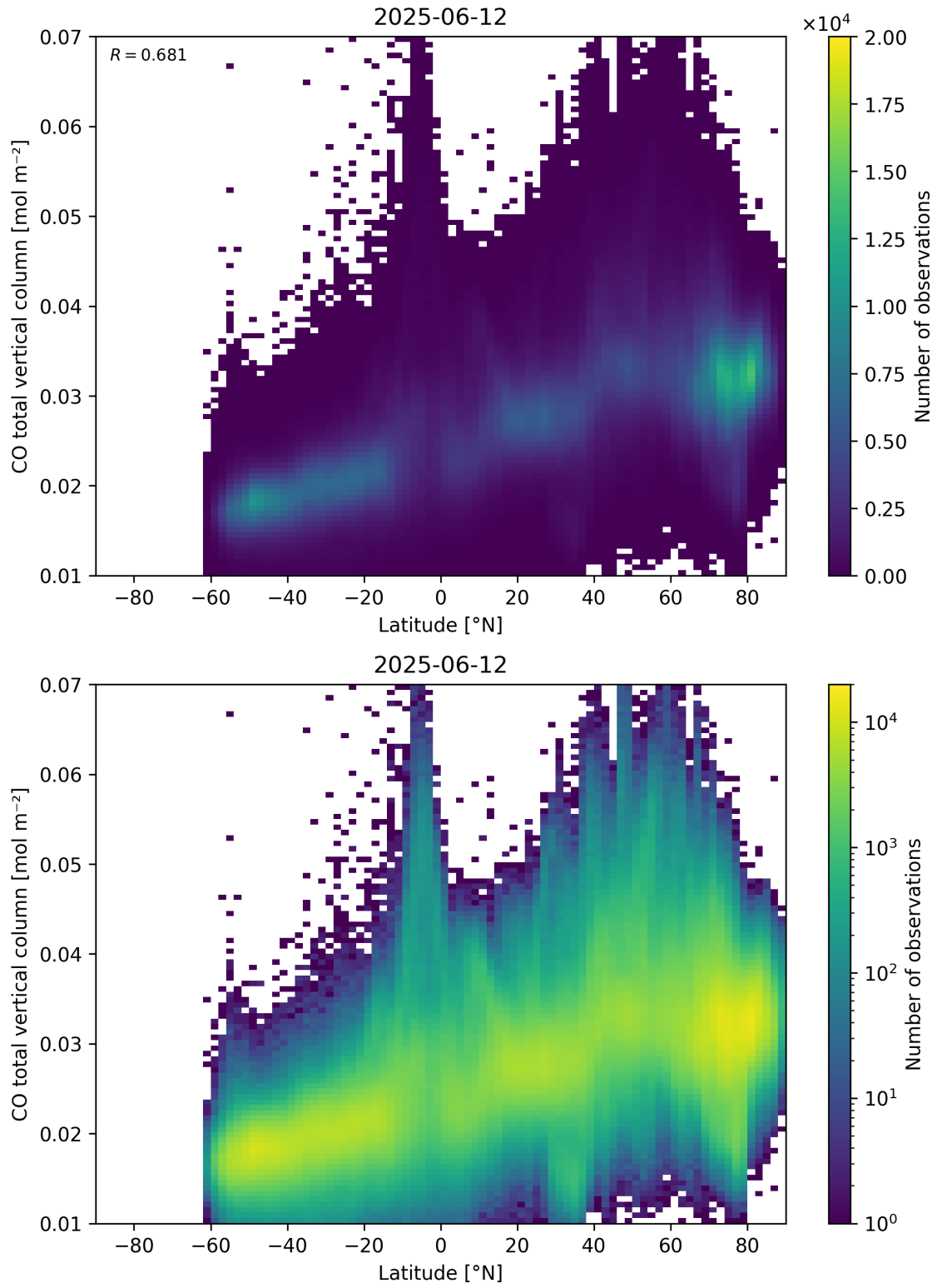
Figure 51: Scatter density plot of “Latitude” against “CO total vertical column” for 2025-06-11 to 2025-06-13.
