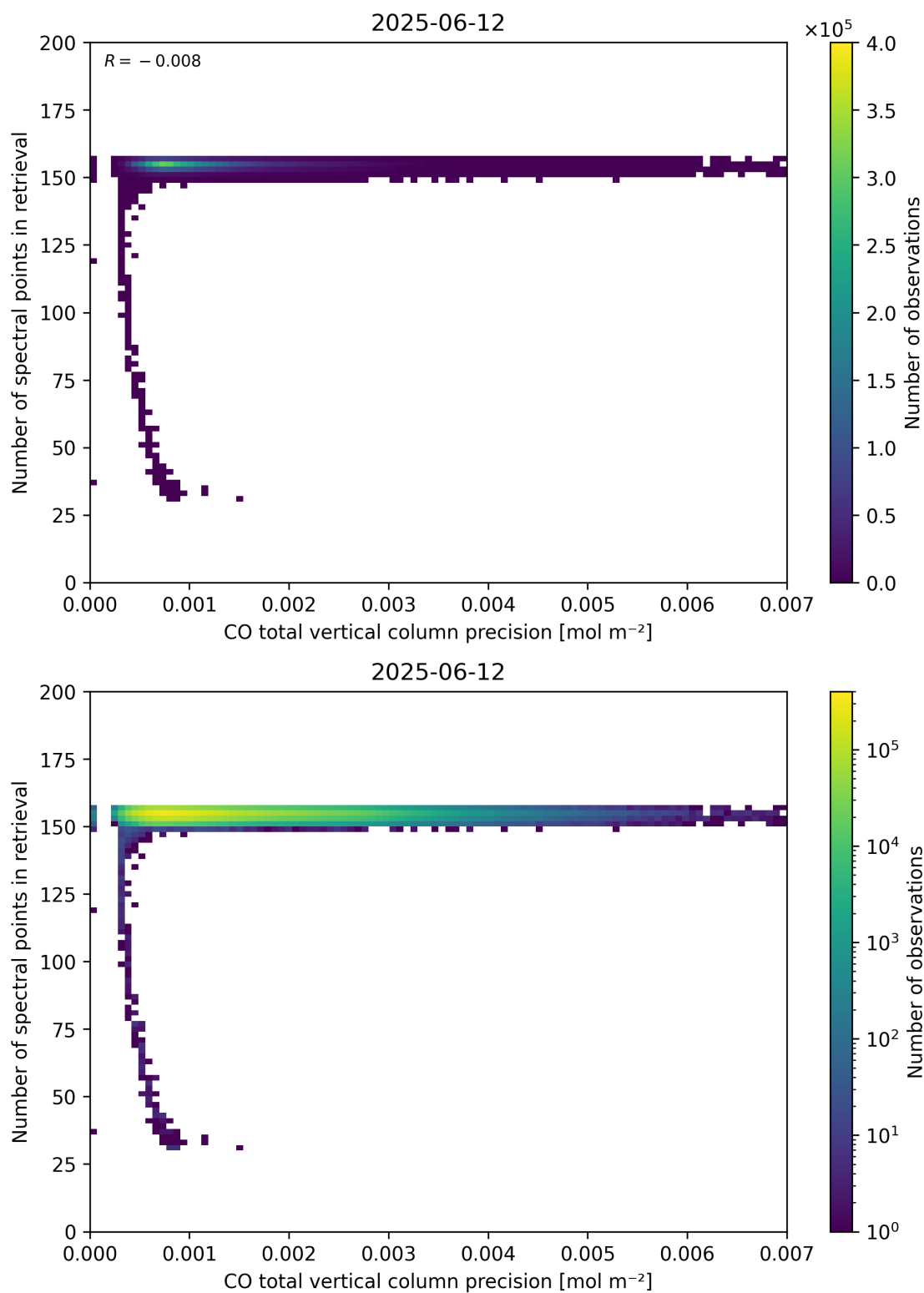
Figure 47: Scatter density plot of “CO total vertical column precision” against “Number of spectral points in retrieval” for 2025-06-11 to 2025-06-13.
