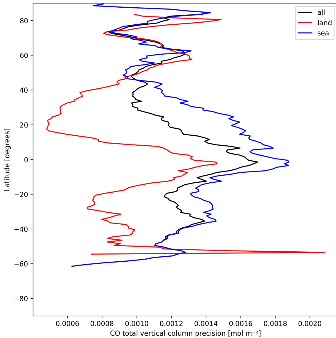
Figure 12: Zonal average of “CO total vertical column precision” for 2025-06-11 to 2025-06-13.
