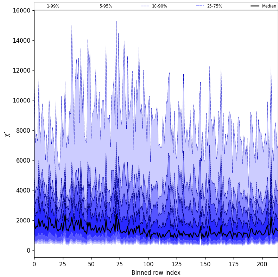
Figure 30: Along track statistics of “ \chi^2 ” for 2025-06-11 to 2025-06-13
