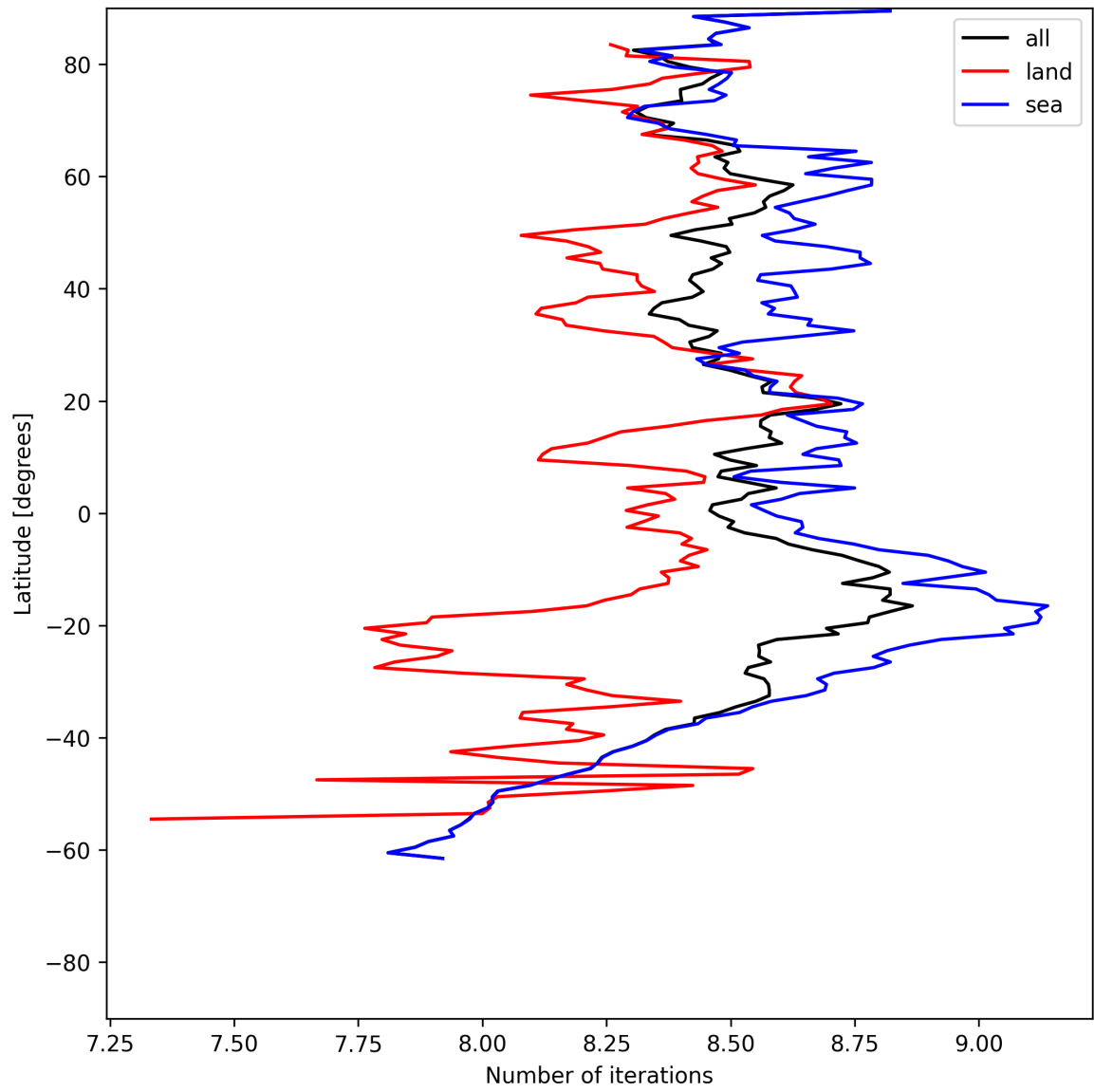
Figure 16: Zonal average of “Number of iterations” for 2025-06-11 to 2025-06-13.
