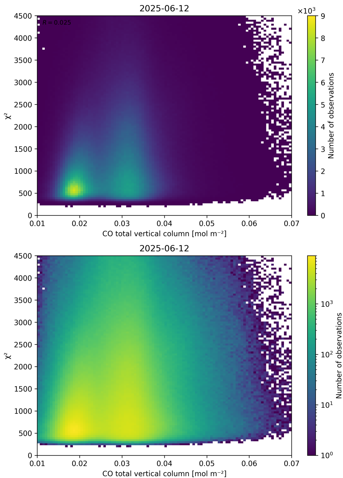
Figure 35: Scatter density plot of “CO total vertical column” against “ \chi^2 ” for 2025-06-11 to 2025-06-13.
