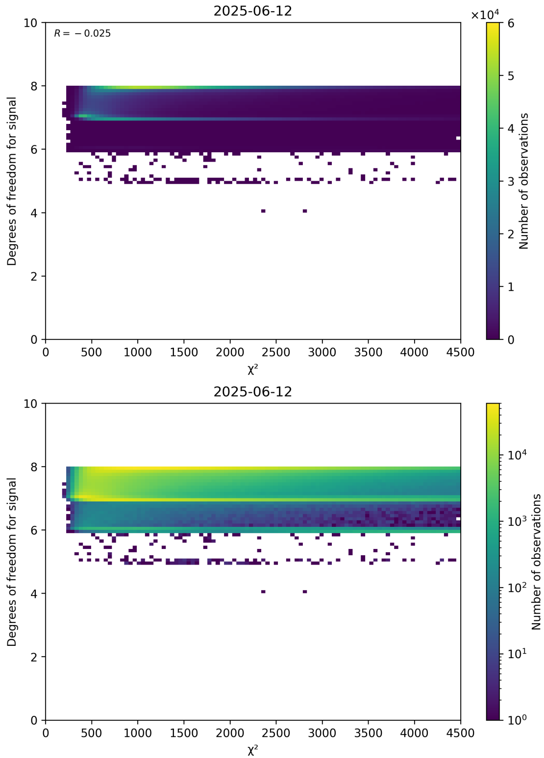
Figure 48: Scatter density plot of “ \chi^2 ” against “Degrees of freedom for signal” for 2025-06-11 to 2025-06-13.
