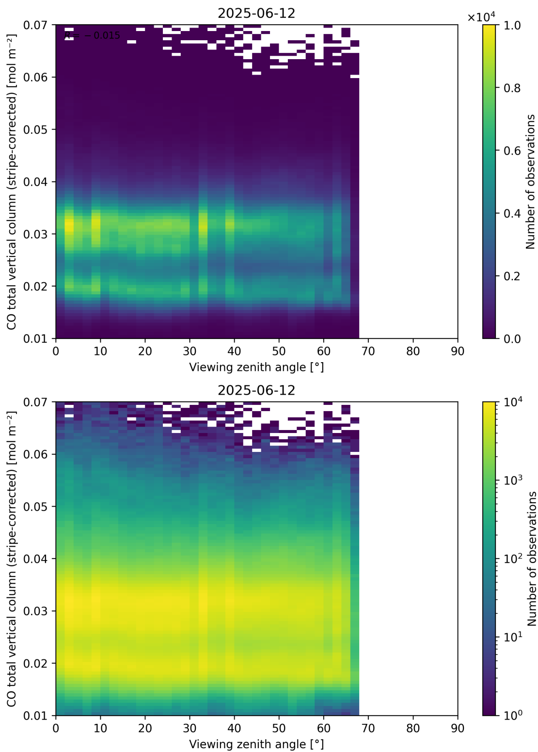
Figure 70: Scatter density plot of “Viewing zenith angle” against “CO total vertical column (stripe-corrected)” for 2025-06-11 to 2025-06-13.
