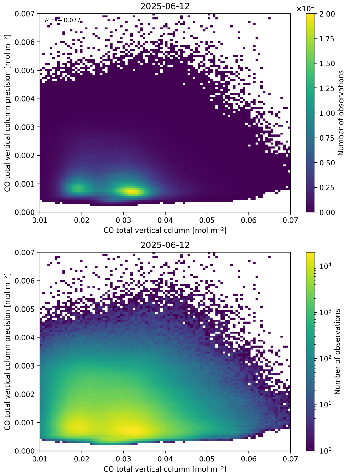
Figure 34: Scatter density plot of “CO total vertical column” against “CO total vertical column precision” for 2025-06-11 to 2025-06-13.
