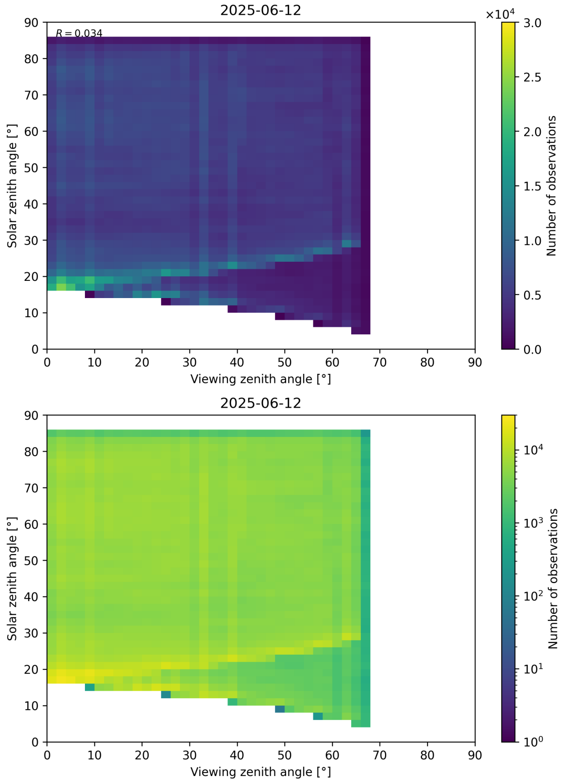
Figure 77: Scatter density plot of “Viewing zenith angle” against “Solar zenith angle” for 2025-06-11 to 2025-06-13.
