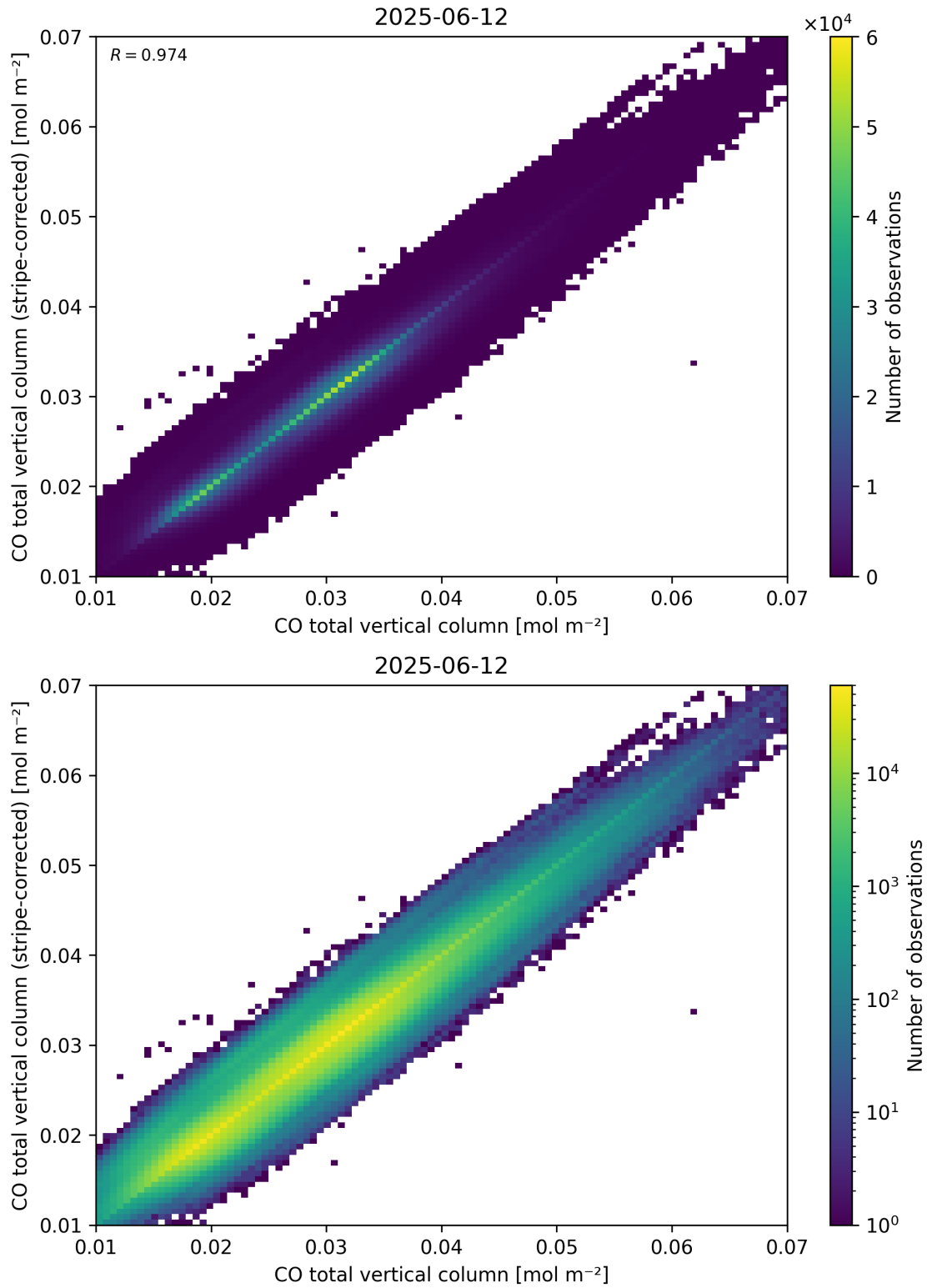
Figure 33: Scatter density plot of “CO total vertical column” against “CO total vertical column (stripe-corrected)” for 2025-06-11 to 2025-06-13.
