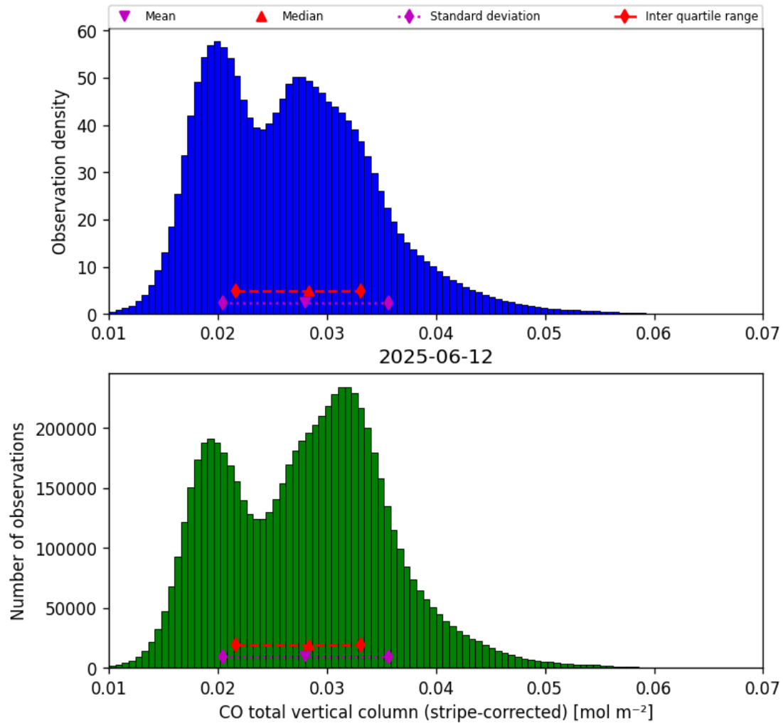
Figure 19: Histogram of “CO total vertical column (stripe-corrected)” for 2025-06-11 to 2025-06-13
