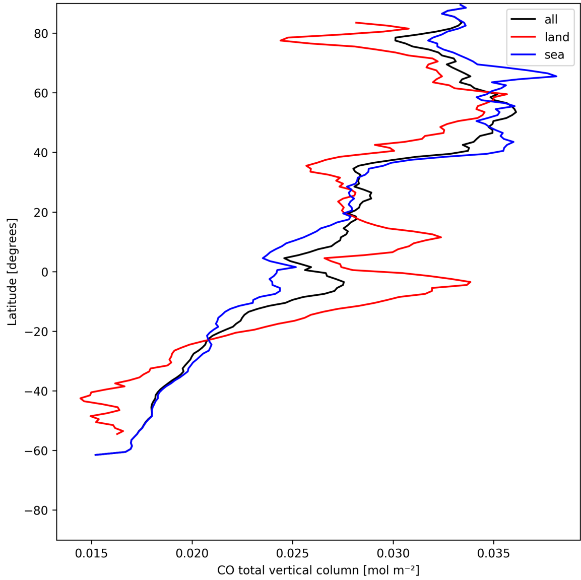
Figure 10: Zonal average of “CO total vertical column” for 2025-06-11 to 2025-06-13.
