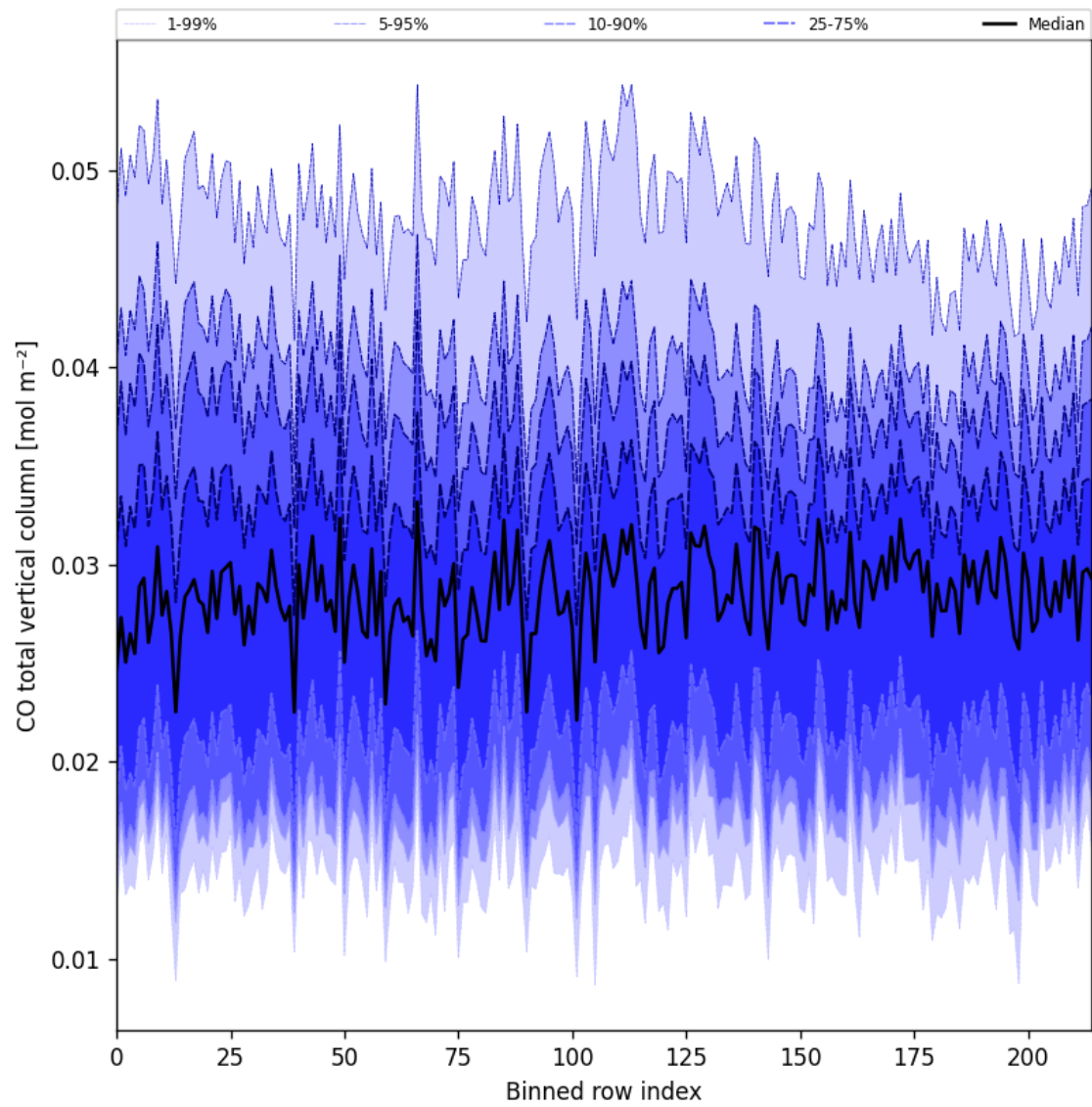
Figure 26: Along track statistics of “CO total vertical column” for 2025-06-11 to 2025-06-13
