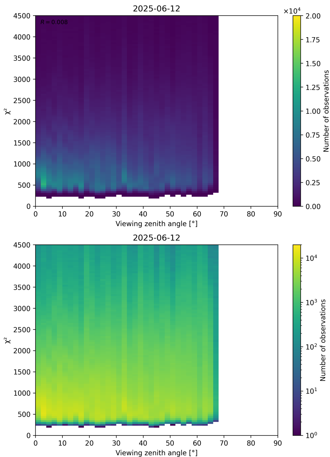
Figure 72: Scatter density plot of “Viewing zenith angle” against “ \chi^2 ” for 2025-06-11 to 2025-06-13.
