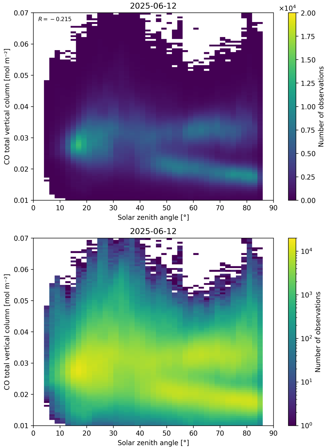
Figure 61: Scatter density plot of “Solar zenith angle” against “CO total vertical column” for 2025-06-11 to 2025-06-13.
