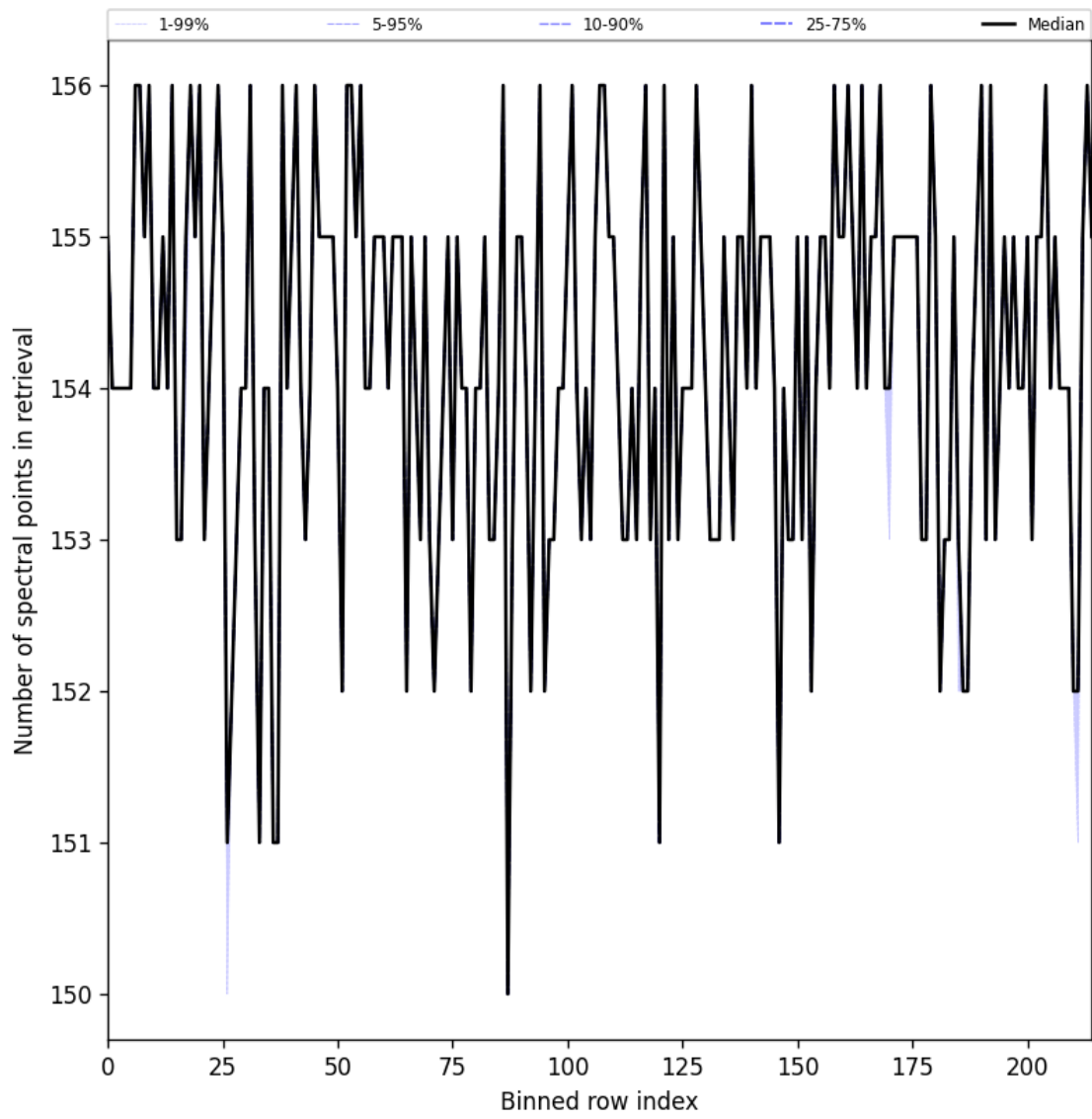
Figure 29: Along track statistics of “Number of spectral points in retrieval” for 2025-06-11 to 2025-06-13
