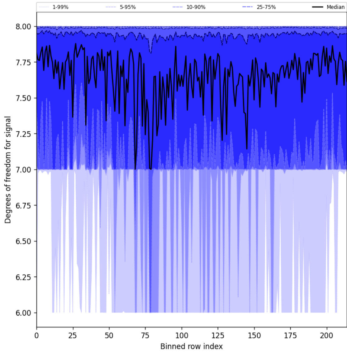
Figure 31: Along track statistics of “Degrees of freedom for signal” for 2025-06-11 to 2025-06-13
