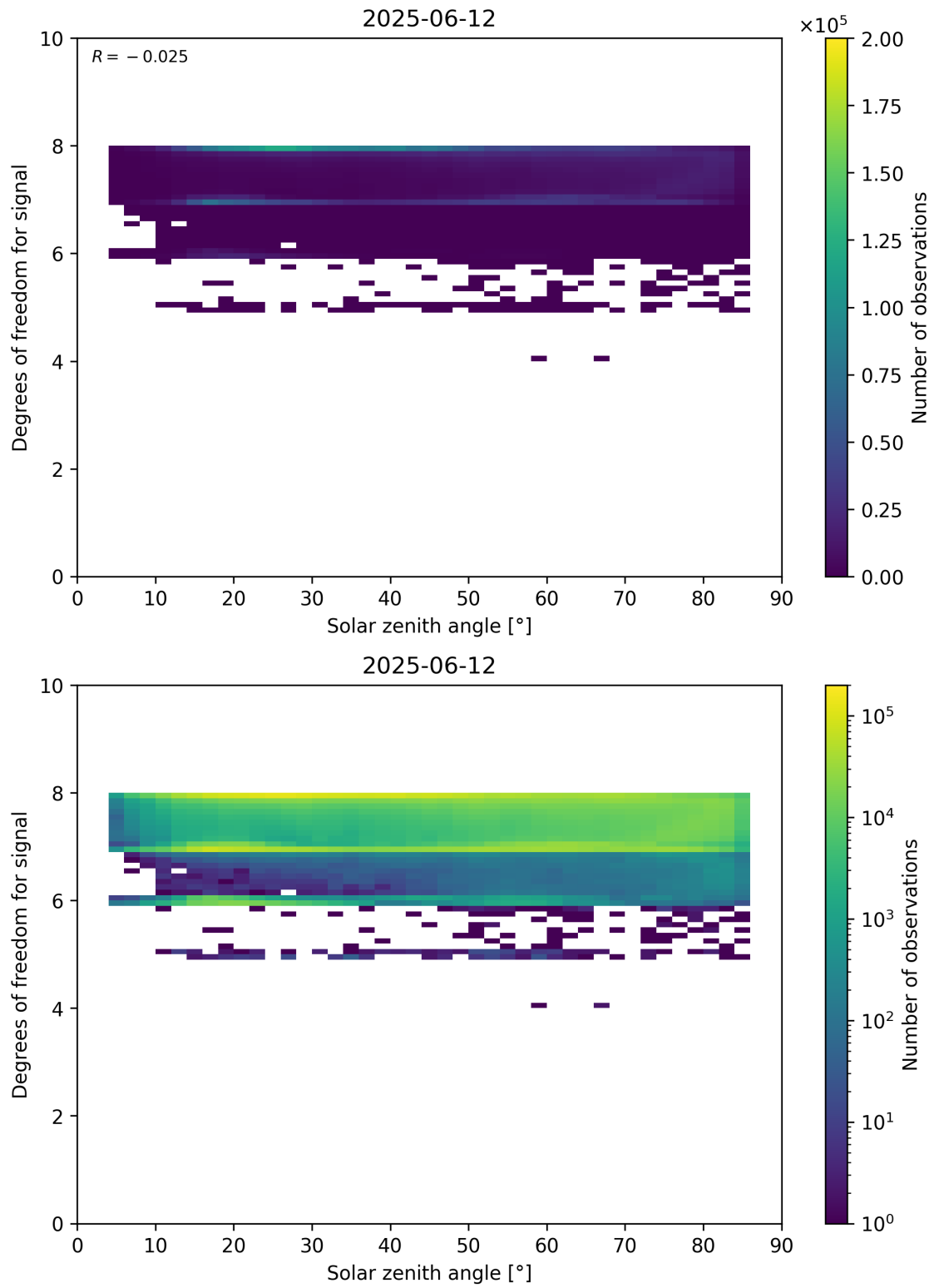
Figure 65: Scatter density plot of “Solar zenith angle” against “Degrees of freedom for signal” for 2025-06-11 to 2025-06-13.
