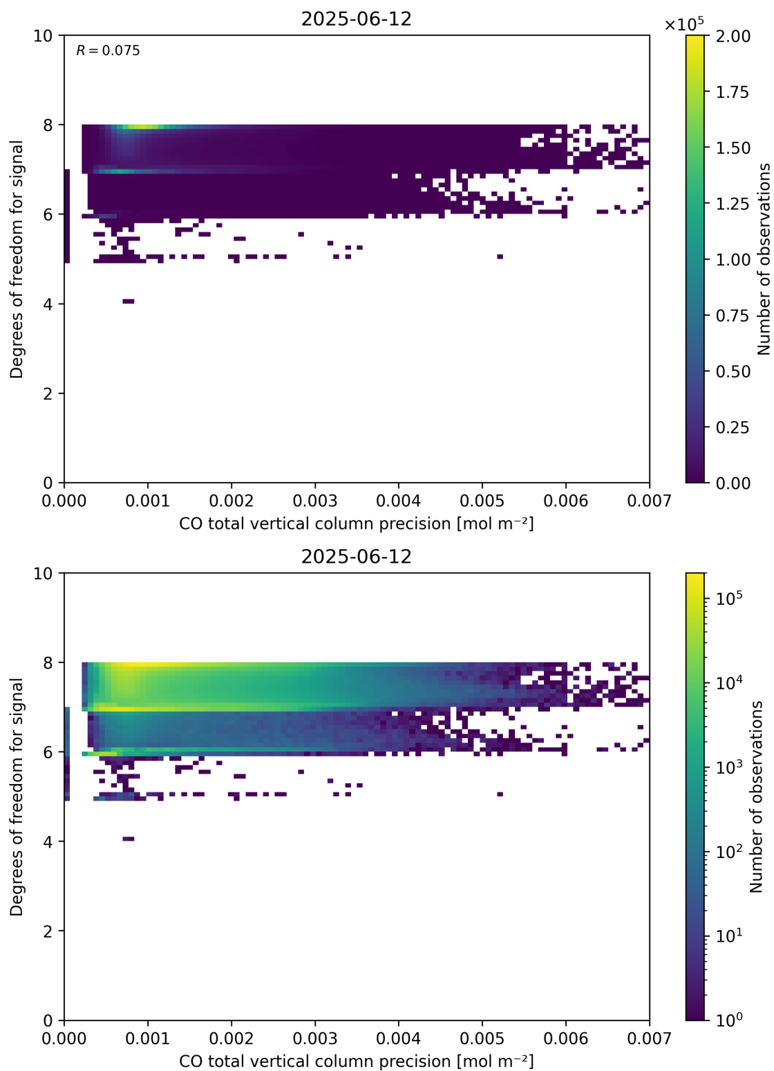
Figure 45: Scatter density plot of “CO total vertical column precision” against “Degrees of freedom for signal” for 2025-06-11 to 2025-06-13.
