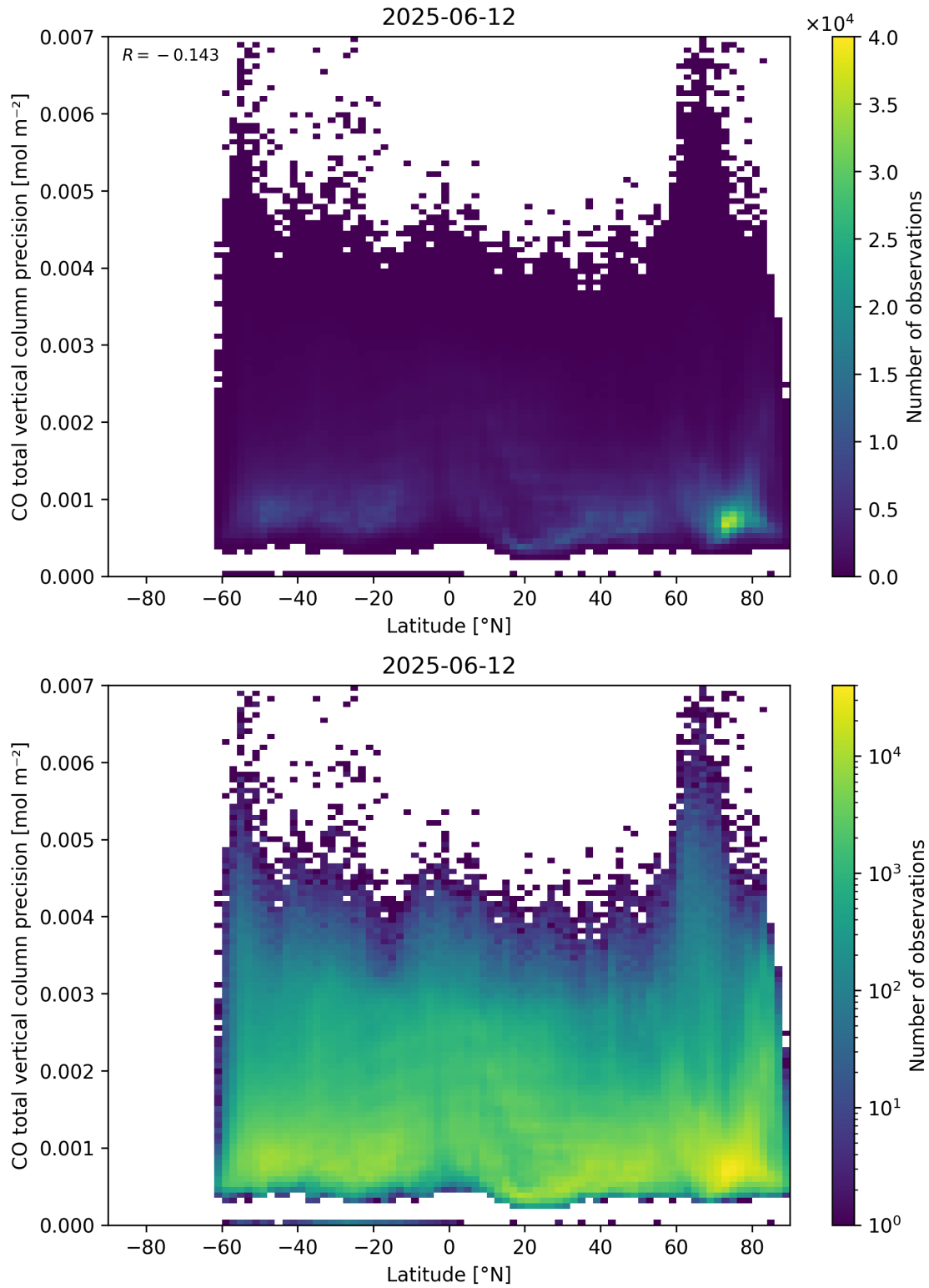
Figure 53: Scatter density plot of “Latitude” against “CO total vertical column precision” for 2025-06-11 to 2025-06-13.
