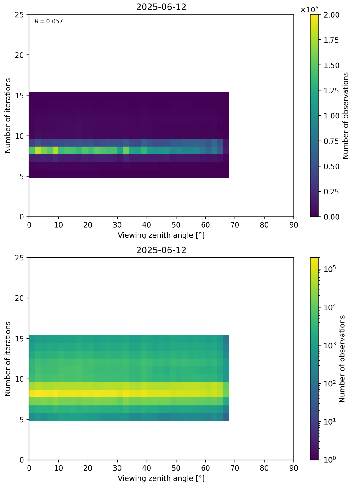
Figure 75: Scatter density plot of “Viewing zenith angle” against “Number of iterations” for 2025-06-11 to 2025-06-13.
