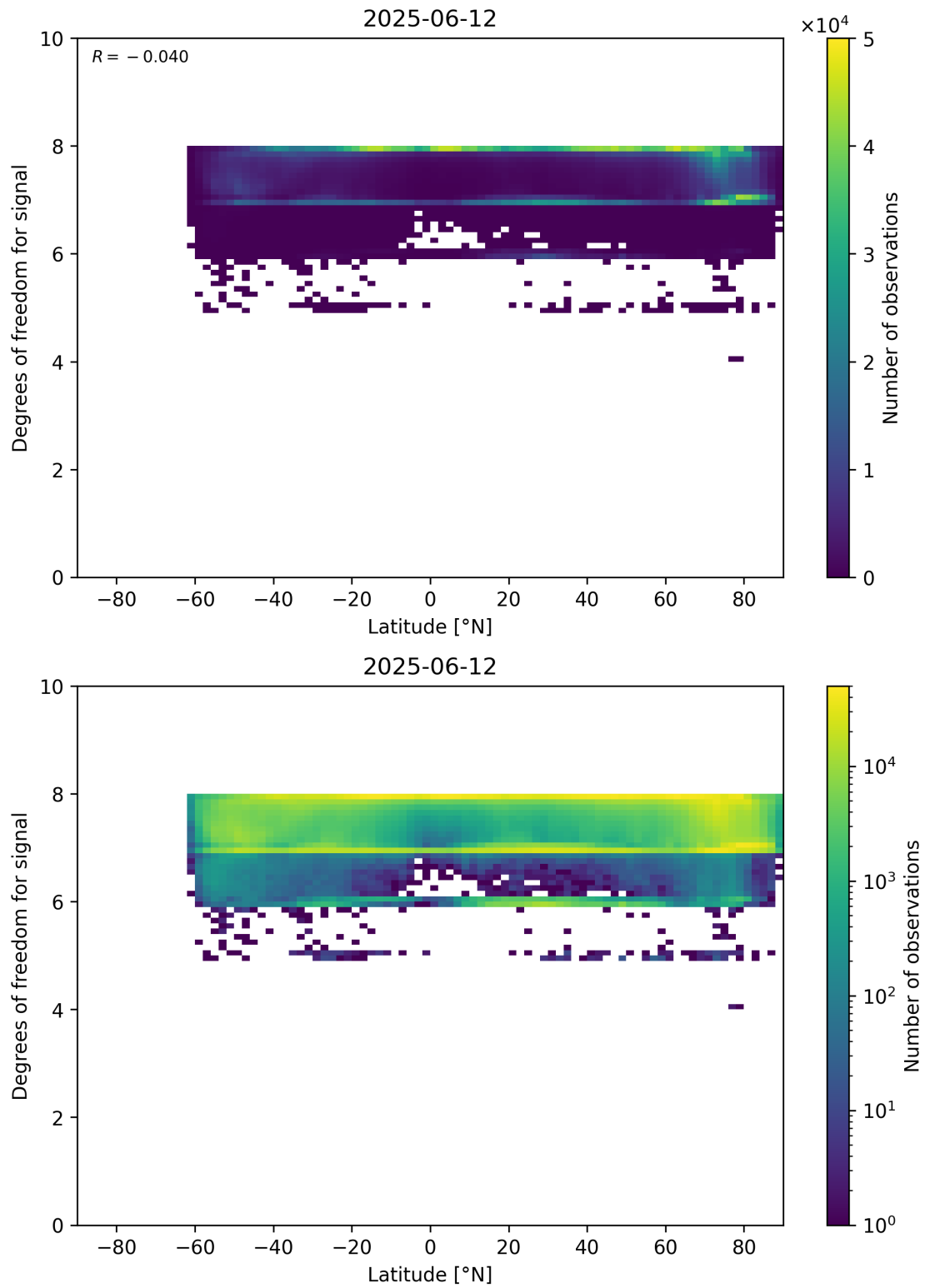
Figure 55: Scatter density plot of “Latitude” against “Degrees of freedom for signal” for 2025-06-11 to 2025-06-13.
