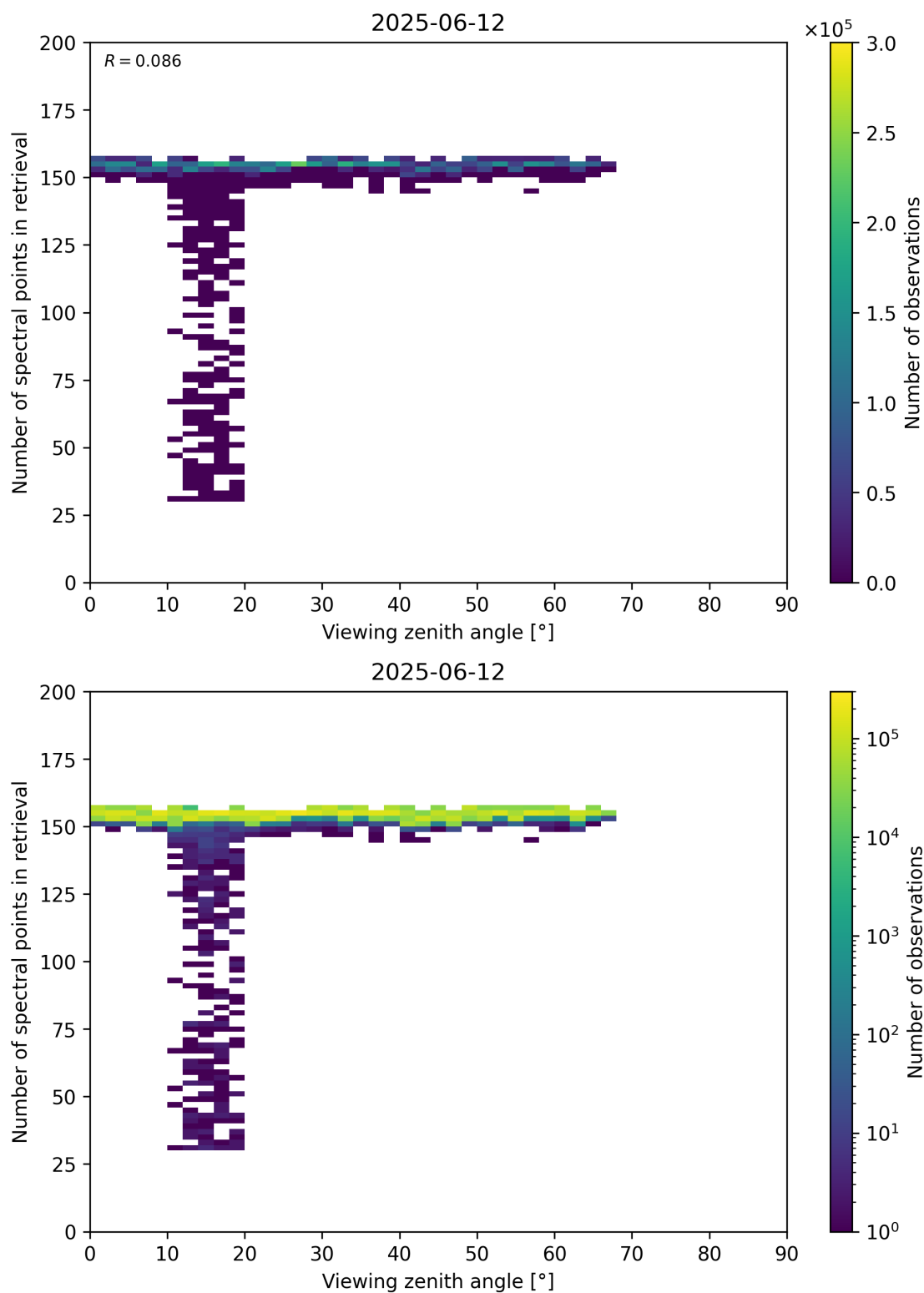
Figure 76: Scatter density plot of “Viewing zenith angle” against “Number of spectral points in retrieval” for 2025-06-11 to 2025-06-13.
