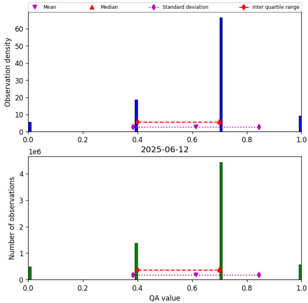
Figure 17: Histogram of “QA value” for 2025-06-11 to 2025-06-13
