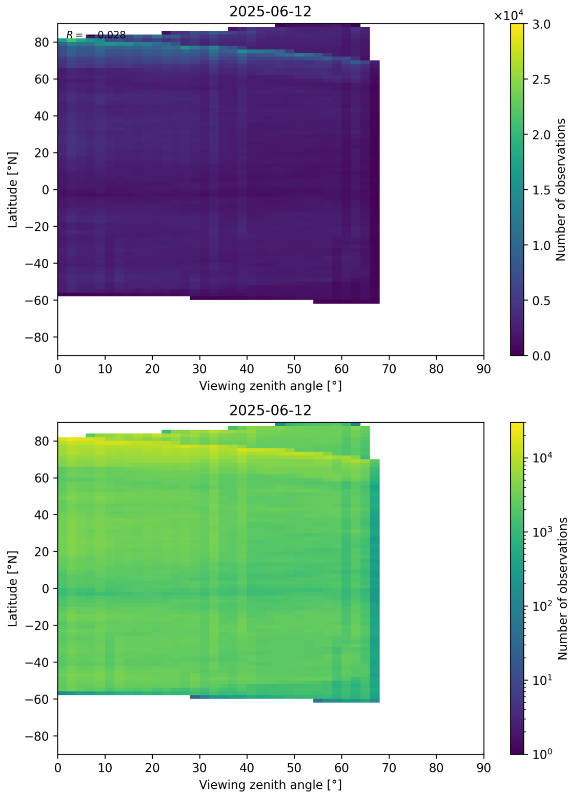
Figure 74: Scatter density plot of “Viewing zenith angle” against “Latitude” for 2025-06-11 to 2025-06-13.
