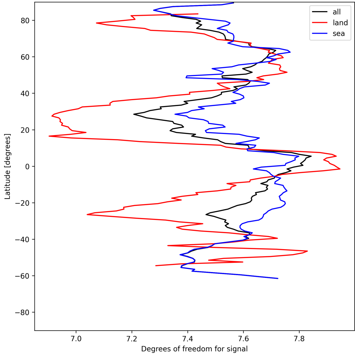
Figure 15: Zonal average of “Degrees of freedom for signal” for 2025-06-11 to 2025-06-13.
