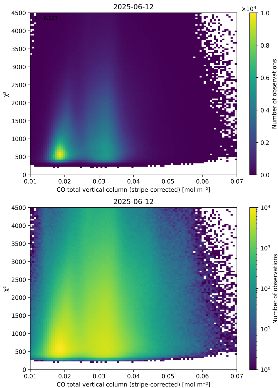
Figure 37: Scatter density plot of “CO total vertical column (stripe-corrected)” against “ \chi^2 ” for 2025-06-11 to 2025-06-13.
