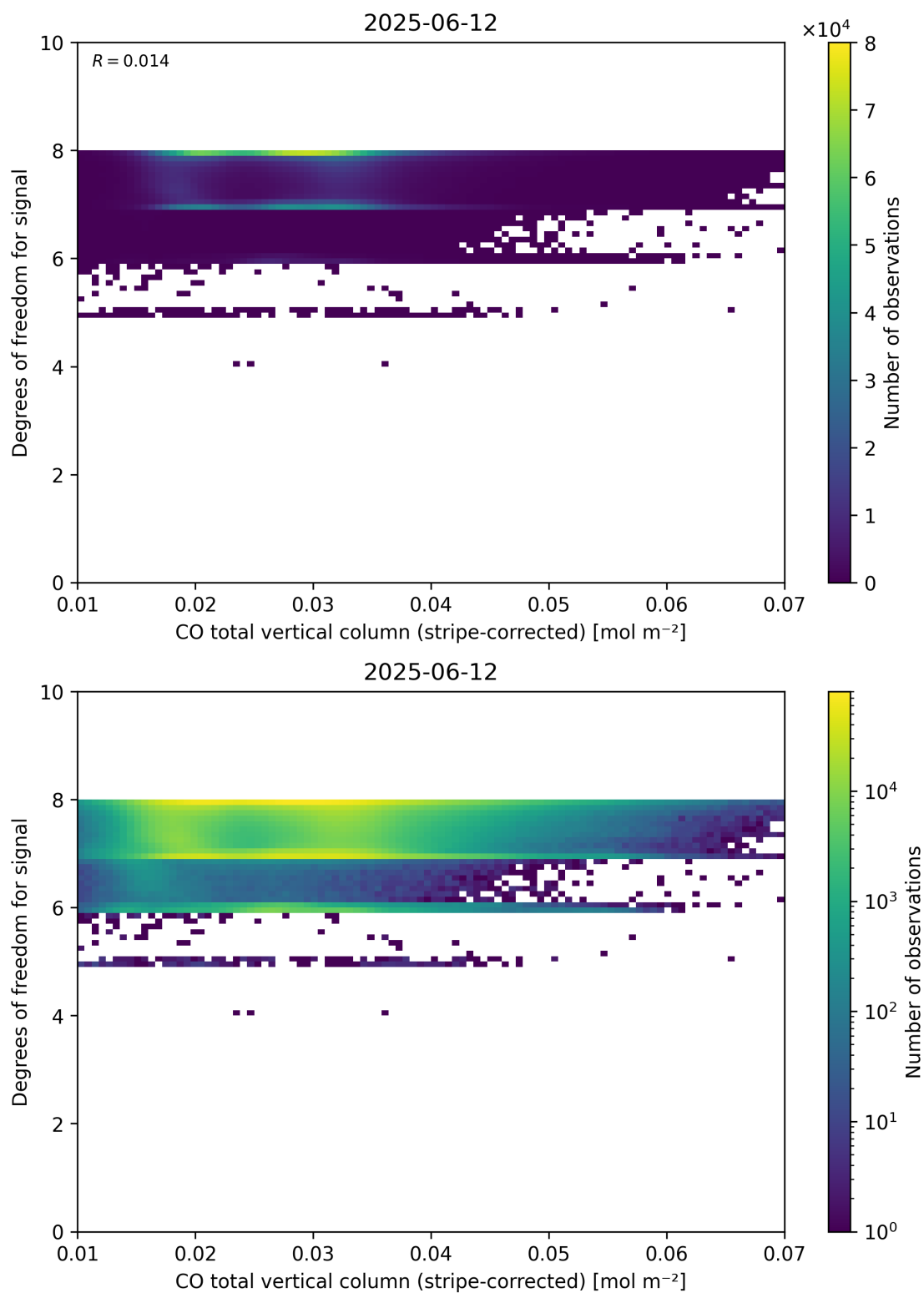
Figure 38: Scatter density plot of “CO total vertical column (stripe-corrected)” against “Degrees of freedom for signal” for 2025-06-11 to 2025-06-13.
