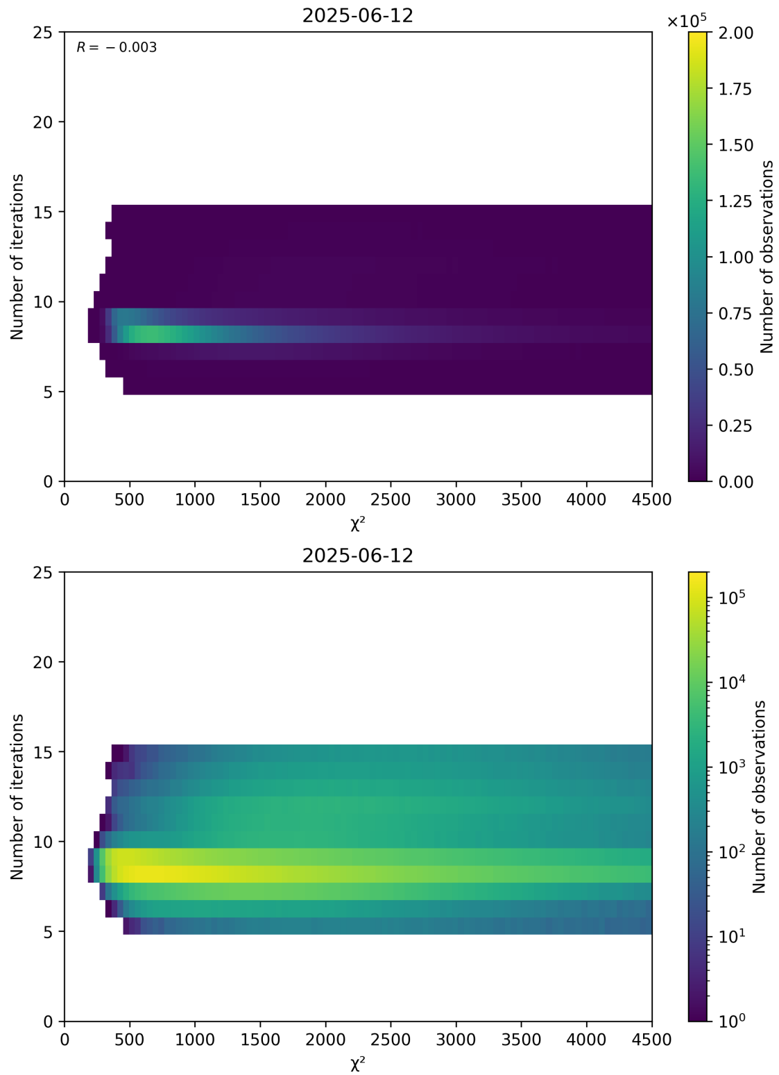
Figure 49: Scatter density plot of “ \chi^2 ” against “Number of iterations” for 2025-06-11 to 2025-06-13.
