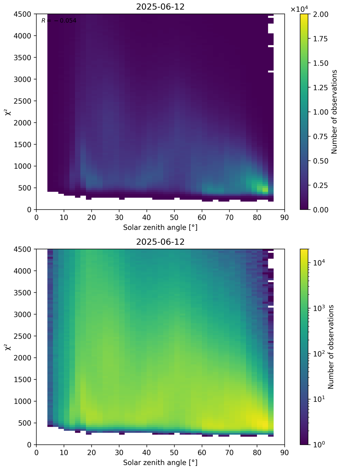
Figure 64: Scatter density plot of “Solar zenith angle” against “ \chi^2 ” for 2025-06-11 to 2025-06-13.
