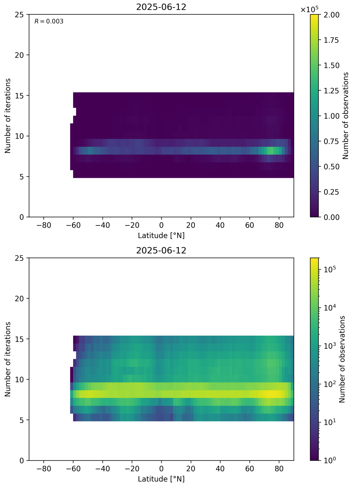
Figure 56: Scatter density plot of “Latitude” against “Number of iterations” for 2025-06-11 to 2025-06-13.
