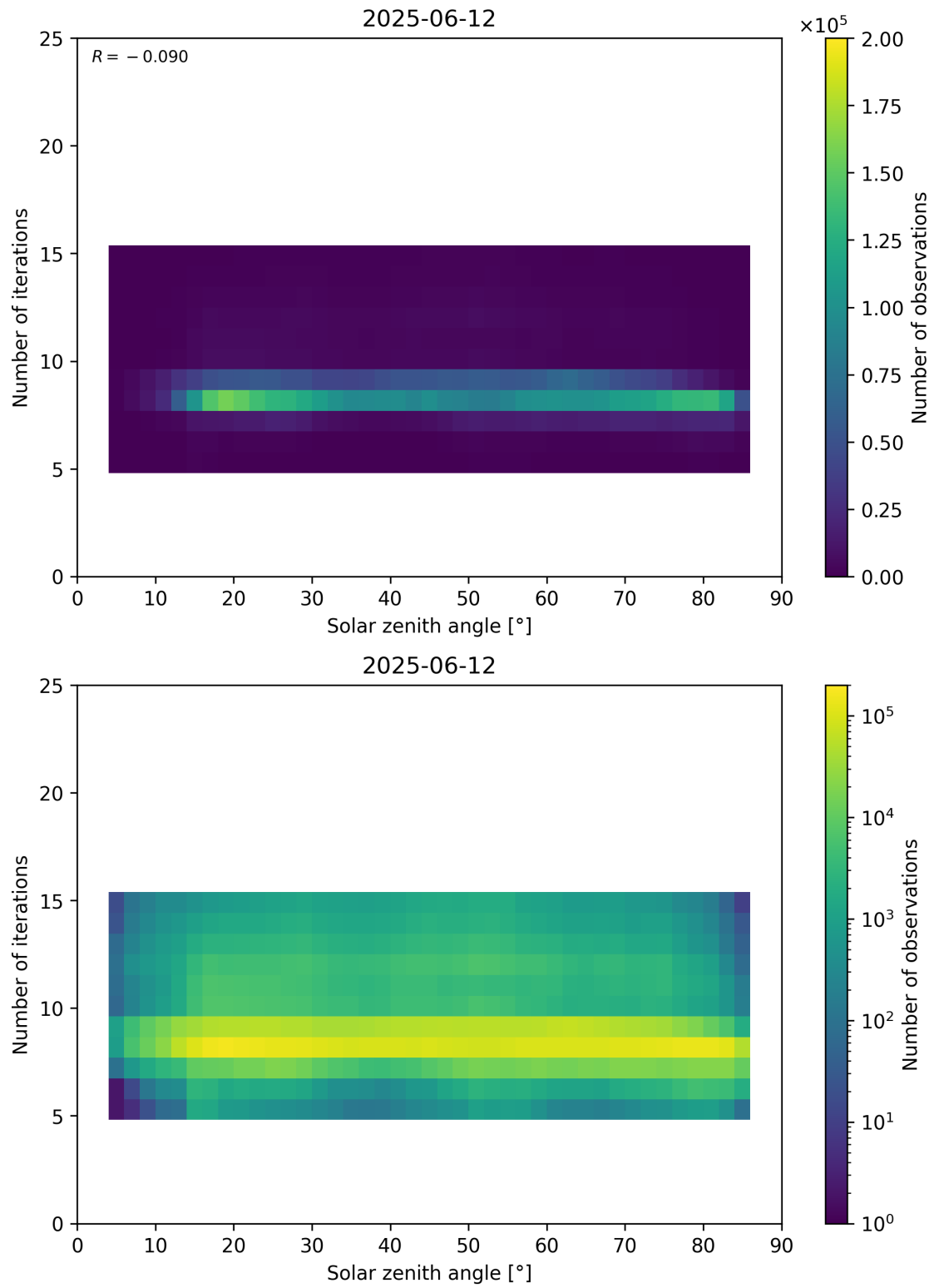
Figure 67: Scatter density plot of “Solar zenith angle” against “Number of iterations” for 2025-06-11 to 2025-06-13.
