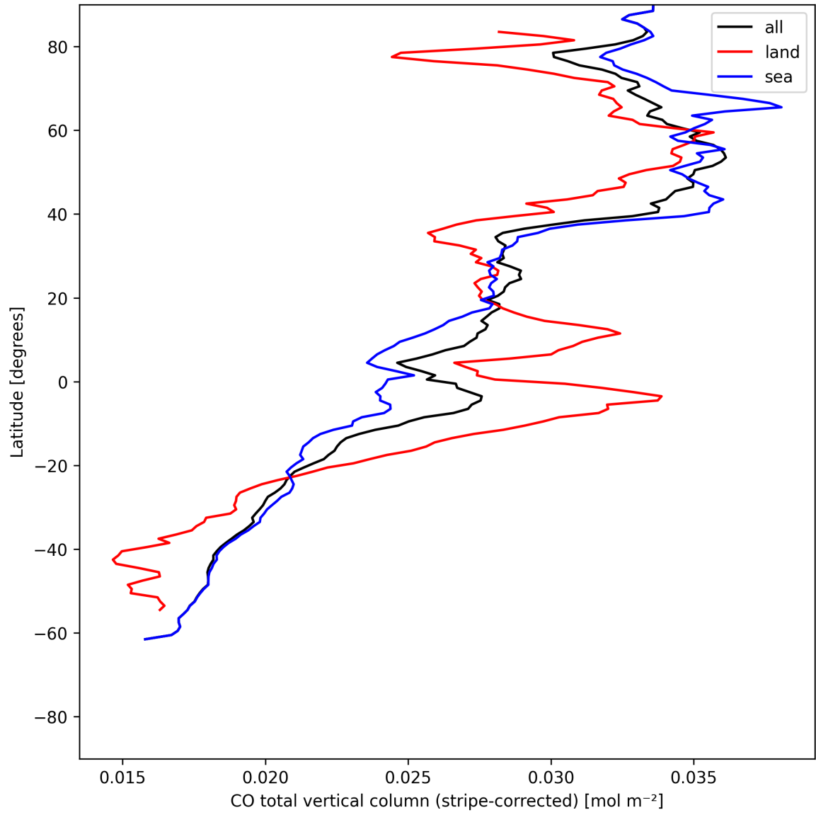
Figure 11: Zonal average of “CO total vertical column (stripe-corrected)” for 2025-06-11 to 2025-06-13.
