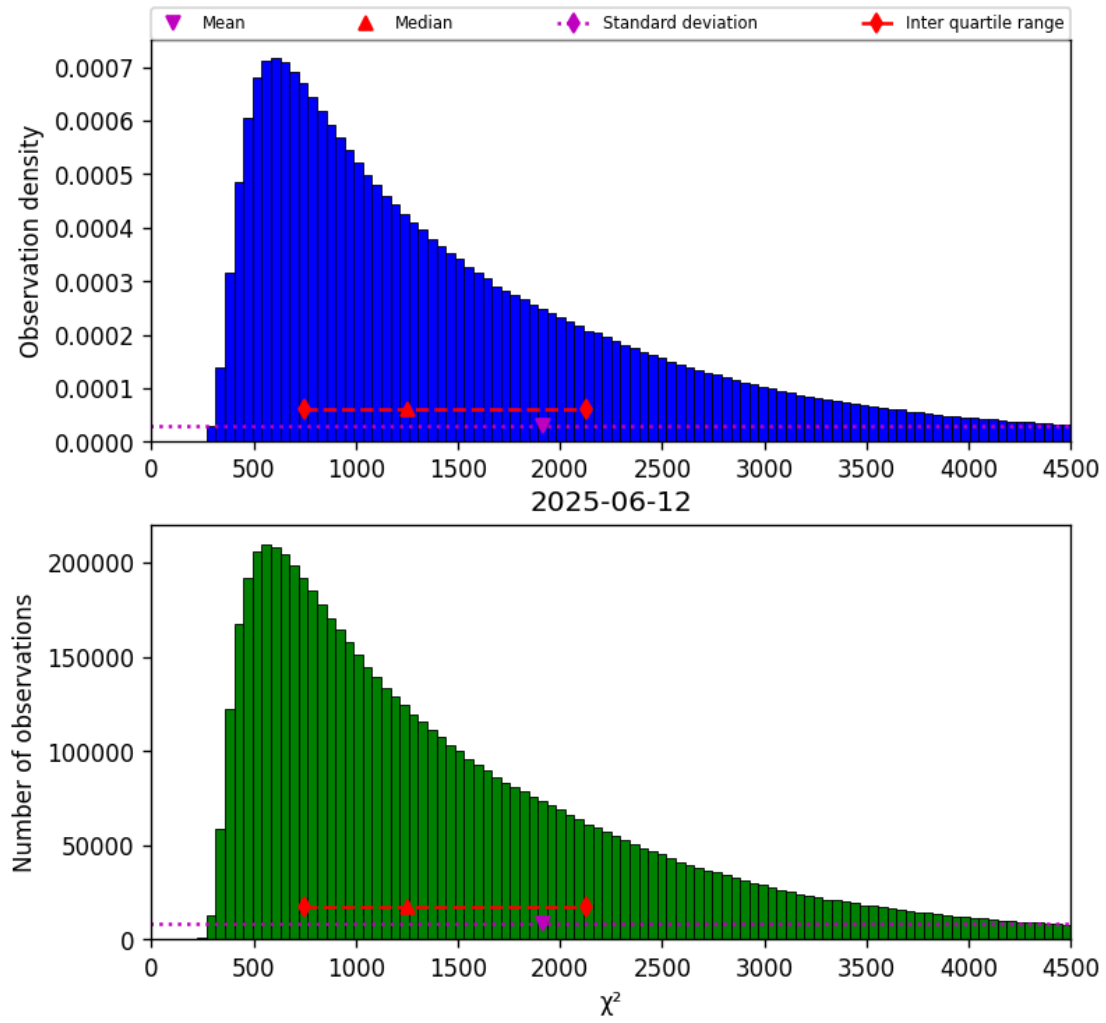
Figure 22: Histogram of “ \chi^2 ” for 2025-06-11 to 2025-06-13
