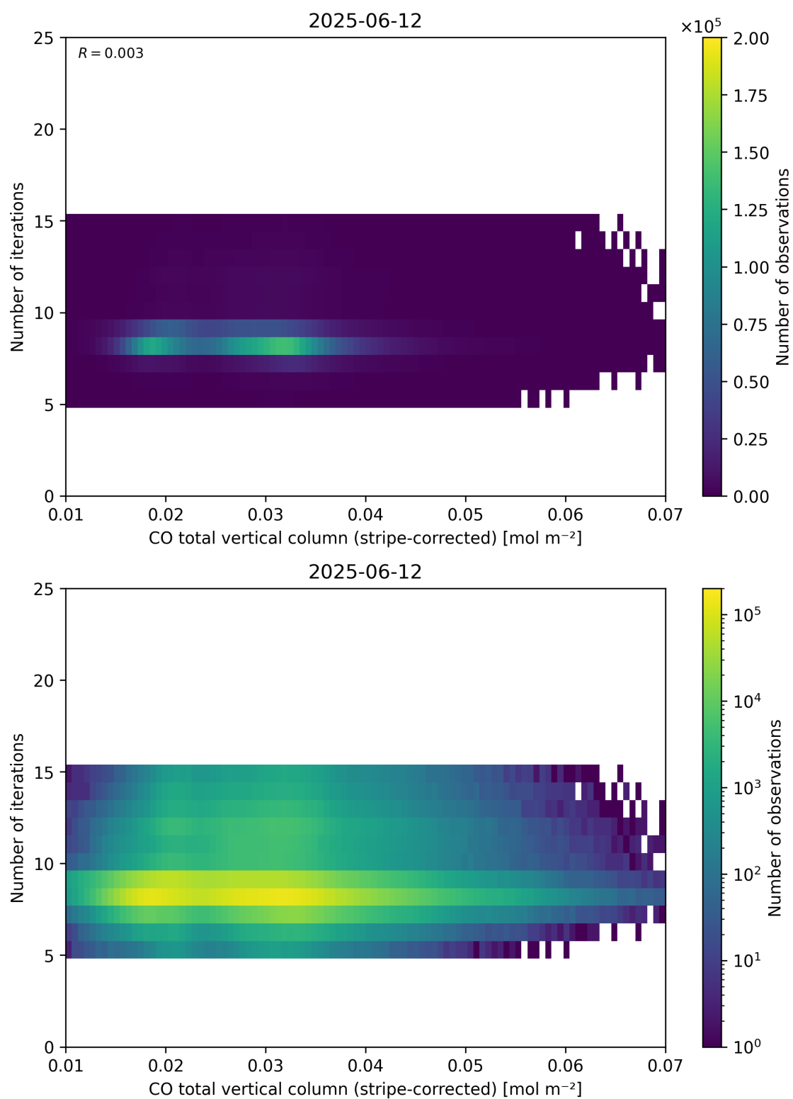
Figure 39: Scatter density plot of “CO total vertical column (stripe-corrected)” against “Number of iterations” for 2025-06-11 to 2025-06-13.
