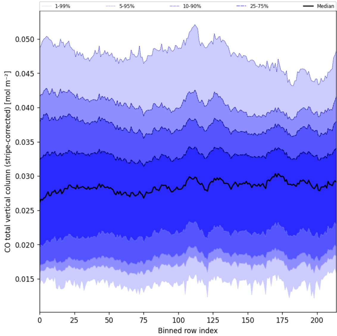
Figure 27: Along track statistics of “CO total vertical column (stripe-corrected)” for 2025-06-11 to 2025-06-13
