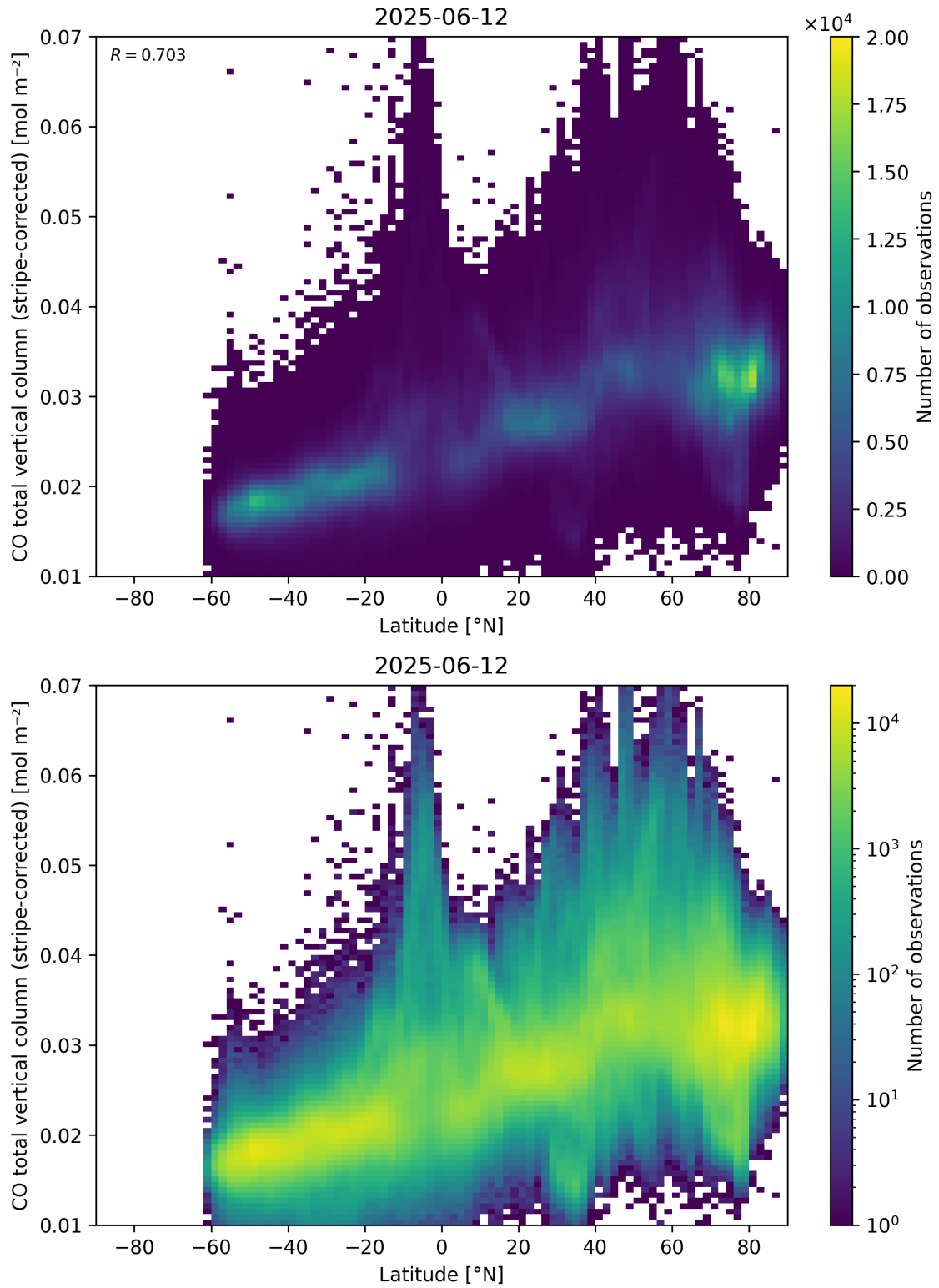
Figure 52: Scatter density plot of “Latitude” against “CO total vertical column (stripe-corrected)” for 2025-06-11 to 2025-06-13.
