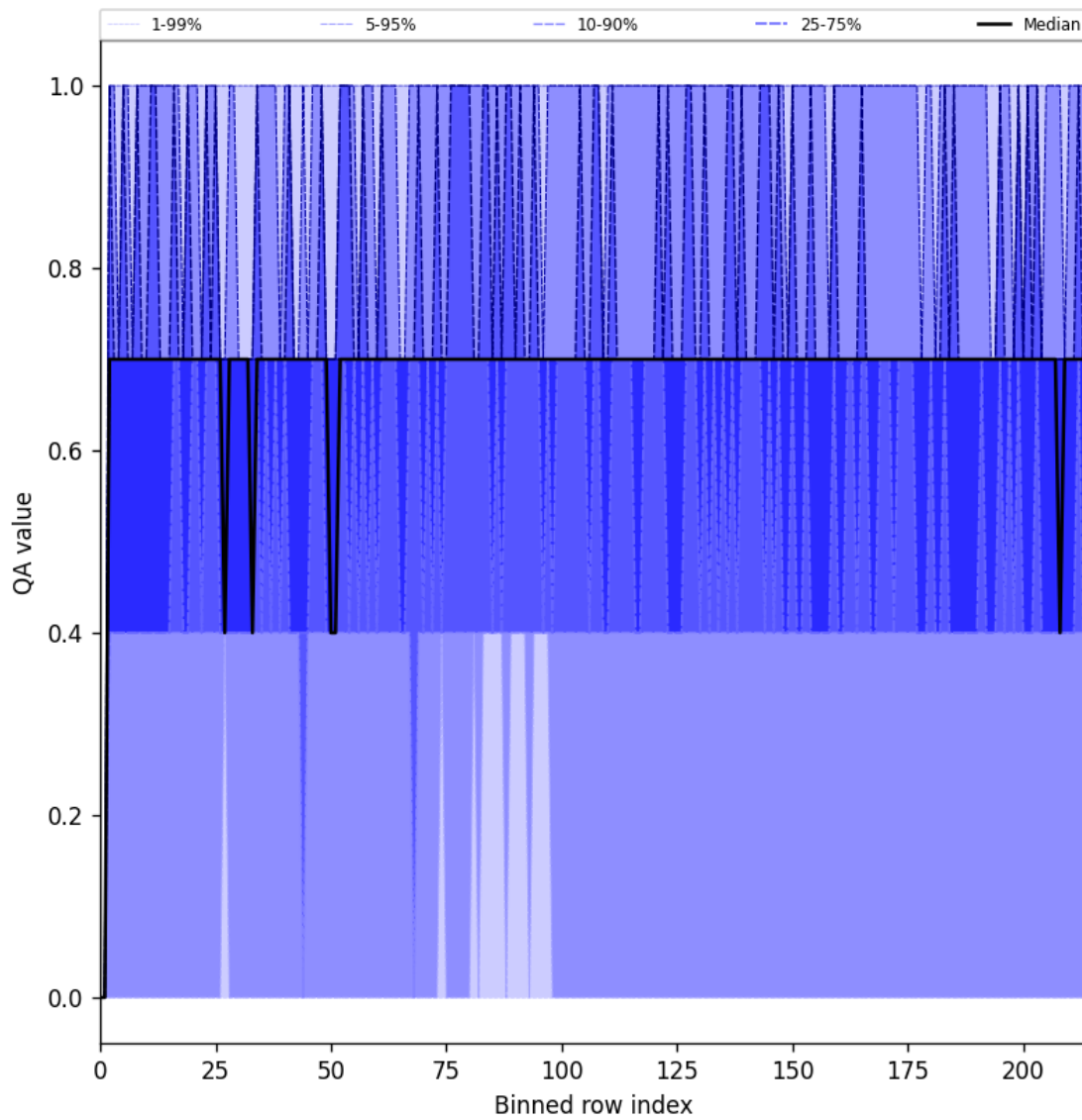
Figure 25: Along track statistics of “QA value” for 2025-06-11 to 2025-06-13
