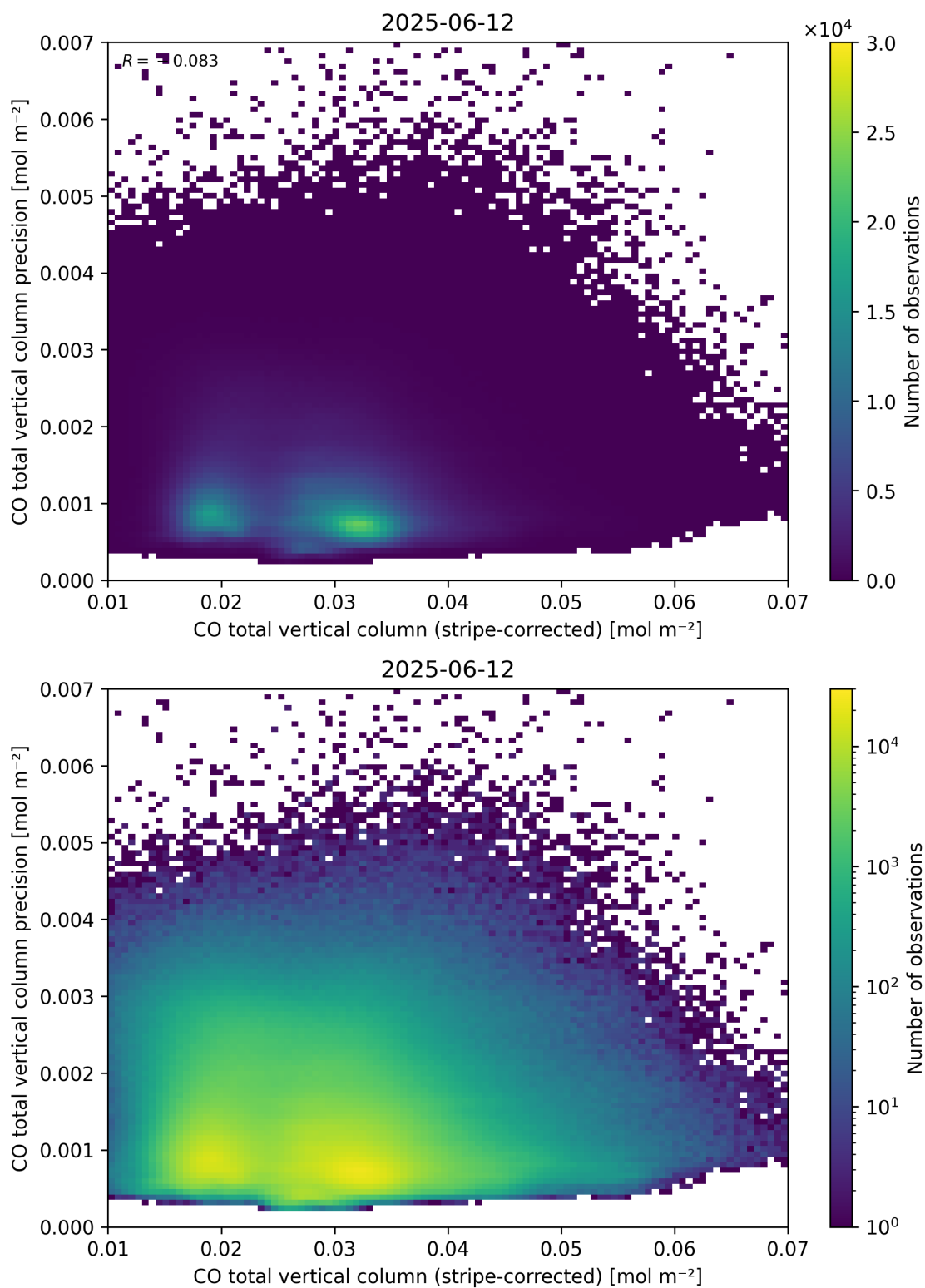
Figure 36: Scatter density plot of “CO total vertical column (stripe-corrected)” against “CO total vertical column precision” for 2025-06-11 to 2025-06-13.
