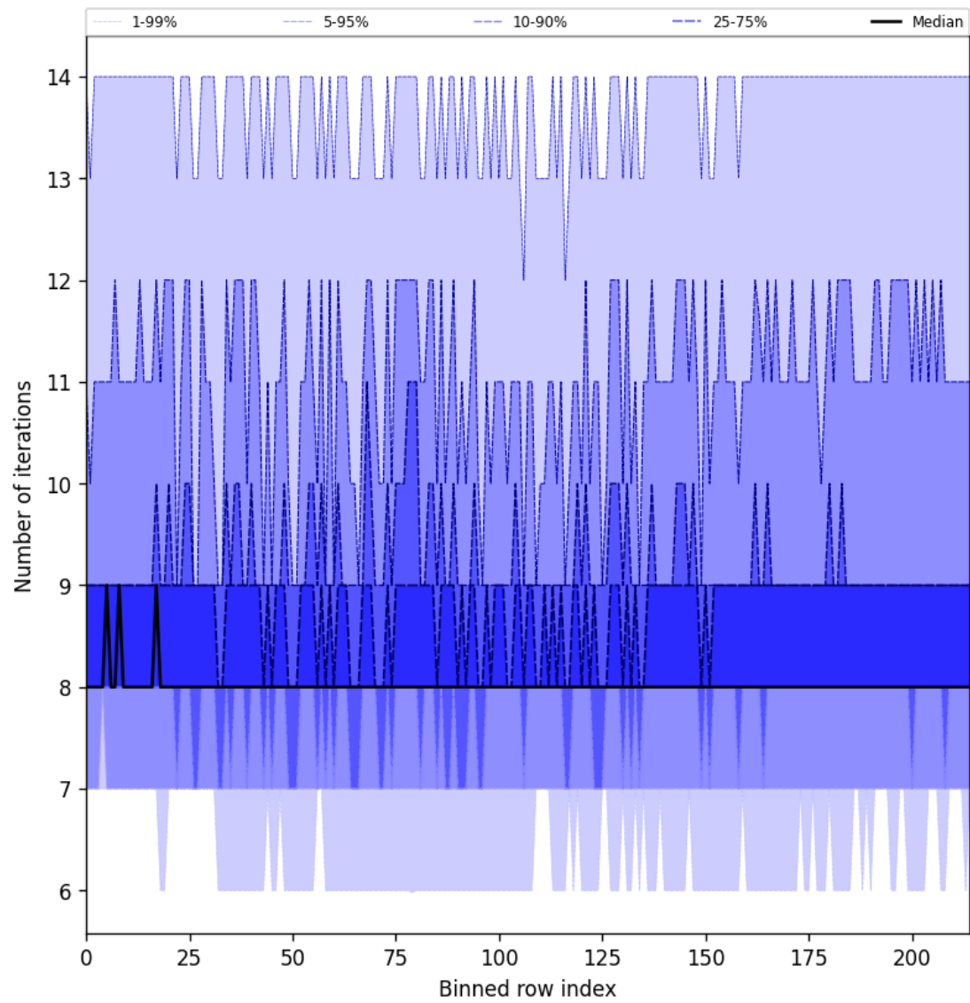
Figure 32: Along track statistics of “Number of iterations” for 2025-06-11 to 2025-06-13
