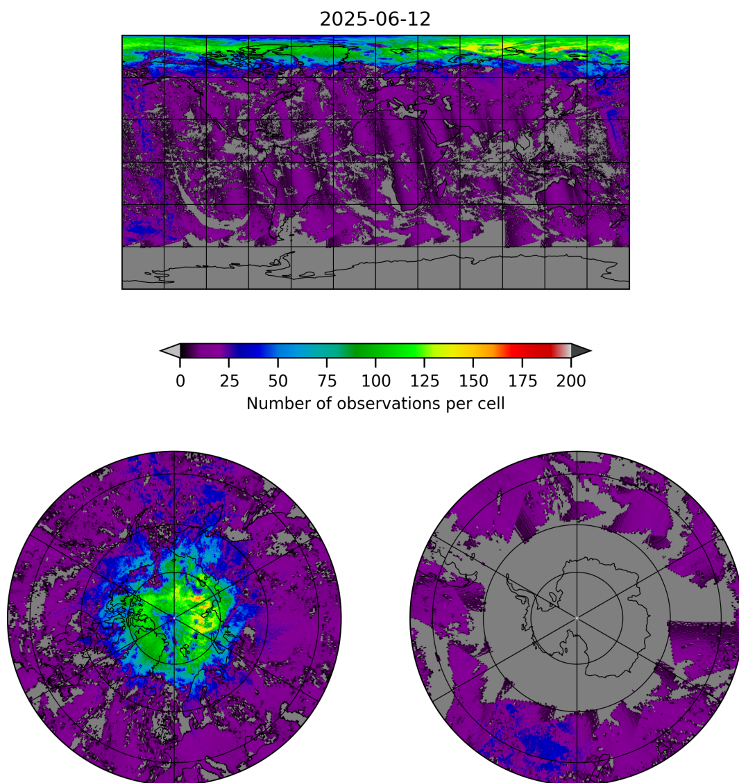
Figure 8: Map of the number of observations for 2025-06-11 to 2025-06-13
