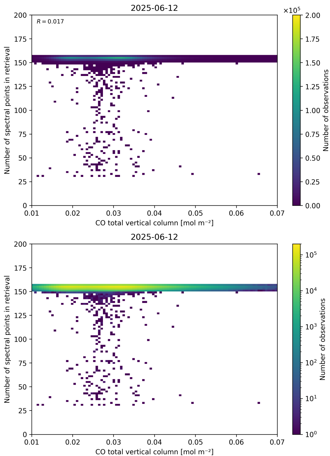
Figure 43: Scatter density plot of “CO total vertical column” against “Number of spectral points in retrieval” for 2025-06-11 to 2025-06-13.
