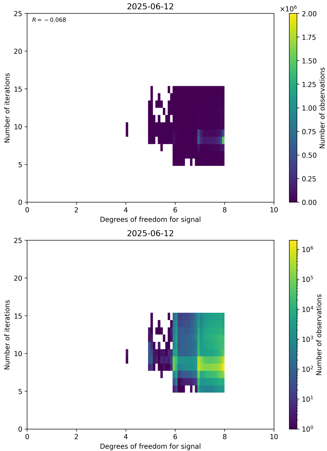
Figure 50: Scatter density plot of “Degrees of freedom for signal” against “Number of iterations” for 2025-06-11 to 2025-06-13.
