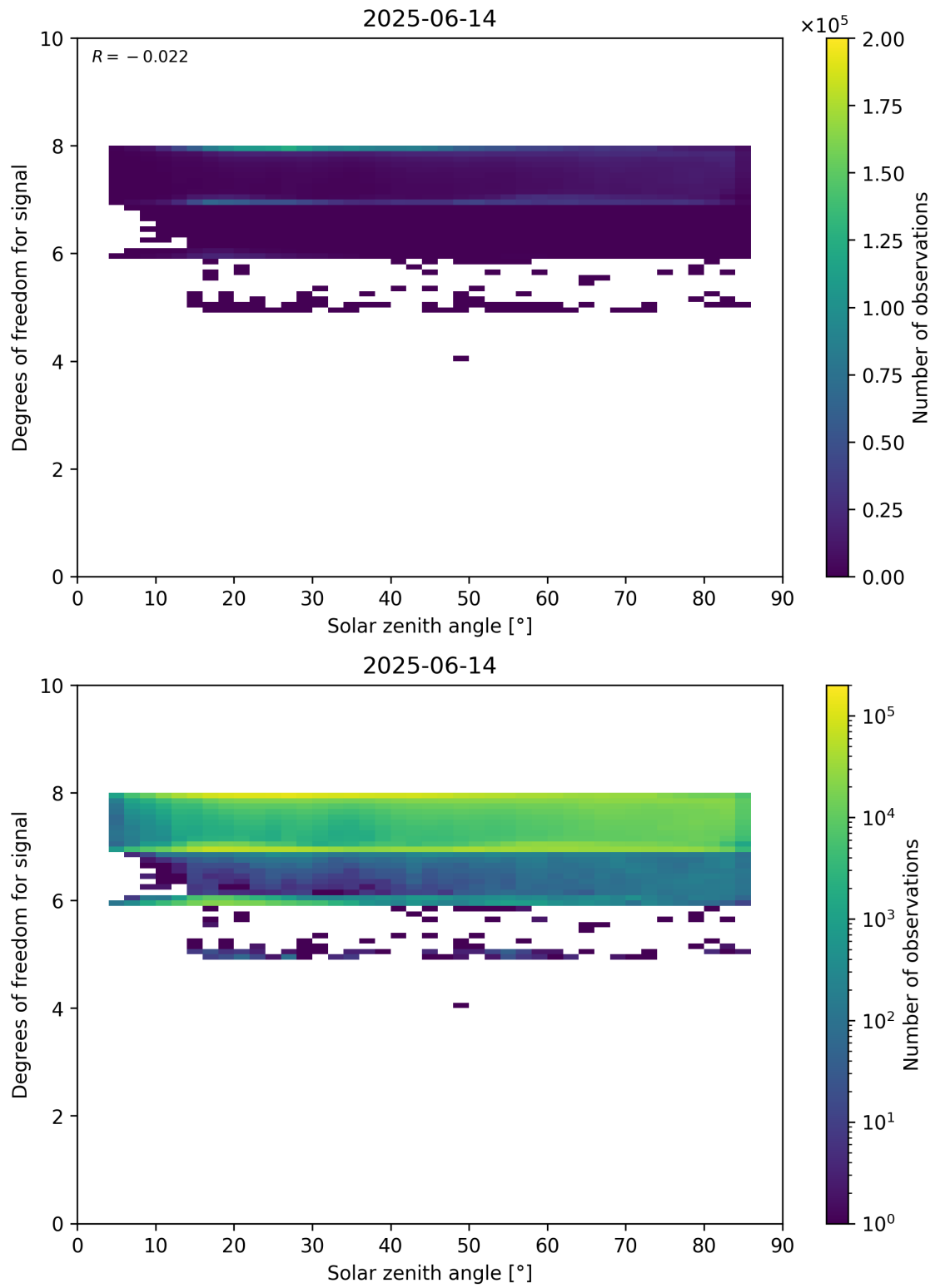
Figure 65: Scatter density plot of “Solar zenith angle” against “Degrees of freedom for signal” for 2025-06-13 to 2025-06-15.
