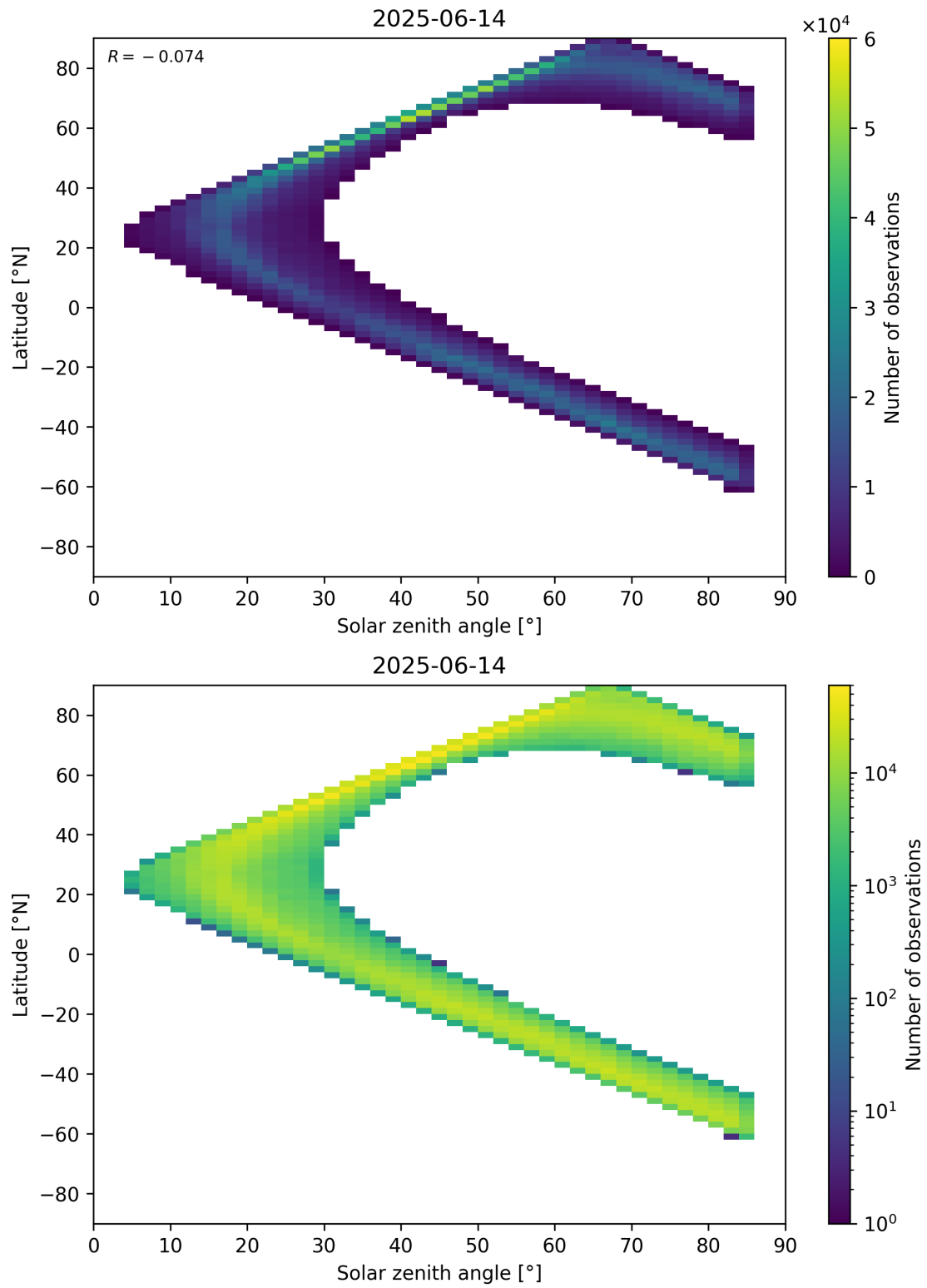
Figure 66: Scatter density plot of “Solar zenith angle” against “Latitude” for 2025-06-13 to 2025-06-15.
