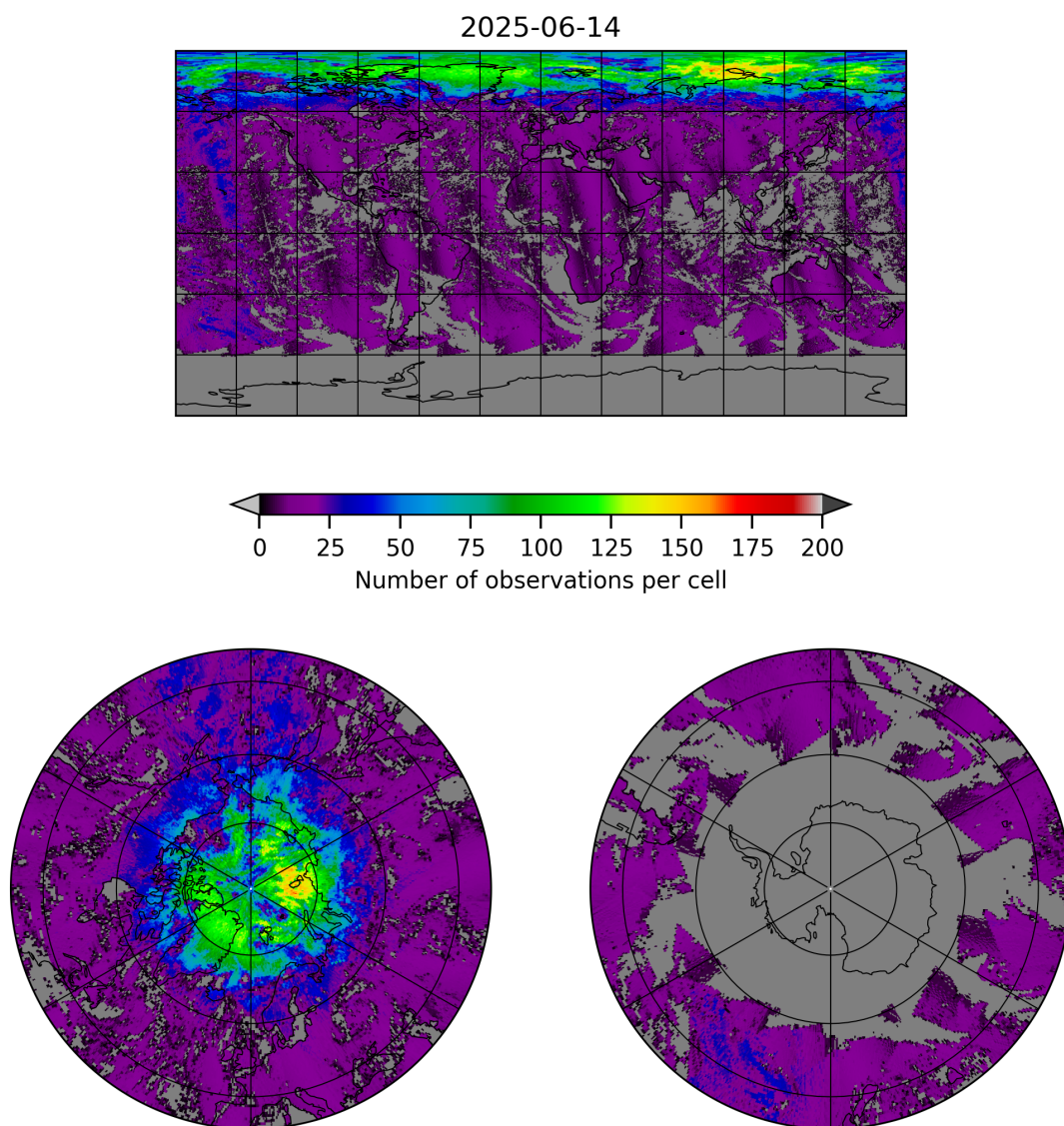
Figure 8: Map of the number of observations for 2025-06-13 to 2025-06-15
