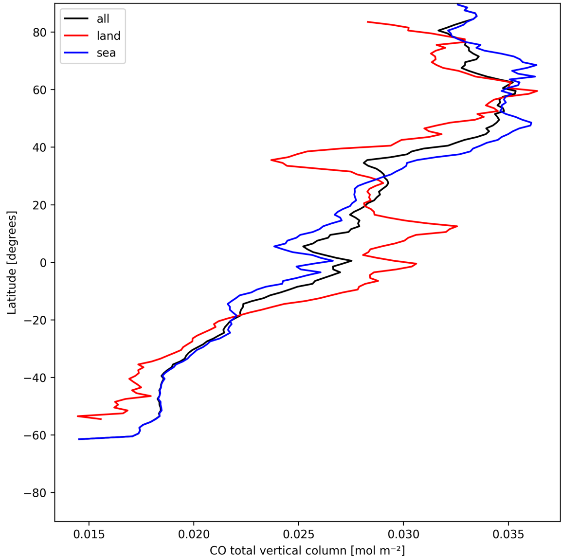
Figure 10: Zonal average of “CO total vertical column” for 2025-06-13 to 2025-06-15.
