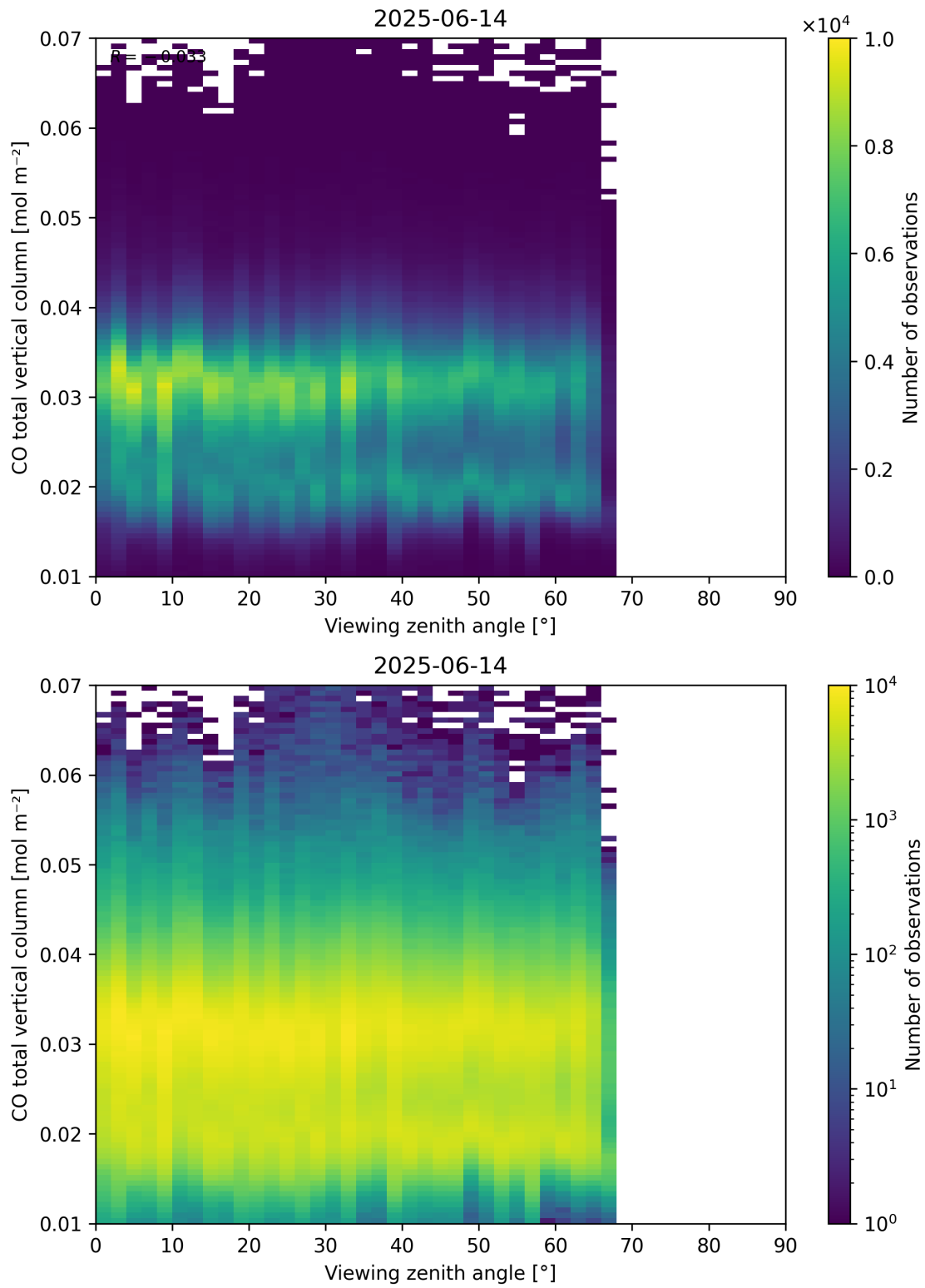
Figure 69: Scatter density plot of “Viewing zenith angle” against “CO total vertical column” for 2025-06-13 to 2025-06-15.
