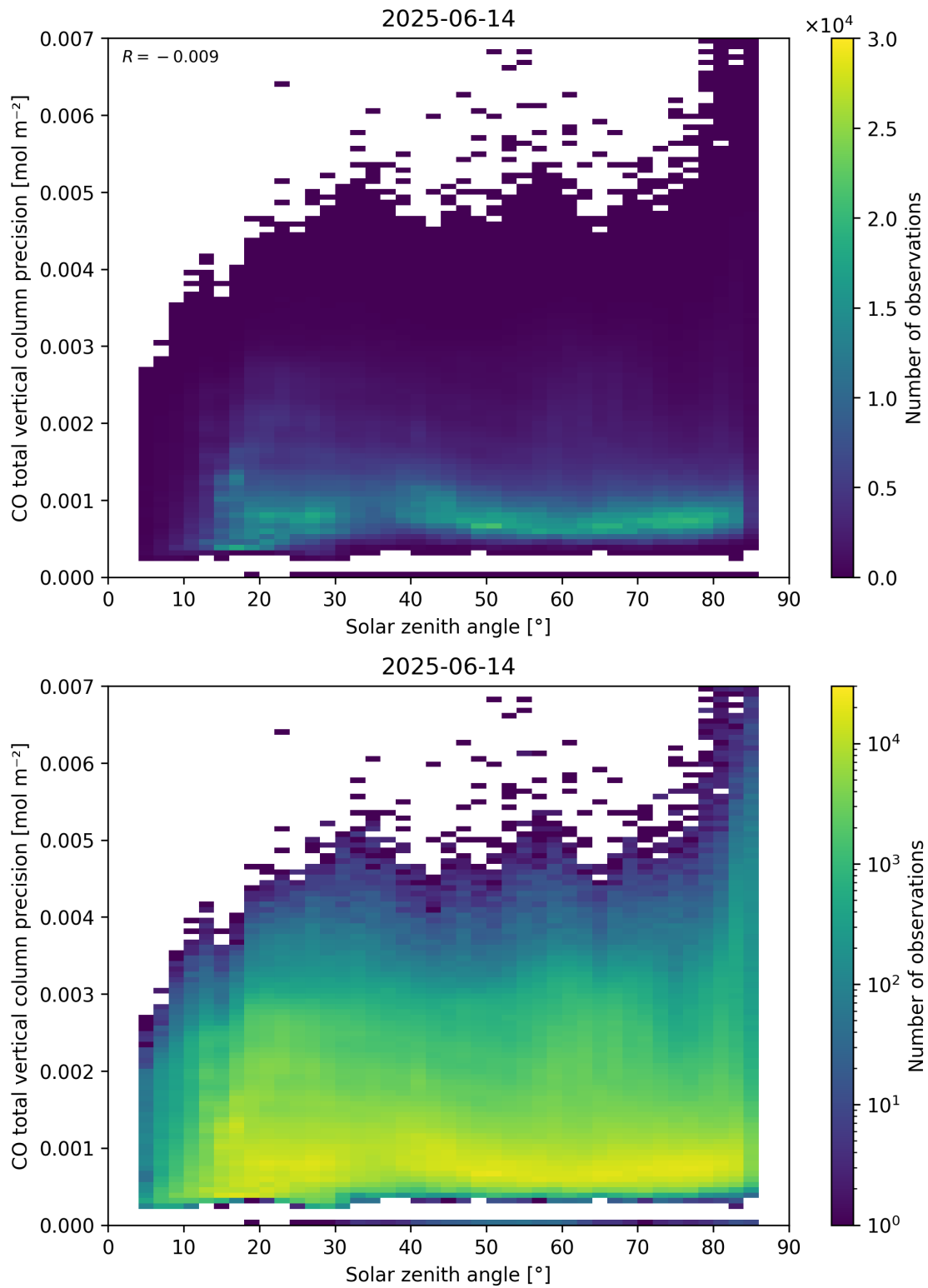
Figure 63: Scatter density plot of “Solar zenith angle” against “CO total vertical column precision” for 2025-06-13 to 2025-06-15.
