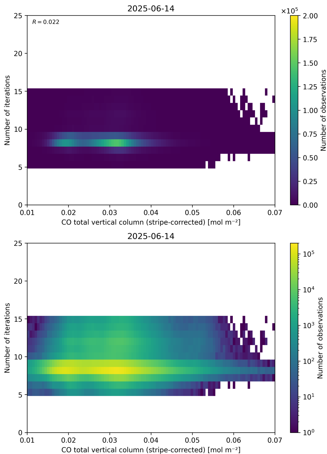
Figure 39: Scatter density plot of “CO total vertical column (stripe-corrected)” against “Number of iterations” for 2025-06-13 to 2025-06-15.
