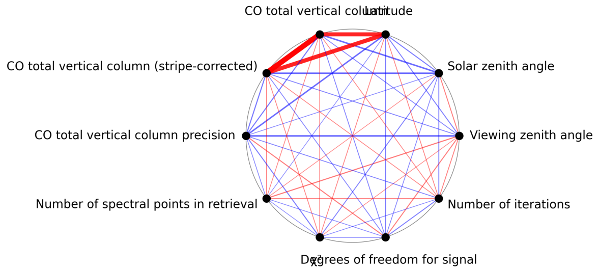
Figure 1: Map of correlation graph for 2025-06-13 to 2025-06-15.
