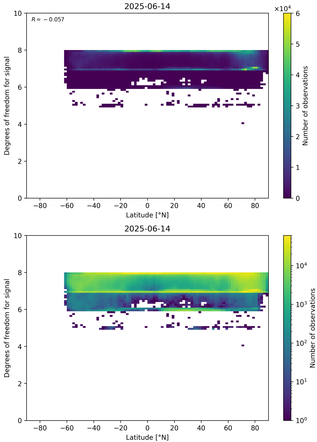
Figure 55: Scatter density plot of “Latitude” against “Degrees of freedom for signal” for 2025-06-13 to 2025-06-15.
