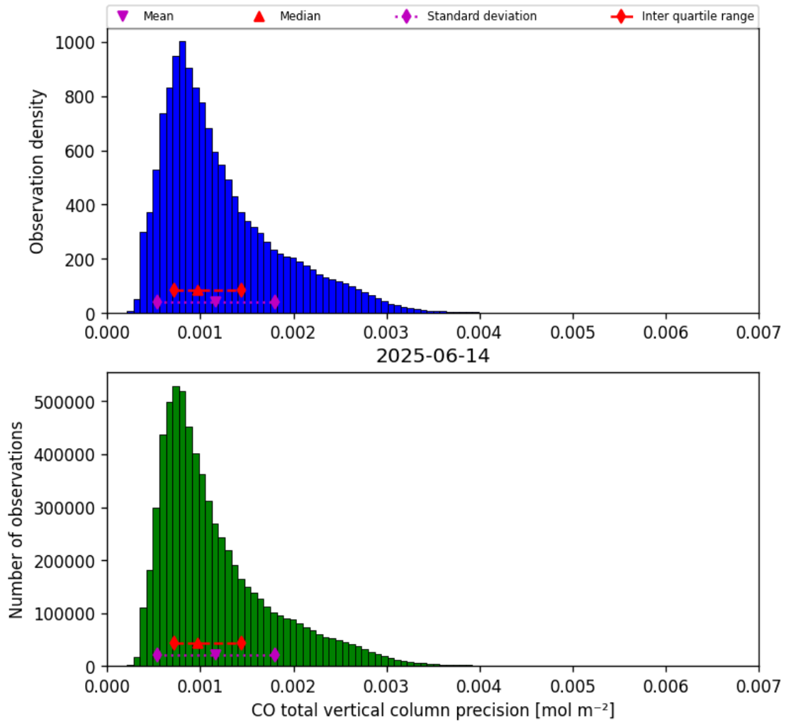
Figure 20: Histogram of “CO total vertical column precision” for 2025-06-13 to 2025-06-15
