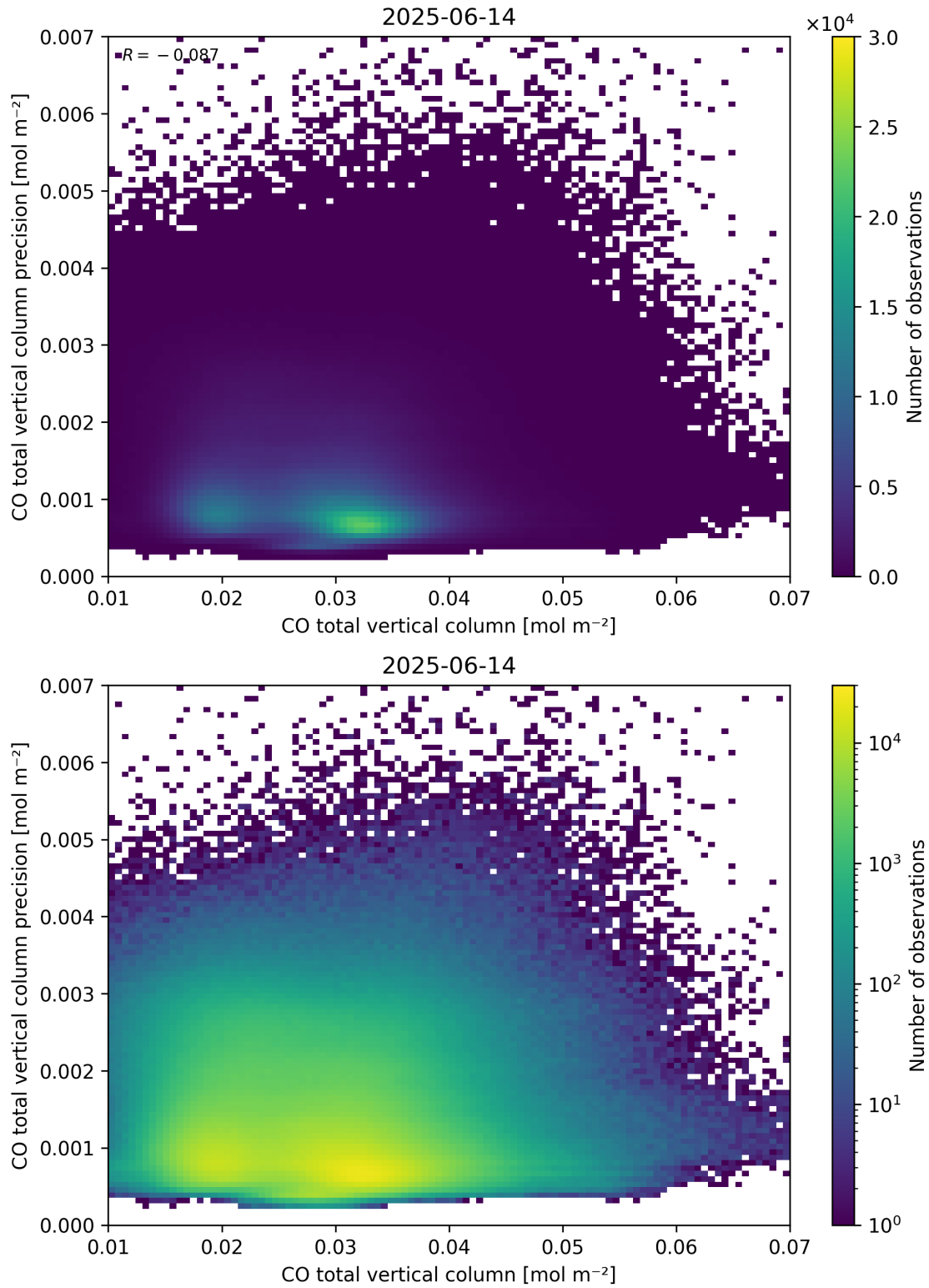
Figure 34: Scatter density plot of “CO total vertical column” against “CO total vertical column precision” for 2025-06-13 to 2025-06-15.
