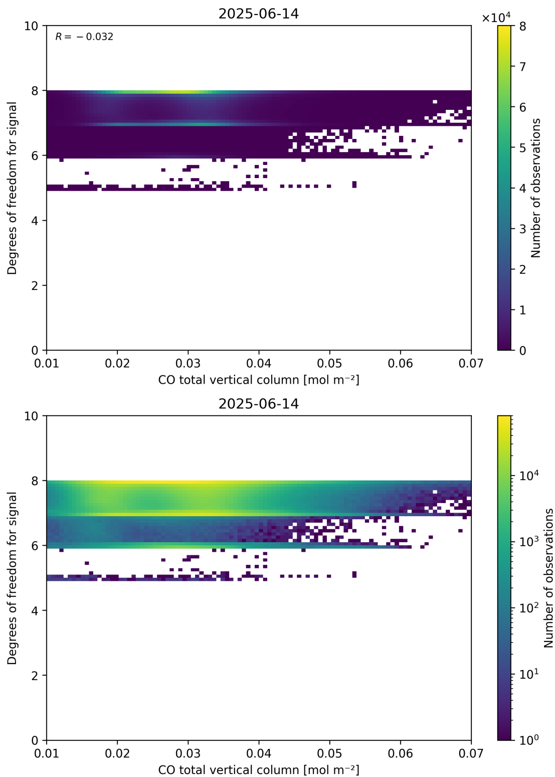
Figure 41: Scatter density plot of “CO total vertical column” against “Degrees of freedom for signal” for 2025-06-13 to 2025-06-15.
