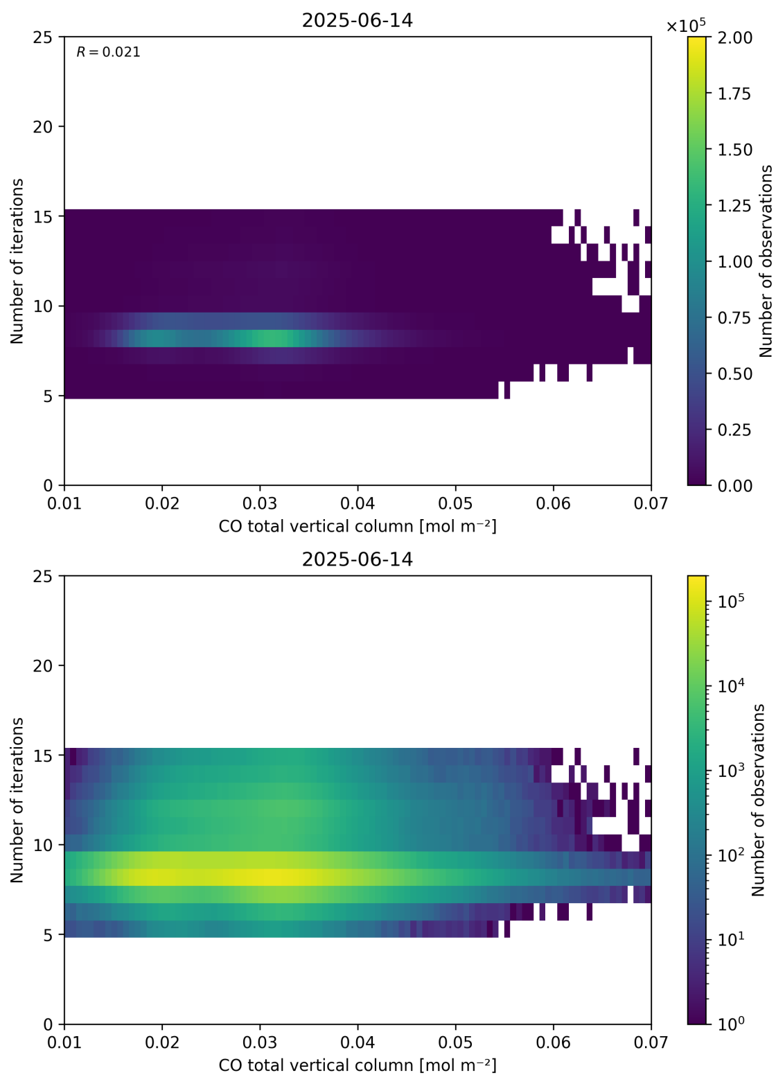
Figure 42: Scatter density plot of “CO total vertical column” against “Number of iterations” for 2025-06-13 to 2025-06-15.
