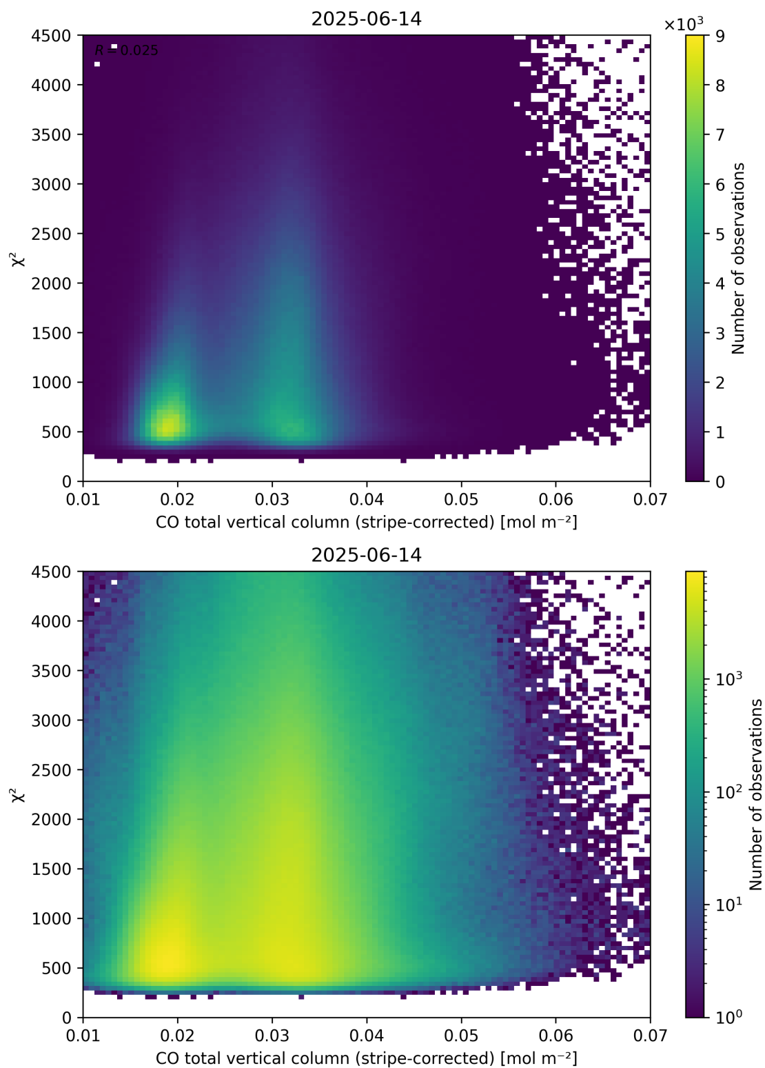
Figure 37: Scatter density plot of “CO total vertical column (stripe-corrected)” against “ \chi^2 ” for 2025-06-13 to 2025-06-15.
