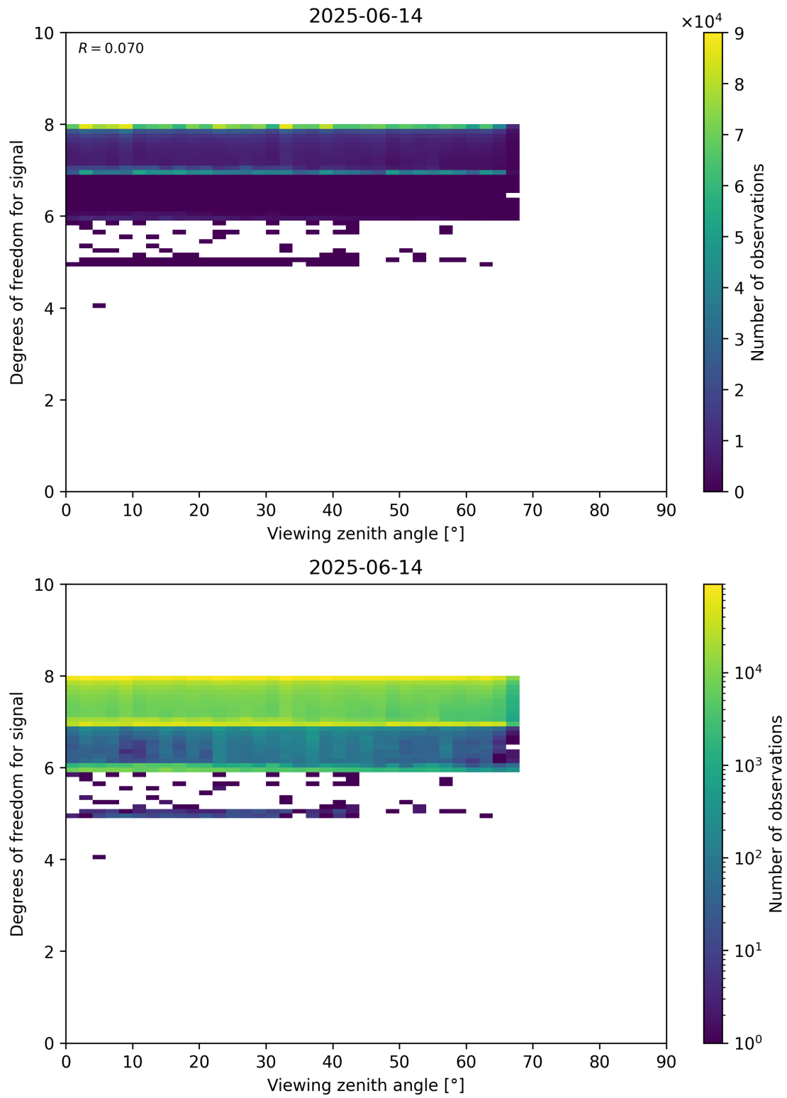
Figure 73: Scatter density plot of “Viewing zenith angle” against “Degrees of freedom for signal” for 2025-06-13 to 2025-06-15.
