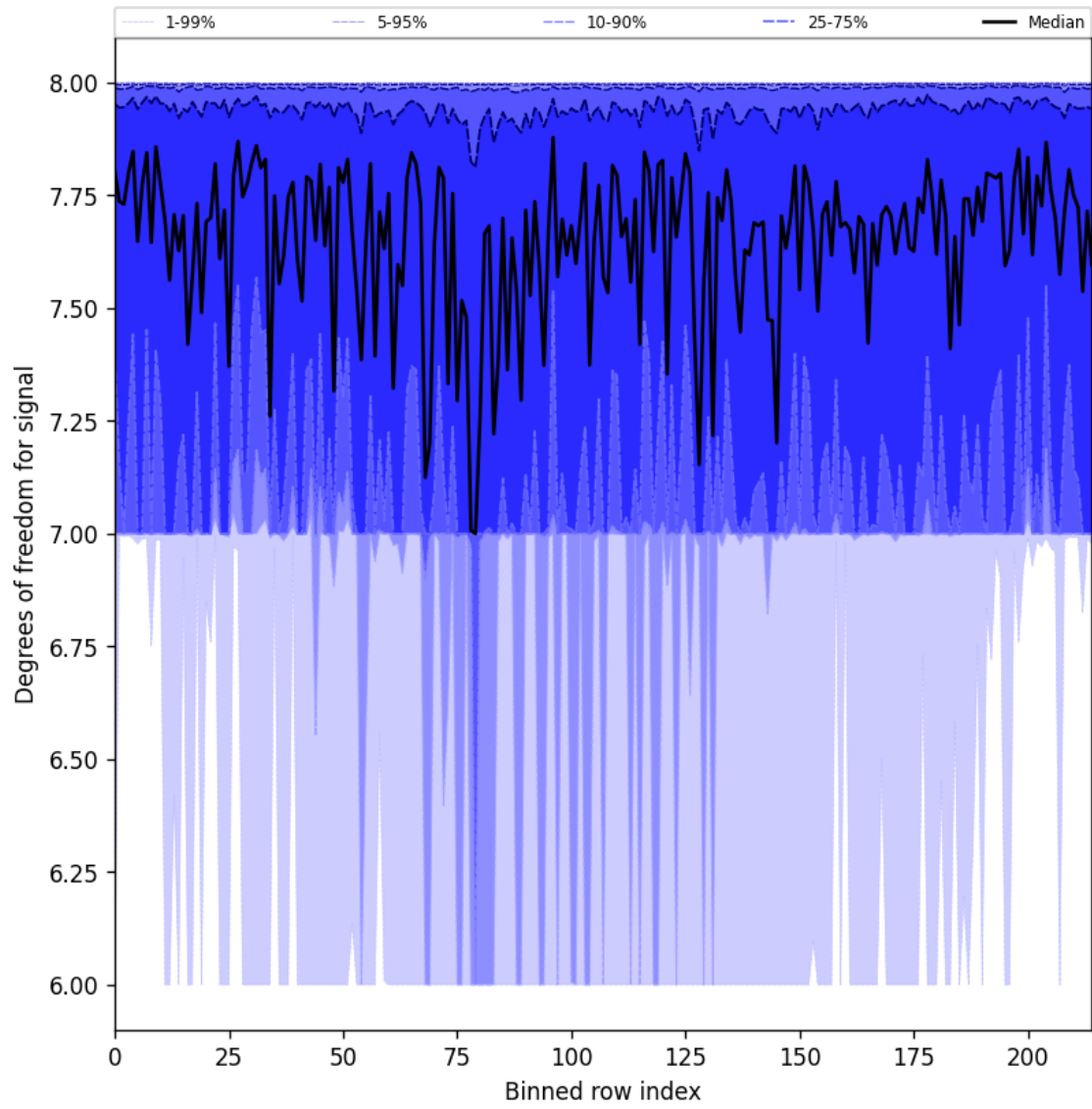
Figure 31: Along track statistics of “Degrees of freedom for signal” for 2025-06-13 to 2025-06-15
