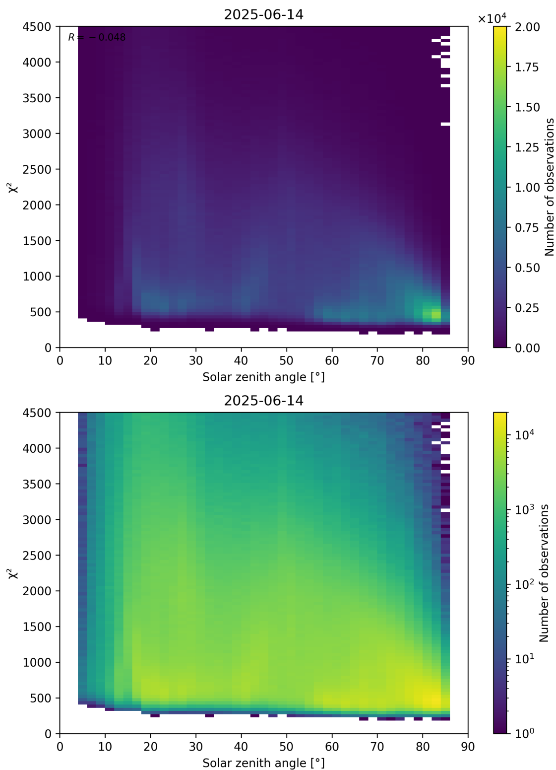
Figure 64: Scatter density plot of “Solar zenith angle” against “ \chi^2 ” for 2025-06-13 to 2025-06-15.
