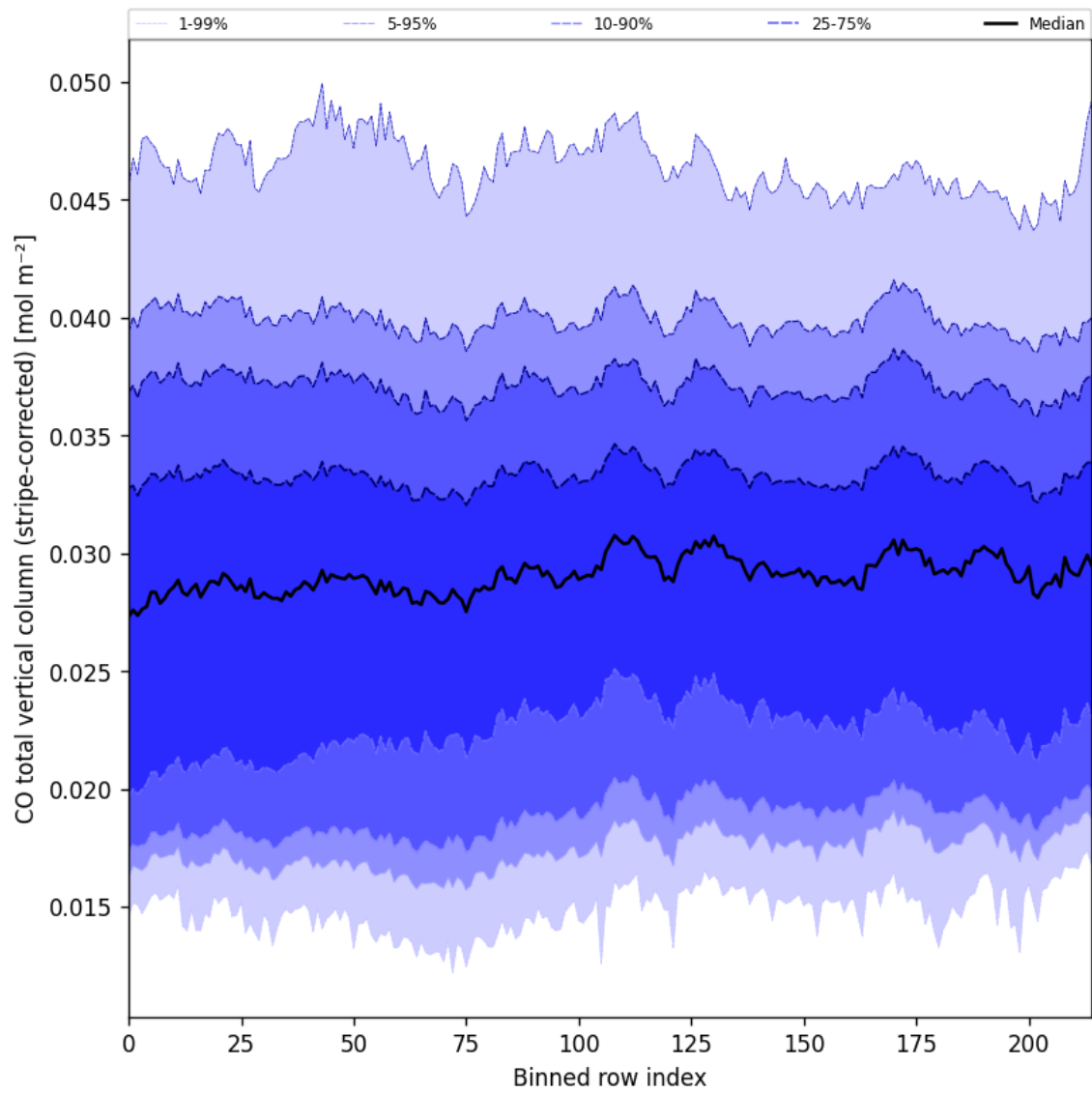
Figure 27: Along track statistics of “CO total vertical column (stripe-corrected)” for 2025-06-13 to 2025-06-15
