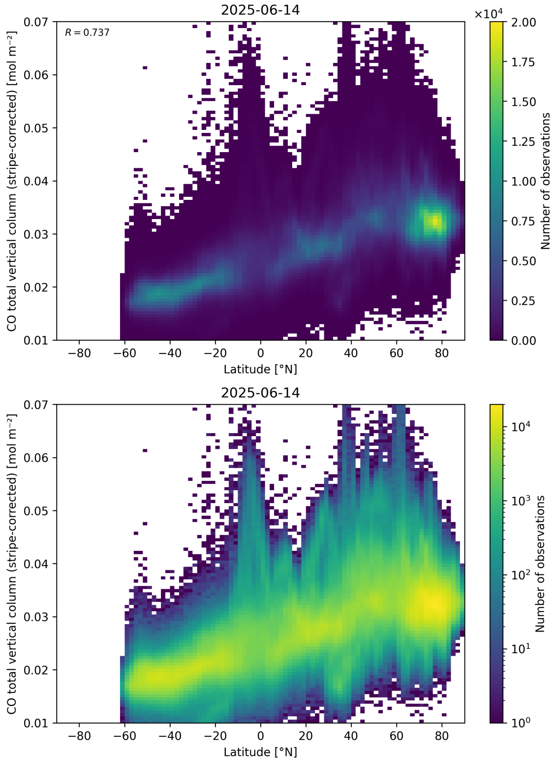
Figure 52: Scatter density plot of “Latitude” against “CO total vertical column (stripe-corrected)” for 2025-06-13 to 2025-06-15.
