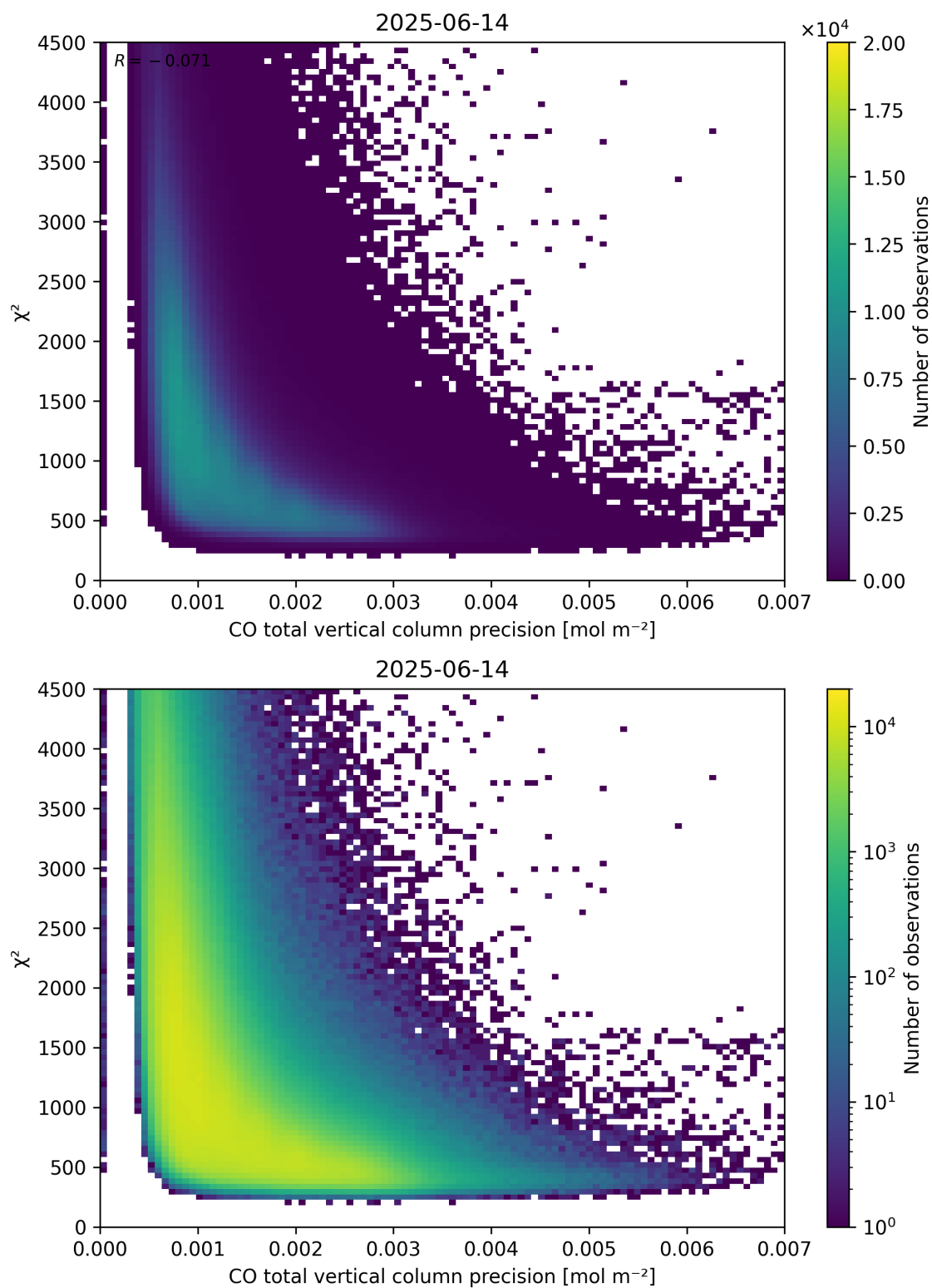
Figure 44: Scatter density plot of “CO total vertical column precision” against “ \chi^2 ” for 2025-06-13 to 2025-06-15.
