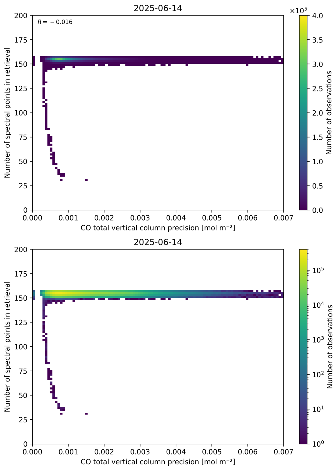
Figure 47: Scatter density plot of “CO total vertical column precision” against “Number of spectral points in retrieval” for 2025-06-13 to 2025-06-15.
