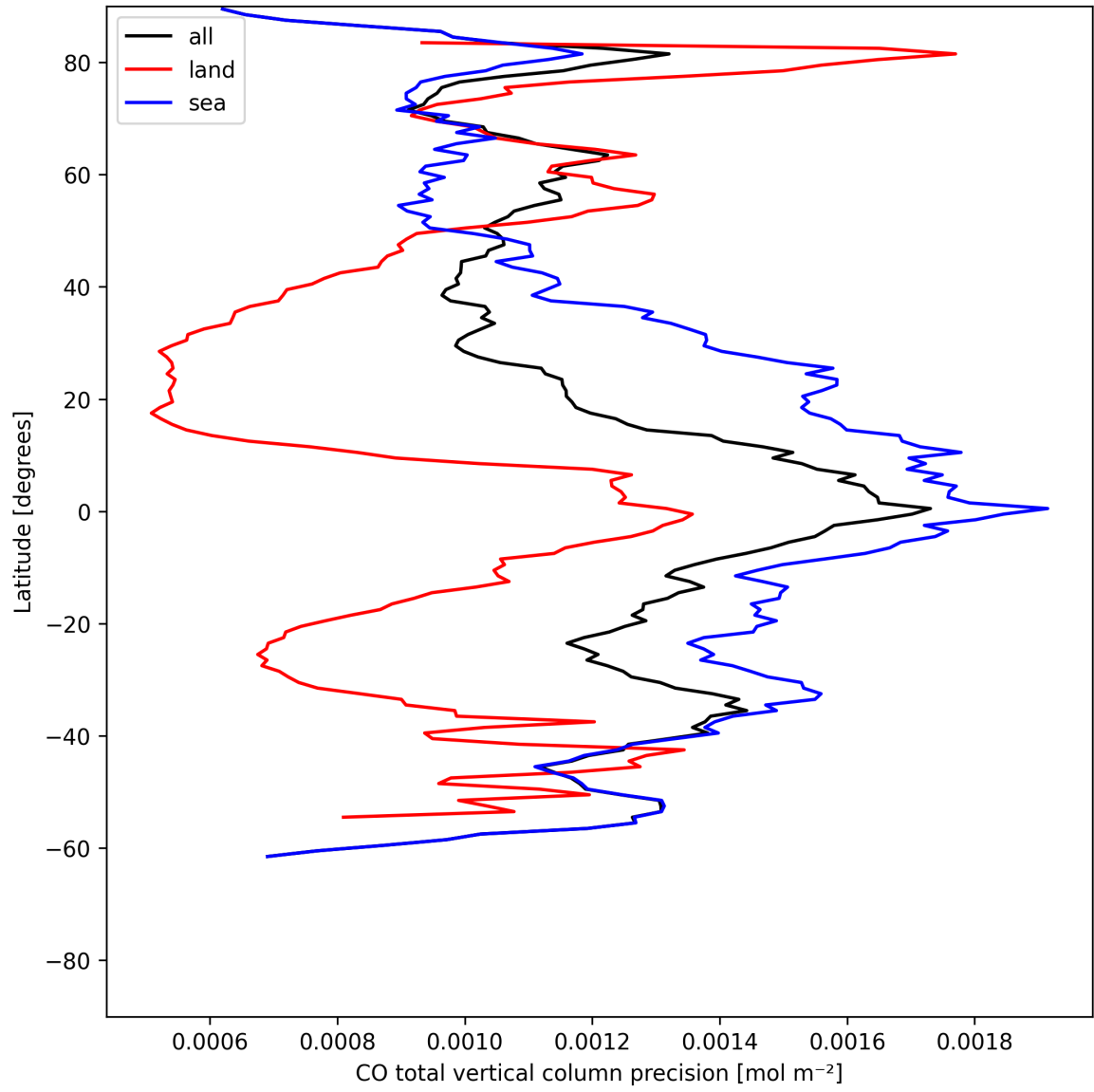
Figure 12: Zonal average of “CO total vertical column precision” for 2025-06-13 to 2025-06-15.
