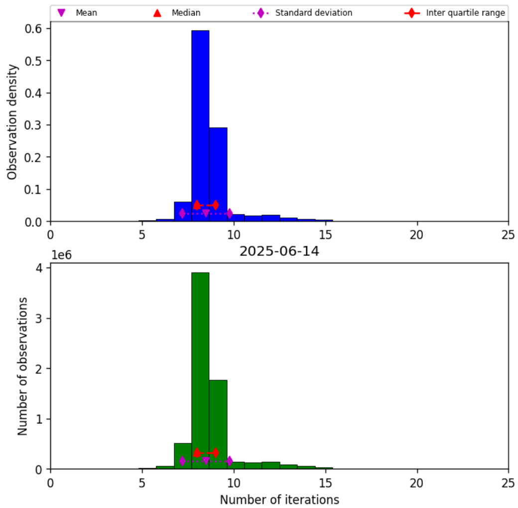
Figure 24: Histogram of “Number of iterations” for 2025-06-13 to 2025-06-15
