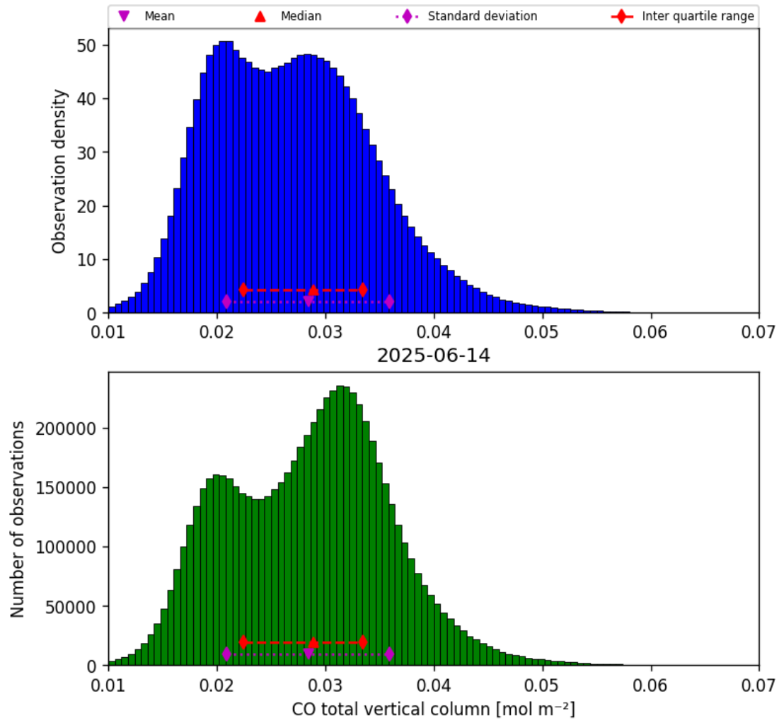
Figure 18: Histogram of “CO total vertical column” for 2025-06-13 to 2025-06-15
