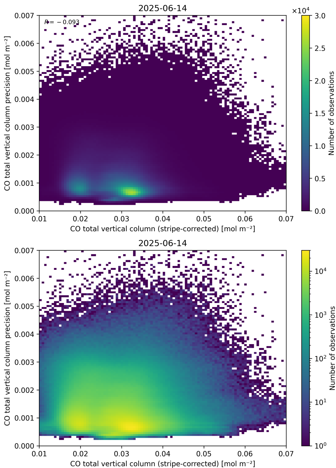
Figure 36: Scatter density plot of “CO total vertical column (stripe-corrected)” against “CO total vertical column precision” for 2025-06-13 to 2025-06-15.
