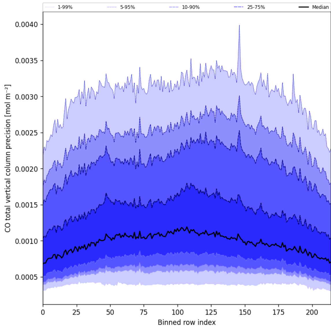
Figure 28: Along track statistics of “CO total vertical column precision” for 2025-06-13 to 2025-06-15
