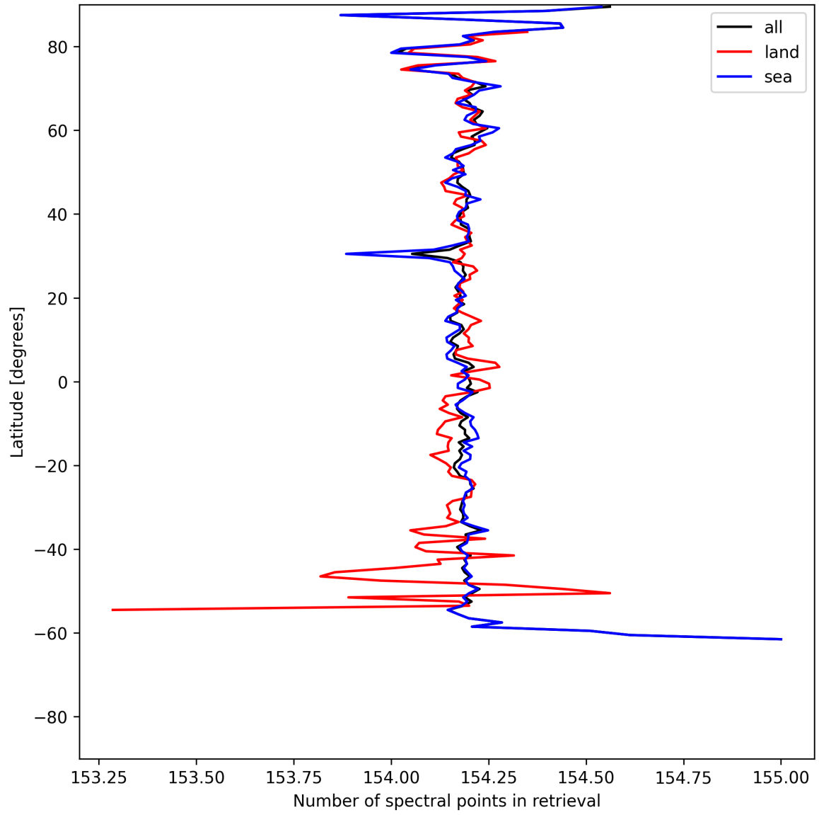
Figure 13: Zonal average of “Number of spectral points in retrieval” for 2025-06-13 to 2025-06-15.
