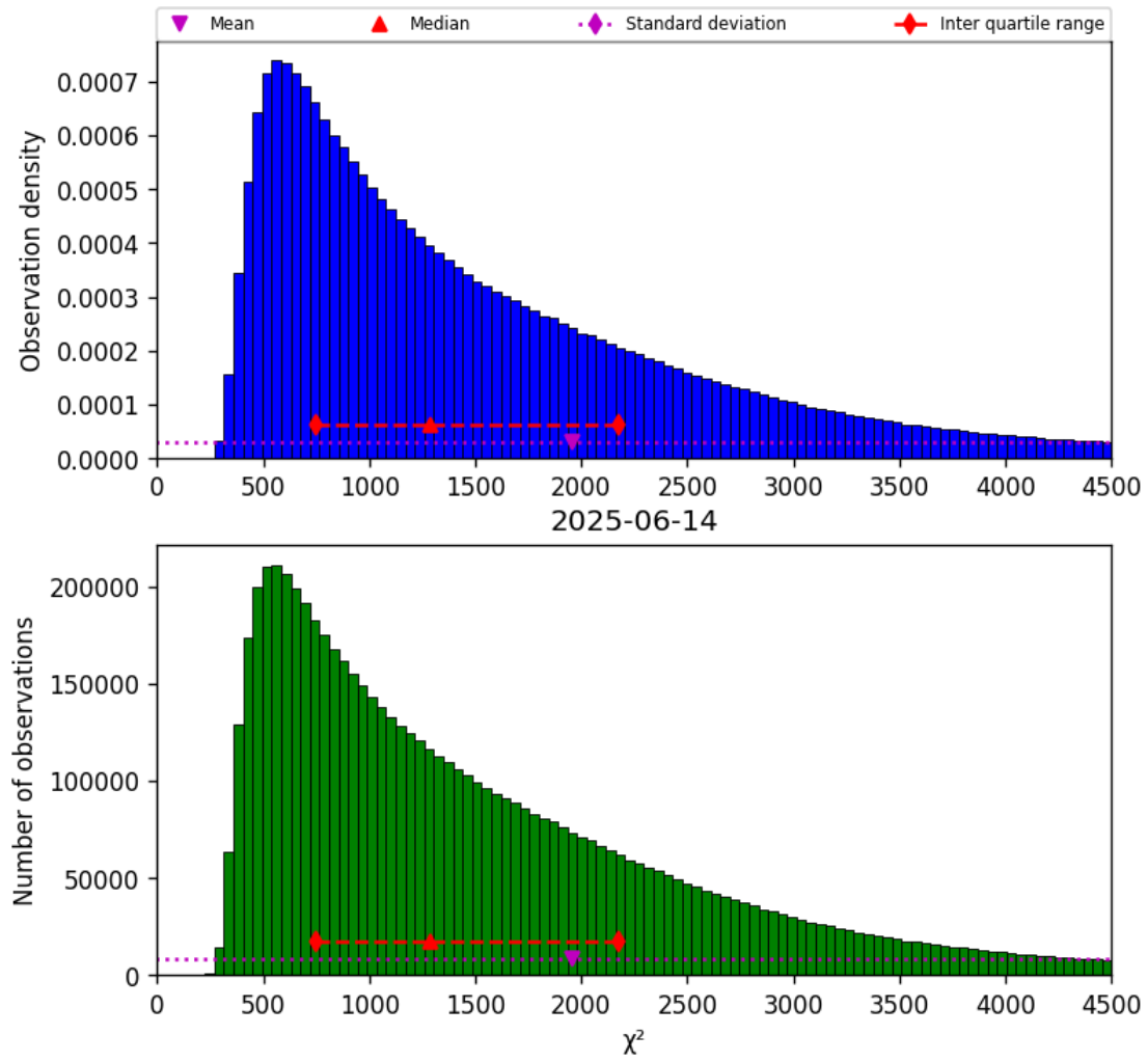
Figure 22: Histogram of “ \chi^2 ” for 2025-06-13 to 2025-06-15
