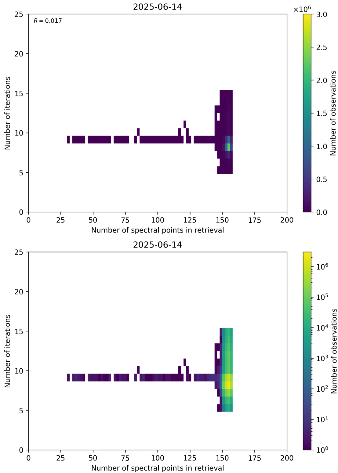
Figure 60: Scatter density plot of “Number of spectral points in retrieval” against “Number of iterations” for 2025-06-13 to 2025-06-15.
