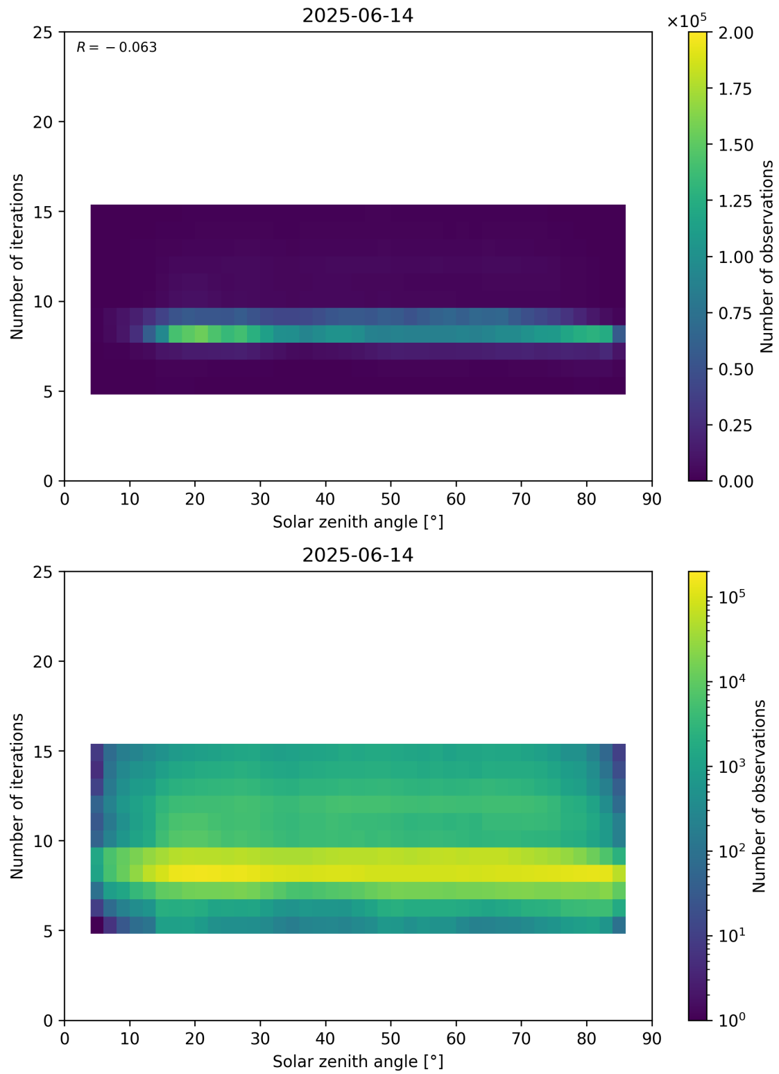
Figure 67: Scatter density plot of “Solar zenith angle” against “Number of iterations” for 2025-06-13 to 2025-06-15.
