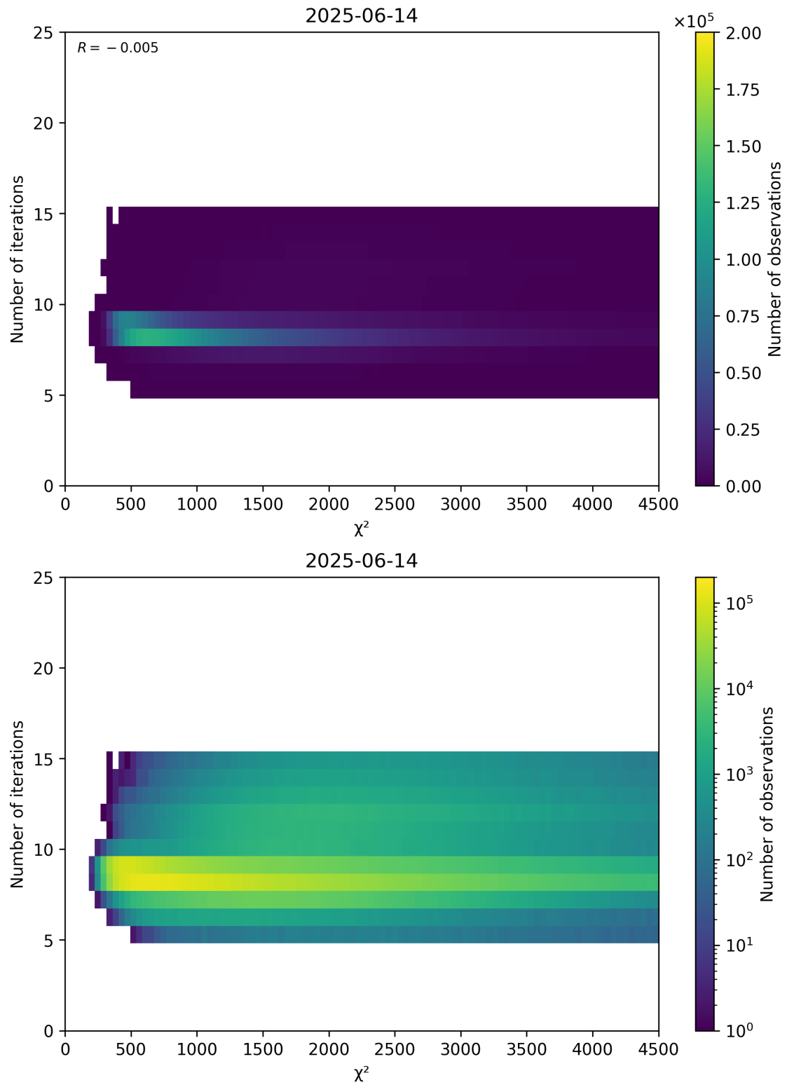
Figure 49: Scatter density plot of “ \chi^2 ” against “Number of iterations” for 2025-06-13 to 2025-06-15.
