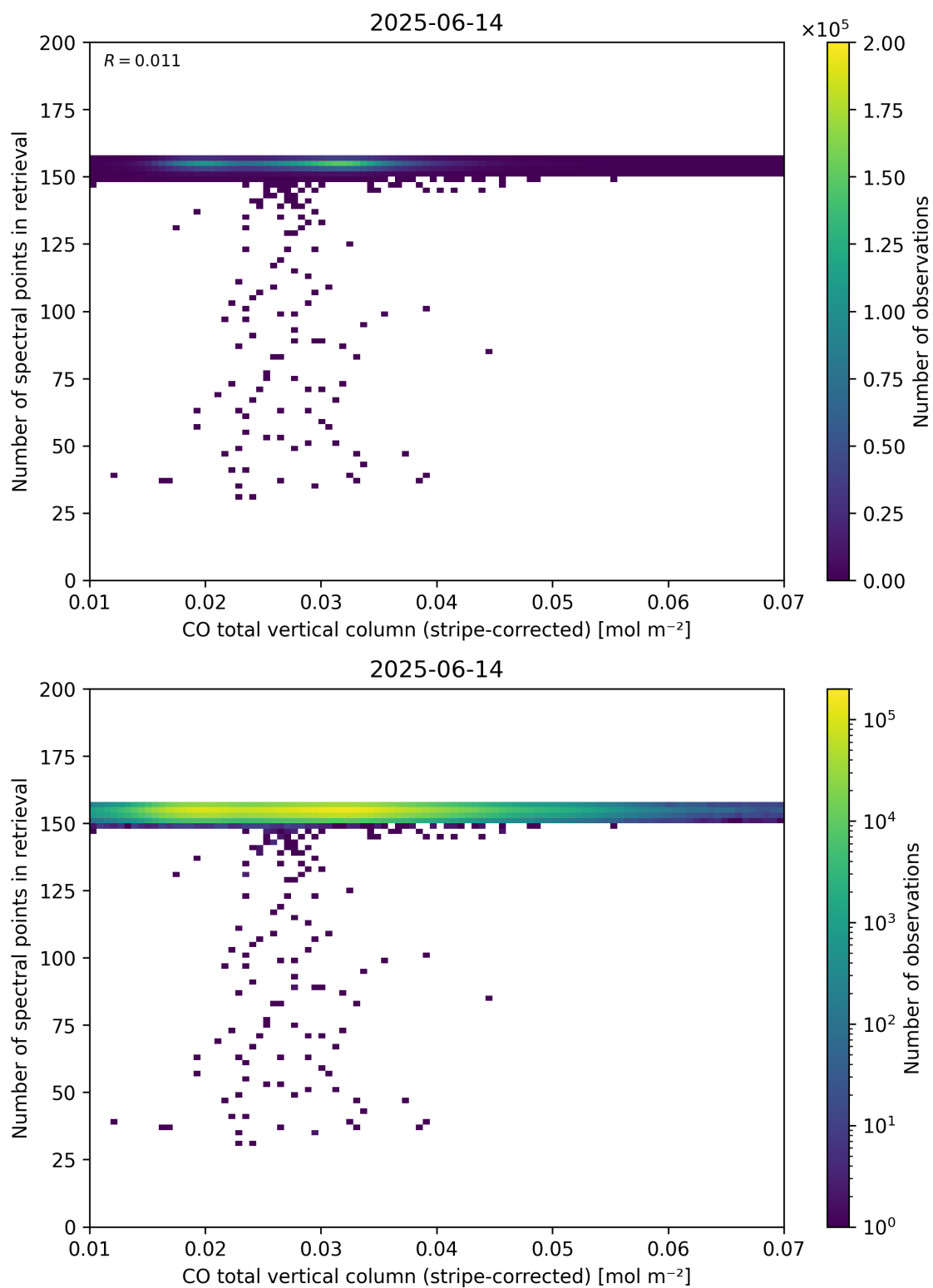
Figure 40: Scatter density plot of “CO total vertical column (stripe-corrected)” against “Number of spectral points in retrieval” for 2025-06-13 to 2025-06-15.
