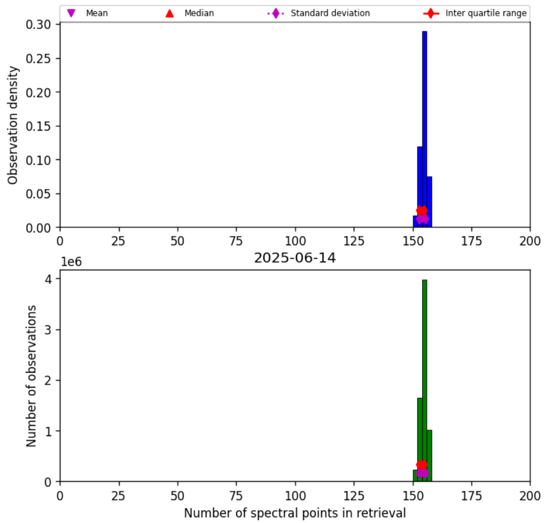
Figure 21: Histogram of “Number of spectral points in retrieval” for 2025-06-13 to 2025-06-15
