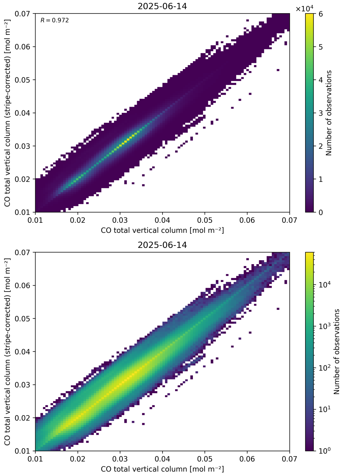
Figure 33: Scatter density plot of “CO total vertical column” against “CO total vertical column (stripe-corrected)” for 2025-06-13 to 2025-06-15.
