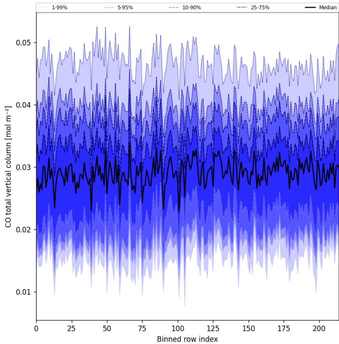
Figure 26: Along track statistics of “CO total vertical column” for 2025-06-13 to 2025-06-15
