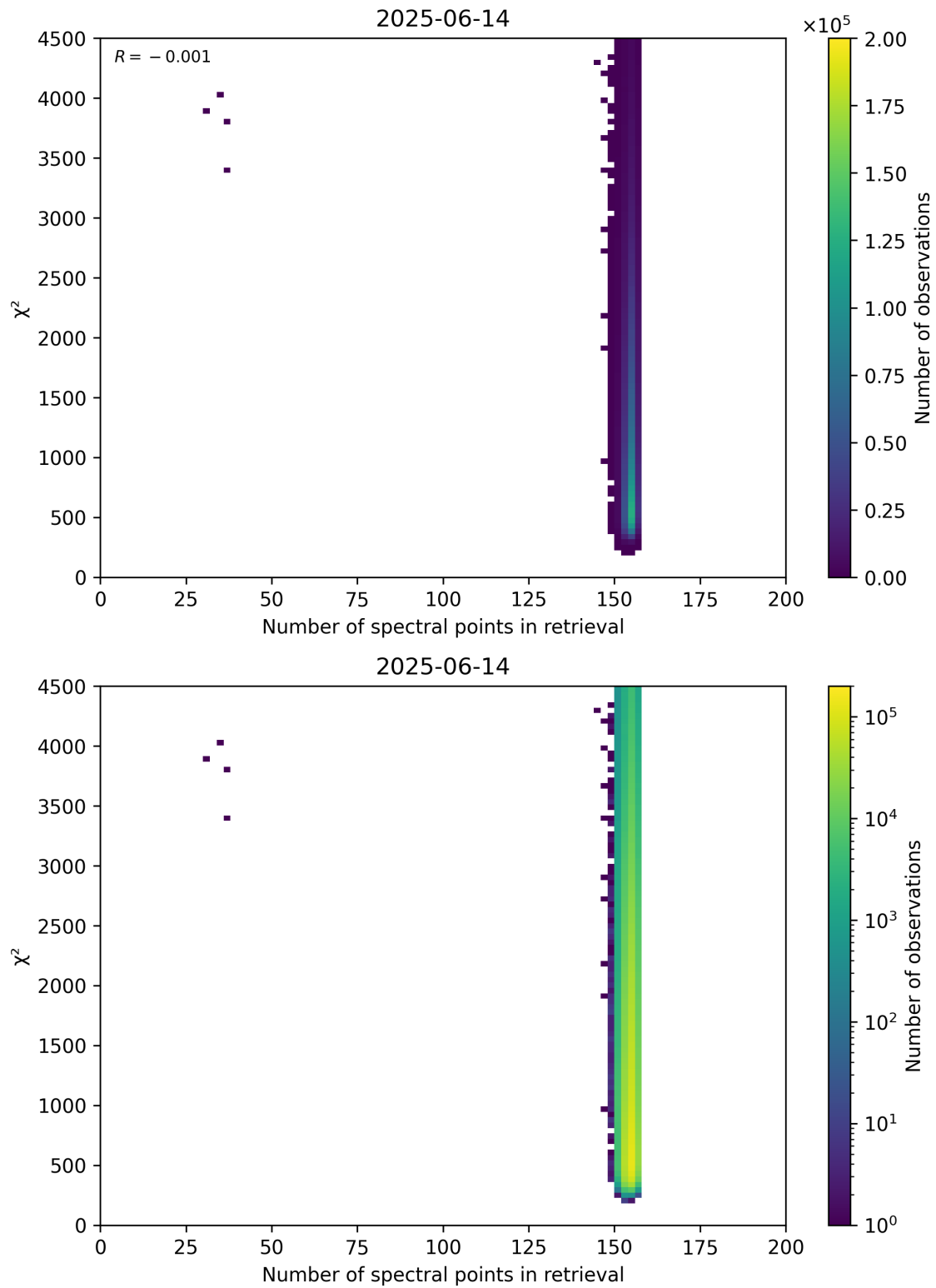
Figure 58: Scatter density plot of “Number of spectral points in retrieval” against “ \chi^2 ” for 2025-06-13 to 2025-06-15.
