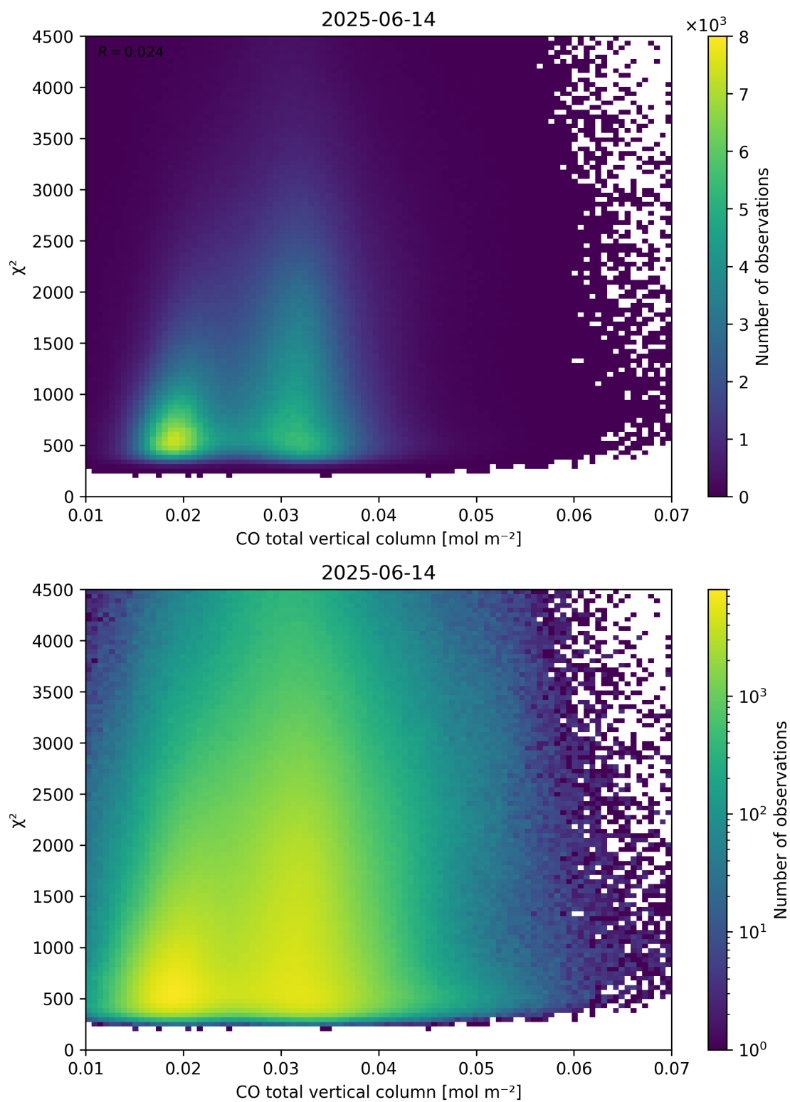
Figure 35: Scatter density plot of “CO total vertical column” against “ \chi^2 ” for 2025-06-13 to 2025-06-15.
