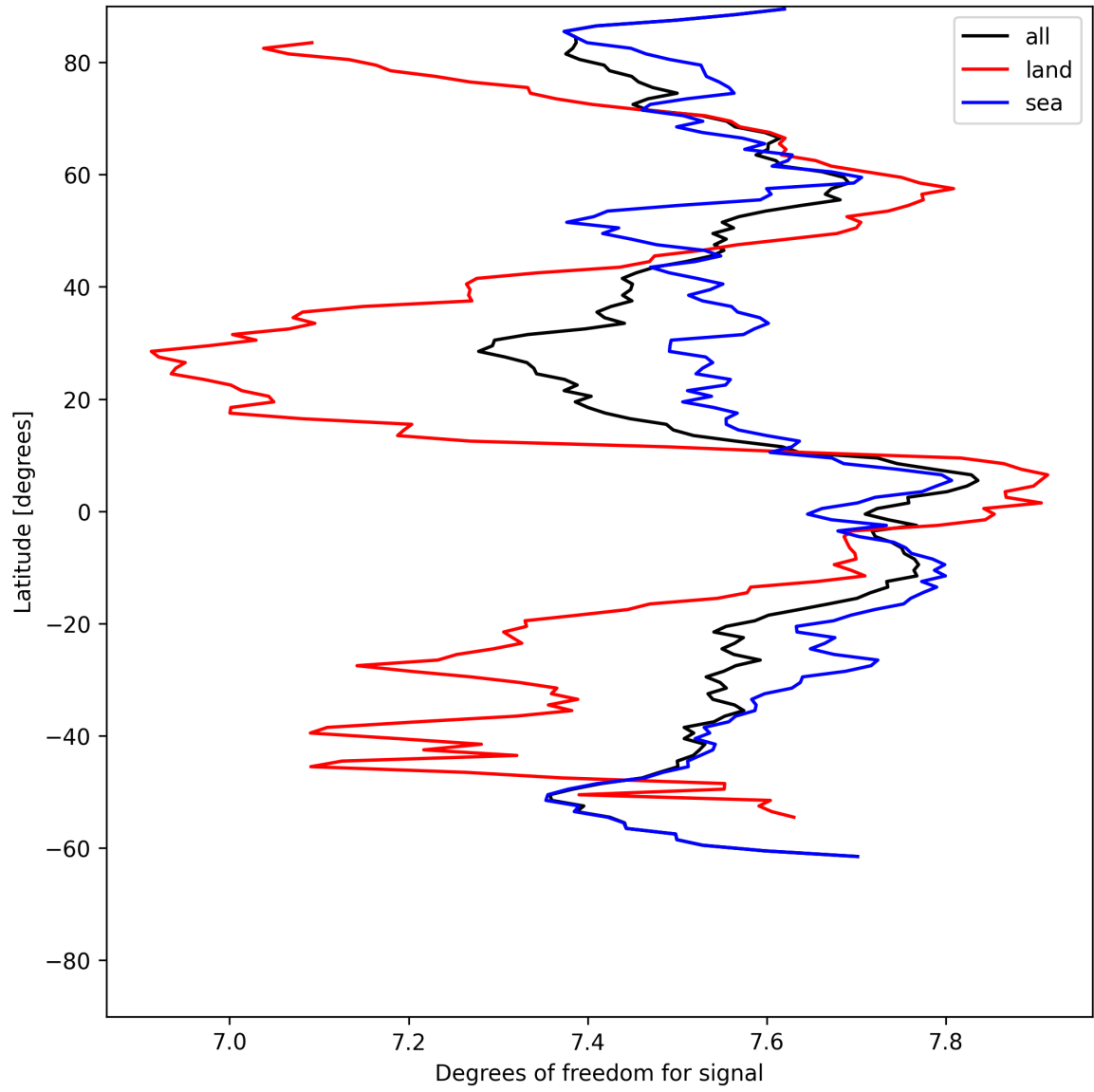
Figure 15: Zonal average of “Degrees of freedom for signal” for 2025-06-13 to 2025-06-15.
