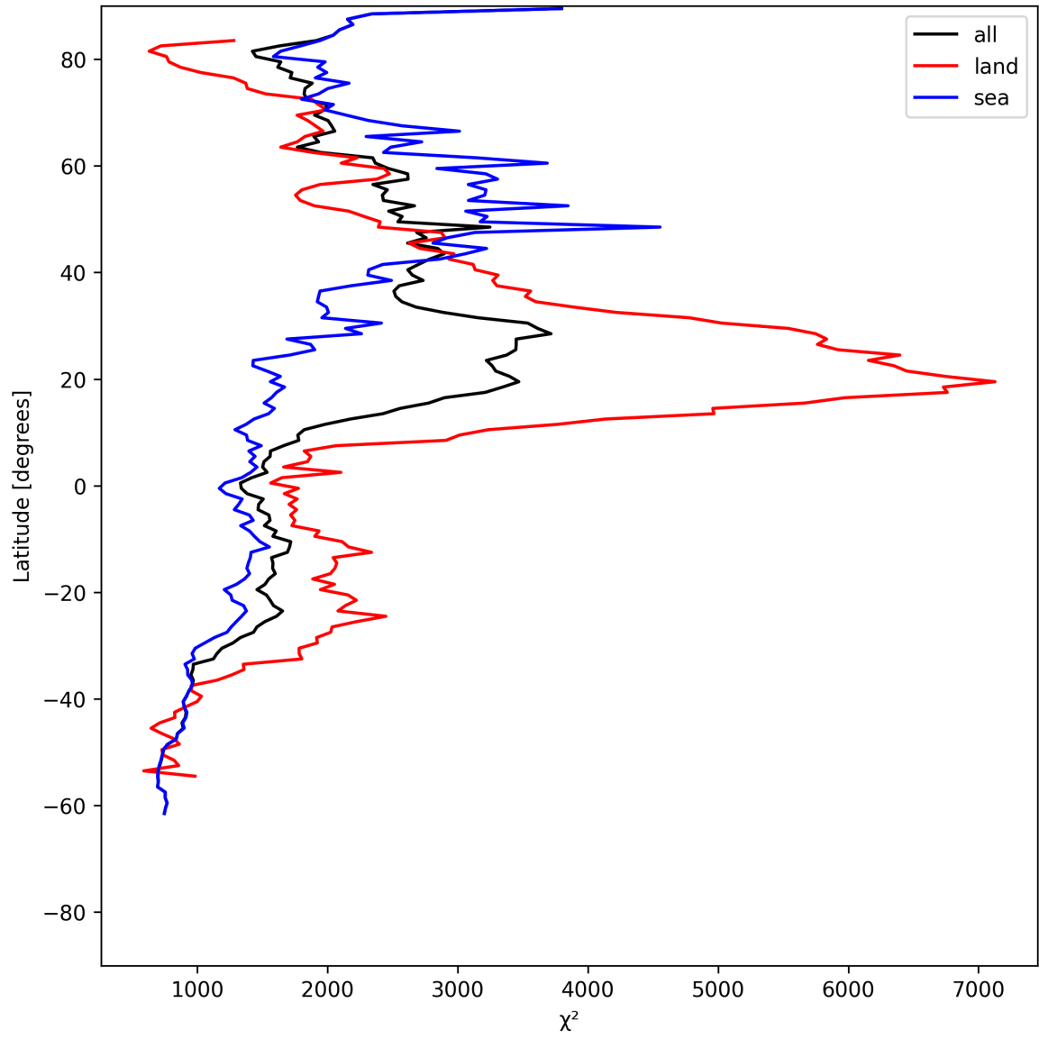
Figure 14: Zonal average of “ \chi^2 ” for 2025-06-13 to 2025-06-15.
