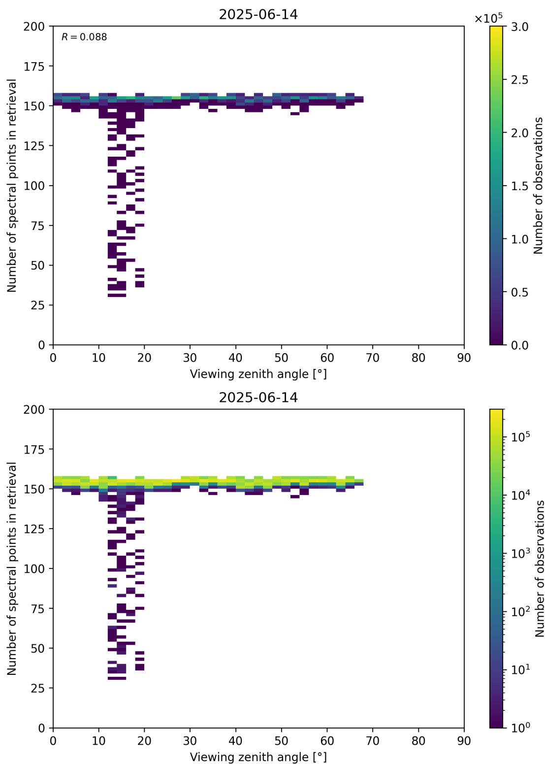
Figure 76: Scatter density plot of “Viewing zenith angle” against “Number of spectral points in retrieval” for 2025-06-13 to 2025-06-15.
