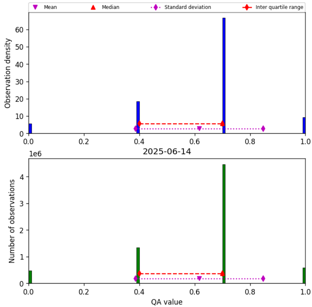
Figure 17: Histogram of “QA value” for 2025-06-13 to 2025-06-15
