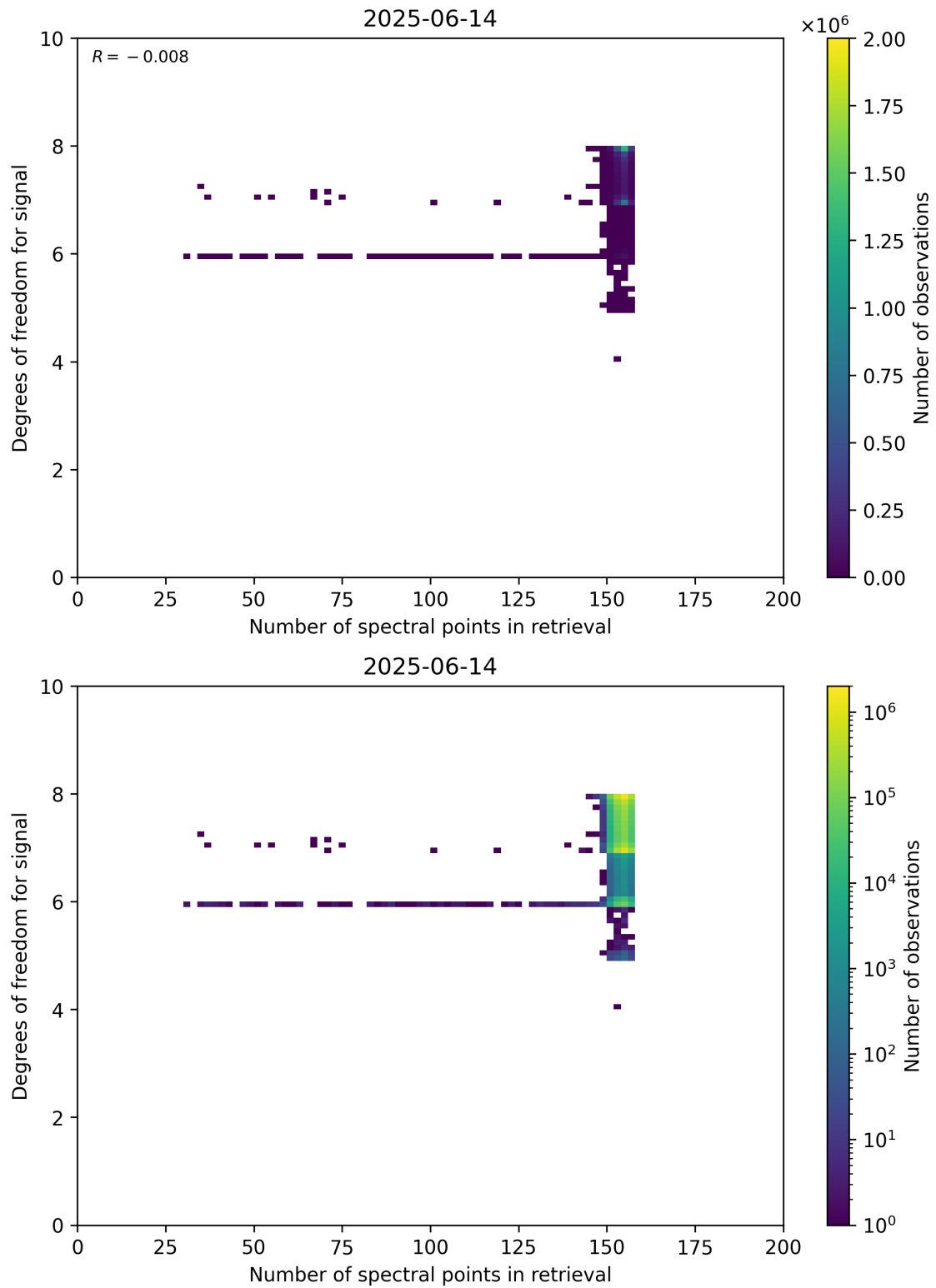
Figure 59: Scatter density plot of “Number of spectral points in retrieval” against “Degrees of freedom for signal” for 2025-06-13 to 2025-06-15.
