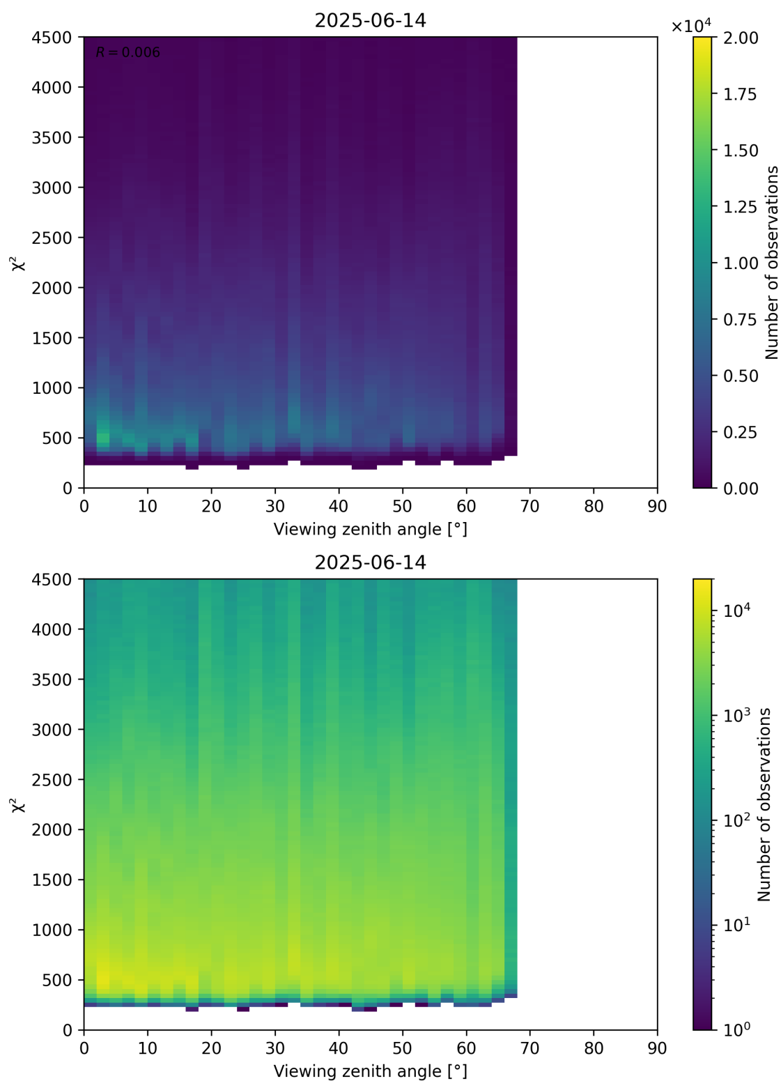
Figure 72: Scatter density plot of “Viewing zenith angle” against “ \chi^2 ” for 2025-06-13 to 2025-06-15.
