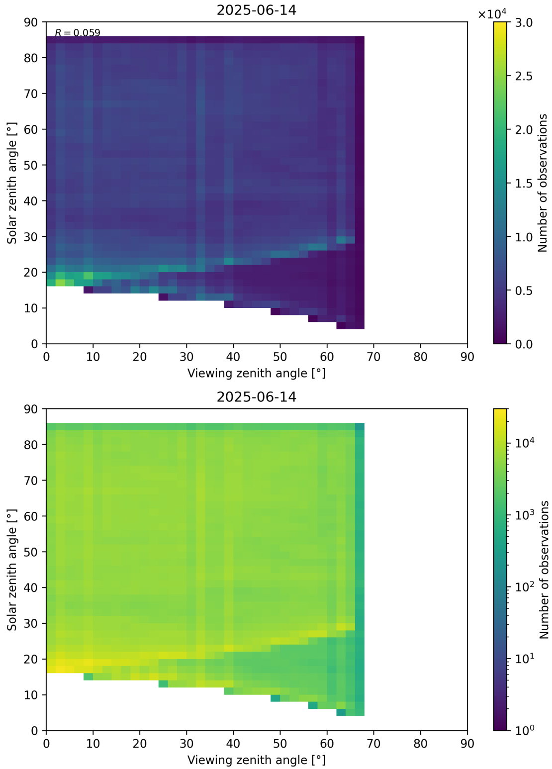
Figure 77: Scatter density plot of “Viewing zenith angle” against “Solar zenith angle” for 2025-06-13 to 2025-06-15.
