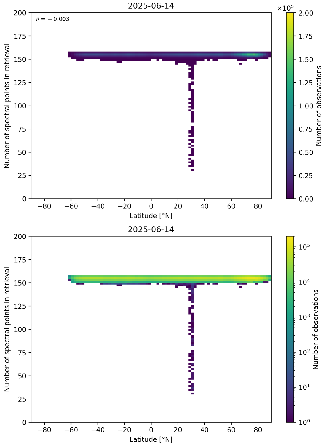
Figure 57: Scatter density plot of “Latitude” against “Number of spectral points in retrieval” for 2025-06-13 to 2025-06-15.
