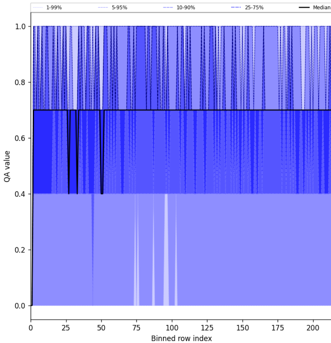
Figure 25: Along track statistics of “QA value” for 2025-06-13 to 2025-06-15
