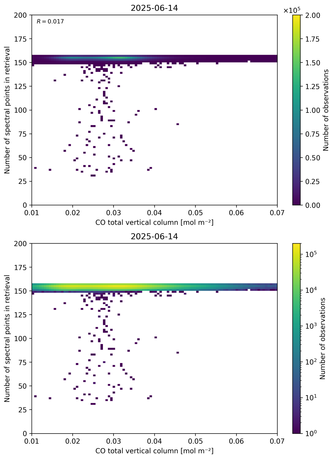
Figure 43: Scatter density plot of “CO total vertical column” against “Number of spectral points in retrieval” for 2025-06-13 to 2025-06-15.
