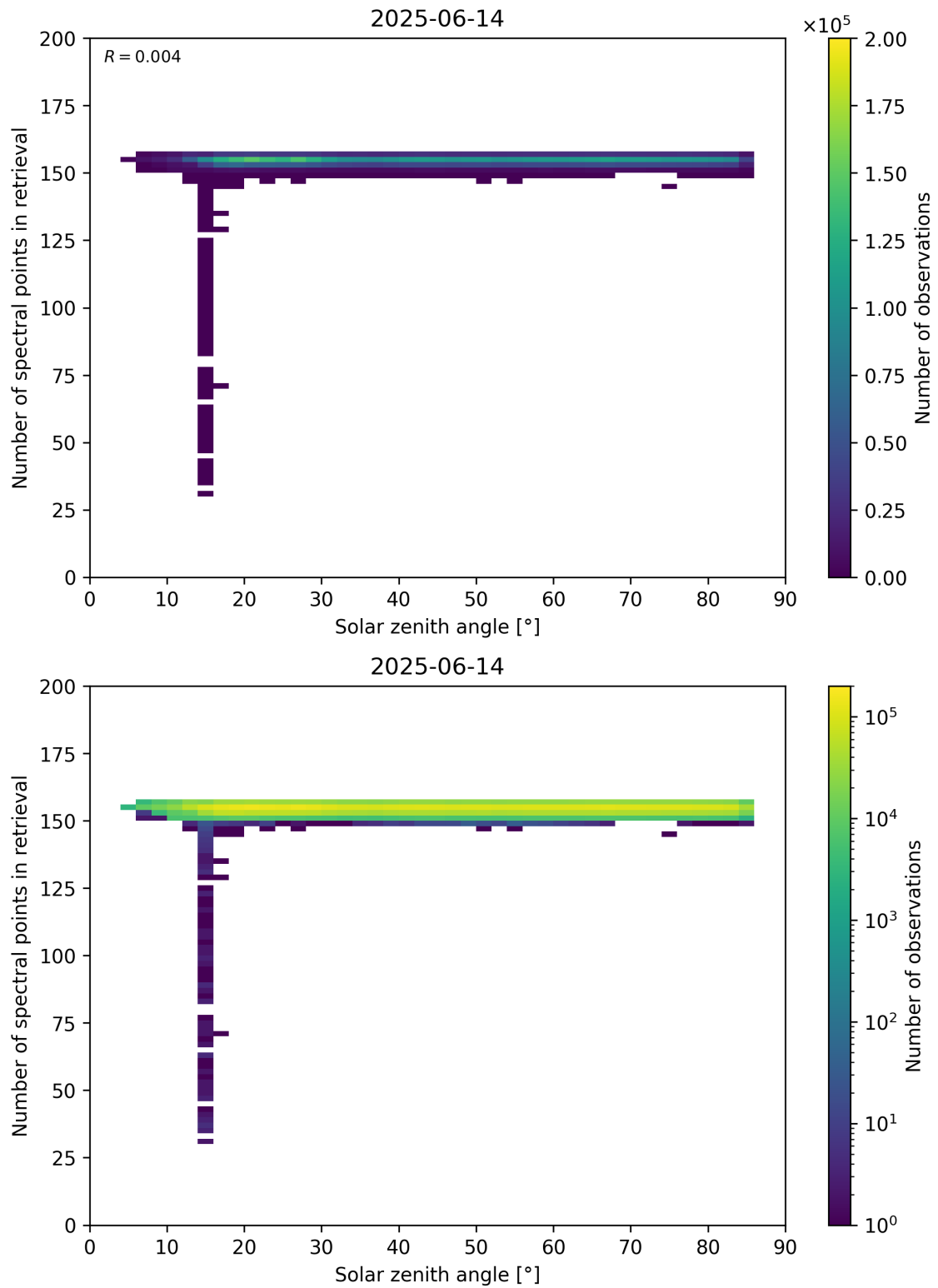
Figure 68: Scatter density plot of “Solar zenith angle” against “Number of spectral points in retrieval” for 2025-06-13 to 2025-06-15.
