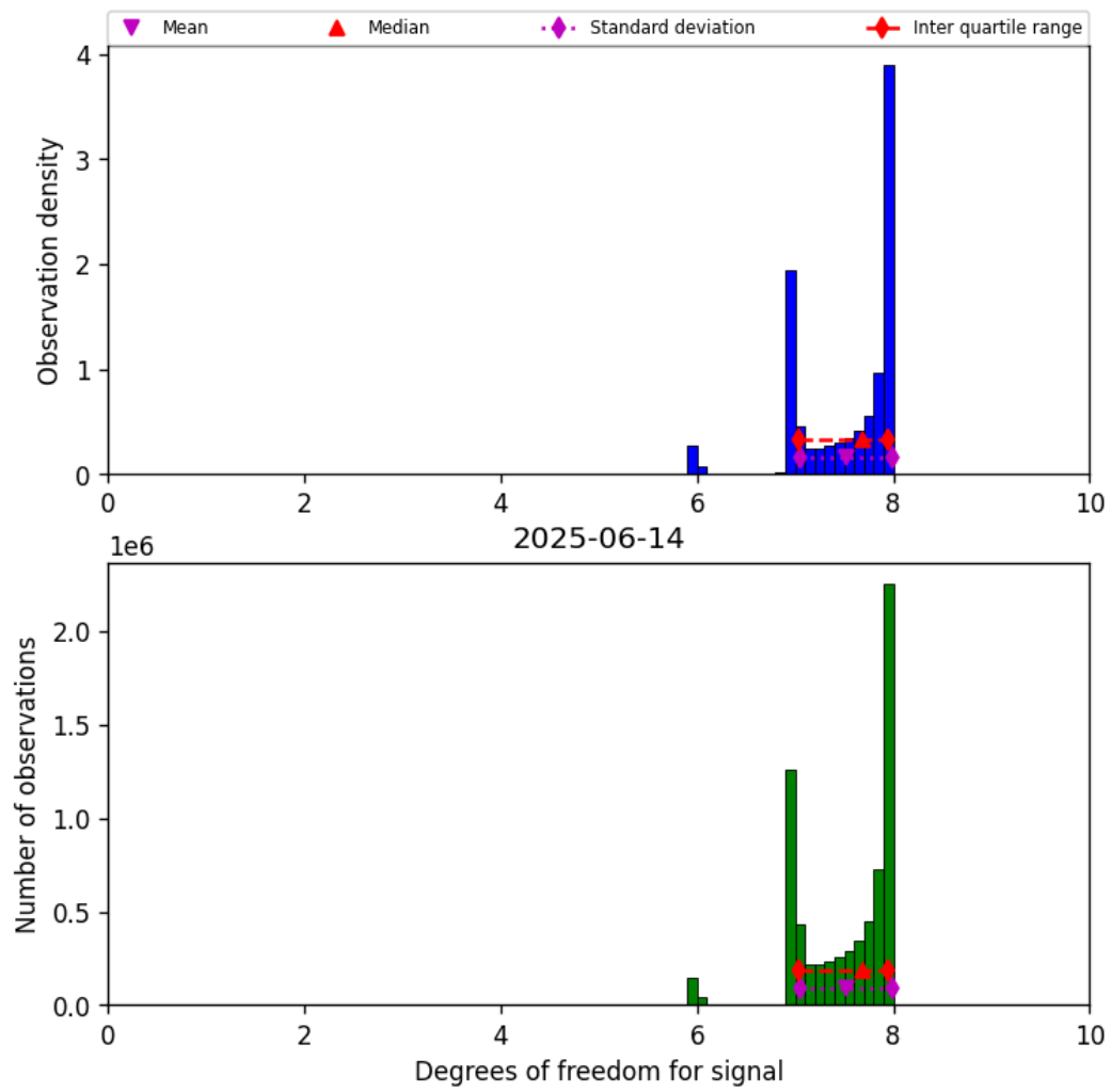
Figure 23: Histogram of “Degrees of freedom for signal” for 2025-06-13 to 2025-06-15
