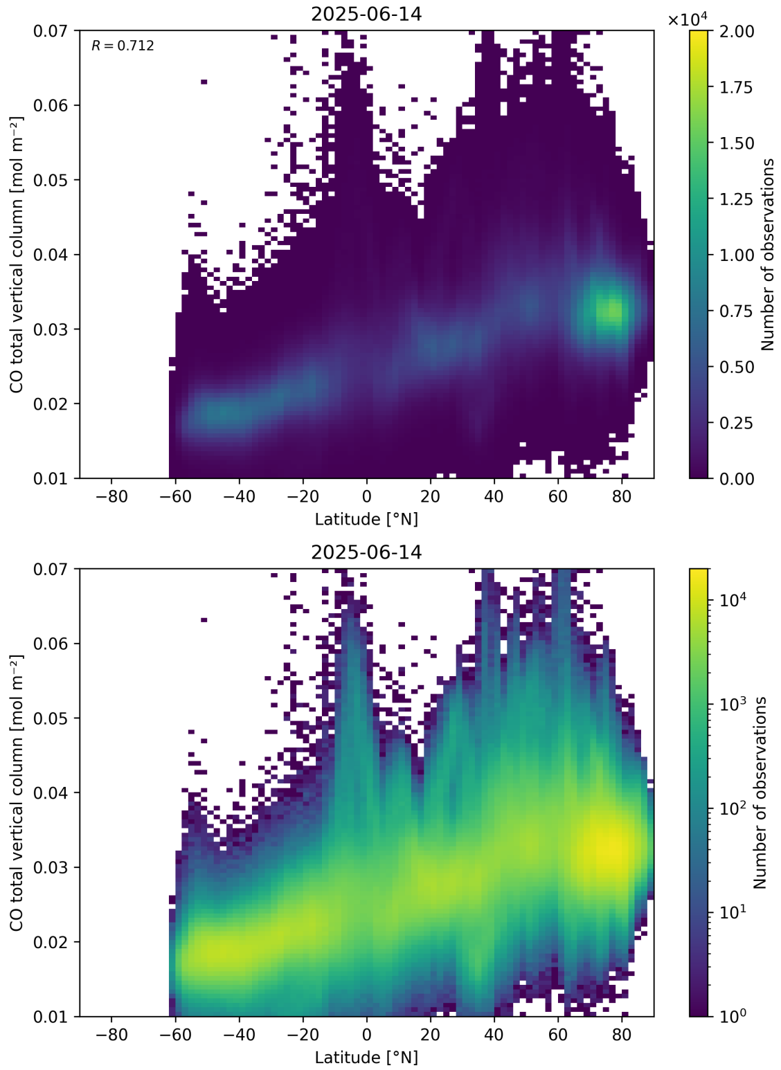
Figure 51: Scatter density plot of “Latitude” against “CO total vertical column” for 2025-06-13 to 2025-06-15.
