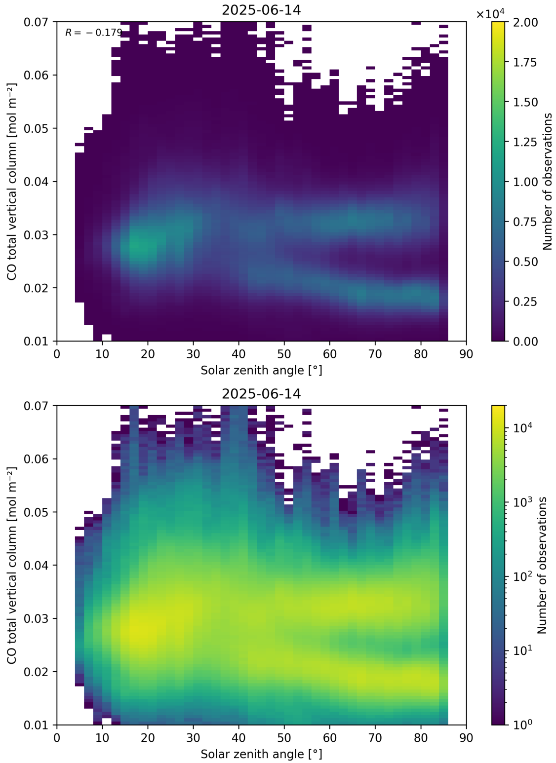
Figure 61: Scatter density plot of “Solar zenith angle” against “CO total vertical column” for 2025-06-13 to 2025-06-15.
