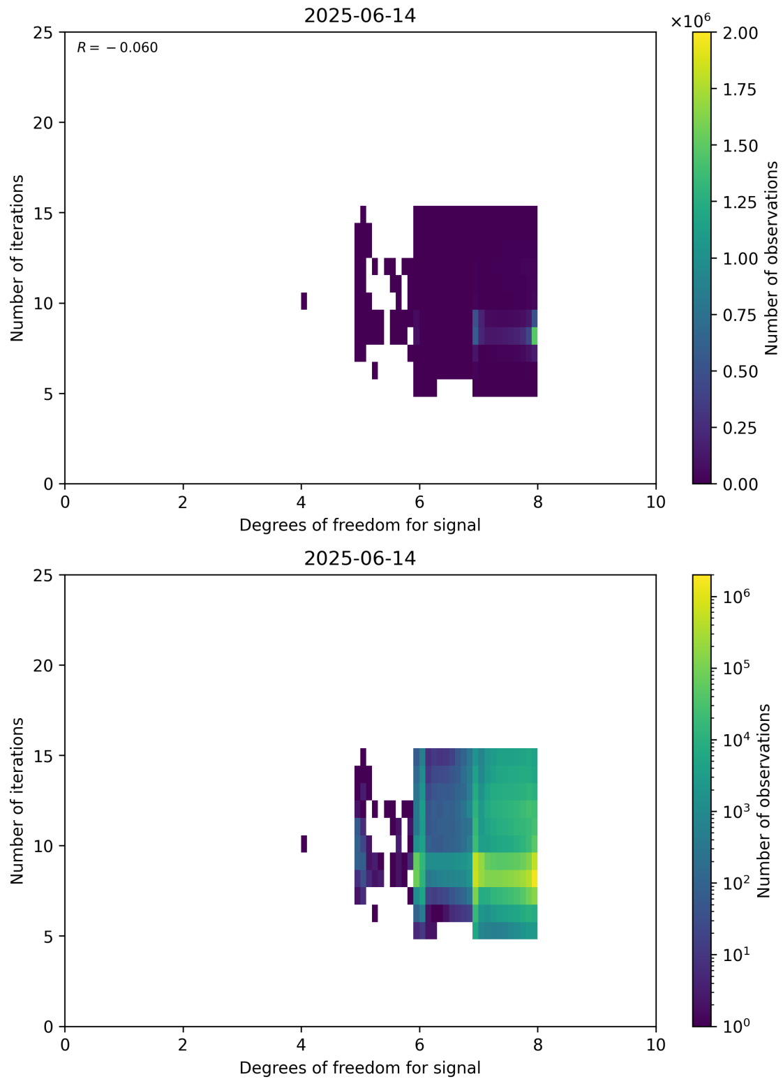
Figure 50: Scatter density plot of “Degrees of freedom for signal” against “Number of iterations” for 2025-06-13 to 2025-06-15.
