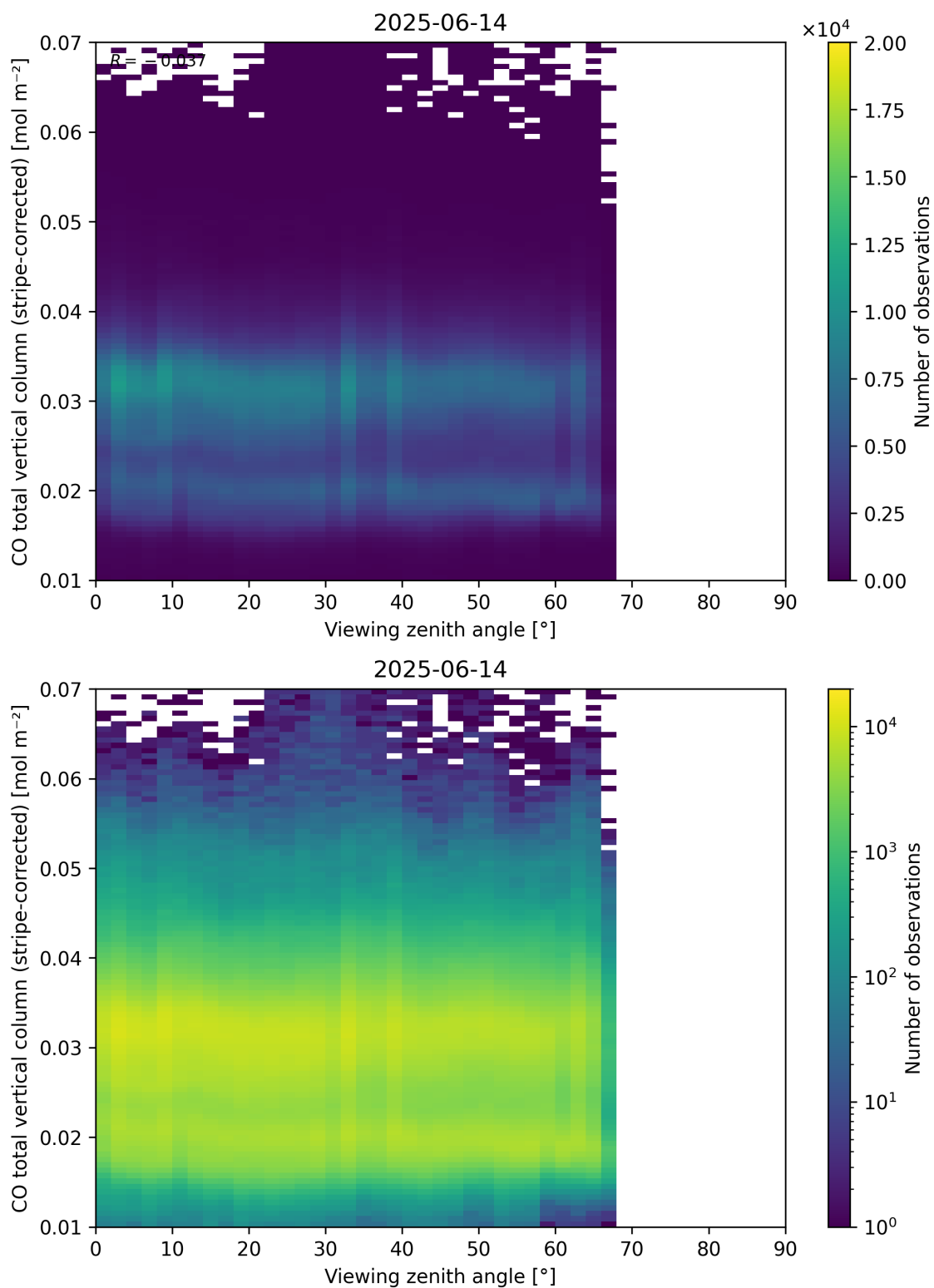
Figure 70: Scatter density plot of “Viewing zenith angle” against “CO total vertical column (stripe-corrected)” for 2025-06-13 to 2025-06-15.
