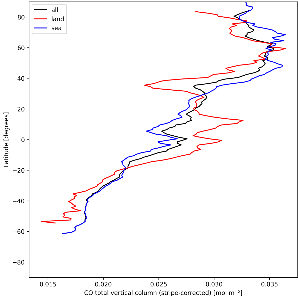
Figure 11: Zonal average of “CO total vertical column (stripe-corrected)” for 2025-06-13 to 2025-06-15.
