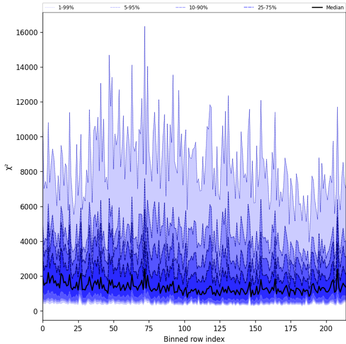
Figure 30: Along track statistics of “ \chi^2 ” for 2025-06-13 to 2025-06-15
