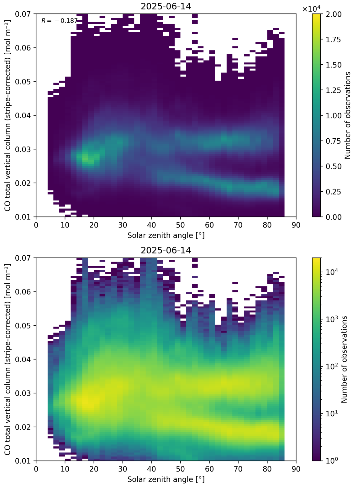
Figure 62: Scatter density plot of “Solar zenith angle” against “CO total vertical column (stripe-corrected)” for 2025-06-13 to 2025-06-15.
