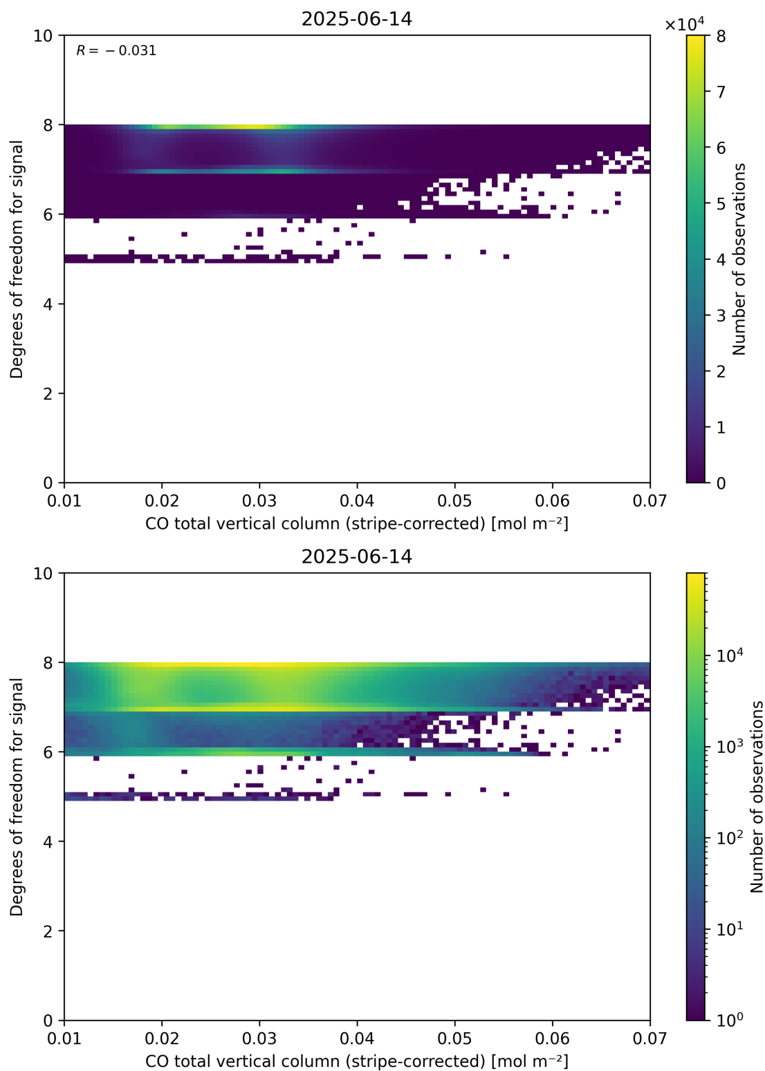
Figure 38: Scatter density plot of “CO total vertical column (stripe-corrected)” against “Degrees of freedom for signal” for 2025-06-13 to 2025-06-15.
