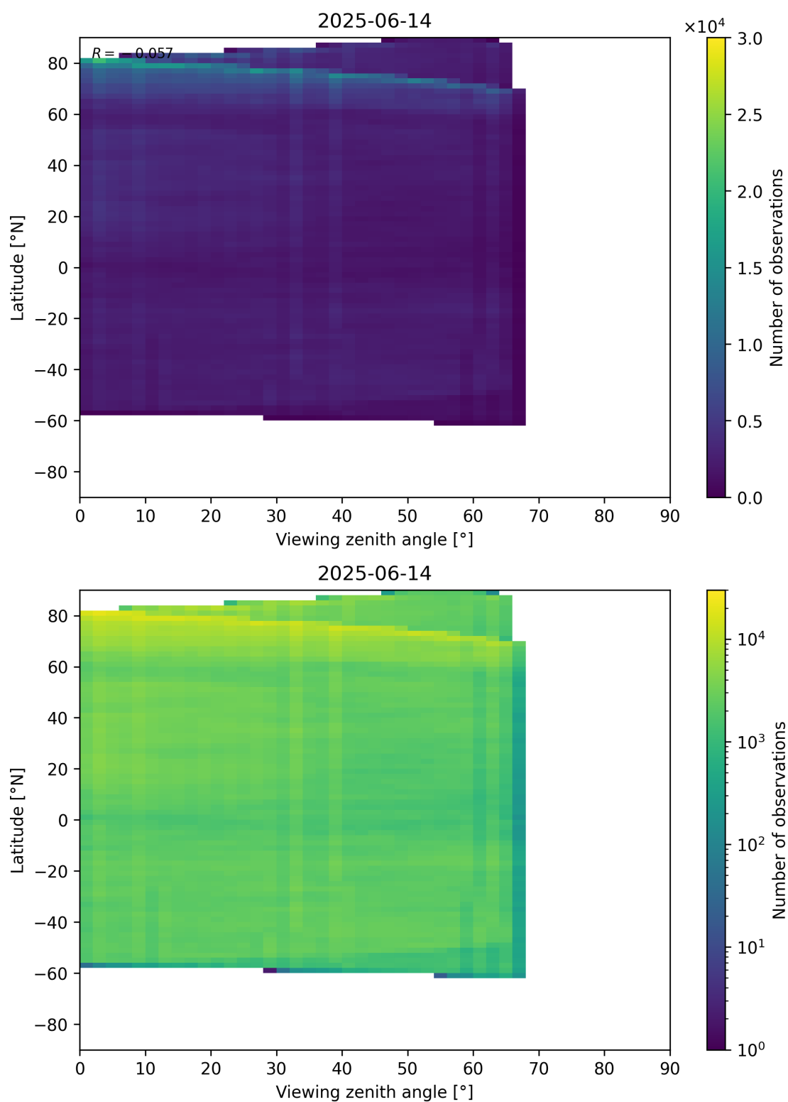
Figure 74: Scatter density plot of “Viewing zenith angle” against “Latitude” for 2025-06-13 to 2025-06-15.
