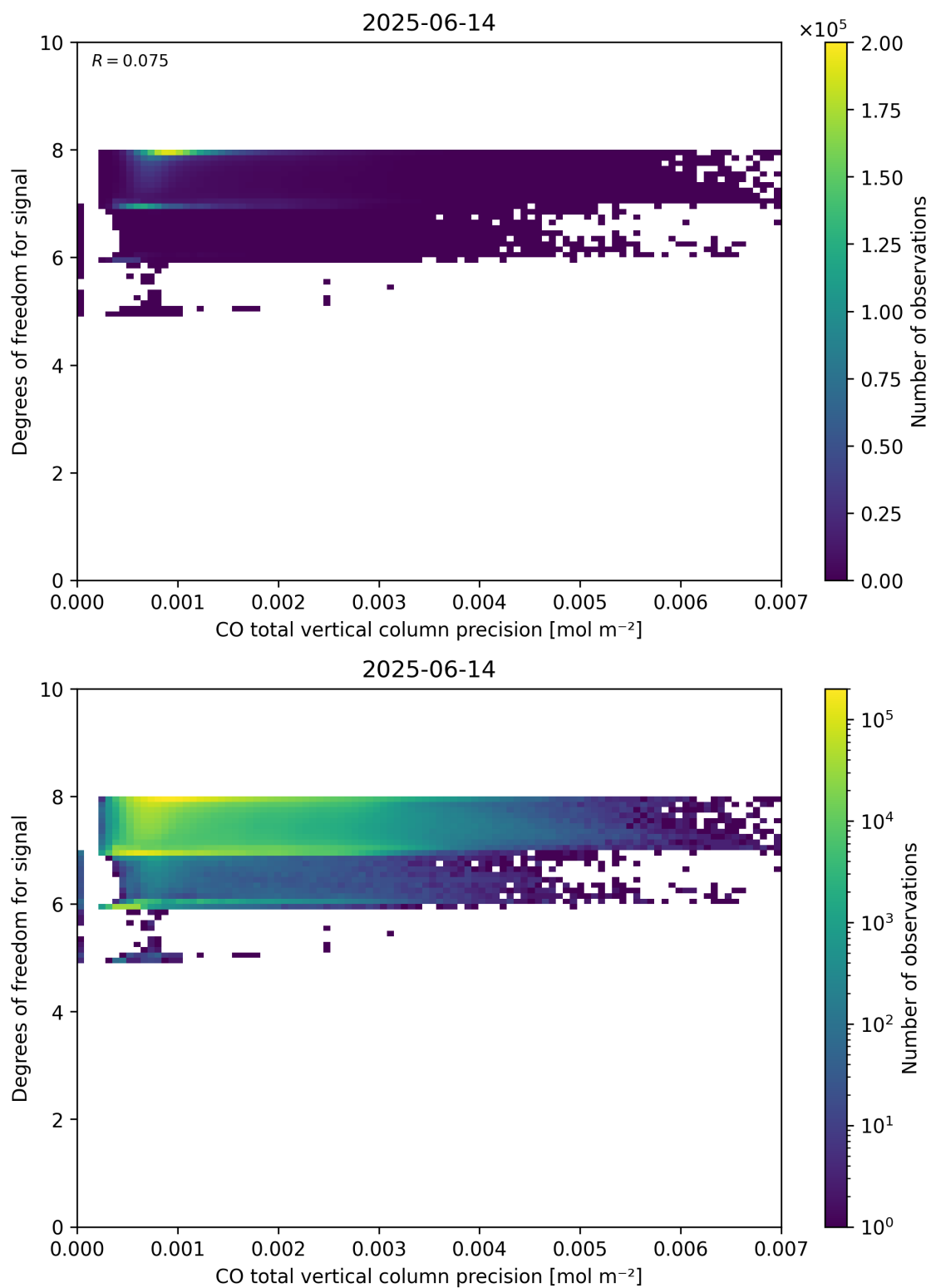
Figure 45: Scatter density plot of “CO total vertical column precision” against “Degrees of freedom for signal” for 2025-06-13 to 2025-06-15.
