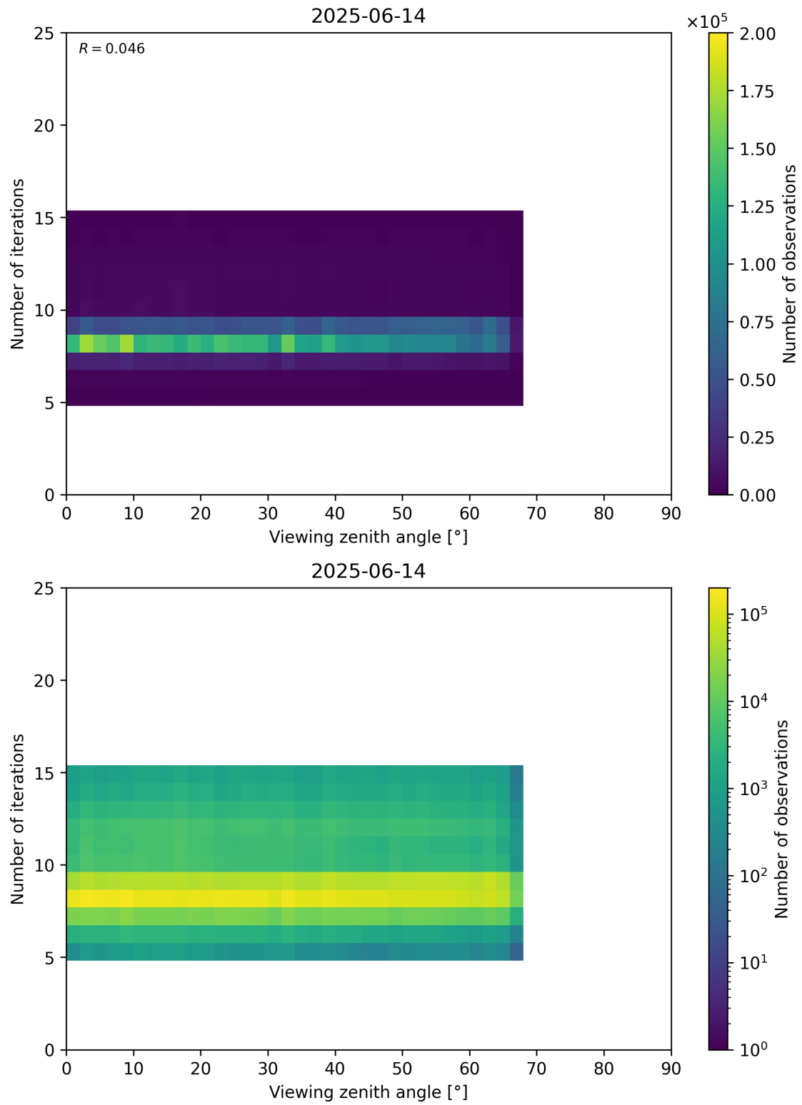
Figure 75: Scatter density plot of “Viewing zenith angle” against “Number of iterations” for 2025-06-13 to 2025-06-15.
