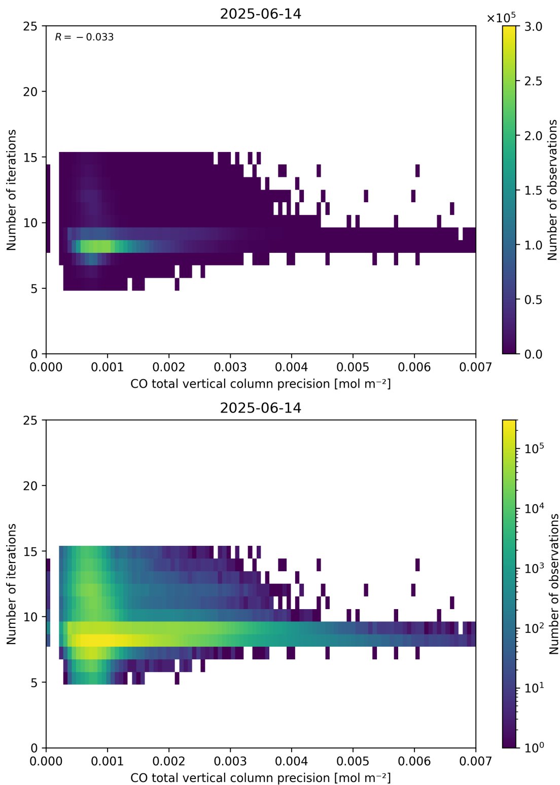
Figure 46: Scatter density plot of “CO total vertical column precision” against “Number of iterations” for 2025-06-13 to 2025-06-15.
