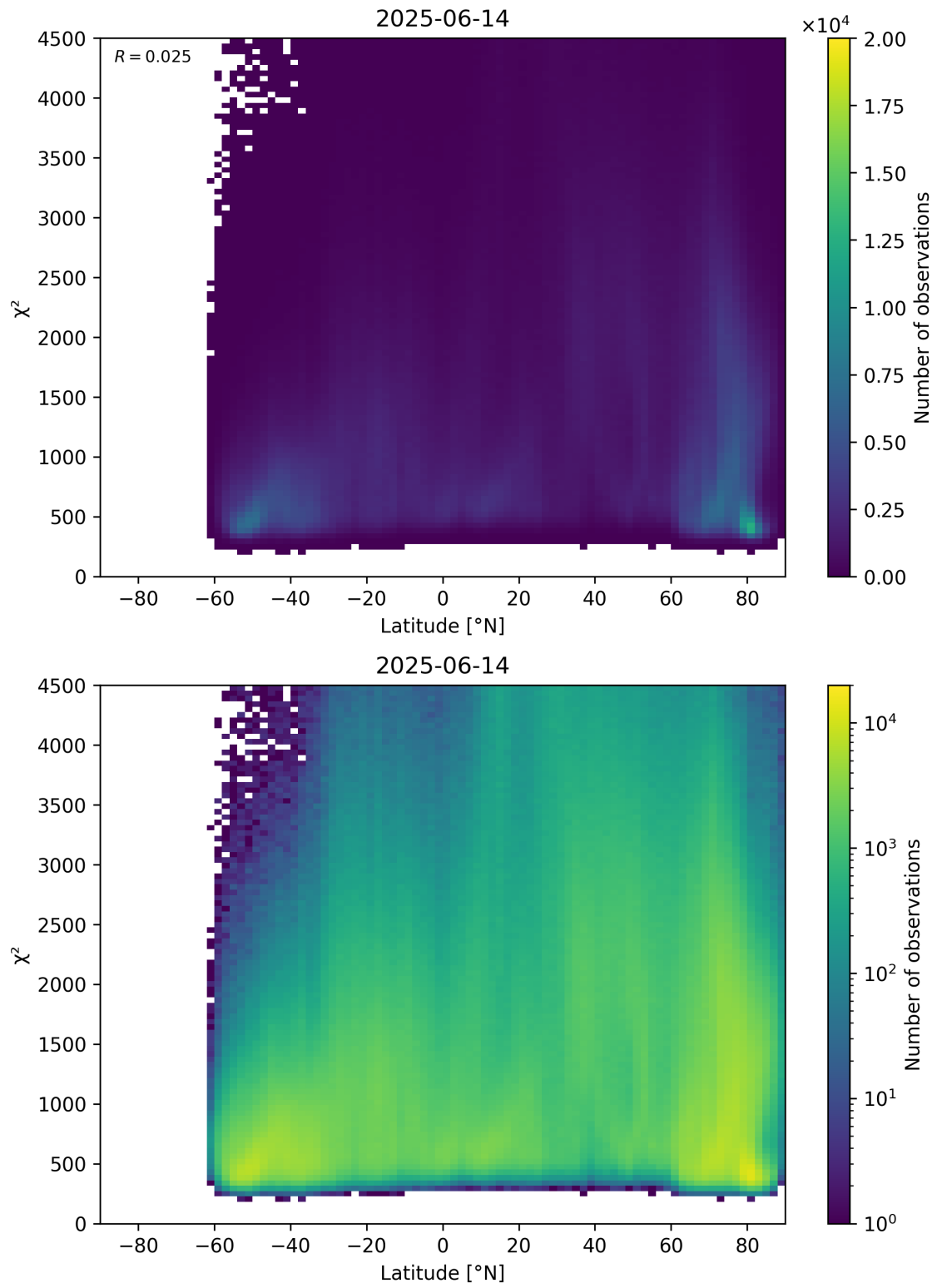
Figure 54: Scatter density plot of “Latitude” against “ \chi^2 ” for 2025-06-13 to 2025-06-15.
