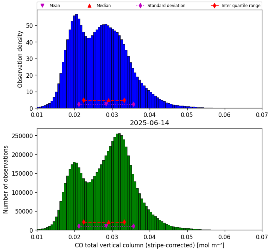
Figure 19: Histogram of “CO total vertical column (stripe-corrected)” for 2025-06-13 to 2025-06-15
