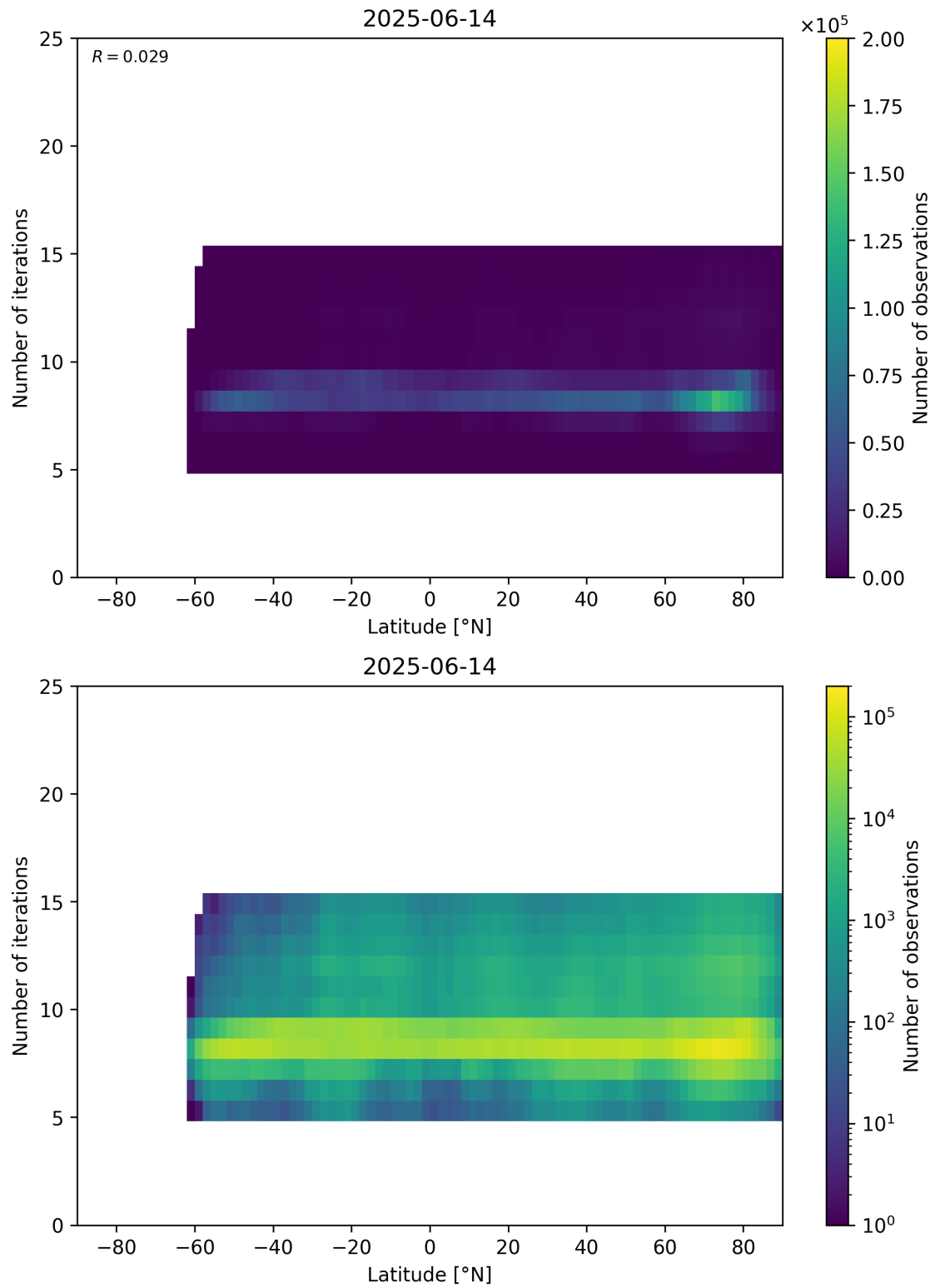
Figure 56: Scatter density plot of “Latitude” against “Number of iterations” for 2025-06-13 to 2025-06-15.
