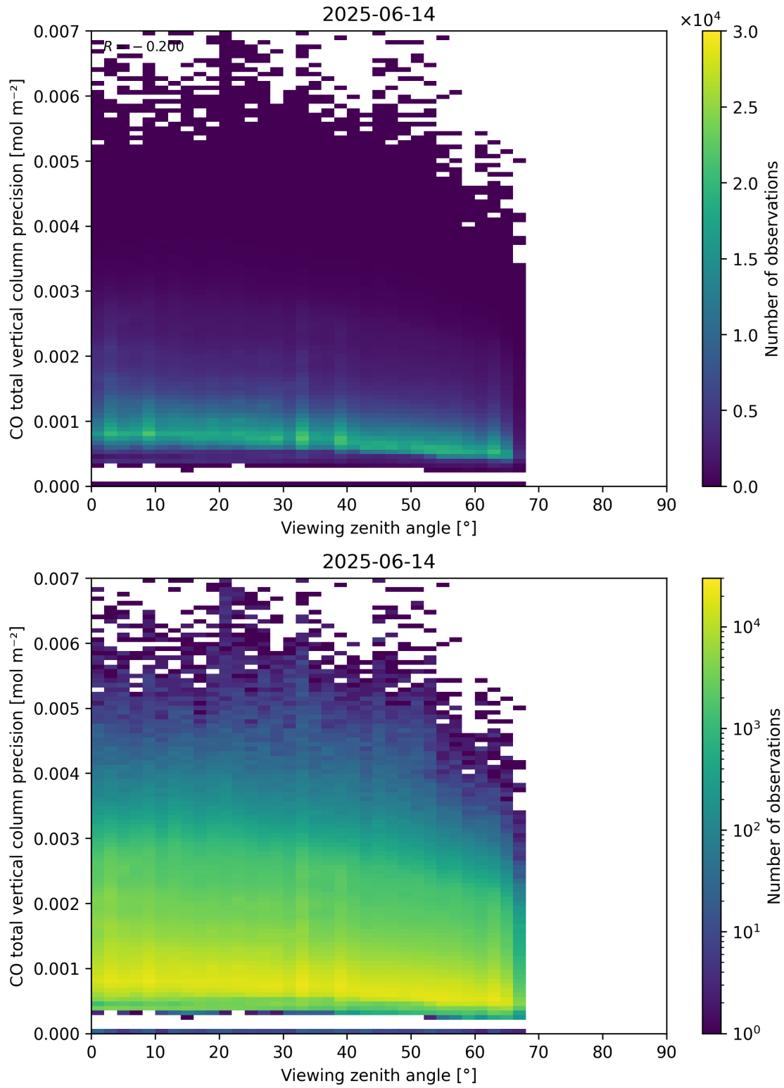
Figure 71: Scatter density plot of “Viewing zenith angle” against “CO total vertical column precision” for 2025-06-13 to 2025-06-15.
