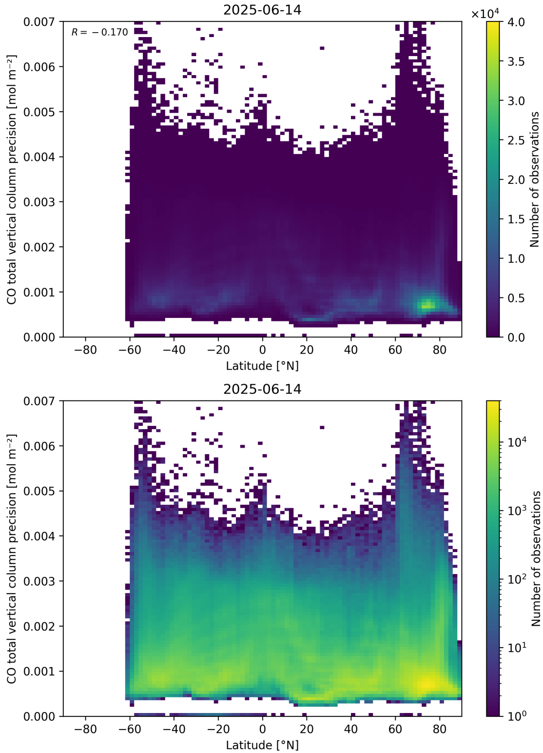
Figure 53: Scatter density plot of “Latitude” against “CO total vertical column precision” for 2025-06-13 to 2025-06-15.
