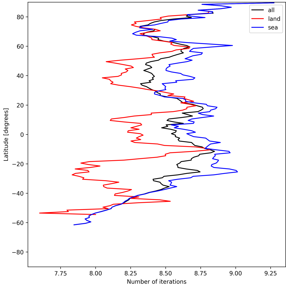
Figure 16: Zonal average of “Number of iterations” for 2025-06-13 to 2025-06-15.
