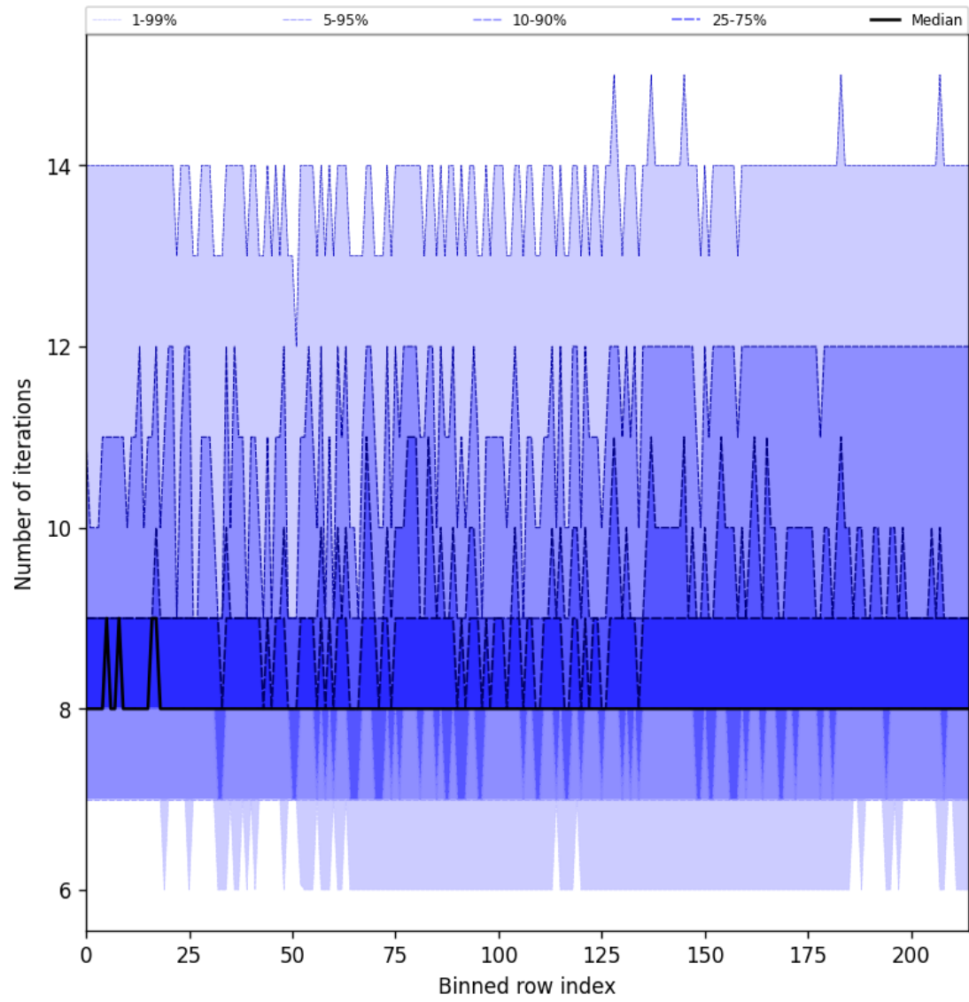
Figure 32: Along track statistics of “Number of iterations” for 2025-06-13 to 2025-06-15
