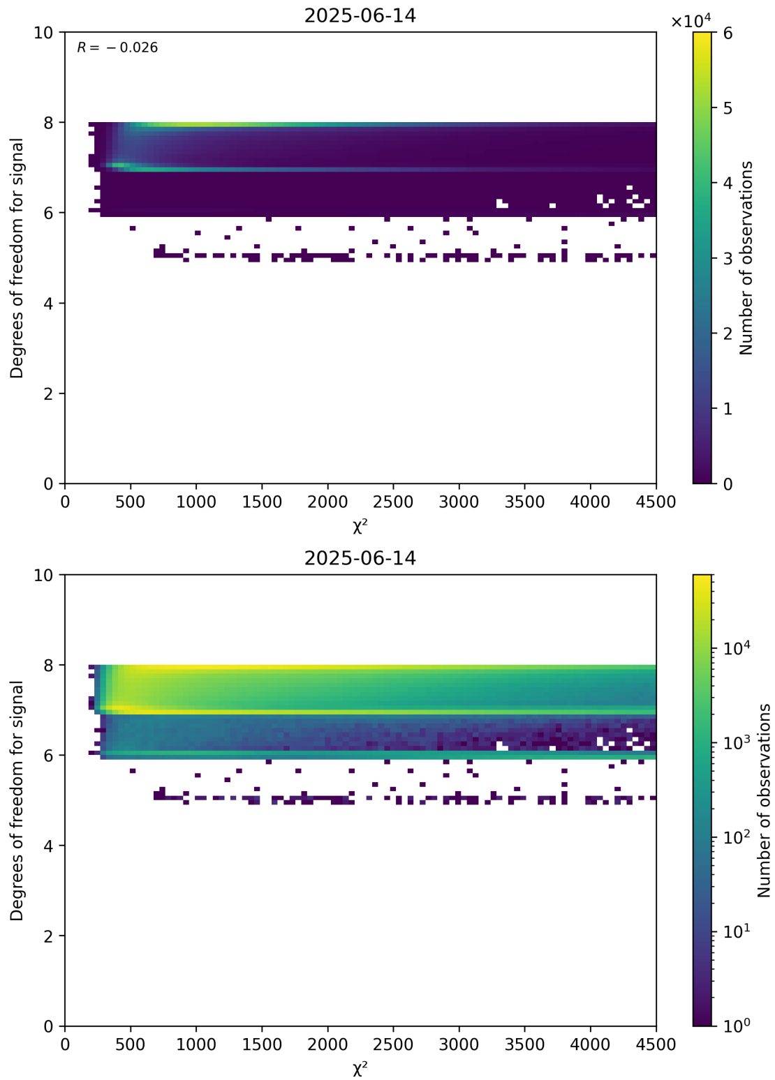
Figure 48: Scatter density plot of " \chi^2 " against "Degrees of freedom for signal" for 2025-06-13 to 2025-06-15.
