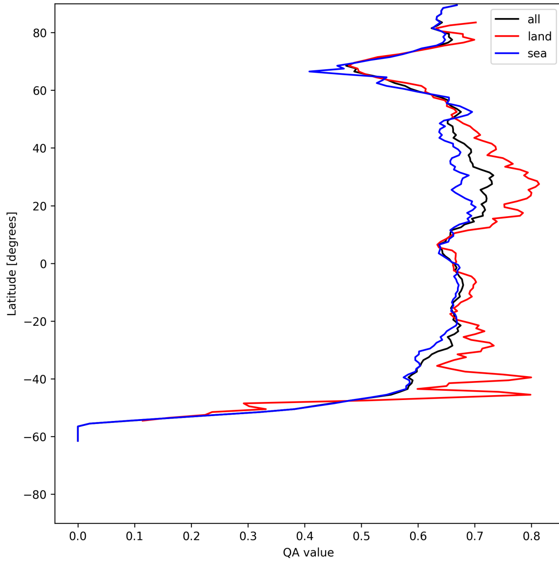
Figure 9: Zonal average of “QA value” for 2025-06-13 to 2025-06-15.
