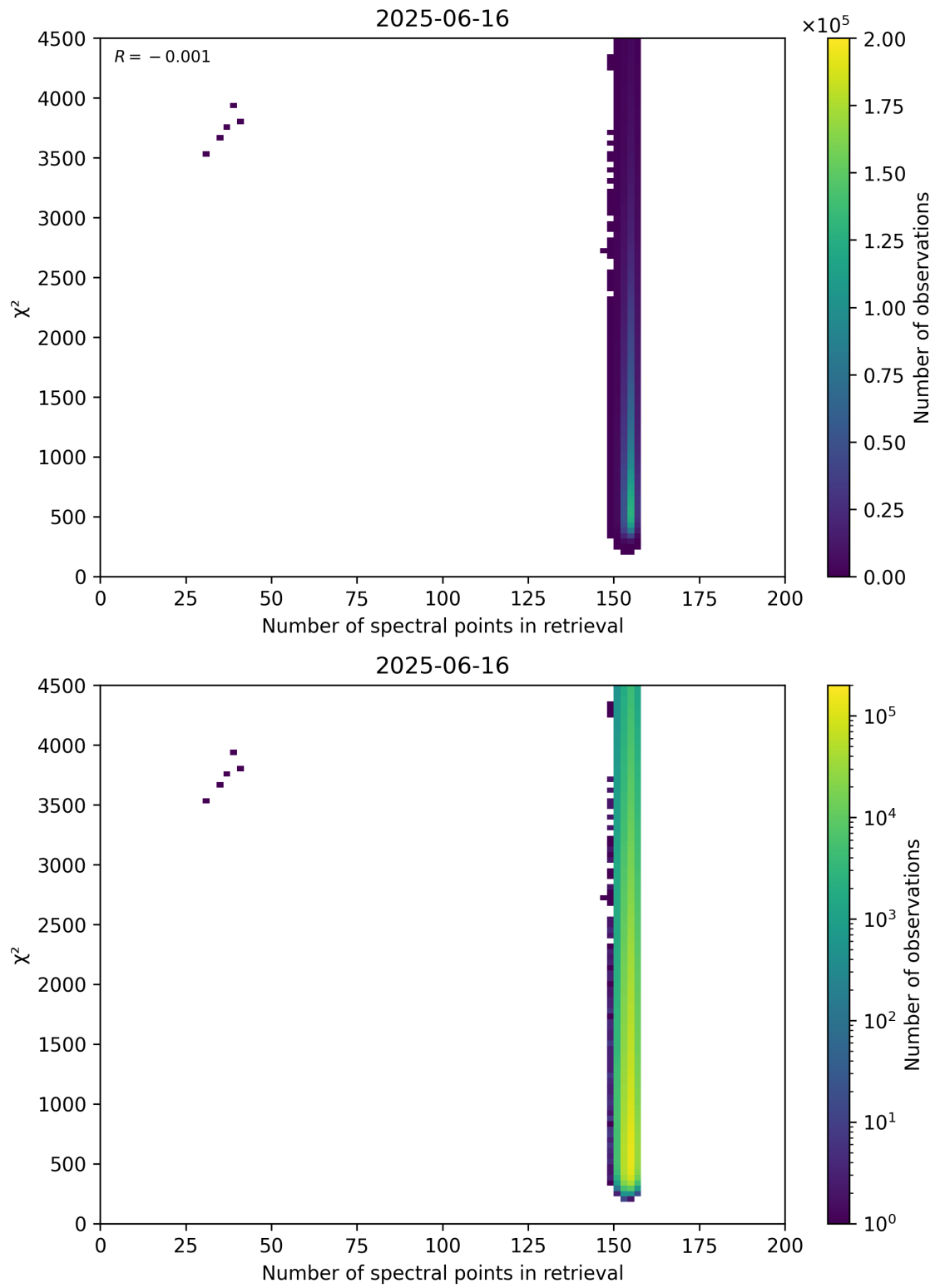
Figure 58: Scatter density plot of “Number of spectral points in retrieval” against “ \chi^2 ” for 2025-06-16 to 2025-06-17.
