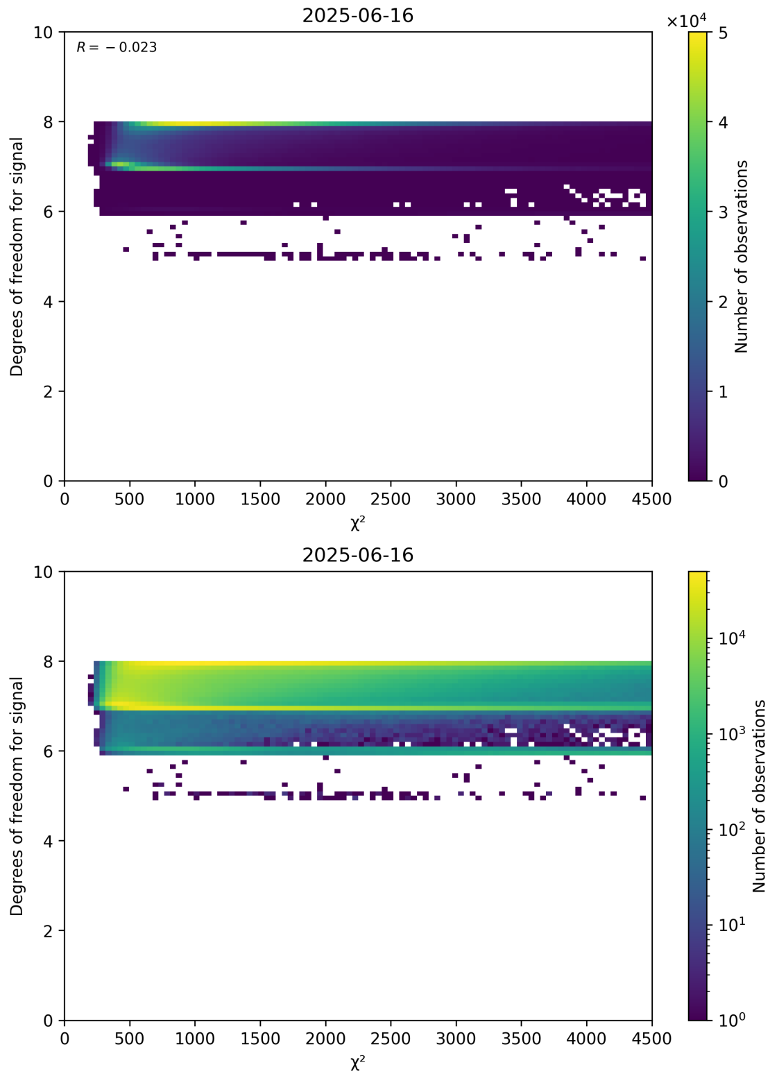
Figure 48: Scatter density plot of “ \chi^2 ” against “Degrees of freedom for signal” for 2025-06-16 to 2025-06-17.
