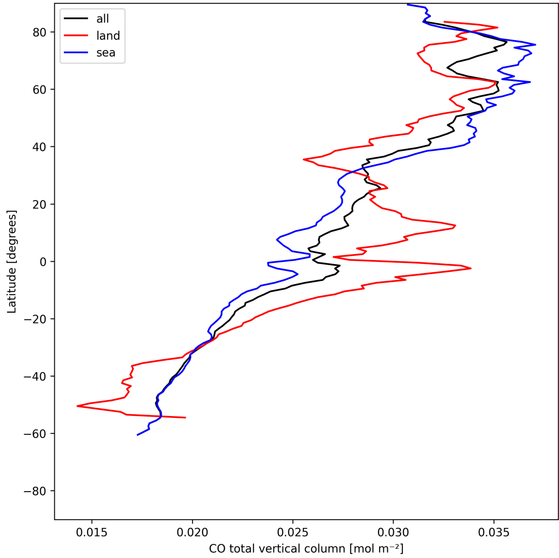
Figure 10: Zonal average of “CO total vertical column” for 2025-06-16 to 2025-06-17.
