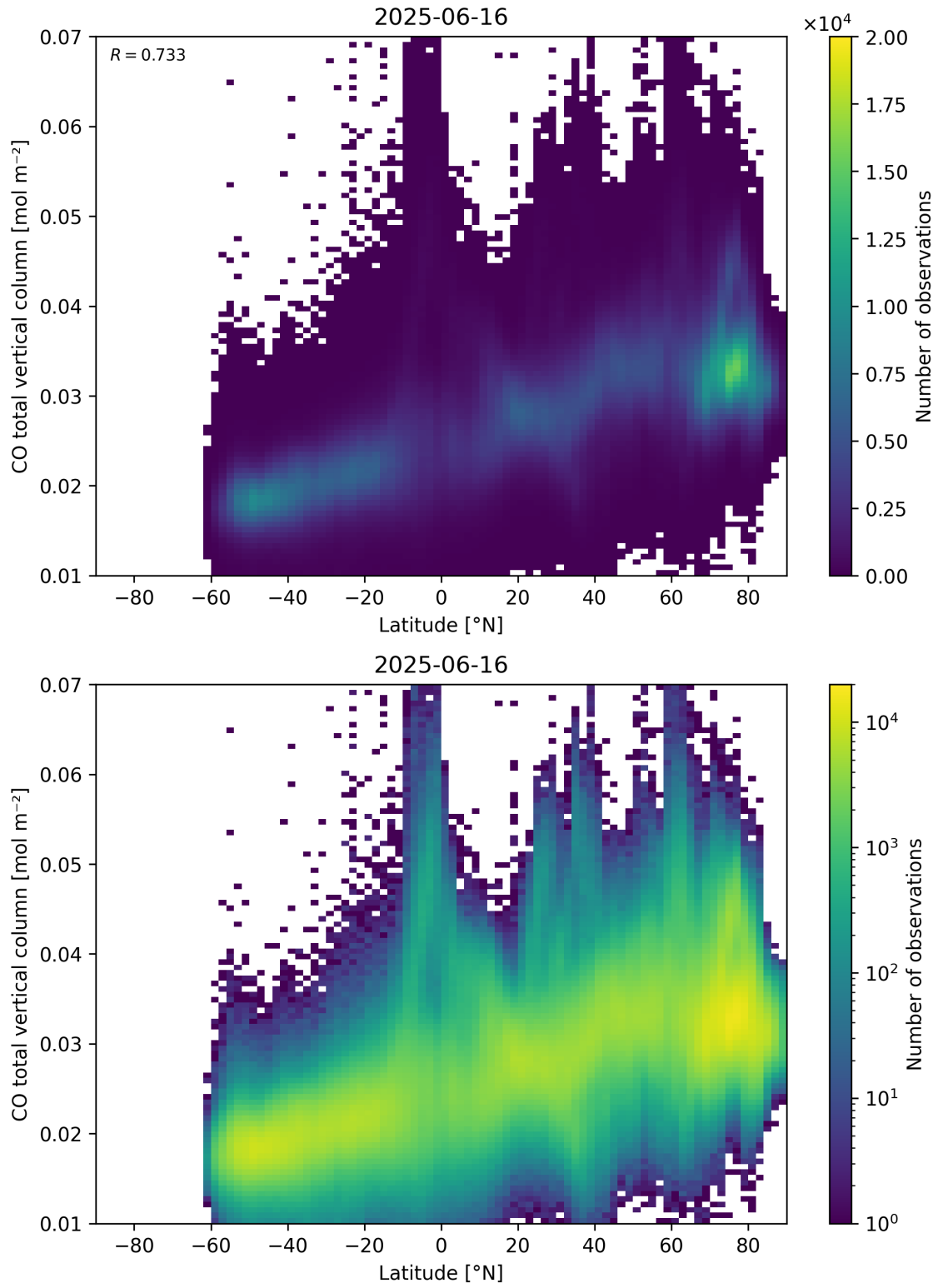
Figure 51: Scatter density plot of “Latitude” against “CO total vertical column” for 2025-06-16 to 2025-06-17.
