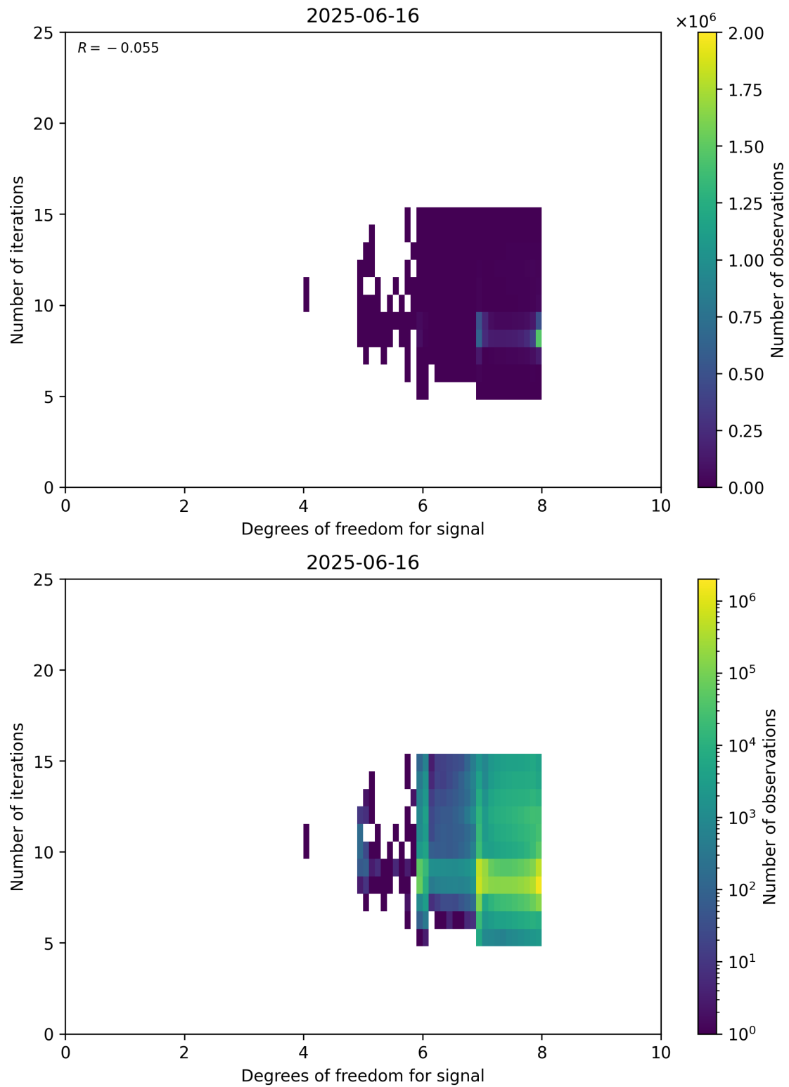
Figure 50: Scatter density plot of “Degrees of freedom for signal” against “Number of iterations” for 2025-06-16 to 2025-06-17.
