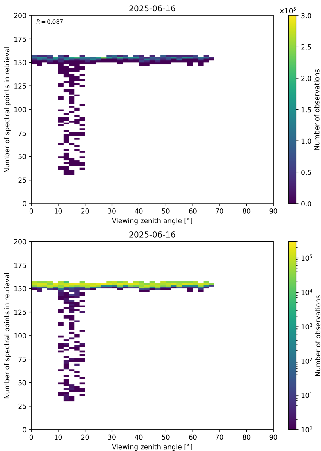
Figure 76: Scatter density plot of “Viewing zenith angle” against “Number of spectral points in retrieval” for 2025-06-16 to 2025-06-17.
