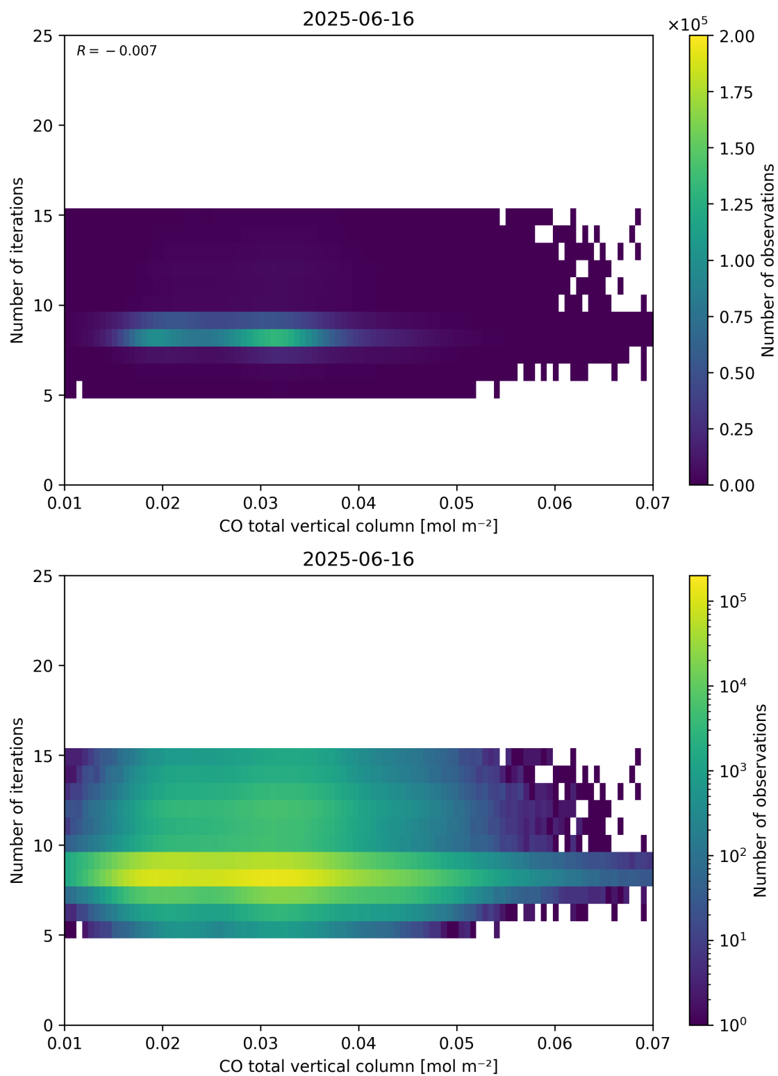
Figure 42: Scatter density plot of “CO total vertical column” against “Number of iterations” for 2025-06-16 to 2025-06-17.
