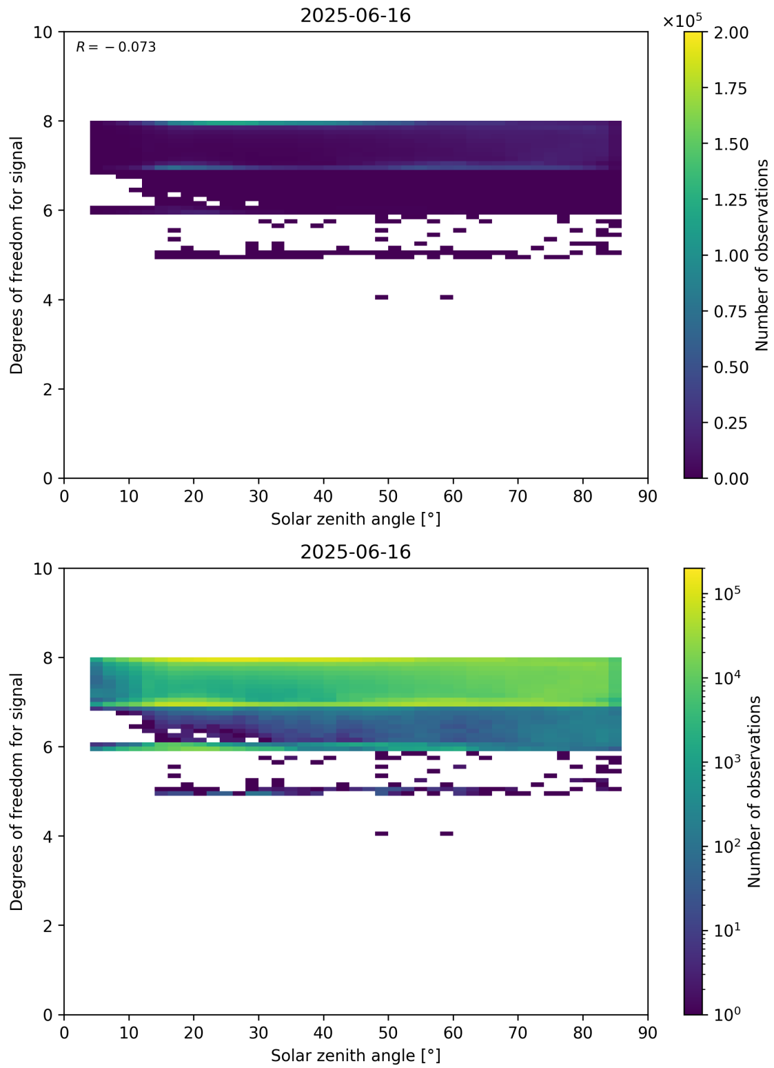
Figure 65: Scatter density plot of “Solar zenith angle” against “Degrees of freedom for signal” for 2025-06-16 to 2025-06-17.
