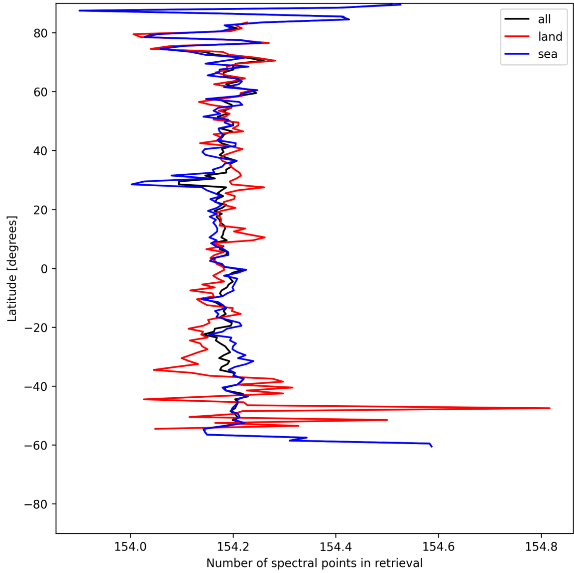
Figure 13: Zonal average of “Number of spectral points in retrieval” for 2025-06-16 to 2025-06-17.
