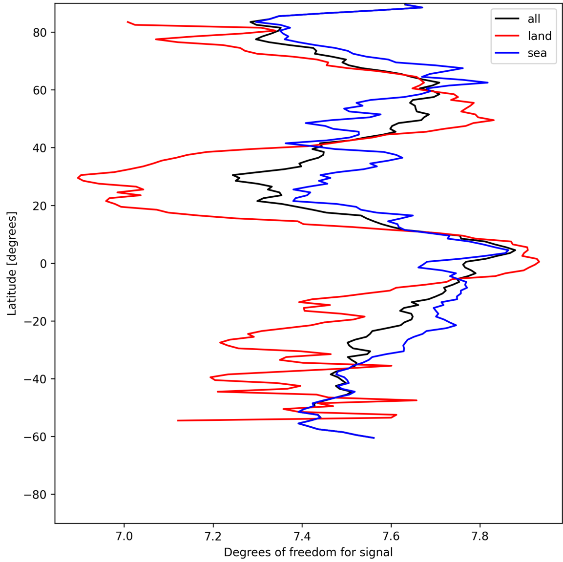
Figure 15: Zonal average of “Degrees of freedom for signal” for 2025-06-16 to 2025-06-17.
