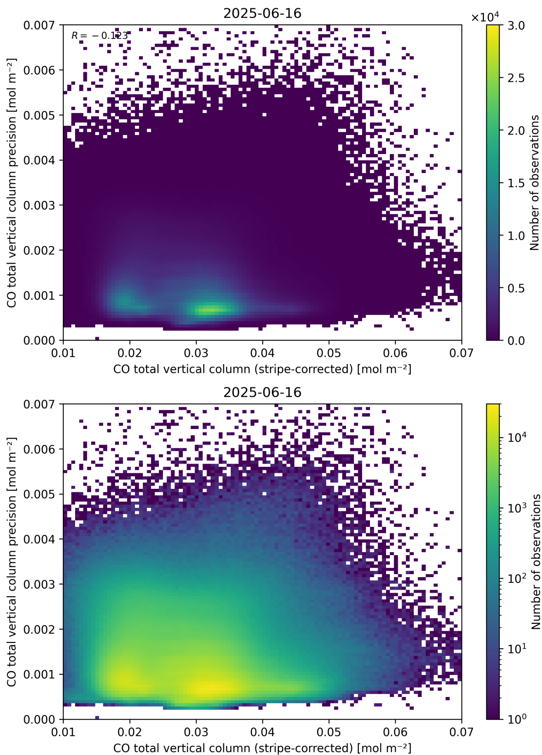
Figure 36: Scatter density plot of “CO total vertical column (stripe-corrected)” against “CO total vertical column precision” for 2025-06-16 to 2025-06-17.
