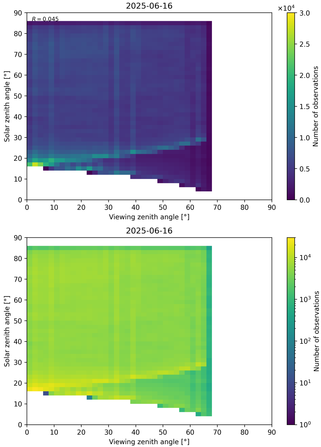
Figure 77: Scatter density plot of “Viewing zenith angle” against “Solar zenith angle” for 2025-06-16 to 2025-06-17.
