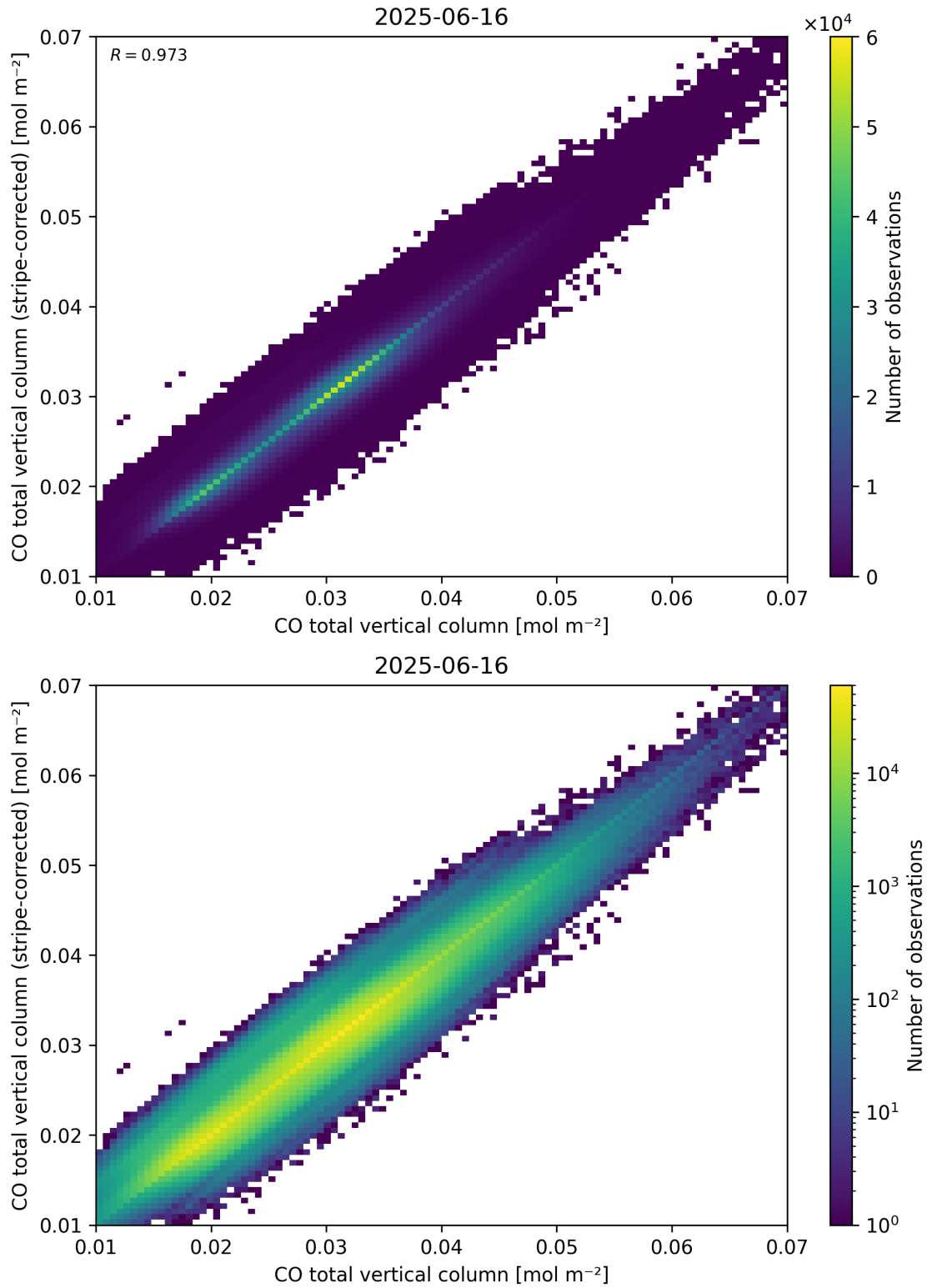
Figure 33: Scatter density plot of “CO total vertical column” against “CO total vertical column (stripe-corrected)” for 2025-06-16 to 2025-06-17.
