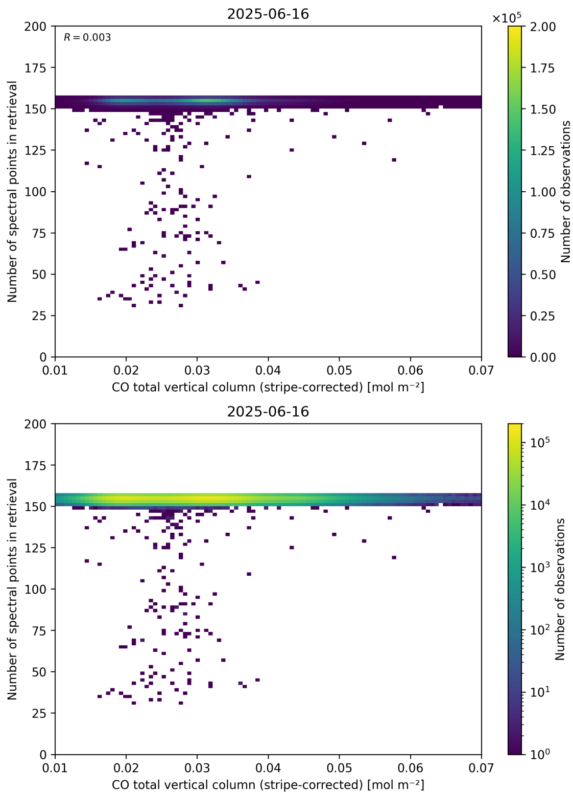
Figure 40: Scatter density plot of “CO total vertical column (stripe-corrected)” against “Number of spectral points in retrieval” for 2025-06-16 to 2025-06-17.
