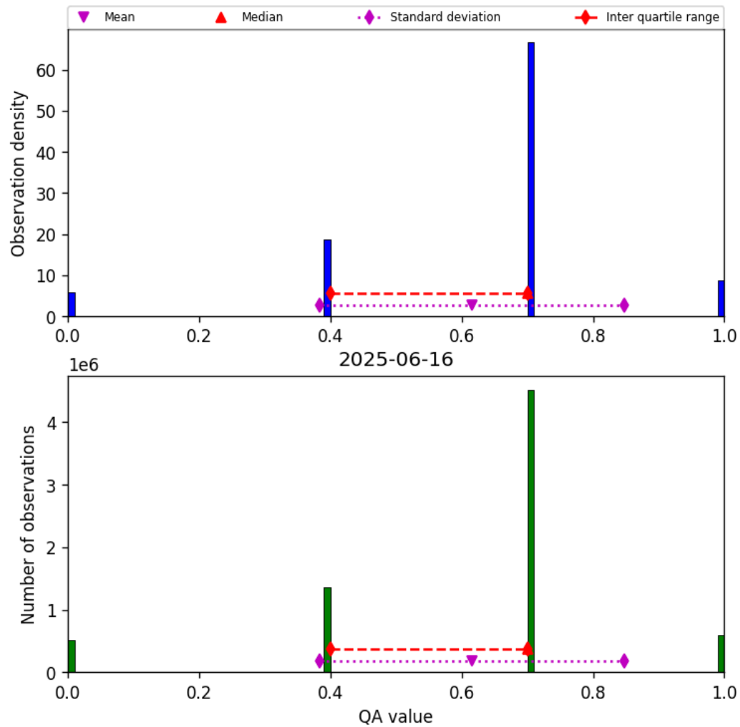
Figure 17: Histogram of “QA value” for 2025-06-16 to 2025-06-17
