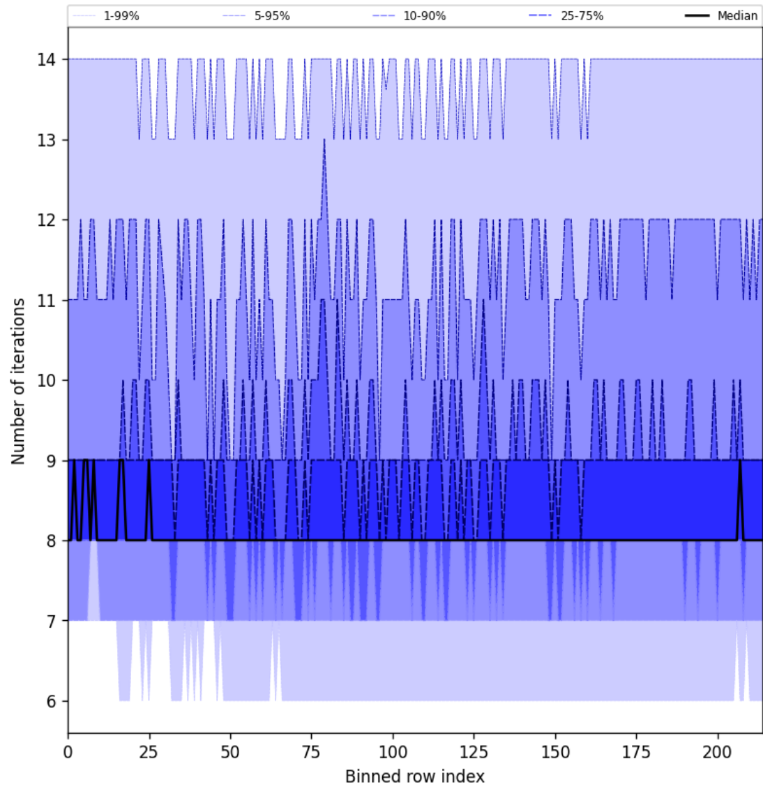
Figure 32: Along track statistics of “Number of iterations” for 2025-06-16 to 2025-06-17
