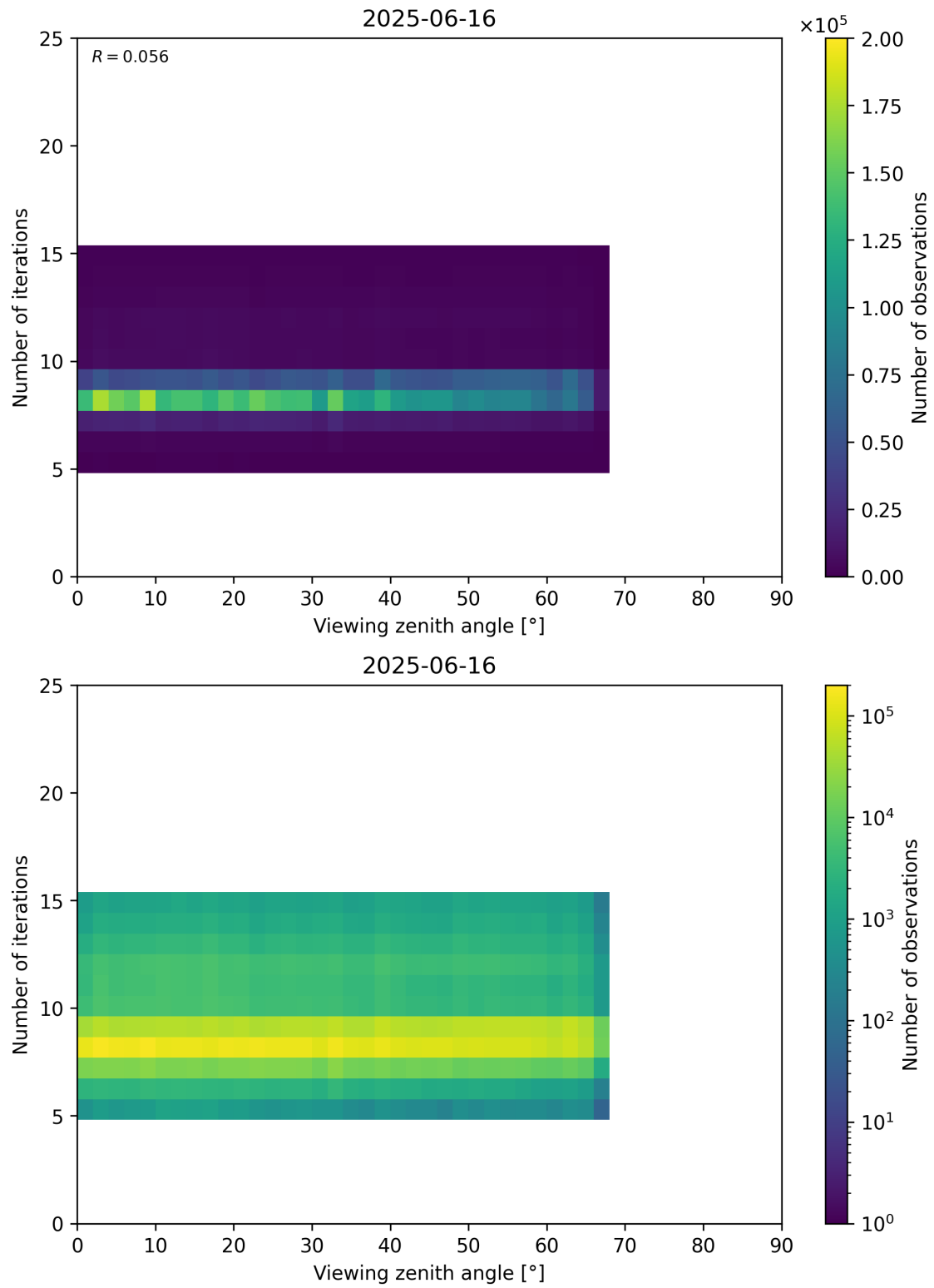
Figure 75: Scatter density plot of “Viewing zenith angle” against “Number of iterations” for 2025-06-16 to 2025-06-17.
