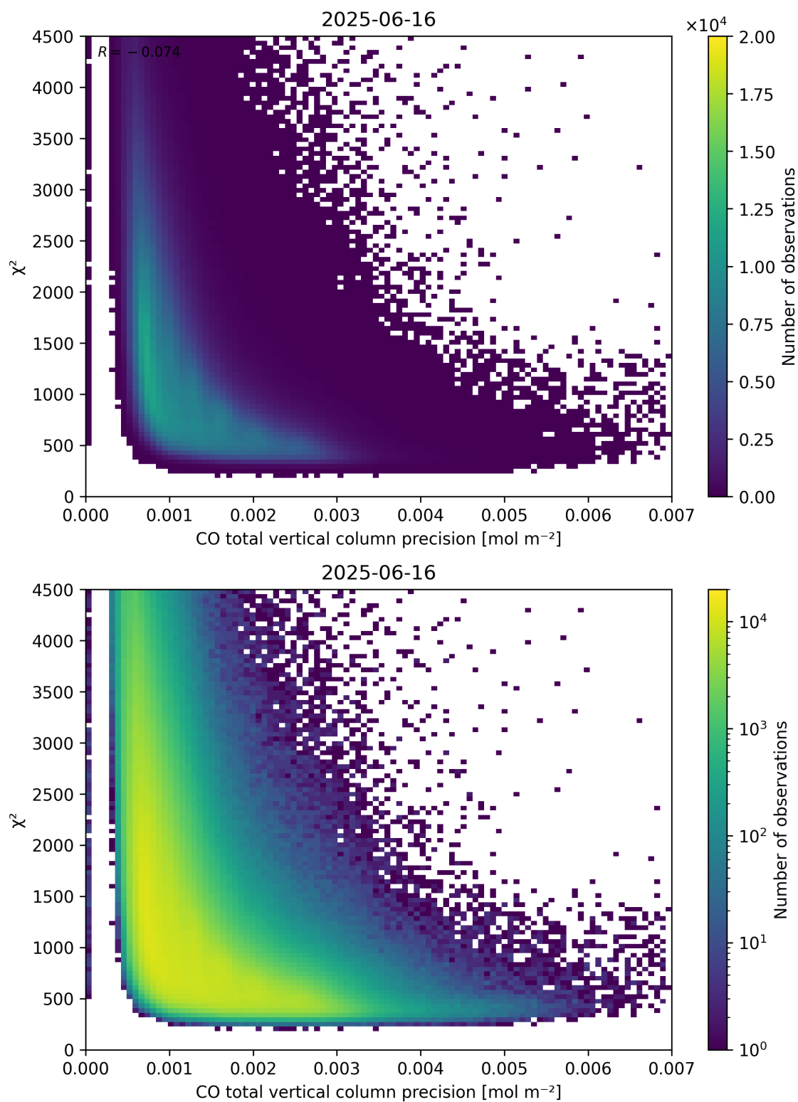
Figure 44: Scatter density plot of “CO total vertical column precision” against “ \chi^2 ” for 2025-06-16 to 2025-06-17.
