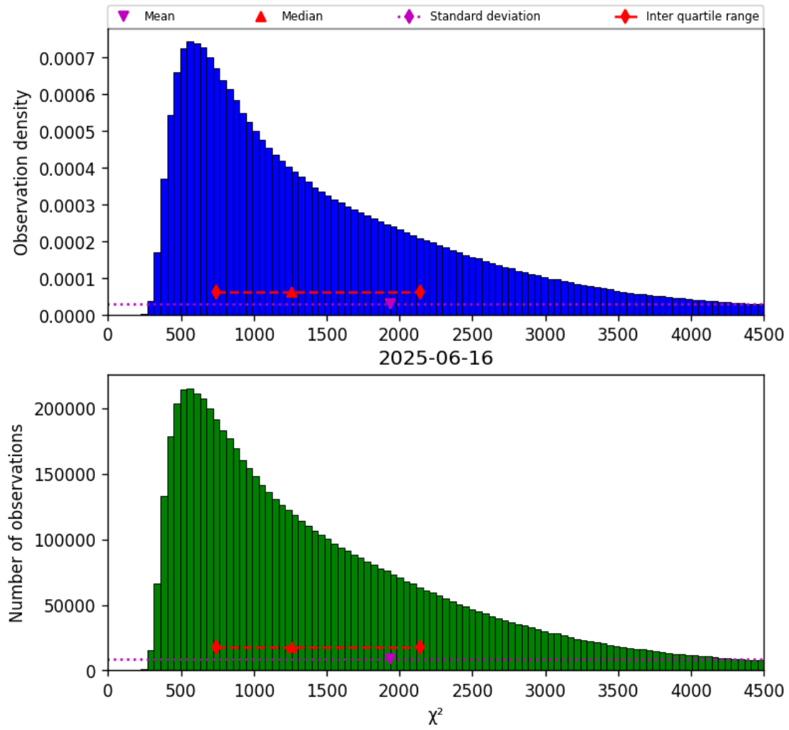
Figure 22: Histogram of “ \chi^2 ” for 2025-06-16 to 2025-06-17
