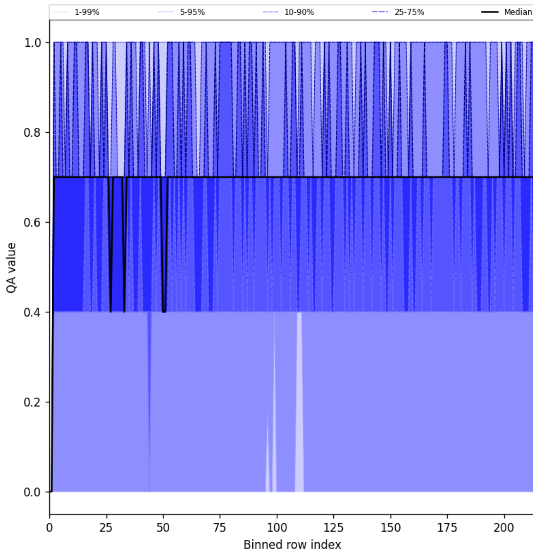
Figure 25: Along track statistics of “QA value” for 2025-06-16 to 2025-06-17
