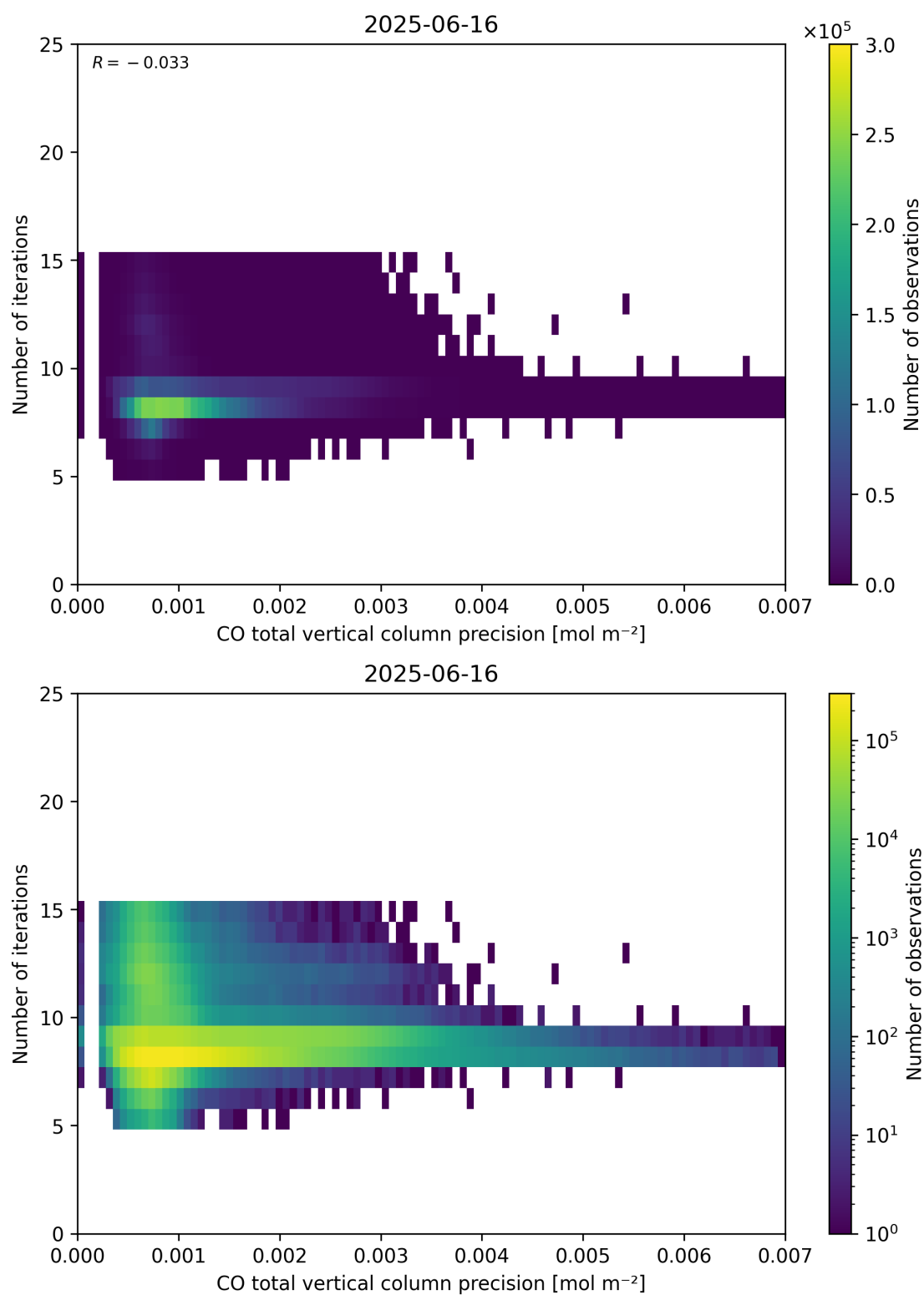
Figure 46: Scatter density plot of “CO total vertical column precision” against “Number of iterations” for 2025-06-16 to 2025-06-17.
