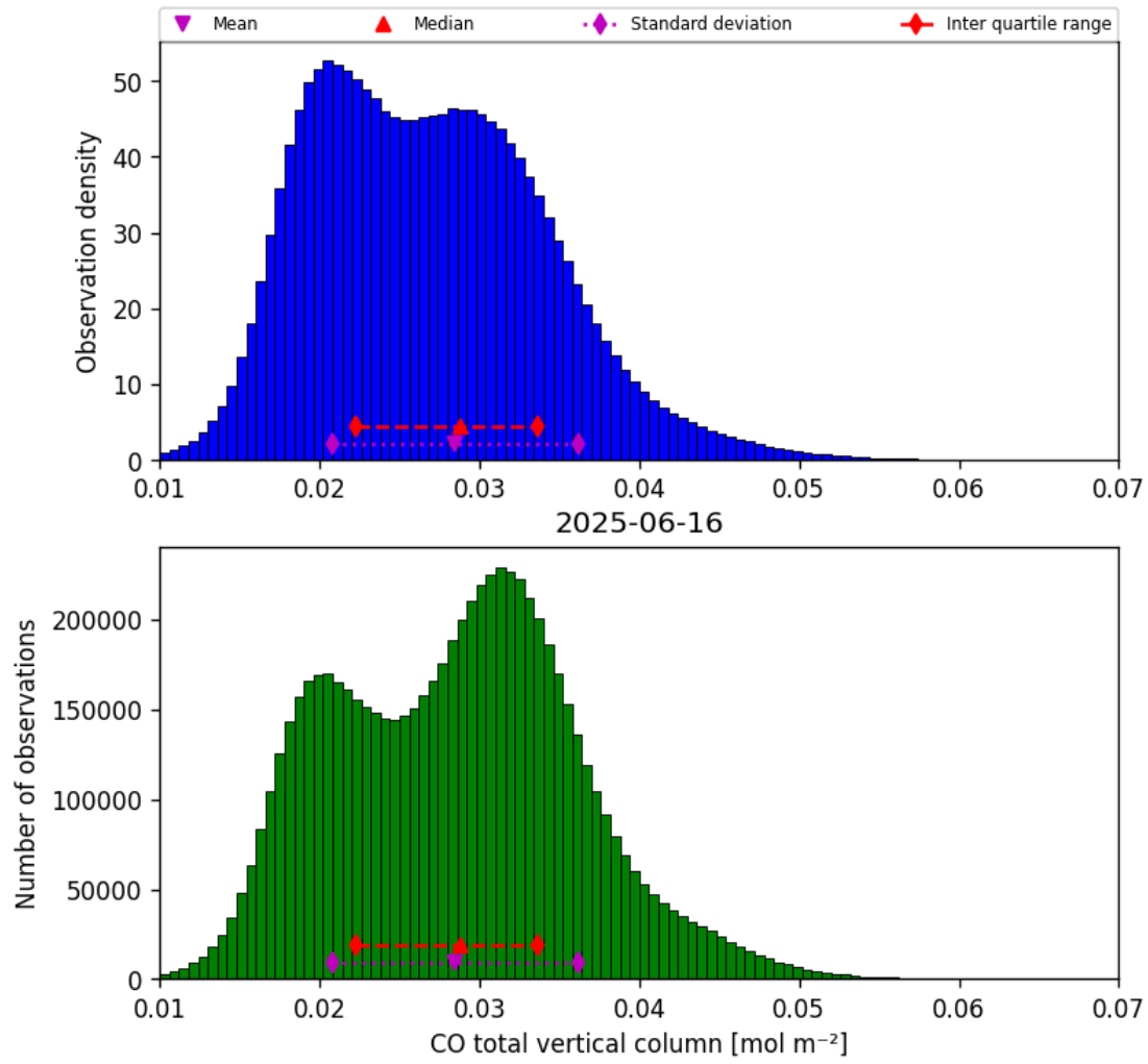
Figure 18: Histogram of “CO total vertical column” for 2025-06-16 to 2025-06-17
