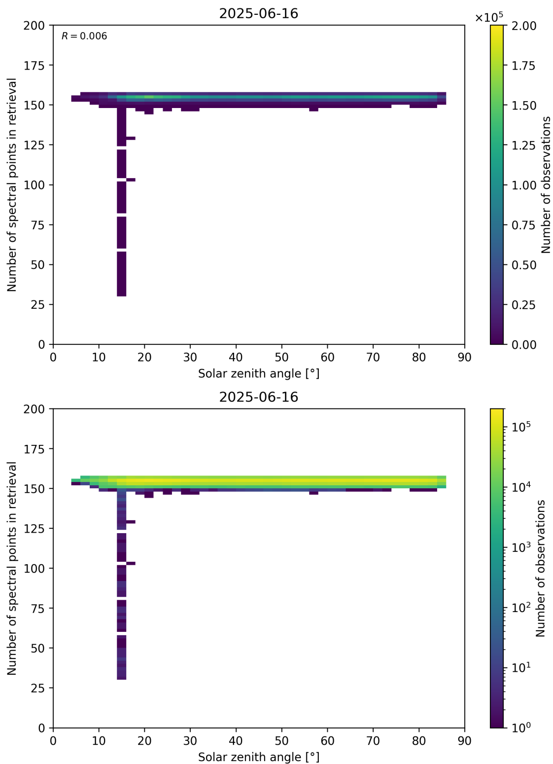
Figure 68: Scatter density plot of “Solar zenith angle” against “Number of spectral points in retrieval” for 2025-06-16 to 2025-06-17.
