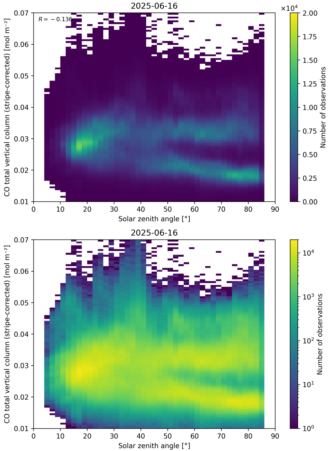
Figure 62: Scatter density plot of “Solar zenith angle” against “CO total vertical column (stripe-corrected)” for 2025-06-16 to 2025-06-17.
