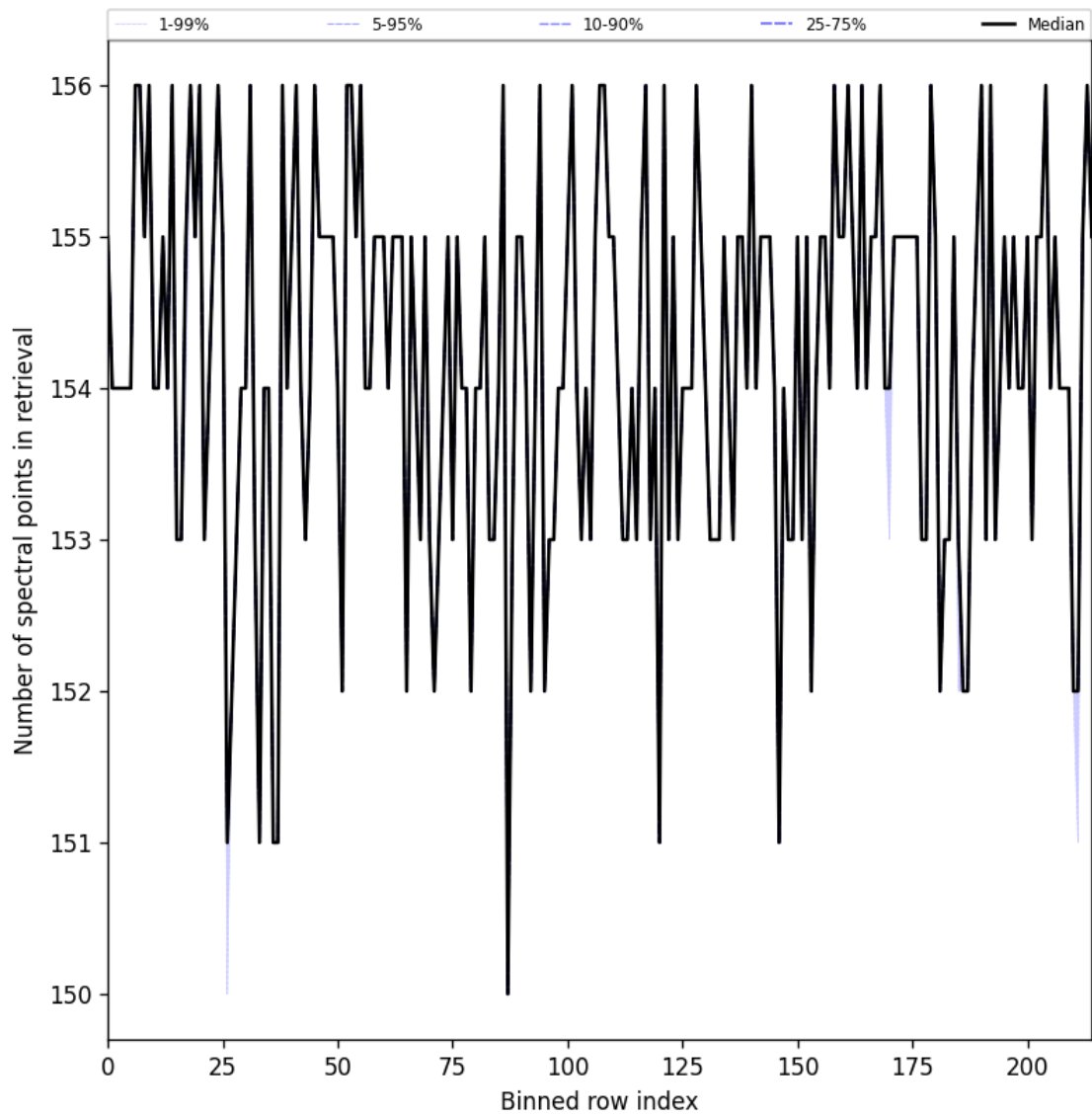
Figure 29: Along track statistics of “Number of spectral points in retrieval” for 2025-06-16 to 2025-06-17
