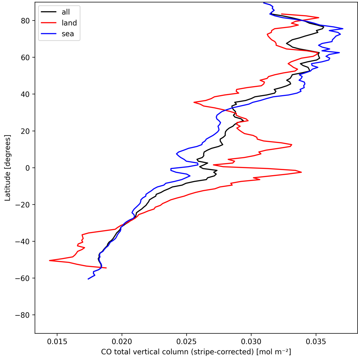
Figure 11: Zonal average of “CO total vertical column (stripe-corrected)” for 2025-06-16 to 2025-06-17.
