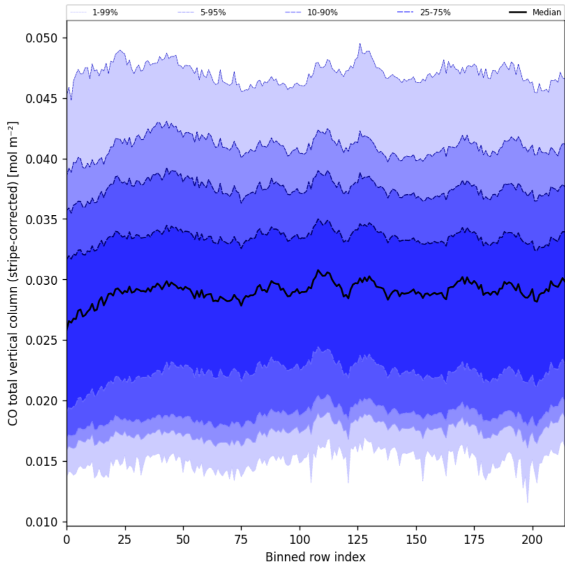
Figure 27: Along track statistics of “CO total vertical column (stripe-corrected)” for 2025-06-16 to 2025-06-17
