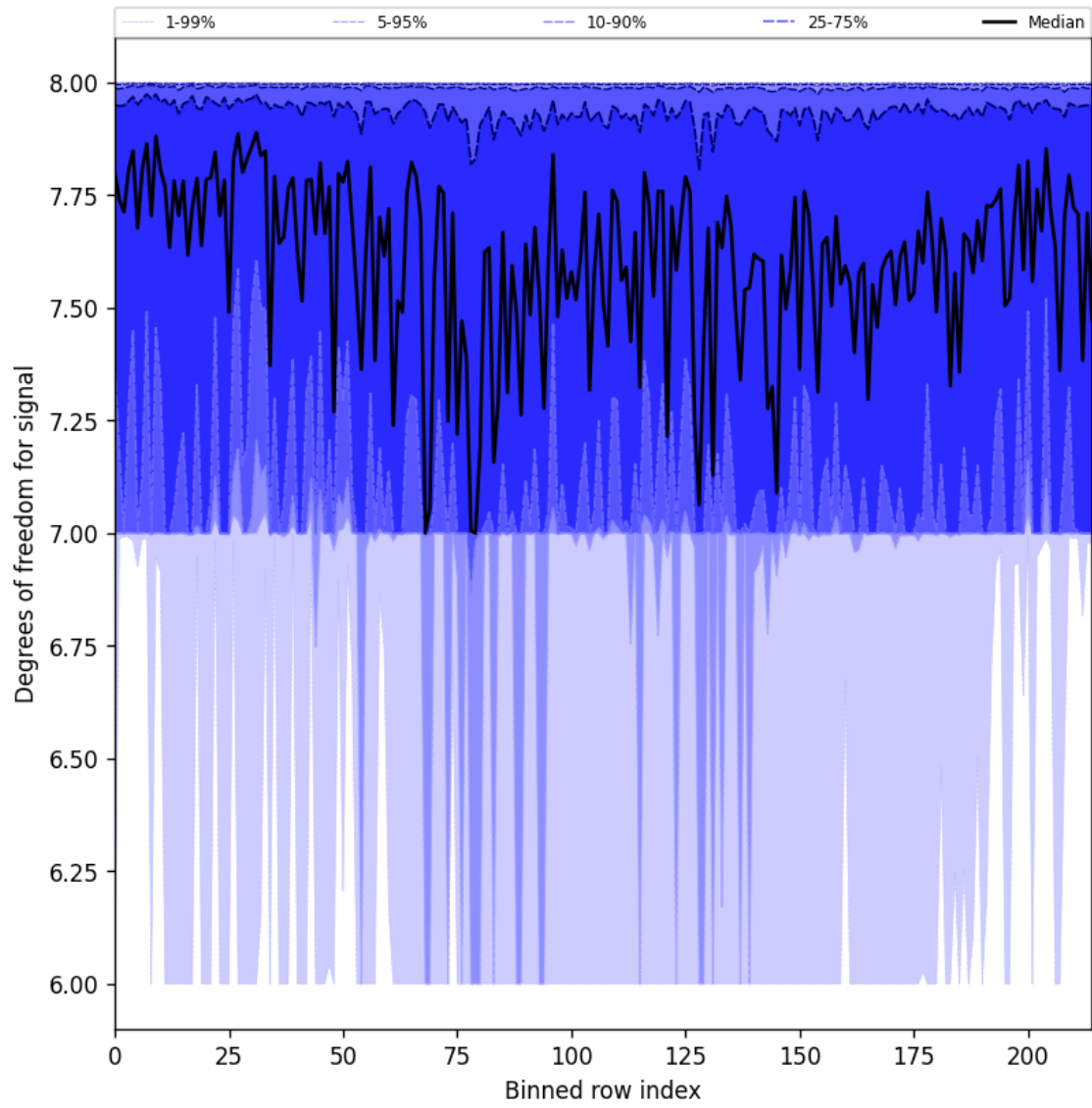
Figure 31: Along track statistics of “Degrees of freedom for signal” for 2025-06-16 to 2025-06-17
