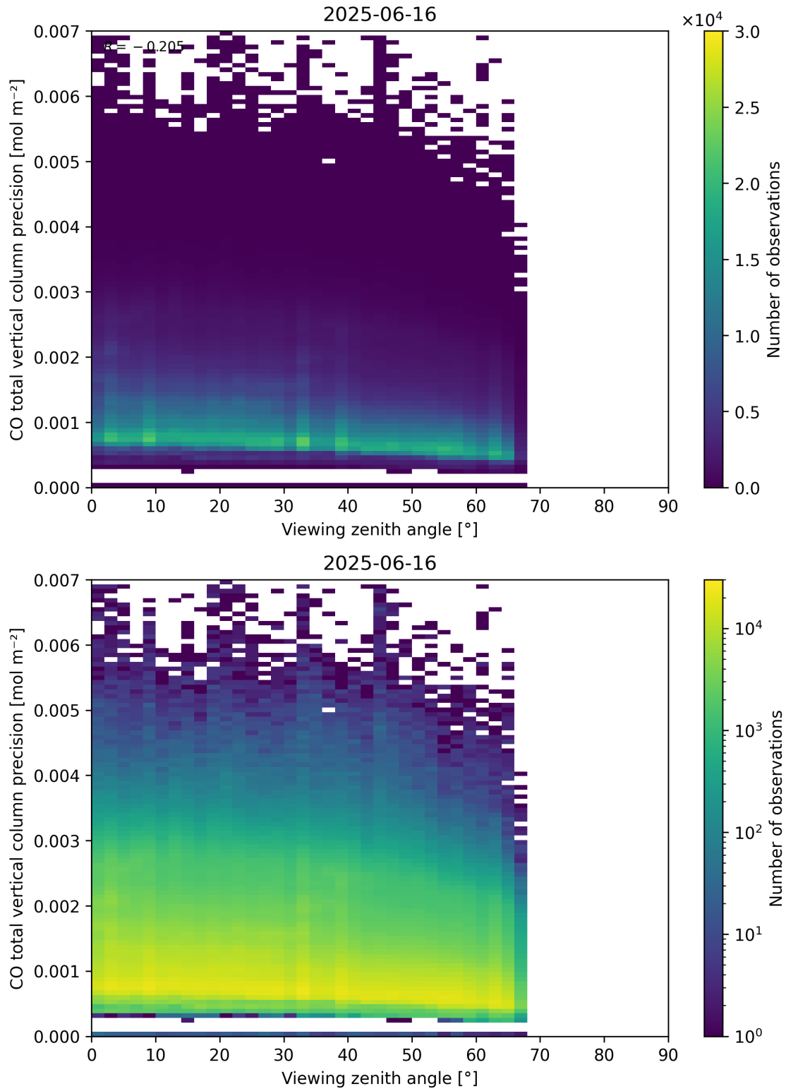
Figure 71: Scatter density plot of “Viewing zenith angle” against “CO total vertical column precision” for 2025-06-16 to 2025-06-17.
