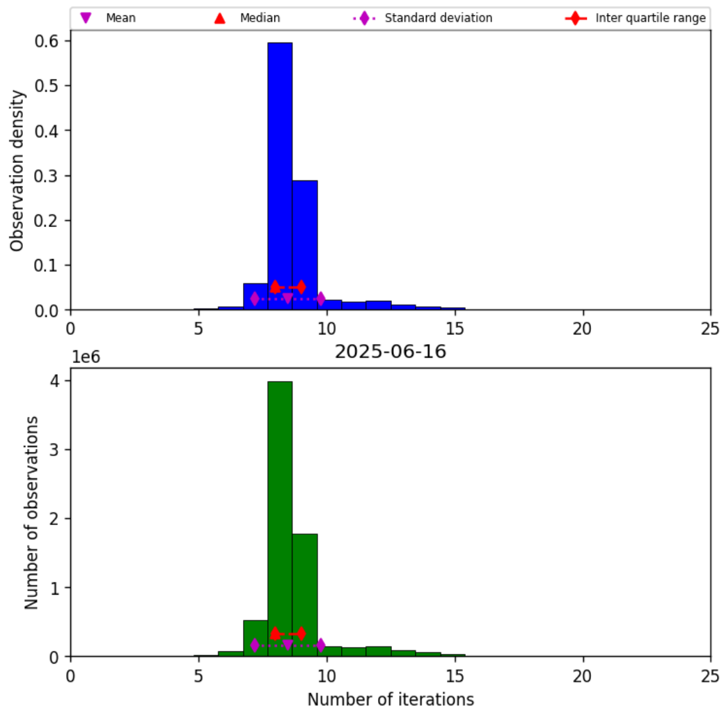
Figure 24: Histogram of “Number of iterations” for 2025-06-16 to 2025-06-17
