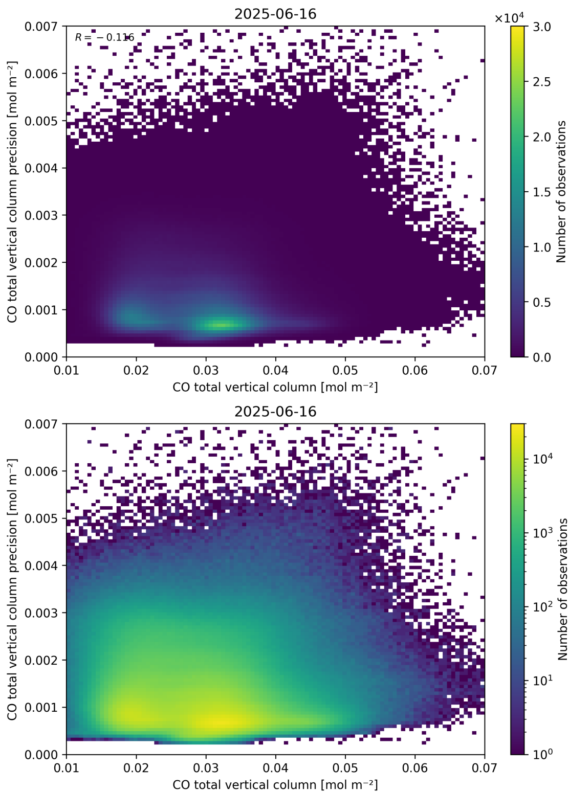
Figure 34: Scatter density plot of “CO total vertical column” against “CO total vertical column precision” for 2025-06-16 to 2025-06-17.
