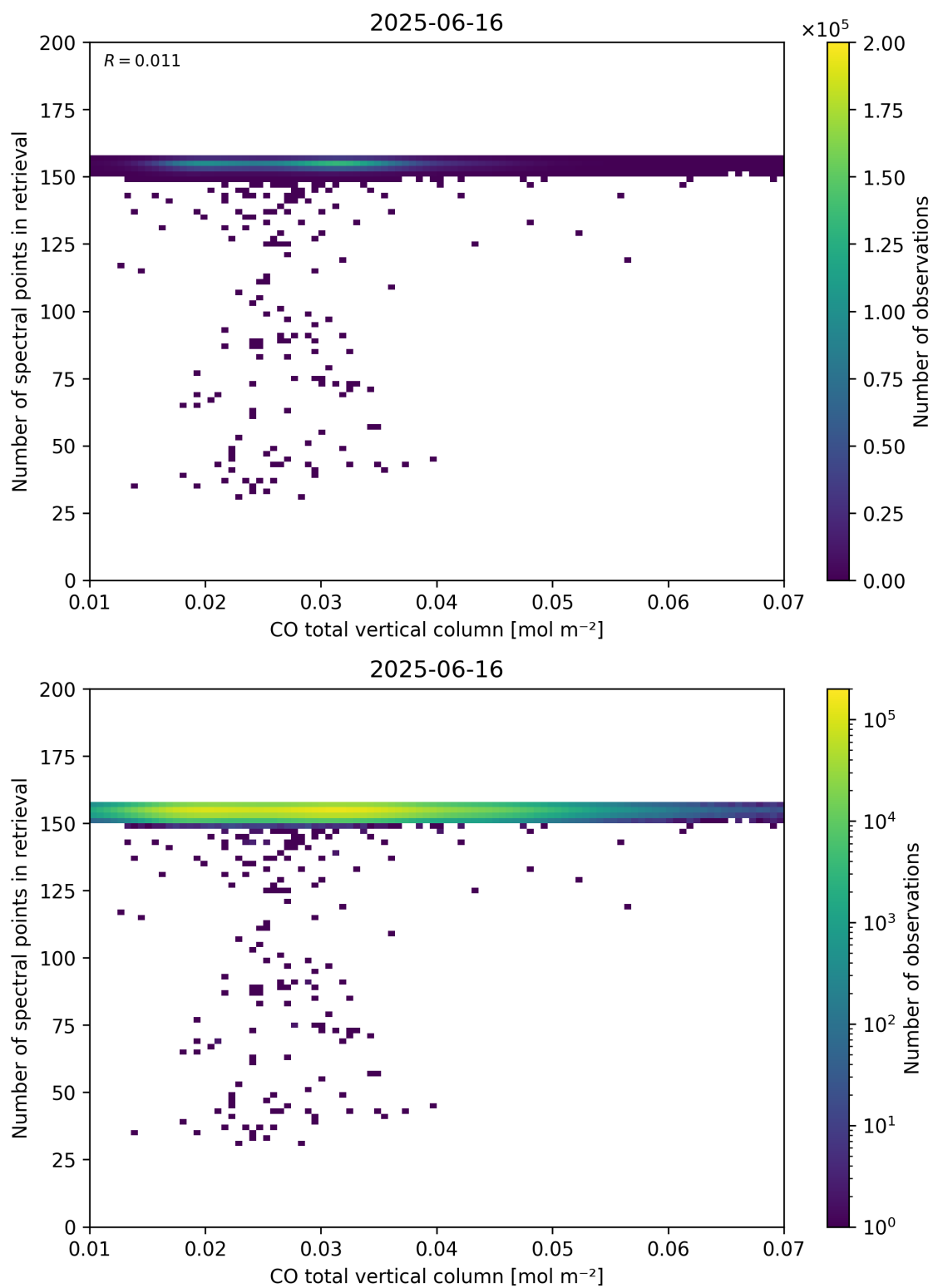
Figure 43: Scatter density plot of “CO total vertical column” against “Number of spectral points in retrieval” for 2025-06-16 to 2025-06-17.
