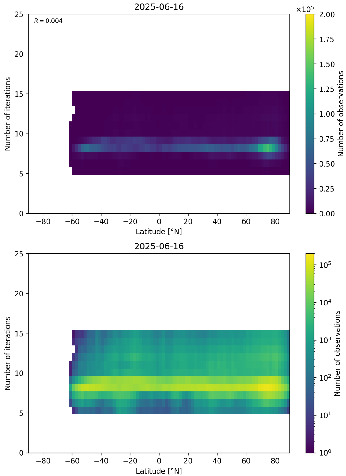
Figure 56: Scatter density plot of “Latitude” against “Number of iterations” for 2025-06-16 to 2025-06-17.
