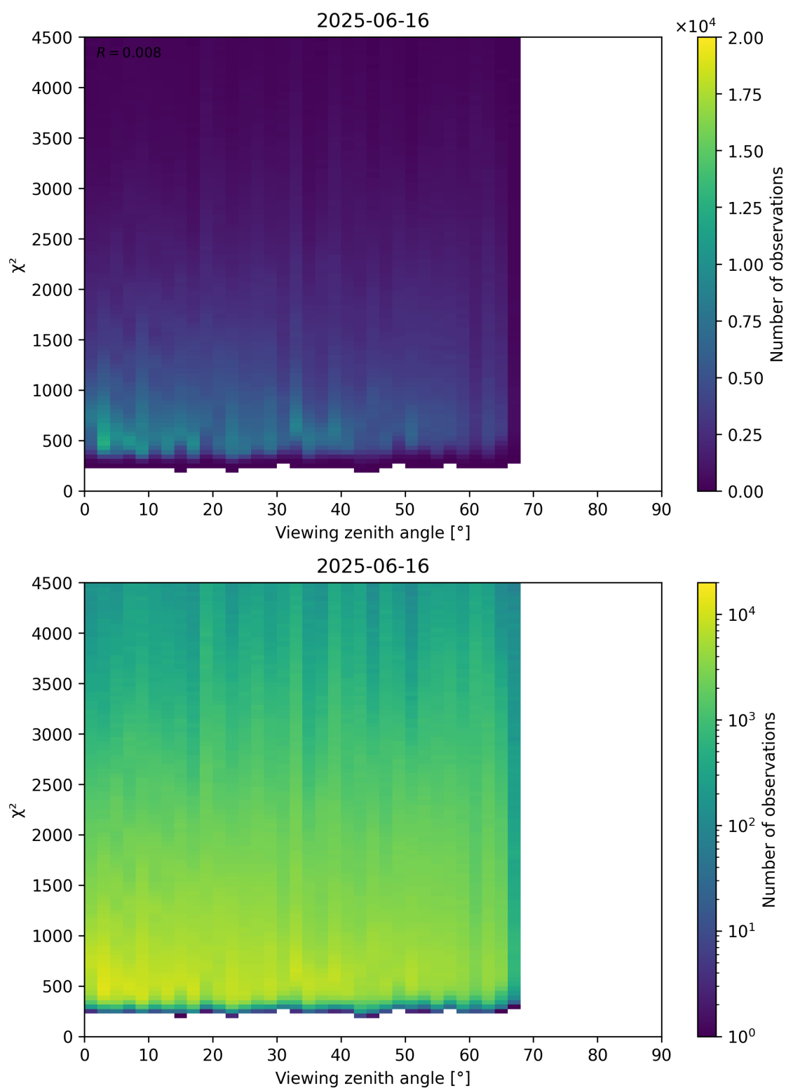
Figure 72: Scatter density plot of “Viewing zenith angle” against “ \chi^2 ” for 2025-06-16 to 2025-06-17.
