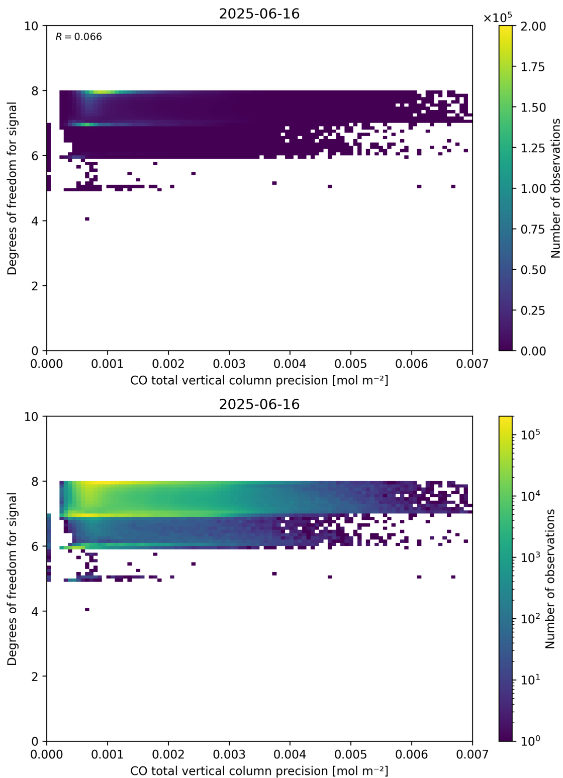
Figure 45: Scatter density plot of “CO total vertical column precision” against “Degrees of freedom for signal” for 2025-06-16 to 2025-06-17.
