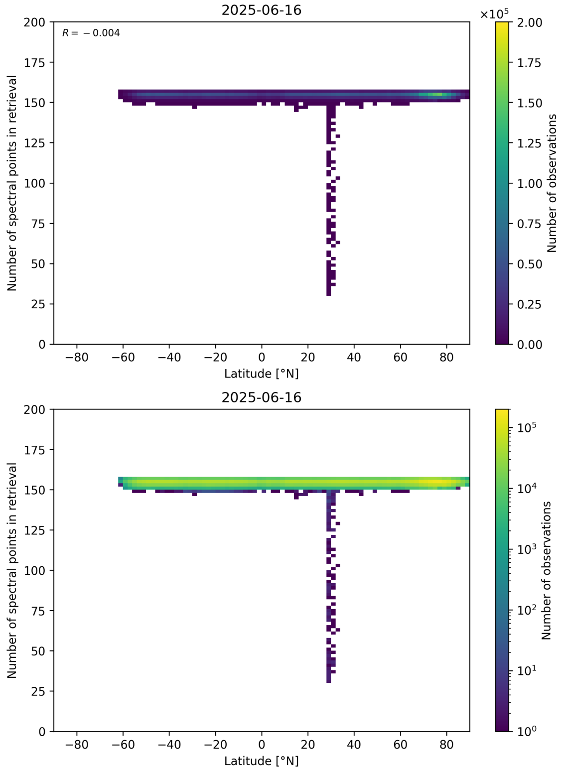
Figure 57: Scatter density plot of “Latitude” against “Number of spectral points in retrieval” for 2025-06-16 to 2025-06-17.
