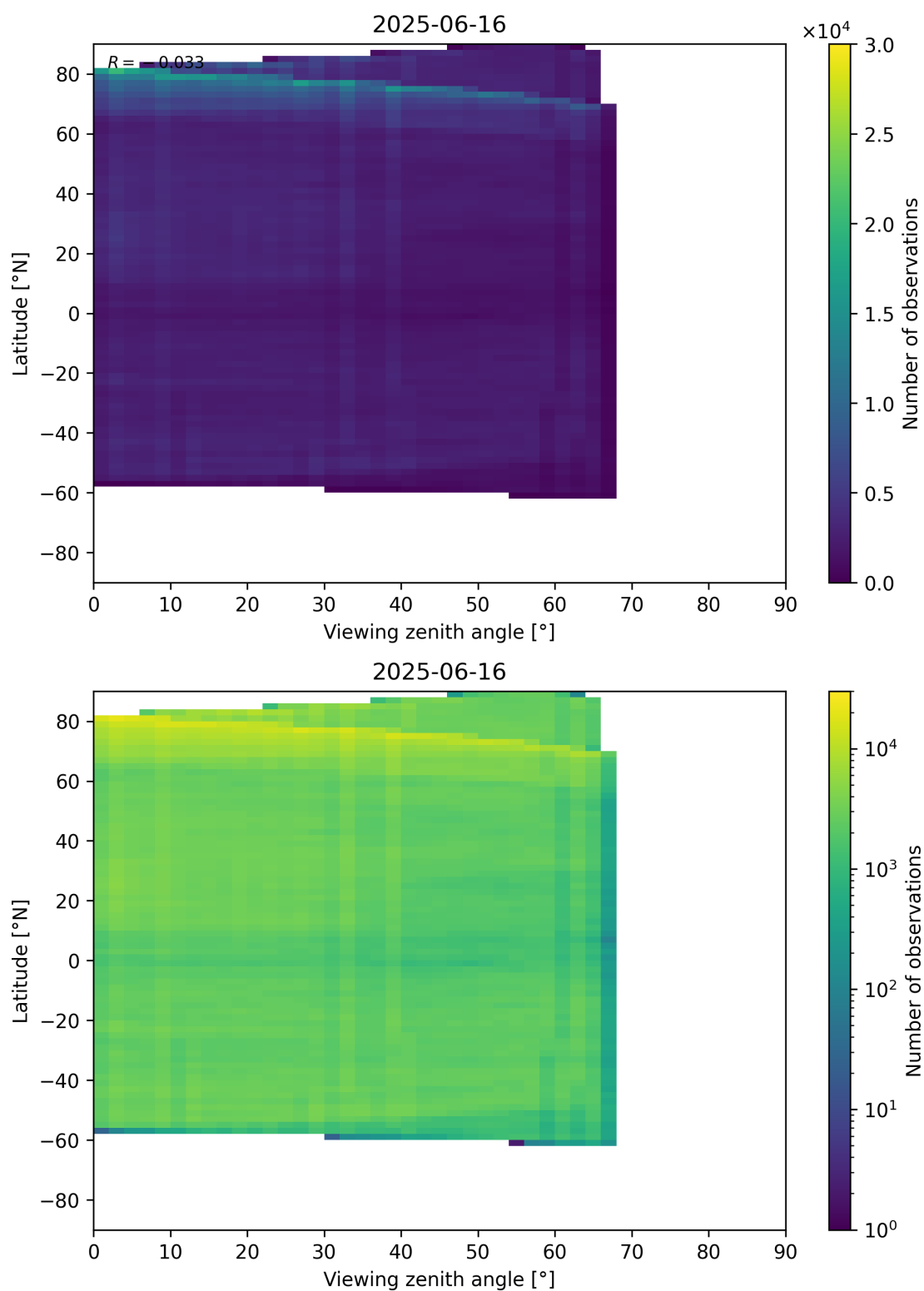
Figure 74: Scatter density plot of “Viewing zenith angle” against “Latitude” for 2025-06-16 to 2025-06-17.
