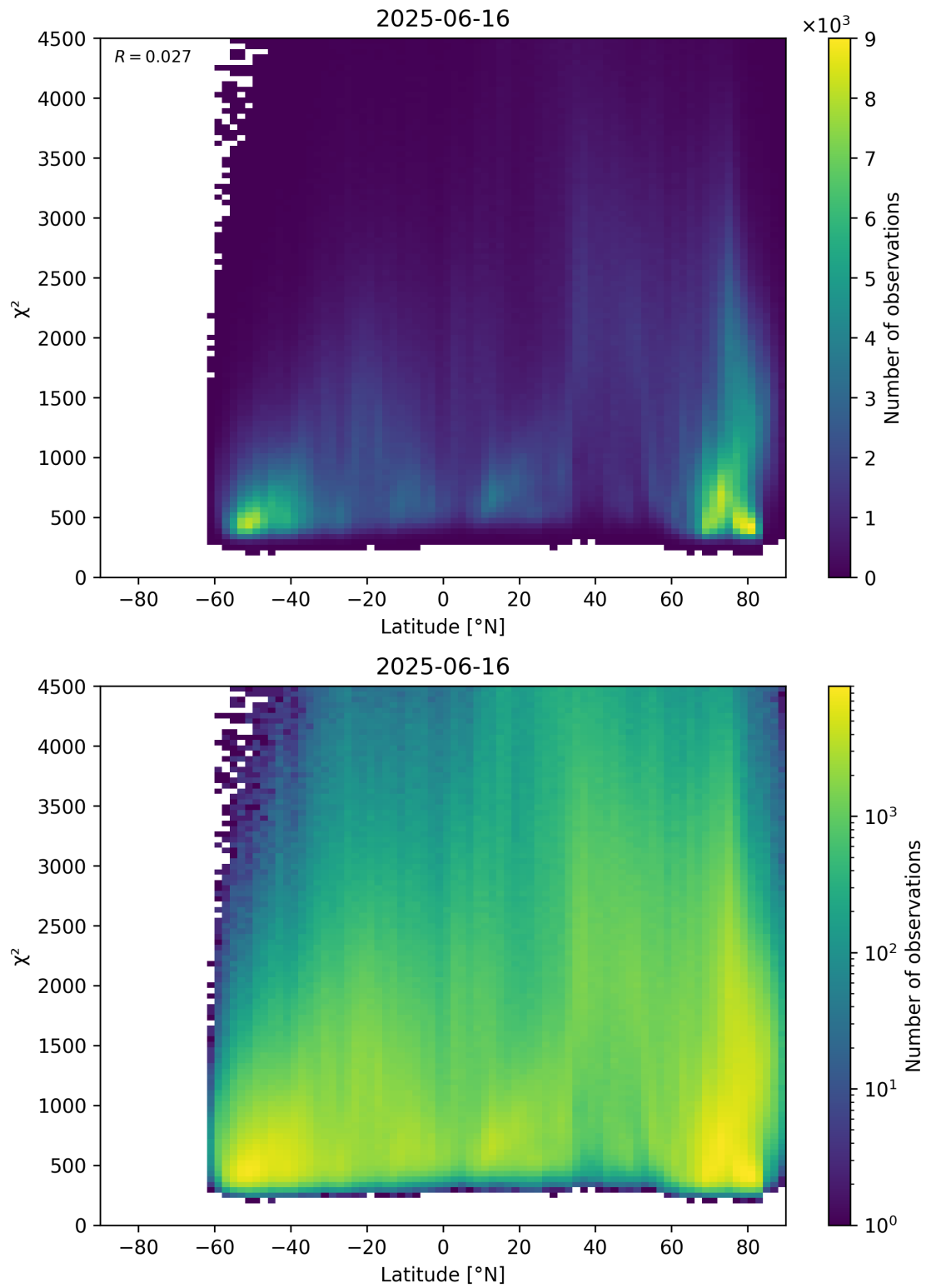
Figure 54: Scatter density plot of “Latitude” against “ \chi^2 ” for 2025-06-16 to 2025-06-17.
