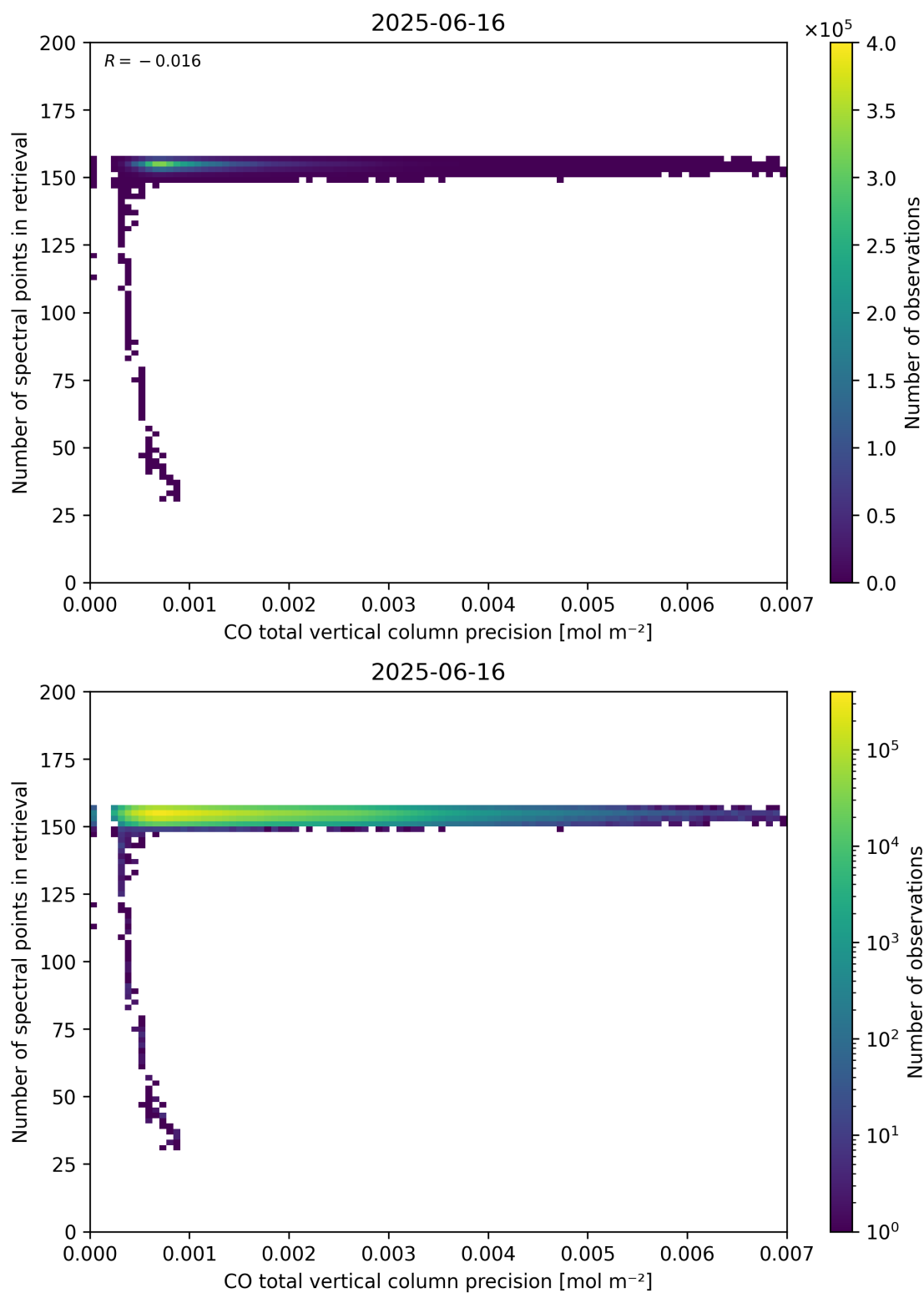
Figure 47: Scatter density plot of “CO total vertical column precision” against “Number of spectral points in retrieval” for 2025-06-16 to 2025-06-17.
