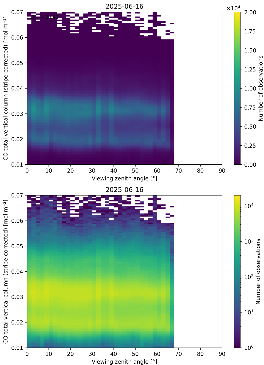
Figure 70: Scatter density plot of “Viewing zenith angle” against “CO total vertical column (stripe-corrected)” for 2025-06-16 to 2025-06-17.
