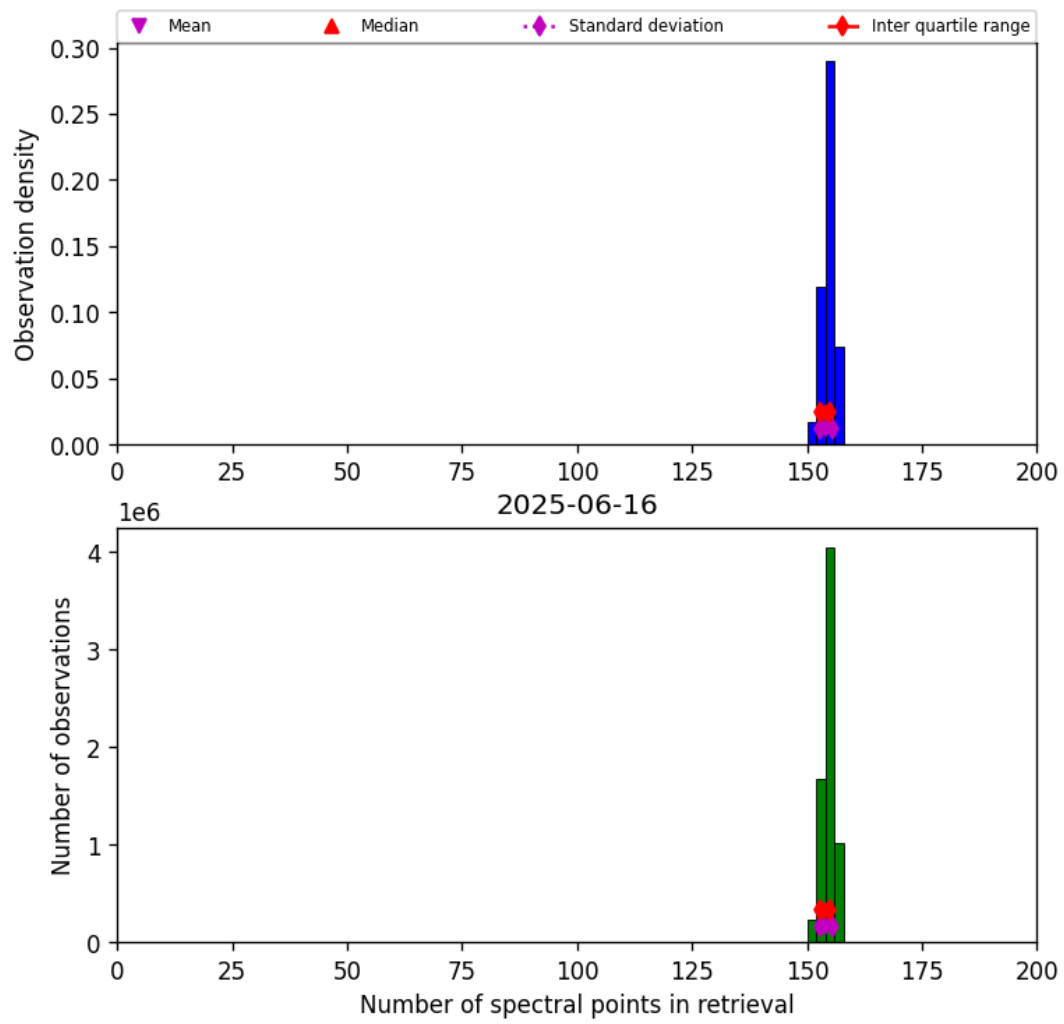
Figure 21: Histogram of “Number of spectral points in retrieval” for 2025-06-16 to 2025-06-17
