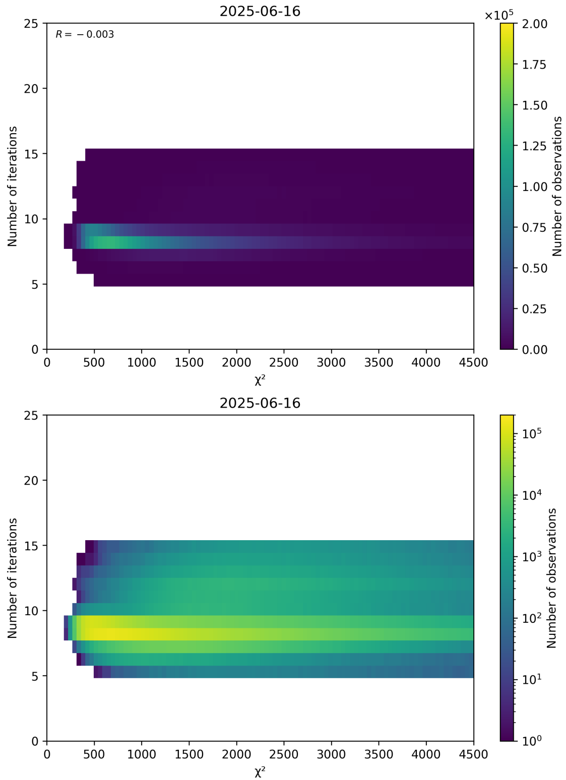
Figure 49: Scatter density plot of “ \chi^2 ” against “Number of iterations” for 2025-06-16 to 2025-06-17.
