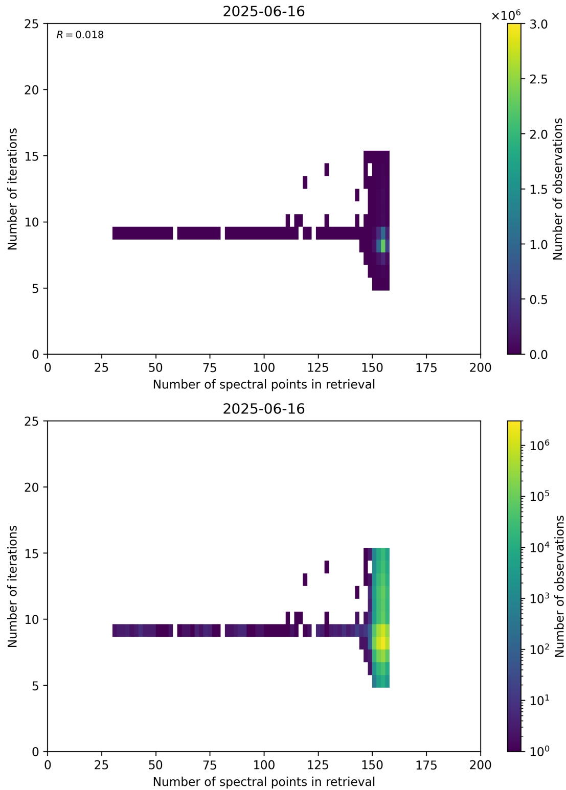
Figure 60: Scatter density plot of “Number of spectral points in retrieval” against “Number of iterations” for 2025-06-16 to 2025-06-17.
