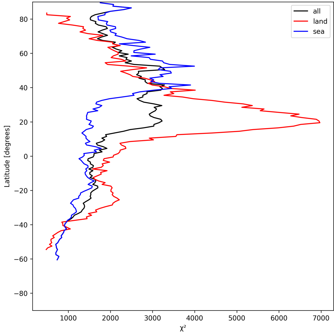
Figure 14: Zonal average of “ \chi^2 ” for 2025-06-16 to 2025-06-17.
