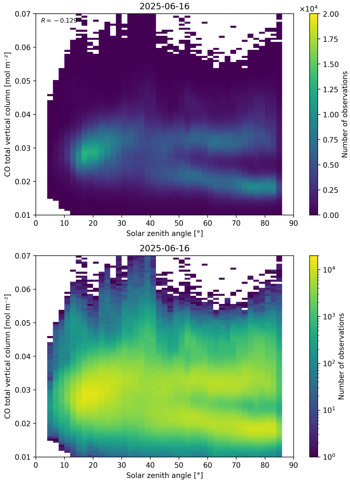
Figure 61: Scatter density plot of “Solar zenith angle” against “CO total vertical column” for 2025-06-16 to 2025-06-17.
