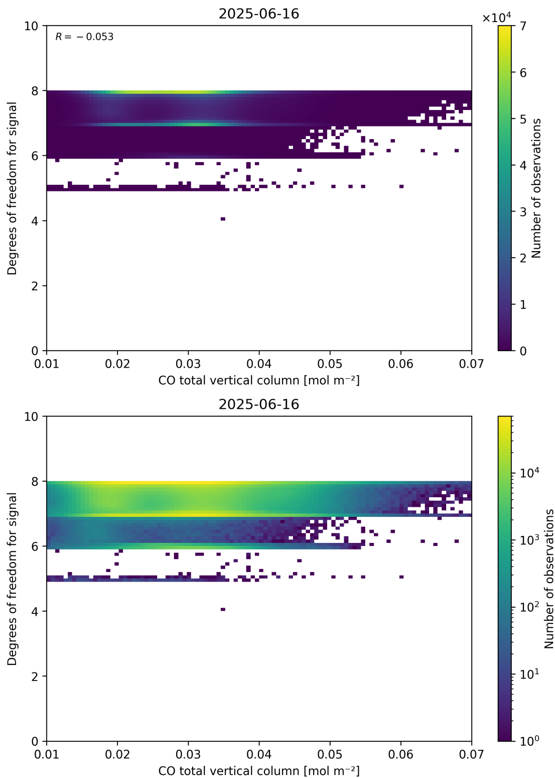
Figure 41: Scatter density plot of “CO total vertical column” against “Degrees of freedom for signal” for 2025-06-16 to 2025-06-17.
