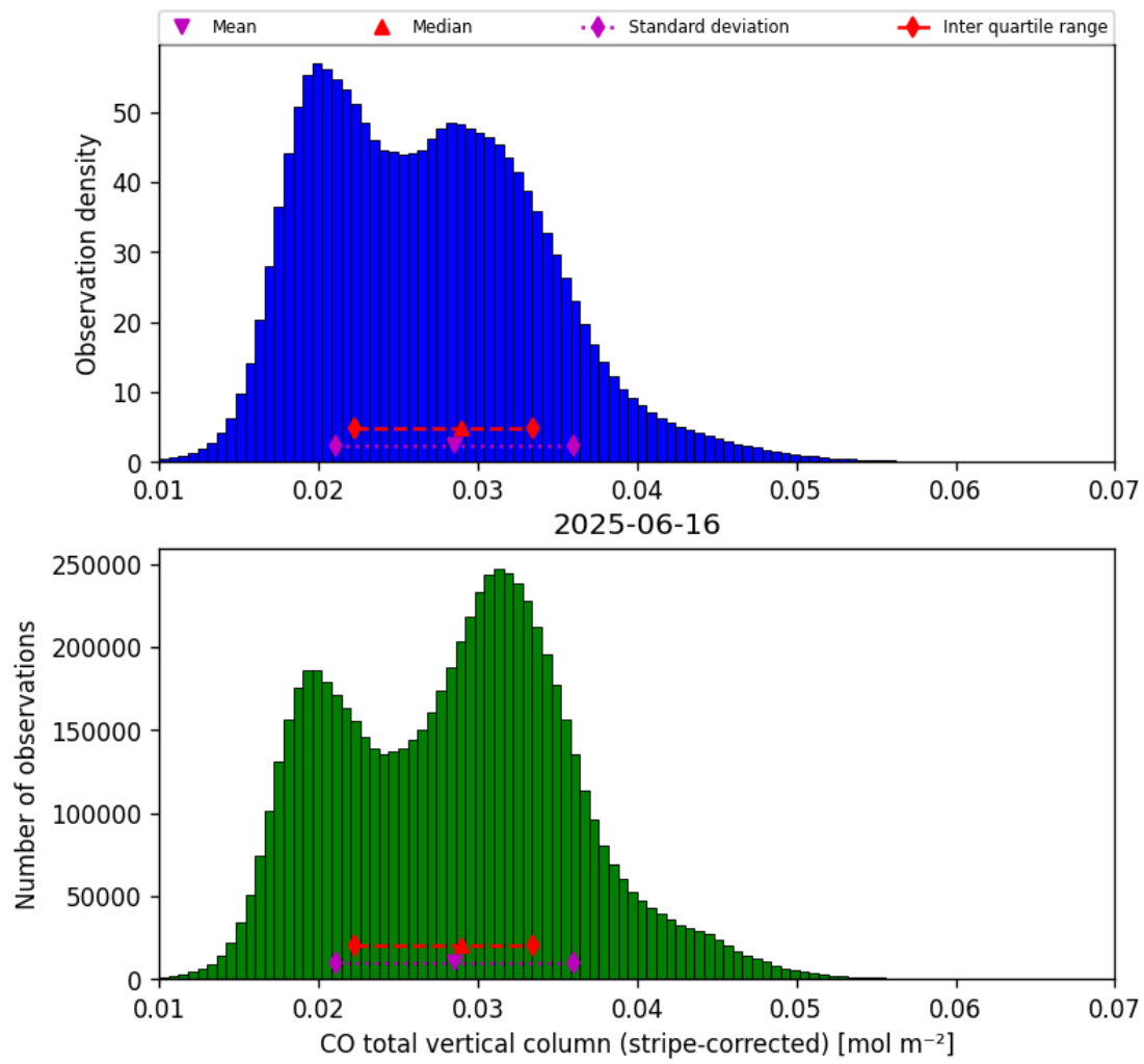
Figure 19: Histogram of “CO total vertical column (stripe-corrected)” for 2025-06-16 to 2025-06-17
