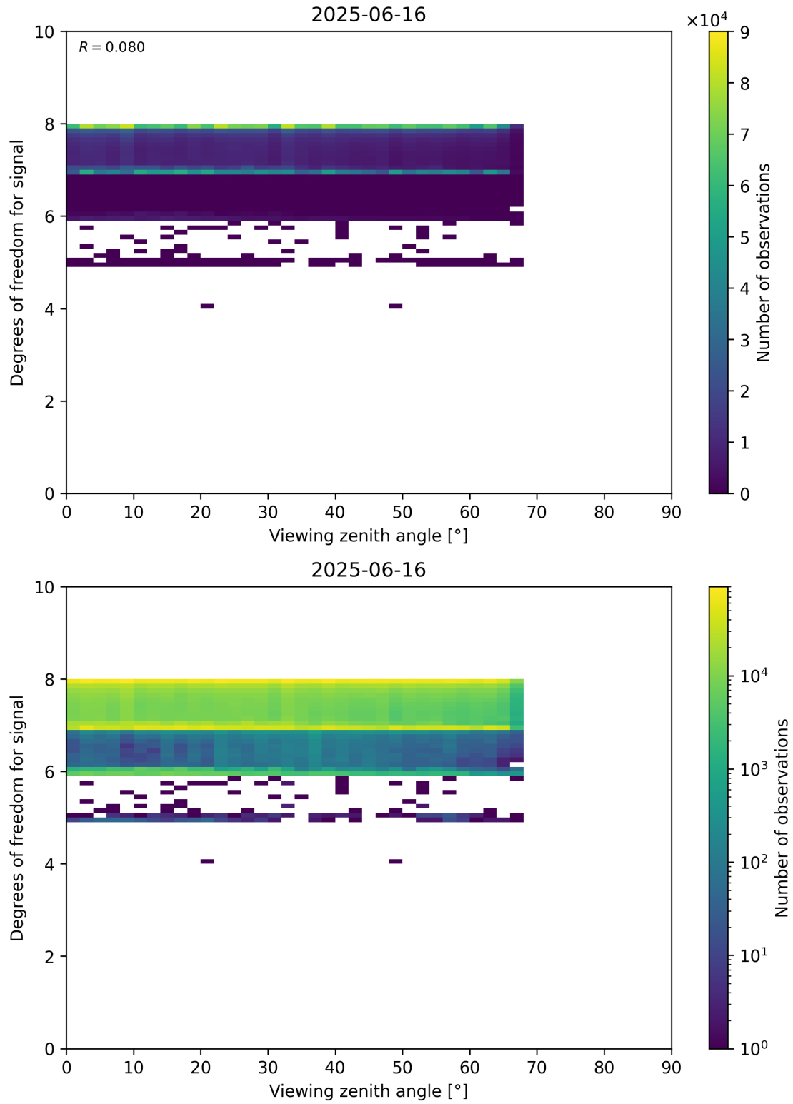
Figure 73: Scatter density plot of “Viewing zenith angle” against “Degrees of freedom for signal” for 2025-06-16 to 2025-06-17.
