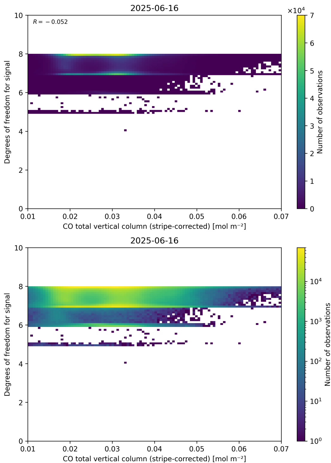
Figure 38: Scatter density plot of “CO total vertical column (stripe-corrected)” against “Degrees of freedom for signal” for 2025-06-16 to 2025-06-17.
