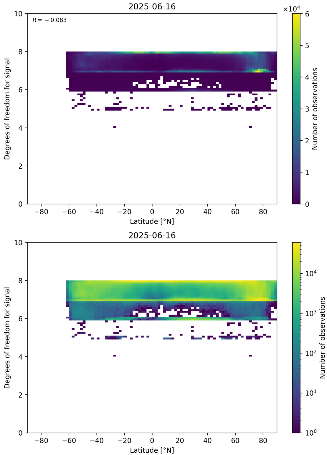
Figure 55: Scatter density plot of “Latitude” against “Degrees of freedom for signal” for 2025-06-16 to 2025-06-17.
