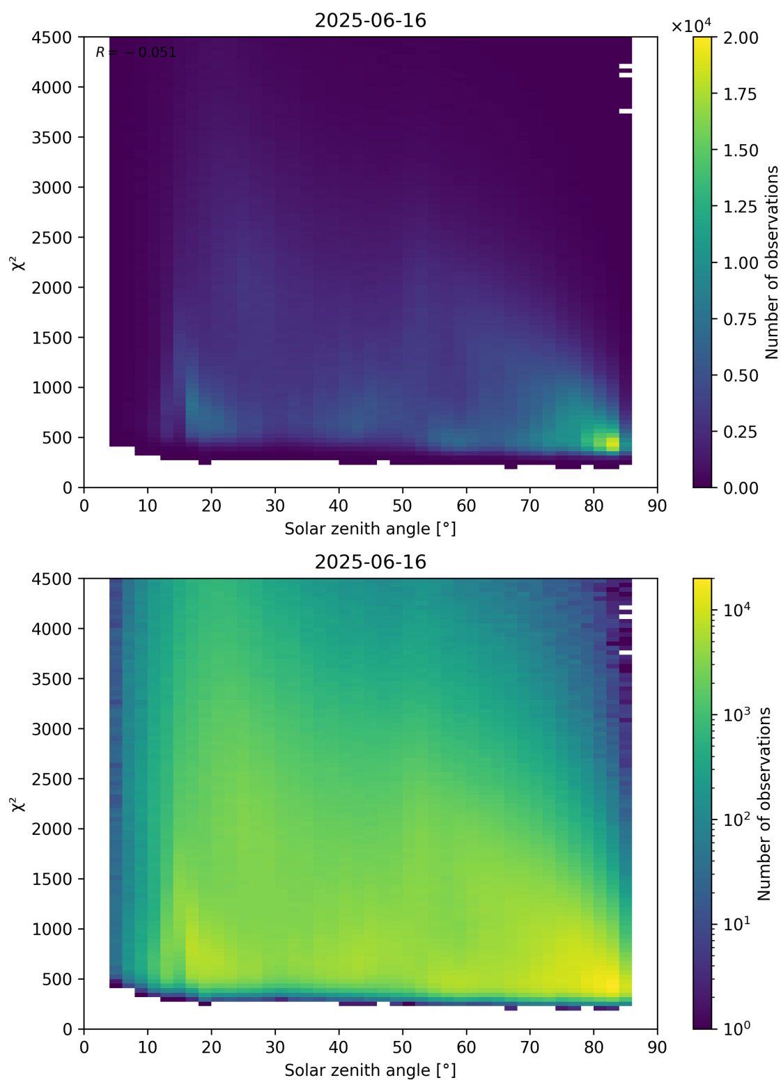
Figure 64: Scatter density plot of “Solar zenith angle” against “ \chi^2 ” for 2025-06-16 to 2025-06-17.
