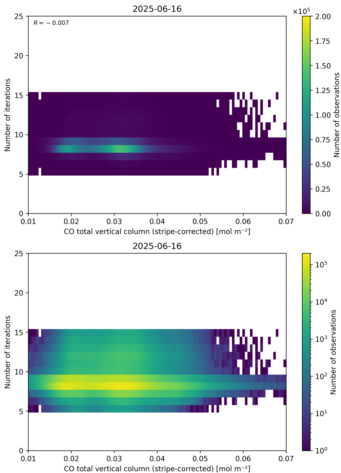
Figure 39: Scatter density plot of “CO total vertical column (stripe-corrected)” against “Number of iterations” for 2025-06-16 to 2025-06-17.
