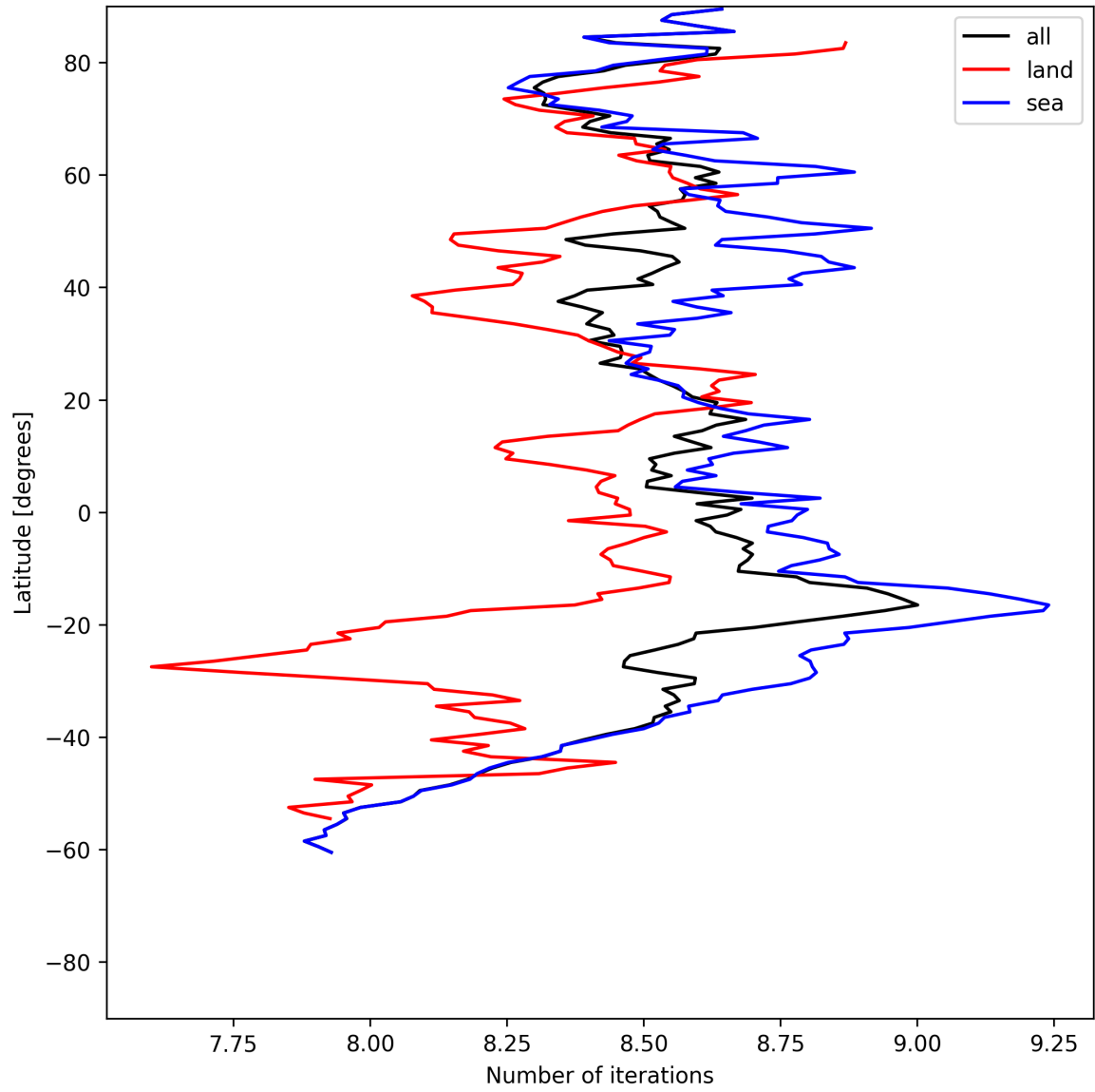
Figure 16: Zonal average of “Number of iterations” for 2025-06-16 to 2025-06-17.
