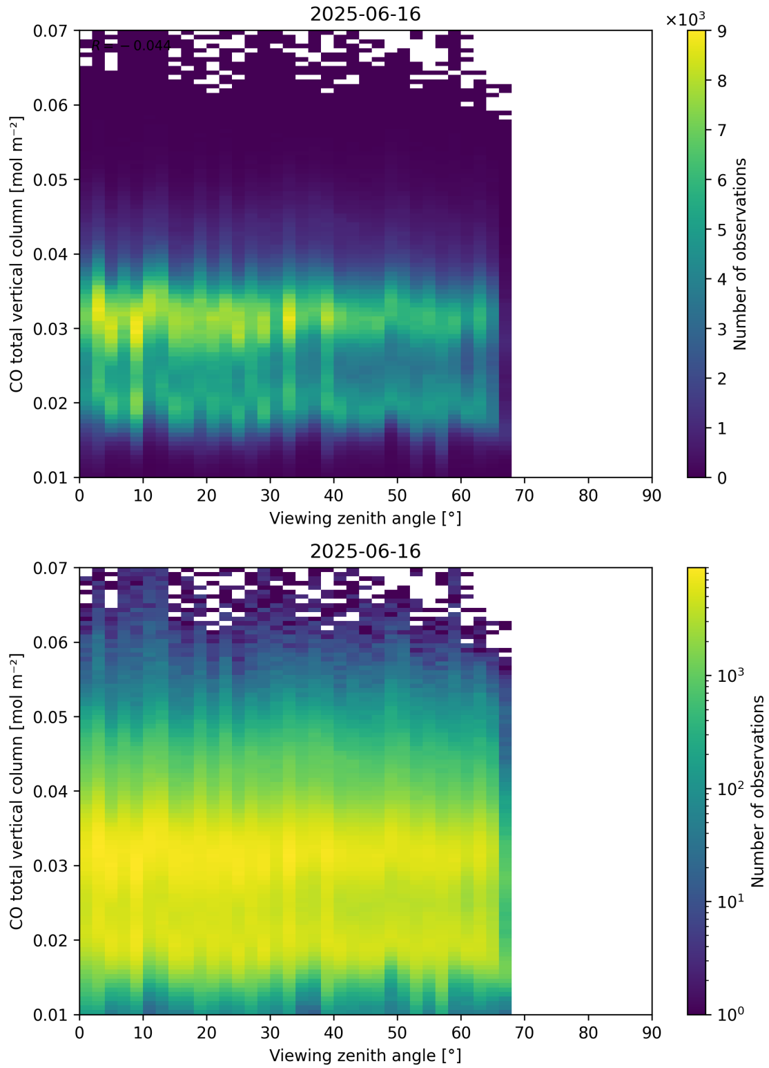
Figure 69: Scatter density plot of “Viewing zenith angle” against “CO total vertical column” for 2025-06-16 to 2025-06-17.
