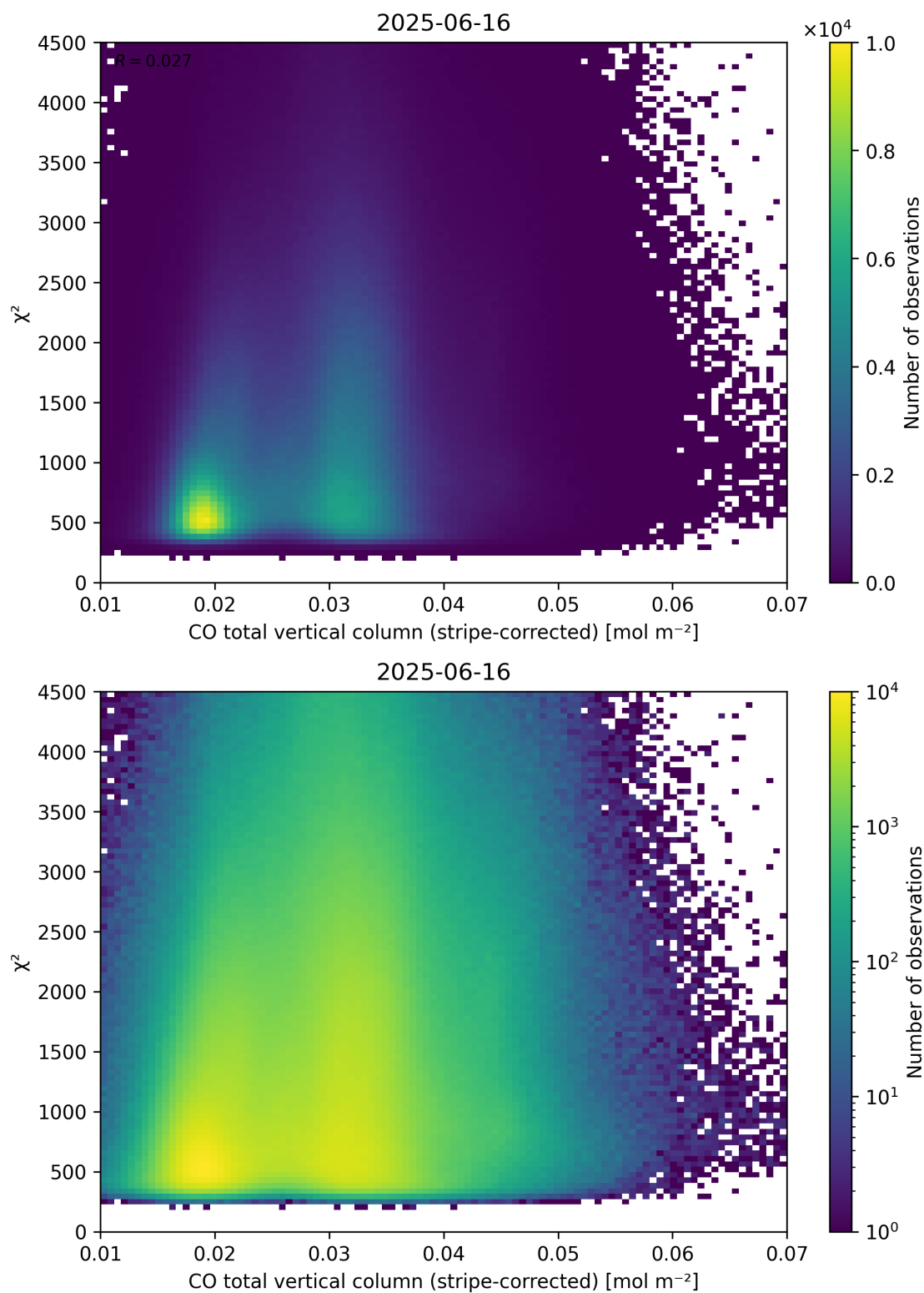
Figure 37: Scatter density plot of “CO total vertical column (stripe-corrected)” against “ \chi^2 ” for 2025-06-16 to 2025-06-17.
