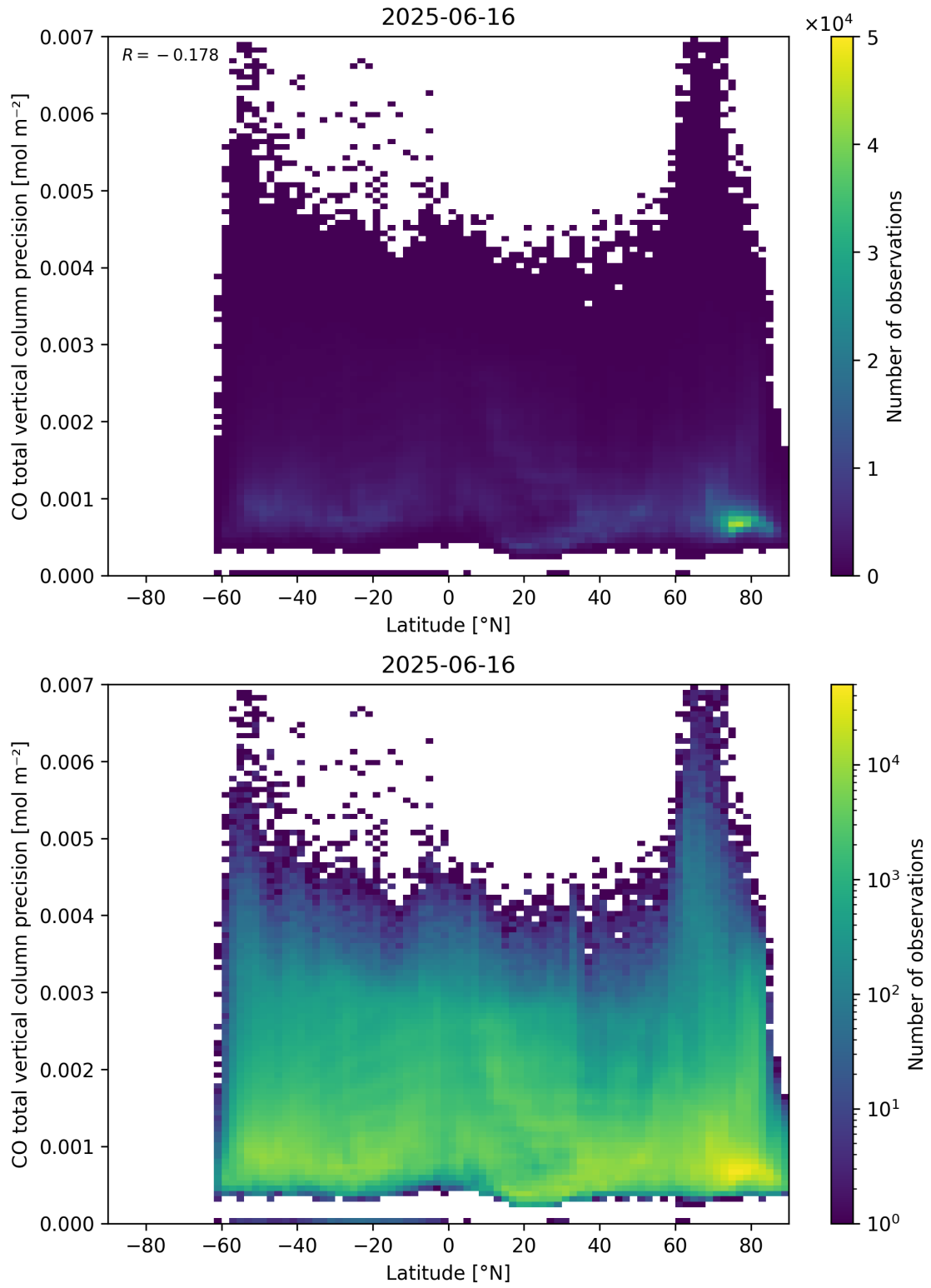
Figure 53: Scatter density plot of “Latitude” against “CO total vertical column precision” for 2025-06-16 to 2025-06-17.
