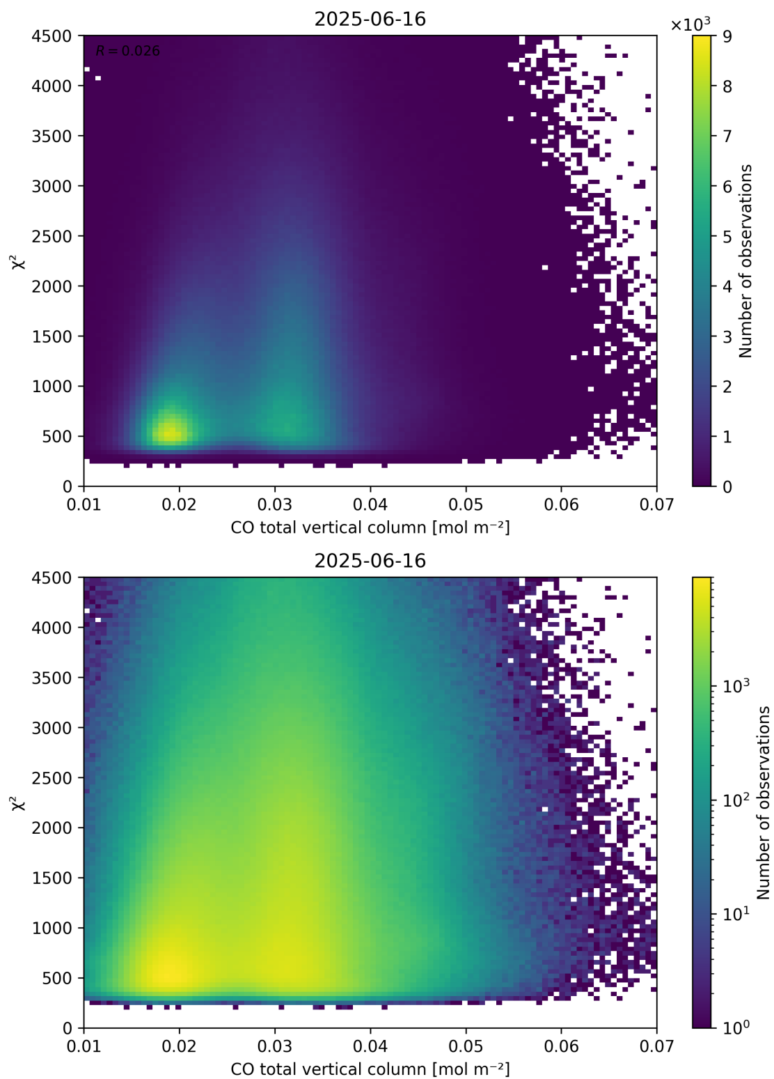
Figure 35: Scatter density plot of “CO total vertical column” against “ \chi^2 ” for 2025-06-16 to 2025-06-17.
