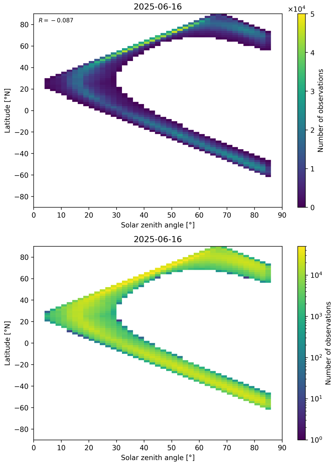
Figure 66: Scatter density plot of “Solar zenith angle” against “Latitude” for 2025-06-16 to 2025-06-17.
