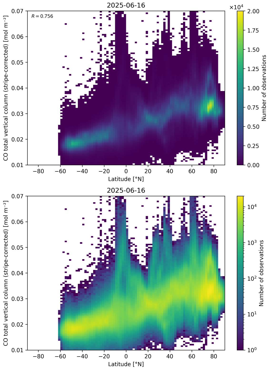
Figure 52: Scatter density plot of “Latitude” against “CO total vertical column (stripe-corrected)” for 2025-06-16 to 2025-06-17.
