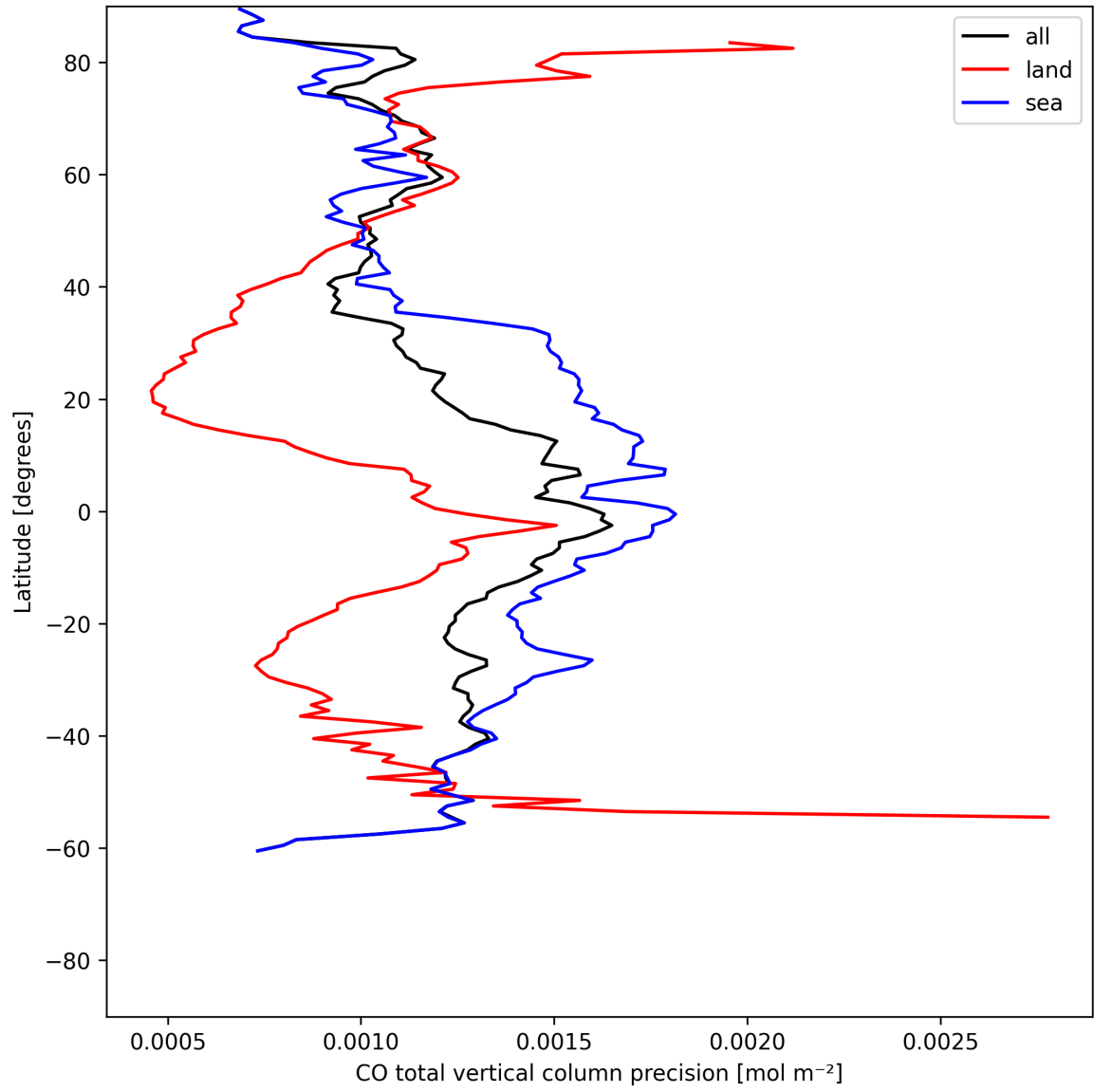
Figure 12: Zonal average of “CO total vertical column precision” for 2025-06-16 to 2025-06-17.
