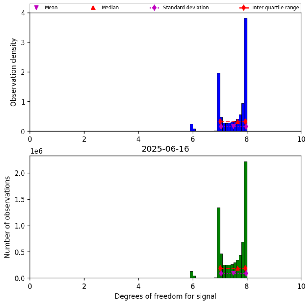
Figure 23: Histogram of “Degrees of freedom for signal” for 2025-06-16 to 2025-06-17
