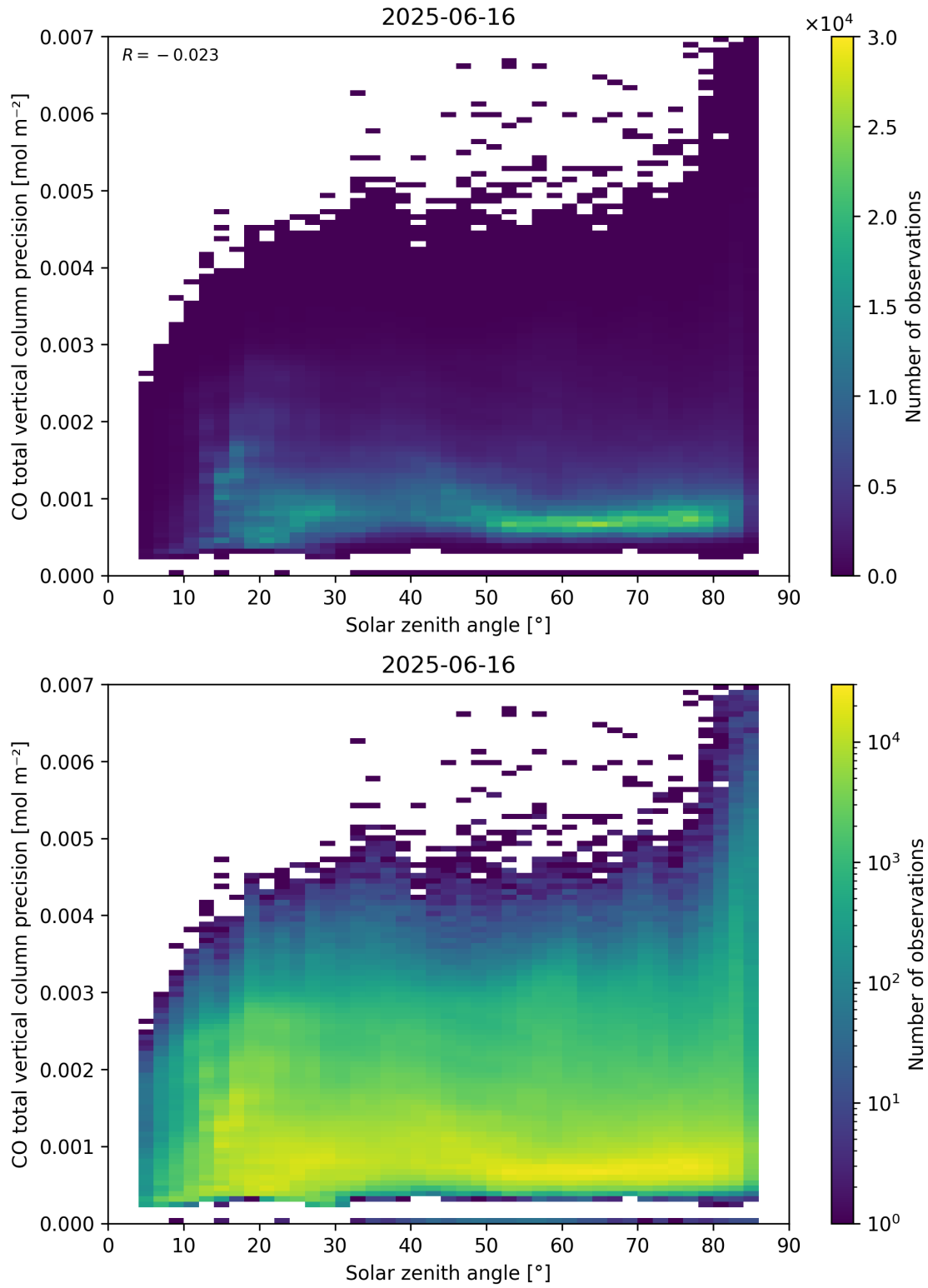
Figure 63: Scatter density plot of “Solar zenith angle” against “CO total vertical column precision” for 2025-06-16 to 2025-06-17.
