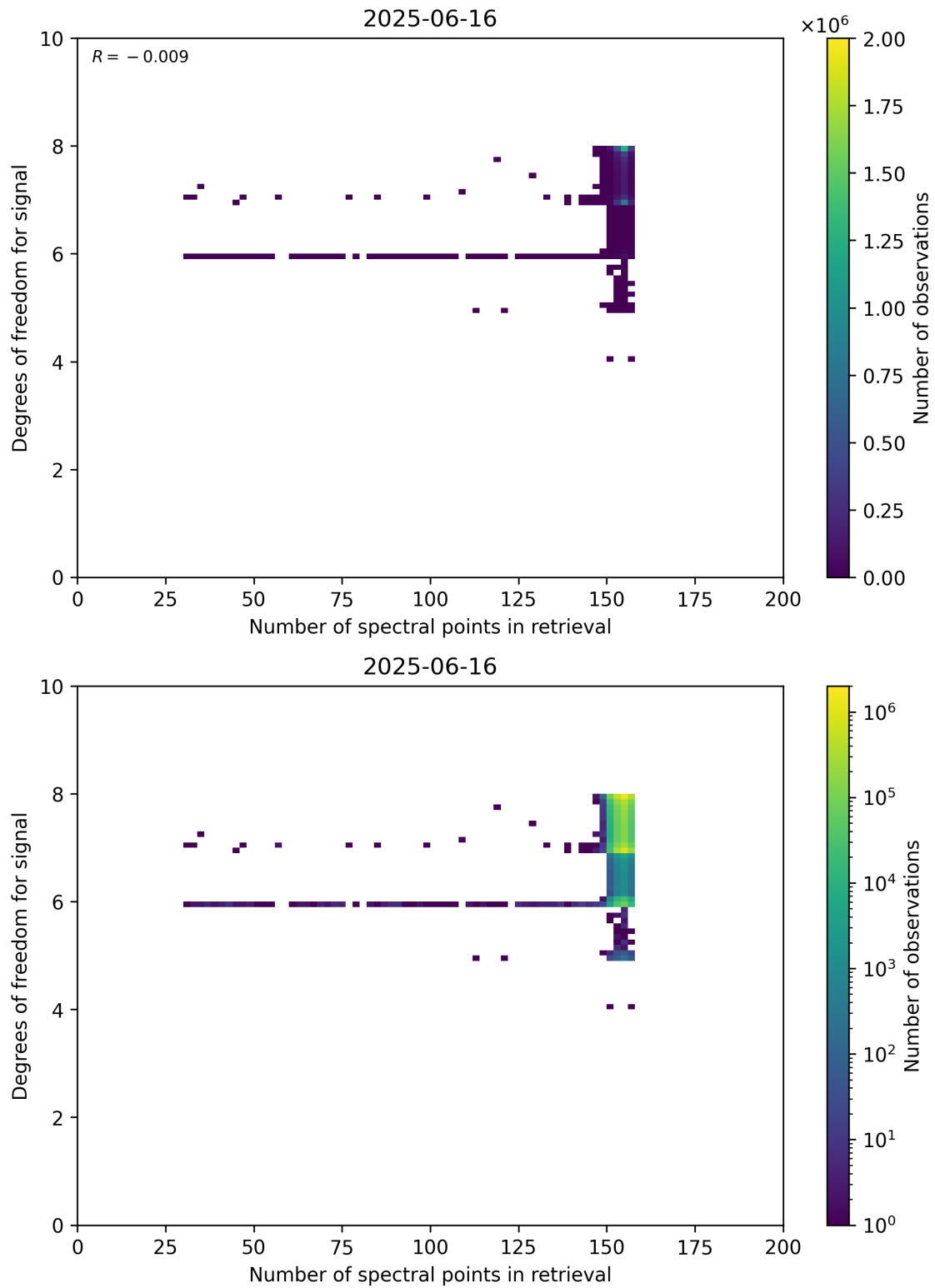
Figure 59: Scatter density plot of “Number of spectral points in retrieval” against “Degrees of freedom for signal” for 2025-06-16 to 2025-06-17.
