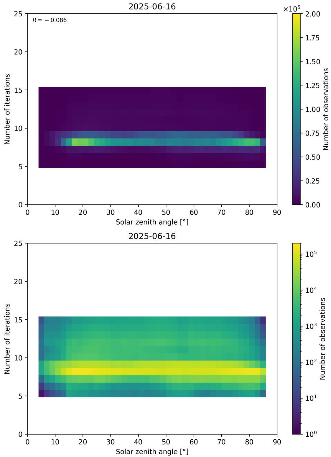
Figure 67: Scatter density plot of “Solar zenith angle” against “Number of iterations” for 2025-06-16 to 2025-06-17.
