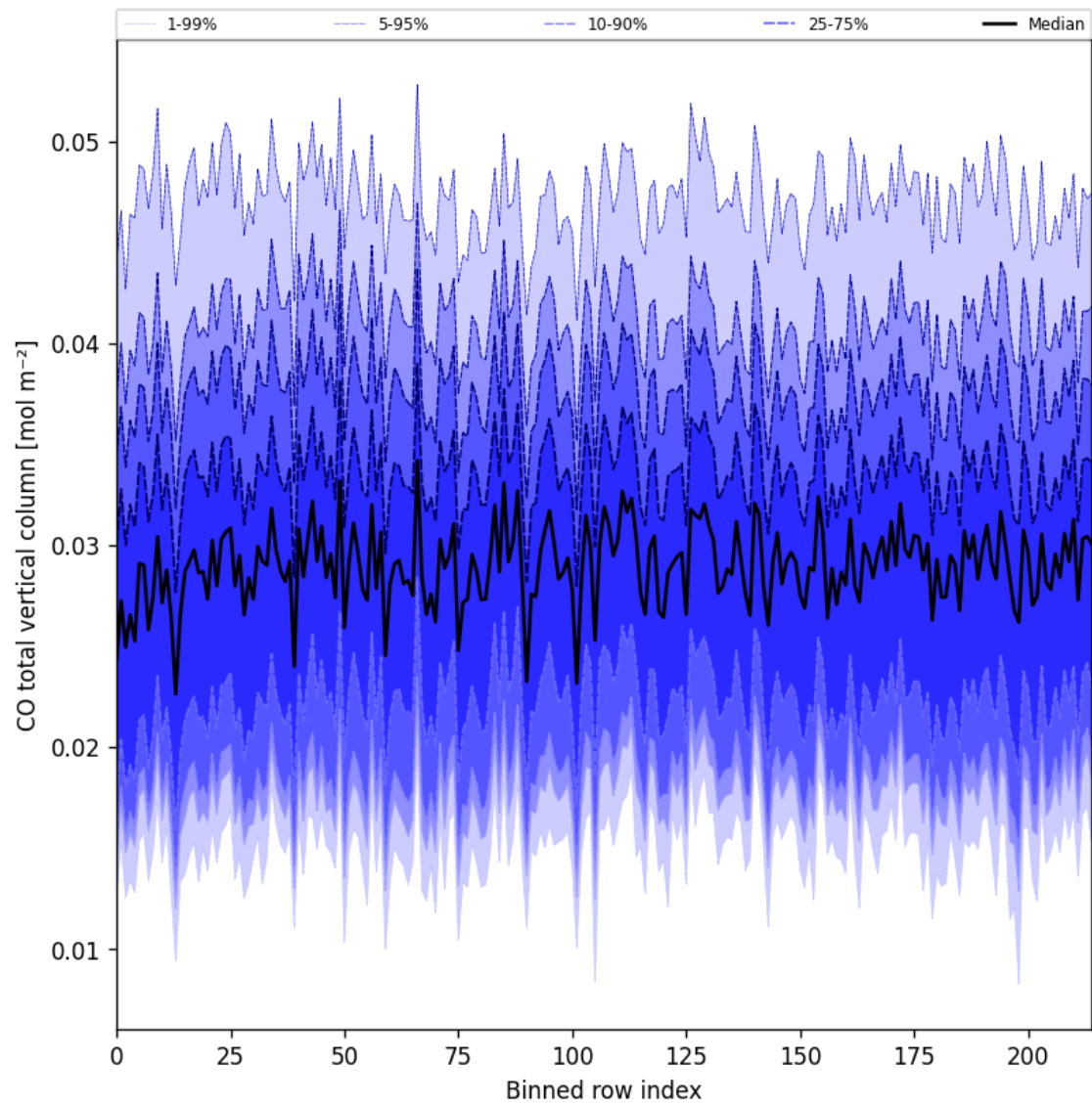
Figure 26: Along track statistics of “CO total vertical column” for 2025-06-16 to 2025-06-17
