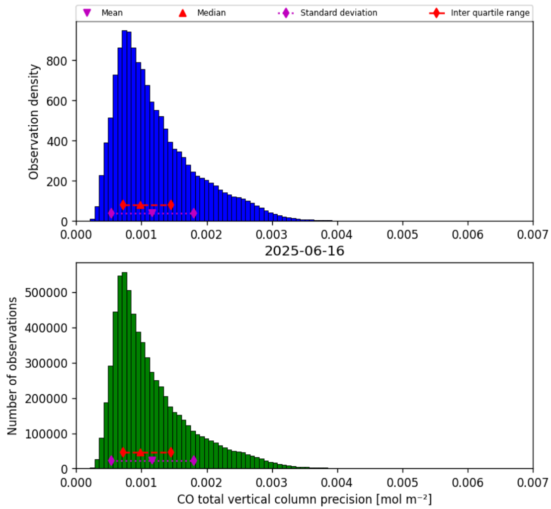
Figure 20: Histogram of “CO total vertical column precision” for 2025-06-16 to 2025-06-17
