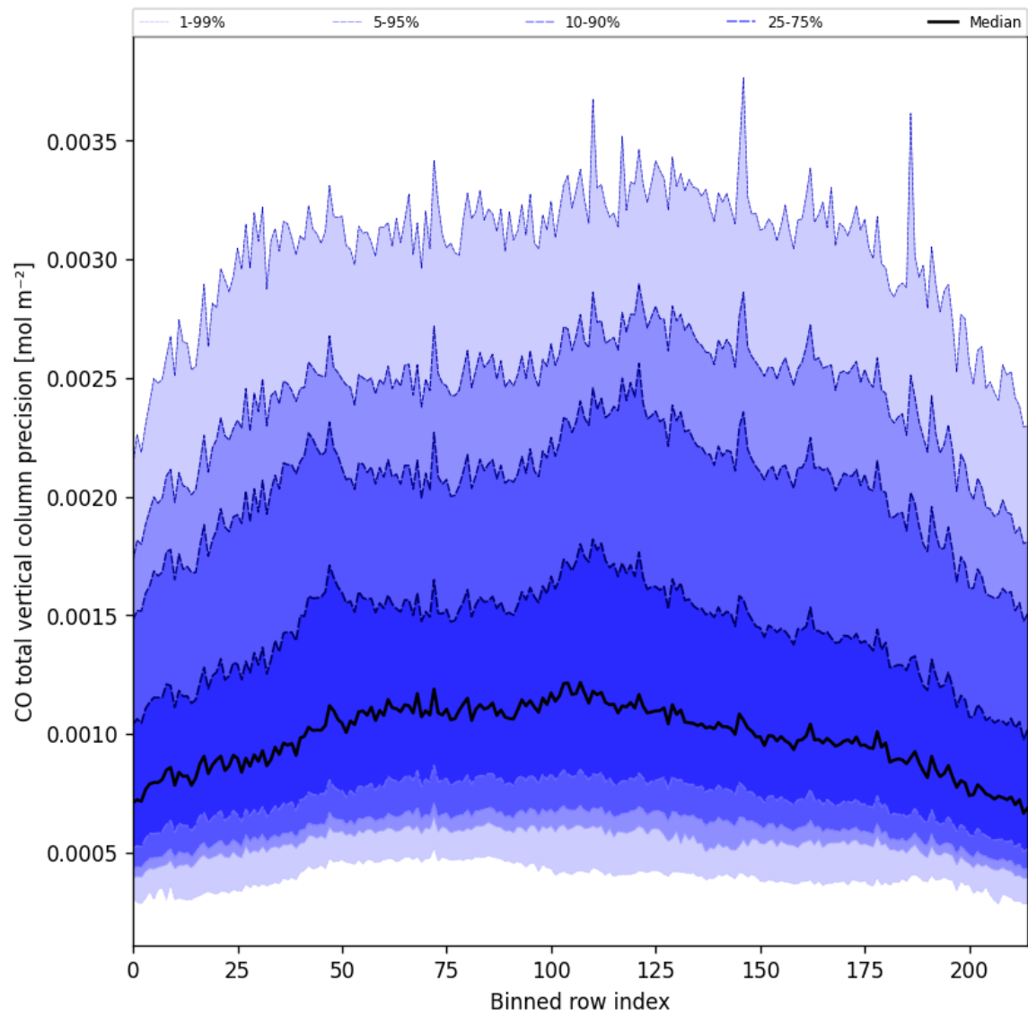
Figure 28: Along track statistics of “CO total vertical column precision” for 2025-06-16 to 2025-06-17
