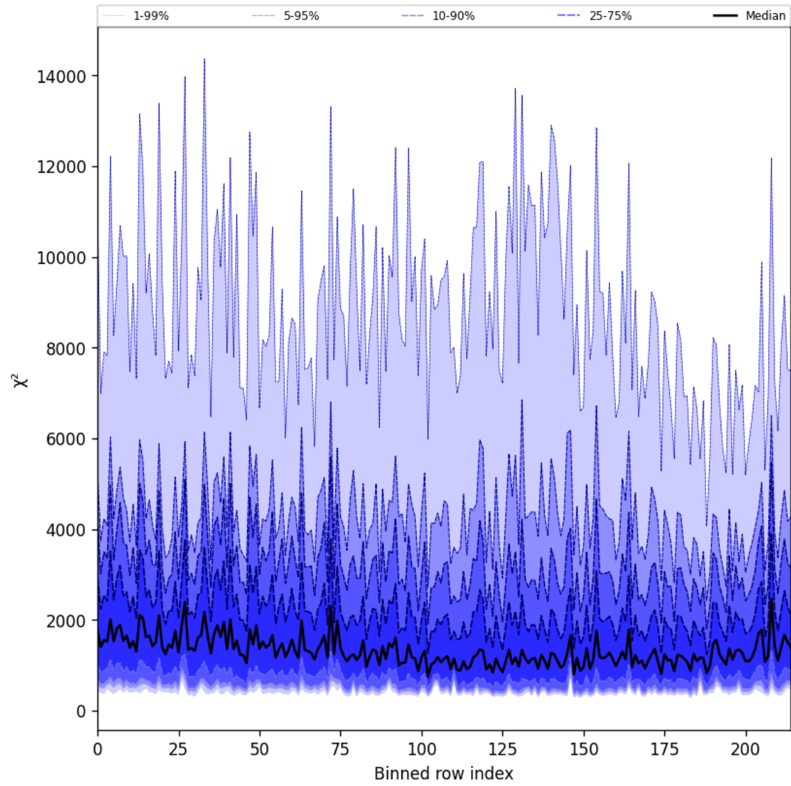
Figure 30: Along track statistics of “ \chi^2 ” for 2025-06-16 to 2025-06-17
