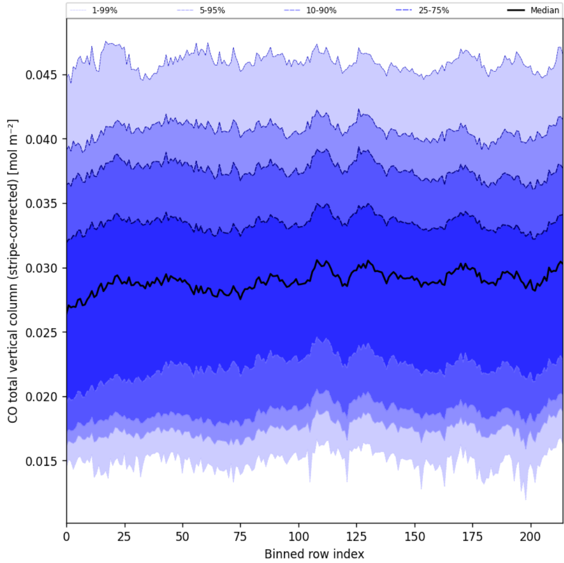
Figure 27: Along track statistics of “CO total vertical column (stripe-corrected)” for 2025-06-17 to 2025-06-18
