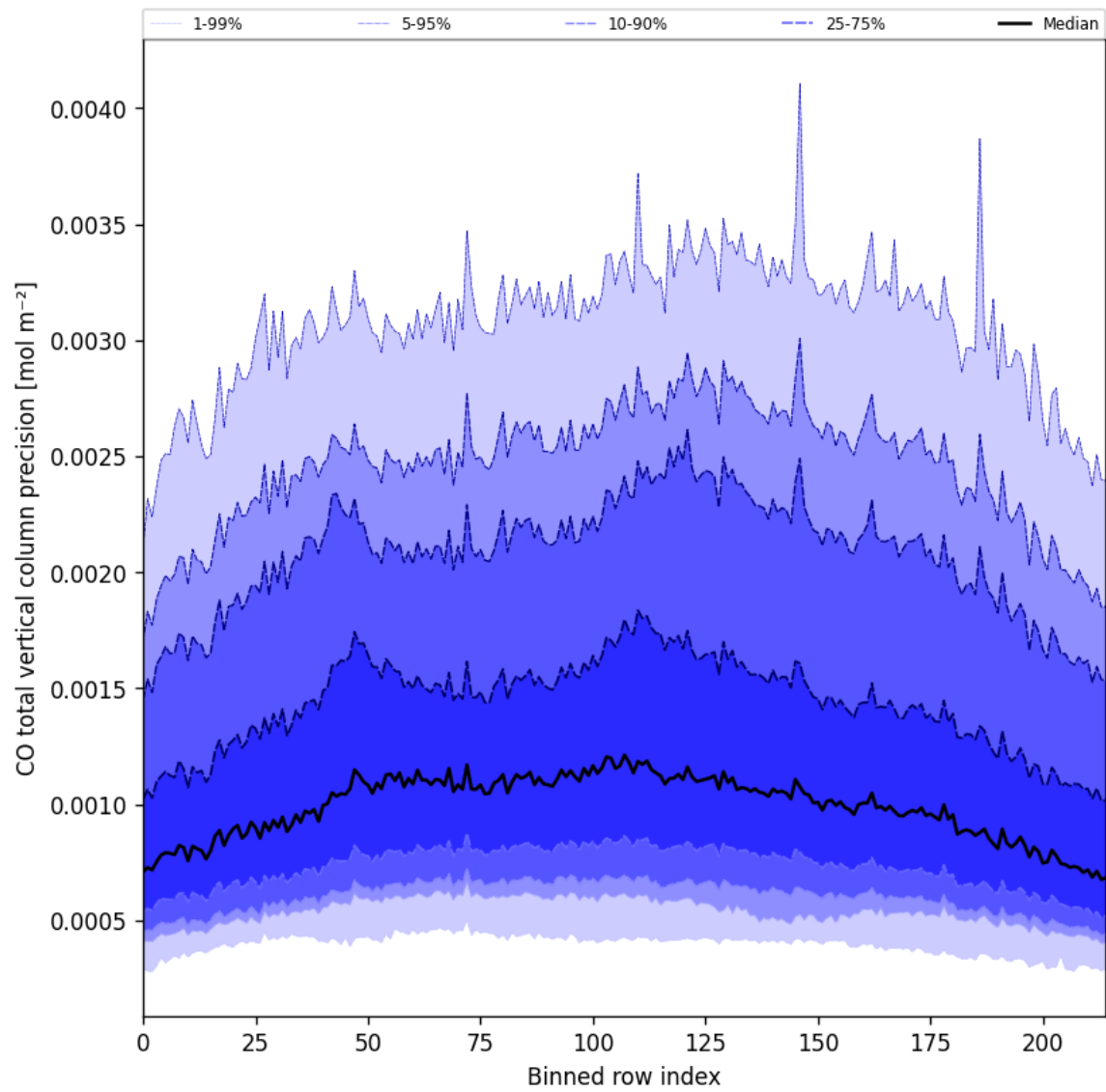
Figure 28: Along track statistics of “CO total vertical column precision” for 2025-06-17 to 2025-06-18
