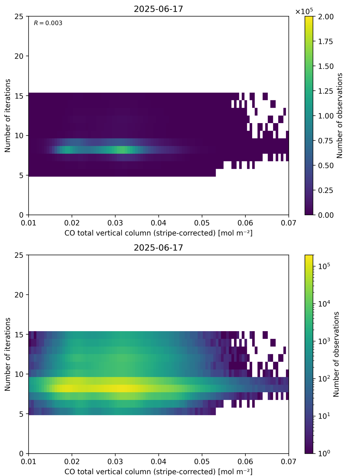
Figure 39: Scatter density plot of “CO total vertical column (stripe-corrected)” against “Number of iterations” for 2025-06-17 to 2025-06-18.
