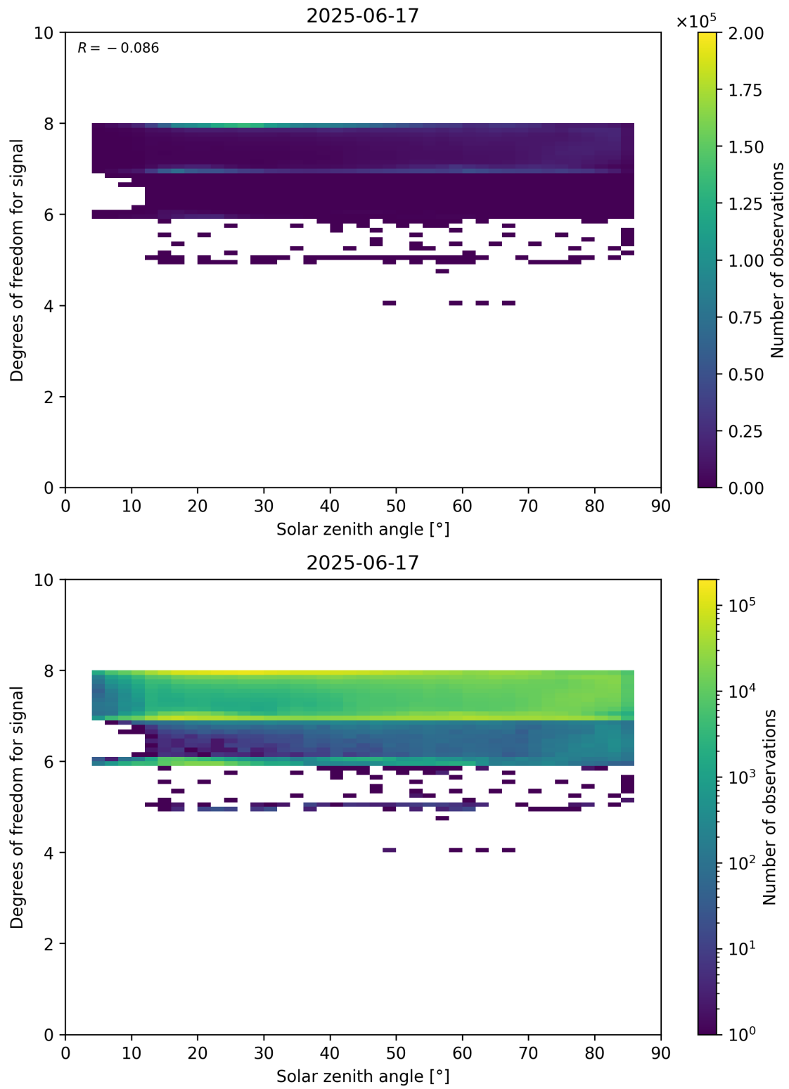
Figure 65: Scatter density plot of “Solar zenith angle” against “Degrees of freedom for signal” for 2025-06-17 to 2025-06-18.
