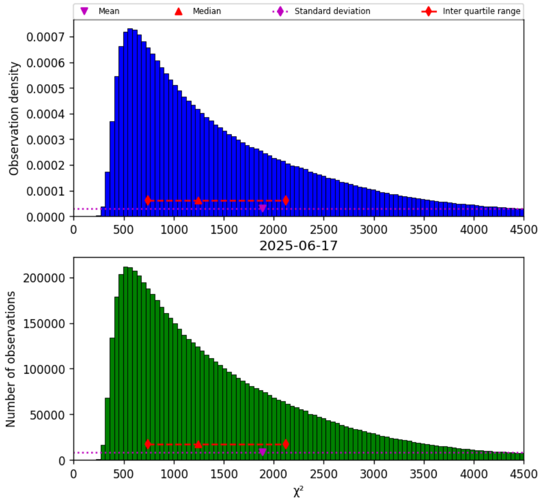
Figure 22: Histogram of “ \chi^2 ” for 2025-06-17 to 2025-06-18
