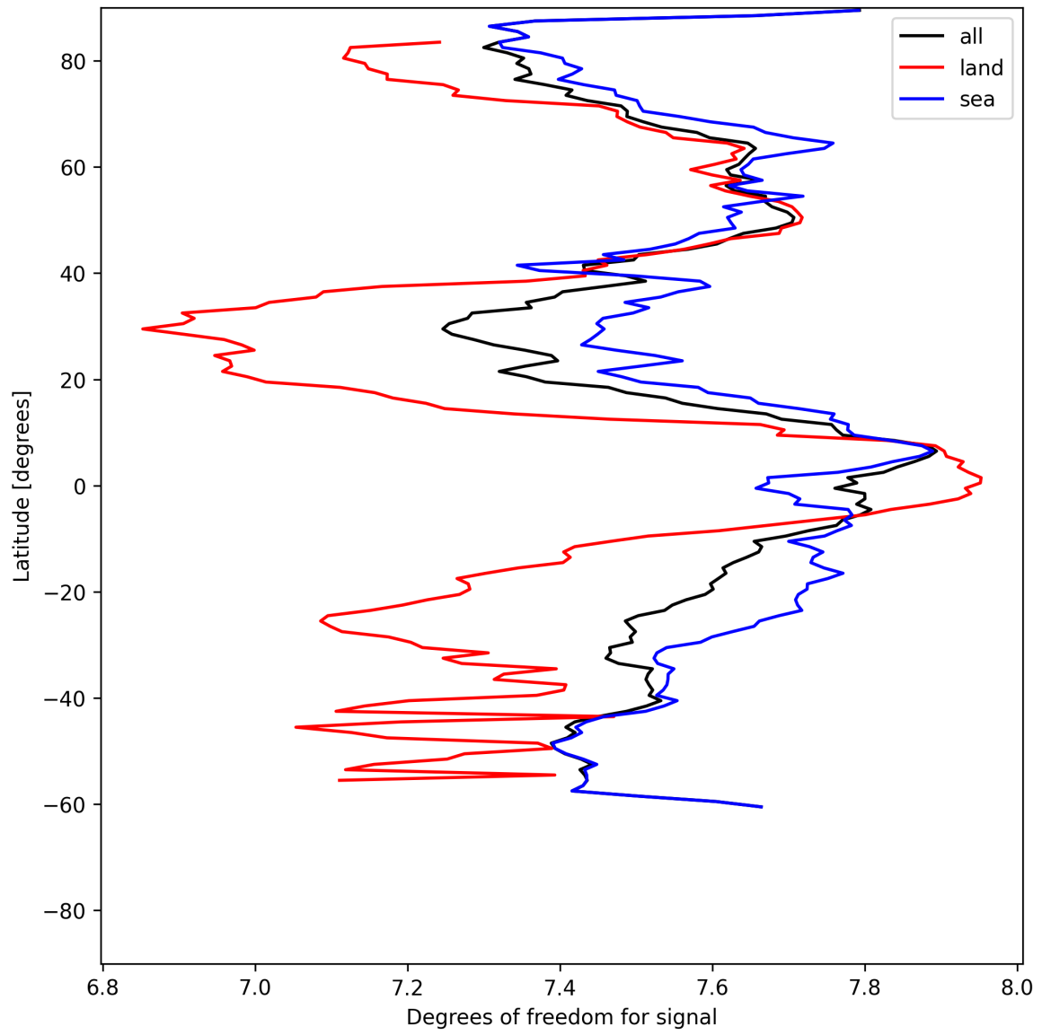
Figure 15: Zonal average of “Degrees of freedom for signal” for 2025-06-17 to 2025-06-18.
