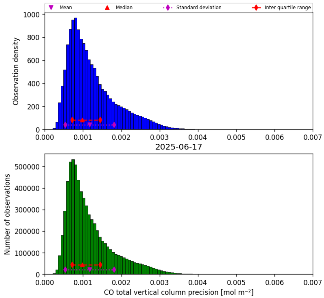
Figure 20: Histogram of “CO total vertical column precision” for 2025-06-17 to 2025-06-18
