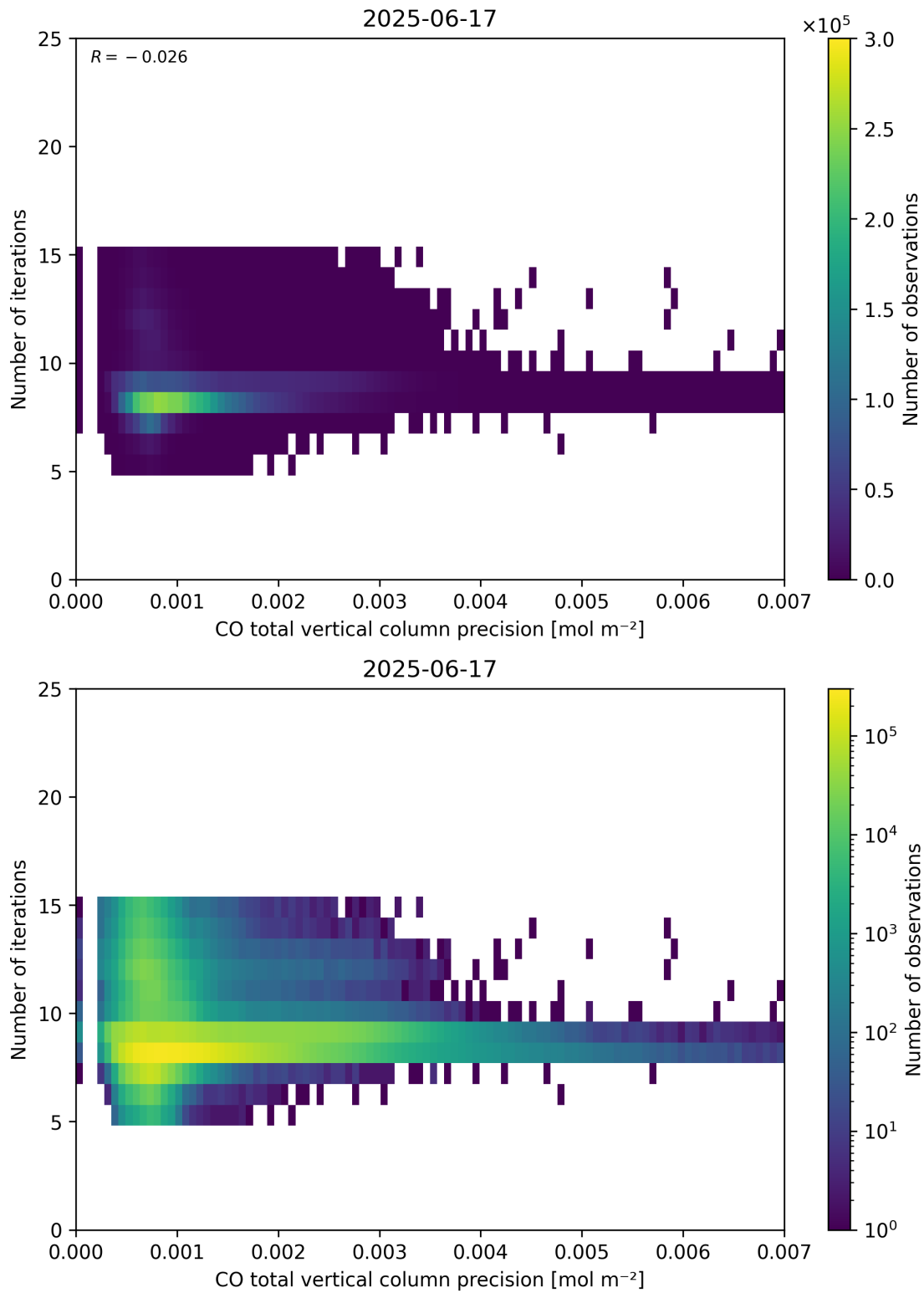
Figure 46: Scatter density plot of “CO total vertical column precision” against “Number of iterations” for 2025-06-17 to 2025-06-18.
