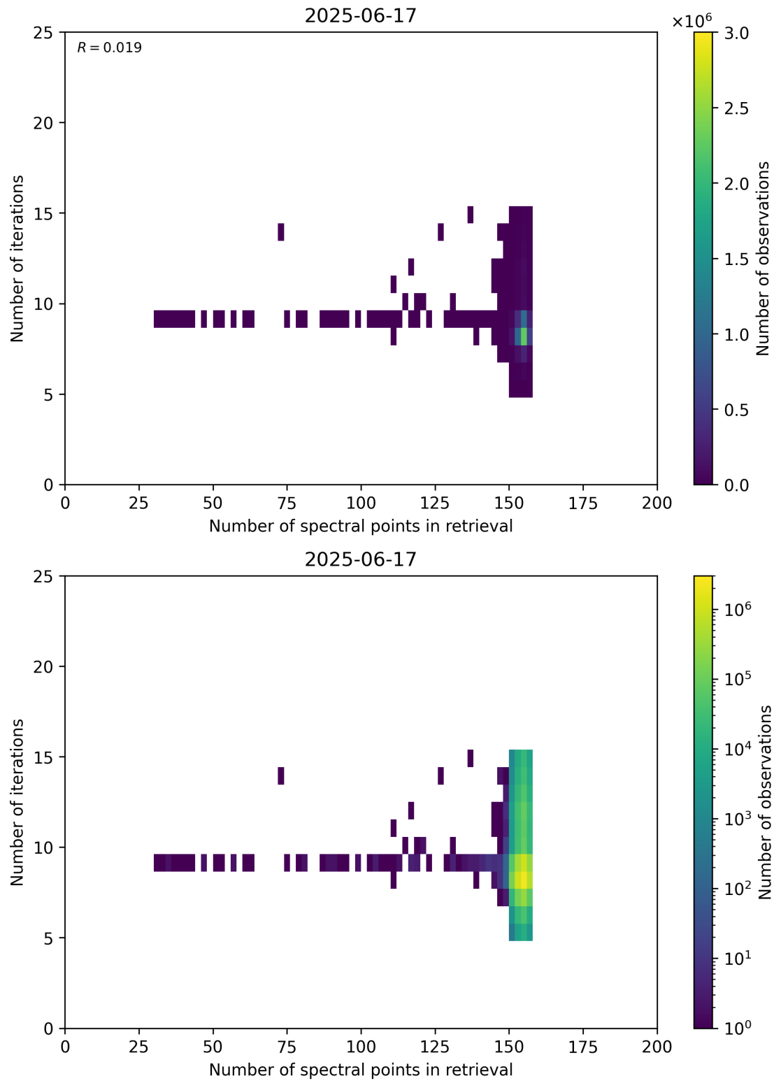
Figure 60: Scatter density plot of “Number of spectral points in retrieval” against “Number of iterations” for 2025-06-17 to 2025-06-18.
