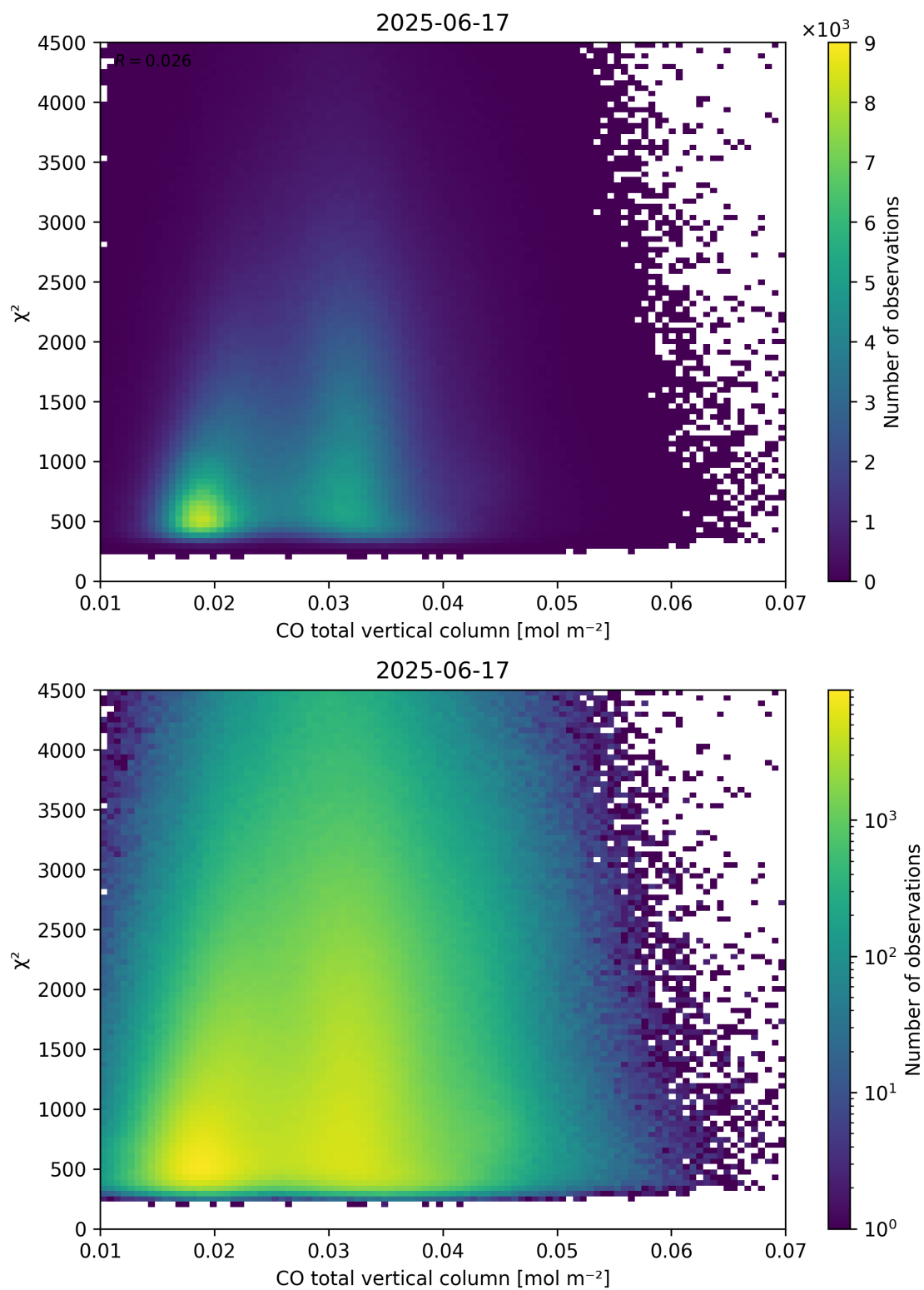
Figure 35: Scatter density plot of “CO total vertical column” against “ \chi^2 ” for 2025-06-17 to 2025-06-18.
