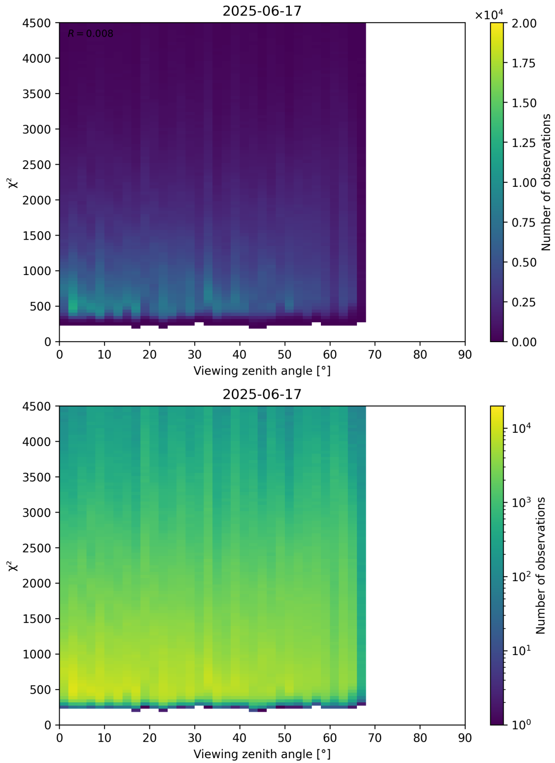
Figure 72: Scatter density plot of “Viewing zenith angle” against “ \chi^2 ” for 2025-06-17 to 2025-06-18.
