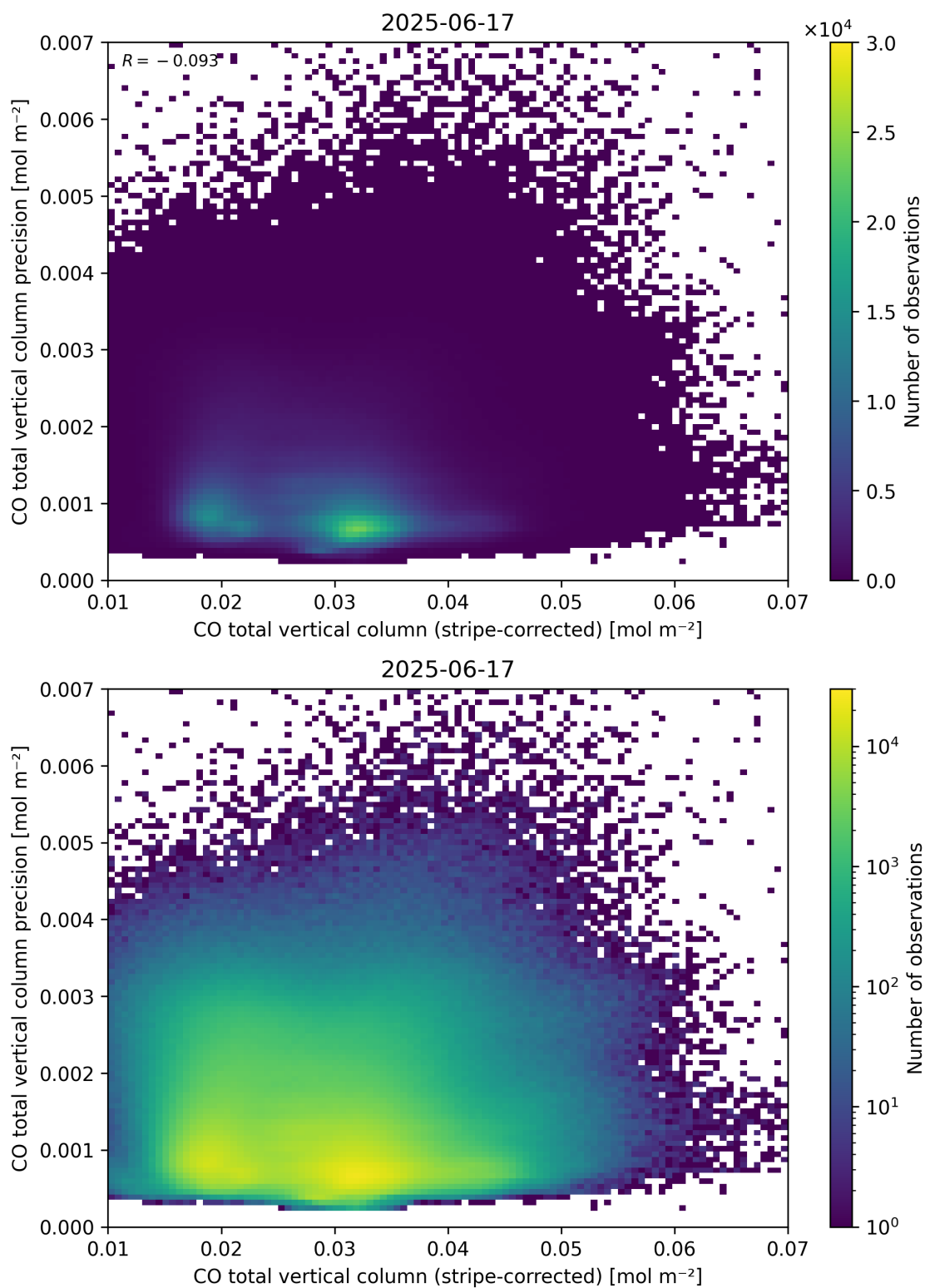
Figure 36: Scatter density plot of “CO total vertical column (stripe-corrected)” against “CO total vertical column precision” for 2025-06-17 to 2025-06-18.
