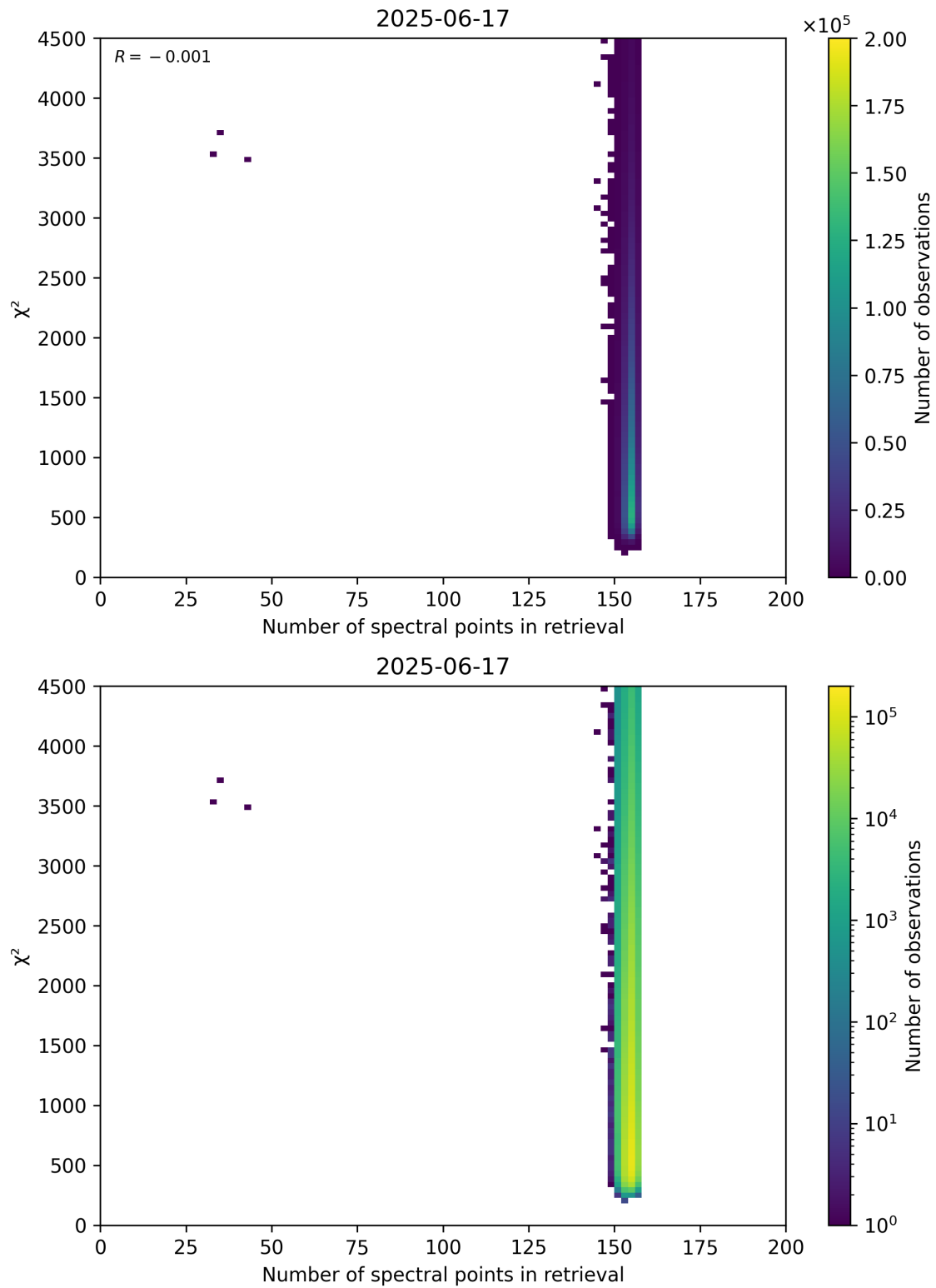
Figure 58: Scatter density plot of “Number of spectral points in retrieval” against “ \chi^2 ” for 2025-06-17 to 2025-06-18.
