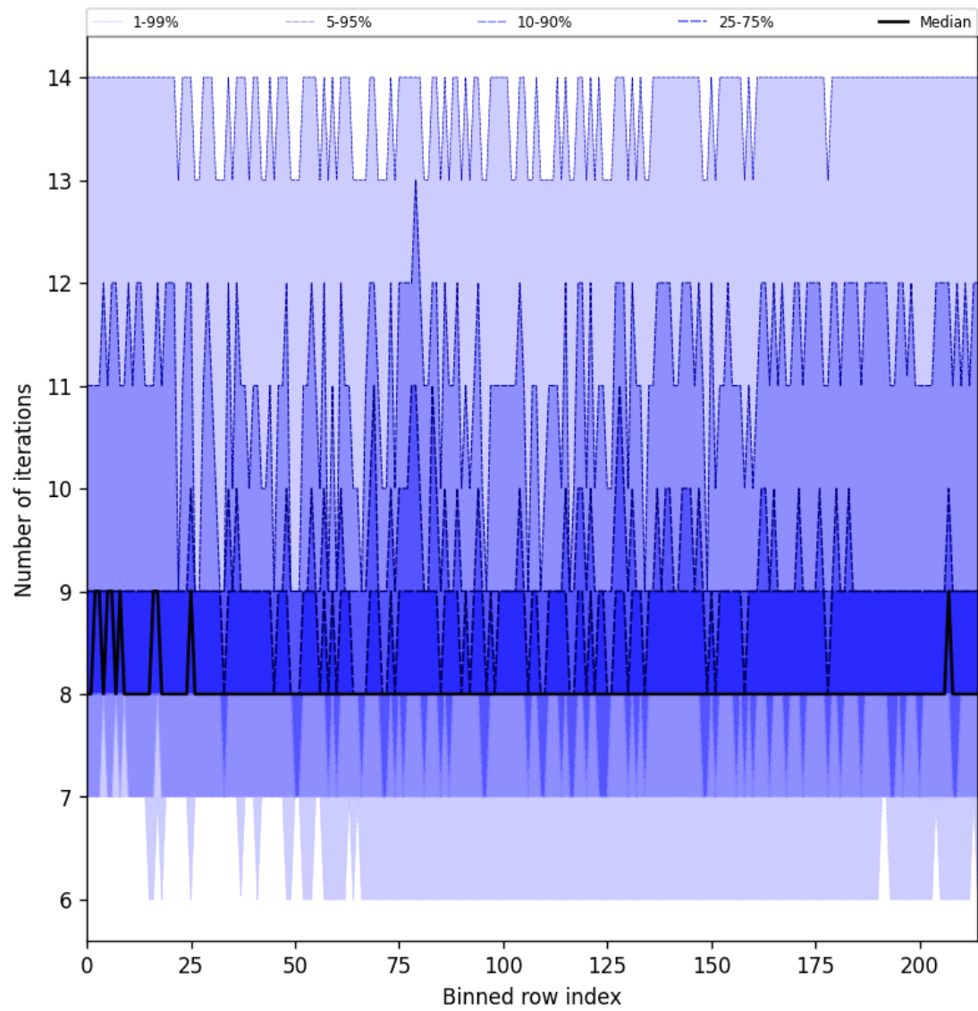
Figure 32: Along track statistics of “Number of iterations” for 2025-06-17 to 2025-06-18
