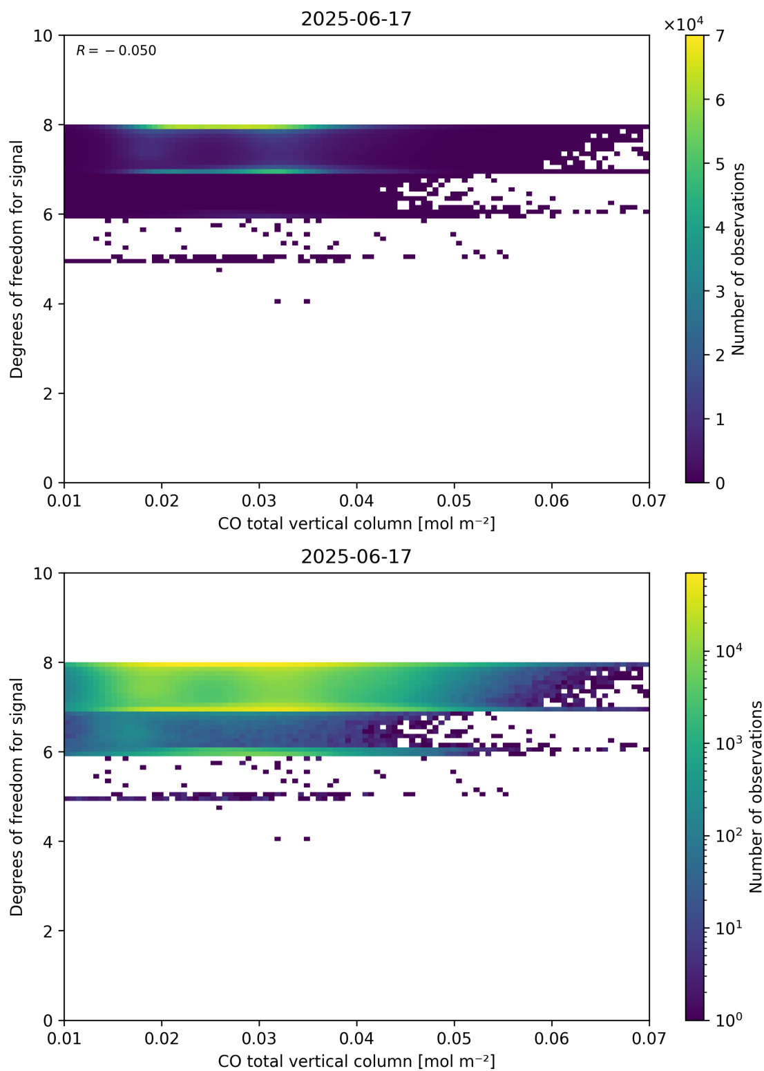
Figure 41: Scatter density plot of “CO total vertical column” against “Degrees of freedom for signal” for 2025-06-17 to 2025-06-18.
