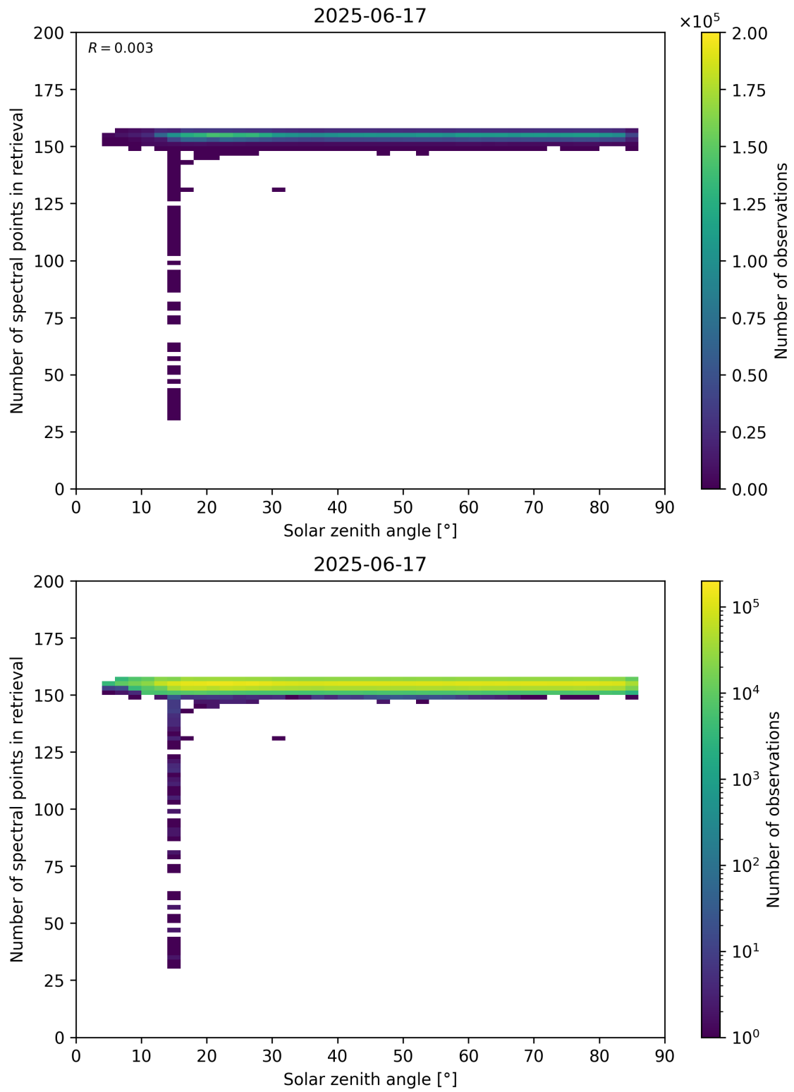
Figure 68: Scatter density plot of “Solar zenith angle” against “Number of spectral points in retrieval” for 2025-06-17 to 2025-06-18.
