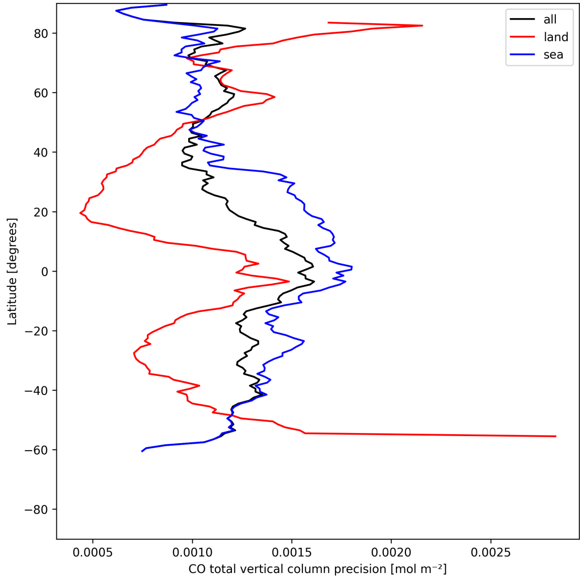
Figure 12: Zonal average of “CO total vertical column precision” for 2025-06-17 to 2025-06-18.
