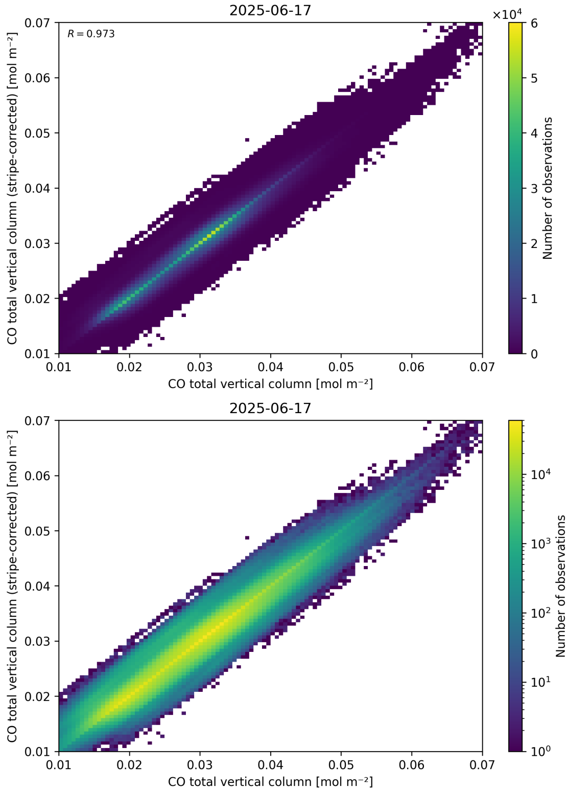
Figure 33: Scatter density plot of “CO total vertical column” against “CO total vertical column (stripe-corrected)” for 2025-06-17 to 2025-06-18.
