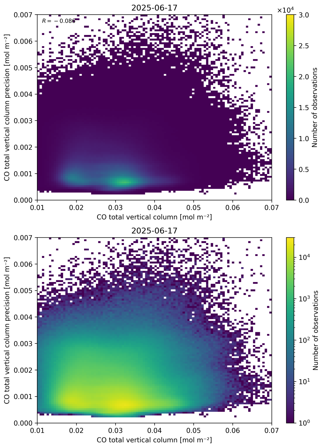
Figure 34: Scatter density plot of “CO total vertical column” against “CO total vertical column precision” for 2025-06-17 to 2025-06-18.
