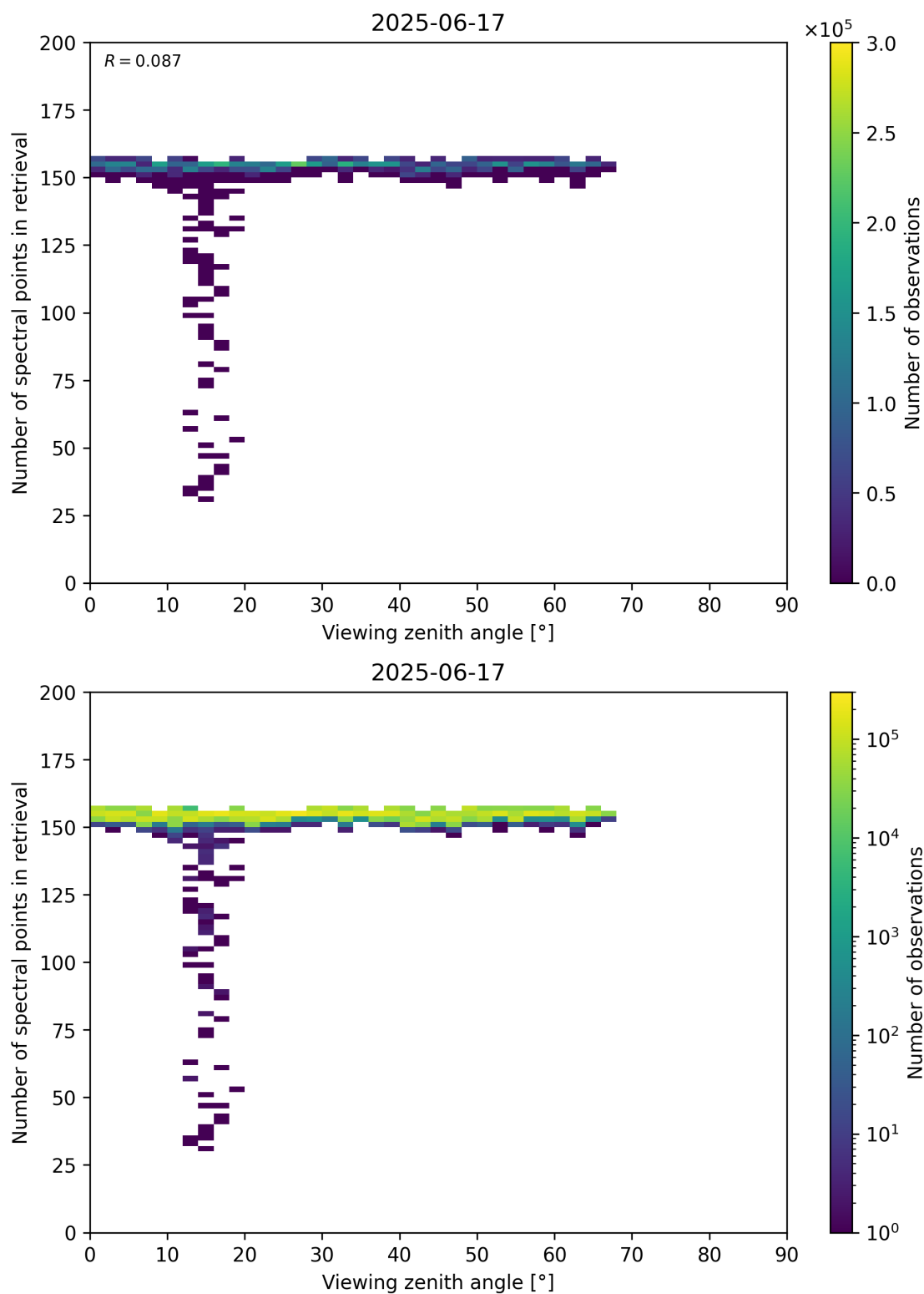
Figure 76: Scatter density plot of “Viewing zenith angle” against “Number of spectral points in retrieval” for 2025-06-17 to 2025-06-18.
