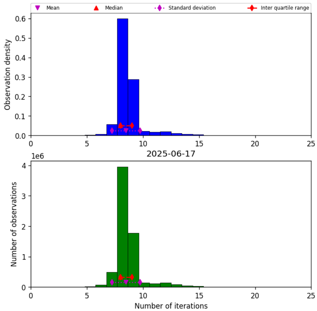
Figure 24: Histogram of “Number of iterations” for 2025-06-17 to 2025-06-18
