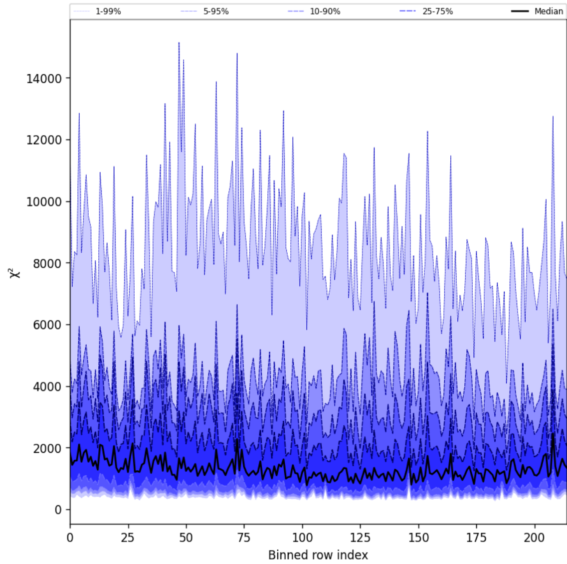
Figure 30: Along track statistics of “ \chi^2 ” for 2025-06-17 to 2025-06-18
