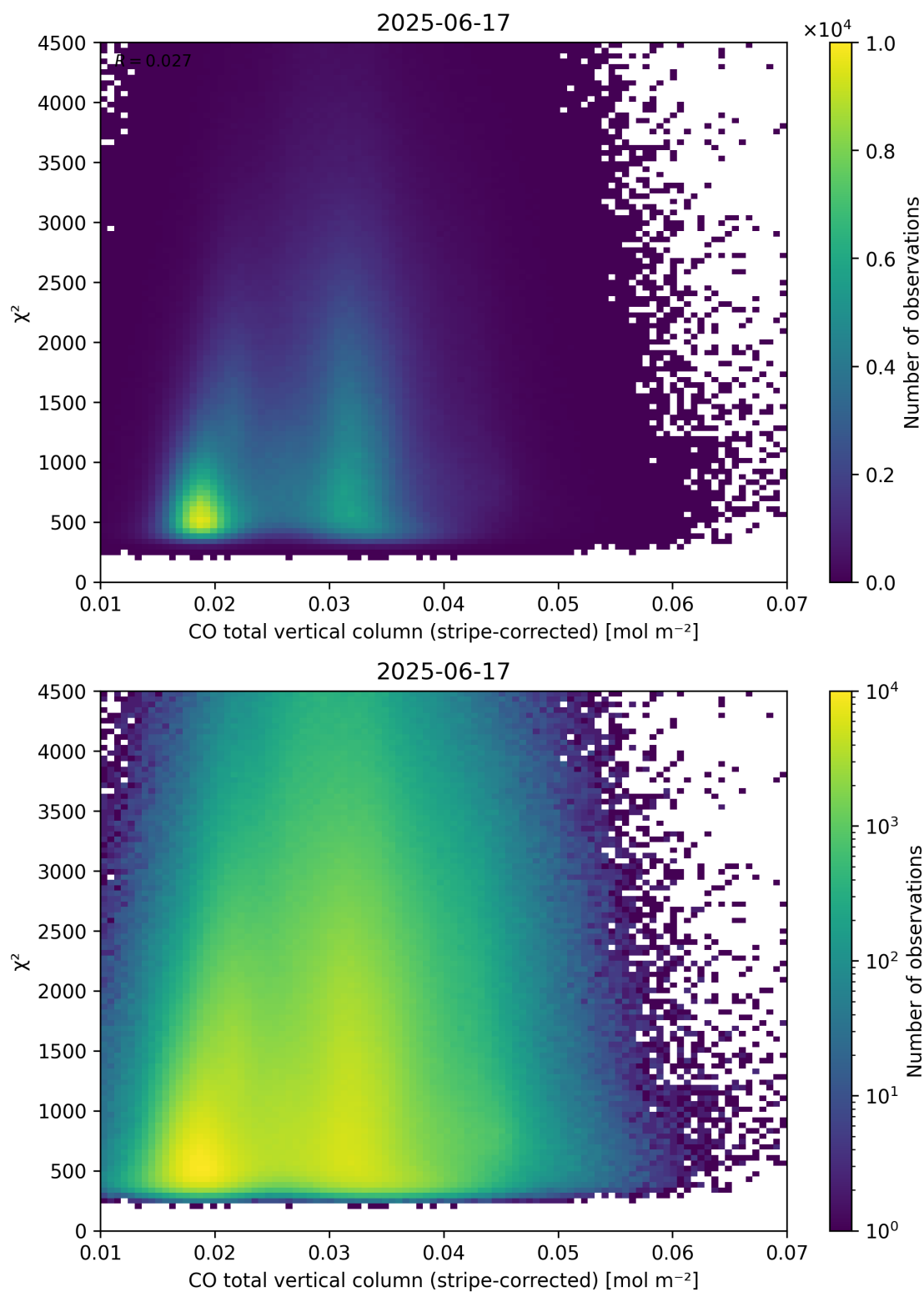
Figure 37: Scatter density plot of “CO total vertical column (stripe-corrected)” against “ \chi^2 ” for 2025-06-17 to 2025-06-18.
