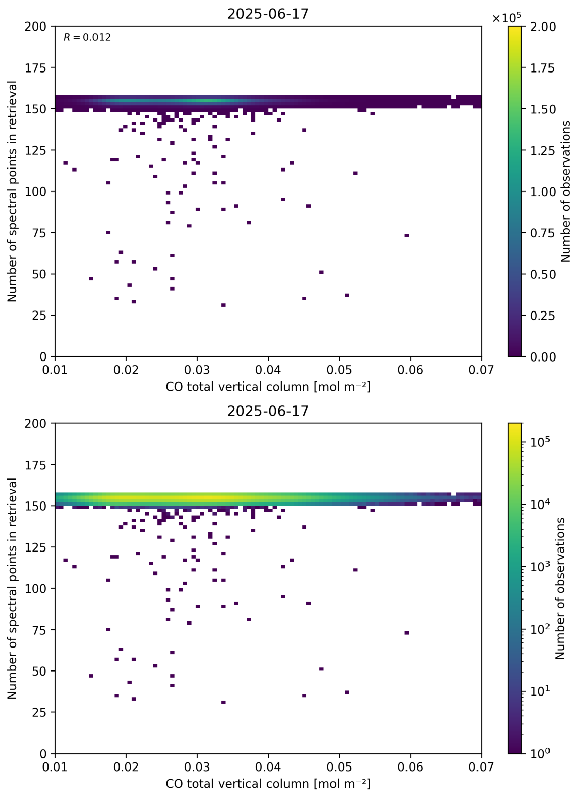
Figure 43: Scatter density plot of “CO total vertical column” against “Number of spectral points in retrieval” for 2025-06-17 to 2025-06-18.
