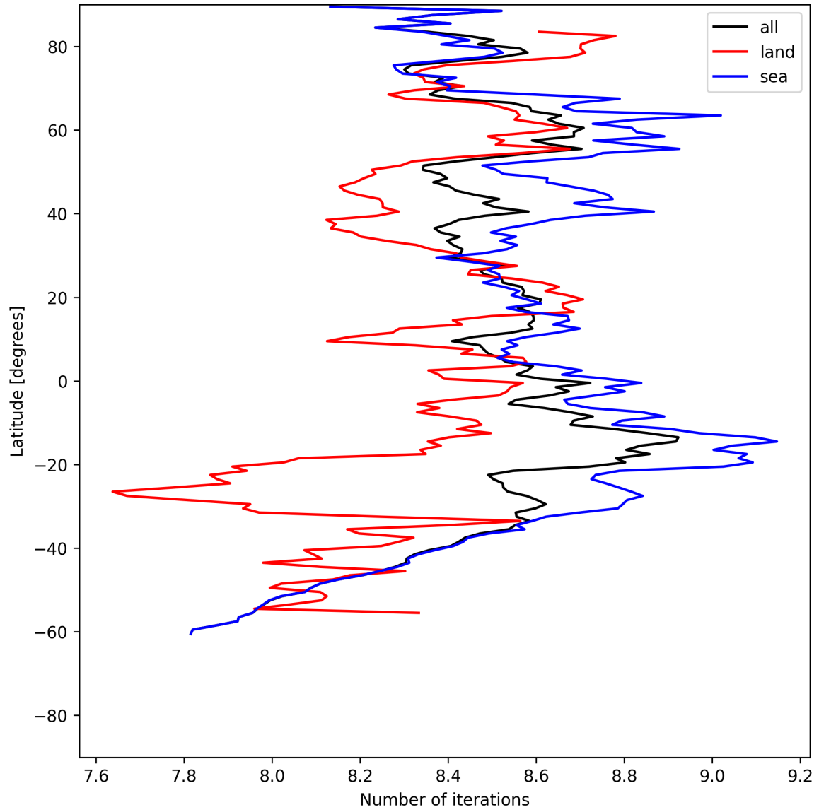
Figure 16: Zonal average of “Number of iterations” for 2025-06-17 to 2025-06-18.
