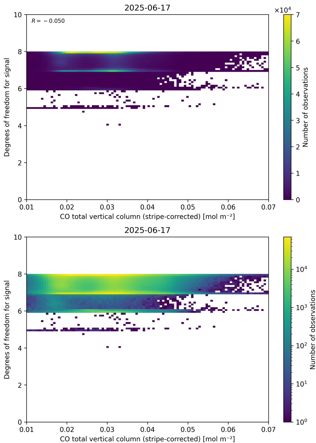
Figure 38: Scatter density plot of “CO total vertical column (stripe-corrected)” against “Degrees of freedom for signal” for 2025-06-17 to 2025-06-18.
