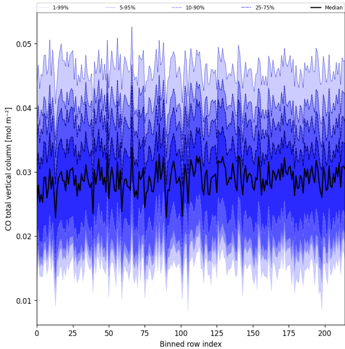
Figure 26: Along track statistics of “CO total vertical column” for 2025-06-17 to 2025-06-18
