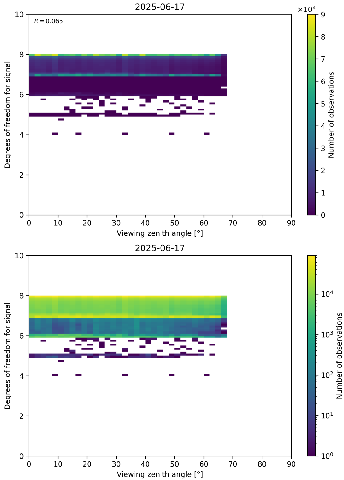
Figure 73: Scatter density plot of “Viewing zenith angle” against “Degrees of freedom for signal” for 2025-06-17 to 2025-06-18.
