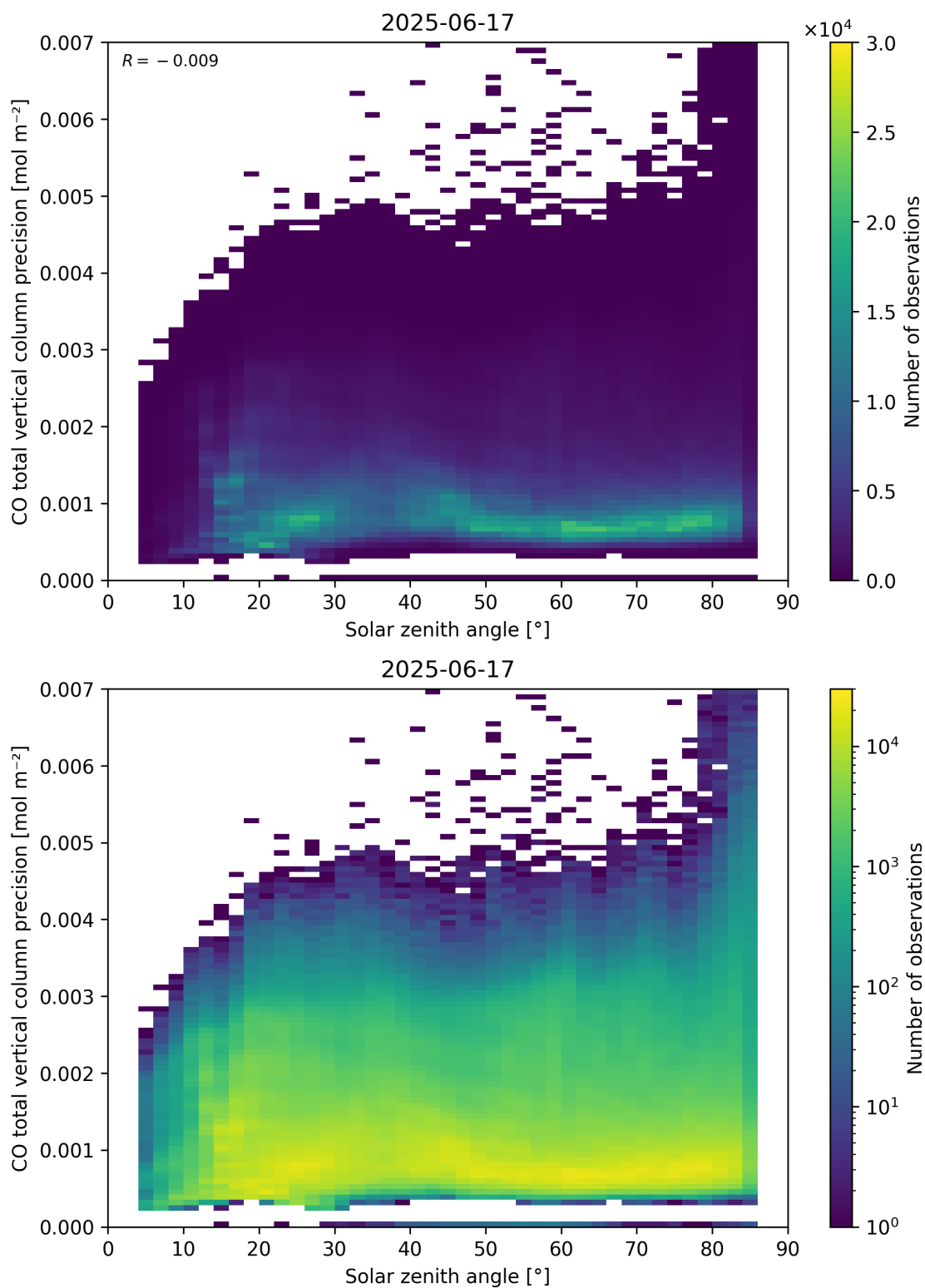
Figure 63: Scatter density plot of “Solar zenith angle” against “CO total vertical column precision” for 2025-06-17 to 2025-06-18.
