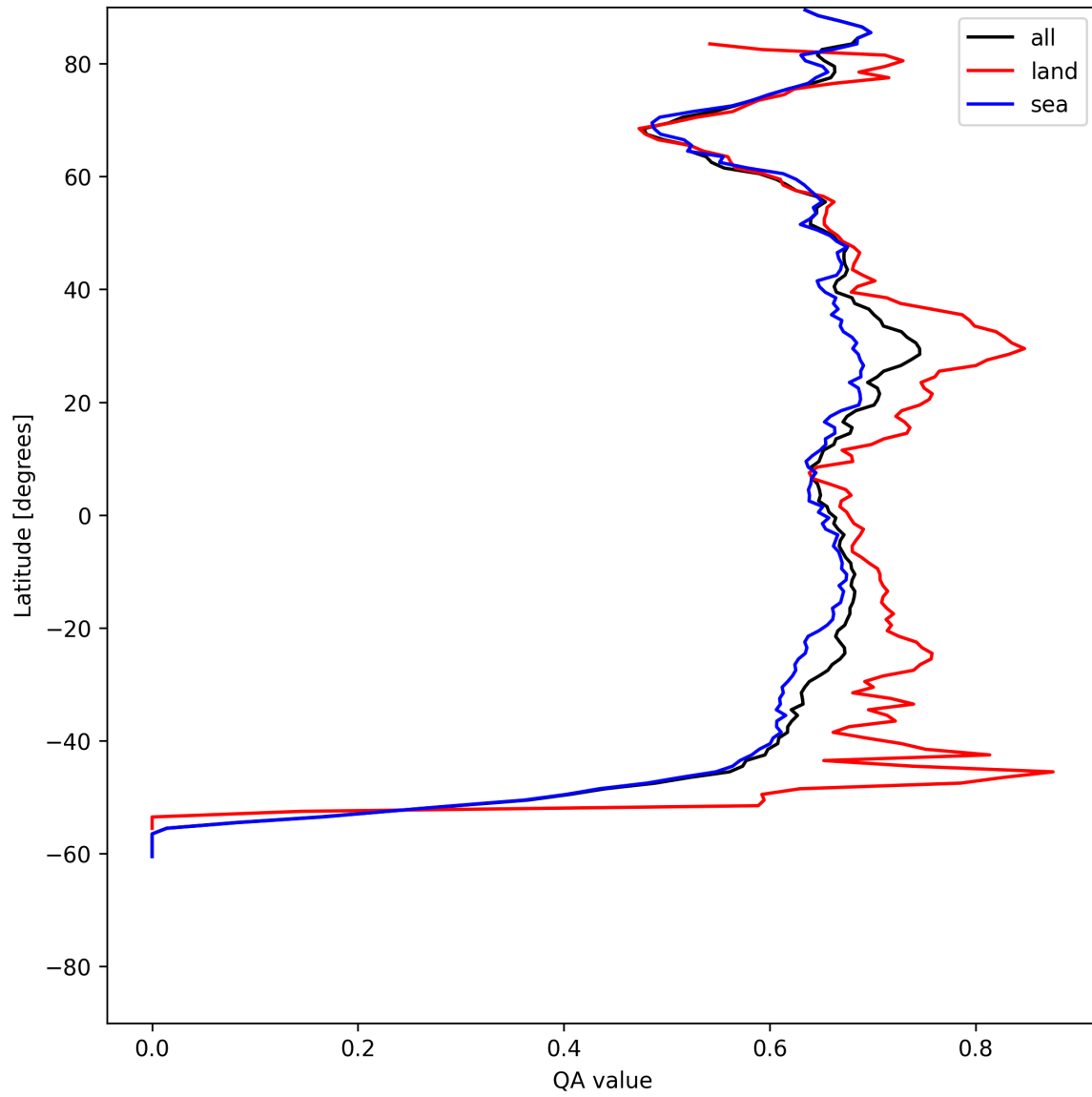
Figure 9: Zonal average of “QA value” for 2025-06-17 to 2025-06-18.
