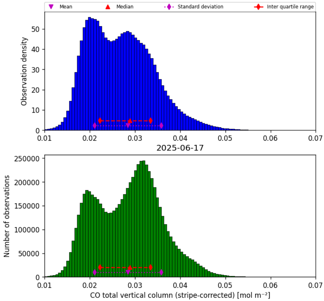
Figure 19: Histogram of “CO total vertical column (stripe-corrected)” for 2025-06-17 to 2025-06-18
