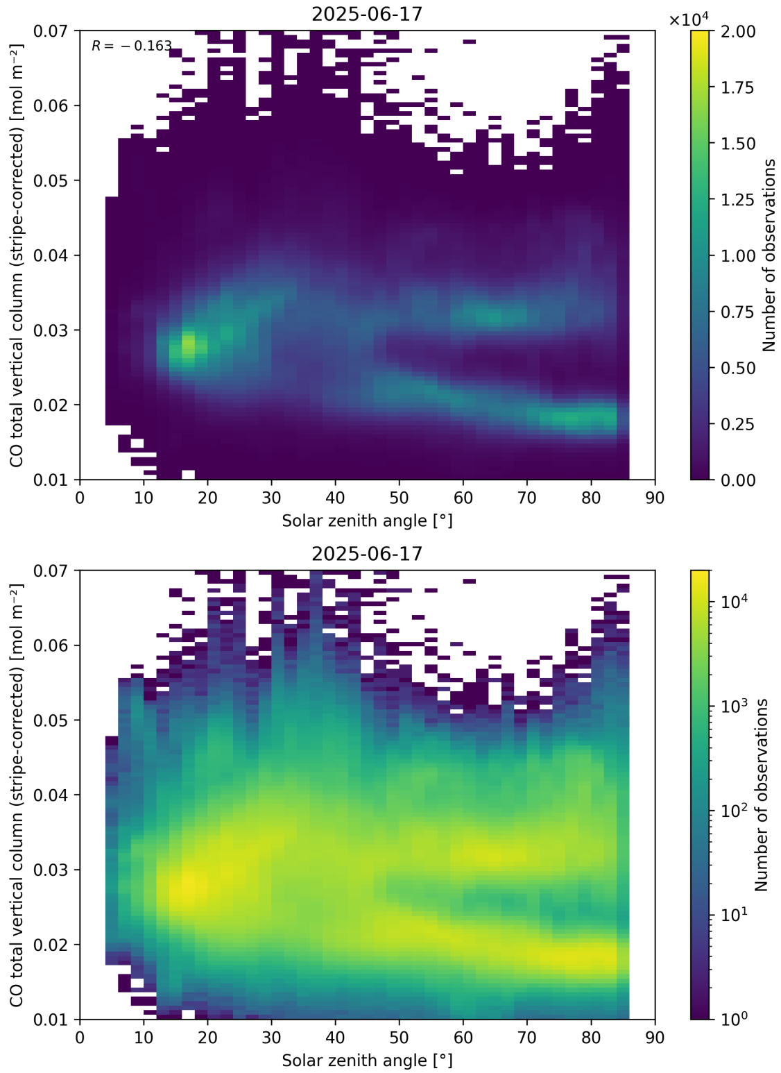
Figure 62: Scatter density plot of “Solar zenith angle” against “CO total vertical column (stripe-corrected)” for 2025-06-17 to 2025-06-18.
