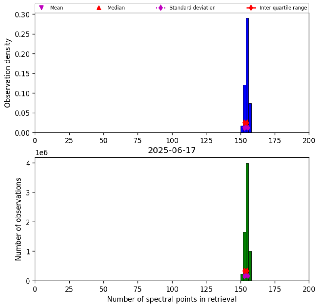
Figure 21: Histogram of “Number of spectral points in retrieval” for 2025-06-17 to 2025-06-18
