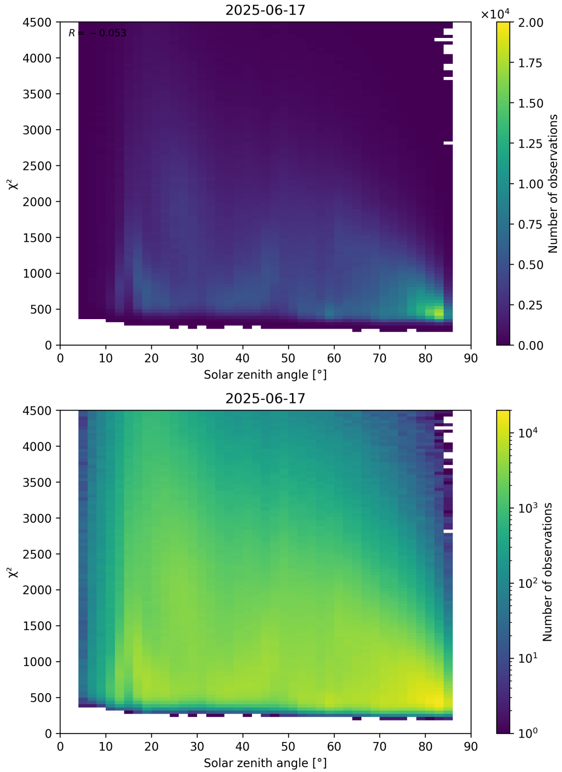
Figure 64: Scatter density plot of “Solar zenith angle” against “ \chi^2 ” for 2025-06-17 to 2025-06-18.
