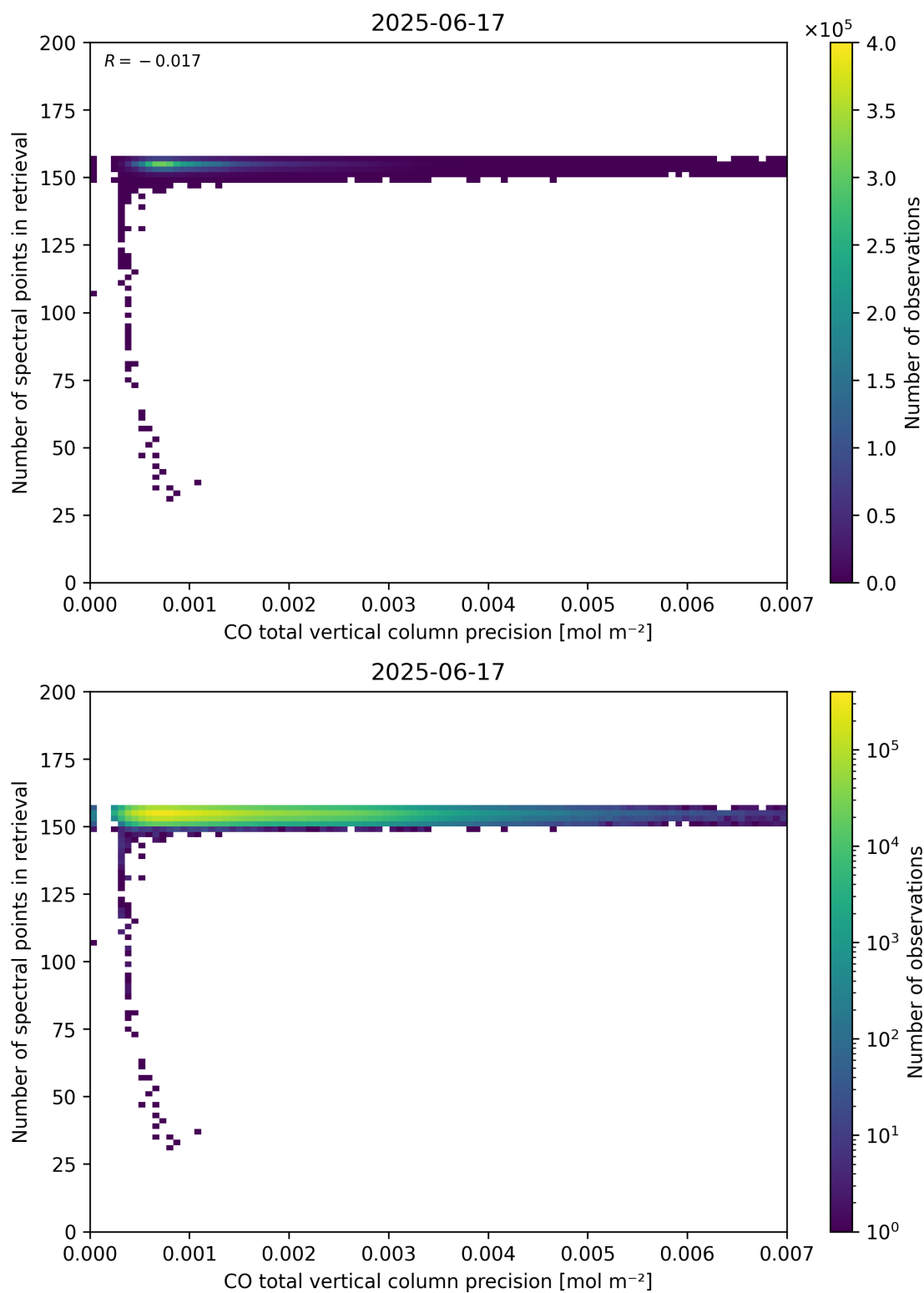
Figure 47: Scatter density plot of “CO total vertical column precision” against “Number of spectral points in retrieval” for 2025-06-17 to 2025-06-18.
