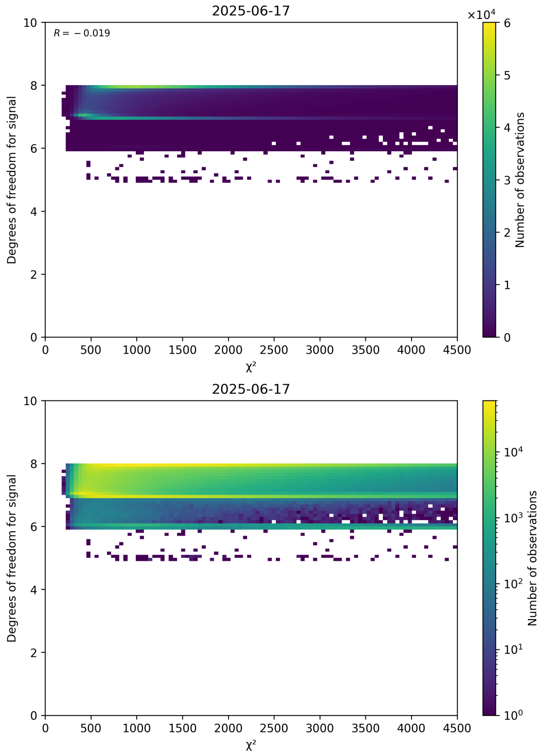
Figure 48: Scatter density plot of “ \chi^2 ” against “Degrees of freedom for signal” for 2025-06-17 to 2025-06-18.
