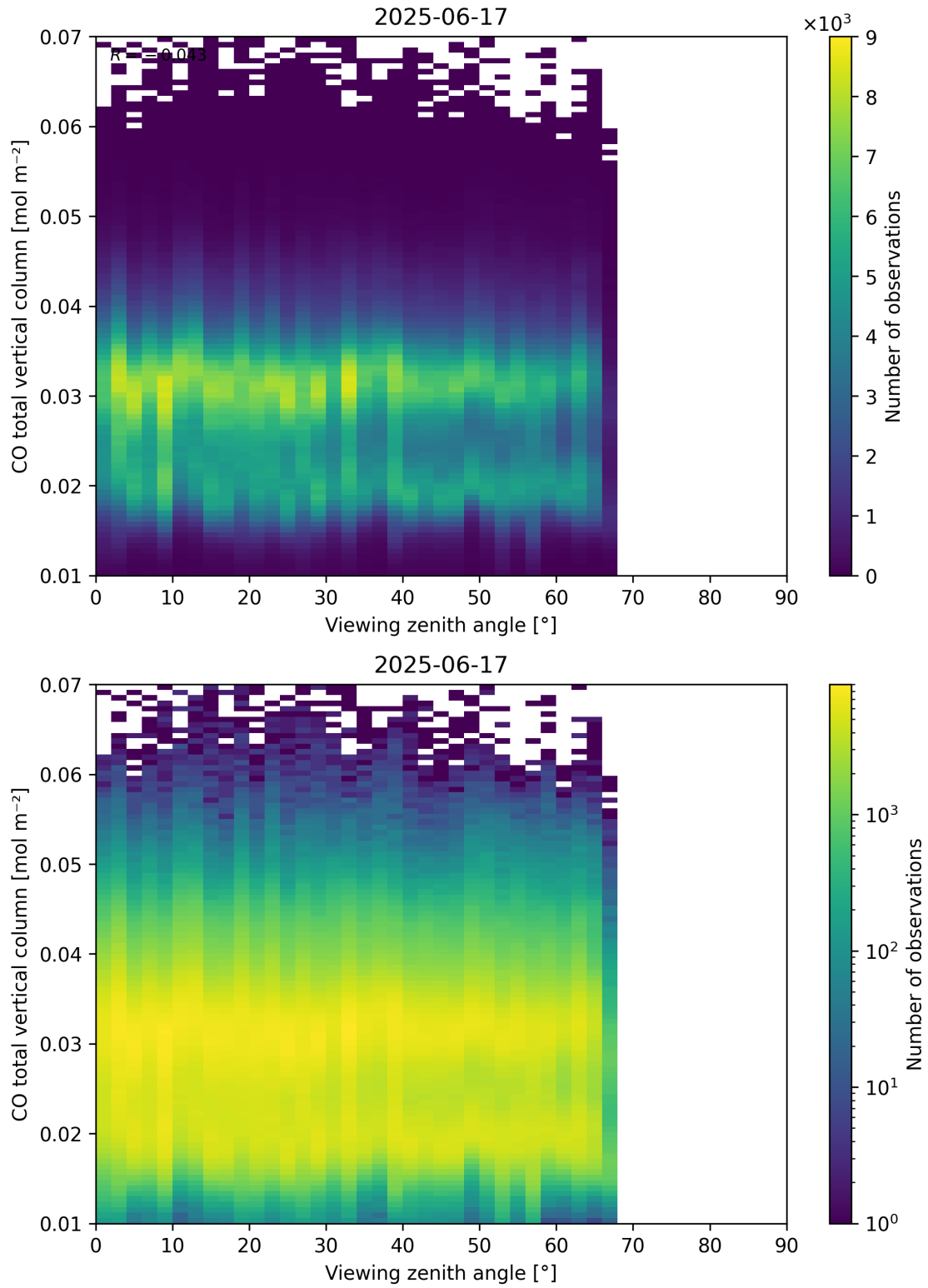
Figure 69: Scatter density plot of “Viewing zenith angle” against “CO total vertical column” for 2025-06-17 to 2025-06-18.
