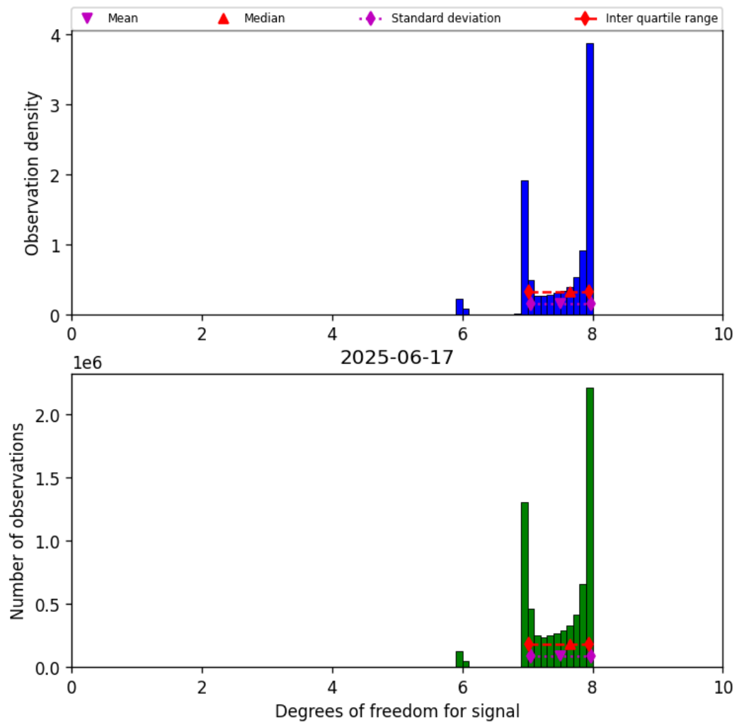
Figure 23: Histogram of “Degrees of freedom for signal” for 2025-06-17 to 2025-06-18
