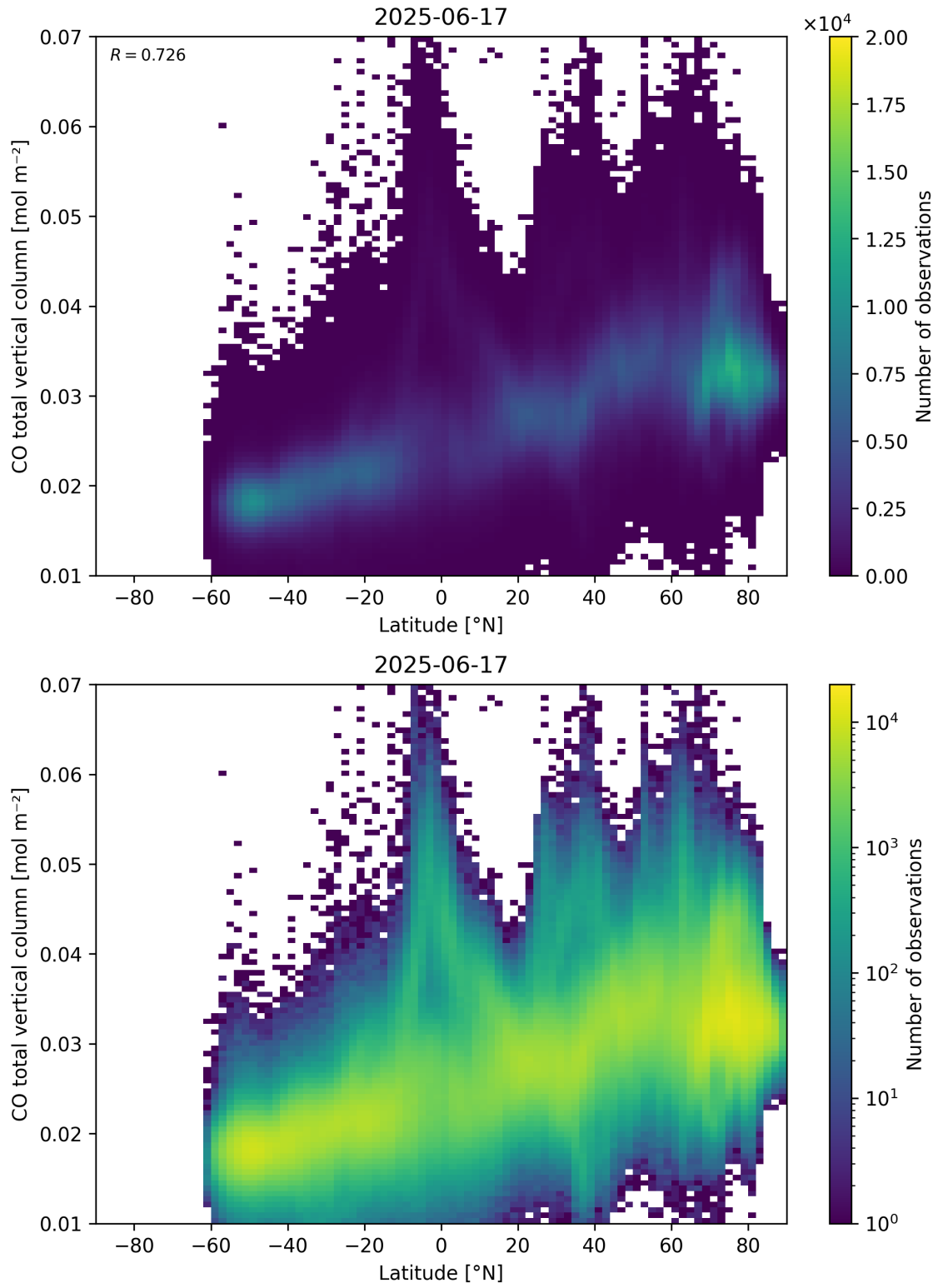
Figure 51: Scatter density plot of “Latitude” against “CO total vertical column” for 2025-06-17 to 2025-06-18.
