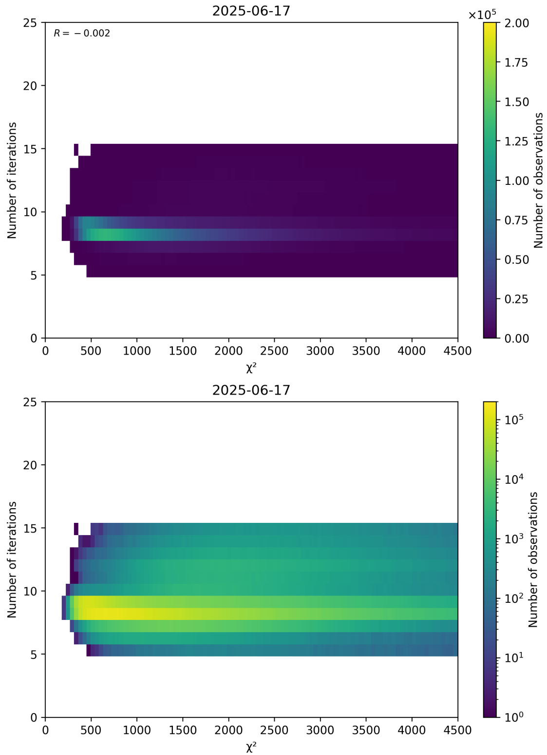
Figure 49: Scatter density plot of “ \chi^2 ” against “Number of iterations” for 2025-06-17 to 2025-06-18.
