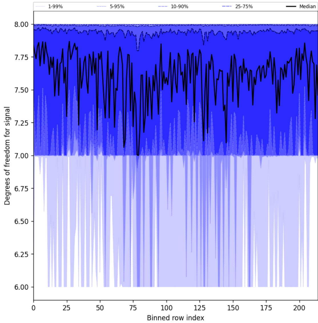
Figure 31: Along track statistics of “Degrees of freedom for signal” for 2025-06-17 to 2025-06-18
