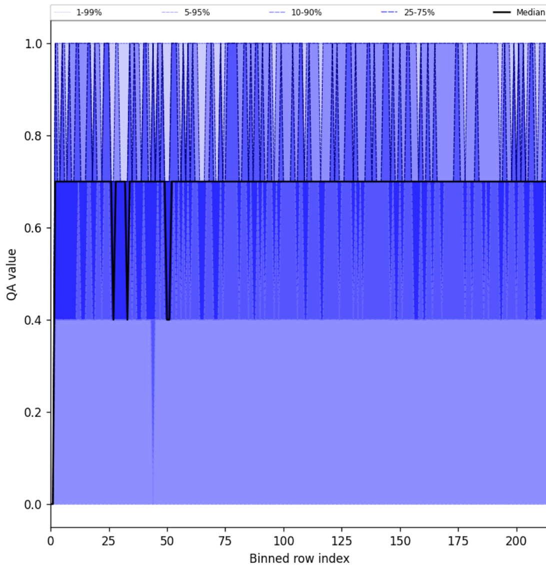
Figure 25: Along track statistics of “QA value” for 2025-06-17 to 2025-06-18
