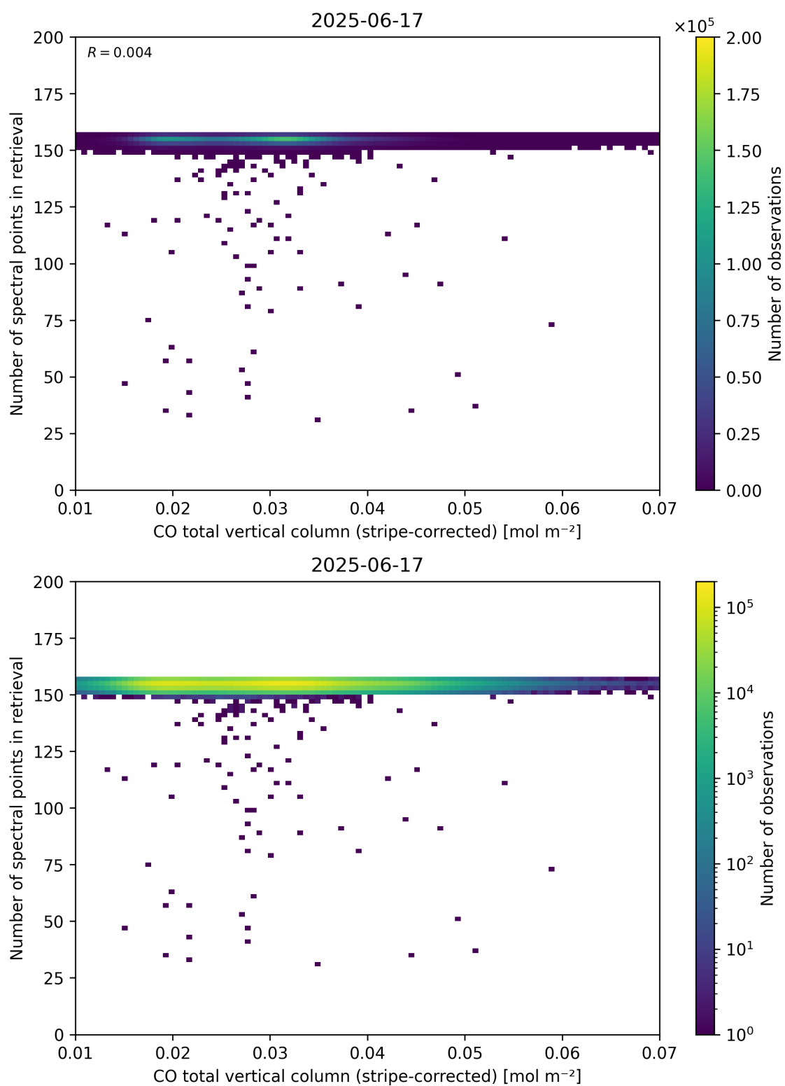
Figure 40: Scatter density plot of “CO total vertical column (stripe-corrected)” against “Number of spectral points in retrieval” for 2025-06-17 to 2025-06-18.
