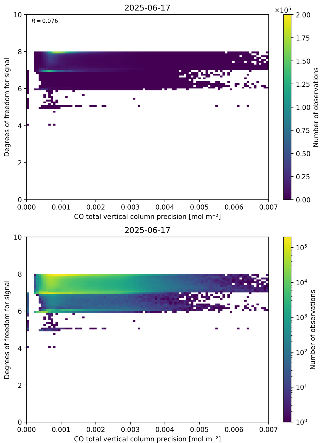
Figure 45: Scatter density plot of “CO total vertical column precision” against “Degrees of freedom for signal” for 2025-06-17 to 2025-06-18.
