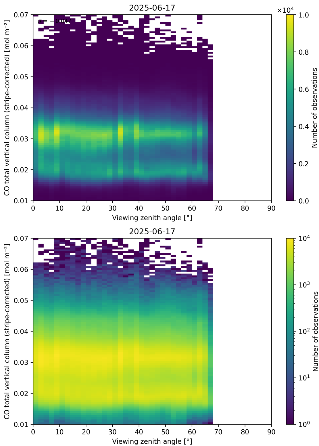
Figure 70: Scatter density plot of “Viewing zenith angle” against “CO total vertical column (stripe-corrected)” for 2025-06-17 to 2025-06-18.
