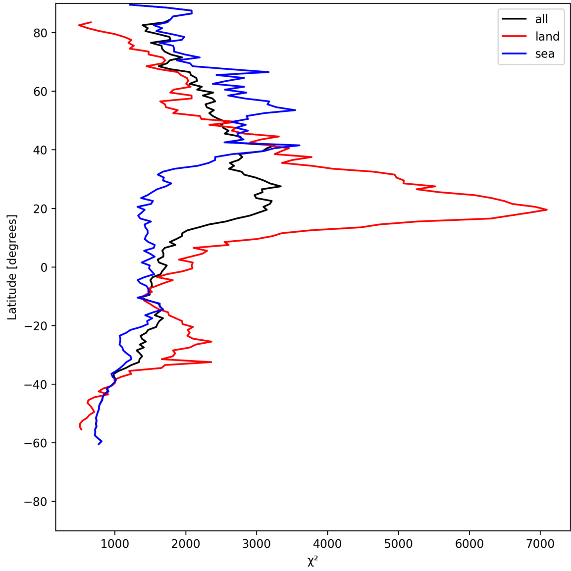
Figure 14: Zonal average of “ \chi^2 ” for 2025-06-17 to 2025-06-18.
