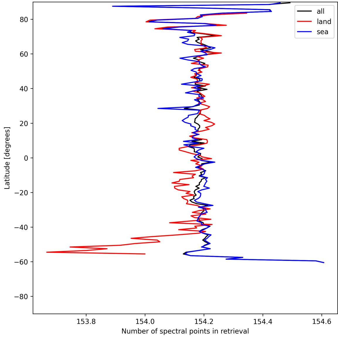
Figure 13: Zonal average of “Number of spectral points in retrieval” for 2025-06-17 to 2025-06-18.
