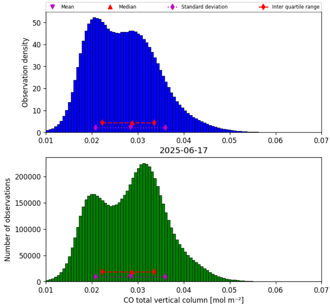
Figure 18: Histogram of “CO total vertical column” for 2025-06-17 to 2025-06-18
