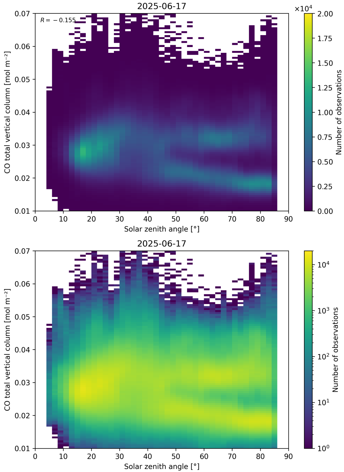
Figure 61: Scatter density plot of “Solar zenith angle” against “CO total vertical column” for 2025-06-17 to 2025-06-18.
