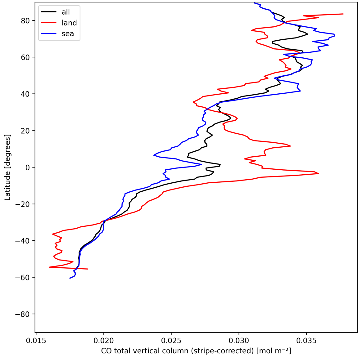
Figure 11: Zonal average of “CO total vertical column (stripe-corrected)” for 2025-06-17 to 2025-06-18.
