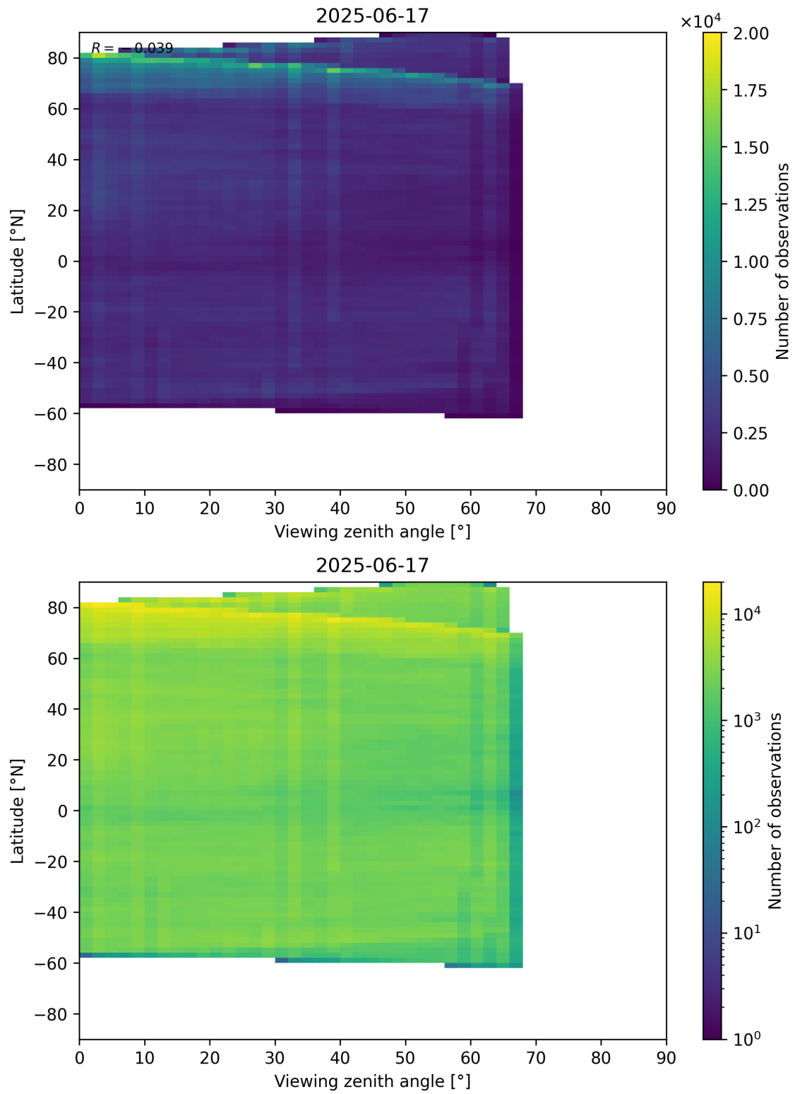
Figure 74: Scatter density plot of “Viewing zenith angle” against “Latitude” for 2025-06-17 to 2025-06-18.
