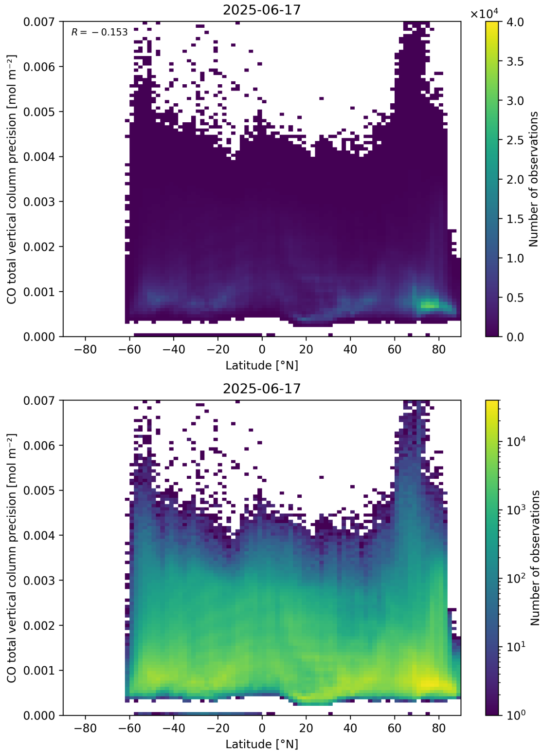
Figure 53: Scatter density plot of “Latitude” against “CO total vertical column precision” for 2025-06-17 to 2025-06-18.
