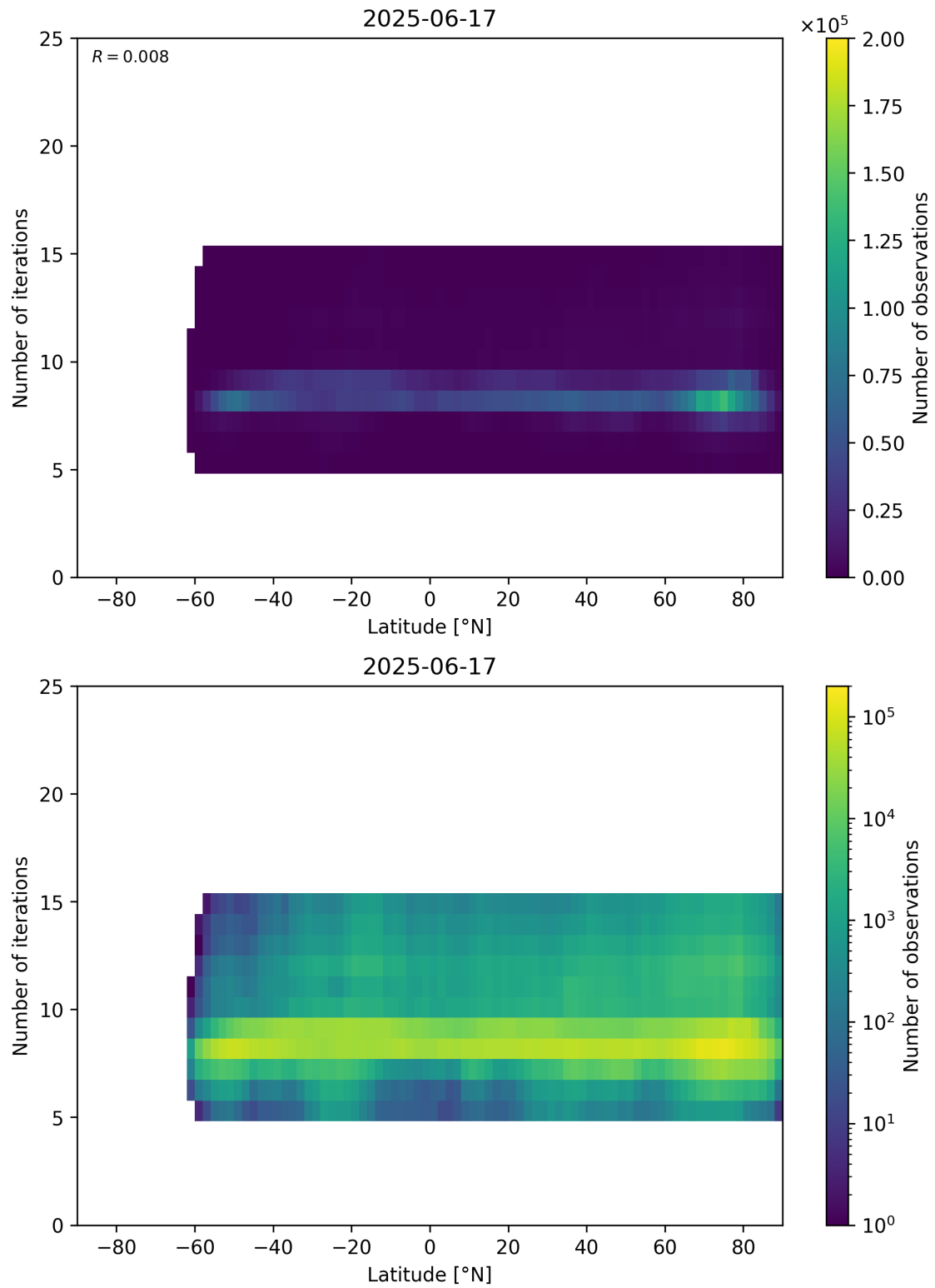
Figure 56: Scatter density plot of “Latitude” against “Number of iterations” for 2025-06-17 to 2025-06-18.
