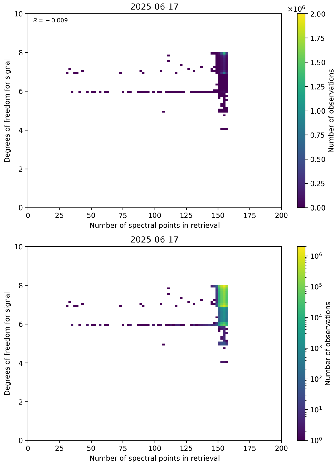
Figure 59: Scatter density plot of “Number of spectral points in retrieval” against “Degrees of freedom for signal” for 2025-06-17 to 2025-06-18.
