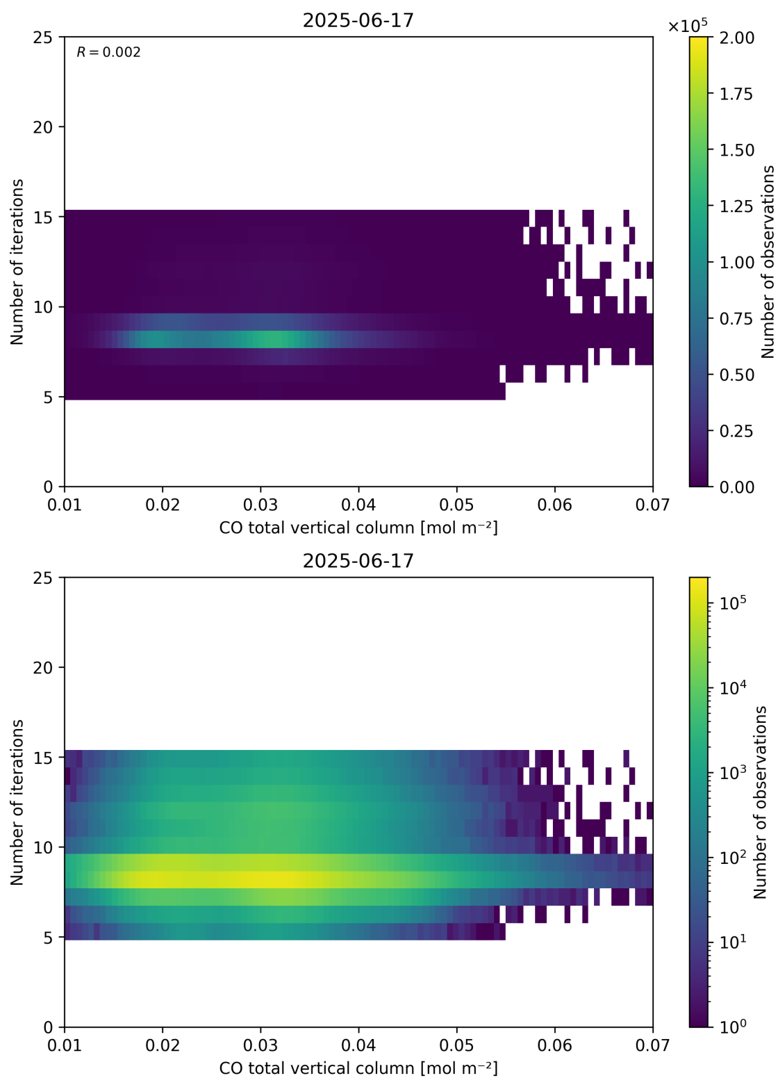
Figure 42: Scatter density plot of “CO total vertical column” against “Number of iterations” for 2025-06-17 to 2025-06-18.
