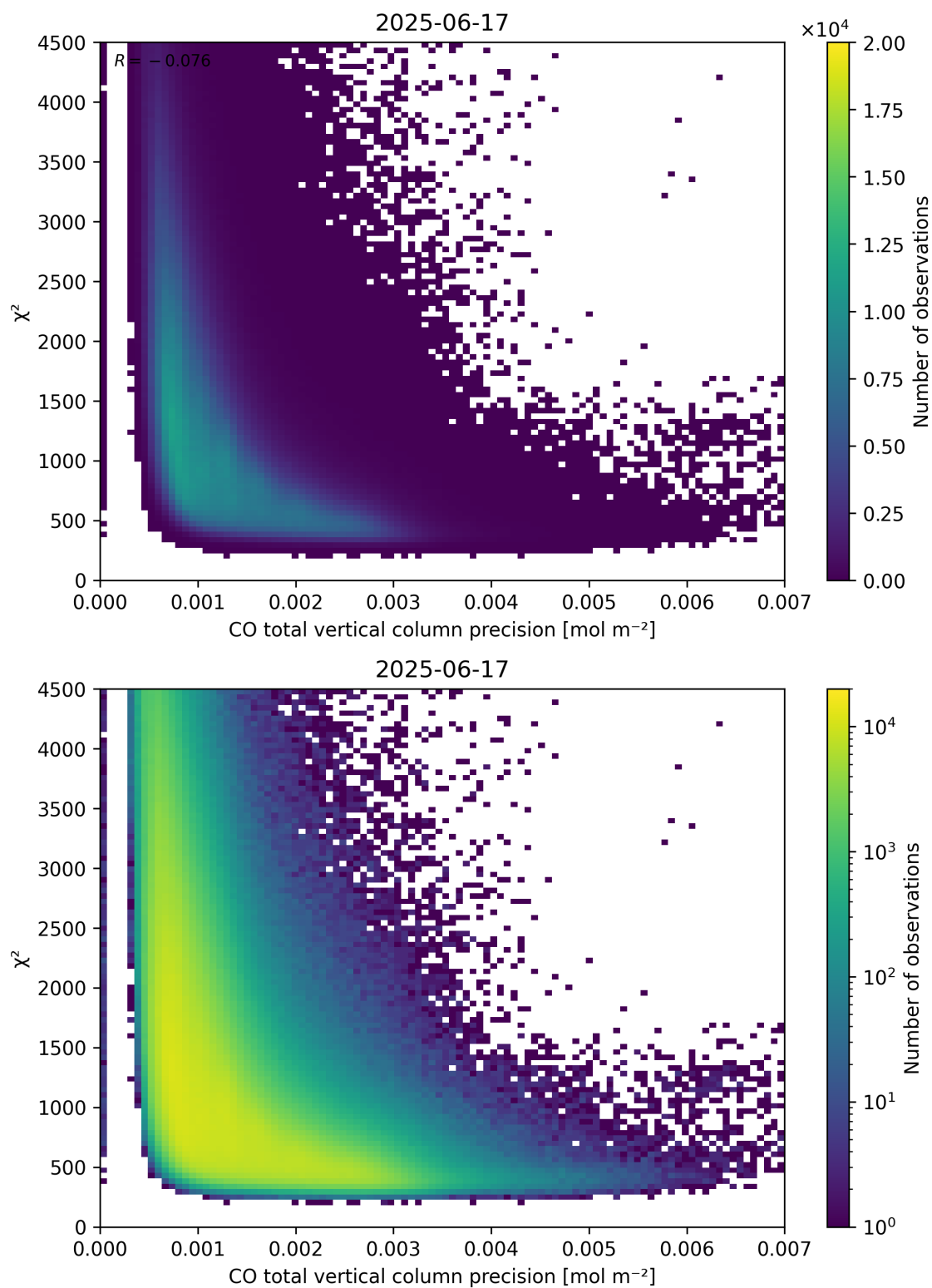
Figure 44: Scatter density plot of “CO total vertical column precision” against “ \chi^2 ” for 2025-06-17 to 2025-06-18.
