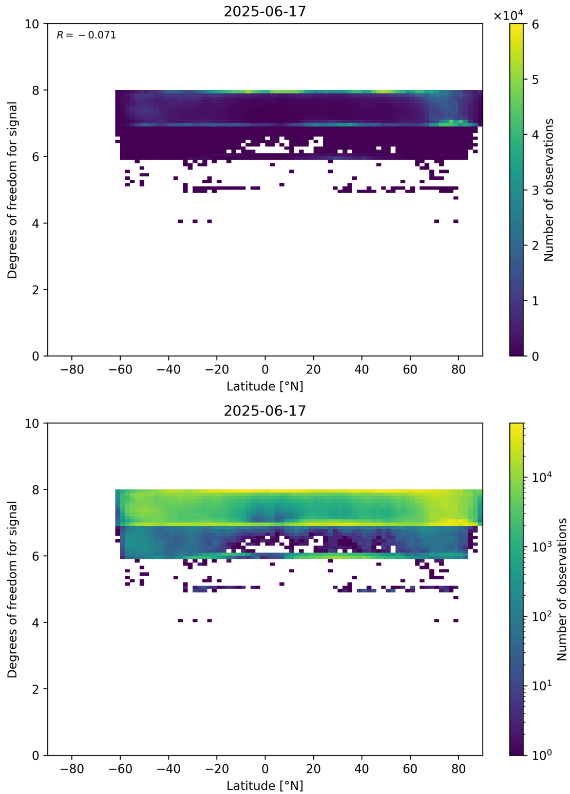
Figure 55: Scatter density plot of “Latitude” against “Degrees of freedom for signal” for 2025-06-17 to 2025-06-18.
