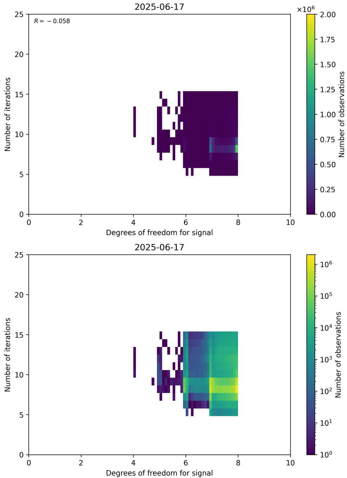
Figure 50: Scatter density plot of “Degrees of freedom for signal” against “Number of iterations” for 2025-06-17 to 2025-06-18.
