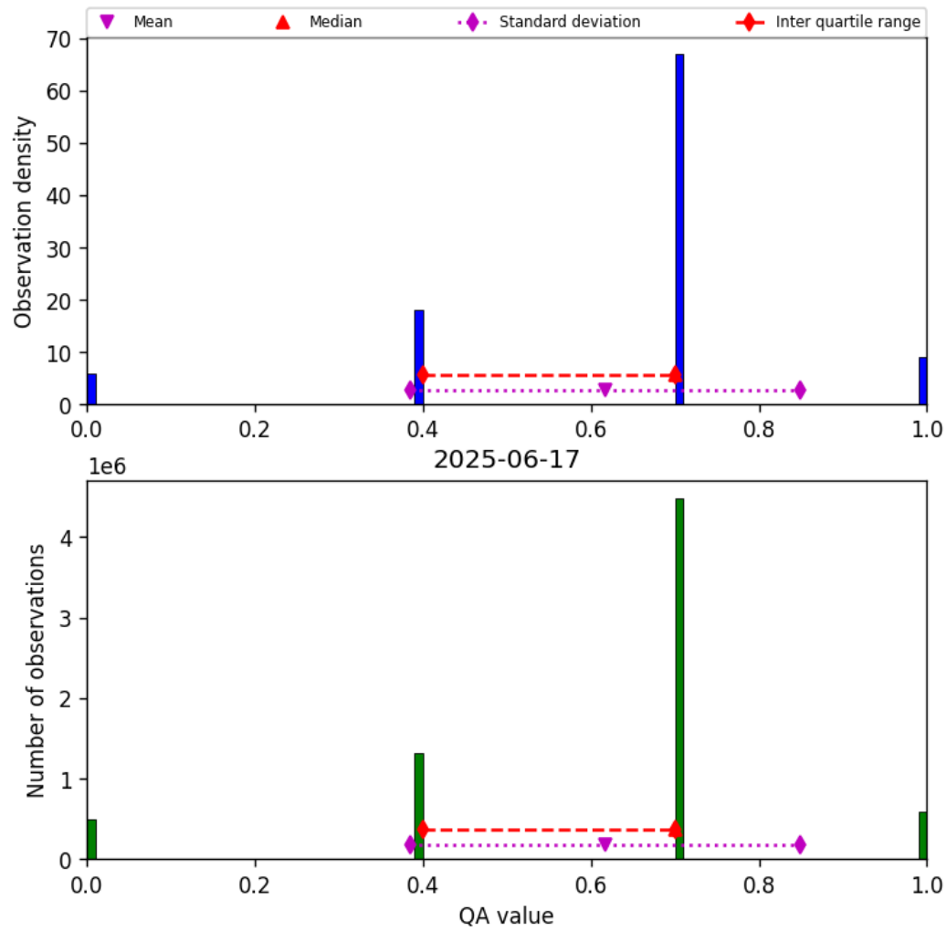
Figure 17: Histogram of “QA value” for 2025-06-17 to 2025-06-18
