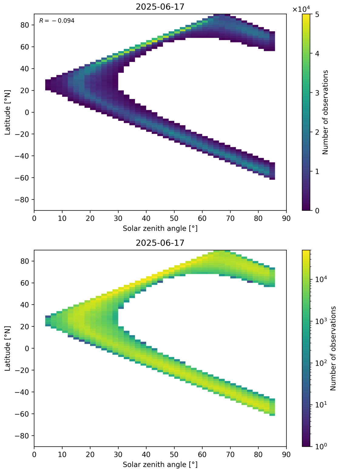
Figure 66: Scatter density plot of “Solar zenith angle” against “Latitude” for 2025-06-17 to 2025-06-18.
