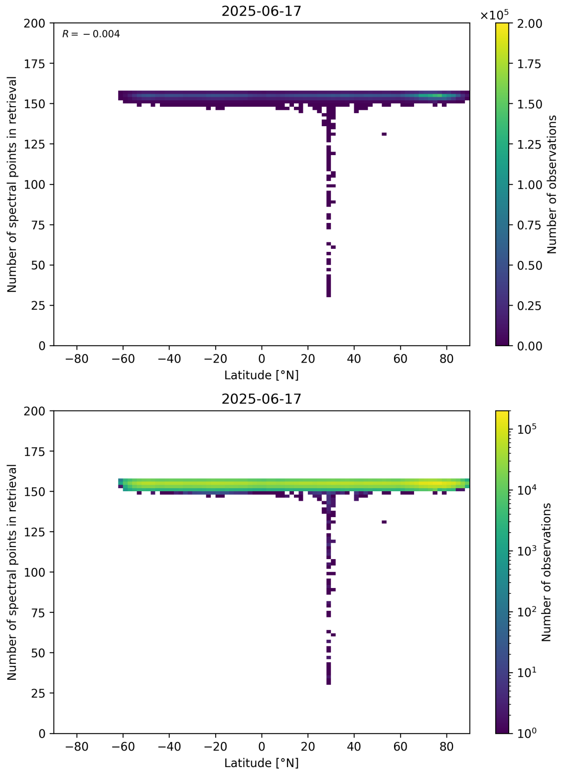
Figure 57: Scatter density plot of “Latitude” against “Number of spectral points in retrieval” for 2025-06-17 to 2025-06-18.
