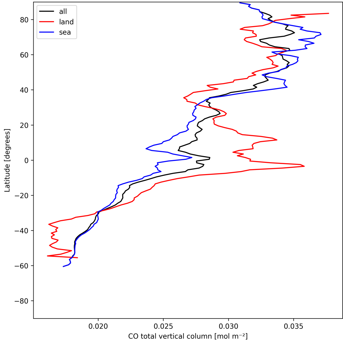
Figure 10: Zonal average of “CO total vertical column” for 2025-06-17 to 2025-06-18.
