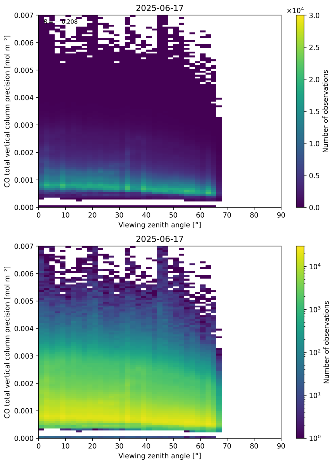
Figure 71: Scatter density plot of “Viewing zenith angle” against “CO total vertical column precision” for 2025-06-17 to 2025-06-18.
