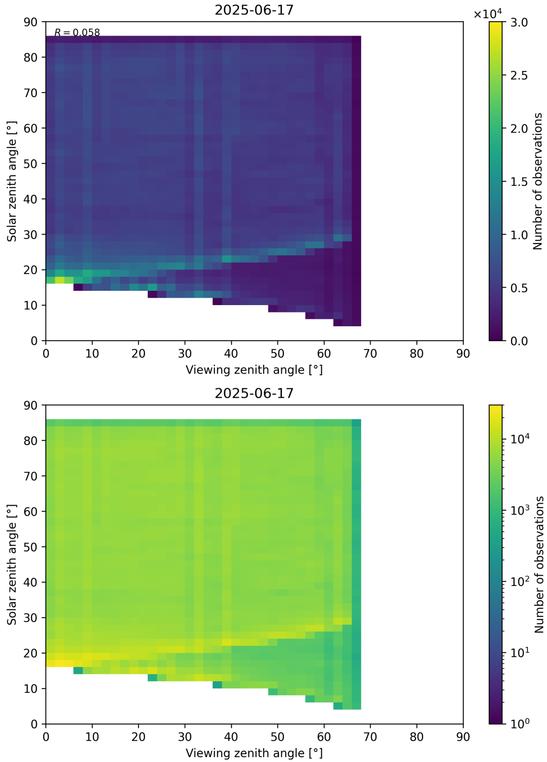
Figure 77: Scatter density plot of “Viewing zenith angle” against “Solar zenith angle” for 2025-06-17 to 2025-06-18.
