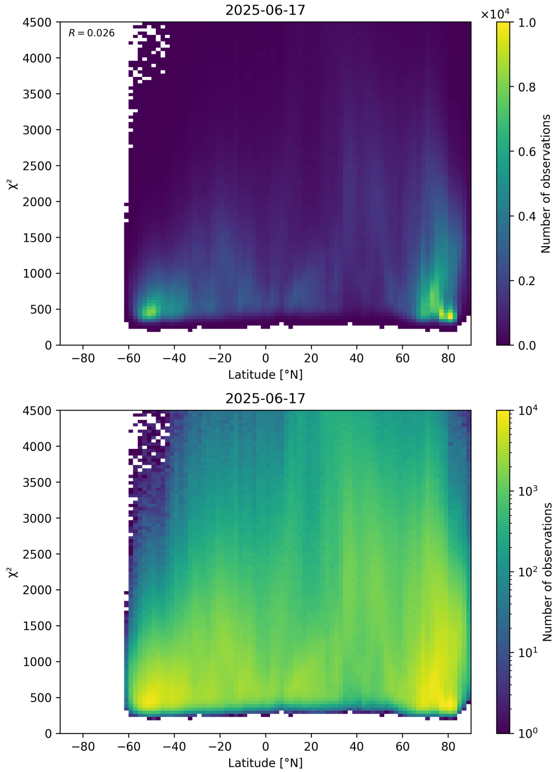
Figure 54: Scatter density plot of “Latitude” against “ \chi^2 ” for 2025-06-17 to 2025-06-18.
