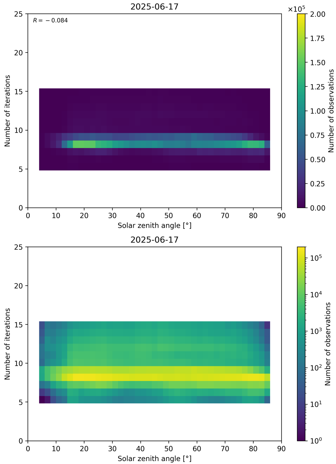
Figure 67: Scatter density plot of “Solar zenith angle” against “Number of iterations” for 2025-06-17 to 2025-06-18.
