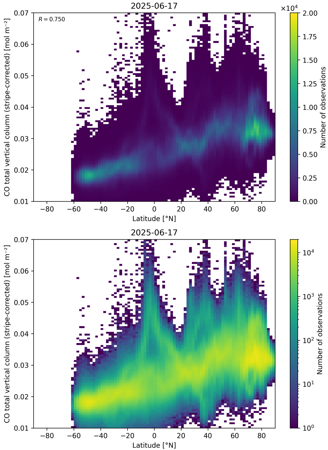
Figure 52: Scatter density plot of “Latitude” against “CO total vertical column (stripe-corrected)” for 2025-06-17 to 2025-06-18.
