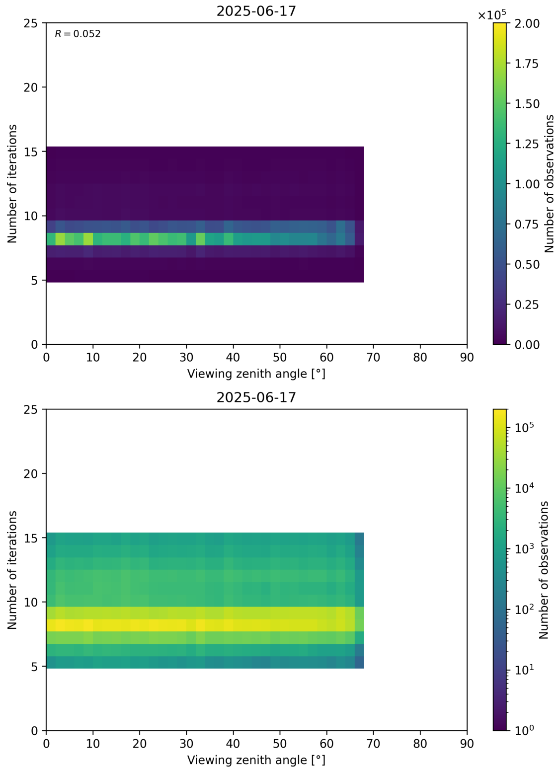
Figure 75: Scatter density plot of “Viewing zenith angle” against “Number of iterations” for 2025-06-17 to 2025-06-18.
