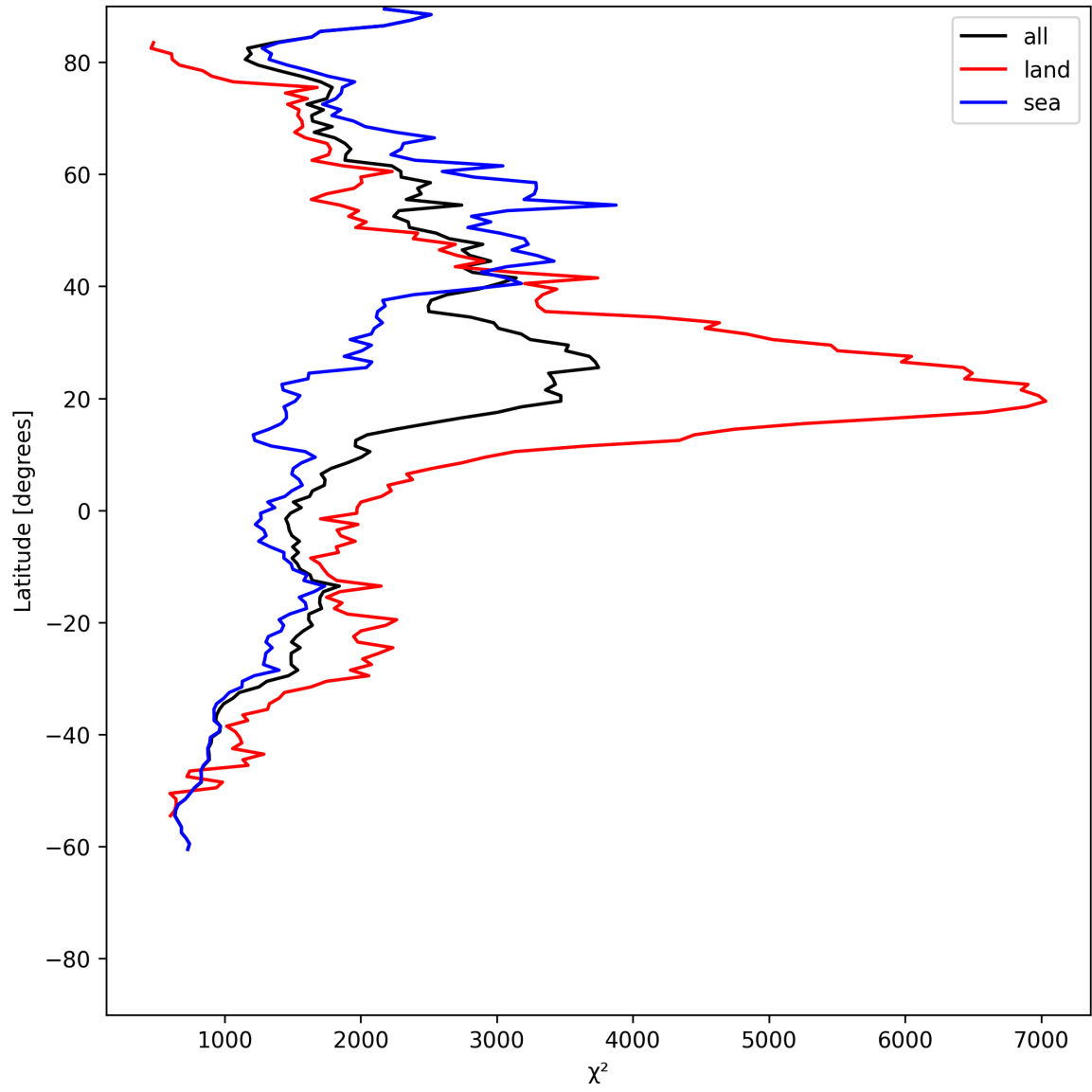
Figure 14: Zonal average of “ \chi^2 ” for 2025-06-18 to 2025-06-20.
