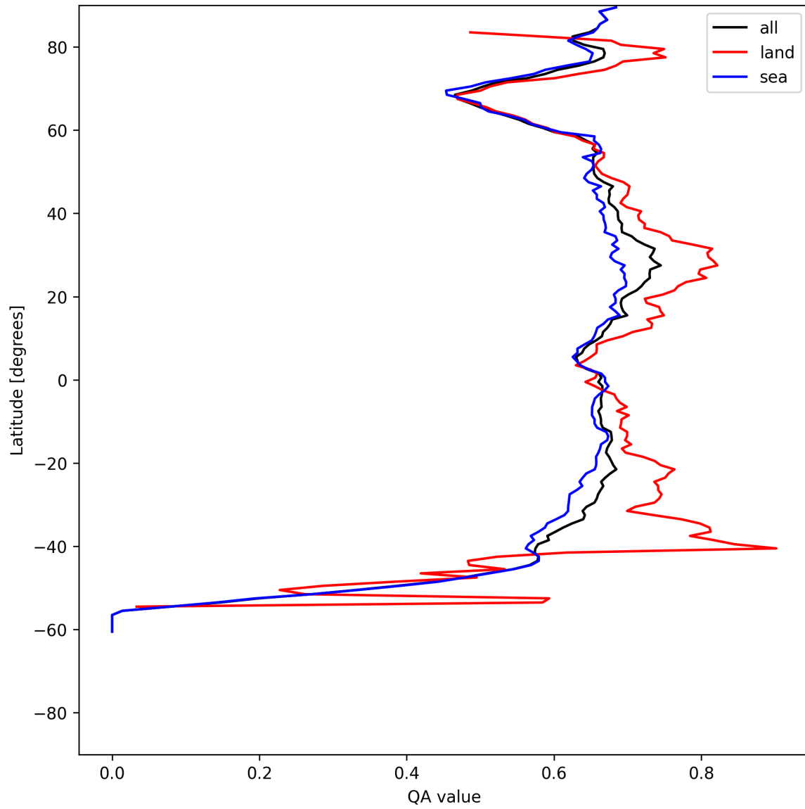
Figure 9: Zonal average of “QA value” for 2025-06-18 to 2025-06-20.
