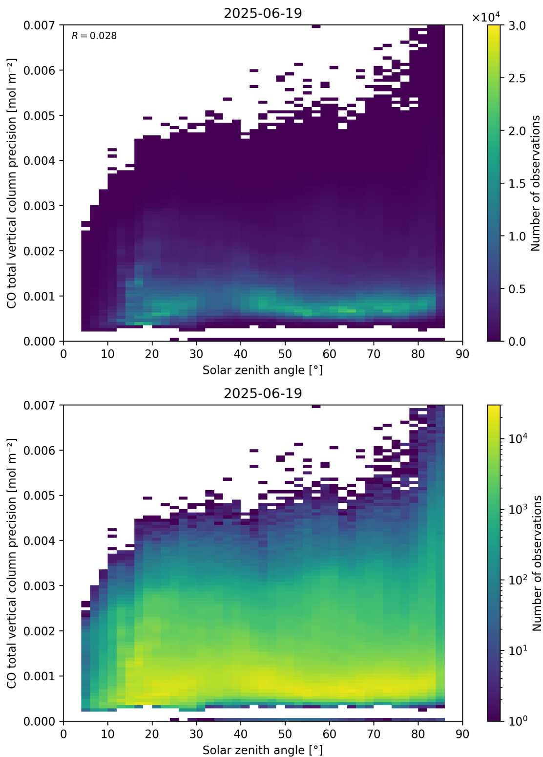
Figure 63: Scatter density plot of “Solar zenith angle” against “CO total vertical column precision” for 2025-06-18 to 2025-06-20.
