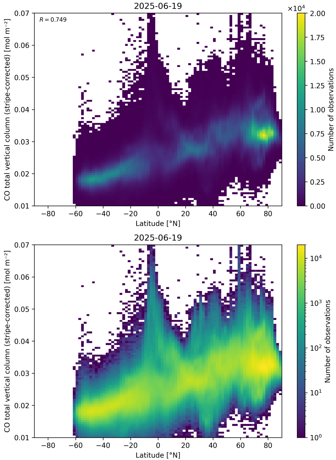
Figure 52: Scatter density plot of “Latitude” against “CO total vertical column (stripe-corrected)” for 2025-06-18 to 2025-06-20.
