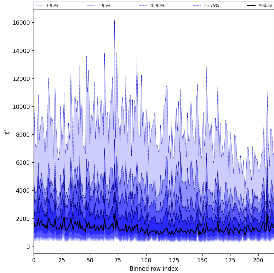
Figure 30: Along track statistics of “ \chi^2 ” for 2025-06-18 to 2025-06-20
