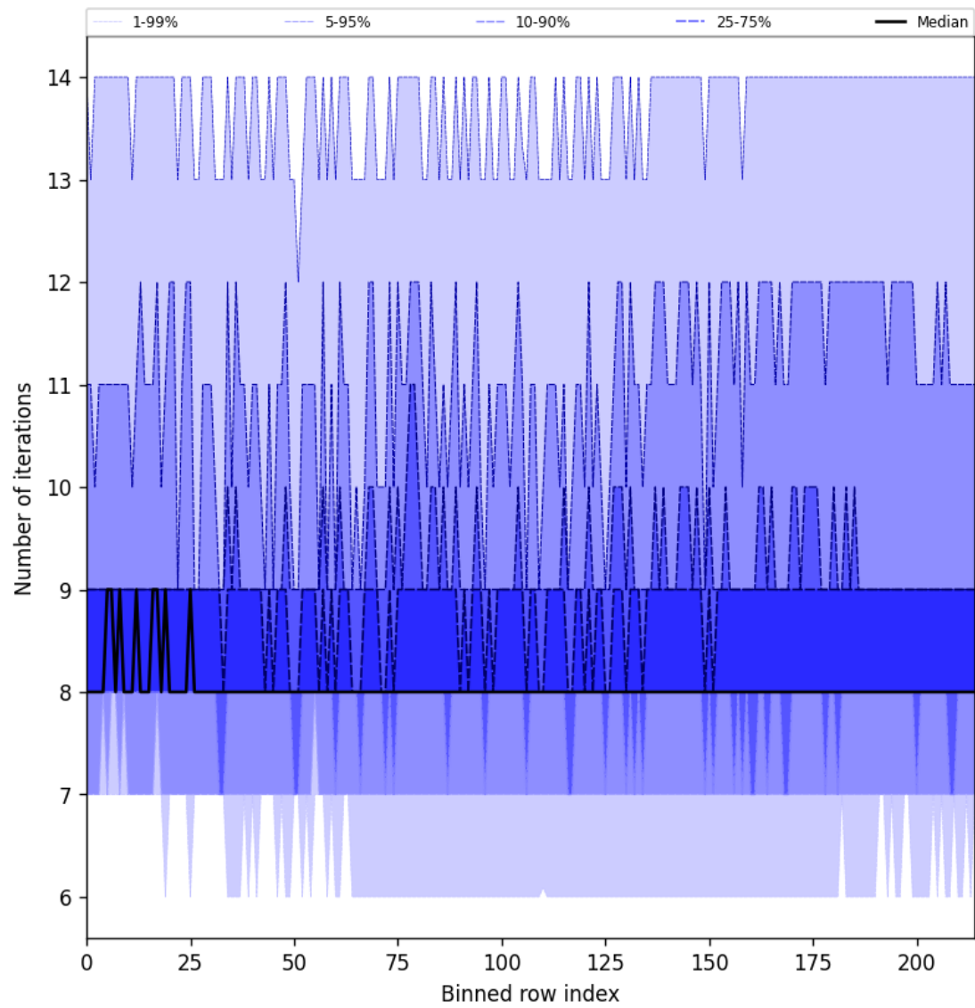
Figure 32: Along track statistics of “Number of iterations” for 2025-06-18 to 2025-06-20
