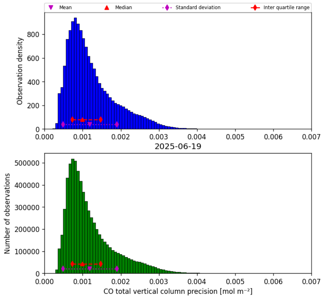
Figure 20: Histogram of “CO total vertical column precision” for 2025-06-18 to 2025-06-20
