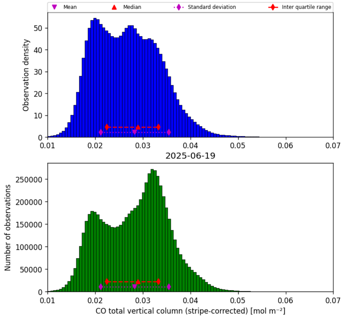
Figure 19: Histogram of “CO total vertical column (stripe-corrected)” for 2025-06-18 to 2025-06-20
