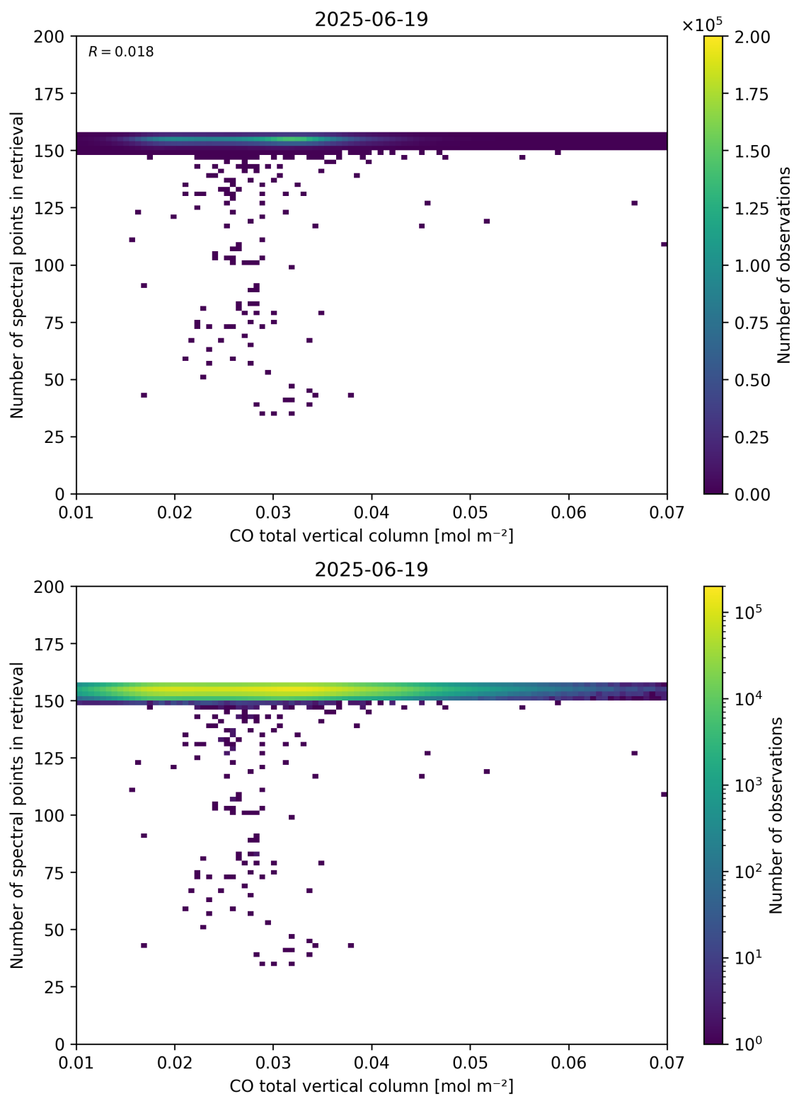
Figure 43: Scatter density plot of “CO total vertical column” against “Number of spectral points in retrieval” for 2025-06-18 to 2025-06-20.
