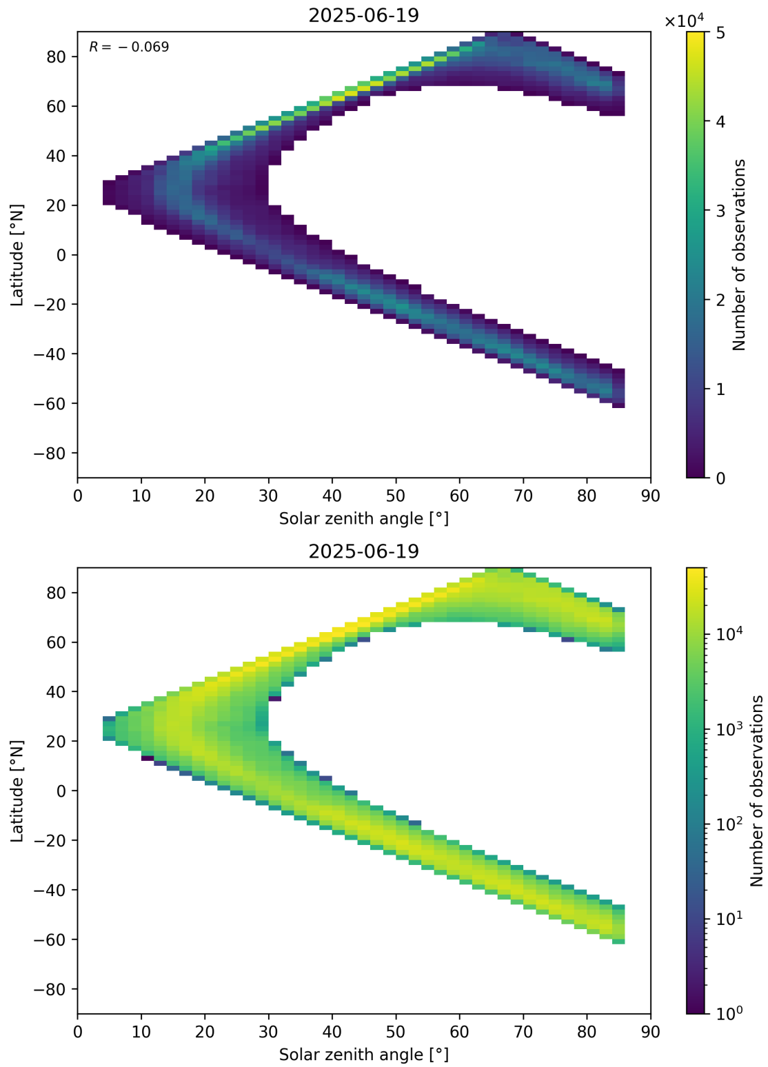
Figure 66: Scatter density plot of “Solar zenith angle” against “Latitude” for 2025-06-18 to 2025-06-20.
