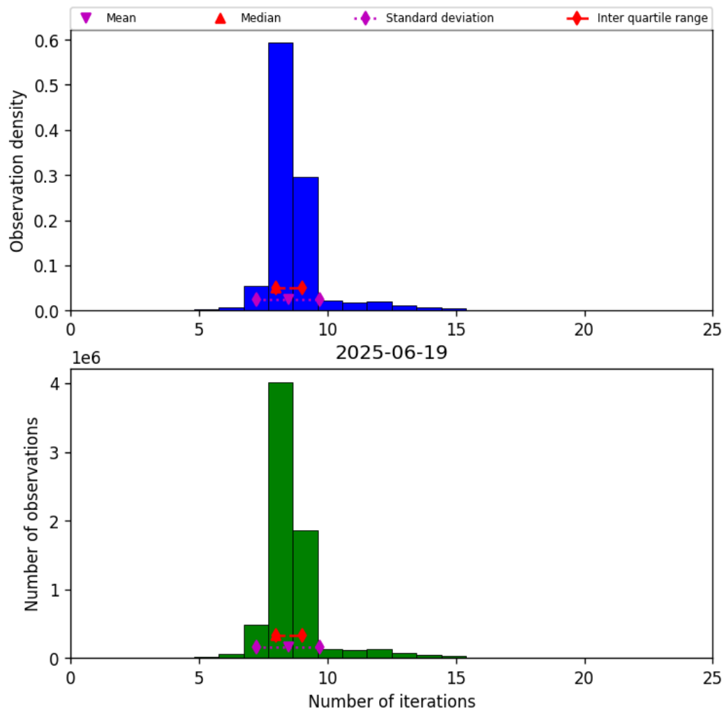
Figure 24: Histogram of “Number of iterations” for 2025-06-18 to 2025-06-20
