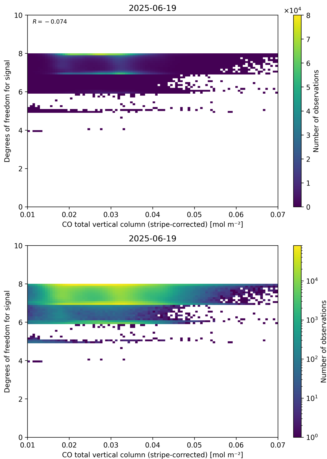
Figure 38: Scatter density plot of “CO total vertical column (stripe-corrected)” against “Degrees of freedom for signal” for 2025-06-18 to 2025-06-20.
