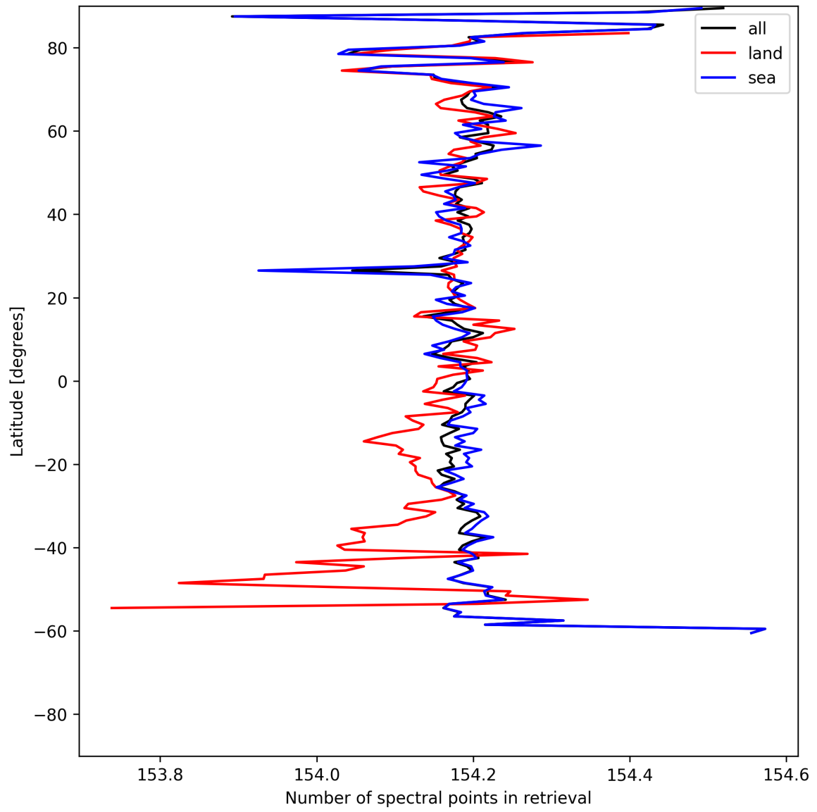
Figure 13: Zonal average of “Number of spectral points in retrieval” for 2025-06-18 to 2025-06-20.
