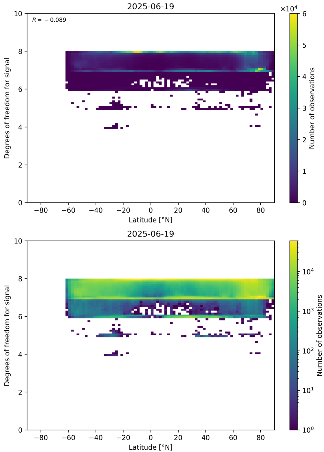
Figure 55: Scatter density plot of “Latitude” against “Degrees of freedom for signal” for 2025-06-18 to 2025-06-20.
