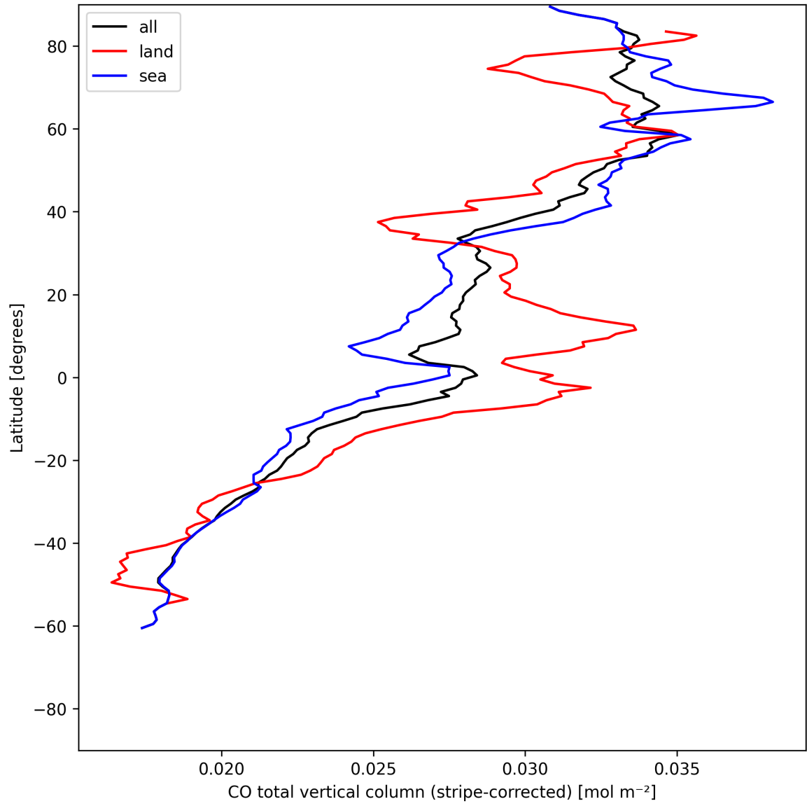
Figure 11: Zonal average of “CO total vertical column (stripe-corrected)” for 2025-06-18 to 2025-06-20.
