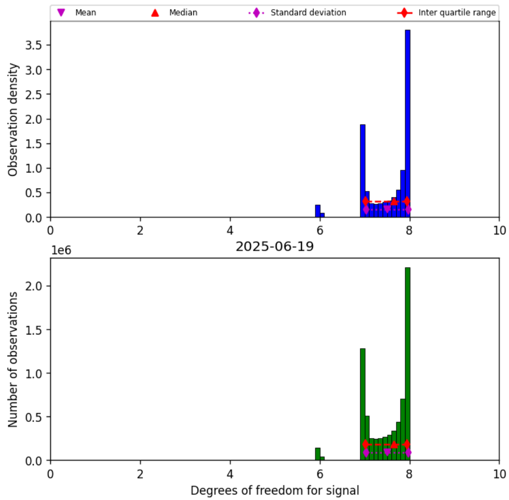
Figure 23: Histogram of “Degrees of freedom for signal” for 2025-06-18 to 2025-06-20
