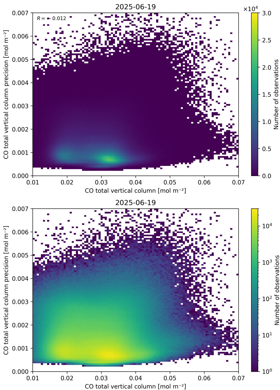
Figure 34: Scatter density plot of “CO total vertical column” against “CO total vertical column precision” for 2025-06-18 to 2025-06-20.
