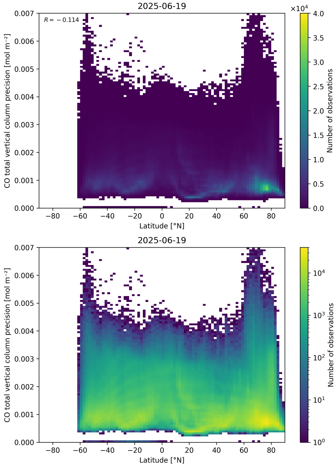
Figure 53: Scatter density plot of “Latitude” against “CO total vertical column precision” for 2025-06-18 to 2025-06-20.
