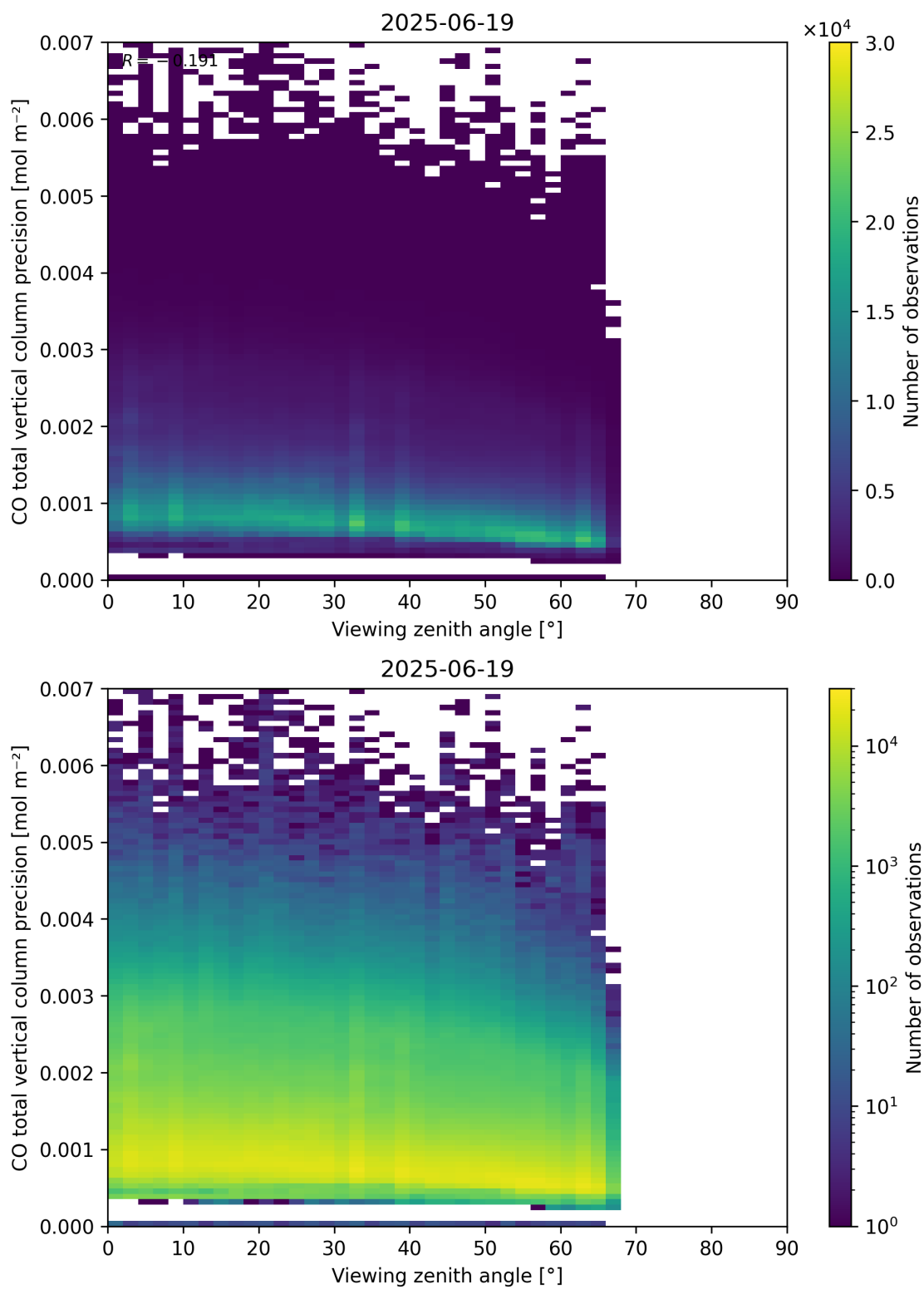
Figure 71: Scatter density plot of “Viewing zenith angle” against “CO total vertical column precision” for 2025-06-18 to 2025-06-20.
