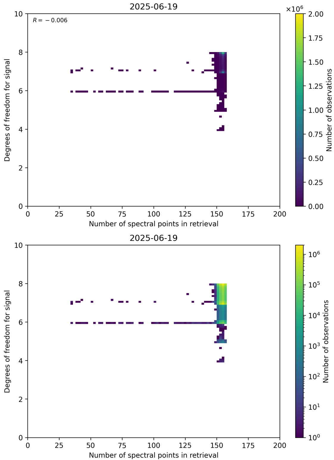
Figure 59: Scatter density plot of “Number of spectral points in retrieval” against “Degrees of freedom for signal” for 2025-06-18 to 2025-06-20.
