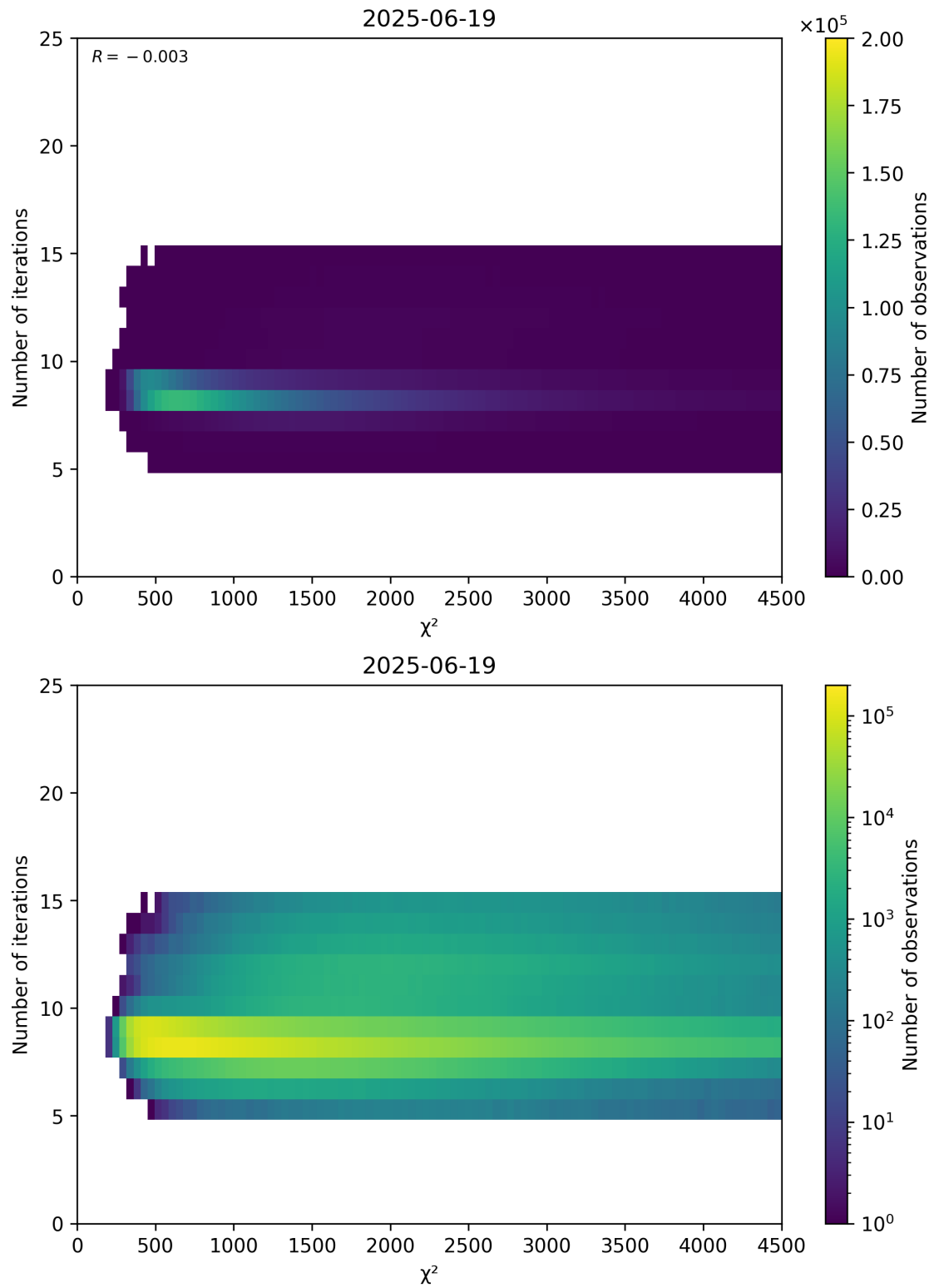
Figure 49: Scatter density plot of “ \chi^2 ” against “Number of iterations” for 2025-06-18 to 2025-06-20.
