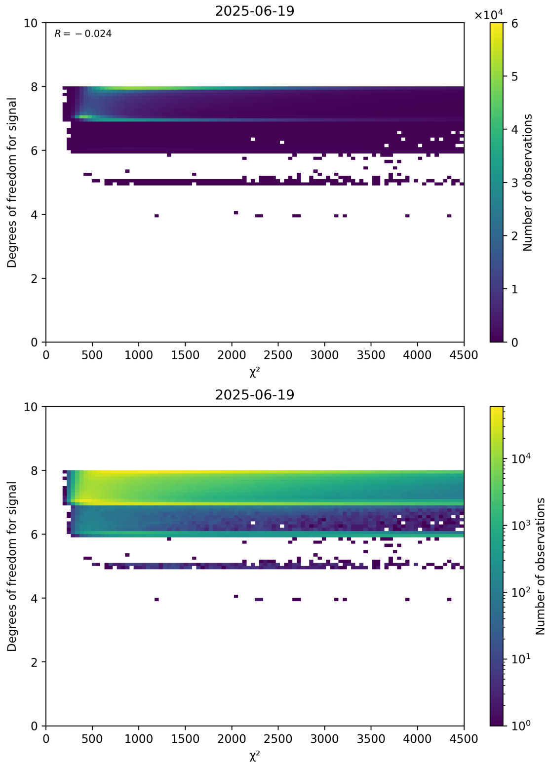
Figure 48: Scatter density plot of “ \chi^2 ” against “Degrees of freedom for signal” for 2025-06-18 to 2025-06-20.
