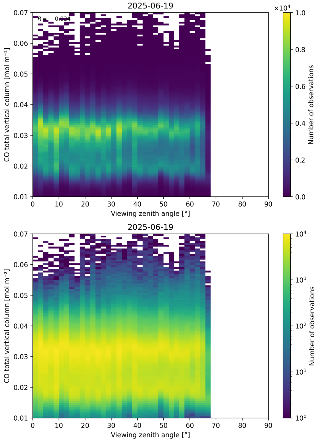
Figure 69: Scatter density plot of “Viewing zenith angle” against “CO total vertical column” for 2025-06-18 to 2025-06-20.
