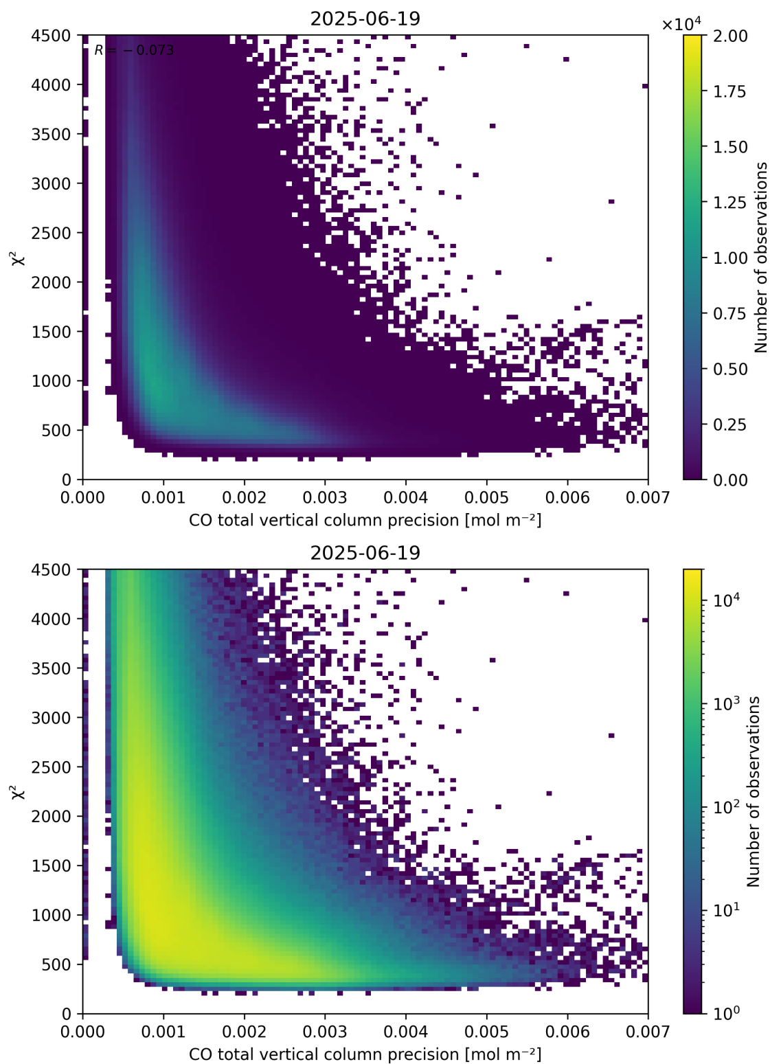
Figure 44: Scatter density plot of “CO total vertical column precision” against “ \chi^2 ” for 2025-06-18 to 2025-06-20.
