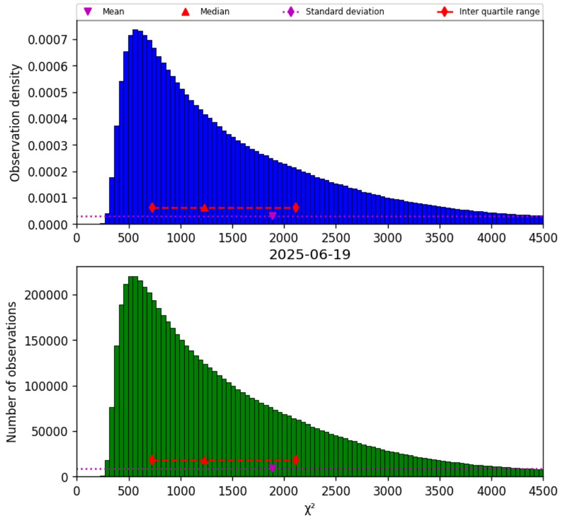
Figure 22: Histogram of “ \chi^2 ” for 2025-06-18 to 2025-06-20
