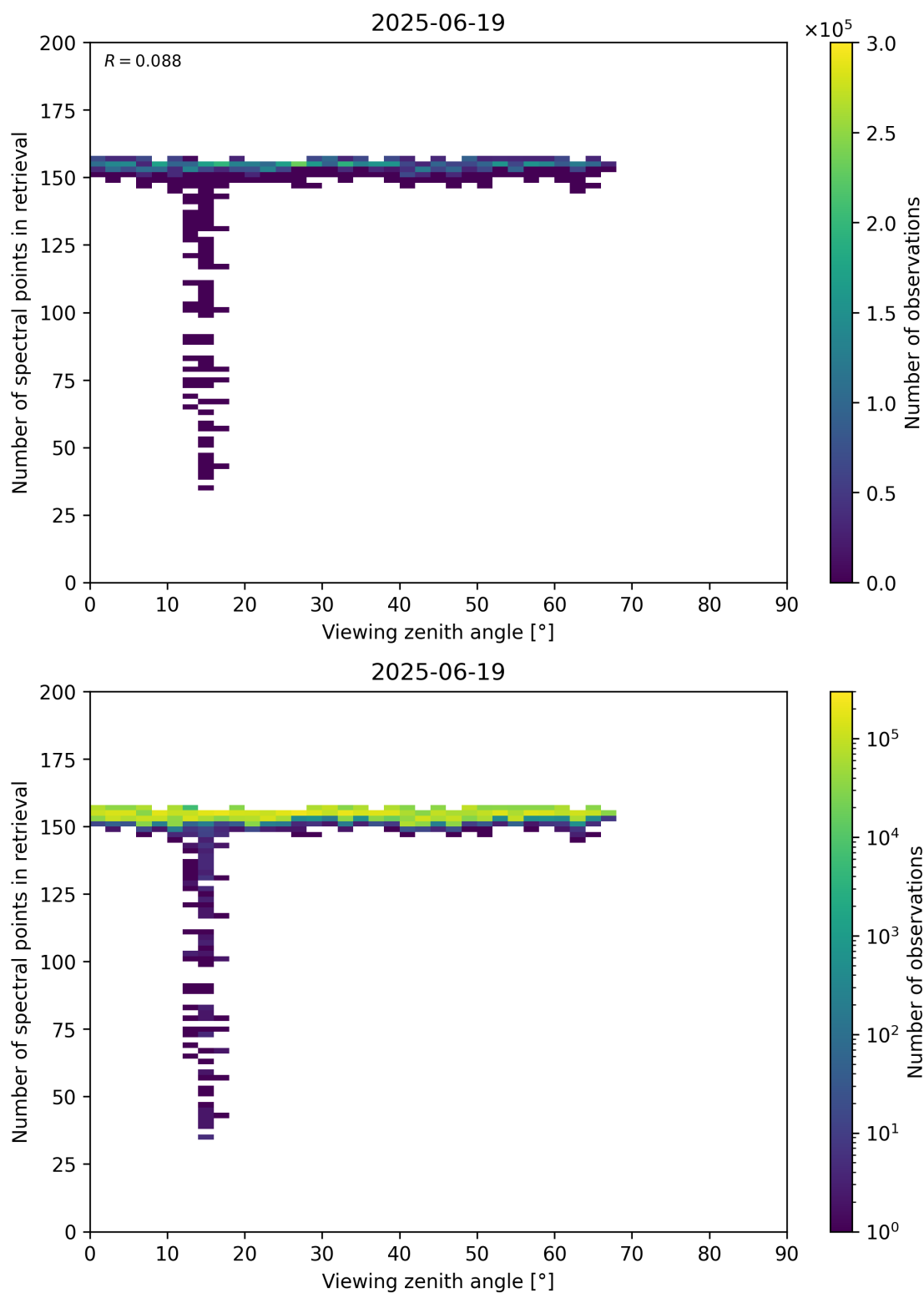
Figure 76: Scatter density plot of “Viewing zenith angle” against “Number of spectral points in retrieval” for 2025-06-18 to 2025-06-20.
