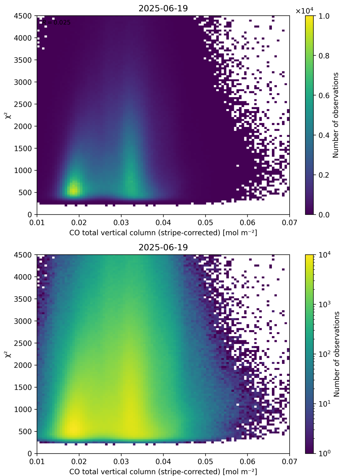
Figure 37: Scatter density plot of “CO total vertical column (stripe-corrected)” against “ \chi^2 ” for 2025-06-18 to 2025-06-20.
