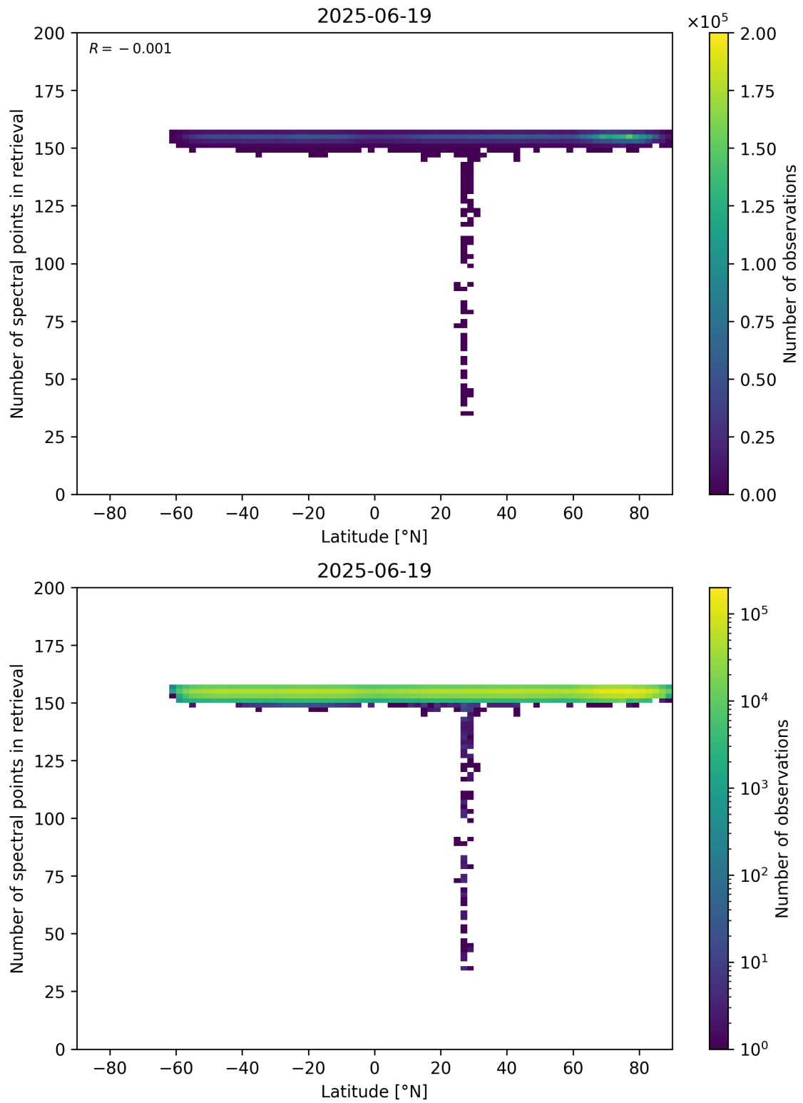
Figure 57: Scatter density plot of “Latitude” against “Number of spectral points in retrieval” for 2025-06-18 to 2025-06-20.
