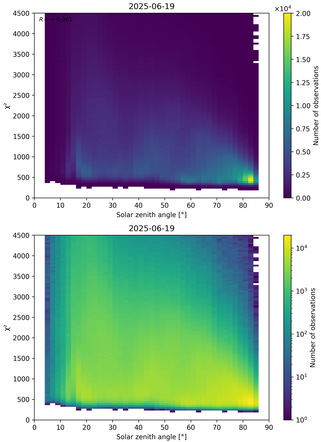
Figure 64: Scatter density plot of “Solar zenith angle” against “ \chi^2 ” for 2025-06-18 to 2025-06-20.
