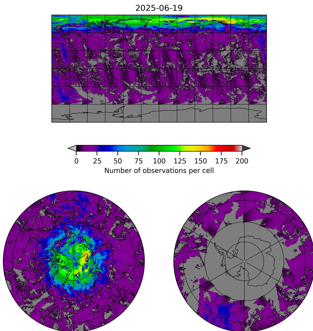
Figure 8: Map of the number of observations for 2025-06-18 to 2025-06-20
