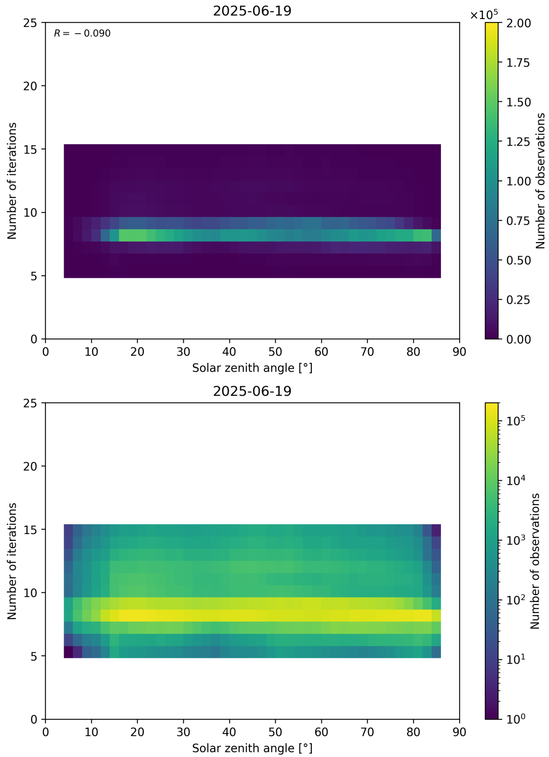
Figure 67: Scatter density plot of “Solar zenith angle” against “Number of iterations” for 2025-06-18 to 2025-06-20.
