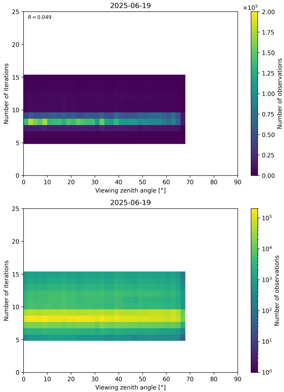
Figure 75: Scatter density plot of “Viewing zenith angle” against “Number of iterations” for 2025-06-18 to 2025-06-20.
