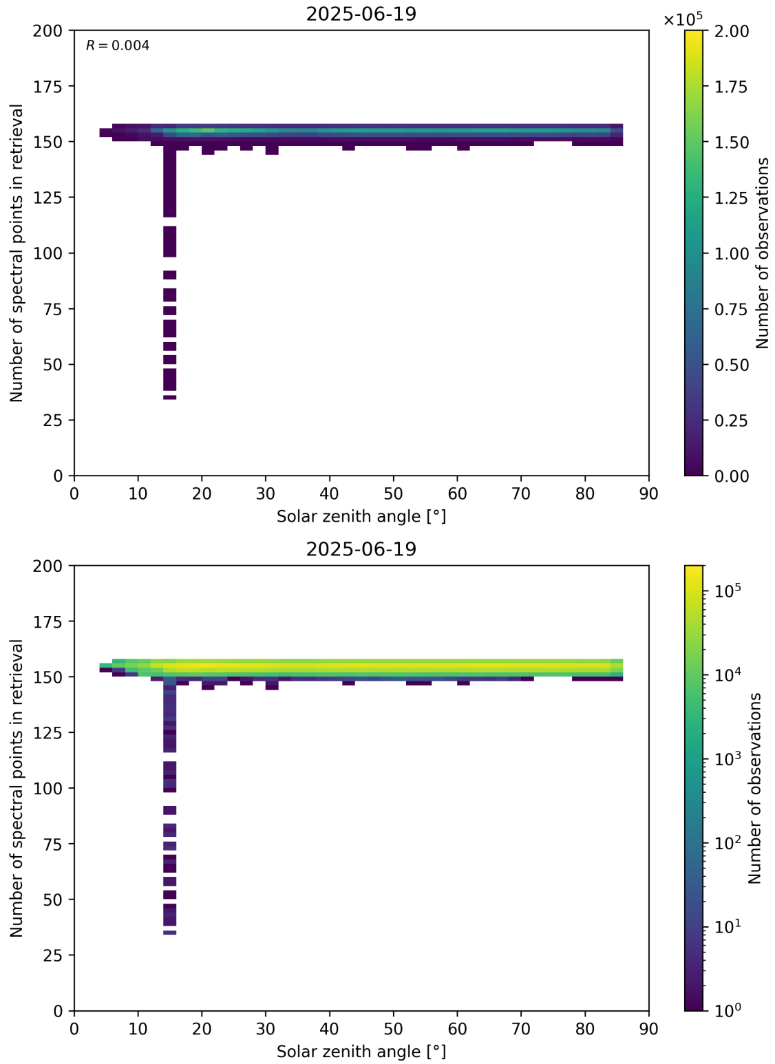
Figure 68: Scatter density plot of “Solar zenith angle” against “Number of spectral points in retrieval” for 2025-06-18 to 2025-06-20.
