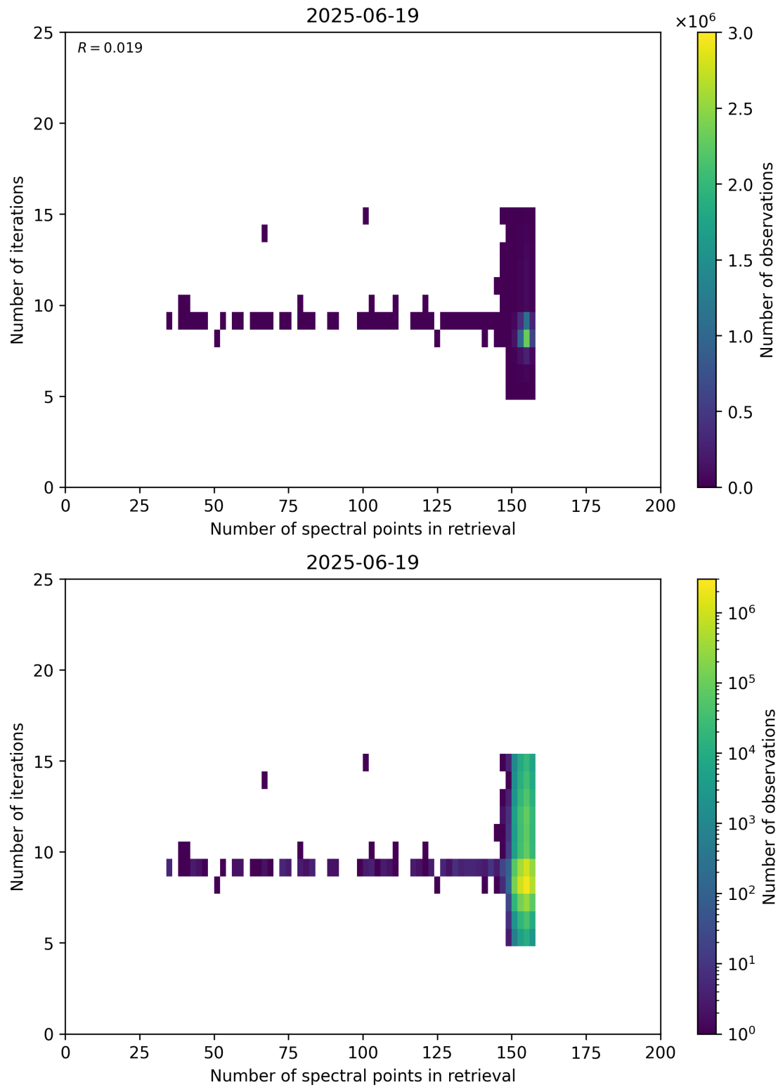
Figure 60: Scatter density plot of “Number of spectral points in retrieval” against “Number of iterations” for 2025-06-18 to 2025-06-20.
