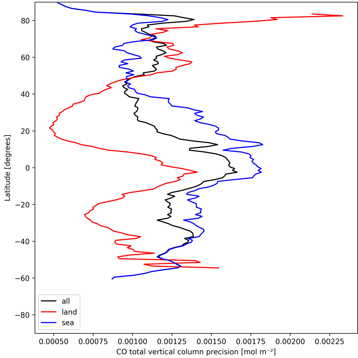
Figure 12: Zonal average of “CO total vertical column precision” for 2025-06-18 to 2025-06-20.
