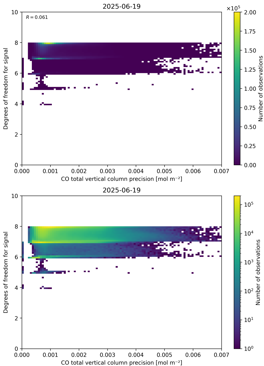
Figure 45: Scatter density plot of “CO total vertical column precision” against “Degrees of freedom for signal” for 2025-06-18 to 2025-06-20.
