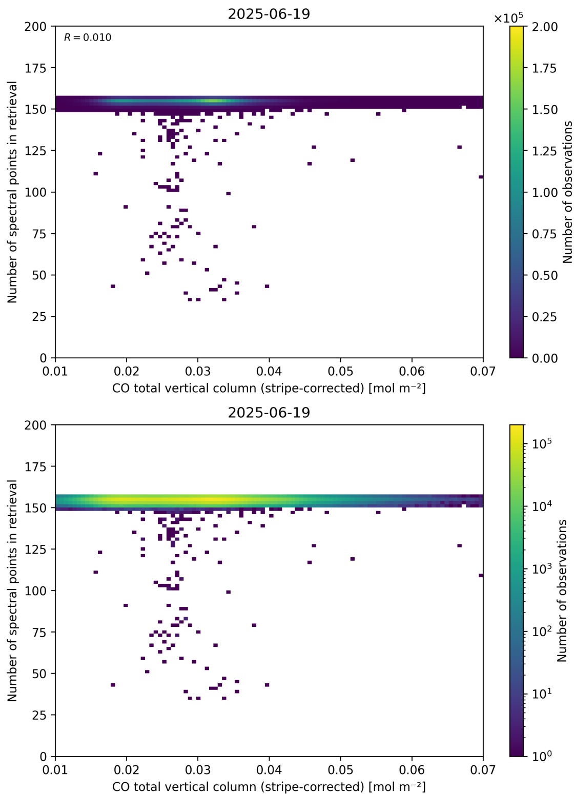
Figure 40: Scatter density plot of “CO total vertical column (stripe-corrected)” against “Number of spectral points in retrieval” for 2025-06-18 to 2025-06-20.
