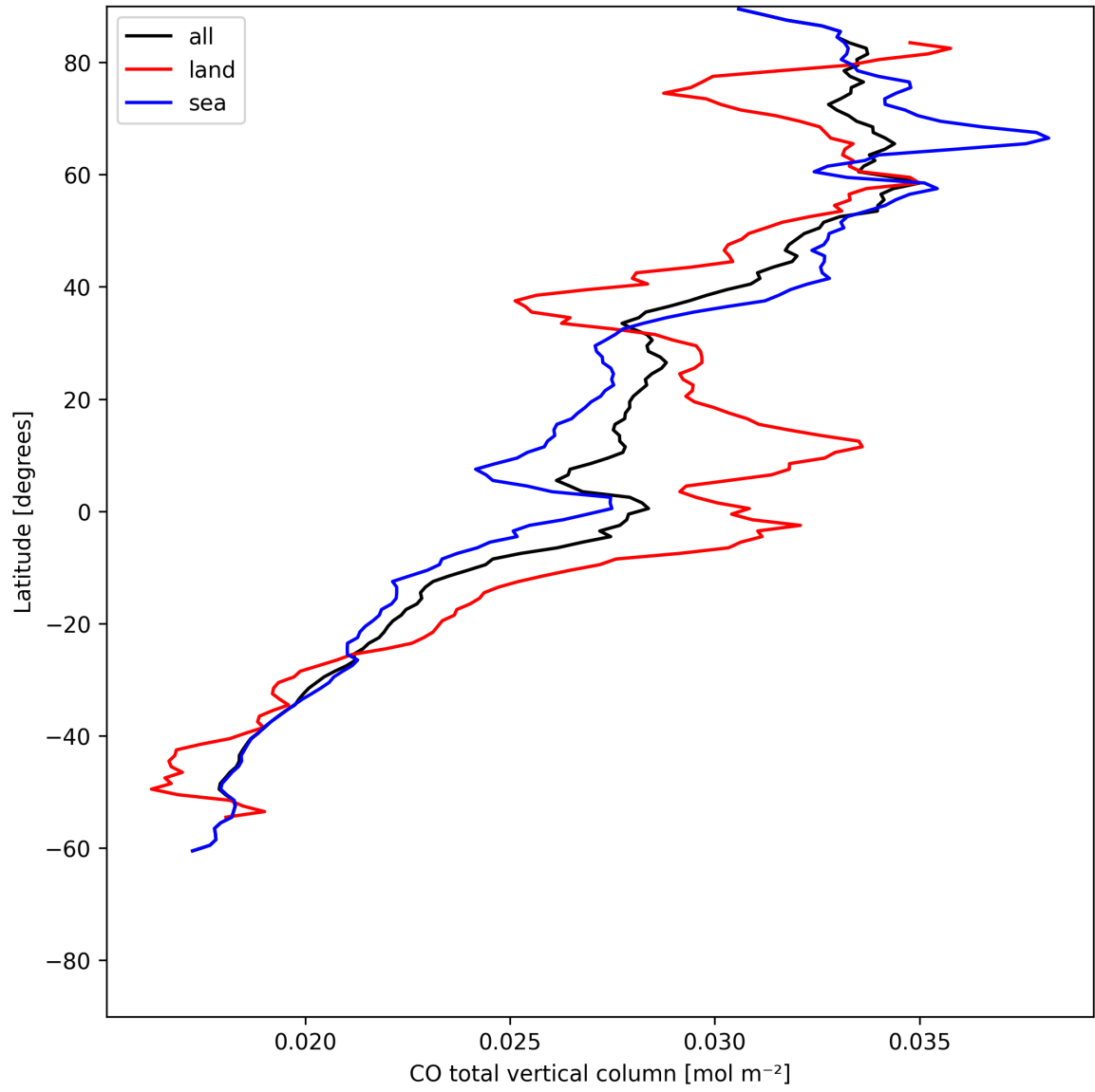
Figure 10: Zonal average of “CO total vertical column” for 2025-06-18 to 2025-06-20.
