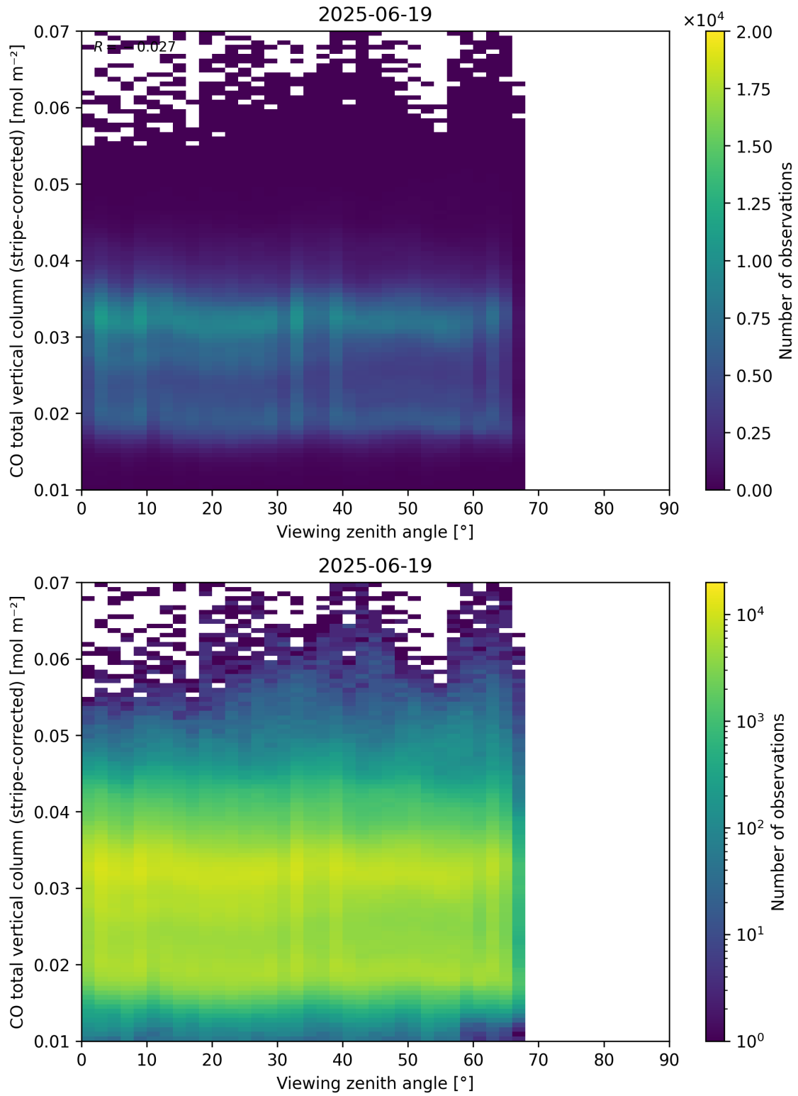
Figure 70: Scatter density plot of “Viewing zenith angle” against “CO total vertical column (stripe-corrected)” for 2025-06-18 to 2025-06-20.
