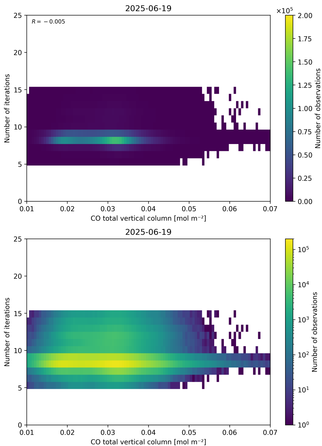
Figure 42: Scatter density plot of “CO total vertical column” against “Number of iterations” for 2025-06-18 to 2025-06-20.
