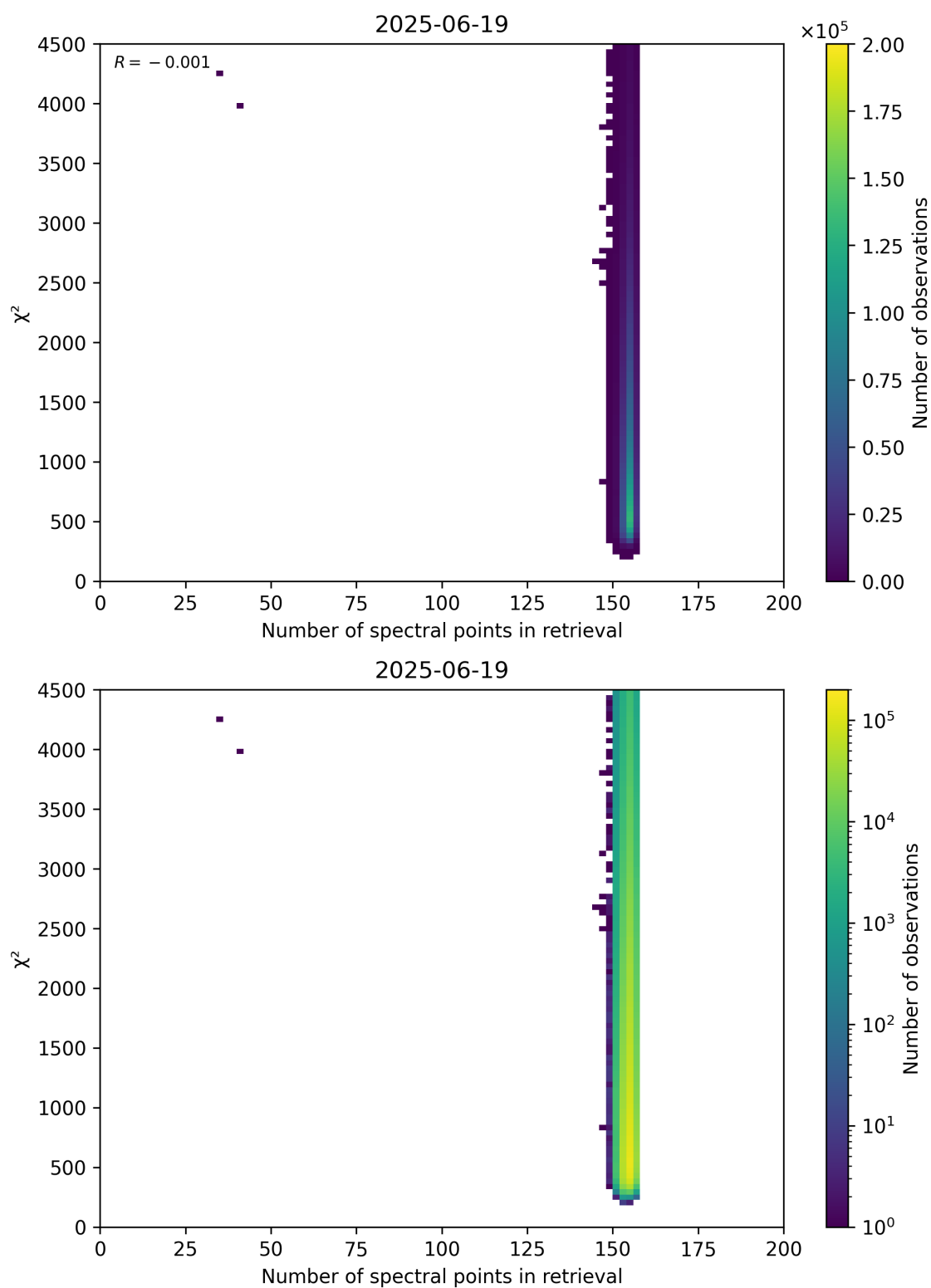
Figure 58: Scatter density plot of “Number of spectral points in retrieval” against “ \chi^2 ” for 2025-06-18 to 2025-06-20.
