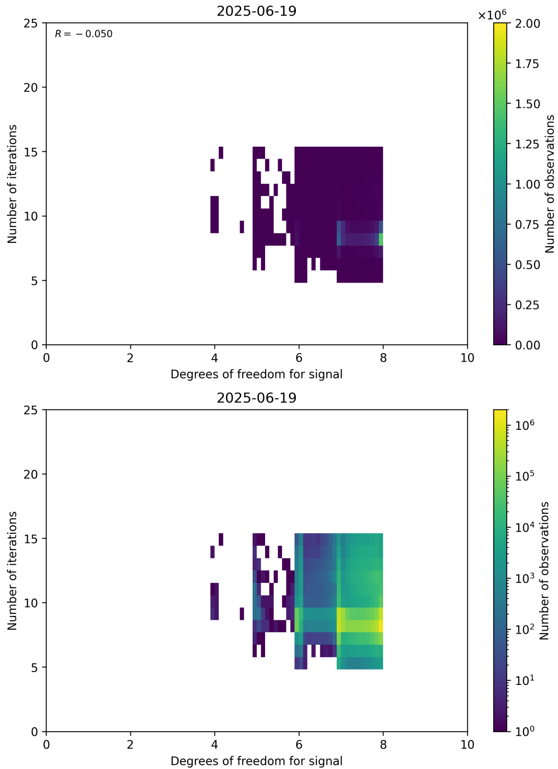
Figure 50: Scatter density plot of “Degrees of freedom for signal” against “Number of iterations” for 2025-06-18 to 2025-06-20.
