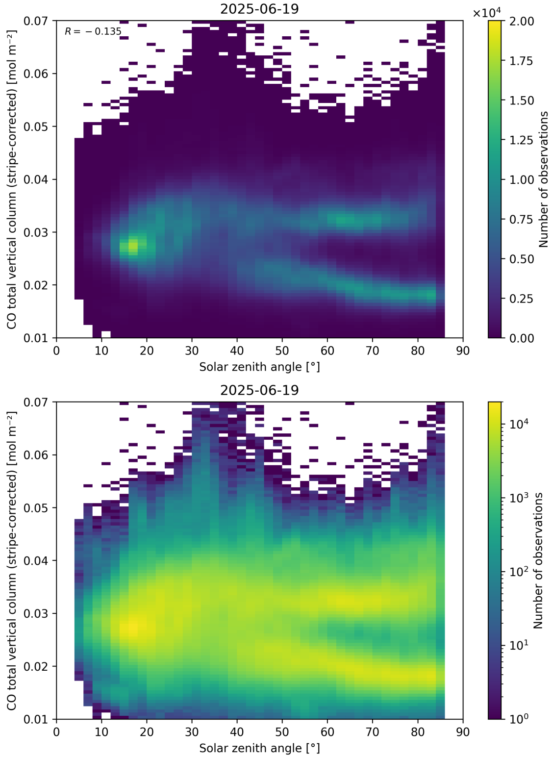
Figure 62: Scatter density plot of “Solar zenith angle” against “CO total vertical column (stripe-corrected)” for 2025-06-18 to 2025-06-20.
