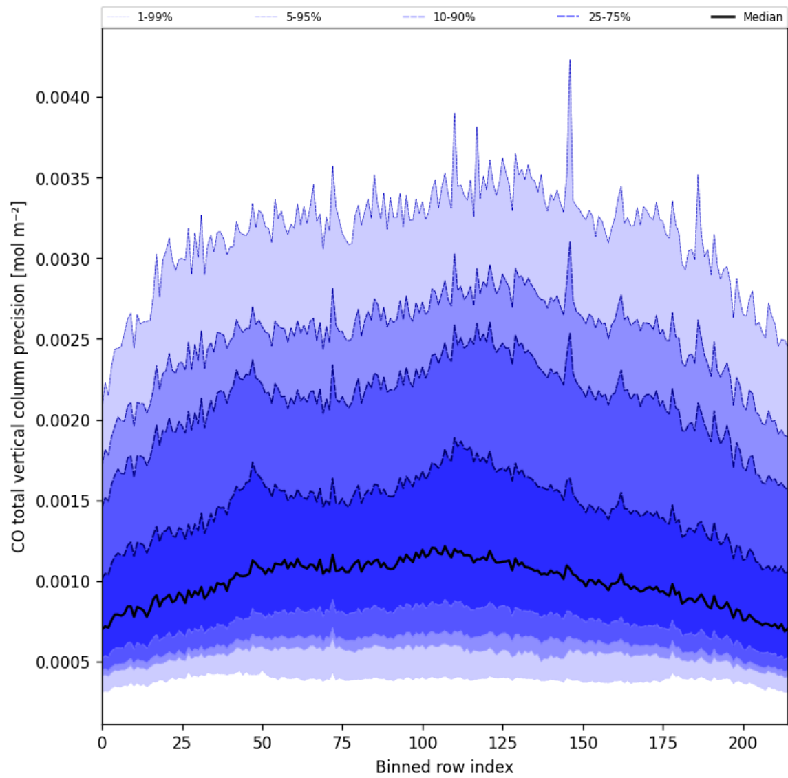
Figure 28: Along track statistics of “CO total vertical column precision” for 2025-06-18 to 2025-06-20
