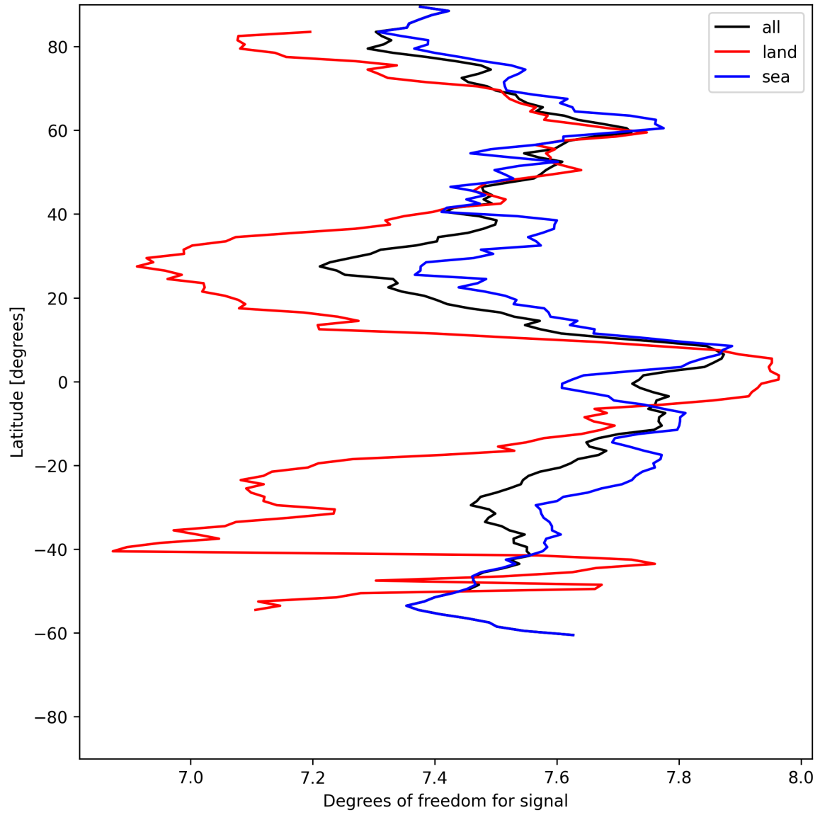
Figure 15: Zonal average of “Degrees of freedom for signal” for 2025-06-18 to 2025-06-20.
