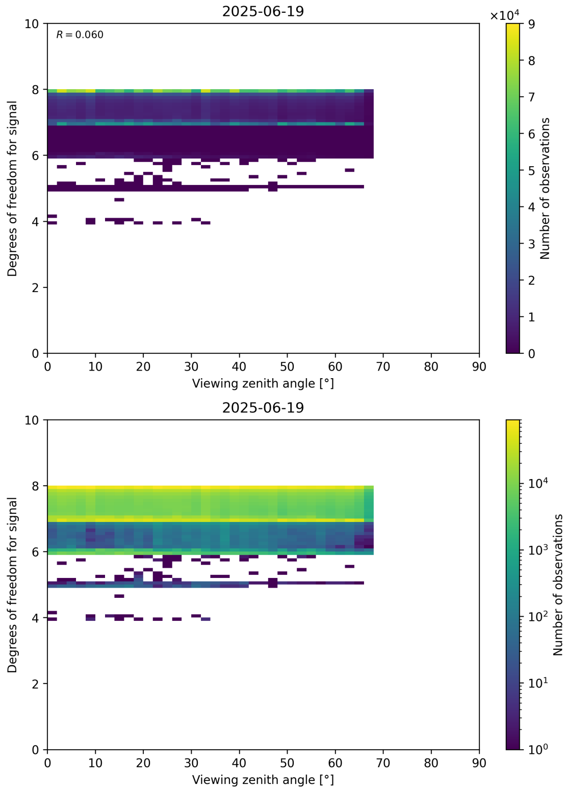
Figure 73: Scatter density plot of “Viewing zenith angle” against “Degrees of freedom for signal” for 2025-06-18 to 2025-06-20.
