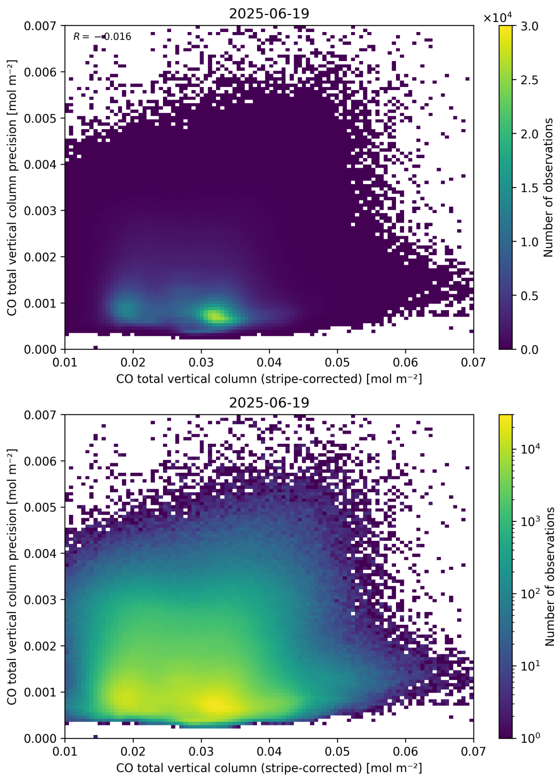
Figure 36: Scatter density plot of “CO total vertical column (stripe-corrected)” against “CO total vertical column precision” for 2025-06-18 to 2025-06-20.
