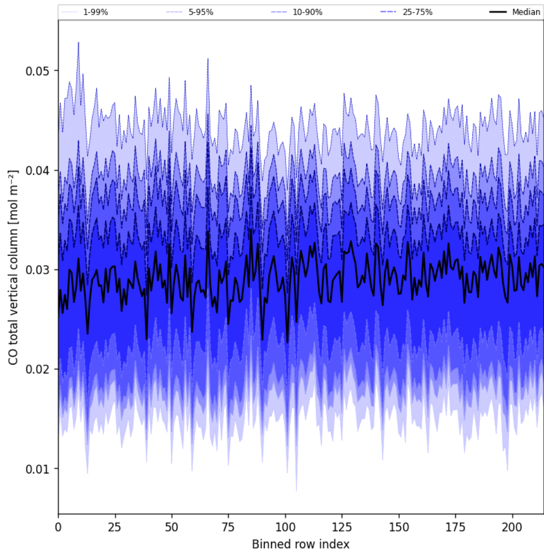
Figure 26: Along track statistics of “CO total vertical column” for 2025-06-18 to 2025-06-20
