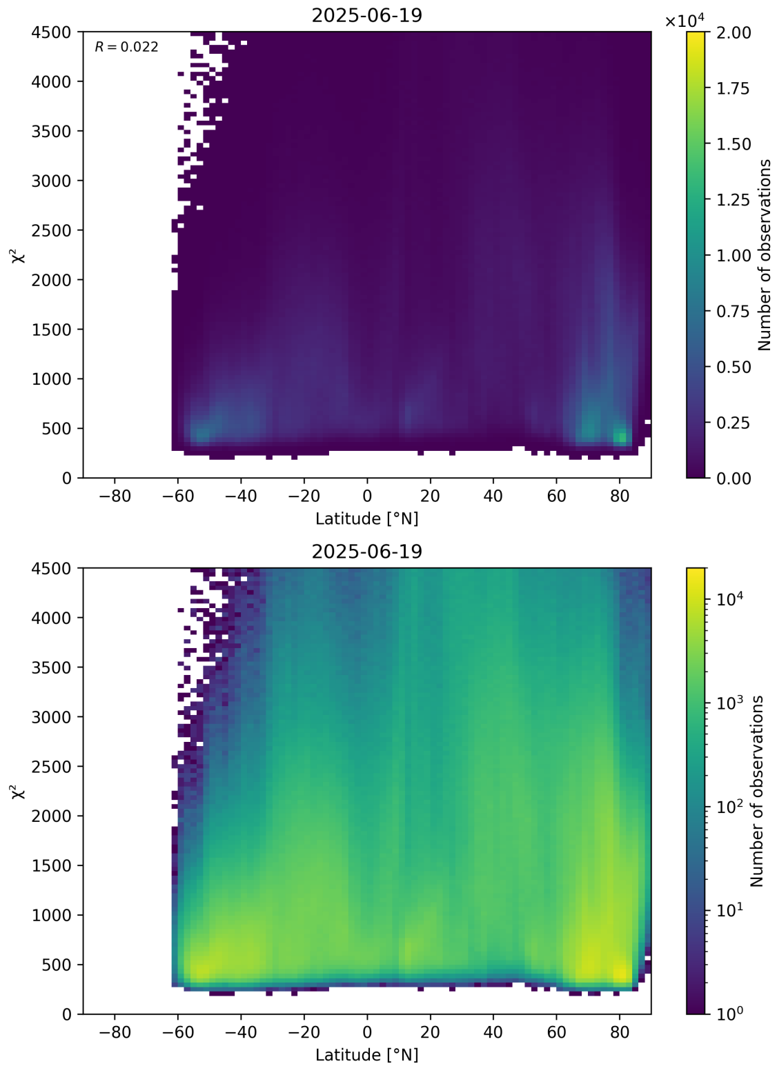
Figure 54: Scatter density plot of “Latitude” against “ \chi^2 ” for 2025-06-18 to 2025-06-20.
