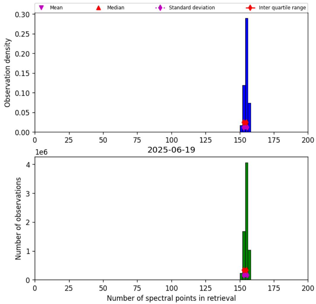
Figure 21: Histogram of “Number of spectral points in retrieval” for 2025-06-18 to 2025-06-20
