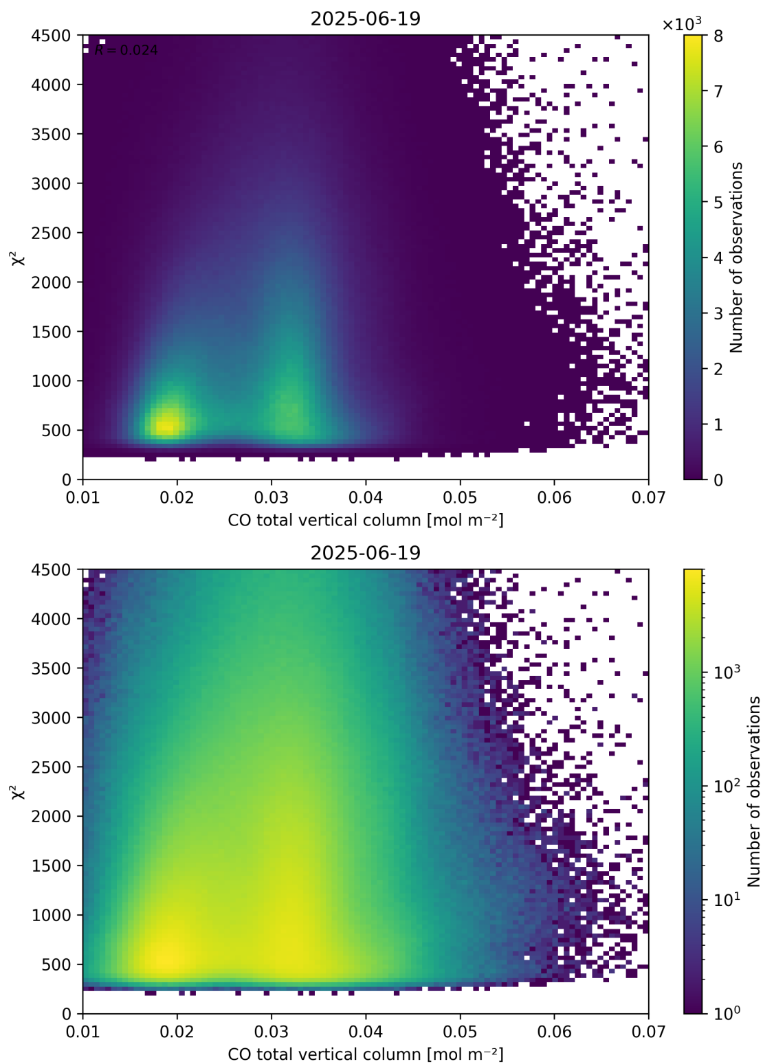
Figure 35: Scatter density plot of “CO total vertical column” against “ \chi^2 ” for 2025-06-18 to 2025-06-20.
