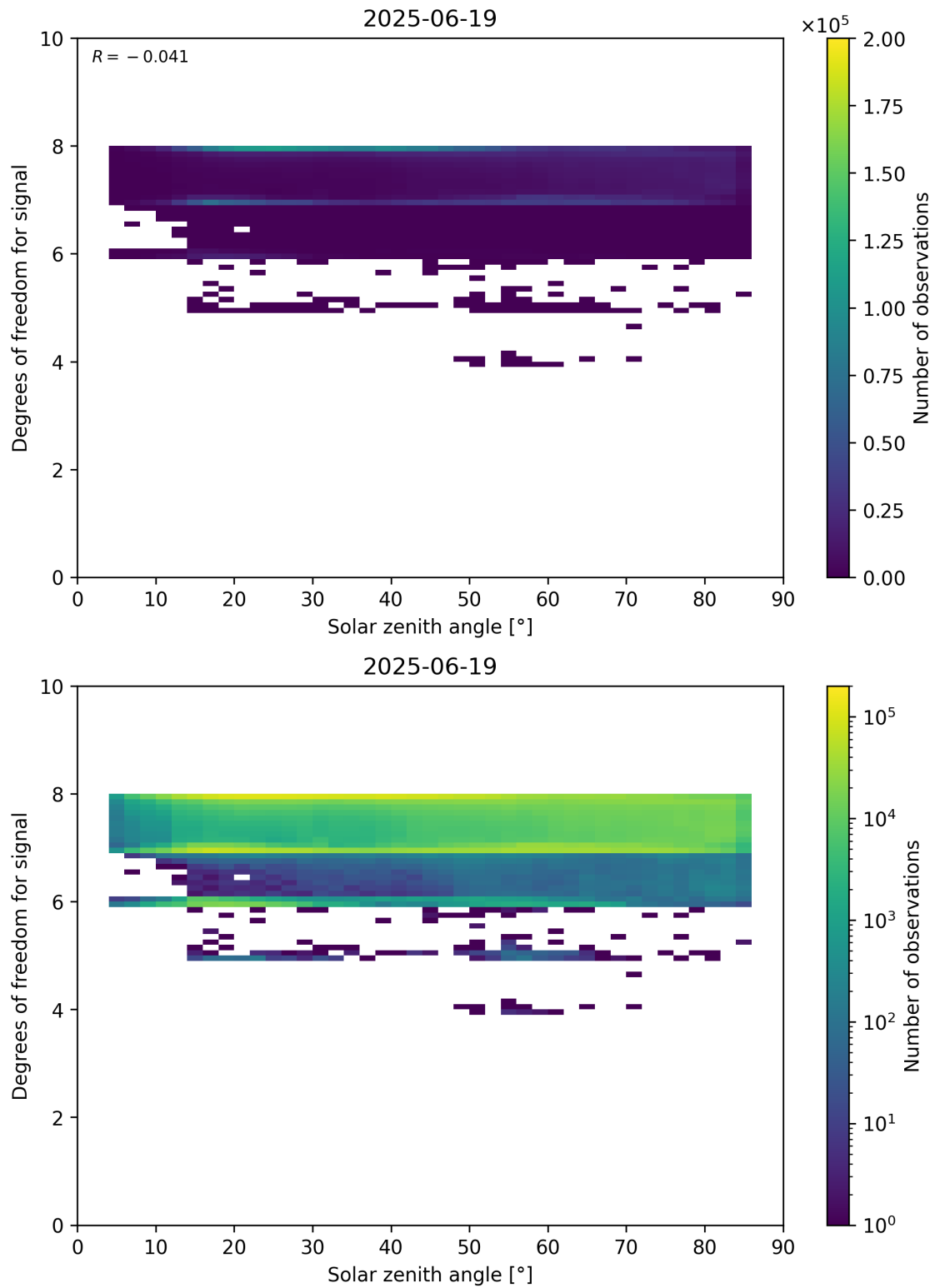
Figure 65: Scatter density plot of “Solar zenith angle” against “Degrees of freedom for signal” for 2025-06-18 to 2025-06-20.
