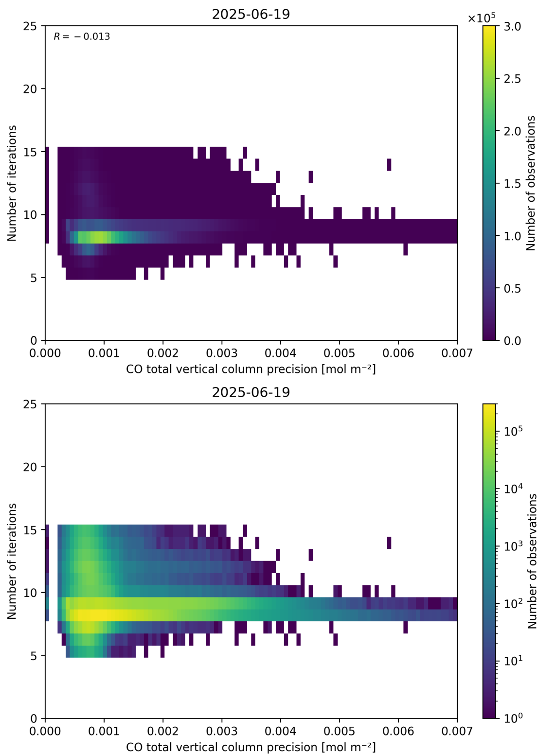
Figure 46: Scatter density plot of “CO total vertical column precision” against “Number of iterations” for 2025-06-18 to 2025-06-20.
