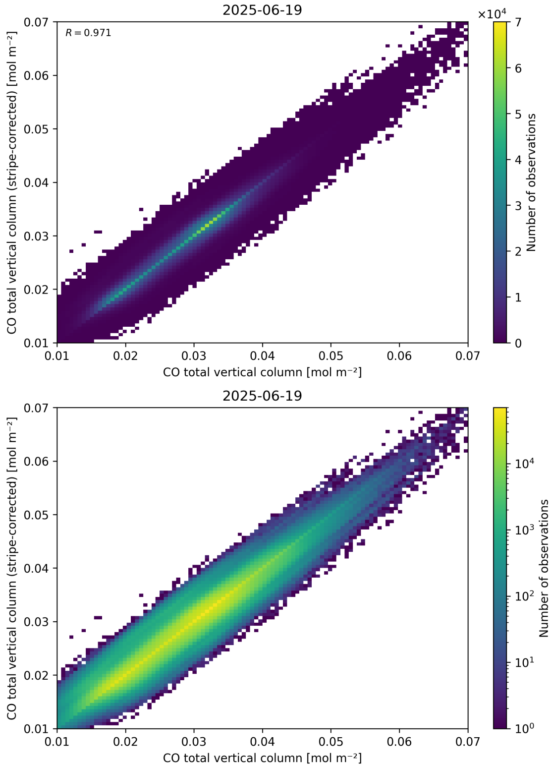
Figure 33: Scatter density plot of “CO total vertical column” against “CO total vertical column (stripe-corrected)” for 2025-06-18 to 2025-06-20.
