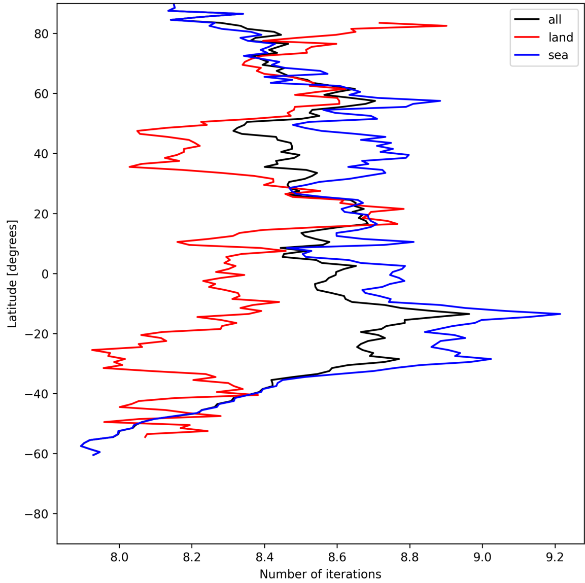
Figure 16: Zonal average of “Number of iterations” for 2025-06-18 to 2025-06-20.
