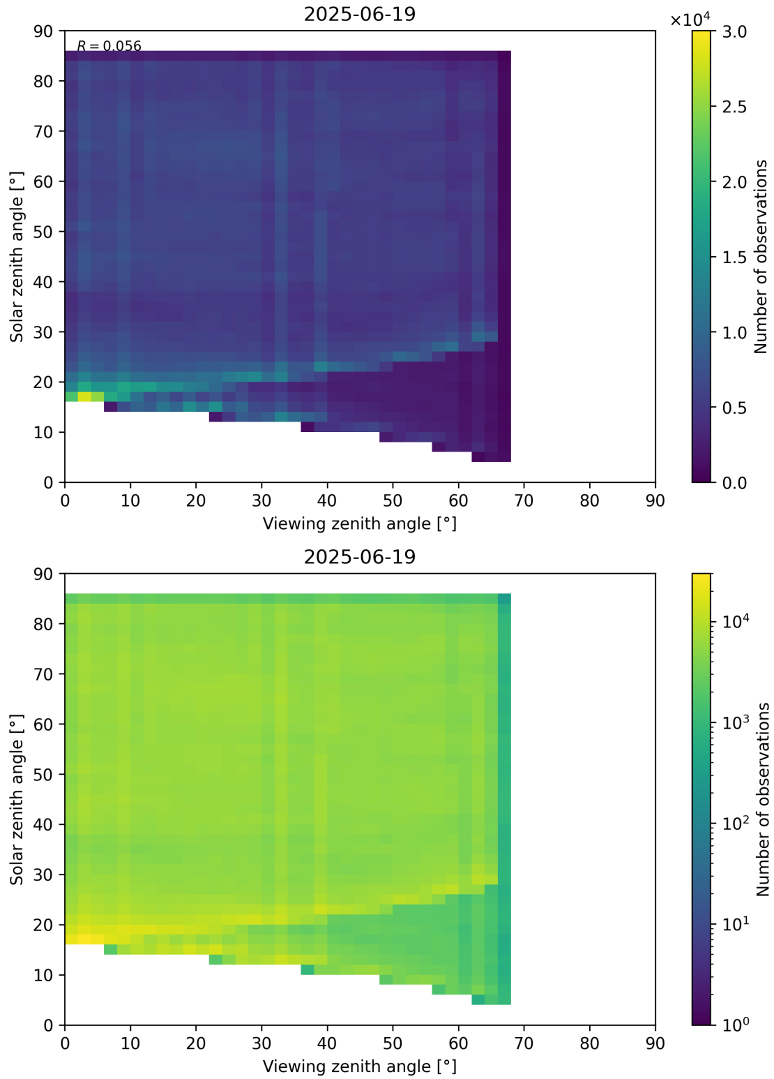
Figure 77: Scatter density plot of “Viewing zenith angle” against “Solar zenith angle” for 2025-06-18 to 2025-06-20.
