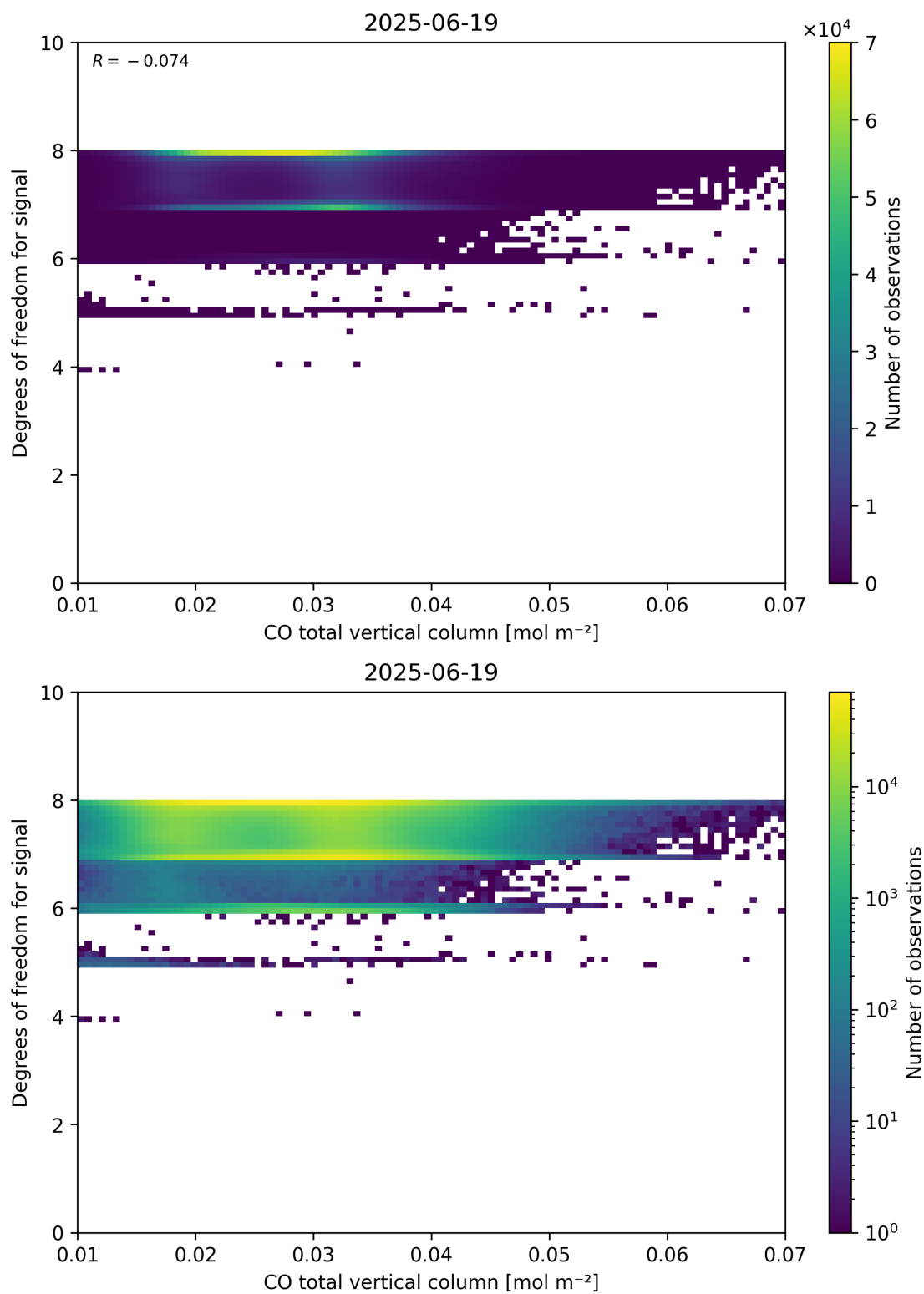
Figure 41: Scatter density plot of “CO total vertical column” against “Degrees of freedom for signal” for 2025-06-18 to 2025-06-20.
