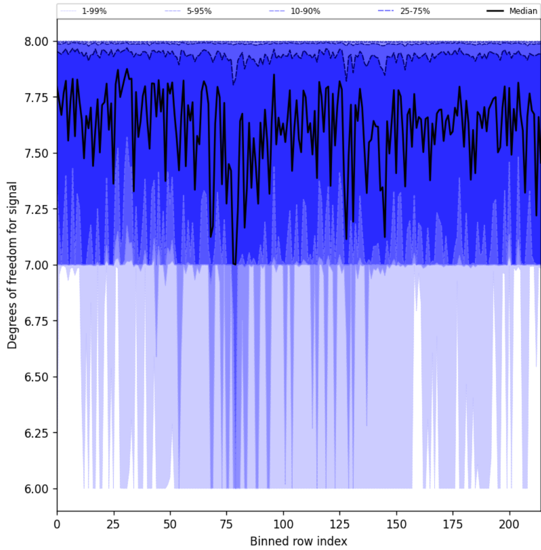
Figure 31: Along track statistics of “Degrees of freedom for signal” for 2025-06-18 to 2025-06-20
