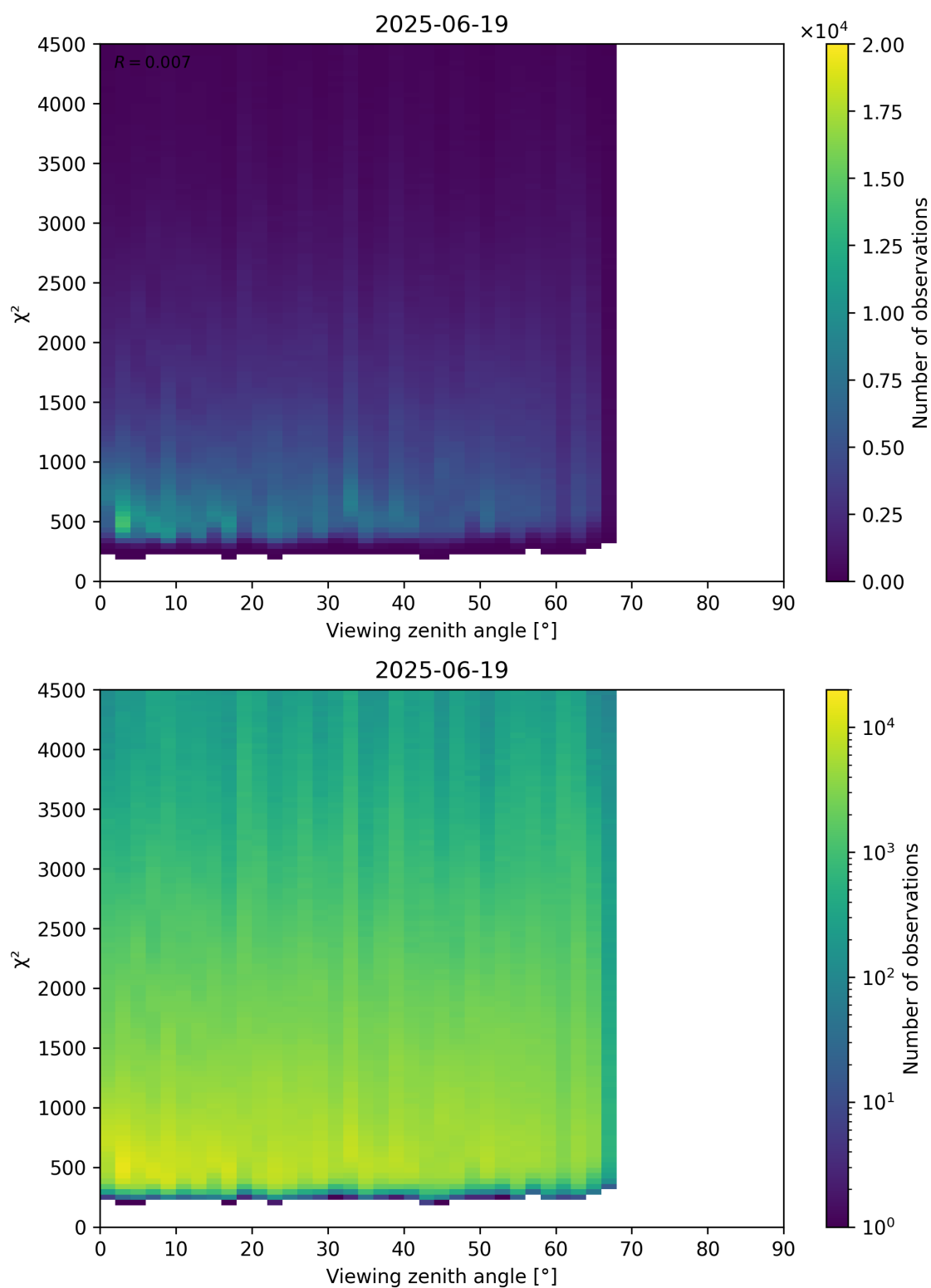
Figure 72: Scatter density plot of “Viewing zenith angle” against “ \chi^2 ” for 2025-06-18 to 2025-06-20.
