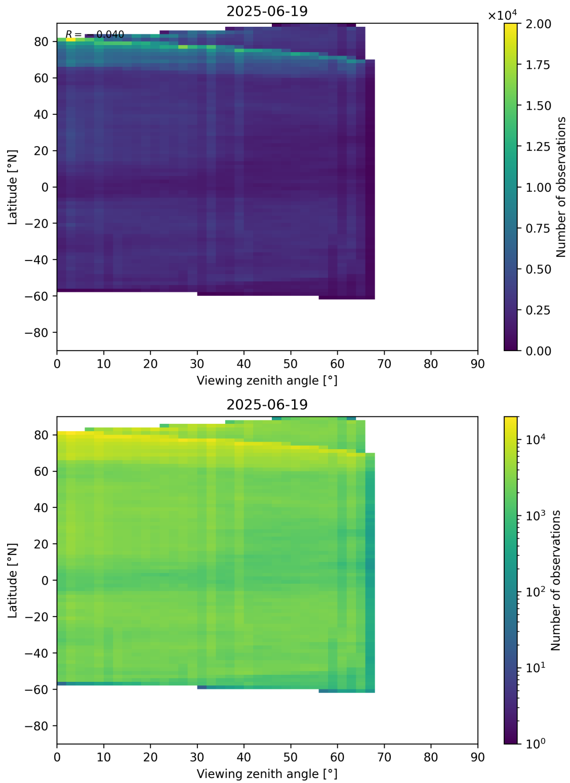
Figure 74: Scatter density plot of “Viewing zenith angle” against “Latitude” for 2025-06-18 to 2025-06-20.
