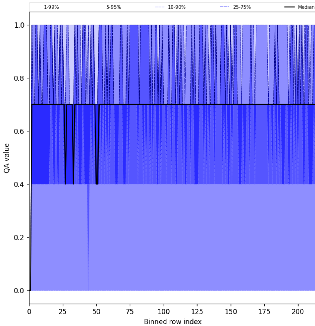
Figure 25: Along track statistics of “QA value” for 2025-06-18 to 2025-06-20
