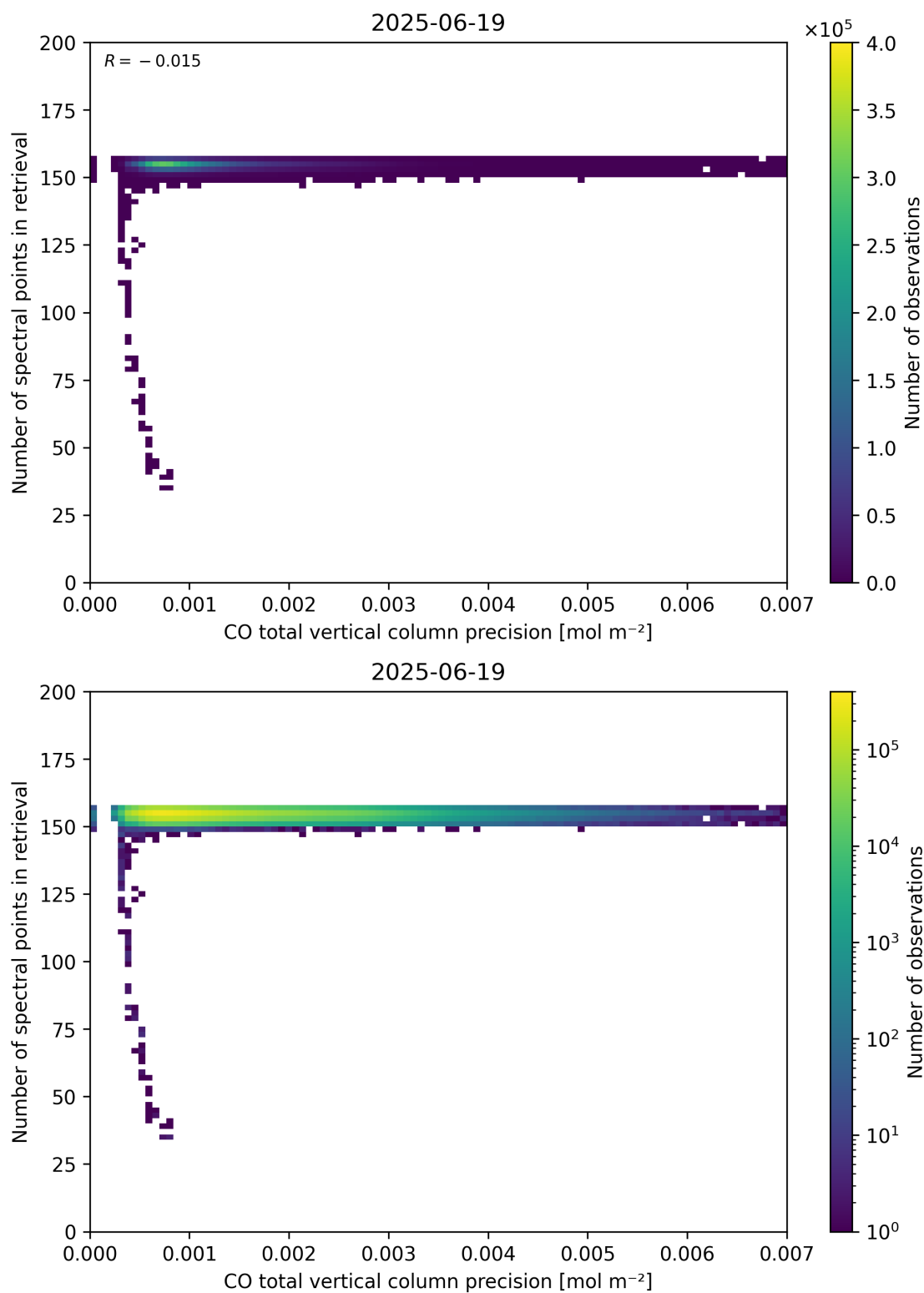
Figure 47: Scatter density plot of “CO total vertical column precision” against “Number of spectral points in retrieval” for 2025-06-18 to 2025-06-20.
