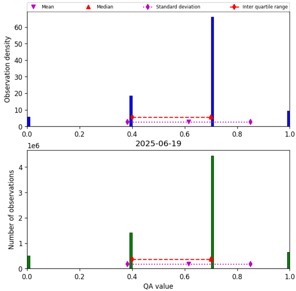
Figure 17: Histogram of “QA value” for 2025-06-18 to 2025-06-20
