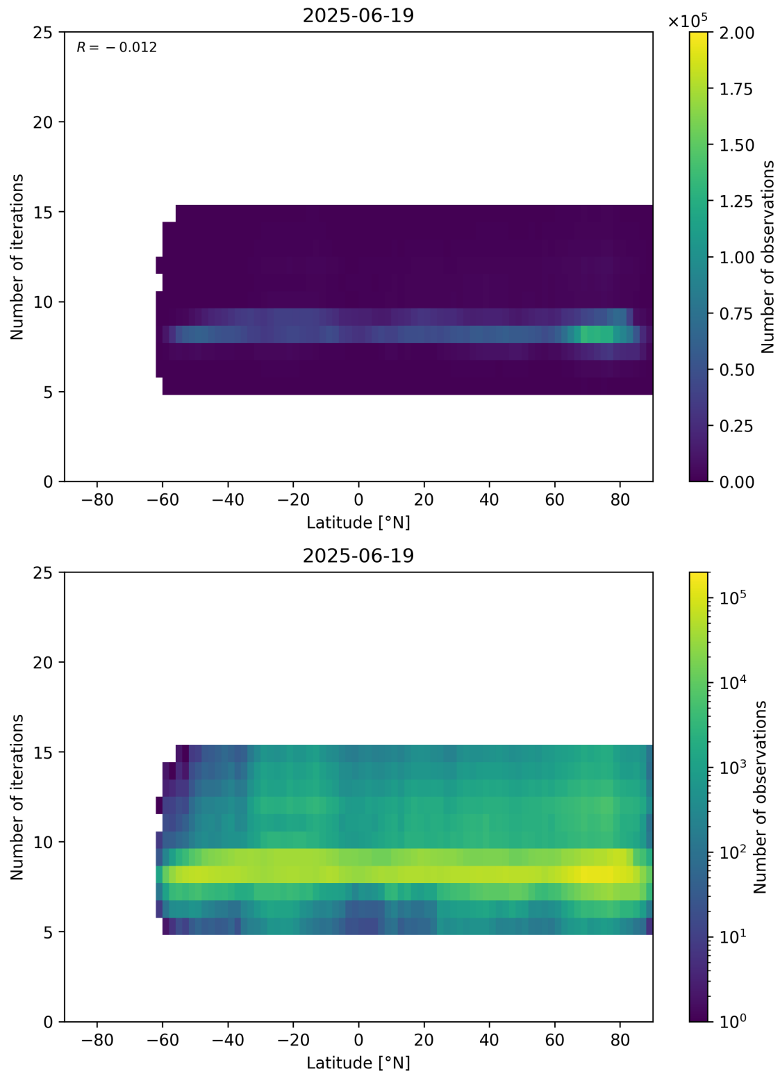
Figure 56: Scatter density plot of “Latitude” against “Number of iterations” for 2025-06-18 to 2025-06-20.
