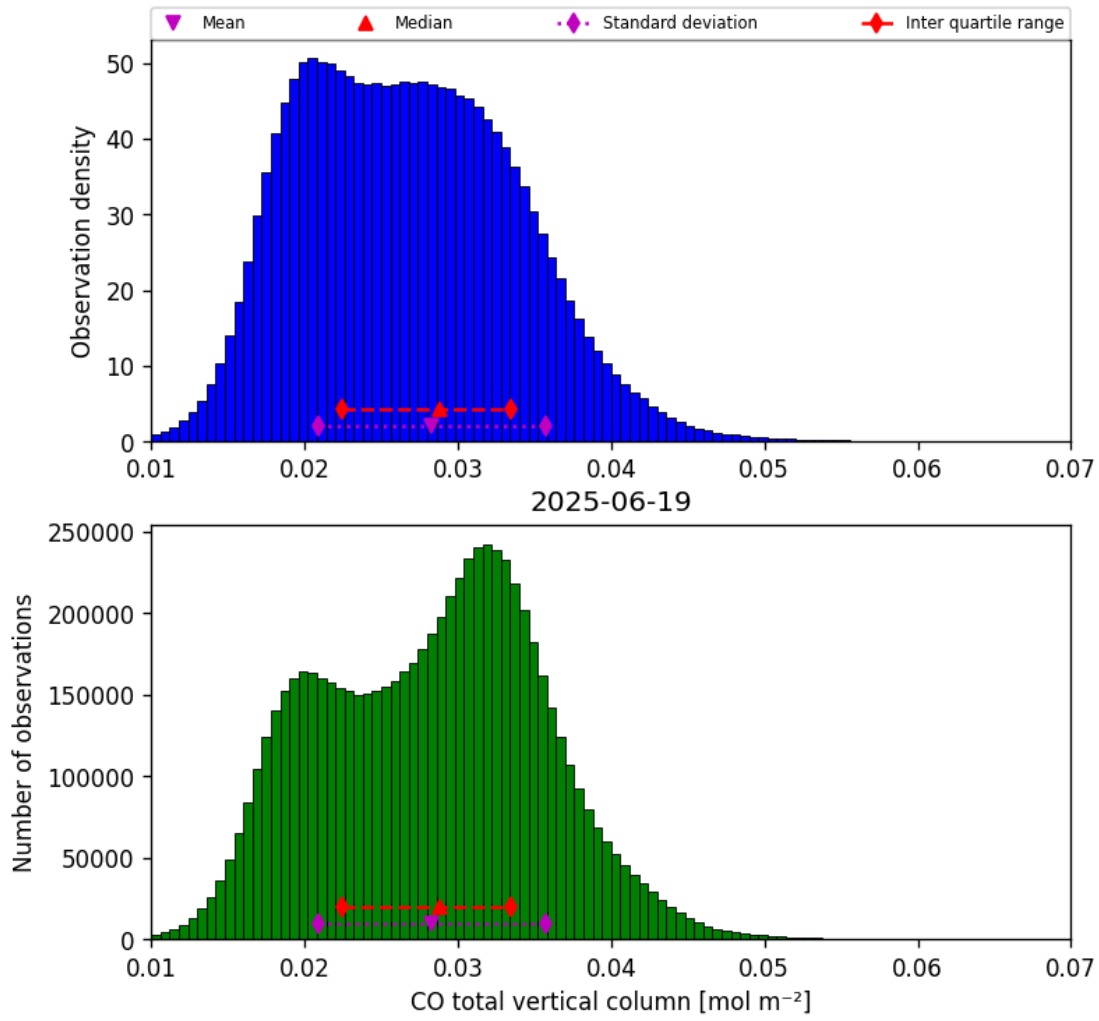
Figure 18: Histogram of “CO total vertical column” for 2025-06-18 to 2025-06-20
