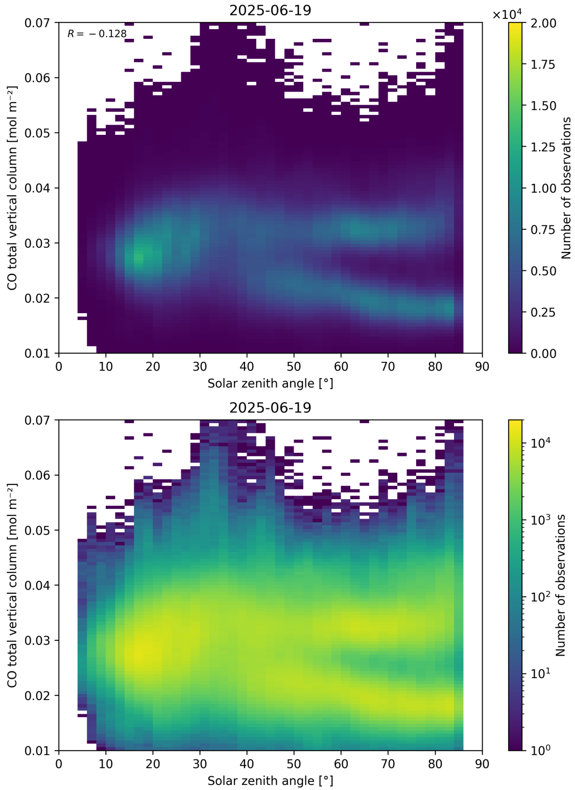
Figure 61: Scatter density plot of “Solar zenith angle” against “CO total vertical column” for 2025-06-18 to 2025-06-20.
