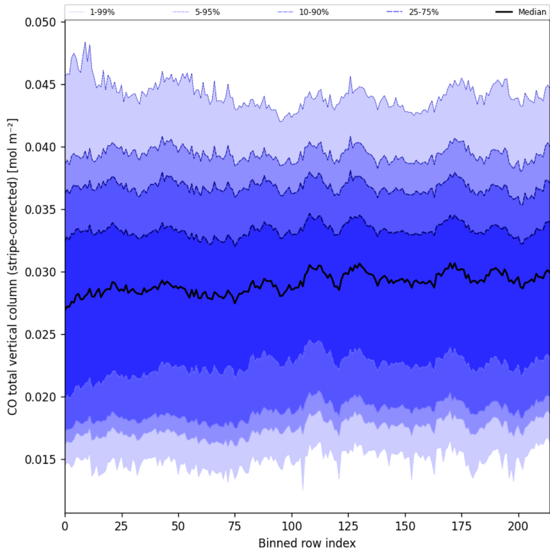
Figure 27: Along track statistics of “CO total vertical column (stripe-corrected)” for 2025-06-18 to 2025-06-20
