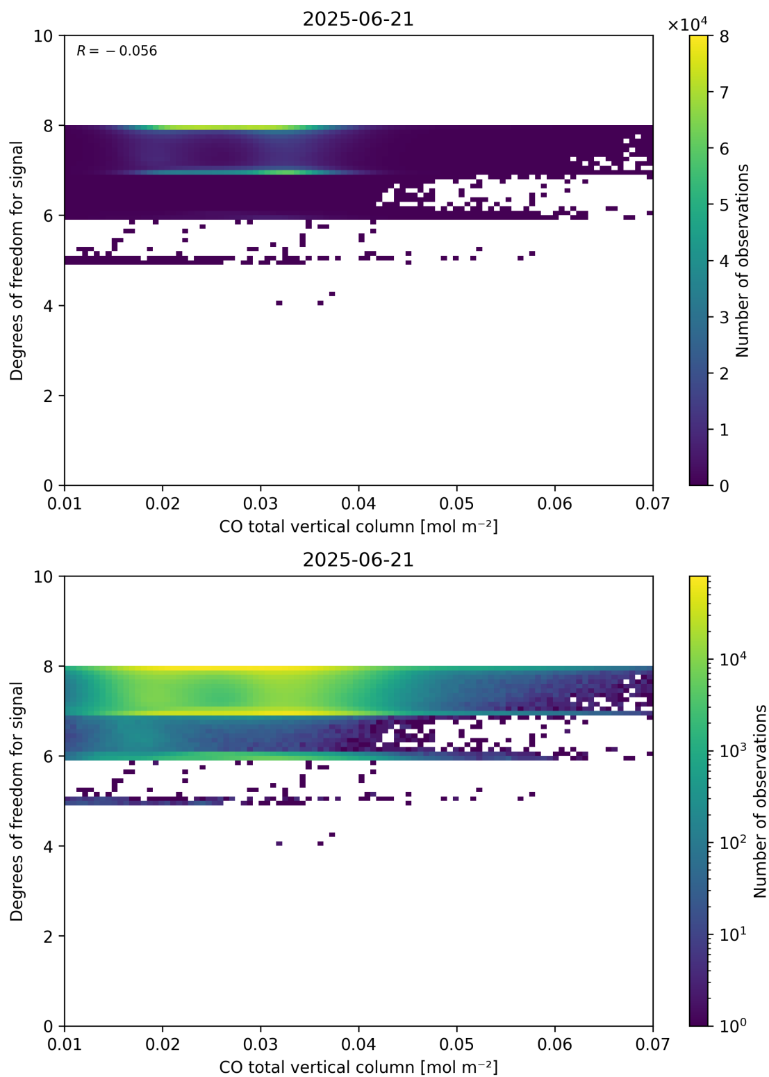
Figure 41: Scatter density plot of “CO total vertical column” against “Degrees of freedom for signal” for 2025-06-20 to 2025-06-22.
