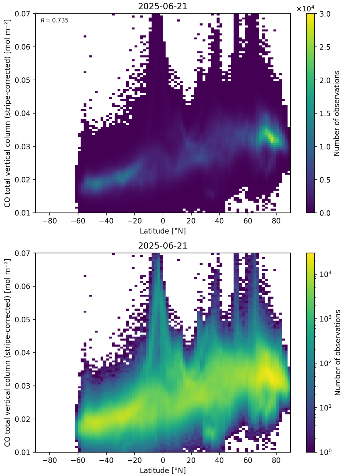
Figure 52: Scatter density plot of “Latitude” against “CO total vertical column (stripe-corrected)” for 2025-06-20 to 2025-06-22.
