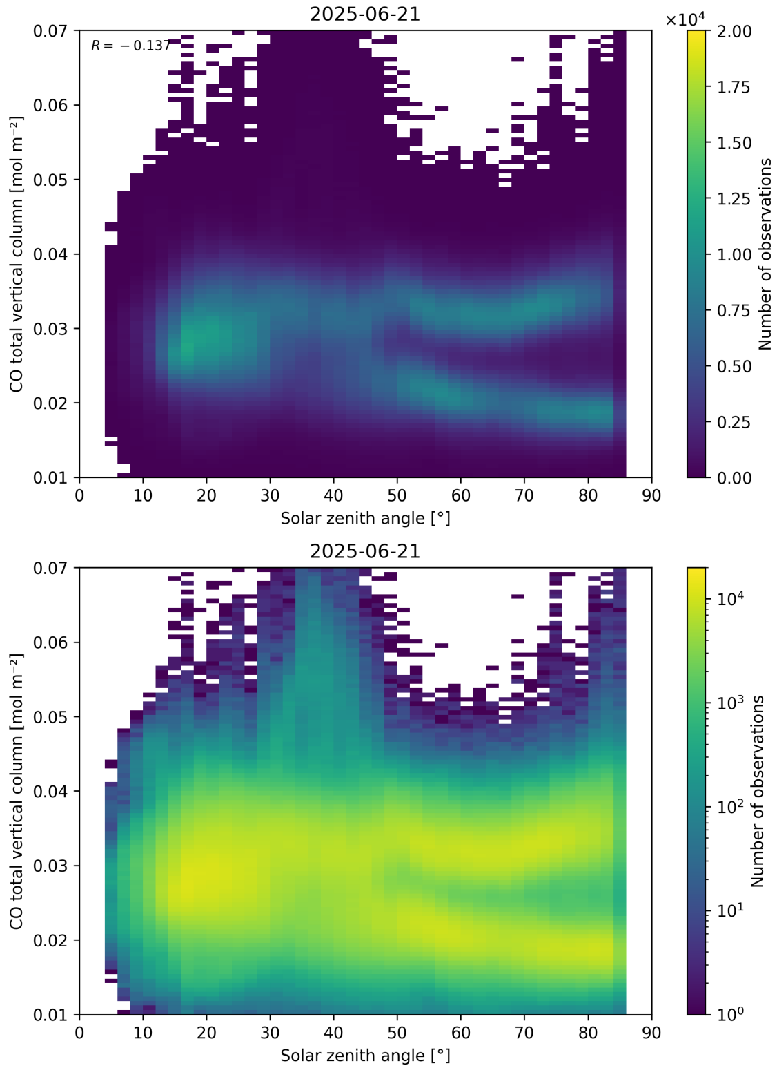
Figure 61: Scatter density plot of “Solar zenith angle” against “CO total vertical column” for 2025-06-20 to 2025-06-22.
