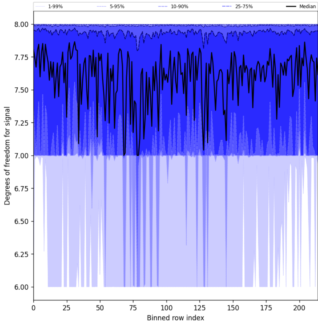
Figure 31: Along track statistics of “Degrees of freedom for signal” for 2025-06-20 to 2025-06-22
