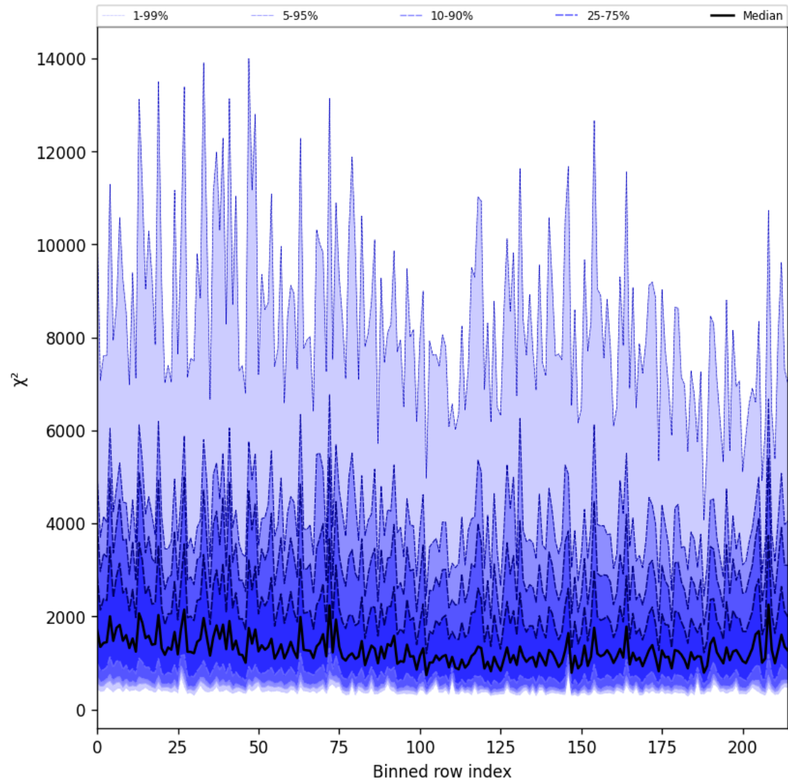
Figure 30: Along track statistics of “ \chi^2 ” for 2025-06-20 to 2025-06-22
