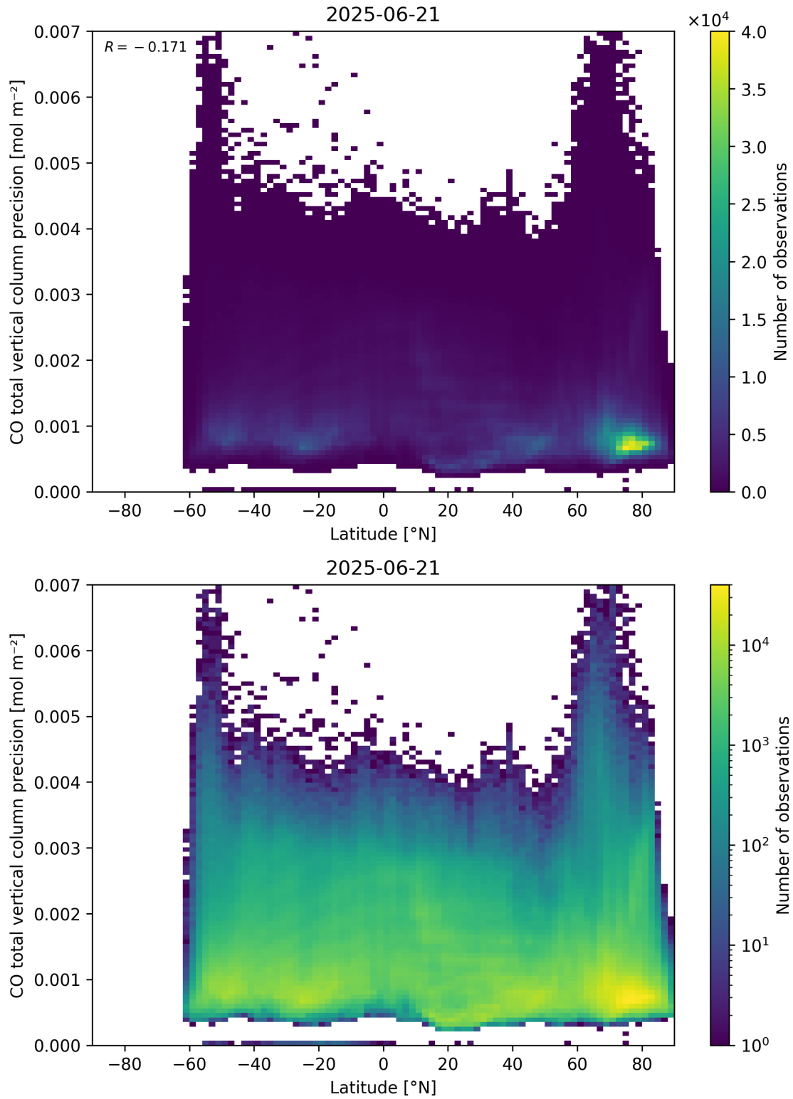
Figure 53: Scatter density plot of “Latitude” against “CO total vertical column precision” for 2025-06-20 to 2025-06-22.
