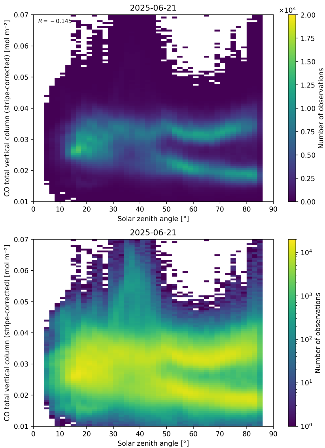
Figure 62: Scatter density plot of “Solar zenith angle” against “CO total vertical column (stripe-corrected)” for 2025-06-20 to 2025-06-22.
