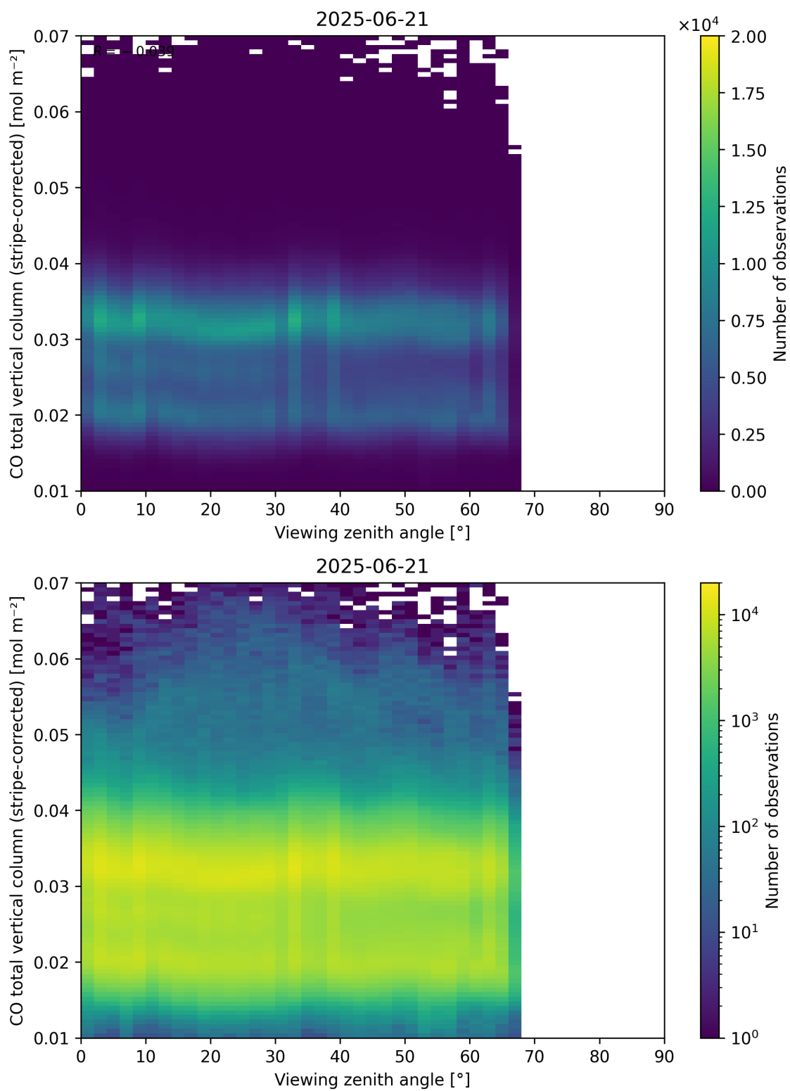
Figure 70: Scatter density plot of “Viewing zenith angle” against “CO total vertical column (stripe-corrected)” for 2025-06-20 to 2025-06-22.
