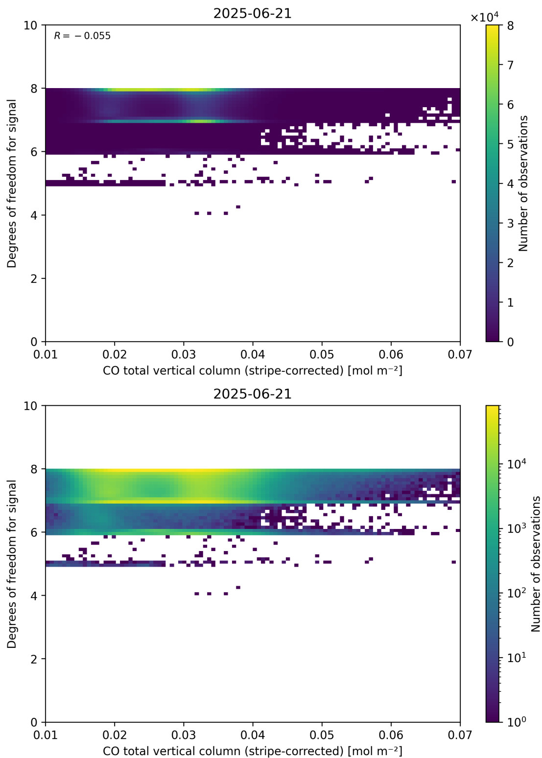
Figure 38: Scatter density plot of “CO total vertical column (stripe-corrected)” against “Degrees of freedom for signal” for 2025-06-20 to 2025-06-22.
