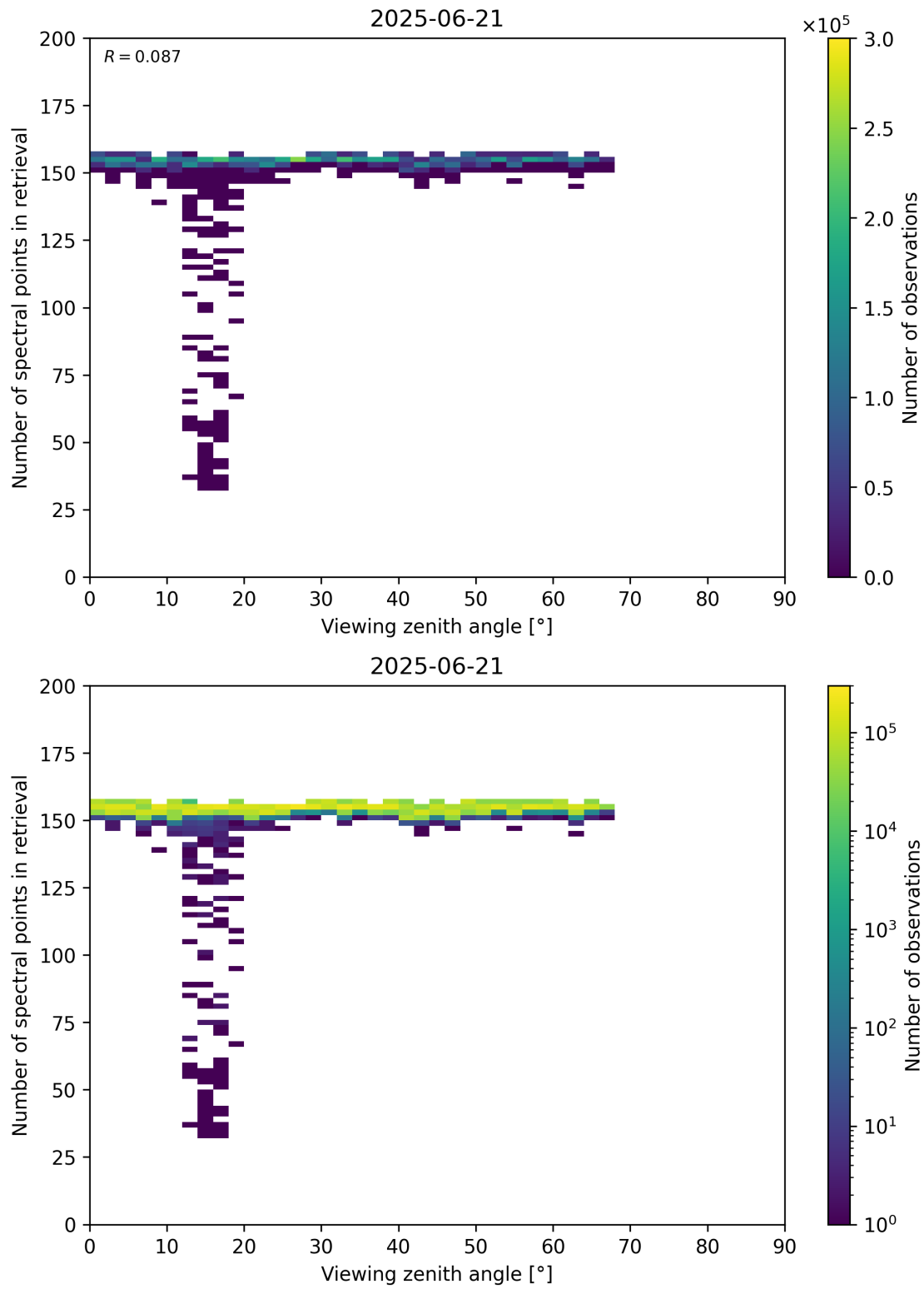
Figure 76: Scatter density plot of “Viewing zenith angle” against “Number of spectral points in retrieval” for 2025-06-20 to 2025-06-22.
