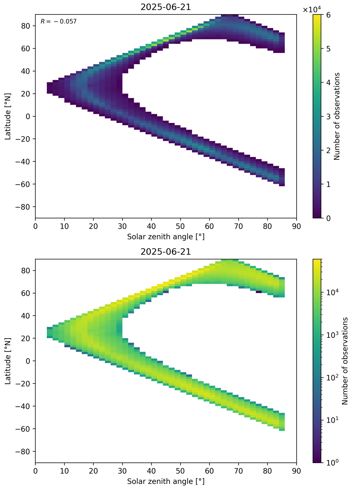
Figure 66: Scatter density plot of “Solar zenith angle” against “Latitude” for 2025-06-20 to 2025-06-22.
