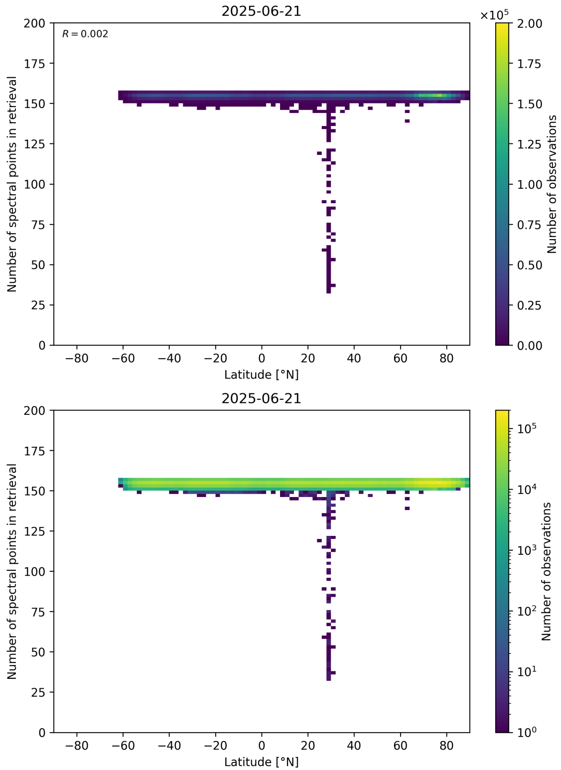
Figure 57: Scatter density plot of “Latitude” against “Number of spectral points in retrieval” for 2025-06-20 to 2025-06-22.
