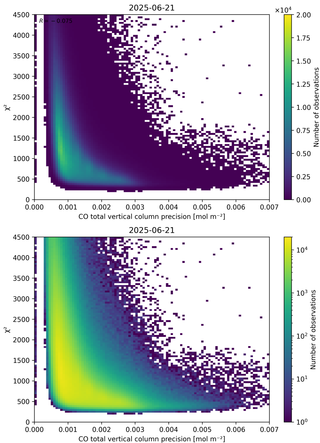
Figure 44: Scatter density plot of “CO total vertical column precision” against “ \chi^2 ” for 2025-06-20 to 2025-06-22.
