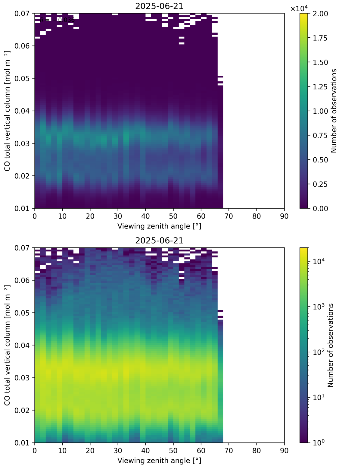
Figure 69: Scatter density plot of “Viewing zenith angle” against “CO total vertical column” for 2025-06-20 to 2025-06-22.
