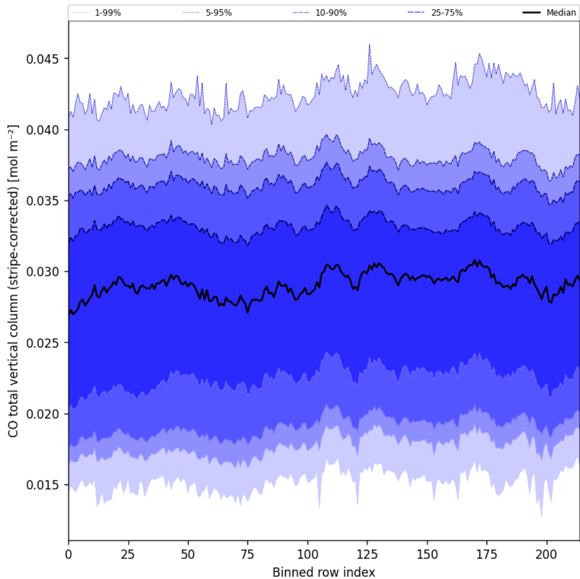
Figure 27: Along track statistics of “CO total vertical column (stripe-corrected)” for 2025-06-20 to 2025-06-22
