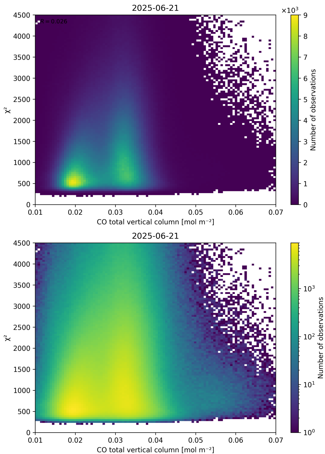
Figure 35: Scatter density plot of “CO total vertical column” against “ \chi^2 ” for 2025-06-20 to 2025-06-22.
