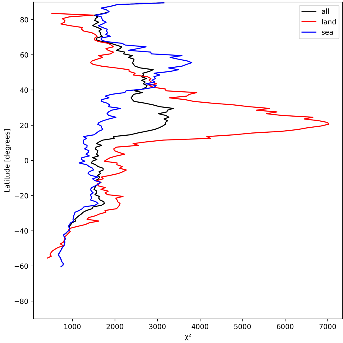
Figure 14: Zonal average of “ \chi^2 ” for 2025-06-20 to 2025-06-22.
