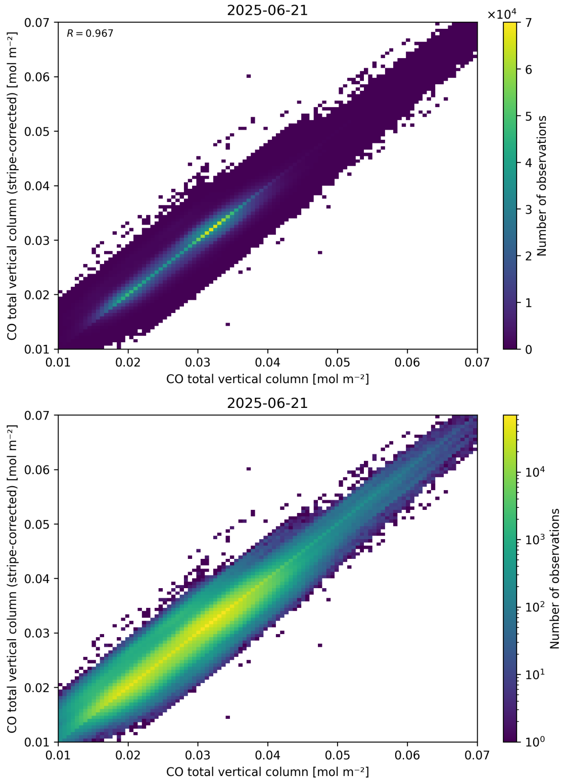
Figure 33: Scatter density plot of “CO total vertical column” against “CO total vertical column (stripe-corrected)” for 2025-06-20 to 2025-06-22.
