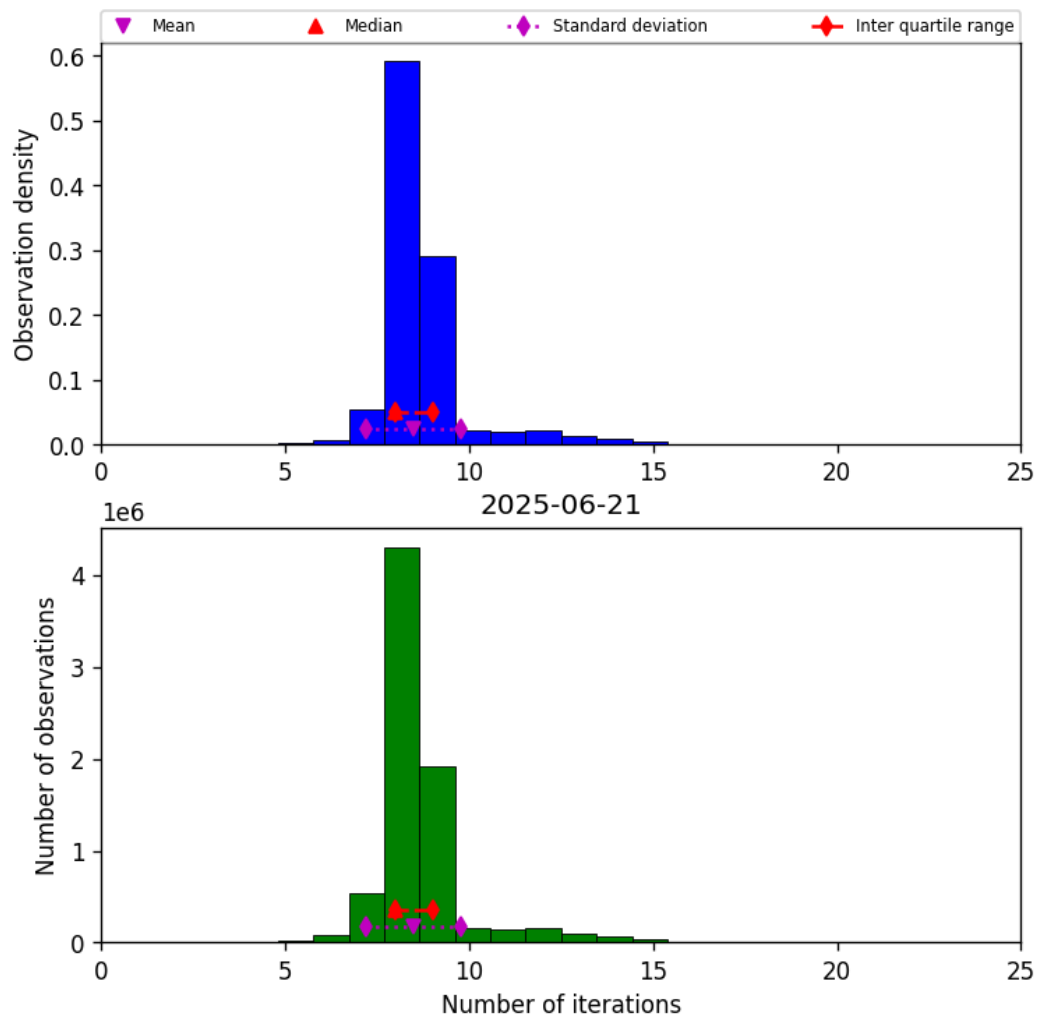
Figure 24: Histogram of “Number of iterations” for 2025-06-20 to 2025-06-22
