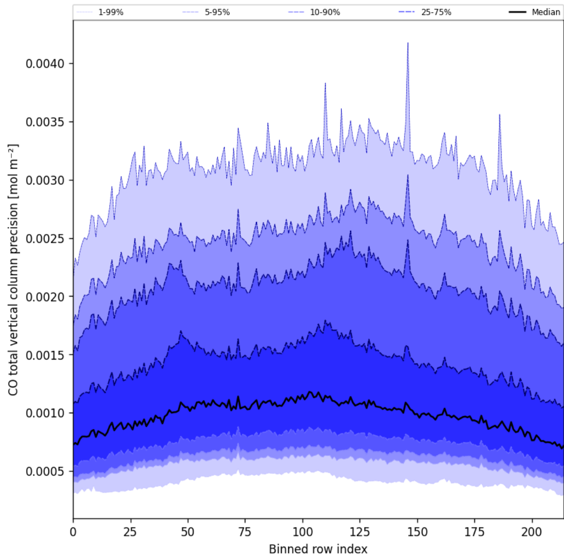
Figure 28: Along track statistics of “CO total vertical column precision” for 2025-06-20 to 2025-06-22
