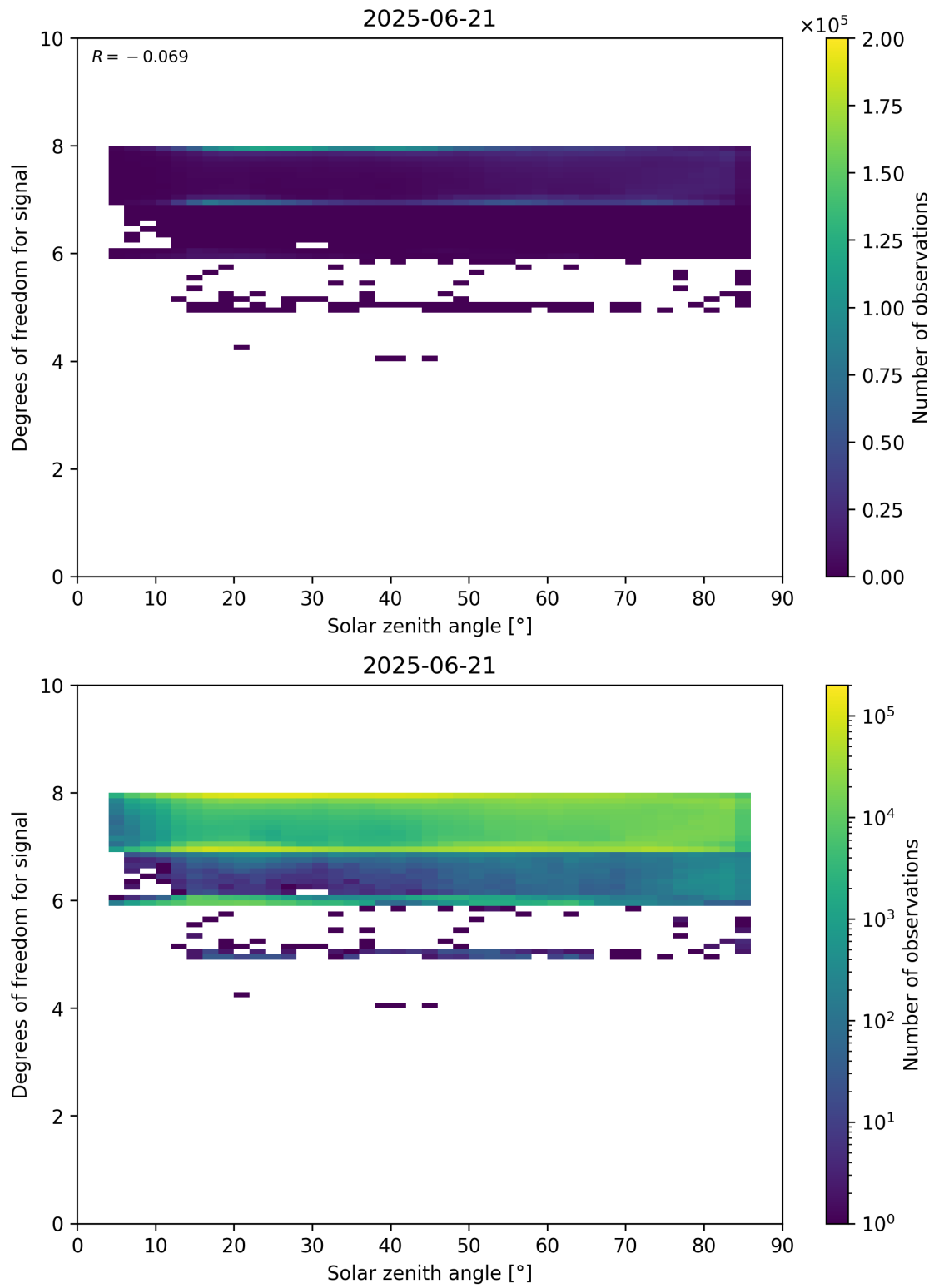
Figure 65: Scatter density plot of “Solar zenith angle” against “Degrees of freedom for signal” for 2025-06-20 to 2025-06-22.
