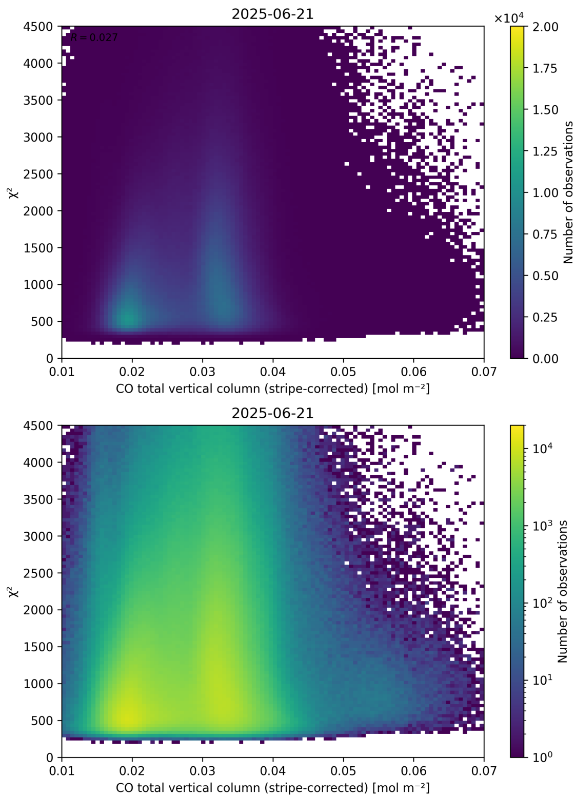
Figure 37: Scatter density plot of “CO total vertical column (stripe-corrected)” against “ \chi^2 ” for 2025-06-20 to 2025-06-22.
