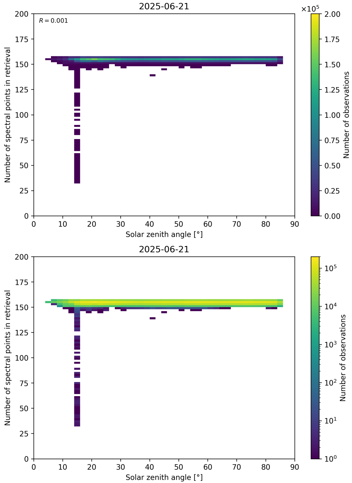
Figure 68: Scatter density plot of “Solar zenith angle” against “Number of spectral points in retrieval” for 2025-06-20 to 2025-06-22.
