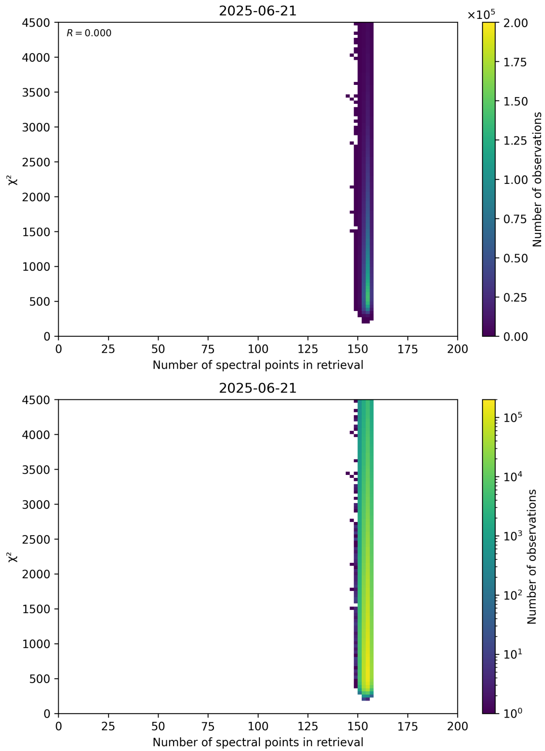
Figure 58: Scatter density plot of “Number of spectral points in retrieval” against “ \chi^2 ” for 2025-06-20 to 2025-06-22.
