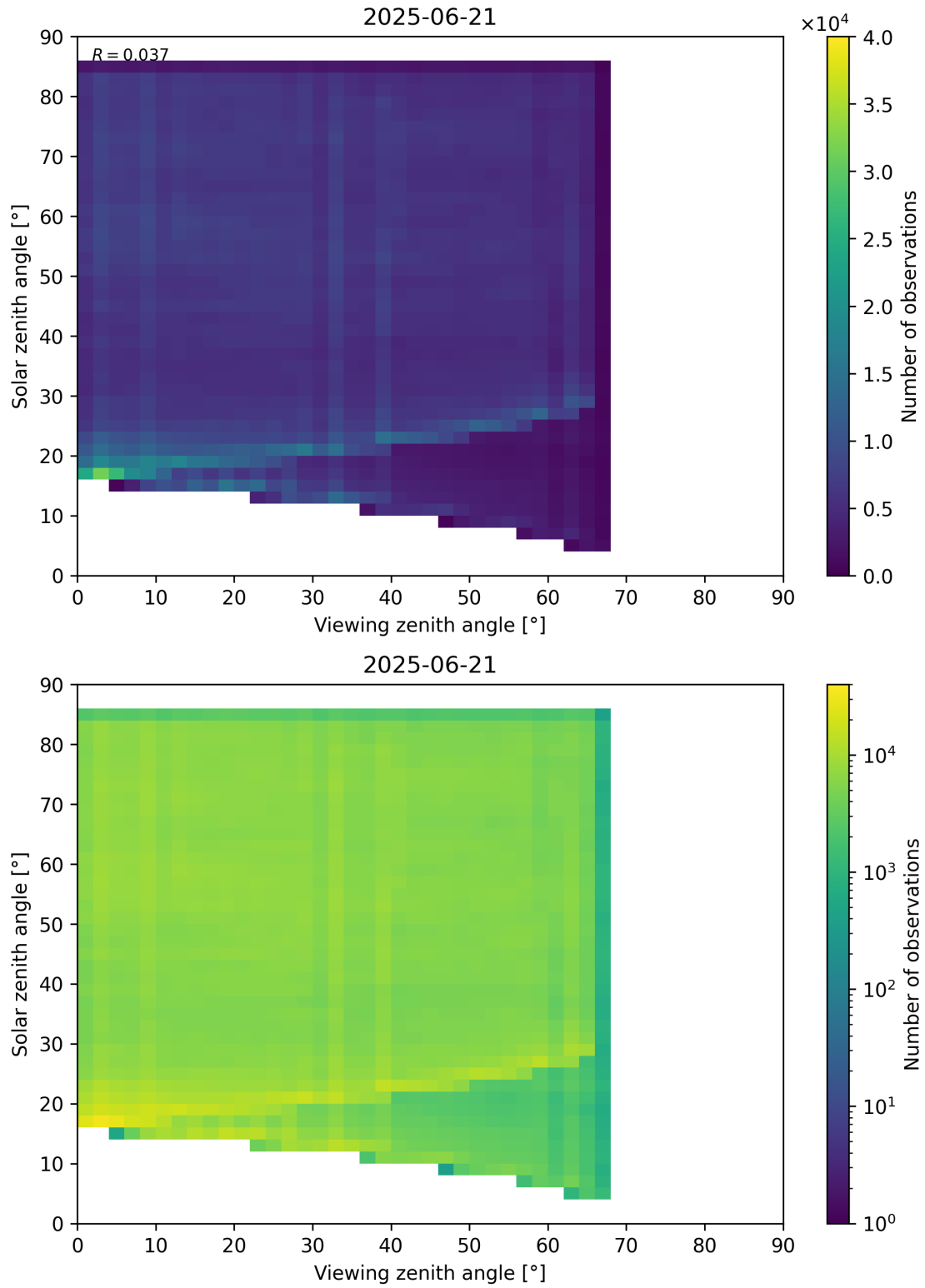
Figure 77: Scatter density plot of “Viewing zenith angle” against “Solar zenith angle” for 2025-06-20 to 2025-06-22.
