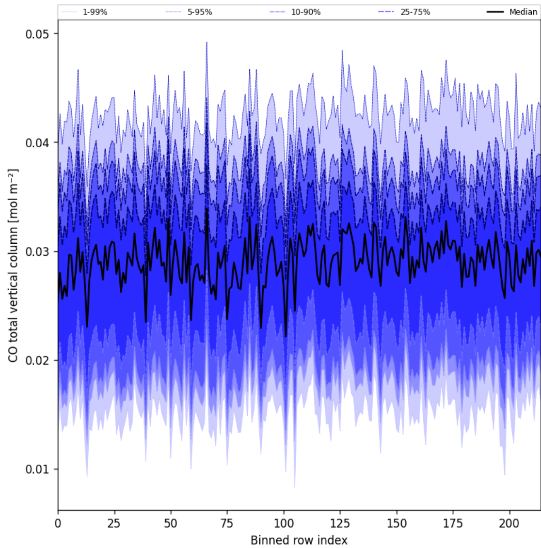
Figure 26: Along track statistics of “CO total vertical column” for 2025-06-20 to 2025-06-22
