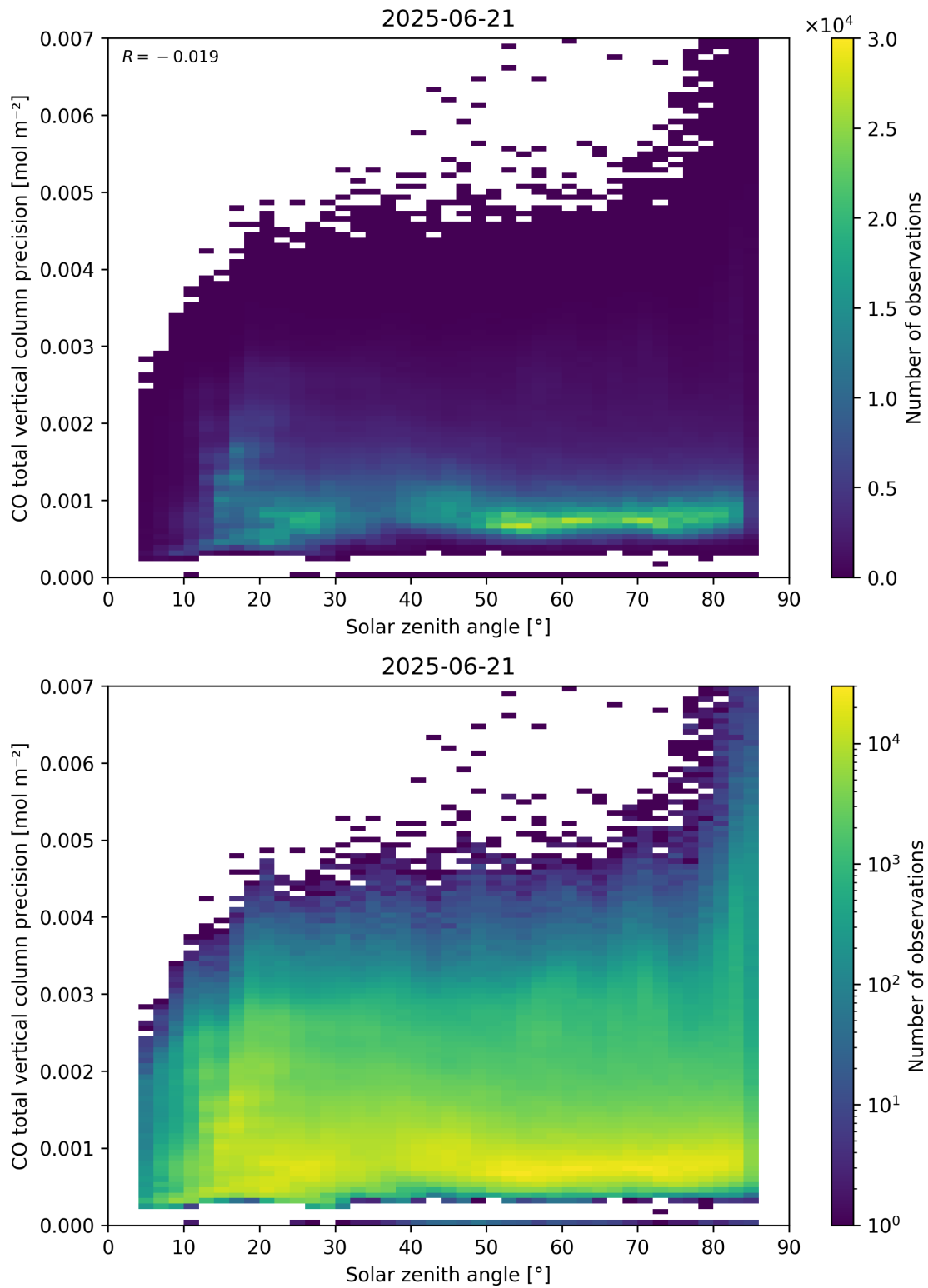
Figure 63: Scatter density plot of “Solar zenith angle” against “CO total vertical column precision” for 2025-06-20 to 2025-06-22.
