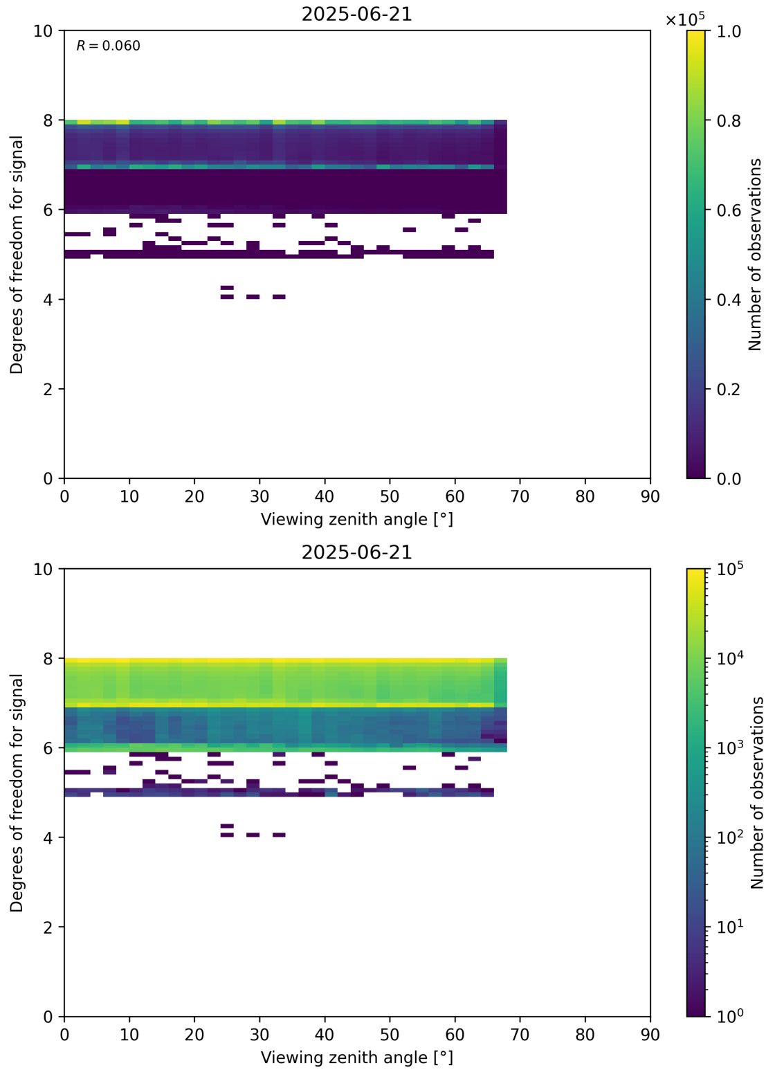
Figure 73: Scatter density plot of “Viewing zenith angle” against “Degrees of freedom for signal” for 2025-06-20 to 2025-06-22.
