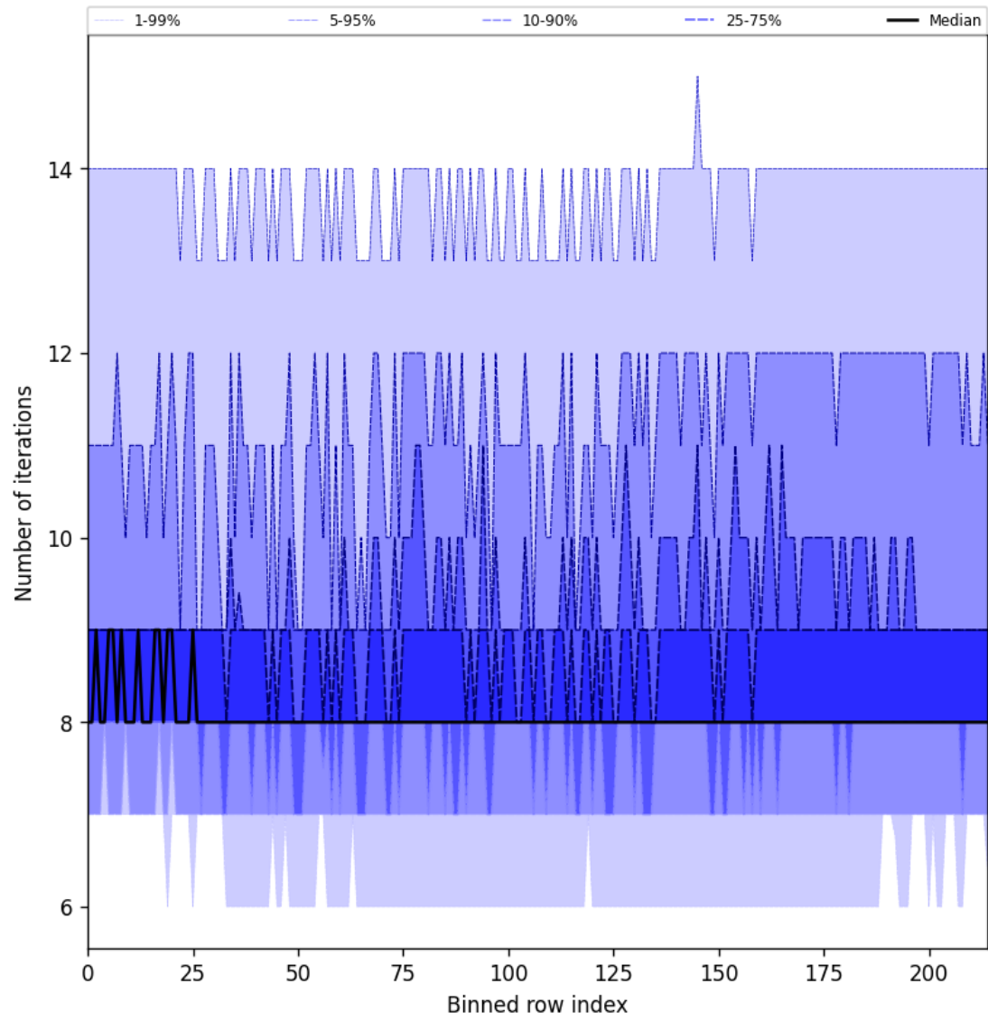
Figure 32: Along track statistics of “Number of iterations” for 2025-06-20 to 2025-06-22
