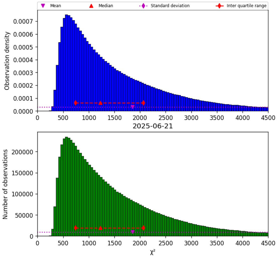
Figure 22: Histogram of “ \chi^2 ” for 2025-06-20 to 2025-06-22
