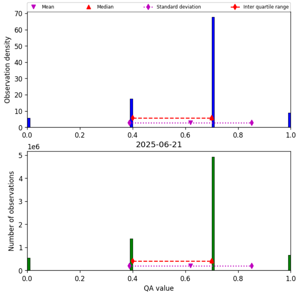
Figure 17: Histogram of “QA value” for 2025-06-20 to 2025-06-22
