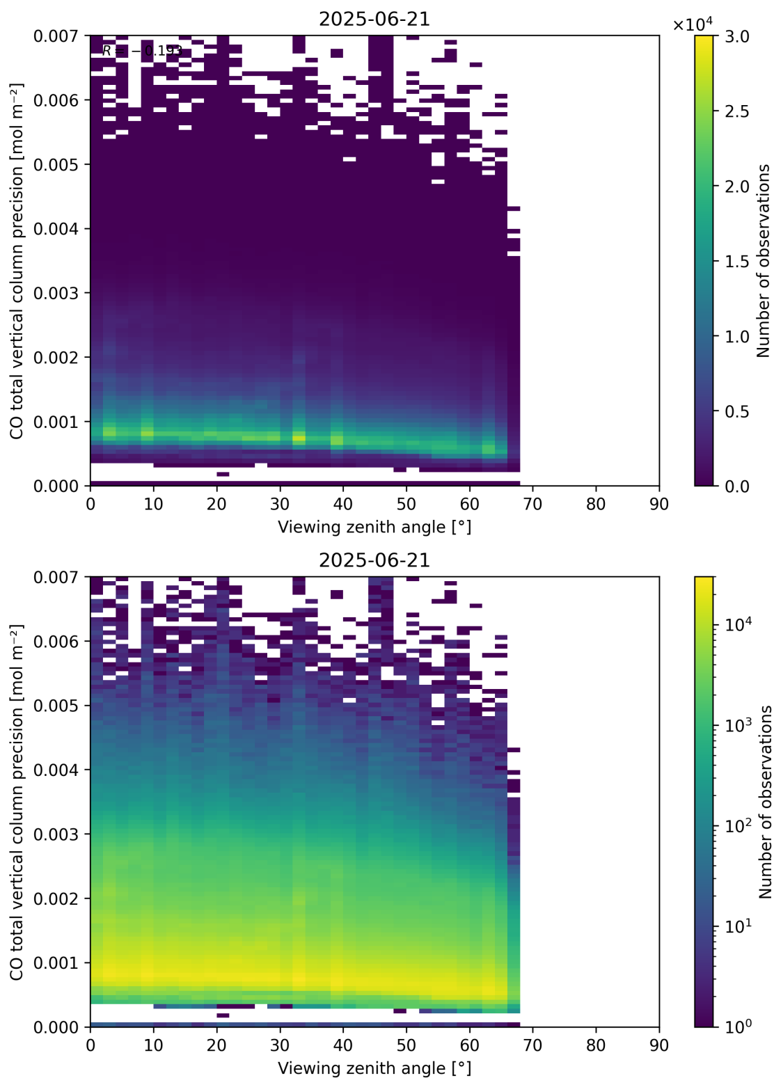
Figure 71: Scatter density plot of “Viewing zenith angle” against “CO total vertical column precision” for 2025-06-20 to 2025-06-22.
