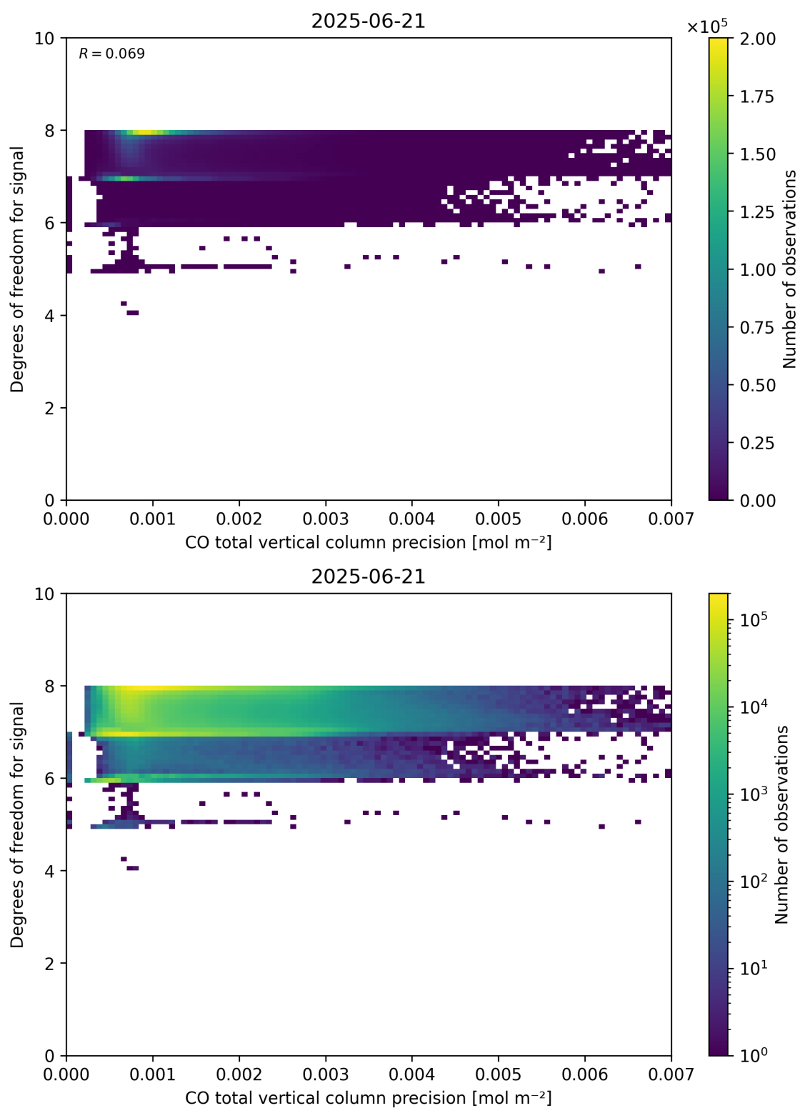
Figure 45: Scatter density plot of “CO total vertical column precision” against “Degrees of freedom for signal” for 2025-06-20 to 2025-06-22.
