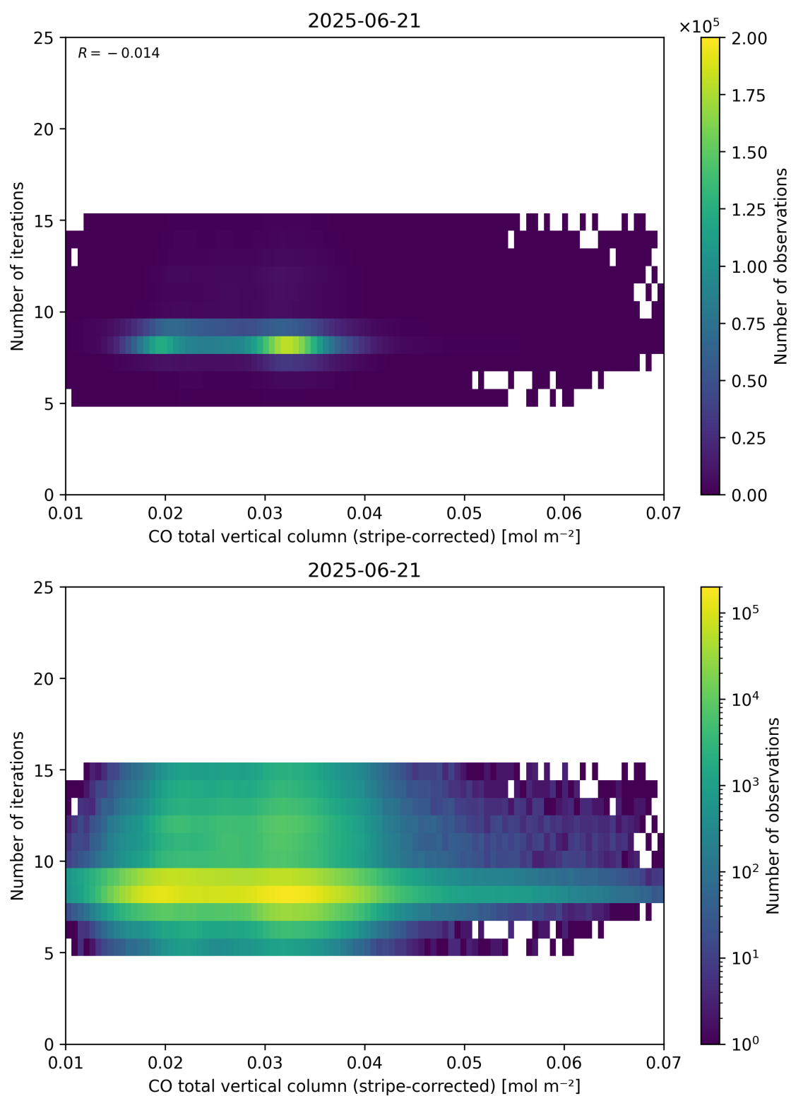
Figure 39: Scatter density plot of “CO total vertical column (stripe-corrected)” against “Number of iterations” for 2025-06-20 to 2025-06-22.
