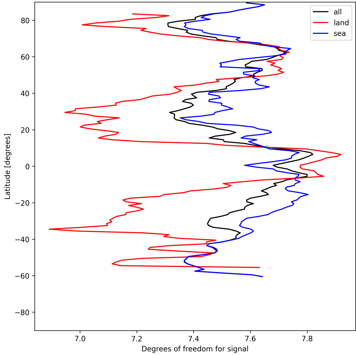
Figure 15: Zonal average of “Degrees of freedom for signal” for 2025-06-20 to 2025-06-22.
