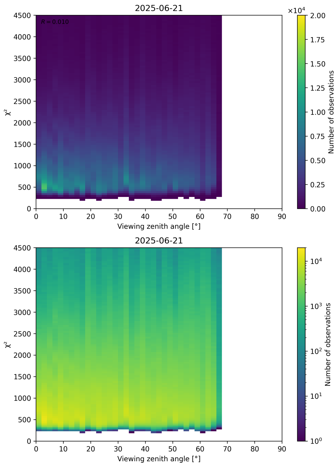
Figure 72: Scatter density plot of “Viewing zenith angle” against “ \chi^2 ” for 2025-06-20 to 2025-06-22.
