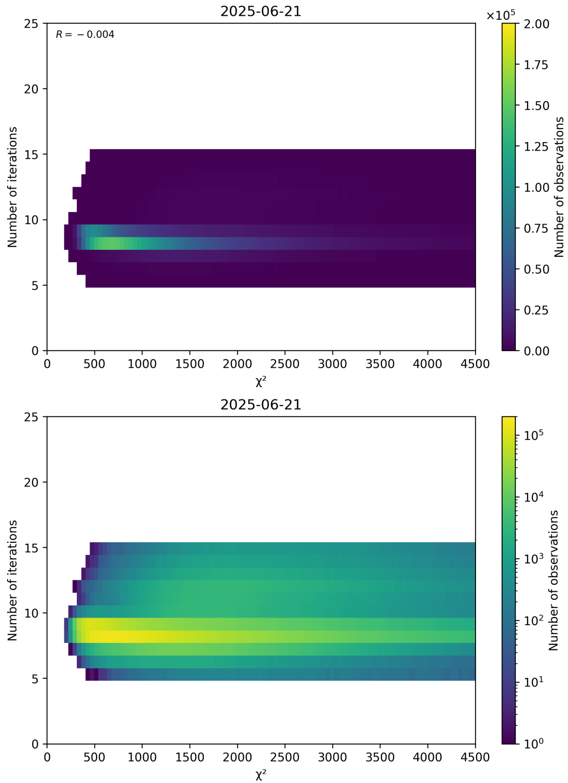
Figure 49: Scatter density plot of “ \chi^2 ” against “Number of iterations” for 2025-06-20 to 2025-06-22.
