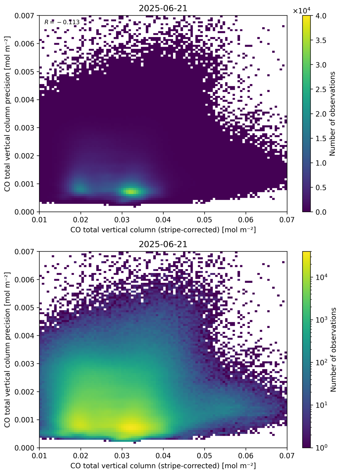
Figure 36: Scatter density plot of “CO total vertical column (stripe-corrected)” against “CO total vertical column precision” for 2025-06-20 to 2025-06-22.
