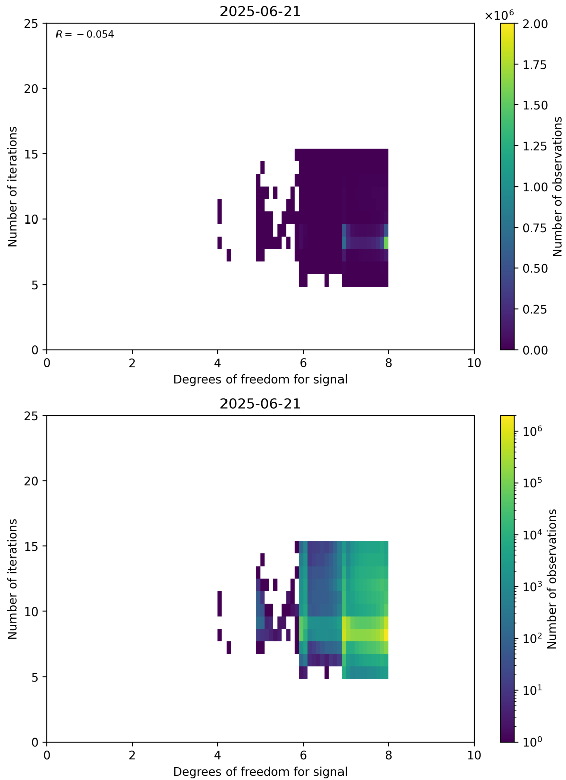
Figure 50: Scatter density plot of “Degrees of freedom for signal” against “Number of iterations” for 2025-06-20 to 2025-06-22.
