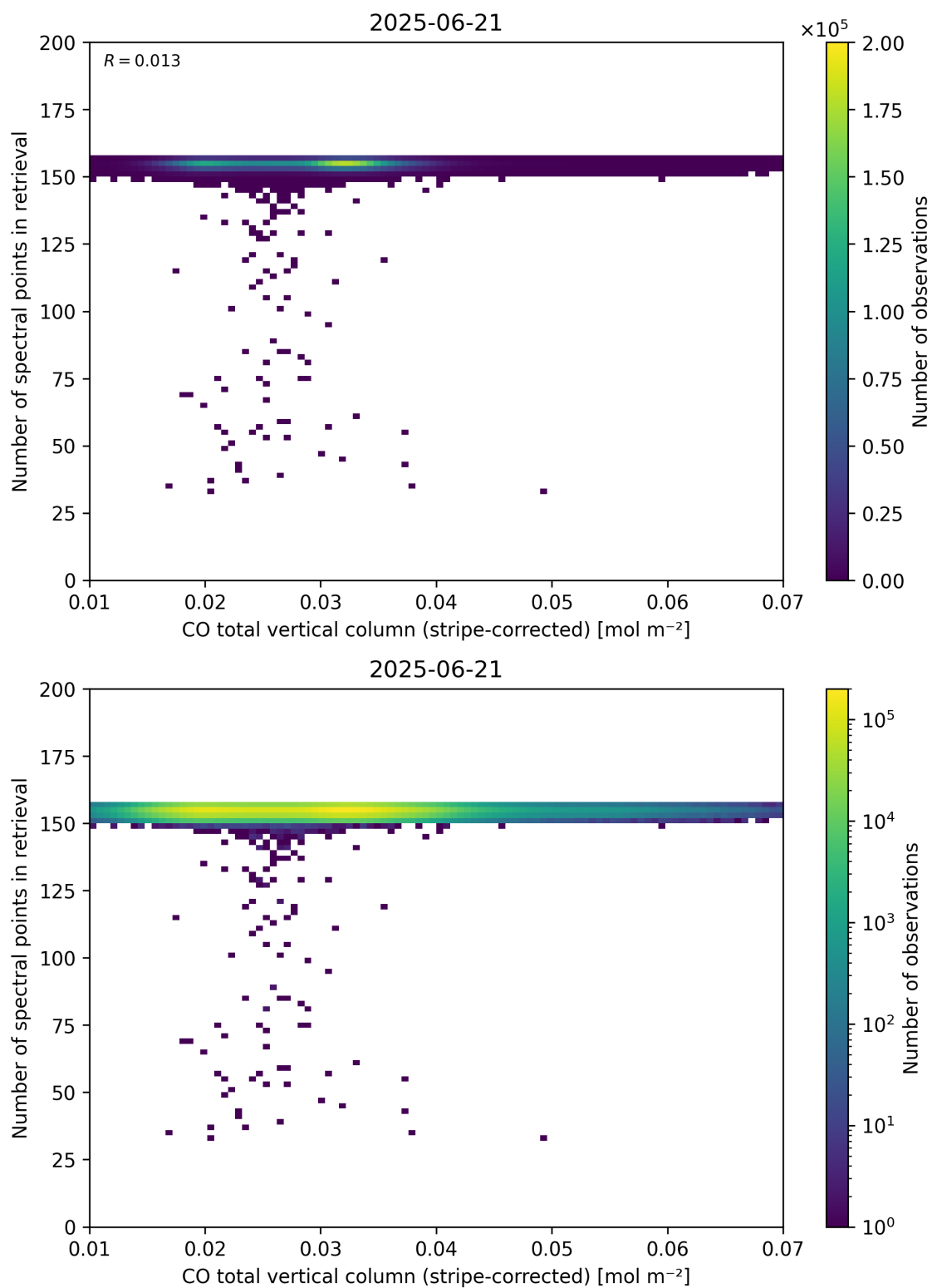
Figure 40: Scatter density plot of “CO total vertical column (stripe-corrected)” against “Number of spectral points in retrieval” for 2025-06-20 to 2025-06-22.
