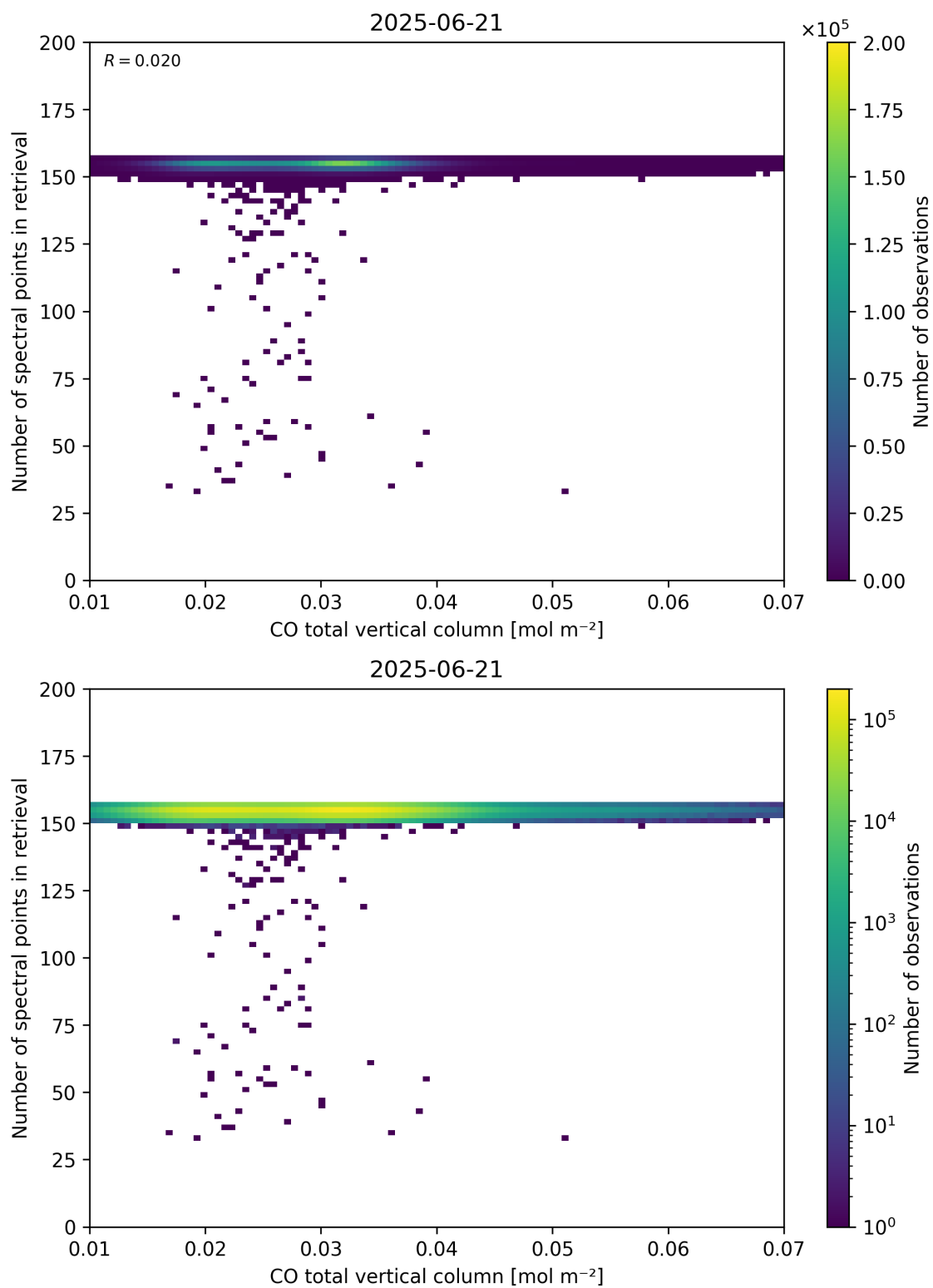
Figure 43: Scatter density plot of “CO total vertical column” against “Number of spectral points in retrieval” for 2025-06-20 to 2025-06-22.
