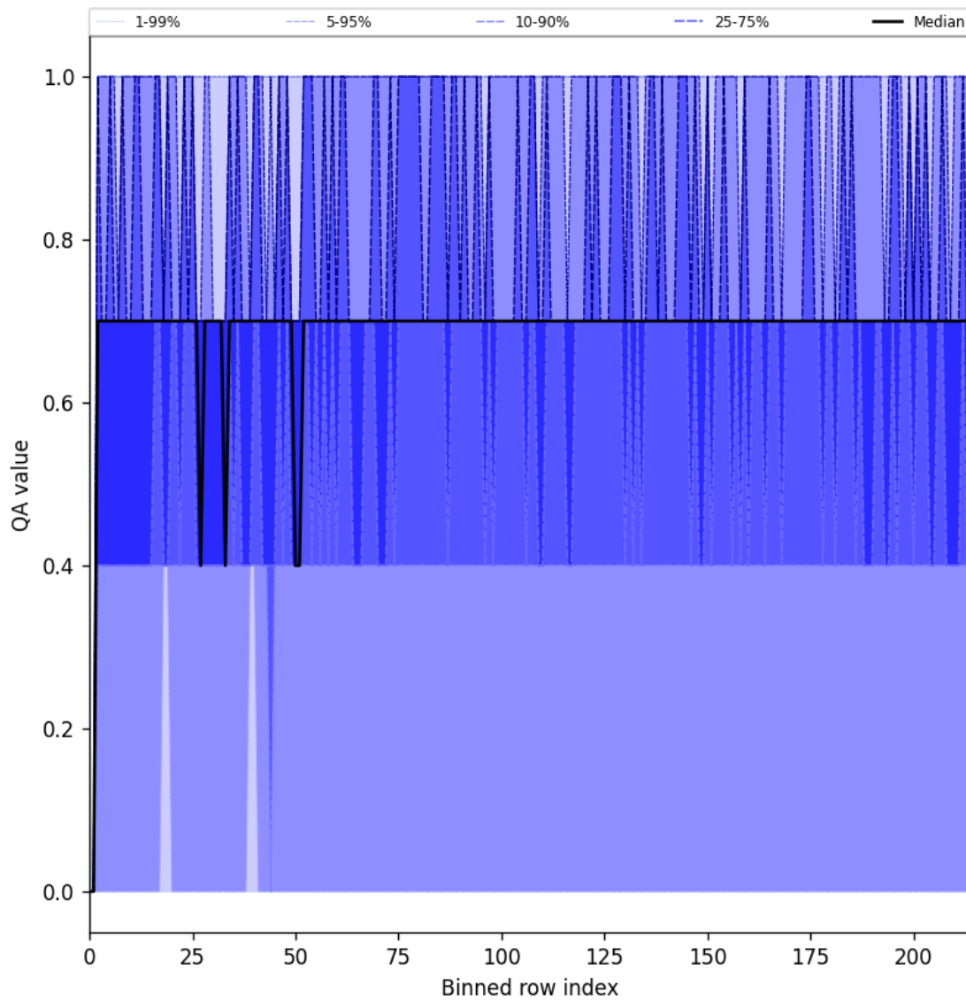
Figure 25: Along track statistics of “QA value” for 2025-06-20 to 2025-06-22
