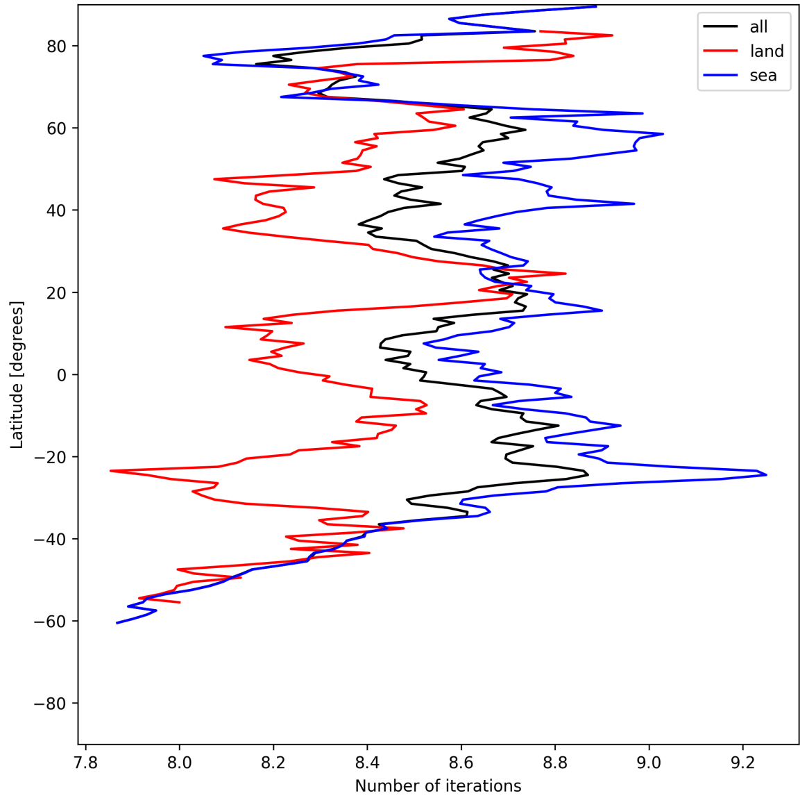
Figure 16: Zonal average of “Number of iterations” for 2025-06-20 to 2025-06-22.
