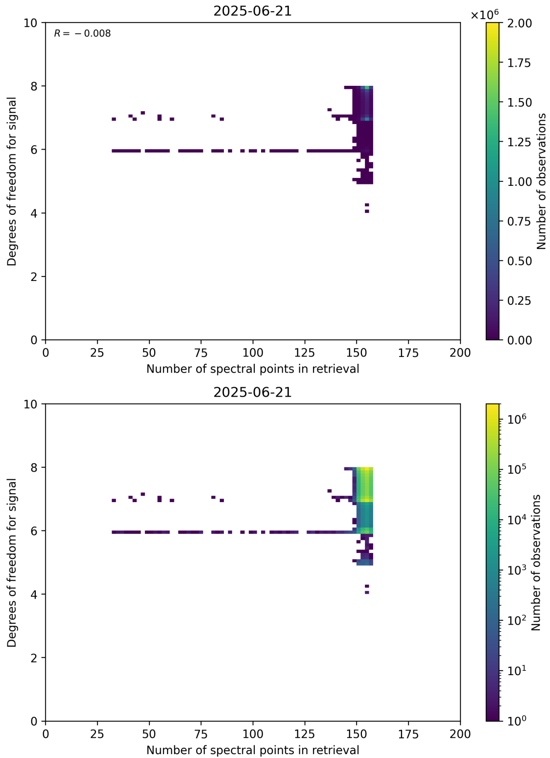
Figure 59: Scatter density plot of “Number of spectral points in retrieval” against “Degrees of freedom for signal” for 2025-06-20 to 2025-06-22.
