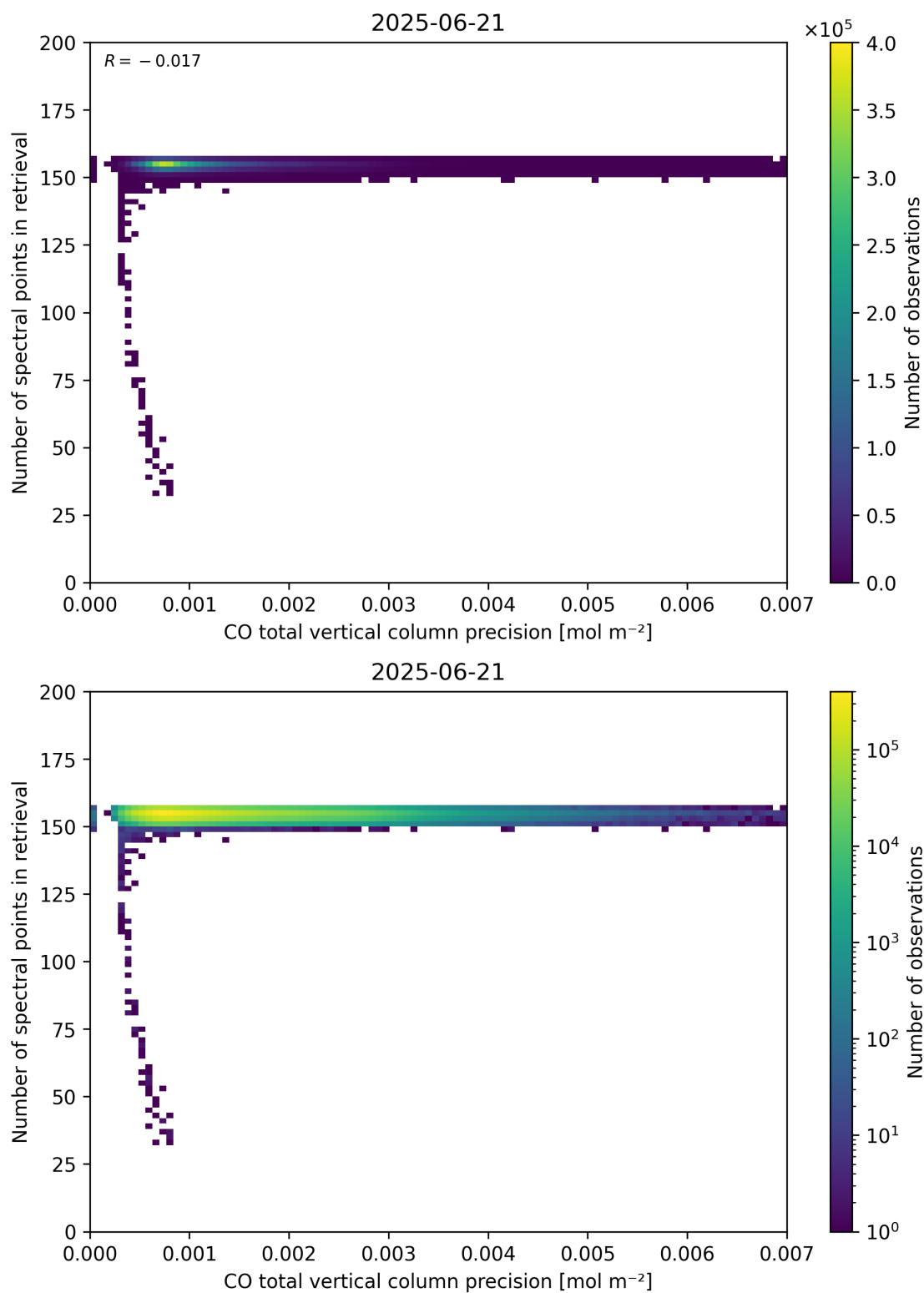
Figure 47: Scatter density plot of “CO total vertical column precision” against “Number of spectral points in retrieval” for 2025-06-20 to 2025-06-22.
