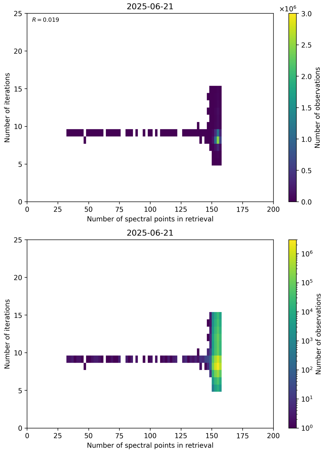
Figure 60: Scatter density plot of “Number of spectral points in retrieval” against “Number of iterations” for 2025-06-20 to 2025-06-22.
