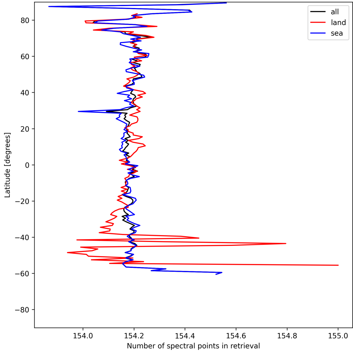
Figure 13: Zonal average of “Number of spectral points in retrieval” for 2025-06-20 to 2025-06-22.
