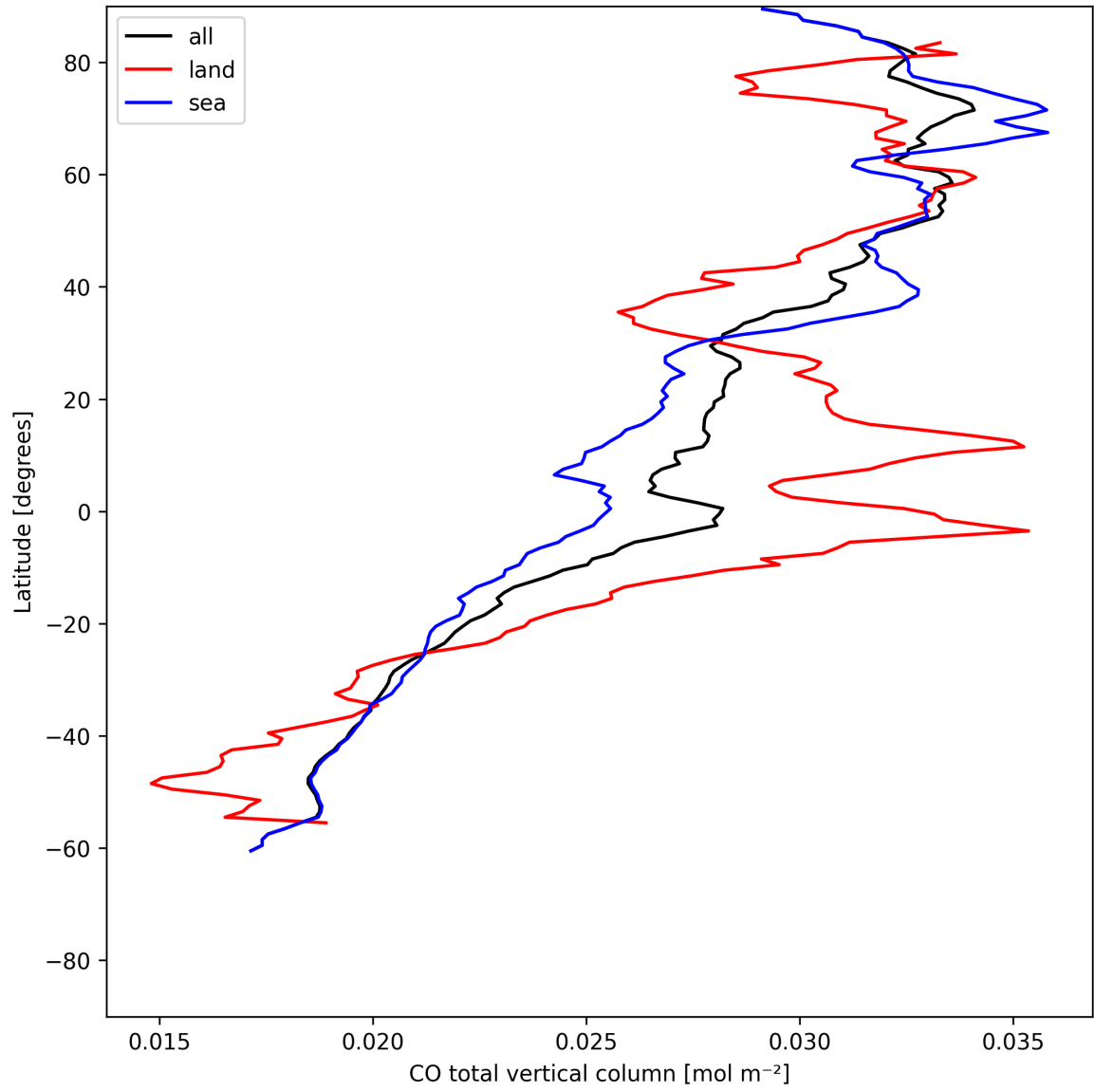
Figure 10: Zonal average of “CO total vertical column” for 2025-06-20 to 2025-06-22.
