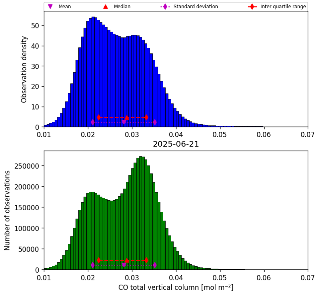
Figure 18: Histogram of “CO total vertical column” for 2025-06-20 to 2025-06-22
