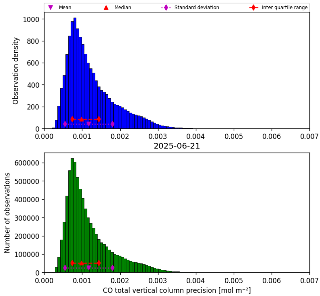
Figure 20: Histogram of “CO total vertical column precision” for 2025-06-20 to 2025-06-22
