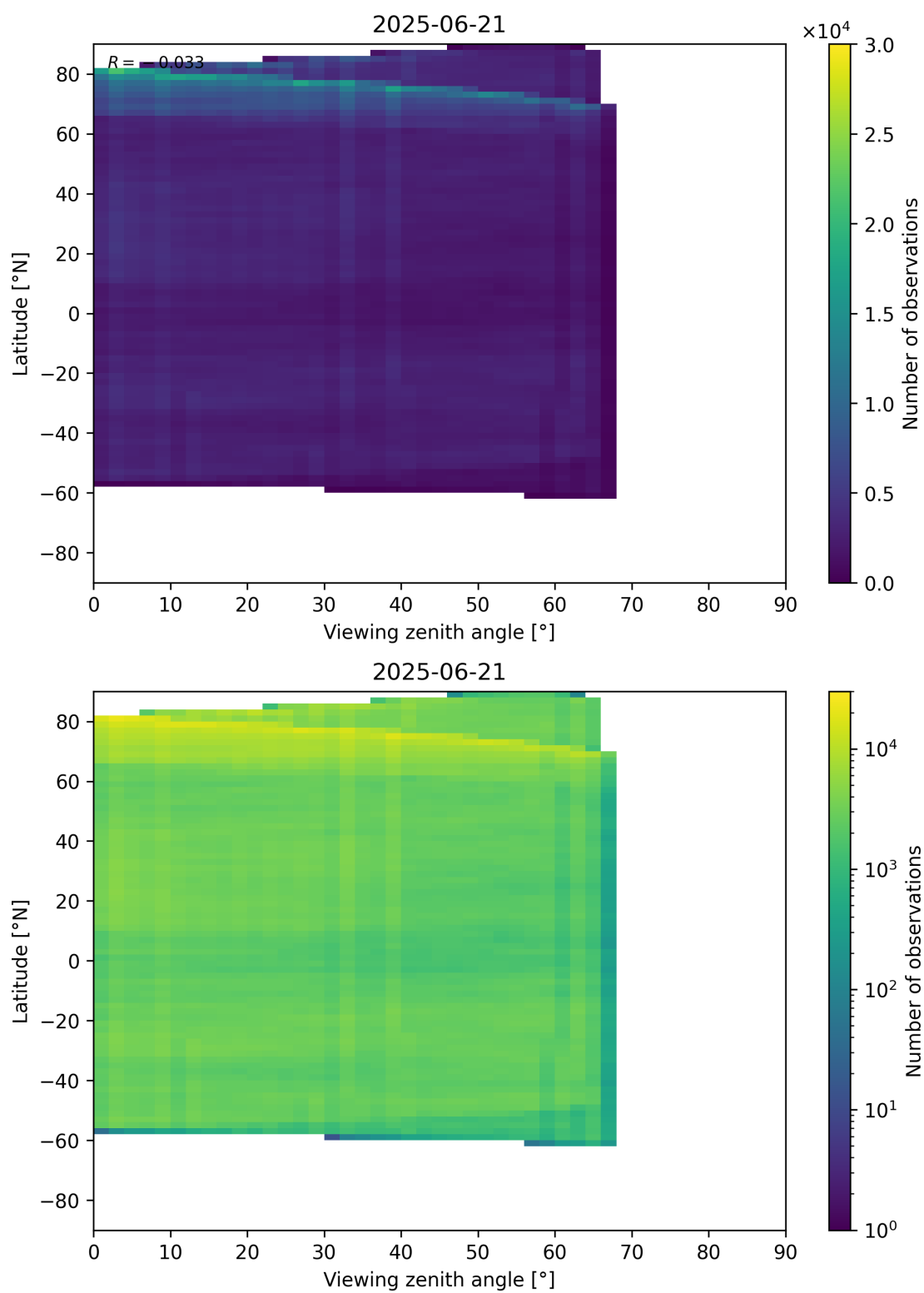
Figure 74: Scatter density plot of “Viewing zenith angle” against “Latitude” for 2025-06-20 to 2025-06-22.
