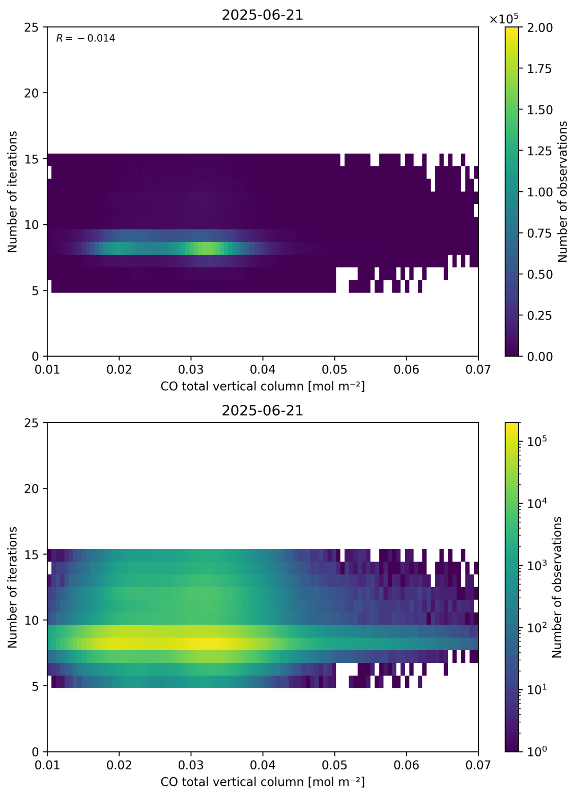
Figure 42: Scatter density plot of “CO total vertical column” against “Number of iterations” for 2025-06-20 to 2025-06-22.
