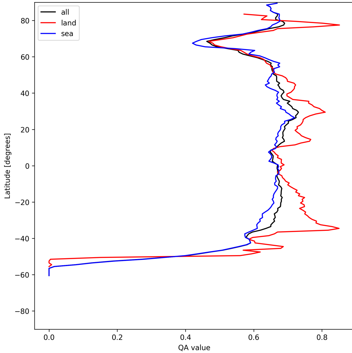
Figure 9: Zonal average of “QA value” for 2025-06-20 to 2025-06-22.
