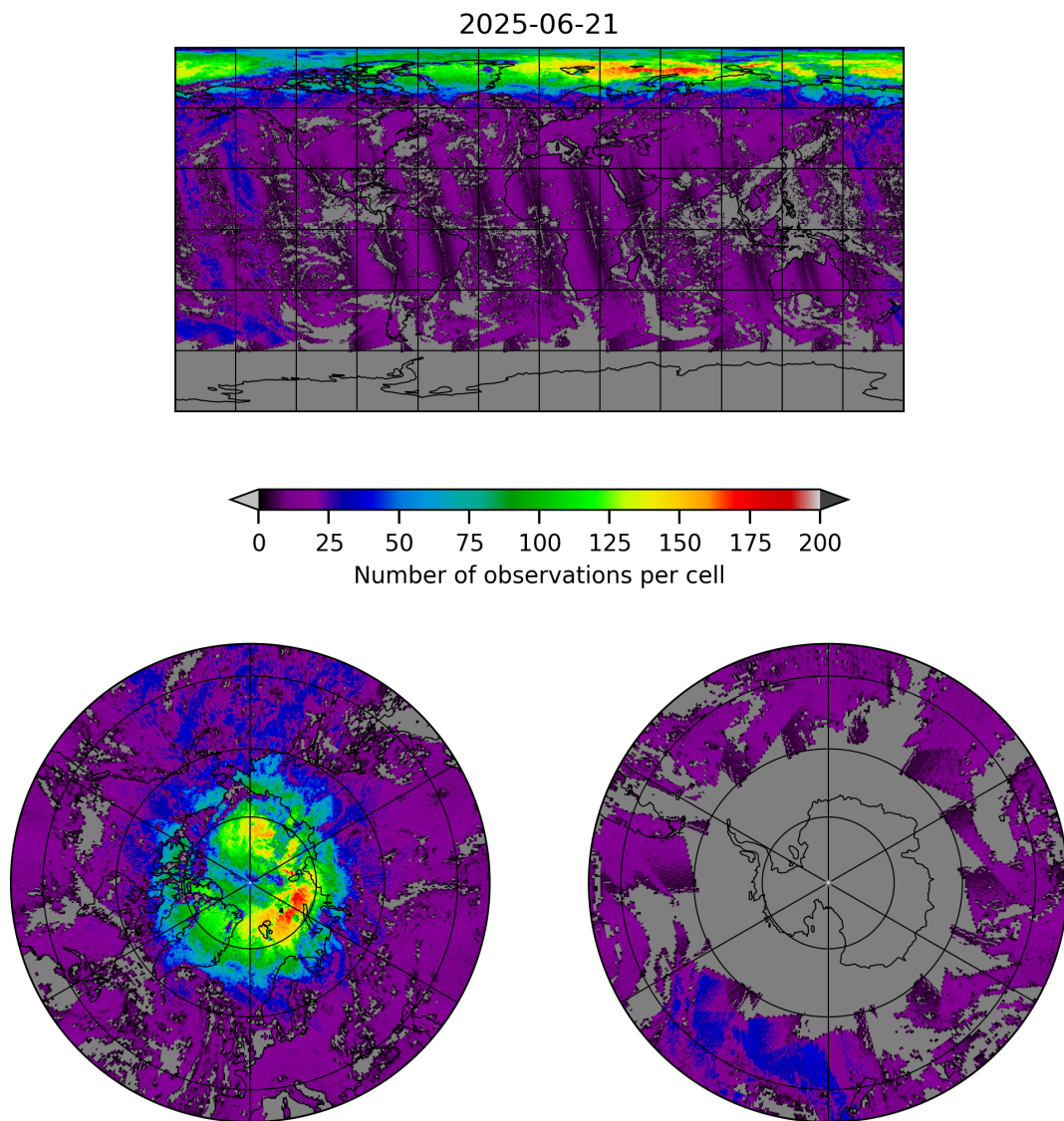
Figure 8: Map of the number of observations for 2025-06-20 to 2025-06-22
