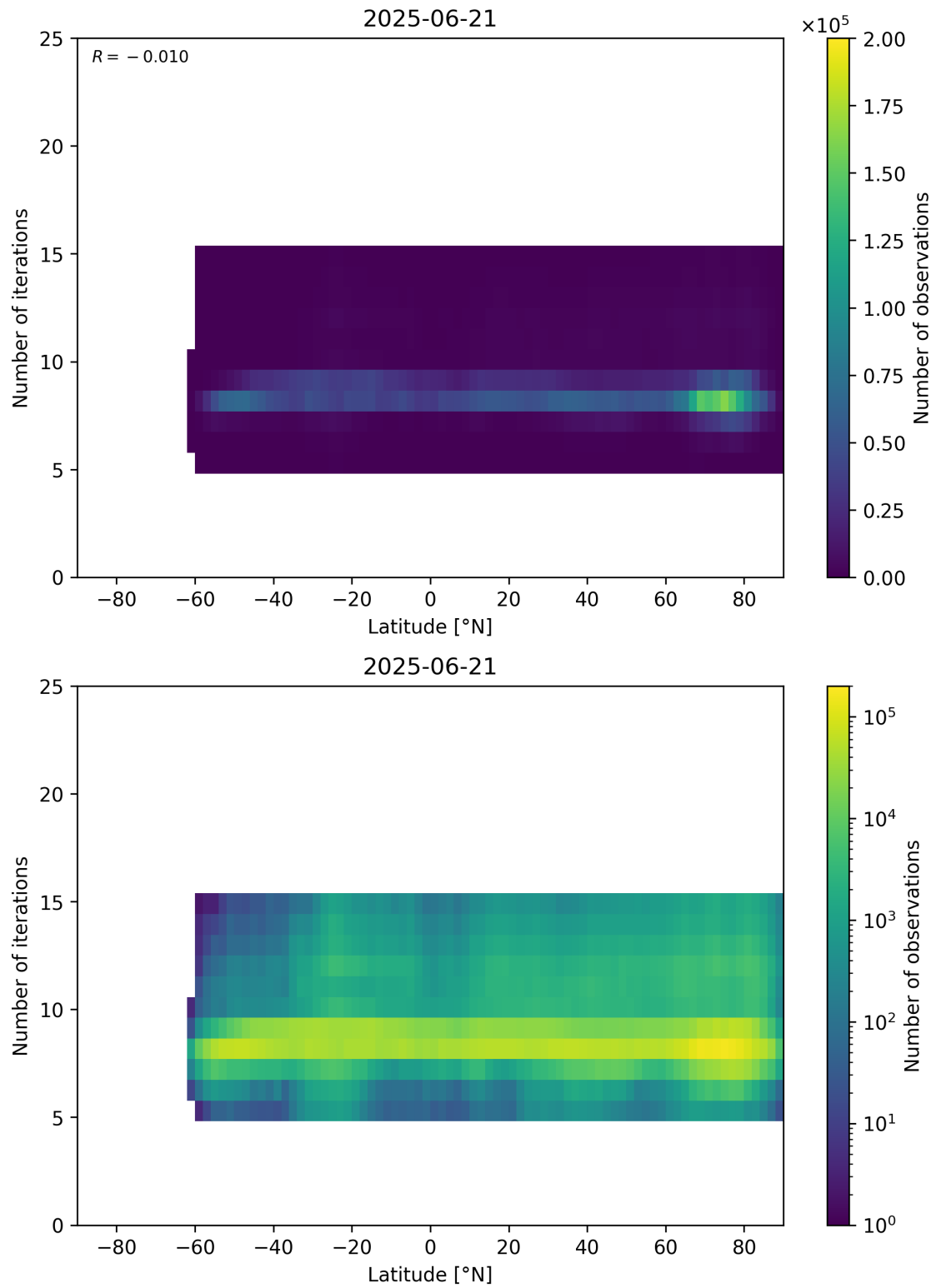
Figure 56: Scatter density plot of “Latitude” against “Number of iterations” for 2025-06-20 to 2025-06-22.
