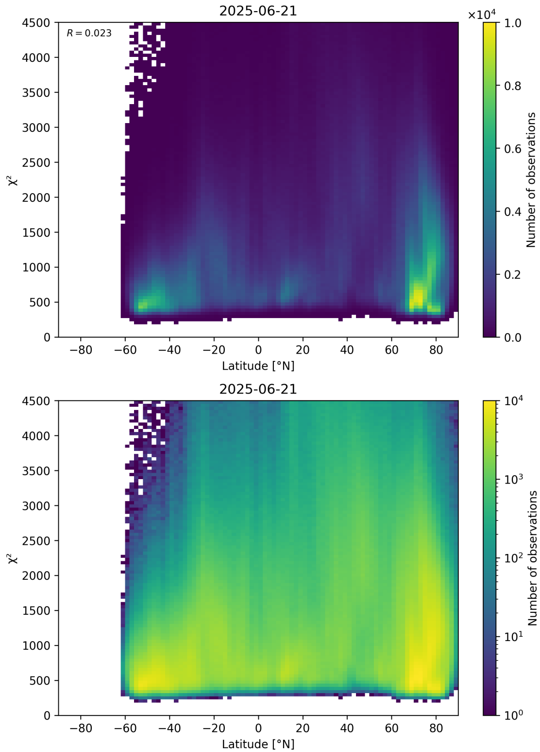
Figure 54: Scatter density plot of “Latitude” against “ \chi^2 ” for 2025-06-20 to 2025-06-22.
