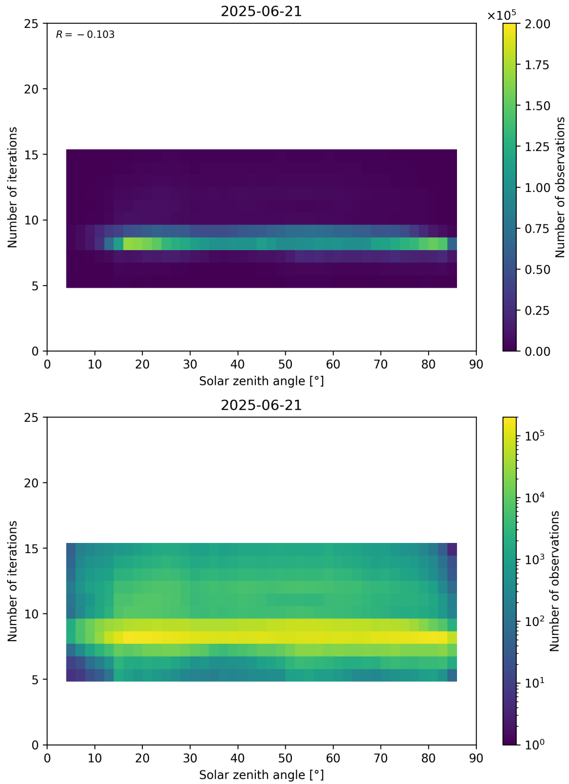
Figure 67: Scatter density plot of “Solar zenith angle” against “Number of iterations” for 2025-06-20 to 2025-06-22.
