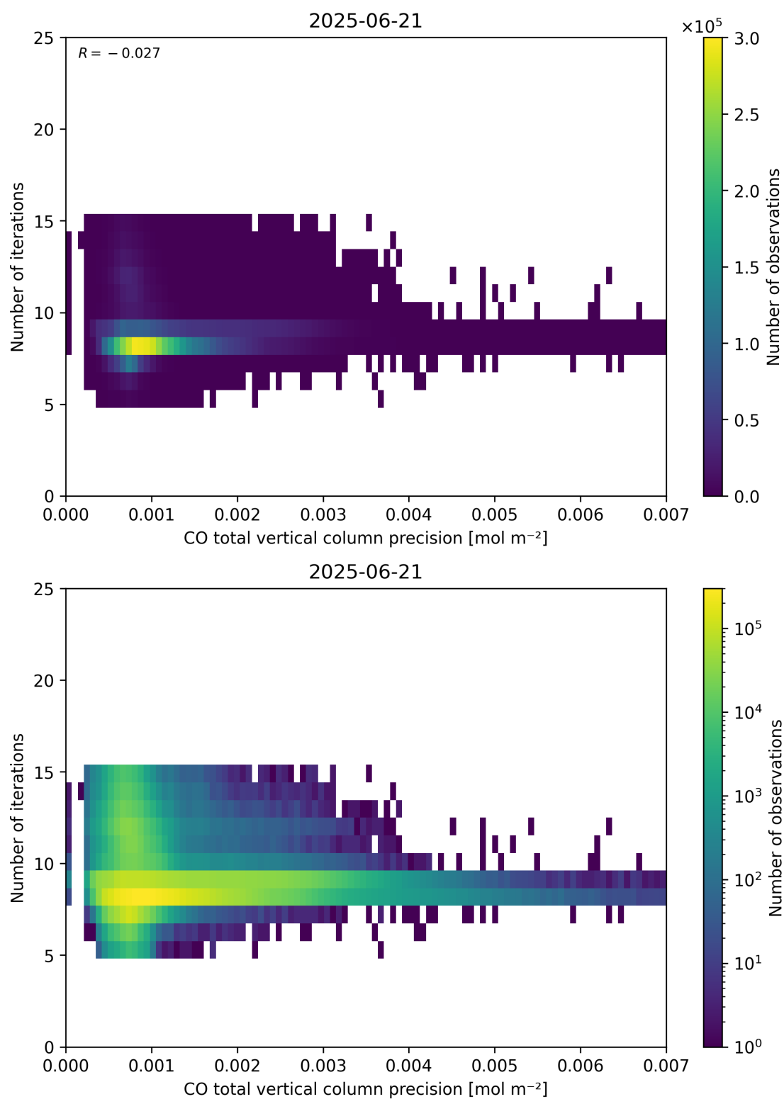
Figure 46: Scatter density plot of “CO total vertical column precision” against “Number of iterations” for 2025-06-20 to 2025-06-22.
