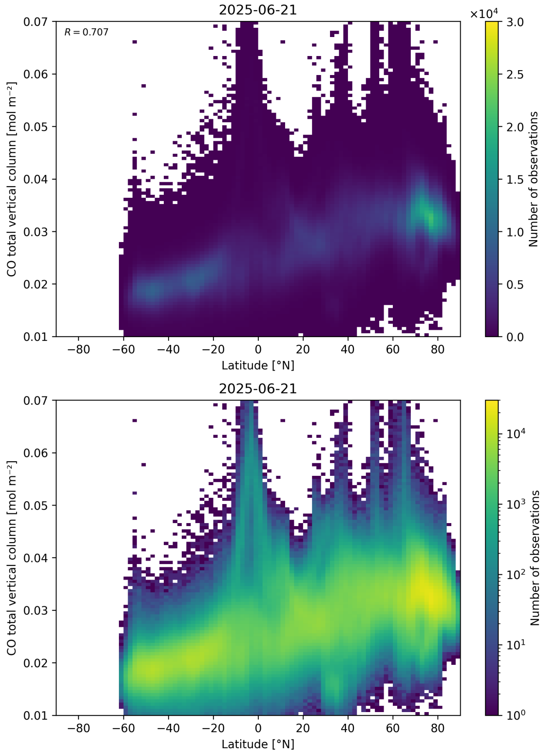
Figure 51: Scatter density plot of “Latitude” against “CO total vertical column” for 2025-06-20 to 2025-06-22.
