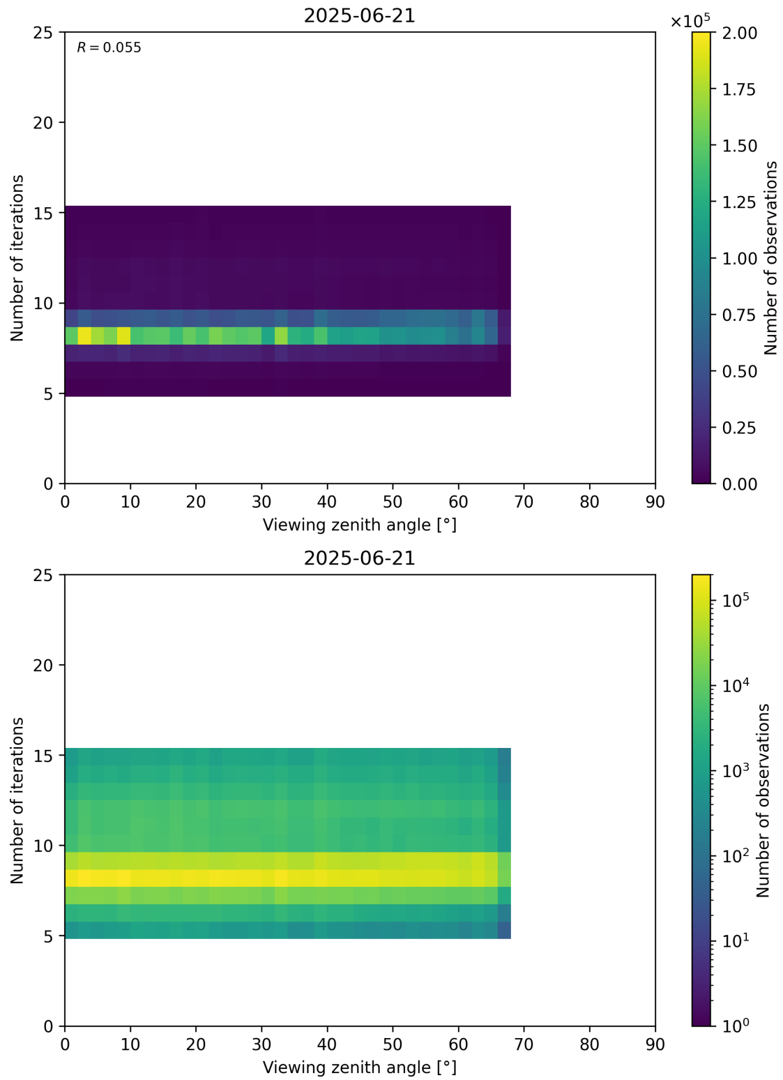
Figure 75: Scatter density plot of “Viewing zenith angle” against “Number of iterations” for 2025-06-20 to 2025-06-22.
