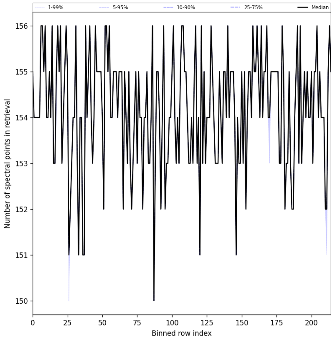
Figure 29: Along track statistics of “Number of spectral points in retrieval” for 2025-06-20 to 2025-06-22
