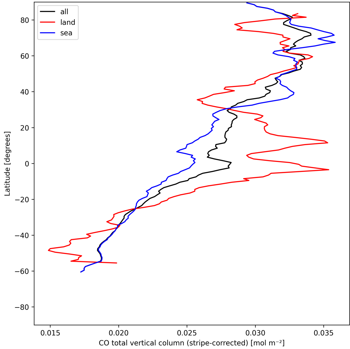
Figure 11: Zonal average of “CO total vertical column (stripe-corrected)” for 2025-06-20 to 2025-06-22.
