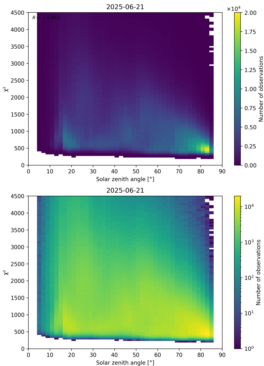
Figure 64: Scatter density plot of “Solar zenith angle” against “ \chi^2 ” for 2025-06-20 to 2025-06-22.
