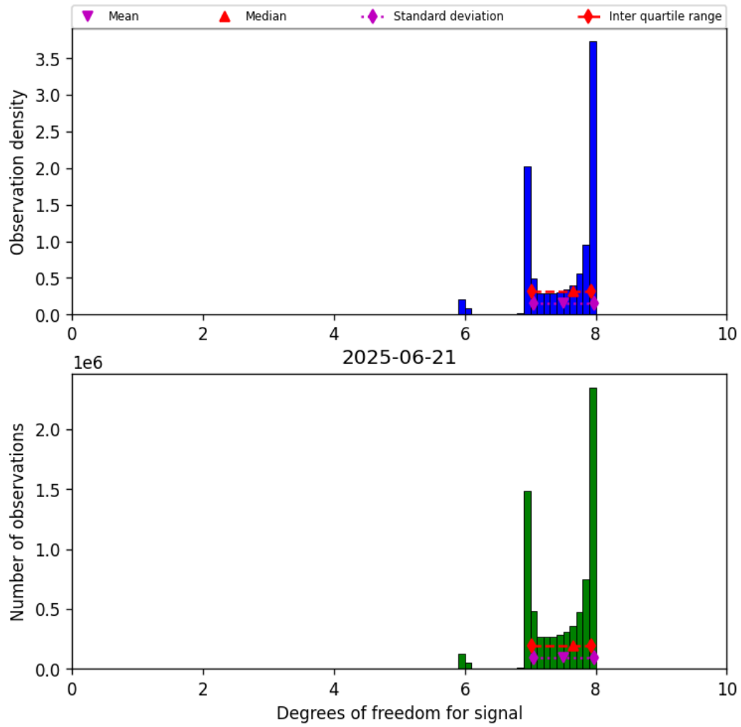
Figure 23: Histogram of “Degrees of freedom for signal” for 2025-06-20 to 2025-06-22
