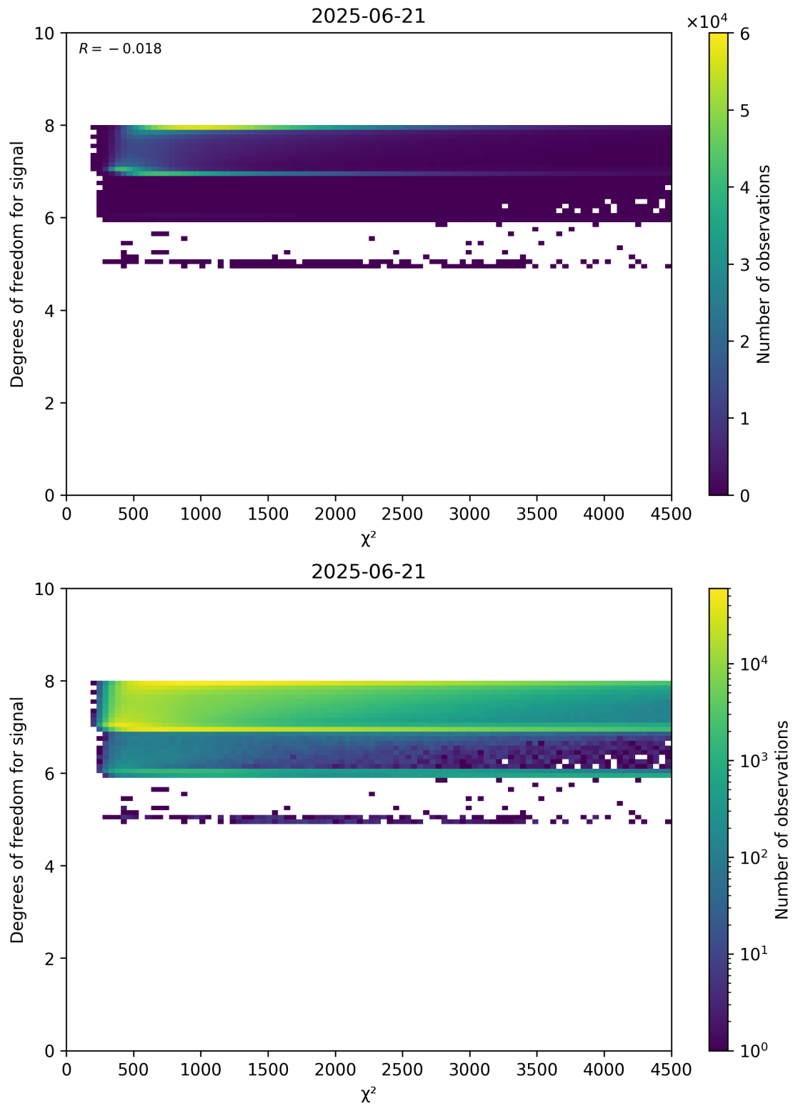
Figure 48: Scatter density plot of “ \chi^2 ” against “Degrees of freedom for signal” for 2025-06-20 to 2025-06-22.
