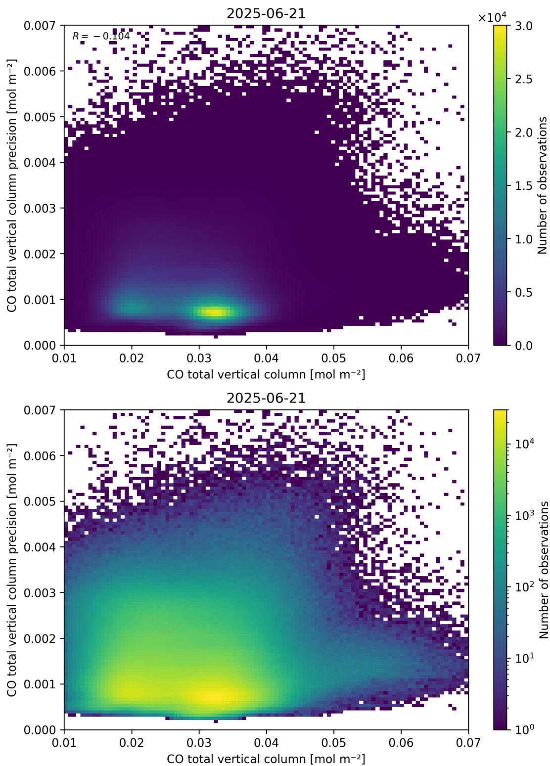
Figure 34: Scatter density plot of “CO total vertical column” against “CO total vertical column precision” for 2025-06-20 to 2025-06-22.
