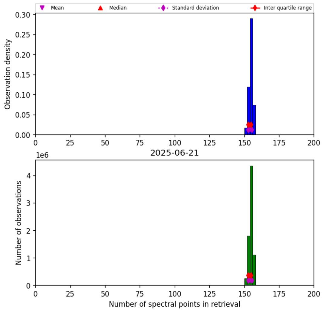
Figure 21: Histogram of “Number of spectral points in retrieval” for 2025-06-20 to 2025-06-22
