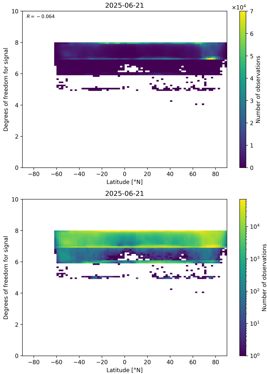
Figure 55: Scatter density plot of “Latitude” against “Degrees of freedom for signal” for 2025-06-20 to 2025-06-22.
