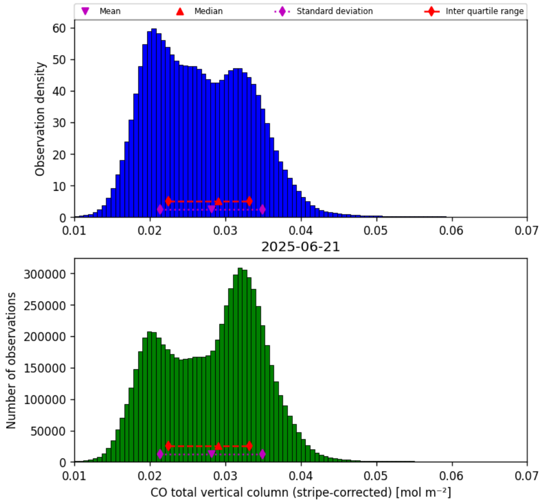
Figure 19: Histogram of “CO total vertical column (stripe-corrected)” for 2025-06-20 to 2025-06-22
