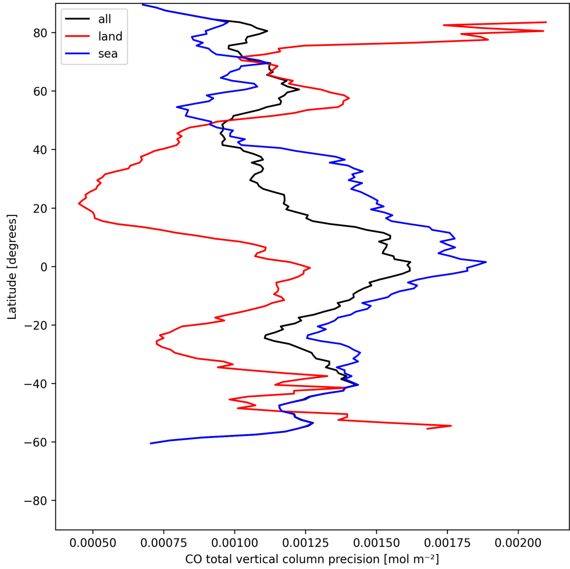
Figure 12: Zonal average of “CO total vertical column precision” for 2025-06-20 to 2025-06-22.
