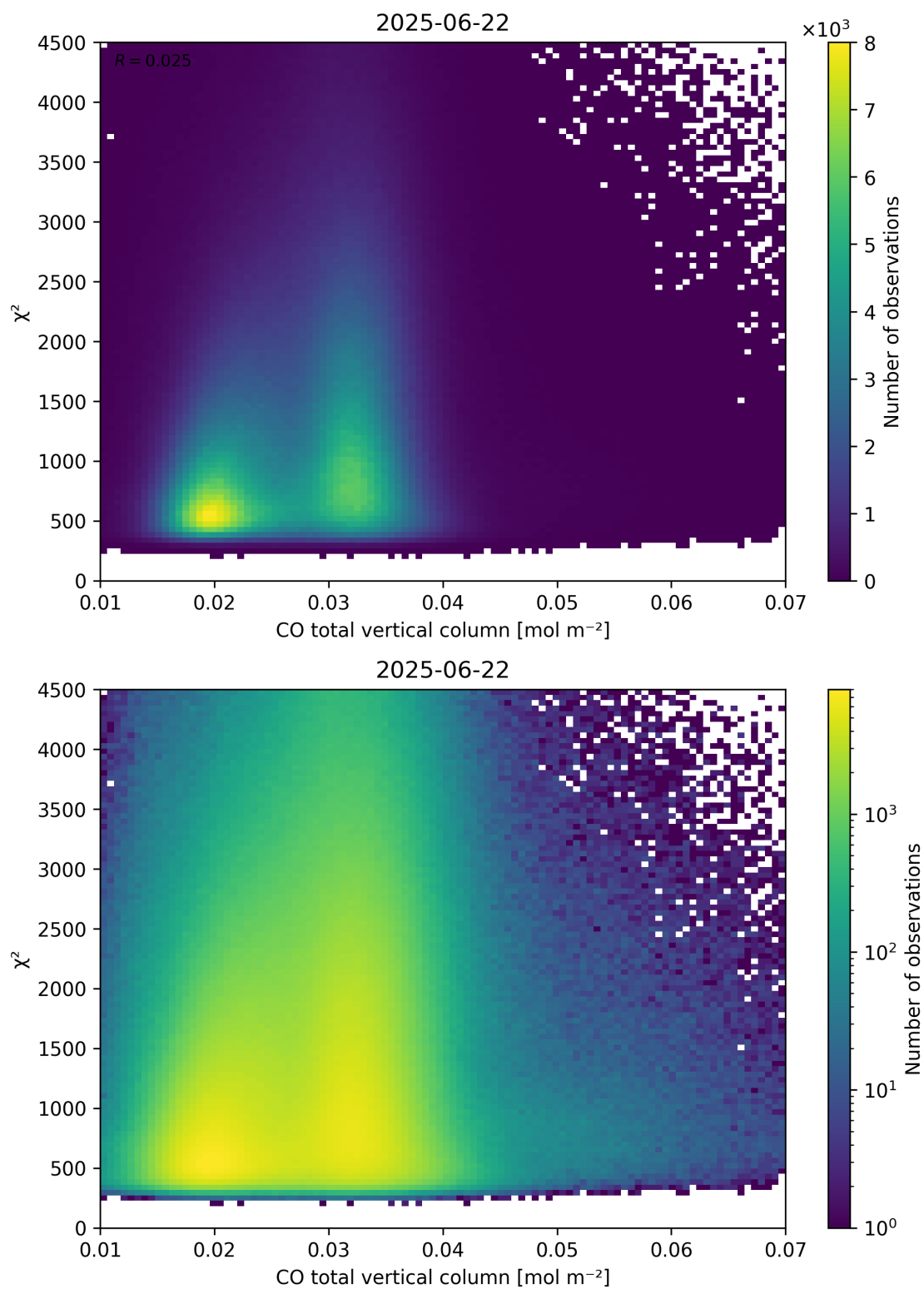
Figure 35: Scatter density plot of “CO total vertical column” against “ \chi^2 ” for 2025-06-22 to 2025-06-23.
