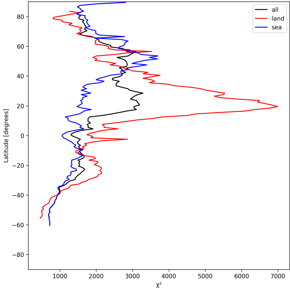
Figure 14: Zonal average of “ \chi^2 ” for 2025-06-22 to 2025-06-23.
