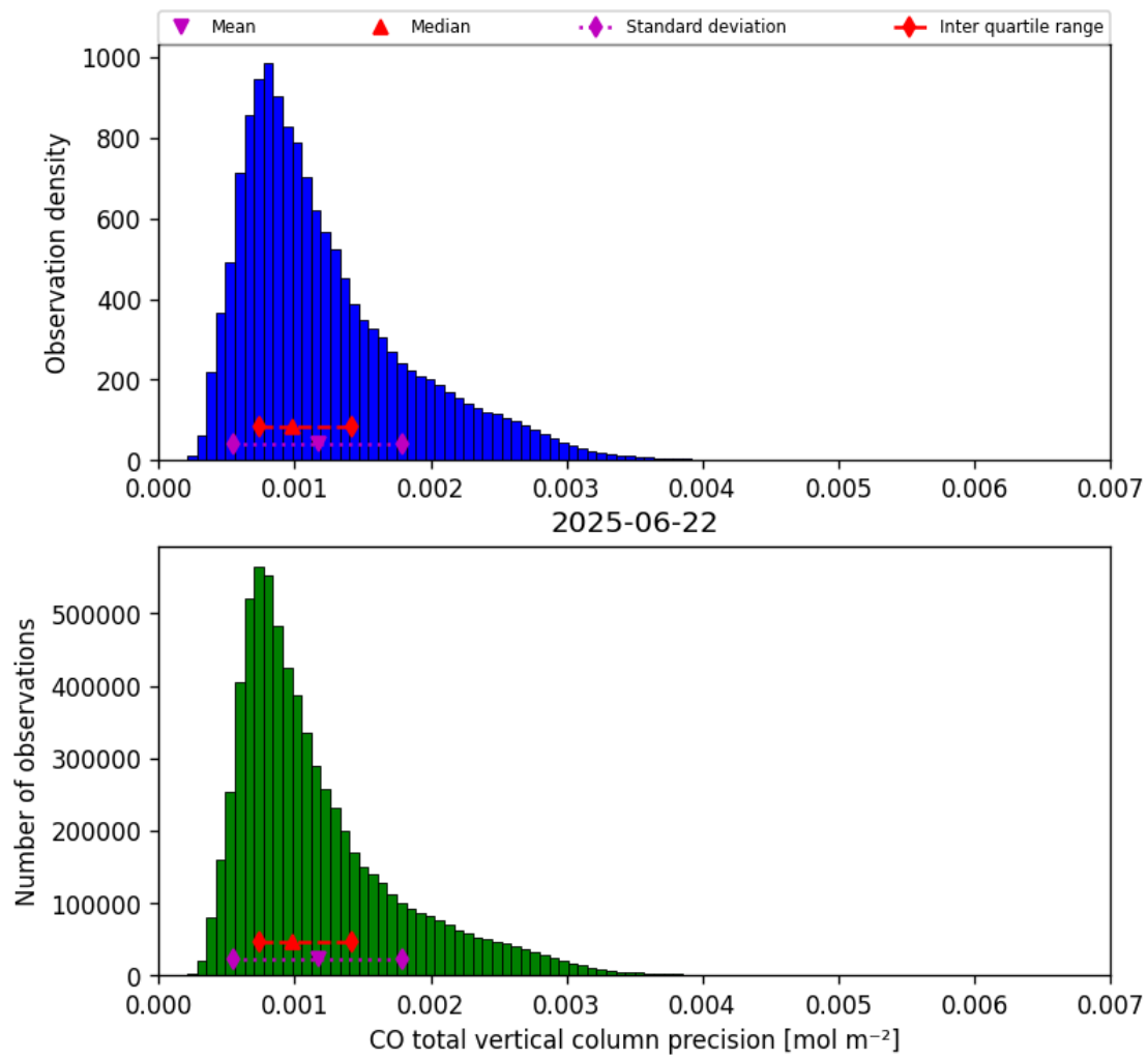
Figure 20: Histogram of “CO total vertical column precision” for 2025-06-22 to 2025-06-23
