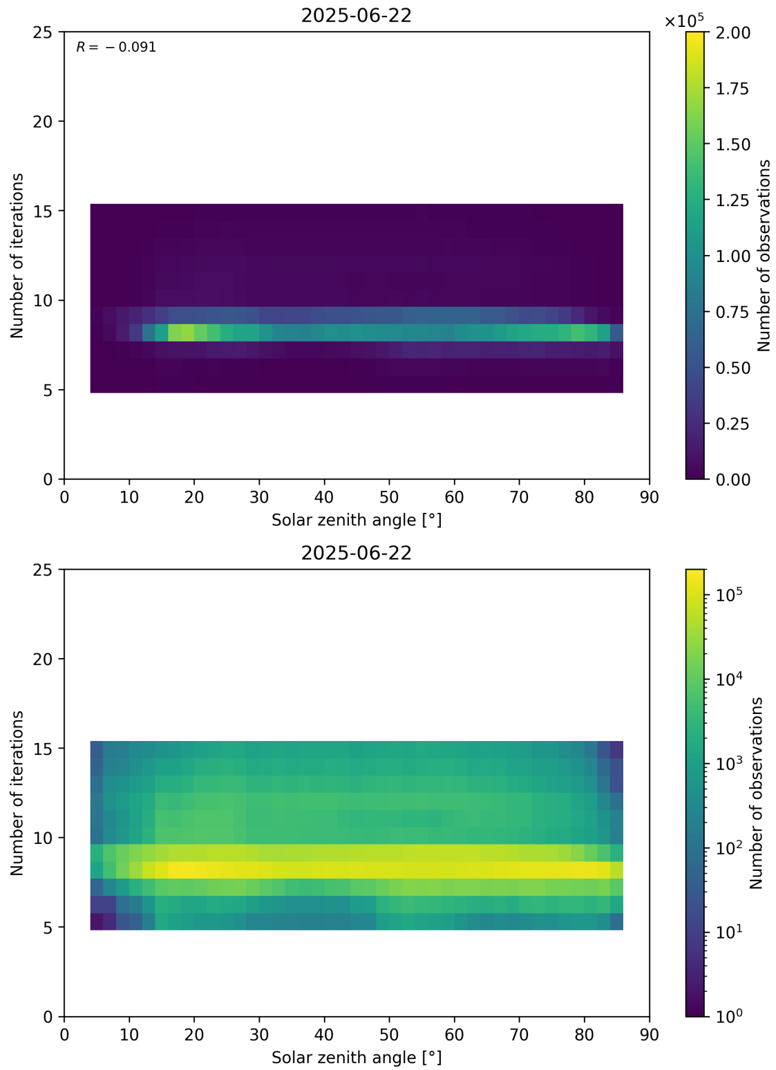
Figure 67: Scatter density plot of “Solar zenith angle” against “Number of iterations” for 2025-06-22 to 2025-06-23.
