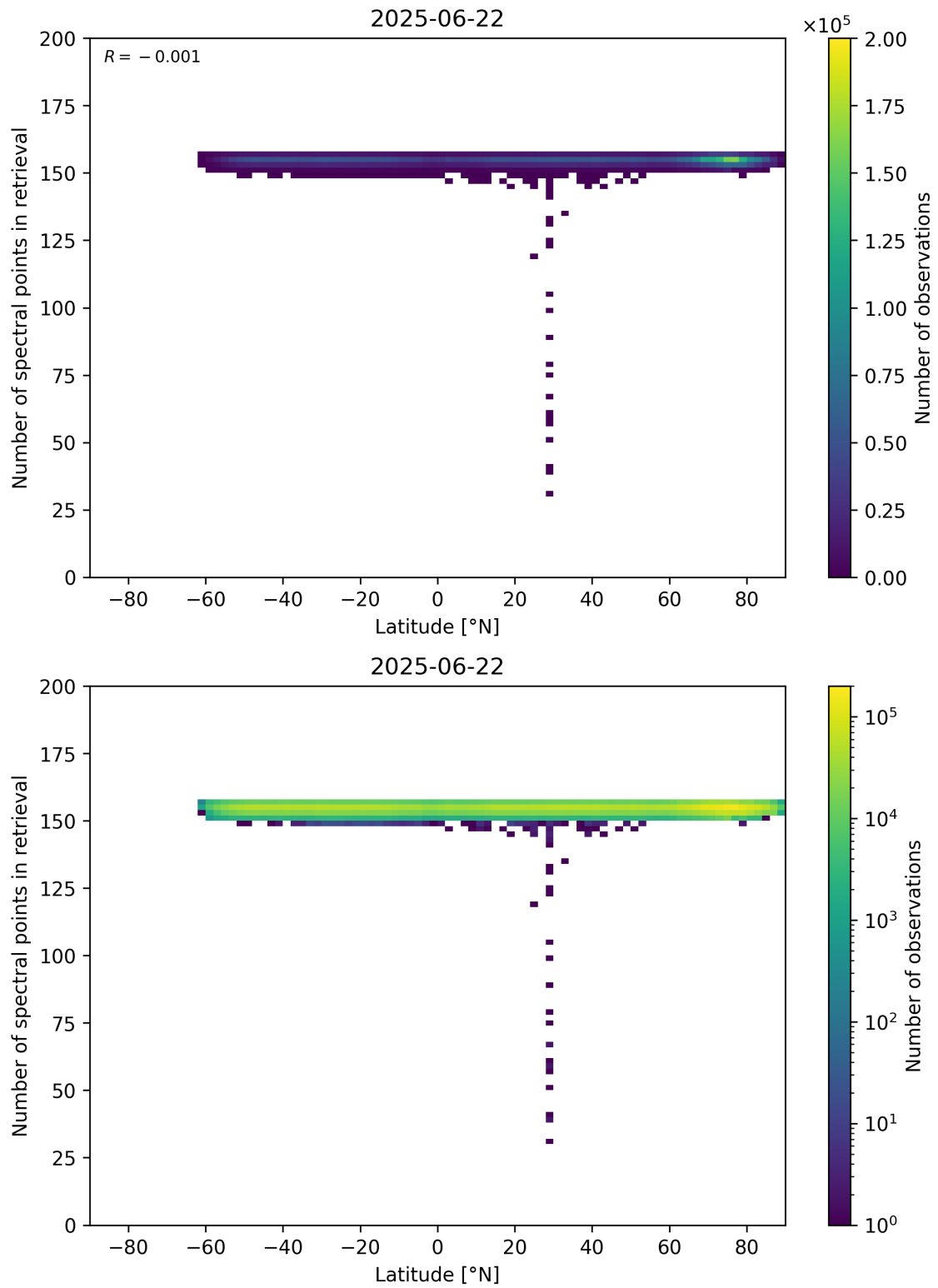
Figure 57: Scatter density plot of “Latitude” against “Number of spectral points in retrieval” for 2025-06-22 to 2025-06-23.
