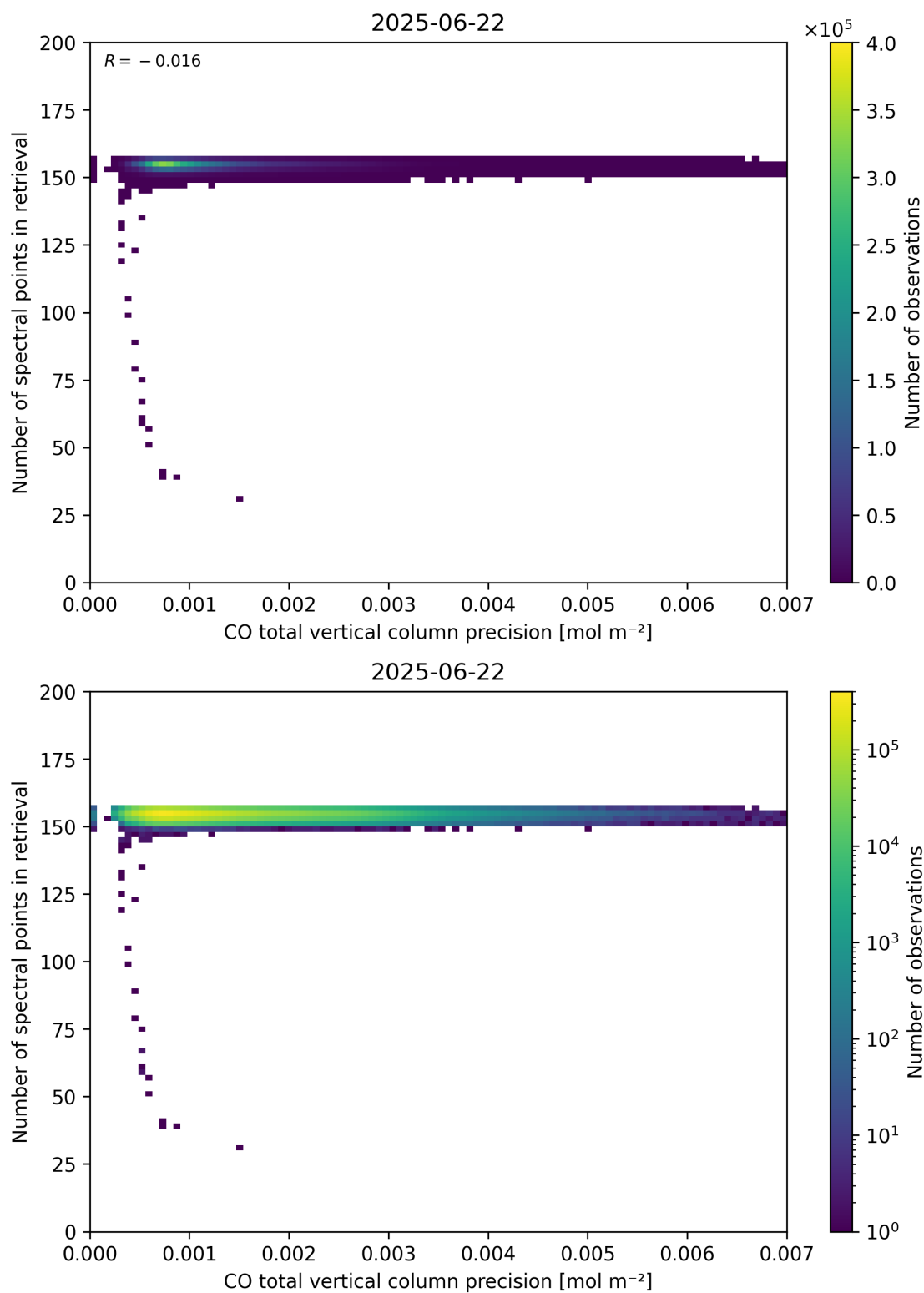
Figure 47: Scatter density plot of “CO total vertical column precision” against “Number of spectral points in retrieval” for 2025-06-22 to 2025-06-23.
