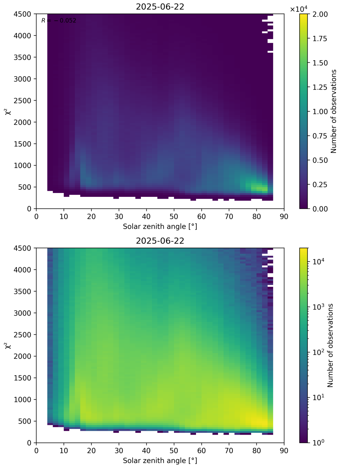
Figure 64: Scatter density plot of “Solar zenith angle” against “ \chi^2 ” for 2025-06-22 to 2025-06-23.
