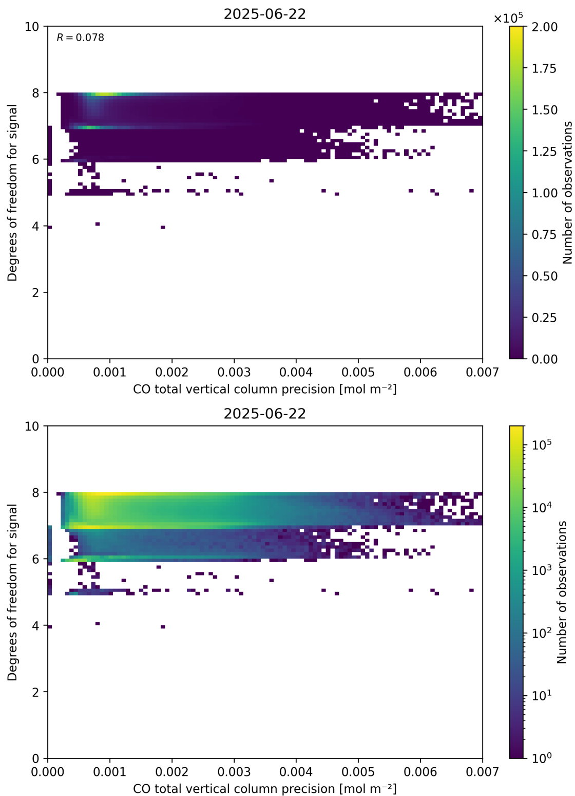
Figure 45: Scatter density plot of “CO total vertical column precision” against “Degrees of freedom for signal” for 2025-06-22 to 2025-06-23.
