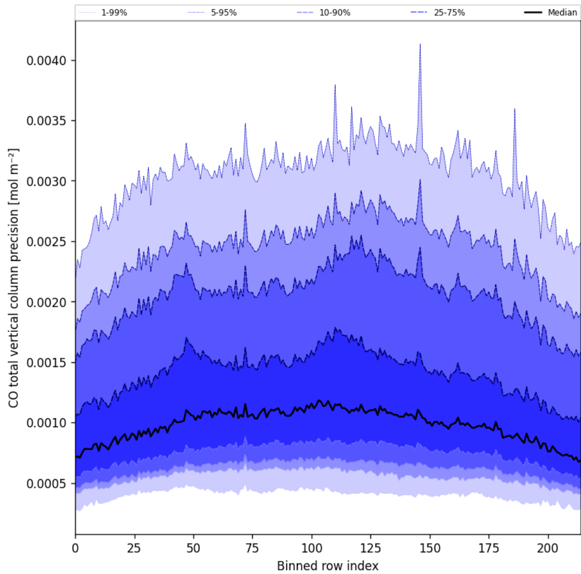
Figure 28: Along track statistics of “CO total vertical column precision” for 2025-06-22 to 2025-06-23
