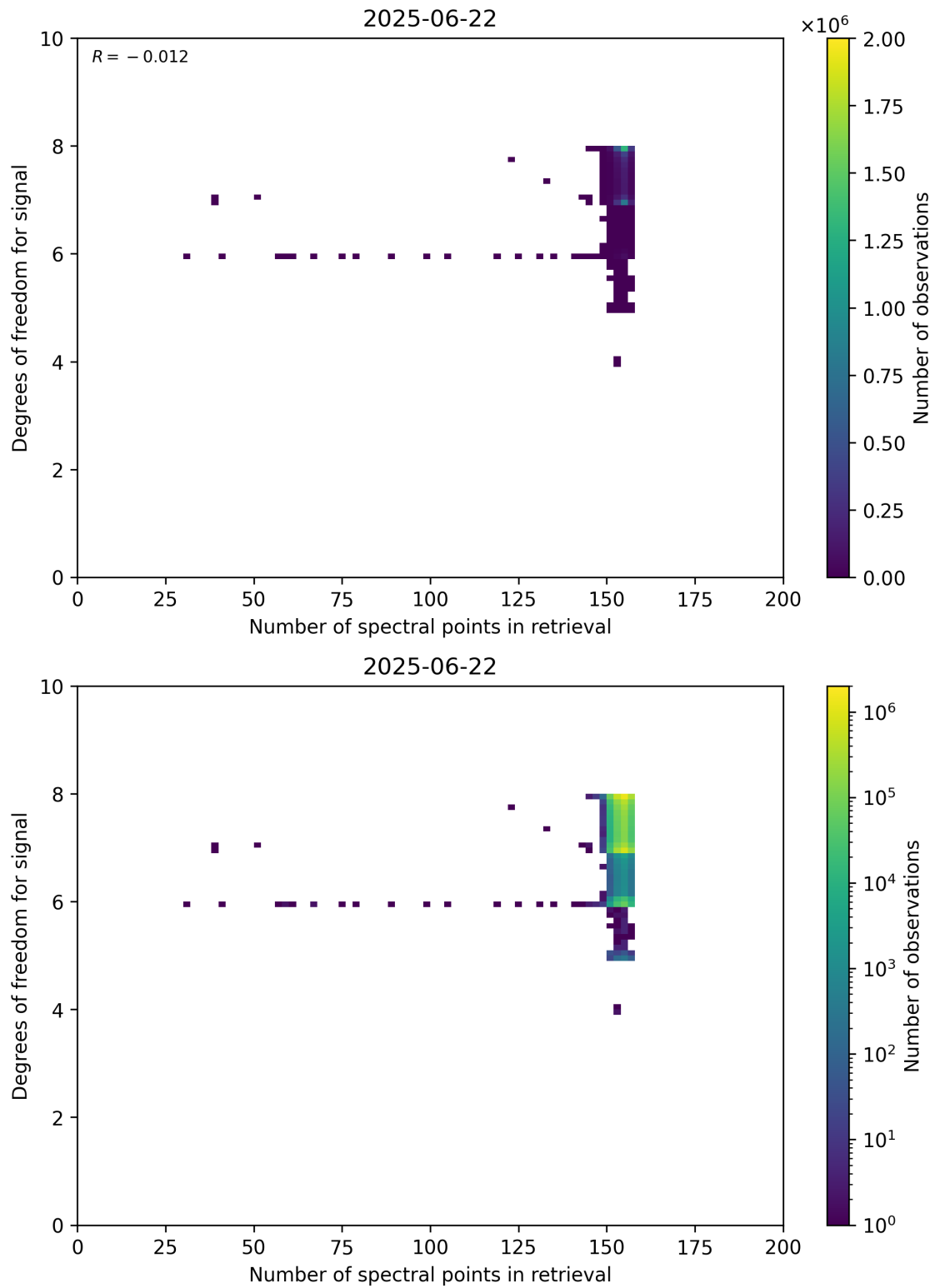
Figure 59: Scatter density plot of “Number of spectral points in retrieval” against “Degrees of freedom for signal” for 2025-06-22 to 2025-06-23.
