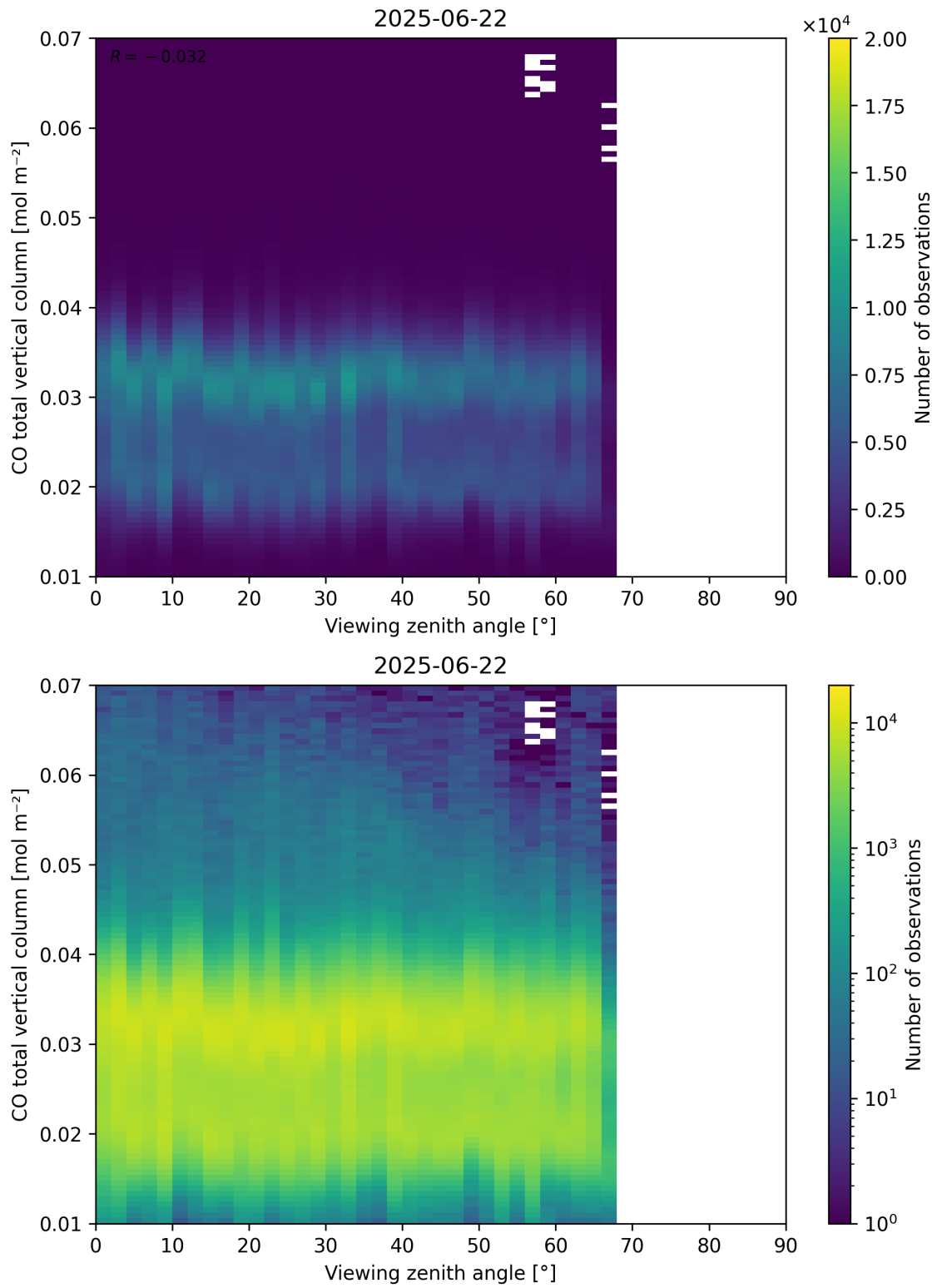
Figure 69: Scatter density plot of “Viewing zenith angle” against “CO total vertical column” for 2025-06-22 to 2025-06-23.
