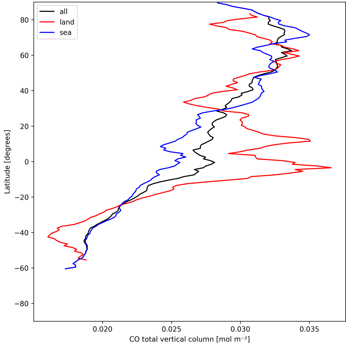
Figure 10: Zonal average of “CO total vertical column” for 2025-06-22 to 2025-06-23.
