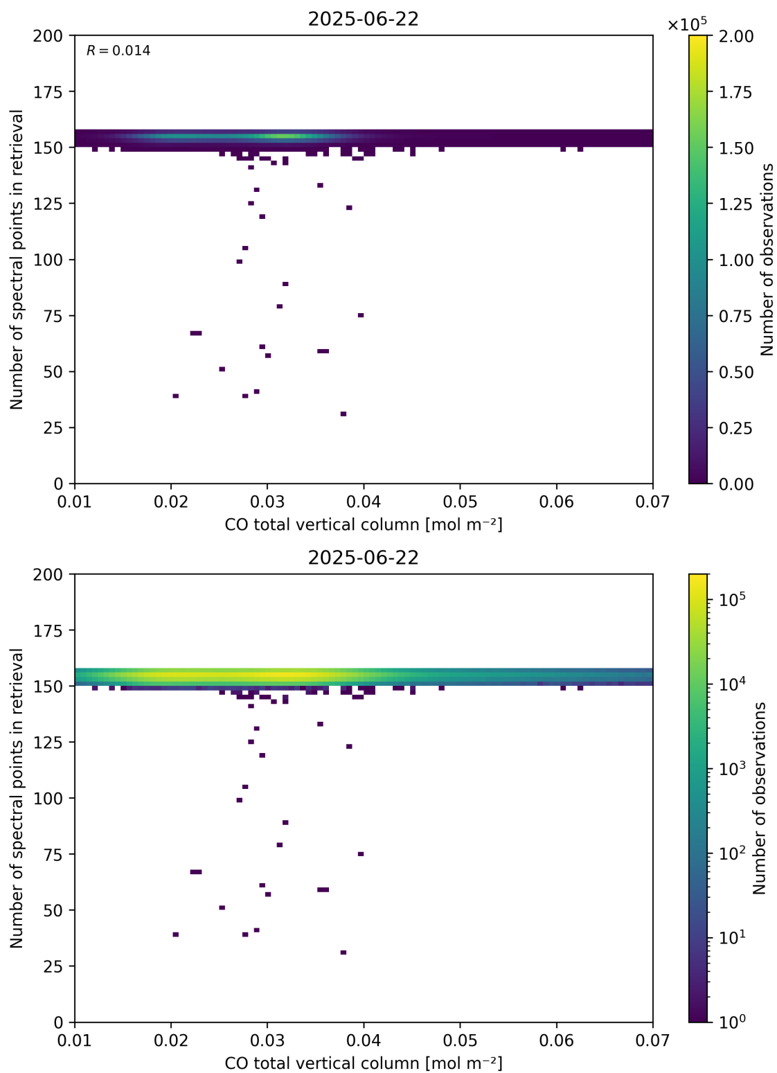
Figure 43: Scatter density plot of “CO total vertical column” against “Number of spectral points in retrieval” for 2025-06-22 to 2025-06-23.
