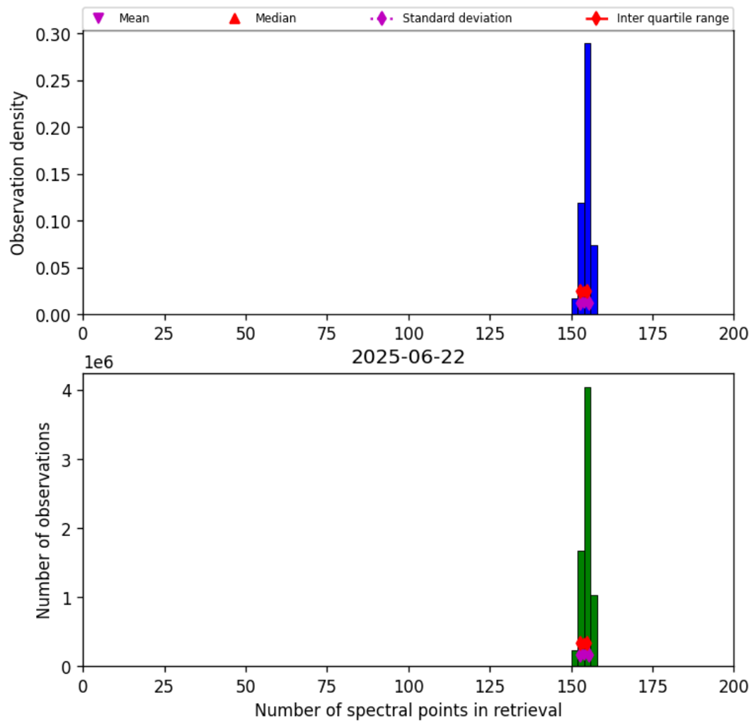
Figure 21: Histogram of “Number of spectral points in retrieval” for 2025-06-22 to 2025-06-23
