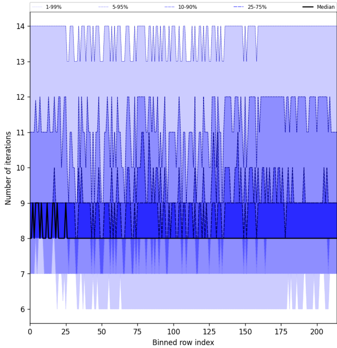
Figure 32: Along track statistics of “Number of iterations” for 2025-06-22 to 2025-06-23
