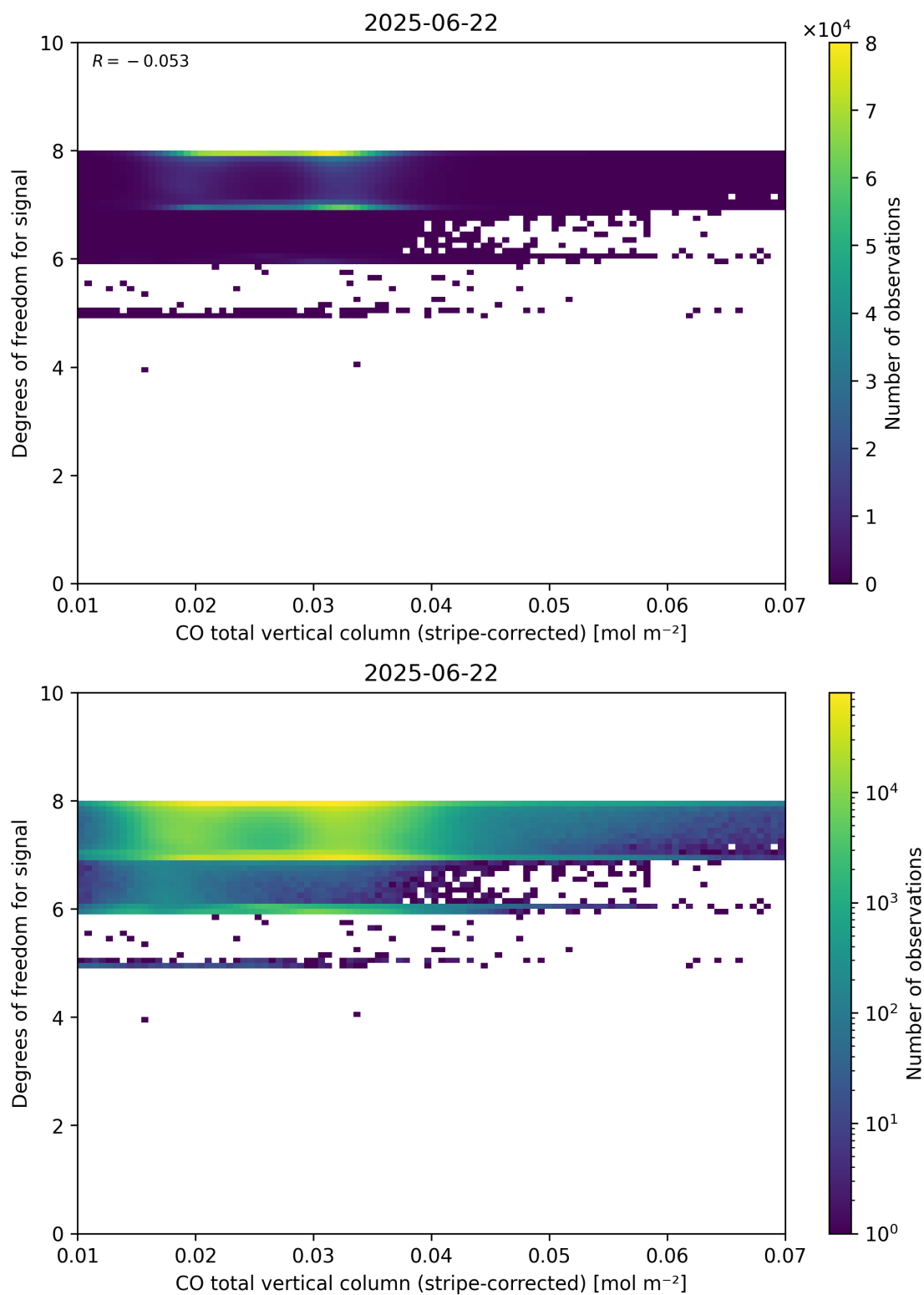
Figure 38: Scatter density plot of “CO total vertical column (stripe-corrected)” against “Degrees of freedom for signal” for 2025-06-22 to 2025-06-23.
