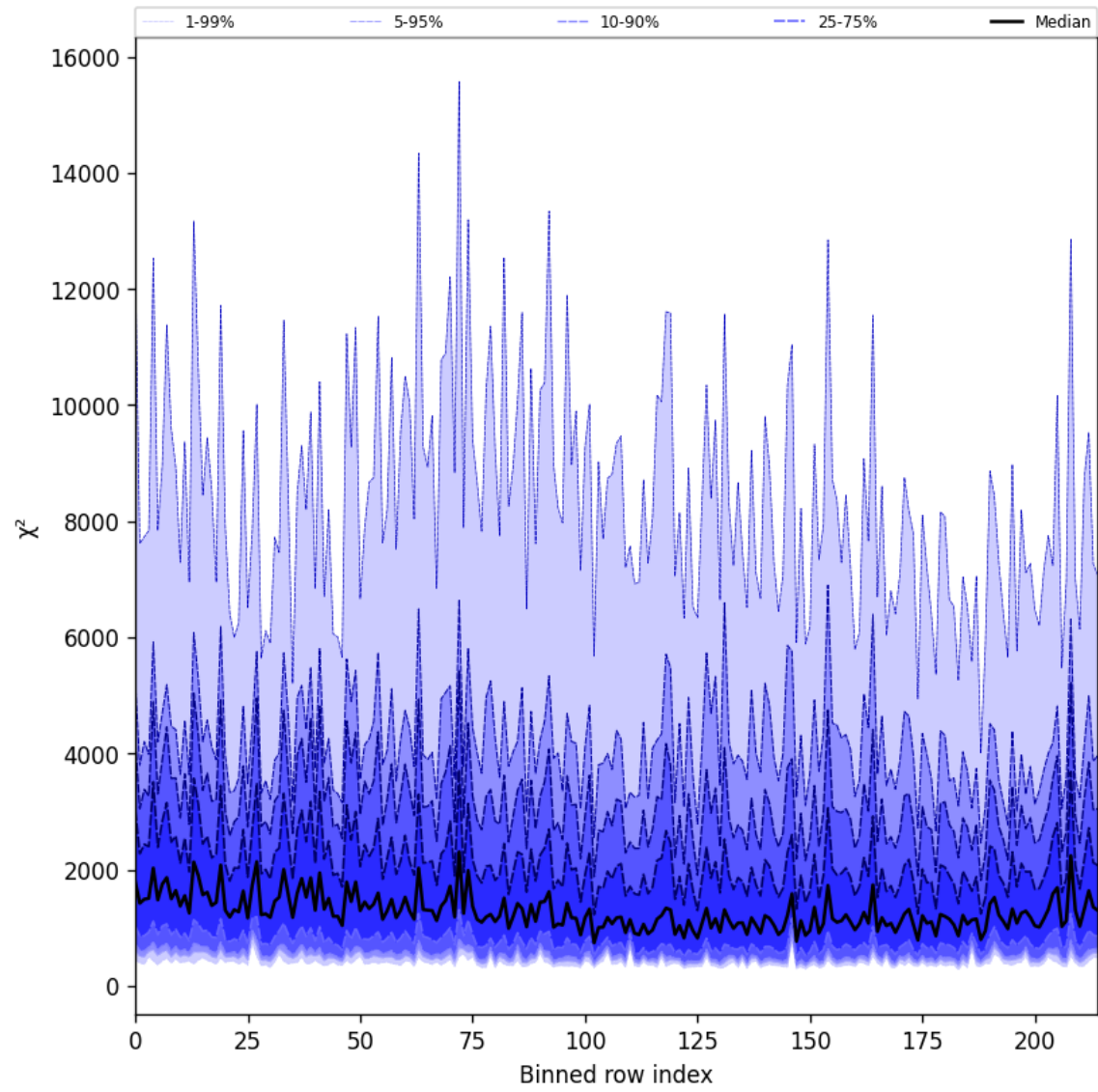
Figure 30: Along track statistics of “ \chi^2 ” for 2025-06-22 to 2025-06-23
