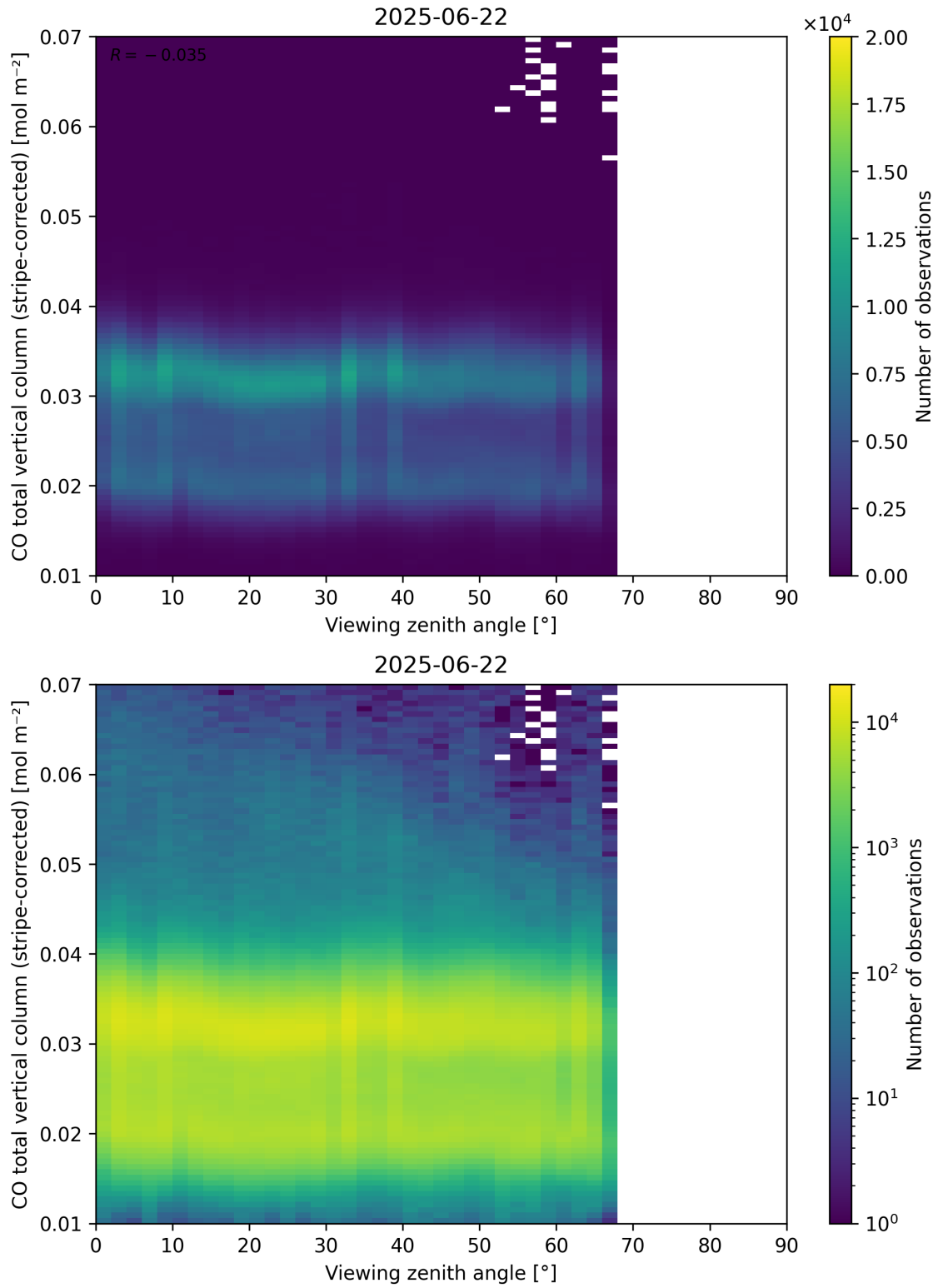
Figure 70: Scatter density plot of “Viewing zenith angle” against “CO total vertical column (stripe-corrected)” for 2025-06-22 to 2025-06-23.
