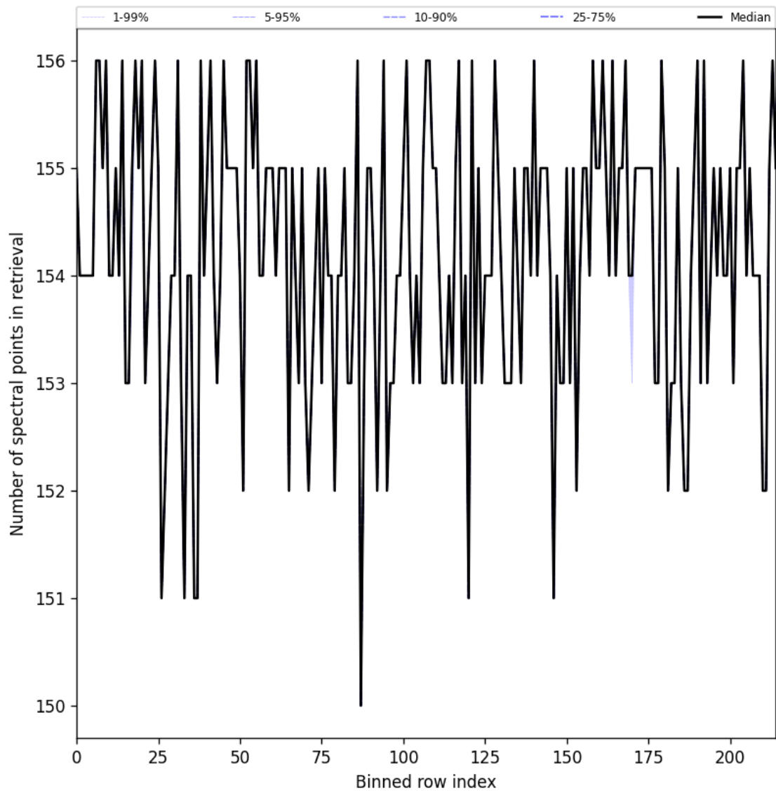
Figure 29: Along track statistics of “Number of spectral points in retrieval” for 2025-06-22 to 2025-06-23
