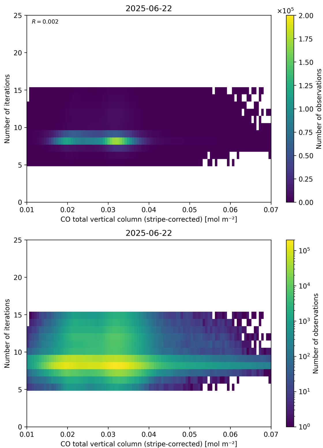
Figure 39: Scatter density plot of “CO total vertical column (stripe-corrected)” against “Number of iterations” for 2025-06-22 to 2025-06-23.
