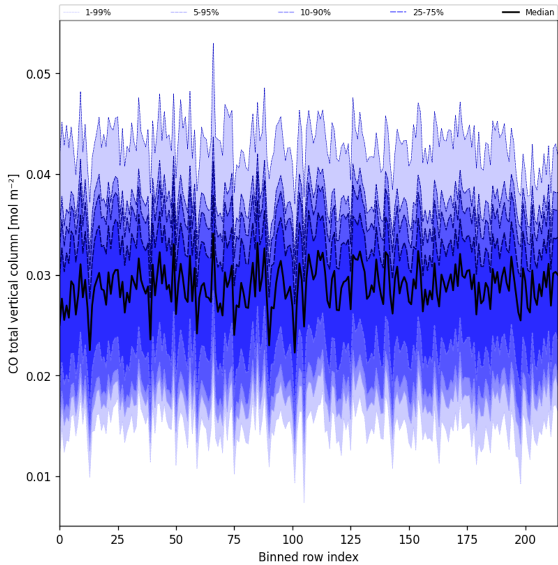
Figure 26: Along track statistics of “CO total vertical column” for 2025-06-22 to 2025-06-23
