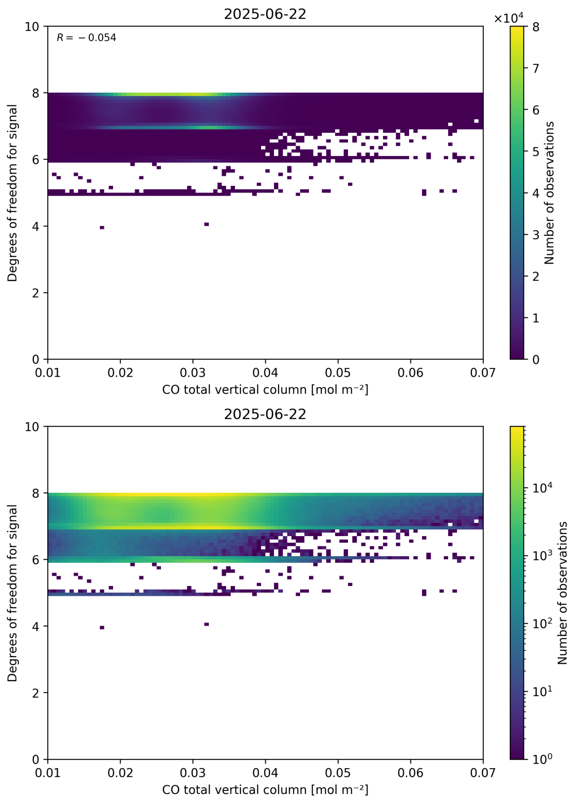
Figure 41: Scatter density plot of “CO total vertical column” against “Degrees of freedom for signal” for 2025-06-22 to 2025-06-23.
