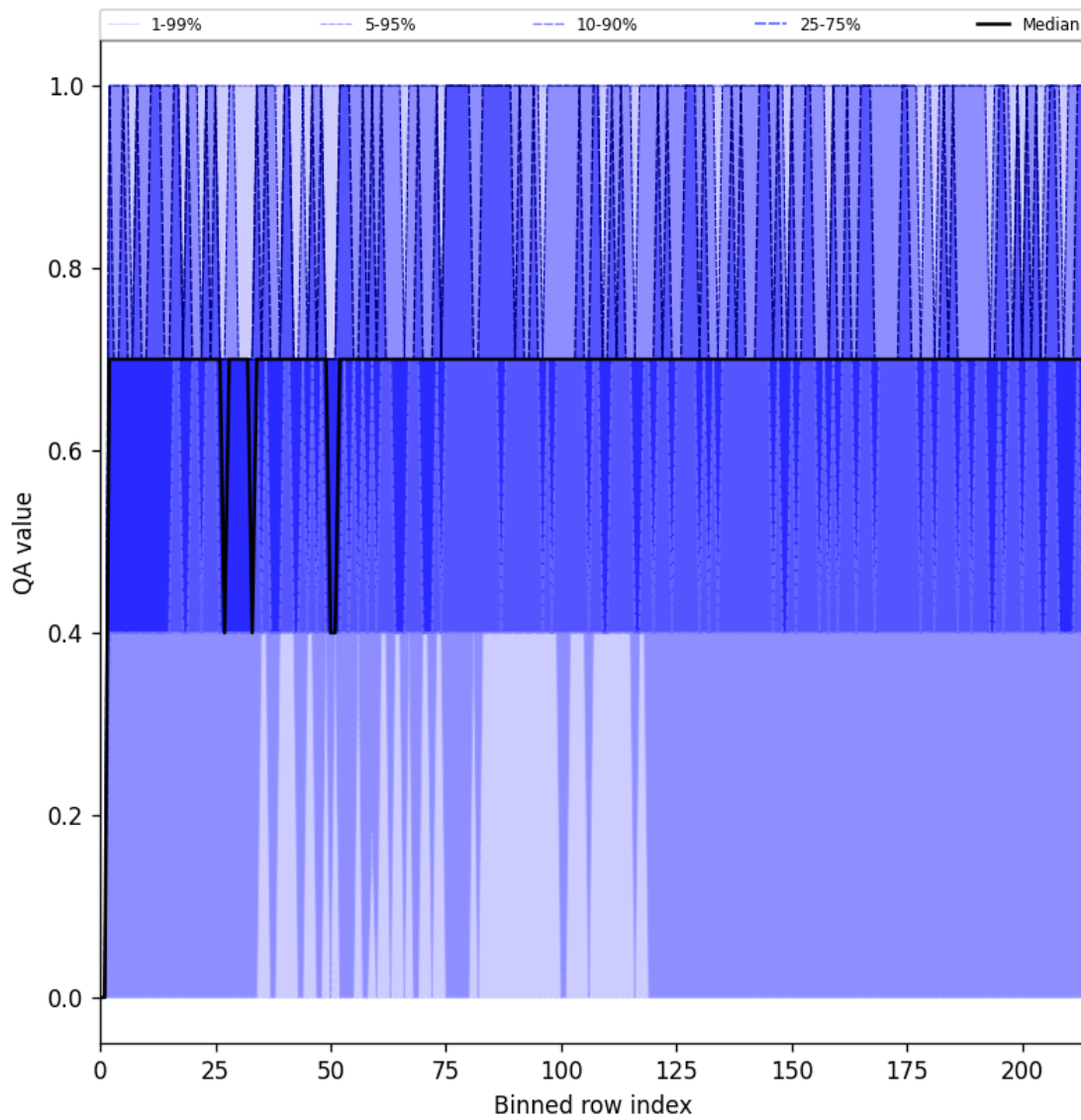
Figure 25: Along track statistics of “QA value” for 2025-06-22 to 2025-06-23
