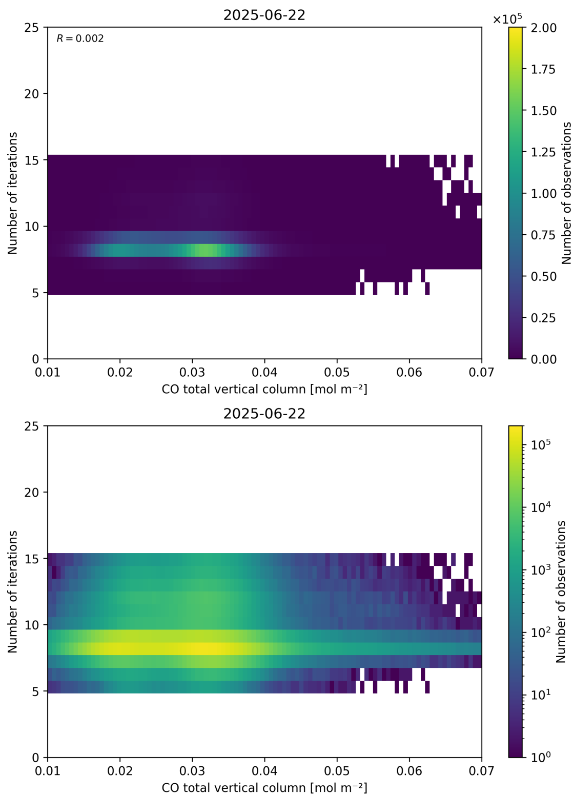
Figure 42: Scatter density plot of “CO total vertical column” against “Number of iterations” for 2025-06-22 to 2025-06-23.
