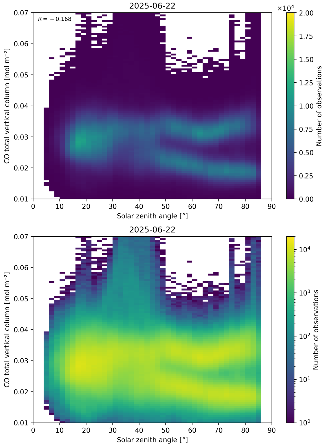
Figure 61: Scatter density plot of “Solar zenith angle” against “CO total vertical column” for 2025-06-22 to 2025-06-23.
