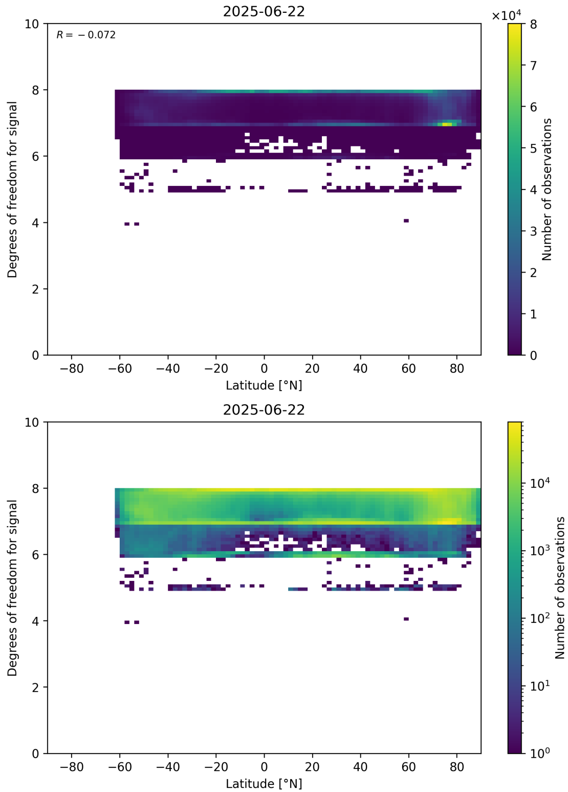
Figure 55: Scatter density plot of “Latitude” against “Degrees of freedom for signal” for 2025-06-22 to 2025-06-23.
