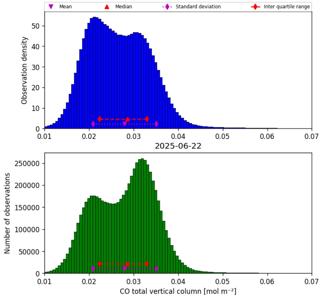
Figure 18: Histogram of “CO total vertical column” for 2025-06-22 to 2025-06-23
