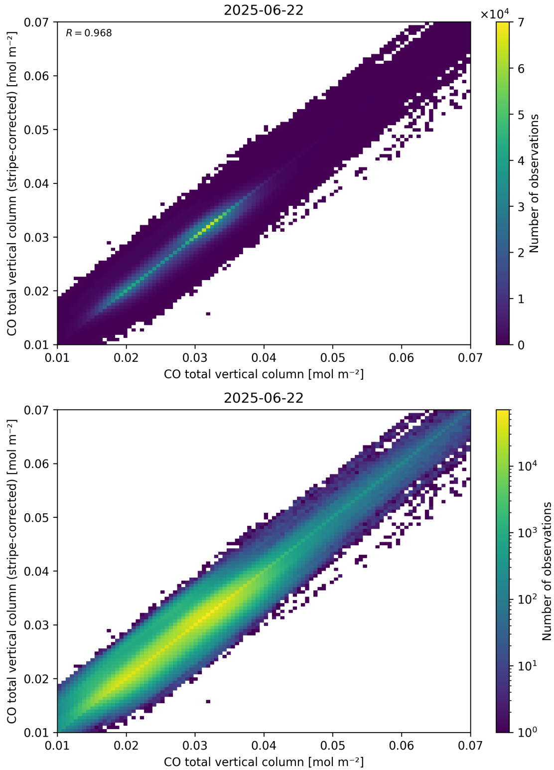
Figure 33: Scatter density plot of “CO total vertical column” against “CO total vertical column (stripe-corrected)” for 2025-06-22 to 2025-06-23.
