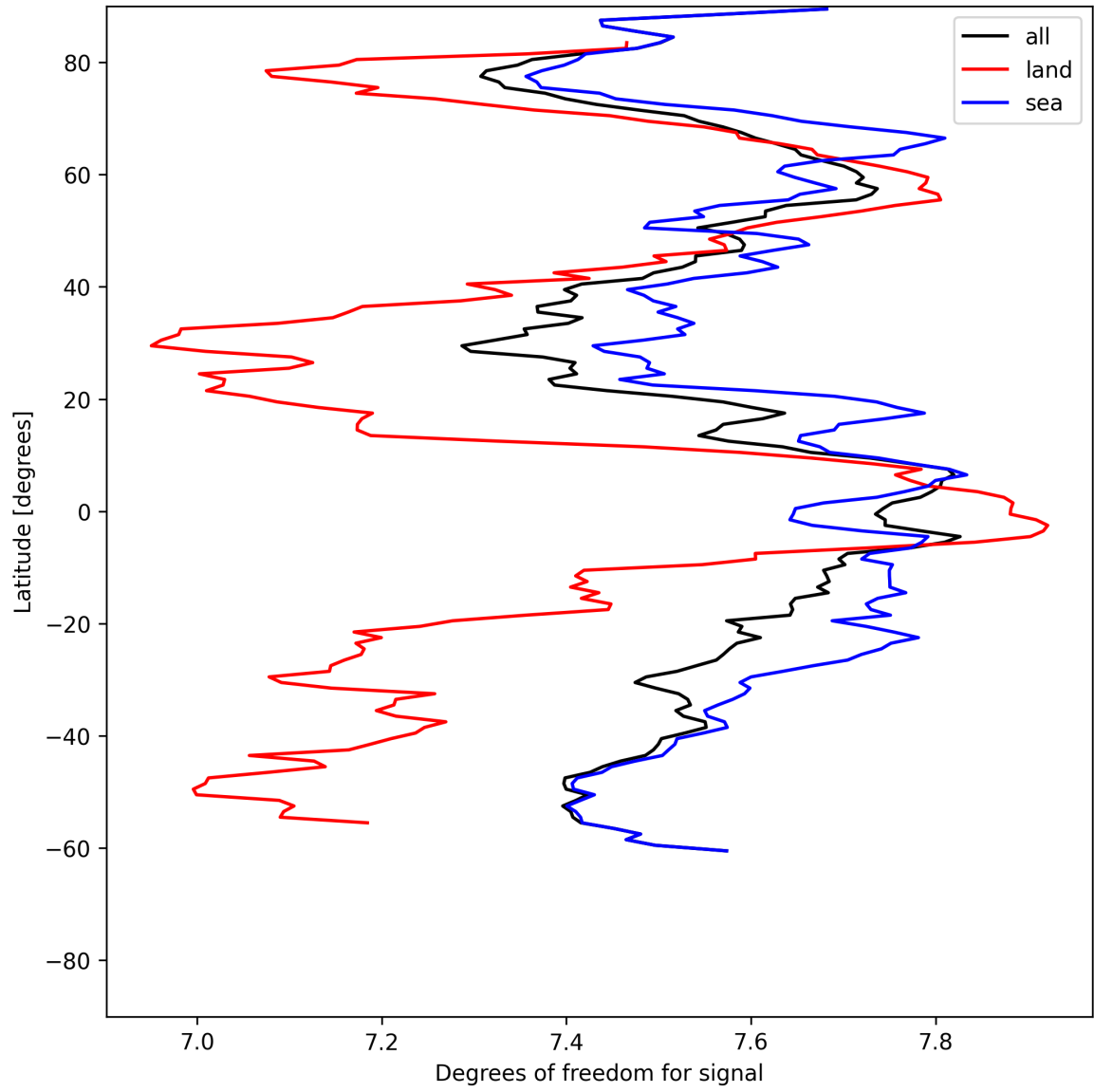
Figure 15: Zonal average of “Degrees of freedom for signal” for 2025-06-22 to 2025-06-23.
