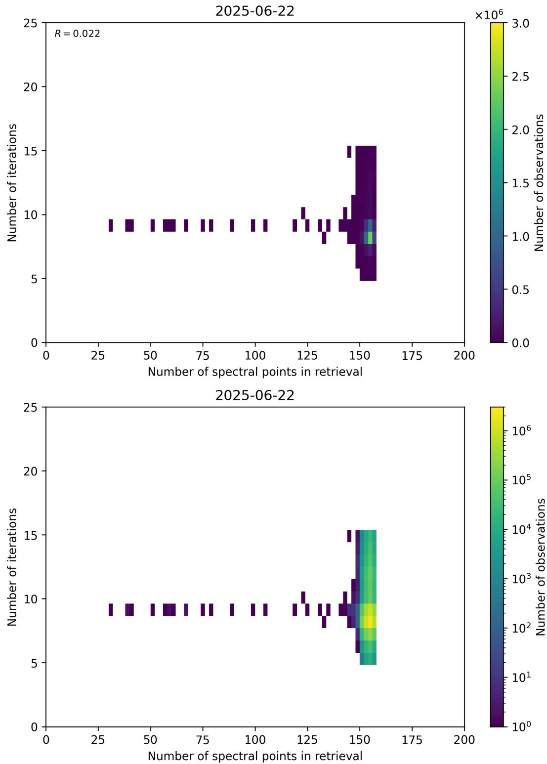
Figure 60: Scatter density plot of “Number of spectral points in retrieval” against “Number of iterations” for 2025-06-22 to 2025-06-23.
