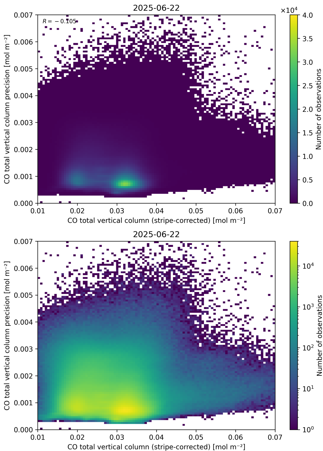
Figure 36: Scatter density plot of “CO total vertical column (stripe-corrected)” against “CO total vertical column precision” for 2025-06-22 to 2025-06-23.
