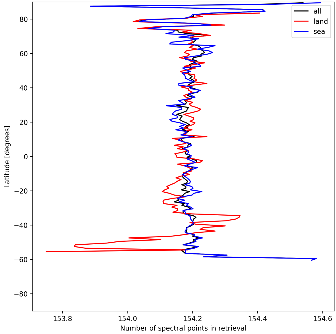
Figure 13: Zonal average of “Number of spectral points in retrieval” for 2025-06-22 to 2025-06-23.
