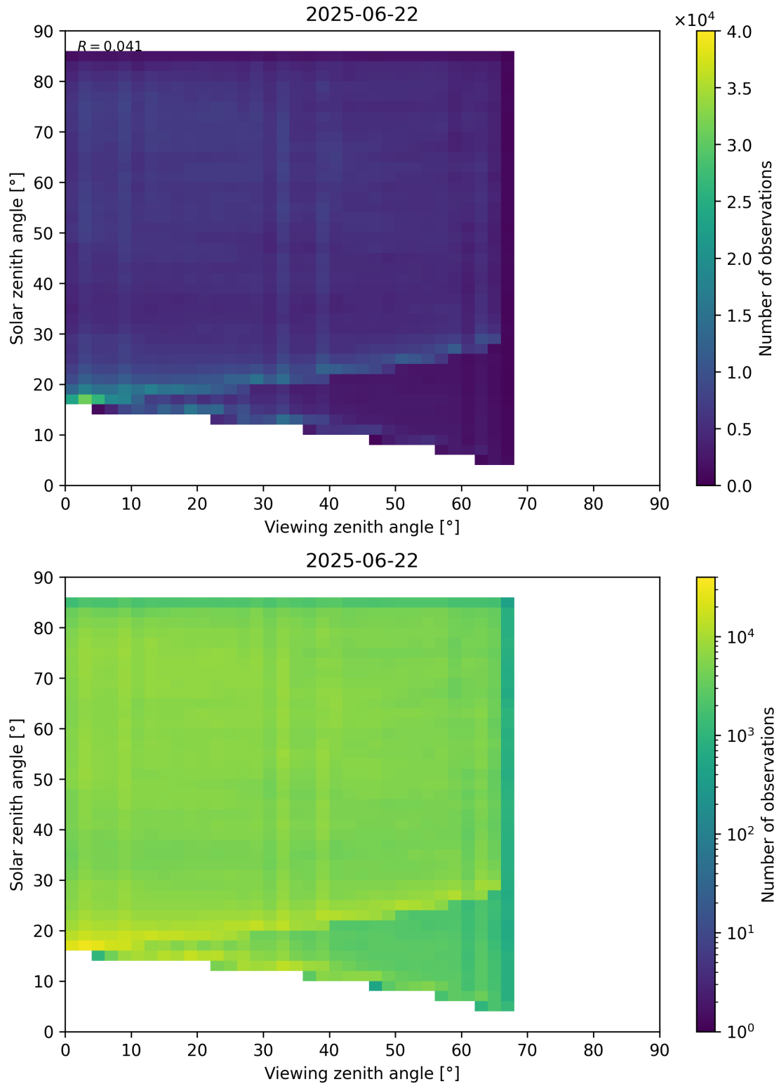
Figure 77: Scatter density plot of “Viewing zenith angle” against “Solar zenith angle” for 2025-06-22 to 2025-06-23.
