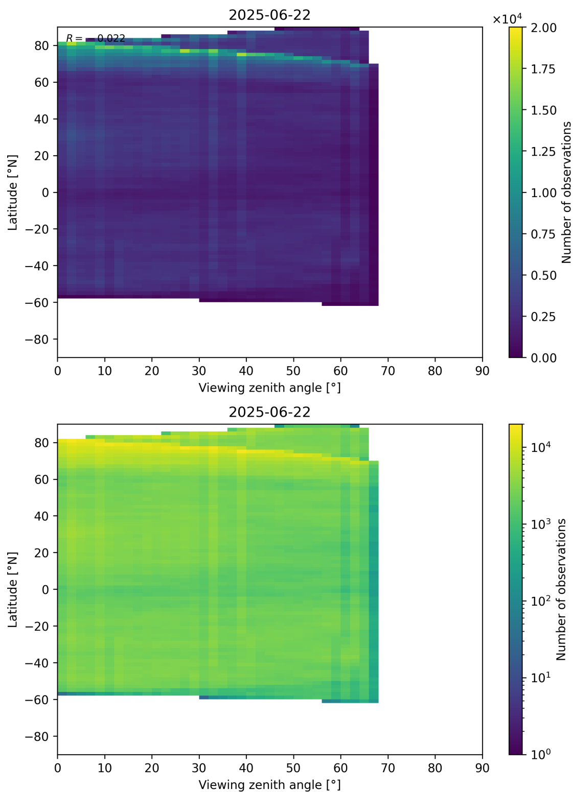
Figure 74: Scatter density plot of “Viewing zenith angle” against “Latitude” for 2025-06-22 to 2025-06-23.
