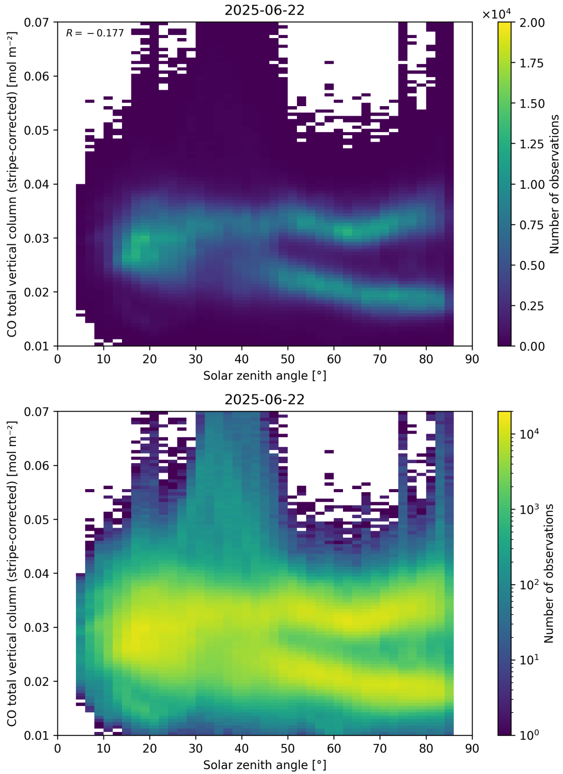
Figure 62: Scatter density plot of “Solar zenith angle” against “CO total vertical column (stripe-corrected)” for 2025-06-22 to 2025-06-23.
