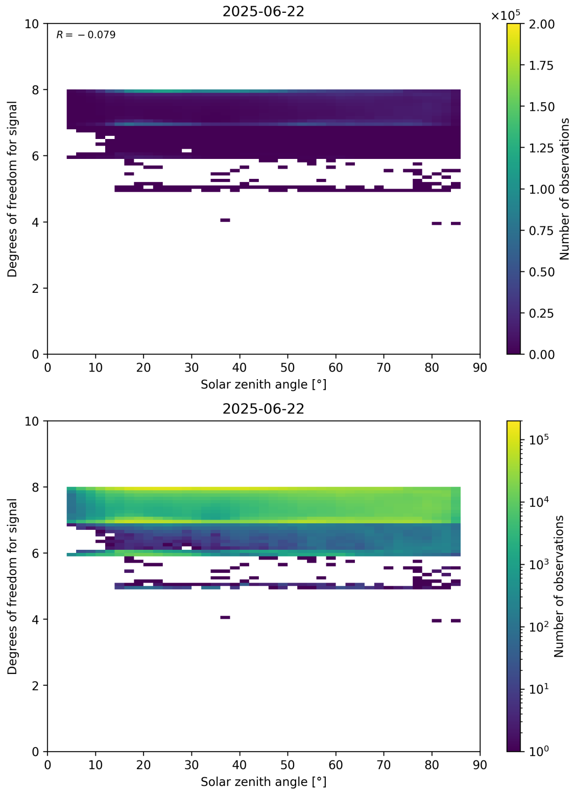
Figure 65: Scatter density plot of “Solar zenith angle” against “Degrees of freedom for signal” for 2025-06-22 to 2025-06-23.
