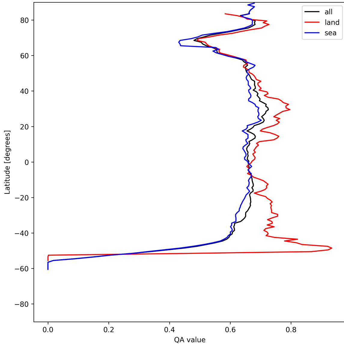
Figure 9: Zonal average of “QA value” for 2025-06-22 to 2025-06-23.
