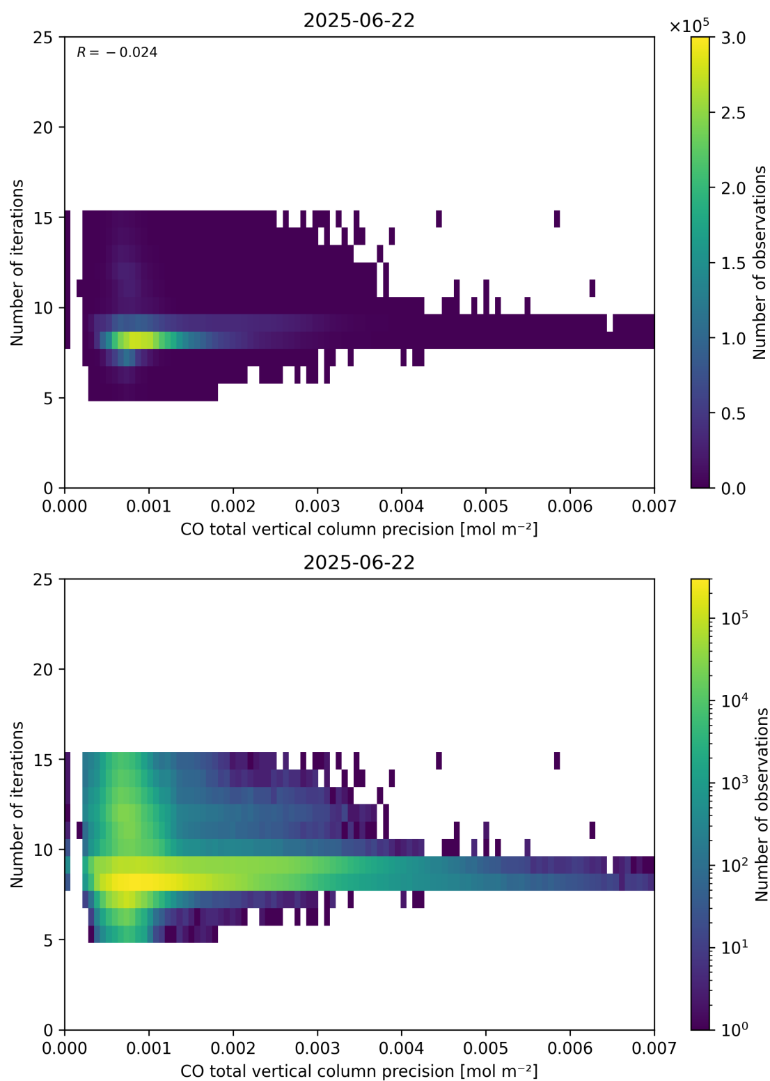
Figure 46: Scatter density plot of “CO total vertical column precision” against “Number of iterations” for 2025-06-22 to 2025-06-23.
