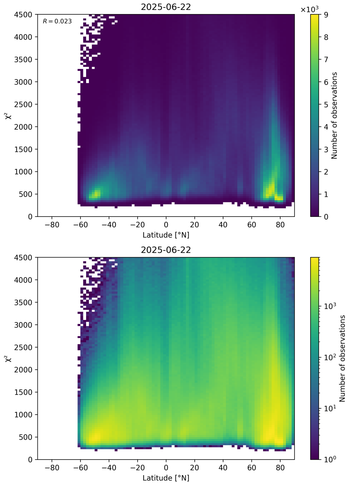
Figure 54: Scatter density plot of “Latitude” against “ \chi^2 ” for 2025-06-22 to 2025-06-23.
