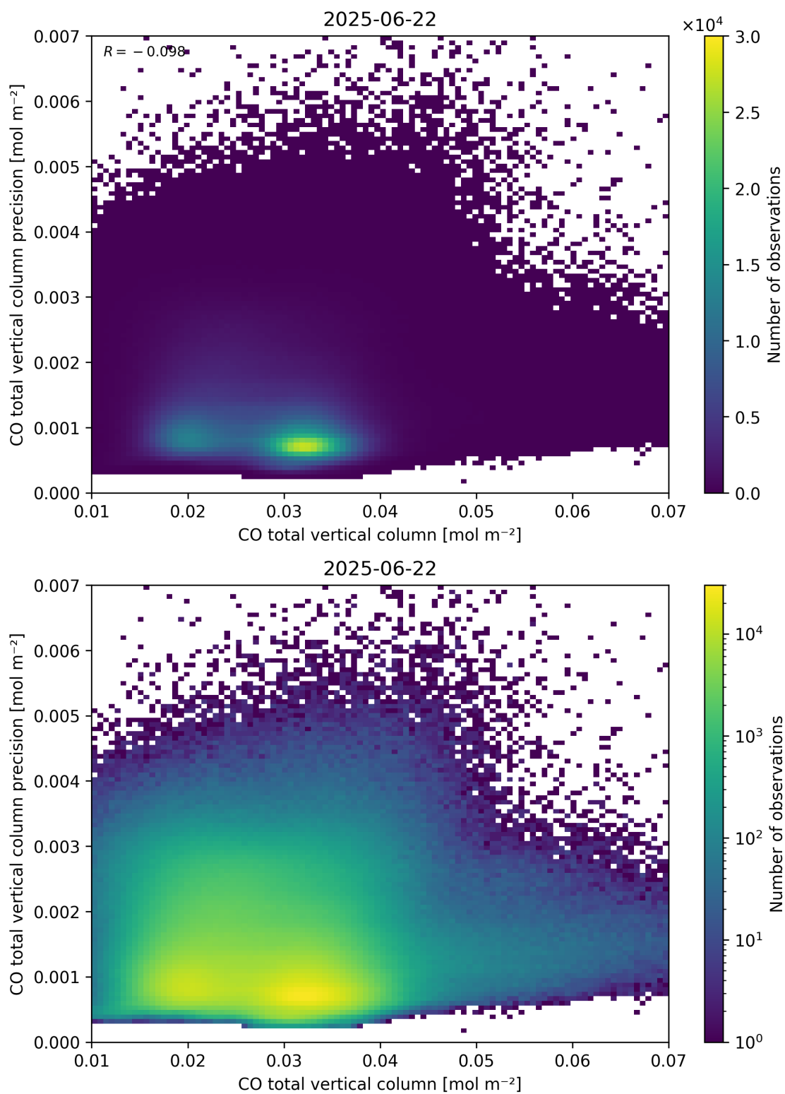
Figure 34: Scatter density plot of “CO total vertical column” against “CO total vertical column precision” for 2025-06-22 to 2025-06-23.
