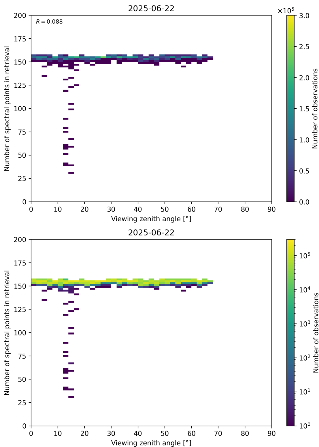
Figure 76: Scatter density plot of “Viewing zenith angle” against “Number of spectral points in retrieval” for 2025-06-22 to 2025-06-23.
