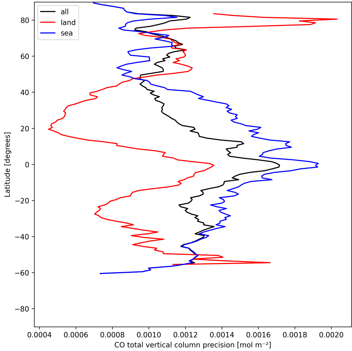
Figure 12: Zonal average of “CO total vertical column precision” for 2025-06-22 to 2025-06-23.
