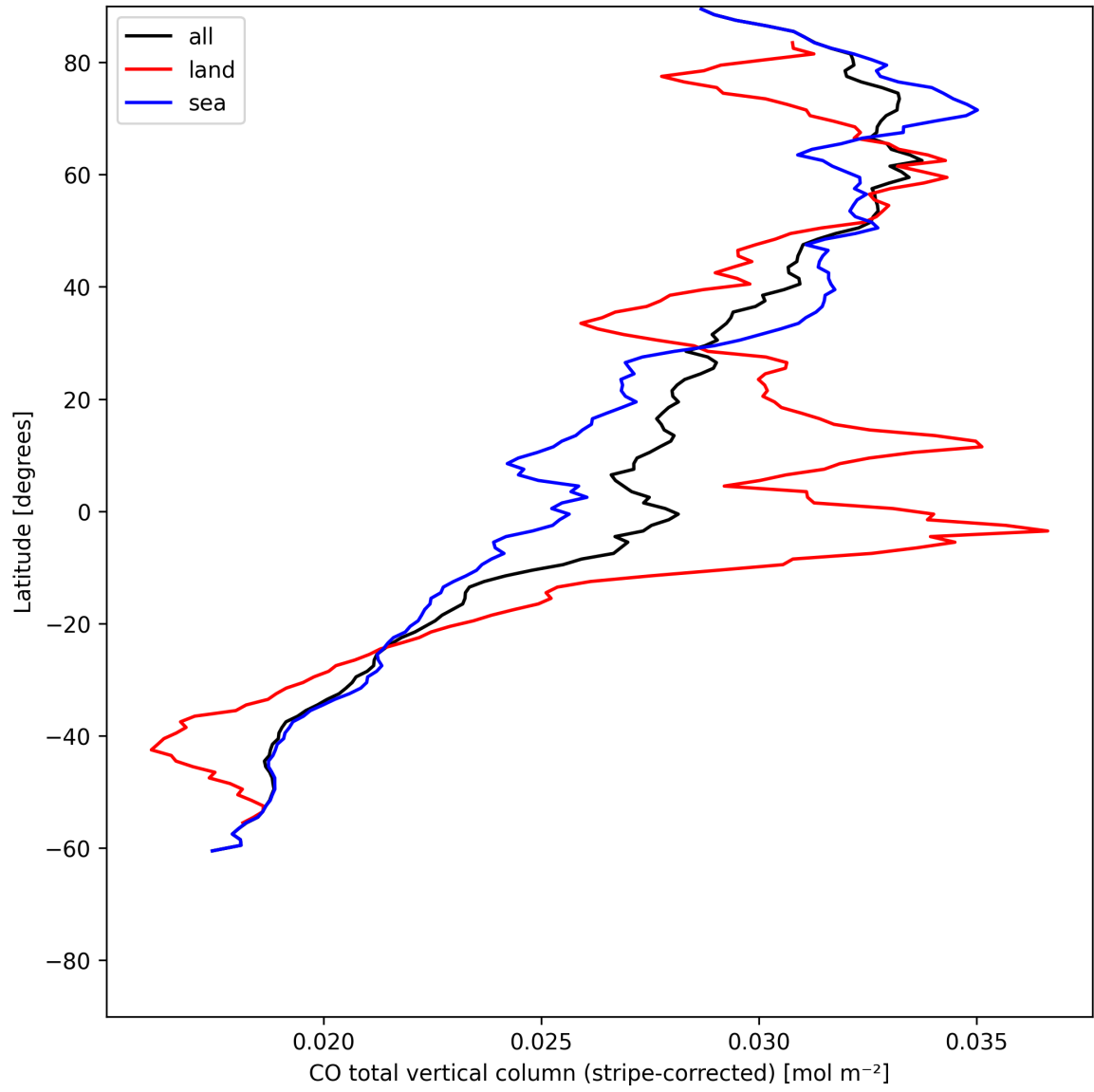
Figure 11: Zonal average of “CO total vertical column (stripe-corrected)” for 2025-06-22 to 2025-06-23.
