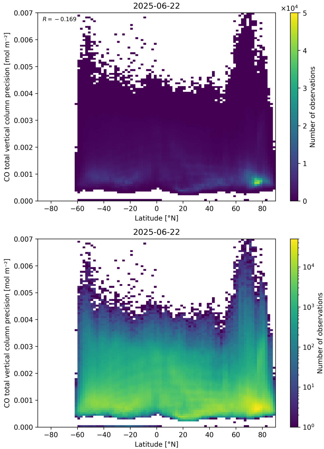
Figure 53: Scatter density plot of “Latitude” against “CO total vertical column precision” for 2025-06-22 to 2025-06-23.
