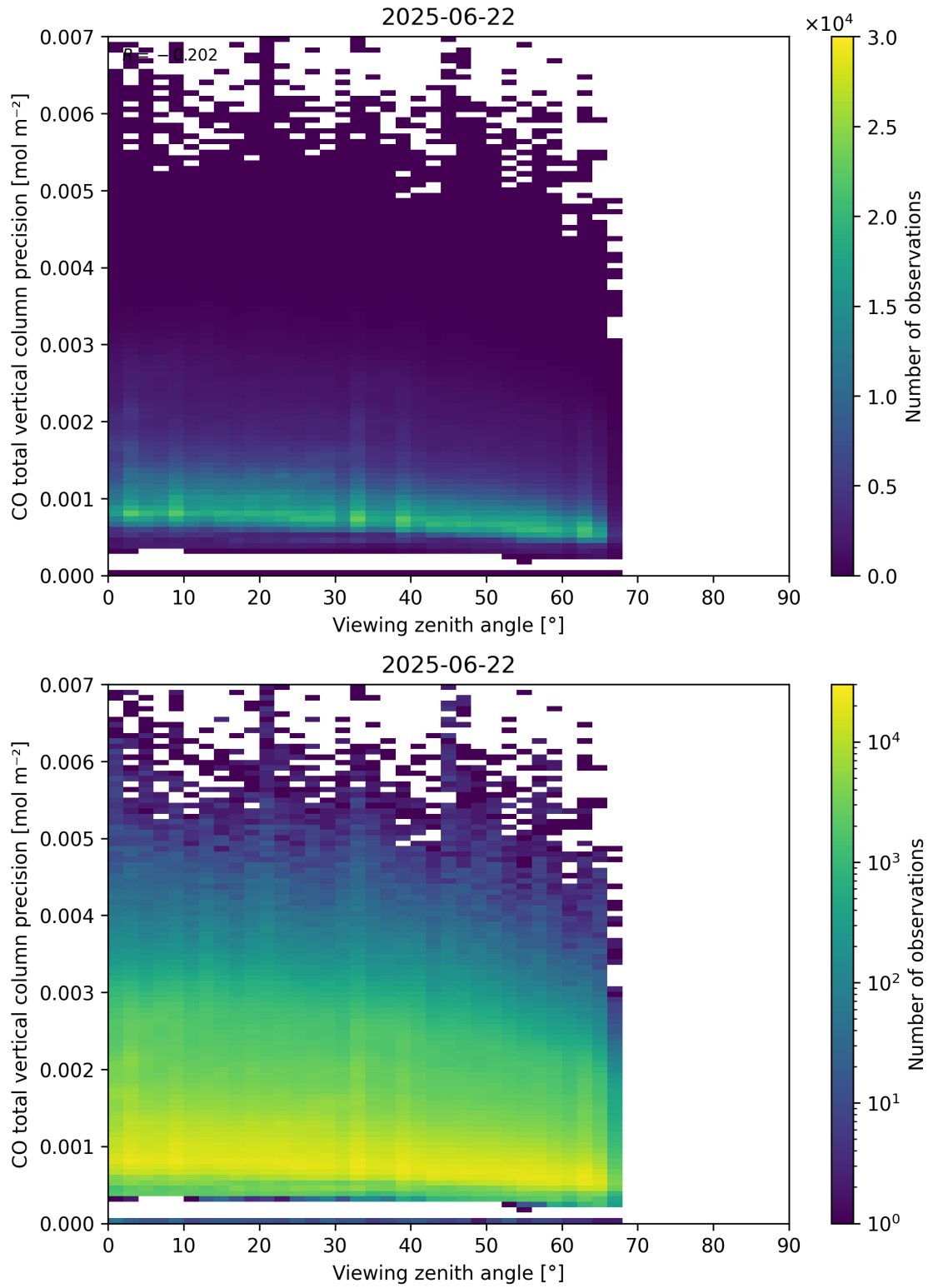
Figure 71: Scatter density plot of “Viewing zenith angle” against “CO total vertical column precision” for 2025-06-22 to 2025-06-23.
