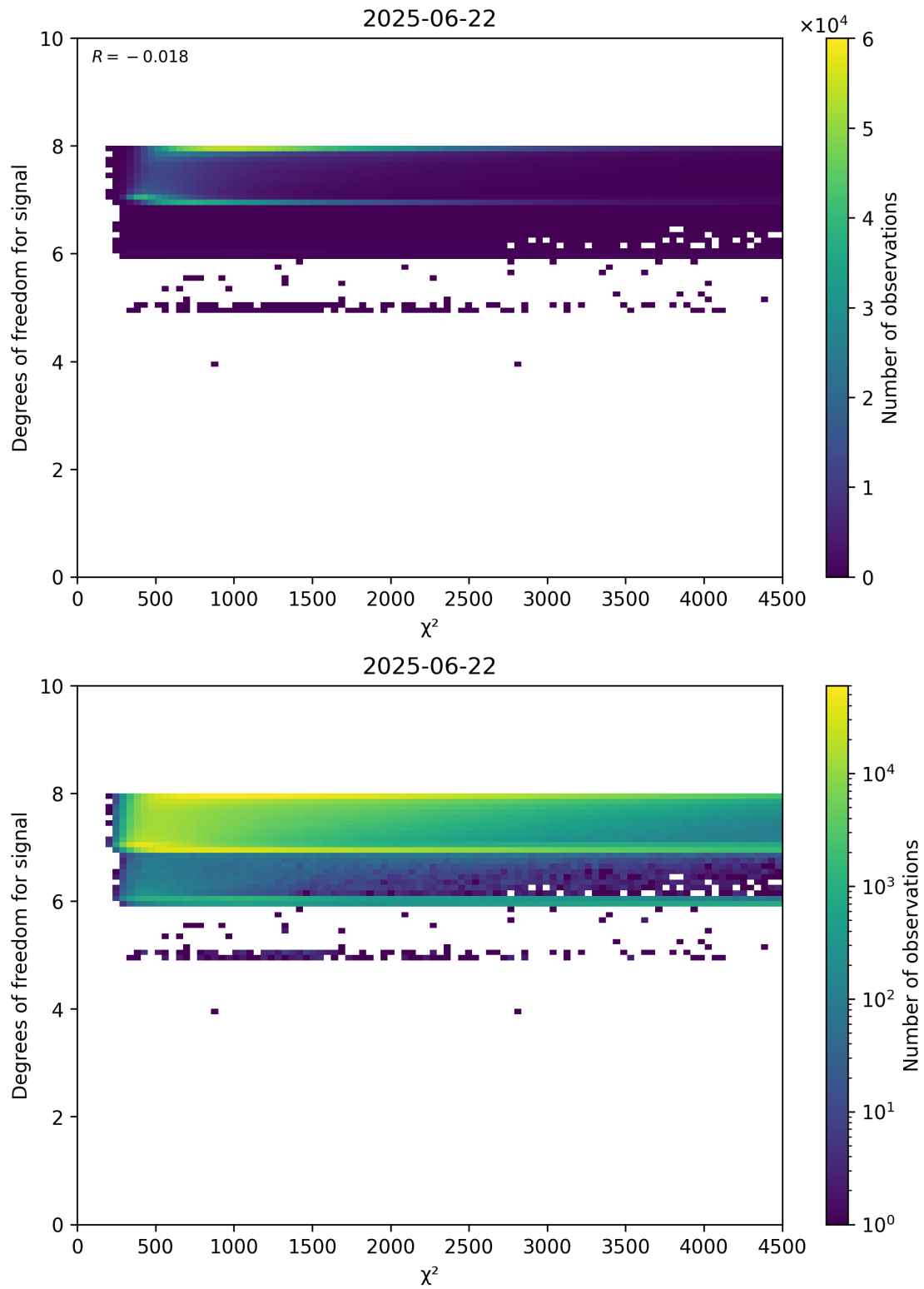
Figure 48: Scatter density plot of “ \chi^2 ” against “Degrees of freedom for signal” for 2025-06-22 to 2025-06-23.
