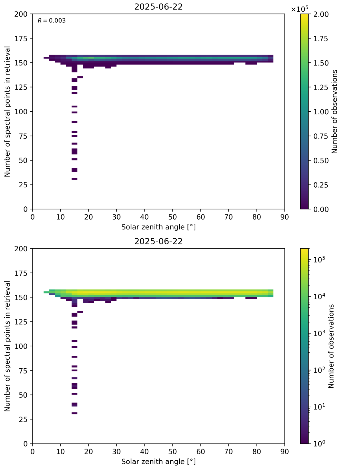
Figure 68: Scatter density plot of “Solar zenith angle” against “Number of spectral points in retrieval” for 2025-06-22 to 2025-06-23.
