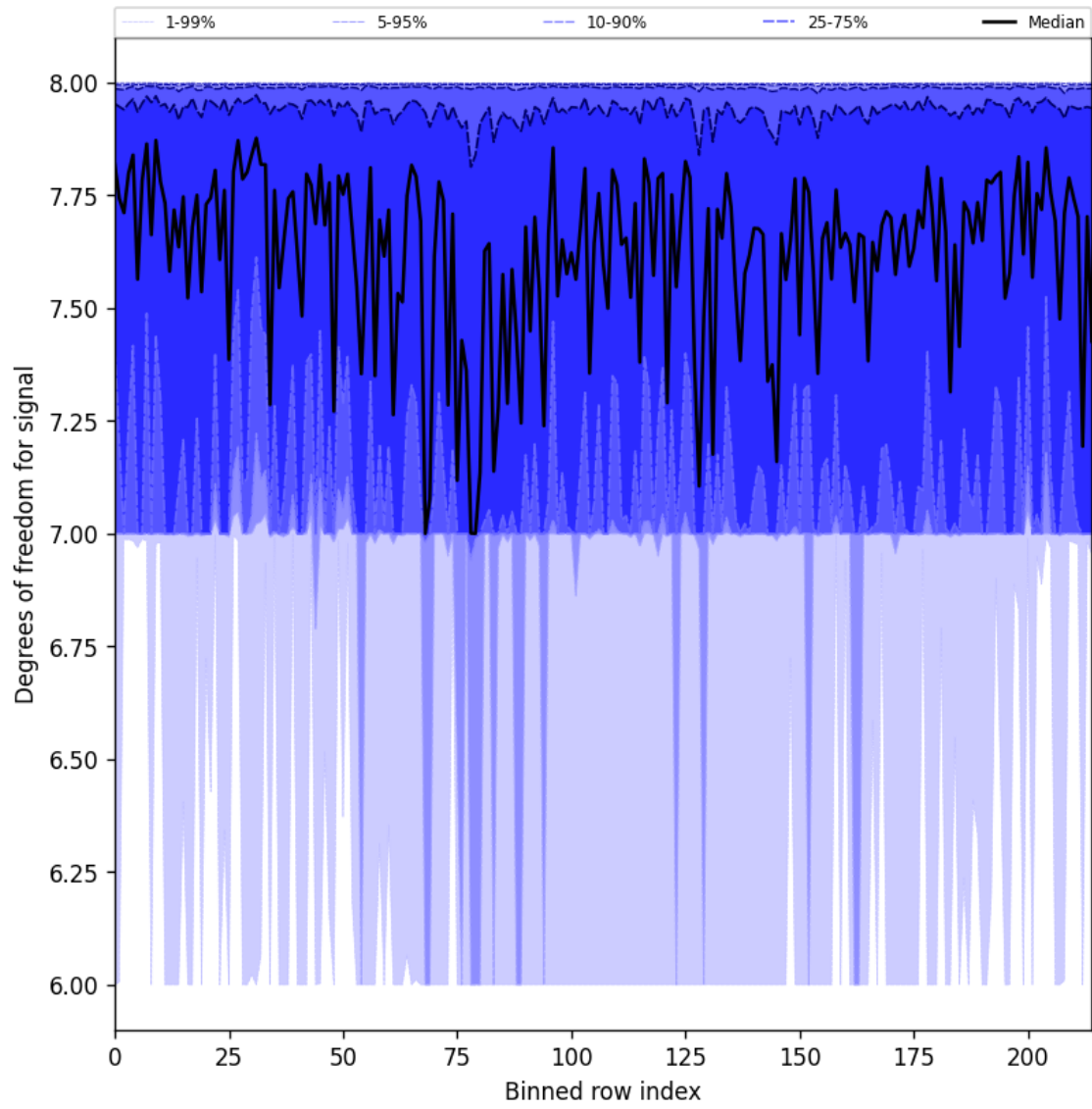
Figure 31: Along track statistics of “Degrees of freedom for signal” for 2025-06-22 to 2025-06-23
