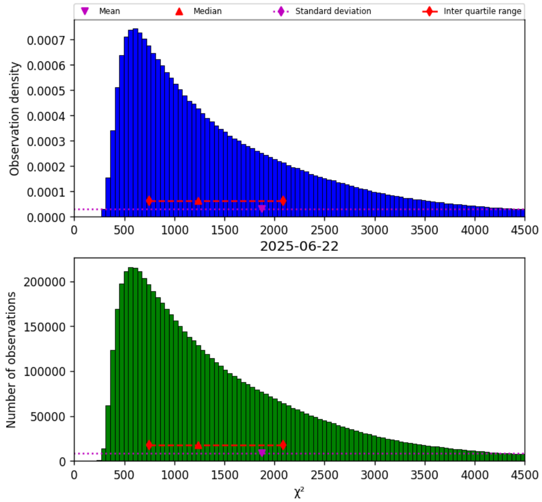
Figure 22: Histogram of “ \chi^2 ” for 2025-06-22 to 2025-06-23
