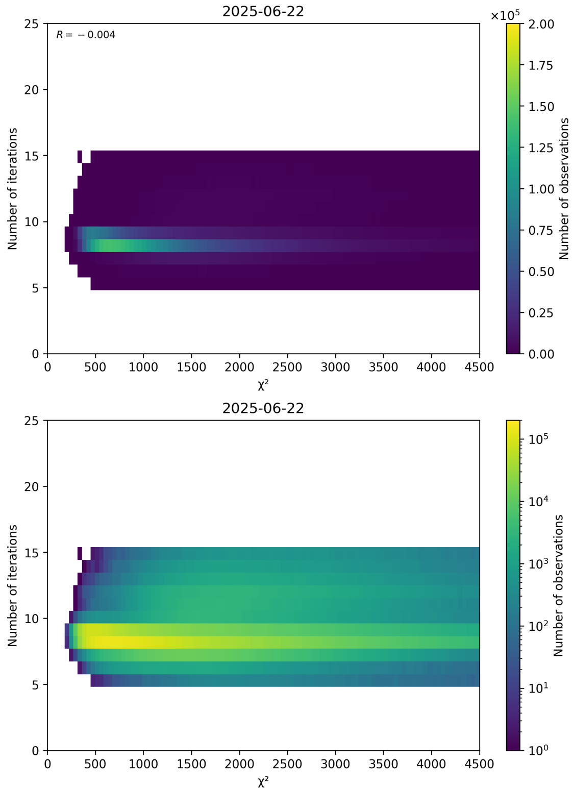
Figure 49: Scatter density plot of “ \chi^2 ” against “Number of iterations” for 2025-06-22 to 2025-06-23.
