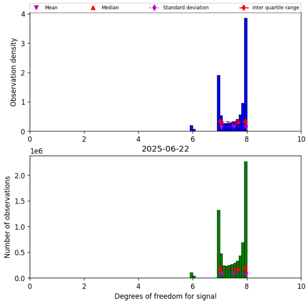
Figure 23: Histogram of “Degrees of freedom for signal” for 2025-06-22 to 2025-06-23
