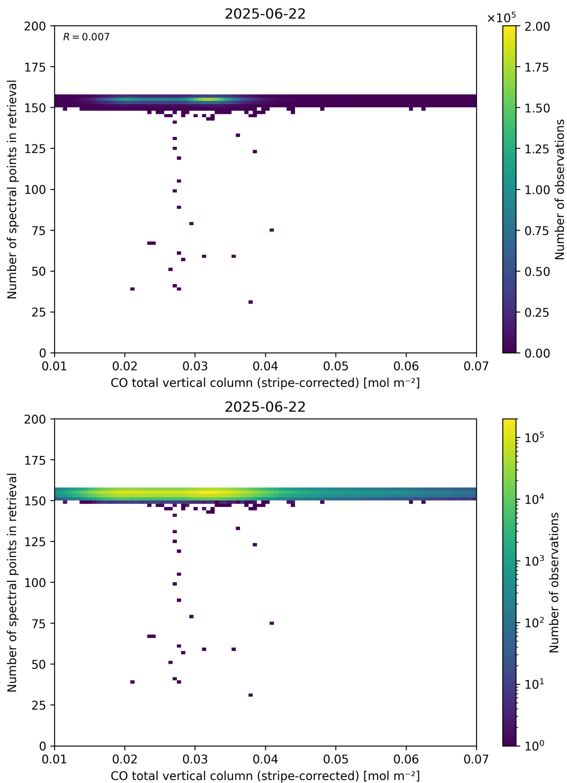
Figure 40: Scatter density plot of “CO total vertical column (stripe-corrected)” against “Number of spectral points in retrieval” for 2025-06-22 to 2025-06-23.
