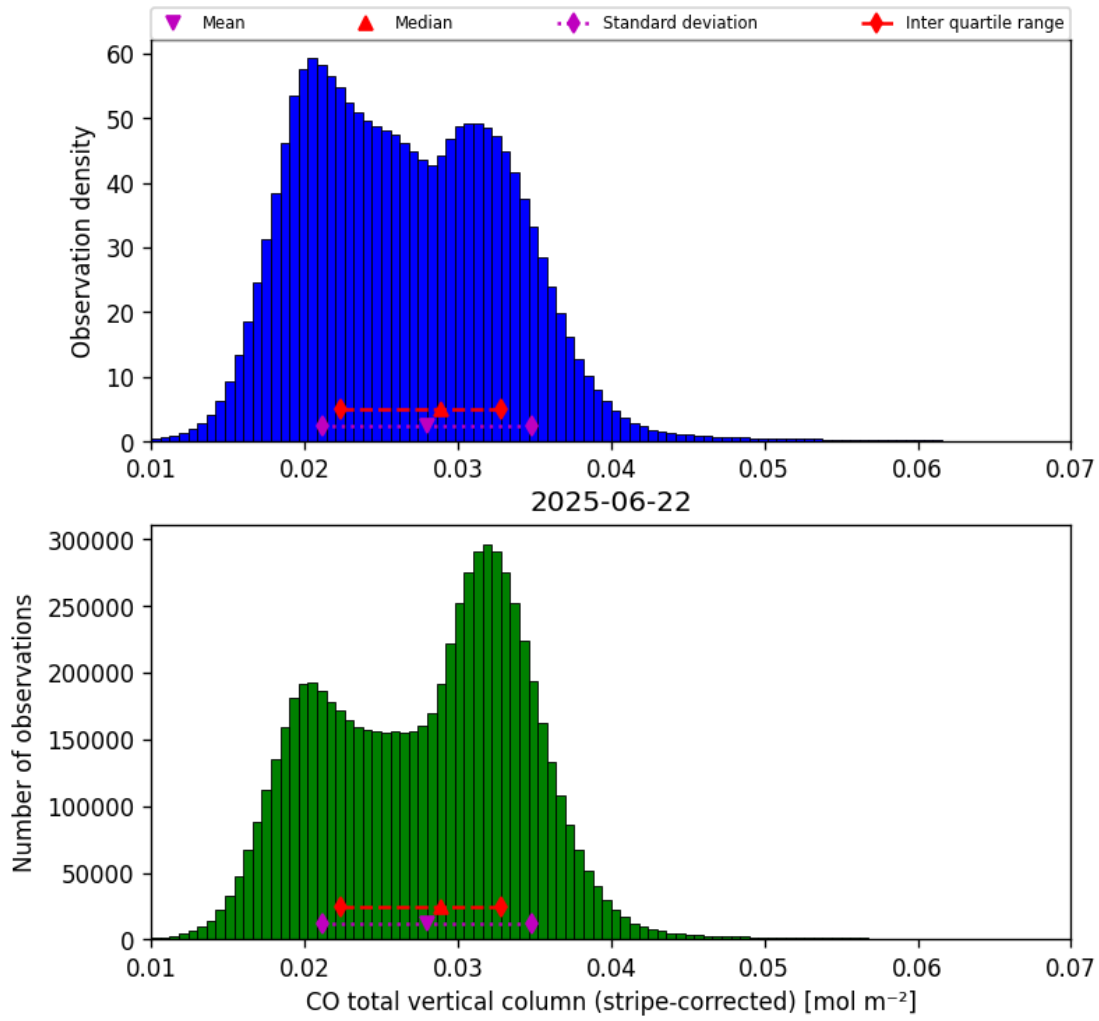
Figure 19: Histogram of “CO total vertical column (stripe-corrected)” for 2025-06-22 to 2025-06-23
