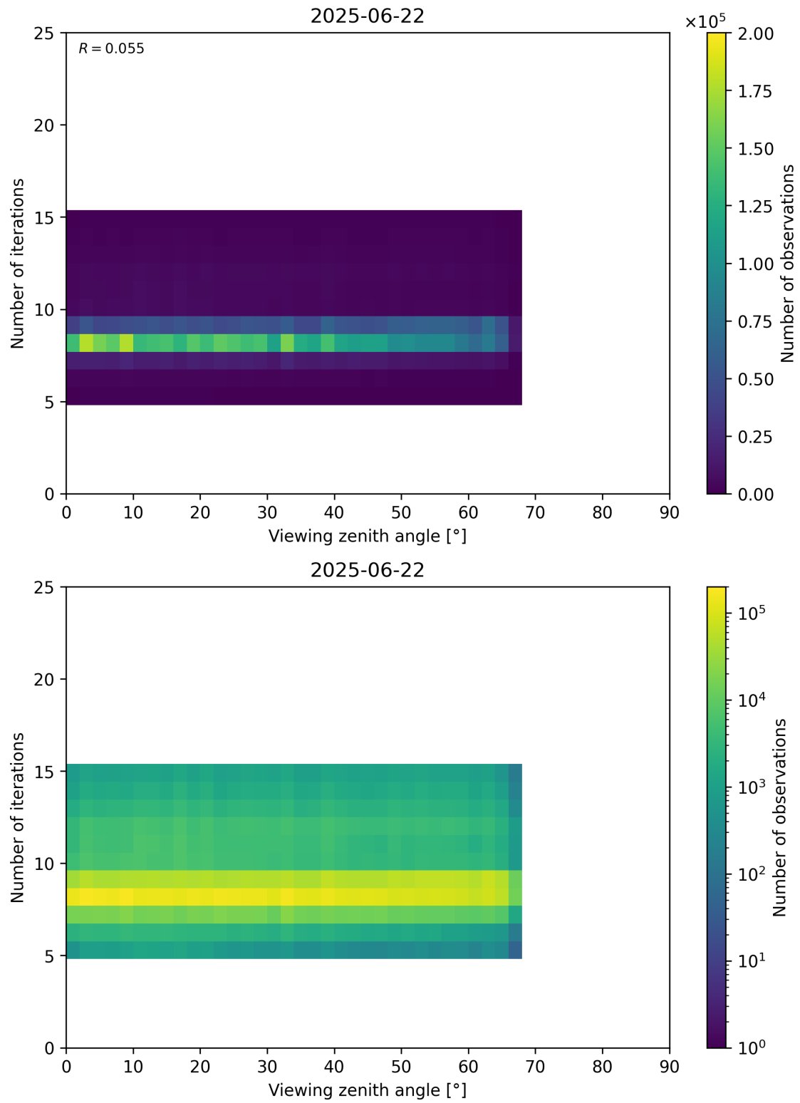
Figure 75: Scatter density plot of “Viewing zenith angle” against “Number of iterations” for 2025-06-22 to 2025-06-23.
