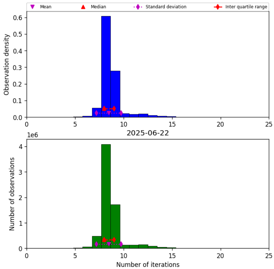
Figure 24: Histogram of “Number of iterations” for 2025-06-22 to 2025-06-23
