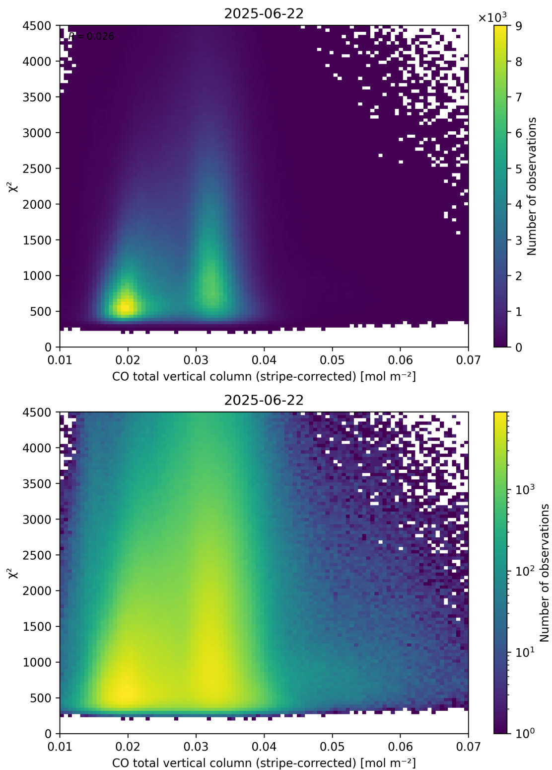
Figure 37: Scatter density plot of “CO total vertical column (stripe-corrected)” against “ \chi^2 ” for 2025-06-22 to 2025-06-23.
