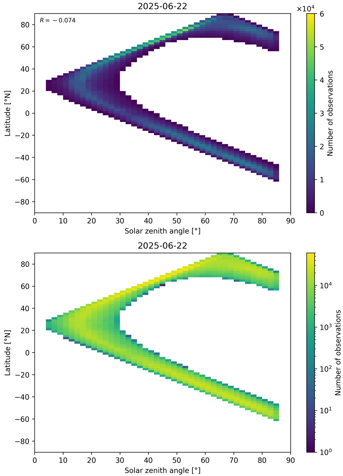
Figure 66: Scatter density plot of “Solar zenith angle” against “Latitude” for 2025-06-22 to 2025-06-23.
