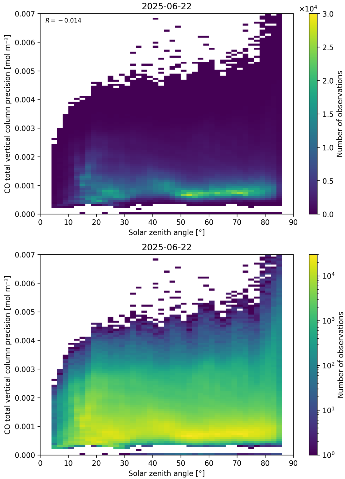
Figure 63: Scatter density plot of “Solar zenith angle” against “CO total vertical column precision” for 2025-06-22 to 2025-06-23.
