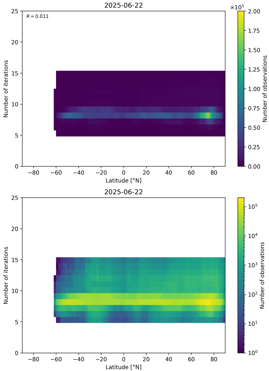
Figure 56: Scatter density plot of “Latitude” against “Number of iterations” for 2025-06-22 to 2025-06-23.
