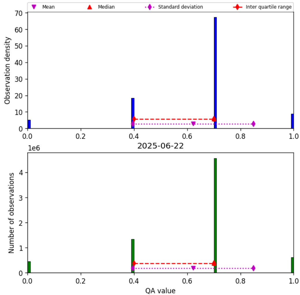
Figure 17: Histogram of “QA value” for 2025-06-22 to 2025-06-23
