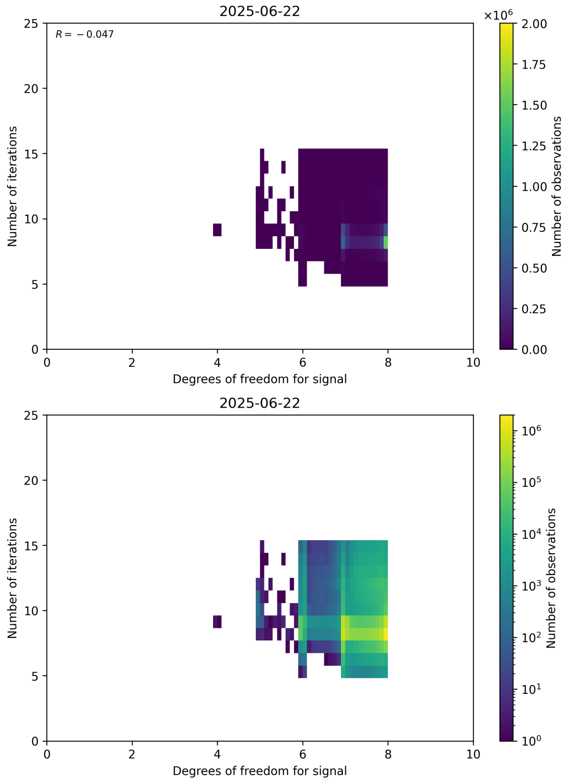
Figure 50: Scatter density plot of “Degrees of freedom for signal” against “Number of iterations” for 2025-06-22 to 2025-06-23.
