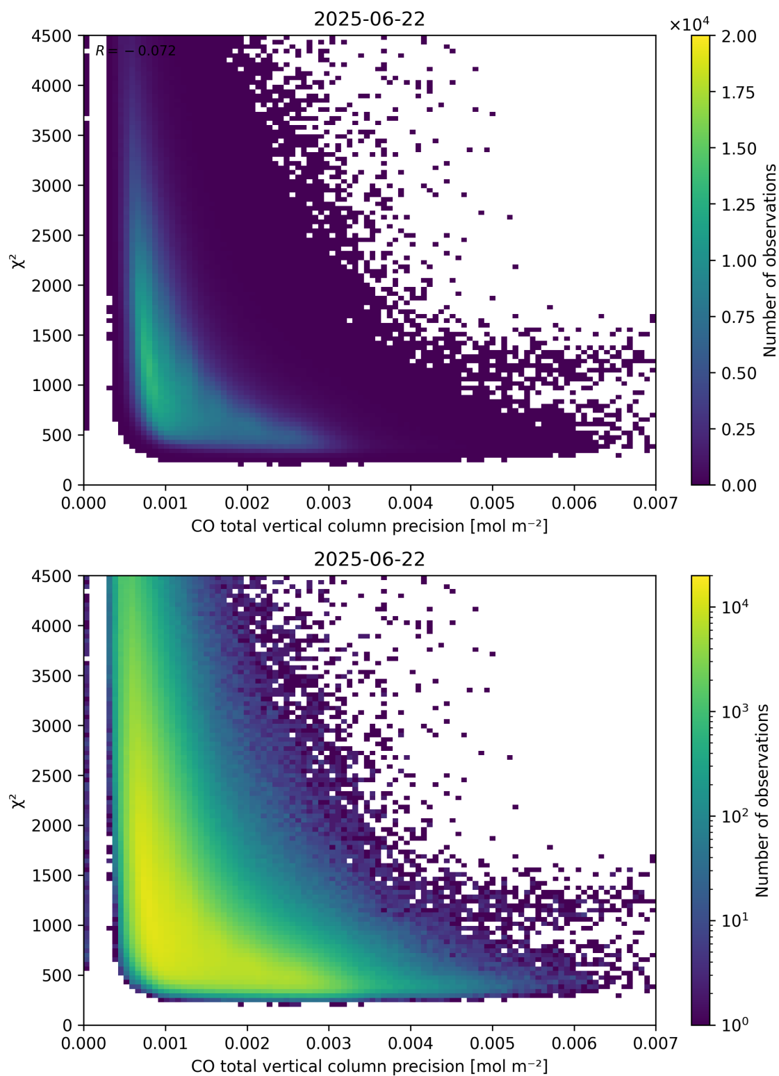
Figure 44: Scatter density plot of “CO total vertical column precision” against “ \chi^2 ” for 2025-06-22 to 2025-06-23.
