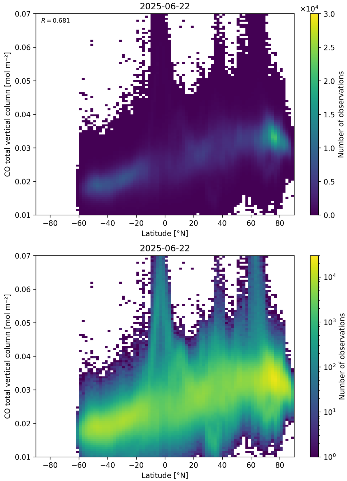
Figure 51: Scatter density plot of “Latitude” against “CO total vertical column” for 2025-06-22 to 2025-06-23.
