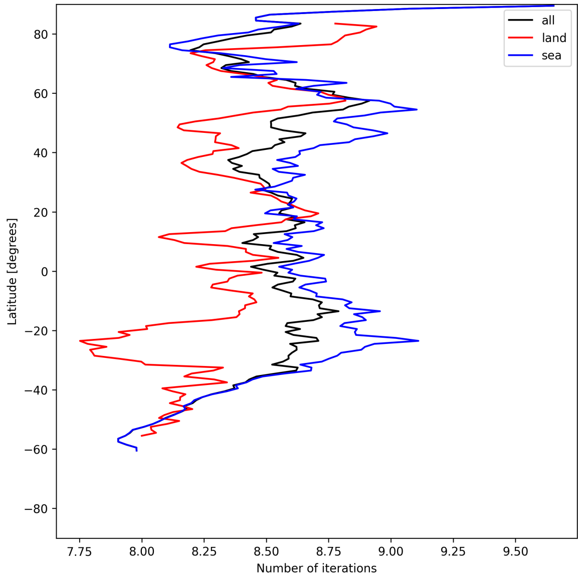
Figure 16: Zonal average of “Number of iterations” for 2025-06-22 to 2025-06-23.
