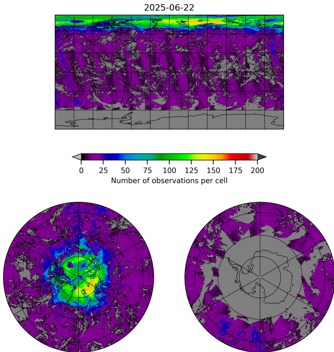
Figure 8: Map of the number of observations for 2025-06-22 to 2025-06-23
