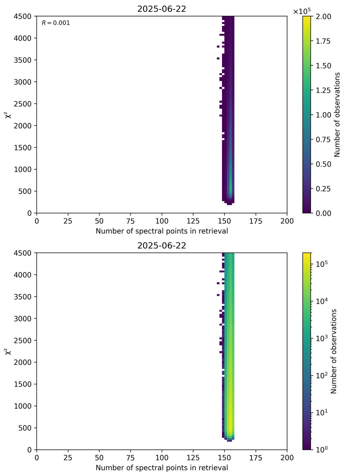
Figure 58: Scatter density plot of “Number of spectral points in retrieval” against “ \chi^2 ” for 2025-06-22 to 2025-06-23.
