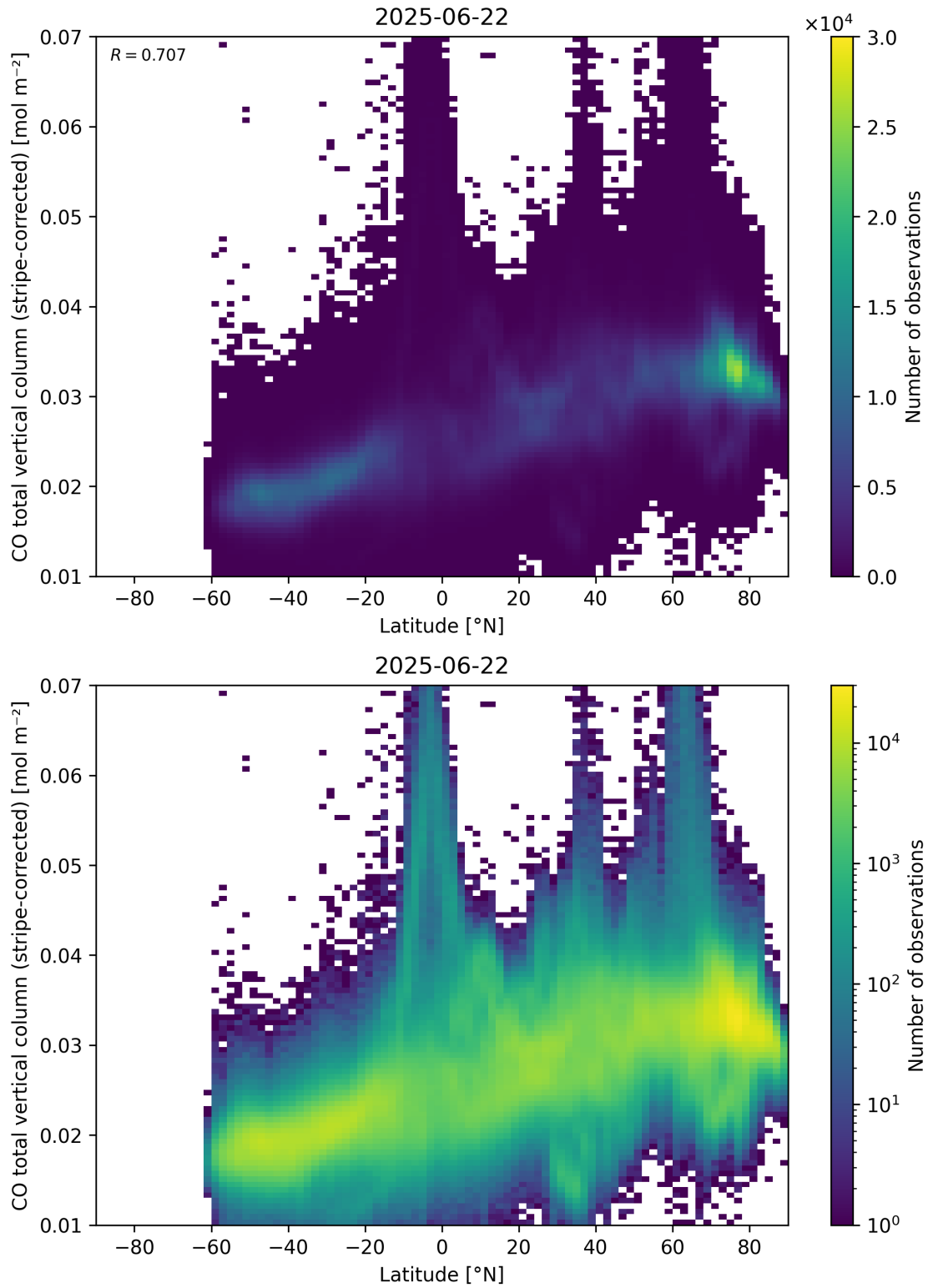
Figure 52: Scatter density plot of “Latitude” against “CO total vertical column (stripe-corrected)” for 2025-06-22 to 2025-06-23.
