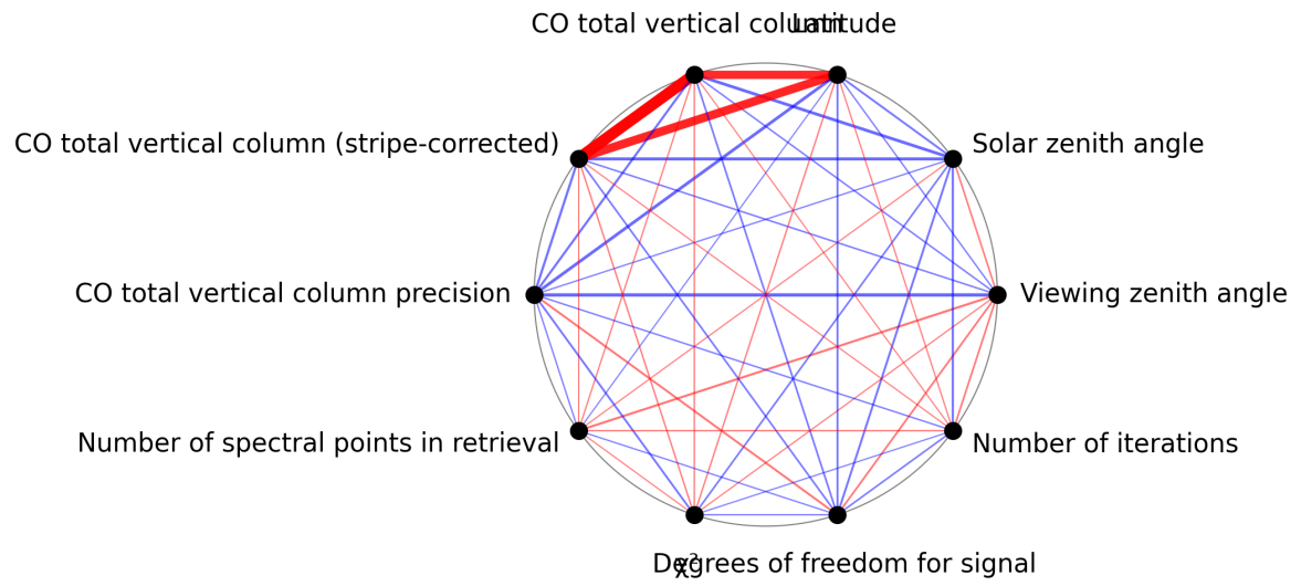
Figure 1: Map of correlation graph for 2025-06-22 to 2025-06-23.
