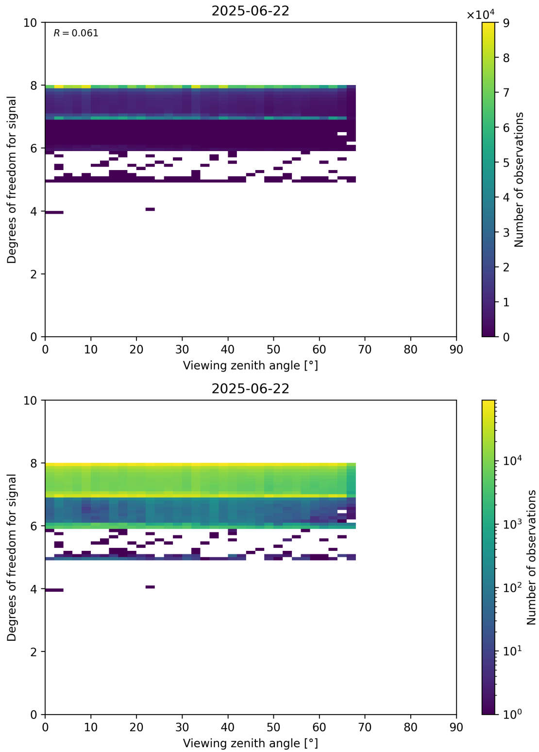
Figure 73: Scatter density plot of “Viewing zenith angle” against “Degrees of freedom for signal” for 2025-06-22 to 2025-06-23.
