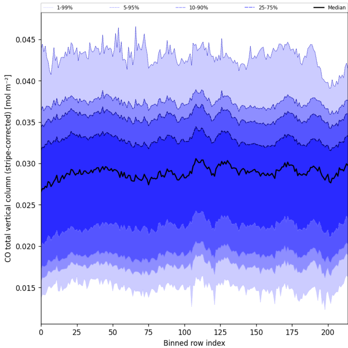
Figure 27: Along track statistics of “CO total vertical column (stripe-corrected)” for 2025-06-22 to 2025-06-23
