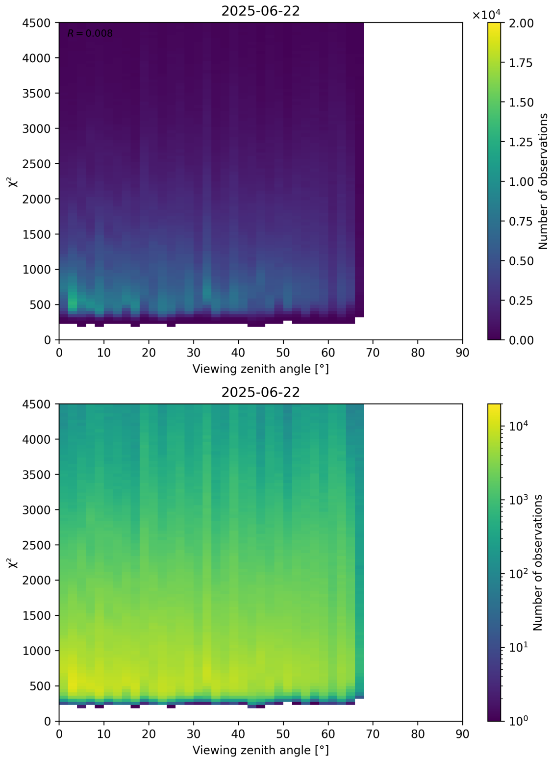
Figure 72: Scatter density plot of “Viewing zenith angle” against “ \chi^2 ” for 2025-06-22 to 2025-06-23.
