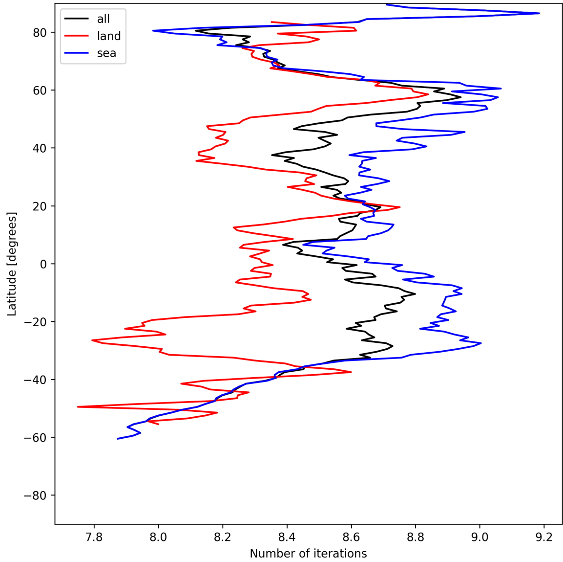
Figure 16: Zonal average of “Number of iterations” for 2025-06-22 to 2025-06-24.
