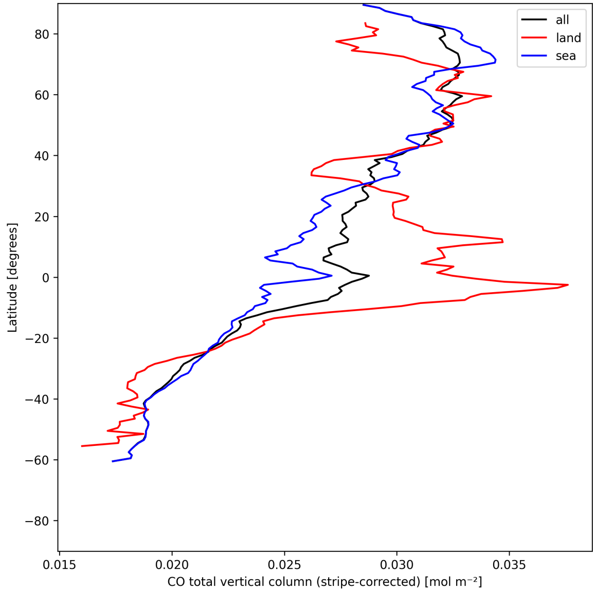
Figure 11: Zonal average of “CO total vertical column (stripe-corrected)” for 2025-06-22 to 2025-06-24.
