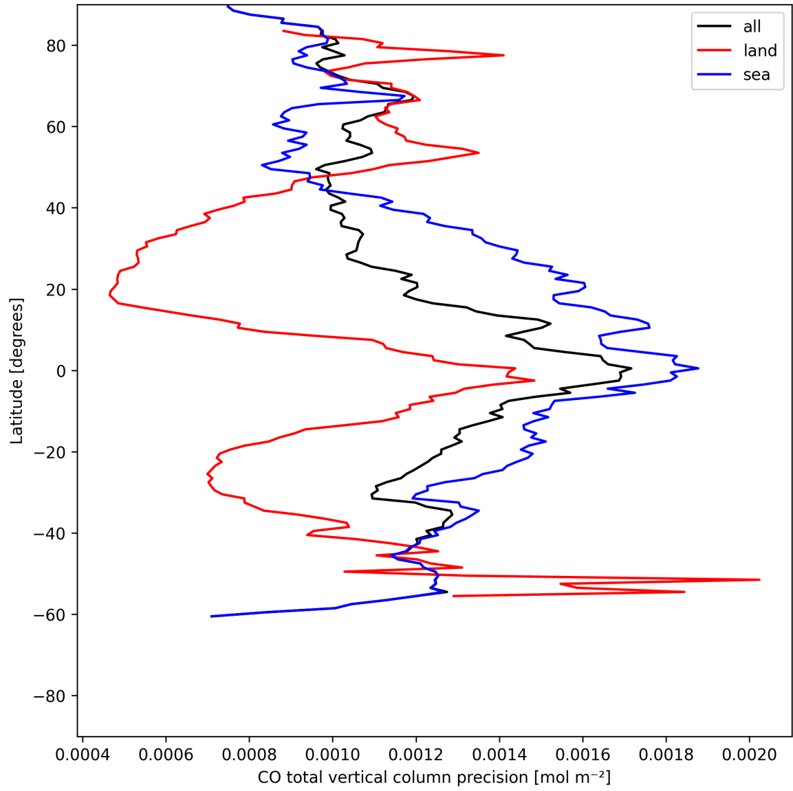
Figure 12: Zonal average of “CO total vertical column precision” for 2025-06-22 to 2025-06-24.
