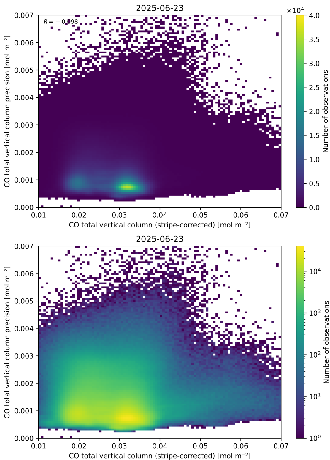
Figure 36: Scatter density plot of “CO total vertical column (stripe-corrected)” against “CO total vertical column precision” for 2025-06-22 to 2025-06-24.
