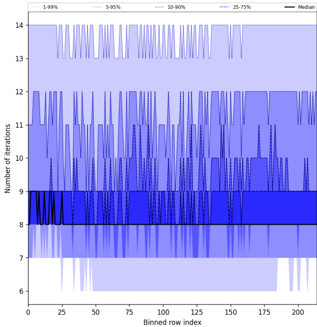
Figure 32: Along track statistics of “Number of iterations” for 2025-06-22 to 2025-06-24
