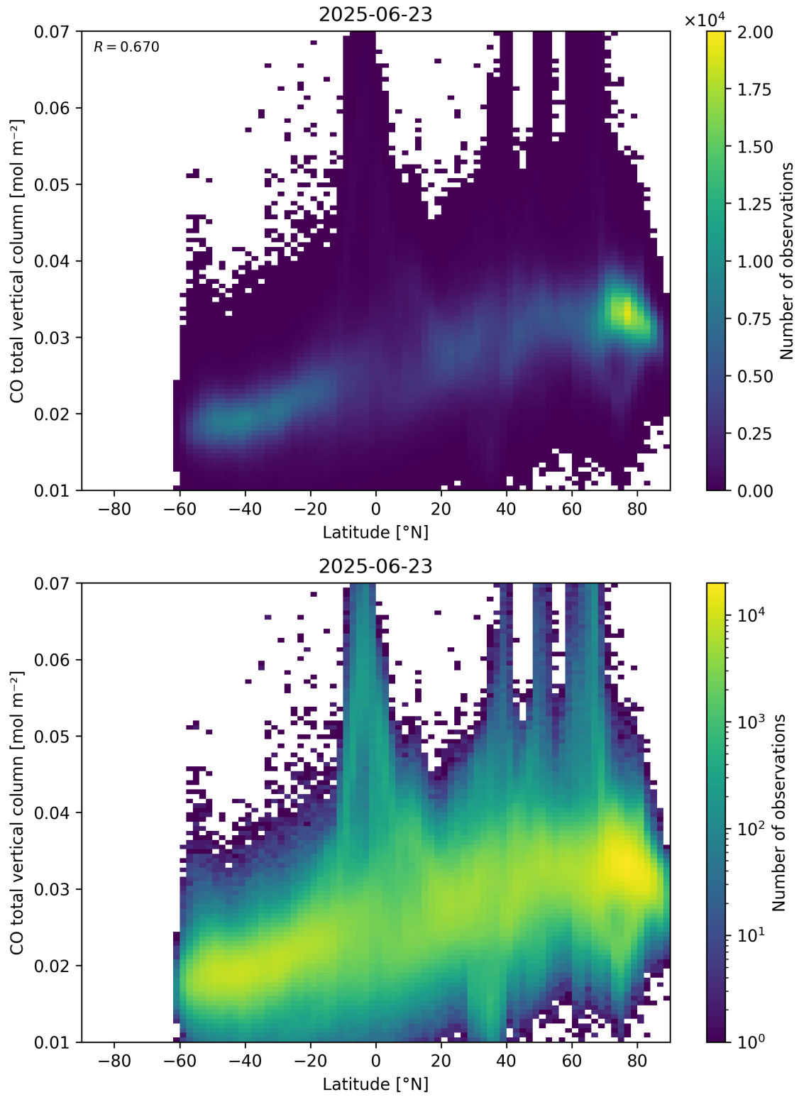
Figure 51: Scatter density plot of “Latitude” against “CO total vertical column” for 2025-06-22 to 2025-06-24.
