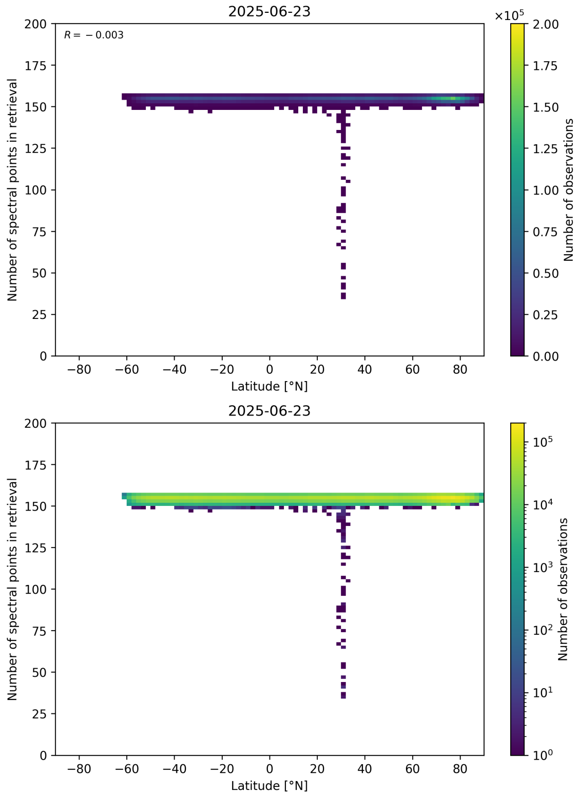
Figure 57: Scatter density plot of “Latitude” against “Number of spectral points in retrieval” for 2025-06-22 to 2025-06-24.
