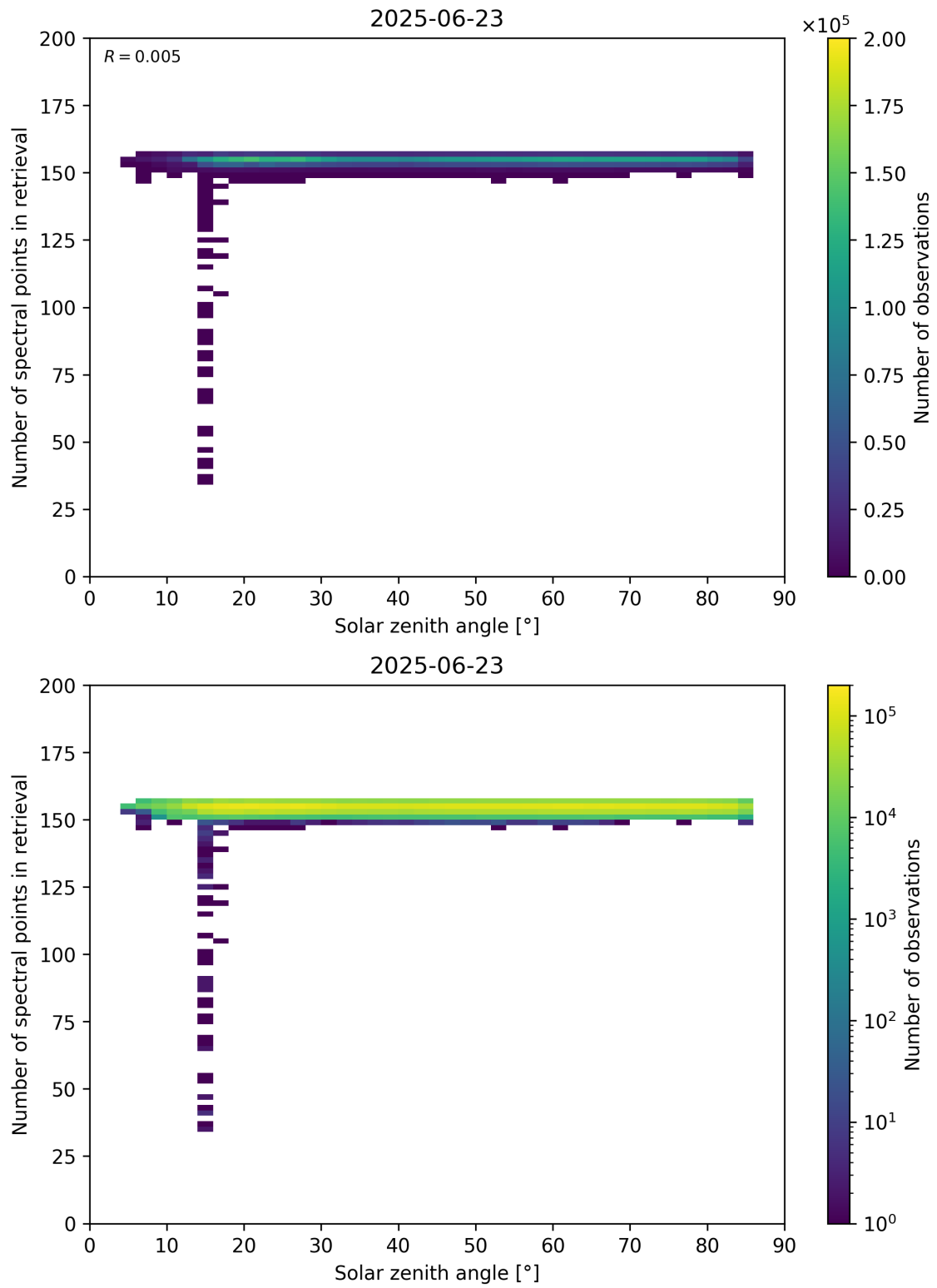
Figure 68: Scatter density plot of “Solar zenith angle” against “Number of spectral points in retrieval” for 2025-06-22 to 2025-06-24.
