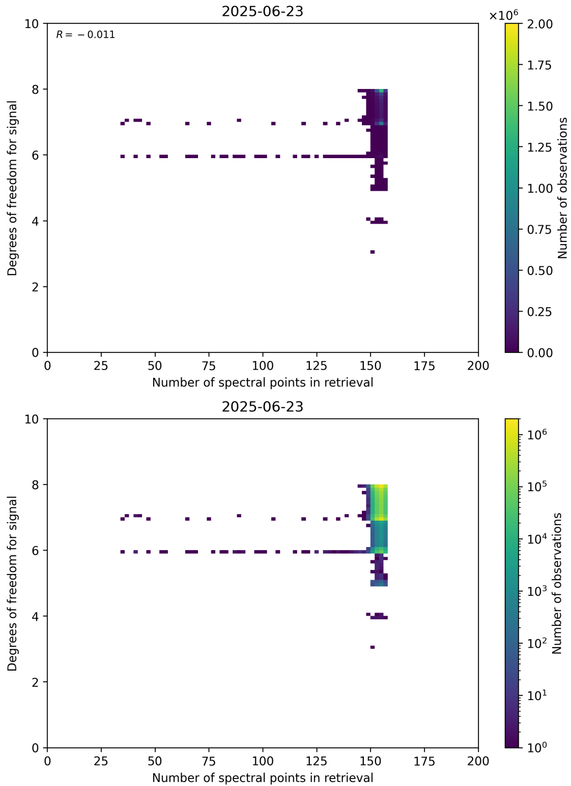
Figure 59: Scatter density plot of “Number of spectral points in retrieval” against “Degrees of freedom for signal” for 2025-06-22 to 2025-06-24.
