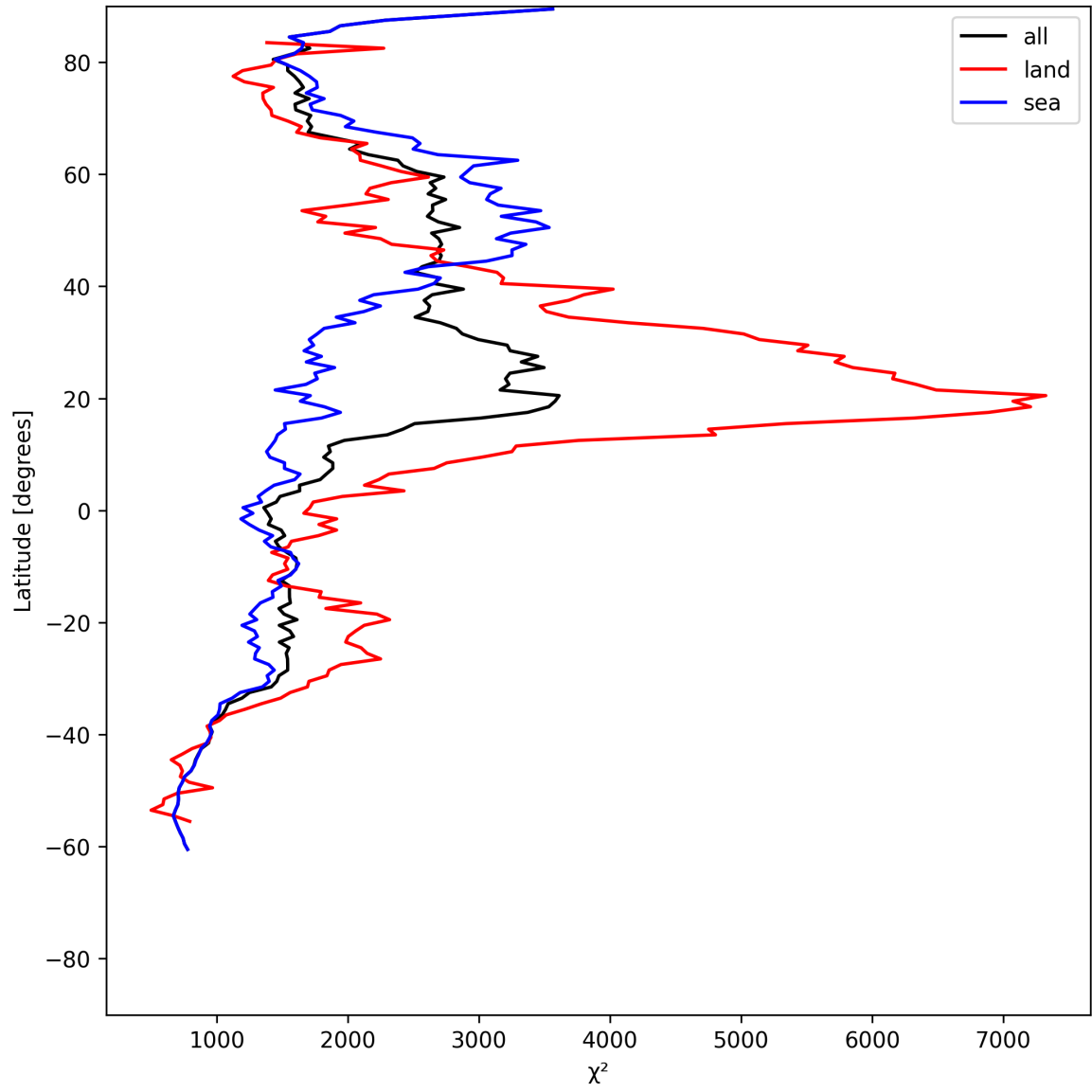
Figure 14: Zonal average of “ \chi^2 ” for 2025-06-22 to 2025-06-24.
