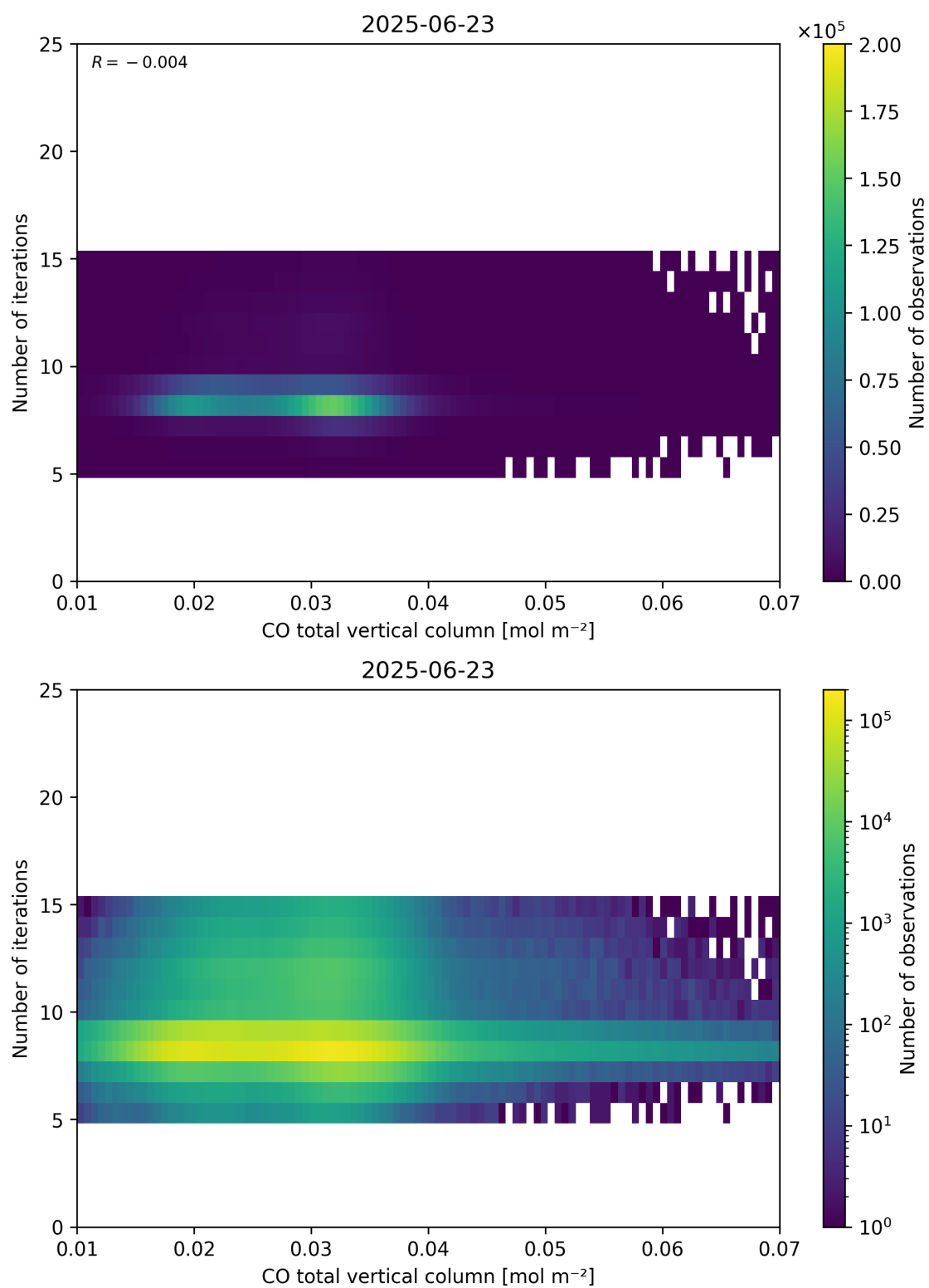
Figure 42: Scatter density plot of “CO total vertical column” against “Number of iterations” for 2025-06-22 to 2025-06-24.
