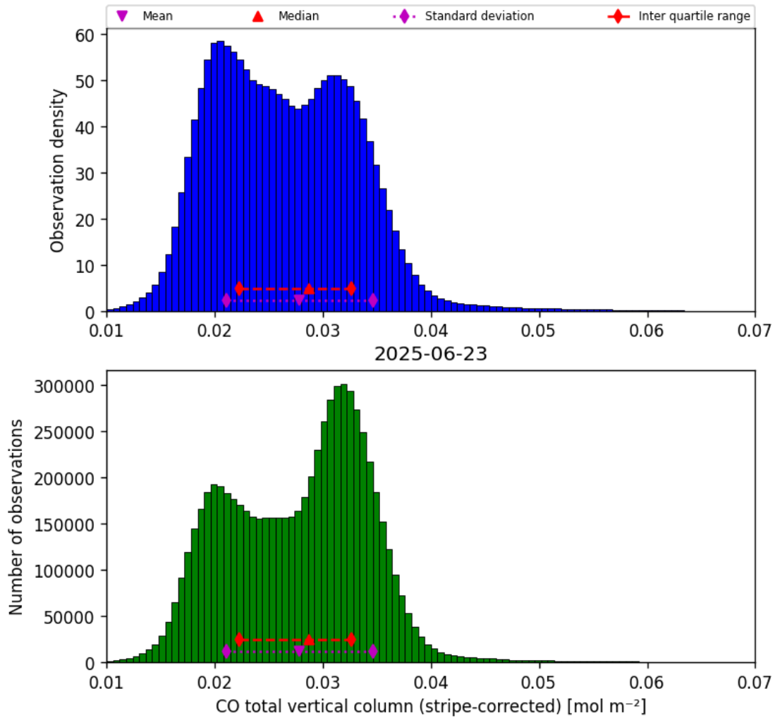
Figure 19: Histogram of “CO total vertical column (stripe-corrected)” for 2025-06-22 to 2025-06-24
