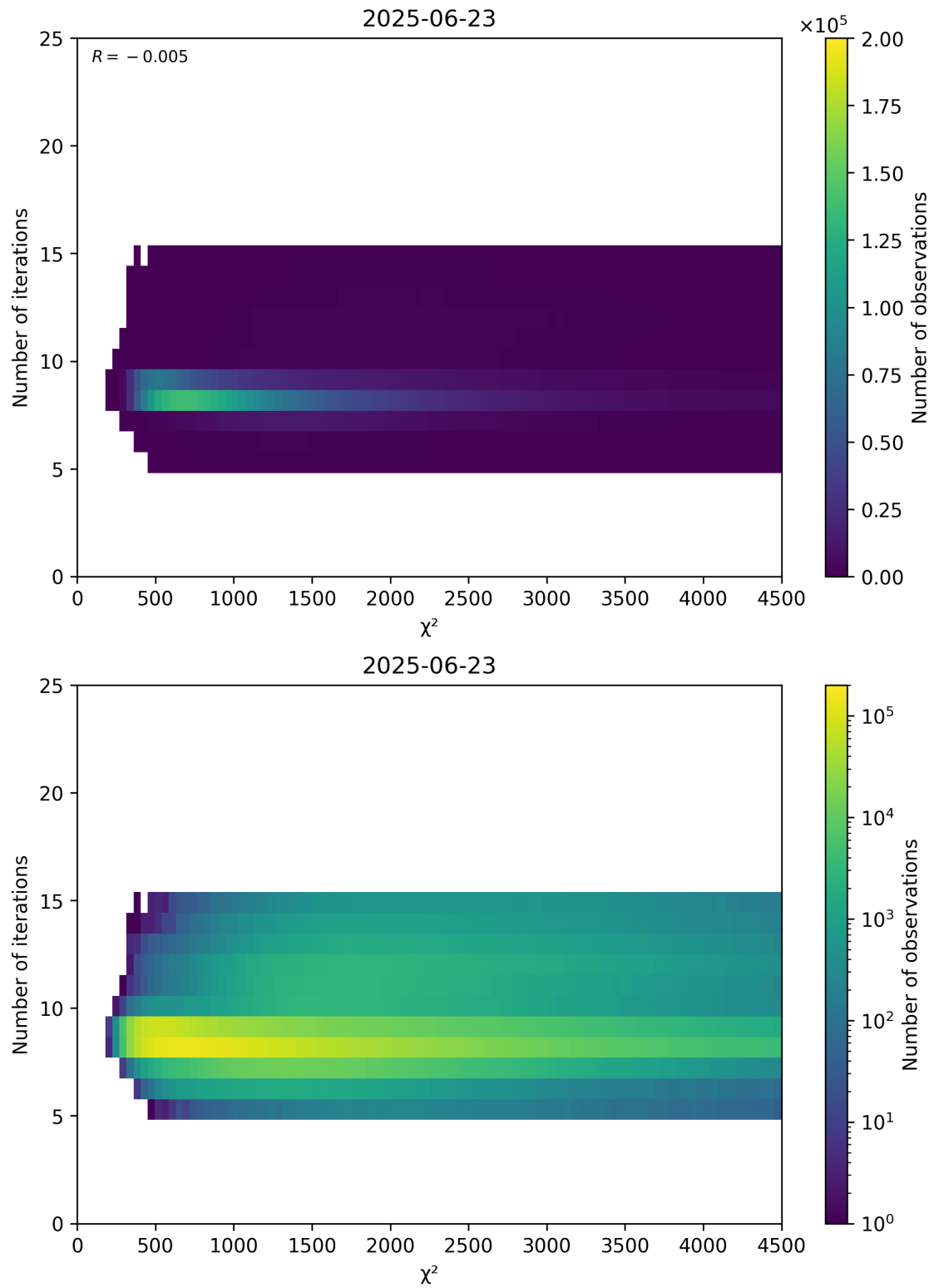
Figure 49: Scatter density plot of “ \chi^2 ” against “Number of iterations” for 2025-06-22 to 2025-06-24.
