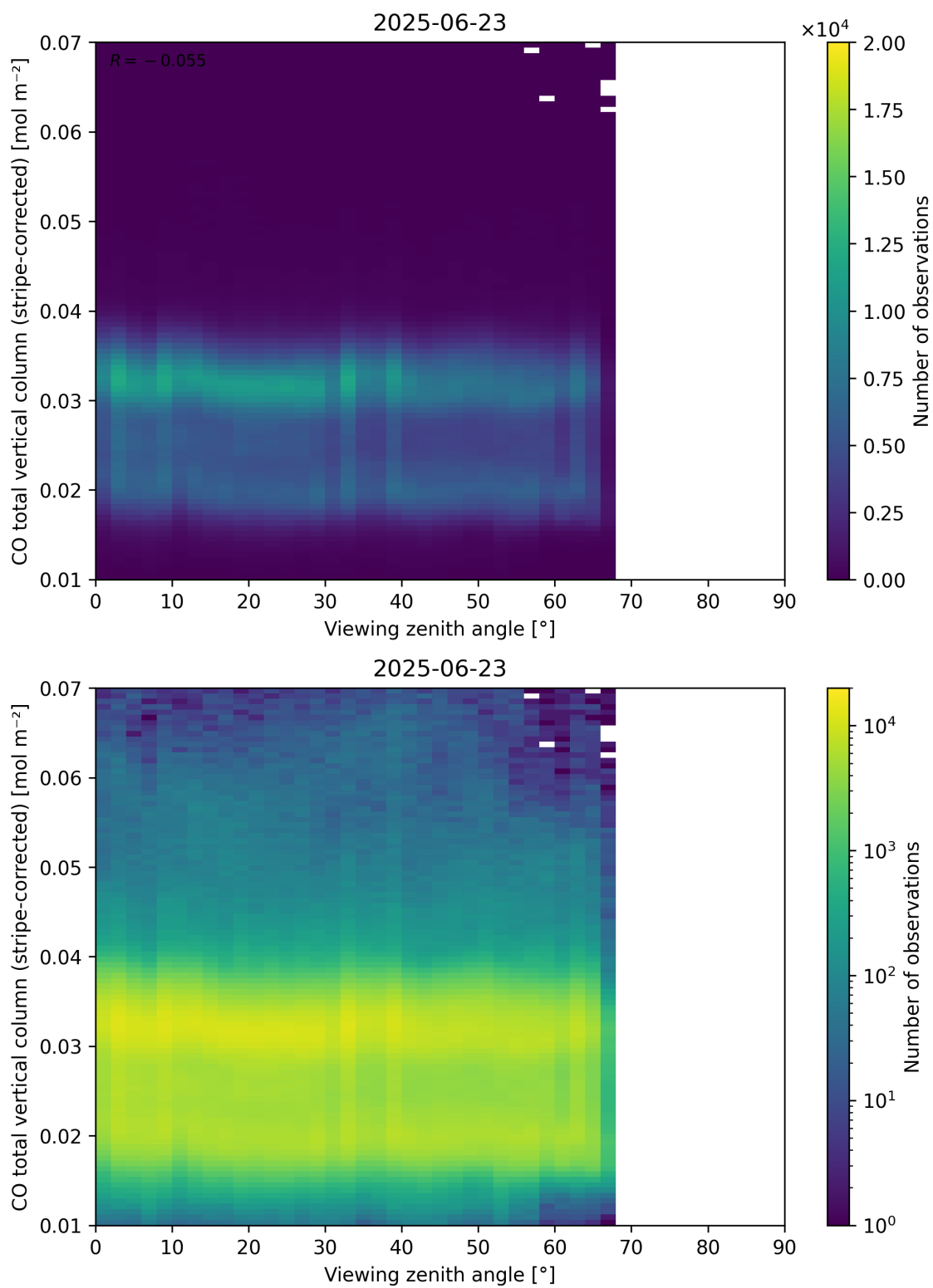
Figure 70: Scatter density plot of “Viewing zenith angle” against “CO total vertical column (stripe-corrected)” for 2025-06-22 to 2025-06-24.
