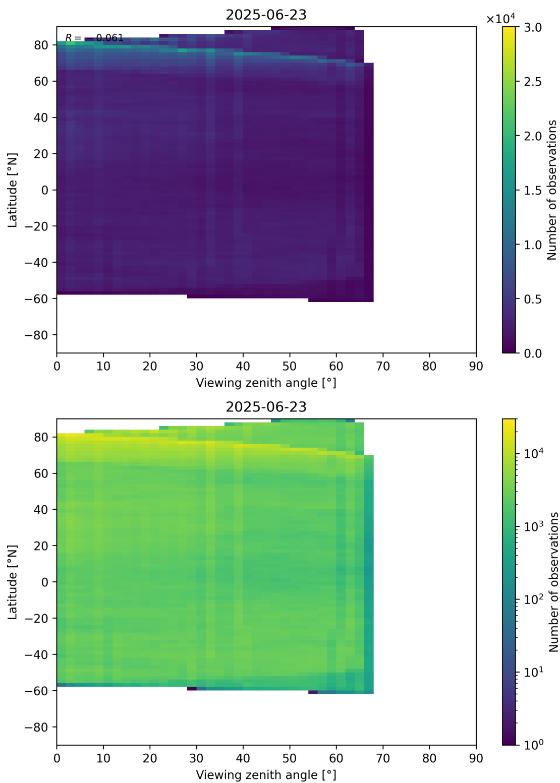
Figure 74: Scatter density plot of “Viewing zenith angle” against “Latitude” for 2025-06-22 to 2025-06-24.
