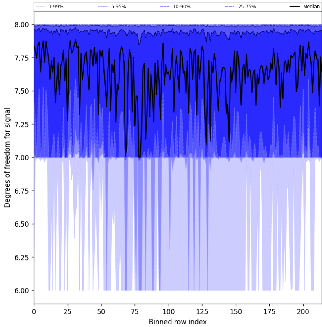
Figure 31: Along track statistics of “Degrees of freedom for signal” for 2025-06-22 to 2025-06-24
