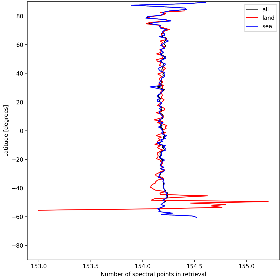
Figure 13: Zonal average of “Number of spectral points in retrieval” for 2025-06-22 to 2025-06-24.
