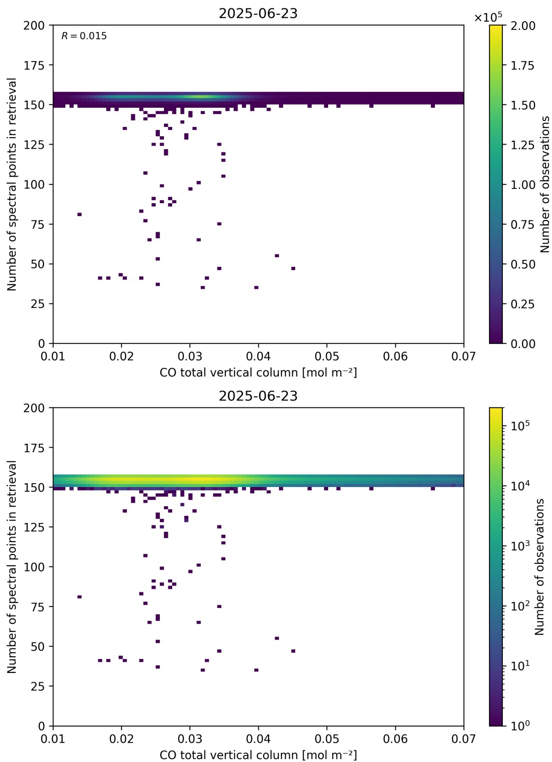
Figure 43: Scatter density plot of “CO total vertical column” against “Number of spectral points in retrieval” for 2025-06-22 to 2025-06-24.
