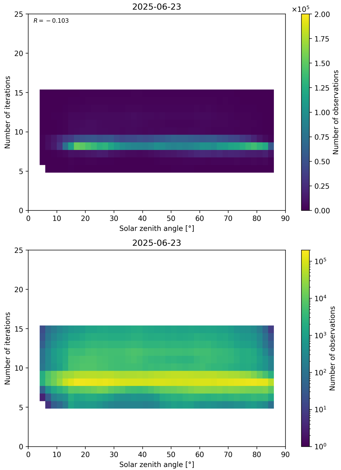
Figure 67: Scatter density plot of “Solar zenith angle” against “Number of iterations” for 2025-06-22 to 2025-06-24.
