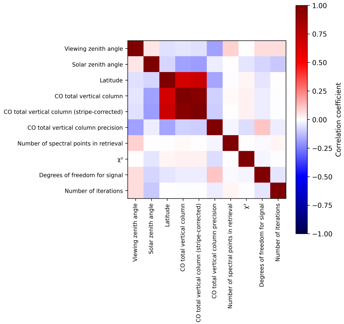
Figure 2: Map of correlation matrix for 2025-06-22 to 2025-06-24.
