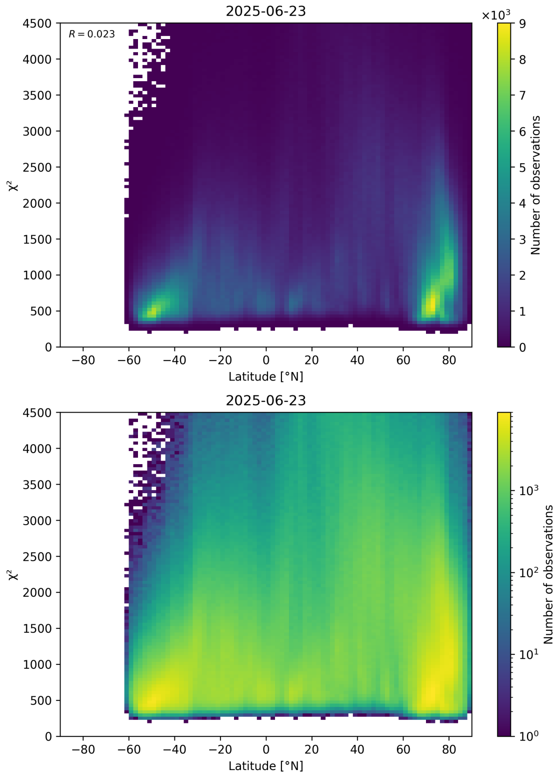
Figure 54: Scatter density plot of “Latitude” against “ \chi^2 ” for 2025-06-22 to 2025-06-24.
