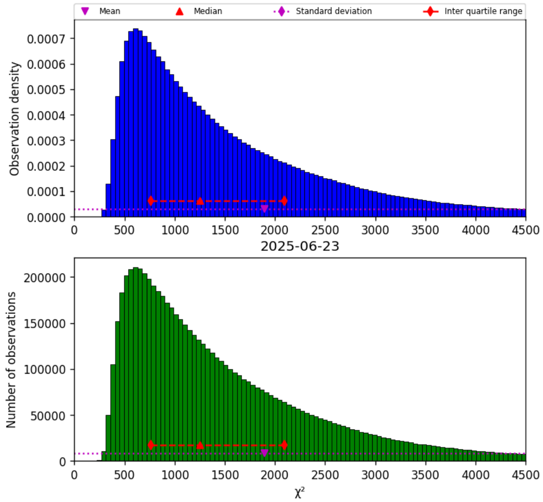
Figure 22: Histogram of “ \chi^2 ” for 2025-06-22 to 2025-06-24
