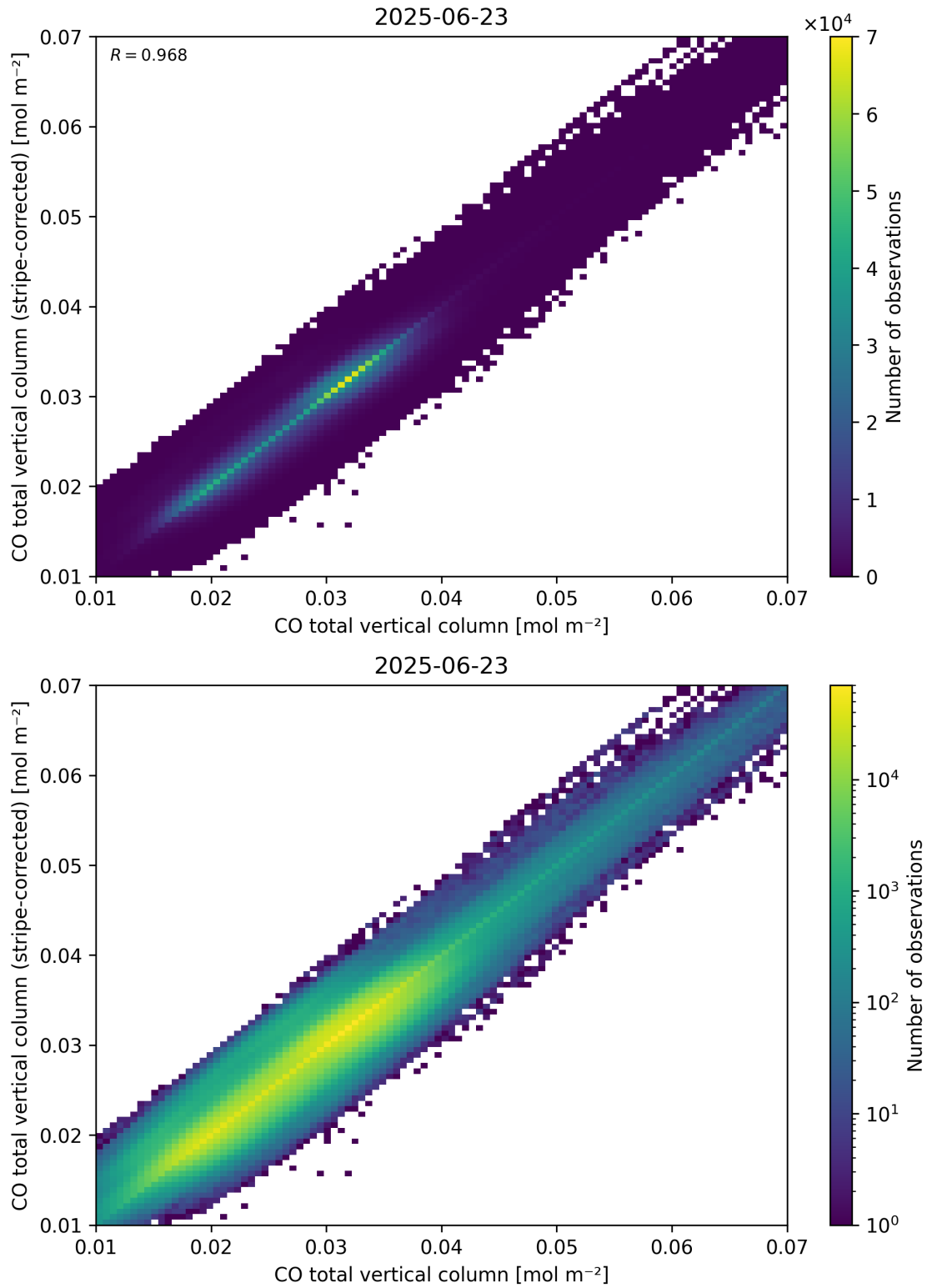
Figure 33: Scatter density plot of “CO total vertical column” against “CO total vertical column (stripe-corrected)” for 2025-06-22 to 2025-06-24.
