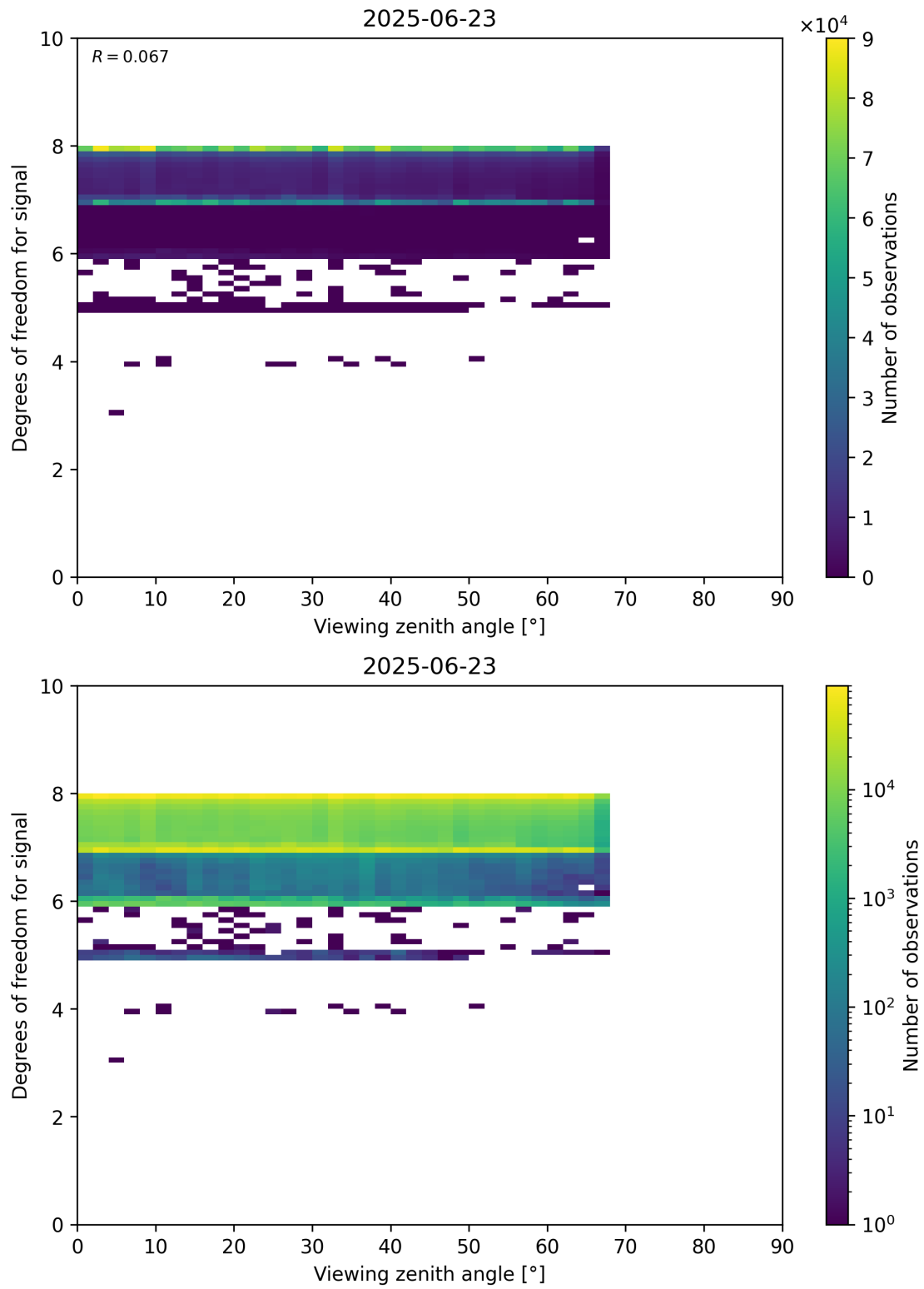
Figure 73: Scatter density plot of “Viewing zenith angle” against “Degrees of freedom for signal” for 2025-06-22 to 2025-06-24.
