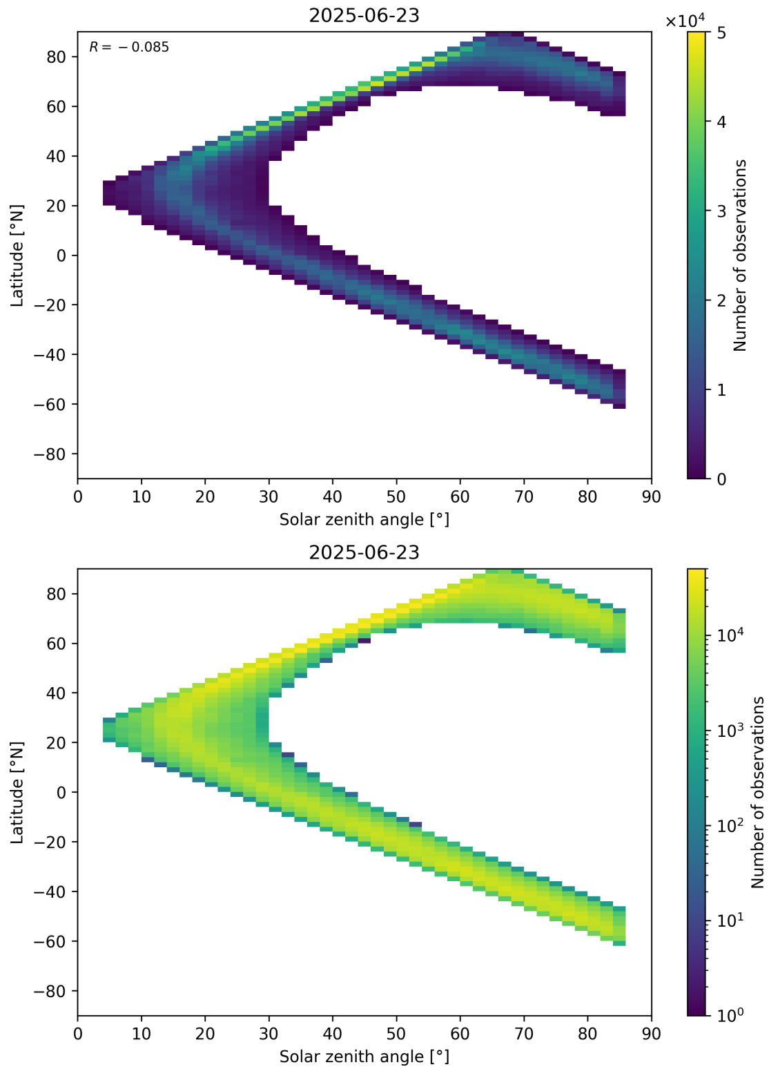
Figure 66: Scatter density plot of “Solar zenith angle” against “Latitude” for 2025-06-22 to 2025-06-24.
