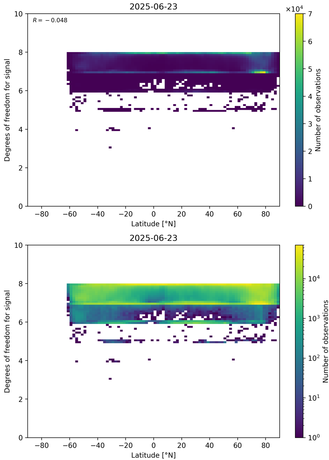
Figure 55: Scatter density plot of “Latitude” against “Degrees of freedom for signal” for 2025-06-22 to 2025-06-24.
