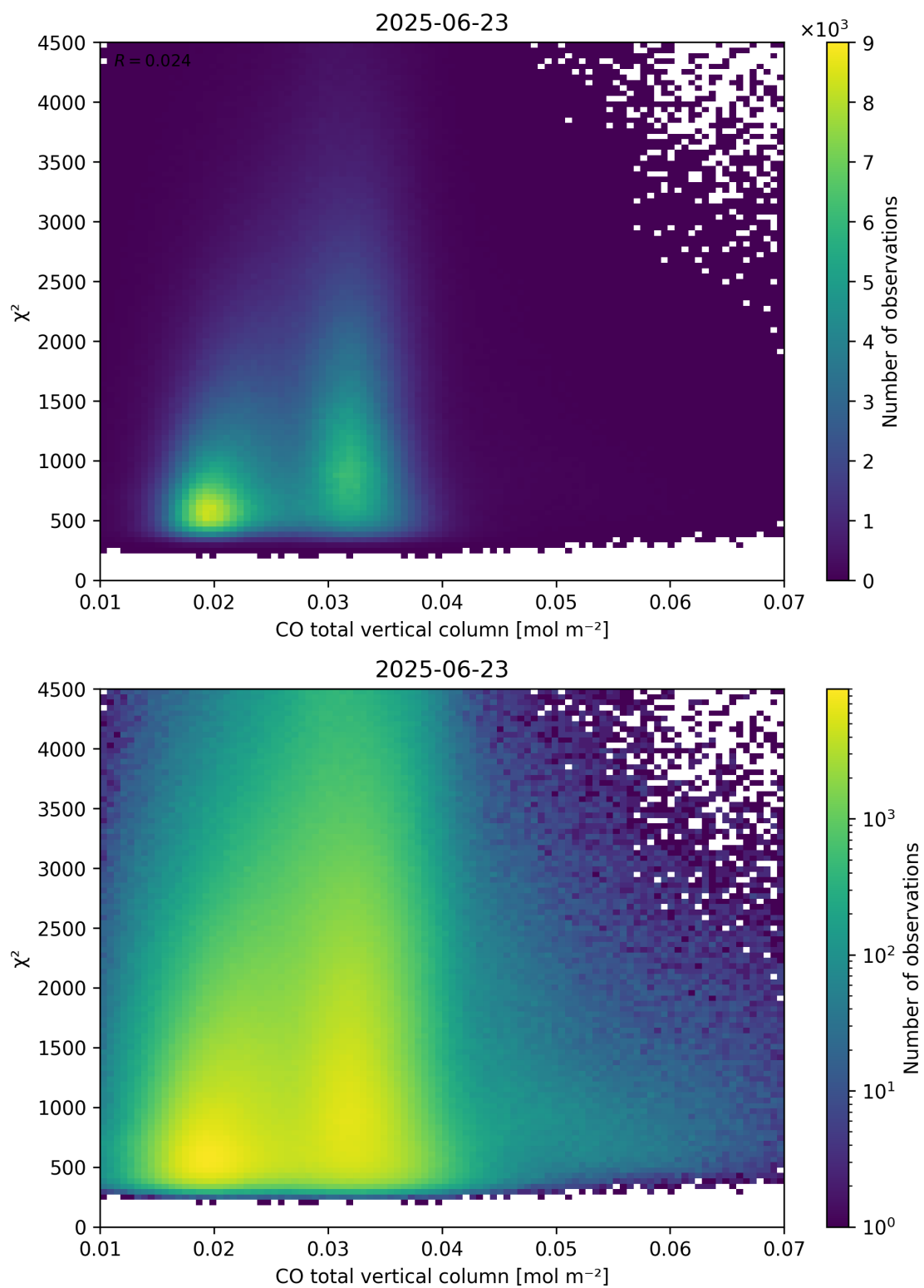
Figure 35: Scatter density plot of “CO total vertical column” against “ \chi^2 ” for 2025-06-22 to 2025-06-24.
