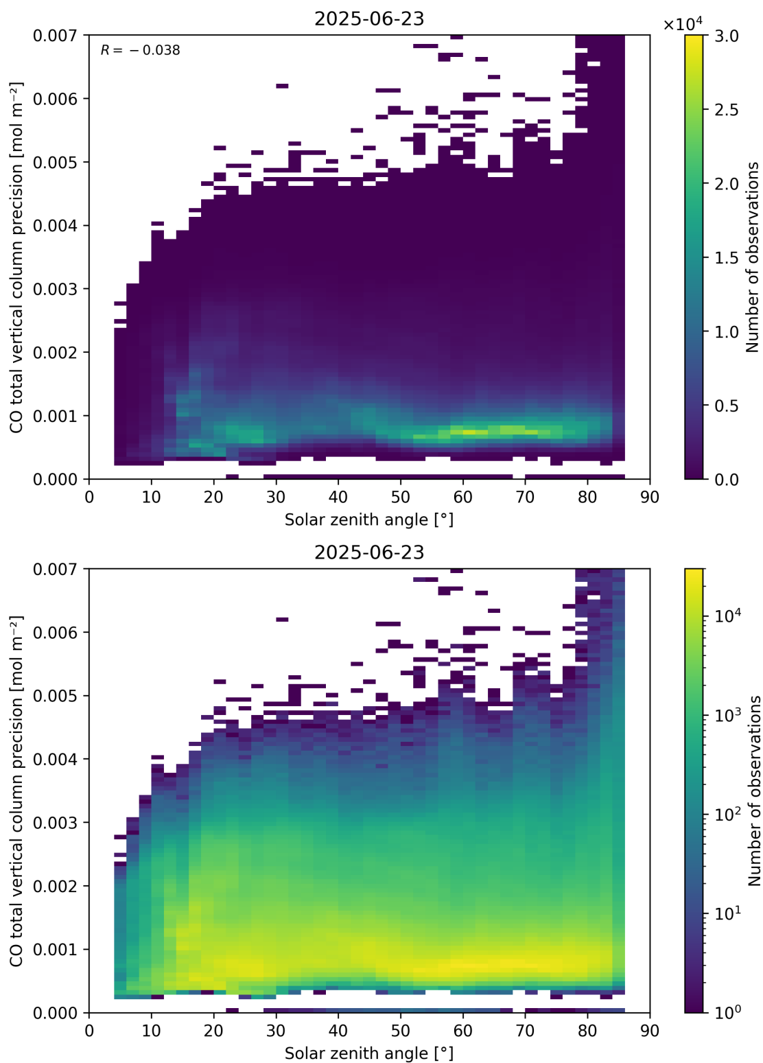
Figure 63: Scatter density plot of “Solar zenith angle” against “CO total vertical column precision” for 2025-06-22 to 2025-06-24.
