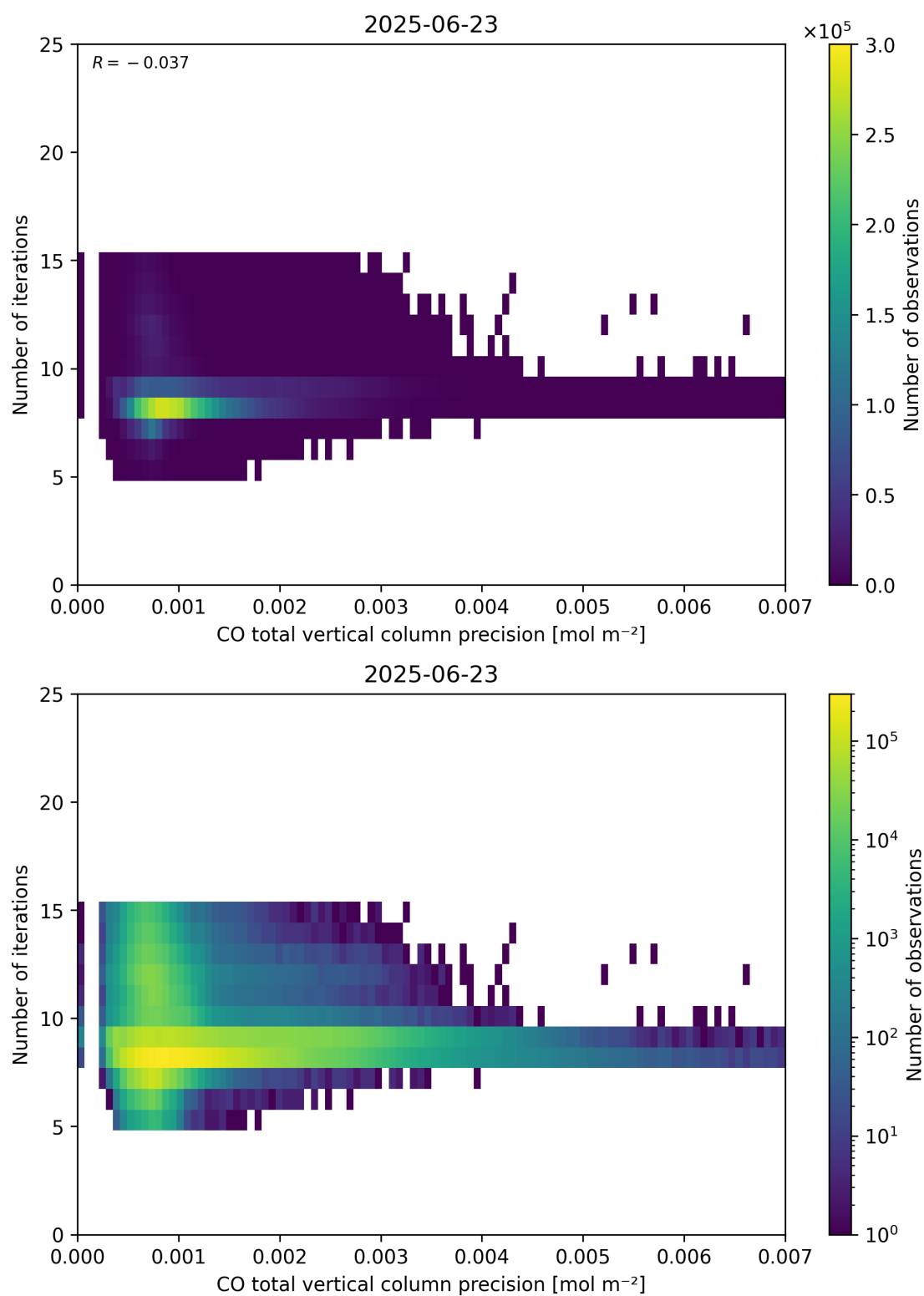
Figure 46: Scatter density plot of “CO total vertical column precision” against “Number of iterations” for 2025-06-22 to 2025-06-24.
