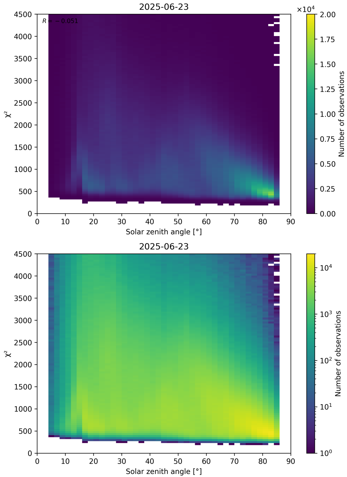
Figure 64: Scatter density plot of “Solar zenith angle” against “ \chi^2 ” for 2025-06-22 to 2025-06-24.
