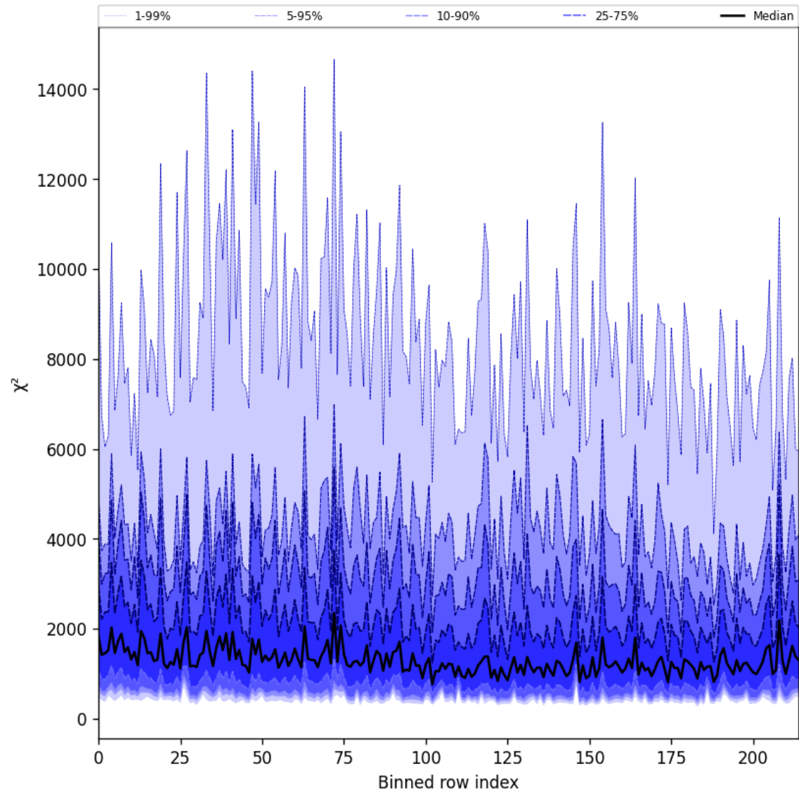
Figure 30: Along track statistics of “ \chi^2 ” for 2025-06-22 to 2025-06-24
