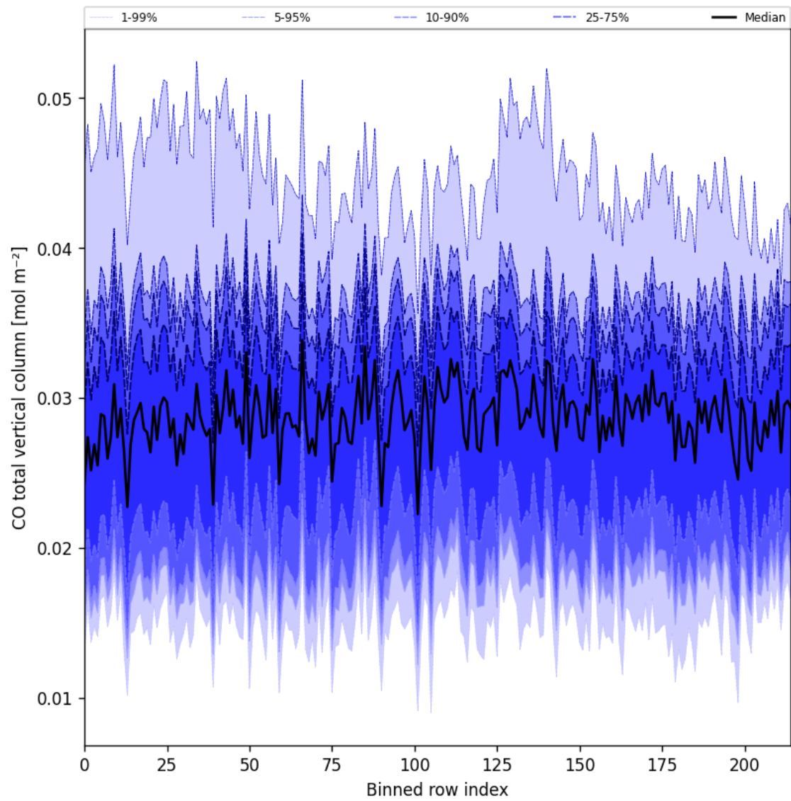
Figure 26: Along track statistics of “CO total vertical column” for 2025-06-22 to 2025-06-24
