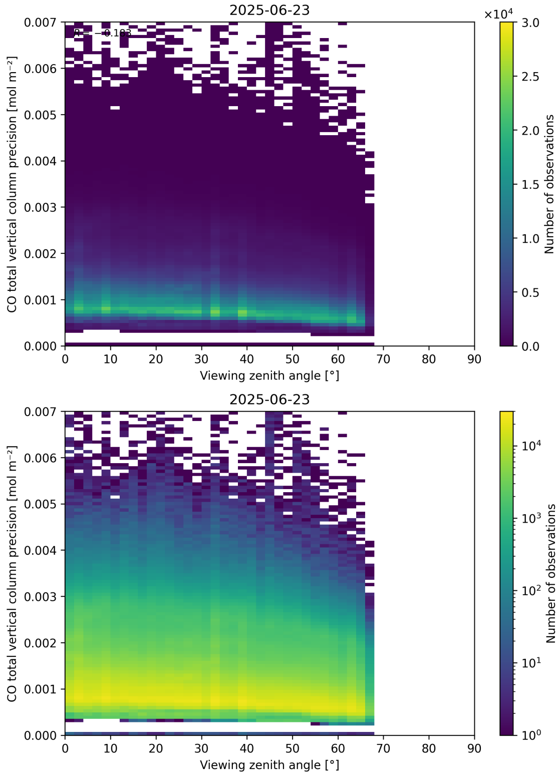
Figure 71: Scatter density plot of “Viewing zenith angle” against “CO total vertical column precision” for 2025-06-22 to 2025-06-24.
