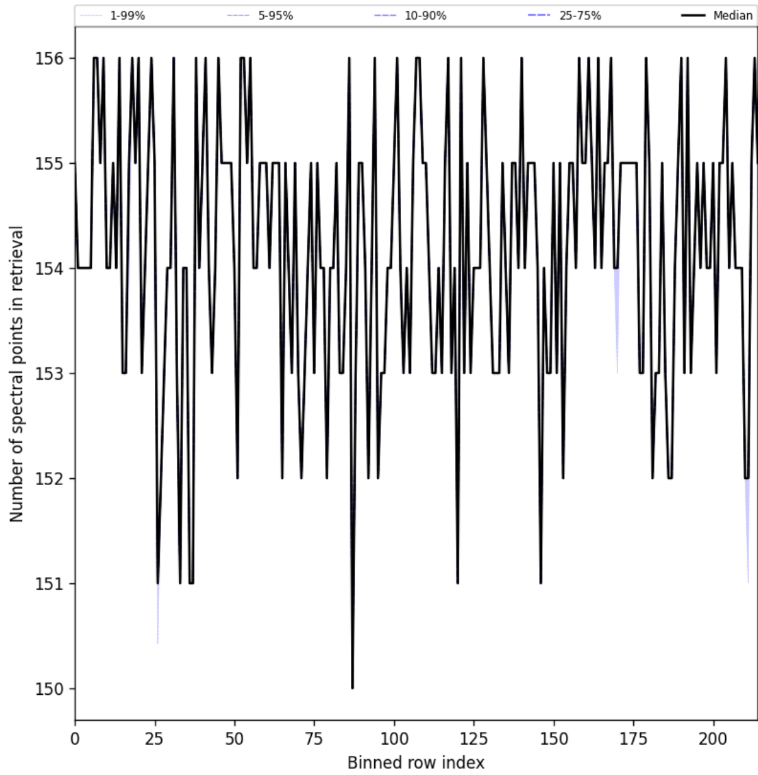
Figure 29: Along track statistics of “Number of spectral points in retrieval” for 2025-06-22 to 2025-06-24
