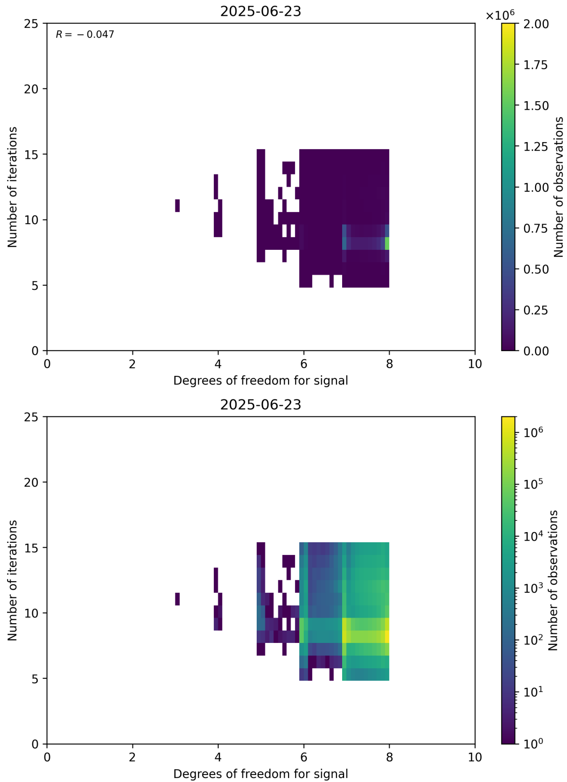
Figure 50: Scatter density plot of “Degrees of freedom for signal” against “Number of iterations” for 2025-06-22 to 2025-06-24.
