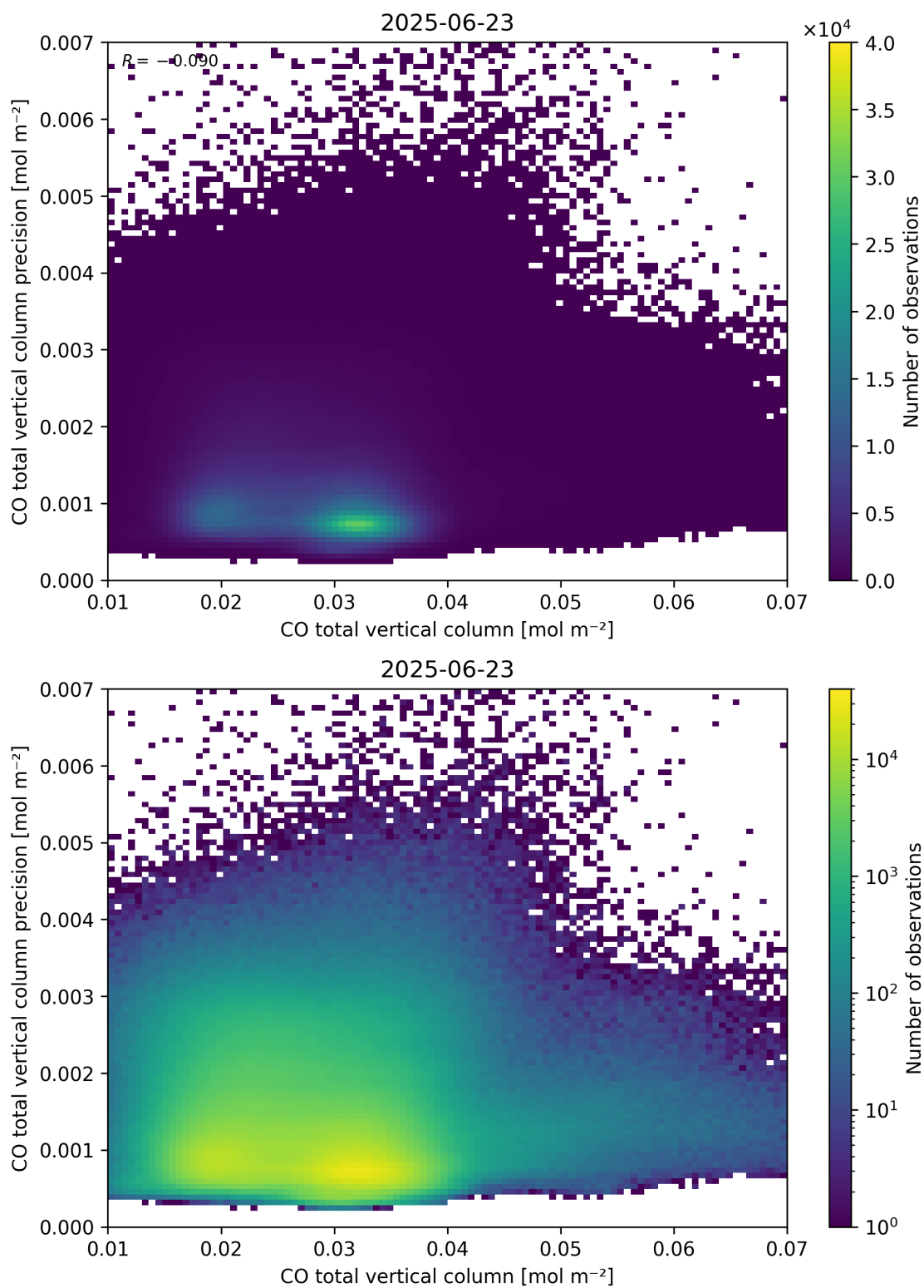
Figure 34: Scatter density plot of “CO total vertical column” against “CO total vertical column precision” for 2025-06-22 to 2025-06-24.
