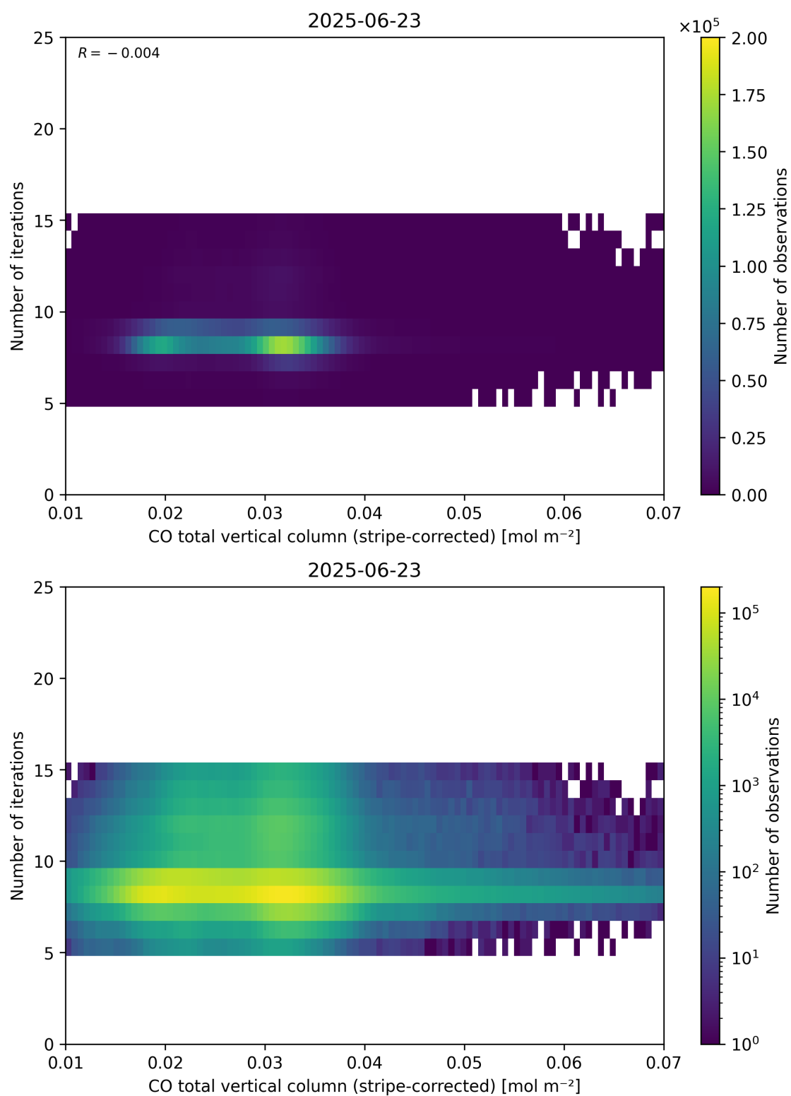
Figure 39: Scatter density plot of “CO total vertical column (stripe-corrected)” against “Number of iterations” for 2025-06-22 to 2025-06-24.
