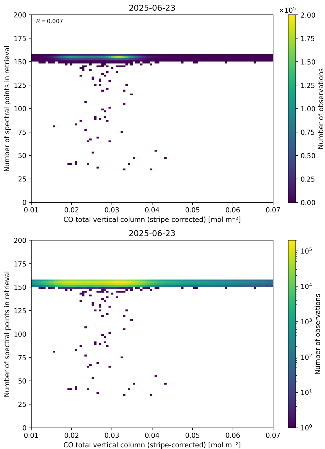
Figure 40: Scatter density plot of “CO total vertical column (stripe-corrected)” against “Number of spectral points in retrieval” for 2025-06-22 to 2025-06-24.
