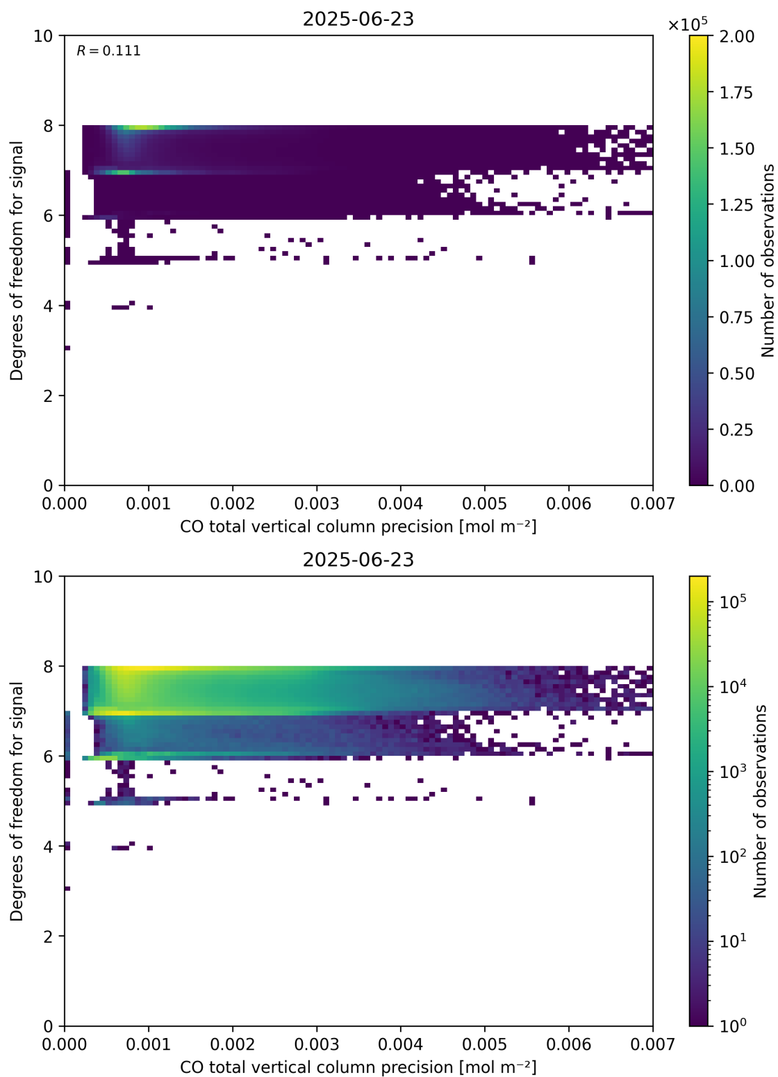
Figure 45: Scatter density plot of “CO total vertical column precision” against “Degrees of freedom for signal” for 2025-06-22 to 2025-06-24.
