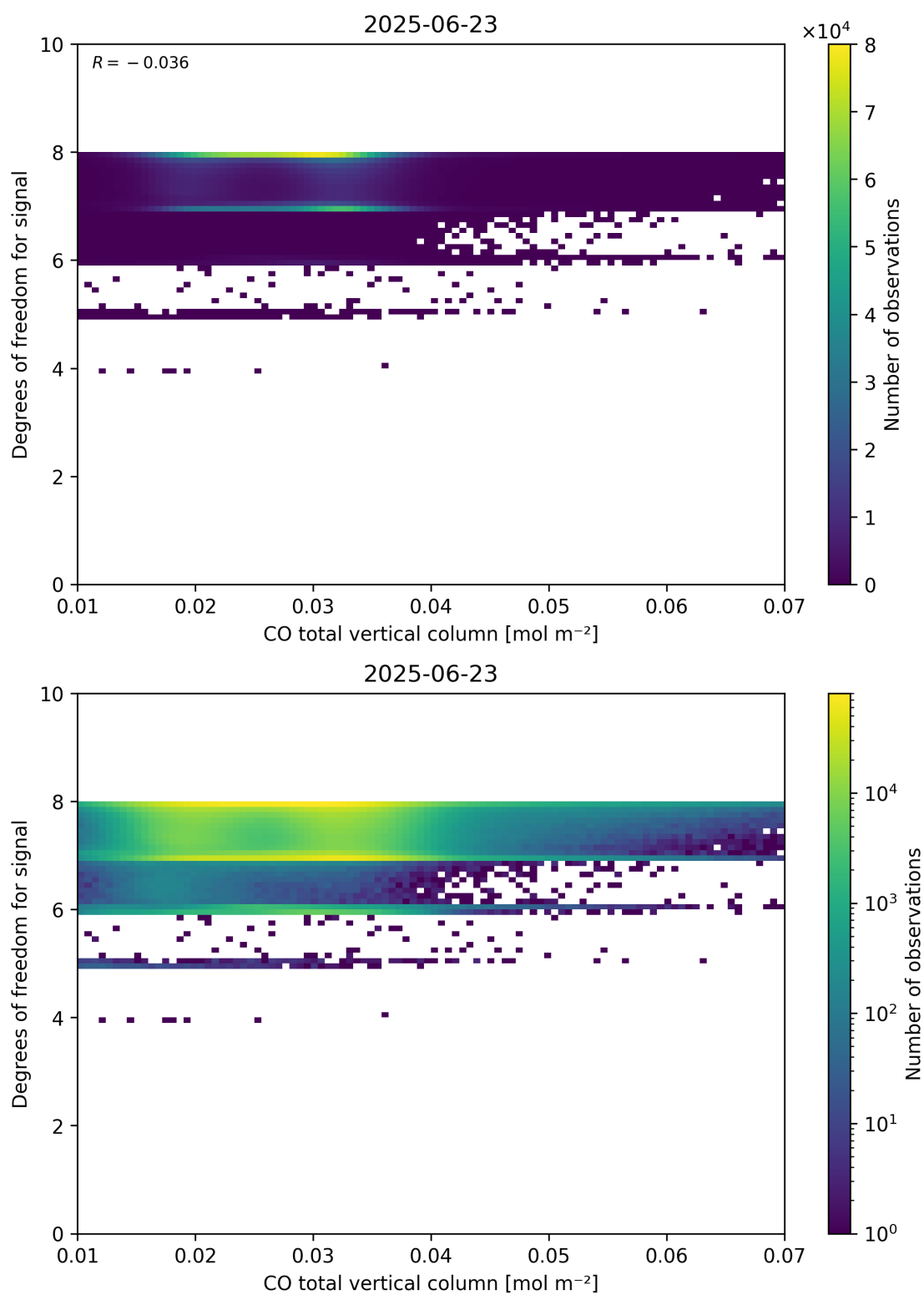
Figure 41: Scatter density plot of “CO total vertical column” against “Degrees of freedom for signal” for 2025-06-22 to 2025-06-24.
