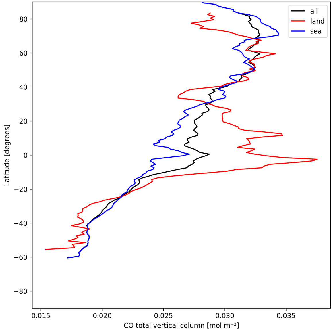
Figure 10: Zonal average of “CO total vertical column” for 2025-06-22 to 2025-06-24.
