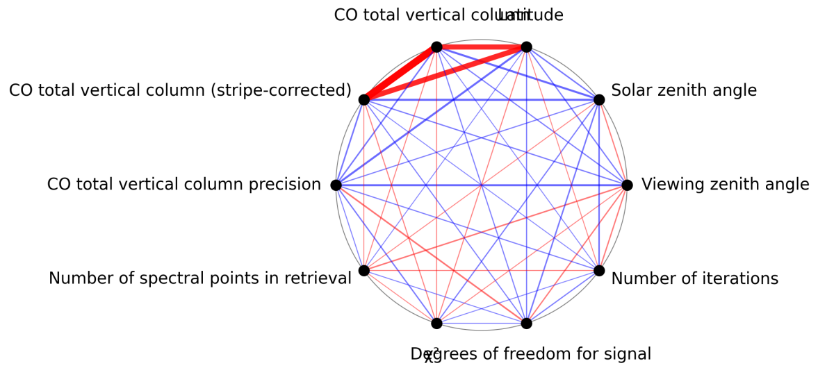
Figure 1: Map of correlation graph for 2025-06-22 to 2025-06-24.
