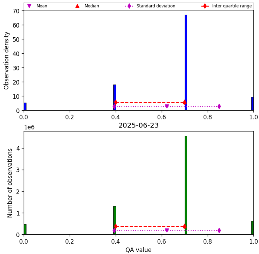
Figure 17: Histogram of “QA value” for 2025-06-22 to 2025-06-24
