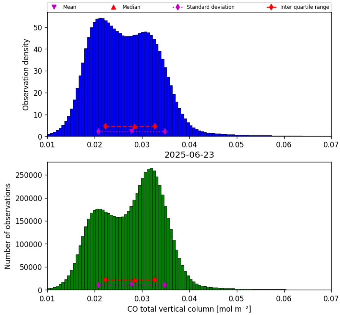
Figure 18: Histogram of “CO total vertical column” for 2025-06-22 to 2025-06-24
