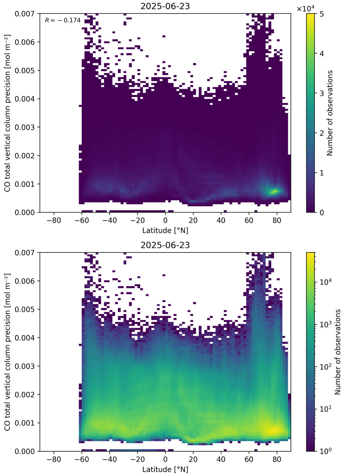
Figure 53: Scatter density plot of “Latitude” against “CO total vertical column precision” for 2025-06-22 to 2025-06-24.
