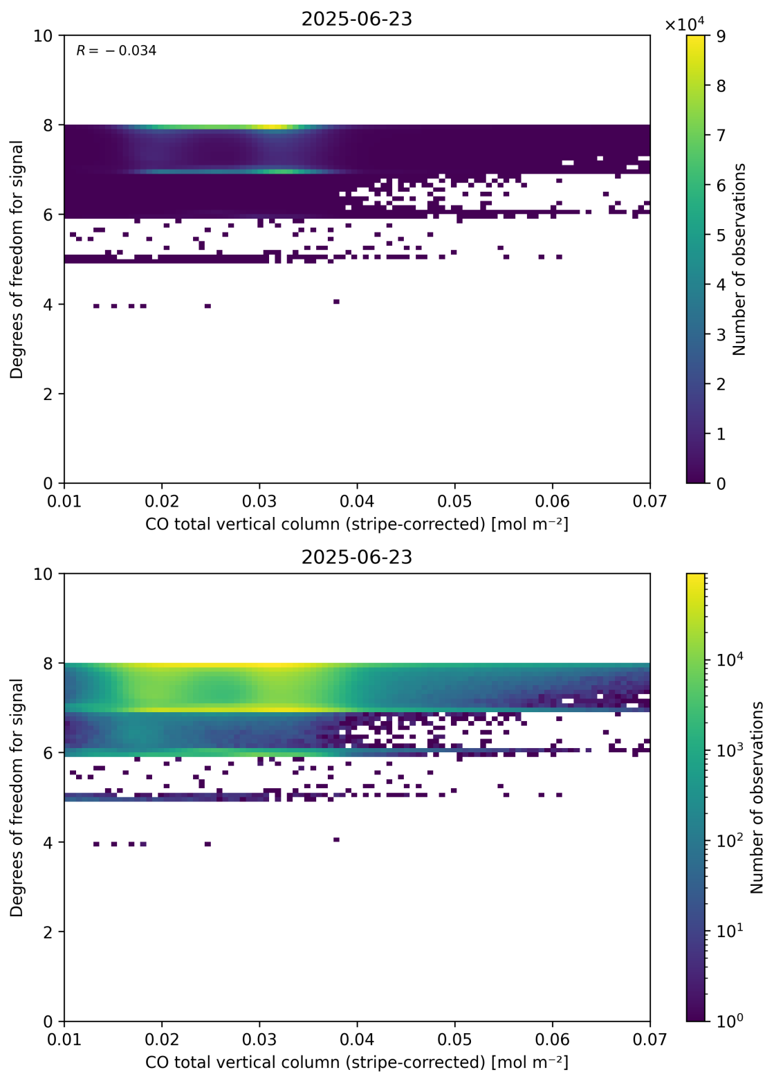
Figure 38: Scatter density plot of “CO total vertical column (stripe-corrected)” against “Degrees of freedom for signal” for 2025-06-22 to 2025-06-24.
