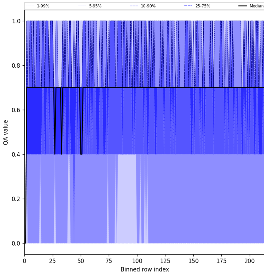
Figure 25: Along track statistics of “QA value” for 2025-06-22 to 2025-06-24
