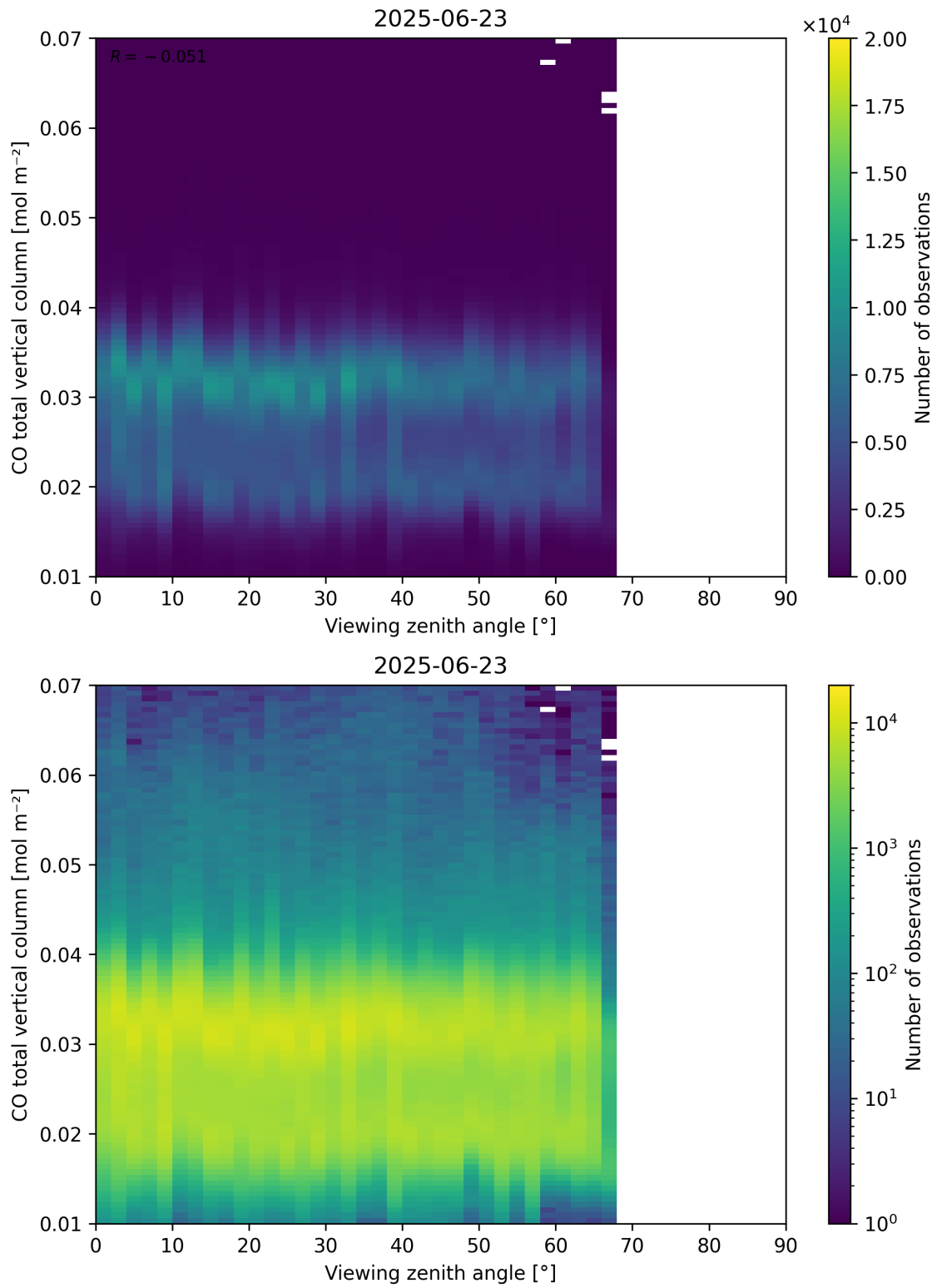
Figure 69: Scatter density plot of “Viewing zenith angle” against “CO total vertical column” for 2025-06-22 to 2025-06-24.
