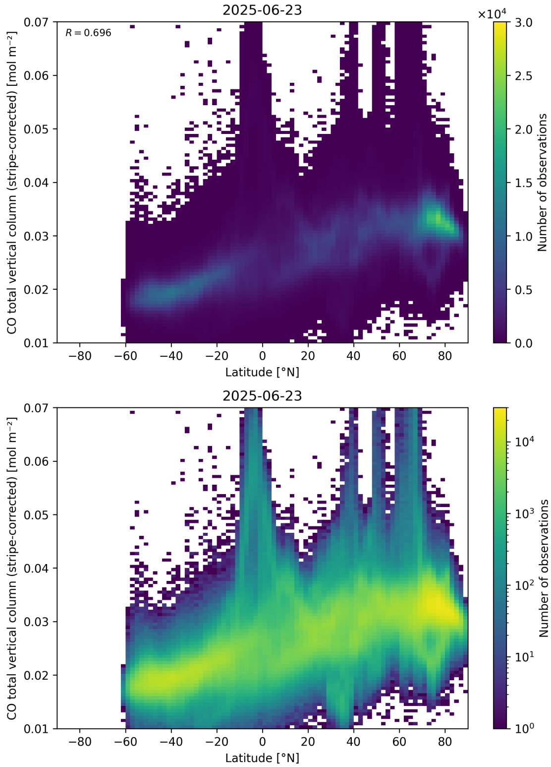
Figure 52: Scatter density plot of “Latitude” against “CO total vertical column (stripe-corrected)” for 2025-06-22 to 2025-06-24.
