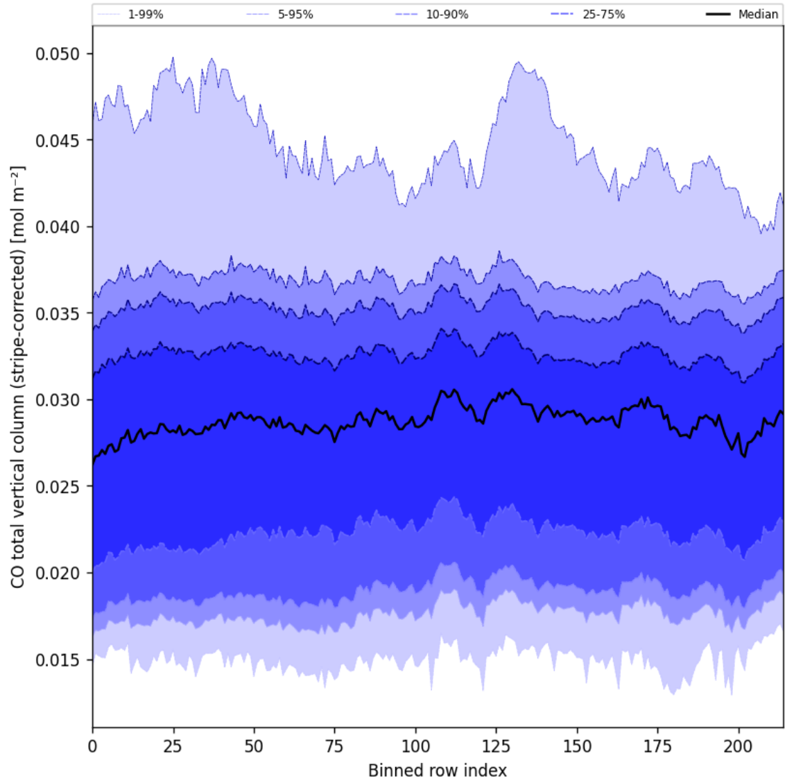
Figure 27: Along track statistics of “CO total vertical column (stripe-corrected)” for 2025-06-22 to 2025-06-24
