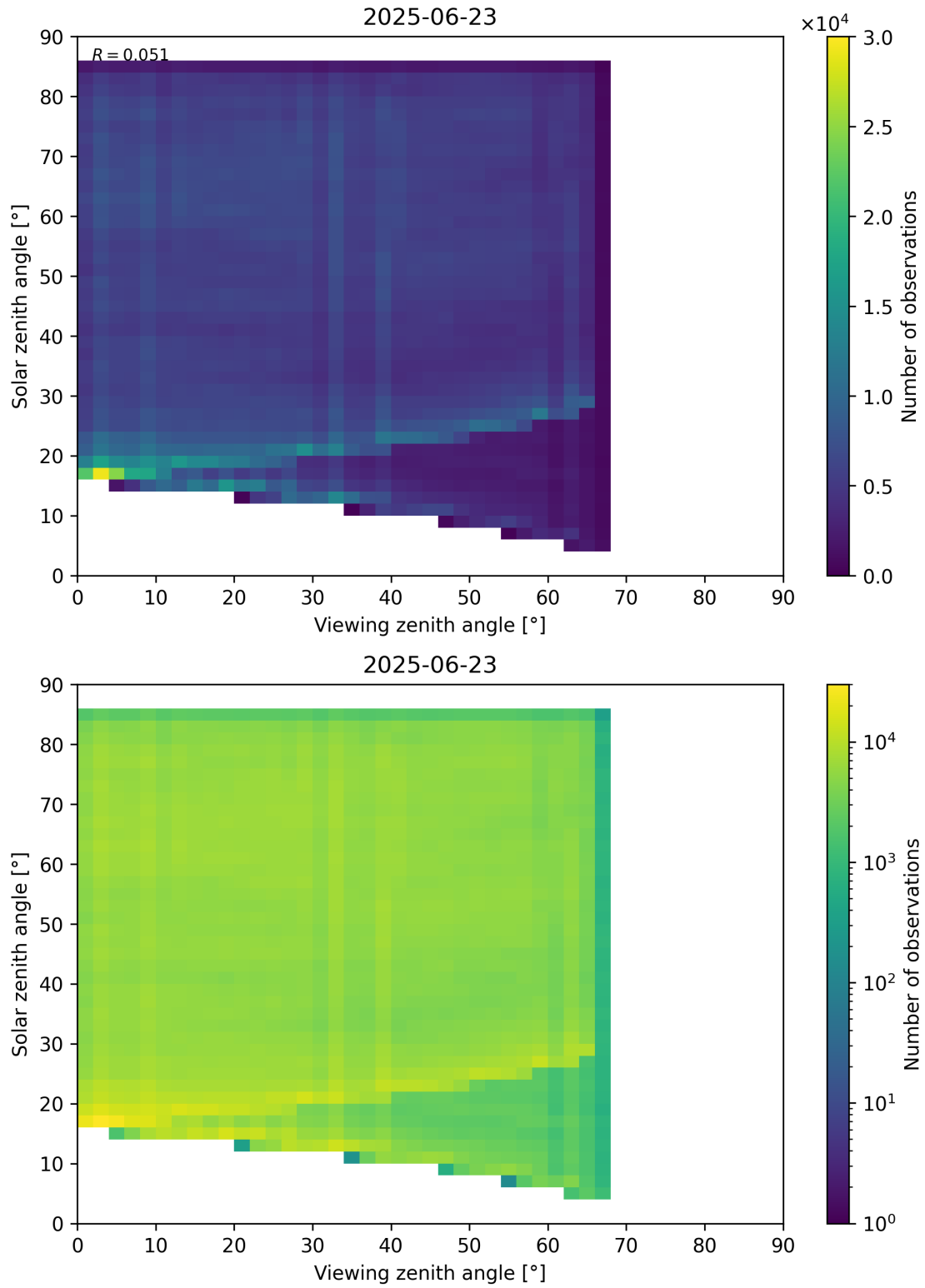
Figure 77: Scatter density plot of “Viewing zenith angle” against “Solar zenith angle” for 2025-06-22 to 2025-06-24.
