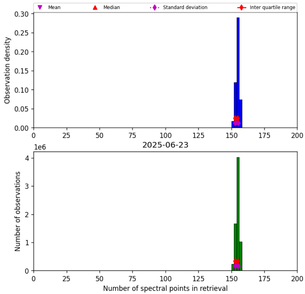
Figure 21: Histogram of “Number of spectral points in retrieval” for 2025-06-22 to 2025-06-24
