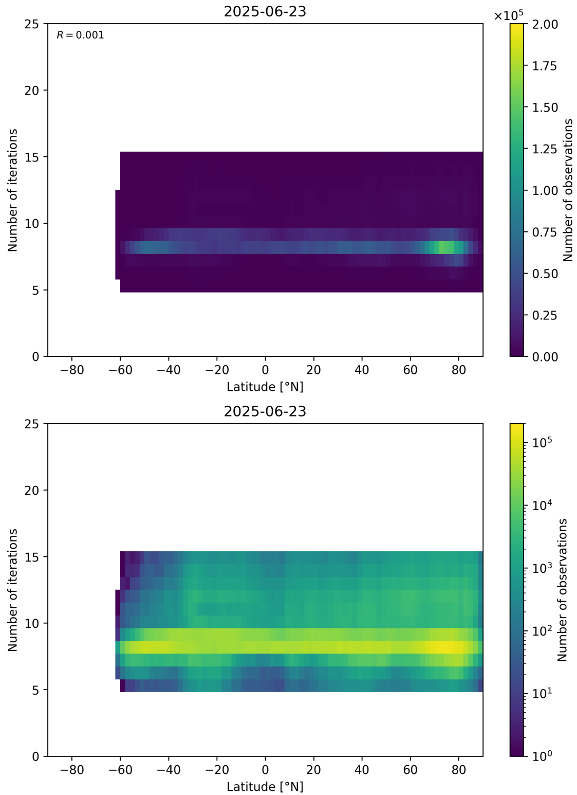
Figure 56: Scatter density plot of “Latitude” against “Number of iterations” for 2025-06-22 to 2025-06-24.
