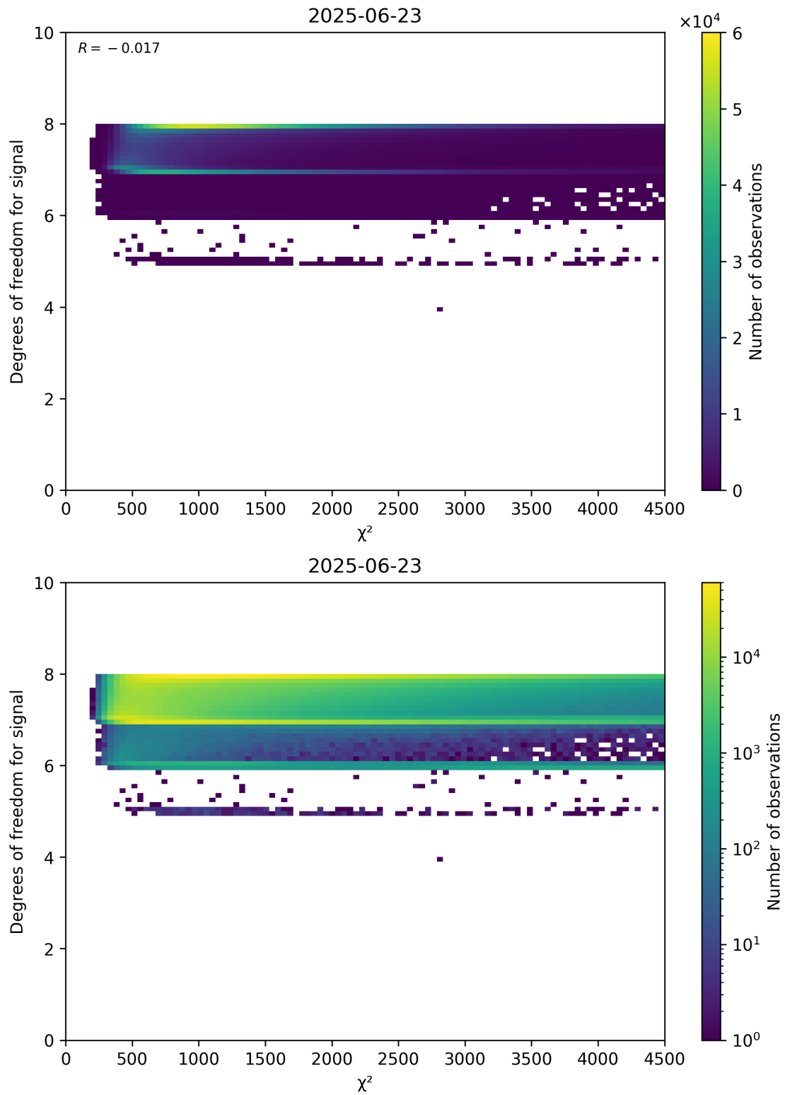
Figure 48: Scatter density plot of “ \chi^2 ” against “Degrees of freedom for signal” for 2025-06-22 to 2025-06-24.
