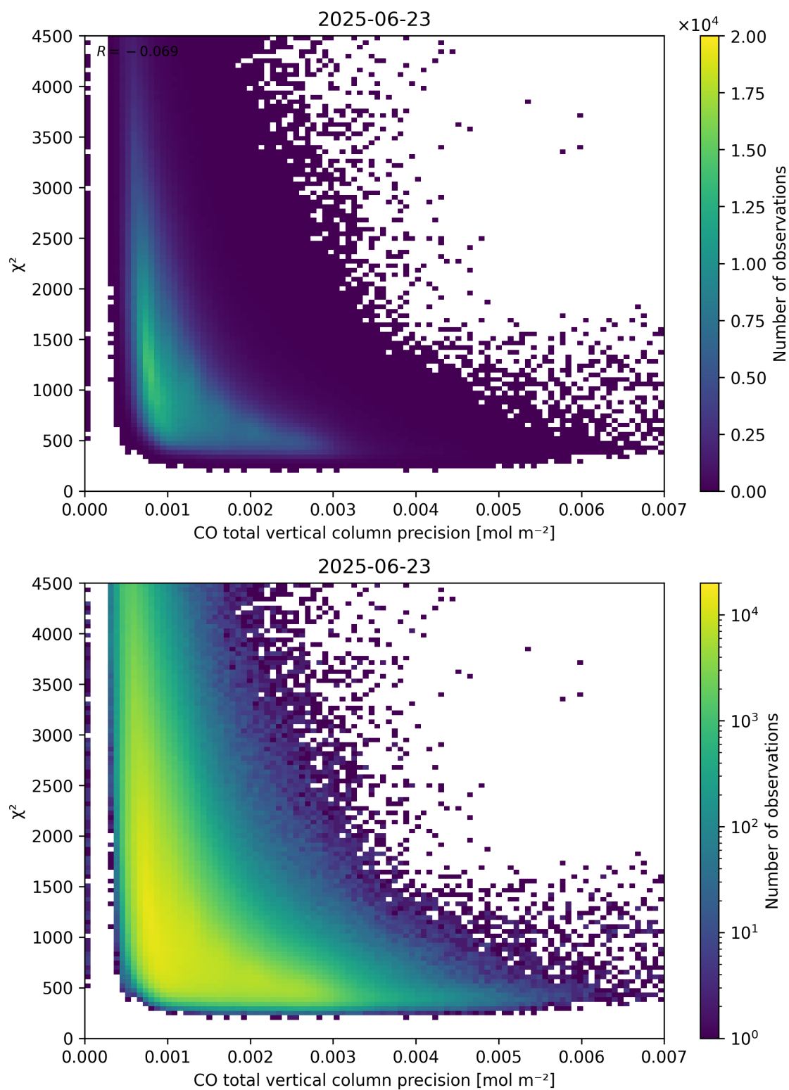
Figure 44: Scatter density plot of “CO total vertical column precision” against “ \chi^2 ” for 2025-06-22 to 2025-06-24.
