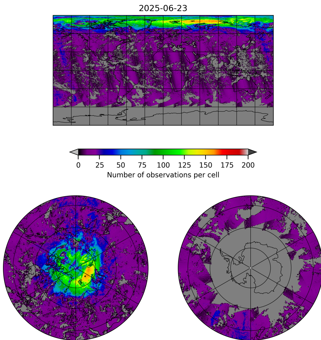
Figure 8: Map of the number of observations for 2025-06-22 to 2025-06-24
