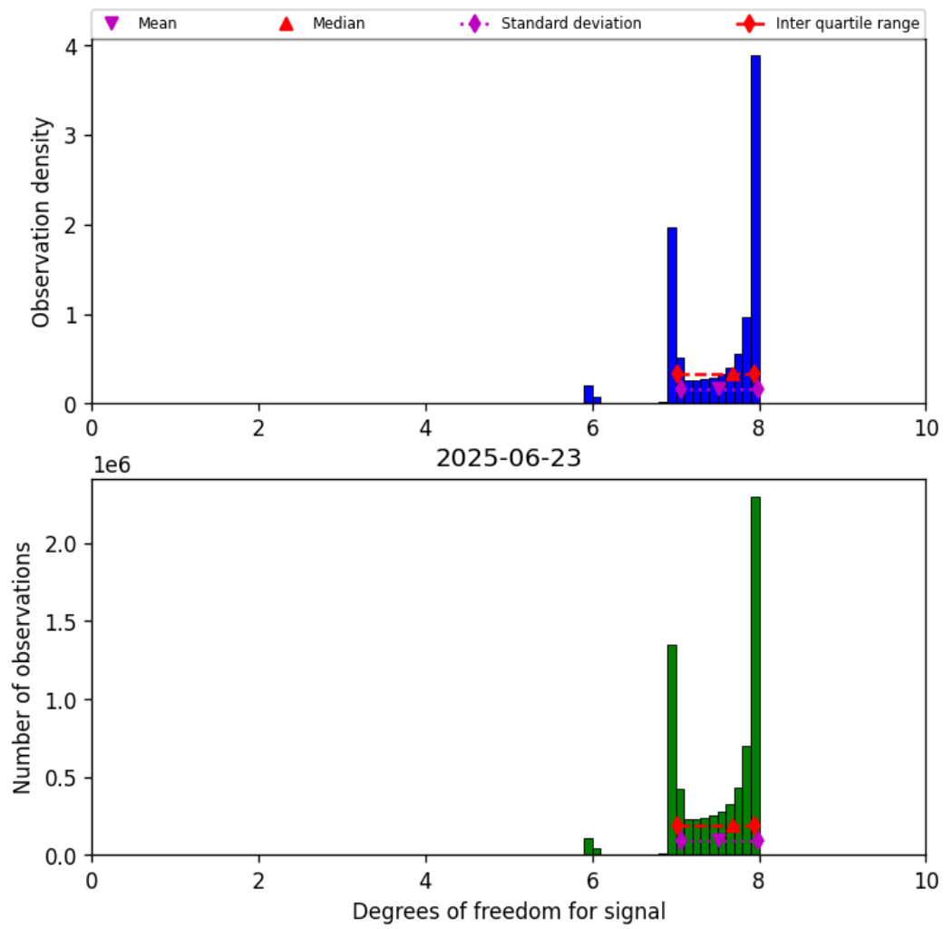
Figure 23: Histogram of “Degrees of freedom for signal” for 2025-06-22 to 2025-06-24
