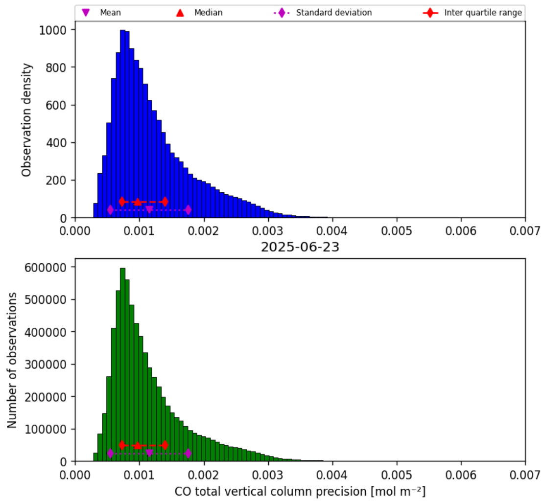
Figure 20: Histogram of “CO total vertical column precision” for 2025-06-22 to 2025-06-24
