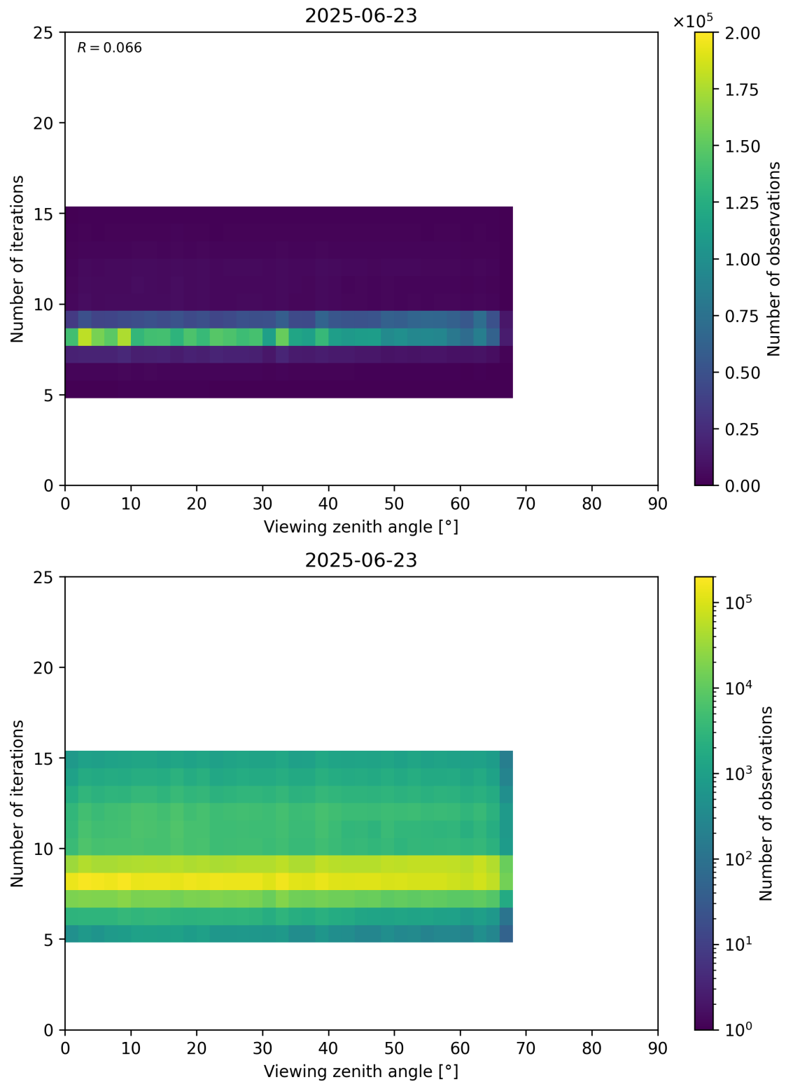
Figure 75: Scatter density plot of “Viewing zenith angle” against “Number of iterations” for 2025-06-22 to 2025-06-24.
