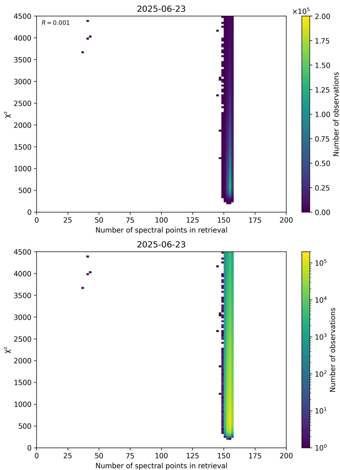
Figure 58: Scatter density plot of “Number of spectral points in retrieval” against “ \chi^2 ” for 2025-06-22 to 2025-06-24.
