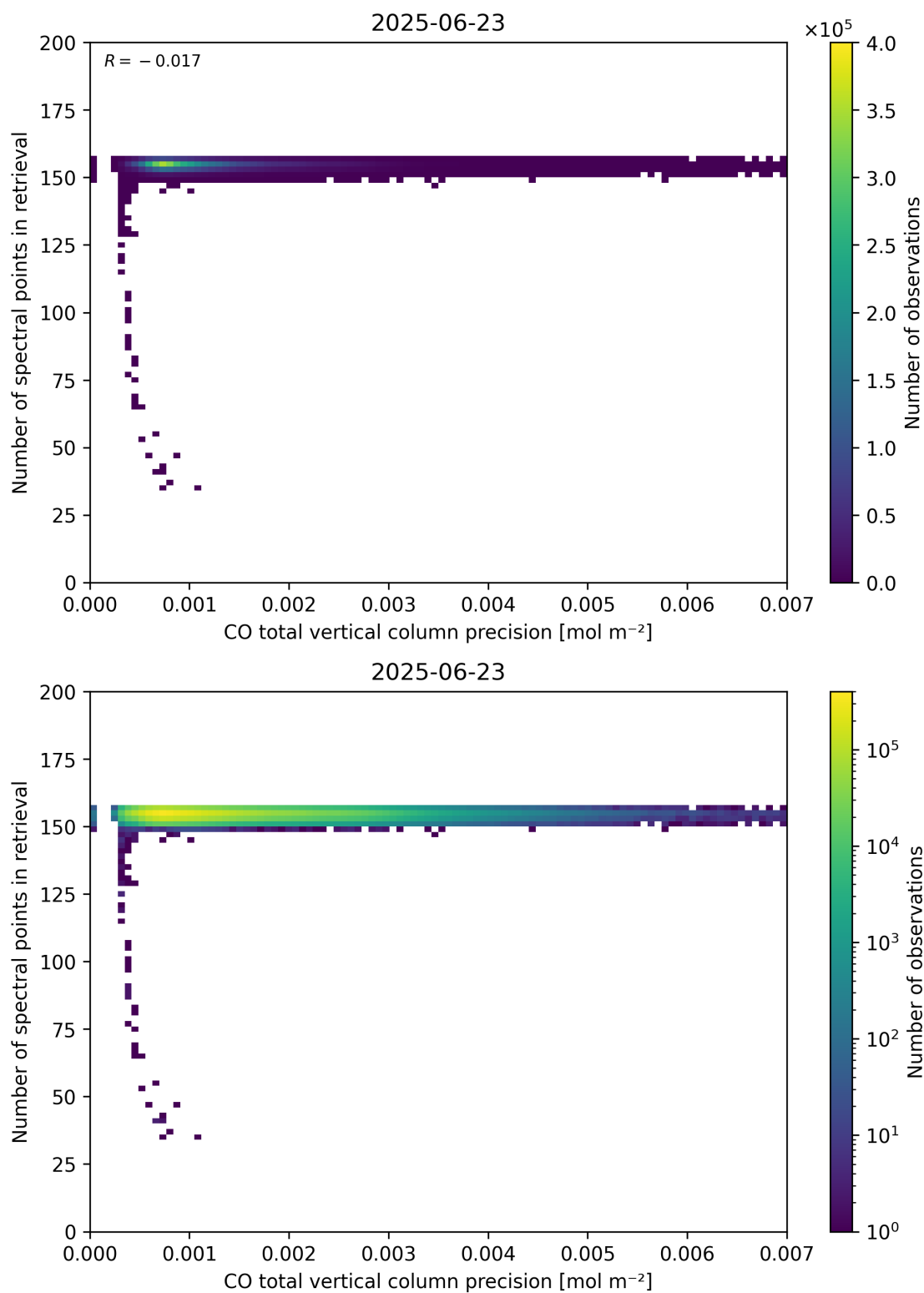
Figure 47: Scatter density plot of “CO total vertical column precision” against “Number of spectral points in retrieval” for 2025-06-22 to 2025-06-24.
