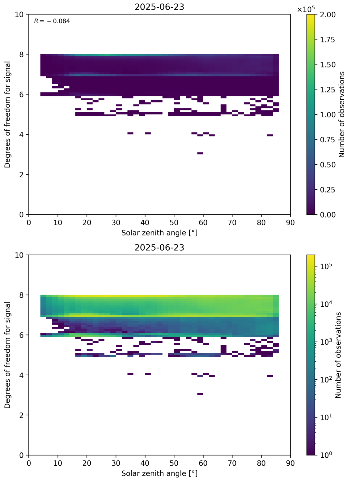
Figure 65: Scatter density plot of “Solar zenith angle” against “Degrees of freedom for signal” for 2025-06-22 to 2025-06-24.
