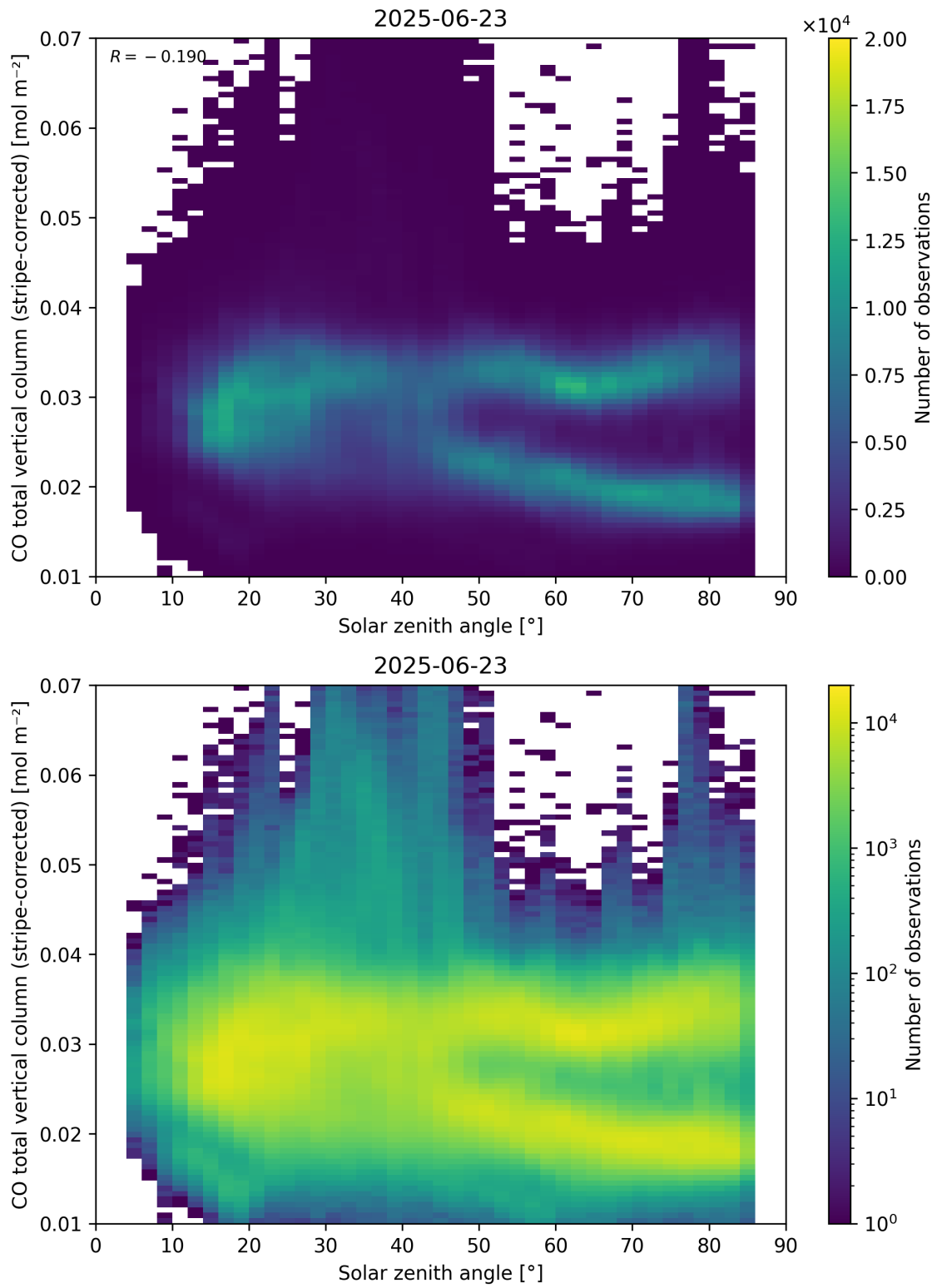
Figure 62: Scatter density plot of “Solar zenith angle” against “CO total vertical column (stripe-corrected)” for 2025-06-22 to 2025-06-24.
