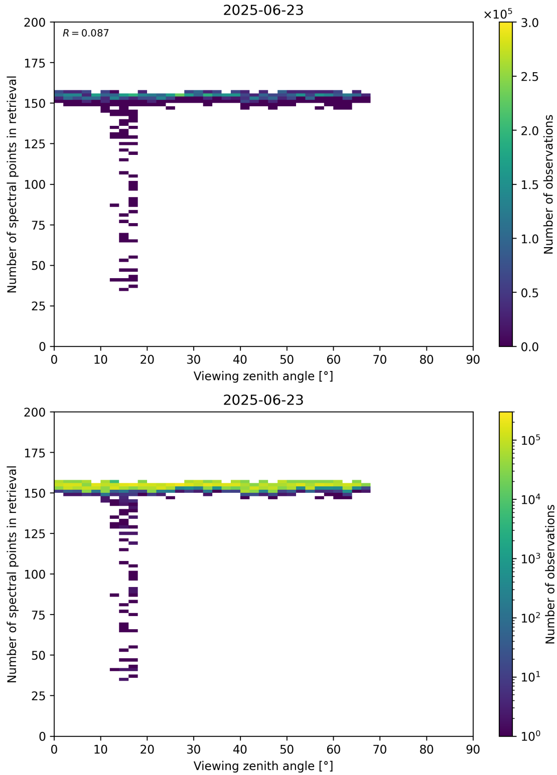
Figure 76: Scatter density plot of “Viewing zenith angle” against “Number of spectral points in retrieval” for 2025-06-22 to 2025-06-24.
