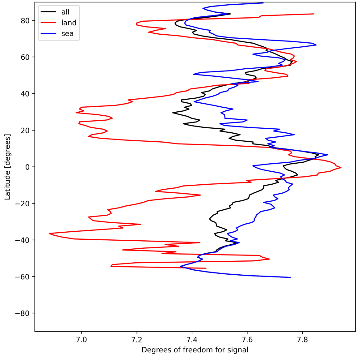
Figure 15: Zonal average of “Degrees of freedom for signal” for 2025-06-22 to 2025-06-24.
