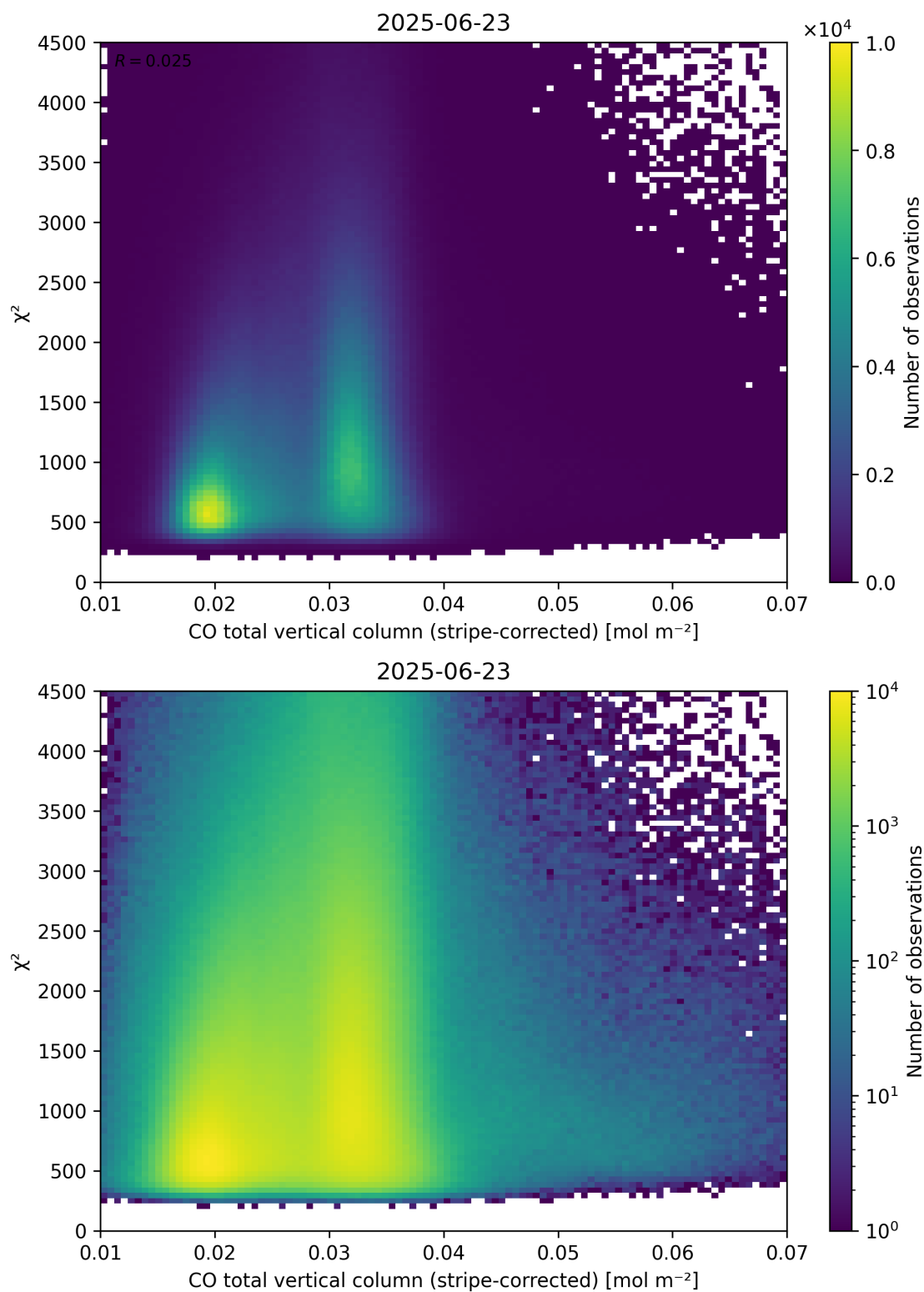
Figure 37: Scatter density plot of “CO total vertical column (stripe-corrected)” against “ \chi^2 ” for 2025-06-22 to 2025-06-24.
