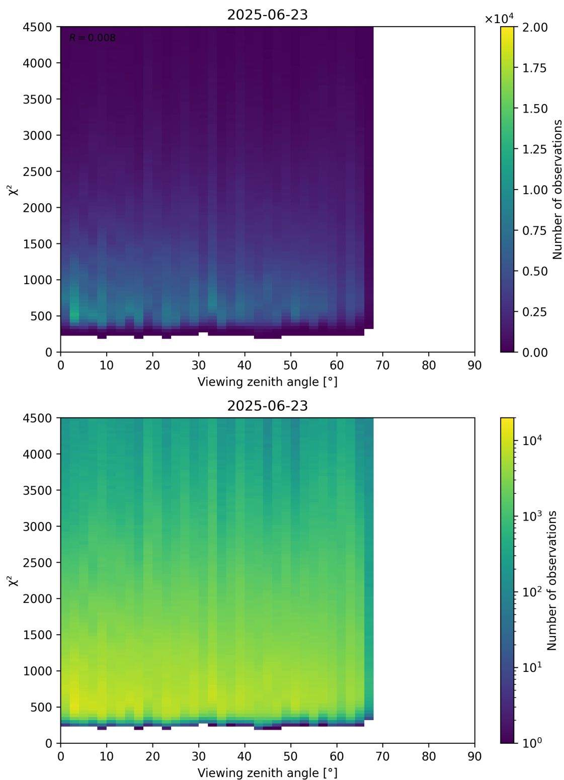
Figure 72: Scatter density plot of “Viewing zenith angle” against “ \chi^2 ” for 2025-06-22 to 2025-06-24.
