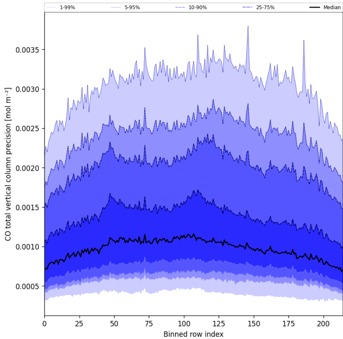
Figure 28: Along track statistics of “CO total vertical column precision” for 2025-06-22 to 2025-06-24
