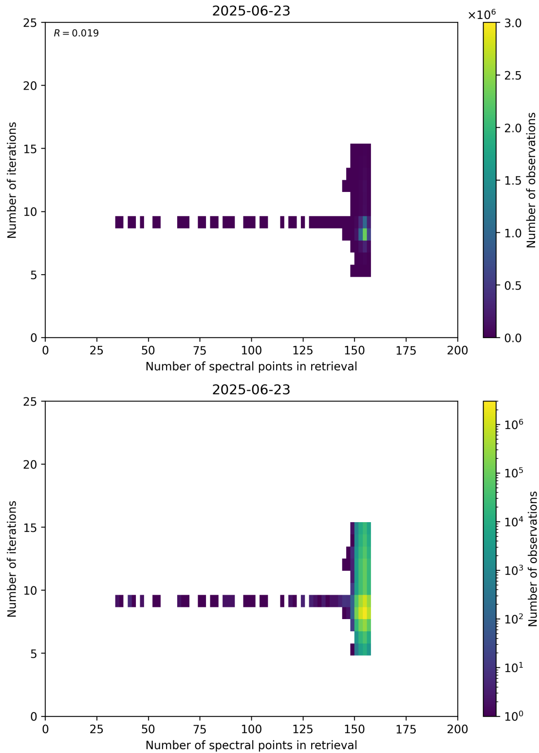
Figure 60: Scatter density plot of “Number of spectral points in retrieval” against “Number of iterations” for 2025-06-22 to 2025-06-24.
