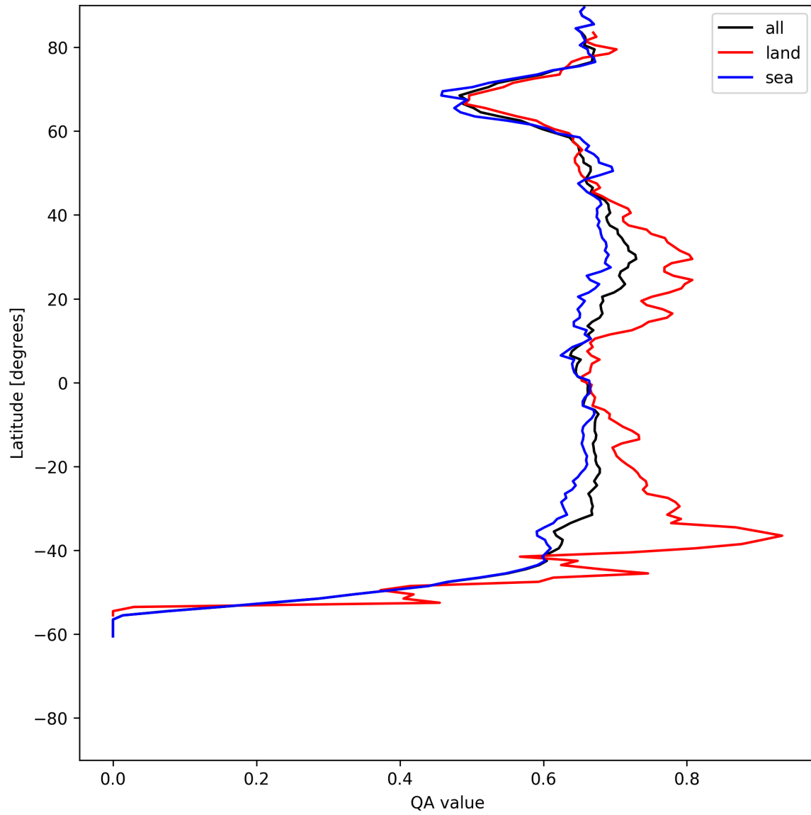
Figure 9: Zonal average of “QA value” for 2025-06-22 to 2025-06-24.
