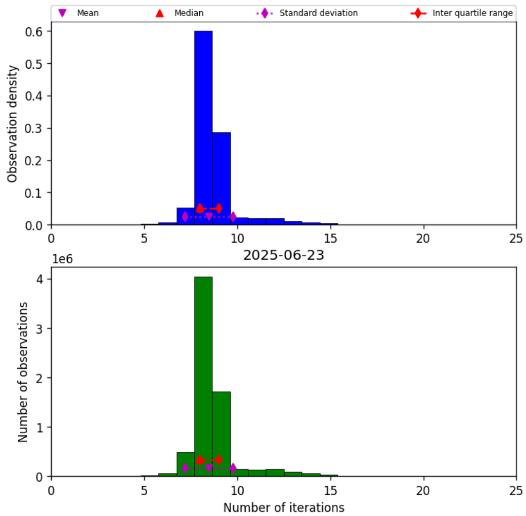
Figure 24: Histogram of “Number of iterations” for 2025-06-22 to 2025-06-24
