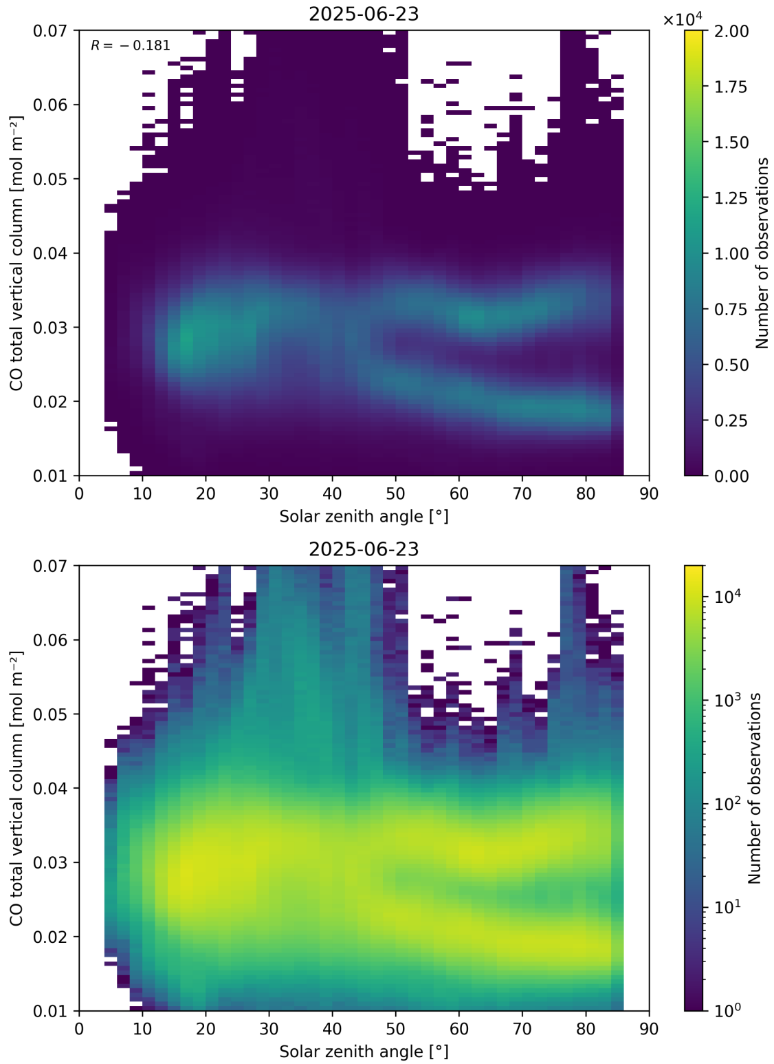
Figure 61: Scatter density plot of “Solar zenith angle” against “CO total vertical column” for 2025-06-22 to 2025-06-24.
