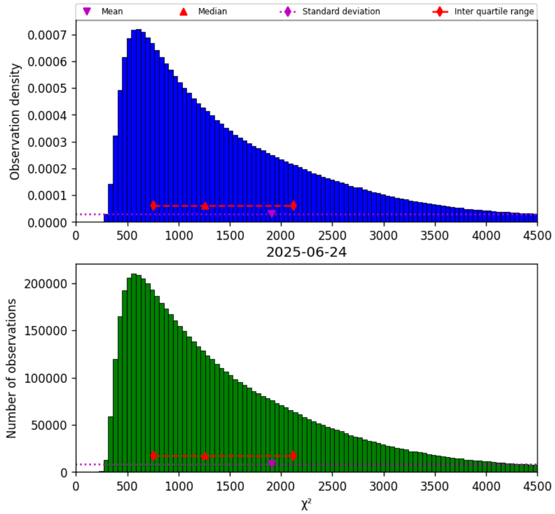
Figure 22: Histogram of “ \chi^2 ” for 2025-06-23 to 2025-06-25
