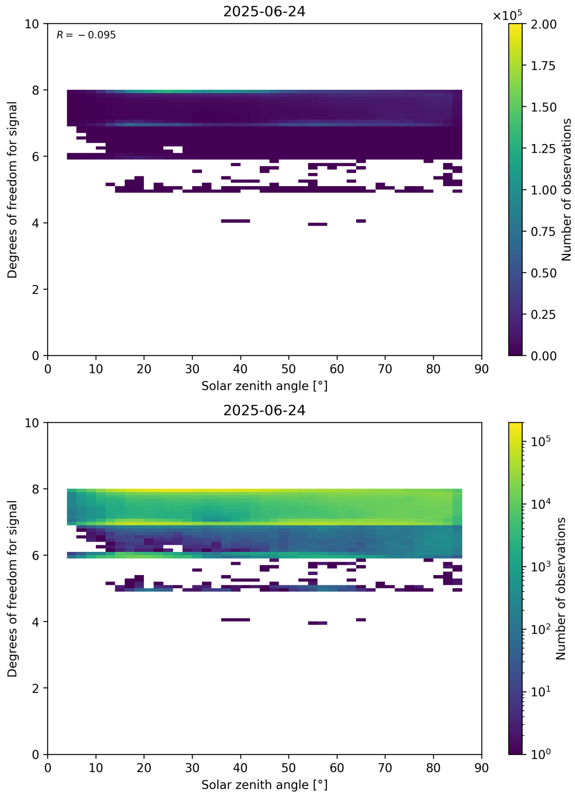
Figure 65: Scatter density plot of “Solar zenith angle” against “Degrees of freedom for signal” for 2025-06-23 to 2025-06-25.
