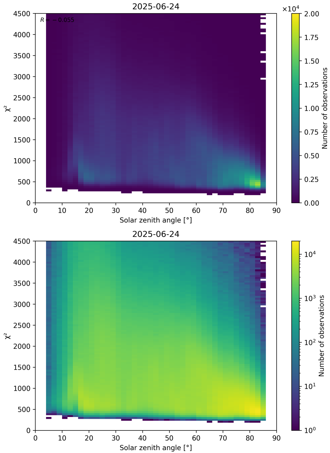
Figure 64: Scatter density plot of “Solar zenith angle” against “ \chi^2 ” for 2025-06-23 to 2025-06-25.
