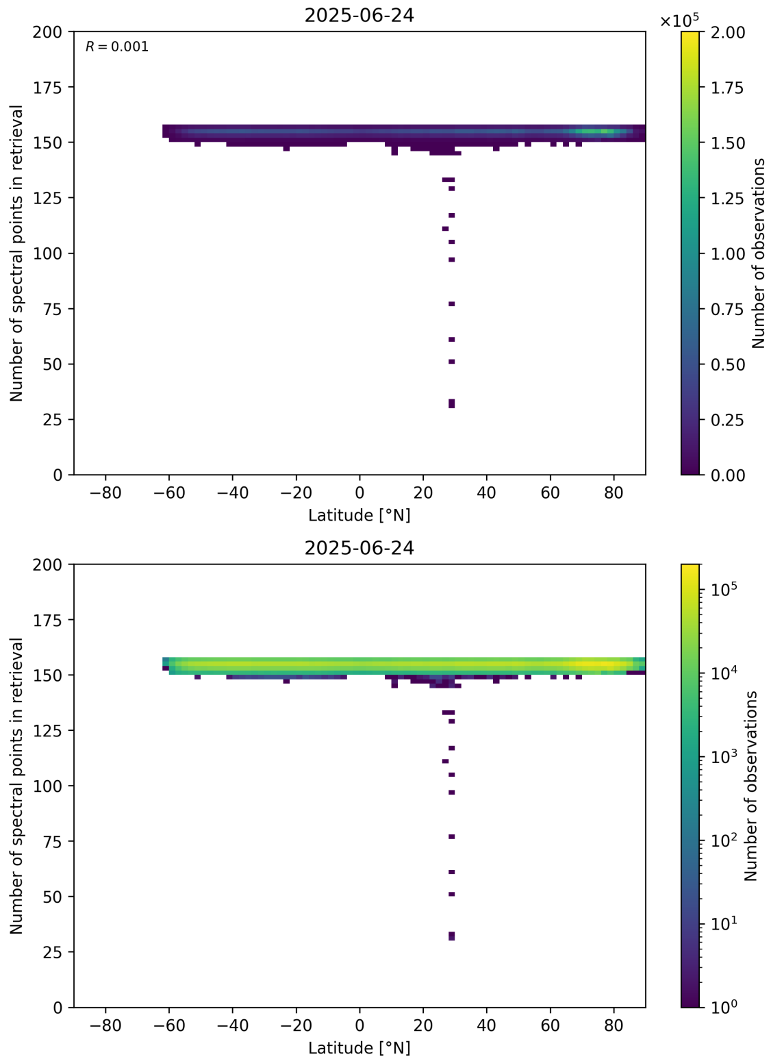
Figure 57: Scatter density plot of “Latitude” against “Number of spectral points in retrieval” for 2025-06-23 to 2025-06-25.
