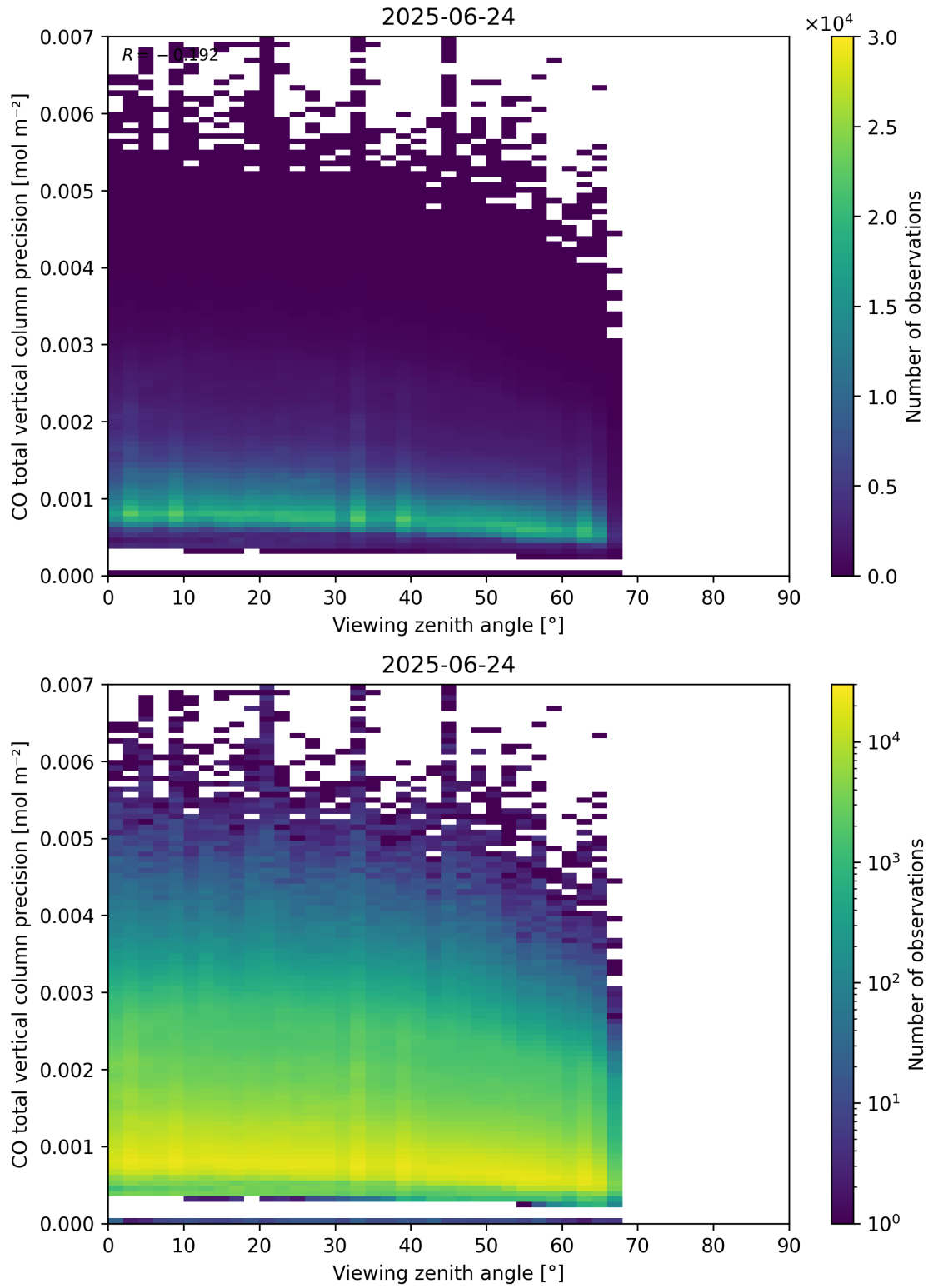
Figure 71: Scatter density plot of “Viewing zenith angle” against “CO total vertical column precision” for 2025-06-23 to 2025-06-25.
