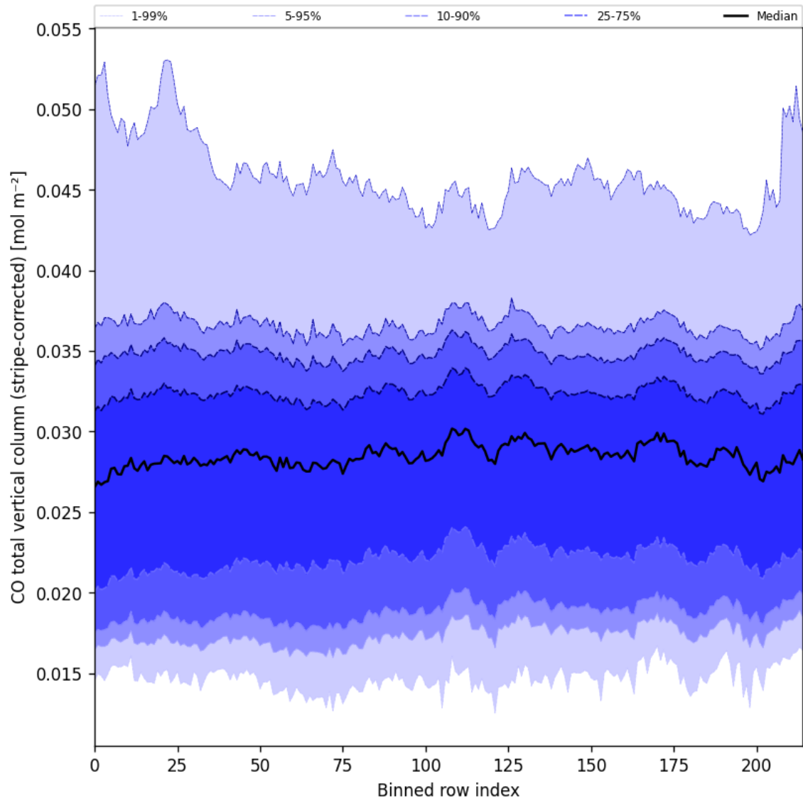
Figure 27: Along track statistics of “CO total vertical column (stripe-corrected)” for 2025-06-23 to 2025-06-25
