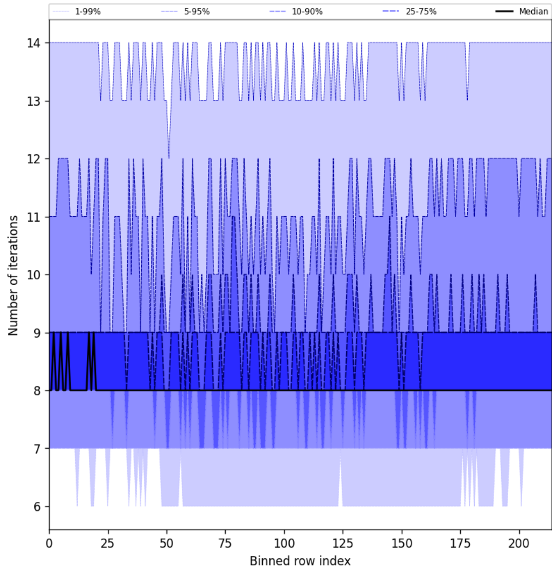
Figure 32: Along track statistics of “Number of iterations” for 2025-06-23 to 2025-06-25
