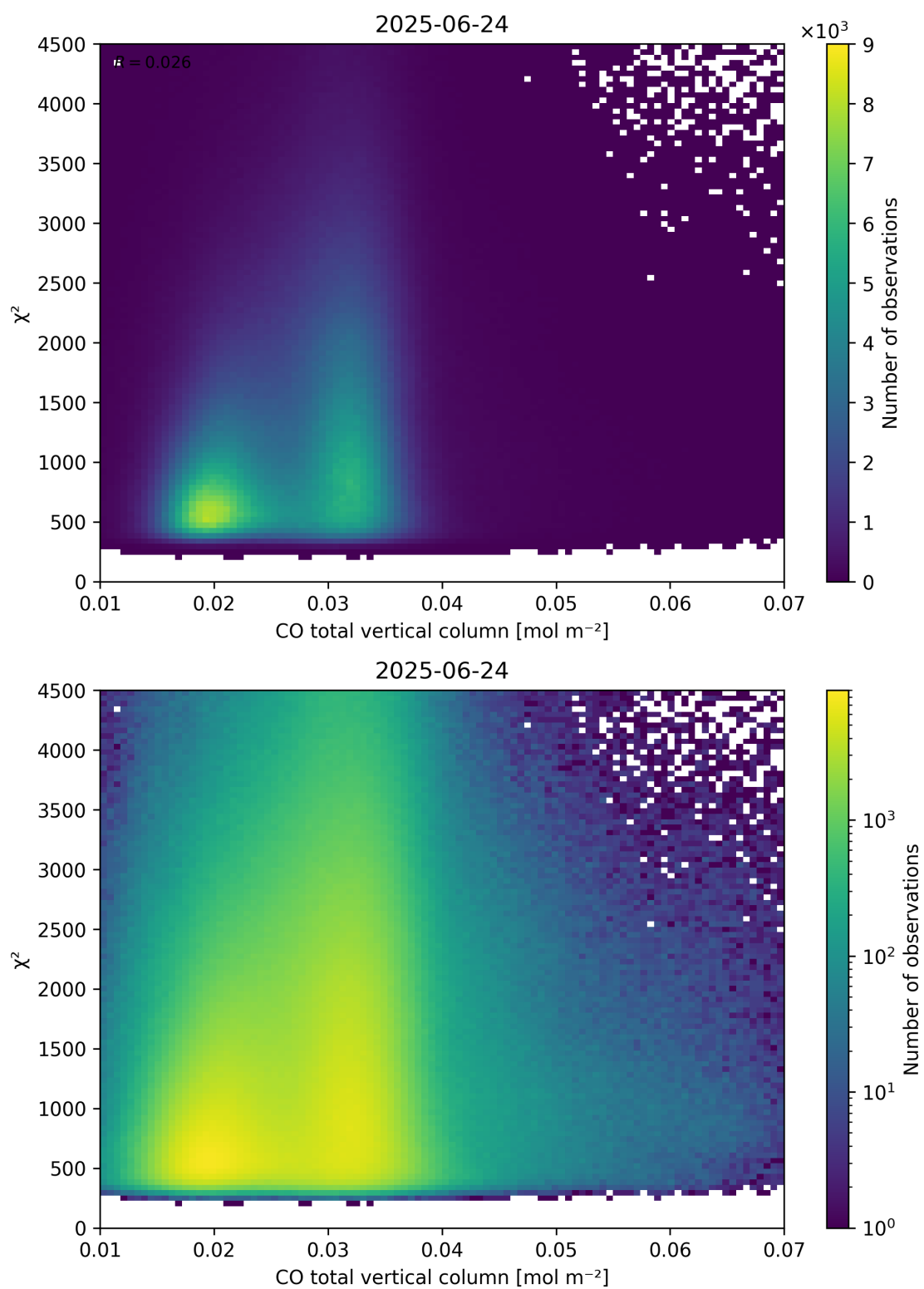
Figure 35: Scatter density plot of “CO total vertical column” against “ \chi^2 ” for 2025-06-23 to 2025-06-25.
