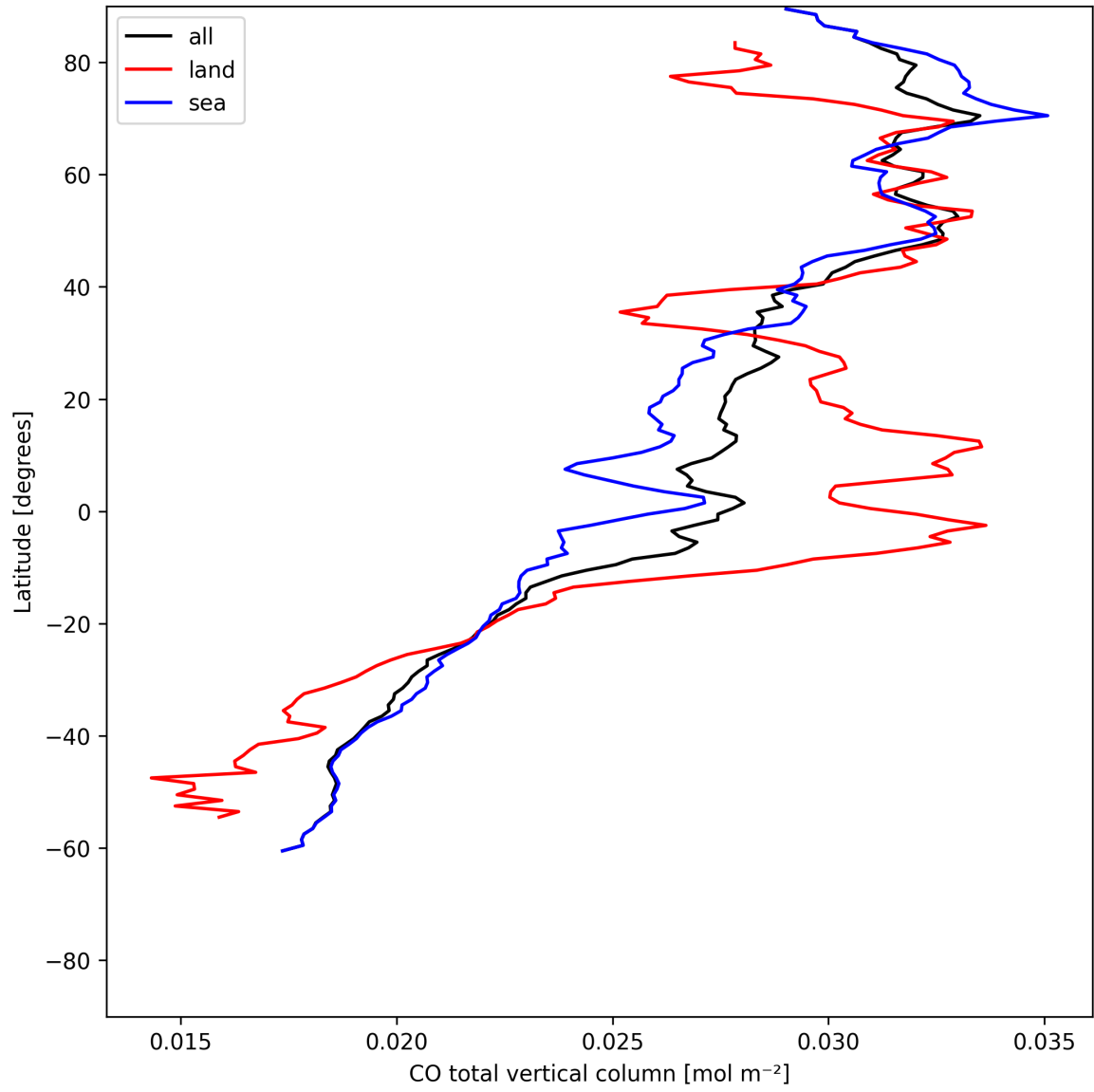
Figure 10: Zonal average of “CO total vertical column” for 2025-06-23 to 2025-06-25.
