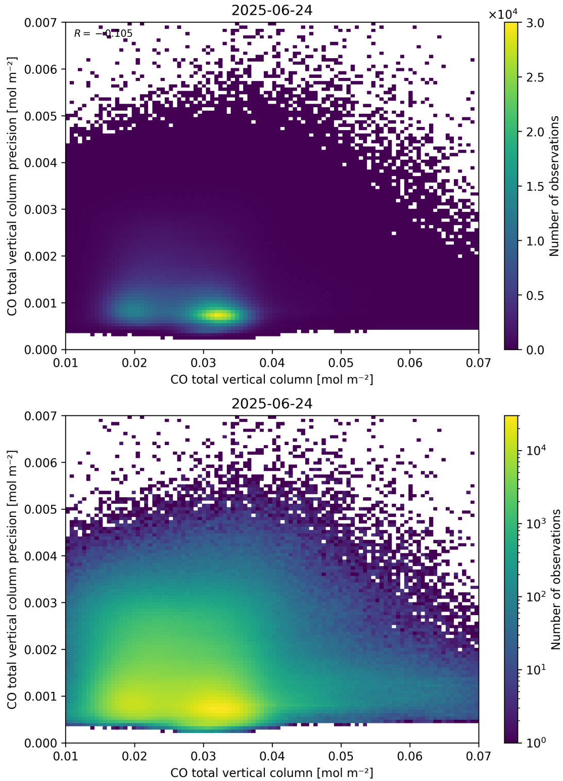
Figure 34: Scatter density plot of “CO total vertical column” against “CO total vertical column precision” for 2025-06-23 to 2025-06-25.
