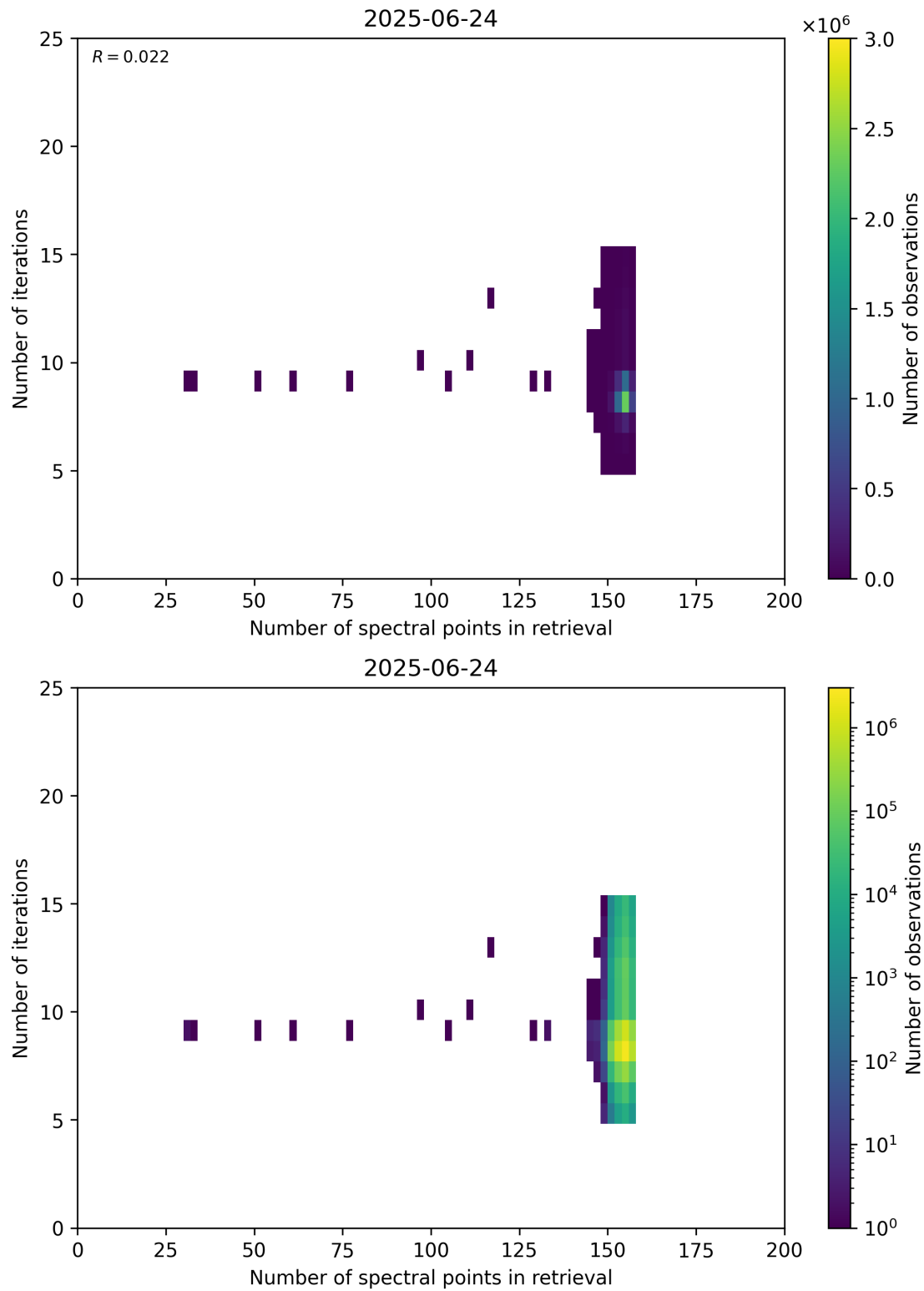
Figure 60: Scatter density plot of “Number of spectral points in retrieval” against “Number of iterations” for 2025-06-23 to 2025-06-25.
