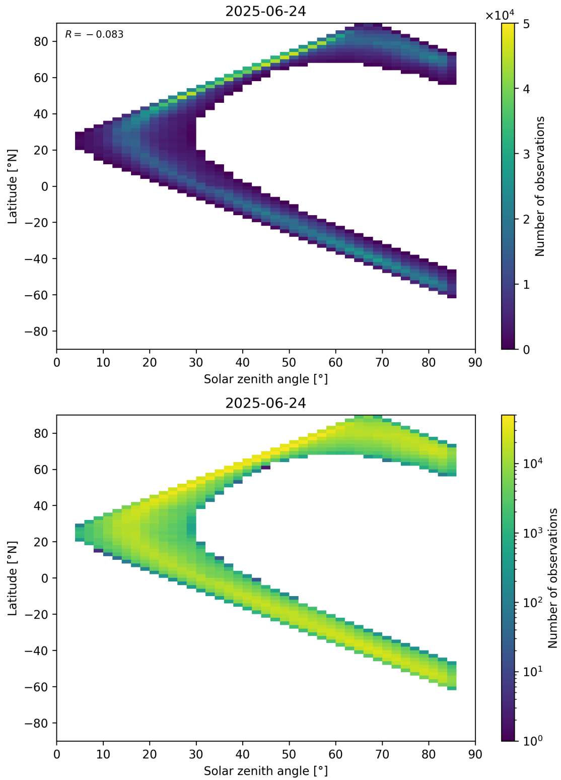
Figure 66: Scatter density plot of “Solar zenith angle” against “Latitude” for 2025-06-23 to 2025-06-25.
