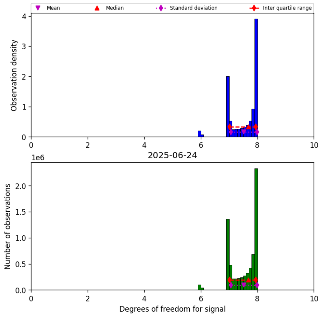
Figure 23: Histogram of “Degrees of freedom for signal” for 2025-06-23 to 2025-06-25
