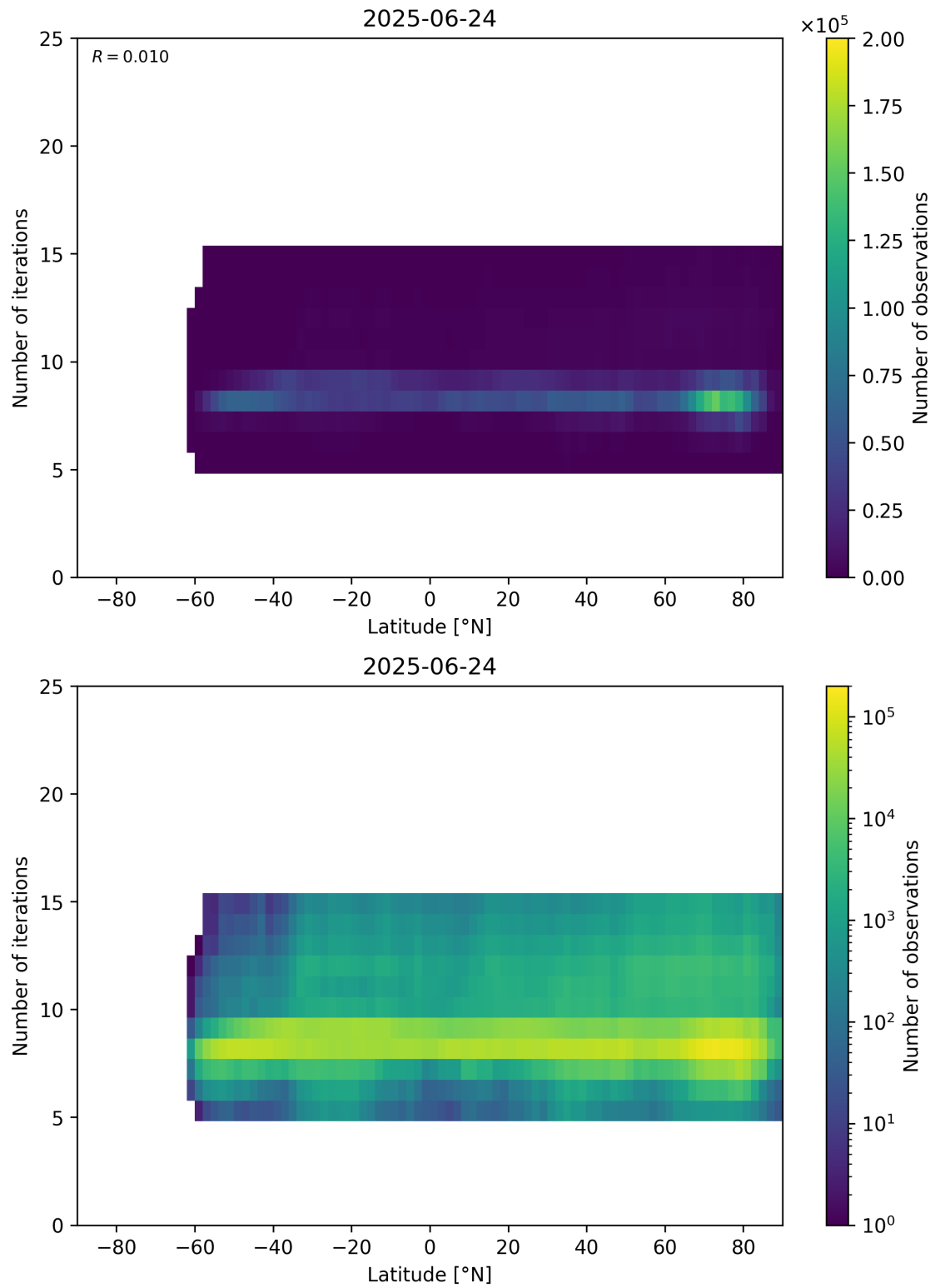
Figure 56: Scatter density plot of “Latitude” against “Number of iterations” for 2025-06-23 to 2025-06-25.
