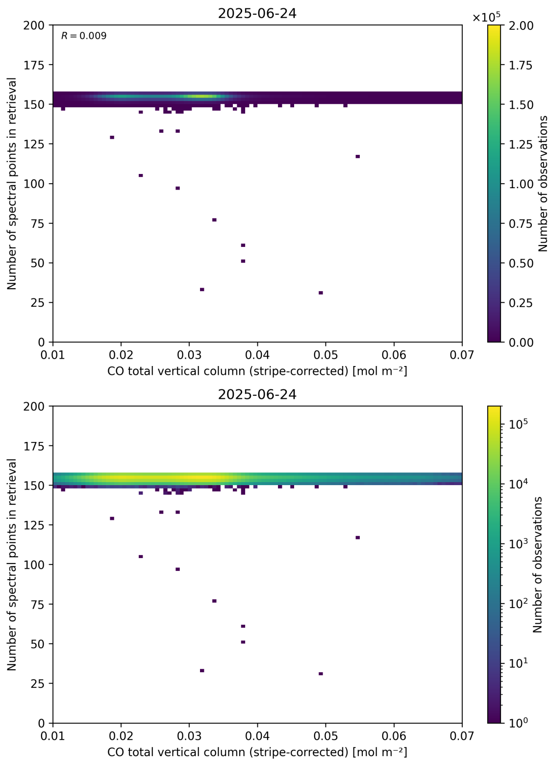
Figure 40: Scatter density plot of “CO total vertical column (stripe-corrected)” against “Number of spectral points in retrieval” for 2025-06-23 to 2025-06-25.
