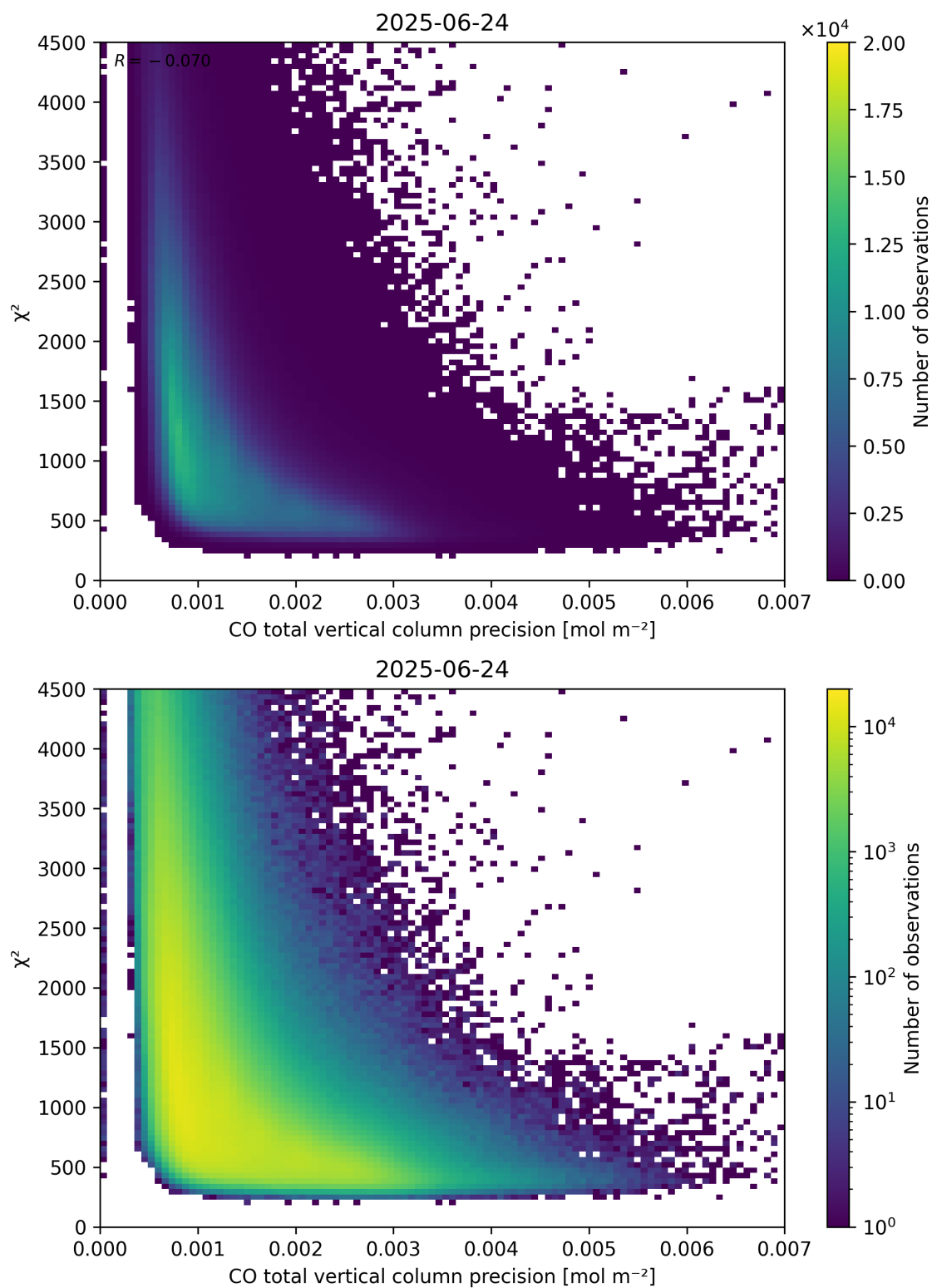
Figure 44: Scatter density plot of “CO total vertical column precision” against “ \chi^2 ” for 2025-06-23 to 2025-06-25.
