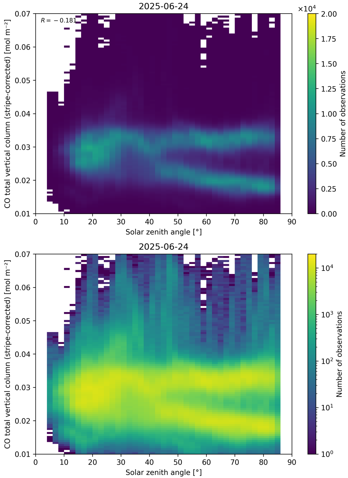
Figure 62: Scatter density plot of “Solar zenith angle” against “CO total vertical column (stripe-corrected)” for 2025-06-23 to 2025-06-25.
