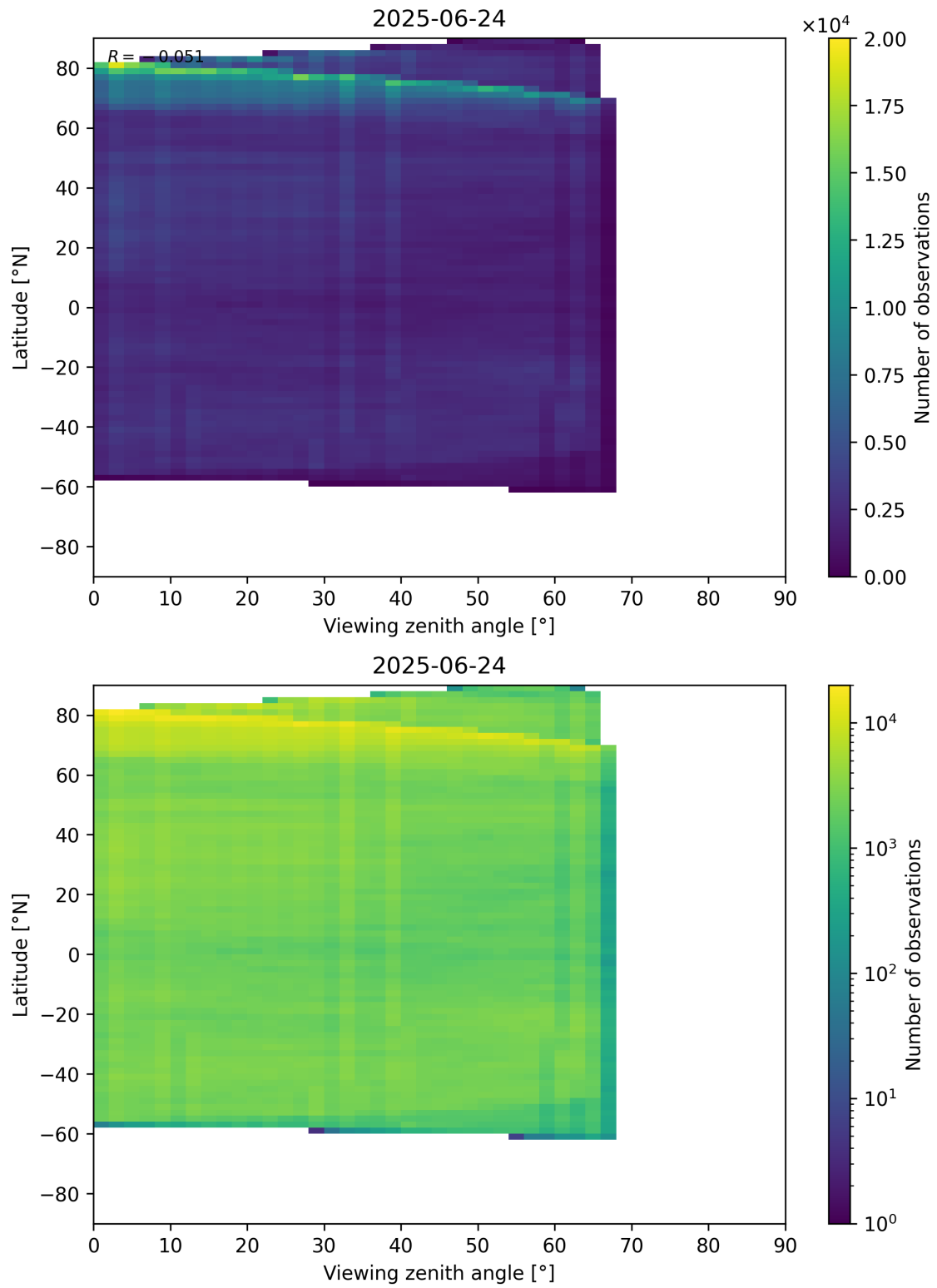
Figure 74: Scatter density plot of “Viewing zenith angle” against “Latitude” for 2025-06-23 to 2025-06-25.
