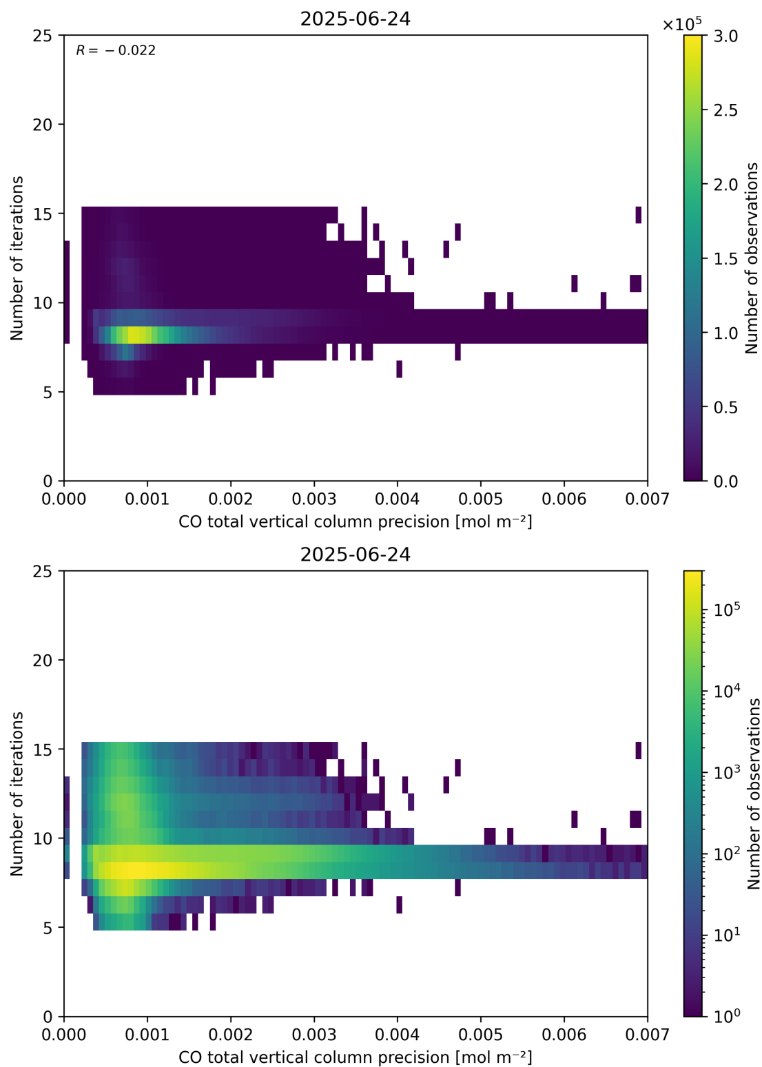
Figure 46: Scatter density plot of “CO total vertical column precision” against “Number of iterations” for 2025-06-23 to 2025-06-25.
