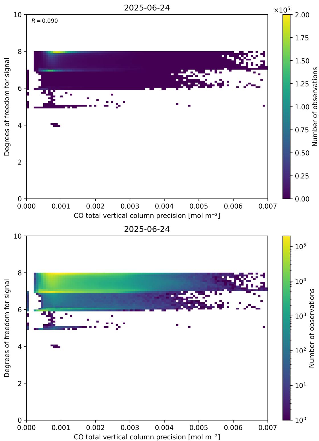
Figure 45: Scatter density plot of “CO total vertical column precision” against “Degrees of freedom for signal” for 2025-06-23 to 2025-06-25.
