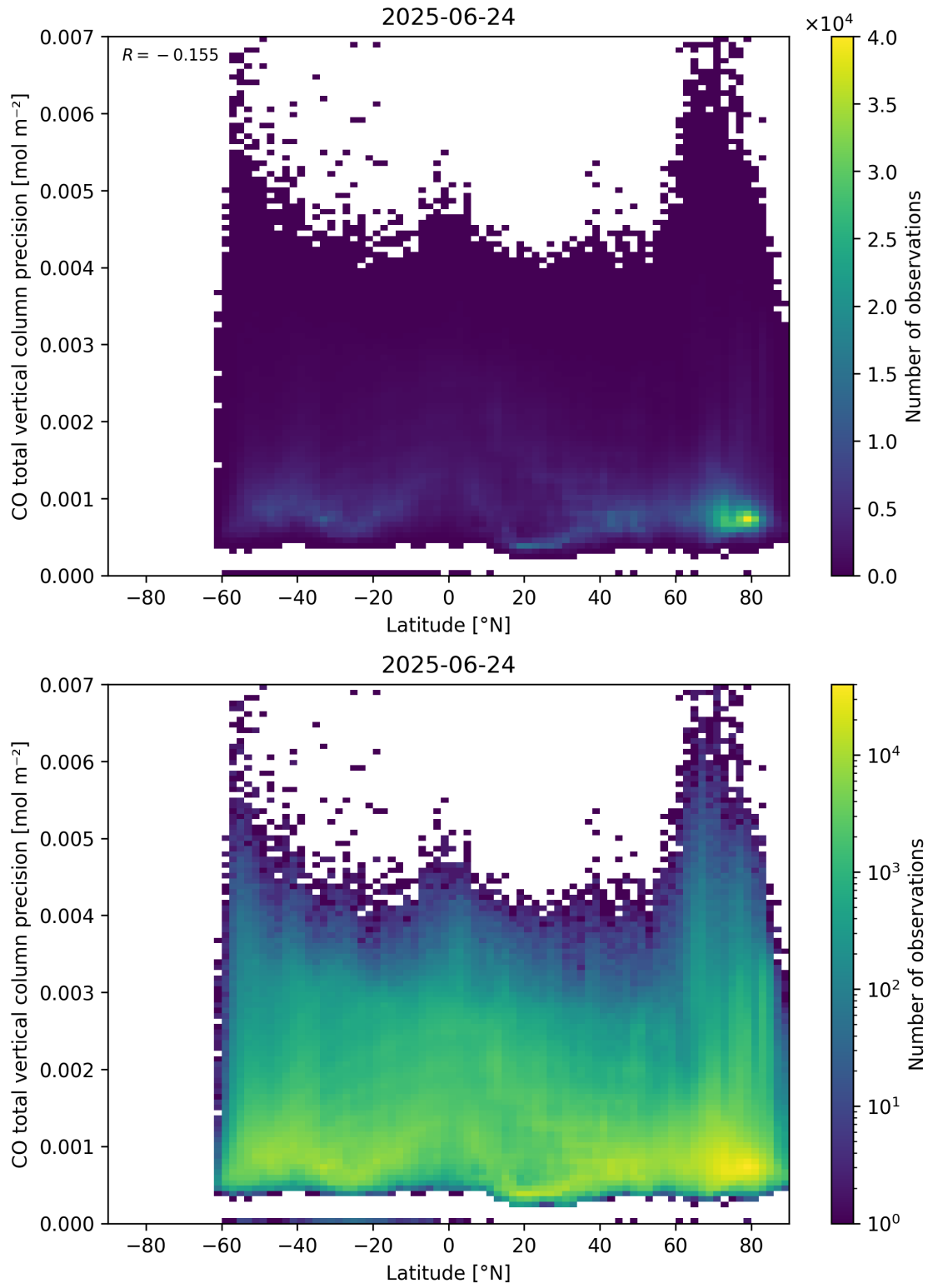
Figure 53: Scatter density plot of “Latitude” against “CO total vertical column precision” for 2025-06-23 to 2025-06-25.
