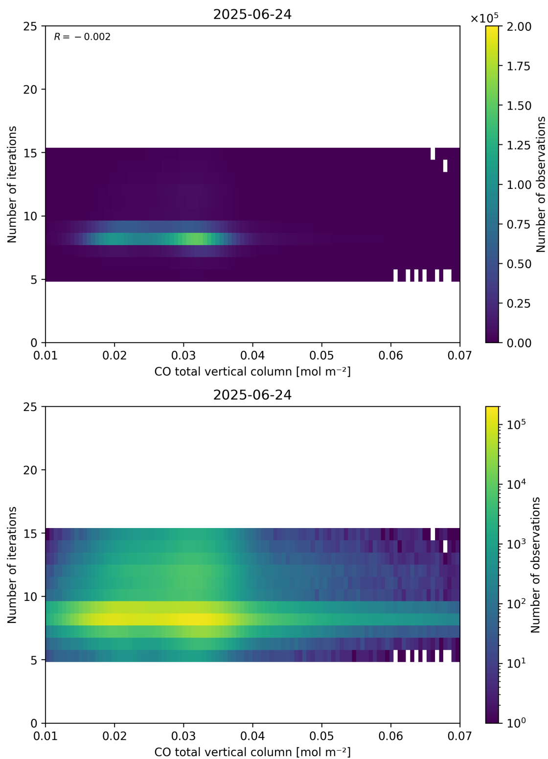
Figure 42: Scatter density plot of “CO total vertical column” against “Number of iterations” for 2025-06-23 to 2025-06-25.
