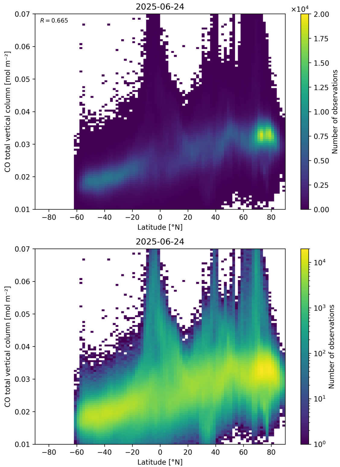
Figure 51: Scatter density plot of “Latitude” against “CO total vertical column” for 2025-06-23 to 2025-06-25.
