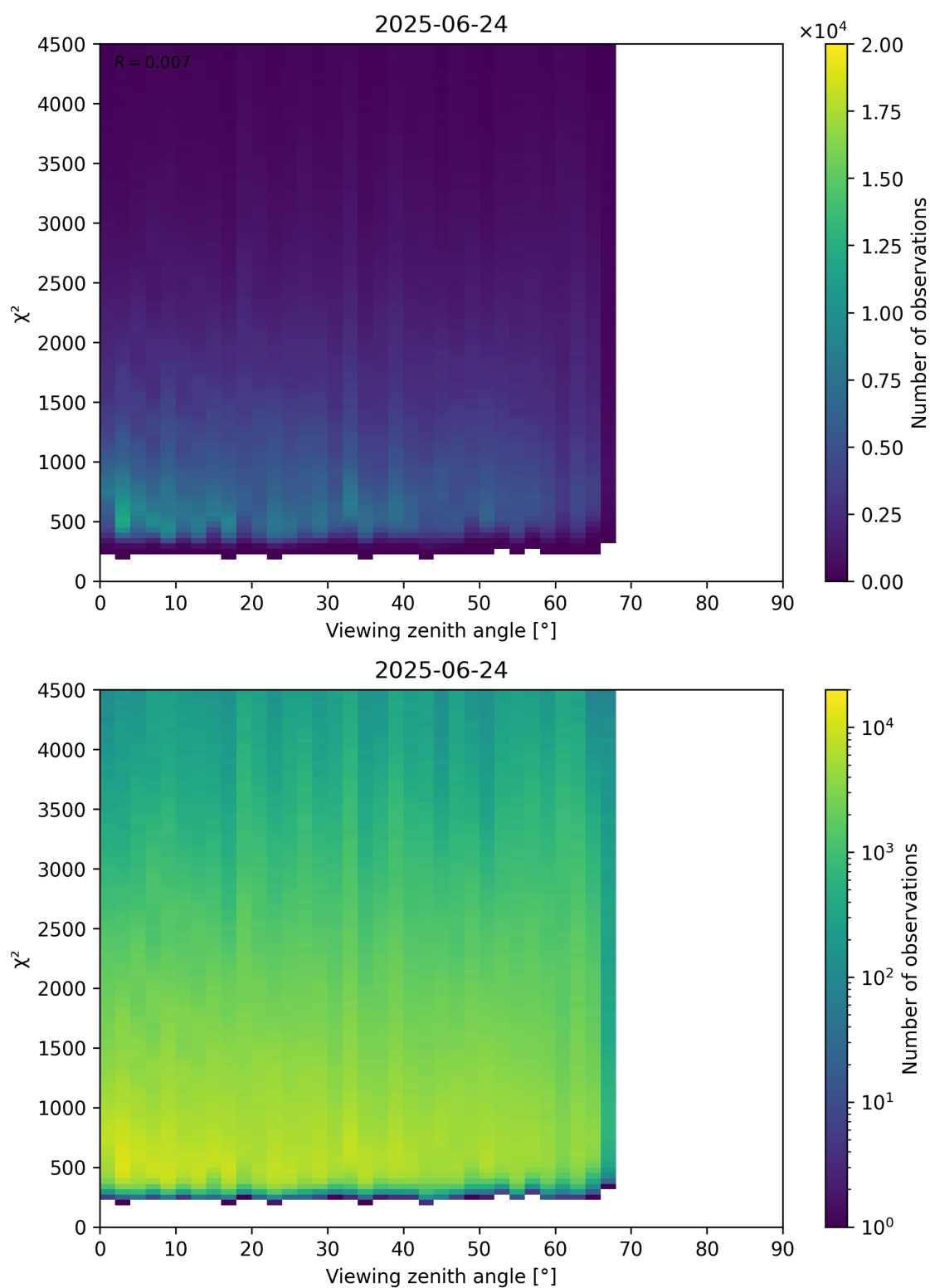
Figure 72: Scatter density plot of “Viewing zenith angle” against “ \chi^2 ” for 2025-06-23 to 2025-06-25.
