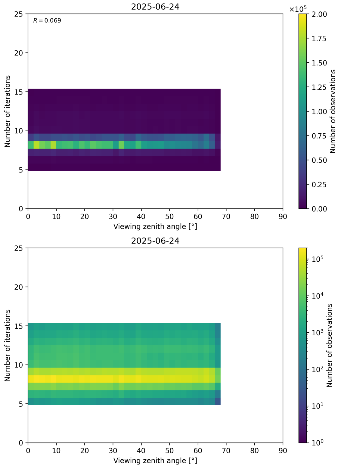
Figure 75: Scatter density plot of “Viewing zenith angle” against “Number of iterations” for 2025-06-23 to 2025-06-25.
