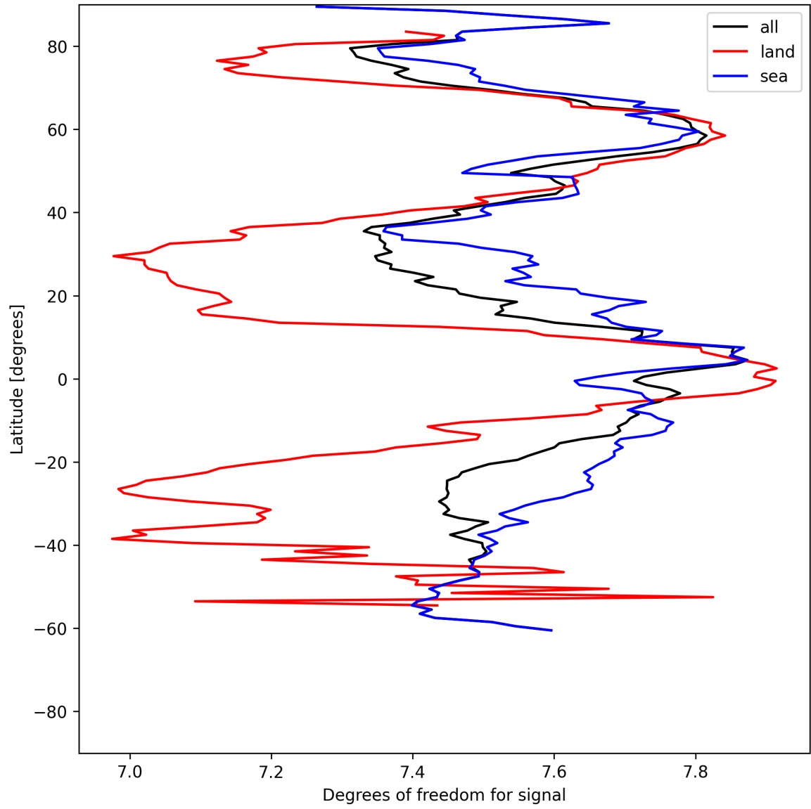
Figure 15: Zonal average of “Degrees of freedom for signal” for 2025-06-23 to 2025-06-25.
