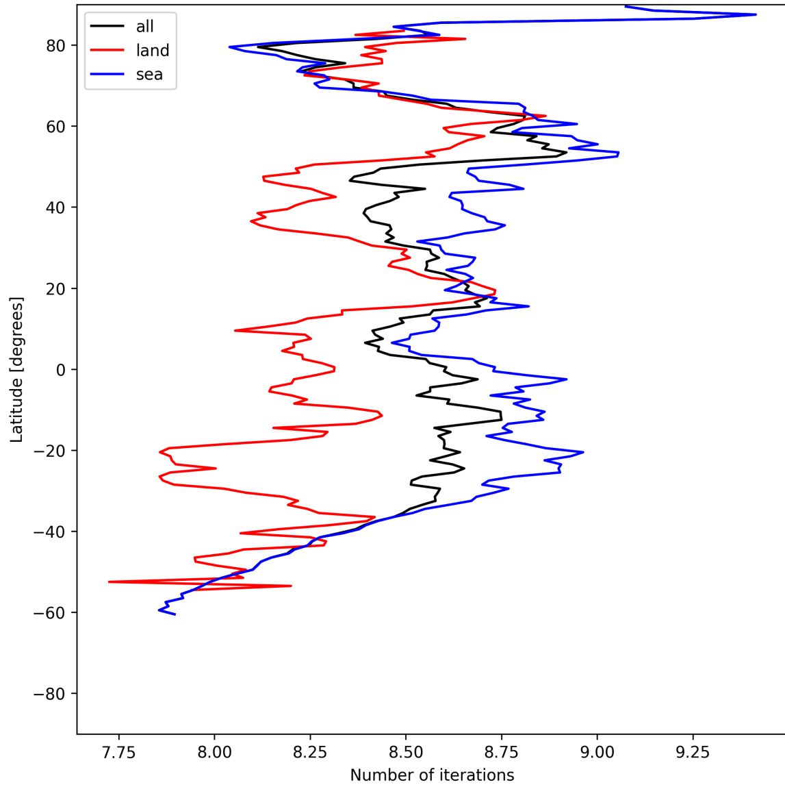
Figure 16: Zonal average of “Number of iterations” for 2025-06-23 to 2025-06-25.
