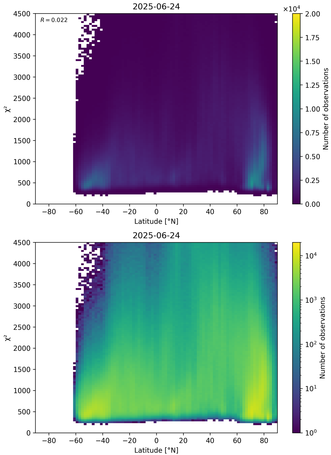
Figure 54: Scatter density plot of “Latitude” against “ \chi^2 ” for 2025-06-23 to 2025-06-25.
