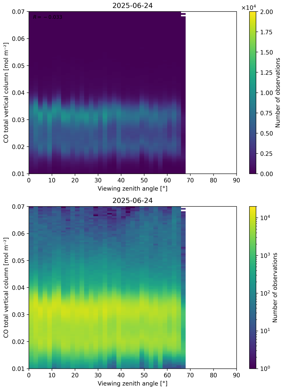
Figure 69: Scatter density plot of “Viewing zenith angle” against “CO total vertical column” for 2025-06-23 to 2025-06-25.
