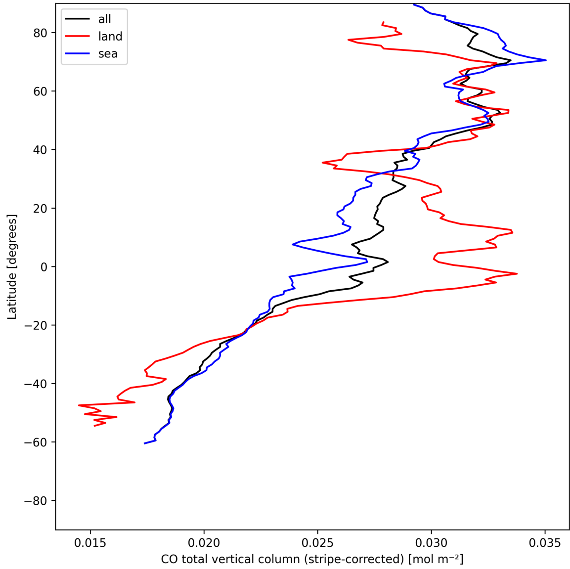
Figure 11: Zonal average of “CO total vertical column (stripe-corrected)” for 2025-06-23 to 2025-06-25.
