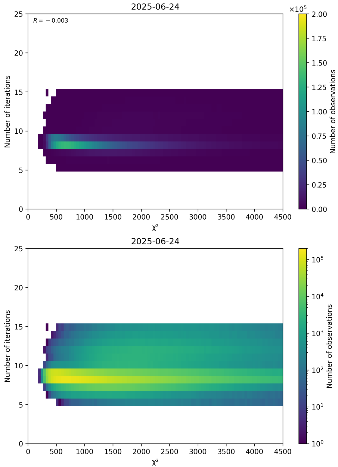
Figure 49: Scatter density plot of “ \chi^2 ” against “Number of iterations” for 2025-06-23 to 2025-06-25.
