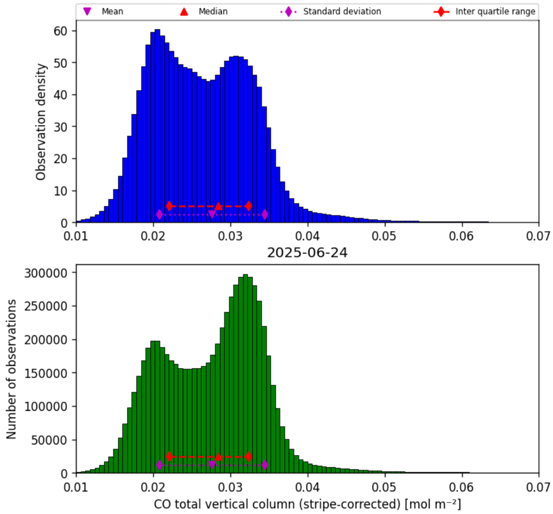
Figure 19: Histogram of “CO total vertical column (stripe-corrected)” for 2025-06-23 to 2025-06-25
