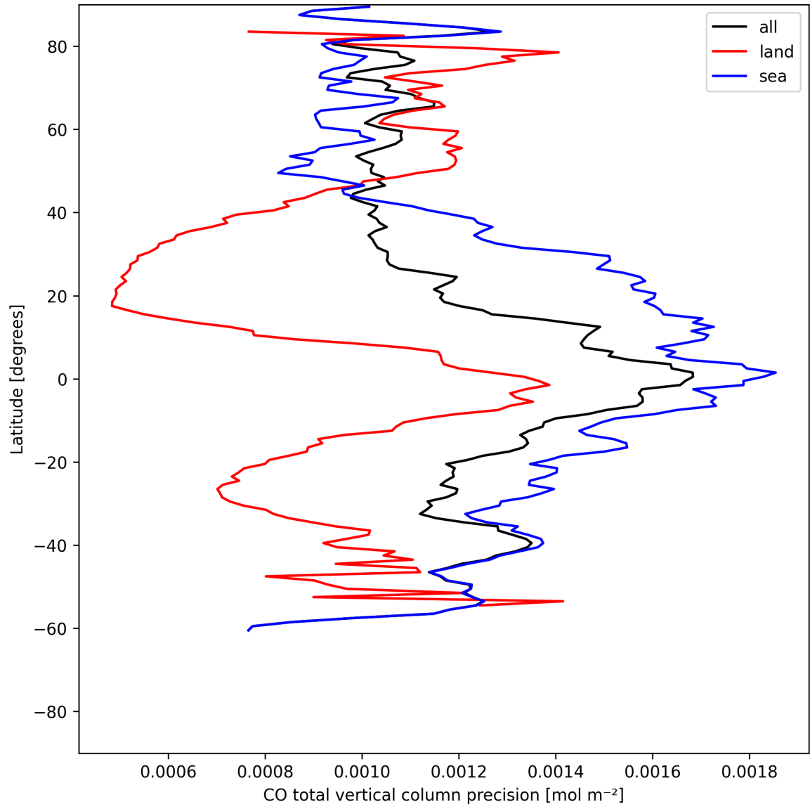
Figure 12: Zonal average of “CO total vertical column precision” for 2025-06-23 to 2025-06-25.
