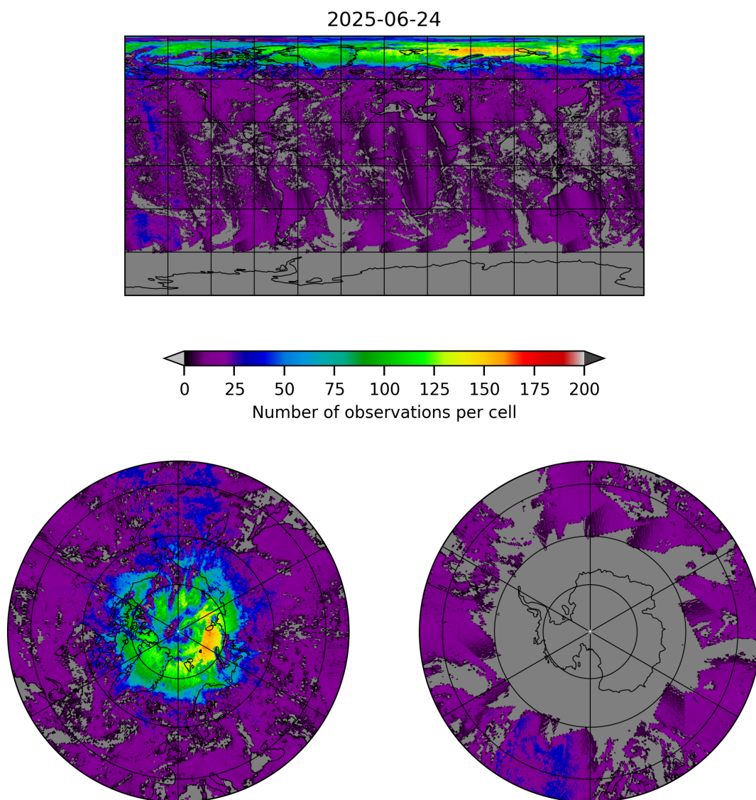
Figure 8: Map of the number of observations for 2025-06-23 to 2025-06-25
