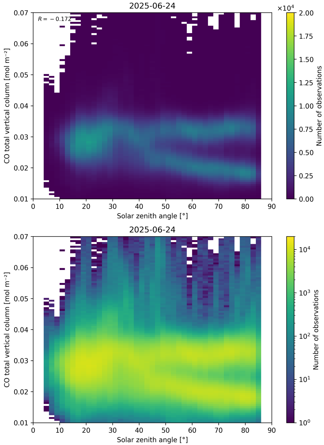
Figure 61: Scatter density plot of “Solar zenith angle” against “CO total vertical column” for 2025-06-23 to 2025-06-25.
