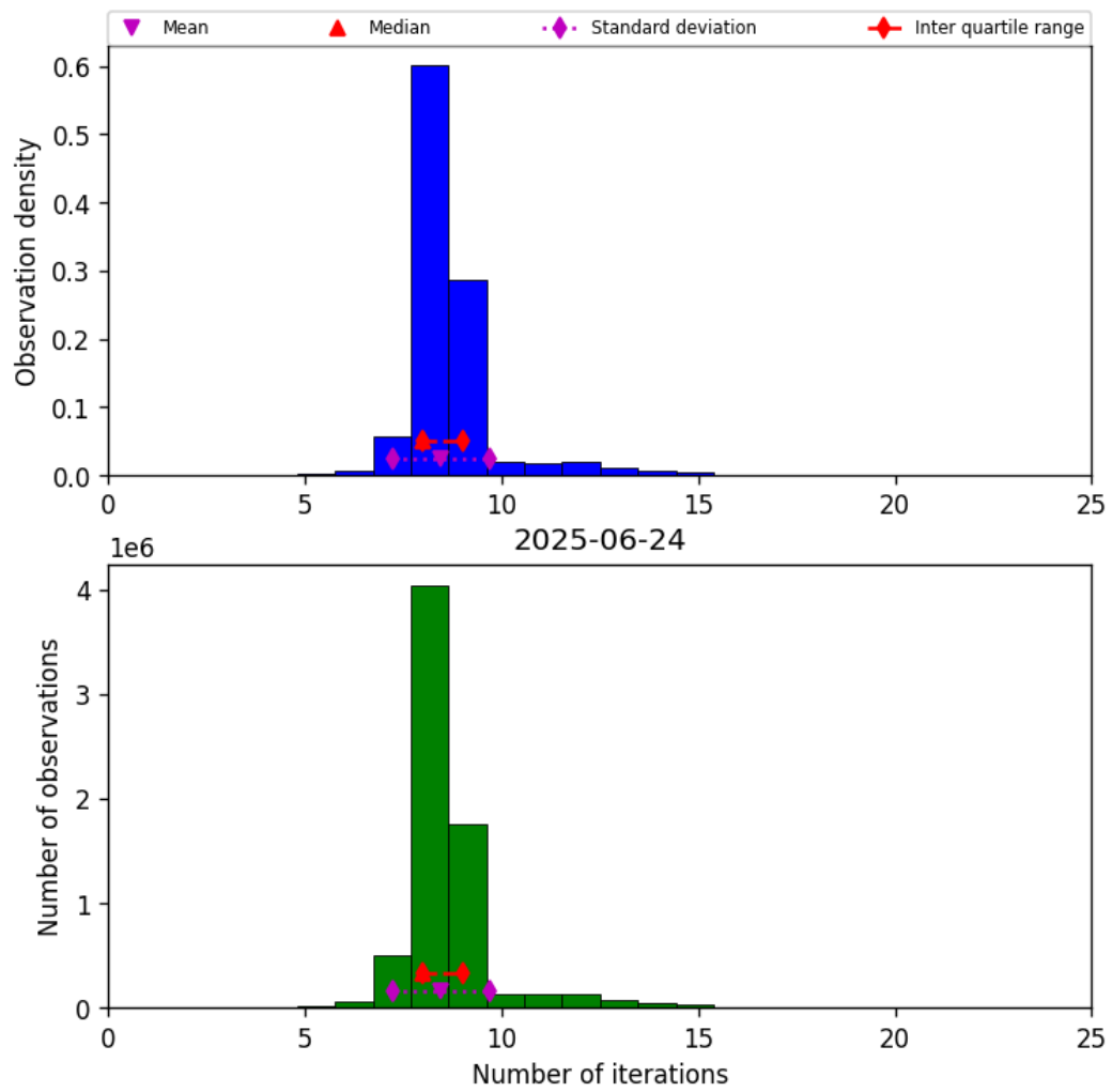
Figure 24: Histogram of “Number of iterations” for 2025-06-23 to 2025-06-25
