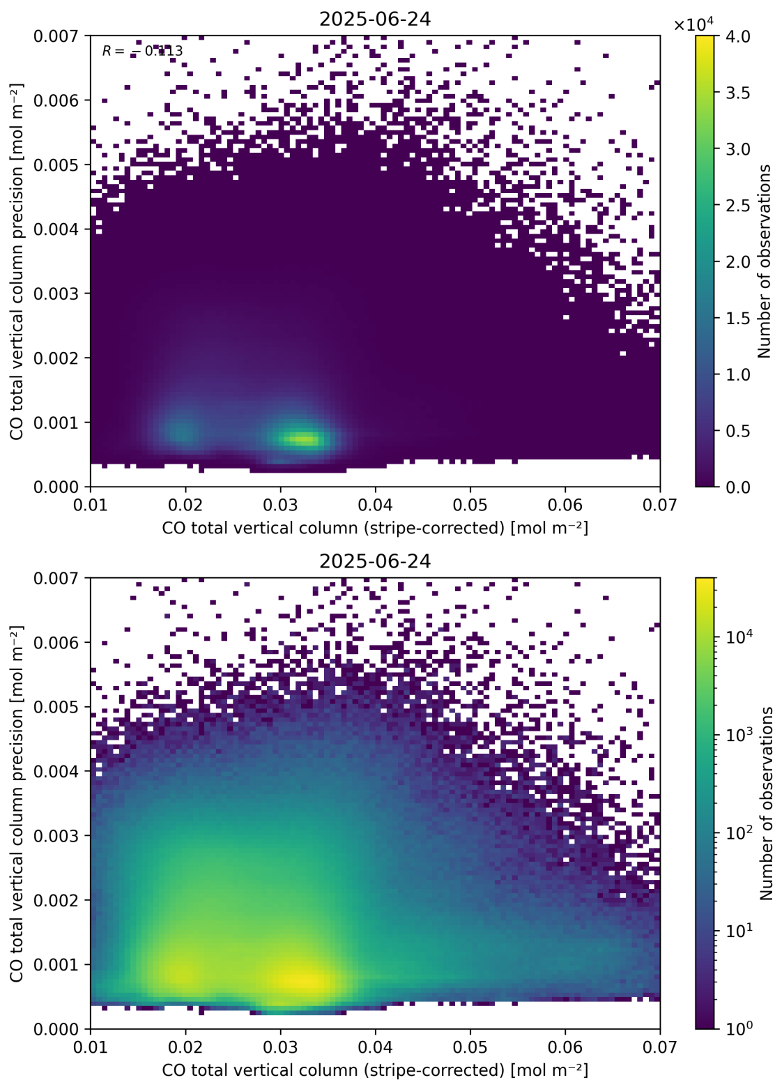
Figure 36: Scatter density plot of “CO total vertical column (stripe-corrected)” against “CO total vertical column precision” for 2025-06-23 to 2025-06-25.
