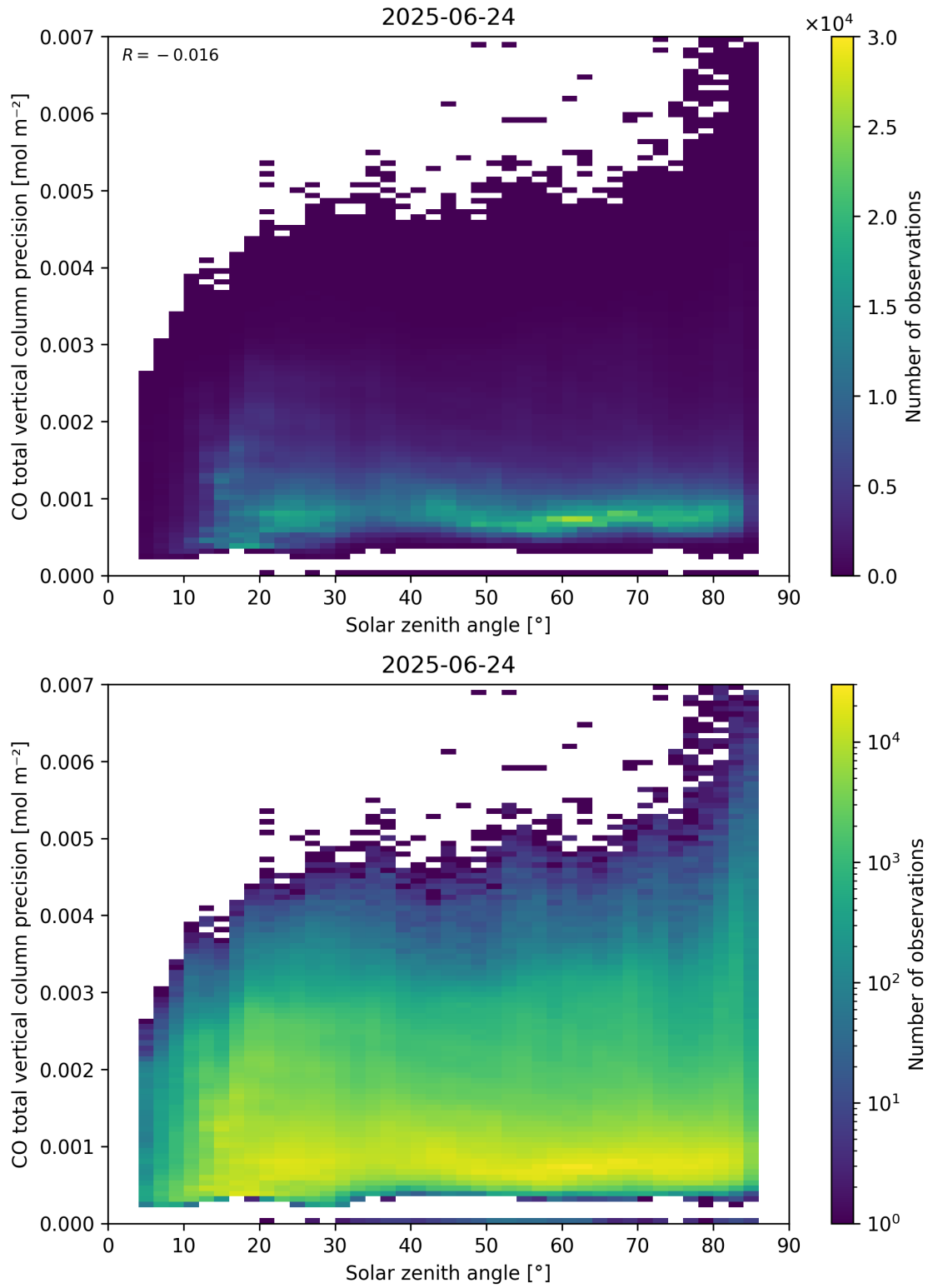
Figure 63: Scatter density plot of “Solar zenith angle” against “CO total vertical column precision” for 2025-06-23 to 2025-06-25.
