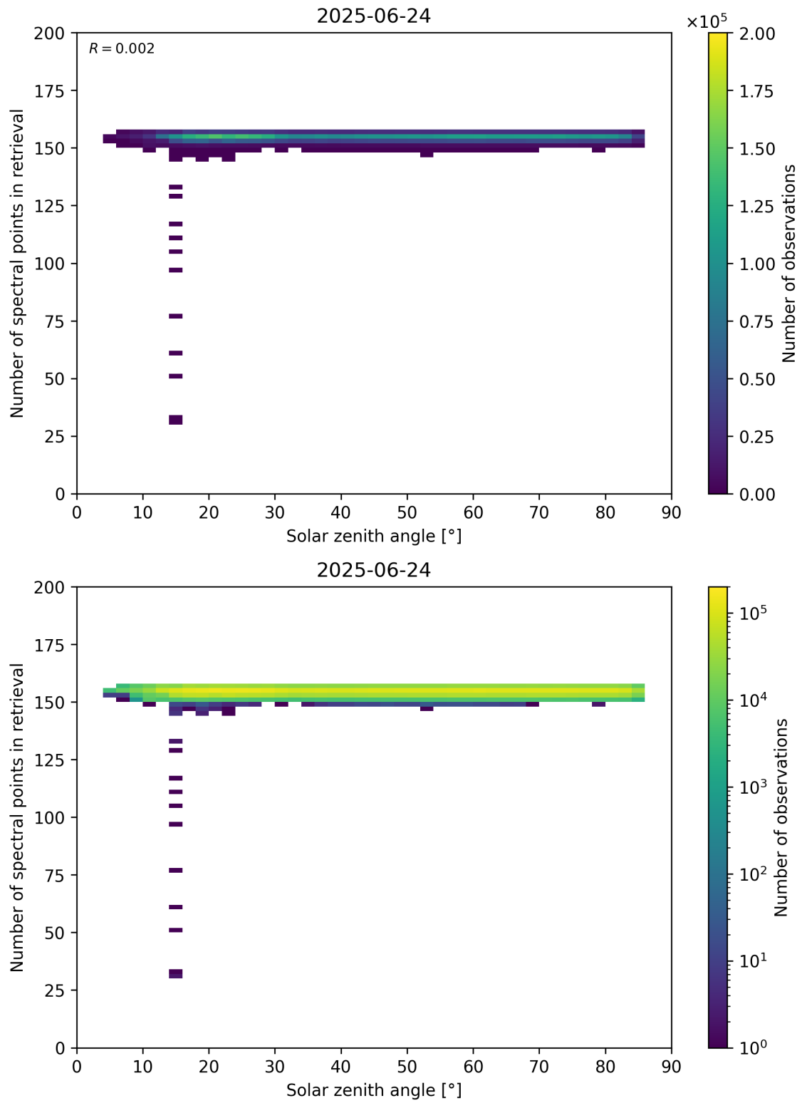
Figure 68: Scatter density plot of “Solar zenith angle” against “Number of spectral points in retrieval” for 2025-06-23 to 2025-06-25.
