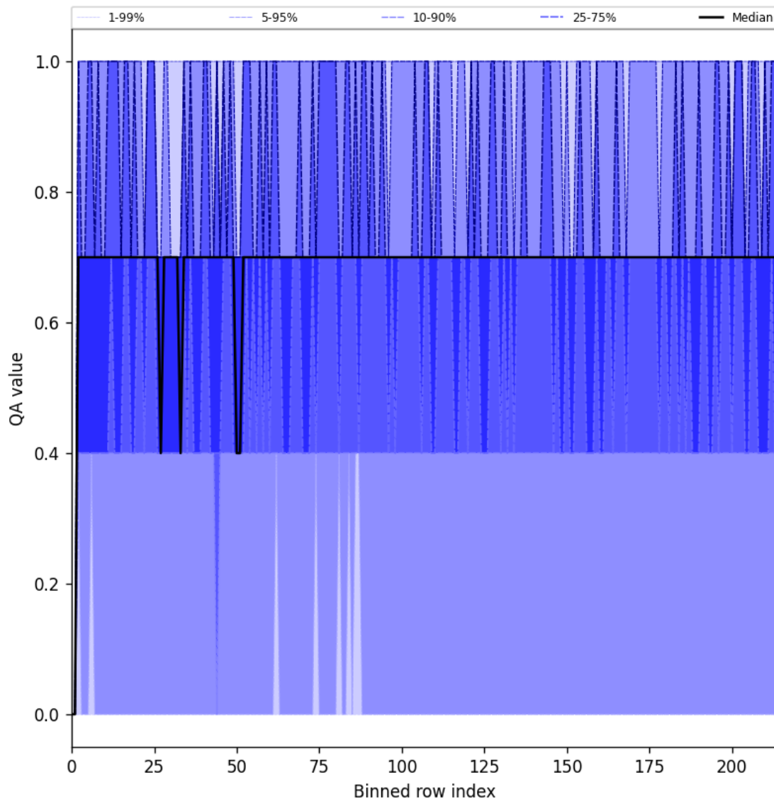
Figure 25: Along track statistics of “QA value” for 2025-06-23 to 2025-06-25
