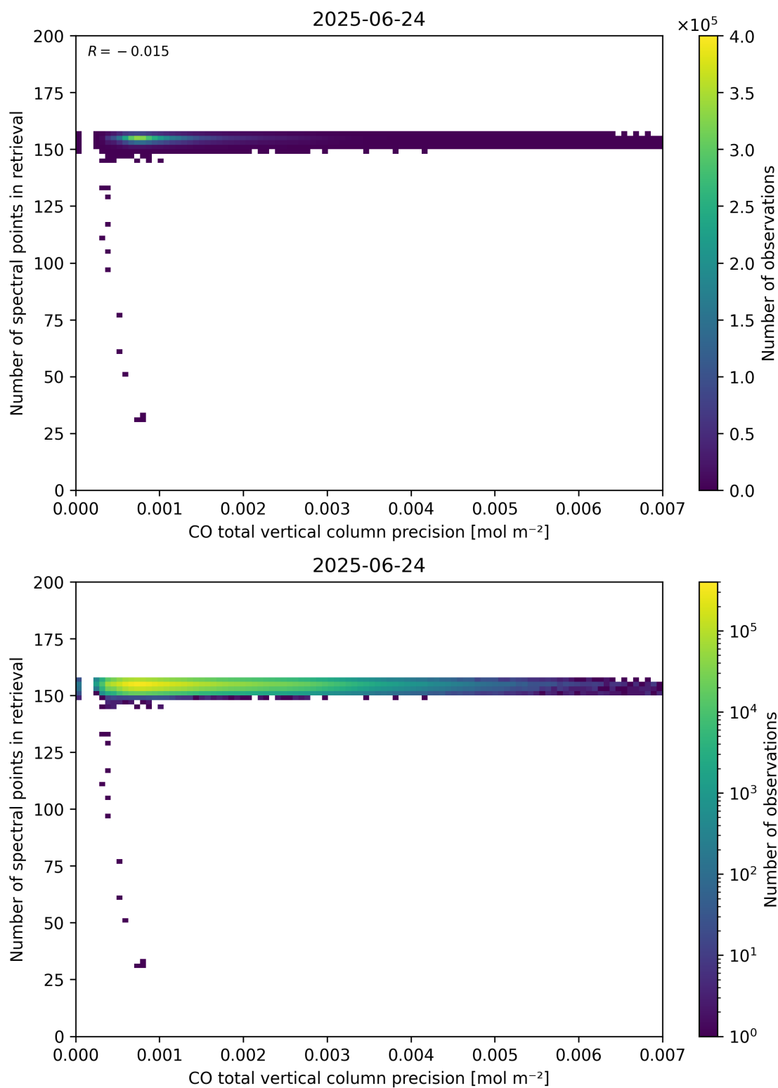
Figure 47: Scatter density plot of “CO total vertical column precision” against “Number of spectral points in retrieval” for 2025-06-23 to 2025-06-25.
