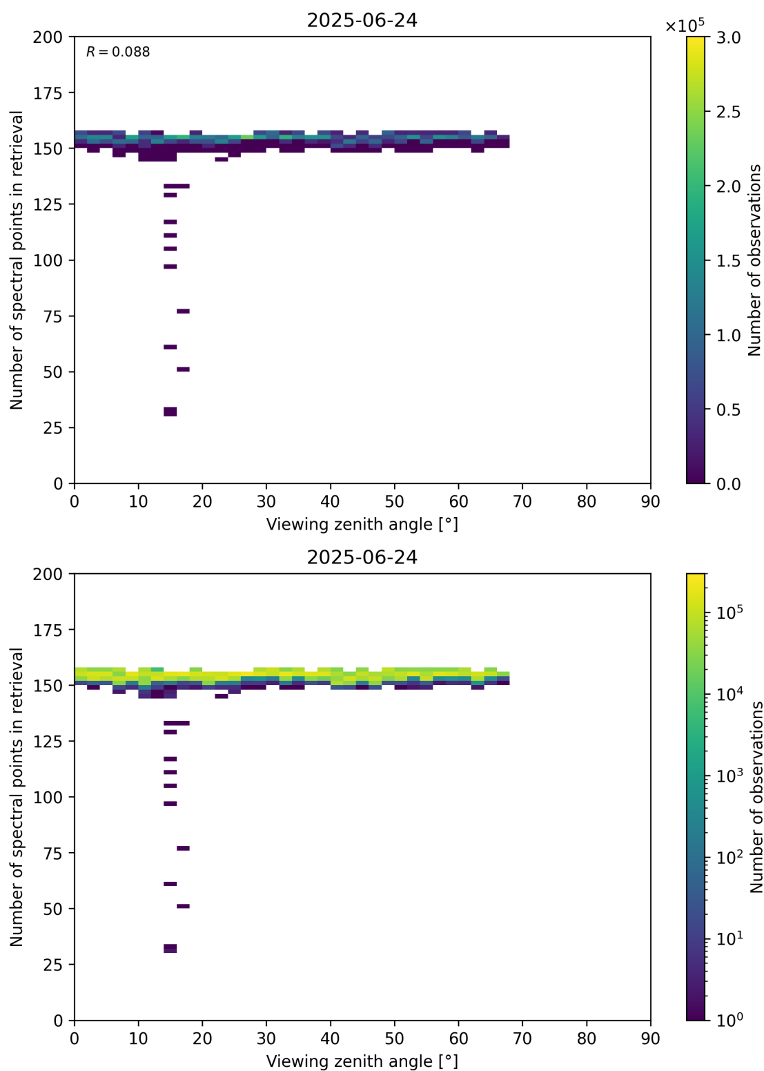
Figure 76: Scatter density plot of “Viewing zenith angle” against “Number of spectral points in retrieval” for 2025-06-23 to 2025-06-25.
