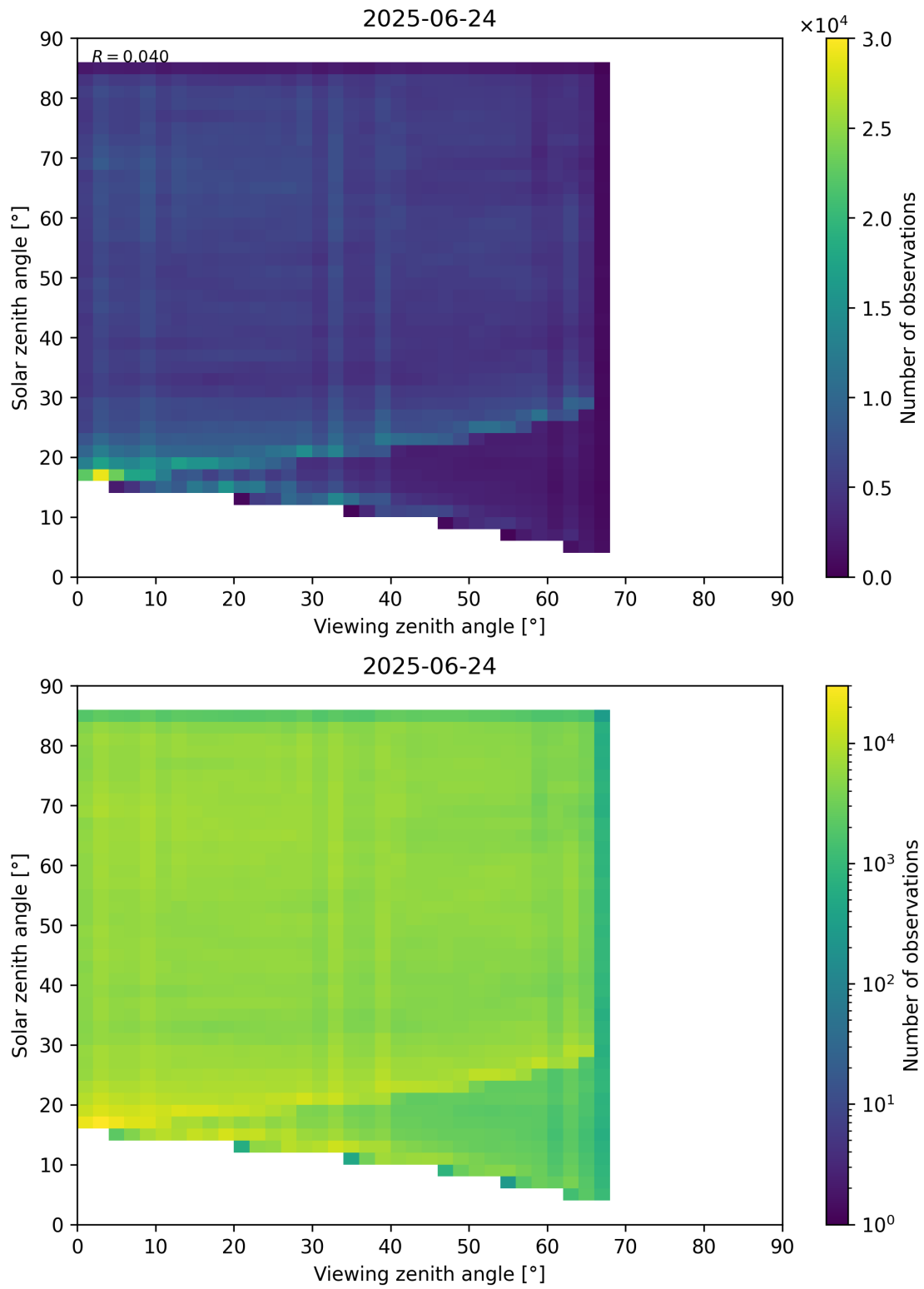
Figure 77: Scatter density plot of “Viewing zenith angle” against “Solar zenith angle” for 2025-06-23 to 2025-06-25.
