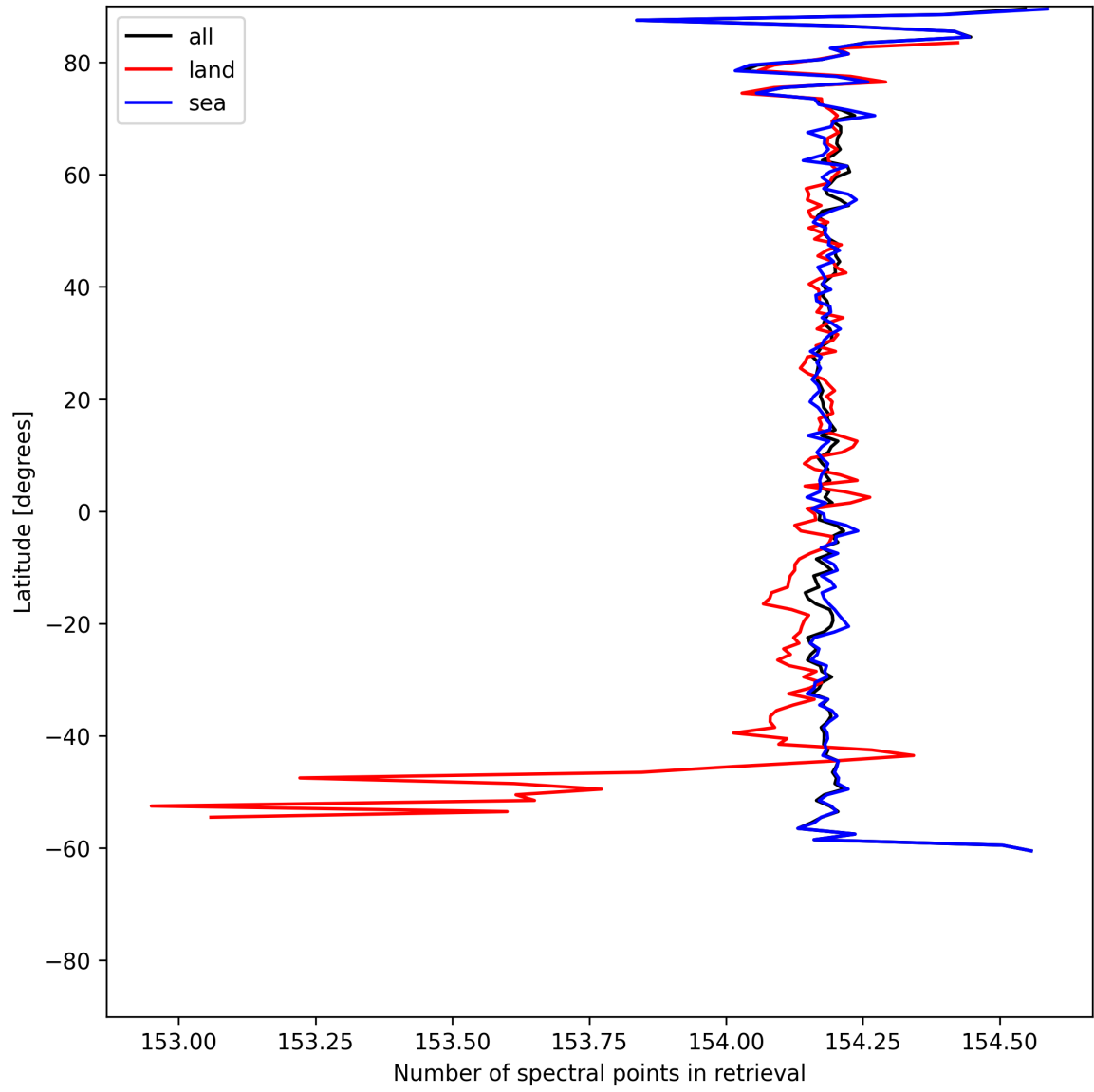
Figure 13: Zonal average of “Number of spectral points in retrieval” for 2025-06-23 to 2025-06-25.
