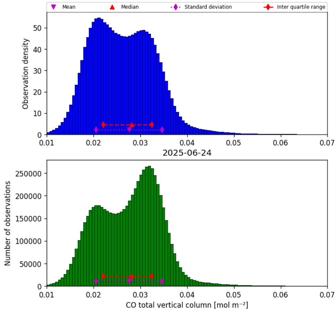
Figure 18: Histogram of “CO total vertical column” for 2025-06-23 to 2025-06-25
