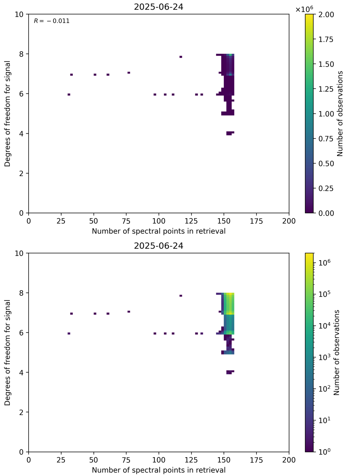
Figure 59: Scatter density plot of “Number of spectral points in retrieval” against “Degrees of freedom for signal” for 2025-06-23 to 2025-06-25.
