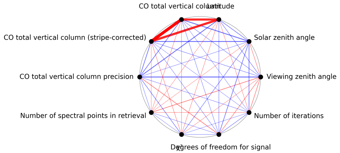
Figure 1: Map of correlation graph for 2025-06-23 to 2025-06-25.
