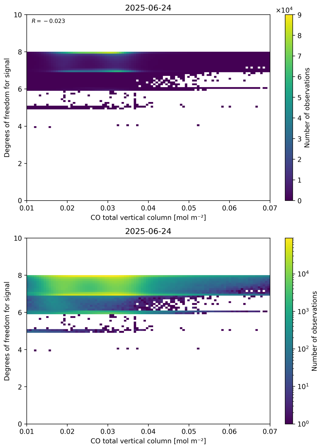
Figure 41: Scatter density plot of “CO total vertical column” against “Degrees of freedom for signal” for 2025-06-23 to 2025-06-25.
