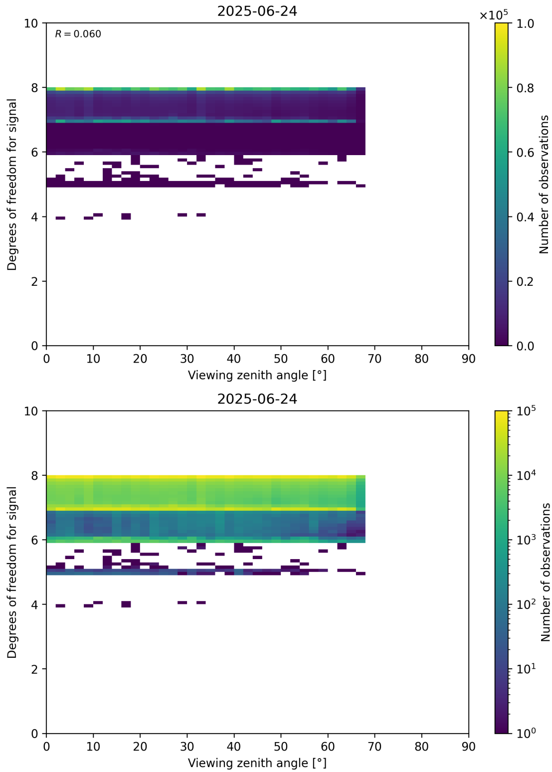
Figure 73: Scatter density plot of “Viewing zenith angle” against “Degrees of freedom for signal” for 2025-06-23 to 2025-06-25.
