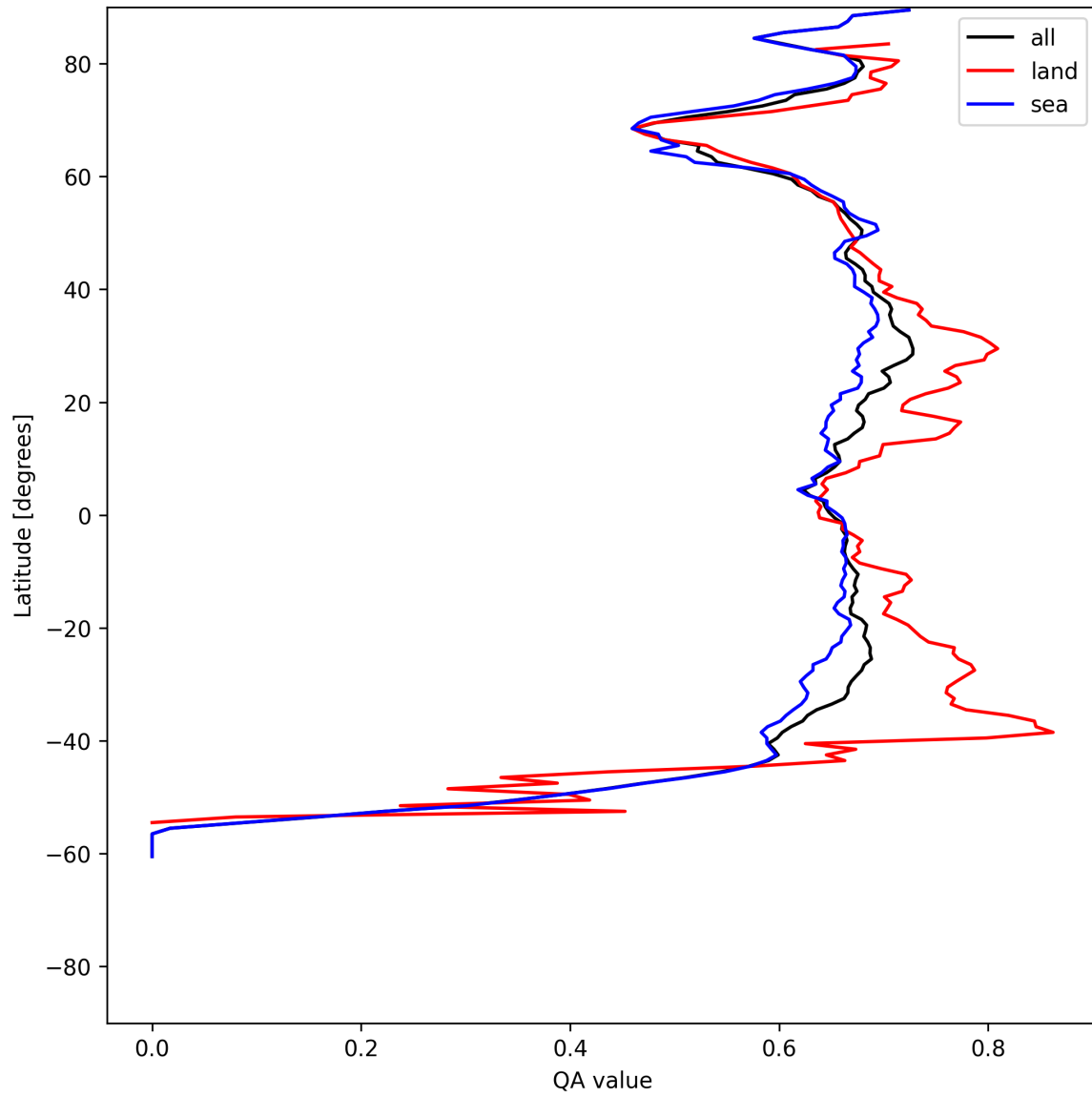
Figure 9: Zonal average of “QA value” for 2025-06-23 to 2025-06-25.
