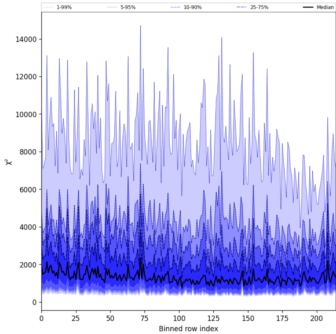
Figure 30: Along track statistics of “ \chi^2 ” for 2025-06-23 to 2025-06-25
