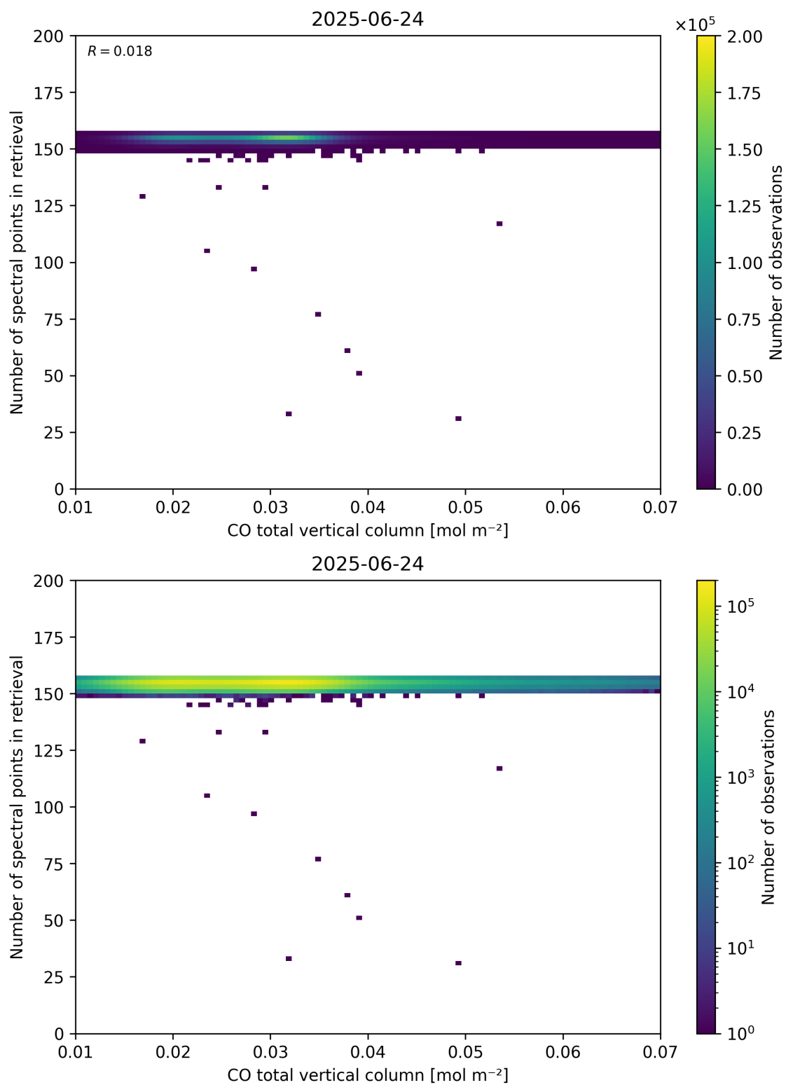
Figure 43: Scatter density plot of “CO total vertical column” against “Number of spectral points in retrieval” for 2025-06-23 to 2025-06-25.
