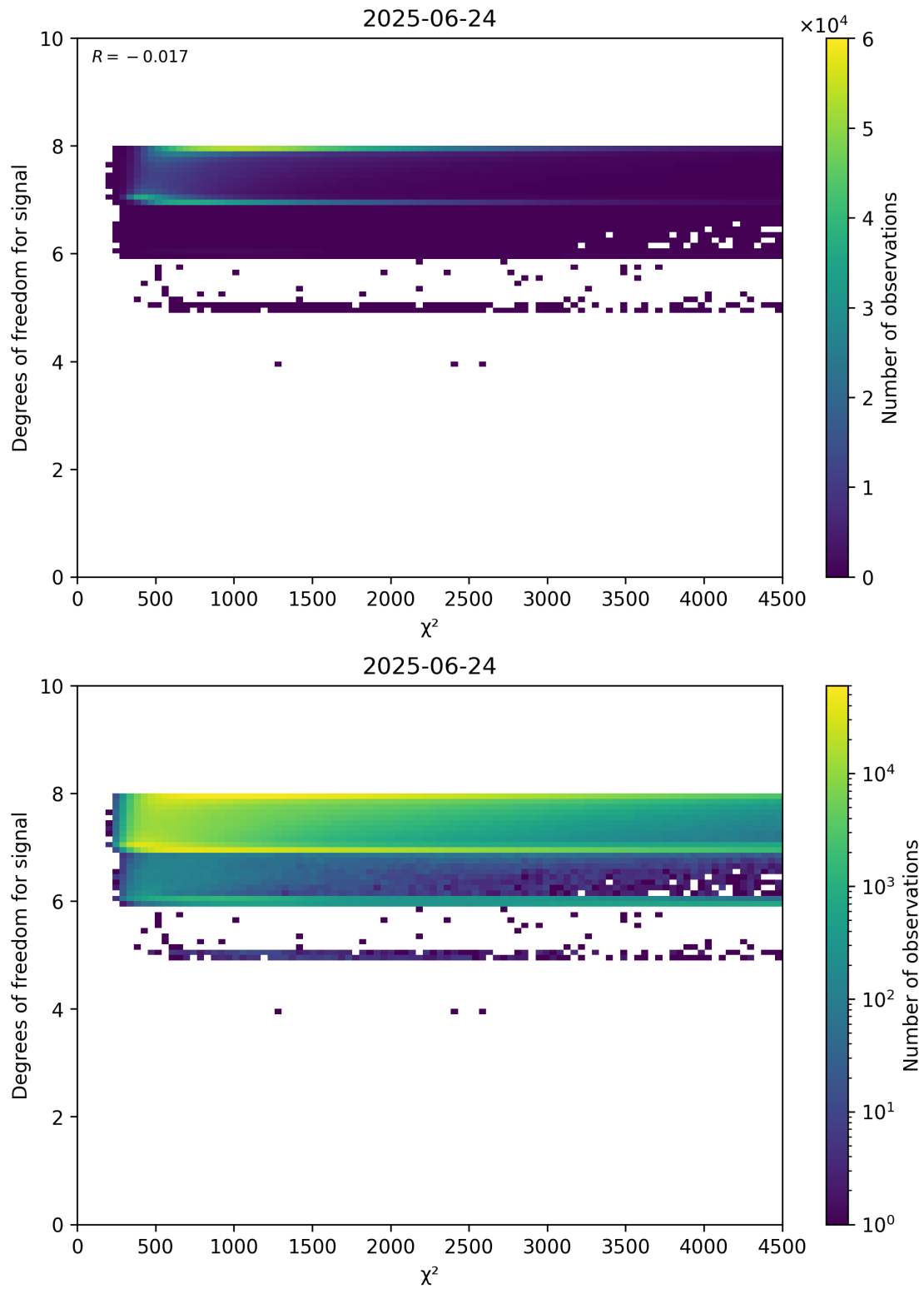
Figure 48: Scatter density plot of “ \chi^2 ” against “Degrees of freedom for signal” for 2025-06-23 to 2025-06-25.
