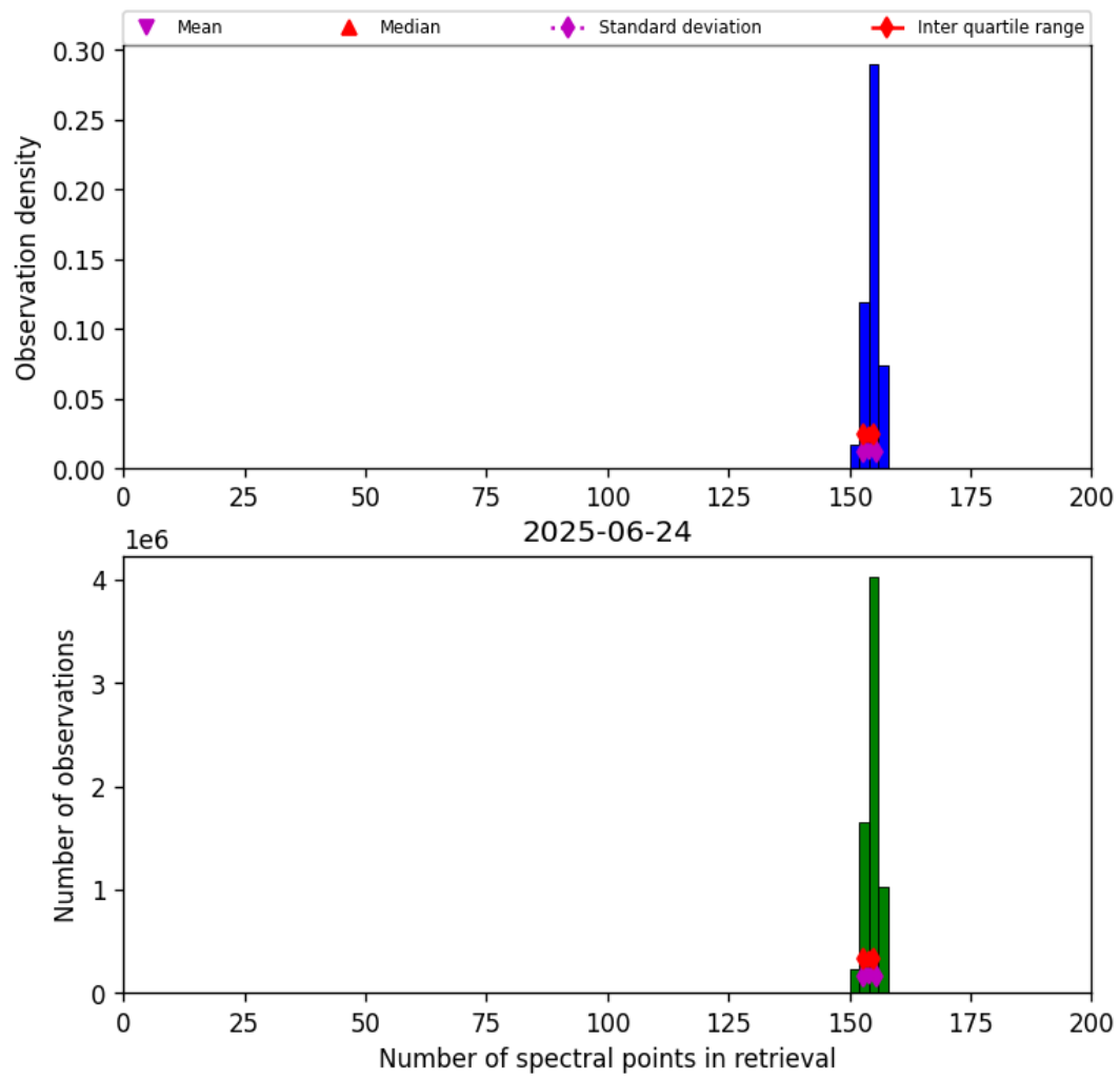
Figure 21: Histogram of “Number of spectral points in retrieval” for 2025-06-23 to 2025-06-25
