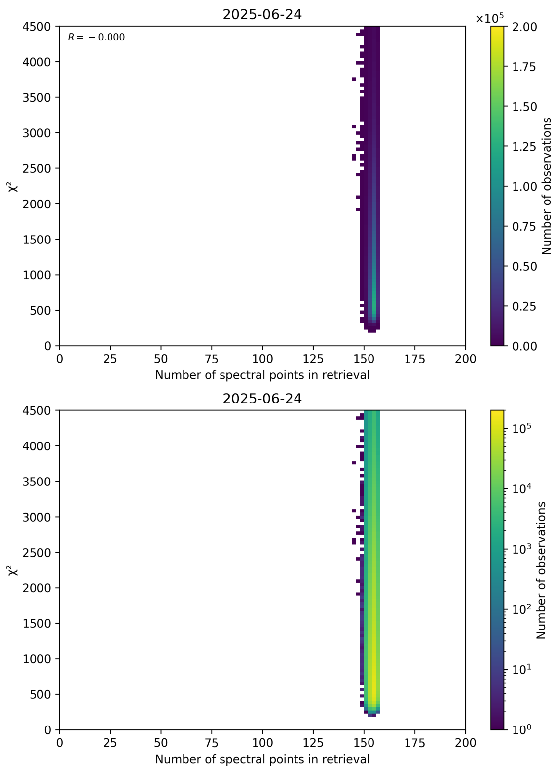
Figure 58: Scatter density plot of “Number of spectral points in retrieval” against “ \chi^2 ” for 2025-06-23 to 2025-06-25.
