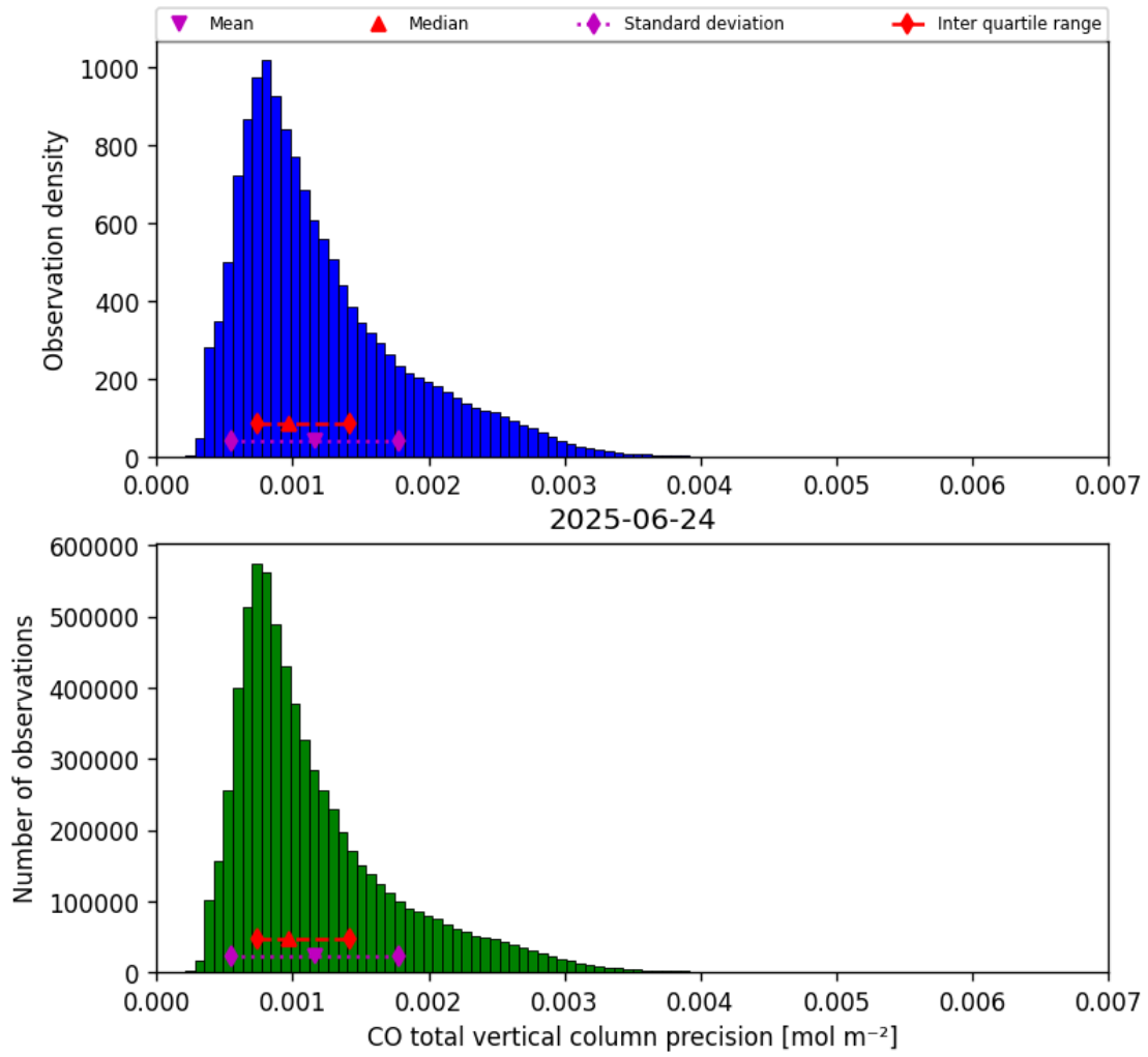
Figure 20: Histogram of “CO total vertical column precision” for 2025-06-23 to 2025-06-25
