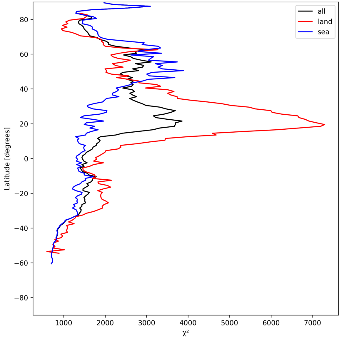
Figure 14: Zonal average of “ \chi^2 ” for 2025-06-23 to 2025-06-25.
