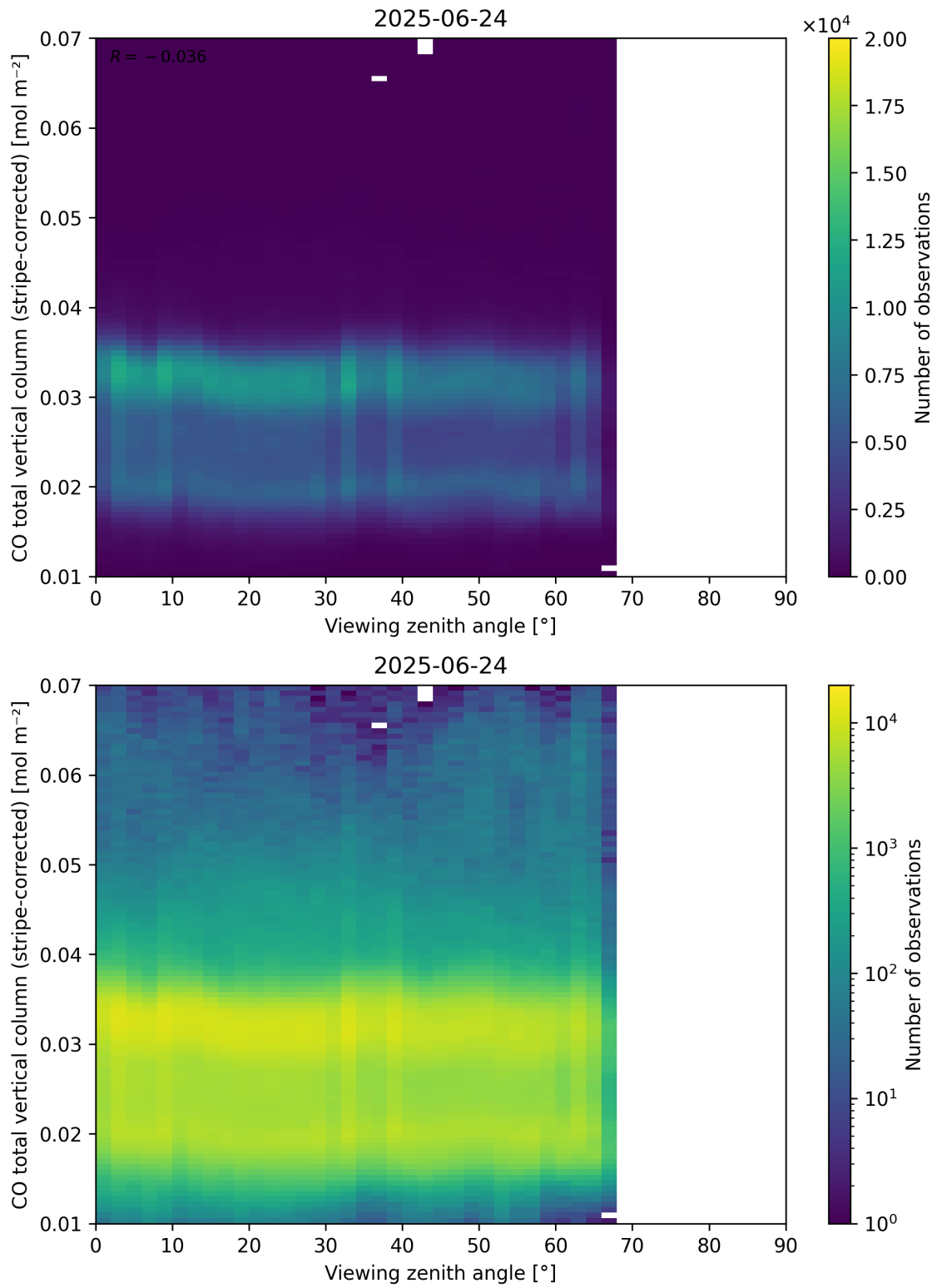
Figure 70: Scatter density plot of “Viewing zenith angle” against “CO total vertical column (stripe-corrected)” for 2025-06-23 to 2025-06-25.
