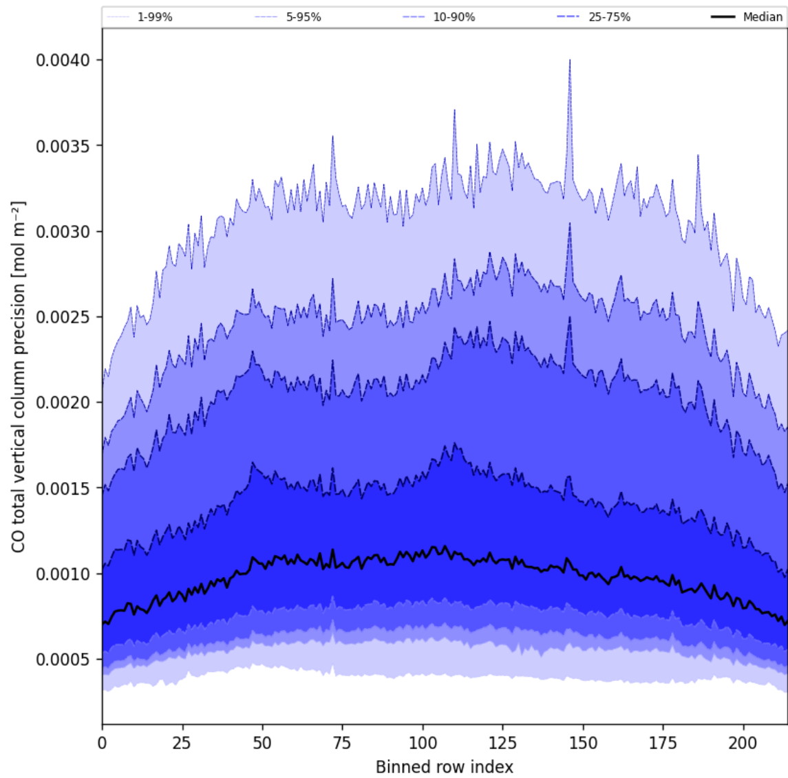
Figure 28: Along track statistics of “CO total vertical column precision” for 2025-06-23 to 2025-06-25
