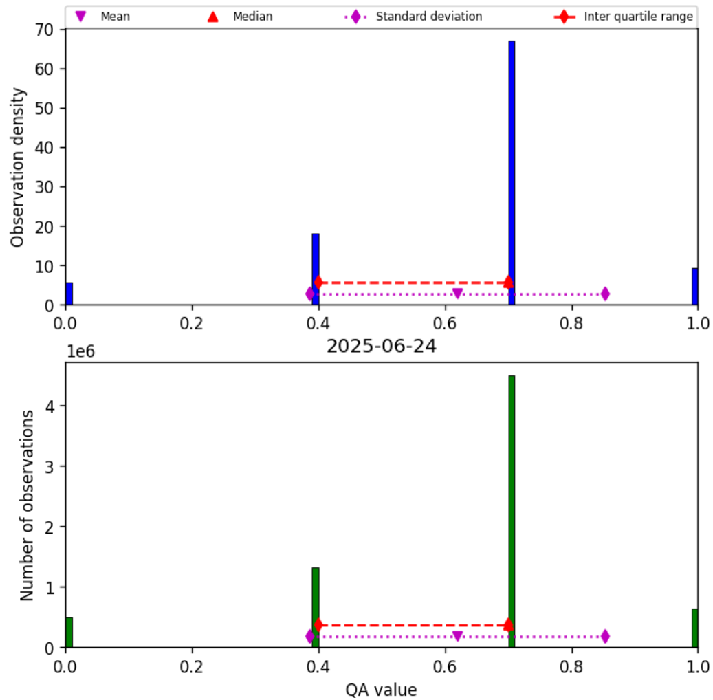
Figure 17: Histogram of “QA value” for 2025-06-23 to 2025-06-25
