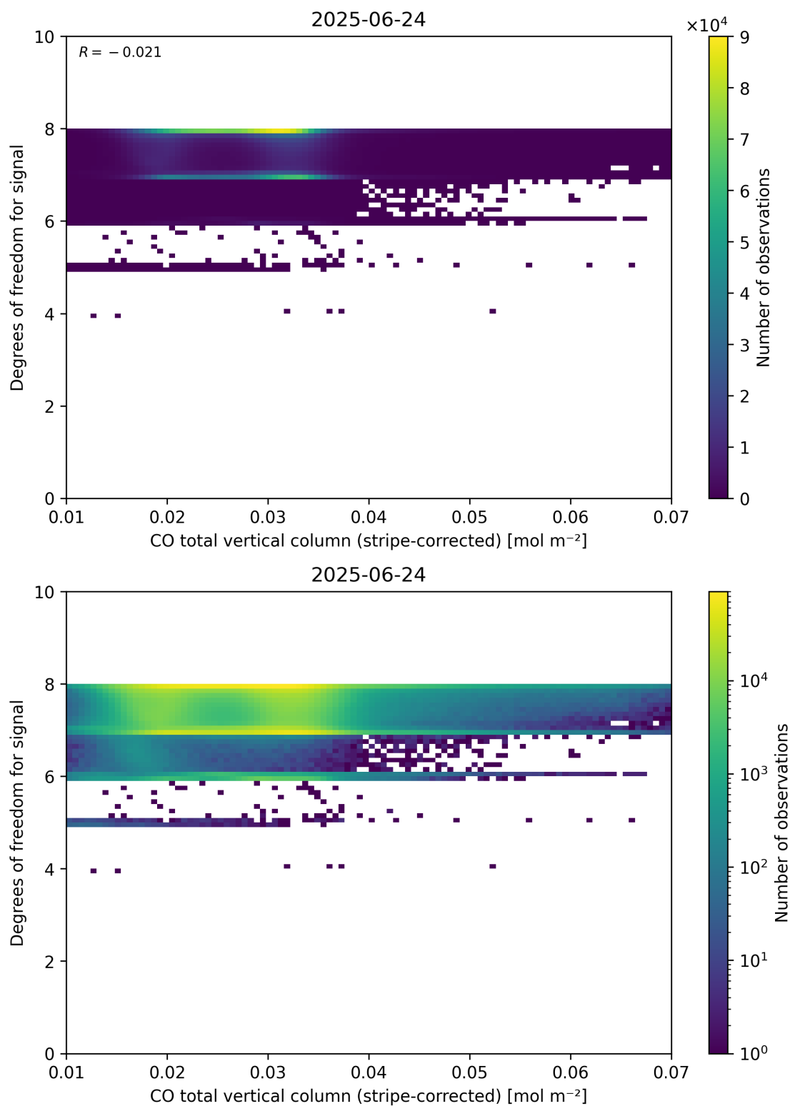
Figure 38: Scatter density plot of “CO total vertical column (stripe-corrected)” against “Degrees of freedom for signal” for 2025-06-23 to 2025-06-25.
