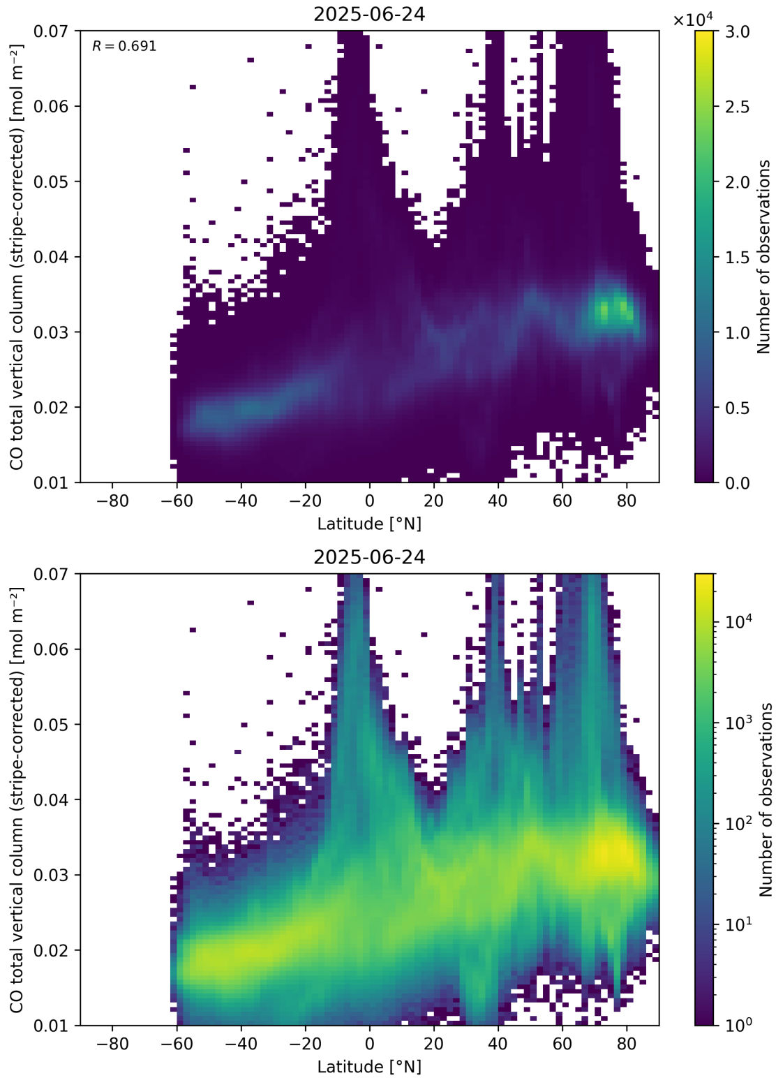
Figure 52: Scatter density plot of “Latitude” against “CO total vertical column (stripe-corrected)” for 2025-06-23 to 2025-06-25.
