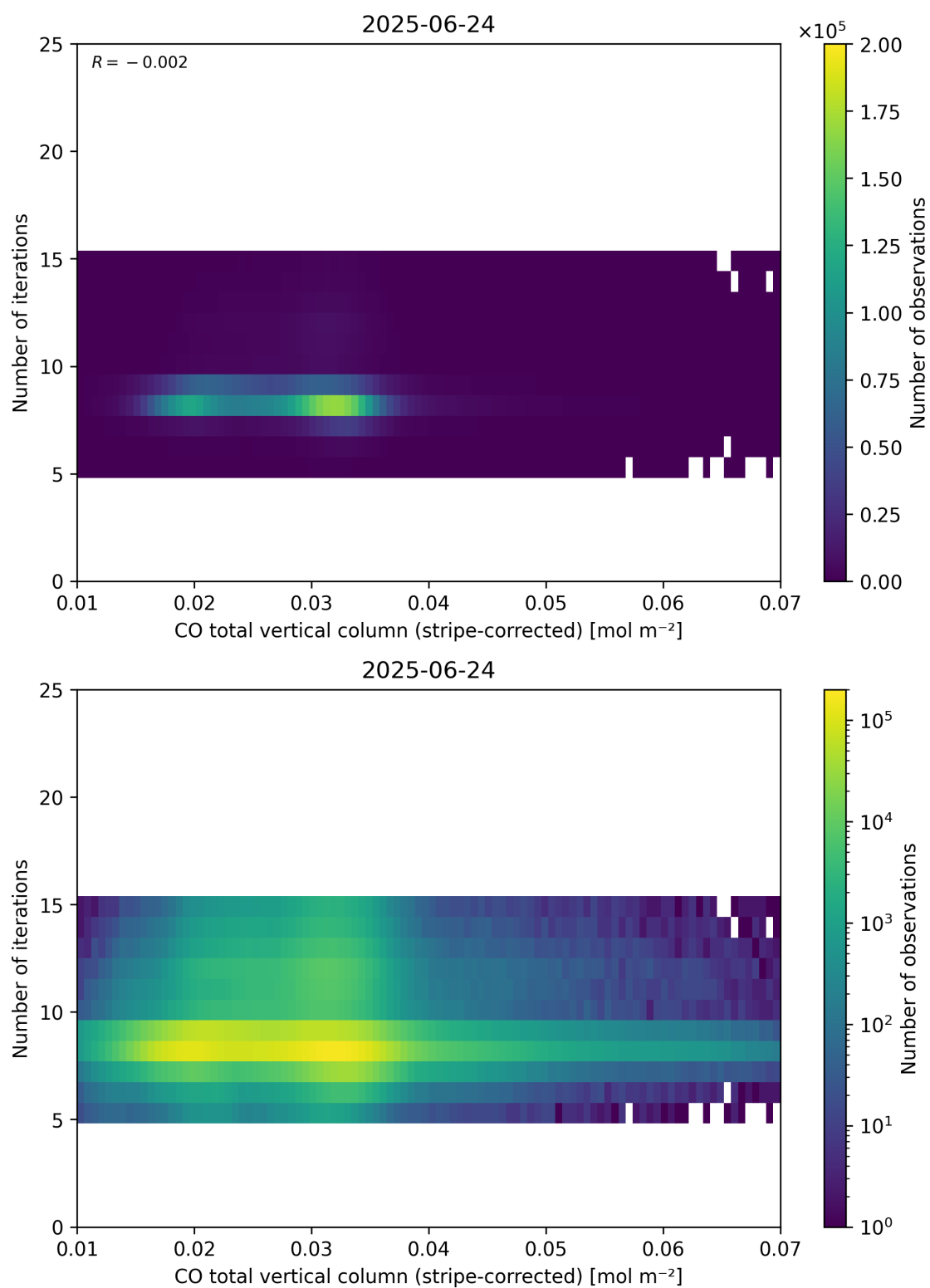
Figure 39: Scatter density plot of “CO total vertical column (stripe-corrected)” against “Number of iterations” for 2025-06-23 to 2025-06-25.
