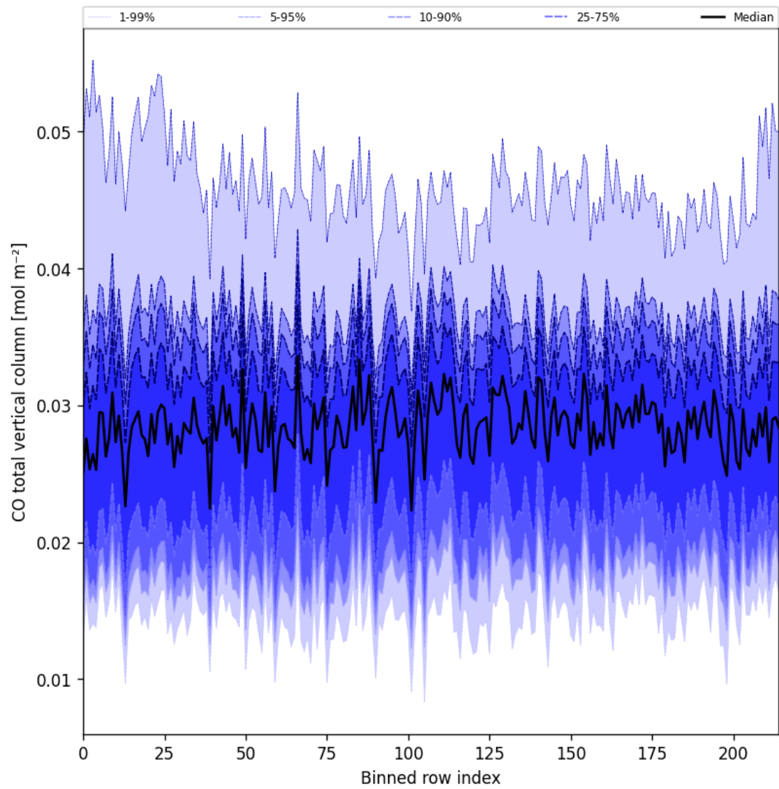
Figure 26: Along track statistics of “CO total vertical column” for 2025-06-23 to 2025-06-25
