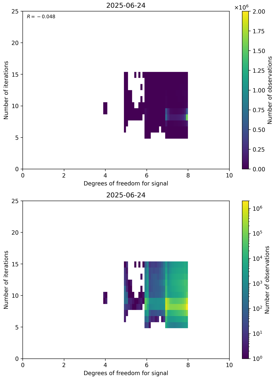
Figure 50: Scatter density plot of “Degrees of freedom for signal” against “Number of iterations” for 2025-06-23 to 2025-06-25.
