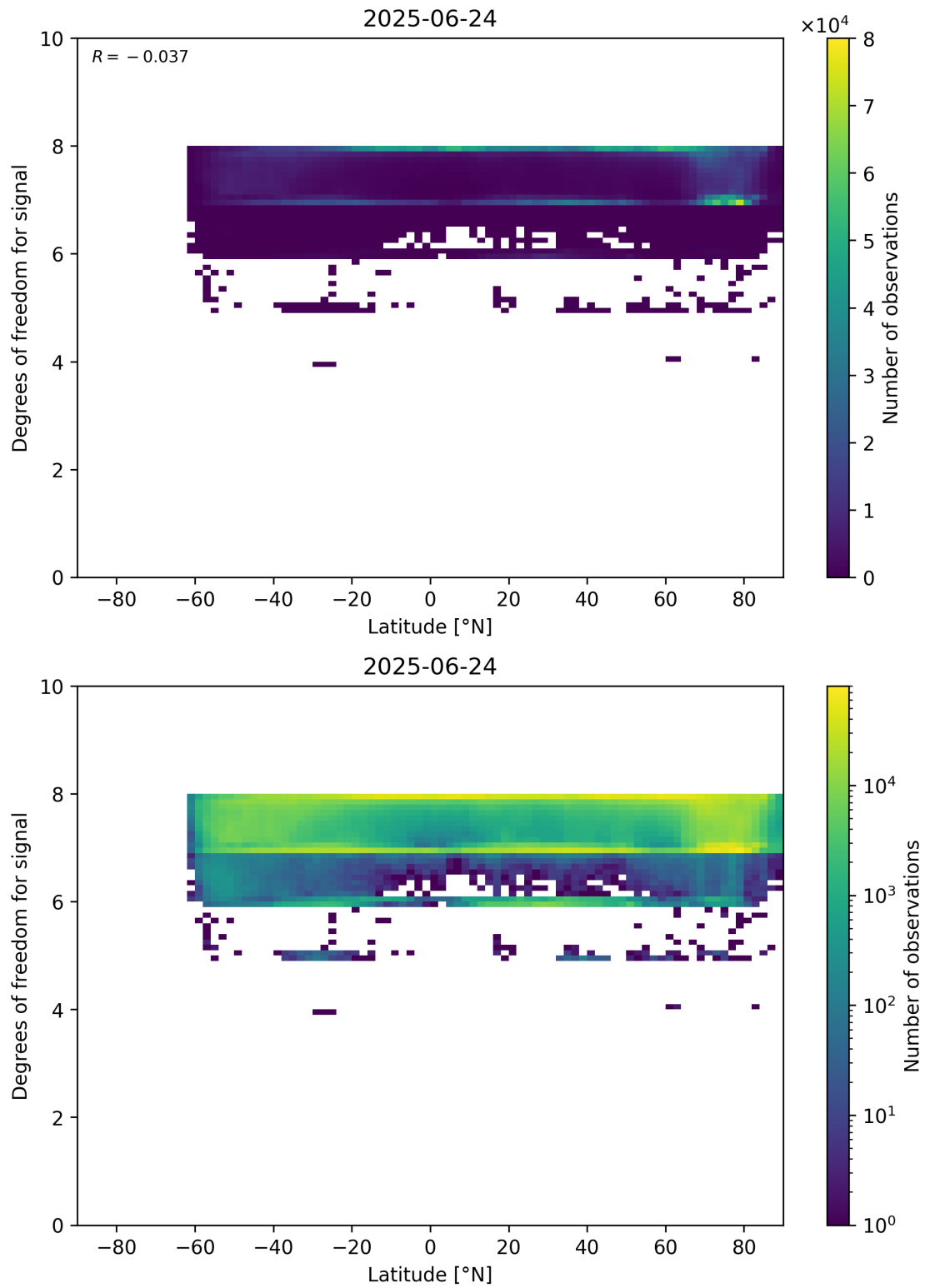
Figure 55: Scatter density plot of “Latitude” against “Degrees of freedom for signal” for 2025-06-23 to 2025-06-25.
