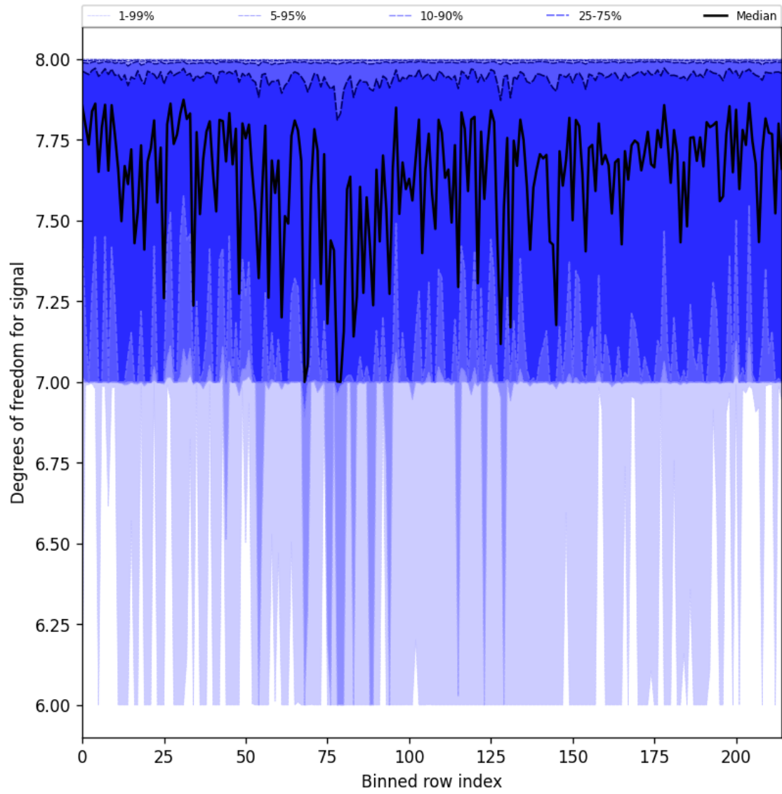
Figure 31: Along track statistics of “Degrees of freedom for signal” for 2025-06-23 to 2025-06-25
