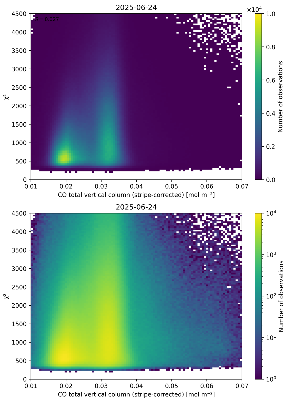
Figure 37: Scatter density plot of “CO total vertical column (stripe-corrected)” against “ \chi^2 ” for 2025-06-23 to 2025-06-25.
