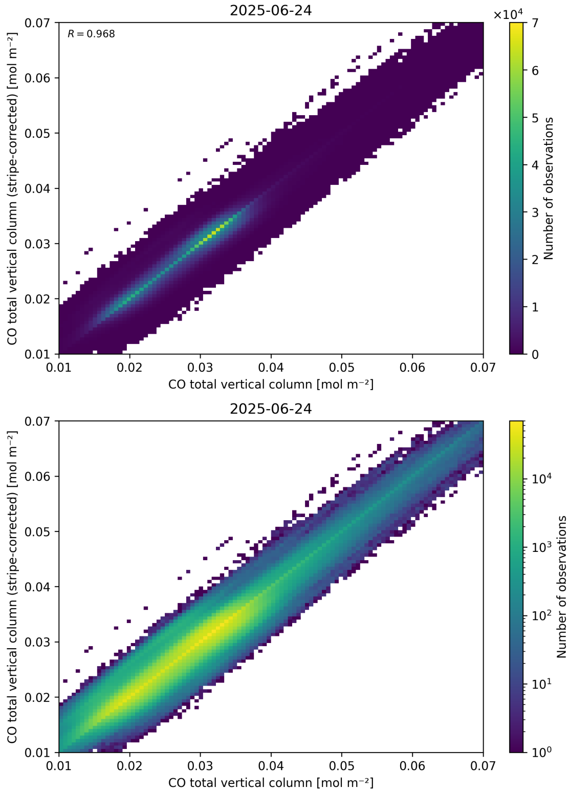
Figure 33: Scatter density plot of “CO total vertical column” against “CO total vertical column (stripe-corrected)” for 2025-06-23 to 2025-06-25.
