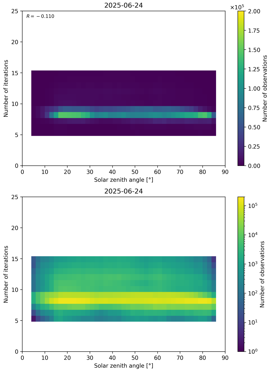
Figure 67: Scatter density plot of “Solar zenith angle” against “Number of iterations” for 2025-06-23 to 2025-06-25.
