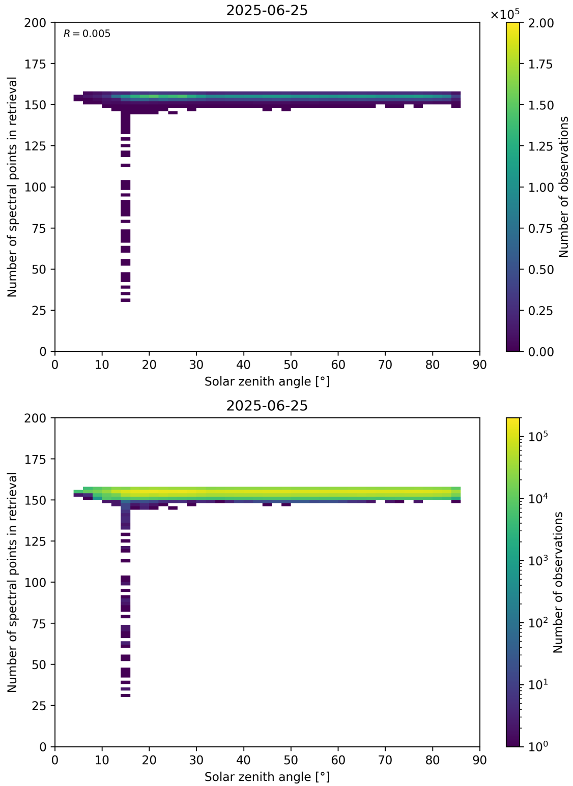
Figure 68: Scatter density plot of “Solar zenith angle” against “Number of spectral points in retrieval” for 2025-06-24 to 2025-06-26.
