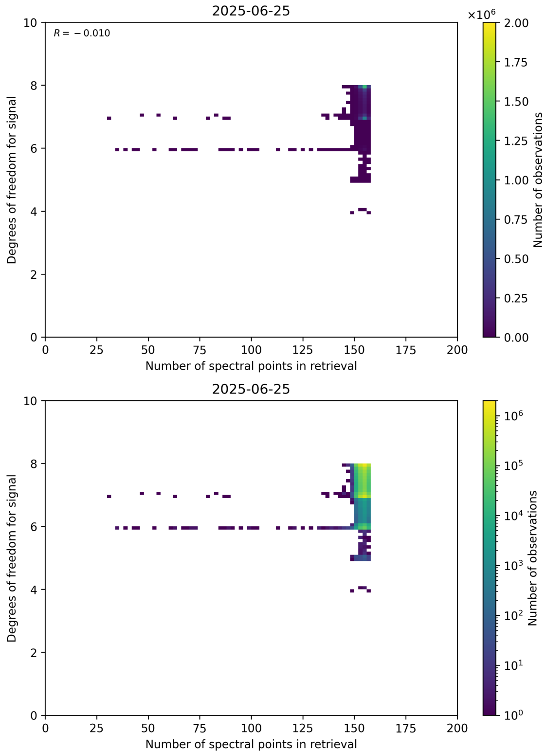
Figure 59: Scatter density plot of “Number of spectral points in retrieval” against “Degrees of freedom for signal” for 2025-06-24 to 2025-06-26.
