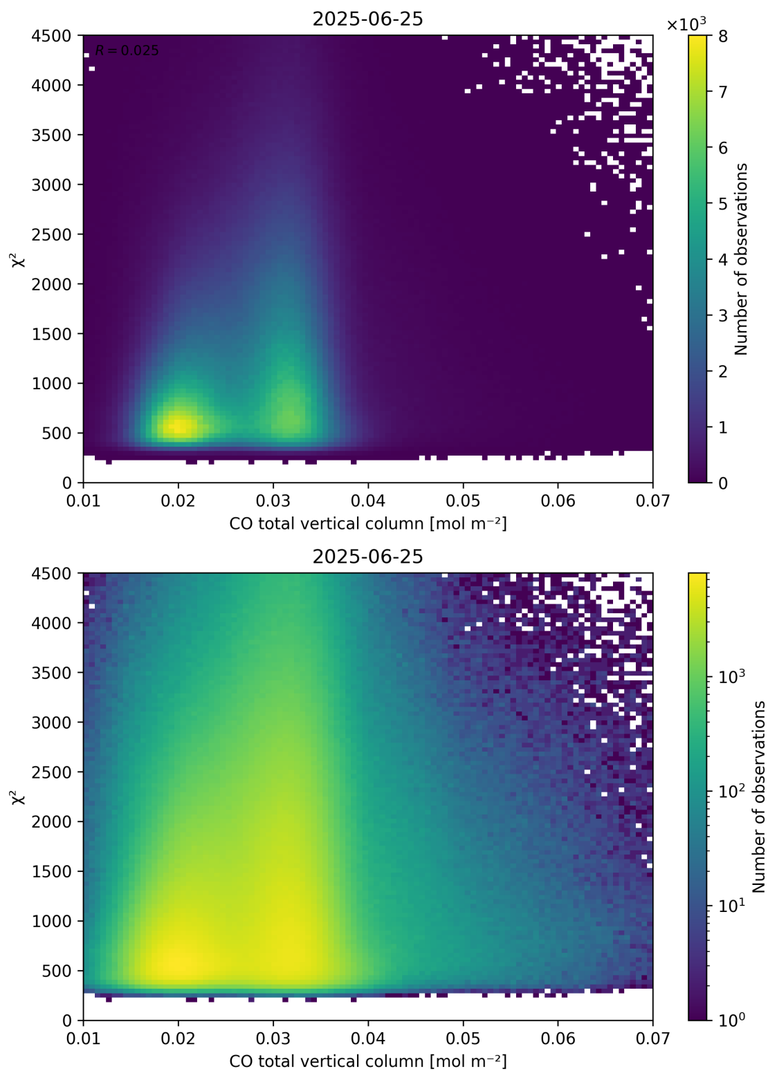
Figure 35: Scatter density plot of “CO total vertical column” against “ \chi^2 ” for 2025-06-24 to 2025-06-26.
