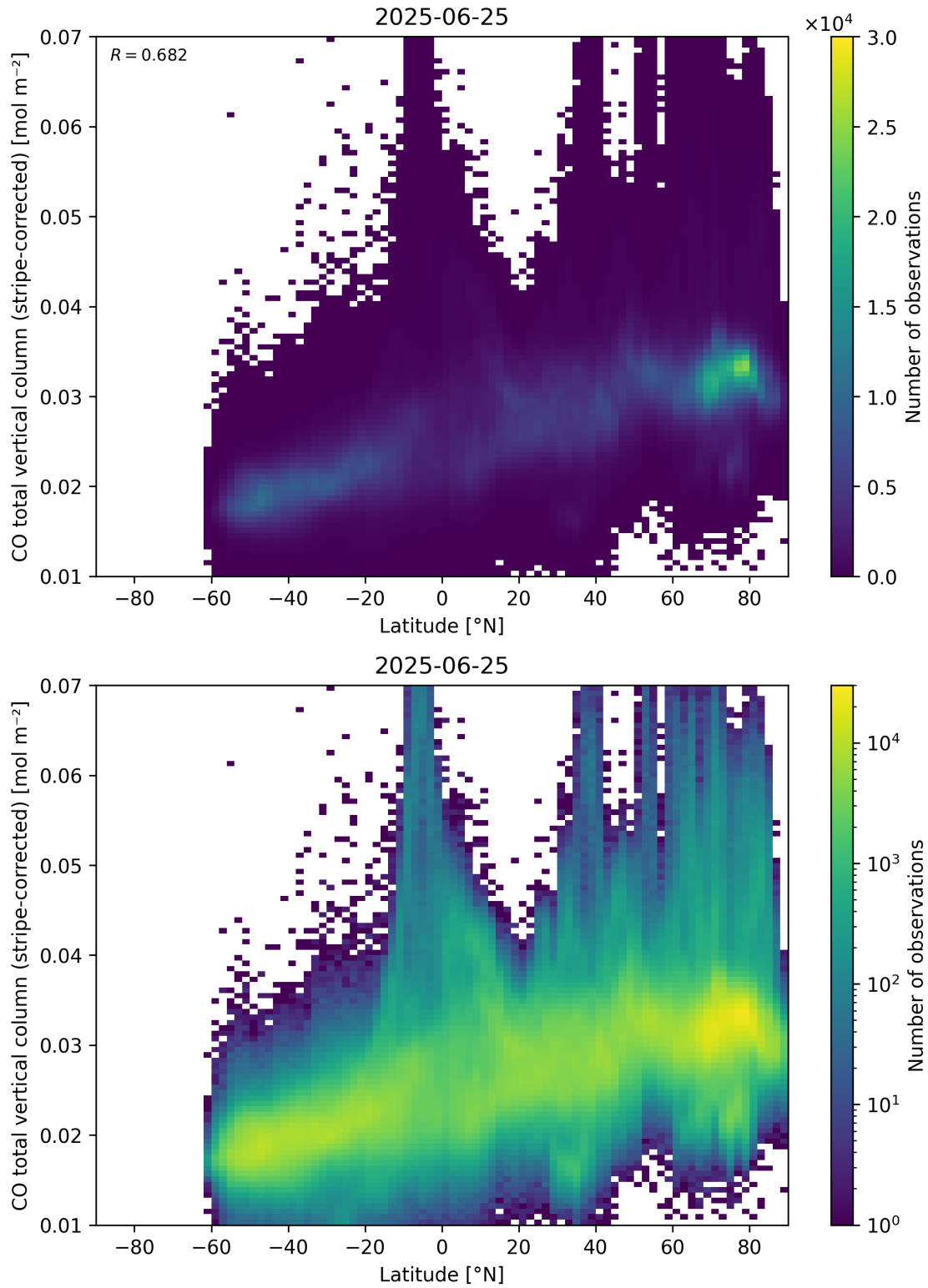
Figure 52: Scatter density plot of “Latitude” against “CO total vertical column (stripe-corrected)” for 2025-06-24 to 2025-06-26.
