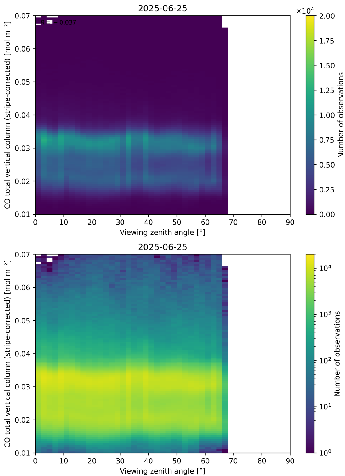
Figure 70: Scatter density plot of “Viewing zenith angle” against “CO total vertical column (stripe-corrected)” for 2025-06-24 to 2025-06-26.
