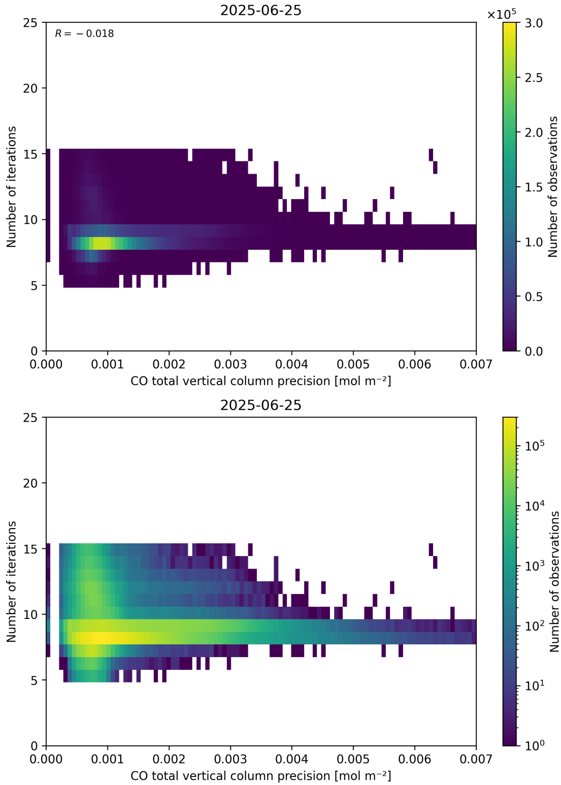
Figure 46: Scatter density plot of “CO total vertical column precision” against “Number of iterations” for 2025-06-24 to 2025-06-26.
