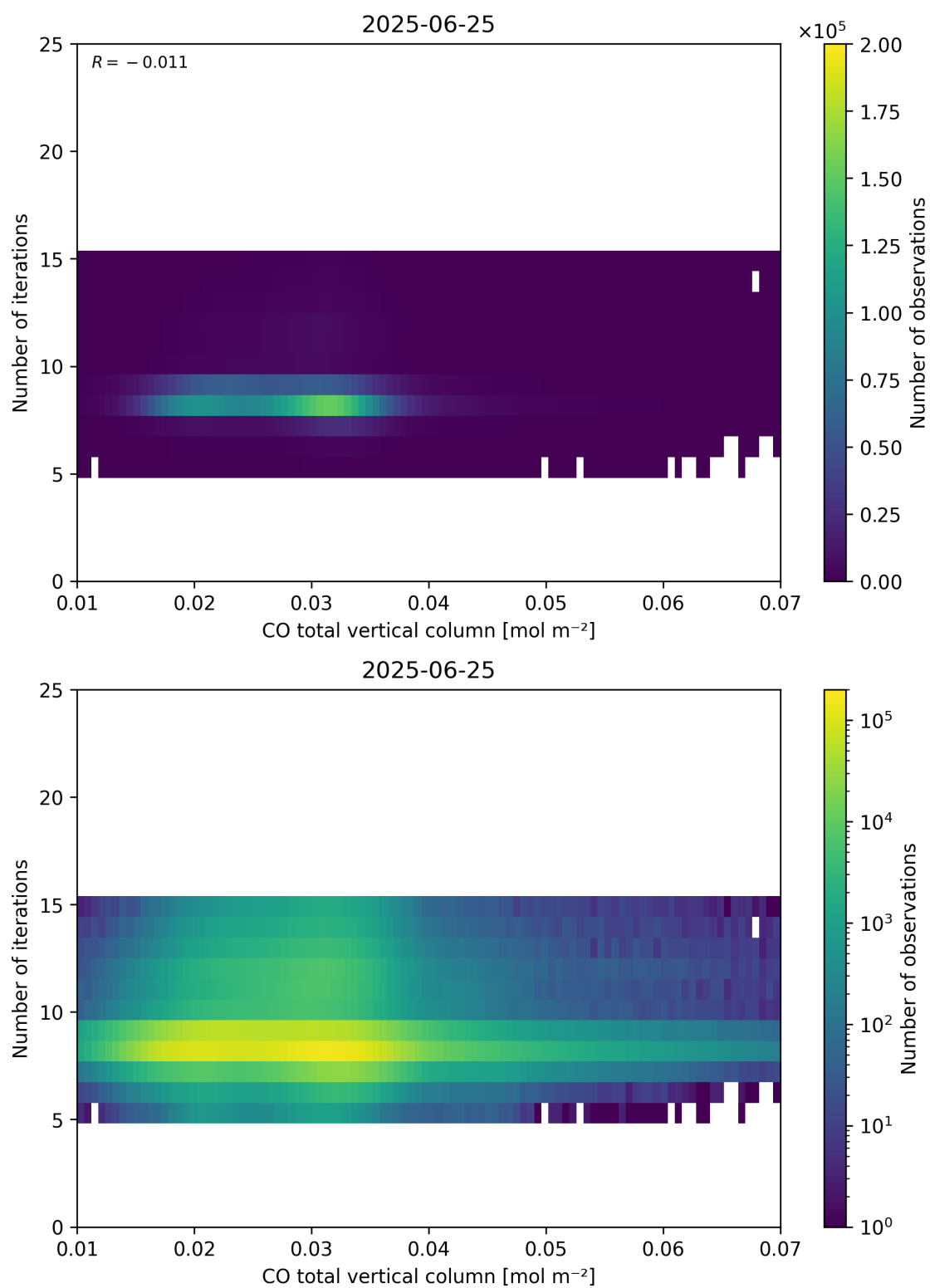
Figure 42: Scatter density plot of “CO total vertical column” against “Number of iterations” for 2025-06-24 to 2025-06-26.
