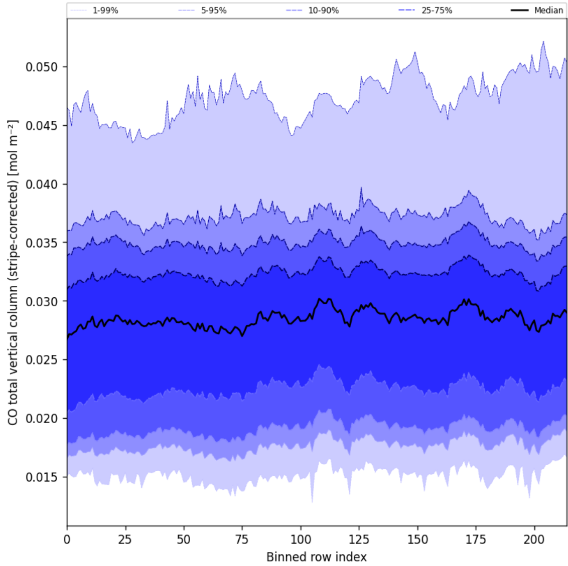
Figure 27: Along track statistics of “CO total vertical column (stripe-corrected)” for 2025-06-24 to 2025-06-26
