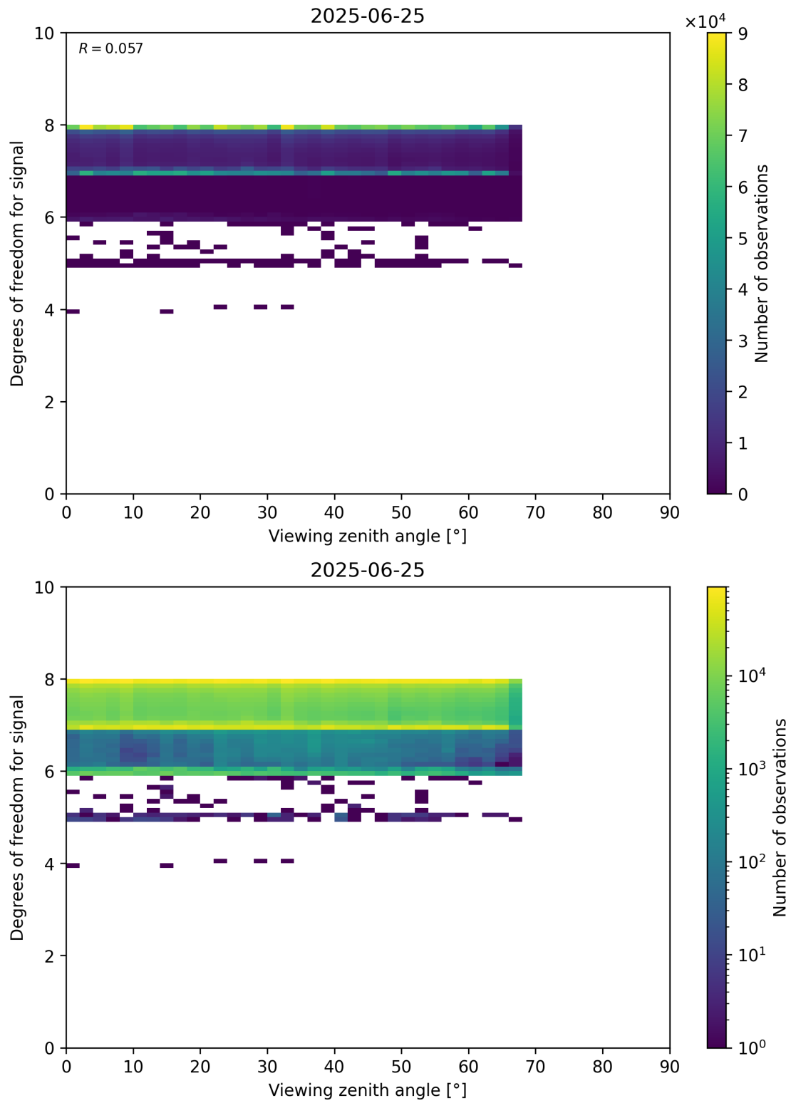
Figure 73: Scatter density plot of “Viewing zenith angle” against “Degrees of freedom for signal” for 2025-06-24 to 2025-06-26.
