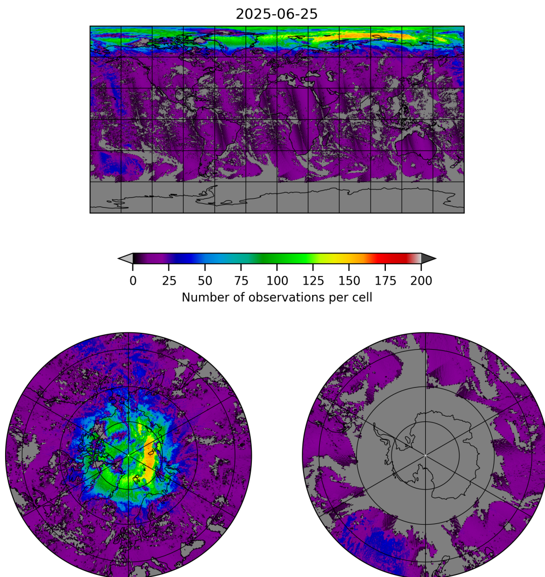
Figure 8: Map of the number of observations for 2025-06-24 to 2025-06-26
