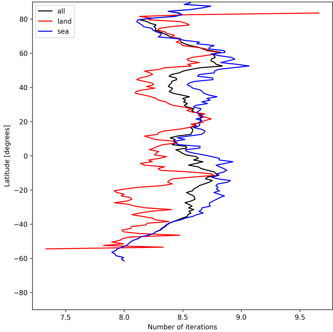
Figure 16: Zonal average of “Number of iterations” for 2025-06-24 to 2025-06-26.
