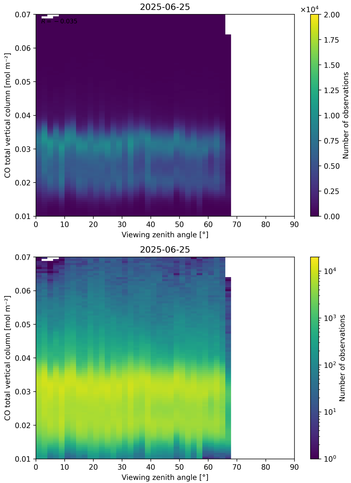
Figure 69: Scatter density plot of “Viewing zenith angle” against “CO total vertical column” for 2025-06-24 to 2025-06-26.
