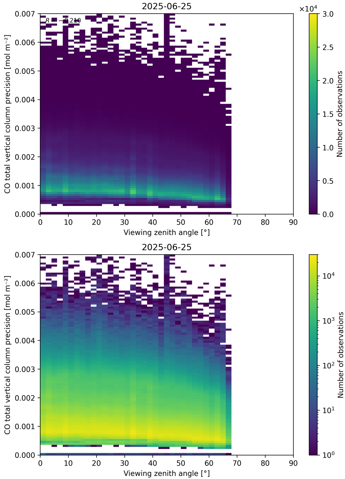
Figure 71: Scatter density plot of “Viewing zenith angle” against “CO total vertical column precision” for 2025-06-24 to 2025-06-26.
