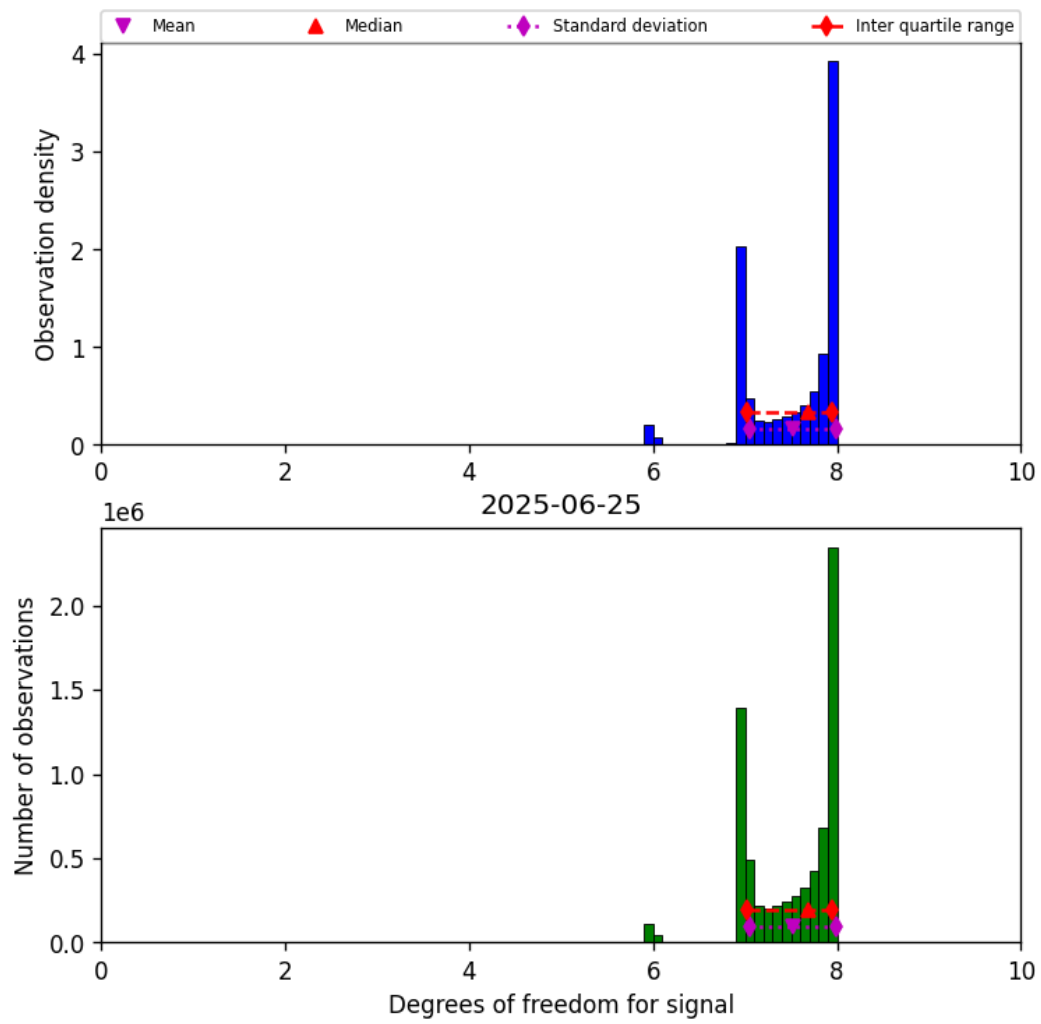
Figure 23: Histogram of “Degrees of freedom for signal” for 2025-06-24 to 2025-06-26
