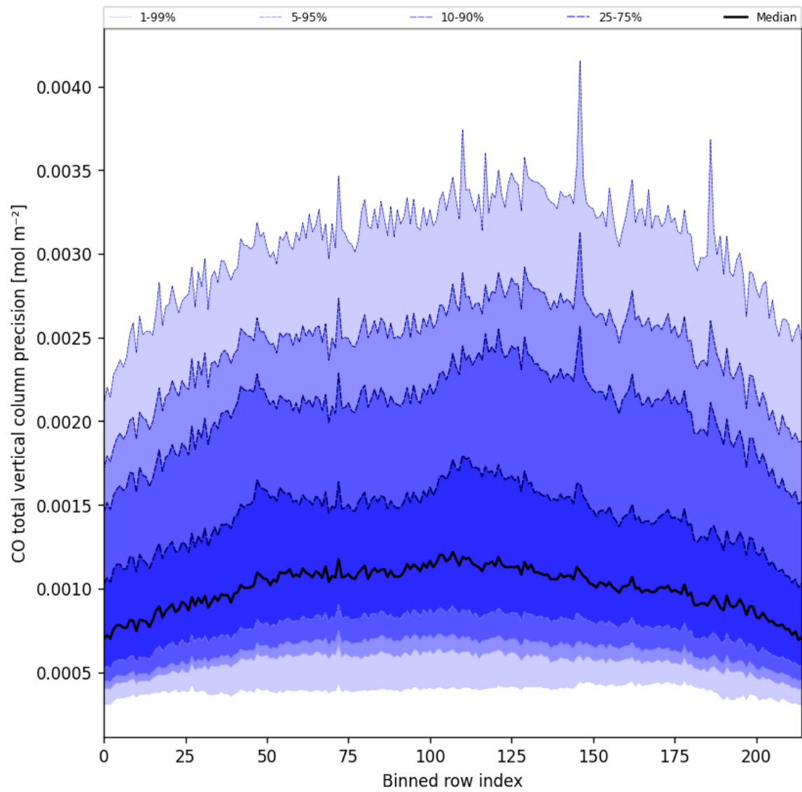
Figure 28: Along track statistics of “CO total vertical column precision” for 2025-06-24 to 2025-06-26
