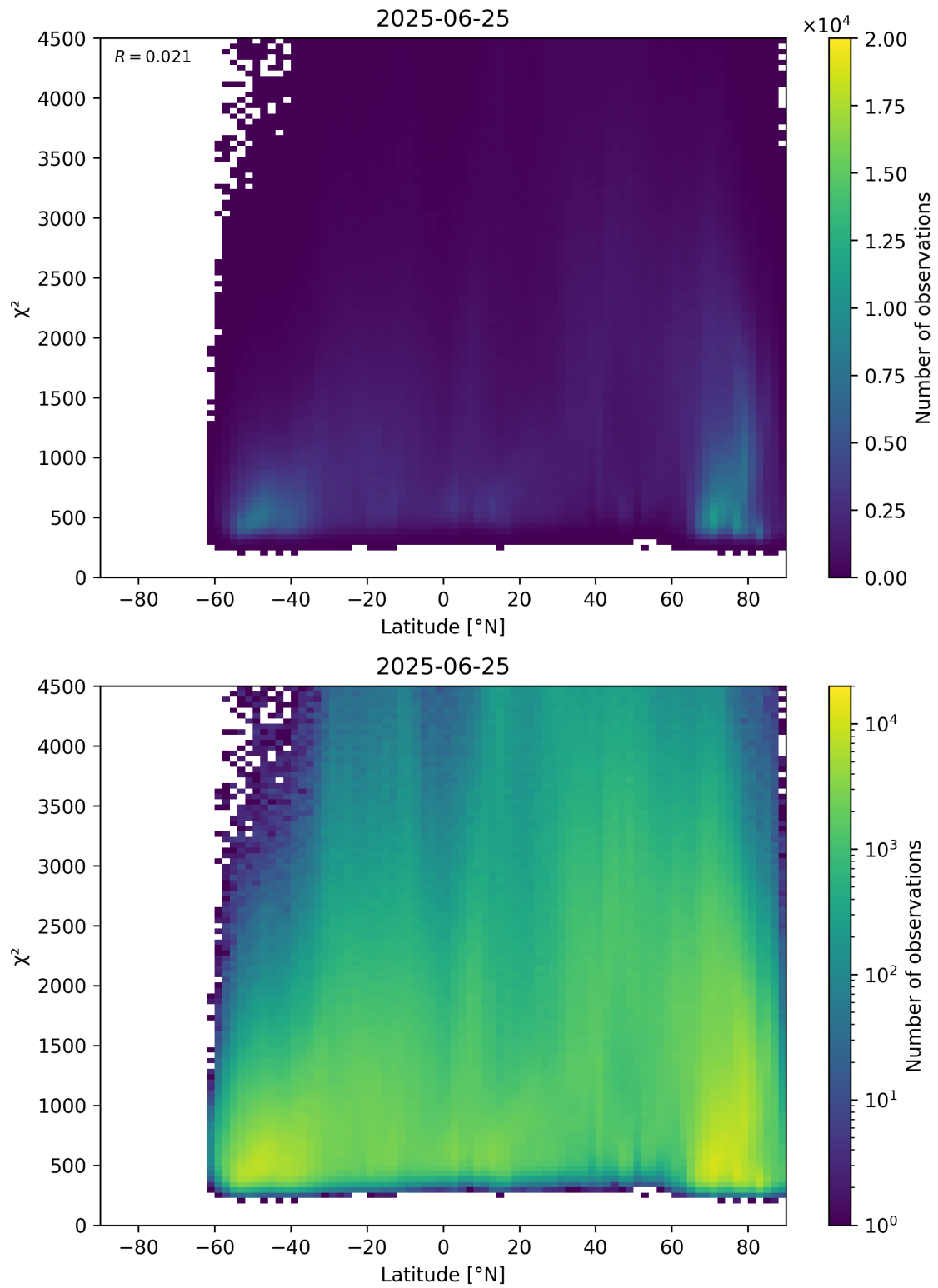
Figure 54: Scatter density plot of “Latitude” against “ \chi^2 ” for 2025-06-24 to 2025-06-26.
