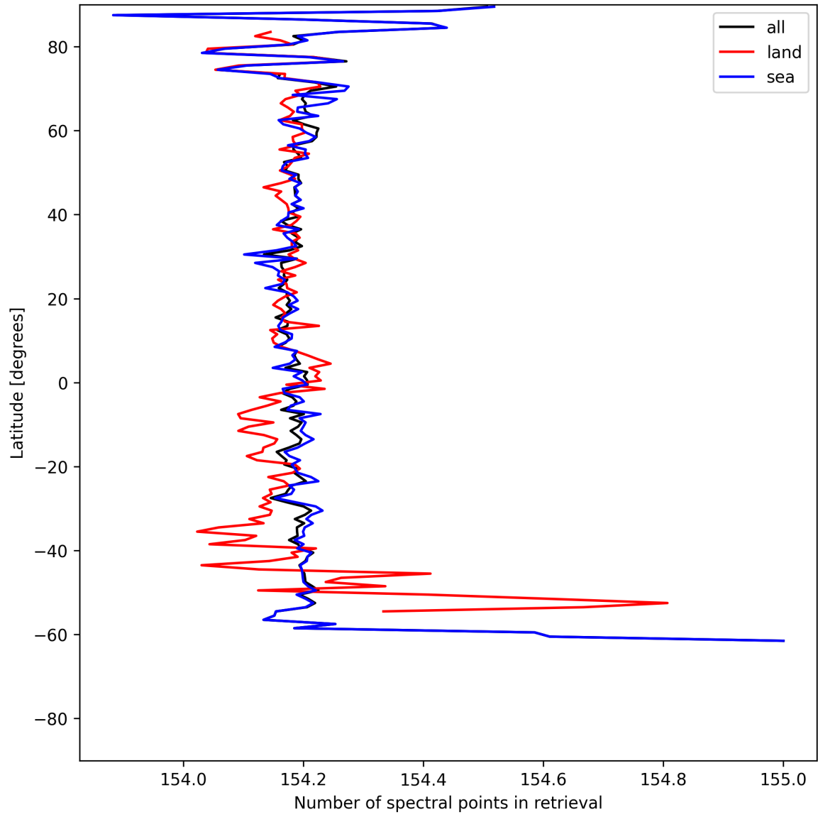
Figure 13: Zonal average of “Number of spectral points in retrieval” for 2025-06-24 to 2025-06-26.
