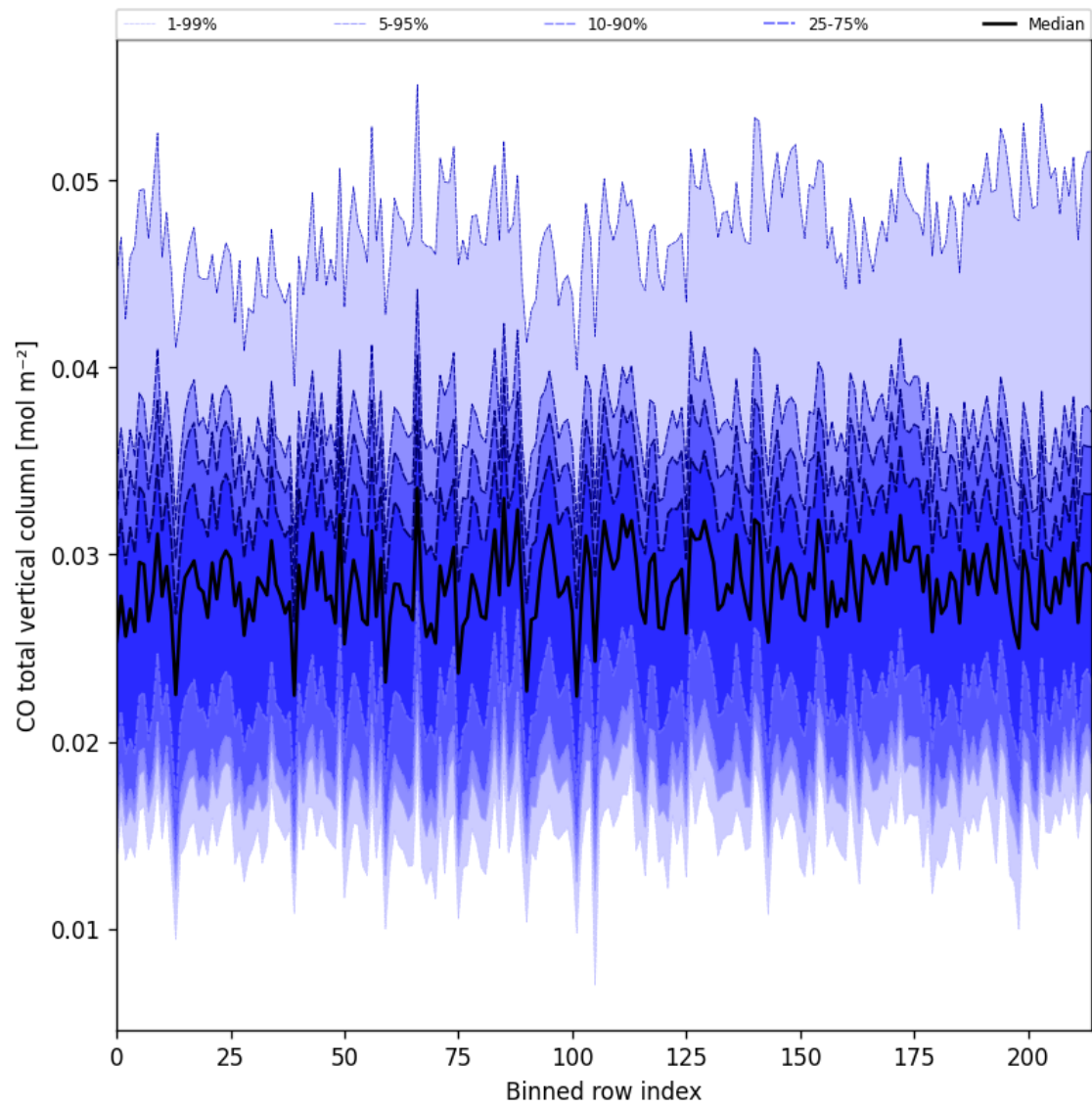
Figure 26: Along track statistics of “CO total vertical column” for 2025-06-24 to 2025-06-26
