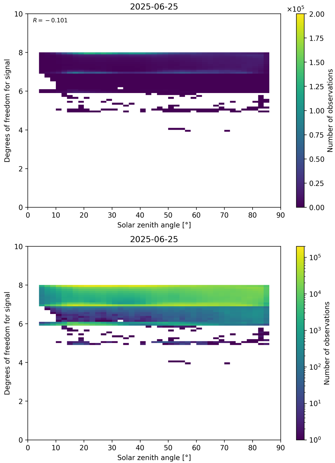
Figure 65: Scatter density plot of “Solar zenith angle” against “Degrees of freedom for signal” for 2025-06-24 to 2025-06-26.
