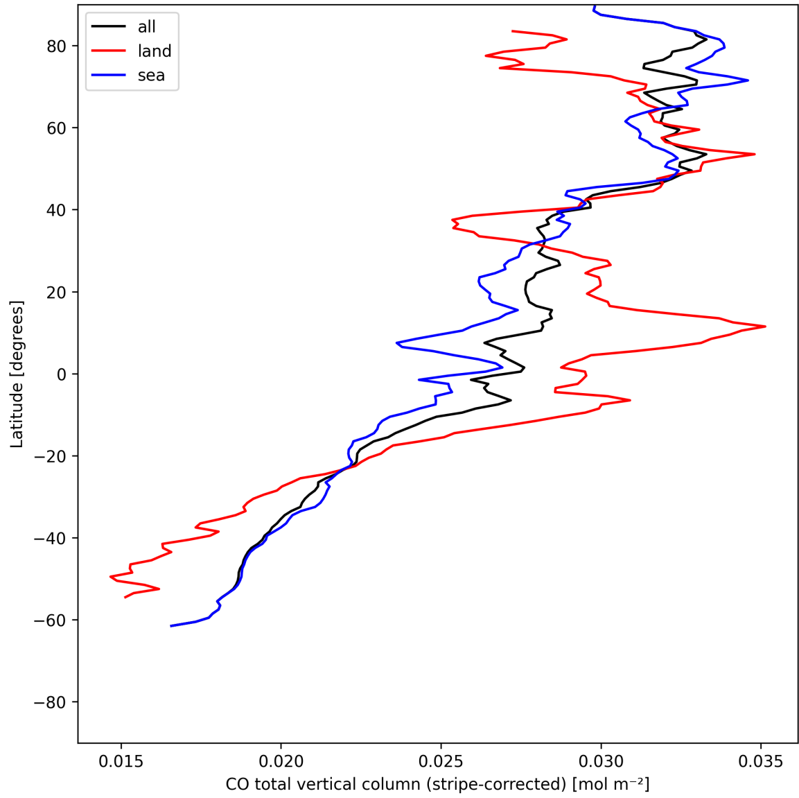
Figure 11: Zonal average of “CO total vertical column (stripe-corrected)” for 2025-06-24 to 2025-06-26.
