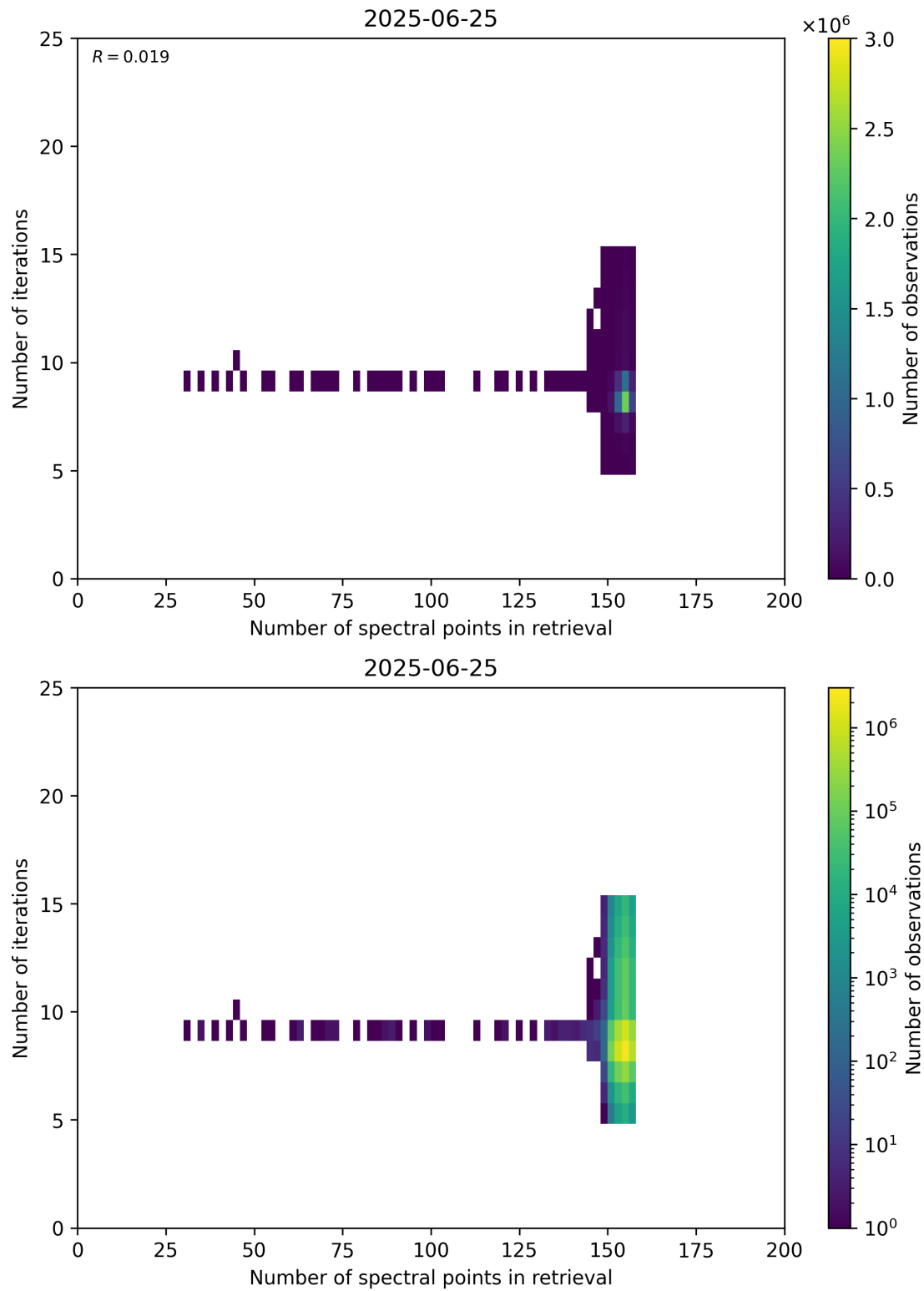
Figure 60: Scatter density plot of “Number of spectral points in retrieval” against “Number of iterations” for 2025-06-24 to 2025-06-26.
