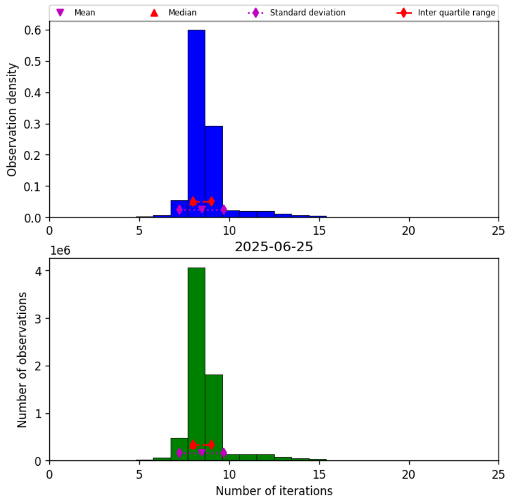
Figure 24: Histogram of “Number of iterations” for 2025-06-24 to 2025-06-26
