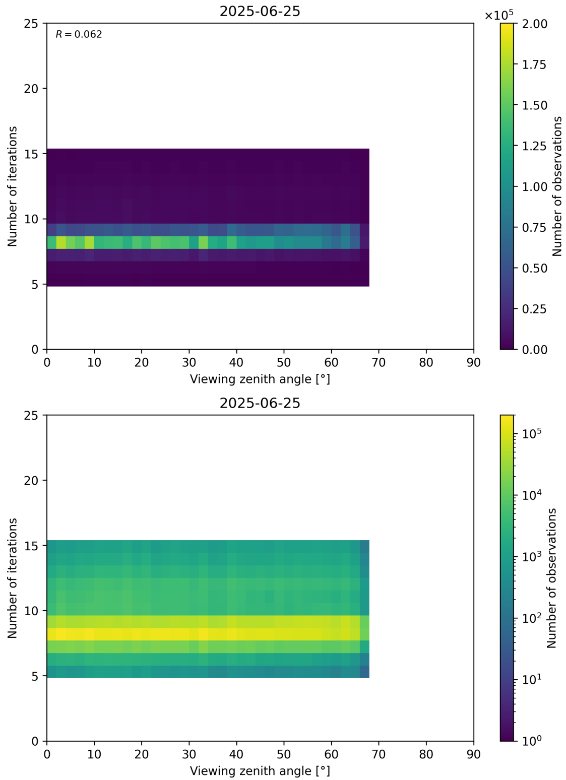
Figure 75: Scatter density plot of “Viewing zenith angle” against “Number of iterations” for 2025-06-24 to 2025-06-26.
