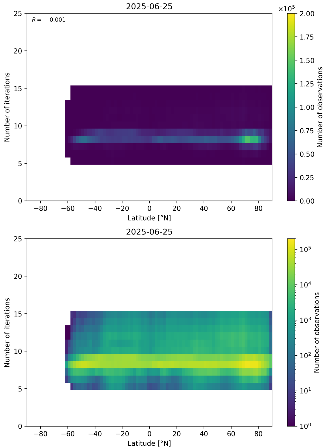
Figure 56: Scatter density plot of “Latitude” against “Number of iterations” for 2025-06-24 to 2025-06-26.
