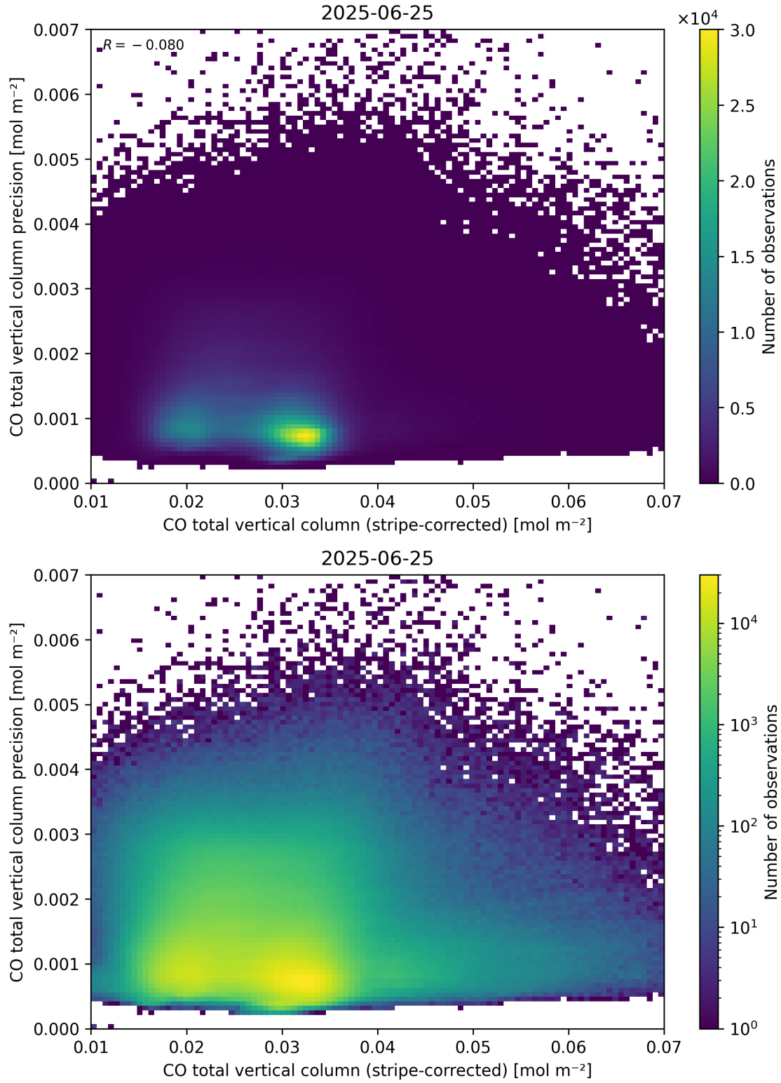
Figure 36: Scatter density plot of “CO total vertical column (stripe-corrected)” against “CO total vertical column precision” for 2025-06-24 to 2025-06-26.
