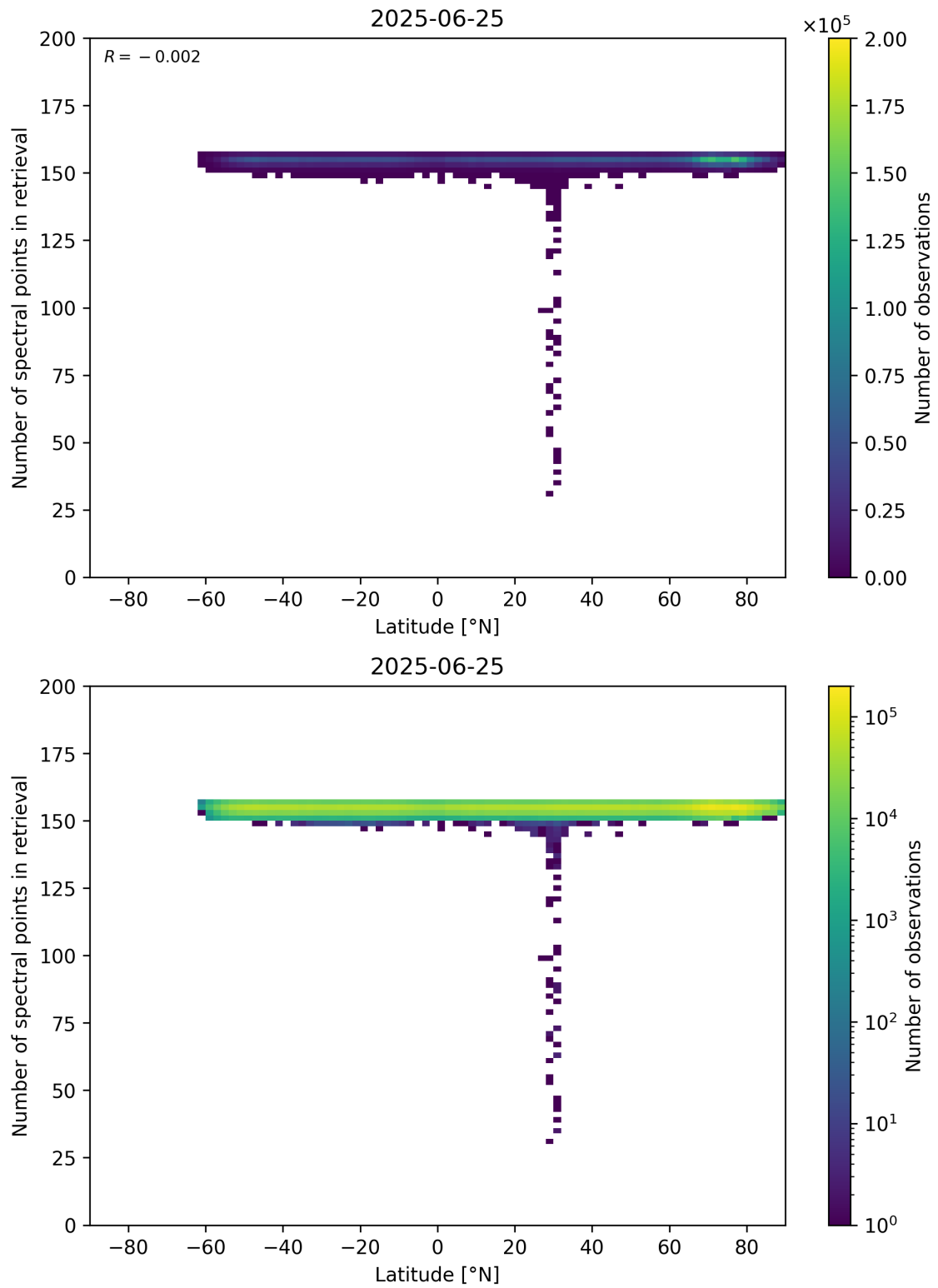
Figure 57: Scatter density plot of “Latitude” against “Number of spectral points in retrieval” for 2025-06-24 to 2025-06-26.
