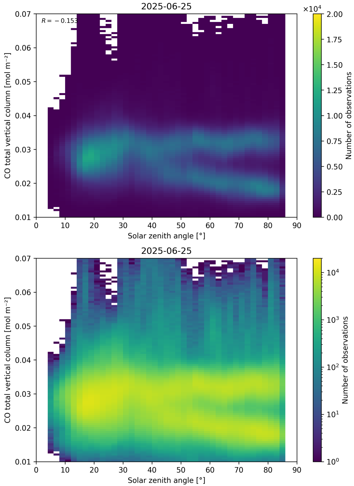
Figure 61: Scatter density plot of “Solar zenith angle” against “CO total vertical column” for 2025-06-24 to 2025-06-26.
