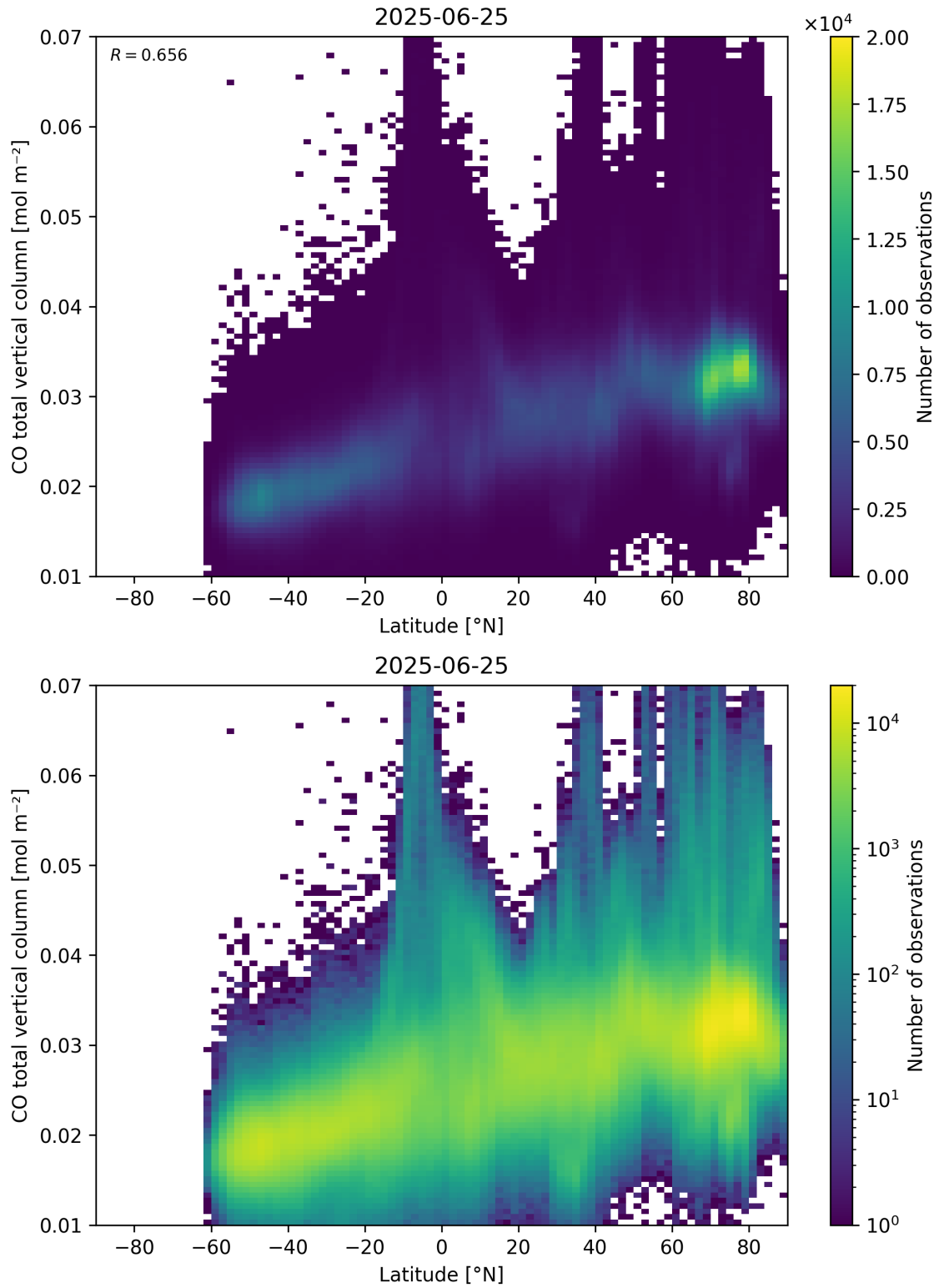
Figure 51: Scatter density plot of “Latitude” against “CO total vertical column” for 2025-06-24 to 2025-06-26.
