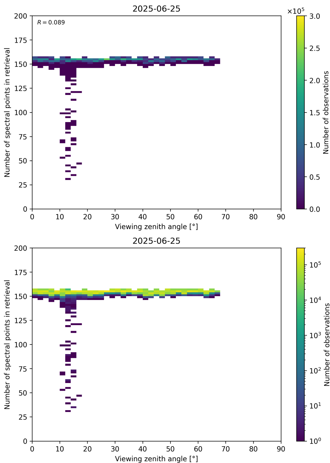
Figure 76: Scatter density plot of “Viewing zenith angle” against “Number of spectral points in retrieval” for 2025-06-24 to 2025-06-26.
