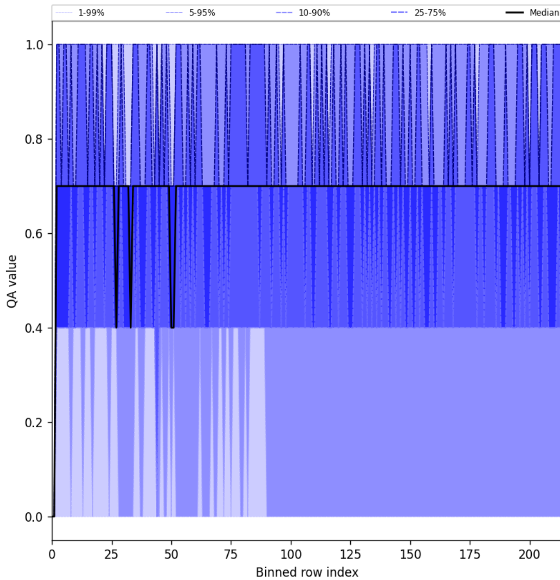
Figure 25: Along track statistics of “QA value” for 2025-06-24 to 2025-06-26
