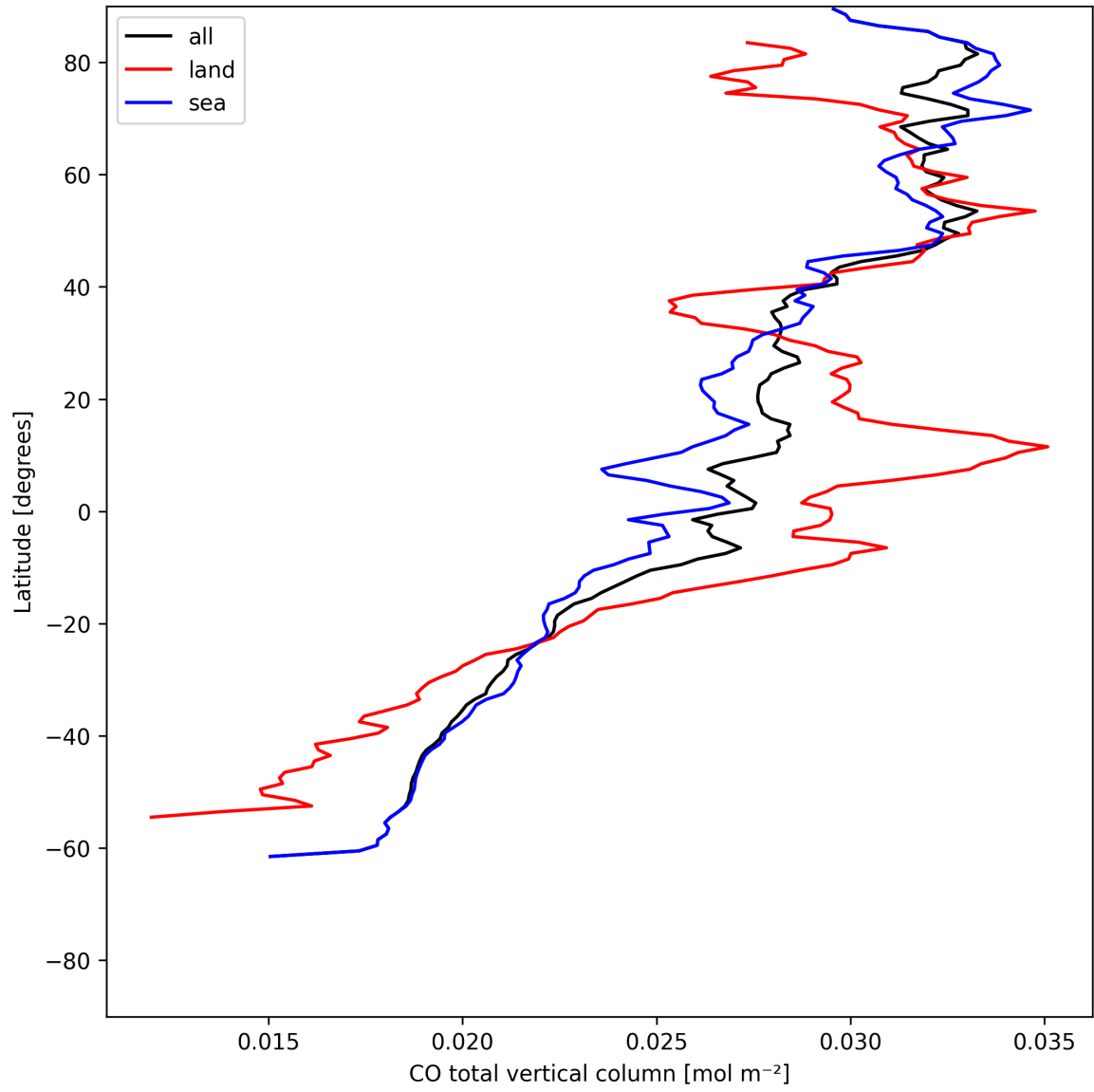
Figure 10: Zonal average of “CO total vertical column” for 2025-06-24 to 2025-06-26.
