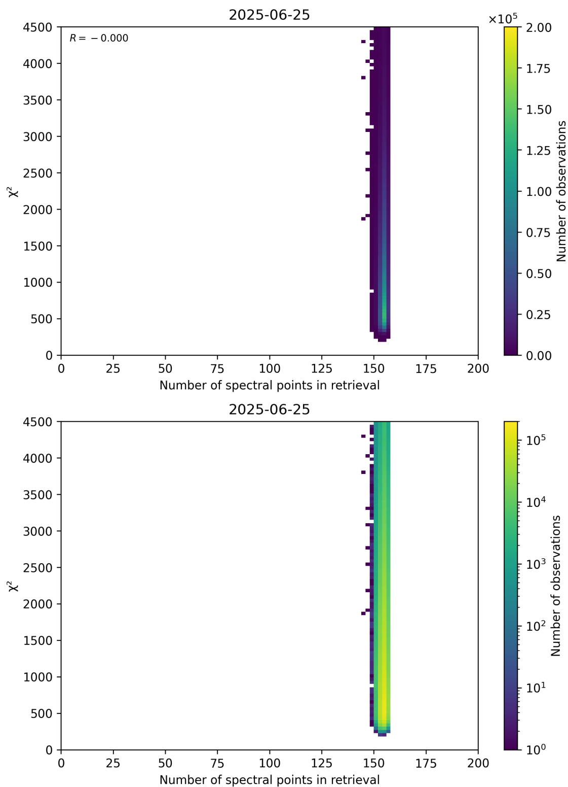
Figure 58: Scatter density plot of “Number of spectral points in retrieval” against “ \chi^2 ” for 2025-06-24 to 2025-06-26.
