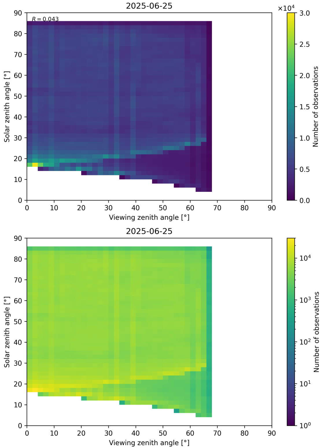
Figure 77: Scatter density plot of “Viewing zenith angle” against “Solar zenith angle” for 2025-06-24 to 2025-06-26.
