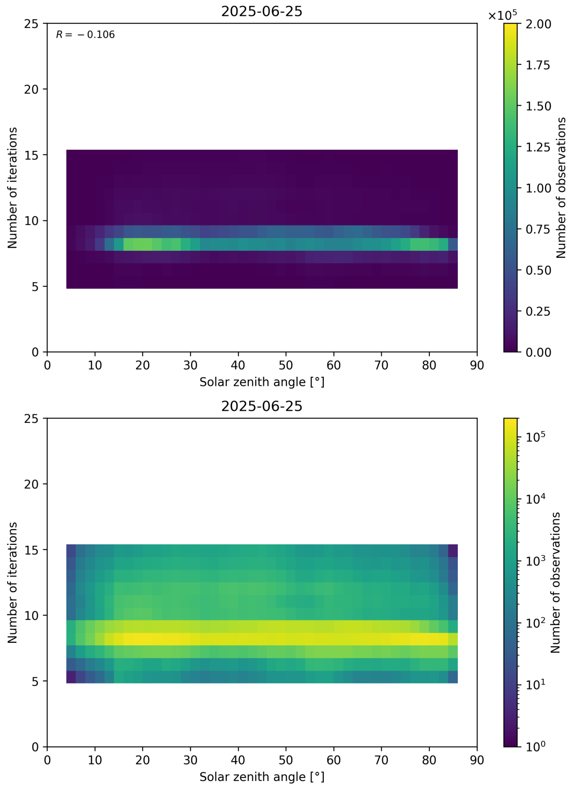
Figure 67: Scatter density plot of “Solar zenith angle” against “Number of iterations” for 2025-06-24 to 2025-06-26.
