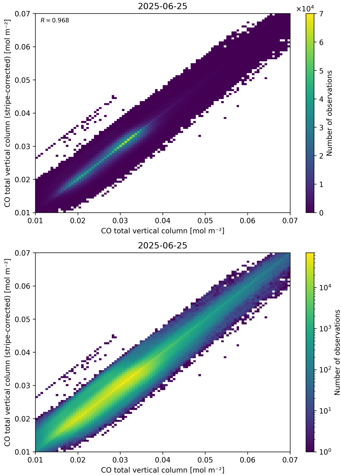
Figure 33: Scatter density plot of “CO total vertical column” against “CO total vertical column (stripe-corrected)” for 2025-06-24 to 2025-06-26.
