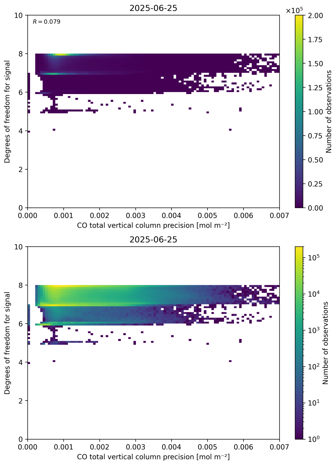
Figure 45: Scatter density plot of “CO total vertical column precision” against “Degrees of freedom for signal” for 2025-06-24 to 2025-06-26.
