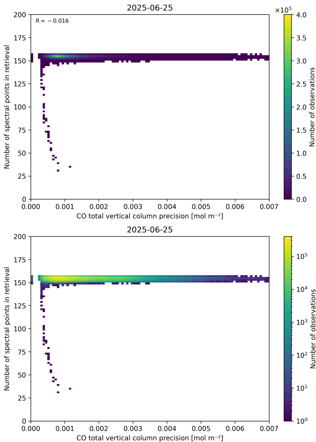
Figure 47: Scatter density plot of “CO total vertical column precision” against “Number of spectral points in retrieval” for 2025-06-24 to 2025-06-26.
