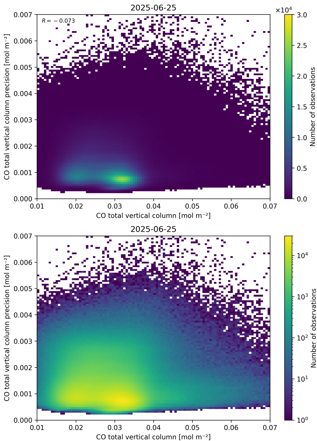
Figure 34: Scatter density plot of “CO total vertical column” against “CO total vertical column precision” for 2025-06-24 to 2025-06-26.
