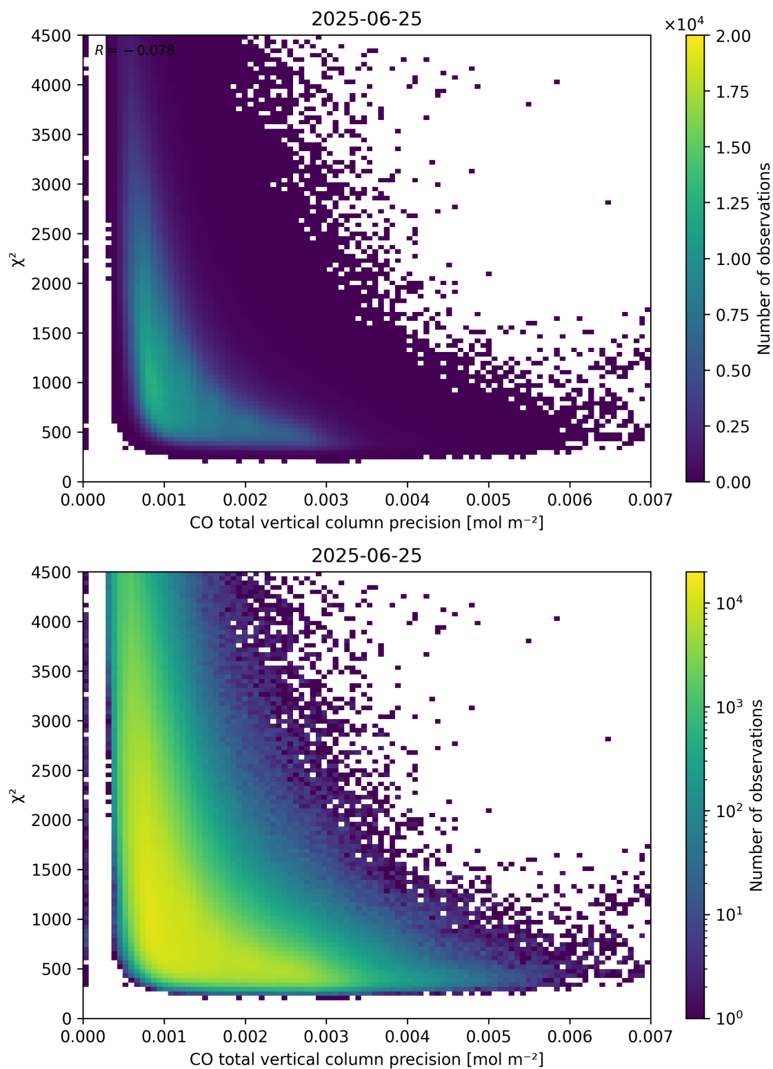
Figure 44: Scatter density plot of “CO total vertical column precision” against “ \chi^2 ” for 2025-06-24 to 2025-06-26.
