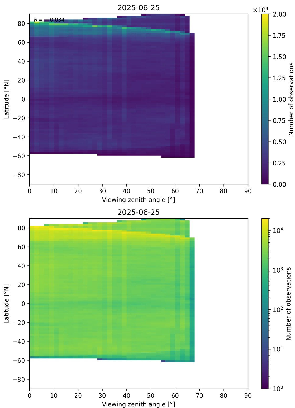
Figure 74: Scatter density plot of “Viewing zenith angle” against “Latitude” for 2025-06-24 to 2025-06-26.
