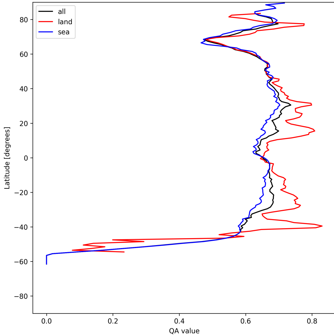
Figure 9: Zonal average of “QA value” for 2025-06-24 to 2025-06-26.
