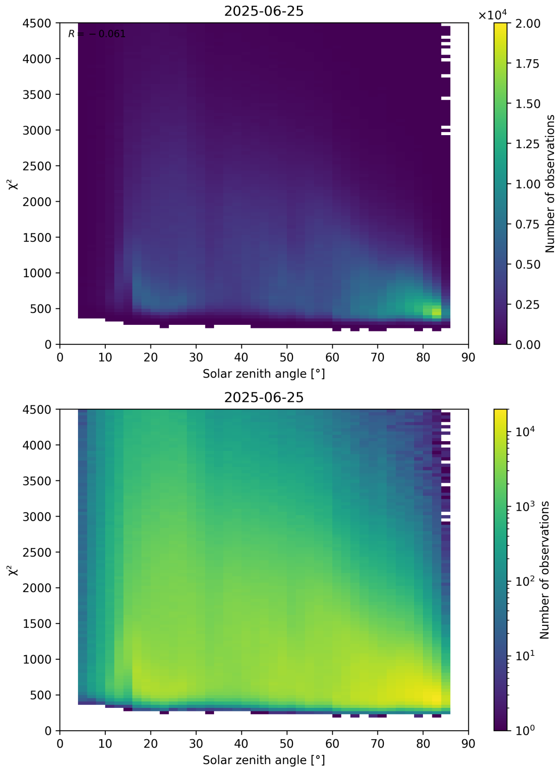
Figure 64: Scatter density plot of “Solar zenith angle” against “ \chi^2 ” for 2025-06-24 to 2025-06-26.
