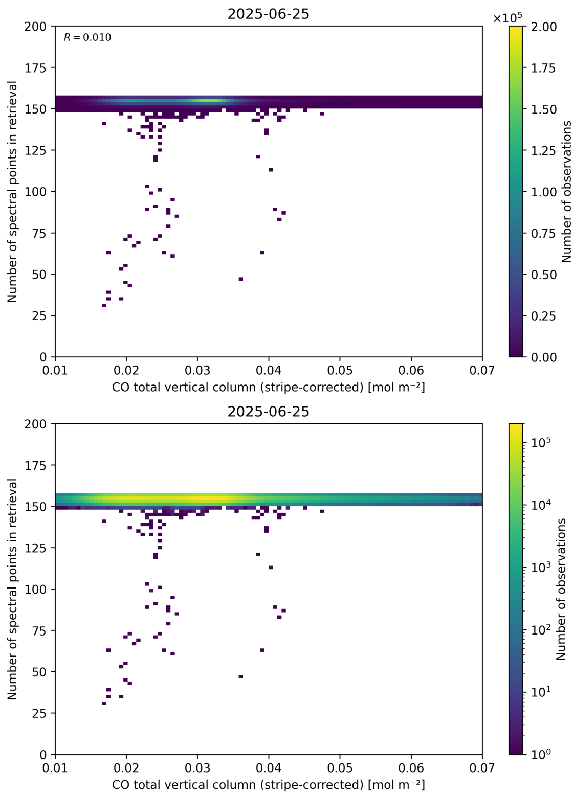
Figure 40: Scatter density plot of “CO total vertical column (stripe-corrected)” against “Number of spectral points in retrieval” for 2025-06-24 to 2025-06-26.
