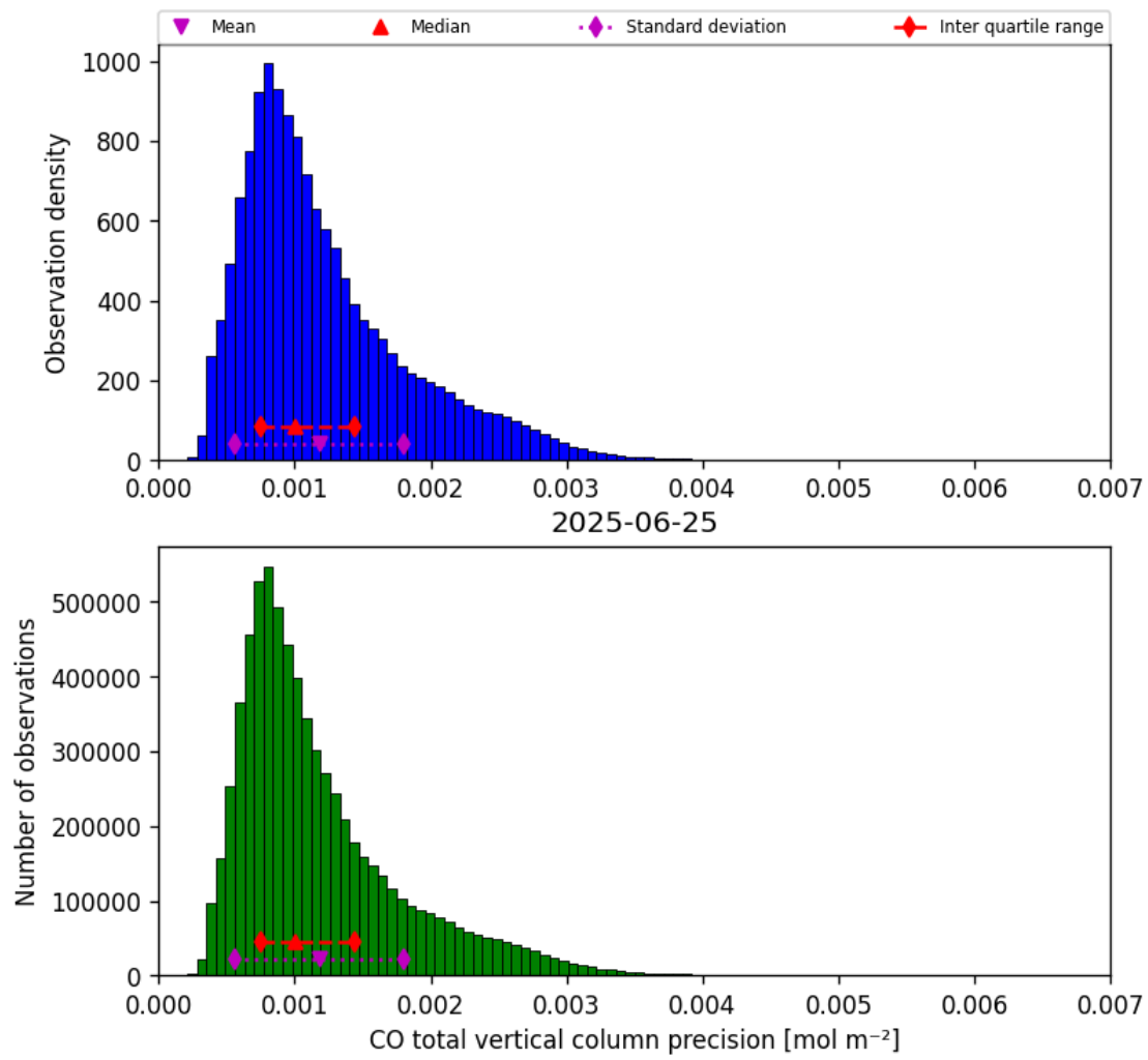
Figure 20: Histogram of “CO total vertical column precision” for 2025-06-24 to 2025-06-26
