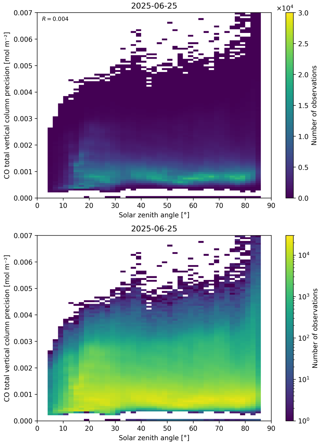
Figure 63: Scatter density plot of “Solar zenith angle” against “CO total vertical column precision” for 2025-06-24 to 2025-06-26.
