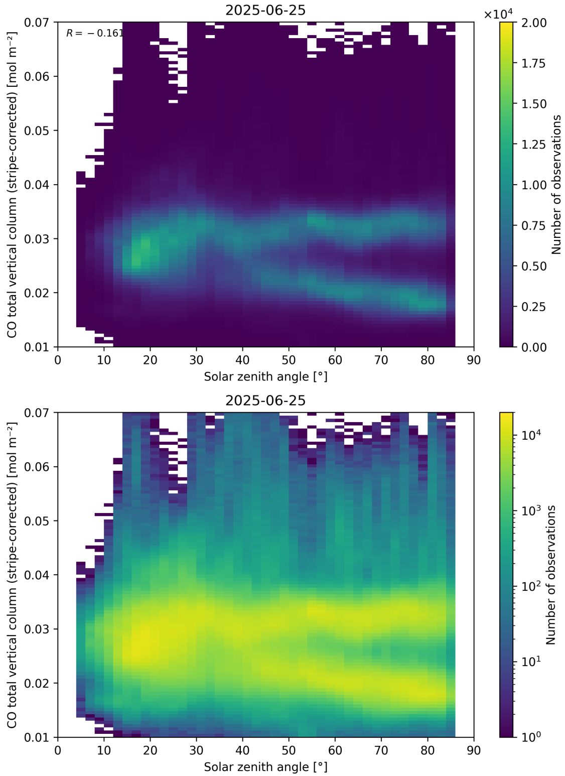
Figure 62: Scatter density plot of “Solar zenith angle” against “CO total vertical column (stripe-corrected)” for 2025-06-24 to 2025-06-26.
