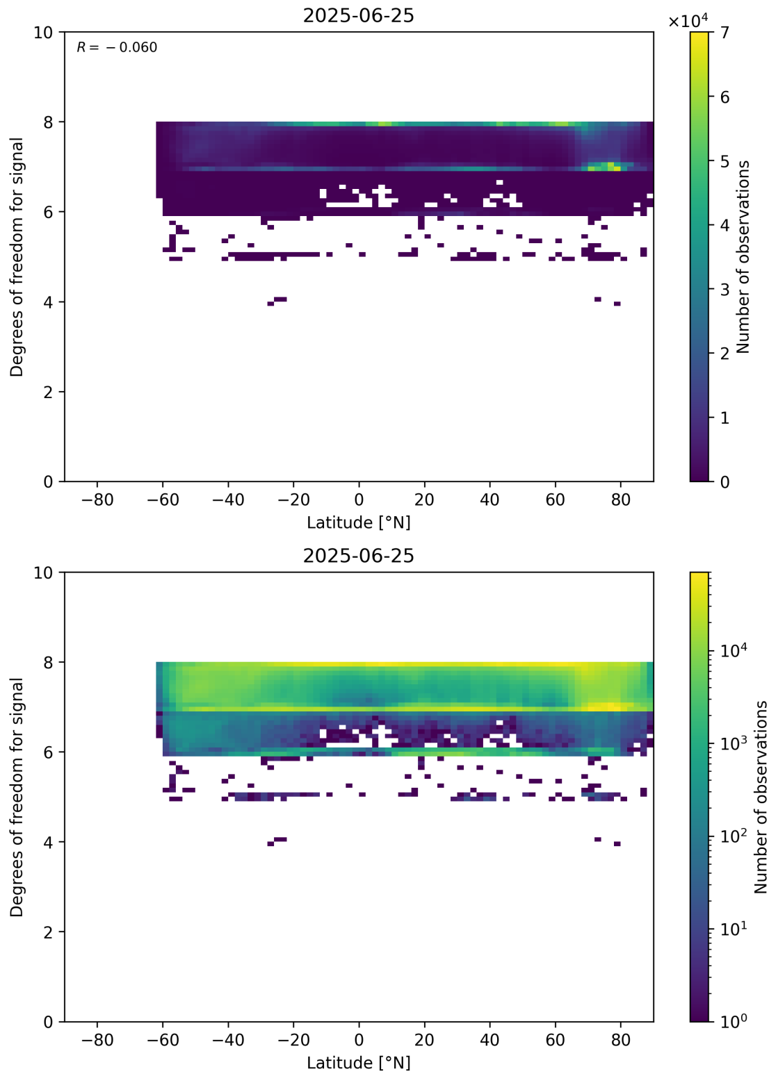
Figure 55: Scatter density plot of “Latitude” against “Degrees of freedom for signal” for 2025-06-24 to 2025-06-26.
