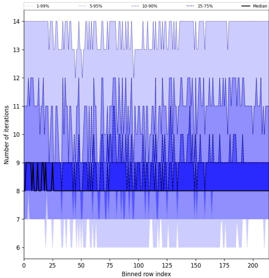
Figure 32: Along track statistics of “Number of iterations” for 2025-06-24 to 2025-06-26
