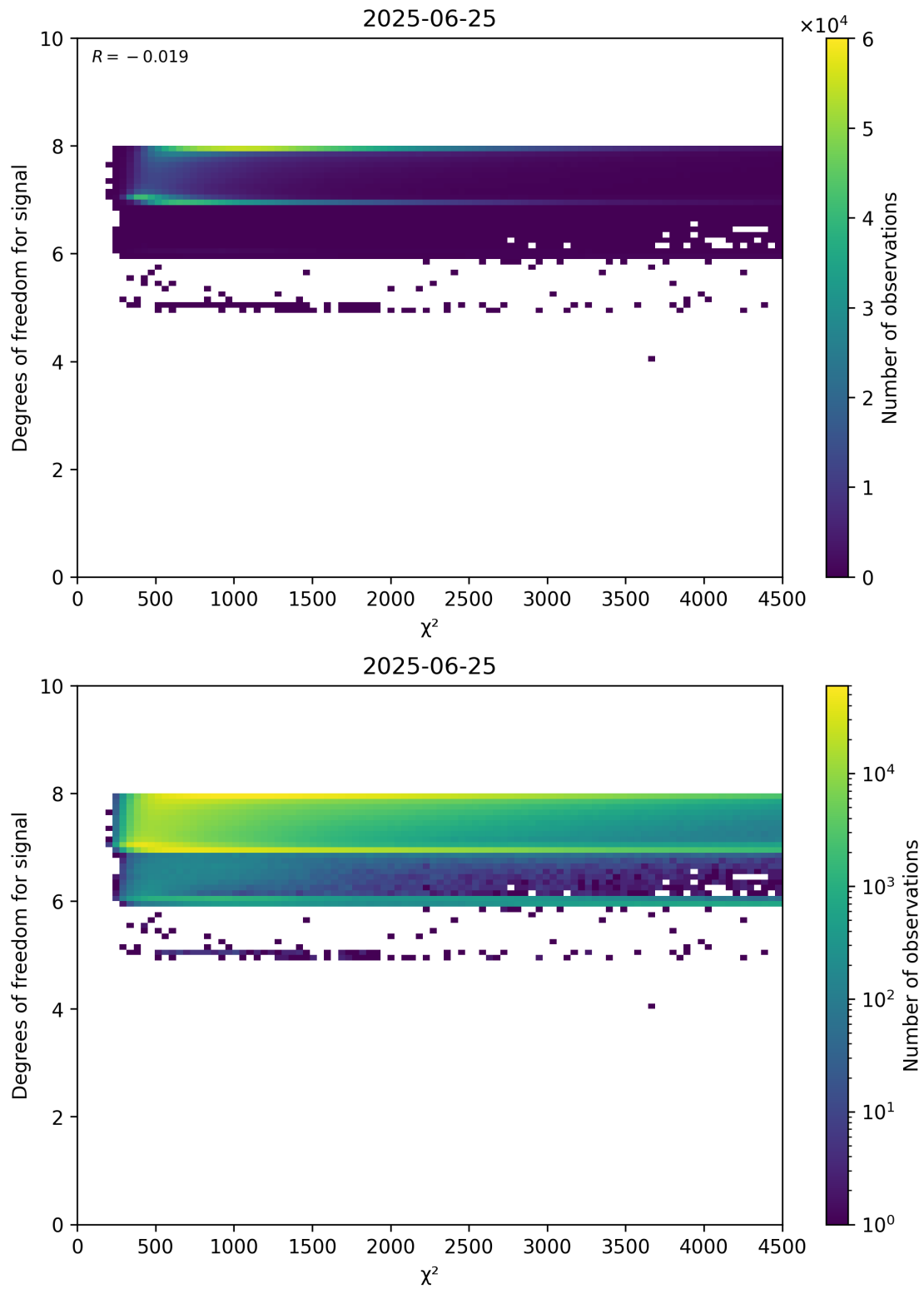
Figure 48: Scatter density plot of “ \chi^2 ” against “Degrees of freedom for signal” for 2025-06-24 to 2025-06-26.
