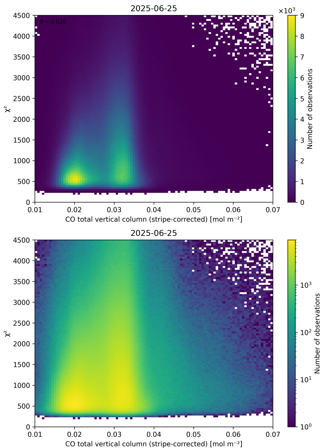
Figure 37: Scatter density plot of “CO total vertical column (stripe-corrected)” against “ \chi^2 ” for 2025-06-24 to 2025-06-26.
