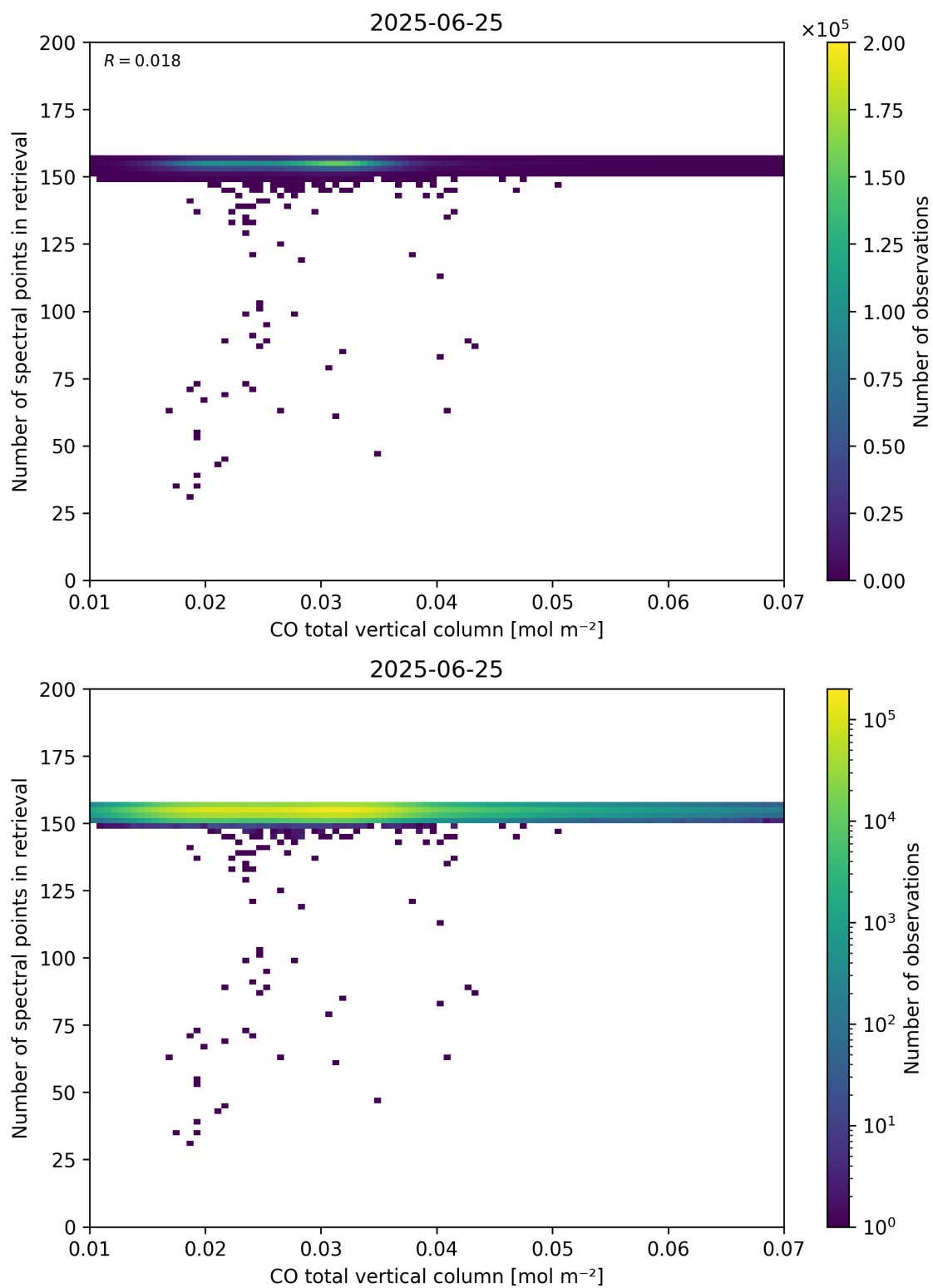
Figure 43: Scatter density plot of “CO total vertical column” against “Number of spectral points in retrieval” for 2025-06-24 to 2025-06-26.
