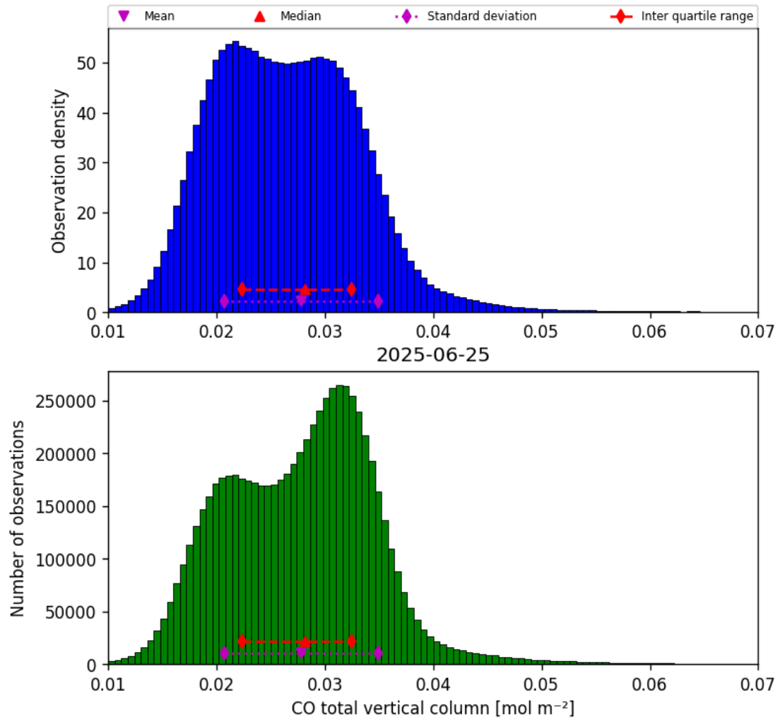
Figure 18: Histogram of “CO total vertical column” for 2025-06-24 to 2025-06-26
