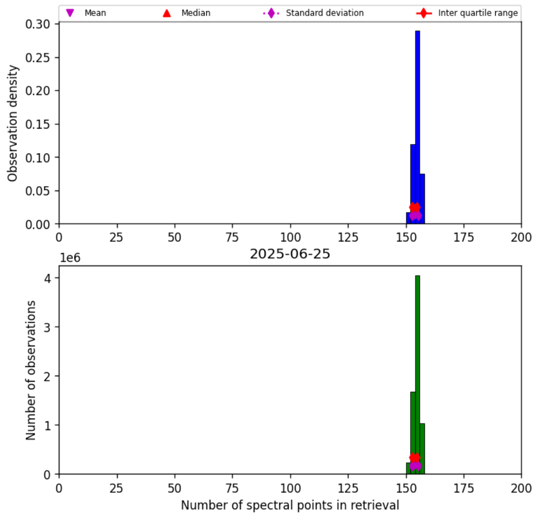
Figure 21: Histogram of “Number of spectral points in retrieval” for 2025-06-24 to 2025-06-26
