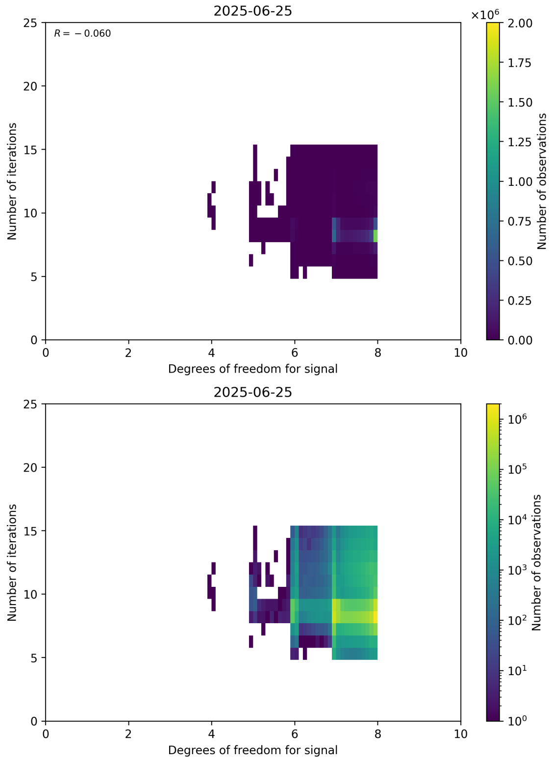
Figure 50: Scatter density plot of “Degrees of freedom for signal” against “Number of iterations” for 2025-06-24 to 2025-06-26.
