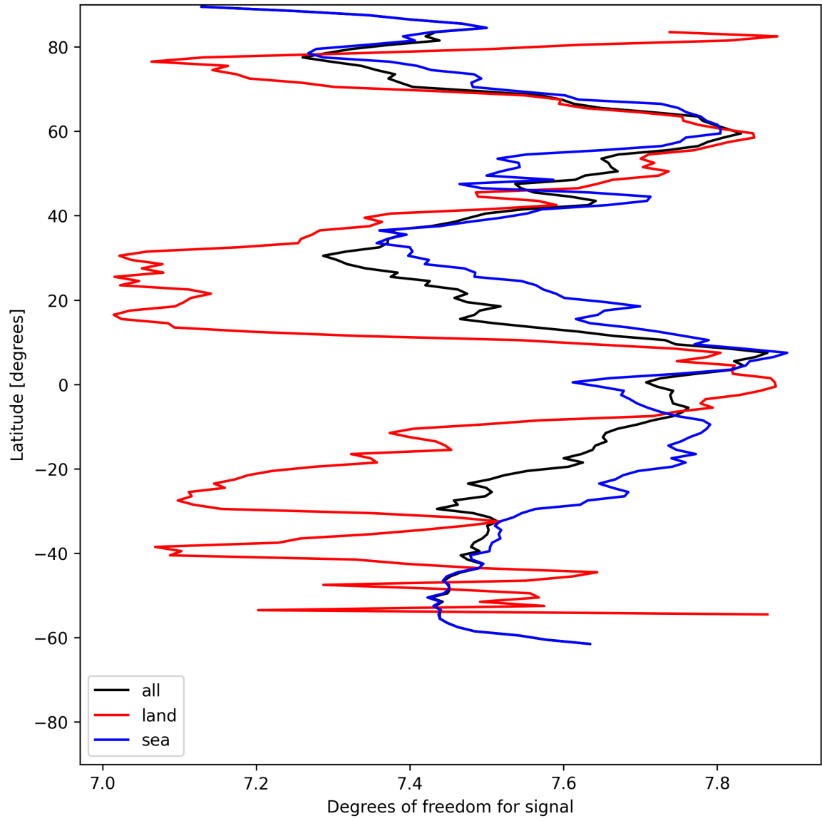
Figure 15: Zonal average of “Degrees of freedom for signal” for 2025-06-24 to 2025-06-26.
