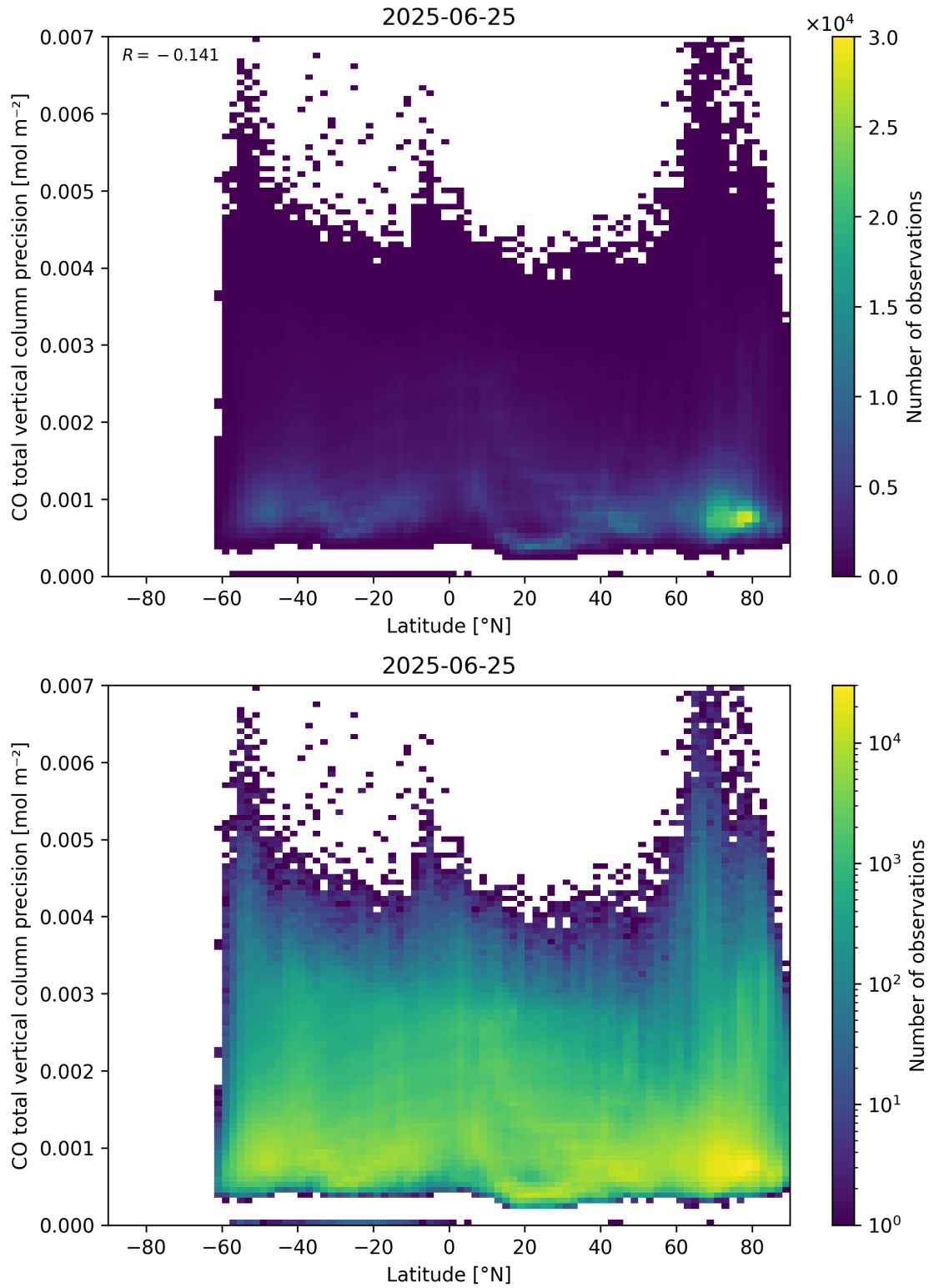
Figure 53: Scatter density plot of “Latitude” against “CO total vertical column precision” for 2025-06-24 to 2025-06-26.
