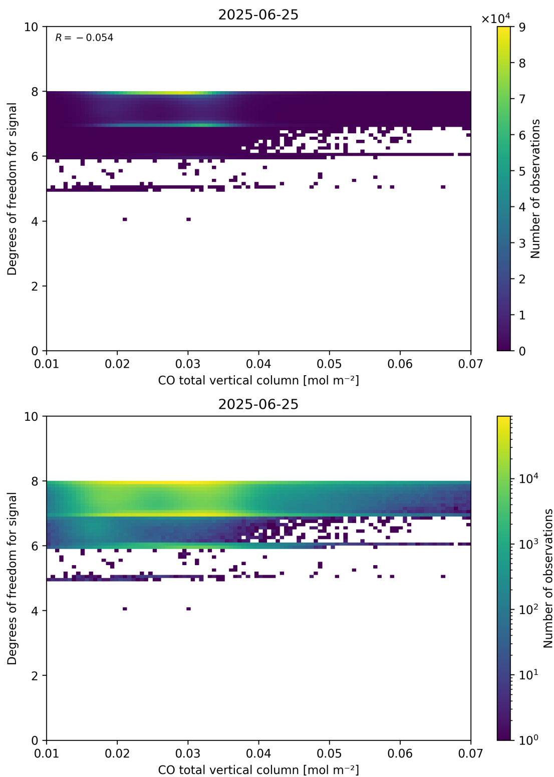
Figure 41: Scatter density plot of “CO total vertical column” against “Degrees of freedom for signal” for 2025-06-24 to 2025-06-26.
