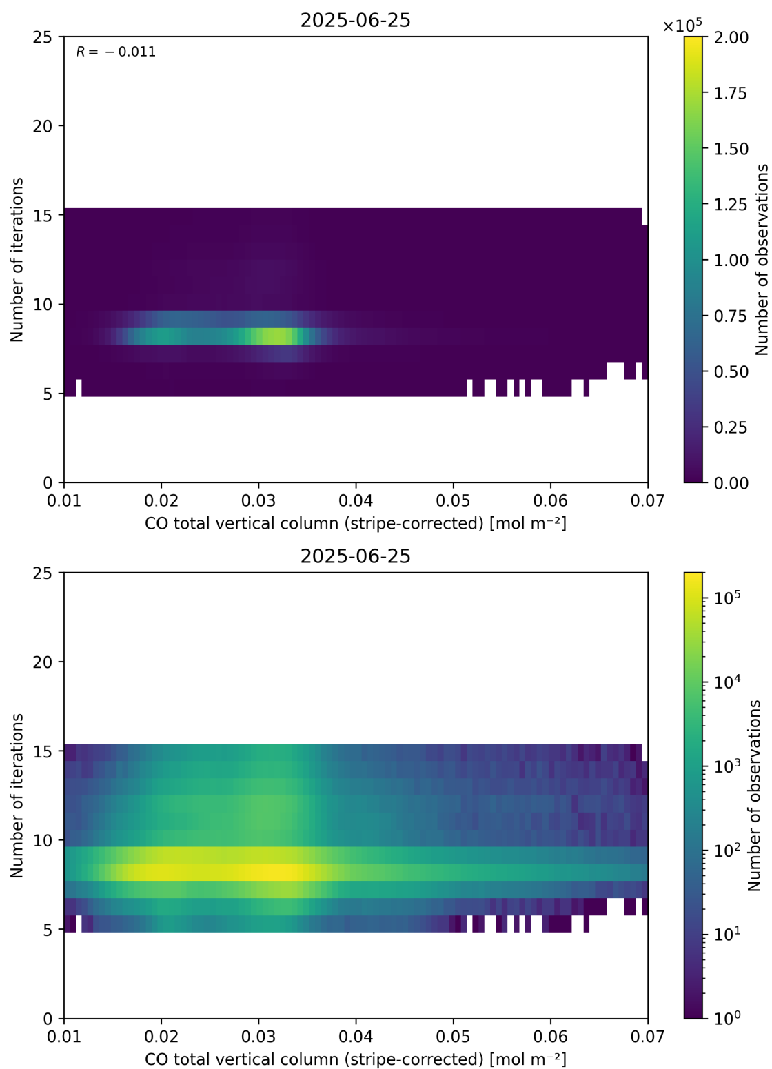
Figure 39: Scatter density plot of “CO total vertical column (stripe-corrected)” against “Number of iterations” for 2025-06-24 to 2025-06-26.
