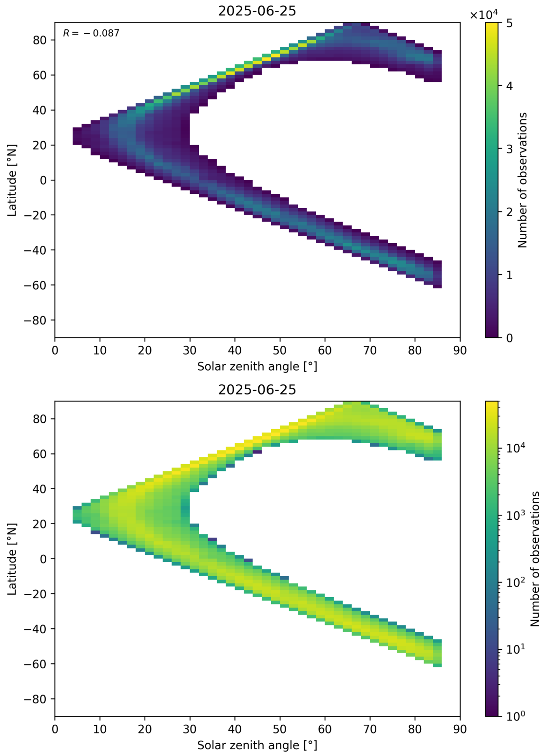
Figure 66: Scatter density plot of “Solar zenith angle” against “Latitude” for 2025-06-24 to 2025-06-26.
