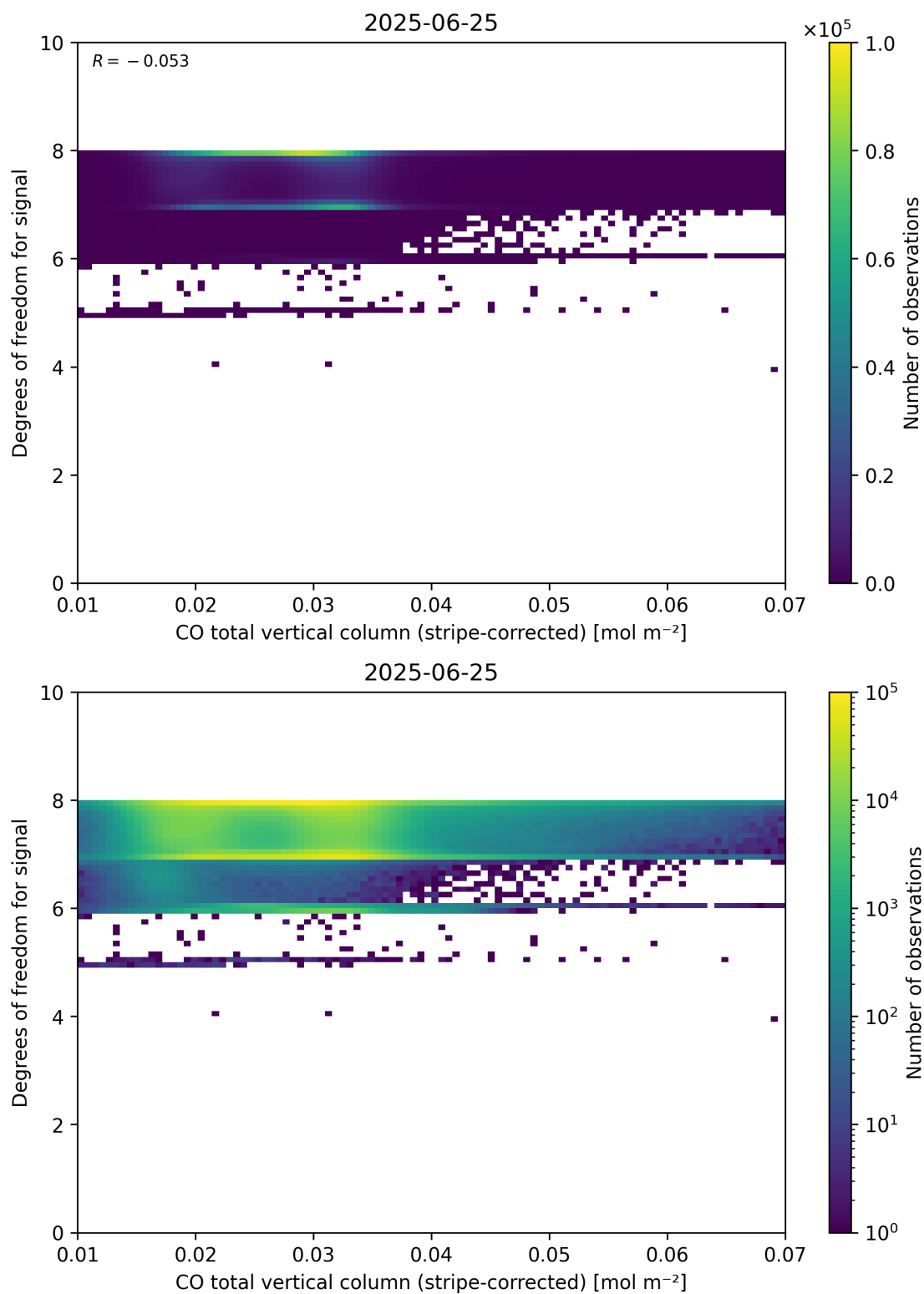
Figure 38: Scatter density plot of “CO total vertical column (stripe-corrected)” against “Degrees of freedom for signal” for 2025-06-24 to 2025-06-26.
