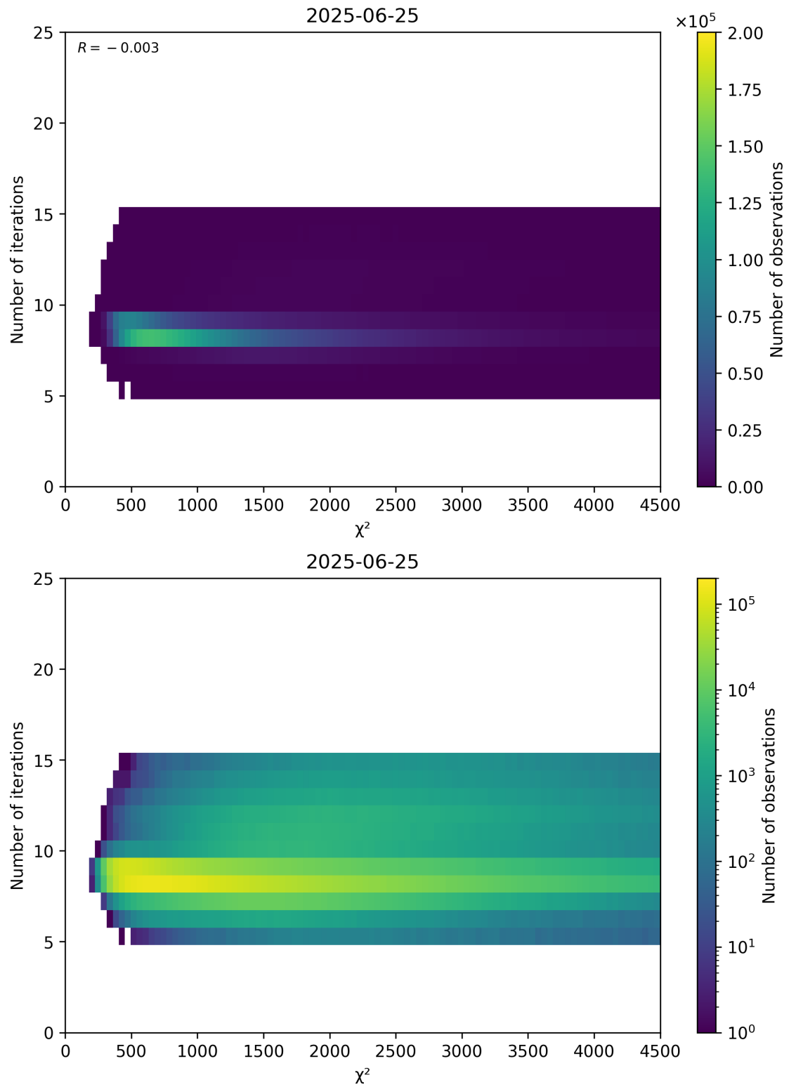
Figure 49: Scatter density plot of “ \chi^2 ” against “Number of iterations” for 2025-06-24 to 2025-06-26.
