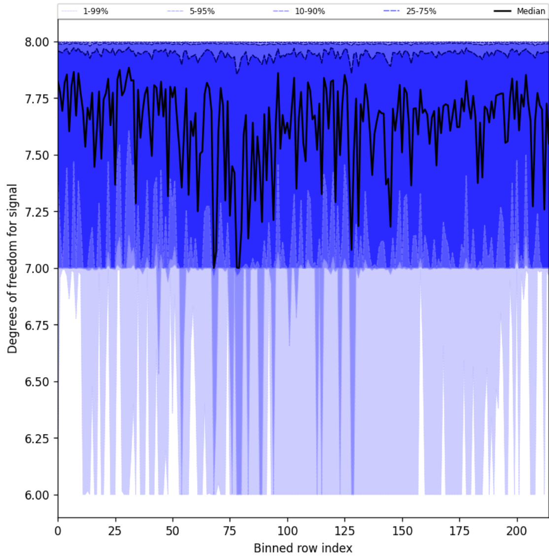
Figure 31: Along track statistics of “Degrees of freedom for signal” for 2025-06-24 to 2025-06-26
