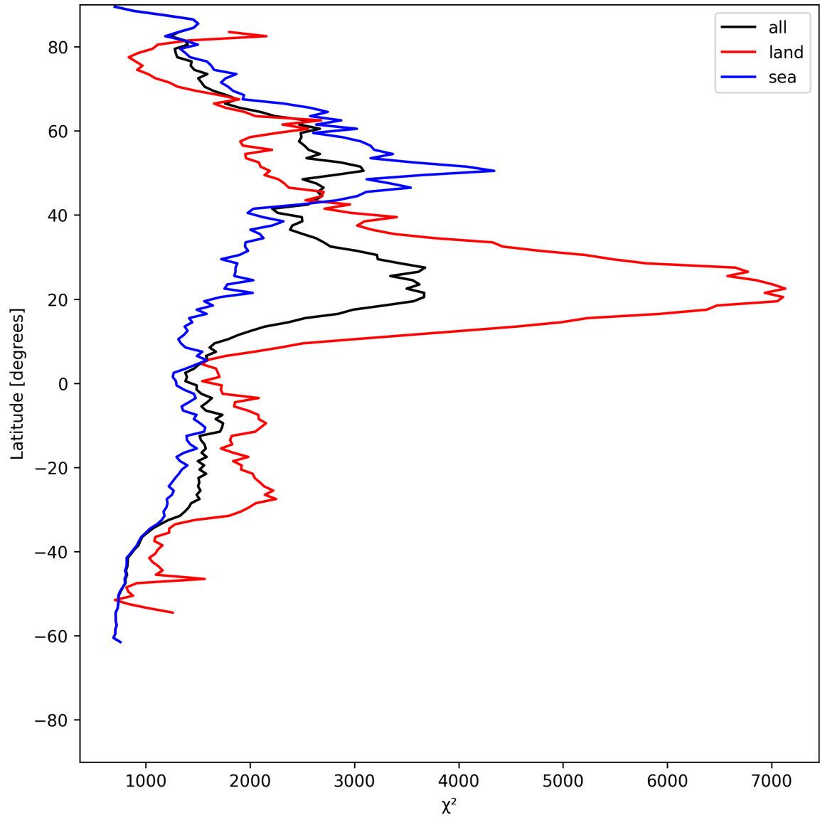
Figure 14: Zonal average of “ \chi^2 ” for 2025-06-24 to 2025-06-26.
