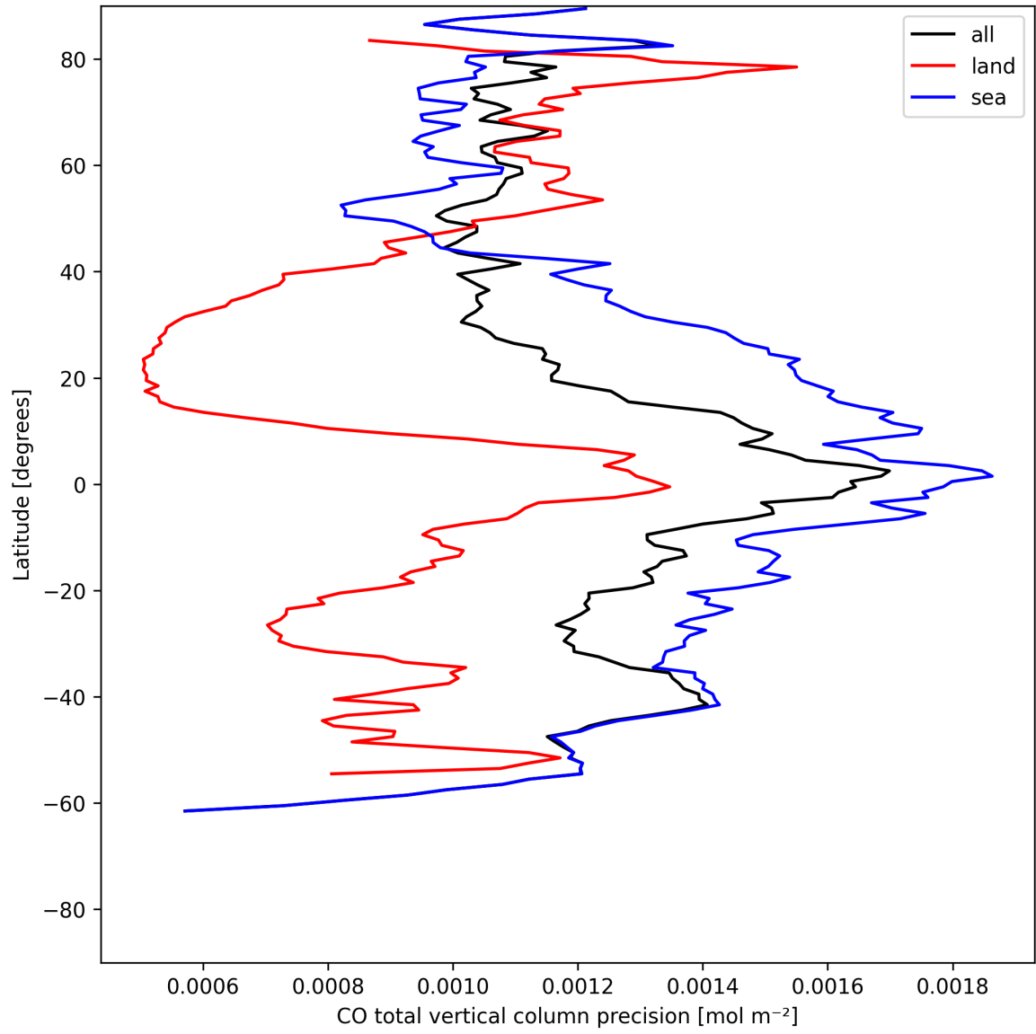
Figure 12: Zonal average of “CO total vertical column precision” for 2025-06-24 to 2025-06-26.
