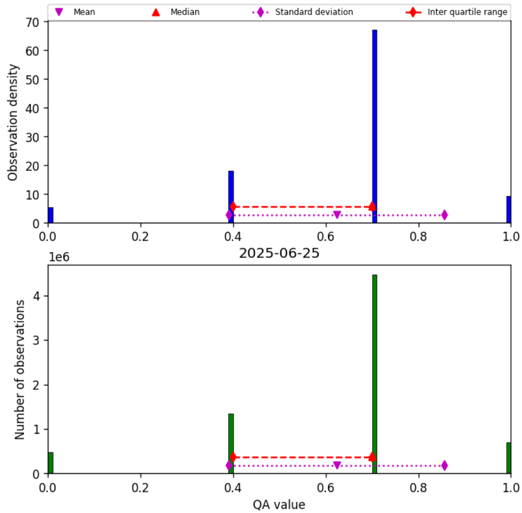
Figure 17: Histogram of “QA value” for 2025-06-24 to 2025-06-26
