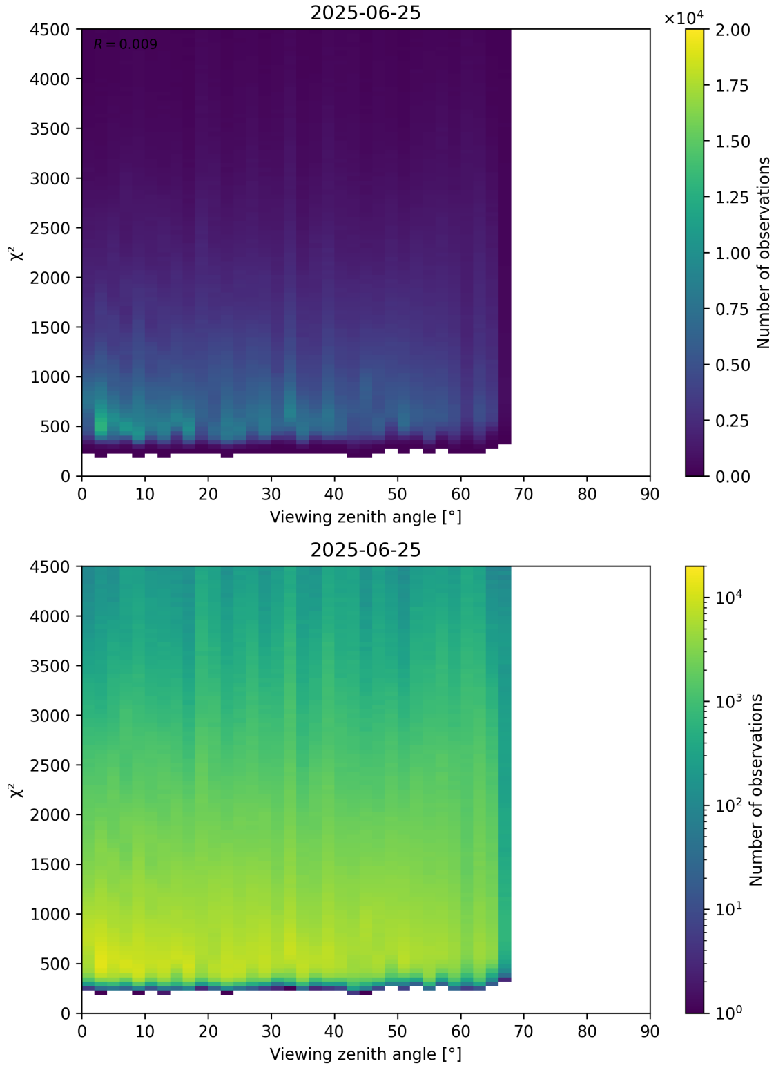
Figure 72: Scatter density plot of “Viewing zenith angle” against “ \chi^2 ” for 2025-06-24 to 2025-06-26.
