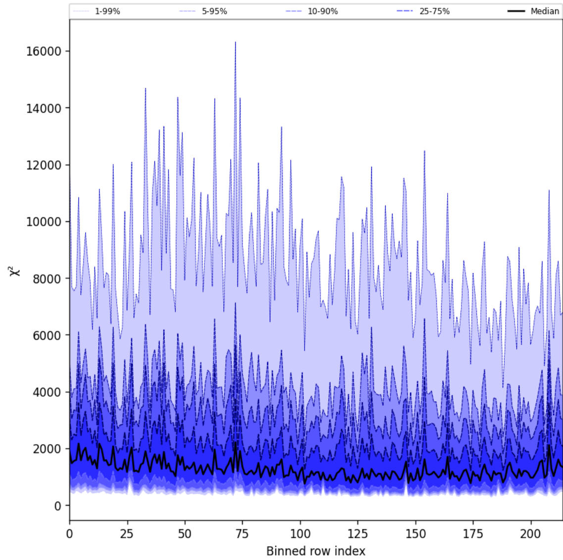
Figure 30: Along track statistics of “ \chi^2 ” for 2025-06-24 to 2025-06-26
