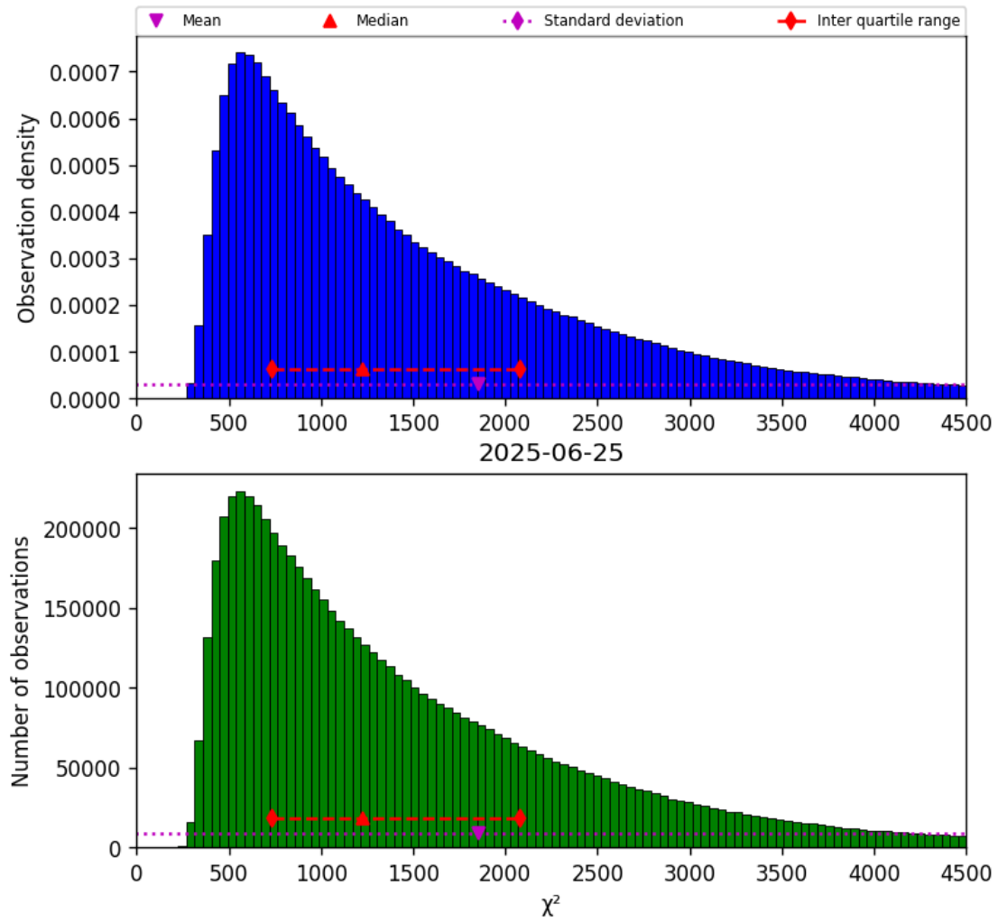
Figure 22: Histogram of “ \chi^2 ” for 2025-06-24 to 2025-06-26
