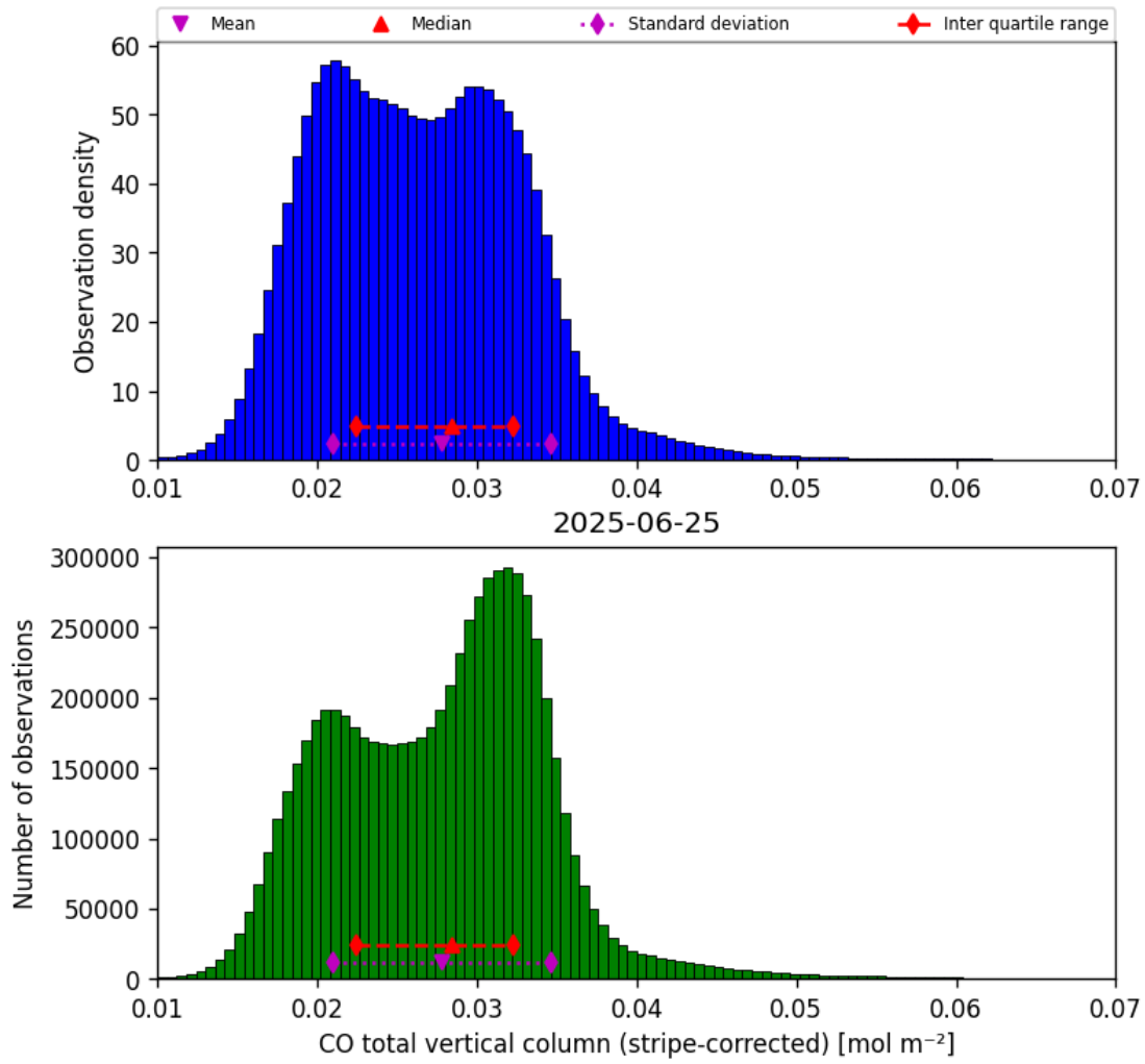
Figure 19: Histogram of “CO total vertical column (stripe-corrected)” for 2025-06-24 to 2025-06-26
