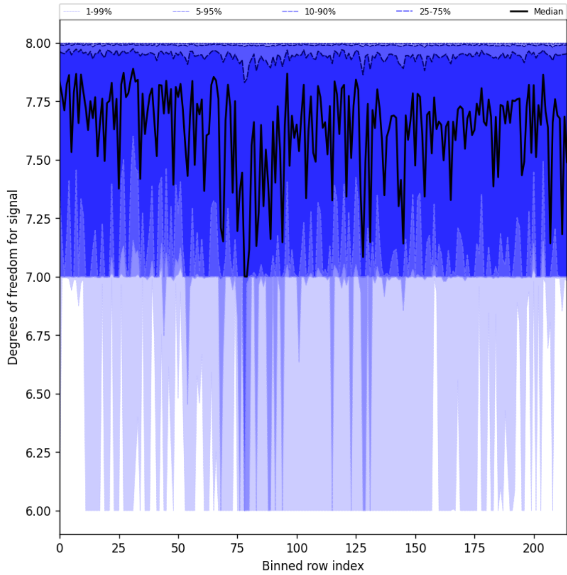
Figure 31: Along track statistics of “Degrees of freedom for signal” for 2025-06-25 to 2025-06-27
