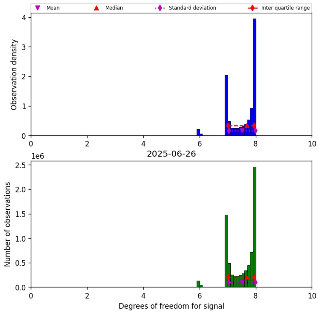
Figure 23: Histogram of “Degrees of freedom for signal” for 2025-06-25 to 2025-06-27
