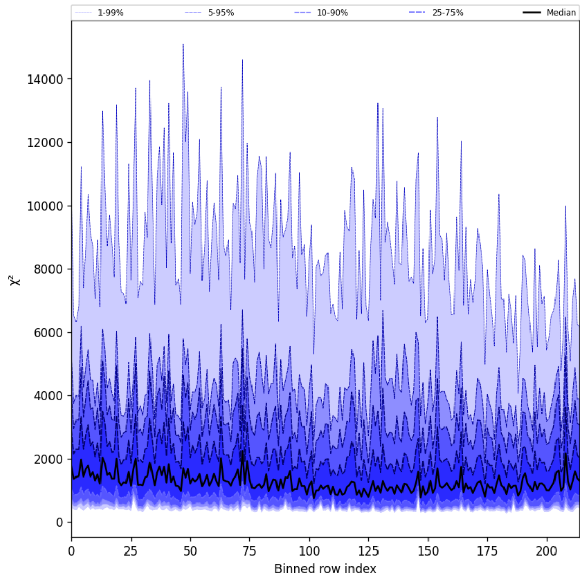
Figure 30: Along track statistics of “ \chi^2 ” for 2025-06-25 to 2025-06-27
