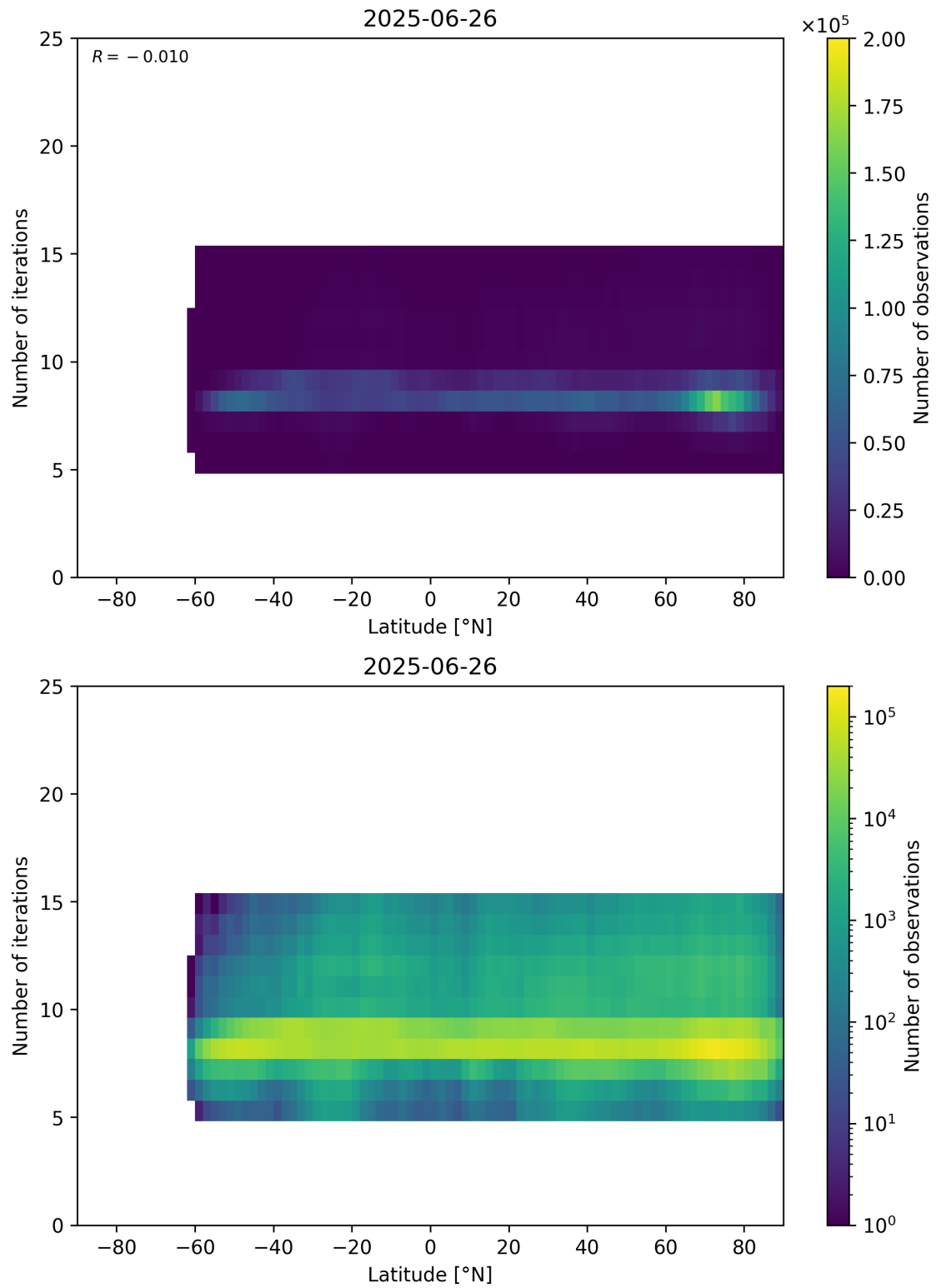
Figure 56: Scatter density plot of “Latitude” against “Number of iterations” for 2025-06-25 to 2025-06-27.
