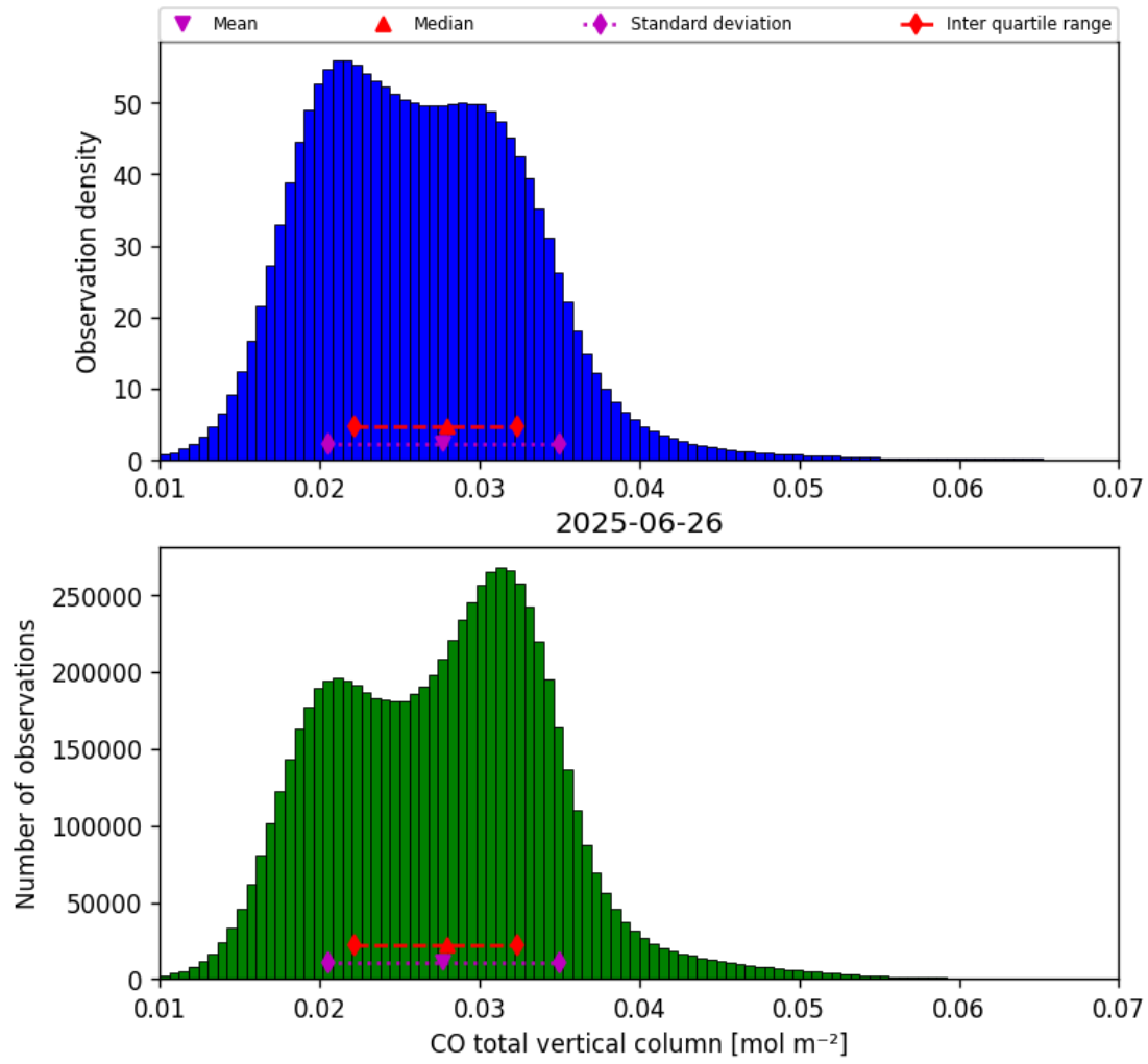
Figure 18: Histogram of “CO total vertical column” for 2025-06-25 to 2025-06-27
