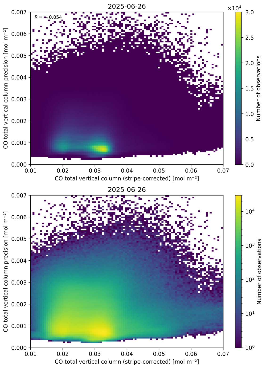
Figure 36: Scatter density plot of “CO total vertical column (stripe-corrected)” against “CO total vertical column precision” for 2025-06-25 to 2025-06-27.
