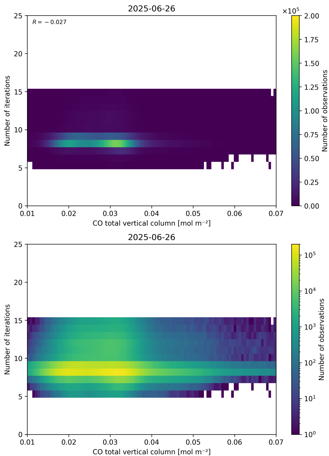
Figure 42: Scatter density plot of “CO total vertical column” against “Number of iterations” for 2025-06-25 to 2025-06-27.
