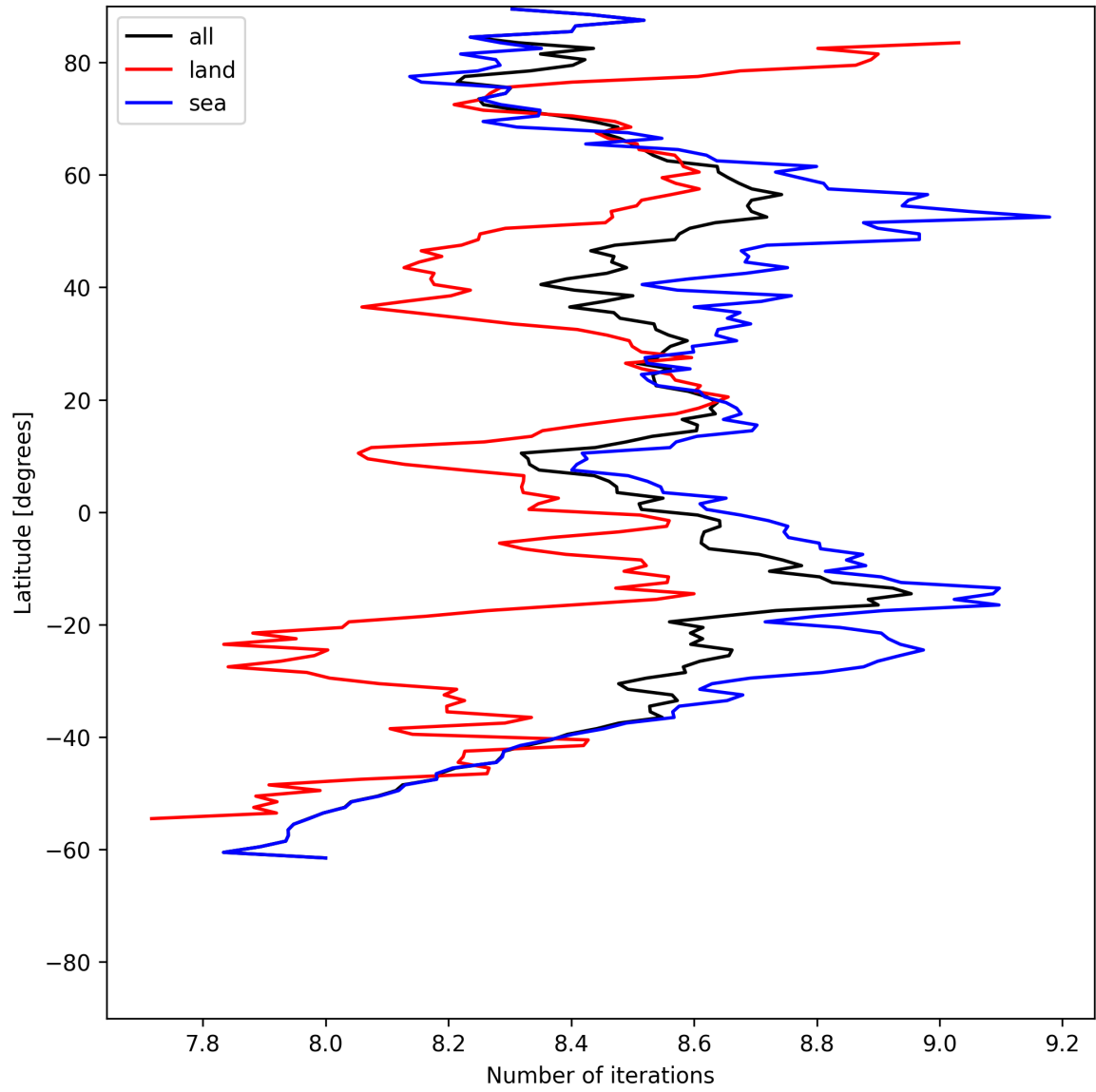
Figure 16: Zonal average of “Number of iterations” for 2025-06-25 to 2025-06-27.
