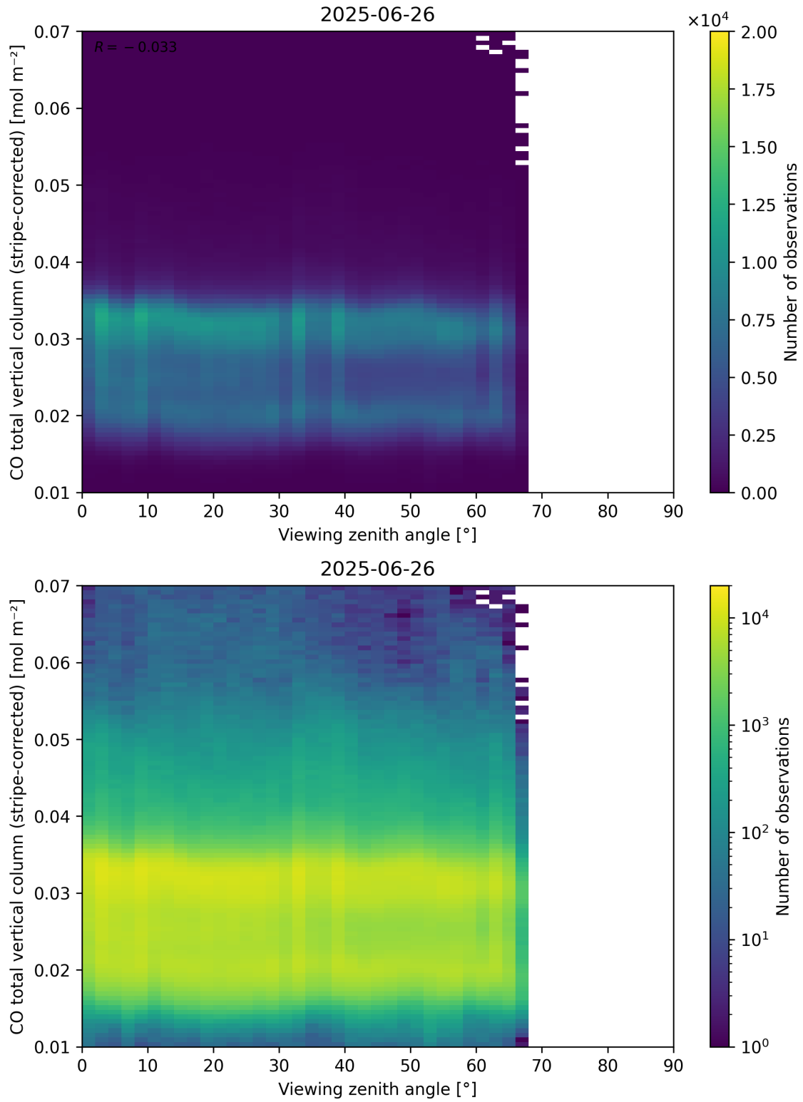
Figure 70: Scatter density plot of “Viewing zenith angle” against “CO total vertical column (stripe-corrected)” for 2025-06-25 to 2025-06-27.
