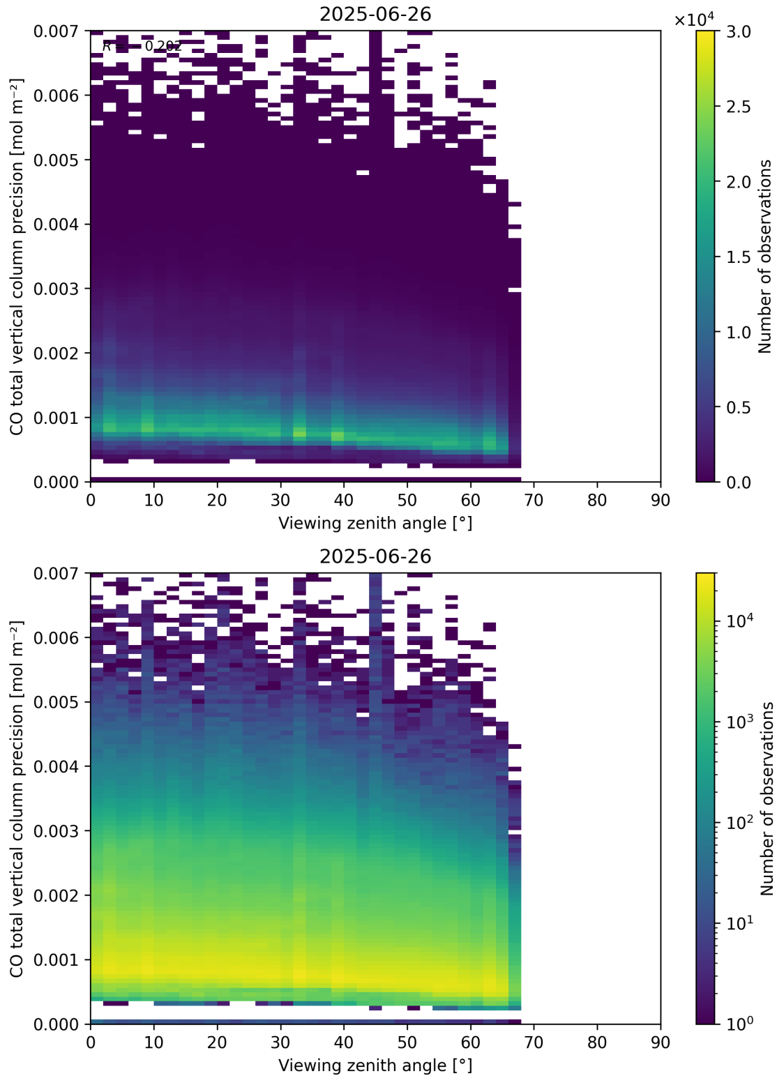
Figure 71: Scatter density plot of “Viewing zenith angle” against “CO total vertical column precision” for 2025-06-25 to 2025-06-27.
