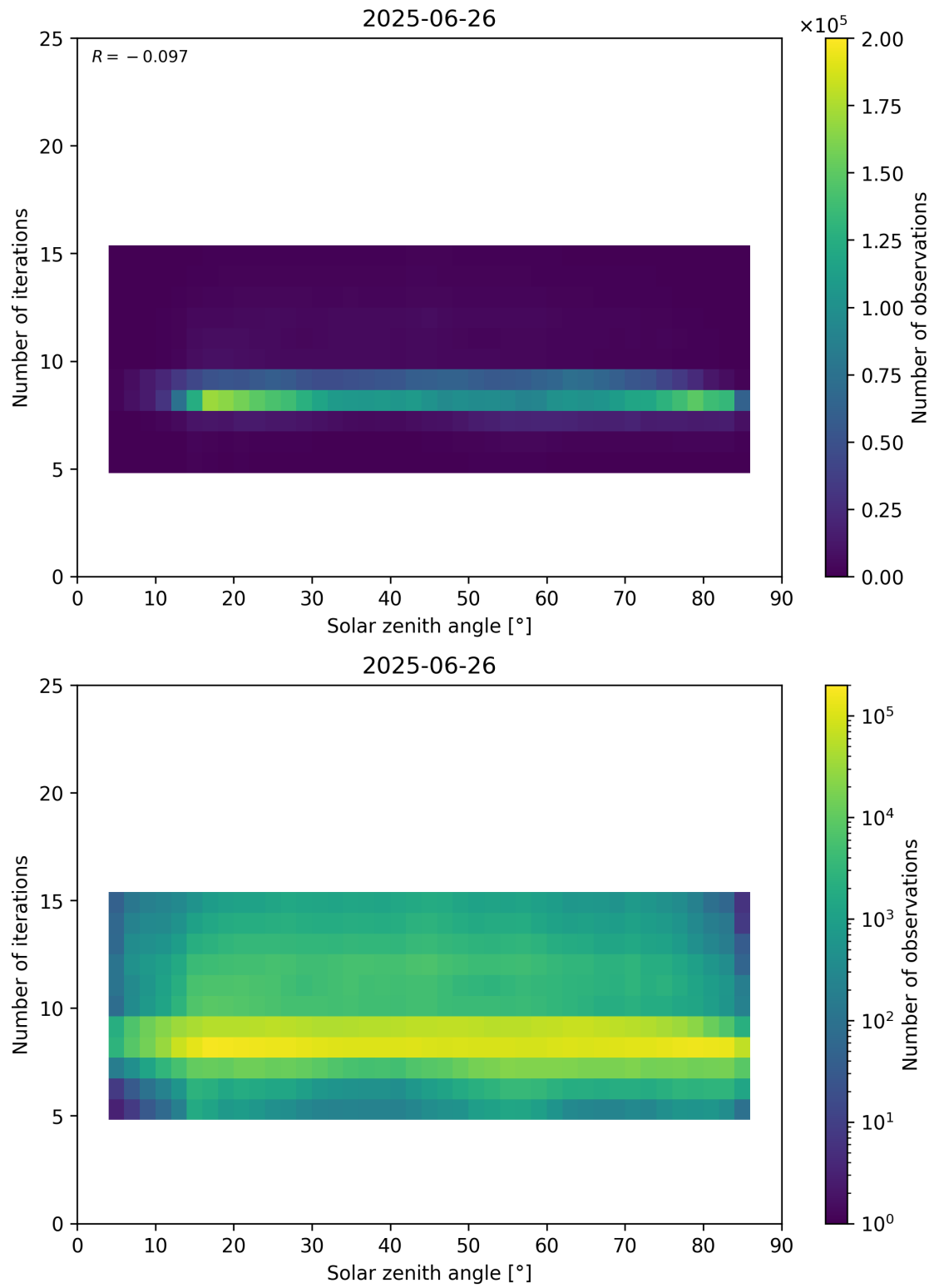
Figure 67: Scatter density plot of “Solar zenith angle” against “Number of iterations” for 2025-06-25 to 2025-06-27.
