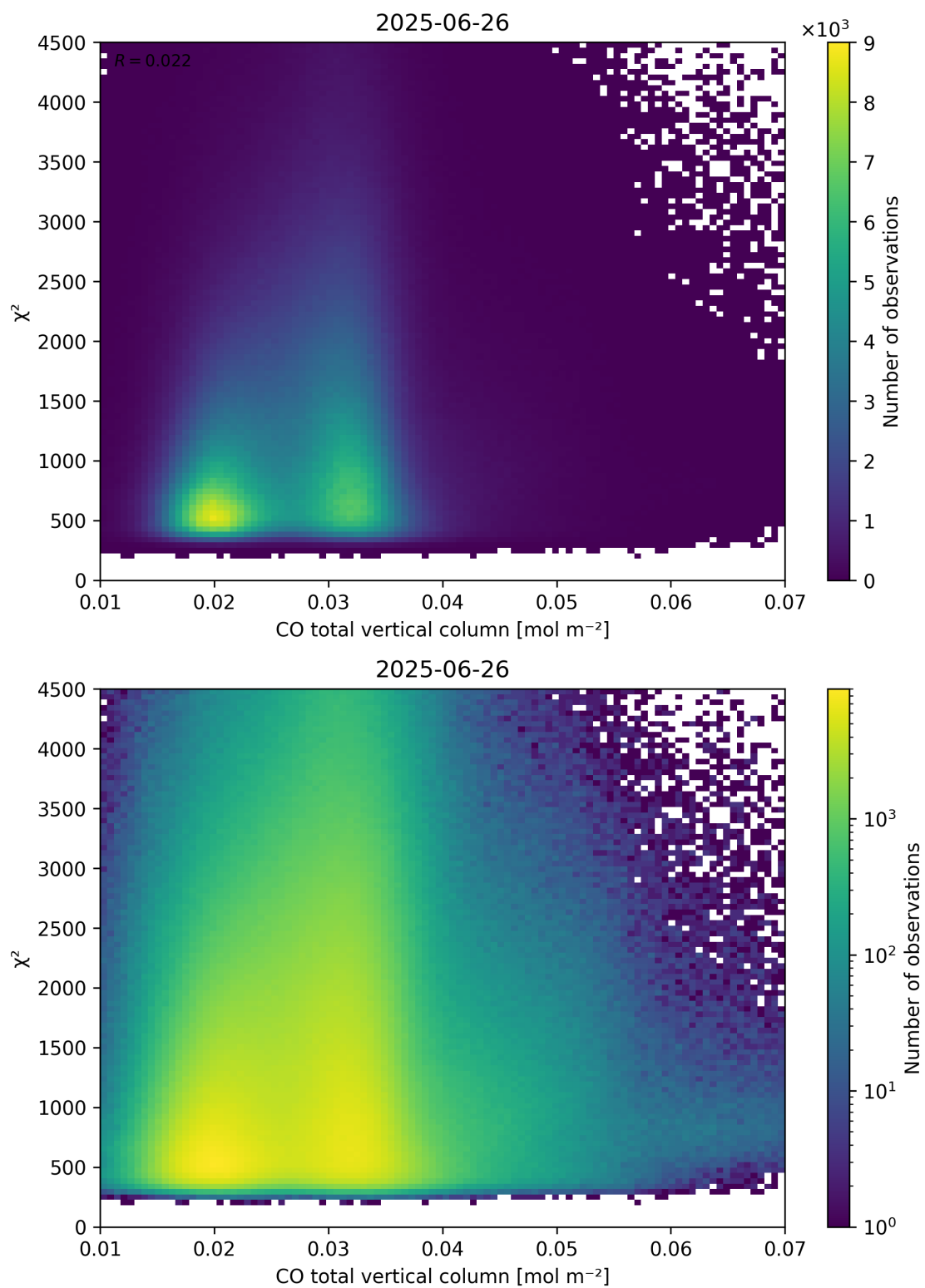
Figure 35: Scatter density plot of “CO total vertical column” against “ \chi^2 ” for 2025-06-25 to 2025-06-27.
