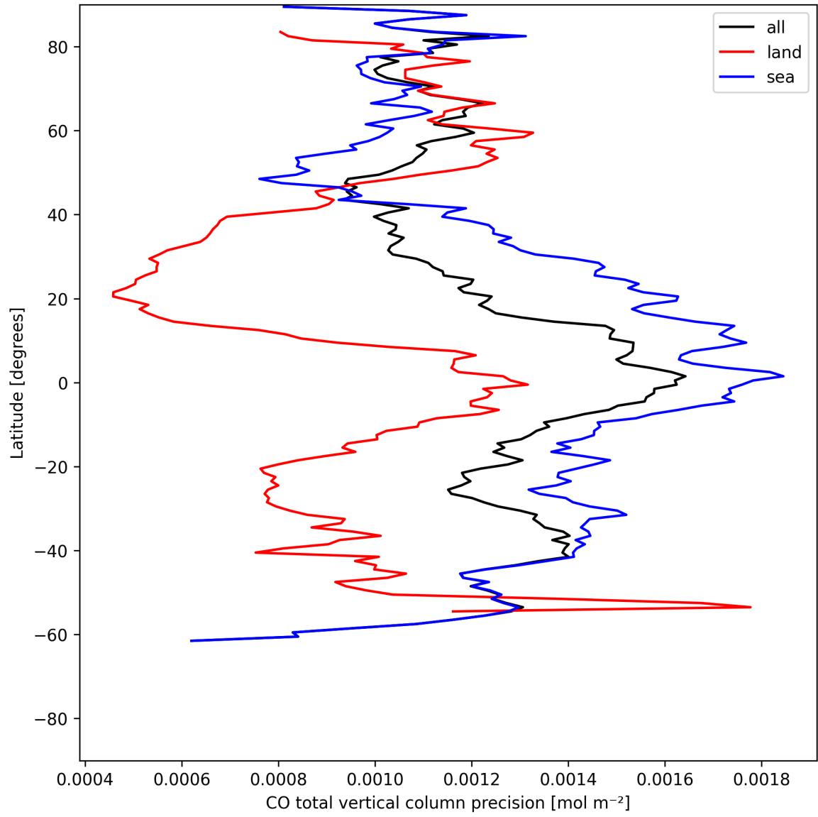
Figure 12: Zonal average of “CO total vertical column precision” for 2025-06-25 to 2025-06-27.
