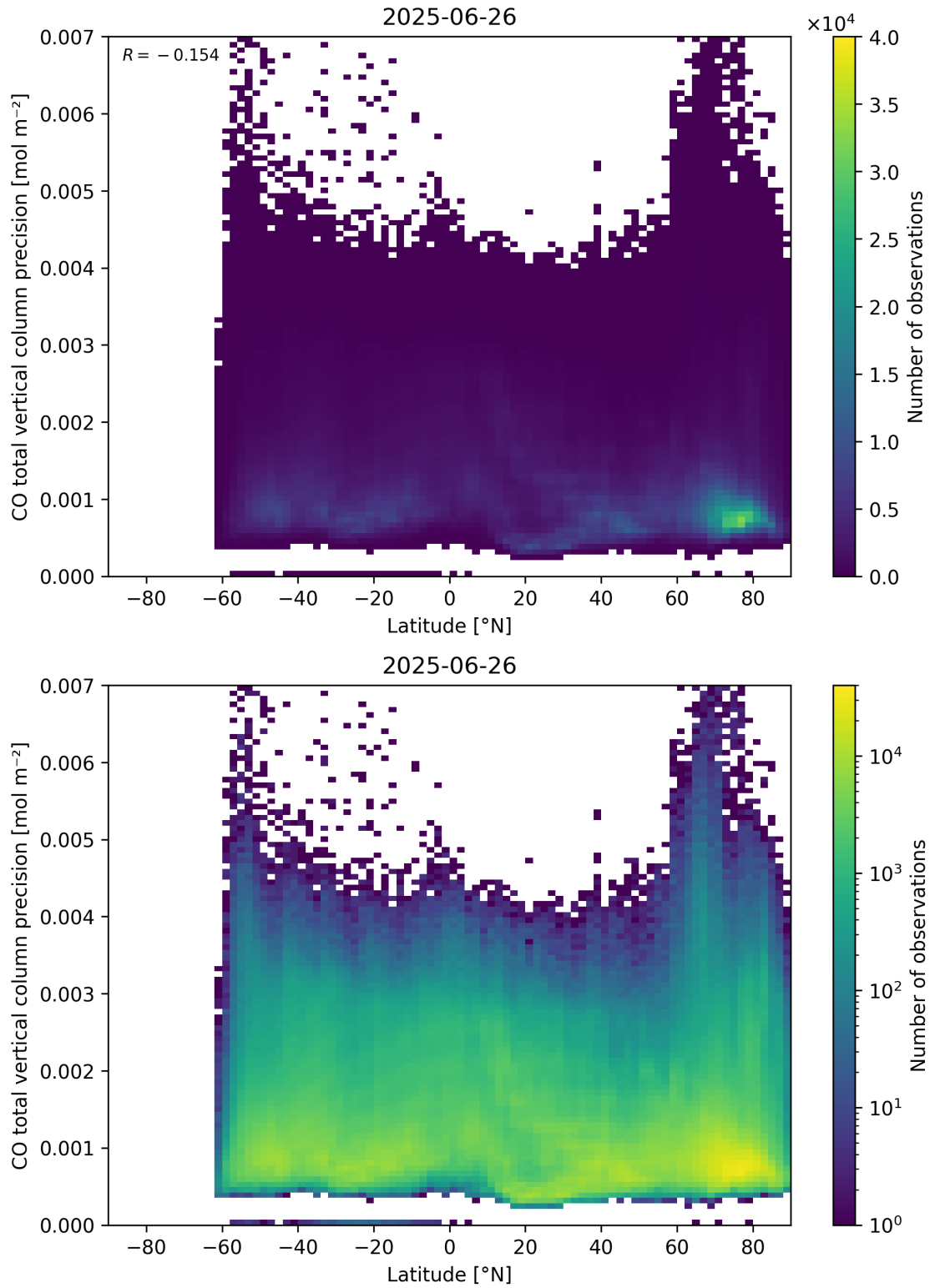
Figure 53: Scatter density plot of “Latitude” against “CO total vertical column precision” for 2025-06-25 to 2025-06-27.
