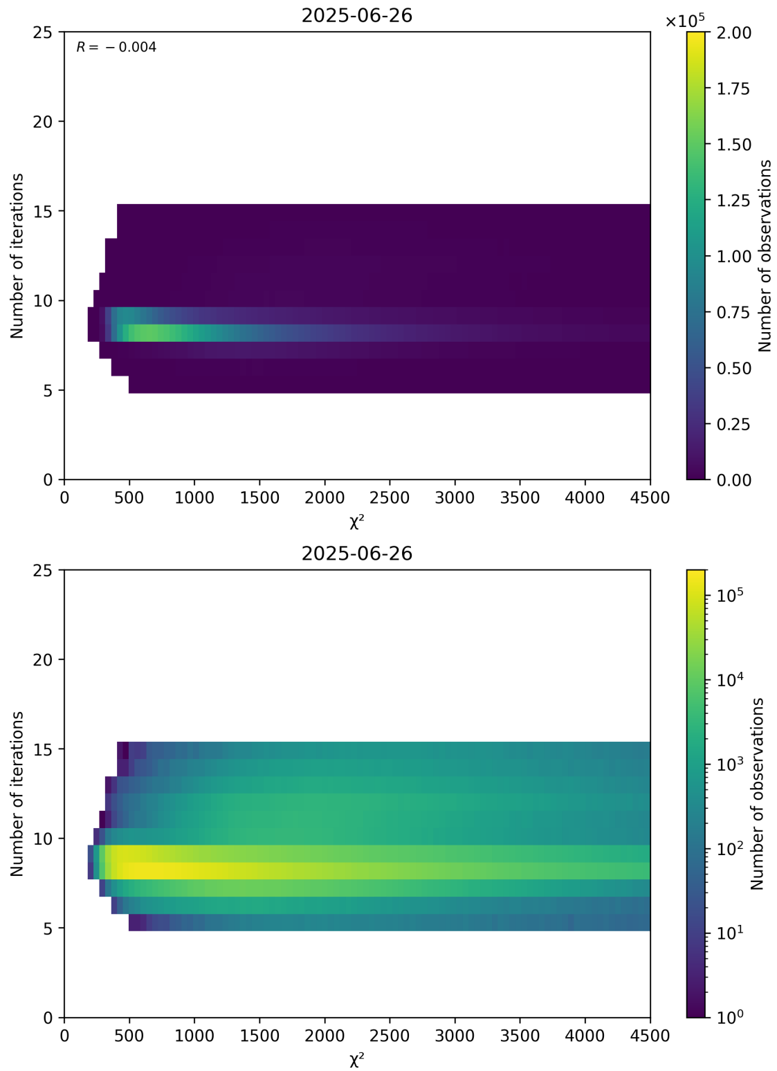
Figure 49: Scatter density plot of " \chi^2 " against "Number of iterations" for 2025-06-25 to 2025-06-27.
