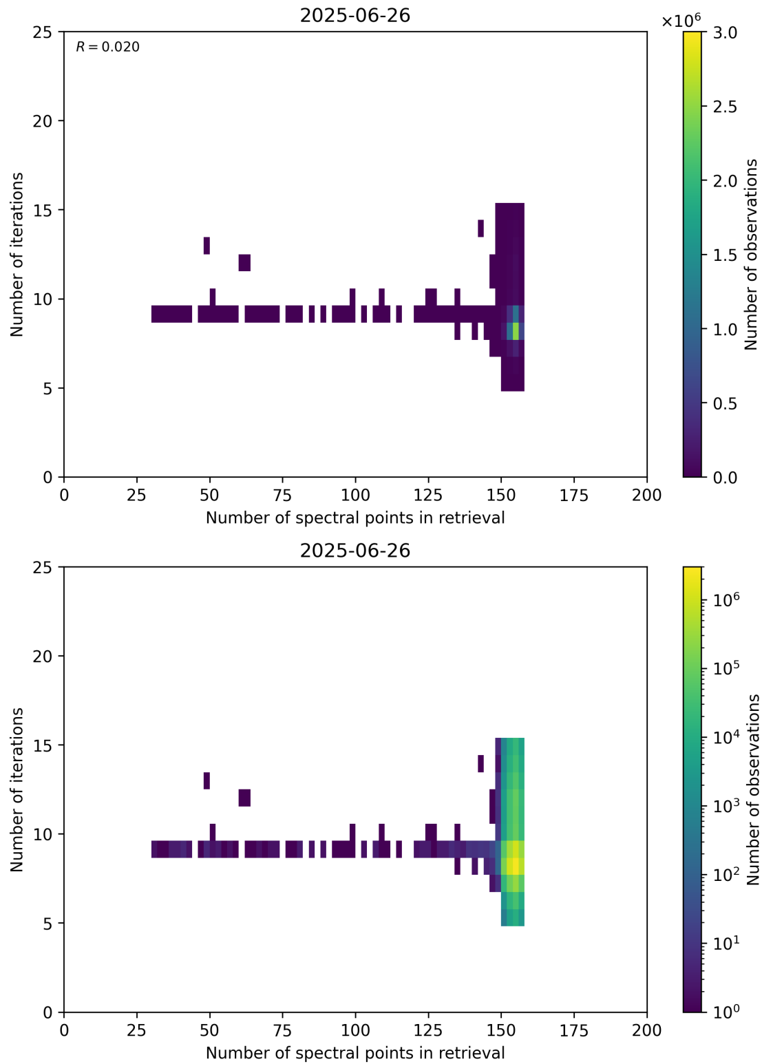
Figure 60: Scatter density plot of “Number of spectral points in retrieval” against “Number of iterations” for 2025-06-25 to 2025-06-27.
