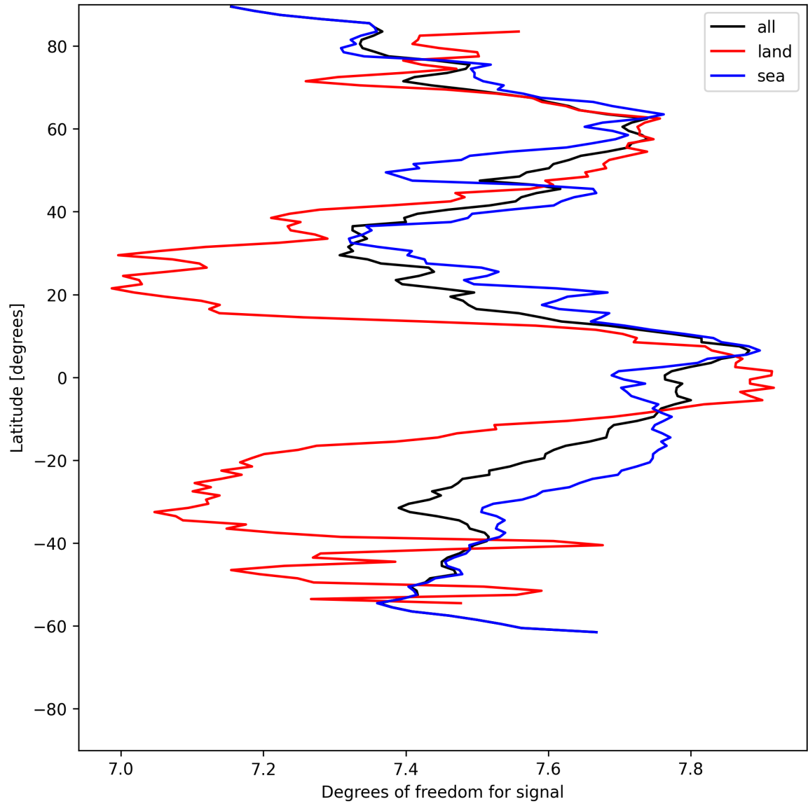
Figure 15: Zonal average of “Degrees of freedom for signal” for 2025-06-25 to 2025-06-27.
