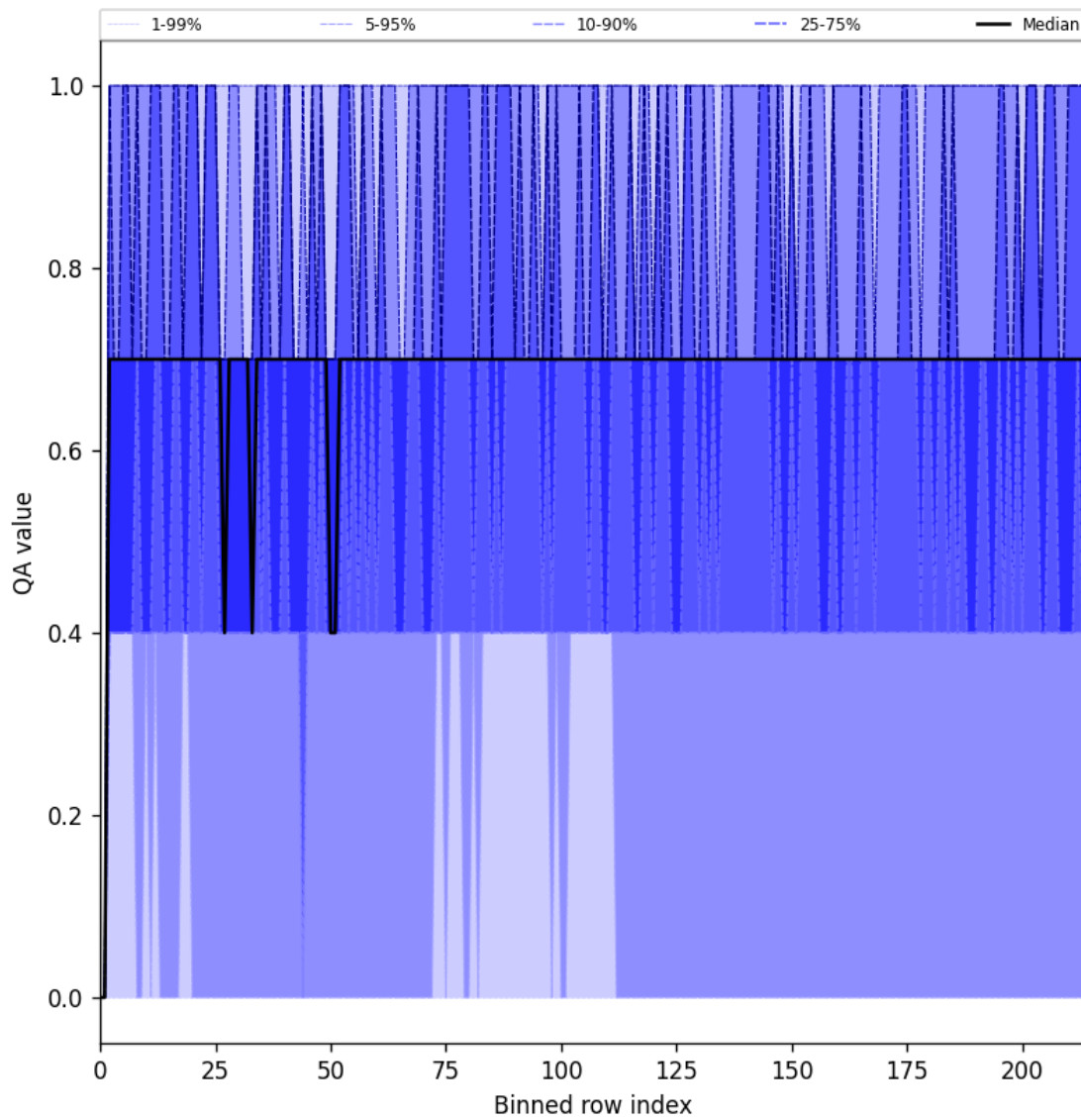
Figure 25: Along track statistics of “QA value” for 2025-06-25 to 2025-06-27
