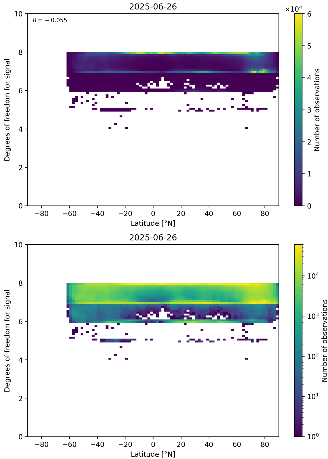
Figure 55: Scatter density plot of “Latitude” against “Degrees of freedom for signal” for 2025-06-25 to 2025-06-27.
