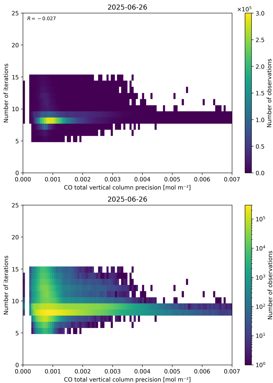
Figure 46: Scatter density plot of “CO total vertical column precision” against “Number of iterations” for 2025-06-25 to 2025-06-27.
