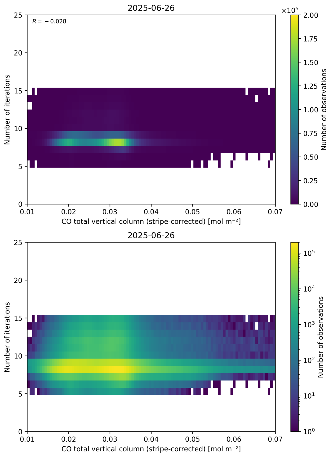
Figure 39: Scatter density plot of “CO total vertical column (stripe-corrected)” against “Number of iterations” for 2025-06-25 to 2025-06-27.
