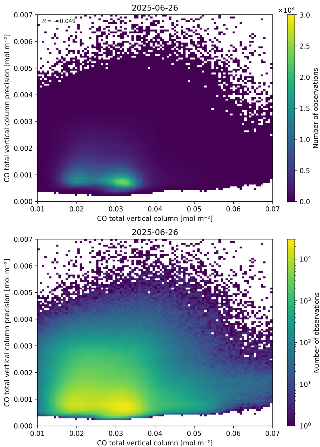
Figure 34: Scatter density plot of “CO total vertical column” against “CO total vertical column precision” for 2025-06-25 to 2025-06-27.
