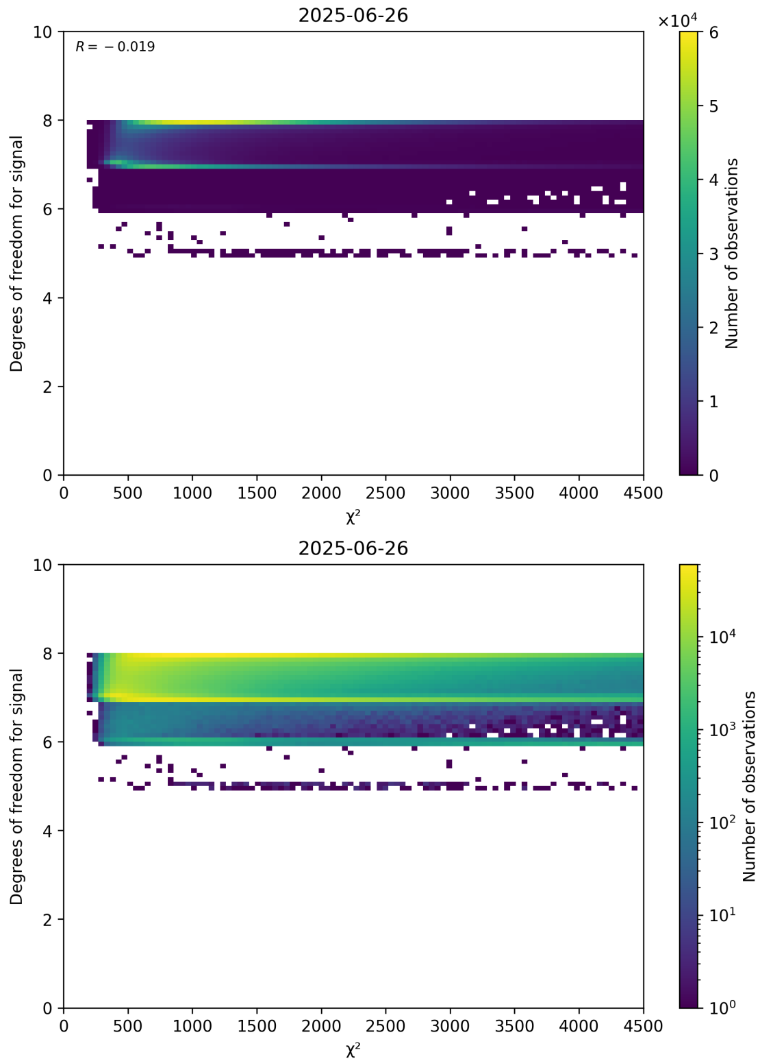
Figure 48: Scatter density plot of “ \chi^2 ” against “Degrees of freedom for signal” for 2025-06-25 to 2025-06-27.
