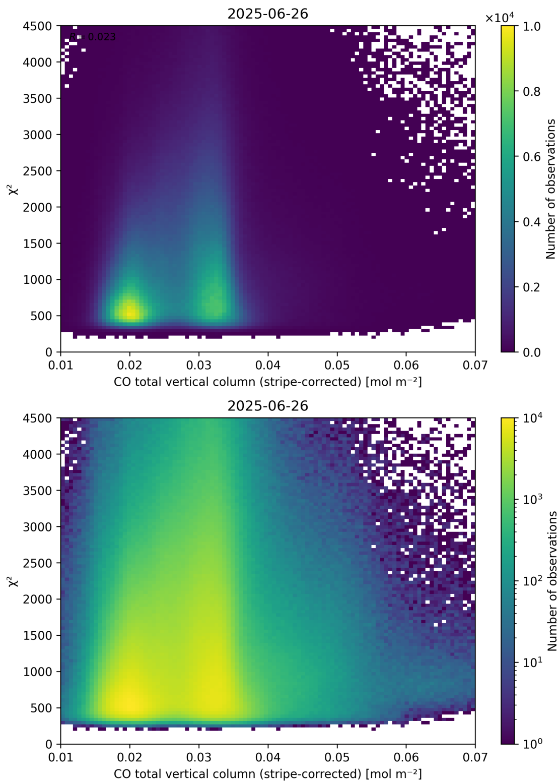
Figure 37: Scatter density plot of “CO total vertical column (stripe-corrected)” against “ \chi^2 ” for 2025-06-25 to 2025-06-27.
