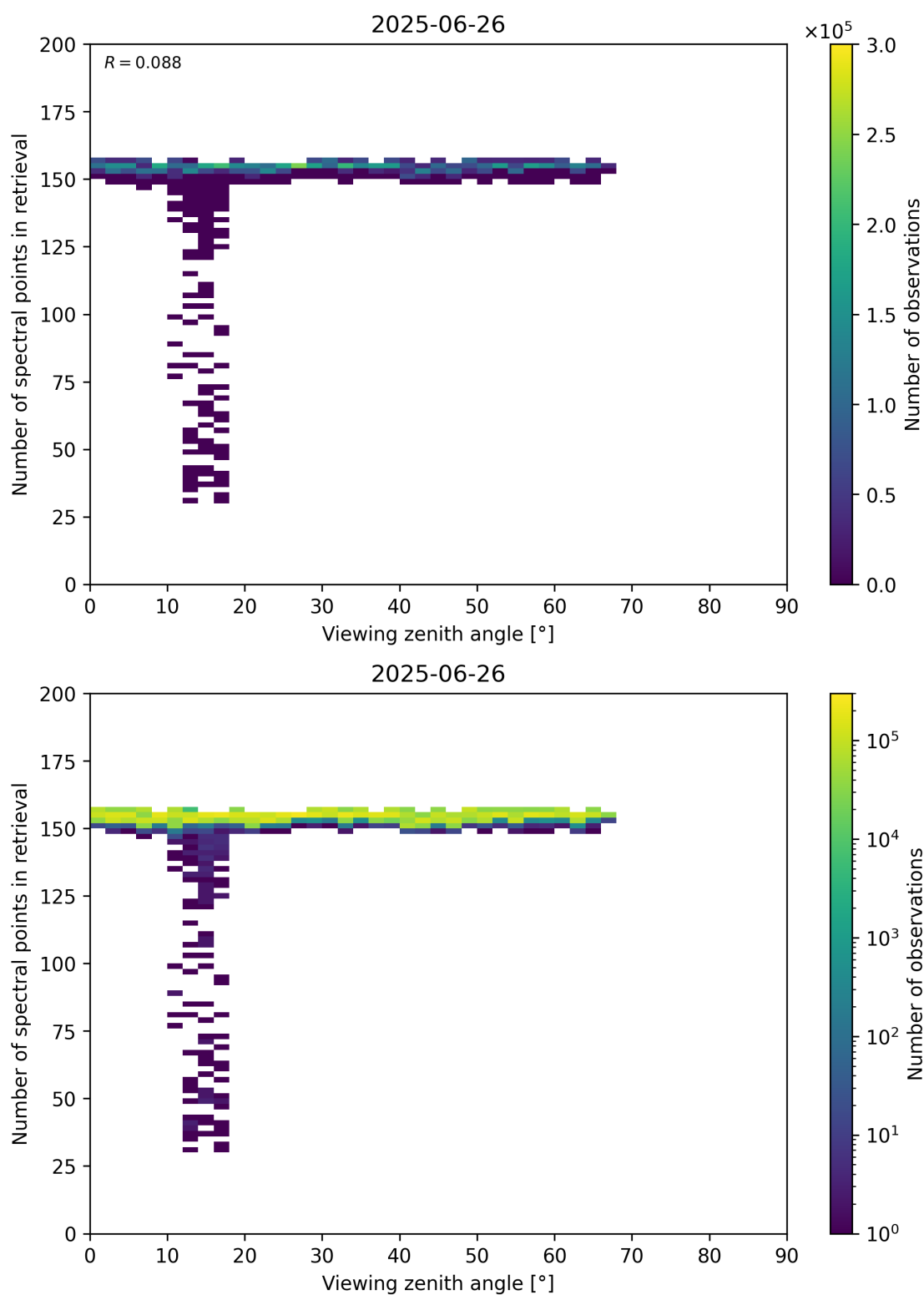
Figure 76: Scatter density plot of “Viewing zenith angle” against “Number of spectral points in retrieval” for 2025-06-25 to 2025-06-27.
