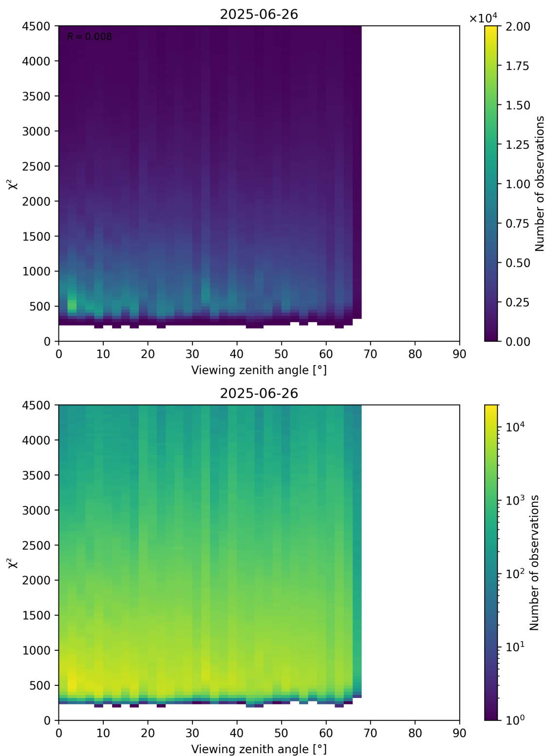
Figure 72: Scatter density plot of “Viewing zenith angle” against “ \chi^2 ” for 2025-06-25 to 2025-06-27.
