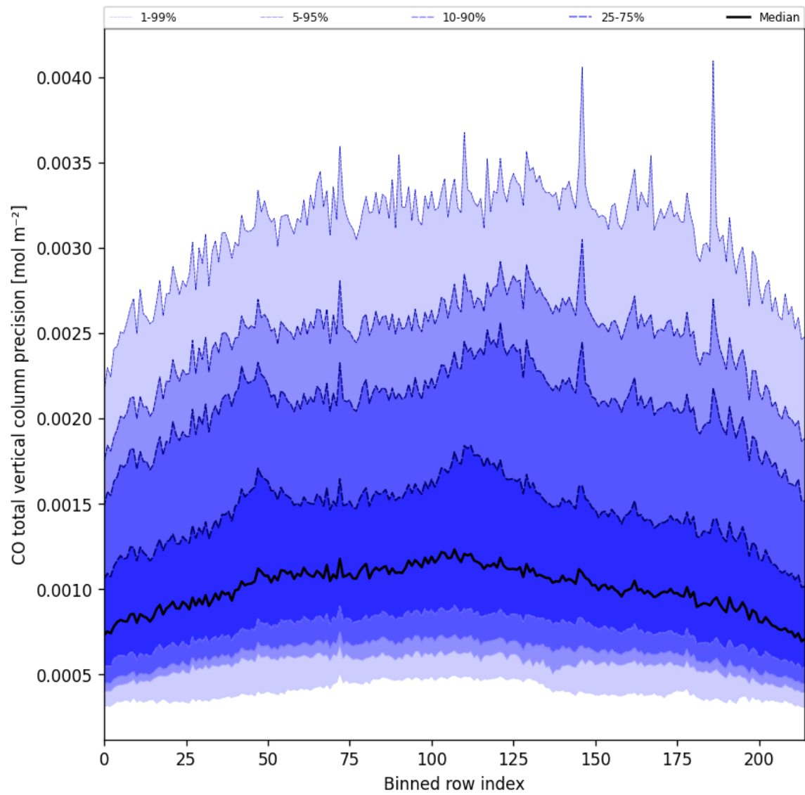
Figure 28: Along track statistics of “CO total vertical column precision” for 2025-06-25 to 2025-06-27
