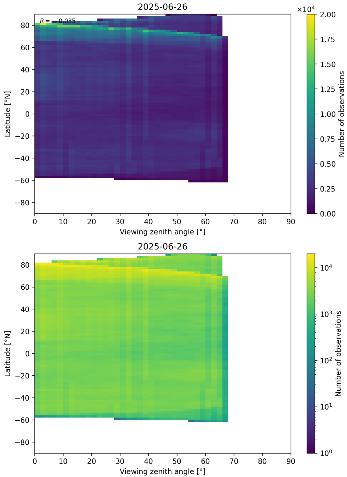
Figure 74: Scatter density plot of “Viewing zenith angle” against “Latitude” for 2025-06-25 to 2025-06-27.
