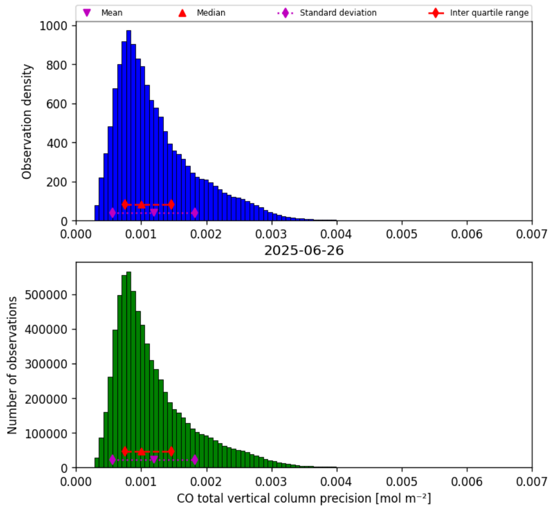
Figure 20: Histogram of “CO total vertical column precision” for 2025-06-25 to 2025-06-27
