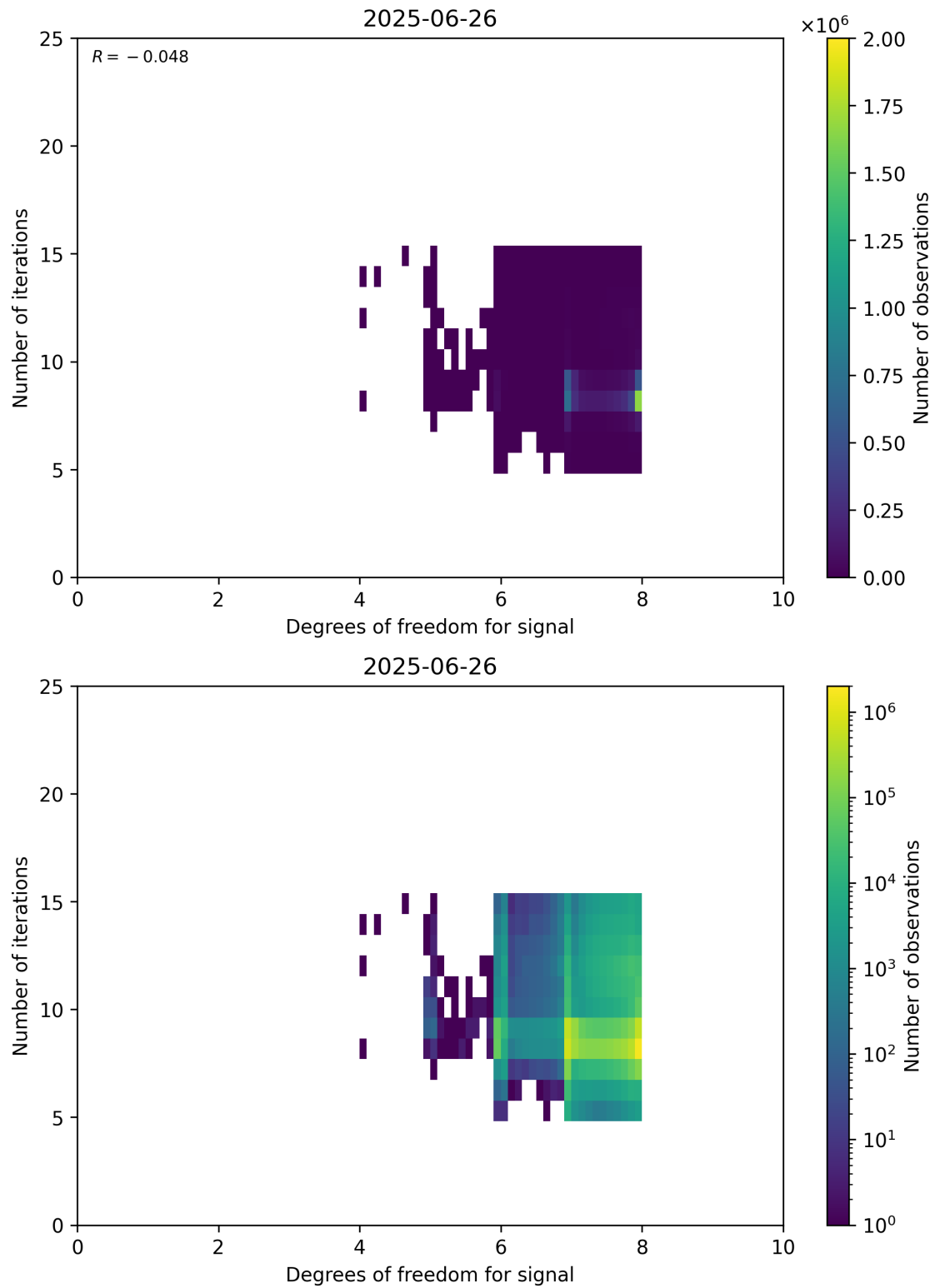
Figure 50: Scatter density plot of “Degrees of freedom for signal” against “Number of iterations” for 2025-06-25 to 2025-06-27.
