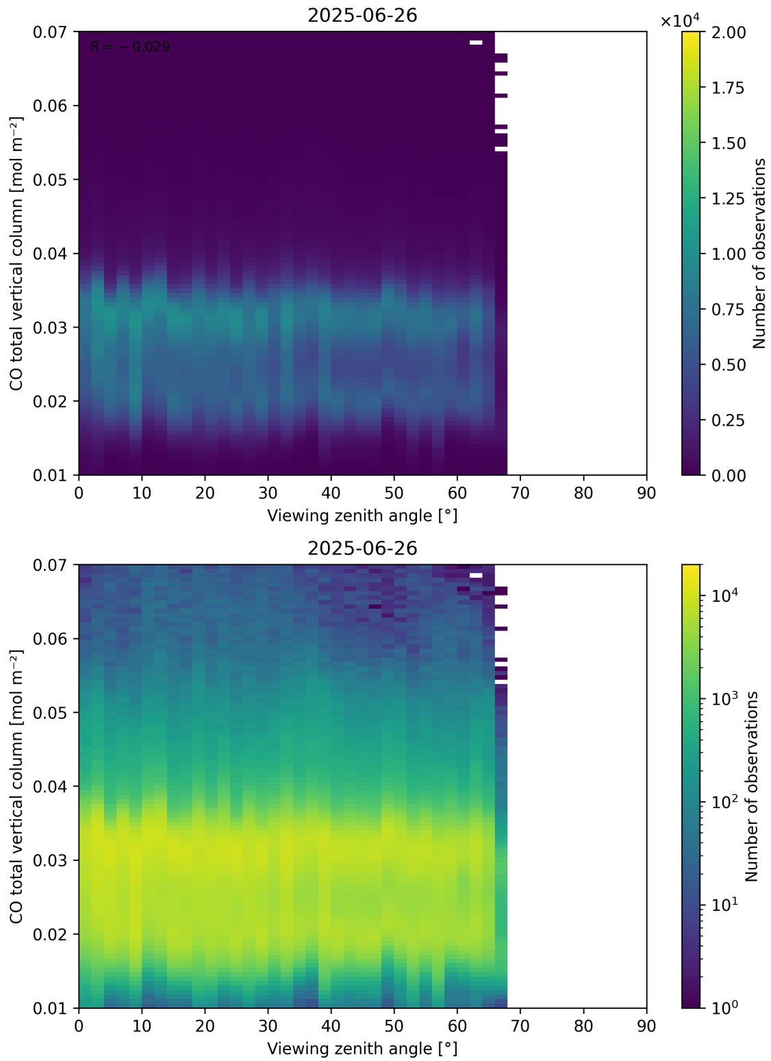
Figure 69: Scatter density plot of “Viewing zenith angle” against “CO total vertical column” for 2025-06-25 to 2025-06-27.
