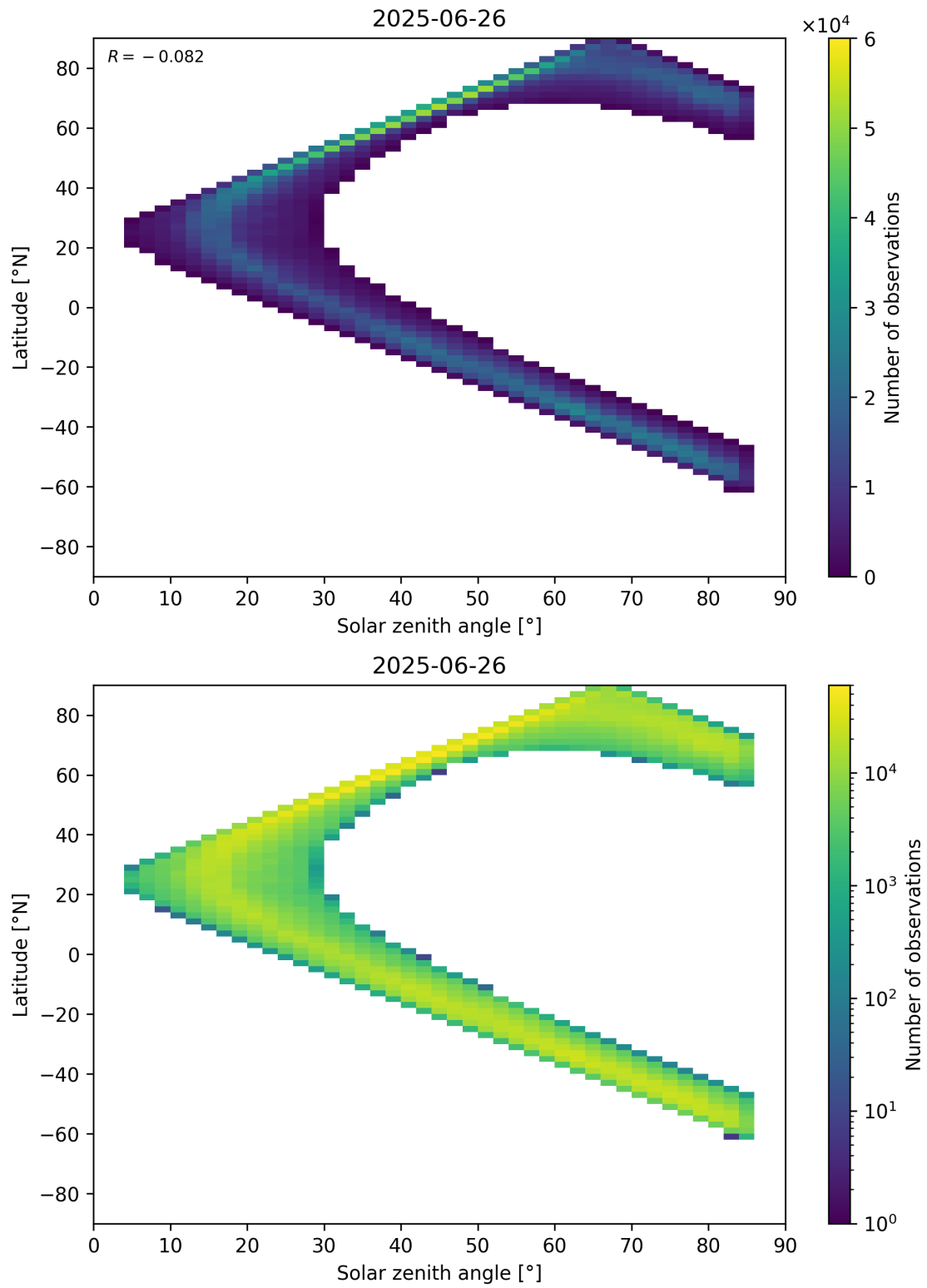
Figure 66: Scatter density plot of “Solar zenith angle” against “Latitude” for 2025-06-25 to 2025-06-27.
