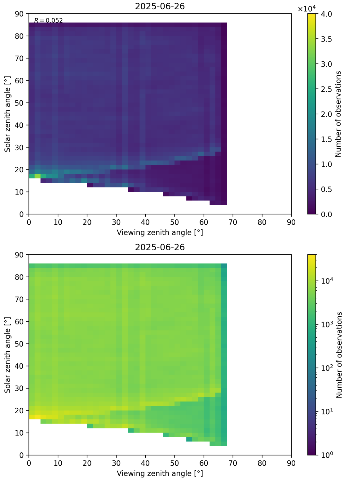
Figure 77: Scatter density plot of “Viewing zenith angle” against “Solar zenith angle” for 2025-06-25 to 2025-06-27.
