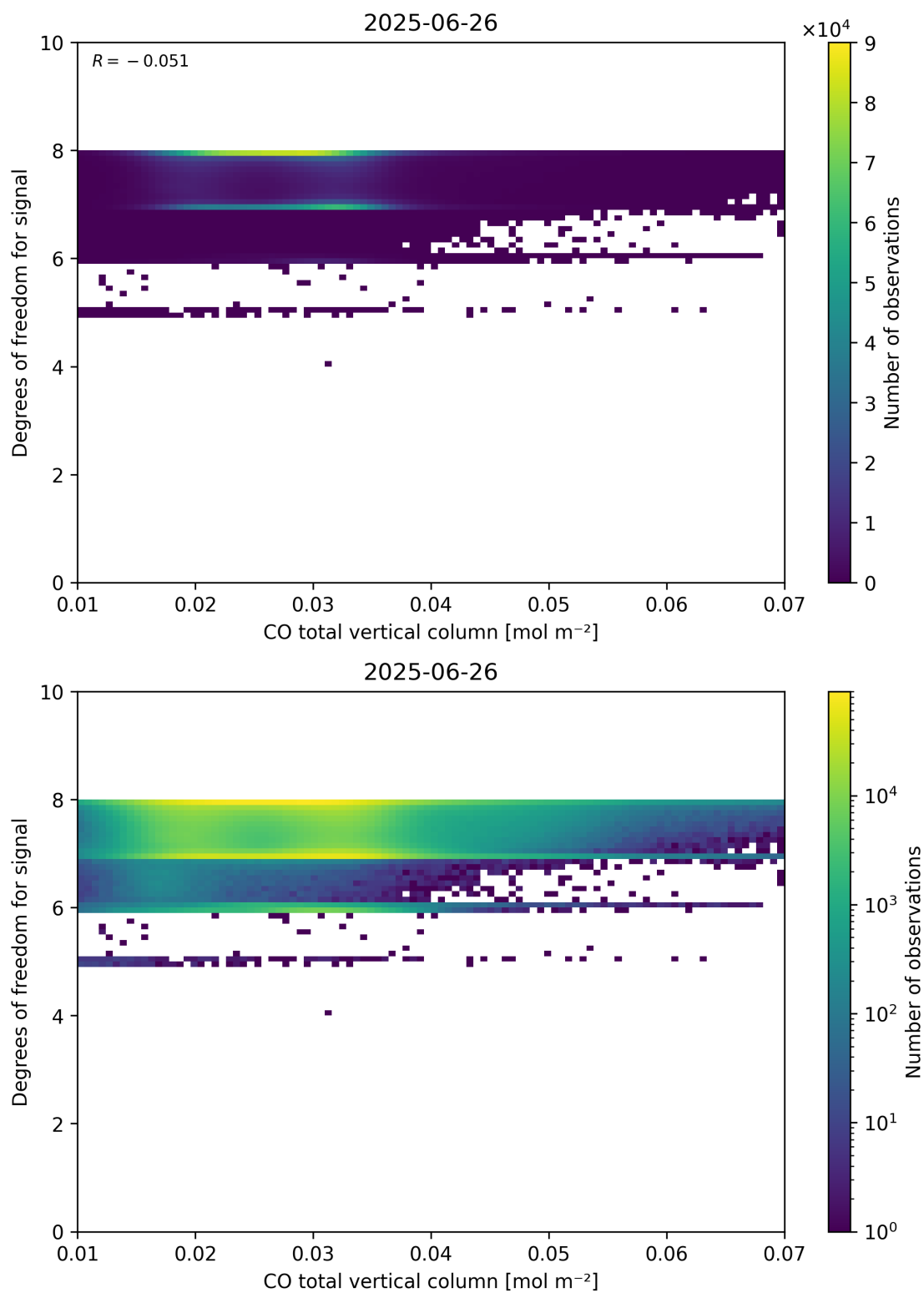
Figure 41: Scatter density plot of “CO total vertical column” against “Degrees of freedom for signal” for 2025-06-25 to 2025-06-27.
