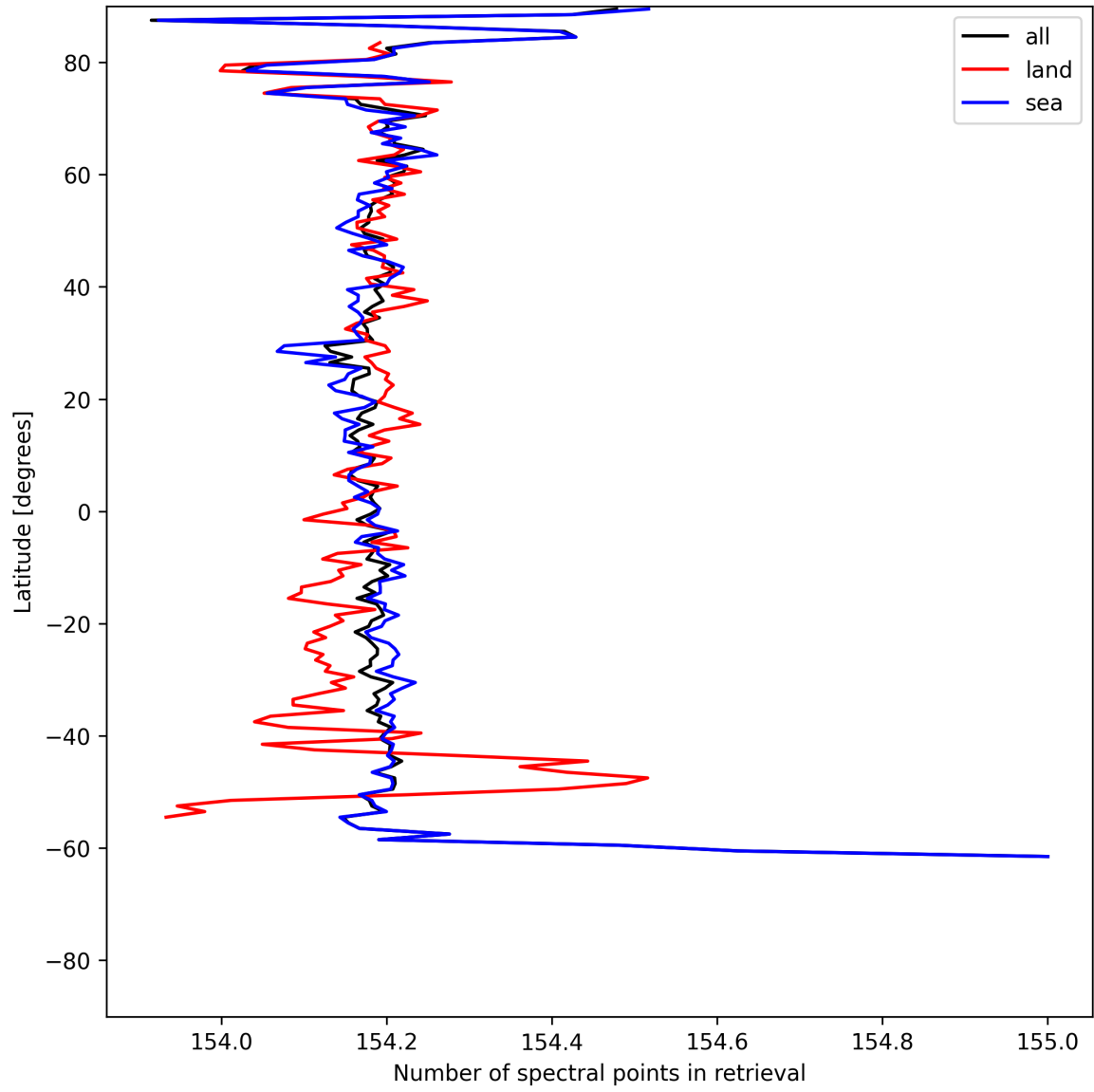
Figure 13: Zonal average of “Number of spectral points in retrieval” for 2025-06-25 to 2025-06-27.
