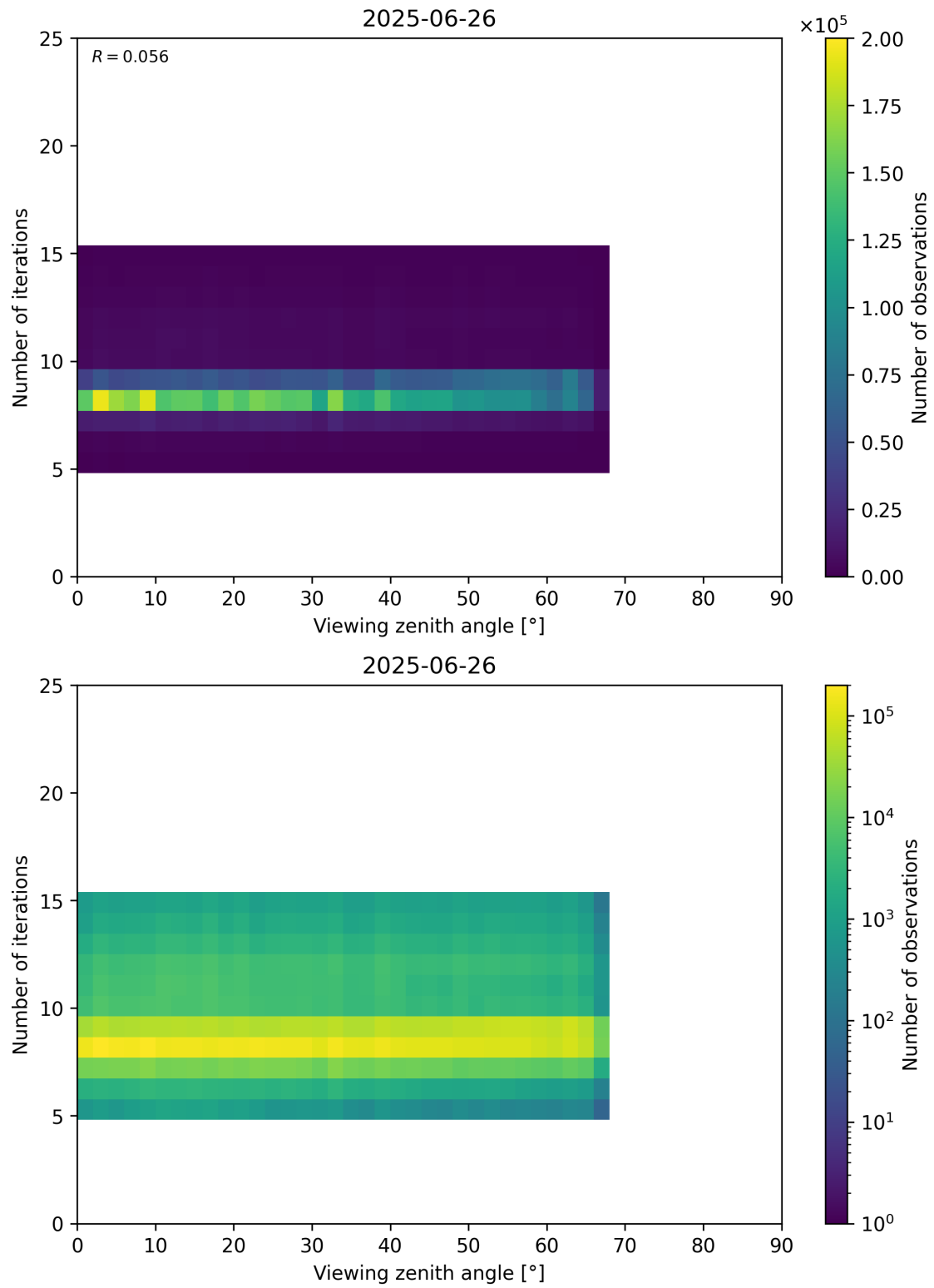
Figure 75: Scatter density plot of “Viewing zenith angle” against “Number of iterations” for 2025-06-25 to 2025-06-27.
