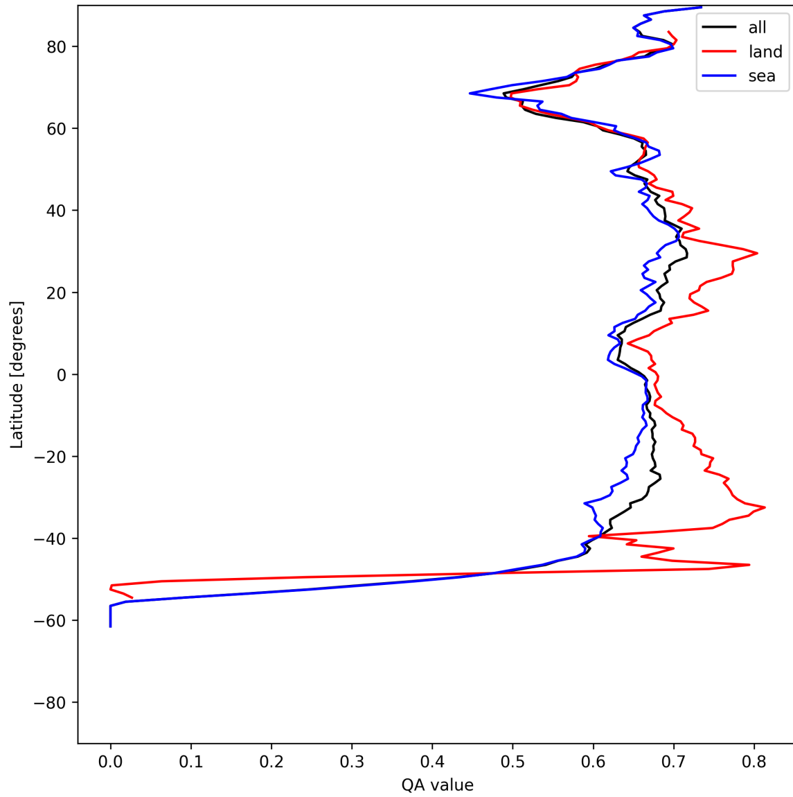
Figure 9: Zonal average of “QA value” for 2025-06-25 to 2025-06-27.
