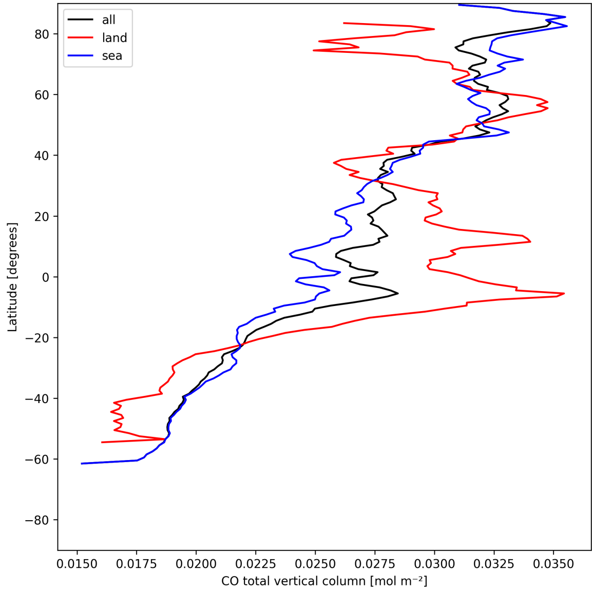
Figure 10: Zonal average of “CO total vertical column” for 2025-06-25 to 2025-06-27.
