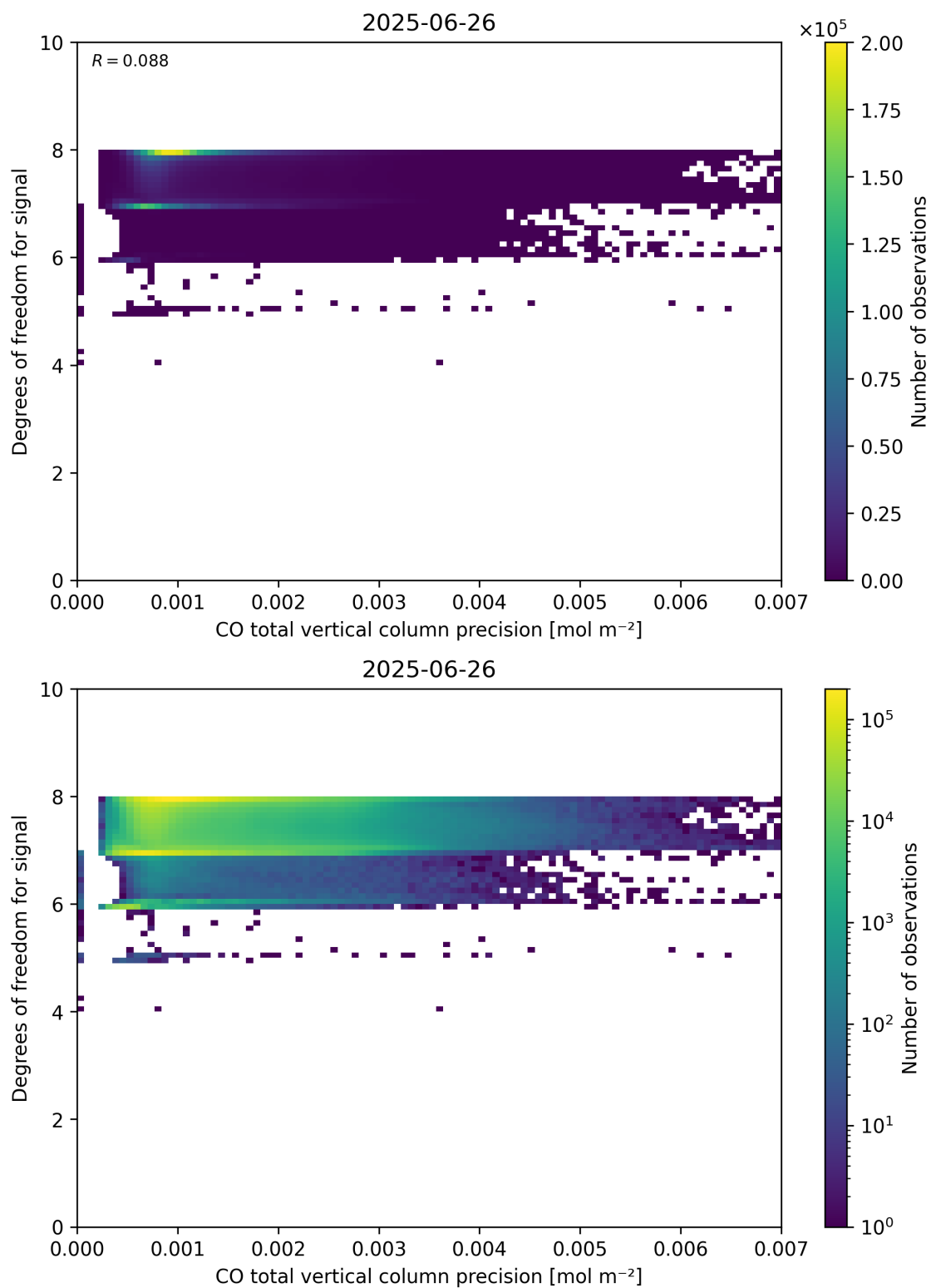
Figure 45: Scatter density plot of “CO total vertical column precision” against “Degrees of freedom for signal” for 2025-06-25 to 2025-06-27.
