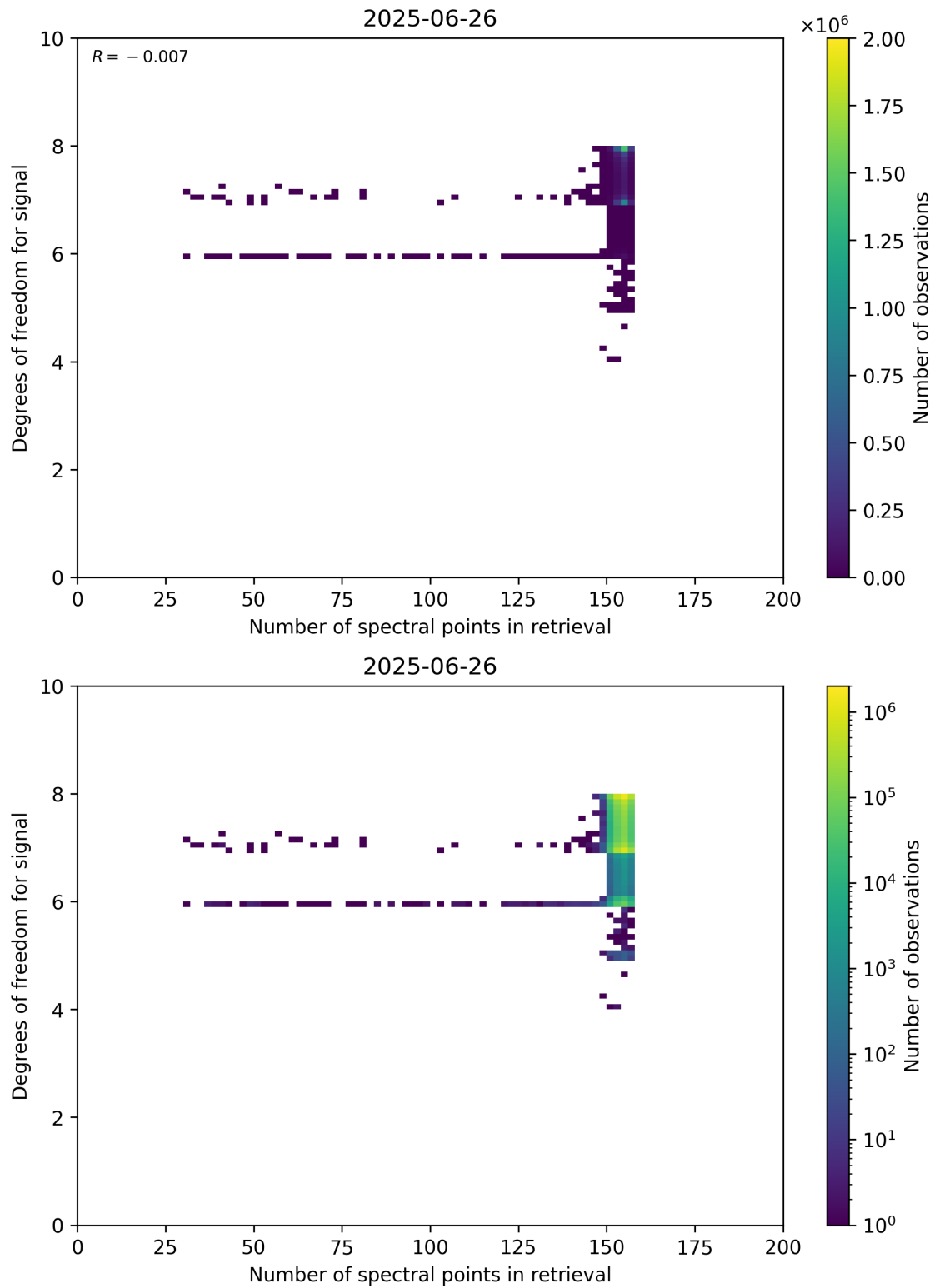
Figure 59: Scatter density plot of “Number of spectral points in retrieval” against “Degrees of freedom for signal” for 2025-06-25 to 2025-06-27.
