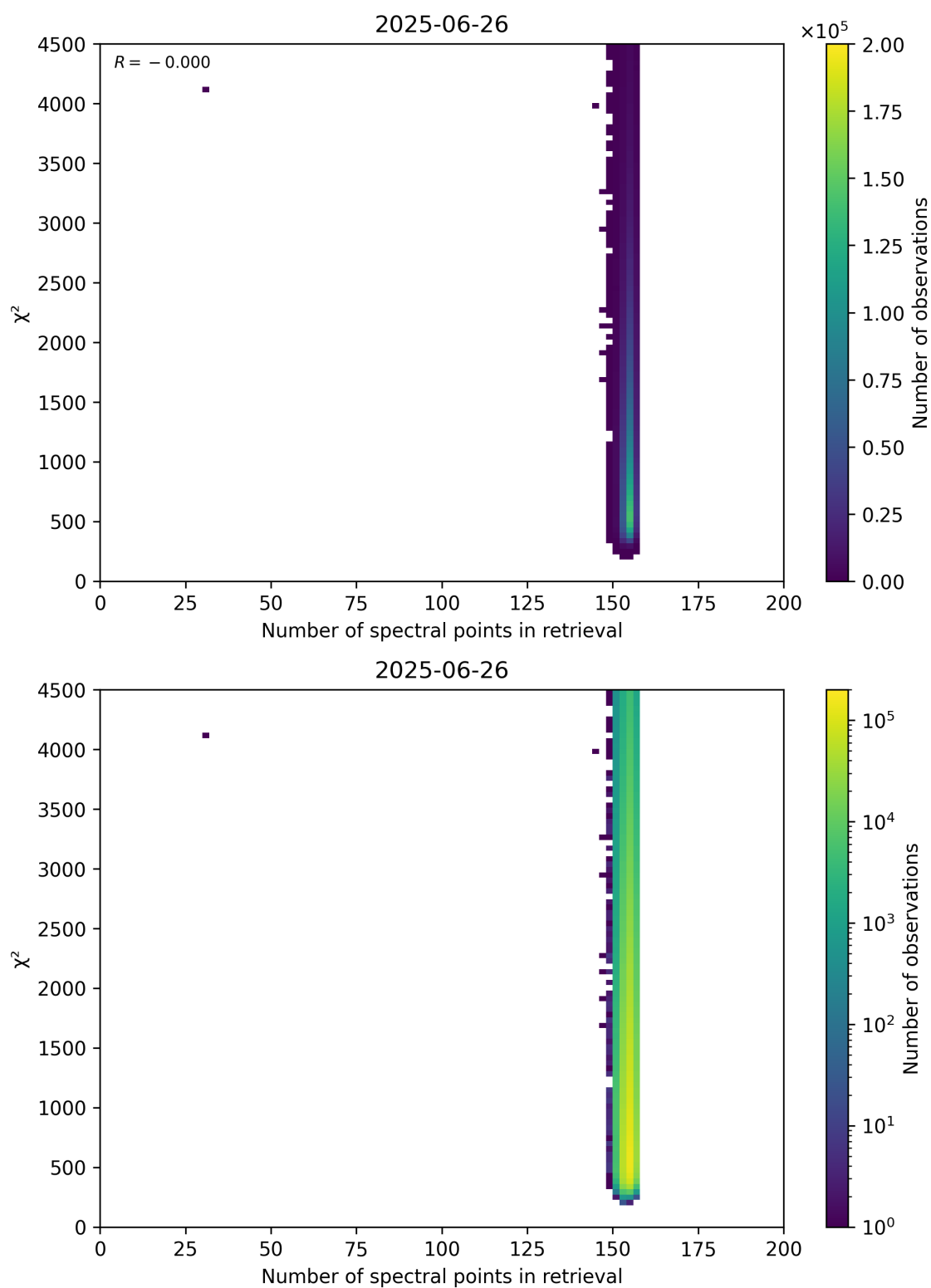
Figure 58: Scatter density plot of “Number of spectral points in retrieval” against “ \chi^2 ” for 2025-06-25 to 2025-06-27.
