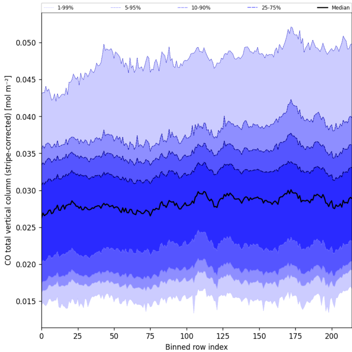
Figure 27: Along track statistics of “CO total vertical column (stripe-corrected)” for 2025-06-25 to 2025-06-27
