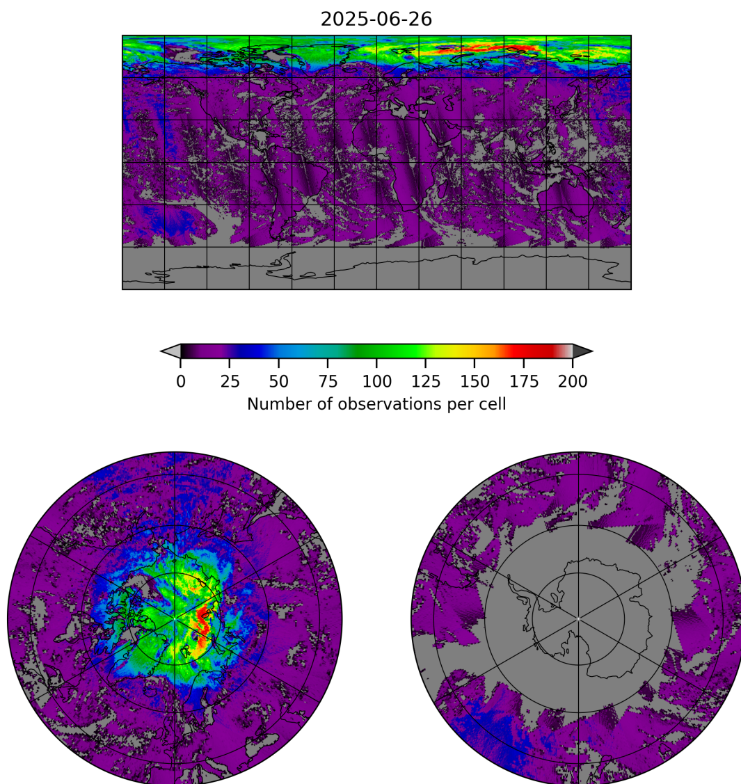
Figure 8: Map of the number of observations for 2025-06-25 to 2025-06-27
