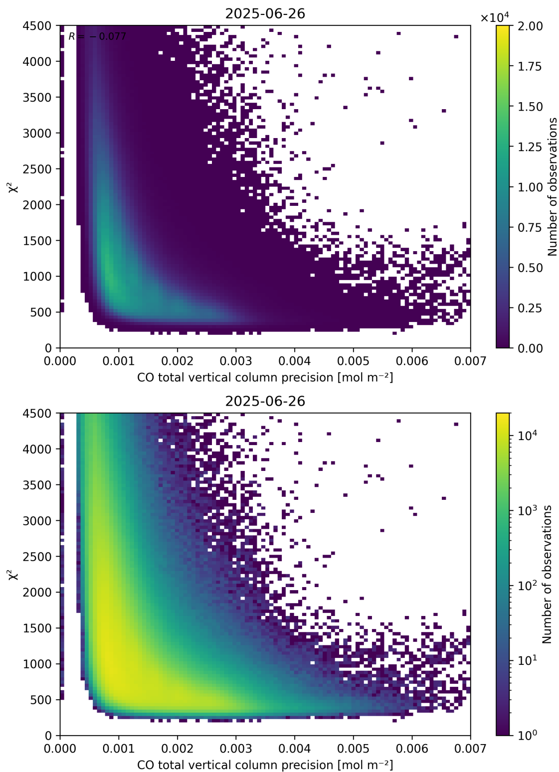
Figure 44: Scatter density plot of “CO total vertical column precision” against “ \chi^2 ” for 2025-06-25 to 2025-06-27.
