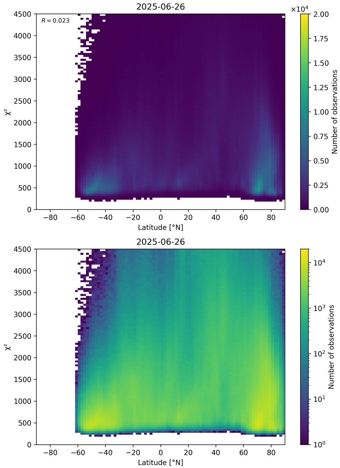
Figure 54: Scatter density plot of “Latitude” against “ \chi^2 ” for 2025-06-25 to 2025-06-27.
