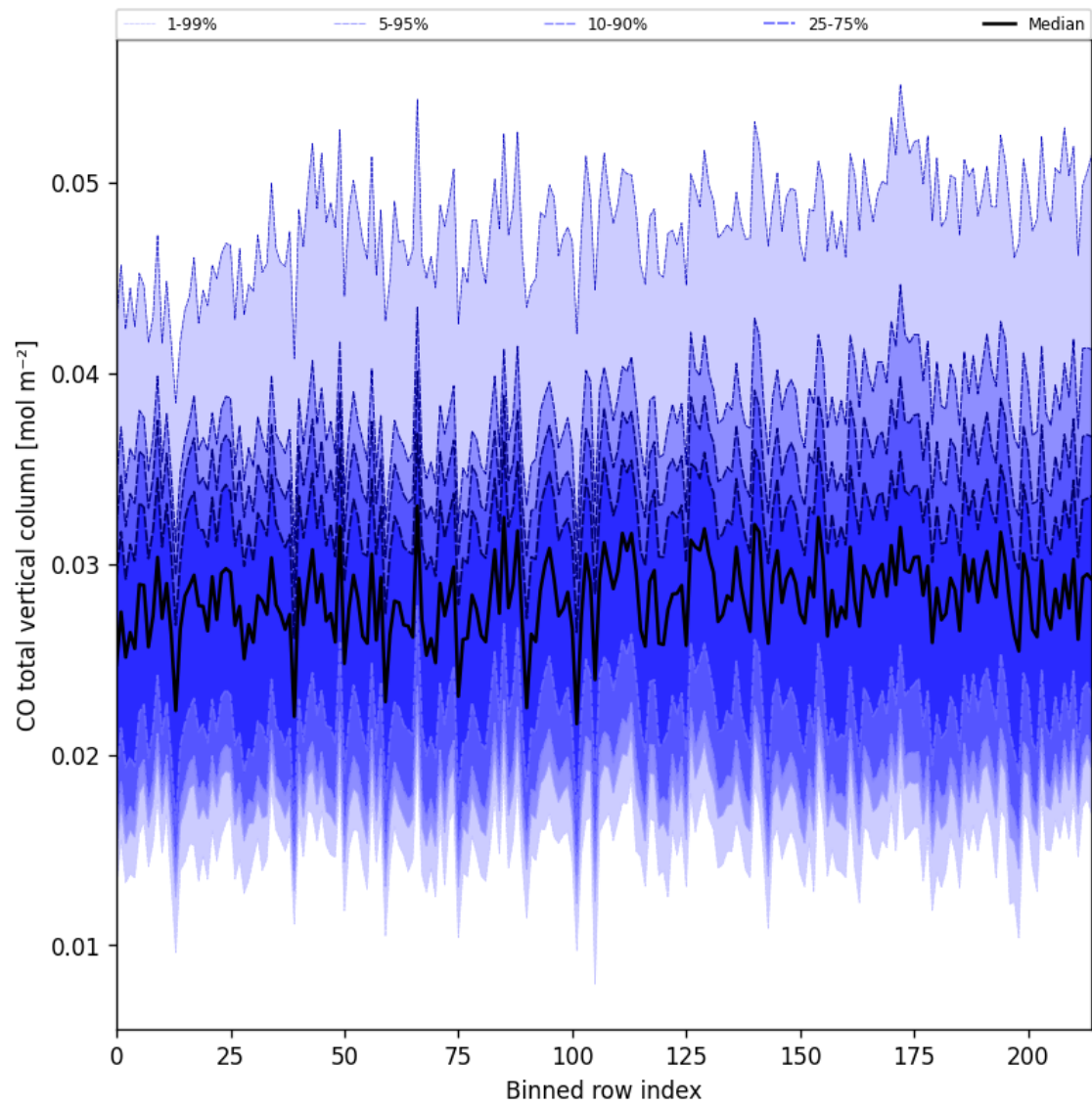
Figure 26: Along track statistics of “CO total vertical column” for 2025-06-25 to 2025-06-27
