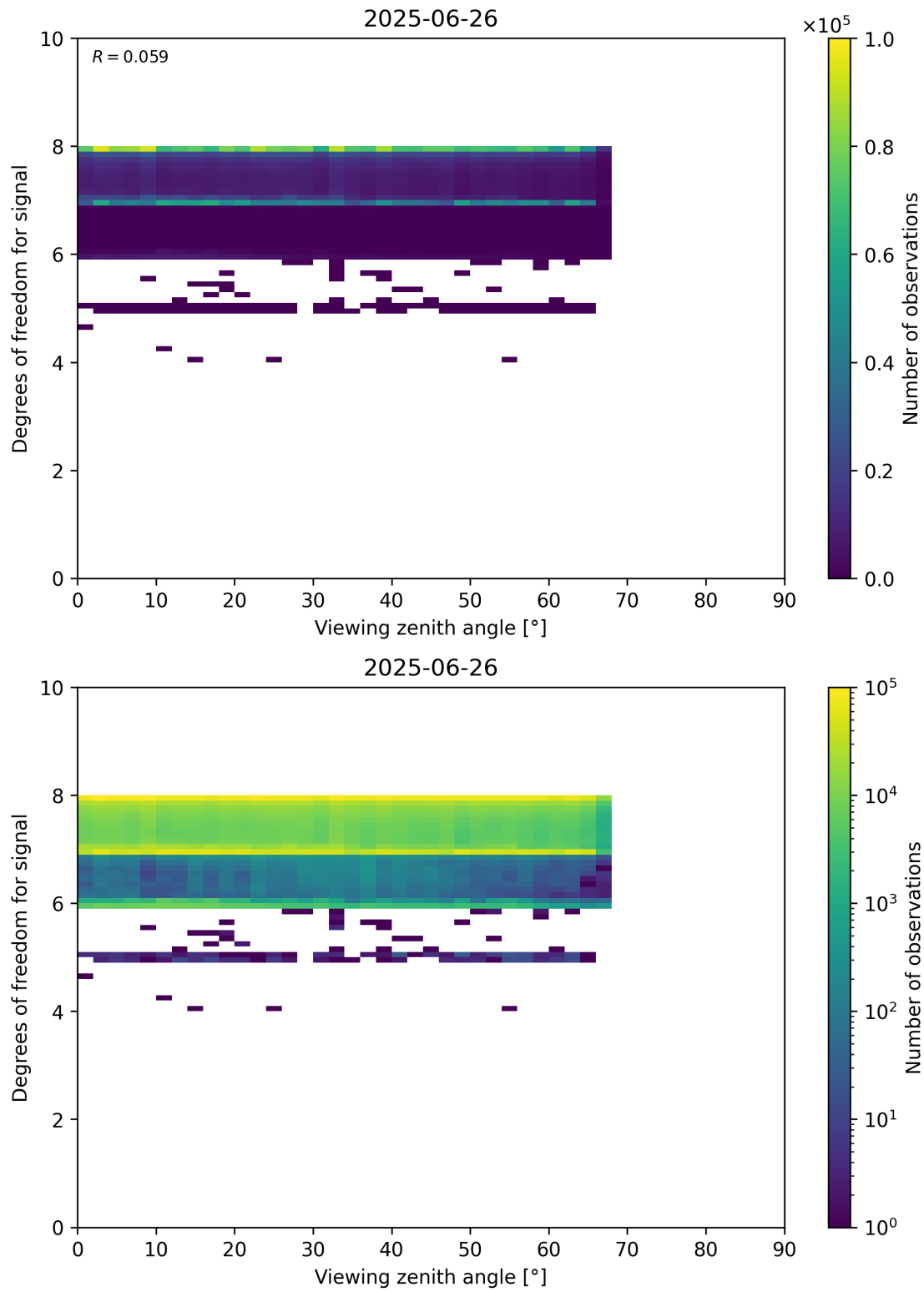
Figure 73: Scatter density plot of “Viewing zenith angle” against “Degrees of freedom for signal” for 2025-06-25 to 2025-06-27.
