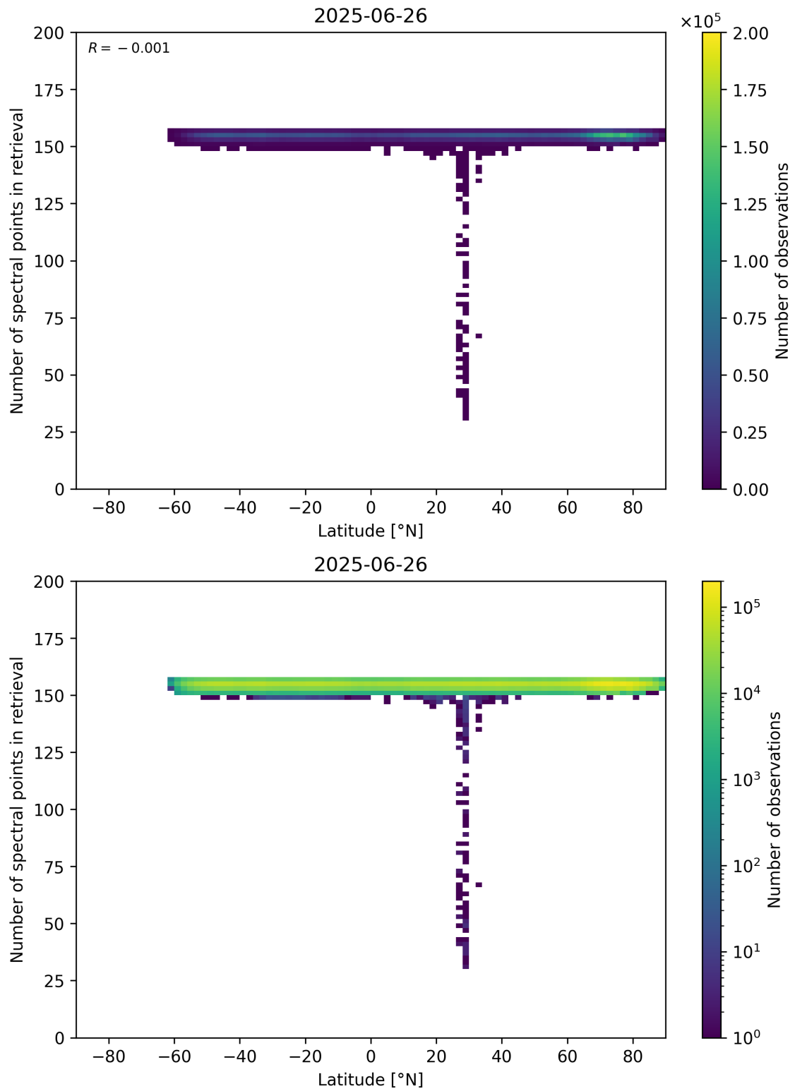
Figure 57: Scatter density plot of “Latitude” against “Number of spectral points in retrieval” for 2025-06-25 to 2025-06-27.
