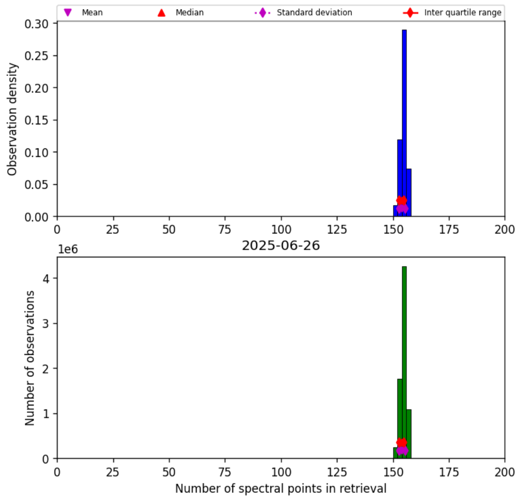
Figure 21: Histogram of “Number of spectral points in retrieval” for 2025-06-25 to 2025-06-27
