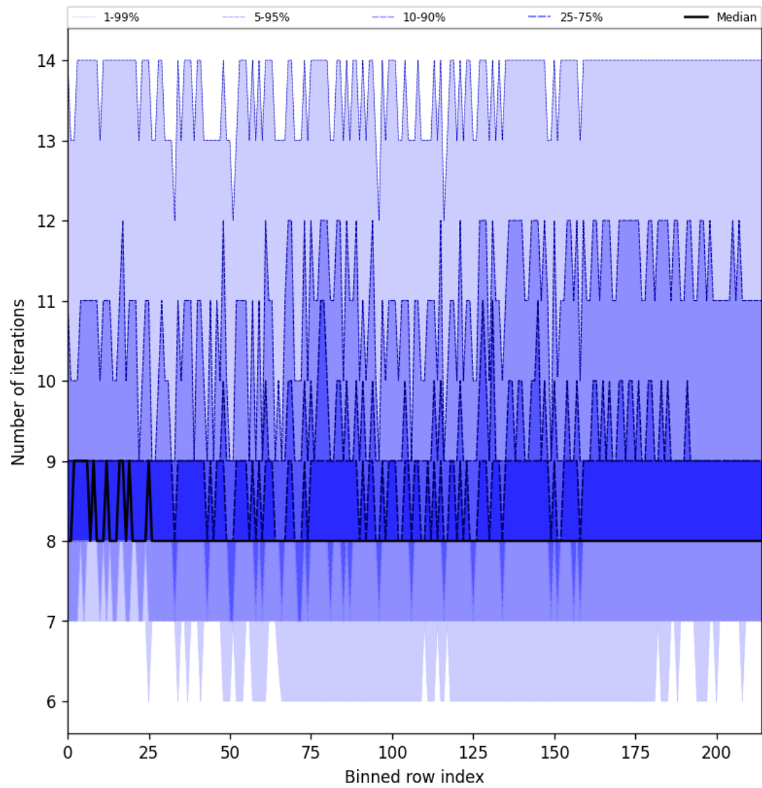
Figure 32: Along track statistics of “Number of iterations” for 2025-06-25 to 2025-06-27
