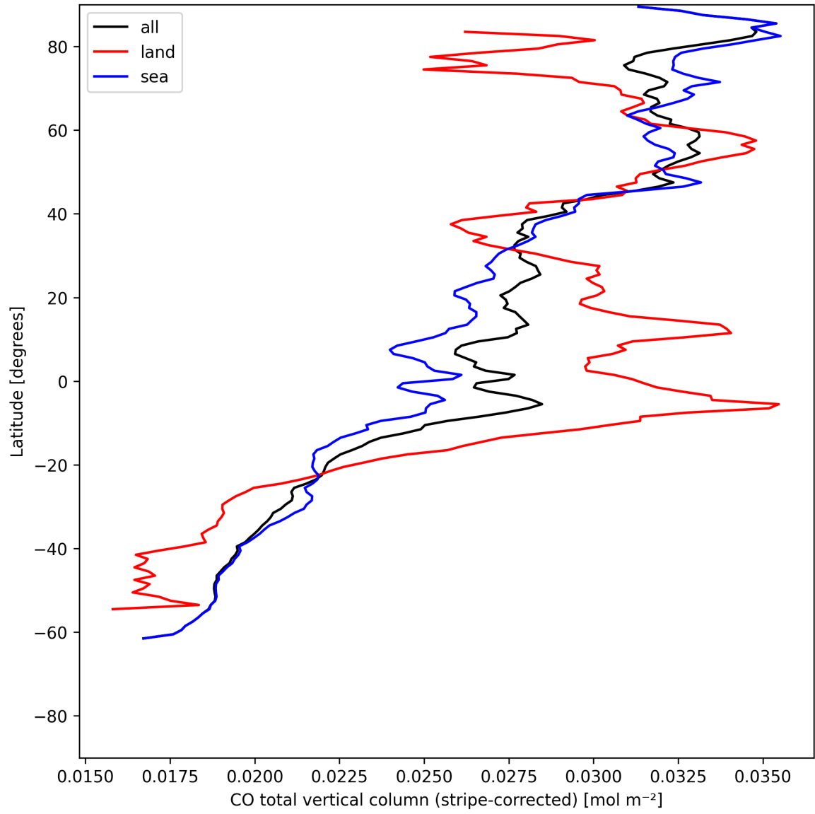
Figure 11: Zonal average of “CO total vertical column (stripe-corrected)” for 2025-06-25 to 2025-06-27.
