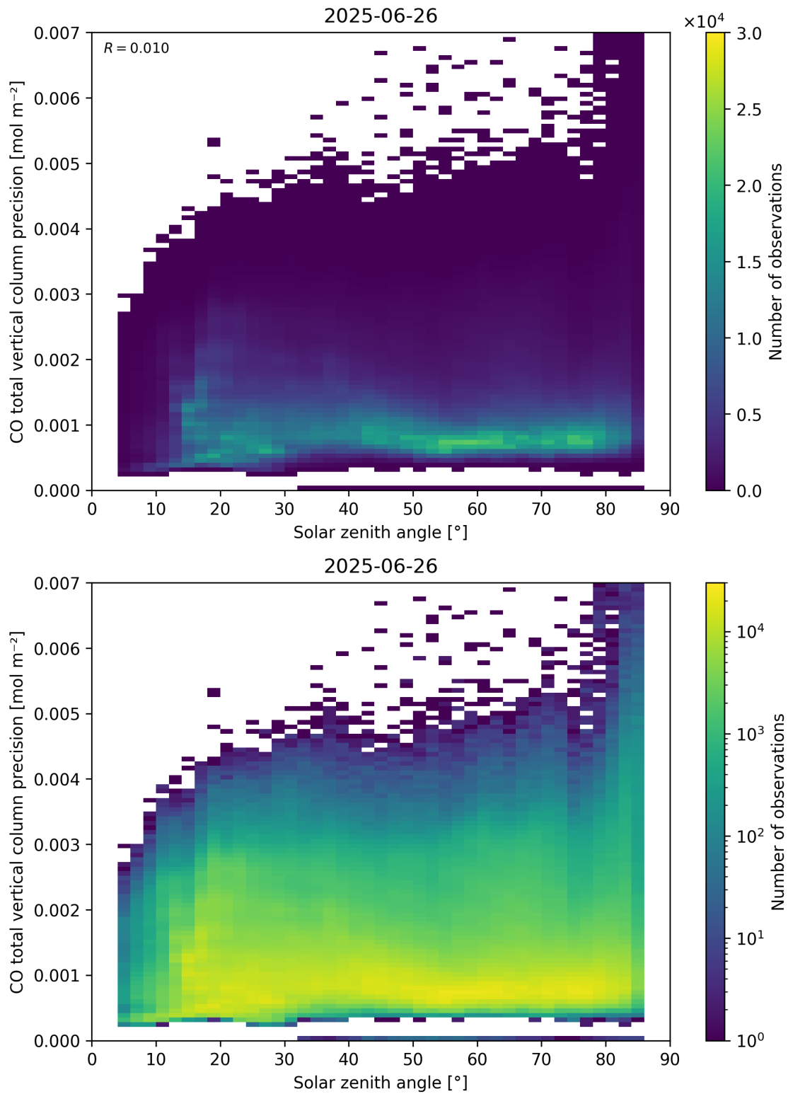
Figure 63: Scatter density plot of “Solar zenith angle” against “CO total vertical column precision” for 2025-06-25 to 2025-06-27.
