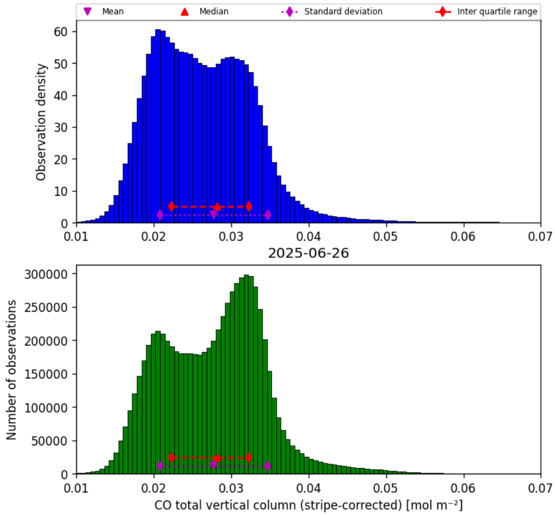
Figure 19: Histogram of “CO total vertical column (stripe-corrected)” for 2025-06-25 to 2025-06-27
