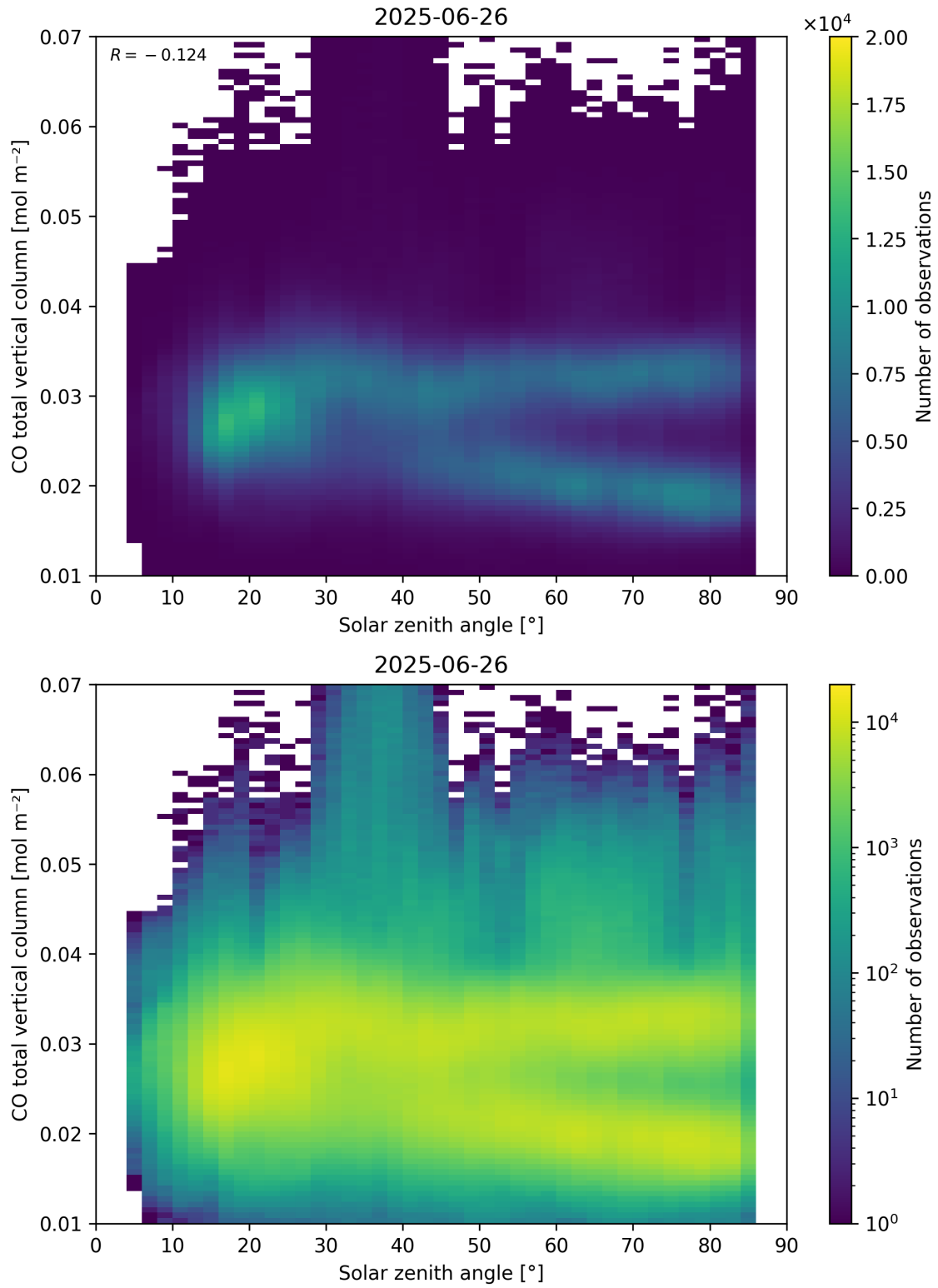
Figure 61: Scatter density plot of “Solar zenith angle” against “CO total vertical column” for 2025-06-25 to 2025-06-27.
