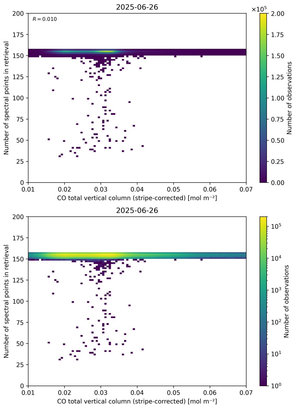
Figure 40: Scatter density plot of “CO total vertical column (stripe-corrected)” against “Number of spectral points in retrieval” for 2025-06-25 to 2025-06-27.
