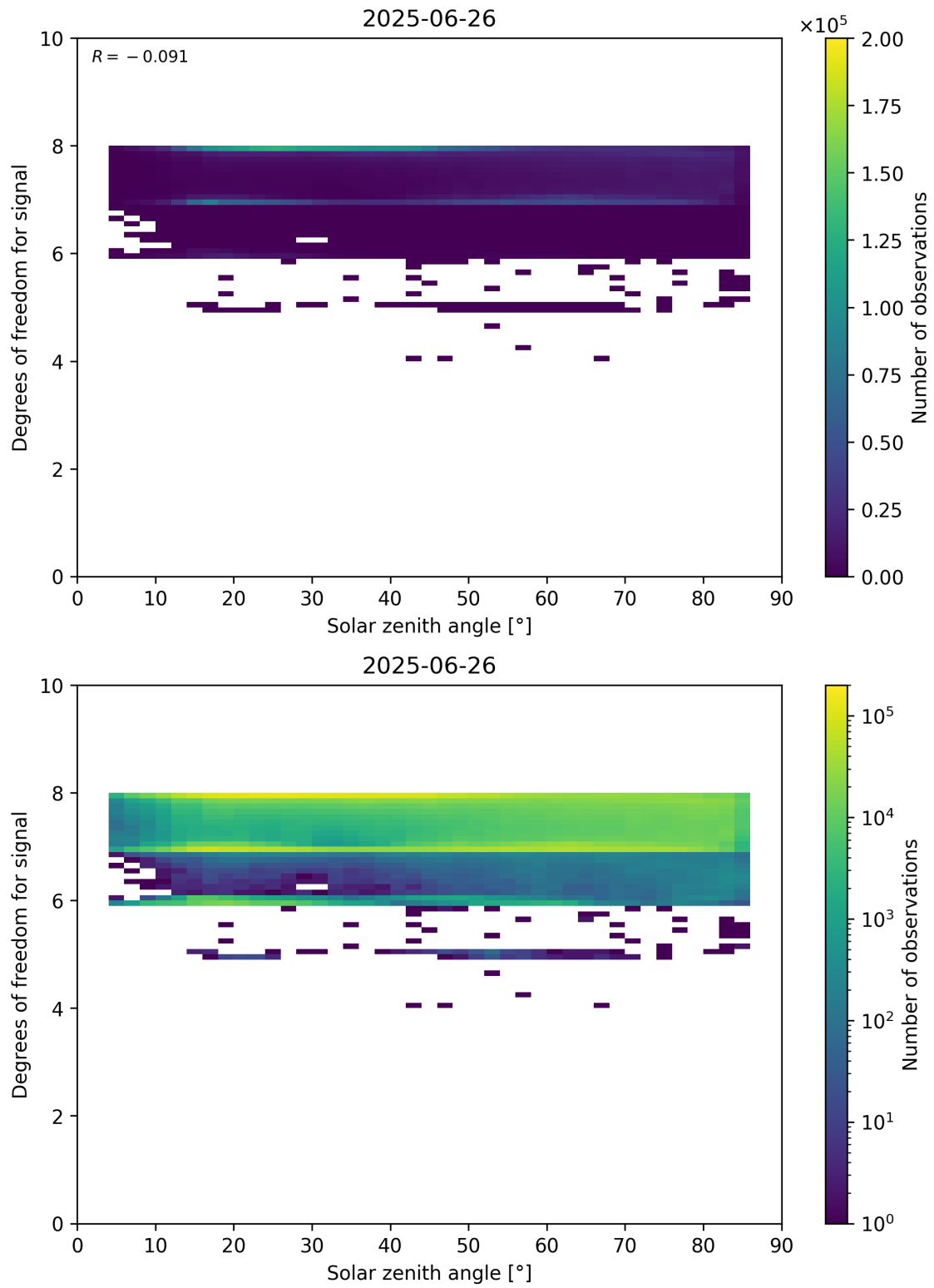
Figure 65: Scatter density plot of “Solar zenith angle” against “Degrees of freedom for signal” for 2025-06-25 to 2025-06-27.
