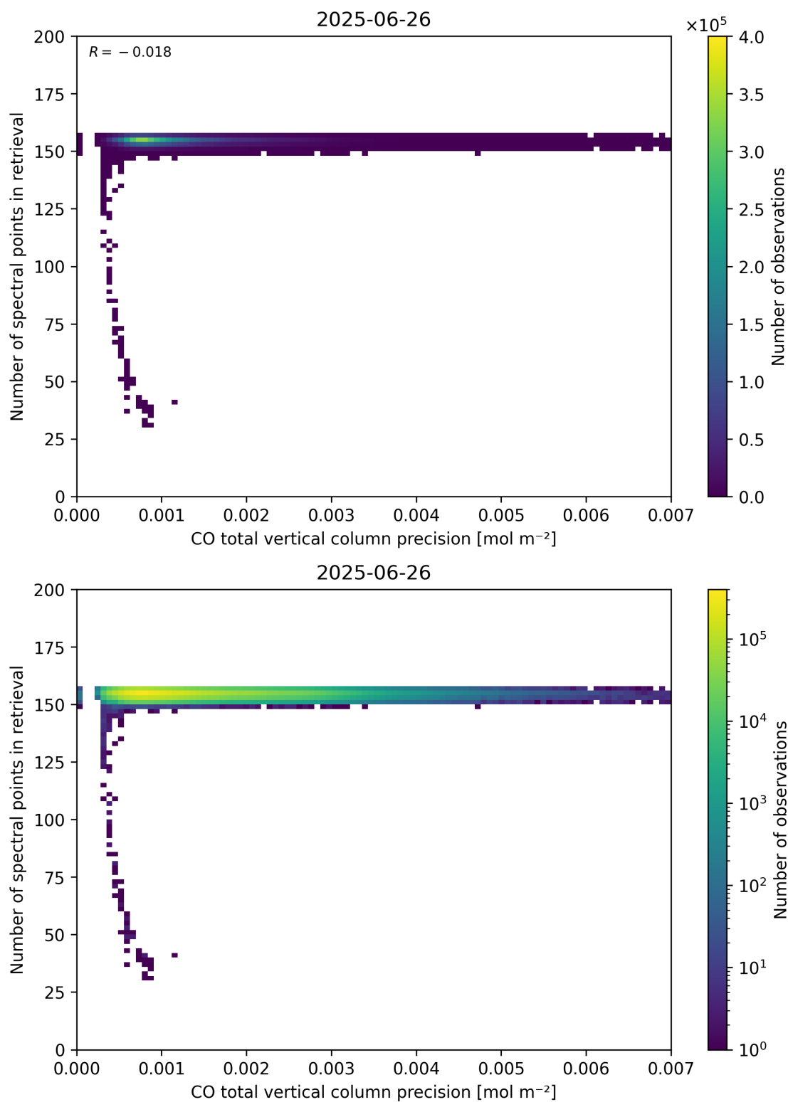
Figure 47: Scatter density plot of “CO total vertical column precision” against “Number of spectral points in retrieval” for 2025-06-25 to 2025-06-27.
