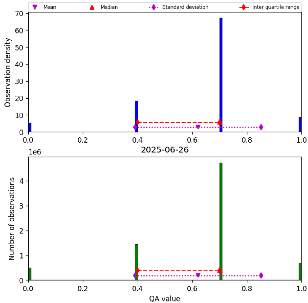
Figure 17: Histogram of “QA value” for 2025-06-25 to 2025-06-27
