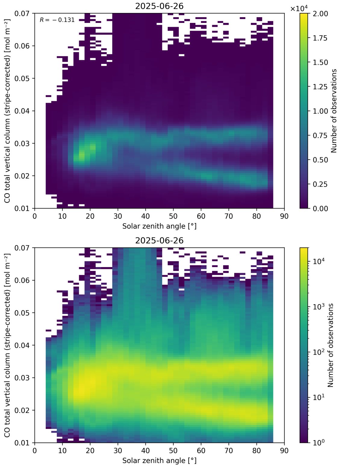
Figure 62: Scatter density plot of “Solar zenith angle” against “CO total vertical column (stripe-corrected)” for 2025-06-25 to 2025-06-27.
