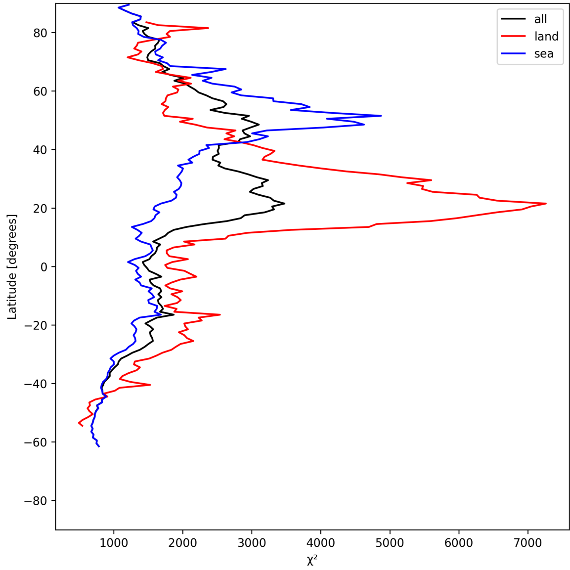
Figure 14: Zonal average of “ \chi^2 ” for 2025-06-25 to 2025-06-27.
