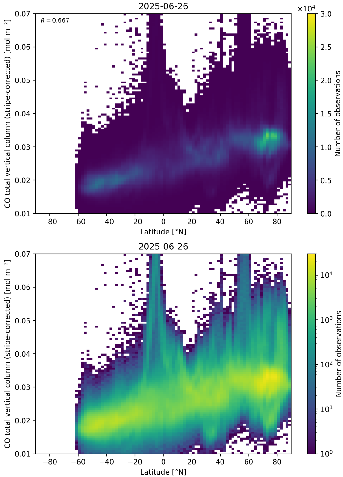
Figure 52: Scatter density plot of “Latitude” against “CO total vertical column (stripe-corrected)” for 2025-06-25 to 2025-06-27.
