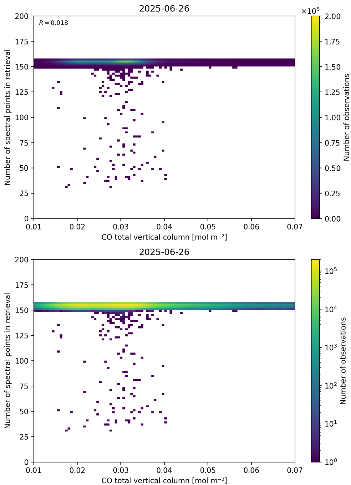
Figure 43: Scatter density plot of “CO total vertical column” against “Number of spectral points in retrieval” for 2025-06-25 to 2025-06-27.
