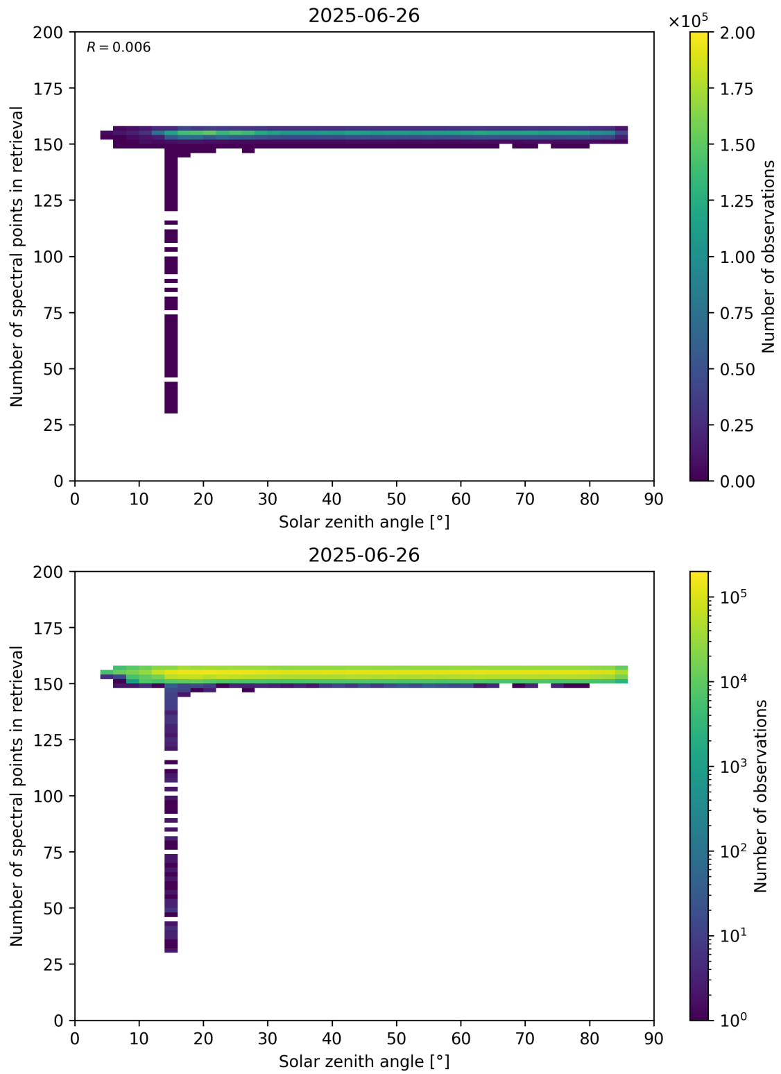
Figure 68: Scatter density plot of “Solar zenith angle” against “Number of spectral points in retrieval” for 2025-06-25 to 2025-06-27.
