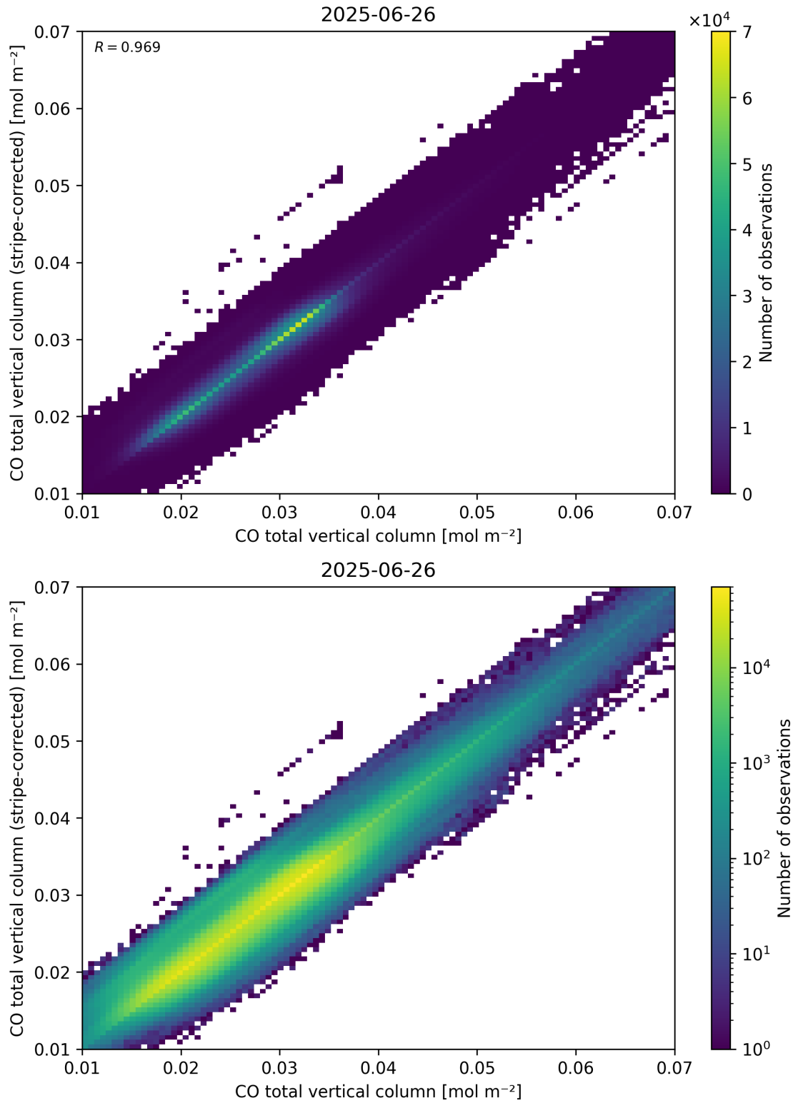
Figure 33: Scatter density plot of “CO total vertical column” against “CO total vertical column (stripe-corrected)” for 2025-06-25 to 2025-06-27.
