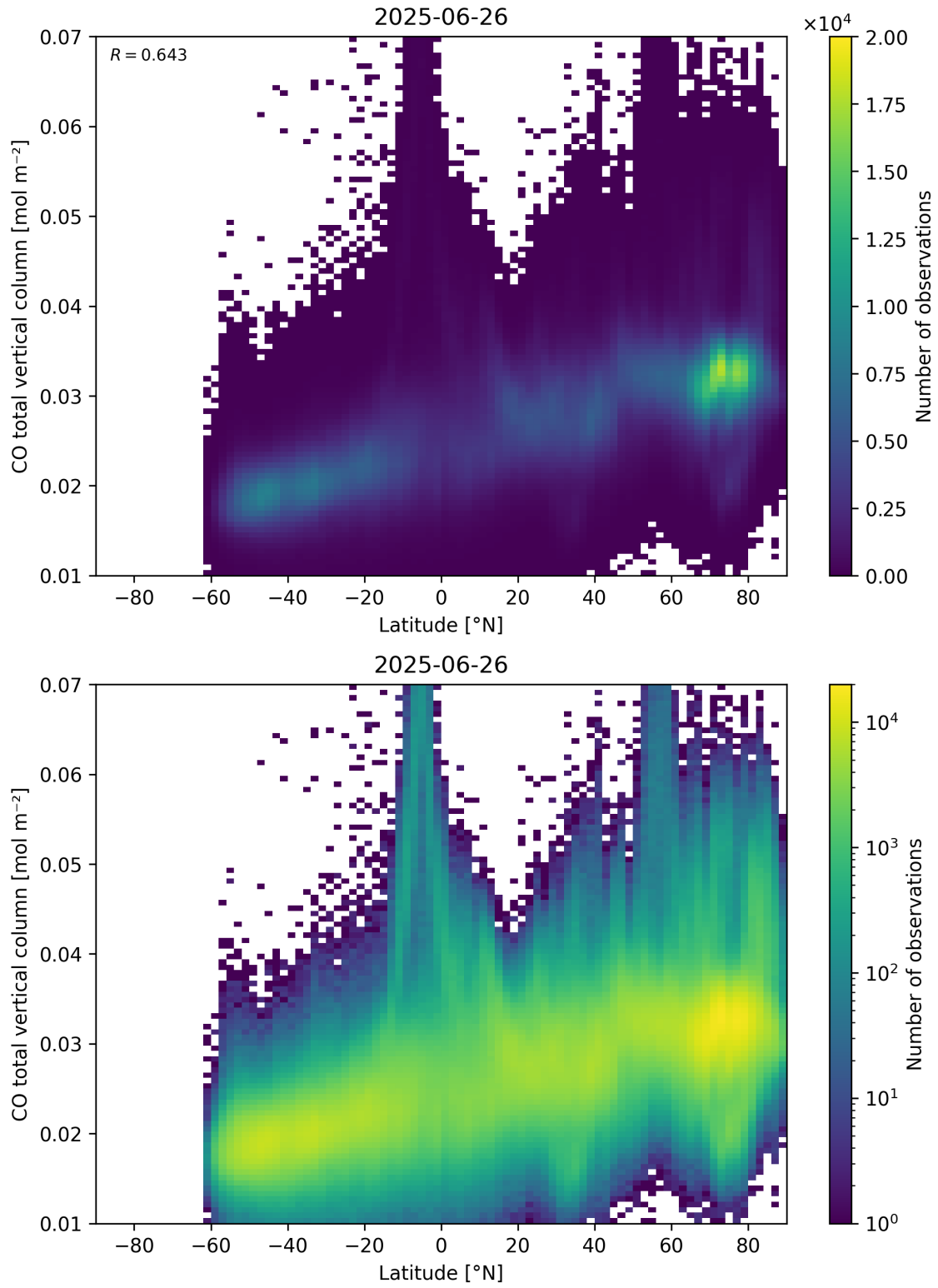
Figure 51: Scatter density plot of “Latitude” against “CO total vertical column” for 2025-06-25 to 2025-06-27.
