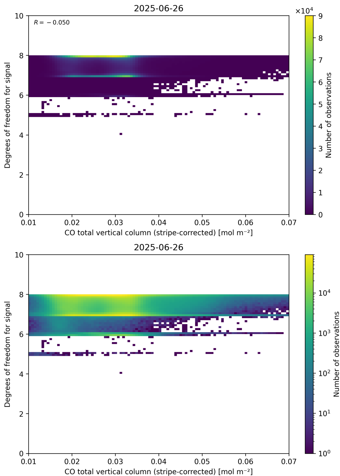
Figure 38: Scatter density plot of “CO total vertical column (stripe-corrected)” against “Degrees of freedom for signal” for 2025-06-25 to 2025-06-27.
