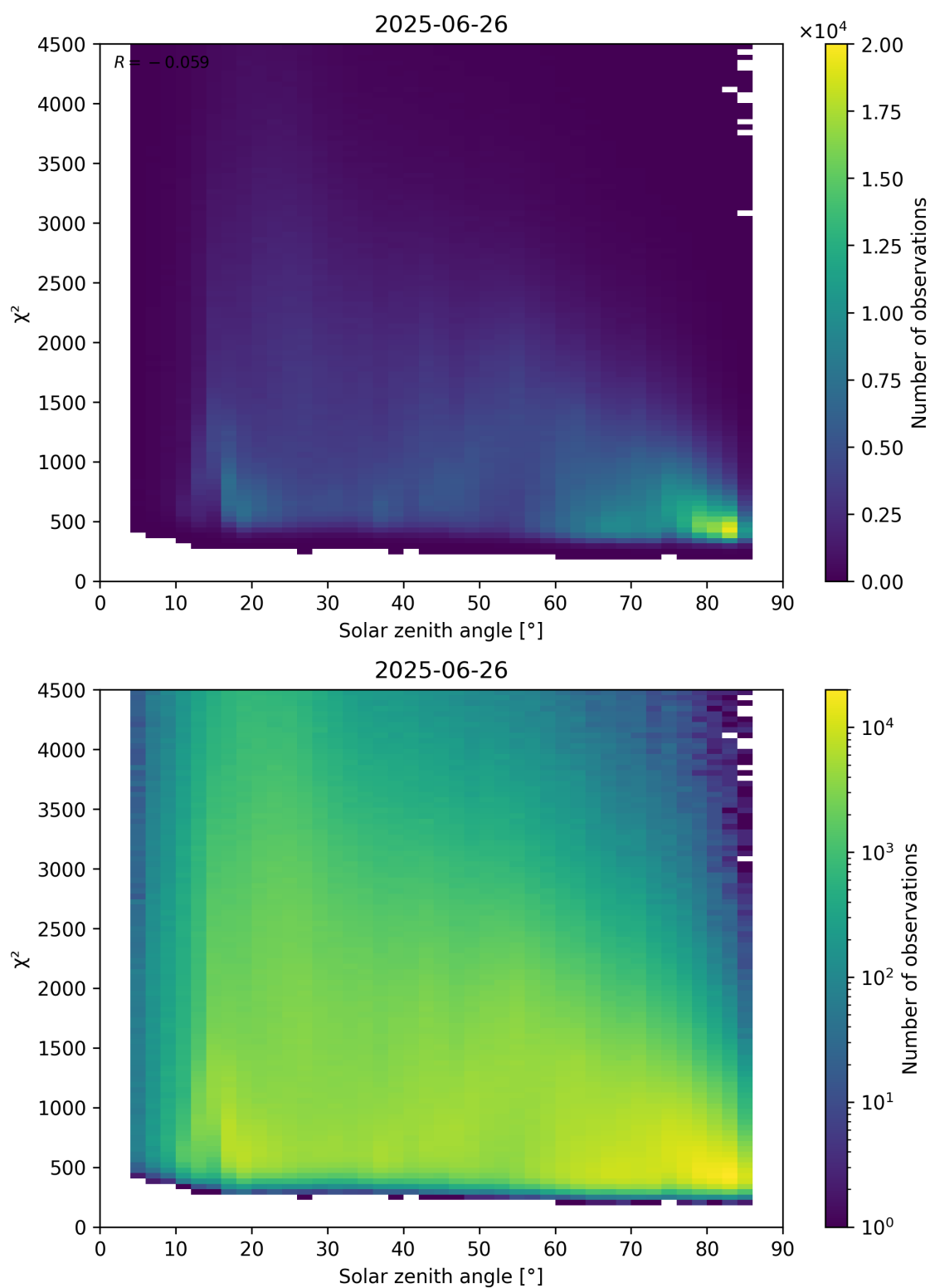
Figure 64: Scatter density plot of “Solar zenith angle” against “ \chi^2 ” for 2025-06-25 to 2025-06-27.
