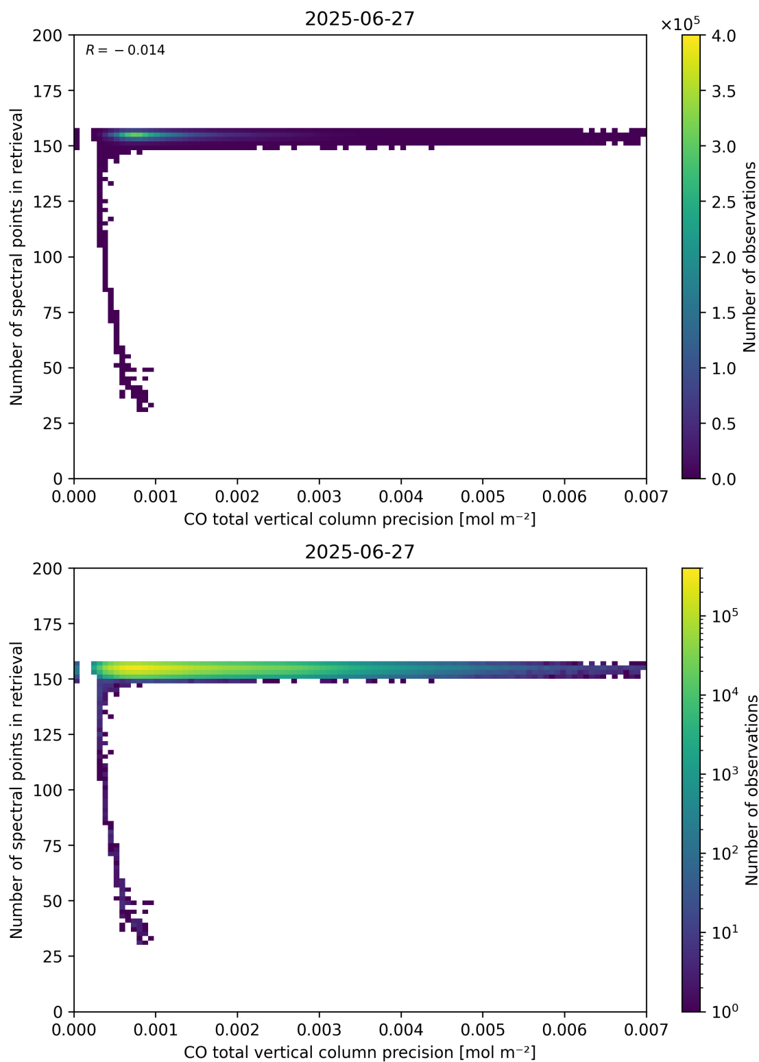
Figure 47: Scatter density plot of “CO total vertical column precision” against “Number of spectral points in retrieval” for 2025-06-27 to 2025-06-28.
