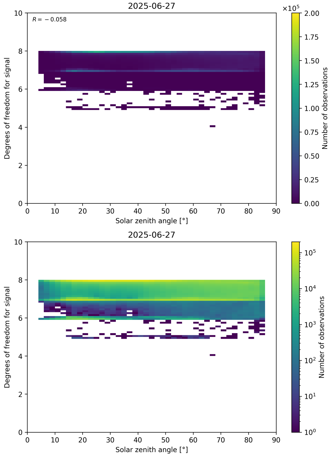
Figure 65: Scatter density plot of “Solar zenith angle” against “Degrees of freedom for signal” for 2025-06-27 to 2025-06-28.
