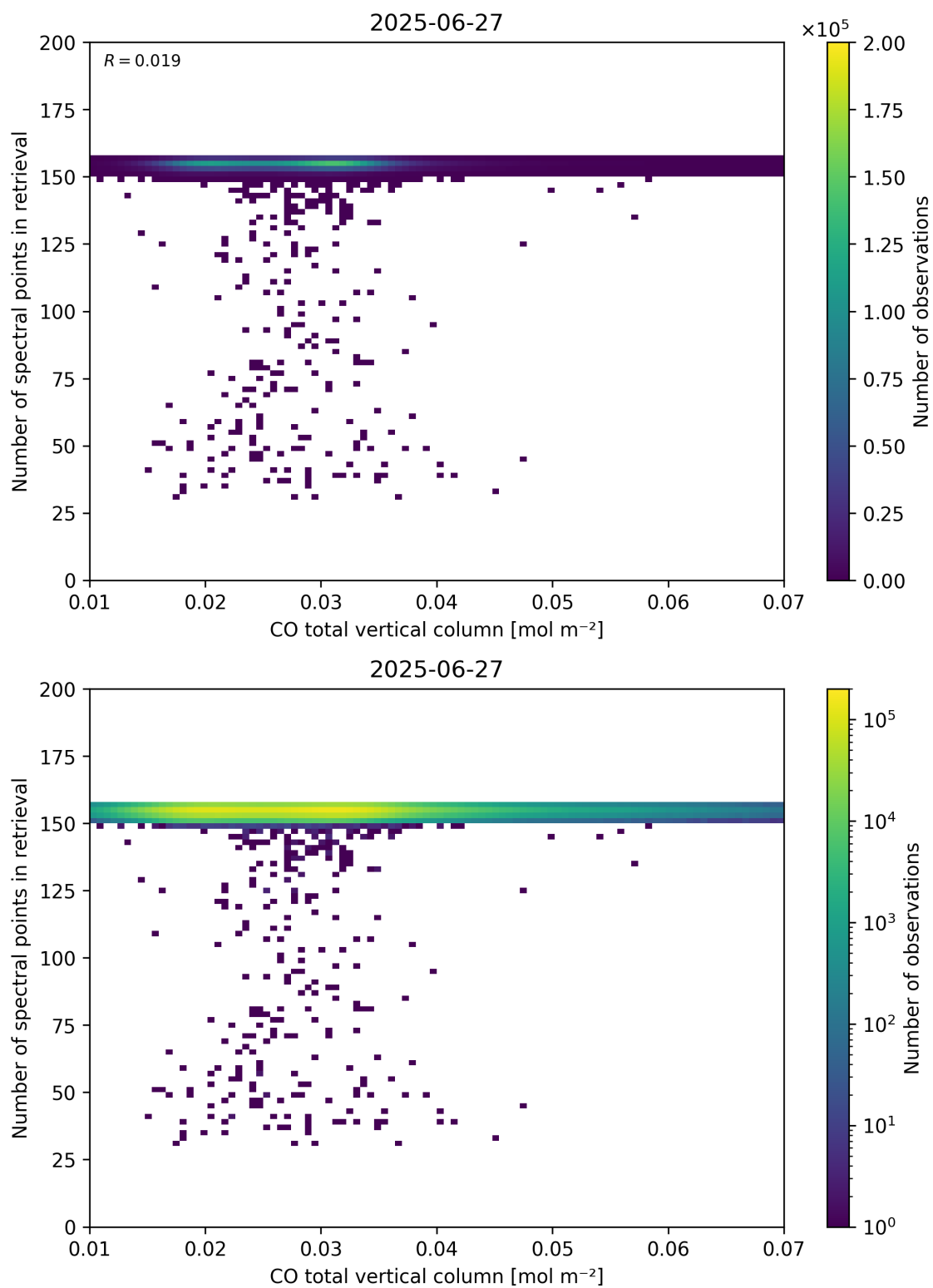
Figure 43: Scatter density plot of “CO total vertical column” against “Number of spectral points in retrieval” for 2025-06-27 to 2025-06-28.
