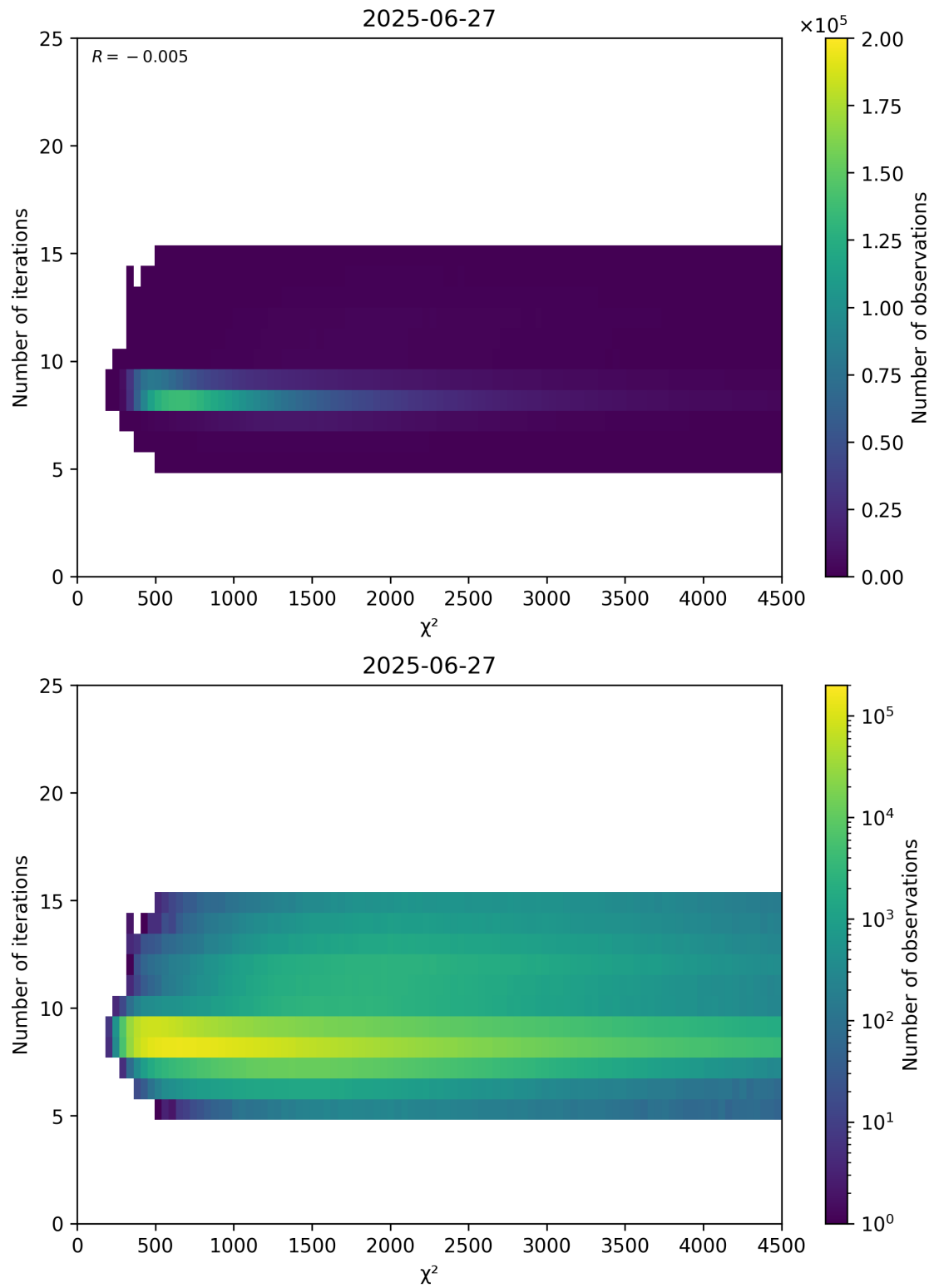
Figure 49: Scatter density plot of “ \chi^2 ” against “Number of iterations” for 2025-06-27 to 2025-06-28.
