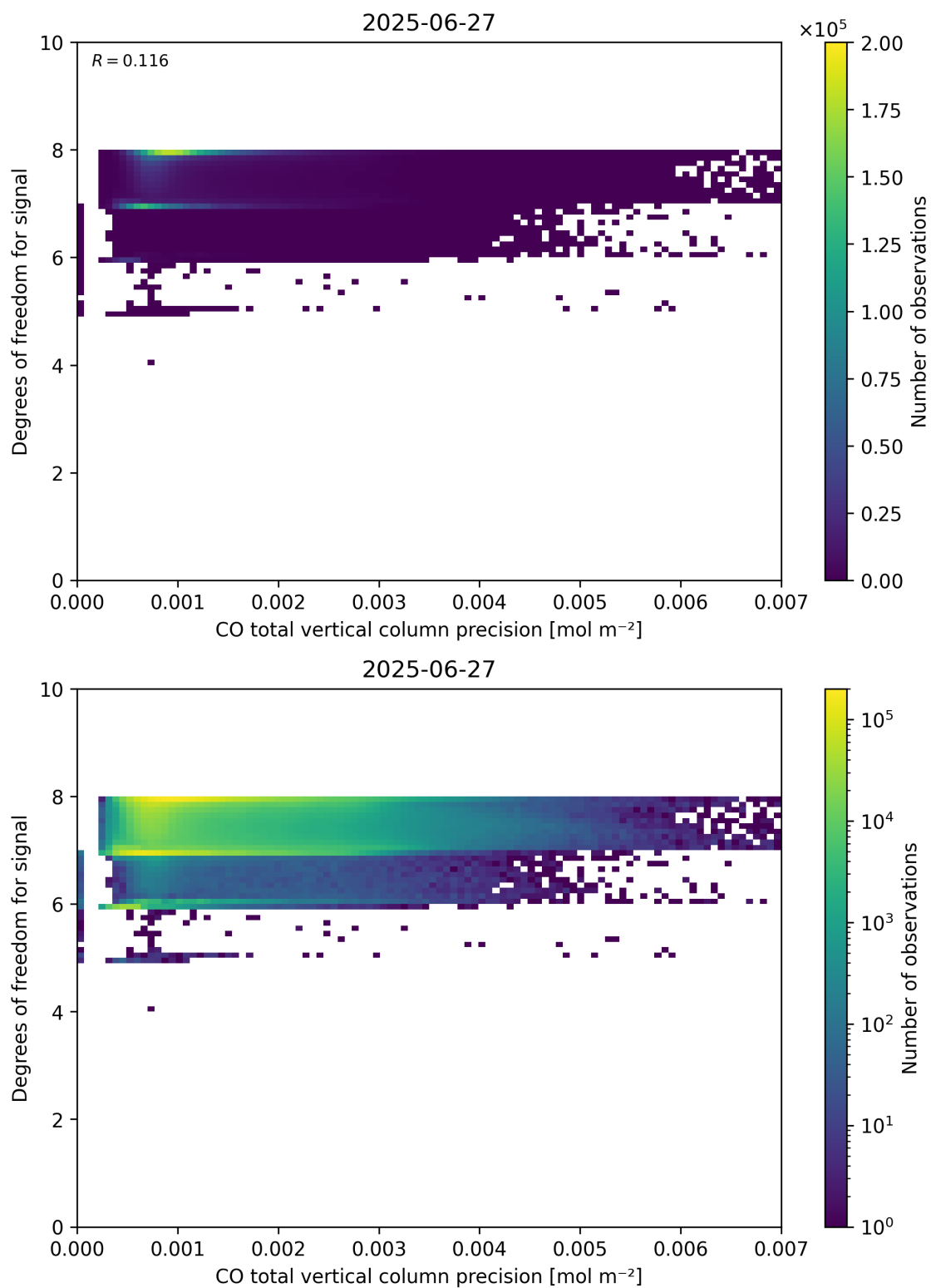
Figure 45: Scatter density plot of “CO total vertical column precision” against “Degrees of freedom for signal” for 2025-06-27 to 2025-06-28.
