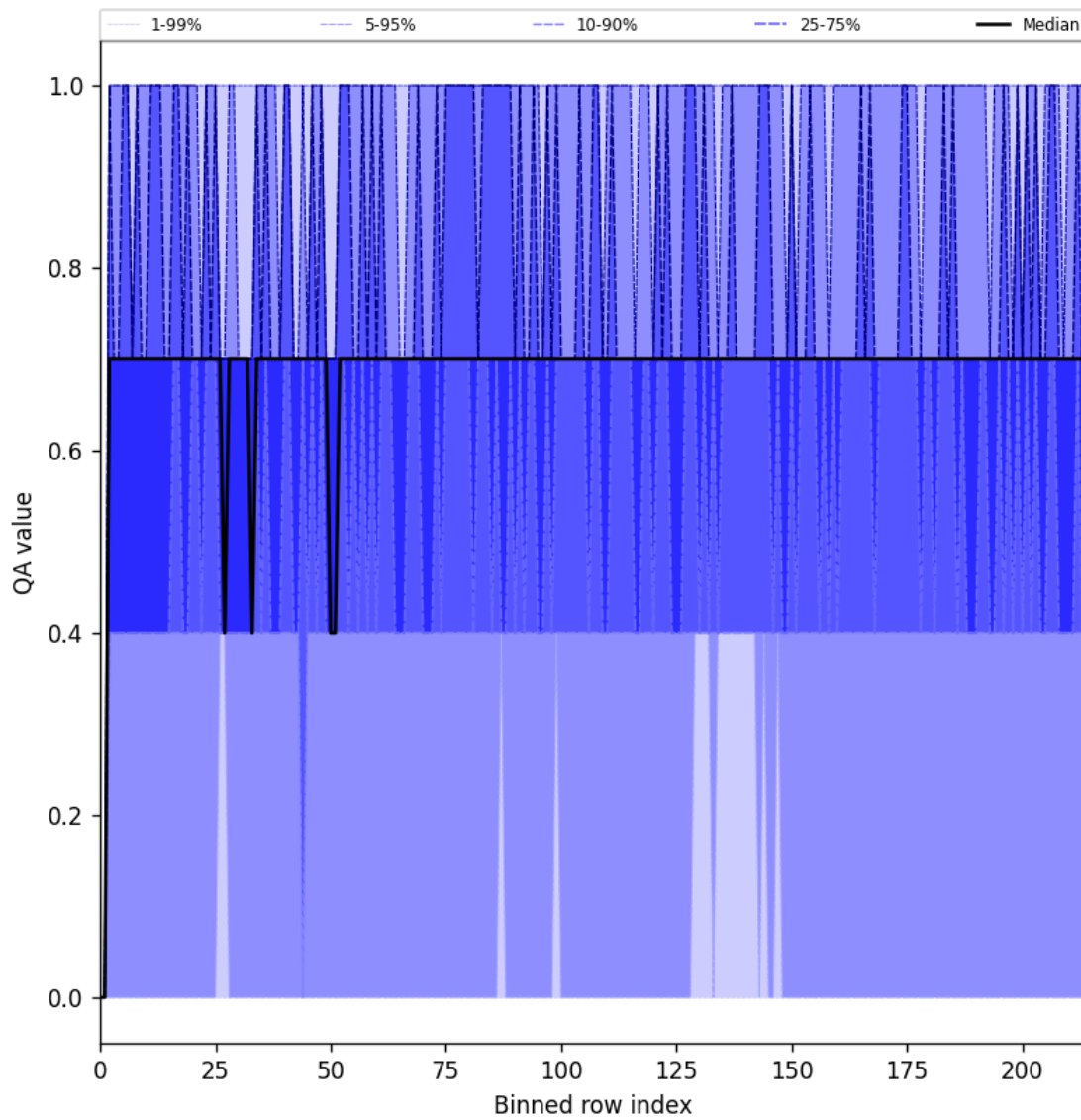
Figure 25: Along track statistics of “QA value” for 2025-06-27 to 2025-06-28
