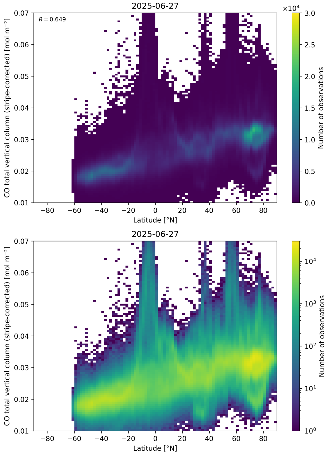
Figure 52: Scatter density plot of “Latitude” against “CO total vertical column (stripe-corrected)” for 2025-06-27 to 2025-06-28.
