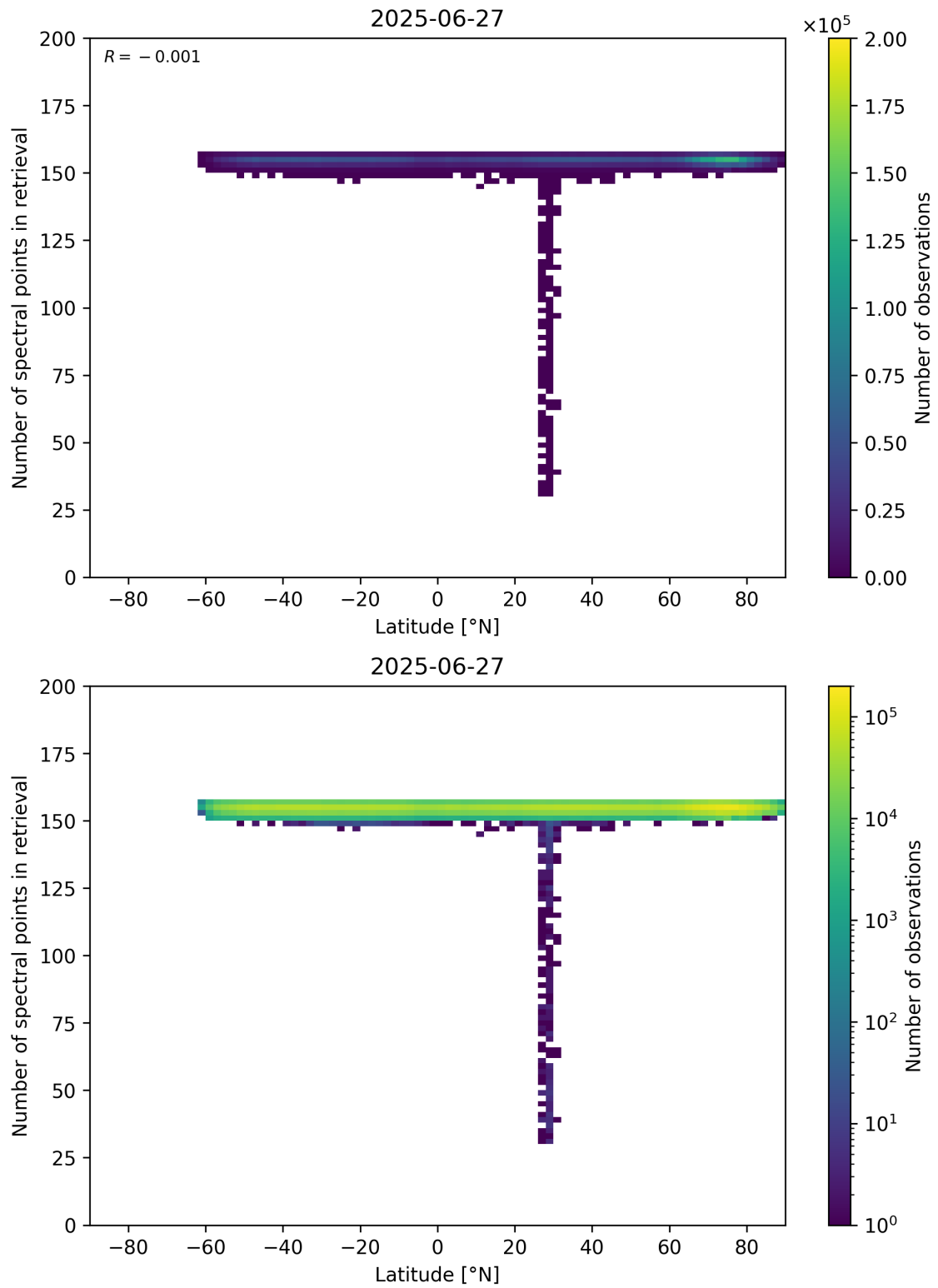
Figure 57: Scatter density plot of “Latitude” against “Number of spectral points in retrieval” for 2025-06-27 to 2025-06-28.
