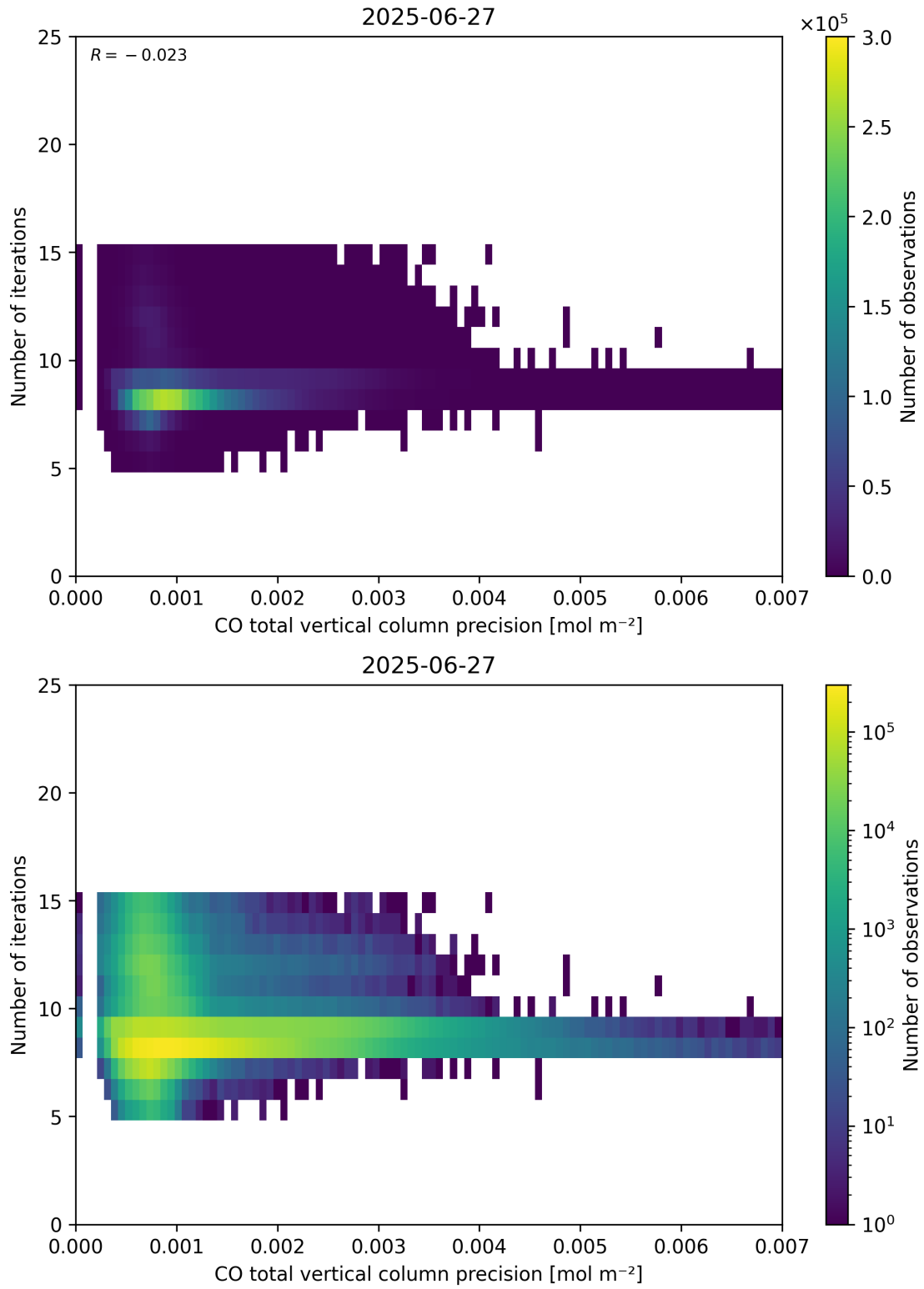
Figure 46: Scatter density plot of “CO total vertical column precision” against “Number of iterations” for 2025-06-27 to 2025-06-28.
