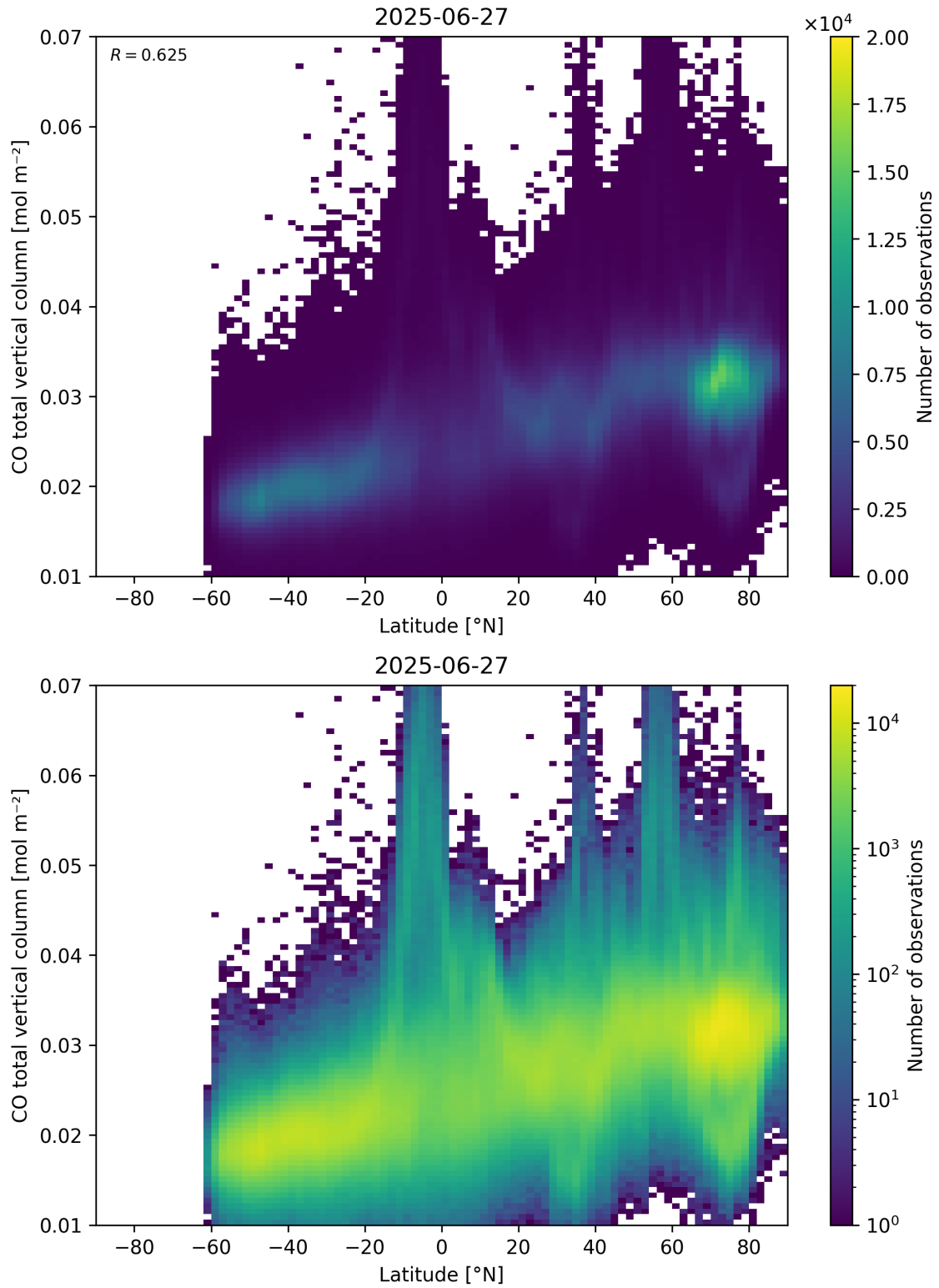
Figure 51: Scatter density plot of “Latitude” against “CO total vertical column” for 2025-06-27 to 2025-06-28.
