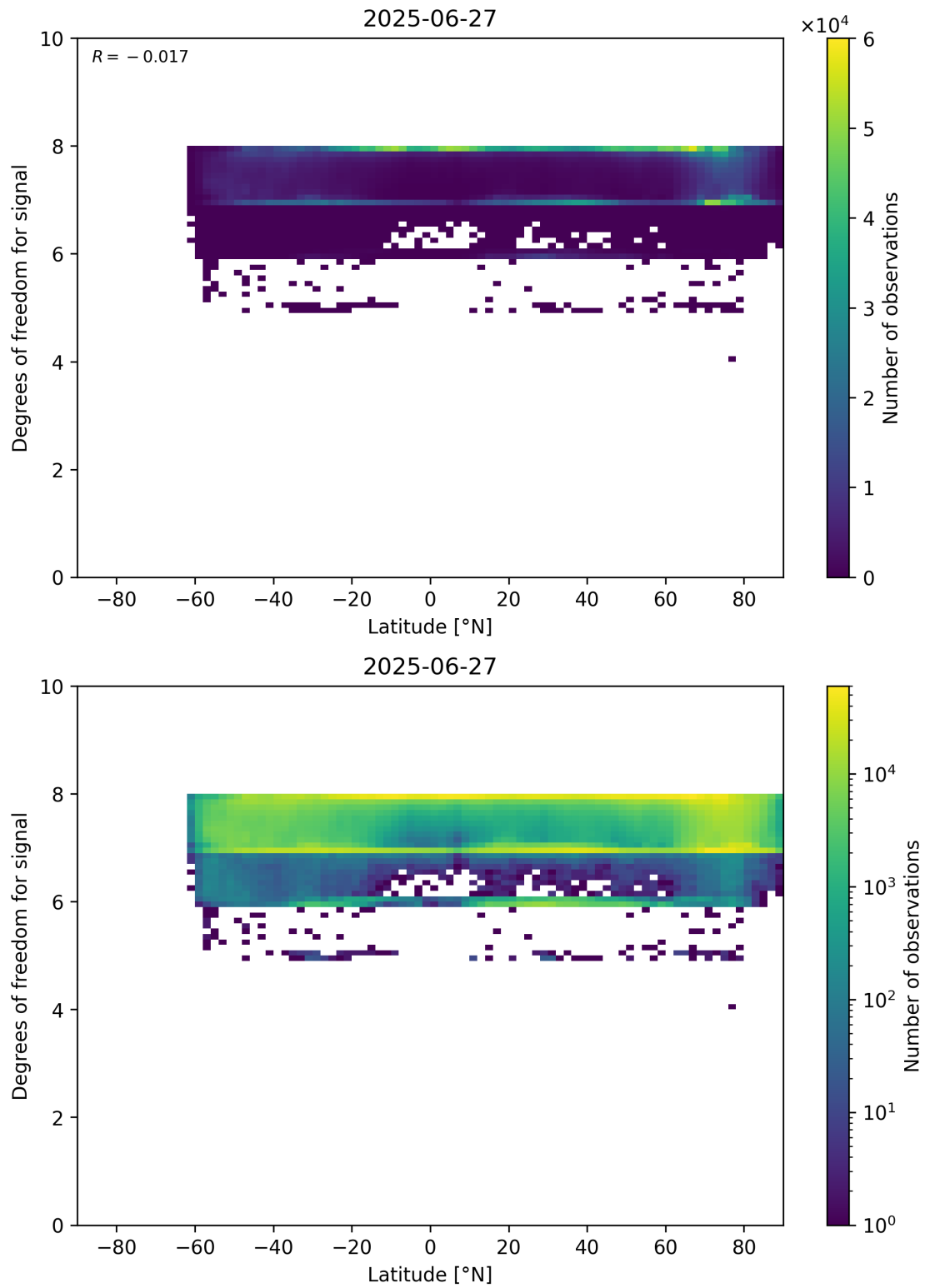
Figure 55: Scatter density plot of “Latitude” against “Degrees of freedom for signal” for 2025-06-27 to 2025-06-28.
