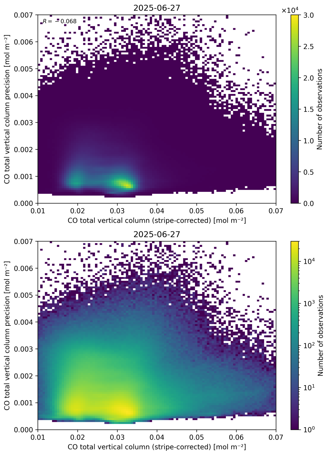
Figure 36: Scatter density plot of “CO total vertical column (stripe-corrected)” against “CO total vertical column precision” for 2025-06-27 to 2025-06-28.
