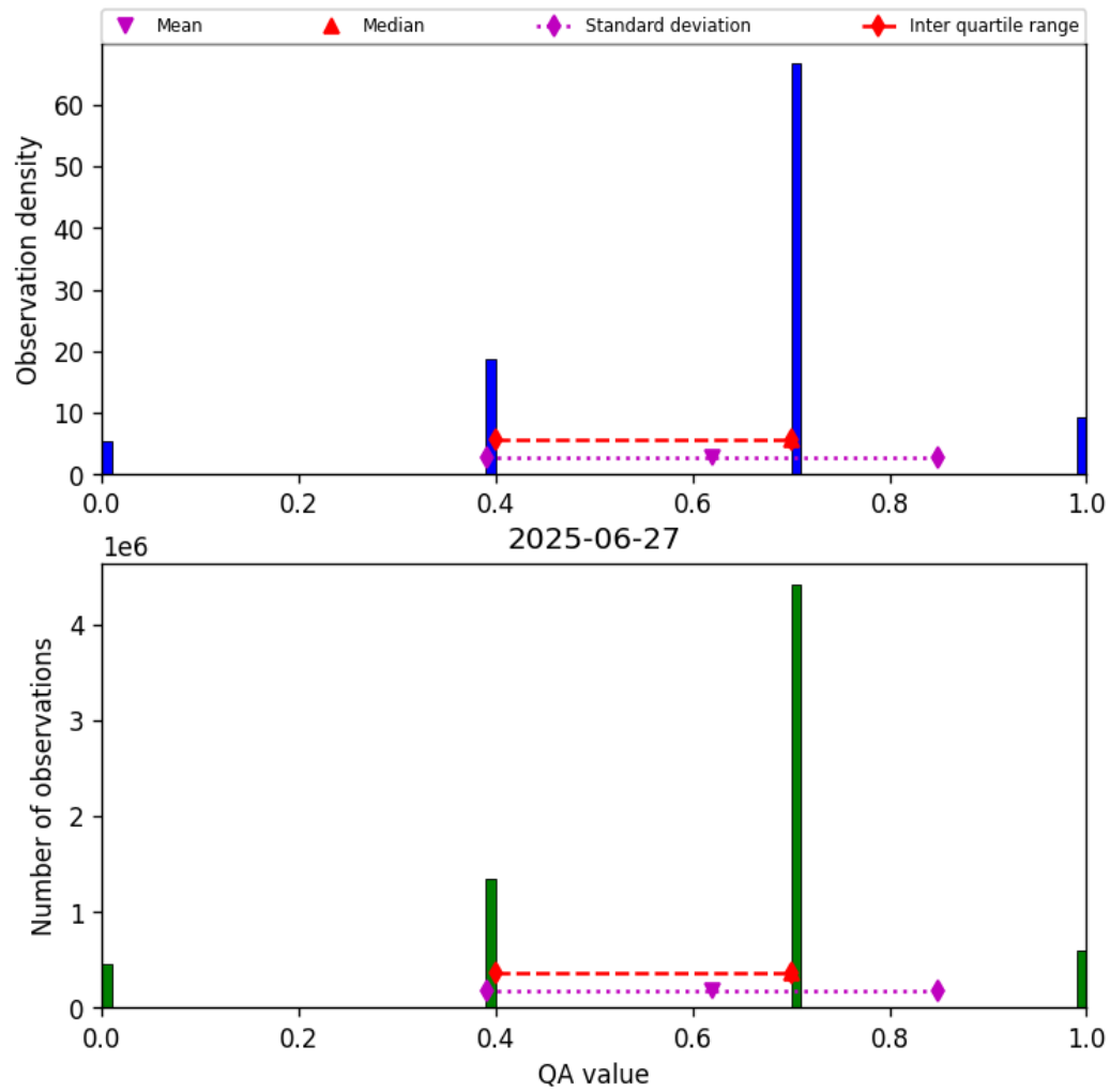
Figure 17: Histogram of “QA value” for 2025-06-27 to 2025-06-28
