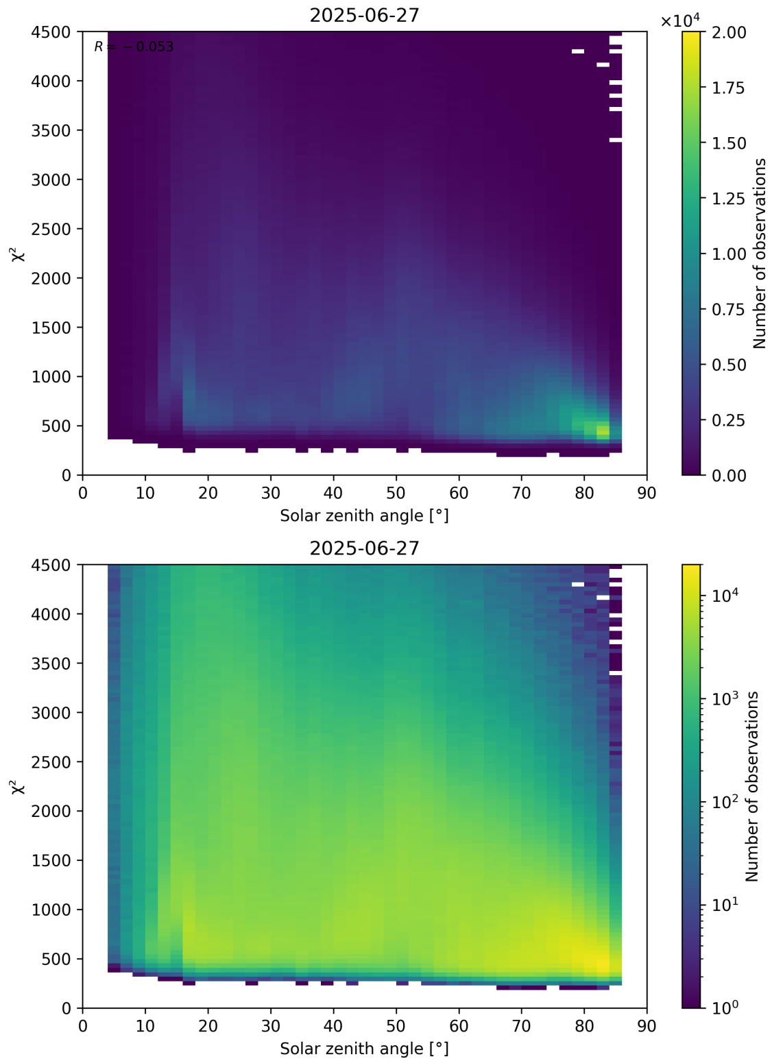
Figure 64: Scatter density plot of “Solar zenith angle” against “ \chi^2 ” for 2025-06-27 to 2025-06-28.
