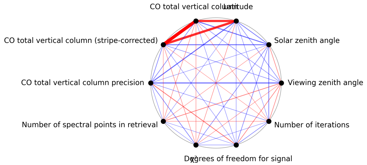
Figure 1: Map of correlation graph for 2025-06-27 to 2025-06-28.
