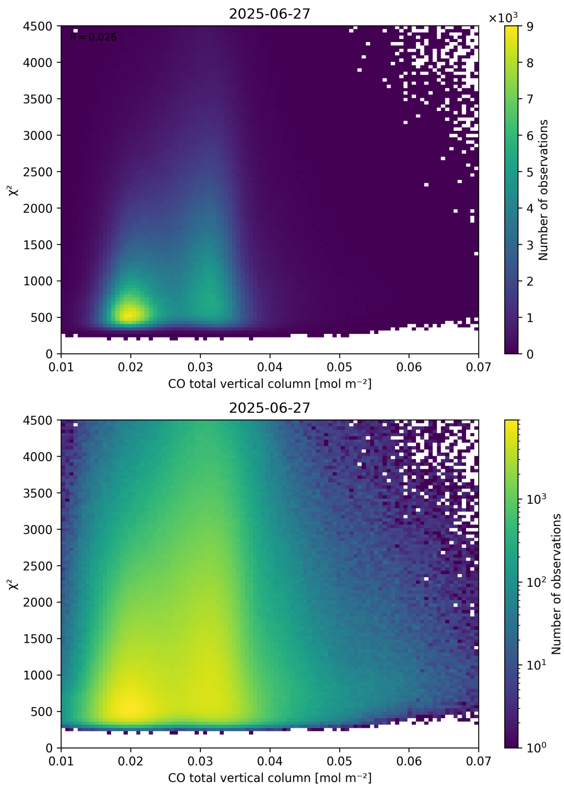
Figure 35: Scatter density plot of “CO total vertical column” against “ \chi^2 ” for 2025-06-27 to 2025-06-28.
