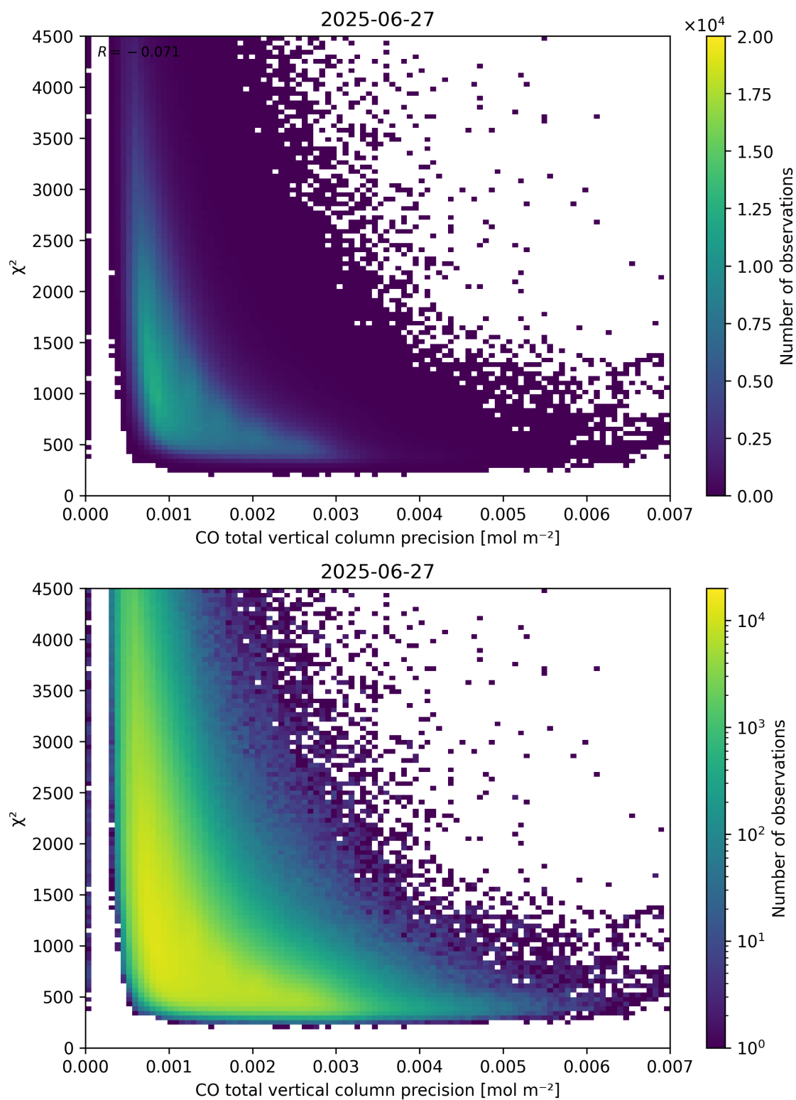
Figure 44: Scatter density plot of “CO total vertical column precision” against “ \chi^2 ” for 2025-06-27 to 2025-06-28.
