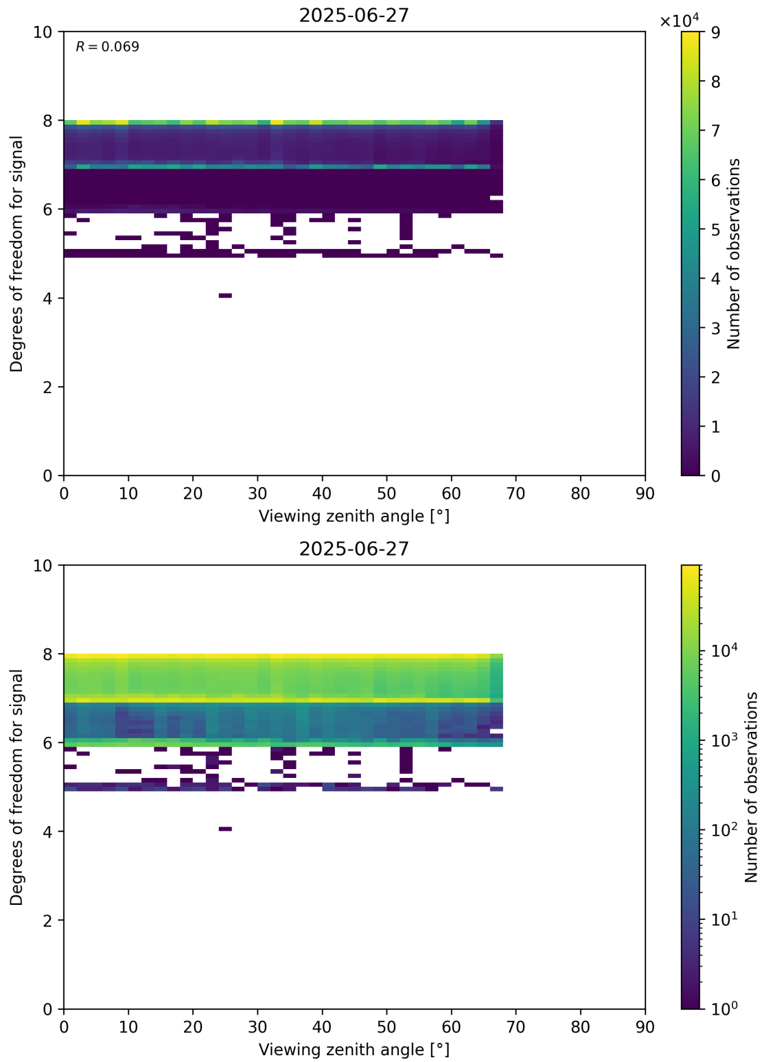
Figure 73: Scatter density plot of “Viewing zenith angle” against “Degrees of freedom for signal” for 2025-06-27 to 2025-06-28.
