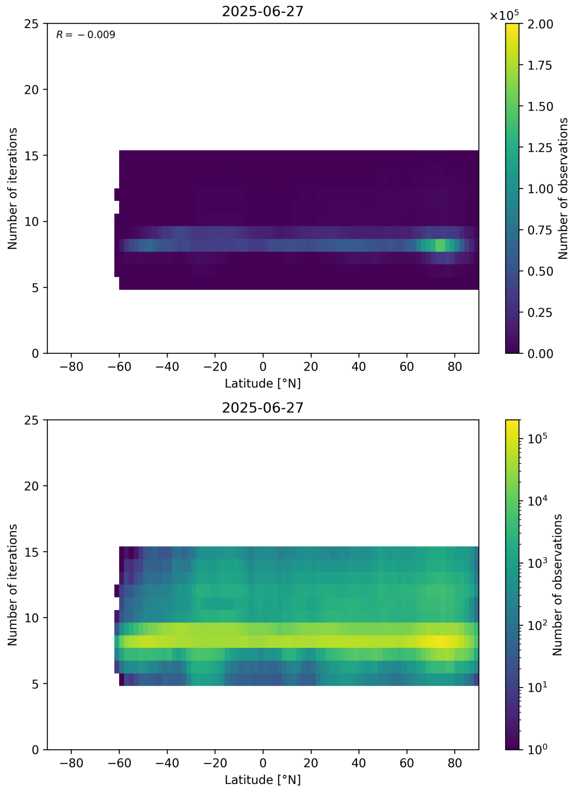
Figure 56: Scatter density plot of “Latitude” against “Number of iterations” for 2025-06-27 to 2025-06-28.
