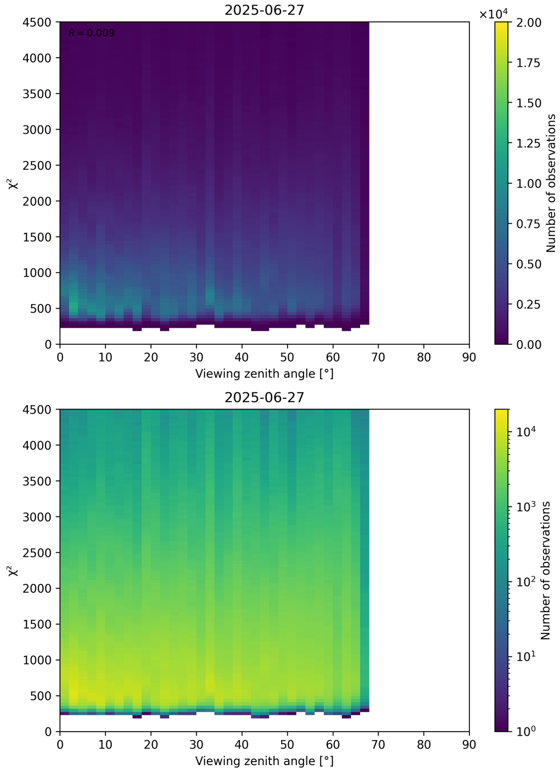
Figure 72: Scatter density plot of “Viewing zenith angle” against “ \chi^2 ” for 2025-06-27 to 2025-06-28.
