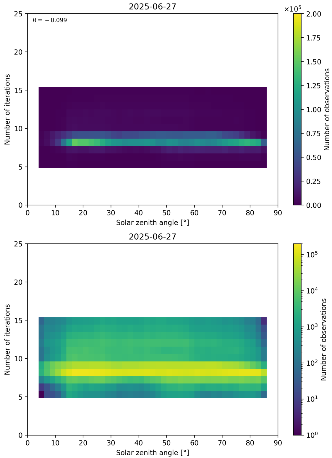
Figure 67: Scatter density plot of “Solar zenith angle” against “Number of iterations” for 2025-06-27 to 2025-06-28.
