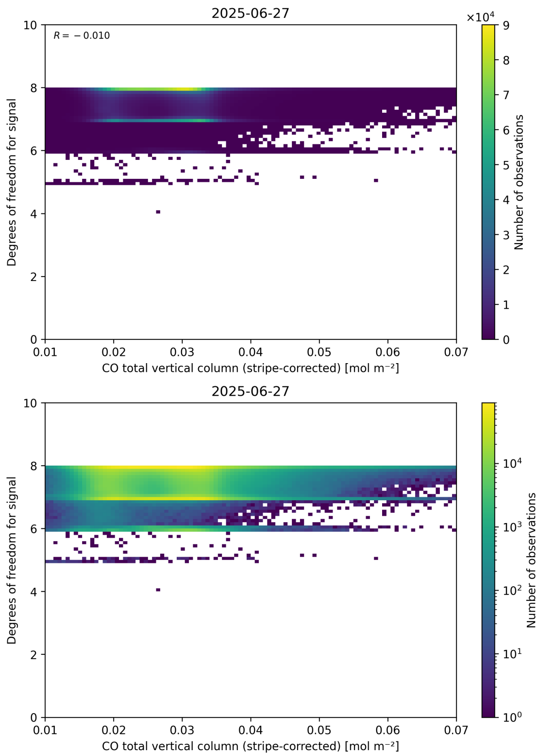
Figure 38: Scatter density plot of “CO total vertical column (stripe-corrected)” against “Degrees of freedom for signal” for 2025-06-27 to 2025-06-28.
