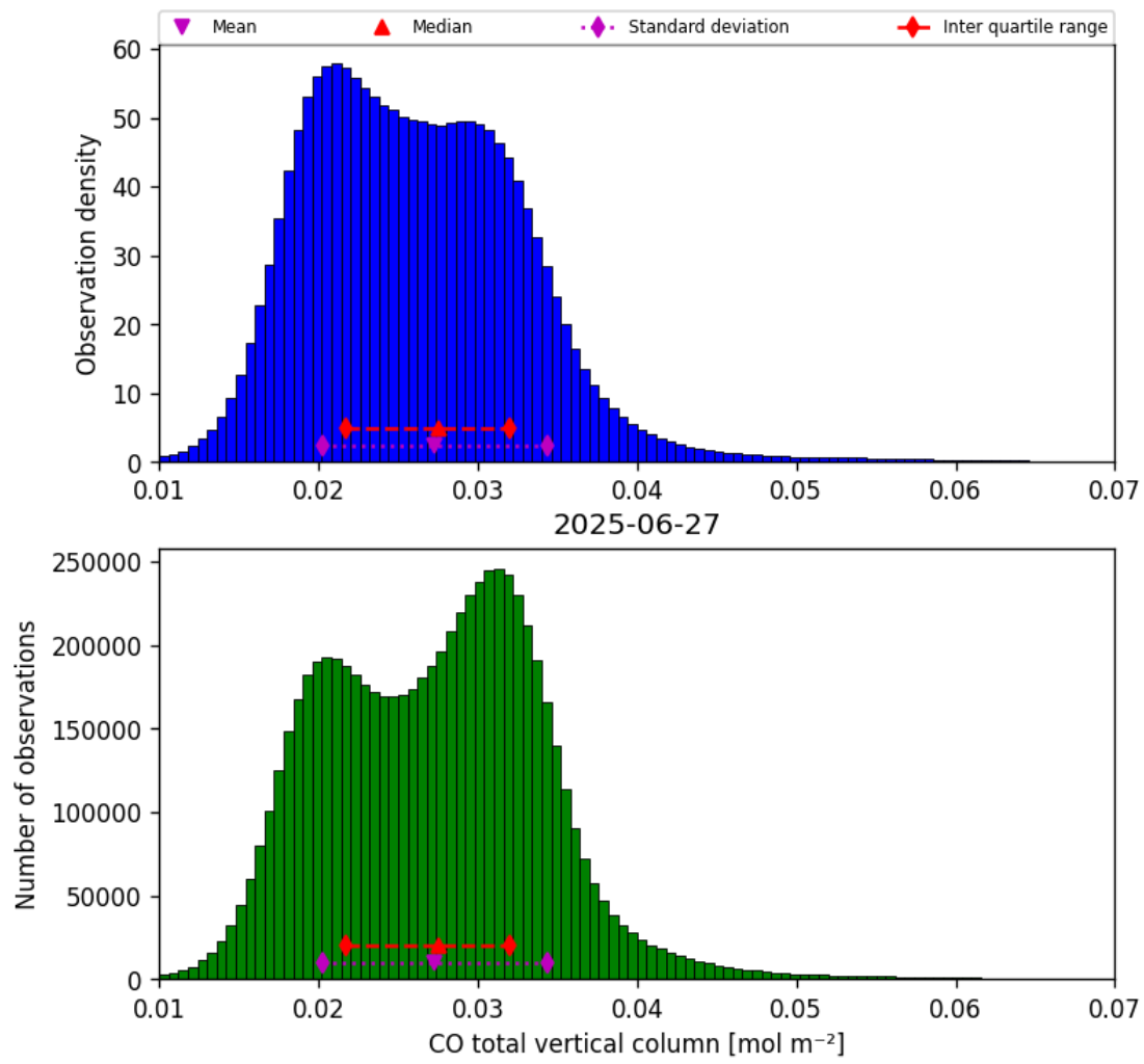
Figure 18: Histogram of “CO total vertical column” for 2025-06-27 to 2025-06-28
