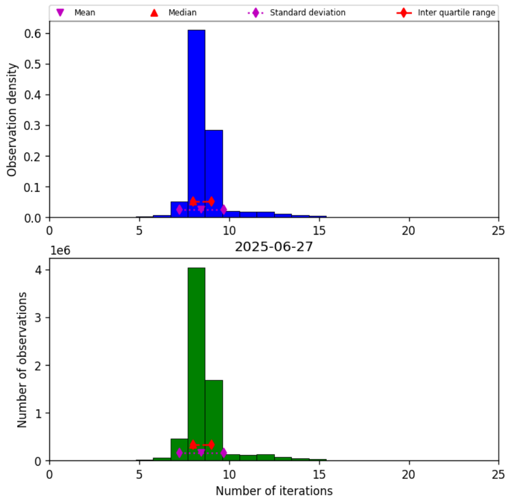
Figure 24: Histogram of “Number of iterations” for 2025-06-27 to 2025-06-28
