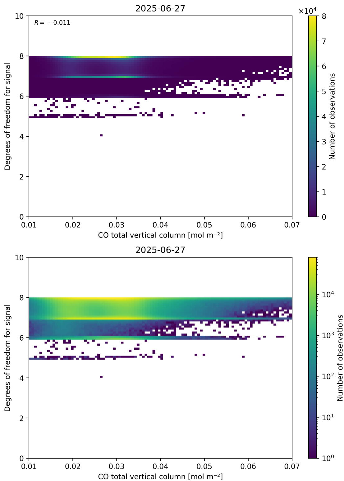
Figure 41: Scatter density plot of “CO total vertical column” against “Degrees of freedom for signal” for 2025-06-27 to 2025-06-28.
