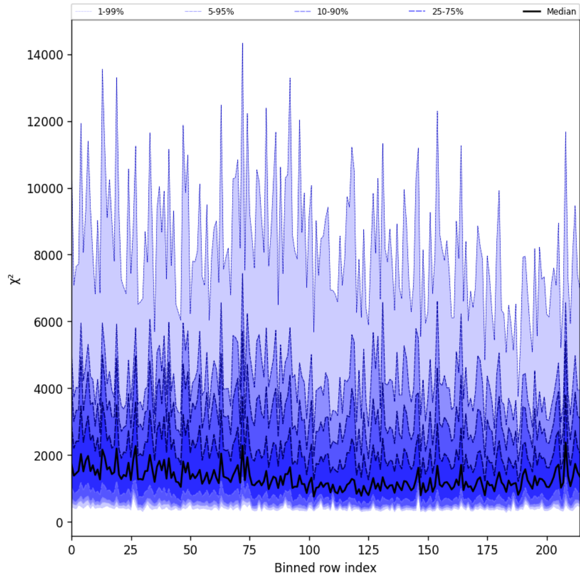
Figure 30: Along track statistics of “ \chi^2 ” for 2025-06-27 to 2025-06-28
