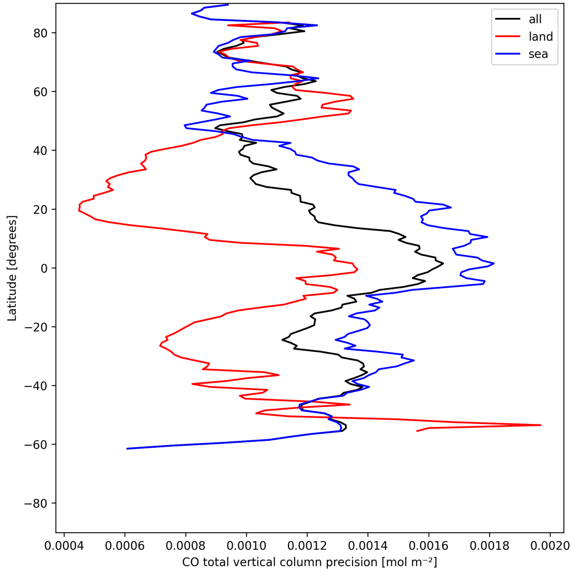
Figure 12: Zonal average of “CO total vertical column precision” for 2025-06-27 to 2025-06-28.
