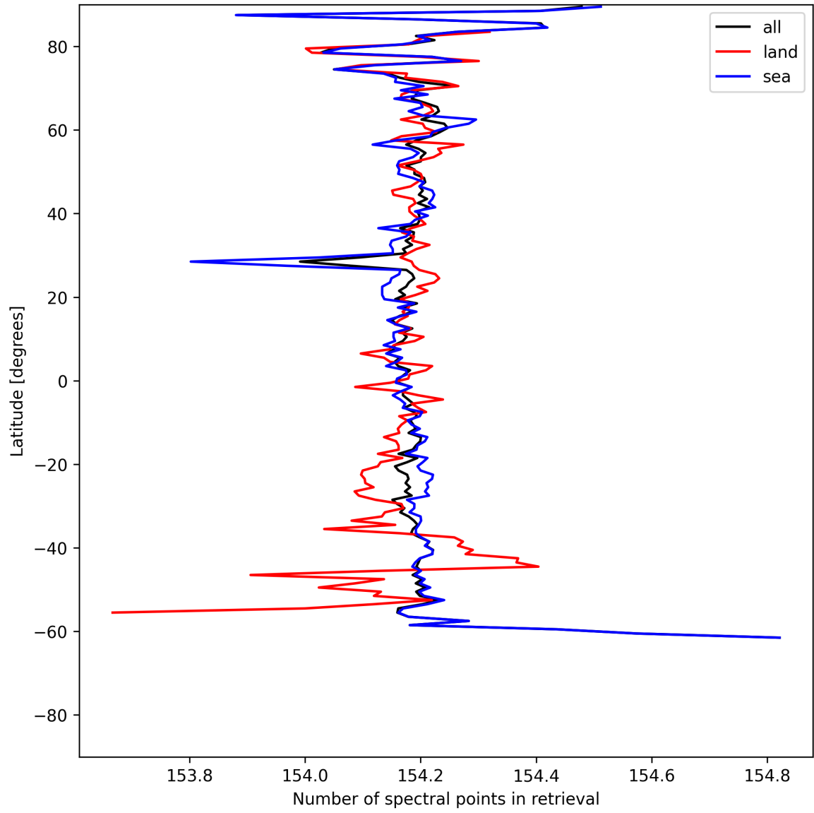
Figure 13: Zonal average of “Number of spectral points in retrieval” for 2025-06-27 to 2025-06-28.
