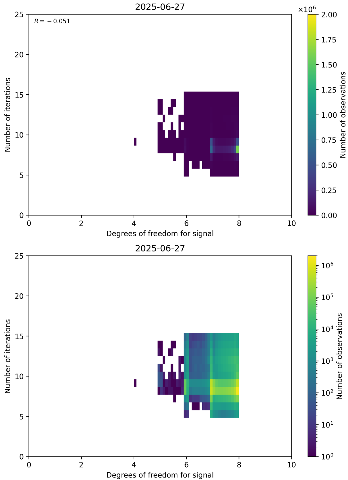
Figure 50: Scatter density plot of “Degrees of freedom for signal” against “Number of iterations” for 2025-06-27 to 2025-06-28.
