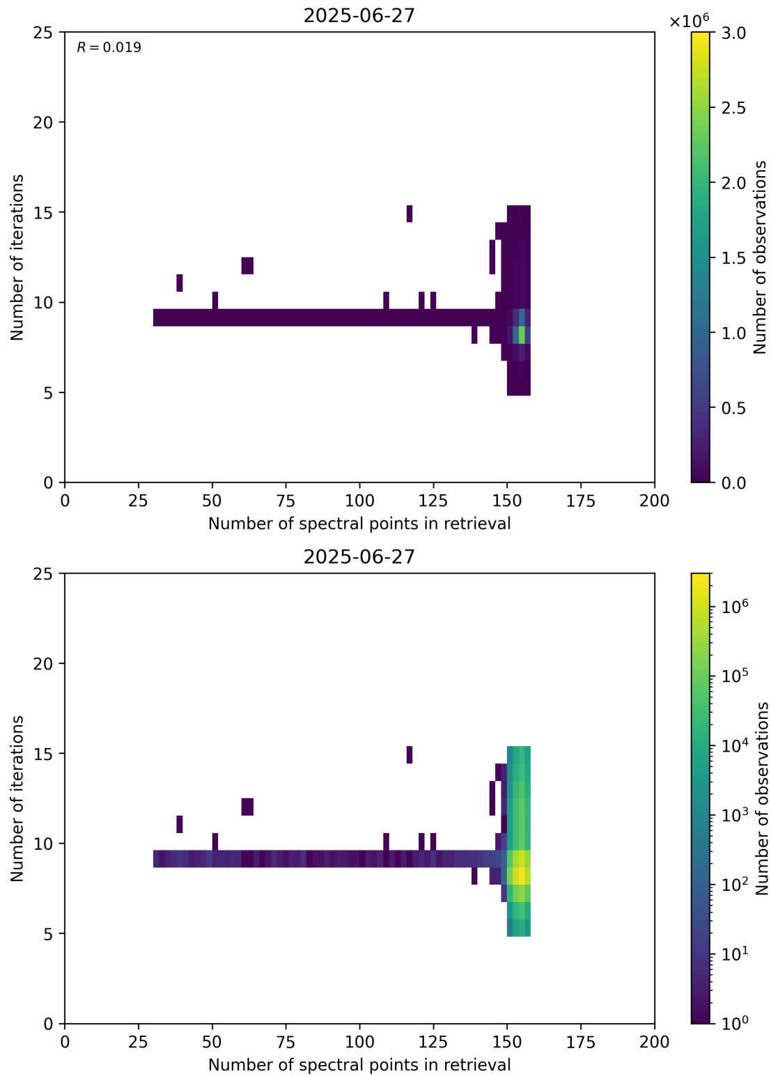
Figure 60: Scatter density plot of “Number of spectral points in retrieval” against “Number of iterations” for 2025-06-27 to 2025-06-28.
