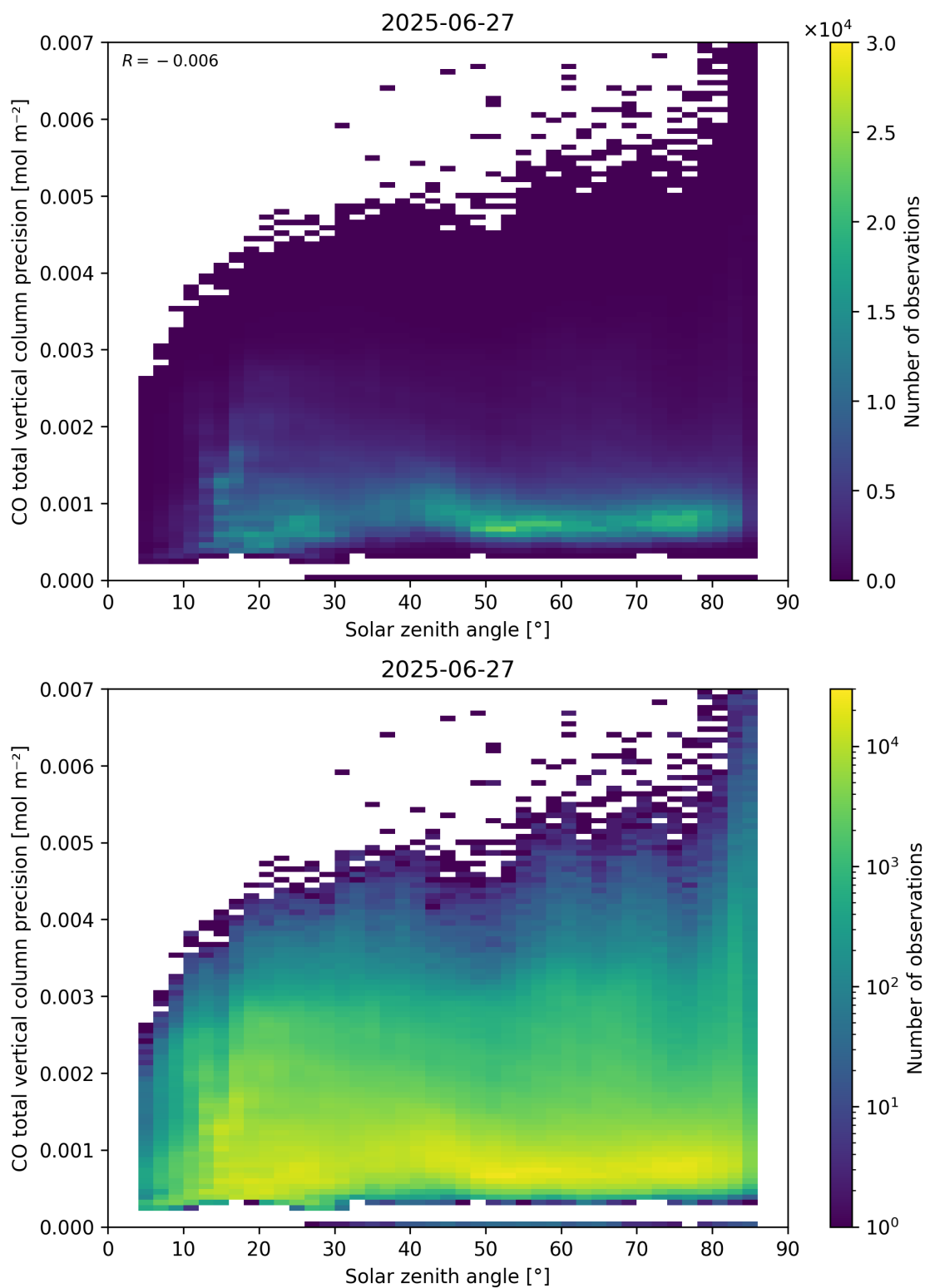
Figure 63: Scatter density plot of “Solar zenith angle” against “CO total vertical column precision” for 2025-06-27 to 2025-06-28.
