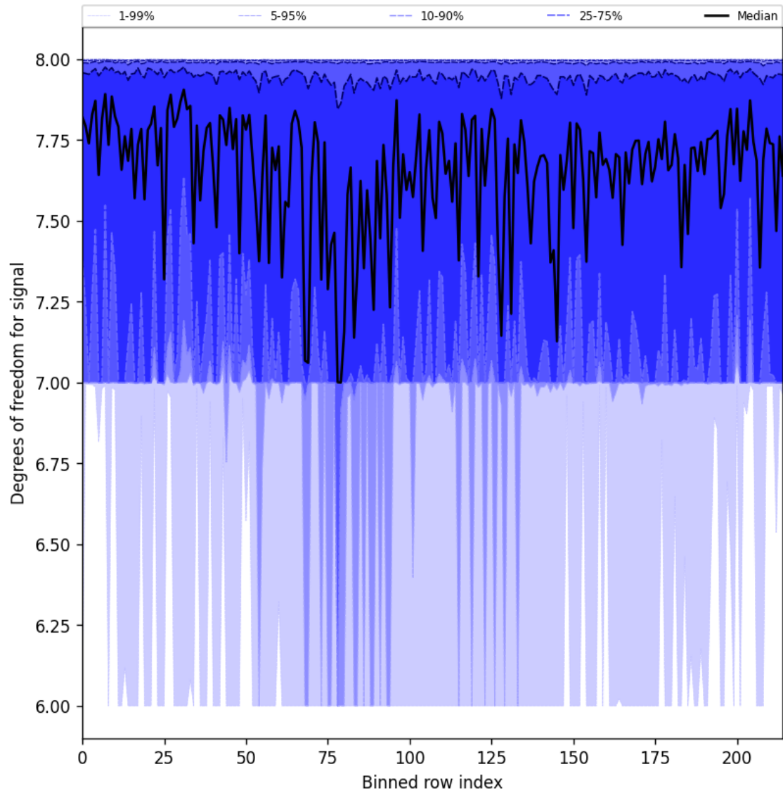
Figure 31: Along track statistics of “Degrees of freedom for signal” for 2025-06-27 to 2025-06-28
