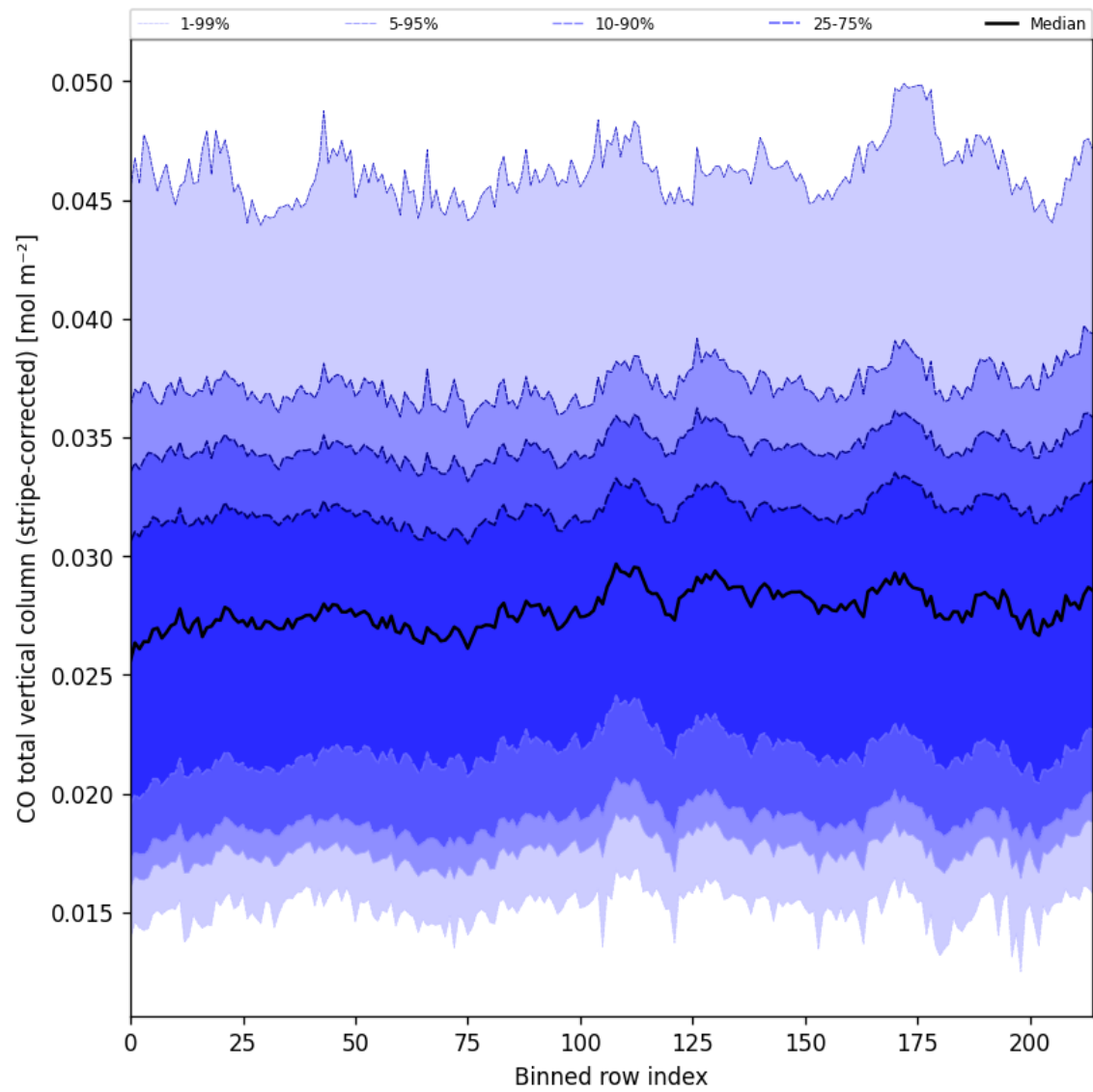
Figure 27: Along track statistics of “CO total vertical column (stripe-corrected)” for 2025-06-27 to 2025-06-28
