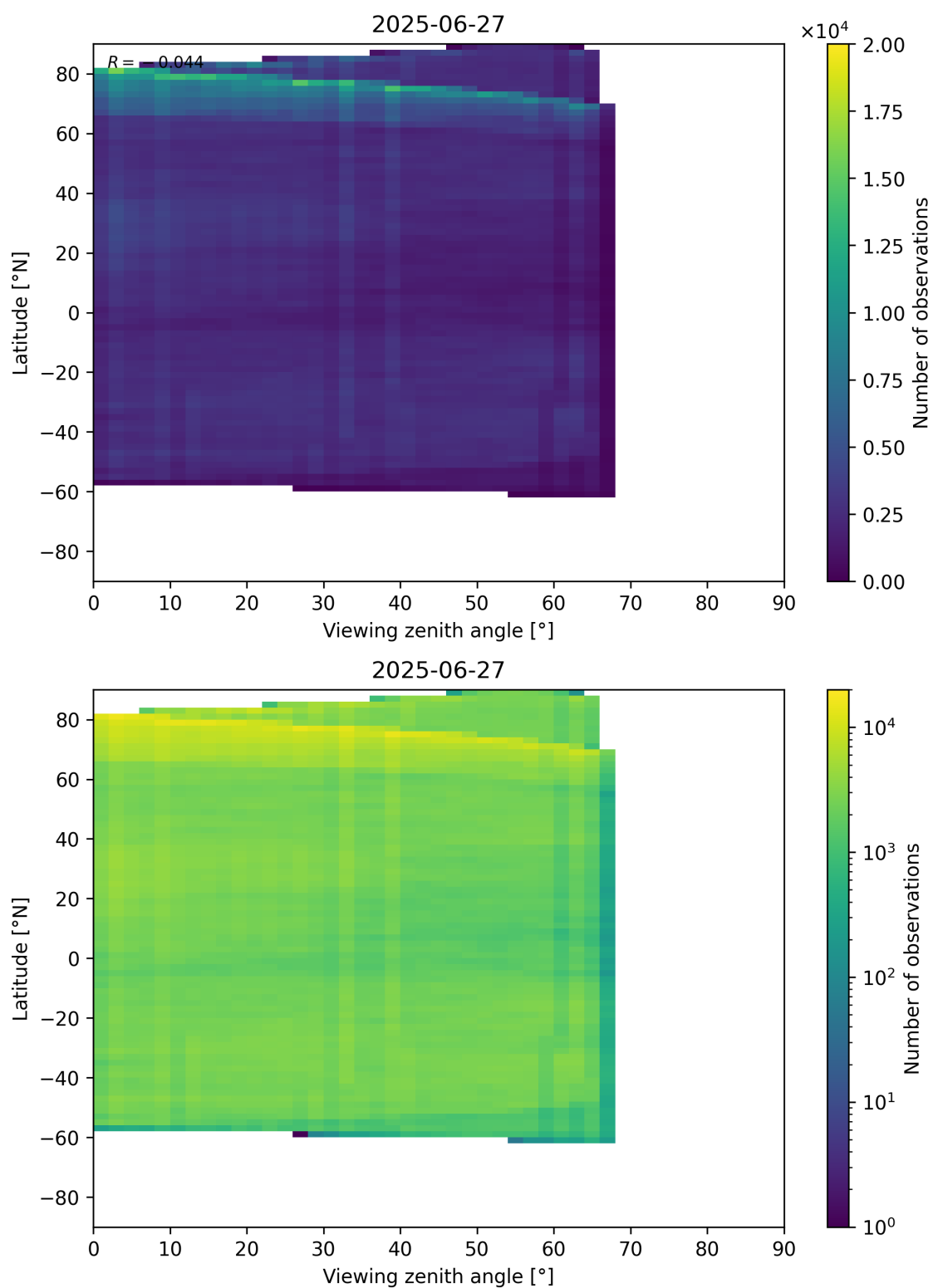
Figure 74: Scatter density plot of “Viewing zenith angle” against “Latitude” for 2025-06-27 to 2025-06-28.
