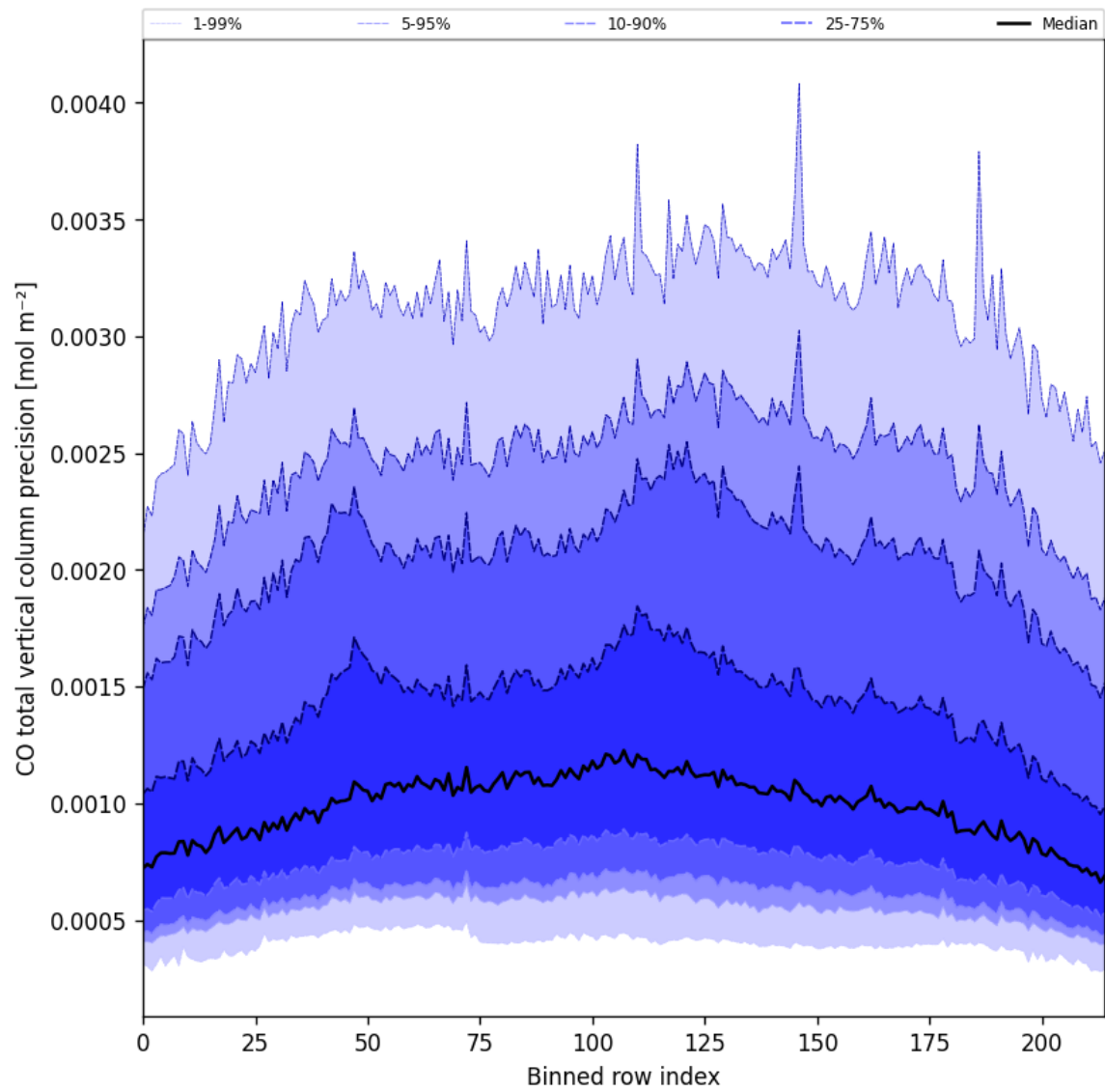
Figure 28: Along track statistics of “CO total vertical column precision” for 2025-06-27 to 2025-06-28
