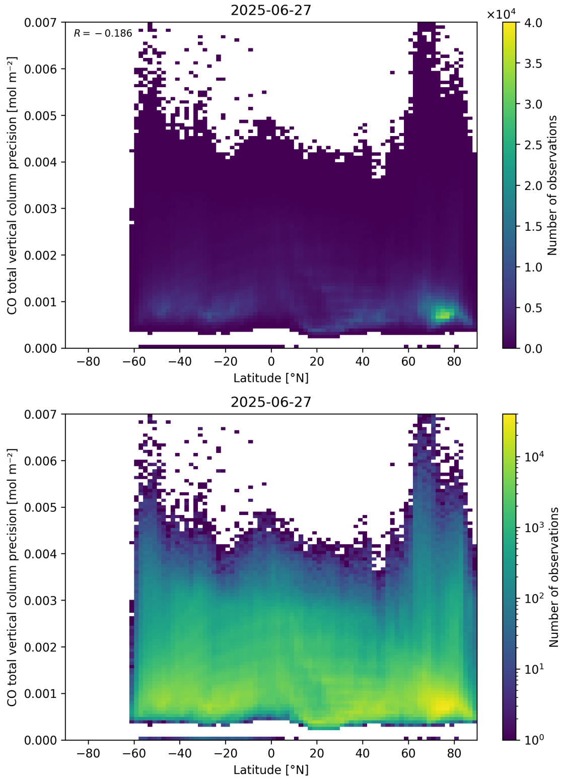
Figure 53: Scatter density plot of “Latitude” against “CO total vertical column precision” for 2025-06-27 to 2025-06-28.
