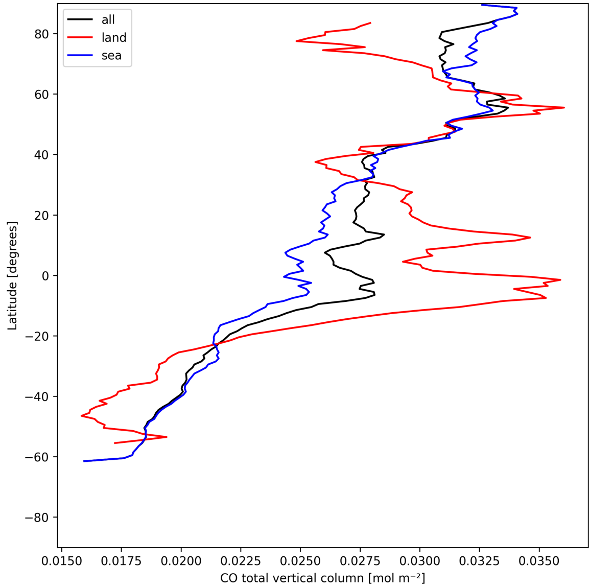
Figure 10: Zonal average of “CO total vertical column” for 2025-06-27 to 2025-06-28.
