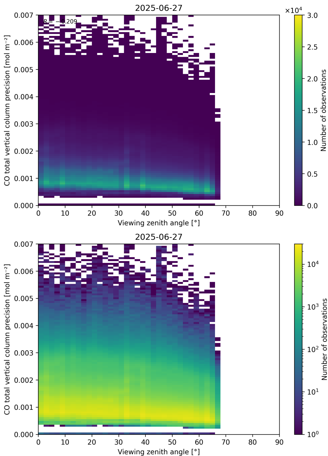
Figure 71: Scatter density plot of “Viewing zenith angle” against “CO total vertical column precision” for 2025-06-27 to 2025-06-28.
