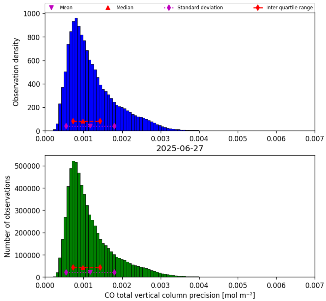
Figure 20: Histogram of “CO total vertical column precision” for 2025-06-27 to 2025-06-28
