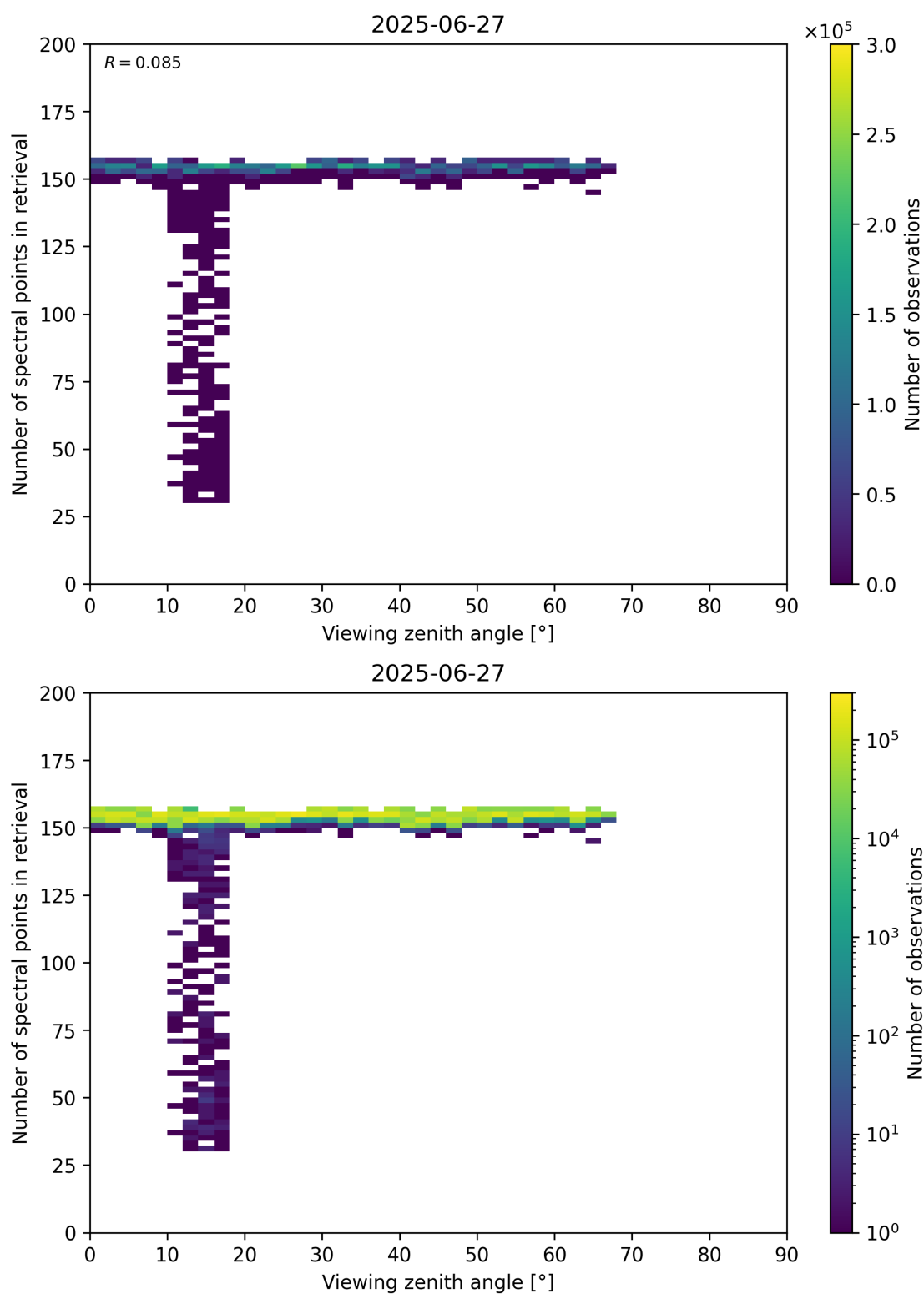
Figure 76: Scatter density plot of “Viewing zenith angle” against “Number of spectral points in retrieval” for 2025-06-27 to 2025-06-28.
