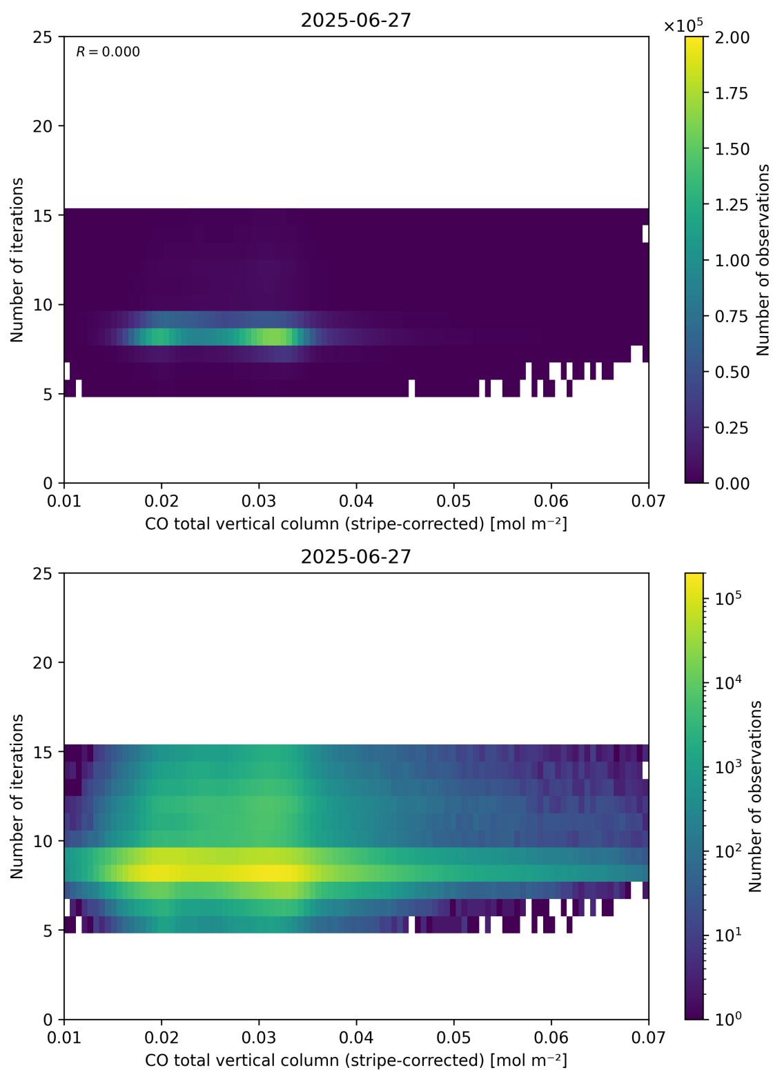
Figure 39: Scatter density plot of “CO total vertical column (stripe-corrected)” against “Number of iterations” for 2025-06-27 to 2025-06-28.
