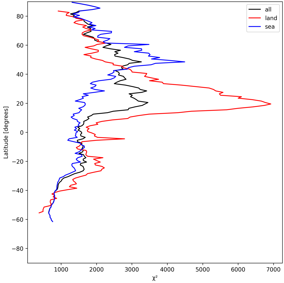
Figure 14: Zonal average of “ \chi^2 ” for 2025-06-27 to 2025-06-28.
