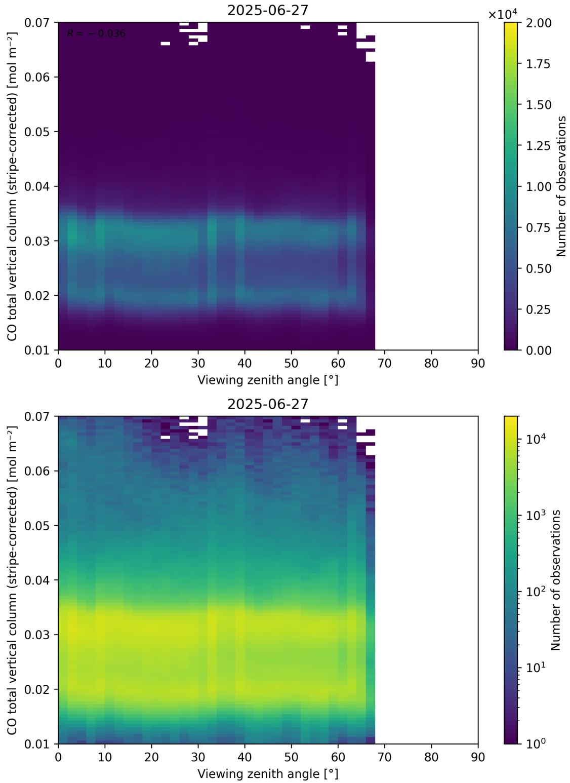
Figure 70: Scatter density plot of “Viewing zenith angle” against “CO total vertical column (stripe-corrected)” for 2025-06-27 to 2025-06-28.
