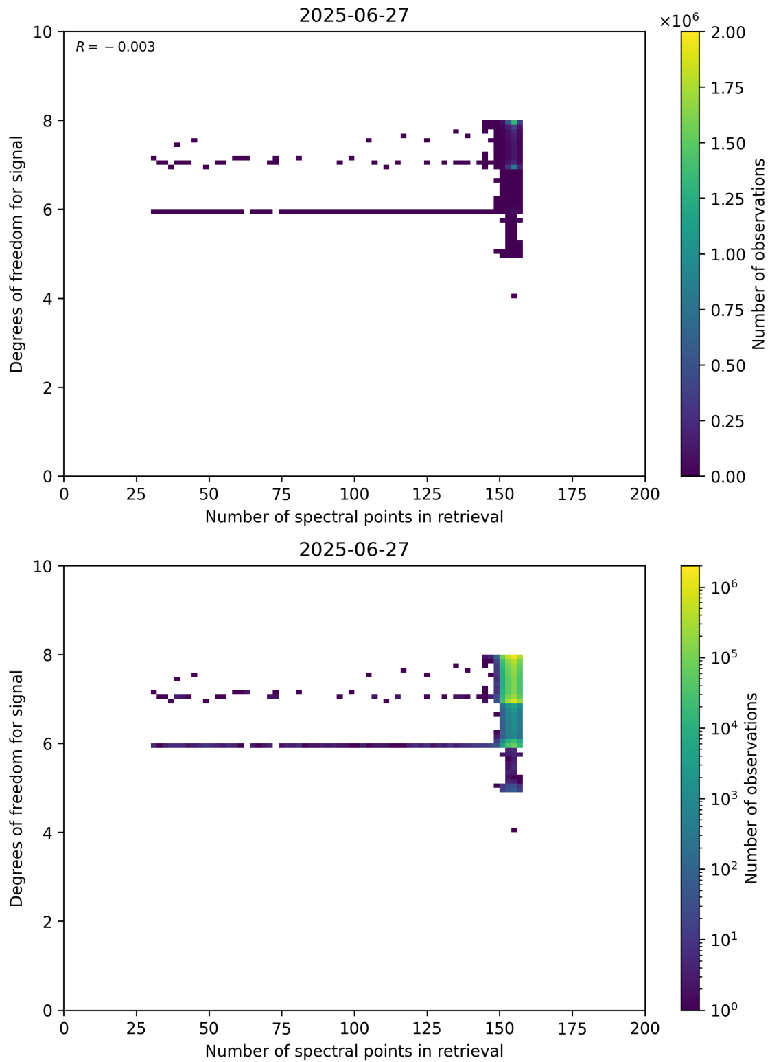
Figure 59: Scatter density plot of “Number of spectral points in retrieval” against “Degrees of freedom for signal” for 2025-06-27 to 2025-06-28.
