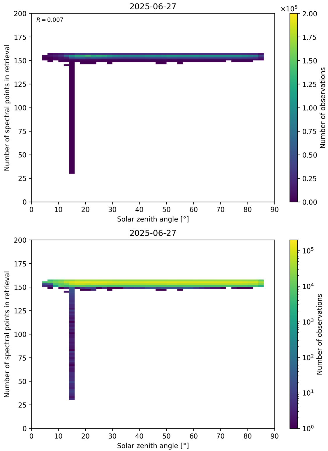
Figure 68: Scatter density plot of “Solar zenith angle” against “Number of spectral points in retrieval” for 2025-06-27 to 2025-06-28.
