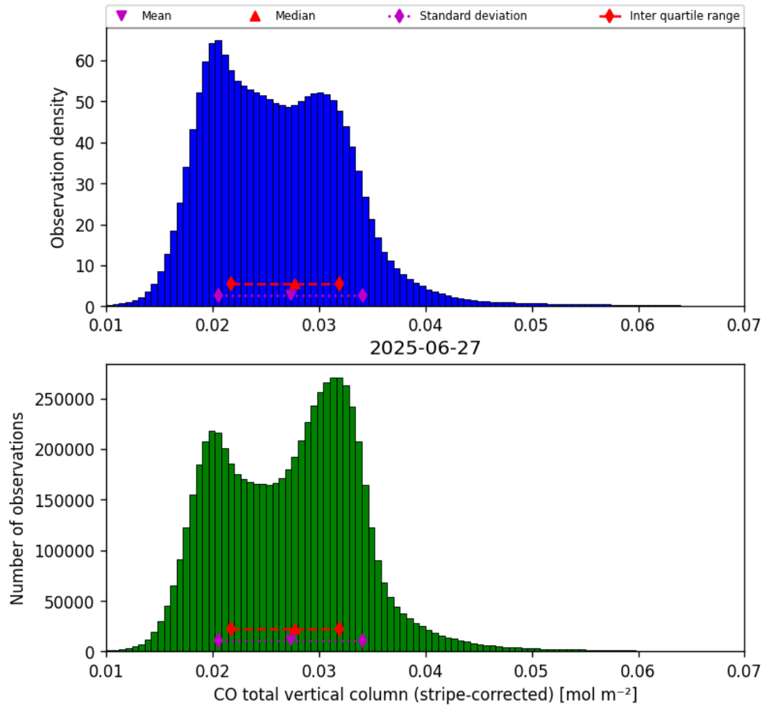
Figure 19: Histogram of “CO total vertical column (stripe-corrected)” for 2025-06-27 to 2025-06-28
