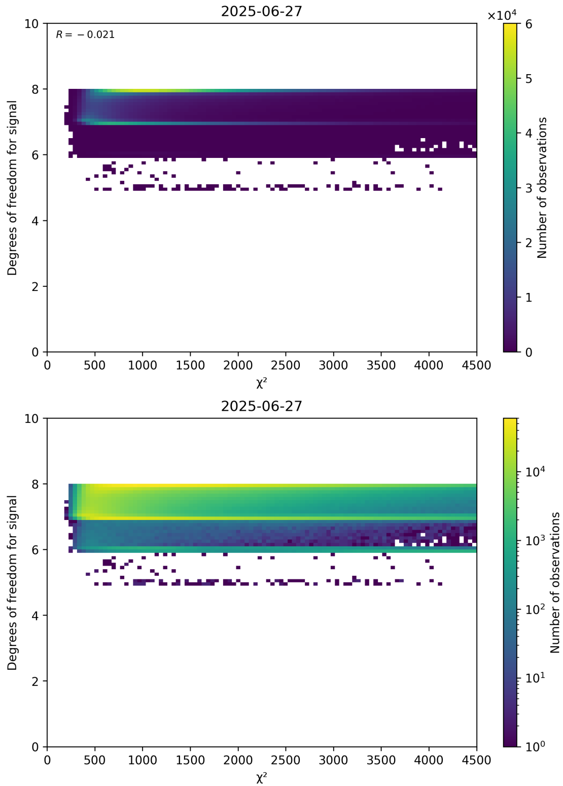
Figure 48: Scatter density plot of " \chi^2 " against "Degrees of freedom for signal" for 2025-06-27 to 2025-06-28.
