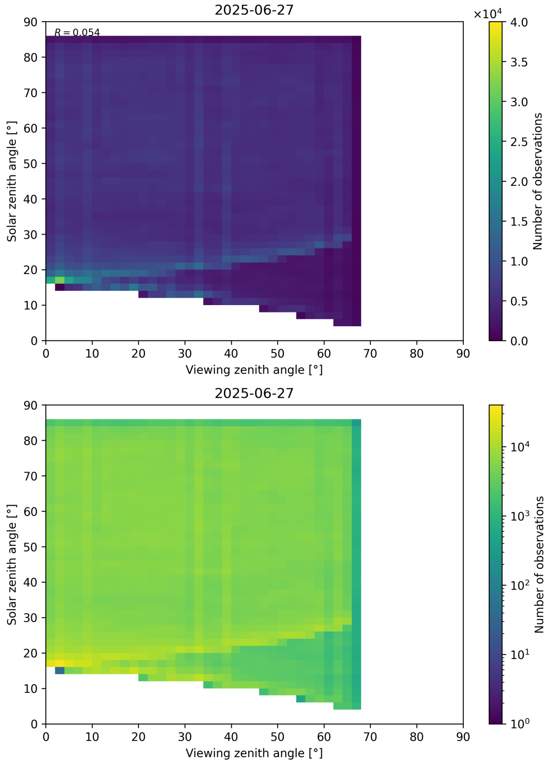
Figure 77: Scatter density plot of “Viewing zenith angle” against “Solar zenith angle” for 2025-06-27 to 2025-06-28.
