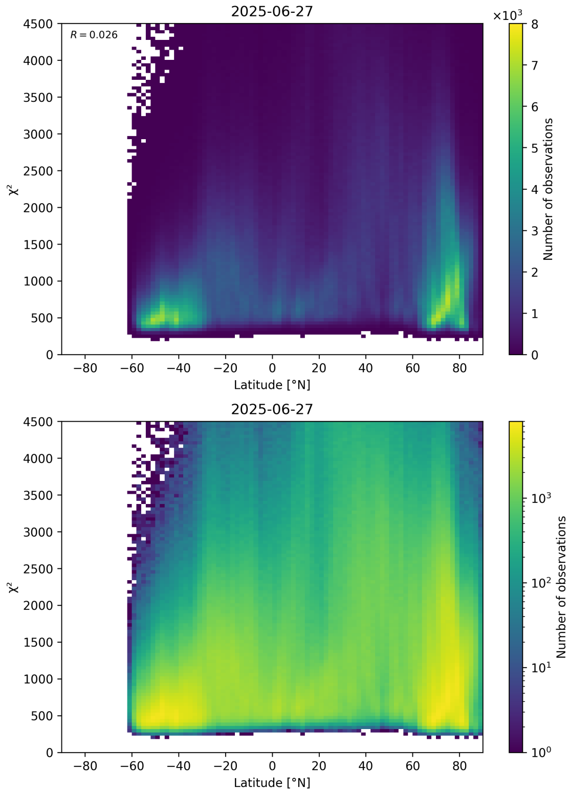
Figure 54: Scatter density plot of “Latitude” against “ \chi^2 ” for 2025-06-27 to 2025-06-28.
