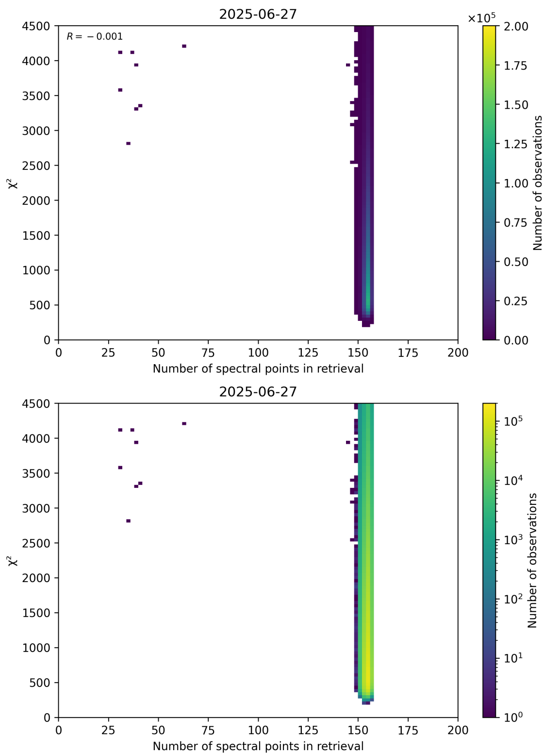
Figure 58: Scatter density plot of “Number of spectral points in retrieval” against “ \chi^2 ” for 2025-06-27 to 2025-06-28.
