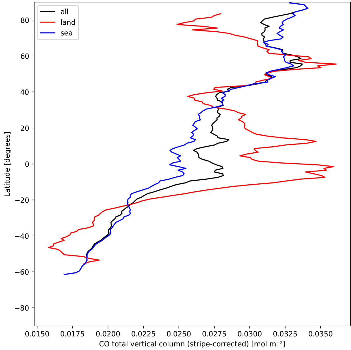
Figure 11: Zonal average of “CO total vertical column (stripe-corrected)” for 2025-06-27 to 2025-06-28.
