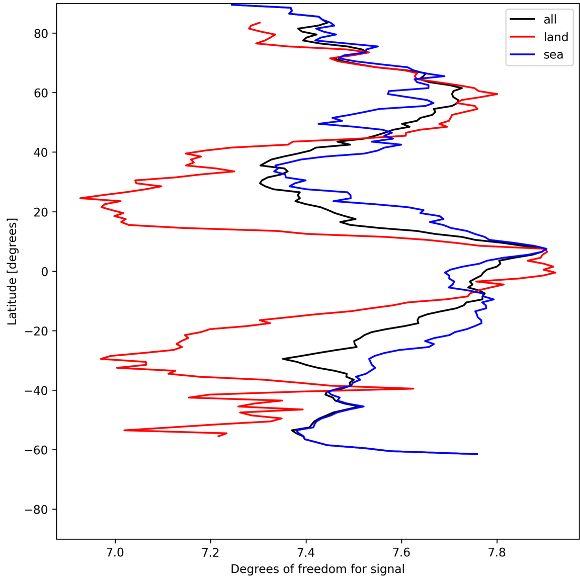
Figure 15: Zonal average of “Degrees of freedom for signal” for 2025-06-27 to 2025-06-28.
