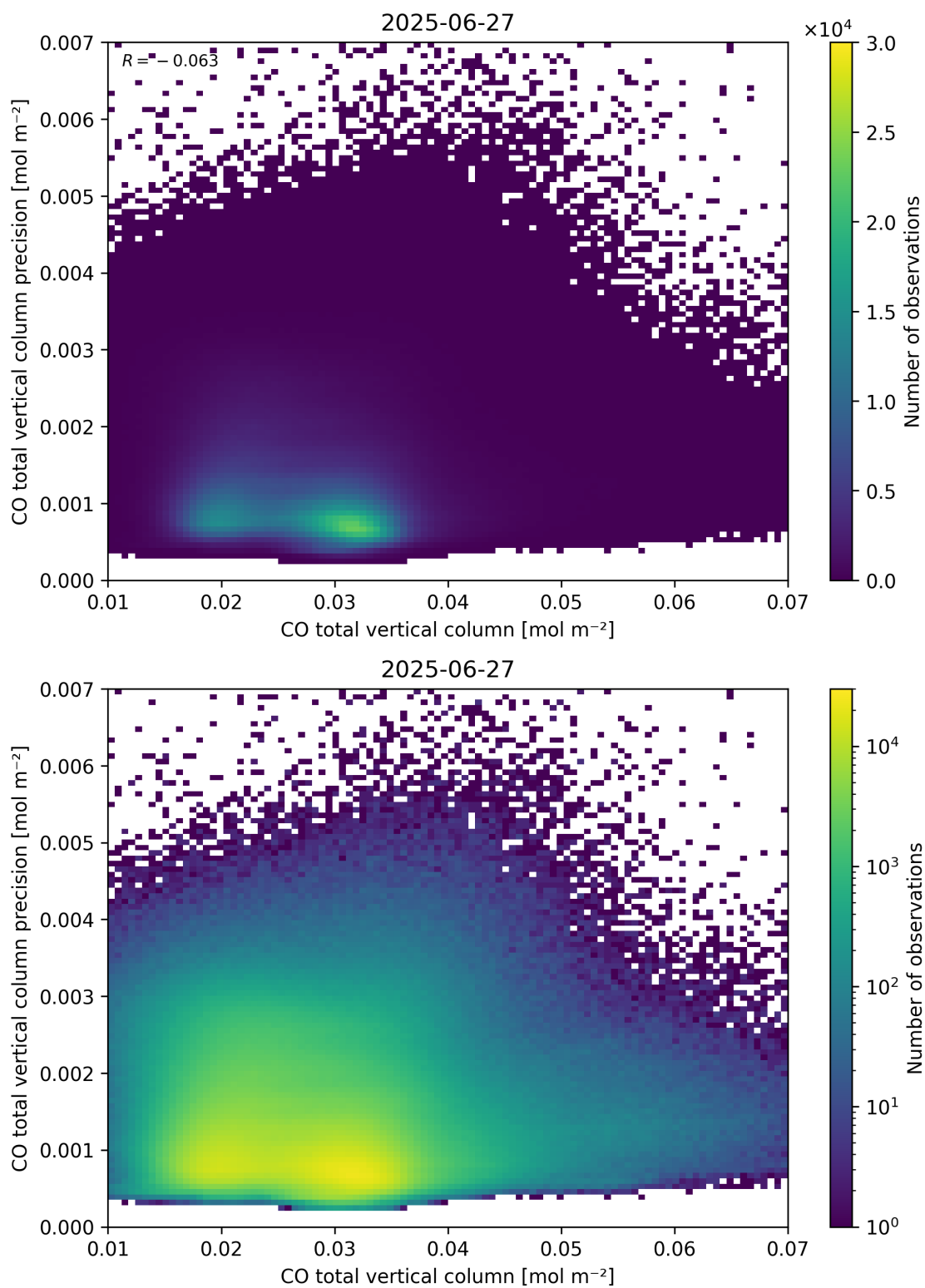
Figure 34: Scatter density plot of “CO total vertical column” against “CO total vertical column precision” for 2025-06-27 to 2025-06-28.
