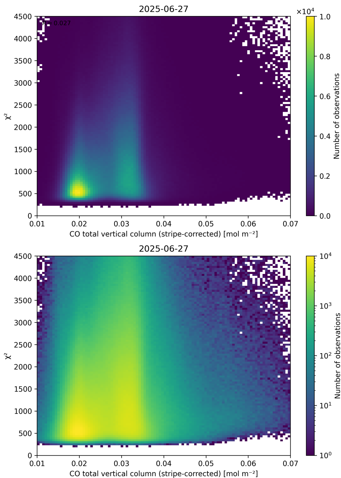
Figure 37: Scatter density plot of “CO total vertical column (stripe-corrected)” against “ \chi^2 ” for 2025-06-27 to 2025-06-28.
