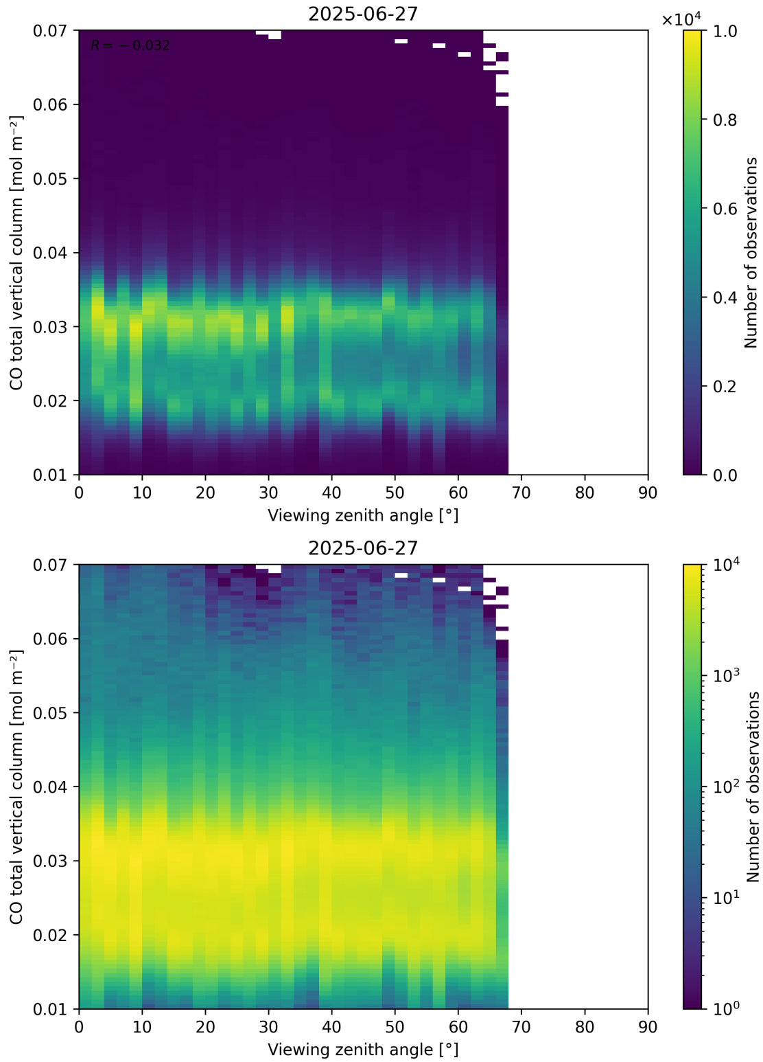
Figure 69: Scatter density plot of “Viewing zenith angle” against “CO total vertical column” for 2025-06-27 to 2025-06-28.
