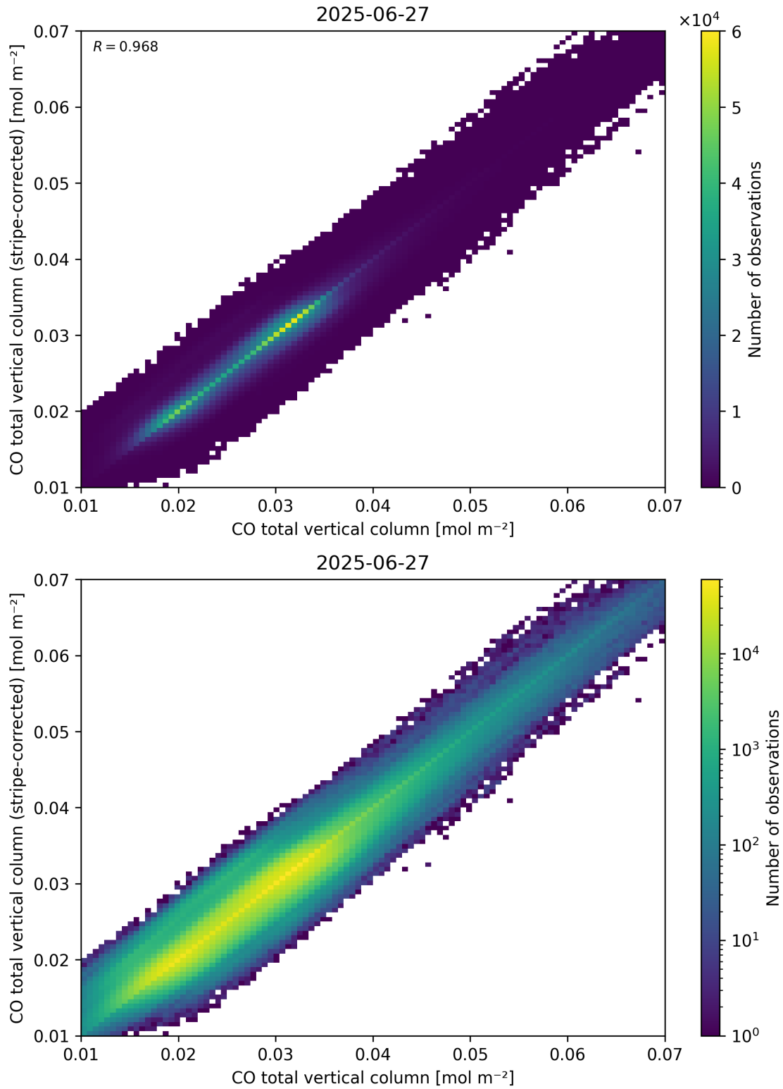
Figure 33: Scatter density plot of “CO total vertical column” against “CO total vertical column (stripe-corrected)” for 2025-06-27 to 2025-06-28.
