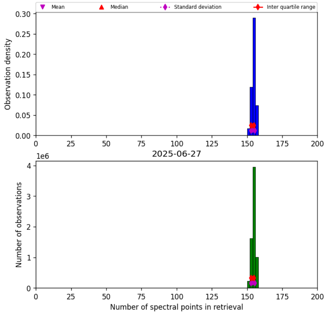
Figure 21: Histogram of “Number of spectral points in retrieval” for 2025-06-27 to 2025-06-28
