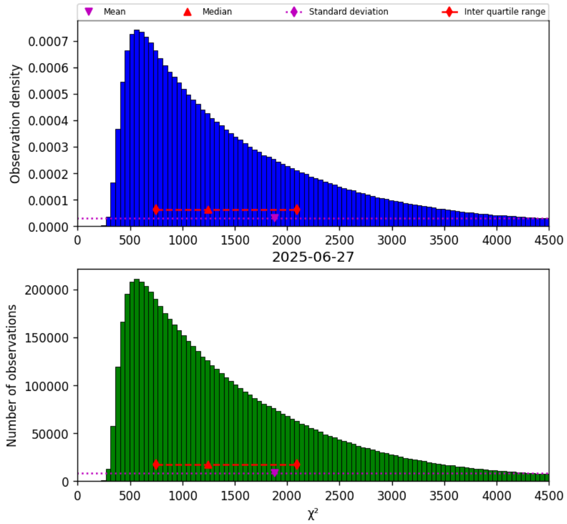
Figure 22: Histogram of “ \chi^2 ” for 2025-06-27 to 2025-06-28
