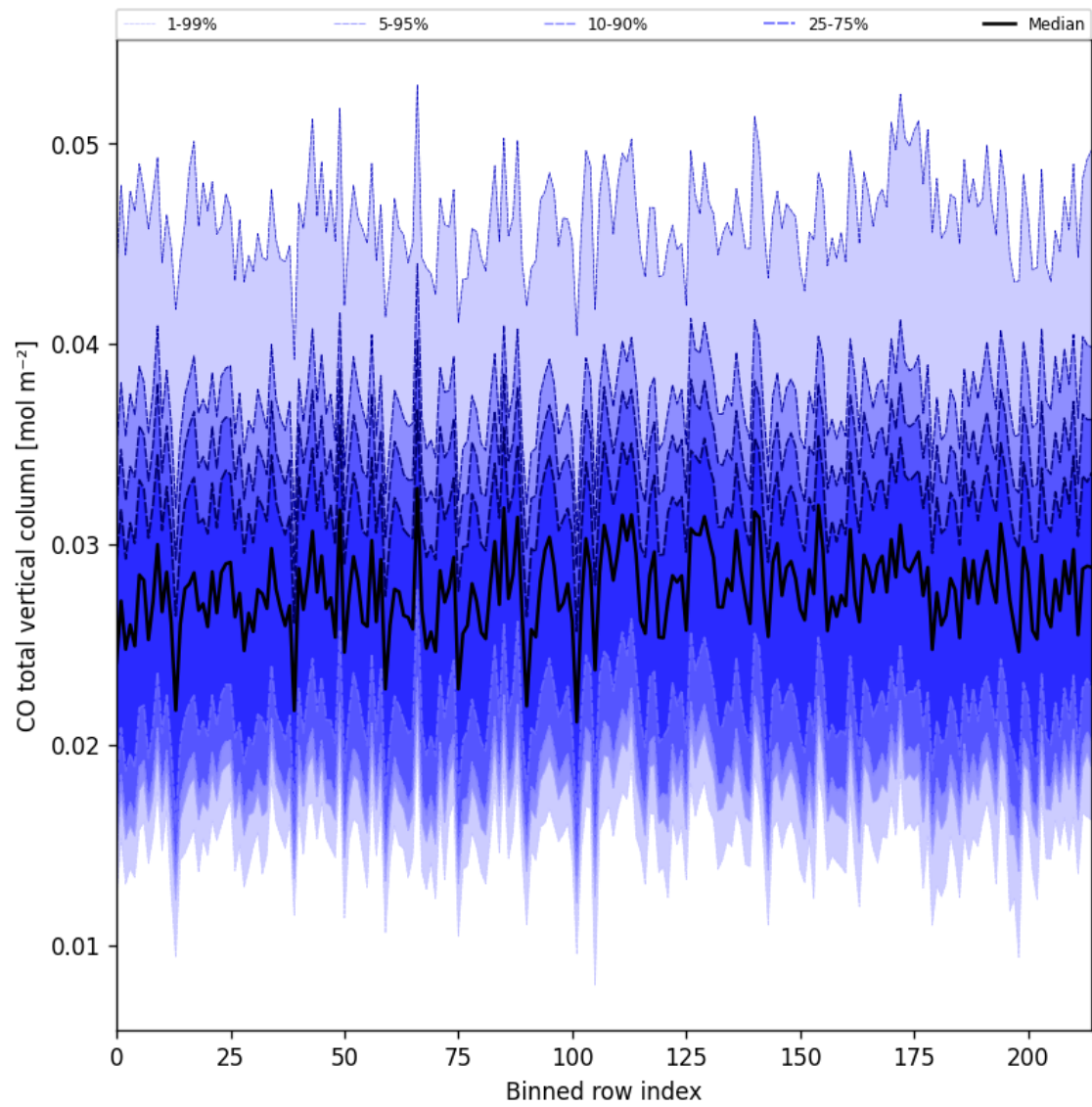
Figure 26: Along track statistics of “CO total vertical column” for 2025-06-27 to 2025-06-28
