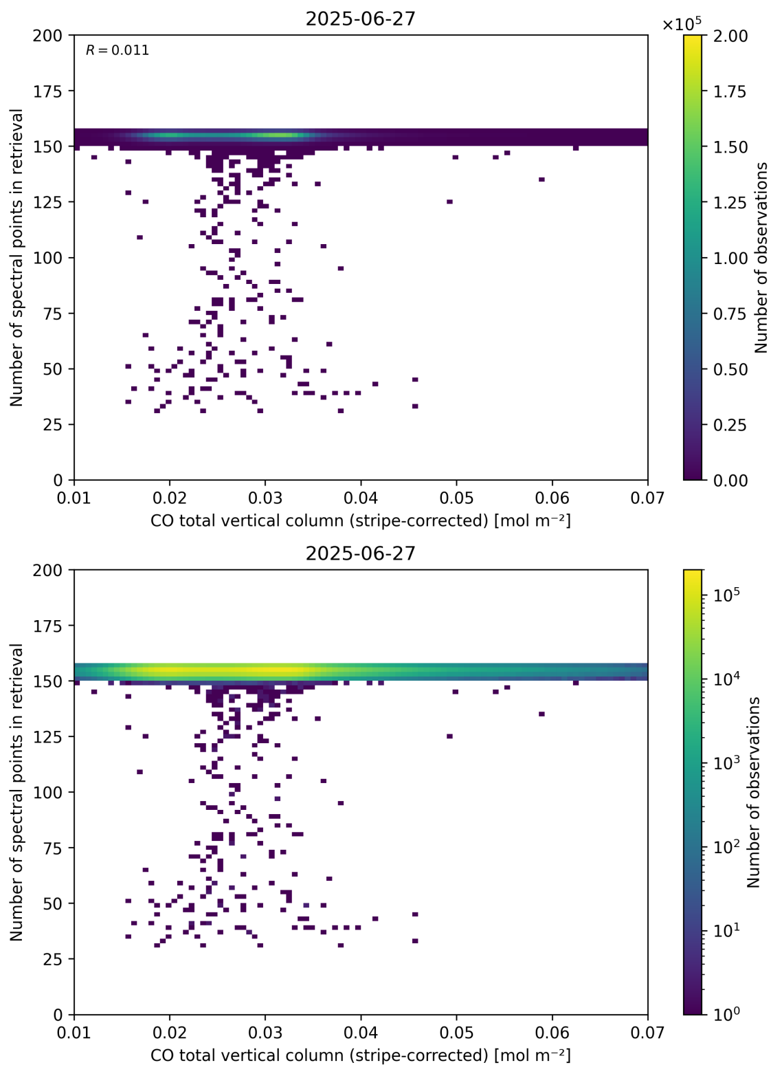
Figure 40: Scatter density plot of “CO total vertical column (stripe-corrected)” against “Number of spectral points in retrieval” for 2025-06-27 to 2025-06-28.
