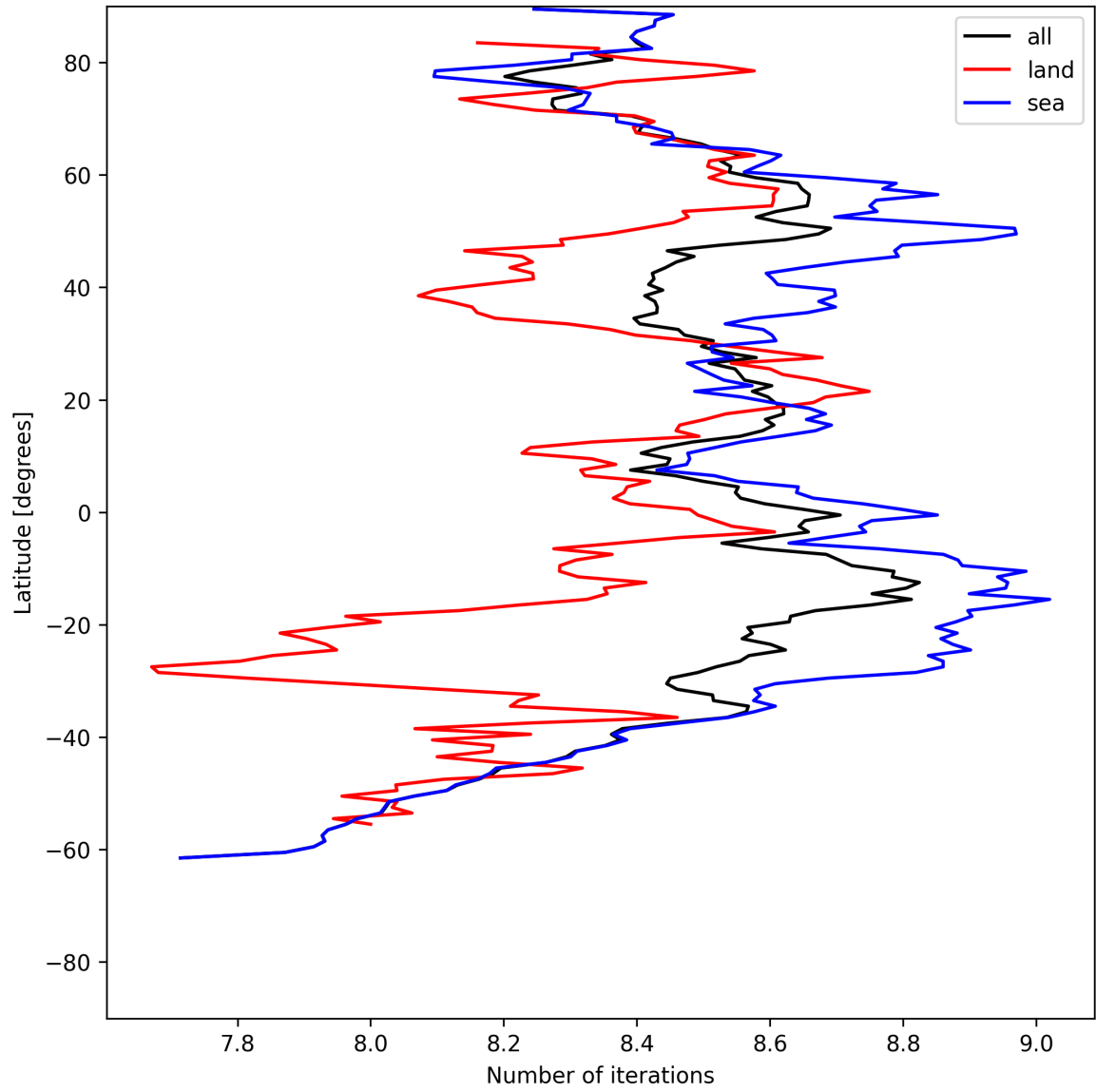
Figure 16: Zonal average of “Number of iterations” for 2025-06-27 to 2025-06-28.
