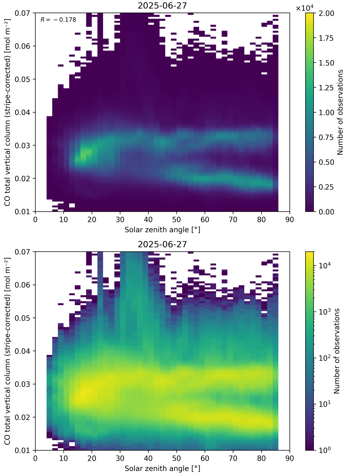
Figure 62: Scatter density plot of “Solar zenith angle” against “CO total vertical column (stripe-corrected)” for 2025-06-27 to 2025-06-28.
