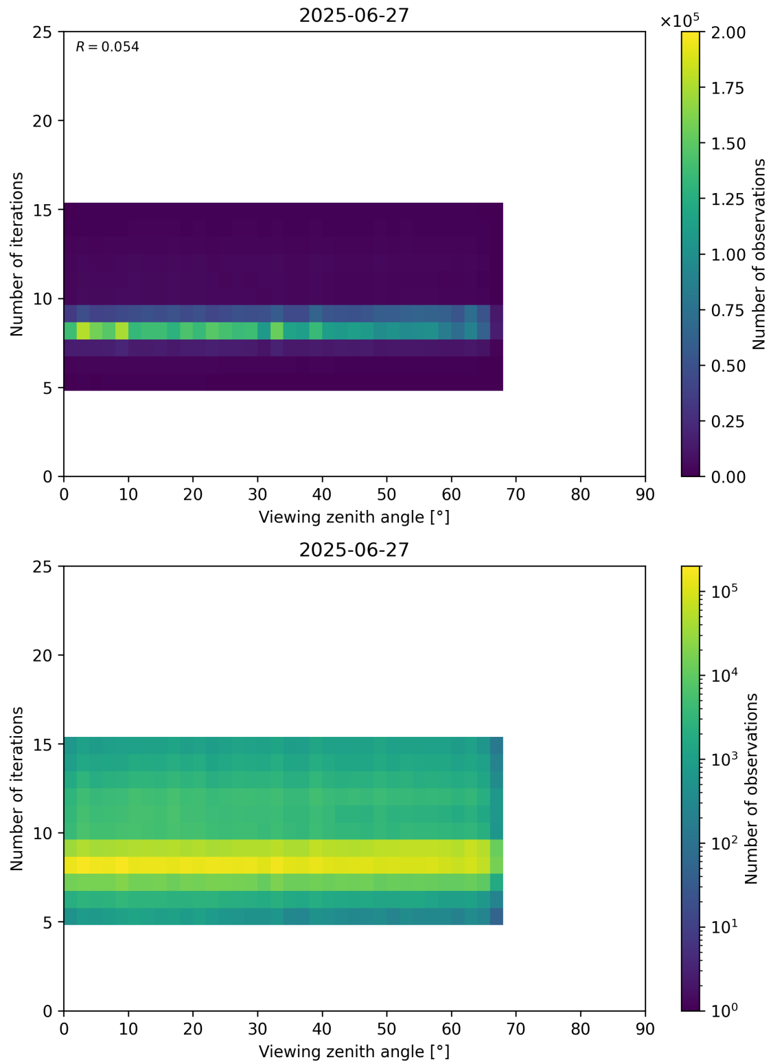
Figure 75: Scatter density plot of “Viewing zenith angle” against “Number of iterations” for 2025-06-27 to 2025-06-28.
