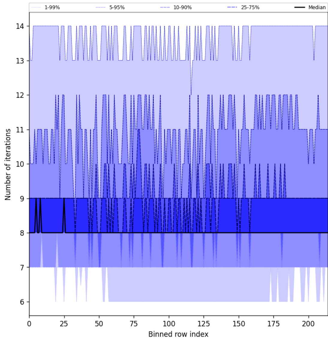
Figure 32: Along track statistics of “Number of iterations” for 2025-06-27 to 2025-06-28
