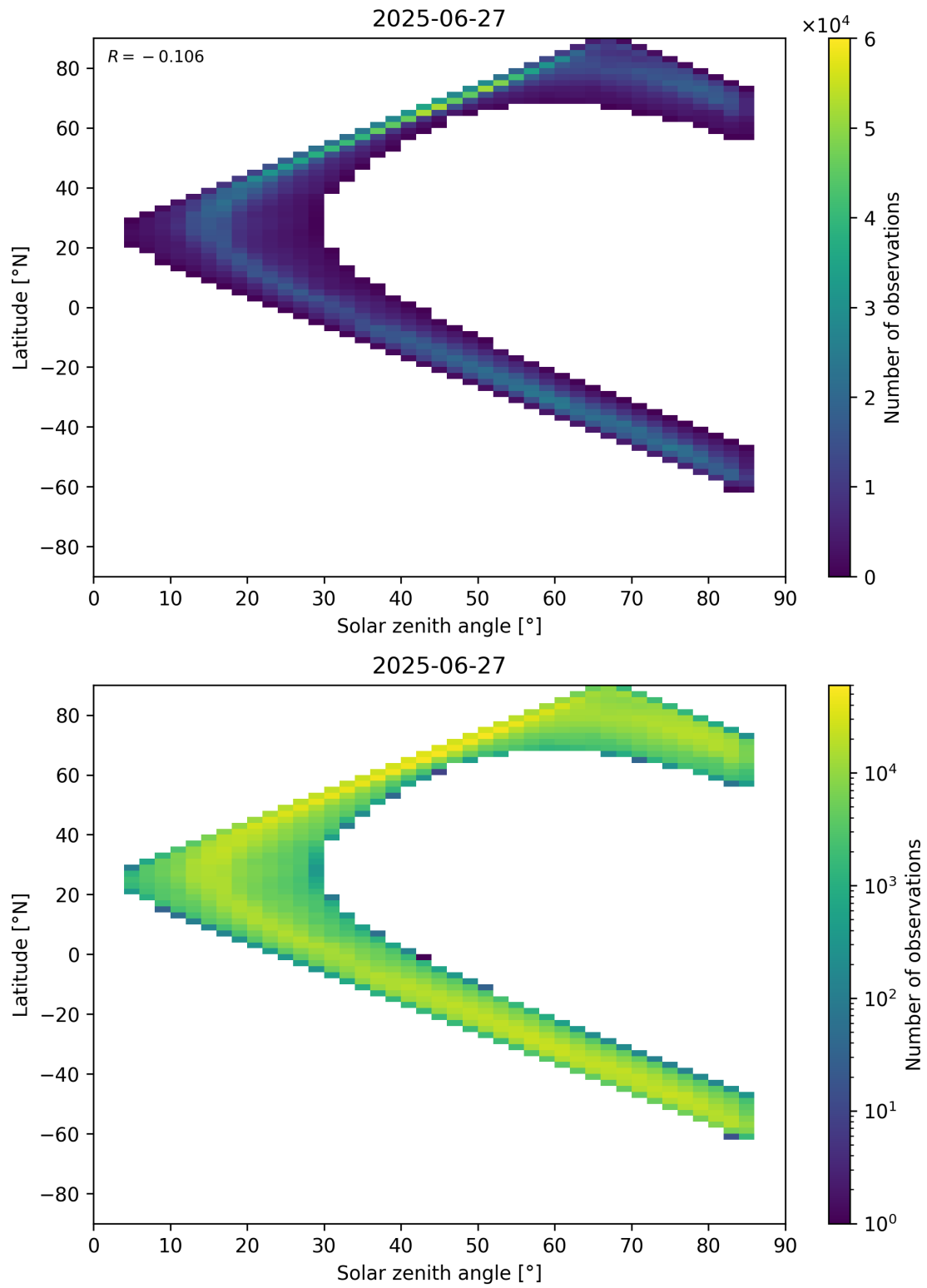
Figure 66: Scatter density plot of “Solar zenith angle” against “Latitude” for 2025-06-27 to 2025-06-28.
