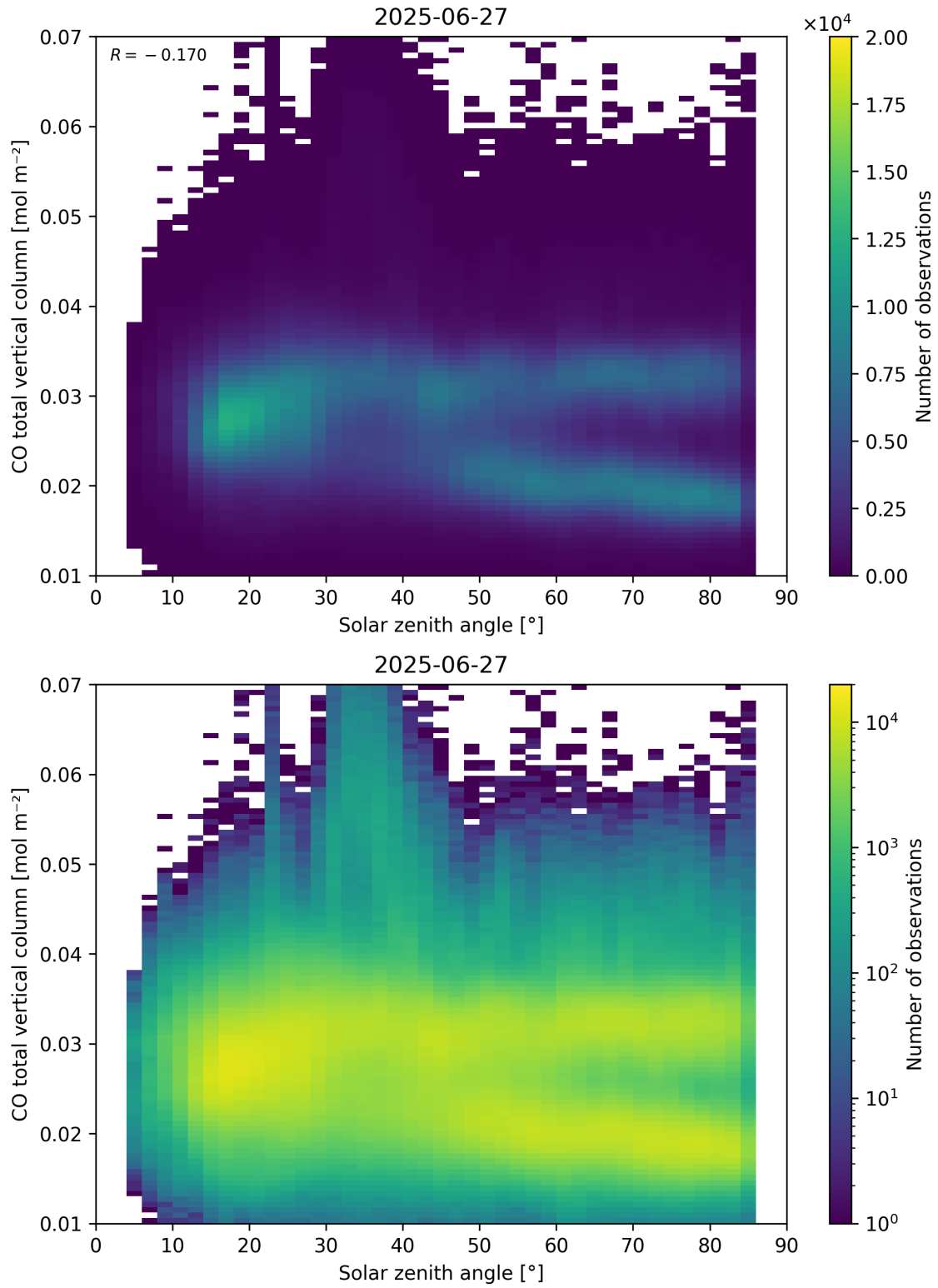
Figure 61: Scatter density plot of “Solar zenith angle” against “CO total vertical column” for 2025-06-27 to 2025-06-28.
