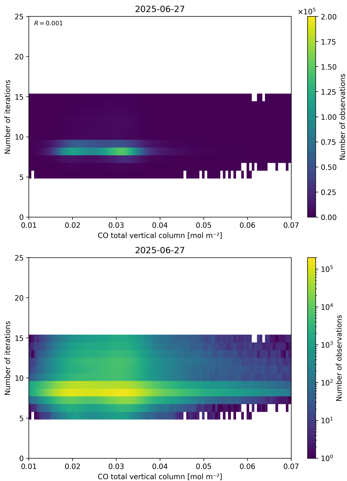
Figure 42: Scatter density plot of “CO total vertical column” against “Number of iterations” for 2025-06-27 to 2025-06-28.
