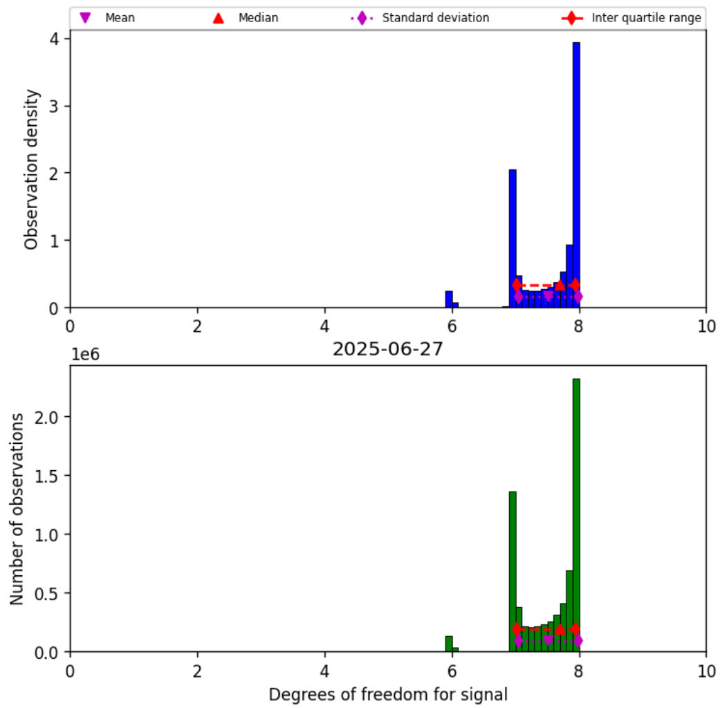
Figure 23: Histogram of “Degrees of freedom for signal” for 2025-06-27 to 2025-06-28
