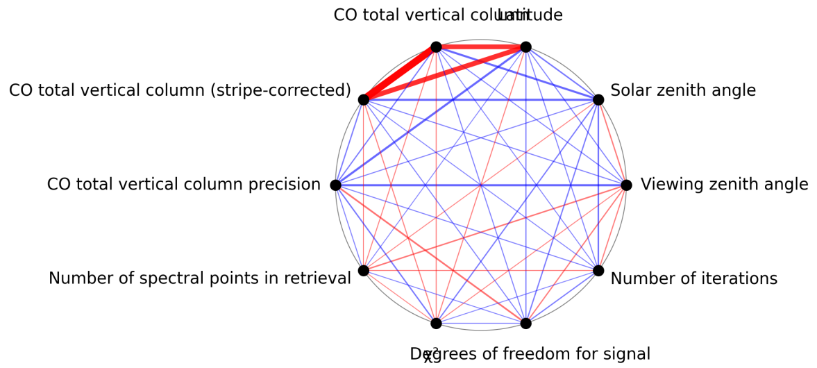
Figure 1: Map of correlation graph for 2025-06-28 to 2025-06-30.
