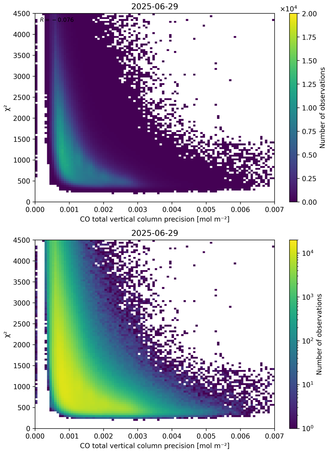
Figure 44: Scatter density plot of “CO total vertical column precision” against “ \chi^2 ” for 2025-06-28 to 2025-06-30.
