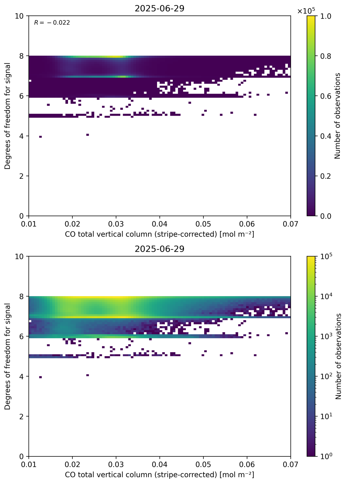
Figure 38: Scatter density plot of “CO total vertical column (stripe-corrected)” against “Degrees of freedom for signal” for 2025-06-28 to 2025-06-30.
