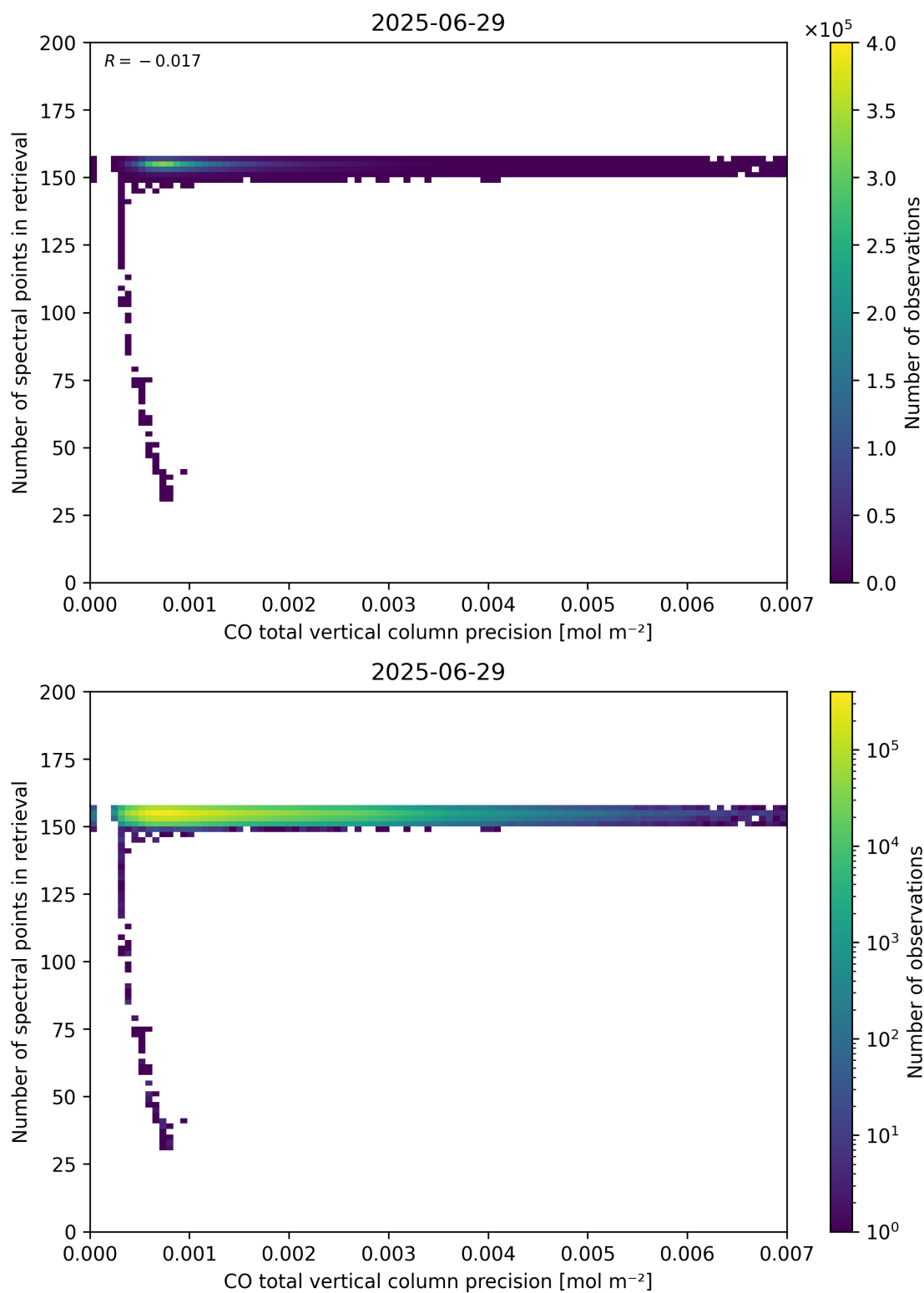
Figure 47: Scatter density plot of “CO total vertical column precision” against “Number of spectral points in retrieval” for 2025-06-28 to 2025-06-30.
