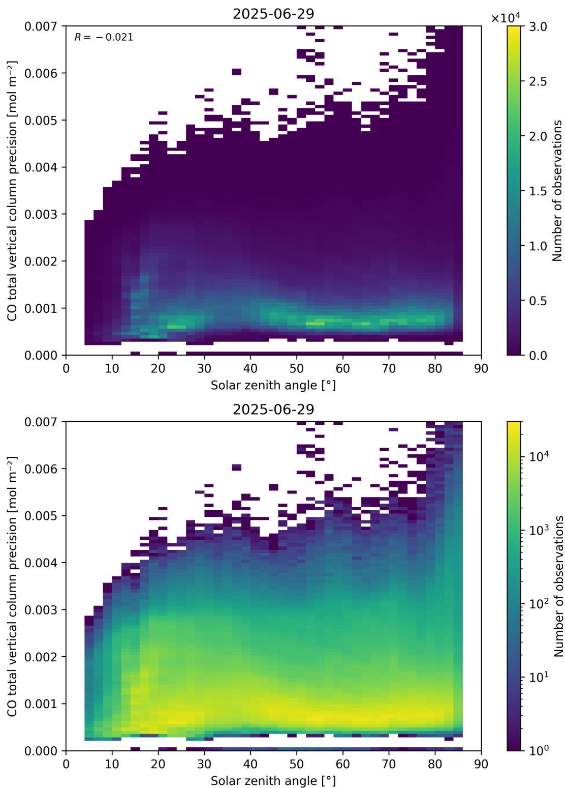
Figure 63: Scatter density plot of “Solar zenith angle” against “CO total vertical column precision” for 2025-06-28 to 2025-06-30.
