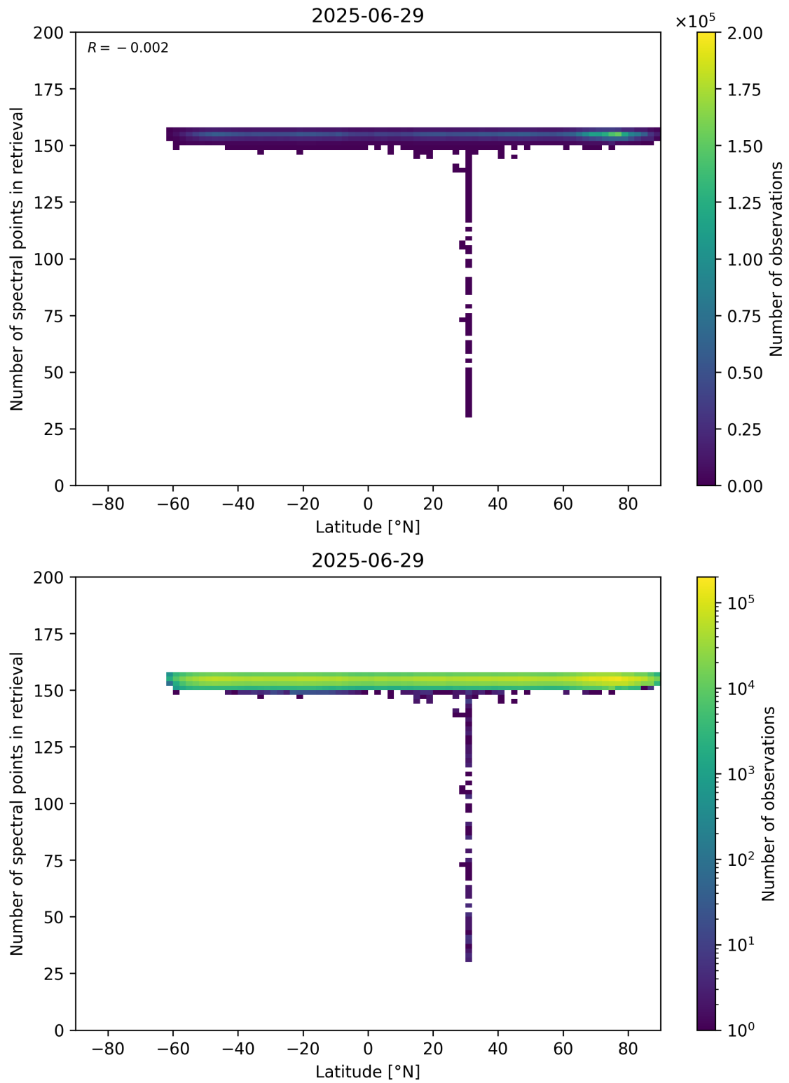
Figure 57: Scatter density plot of “Latitude” against “Number of spectral points in retrieval” for 2025-06-28 to 2025-06-30.
