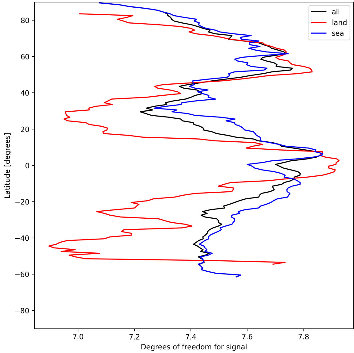
Figure 15: Zonal average of “Degrees of freedom for signal” for 2025-06-28 to 2025-06-30.
