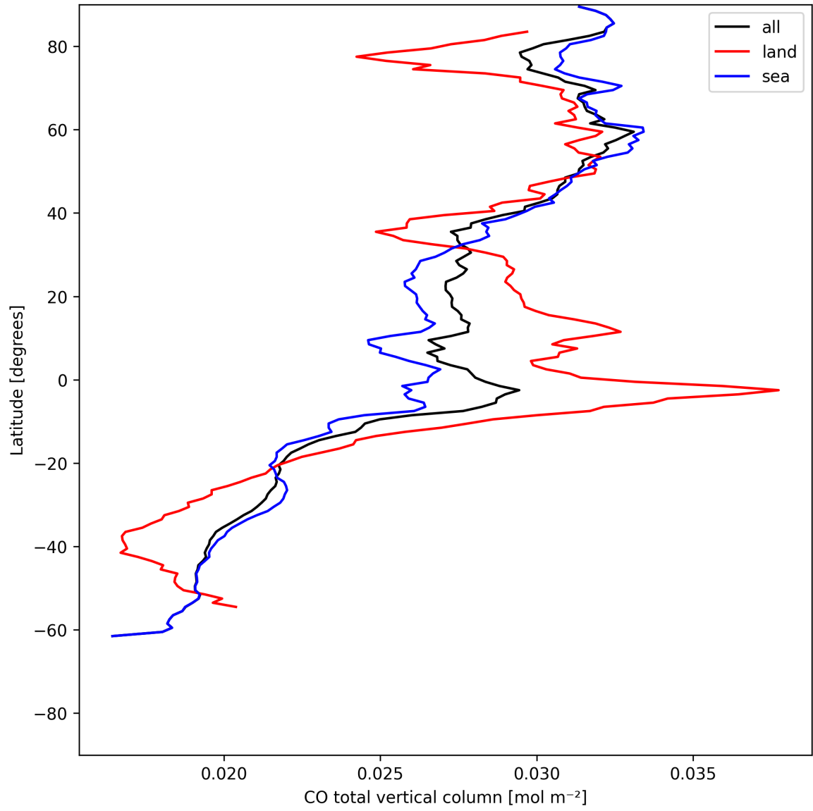
Figure 10: Zonal average of “CO total vertical column” for 2025-06-28 to 2025-06-30.
