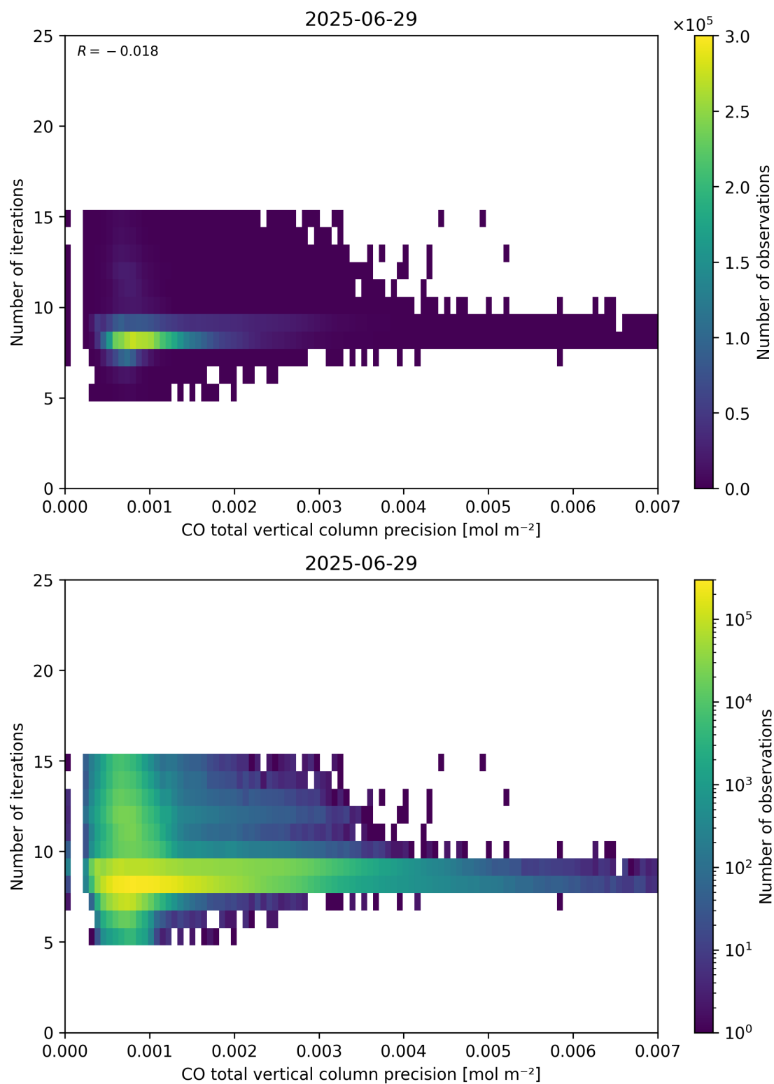
Figure 46: Scatter density plot of “CO total vertical column precision” against “Number of iterations” for 2025-06-28 to 2025-06-30.
