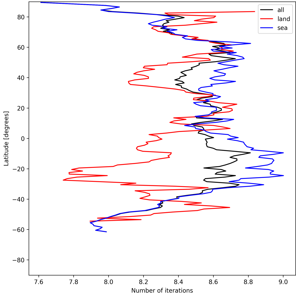
Figure 16: Zonal average of “Number of iterations” for 2025-06-28 to 2025-06-30.
