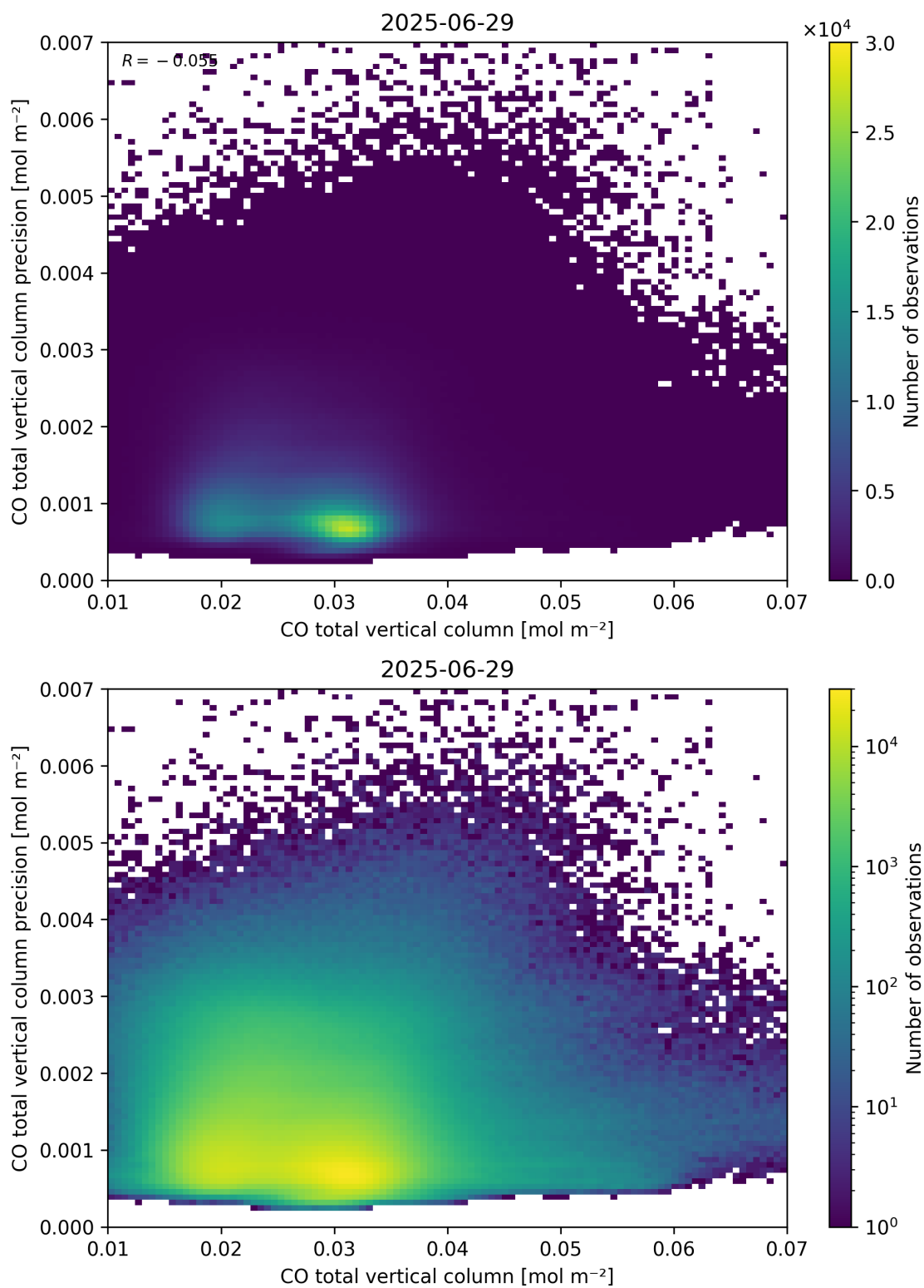
Figure 34: Scatter density plot of “CO total vertical column” against “CO total vertical column precision” for 2025-06-28 to 2025-06-30.
