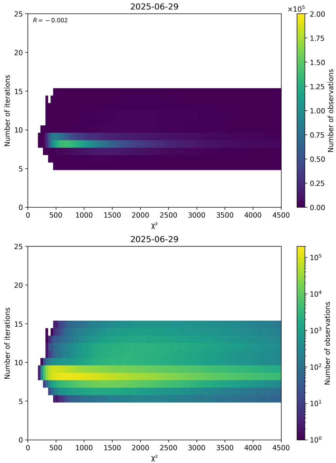
Figure 49: Scatter density plot of “ \chi^2 ” against “Number of iterations” for 2025-06-28 to 2025-06-30.
