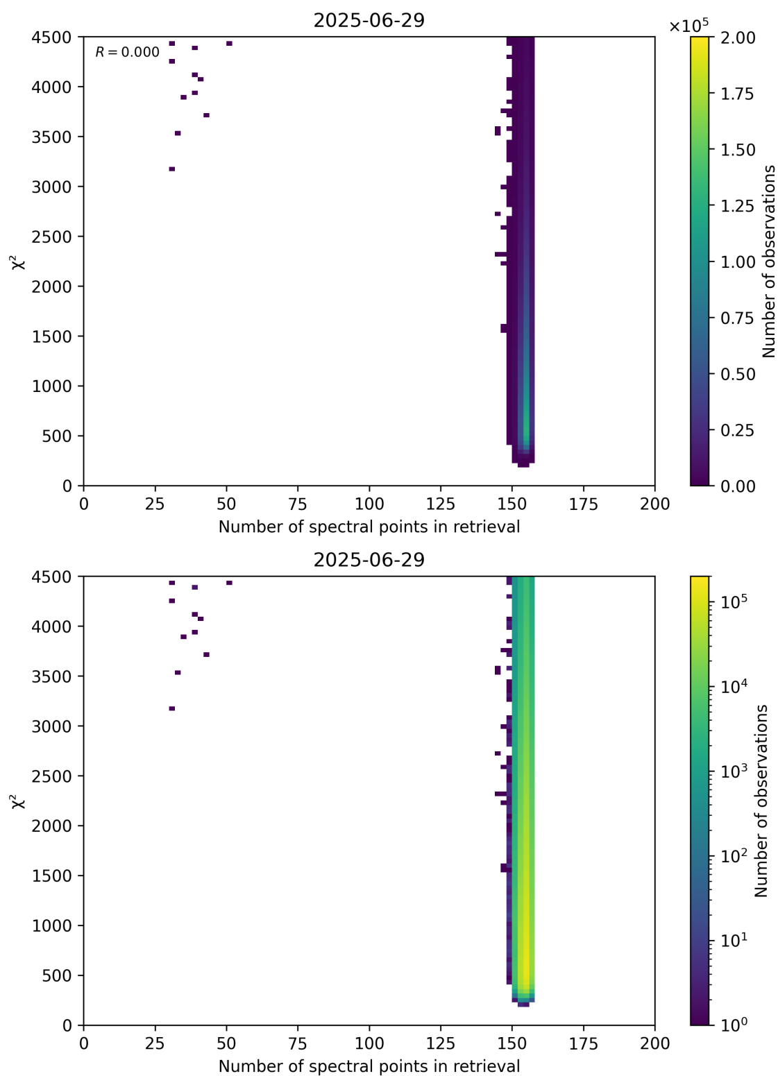
Figure 58: Scatter density plot of “Number of spectral points in retrieval” against “ \chi^2 ” for 2025-06-28 to 2025-06-30.
