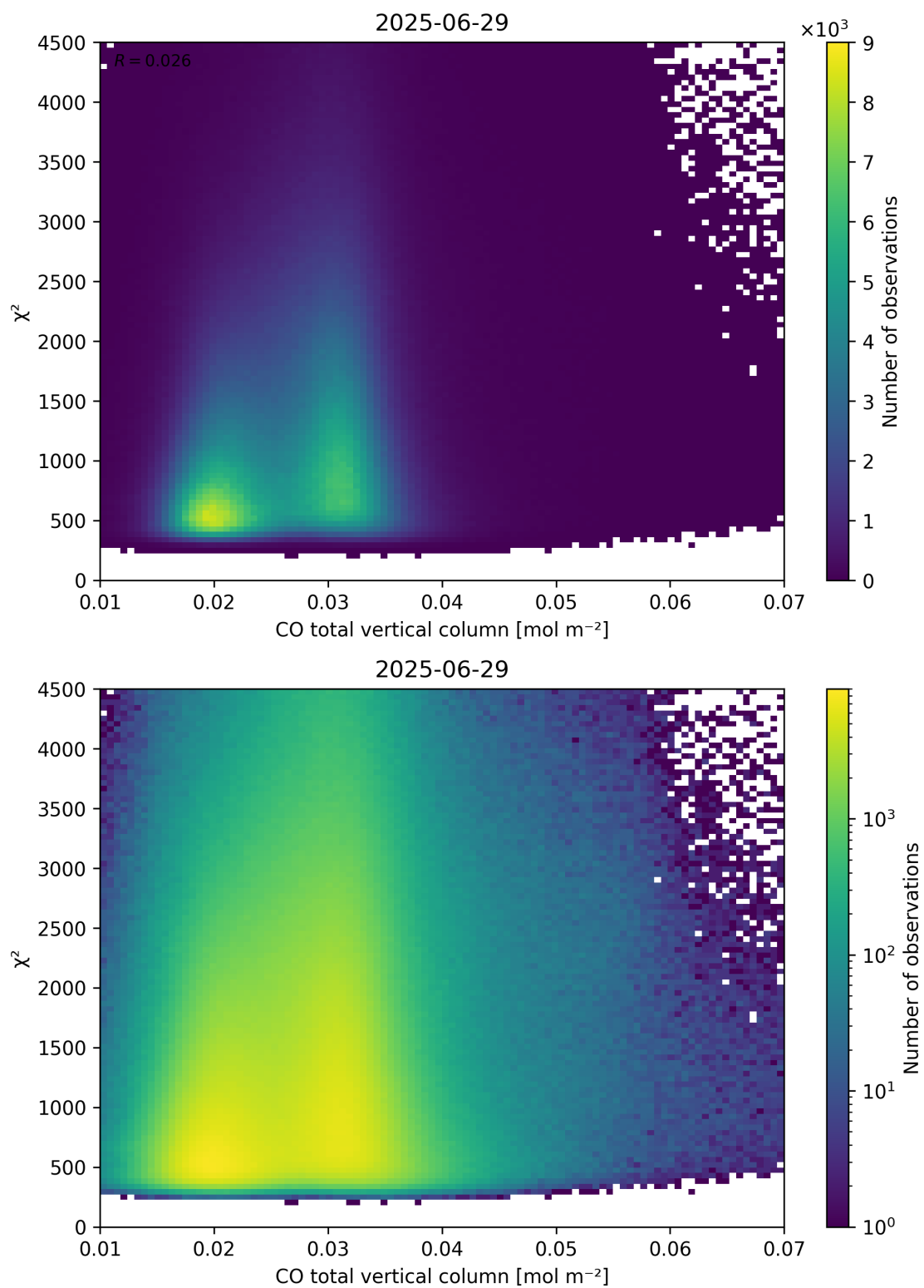
Figure 35: Scatter density plot of “CO total vertical column” against “ \chi^2 ” for 2025-06-28 to 2025-06-30.
