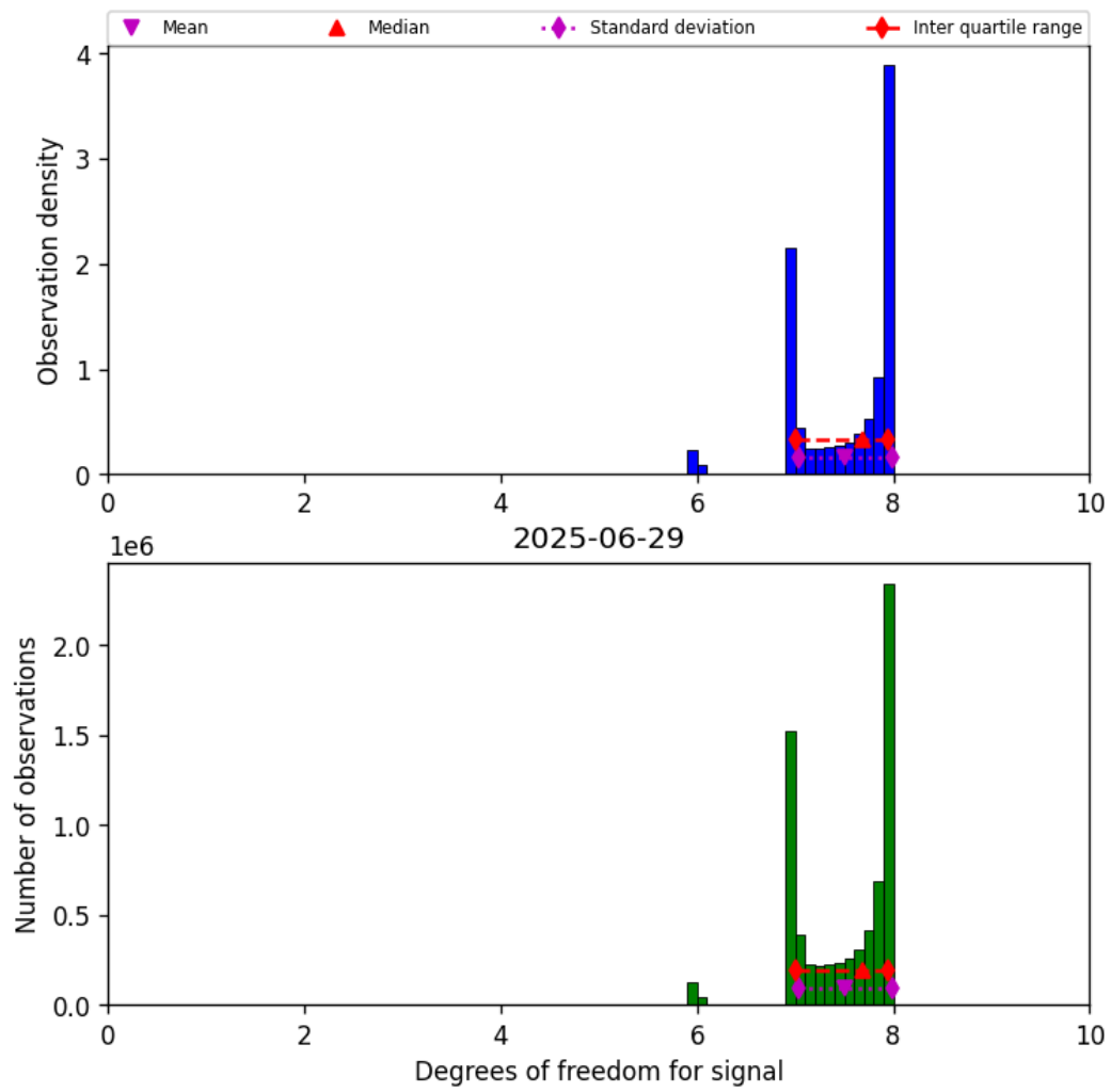
Figure 23: Histogram of “Degrees of freedom for signal” for 2025-06-28 to 2025-06-30
