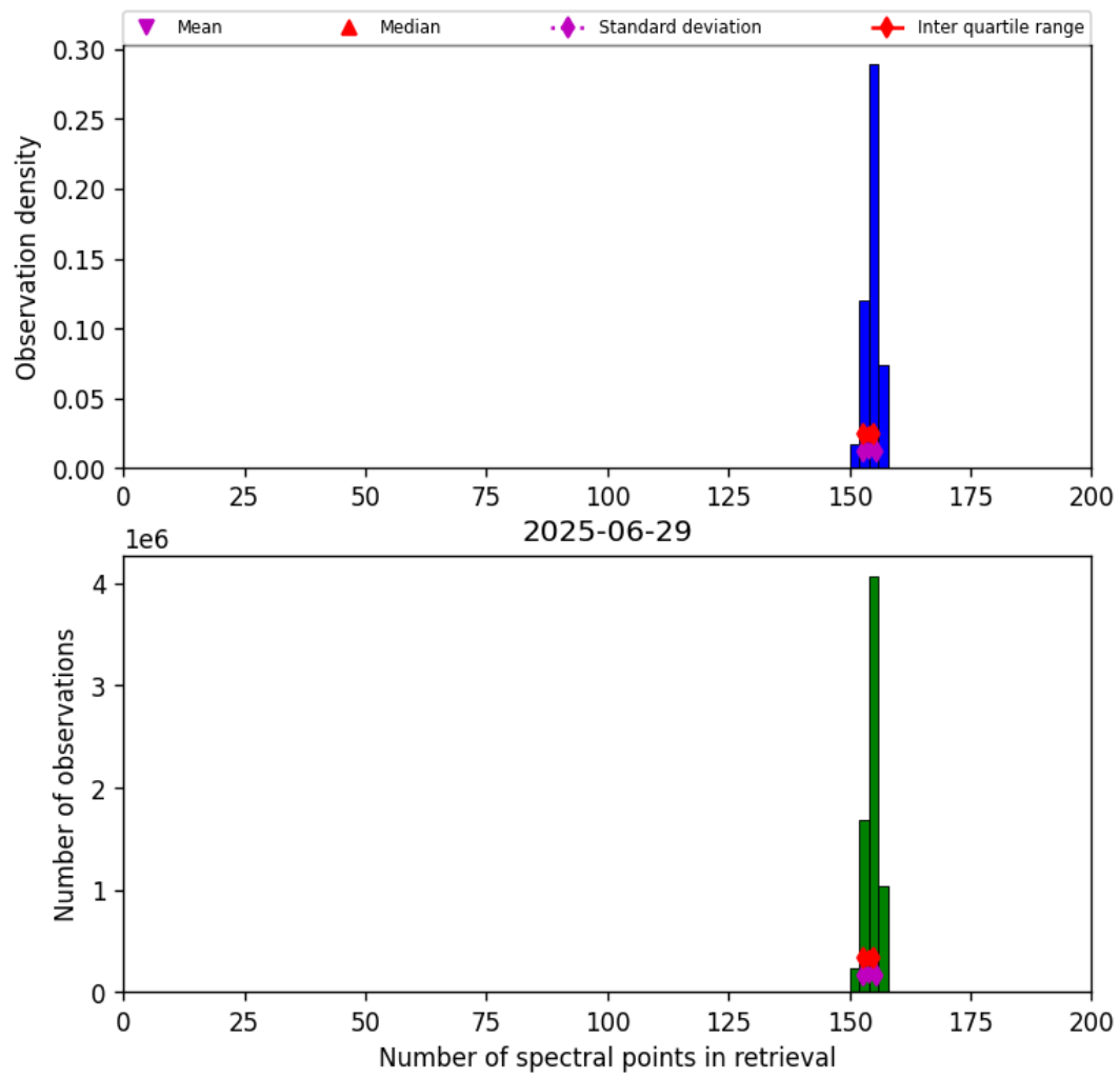
Figure 21: Histogram of “Number of spectral points in retrieval” for 2025-06-28 to 2025-06-30
