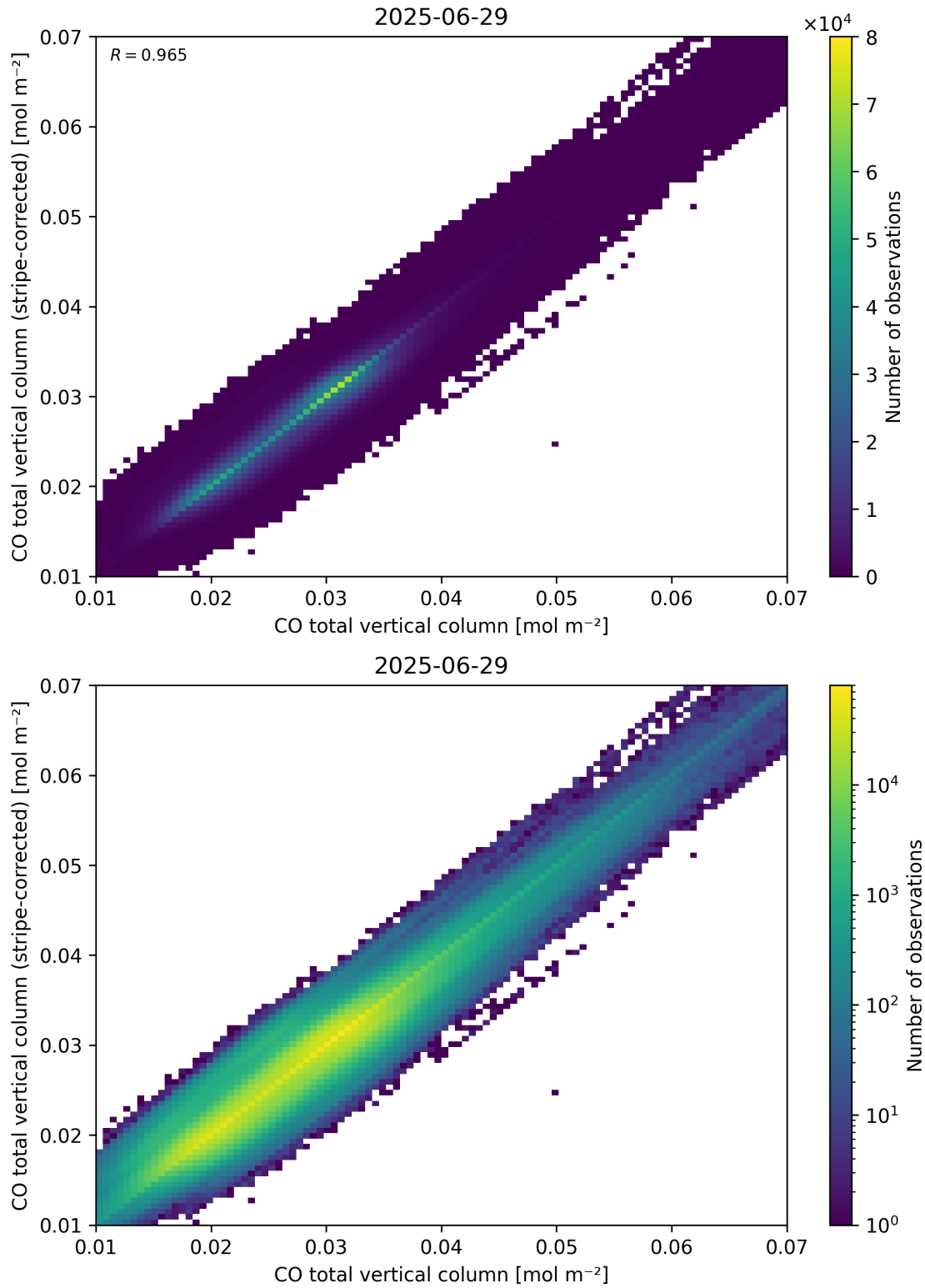
Figure 33: Scatter density plot of “CO total vertical column” against “CO total vertical column (stripe-corrected)” for 2025-06-28 to 2025-06-30.
