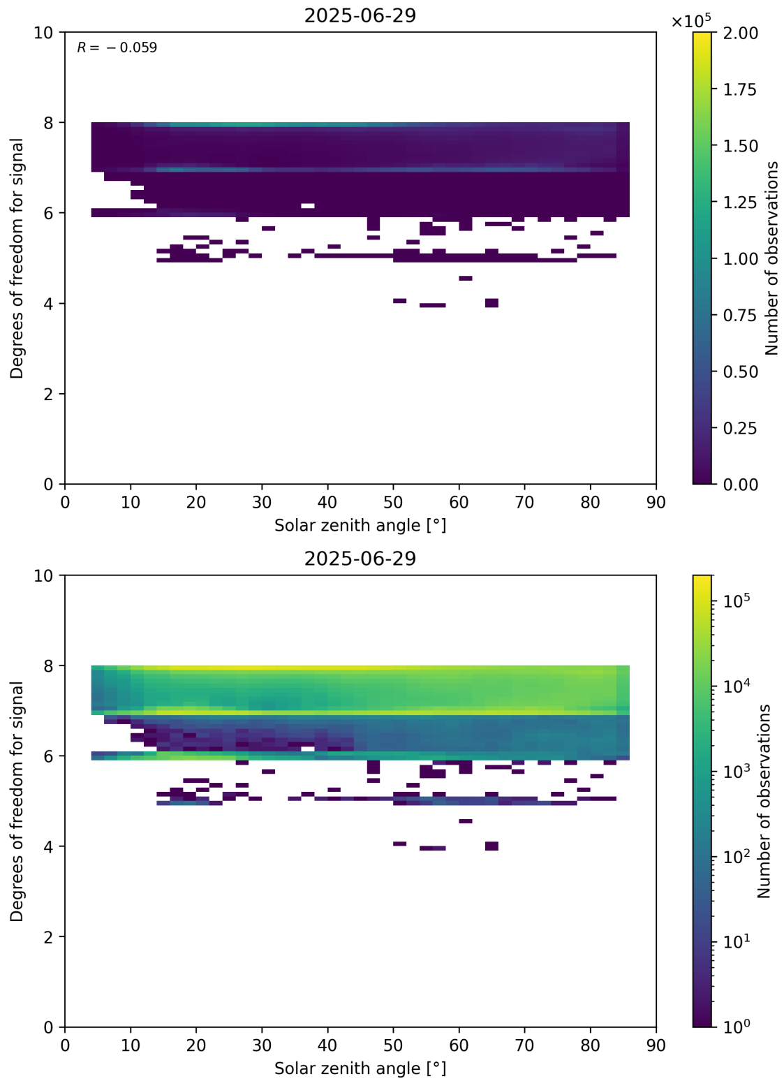
Figure 65: Scatter density plot of “Solar zenith angle” against “Degrees of freedom for signal” for 2025-06-28 to 2025-06-30.
