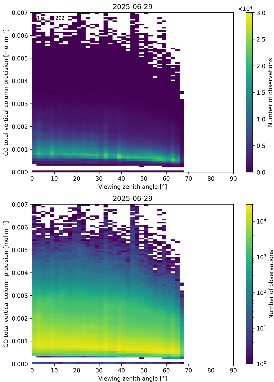
Figure 71: Scatter density plot of “Viewing zenith angle” against “CO total vertical column precision” for 2025-06-28 to 2025-06-30.
