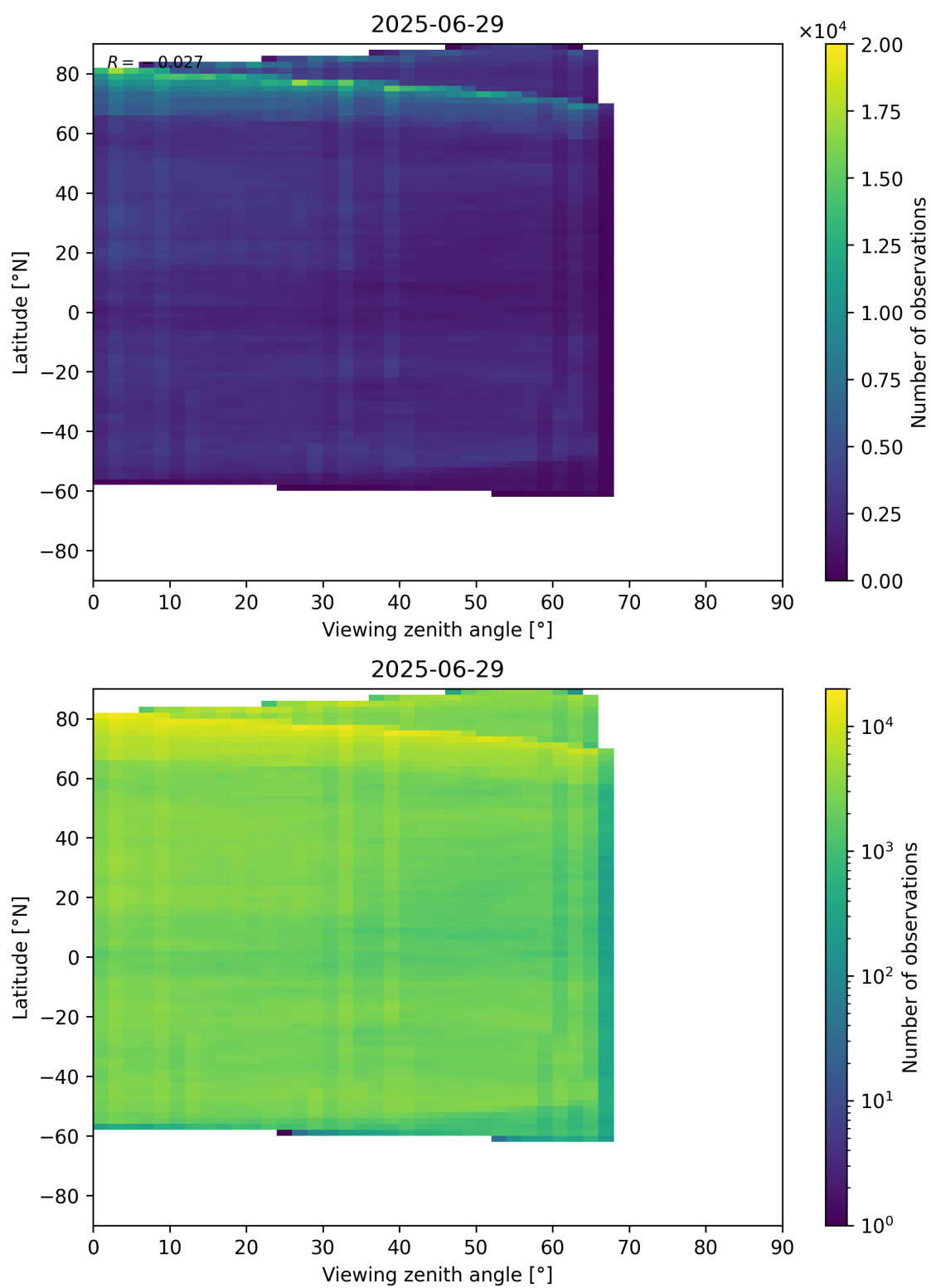
Figure 74: Scatter density plot of “Viewing zenith angle” against “Latitude” for 2025-06-28 to 2025-06-30.
