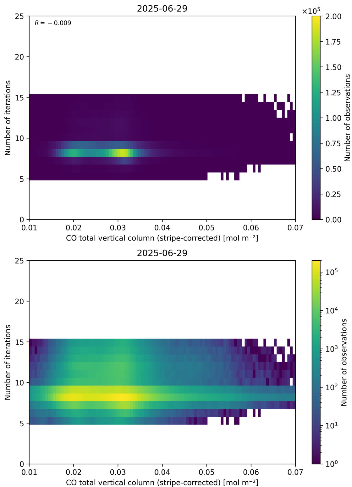
Figure 39: Scatter density plot of “CO total vertical column (stripe-corrected)” against “Number of iterations” for 2025-06-28 to 2025-06-30.
