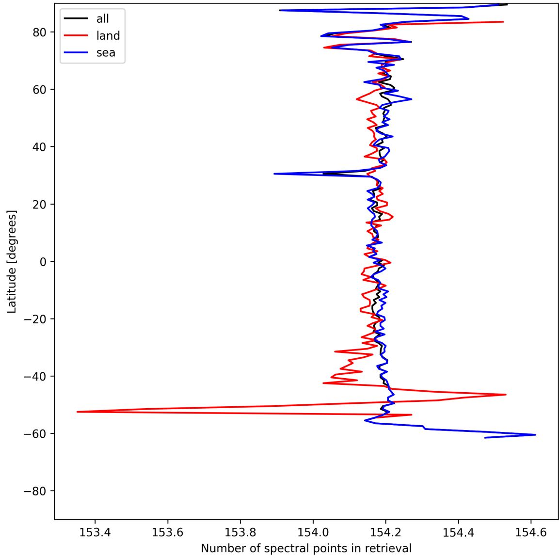
Figure 13: Zonal average of “Number of spectral points in retrieval” for 2025-06-28 to 2025-06-30.
