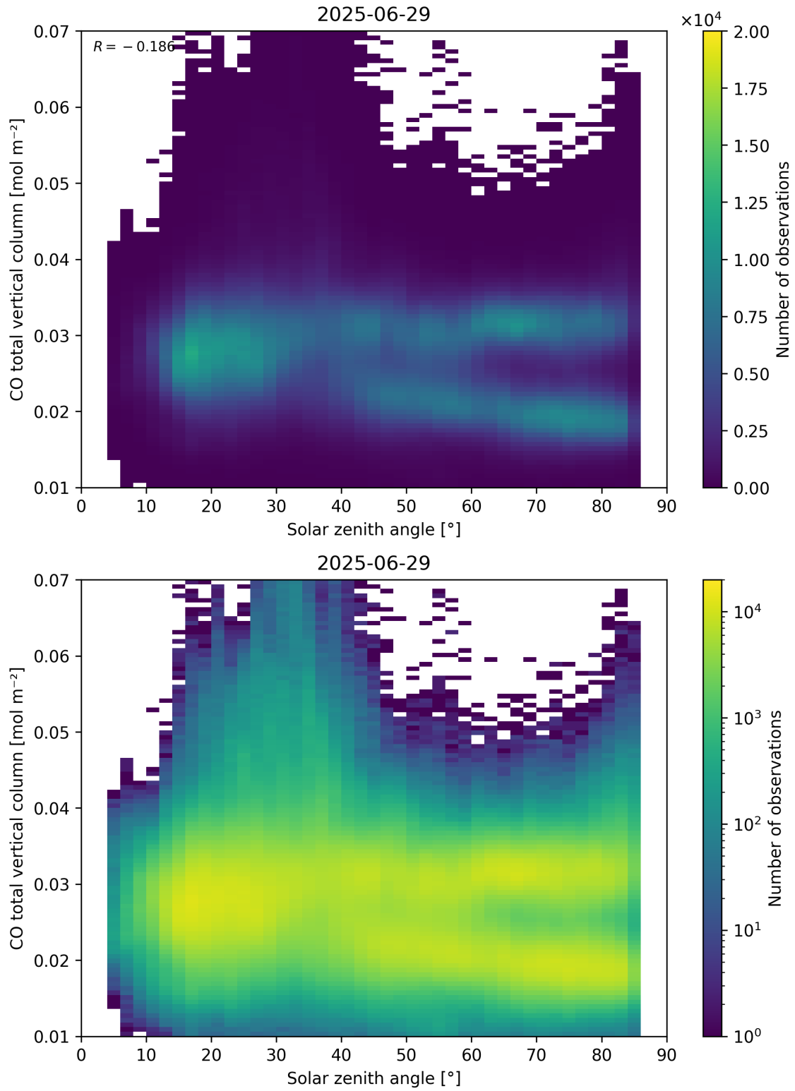
Figure 61: Scatter density plot of “Solar zenith angle” against “CO total vertical column” for 2025-06-28 to 2025-06-30.
