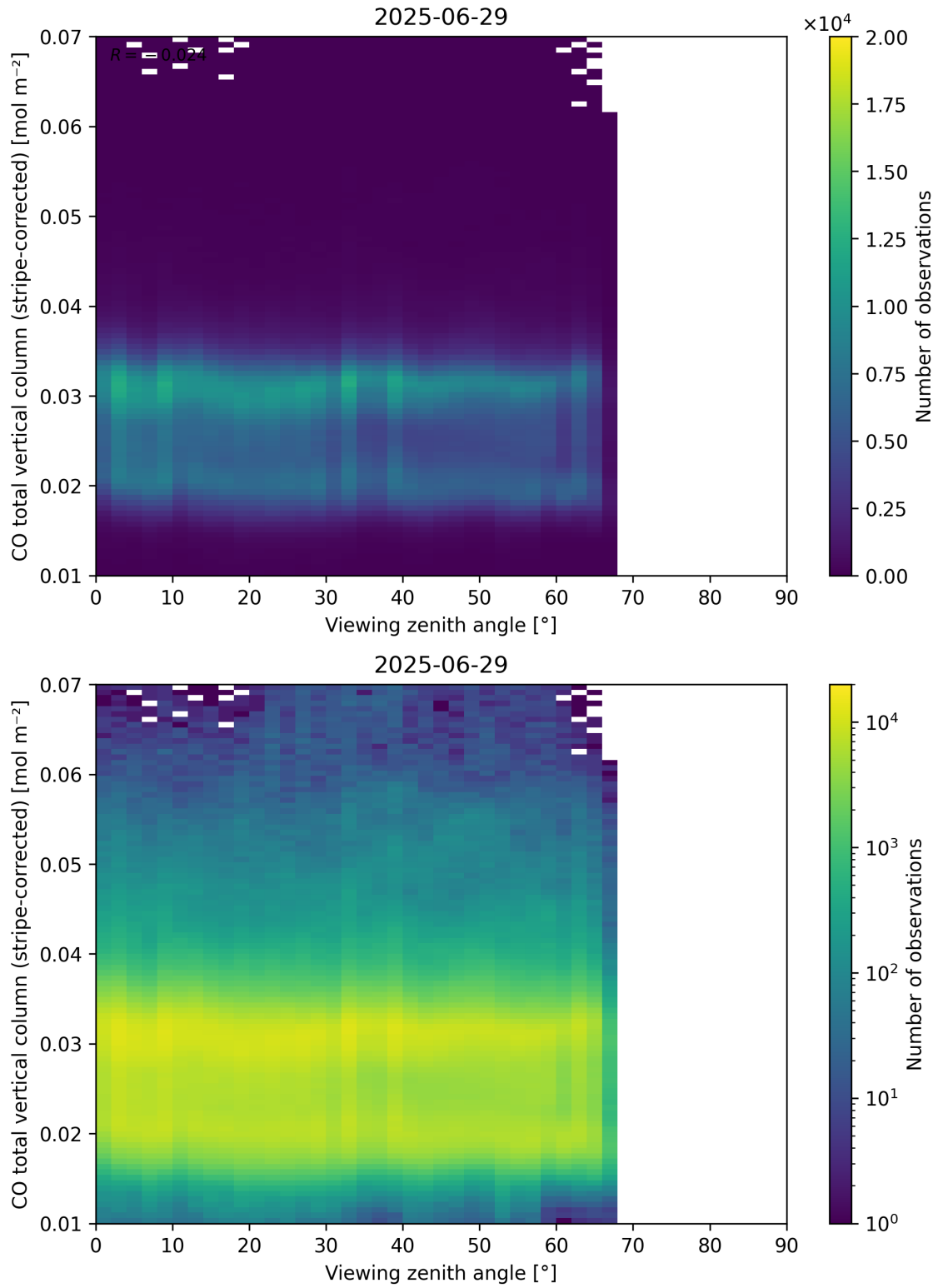
Figure 70: Scatter density plot of “Viewing zenith angle” against “CO total vertical column (stripe-corrected)” for 2025-06-28 to 2025-06-30.
