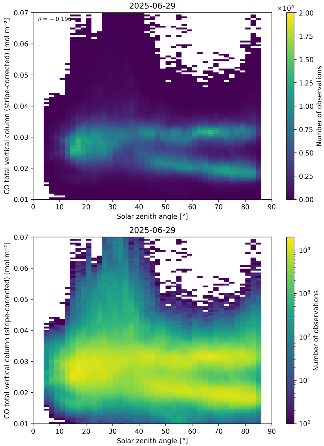
Figure 62: Scatter density plot of “Solar zenith angle” against “CO total vertical column (stripe-corrected)” for 2025-06-28 to 2025-06-30.
