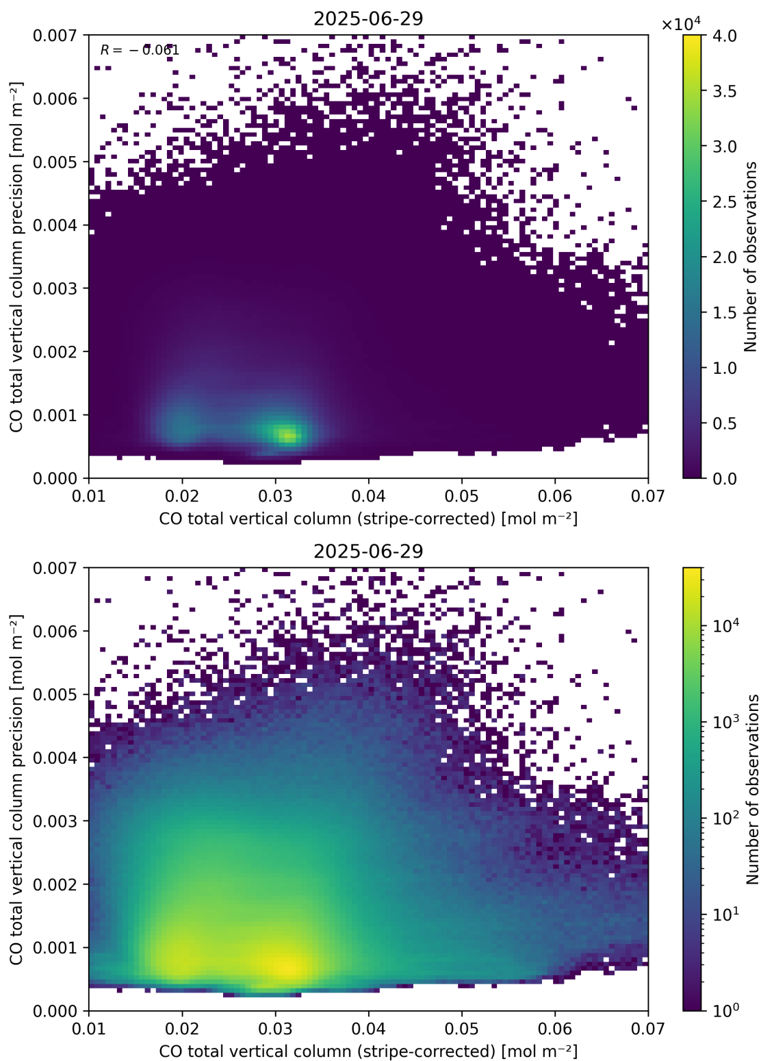
Figure 36: Scatter density plot of “CO total vertical column (stripe-corrected)” against “CO total vertical column precision” for 2025-06-28 to 2025-06-30.
