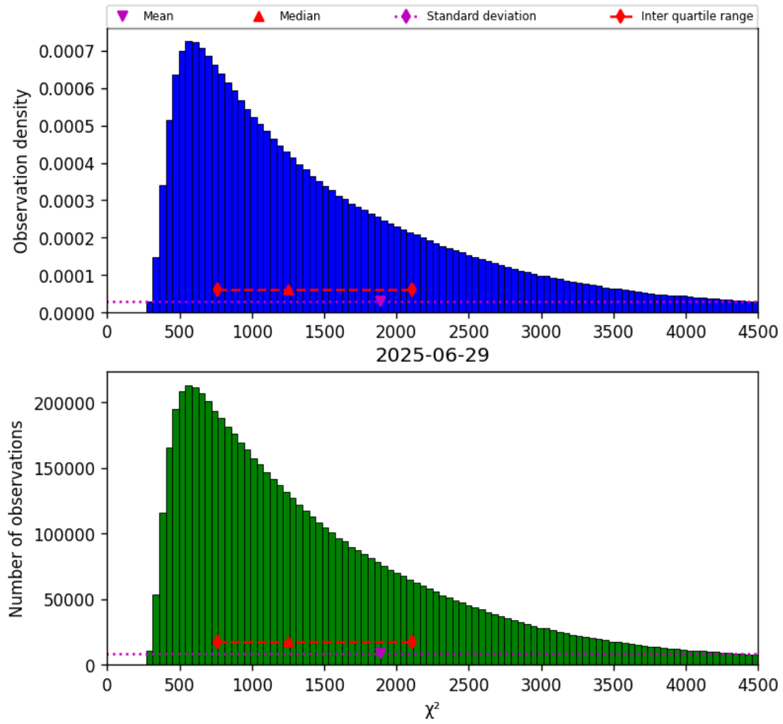
Figure 22: Histogram of “ \chi^2 ” for 2025-06-28 to 2025-06-30
