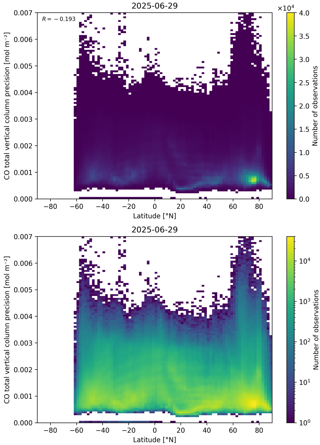
Figure 53: Scatter density plot of “Latitude” against “CO total vertical column precision” for 2025-06-28 to 2025-06-30.
