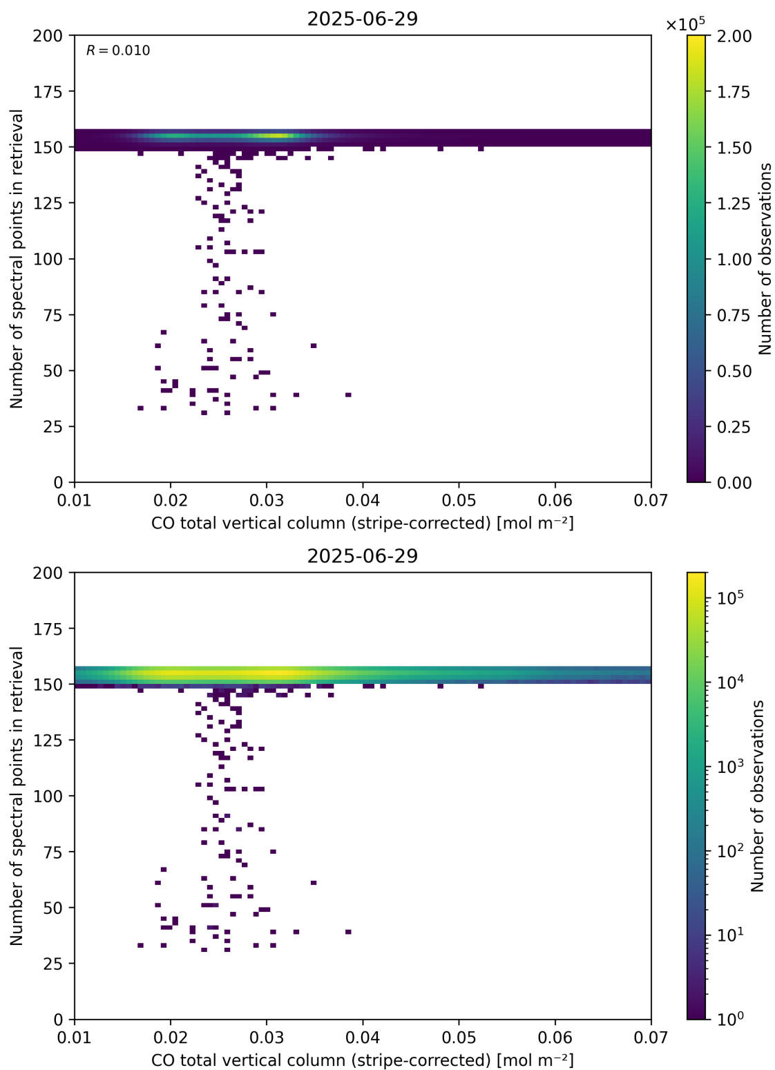
Figure 40: Scatter density plot of “CO total vertical column (stripe-corrected)” against “Number of spectral points in retrieval” for 2025-06-28 to 2025-06-30.
