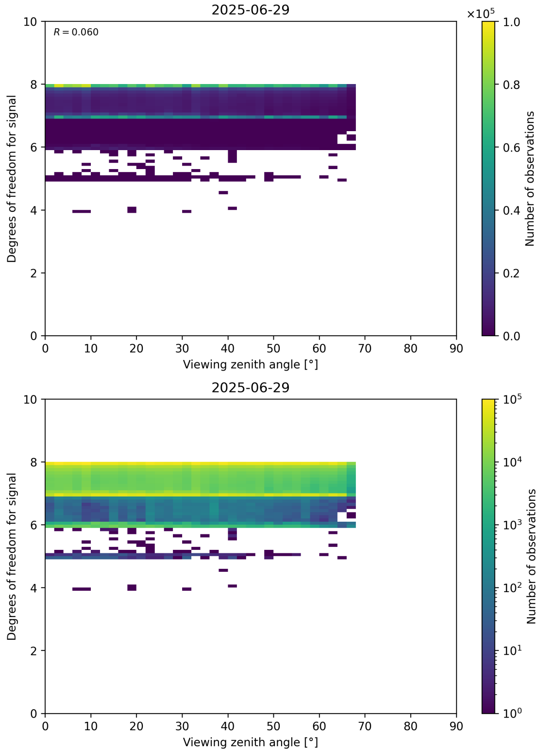
Figure 73: Scatter density plot of “Viewing zenith angle” against “Degrees of freedom for signal” for 2025-06-28 to 2025-06-30.
