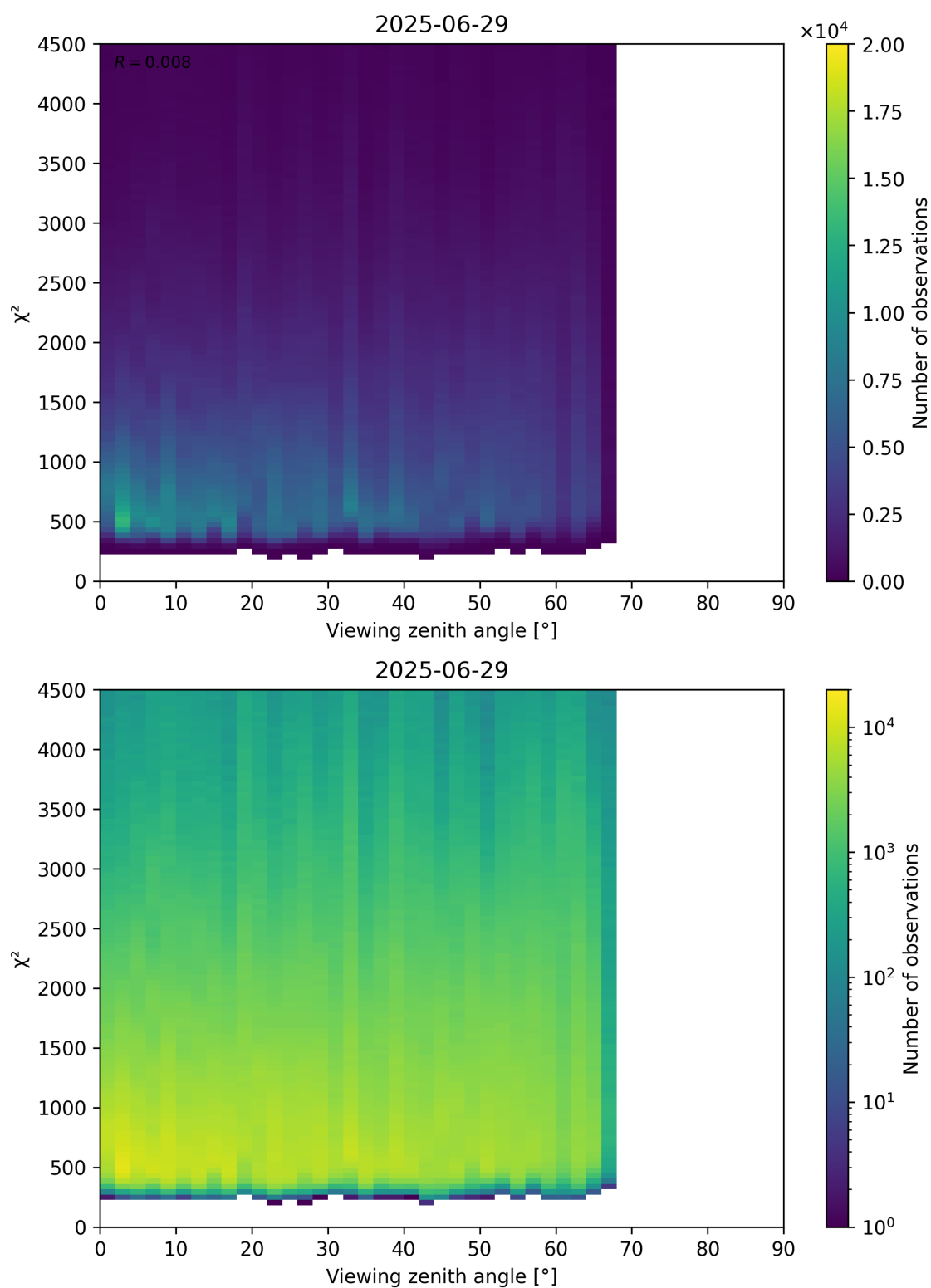
Figure 72: Scatter density plot of “Viewing zenith angle” against “ \chi^2 ” for 2025-06-28 to 2025-06-30.
