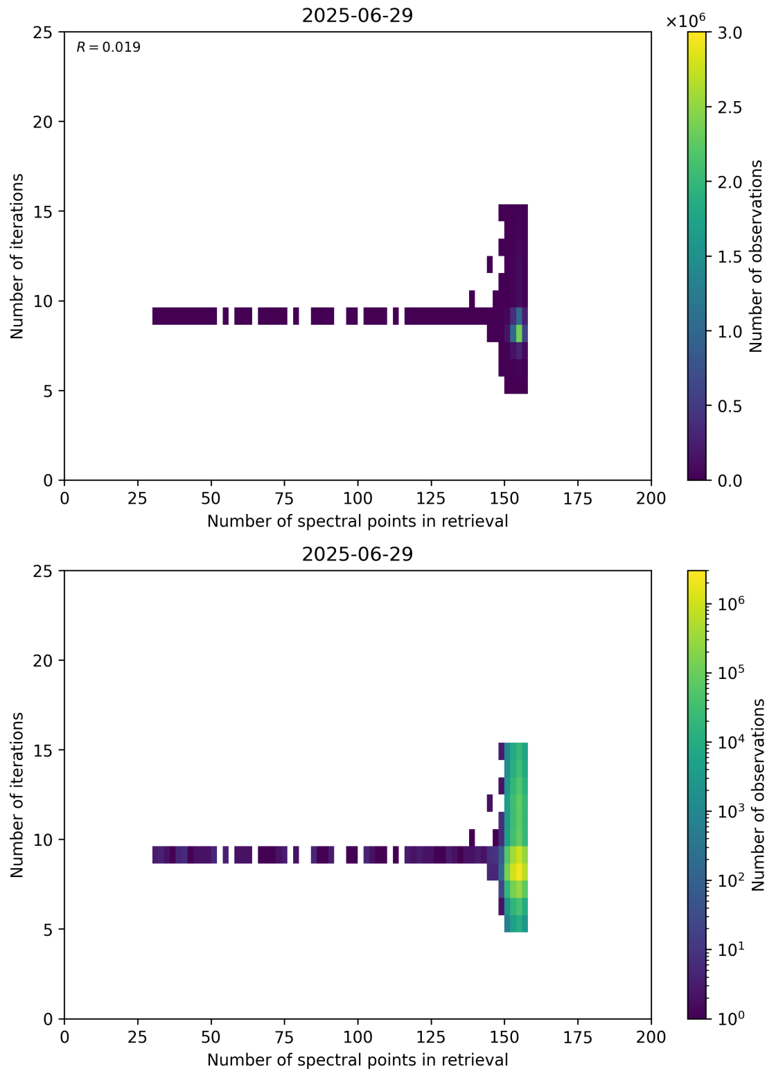
Figure 60: Scatter density plot of “Number of spectral points in retrieval” against “Number of iterations” for 2025-06-28 to 2025-06-30.
