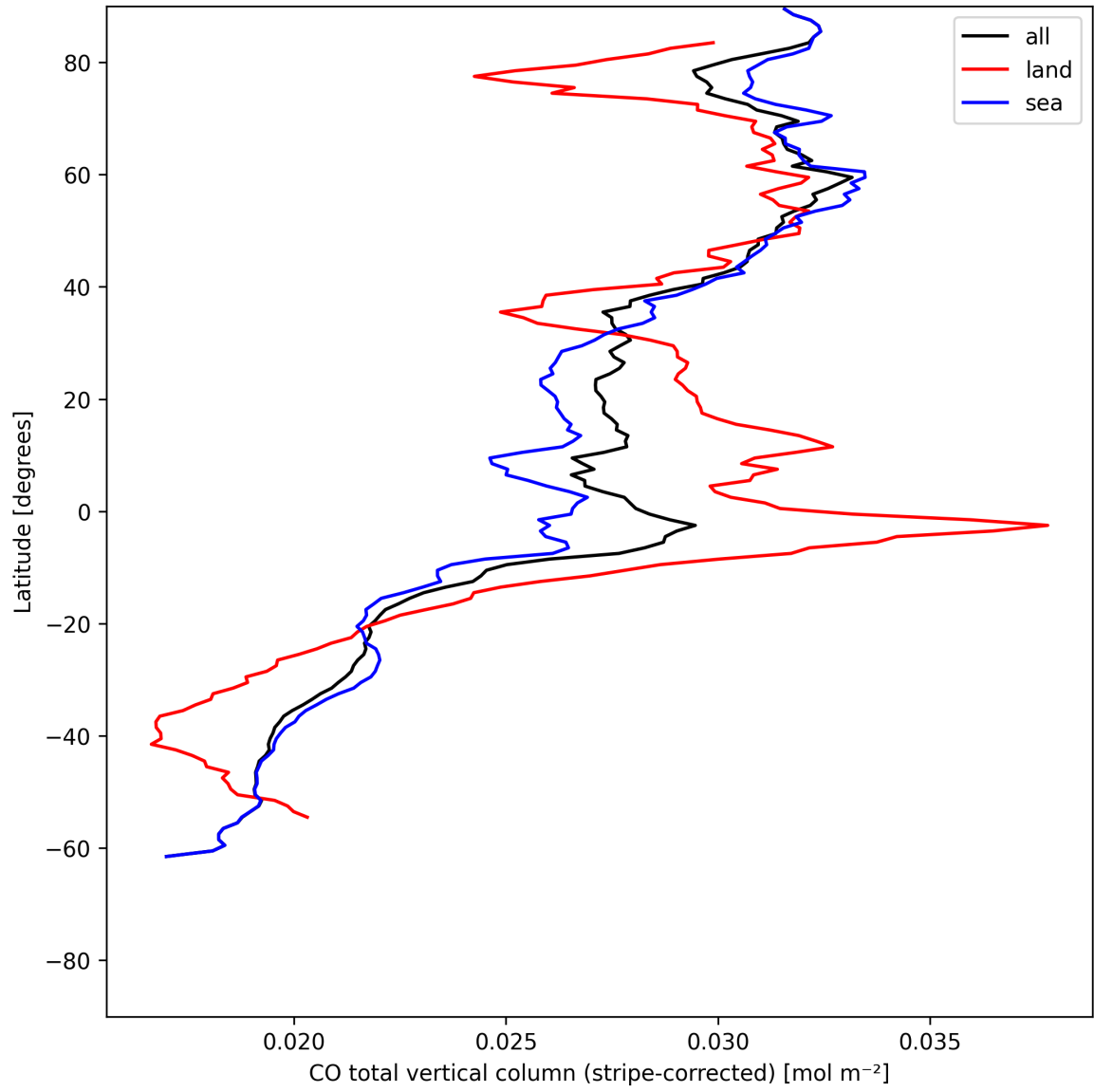
Figure 11: Zonal average of “CO total vertical column (stripe-corrected)” for 2025-06-28 to 2025-06-30.
