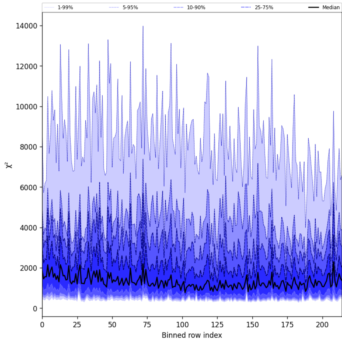
Figure 30: Along track statistics of “ \chi^2 ” for 2025-06-28 to 2025-06-30
