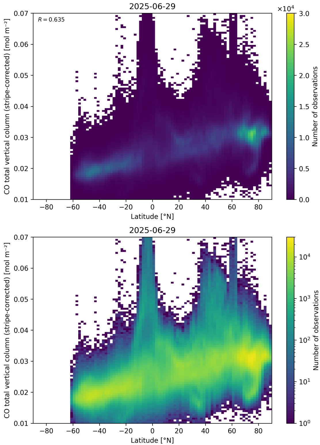
Figure 52: Scatter density plot of “Latitude” against “CO total vertical column (stripe-corrected)” for 2025-06-28 to 2025-06-30.
