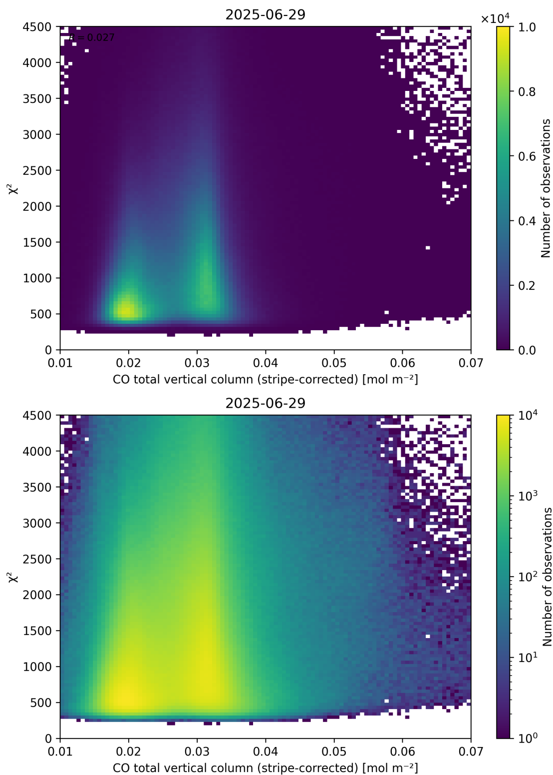
Figure 37: Scatter density plot of “CO total vertical column (stripe-corrected)” against “ \chi^2 ” for 2025-06-28 to 2025-06-30.
