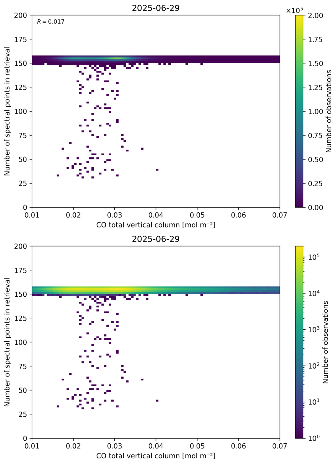
Figure 43: Scatter density plot of “CO total vertical column” against “Number of spectral points in retrieval” for 2025-06-28 to 2025-06-30.
