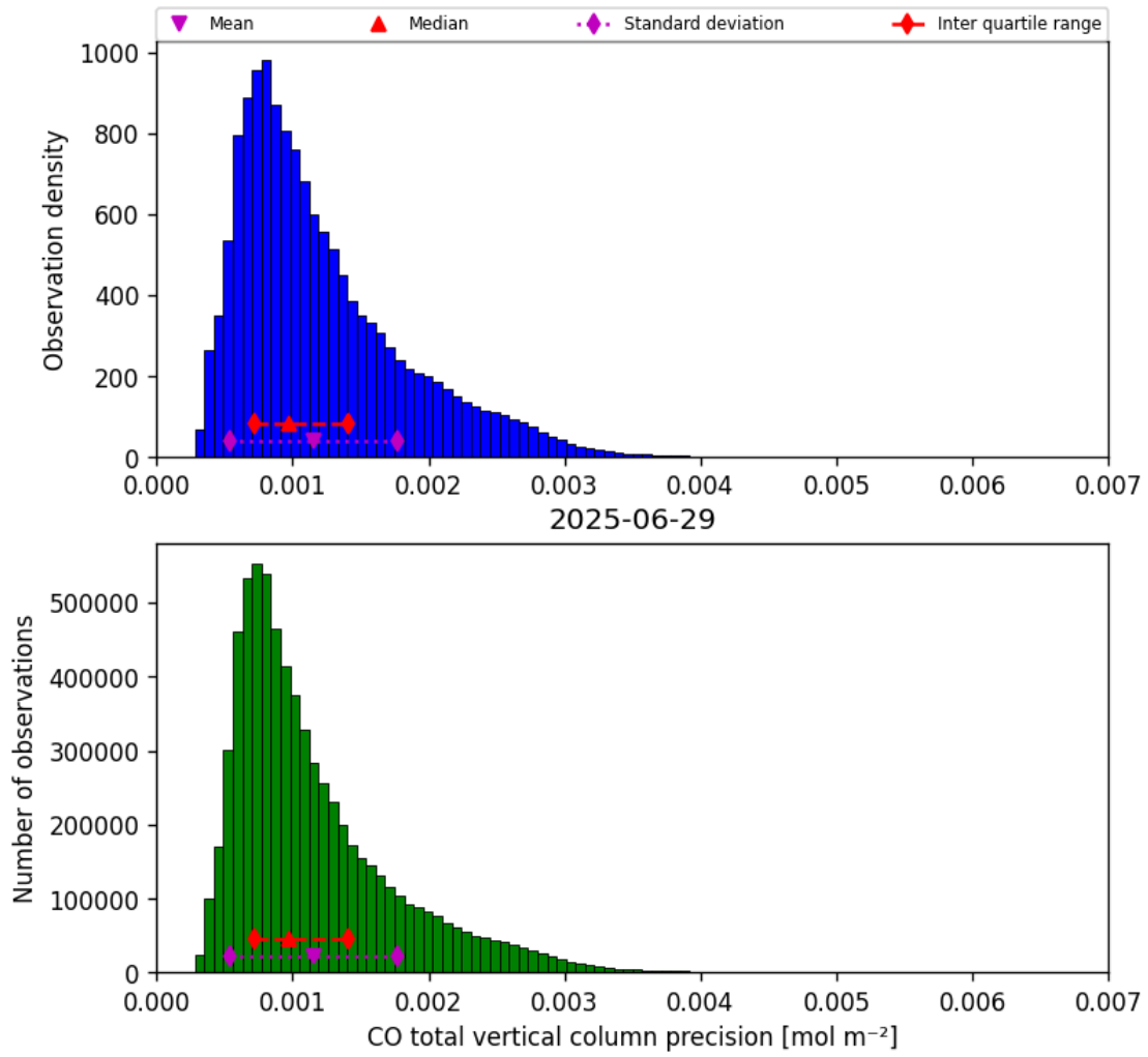
Figure 20: Histogram of “CO total vertical column precision” for 2025-06-28 to 2025-06-30
