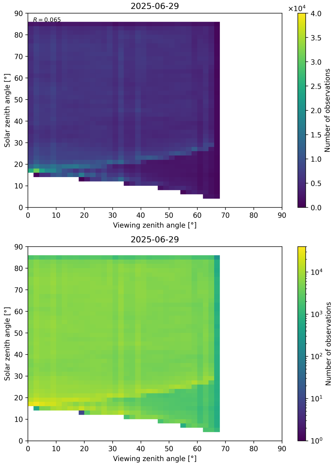
Figure 77: Scatter density plot of “Viewing zenith angle” against “Solar zenith angle” for 2025-06-28 to 2025-06-30.
