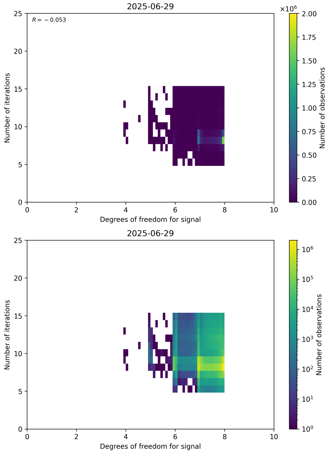
Figure 50: Scatter density plot of “Degrees of freedom for signal” against “Number of iterations” for 2025-06-28 to 2025-06-30.
