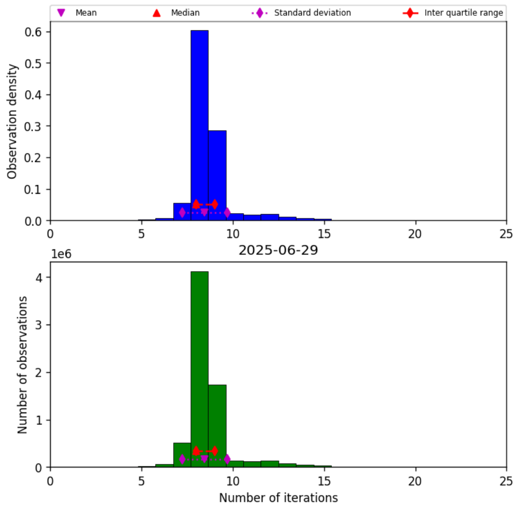
Figure 24: Histogram of “Number of iterations” for 2025-06-28 to 2025-06-30
