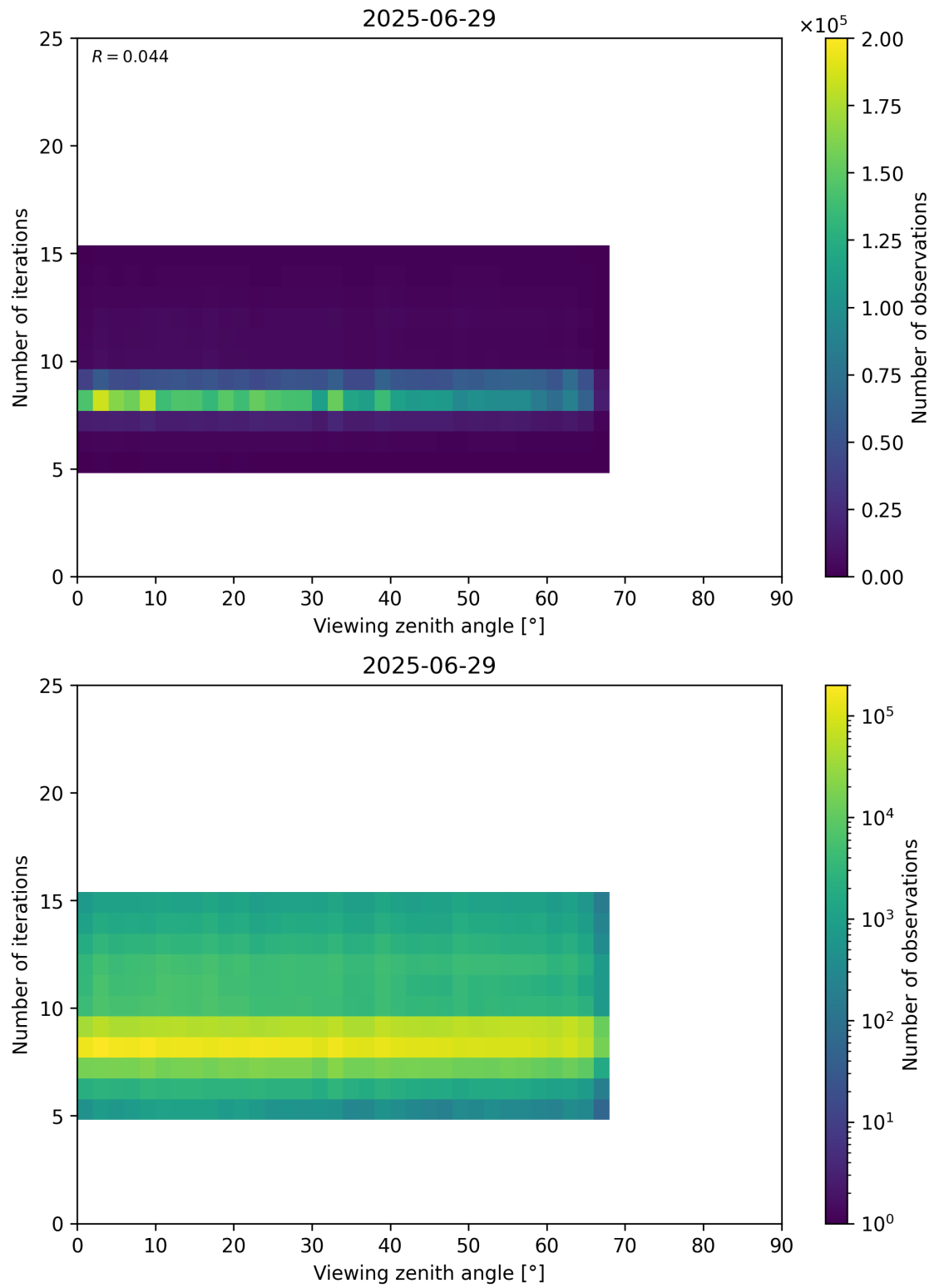
Figure 75: Scatter density plot of “Viewing zenith angle” against “Number of iterations” for 2025-06-28 to 2025-06-30.
