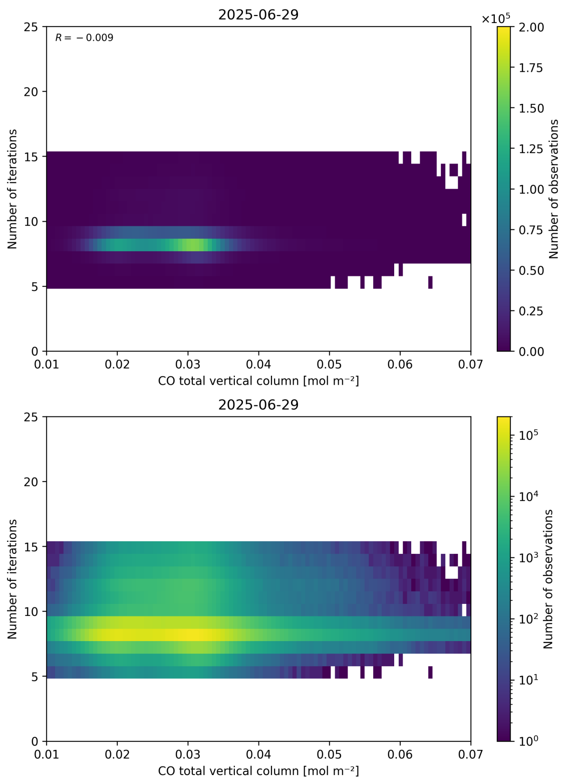
Figure 42: Scatter density plot of “CO total vertical column” against “Number of iterations” for 2025-06-28 to 2025-06-30.
