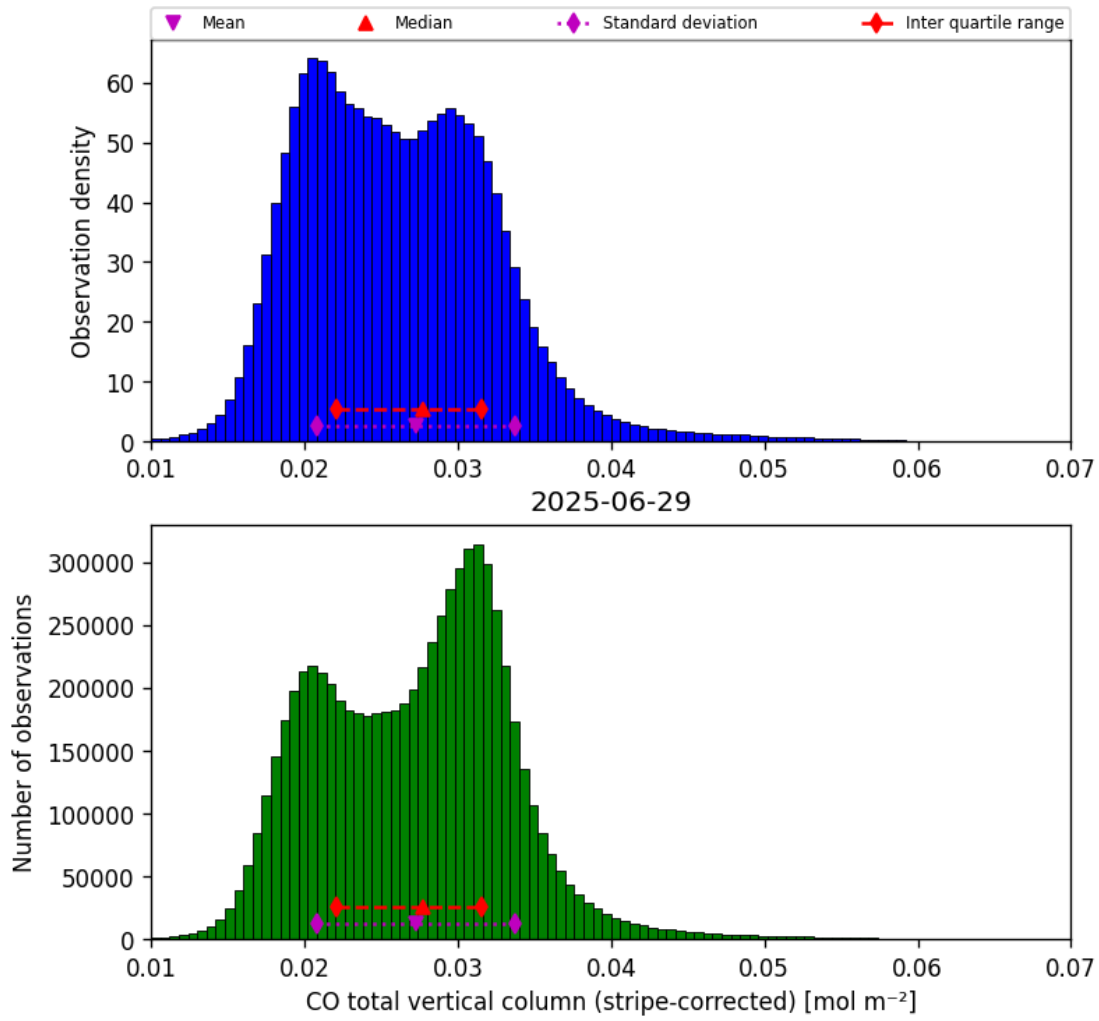
Figure 19: Histogram of “CO total vertical column (stripe-corrected)” for 2025-06-28 to 2025-06-30
