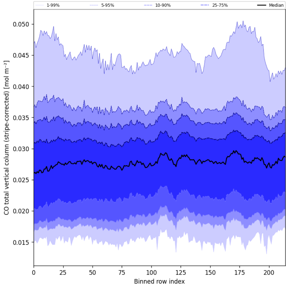
Figure 27: Along track statistics of “CO total vertical column (stripe-corrected)” for 2025-06-28 to 2025-06-30
