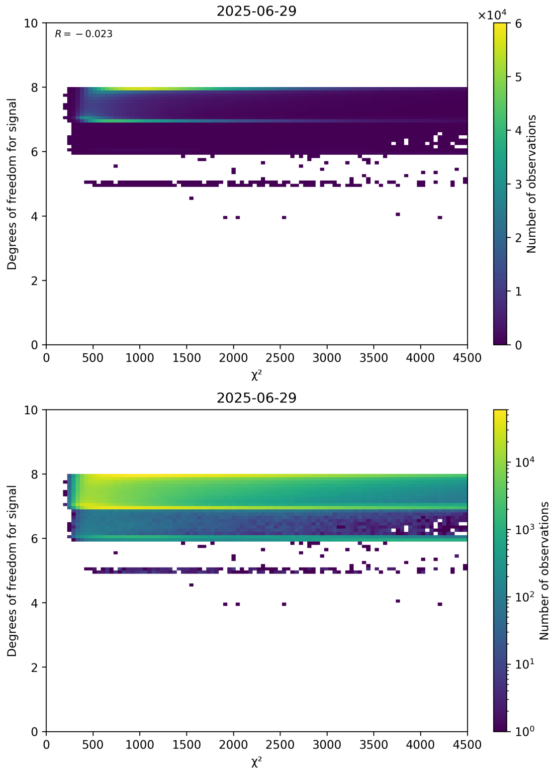
Figure 48: Scatter density plot of “ \chi^2 ” against “Degrees of freedom for signal” for 2025-06-28 to 2025-06-30.
