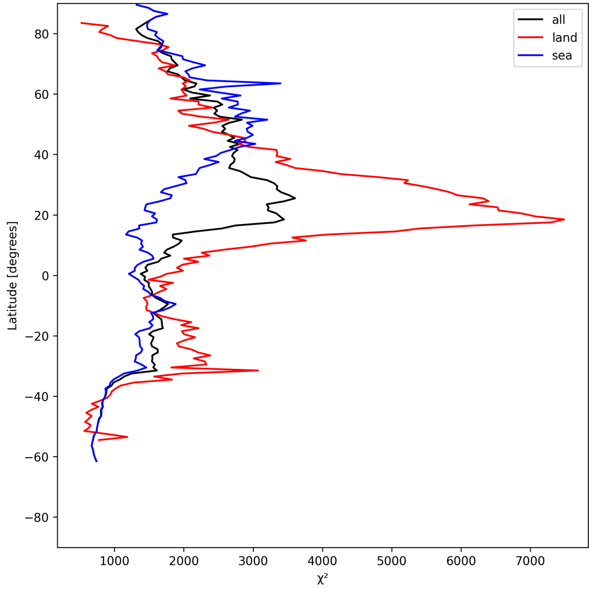
Figure 14: Zonal average of “ \chi^2 ” for 2025-06-28 to 2025-06-30.
