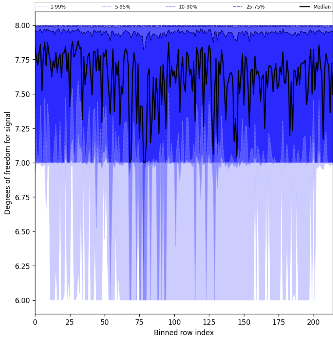
Figure 31: Along track statistics of “Degrees of freedom for signal” for 2025-06-28 to 2025-06-30
