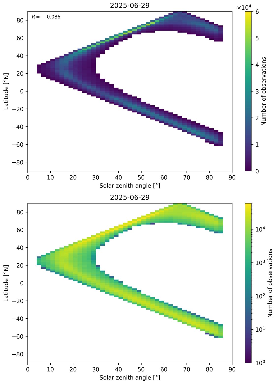
Figure 66: Scatter density plot of “Solar zenith angle” against “Latitude” for 2025-06-28 to 2025-06-30.
