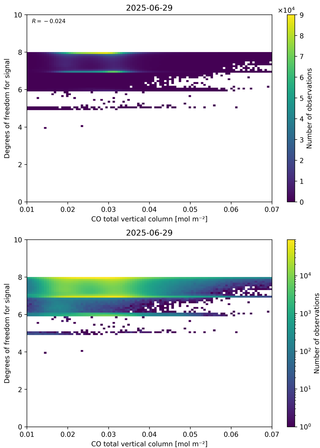
Figure 41: Scatter density plot of “CO total vertical column” against “Degrees of freedom for signal” for 2025-06-28 to 2025-06-30.
