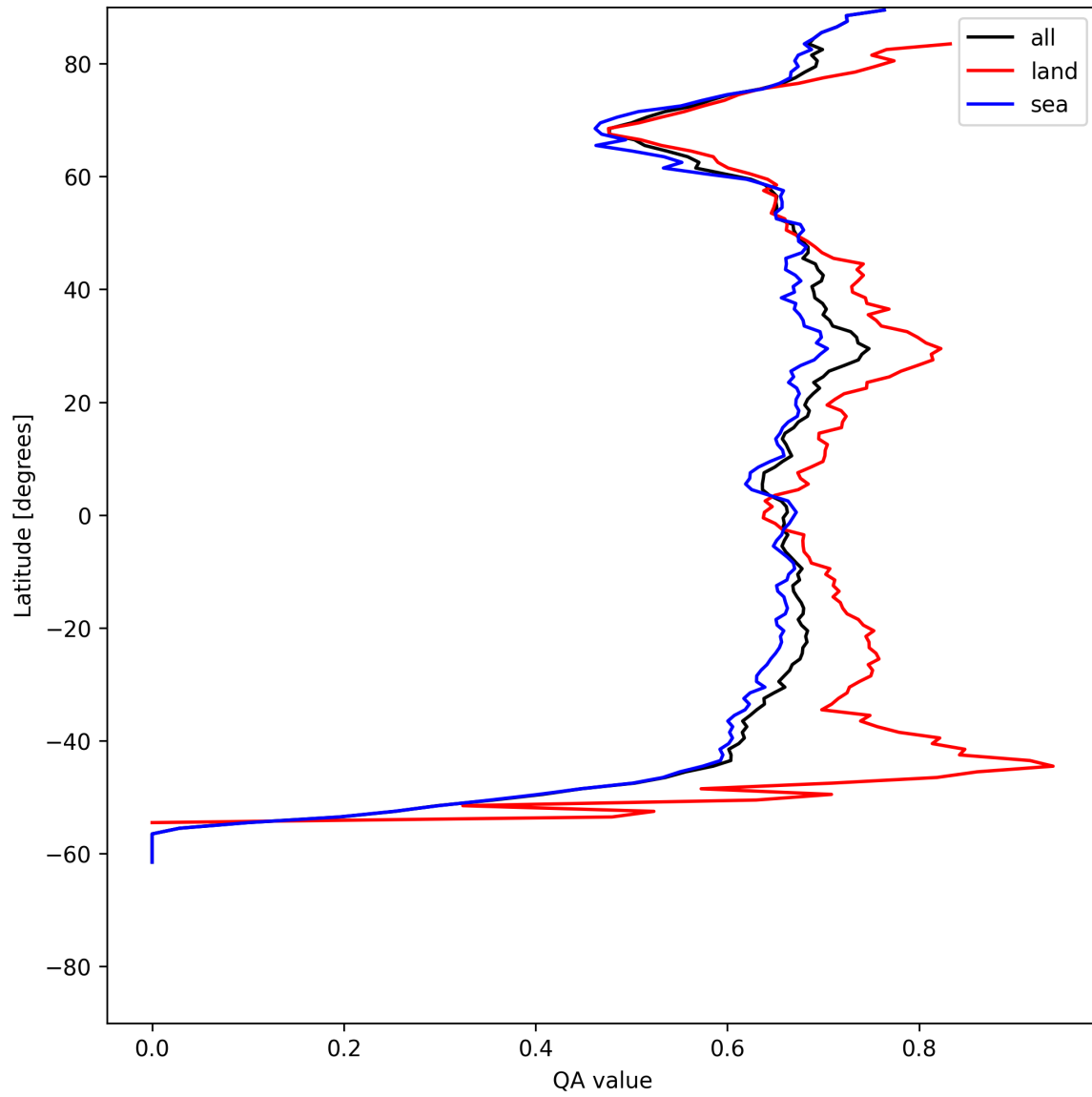
Figure 9: Zonal average of “QA value” for 2025-06-28 to 2025-06-30.
