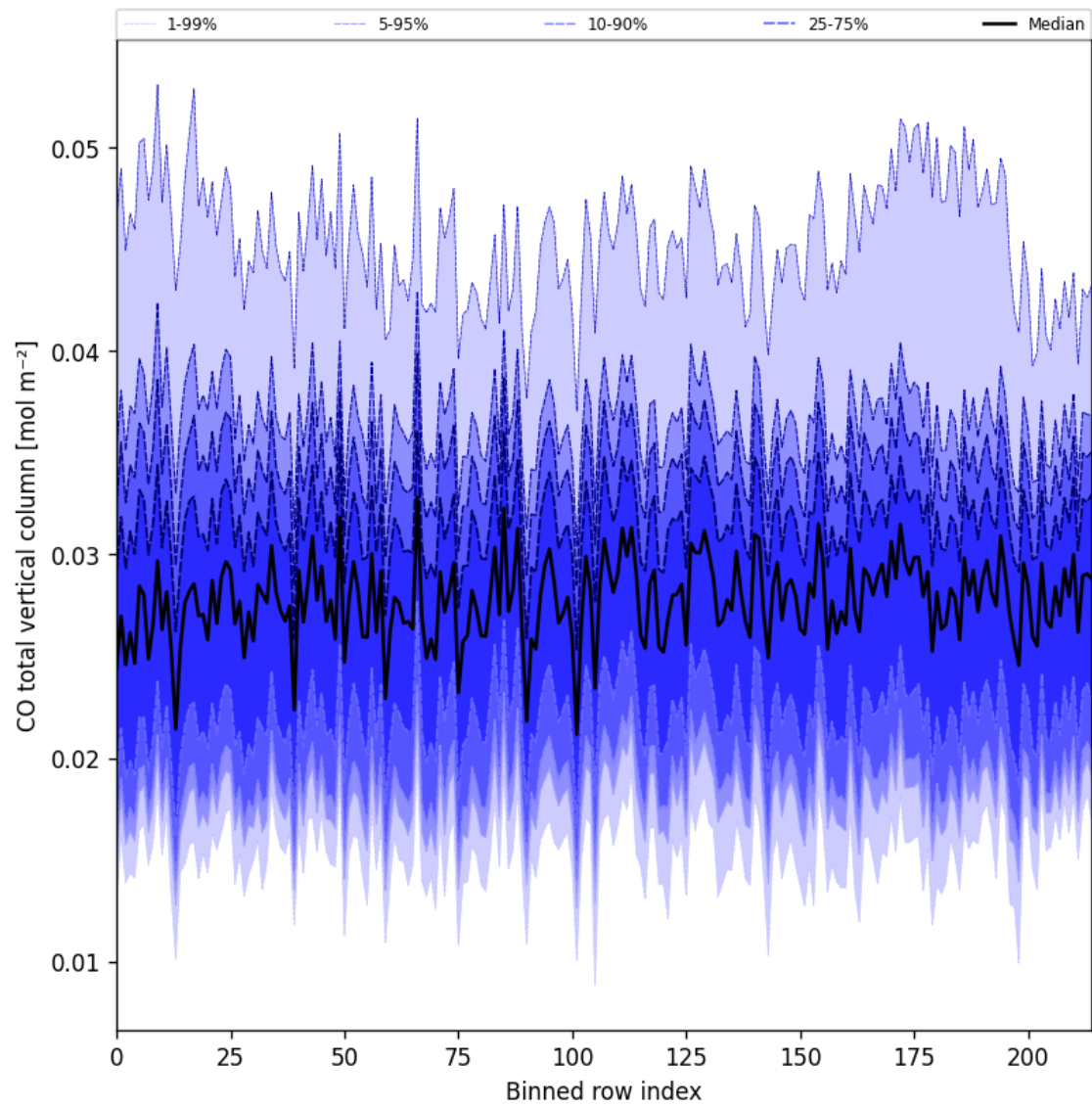
Figure 26: Along track statistics of “CO total vertical column” for 2025-06-28 to 2025-06-30
