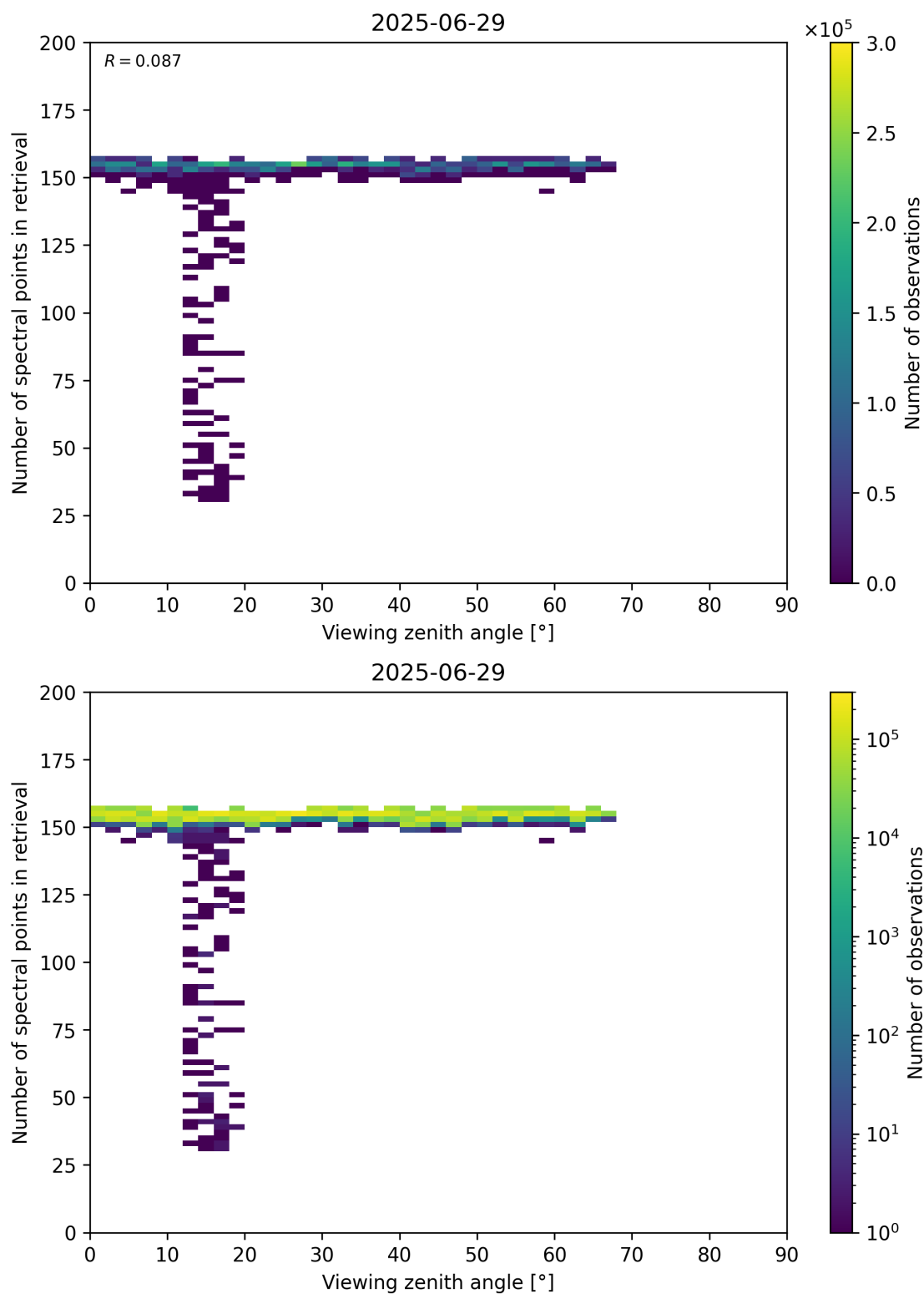
Figure 76: Scatter density plot of “Viewing zenith angle” against “Number of spectral points in retrieval” for 2025-06-28 to 2025-06-30.
