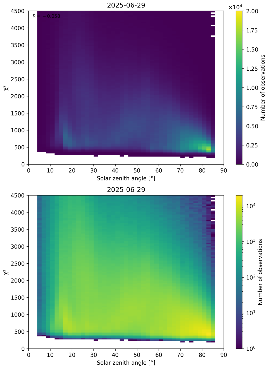
Figure 64: Scatter density plot of “Solar zenith angle” against “ \chi^2 ” for 2025-06-28 to 2025-06-30.
