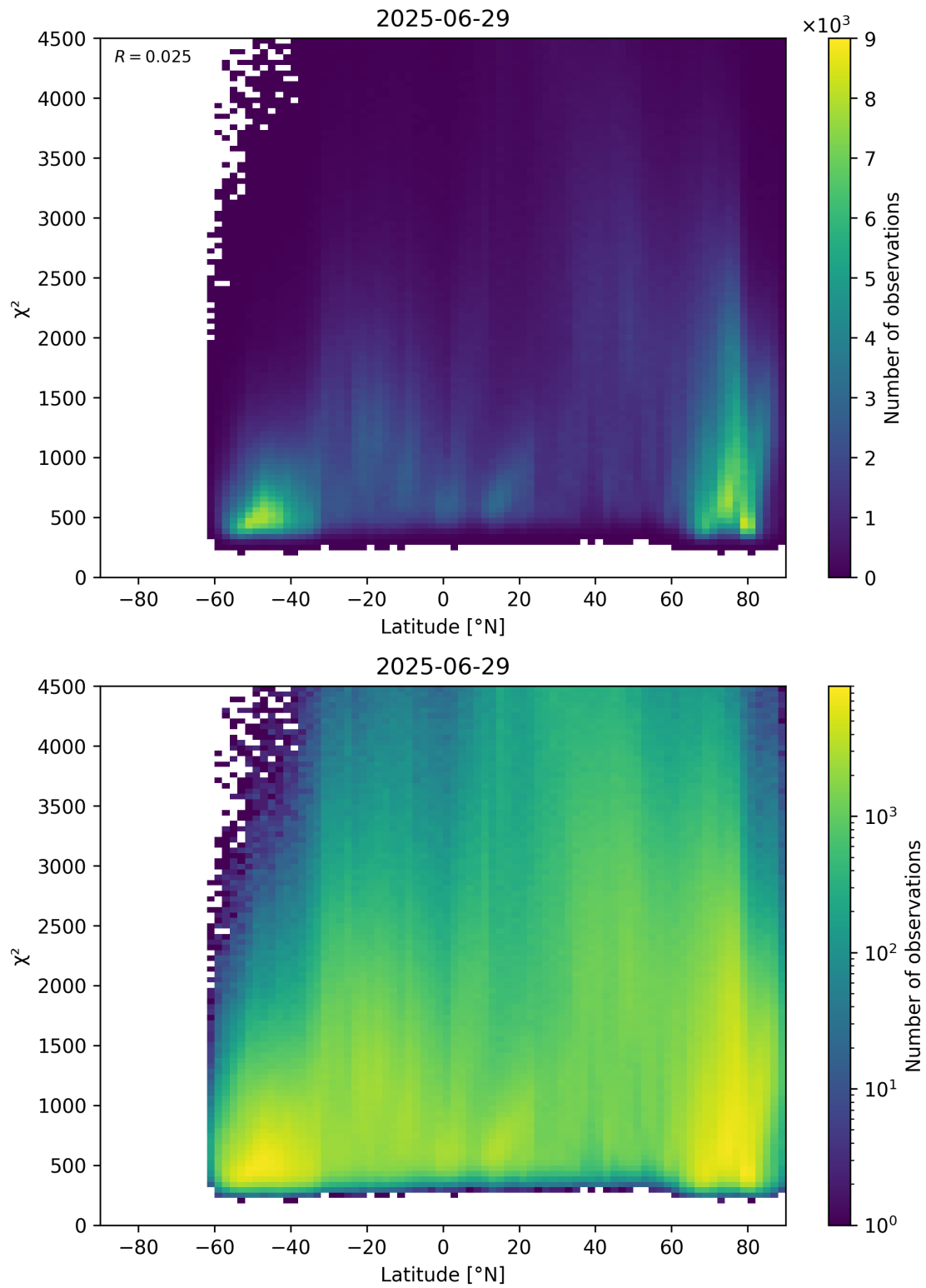
Figure 54: Scatter density plot of “Latitude” against “ \chi^2 ” for 2025-06-28 to 2025-06-30.
