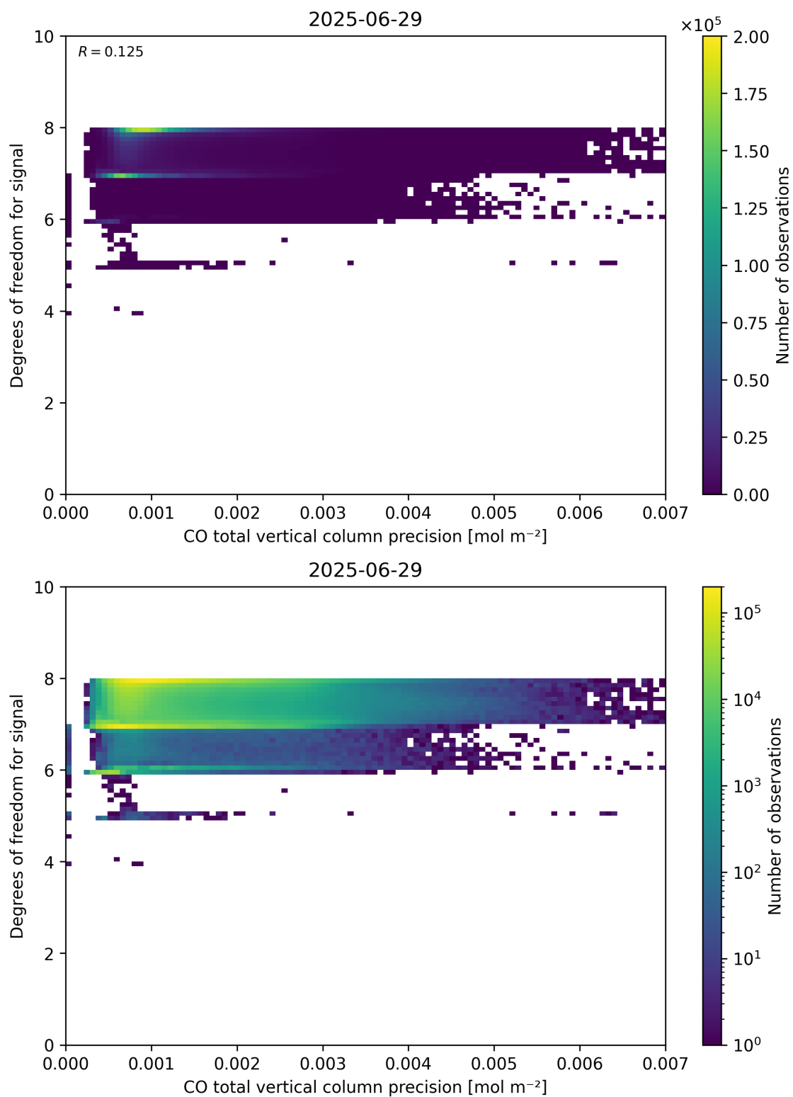
Figure 45: Scatter density plot of “CO total vertical column precision” against “Degrees of freedom for signal” for 2025-06-28 to 2025-06-30.
