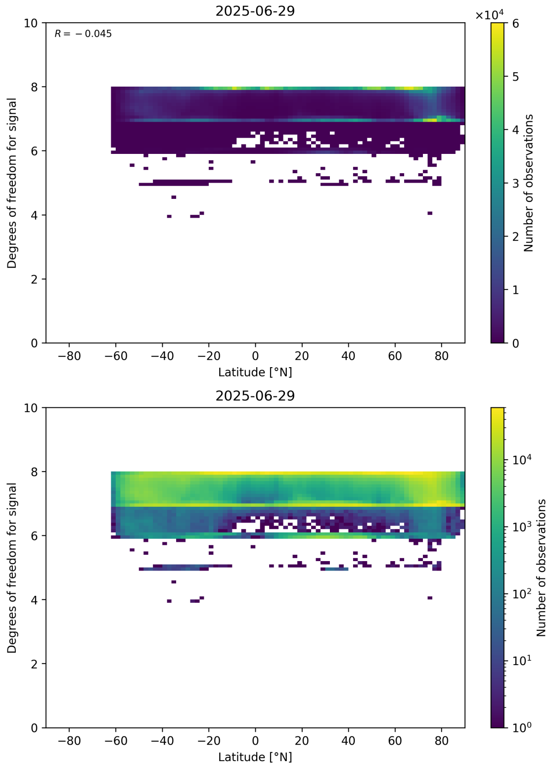
Figure 55: Scatter density plot of “Latitude” against “Degrees of freedom for signal” for 2025-06-28 to 2025-06-30.
