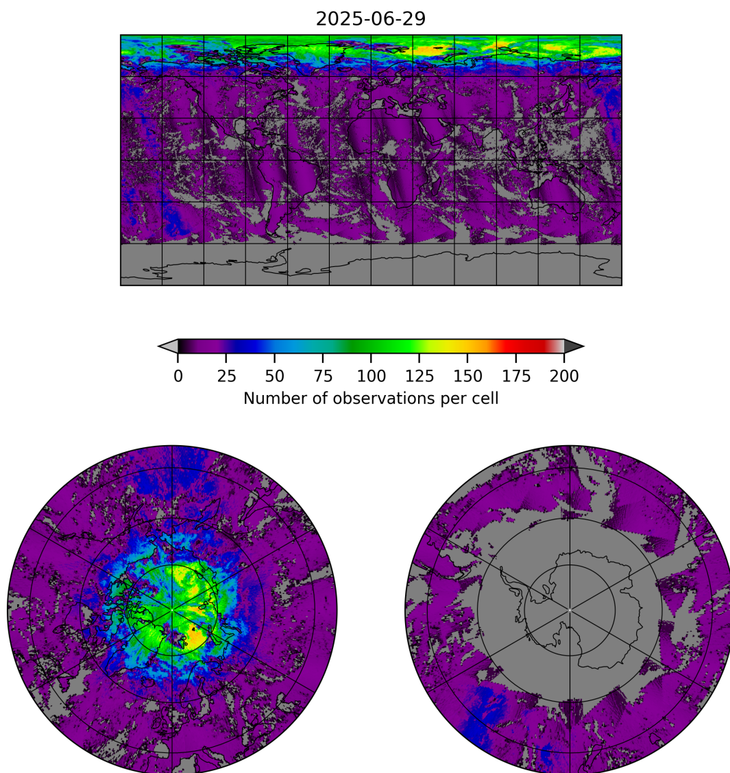
Figure 8: Map of the number of observations for 2025-06-28 to 2025-06-30
