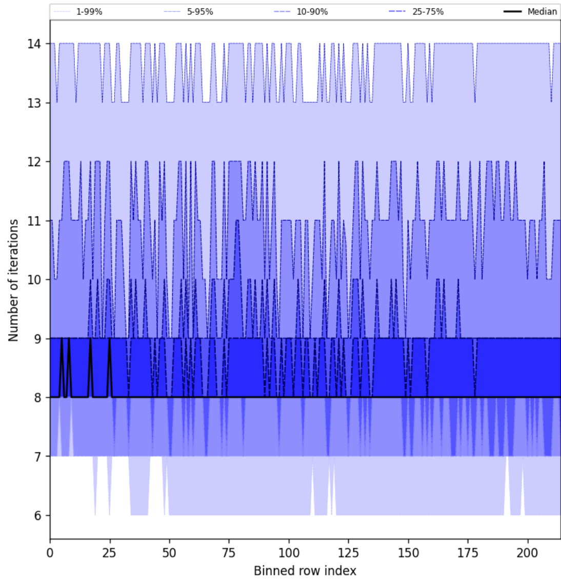
Figure 32: Along track statistics of “Number of iterations” for 2025-06-28 to 2025-06-30
