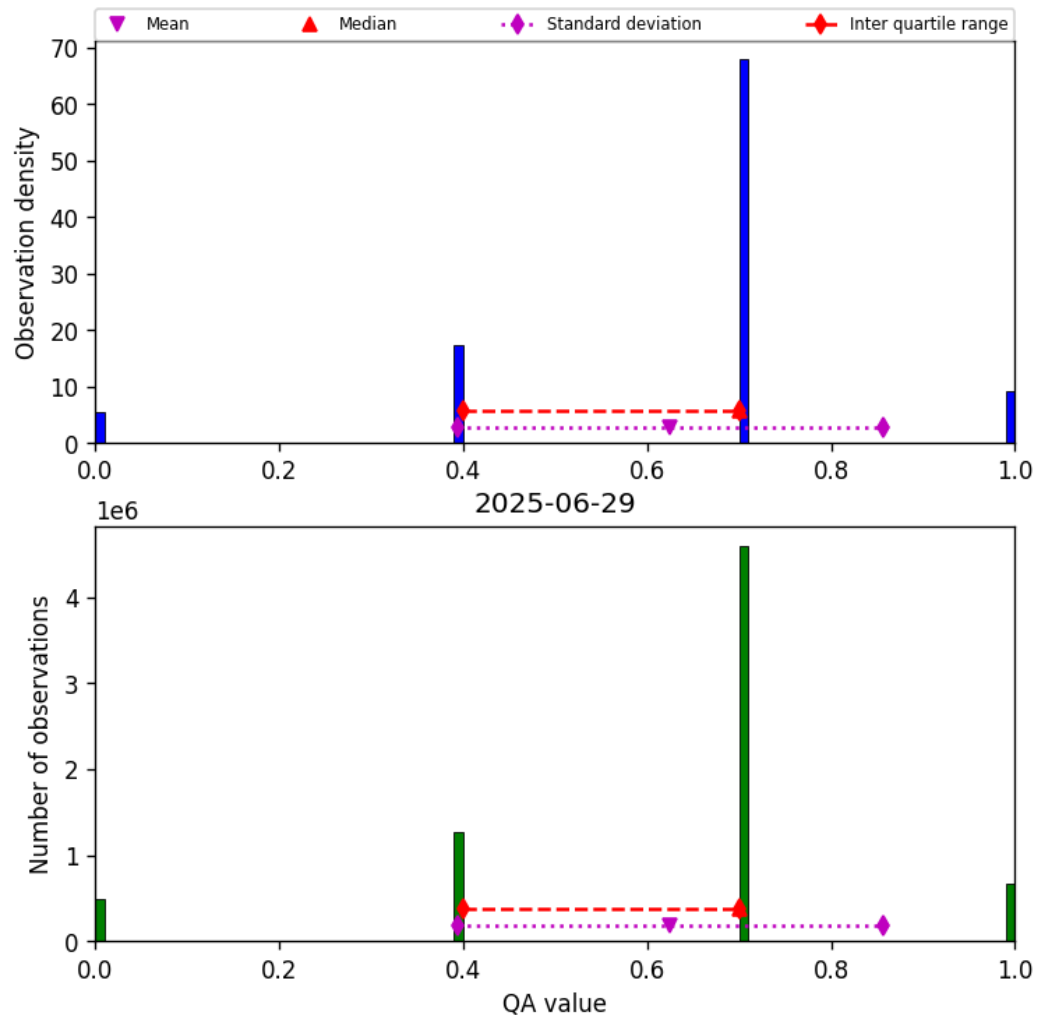
Figure 17: Histogram of “QA value” for 2025-06-28 to 2025-06-30
