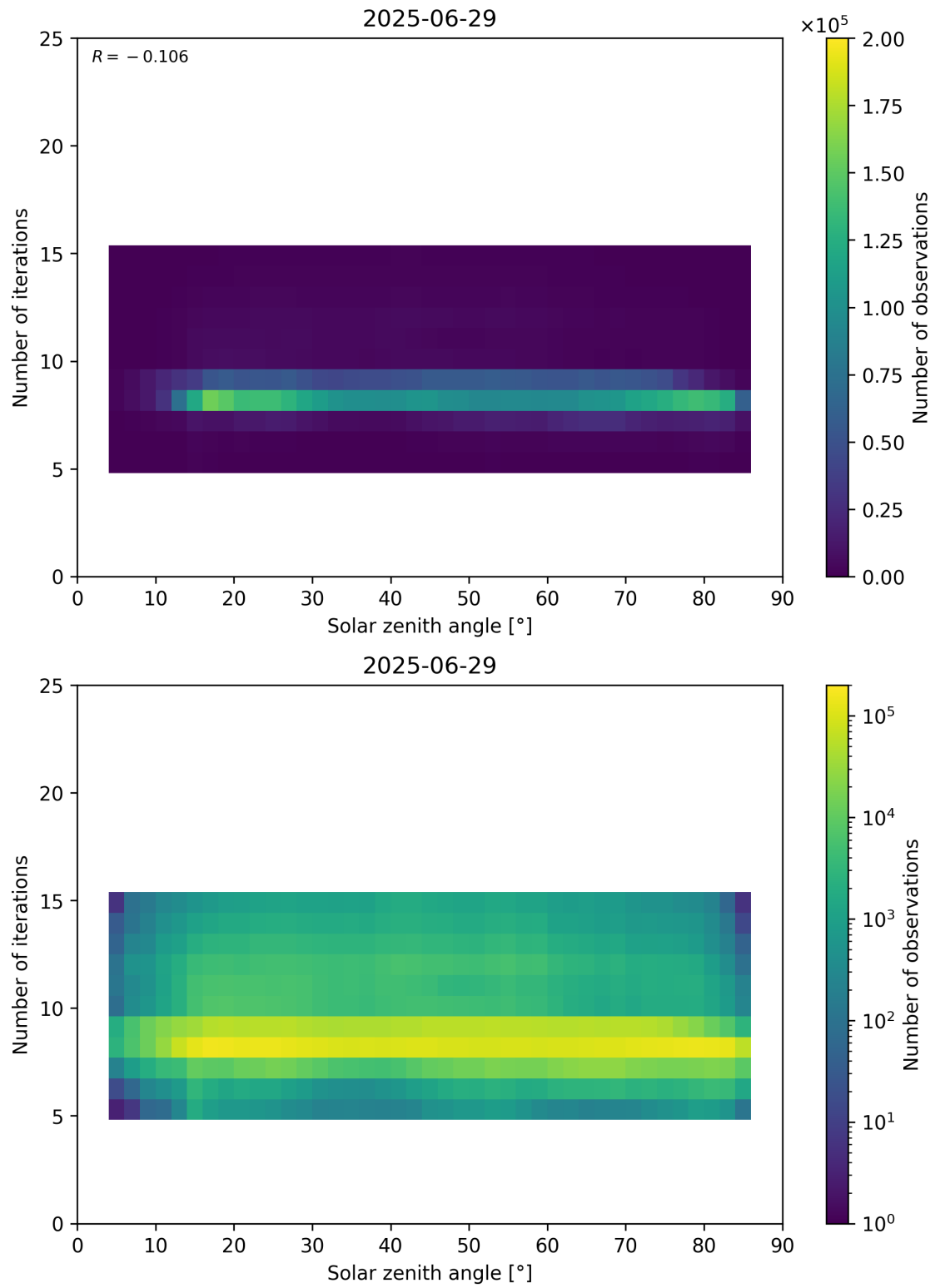
Figure 67: Scatter density plot of “Solar zenith angle” against “Number of iterations” for 2025-06-28 to 2025-06-30.
