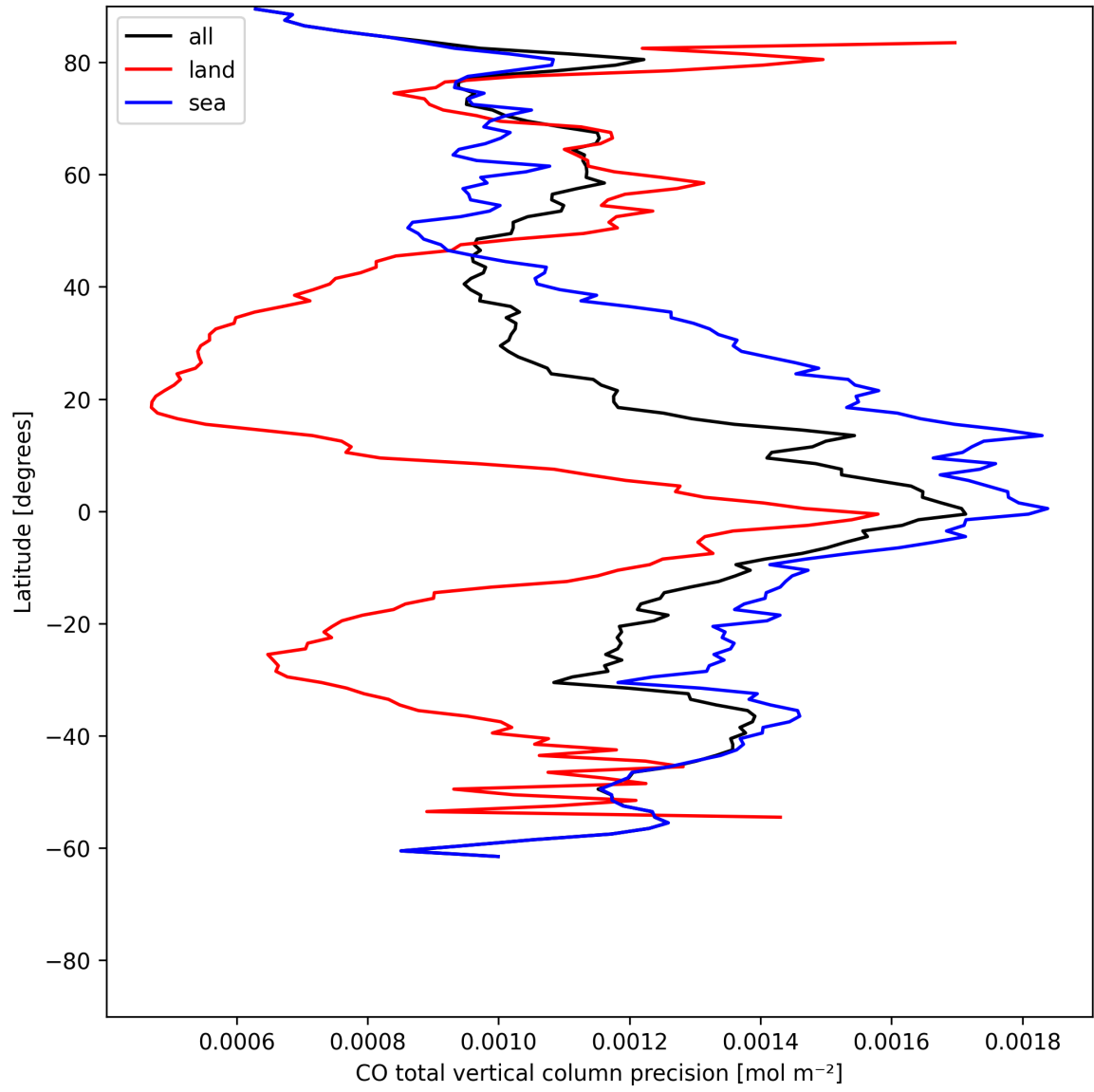
Figure 12: Zonal average of “CO total vertical column precision” for 2025-06-28 to 2025-06-30.
