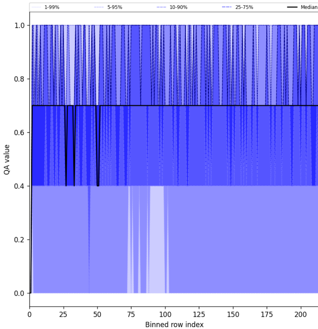
Figure 25: Along track statistics of “QA value” for 2025-06-28 to 2025-06-30
