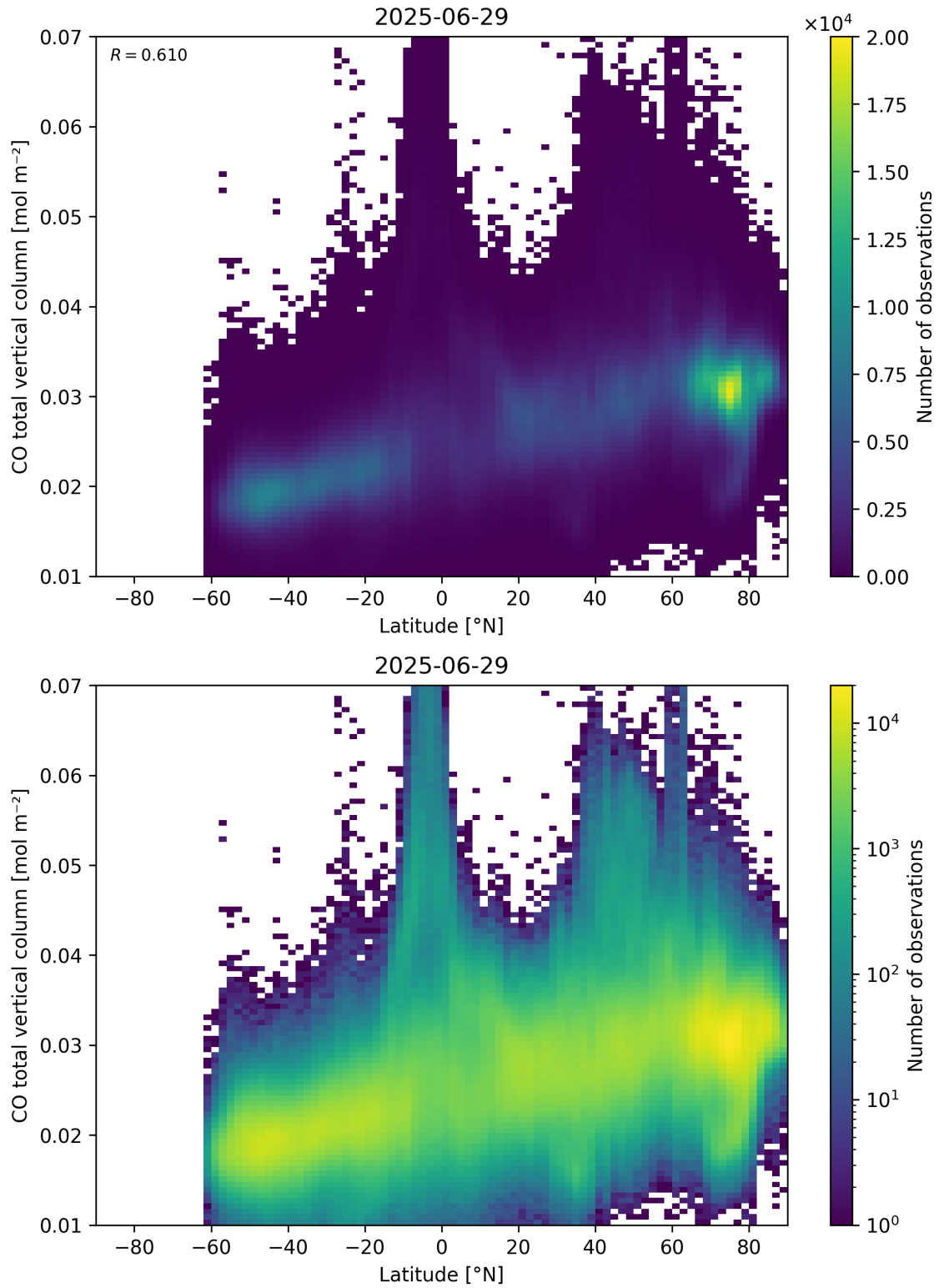
Figure 51: Scatter density plot of “Latitude” against “CO total vertical column” for 2025-06-28 to 2025-06-30.
