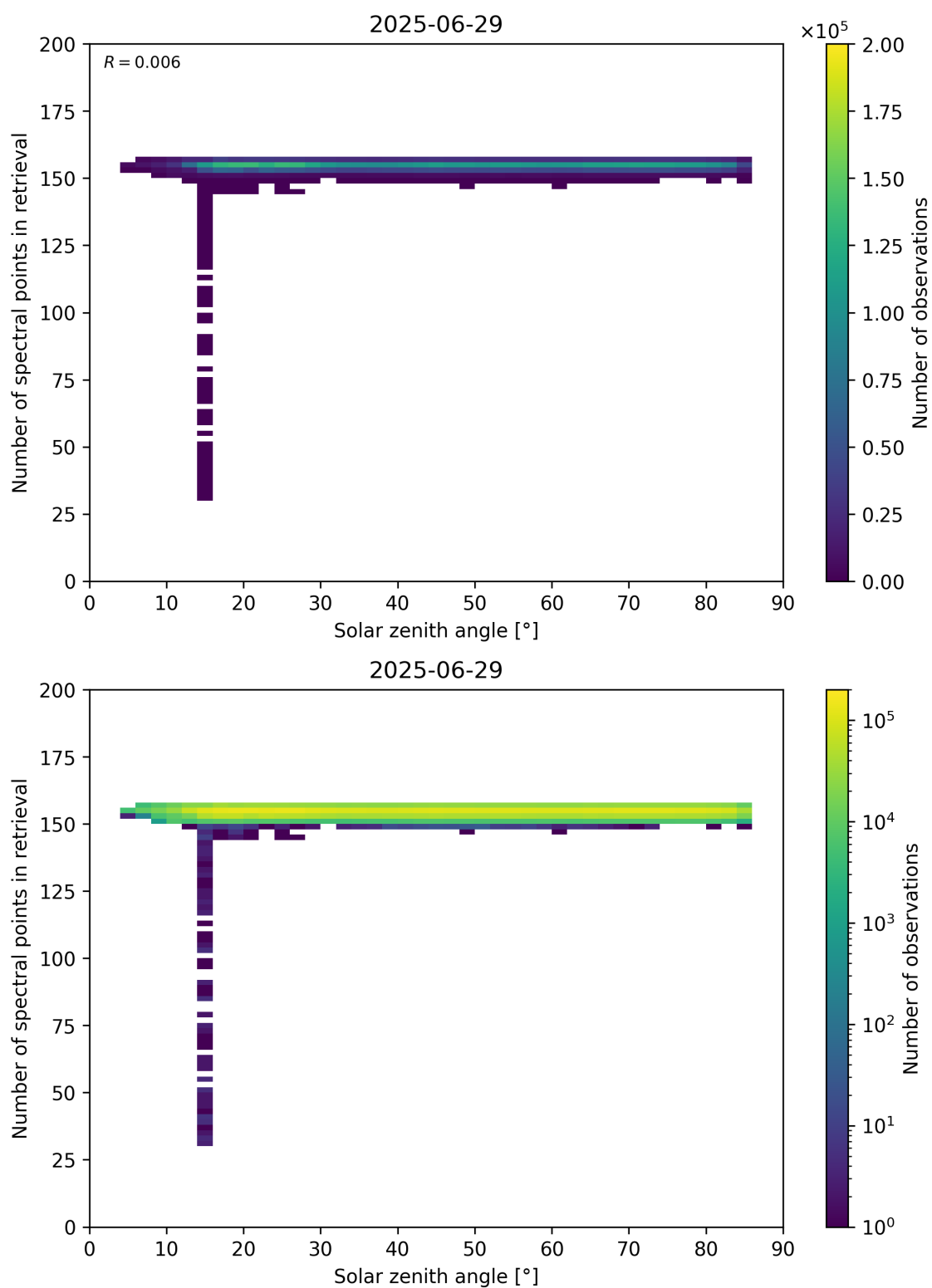
Figure 68: Scatter density plot of “Solar zenith angle” against “Number of spectral points in retrieval” for 2025-06-28 to 2025-06-30.
