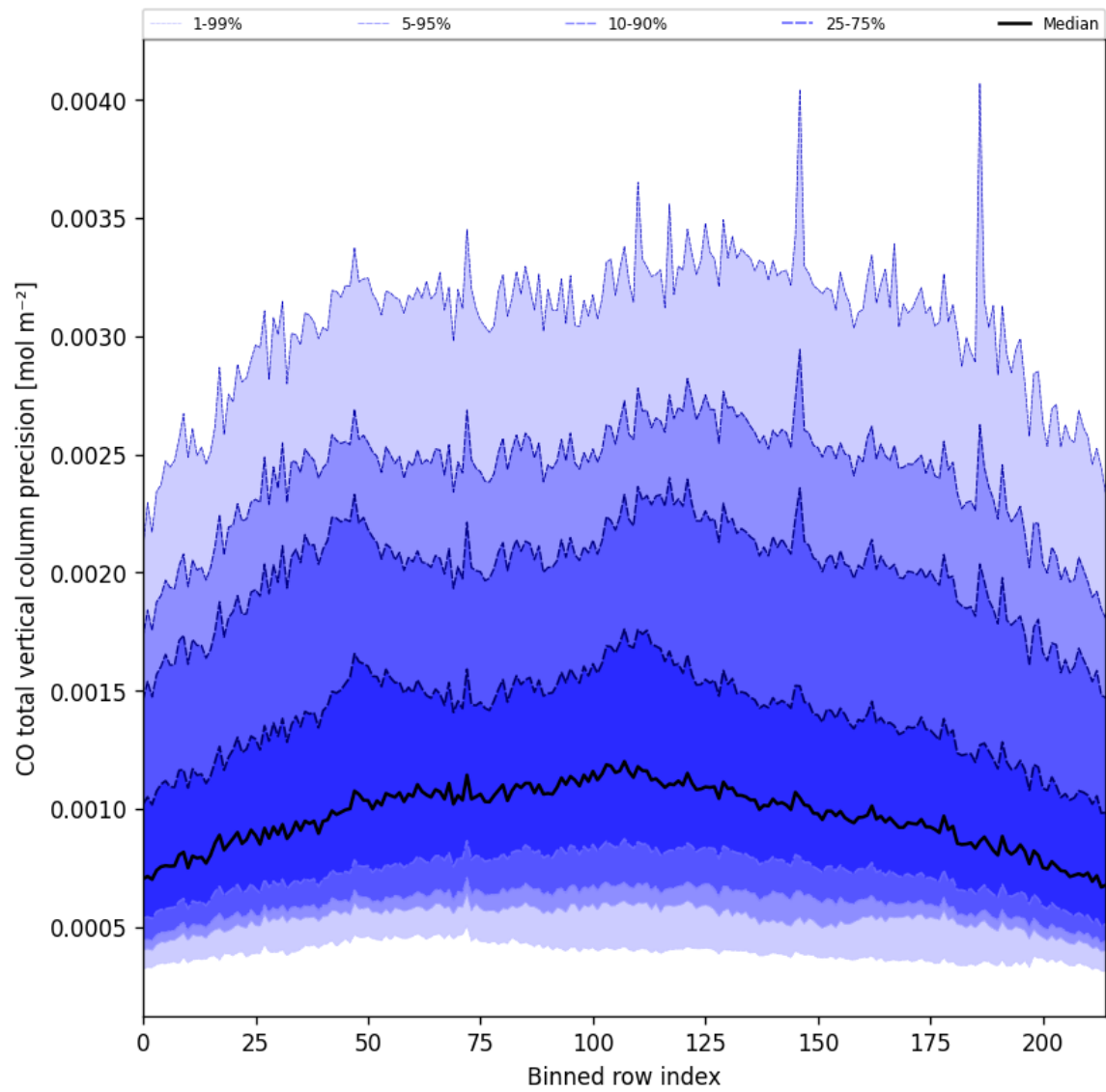
Figure 28: Along track statistics of “CO total vertical column precision” for 2025-06-28 to 2025-06-30
