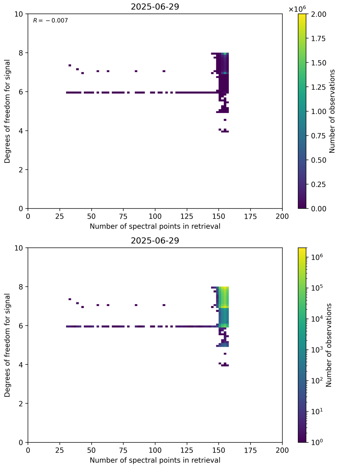
Figure 59: Scatter density plot of “Number of spectral points in retrieval” against “Degrees of freedom for signal” for 2025-06-28 to 2025-06-30.
