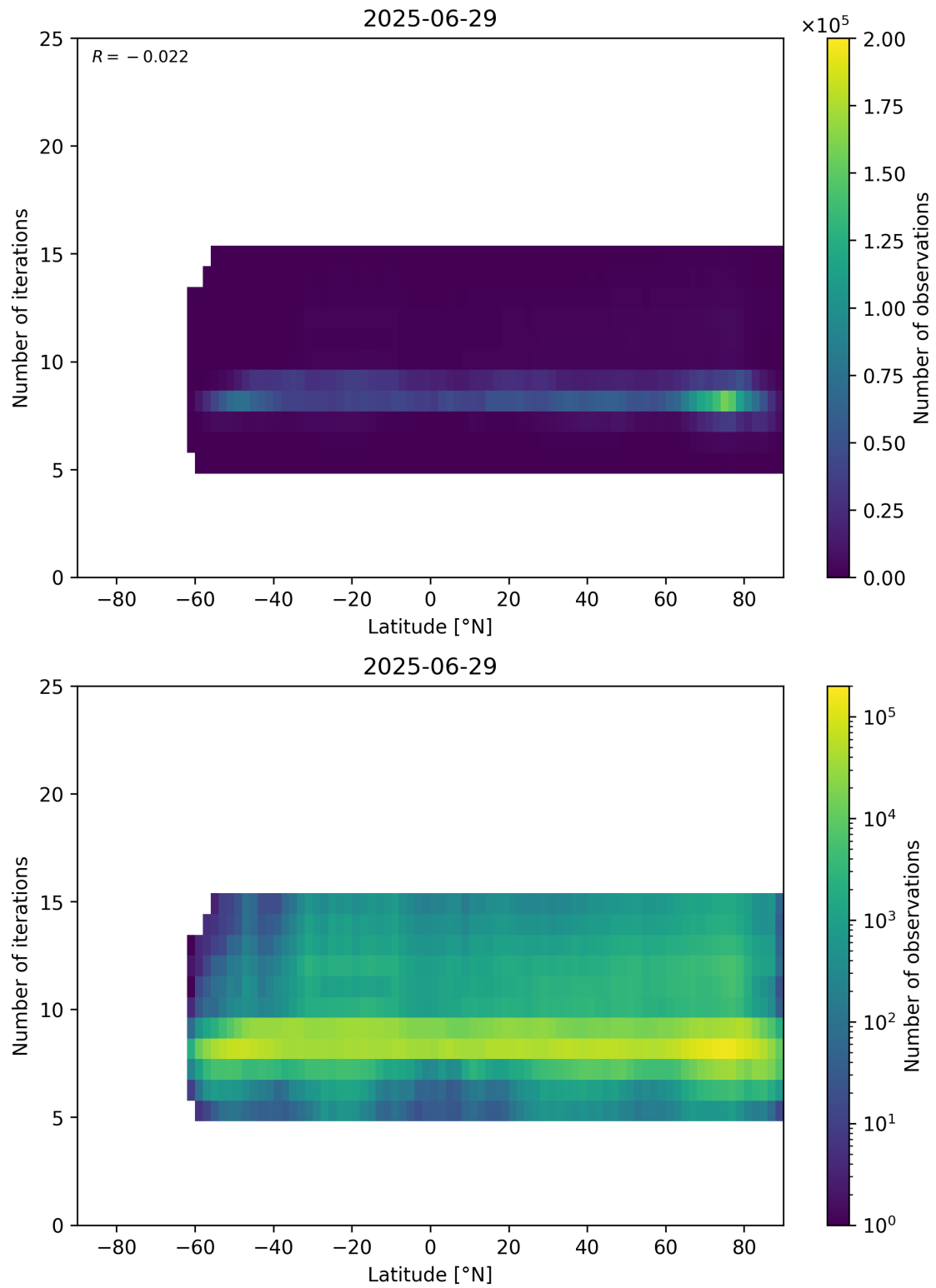
Figure 56: Scatter density plot of “Latitude” against “Number of iterations” for 2025-06-28 to 2025-06-30.
