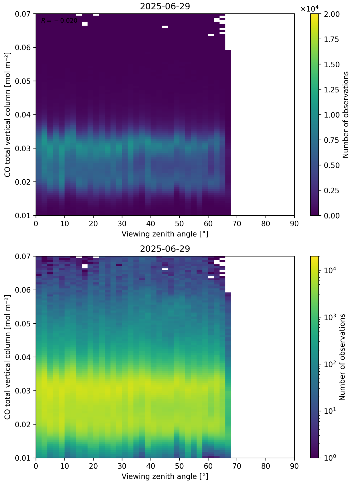
Figure 69: Scatter density plot of “Viewing zenith angle” against “CO total vertical column” for 2025-06-28 to 2025-06-30.
