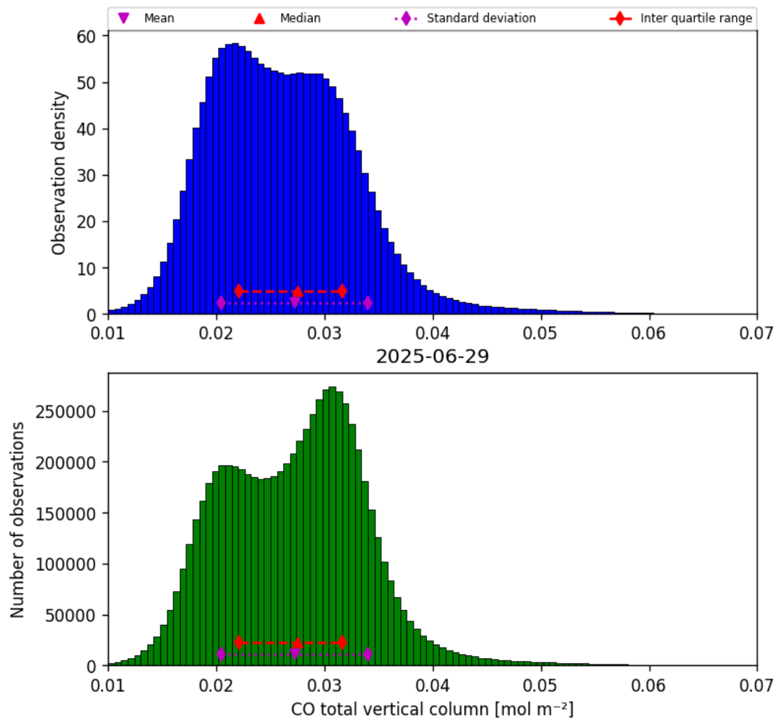
Figure 18: Histogram of “CO total vertical column” for 2025-06-28 to 2025-06-30
