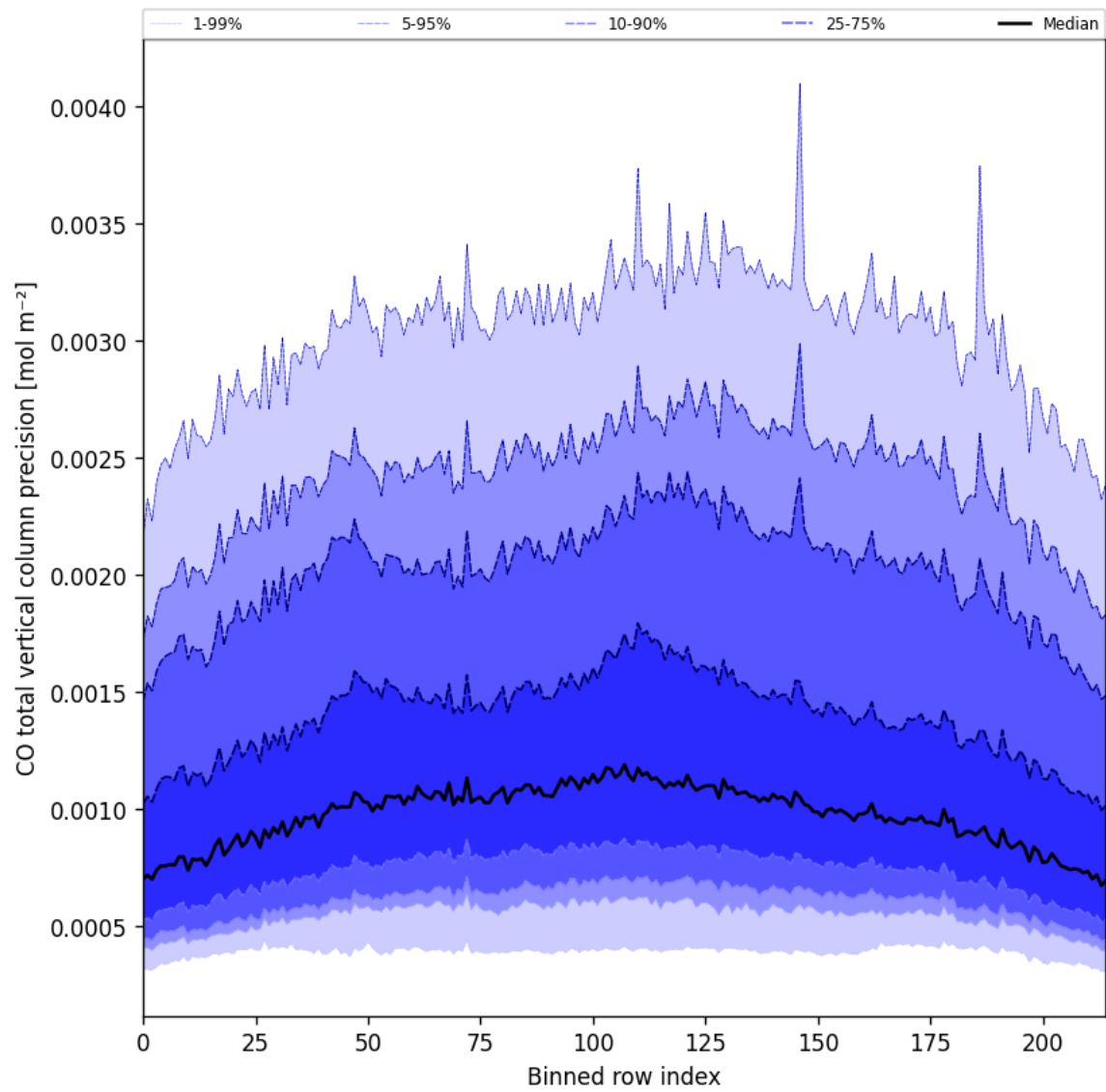
Figure 28: Along track statistics of “CO total vertical column precision” for 2025-06-29 to 2025-07-01
