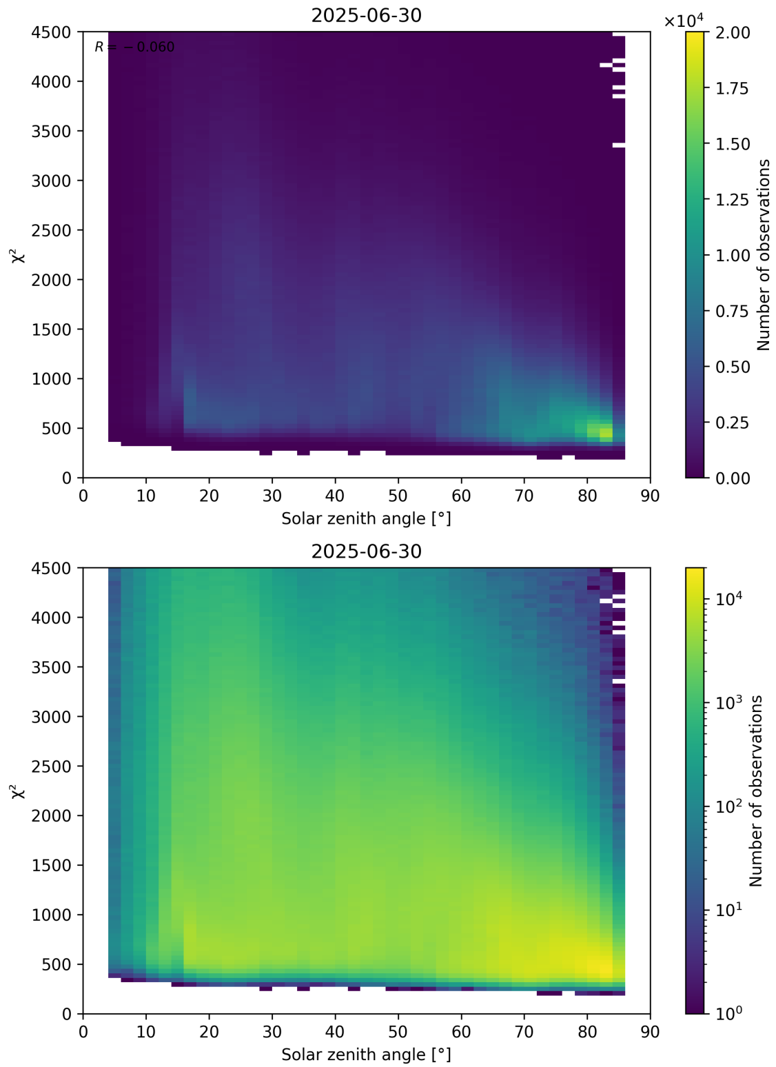
Figure 64: Scatter density plot of “Solar zenith angle” against “ \chi^2 ” for 2025-06-29 to 2025-07-01.
