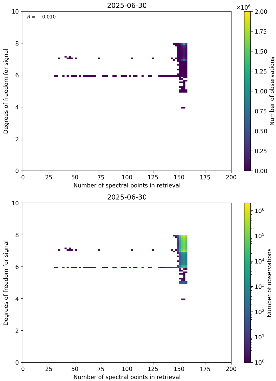
Figure 59: Scatter density plot of “Number of spectral points in retrieval” against “Degrees of freedom for signal” for 2025-06-29 to 2025-07-01.
