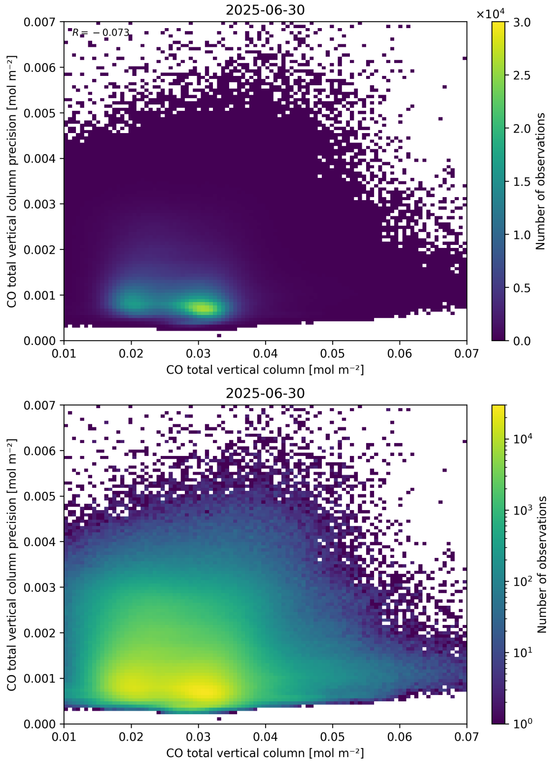
Figure 34: Scatter density plot of “CO total vertical column” against “CO total vertical column precision” for 2025-06-29 to 2025-07-01.
