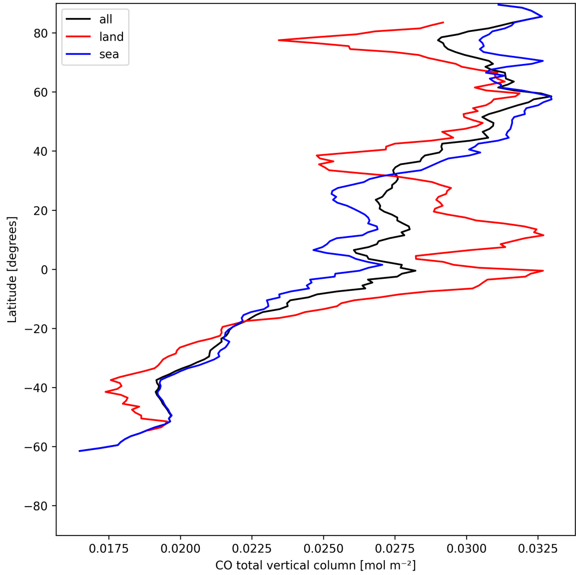
Figure 10: Zonal average of “CO total vertical column” for 2025-06-29 to 2025-07-01.
