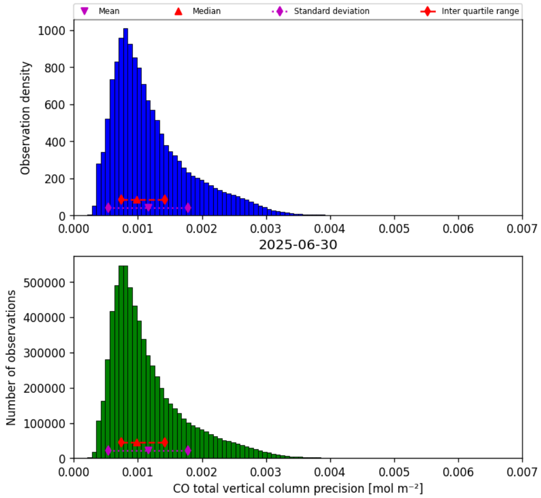
Figure 20: Histogram of “CO total vertical column precision” for 2025-06-29 to 2025-07-01
