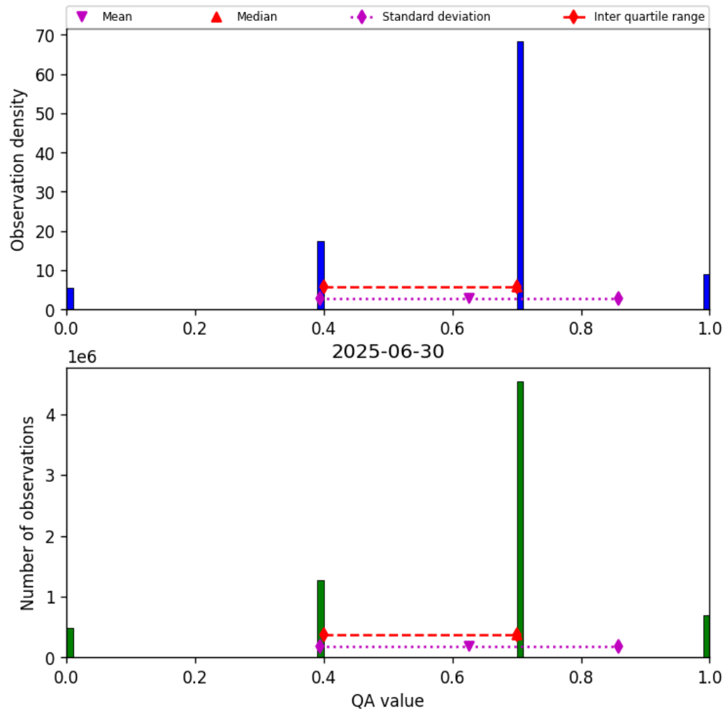
Figure 17: Histogram of “QA value” for 2025-06-29 to 2025-07-01
