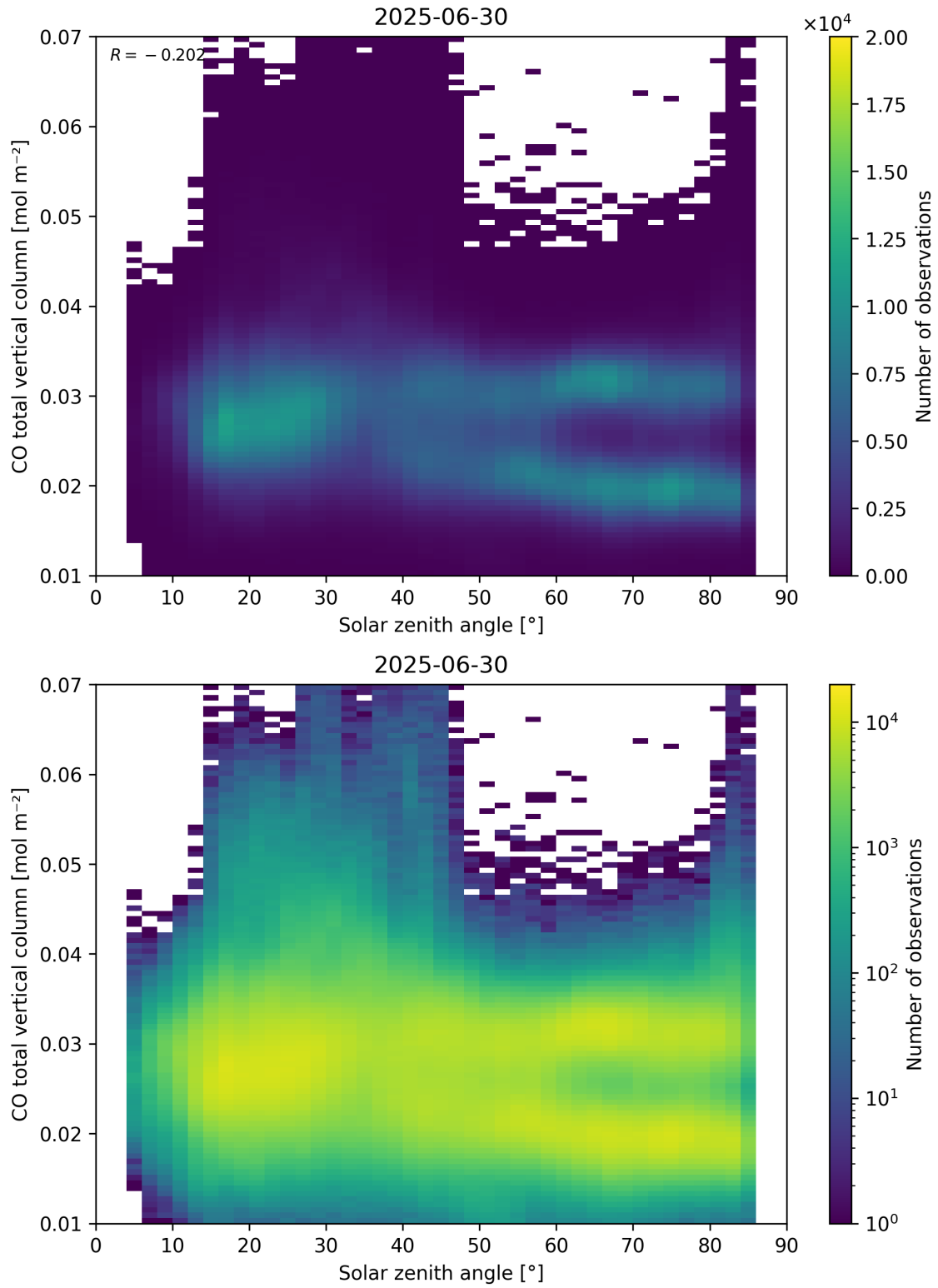
Figure 61: Scatter density plot of “Solar zenith angle” against “CO total vertical column” for 2025-06-29 to 2025-07-01.
