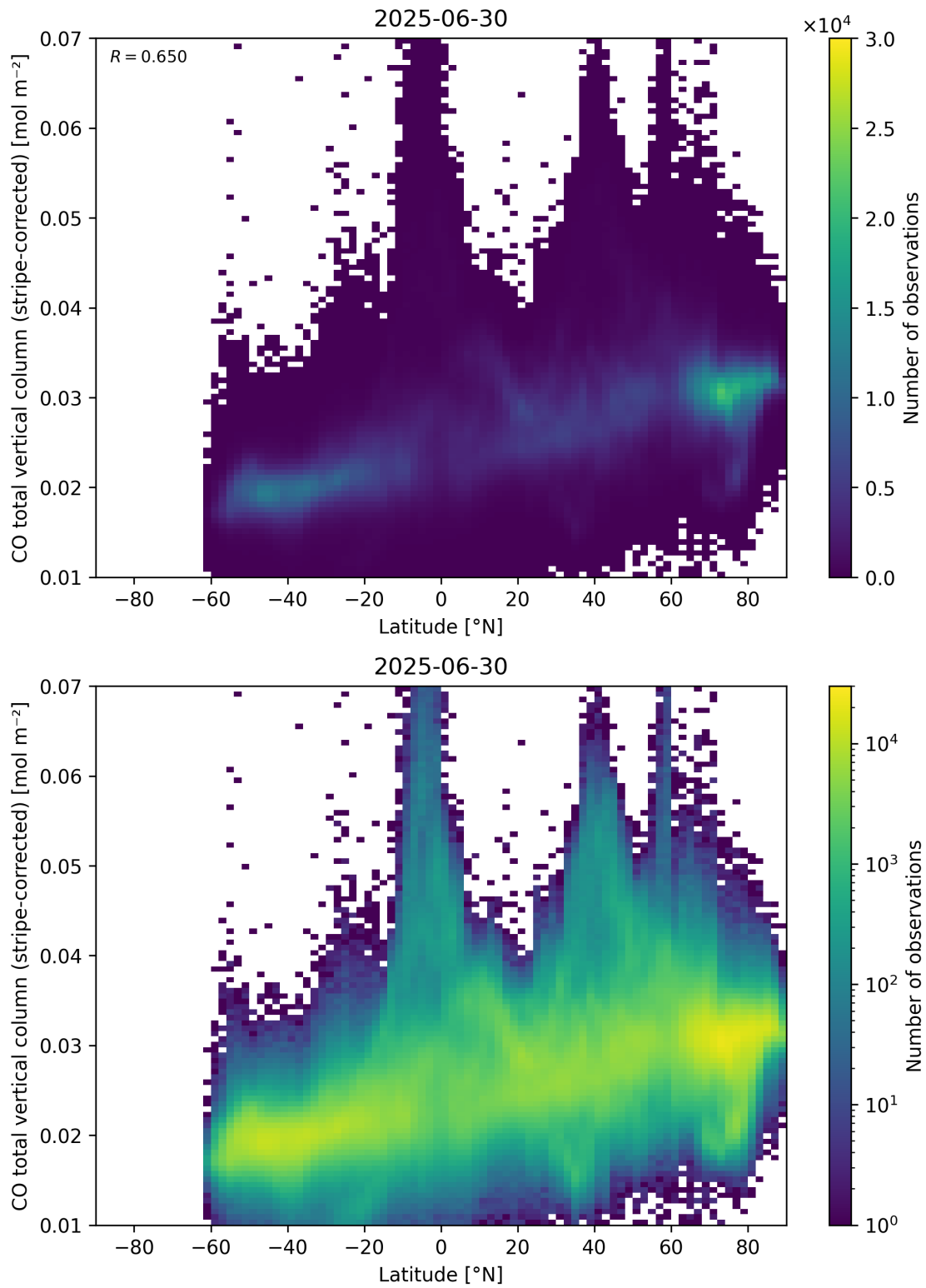
Figure 52: Scatter density plot of “Latitude” against “CO total vertical column (stripe-corrected)” for 2025-06-29 to 2025-07-01.
