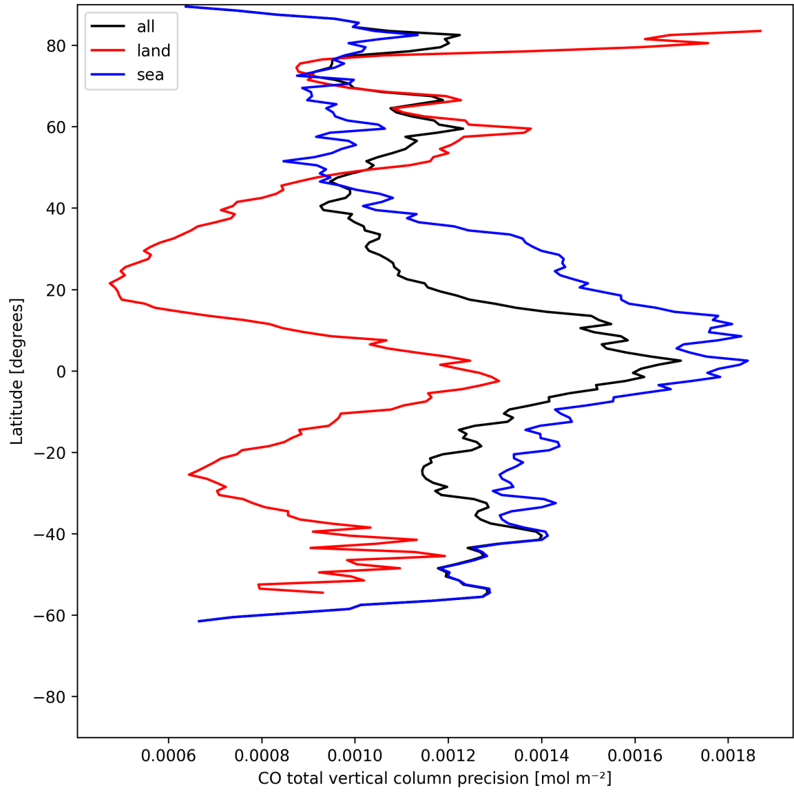
Figure 12: Zonal average of “CO total vertical column precision” for 2025-06-29 to 2025-07-01.
