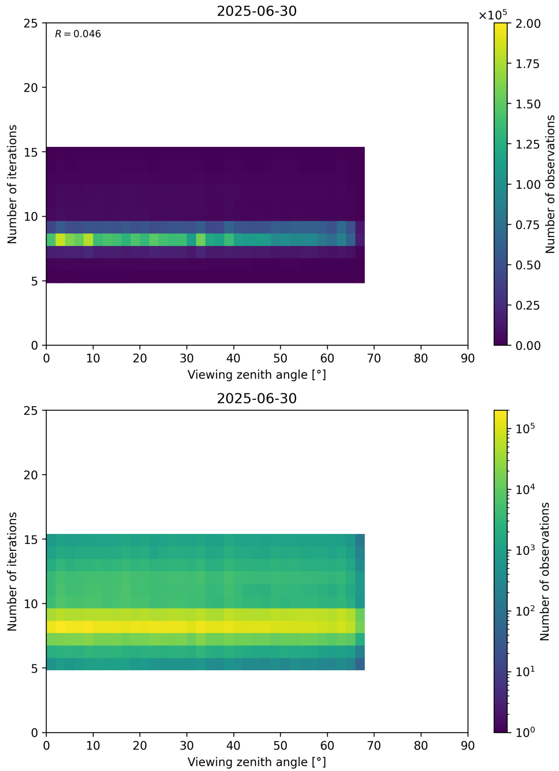
Figure 75: Scatter density plot of “Viewing zenith angle” against “Number of iterations” for 2025-06-29 to 2025-07-01.
