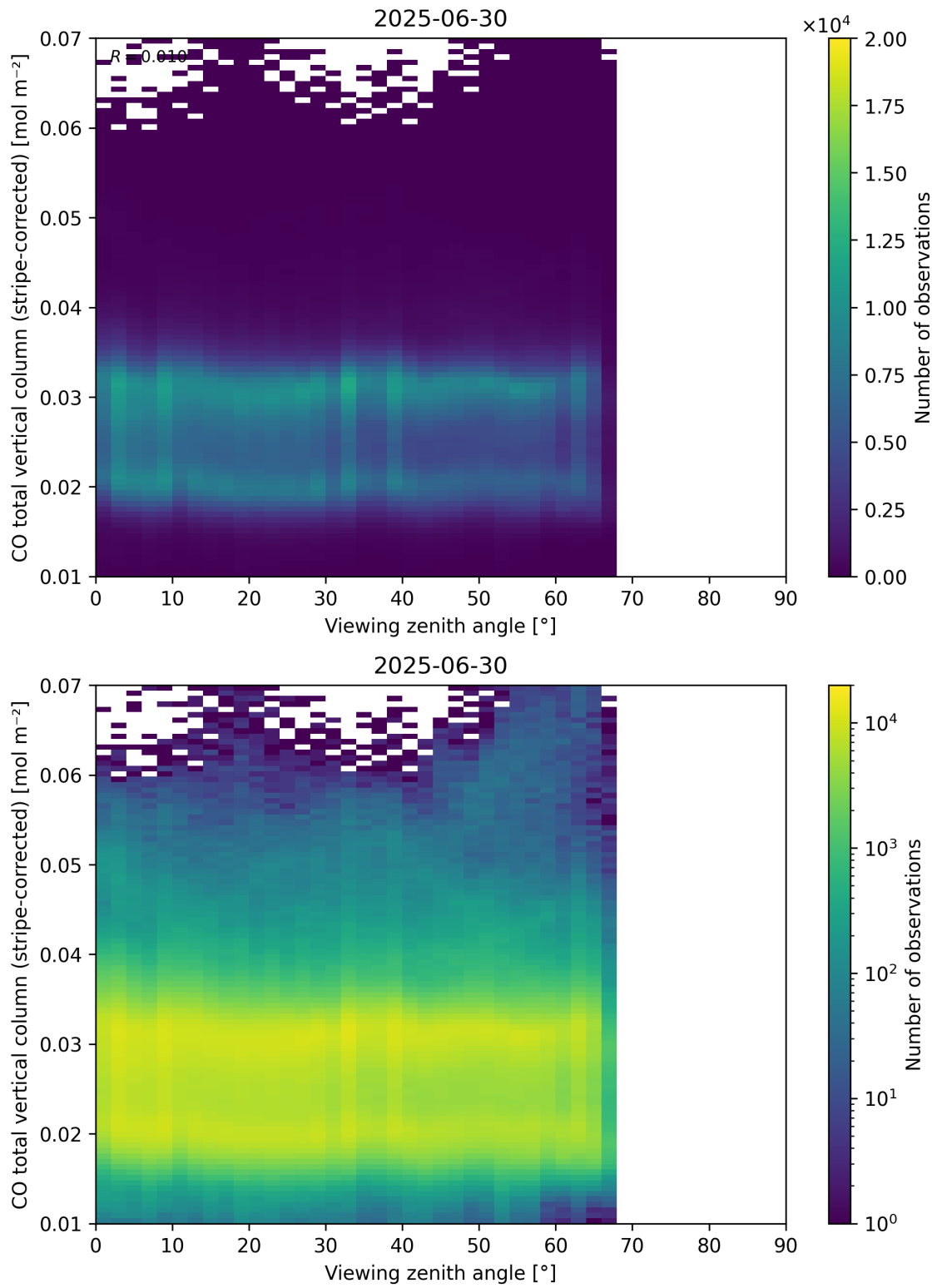
Figure 70: Scatter density plot of “Viewing zenith angle” against “CO total vertical column (stripe-corrected)” for 2025-06-29 to 2025-07-01.
