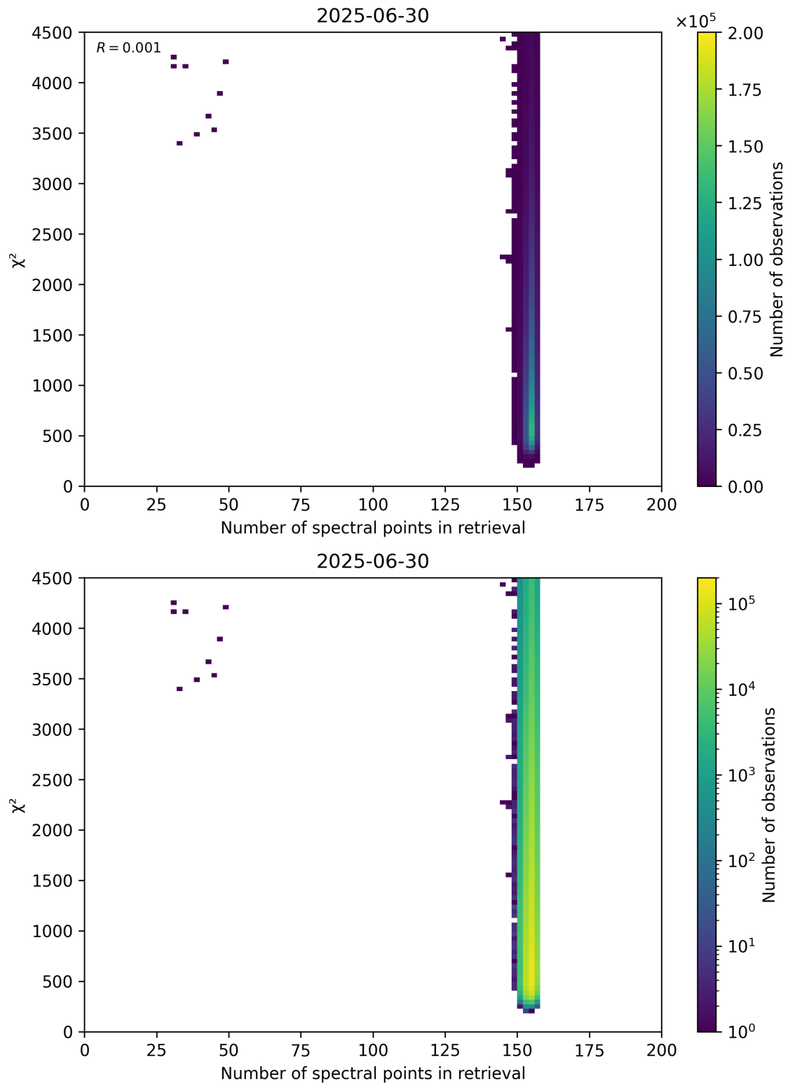
Figure 58: Scatter density plot of “Number of spectral points in retrieval” against “ \chi^2 ” for 2025-06-29 to 2025-07-01.
