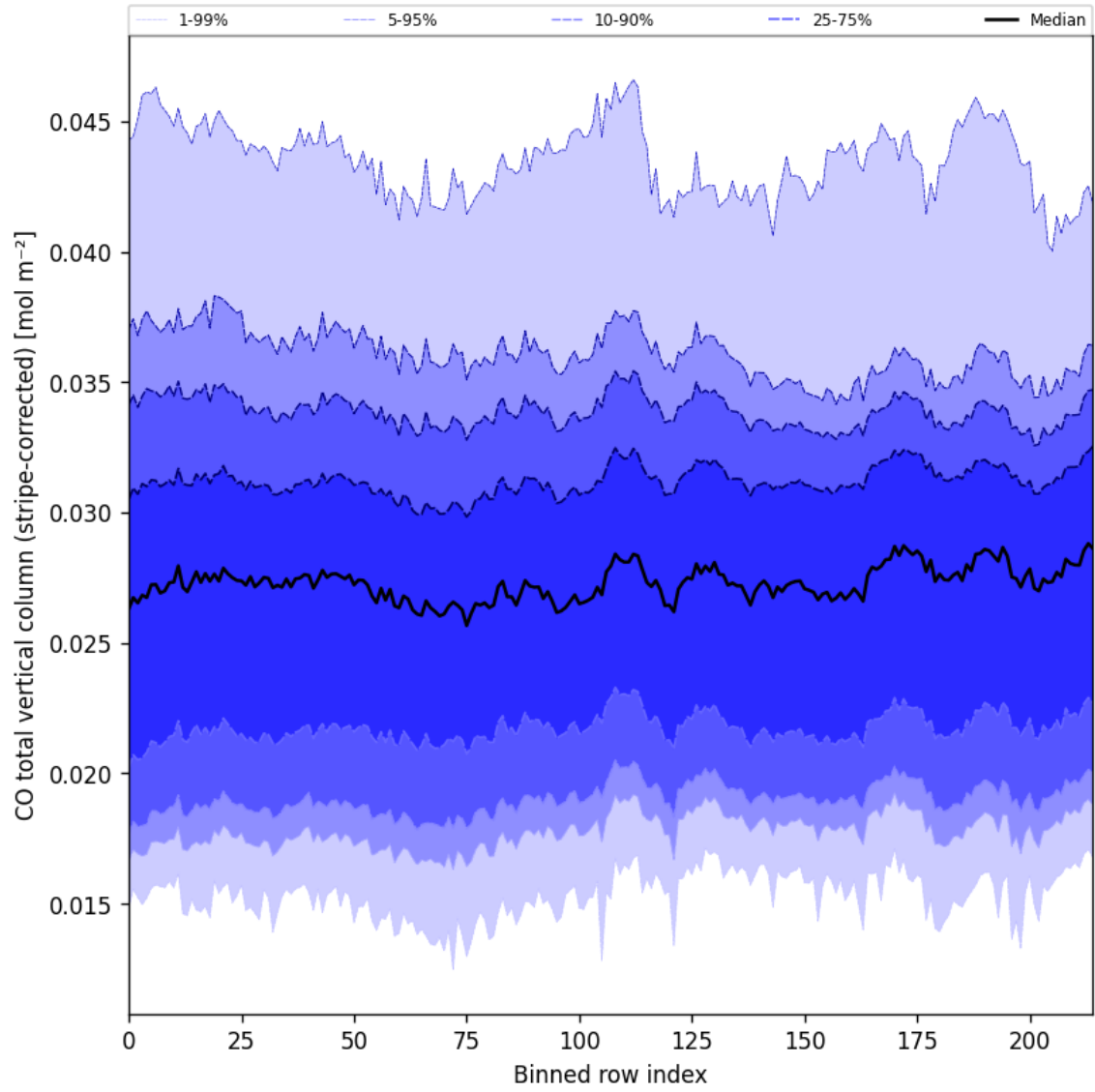
Figure 27: Along track statistics of “CO total vertical column (stripe-corrected)” for 2025-06-29 to 2025-07-01
