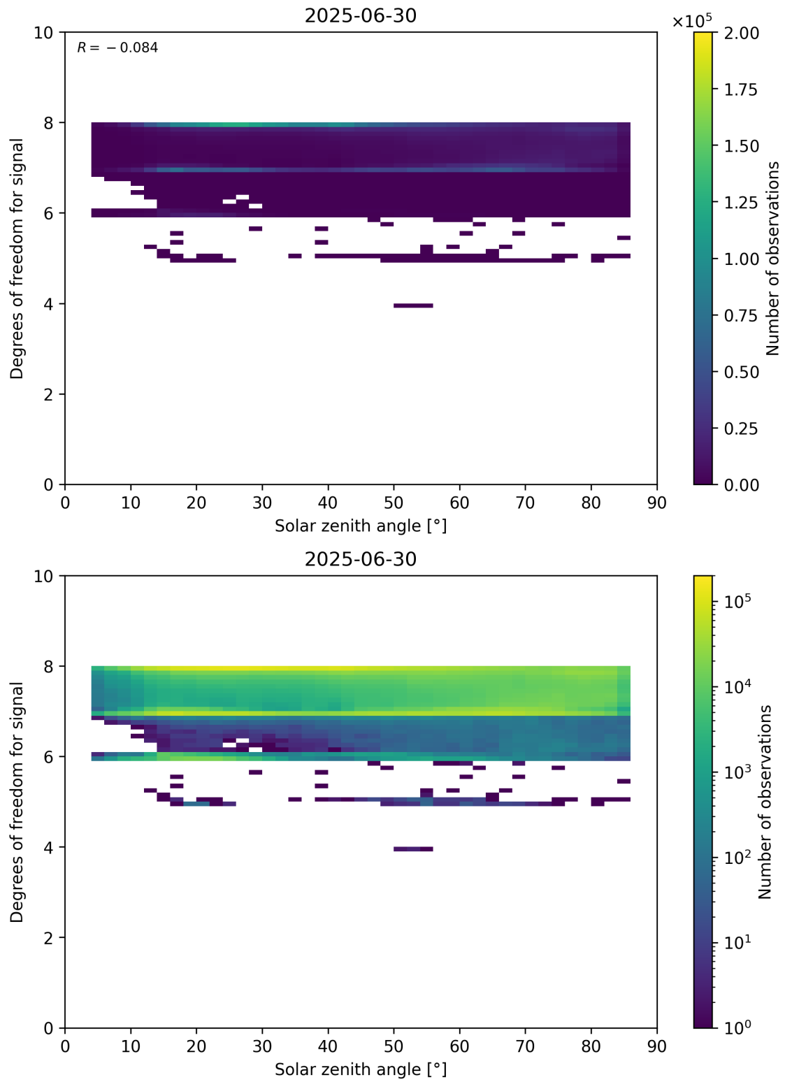
Figure 65: Scatter density plot of “Solar zenith angle” against “Degrees of freedom for signal” for 2025-06-29 to 2025-07-01.
