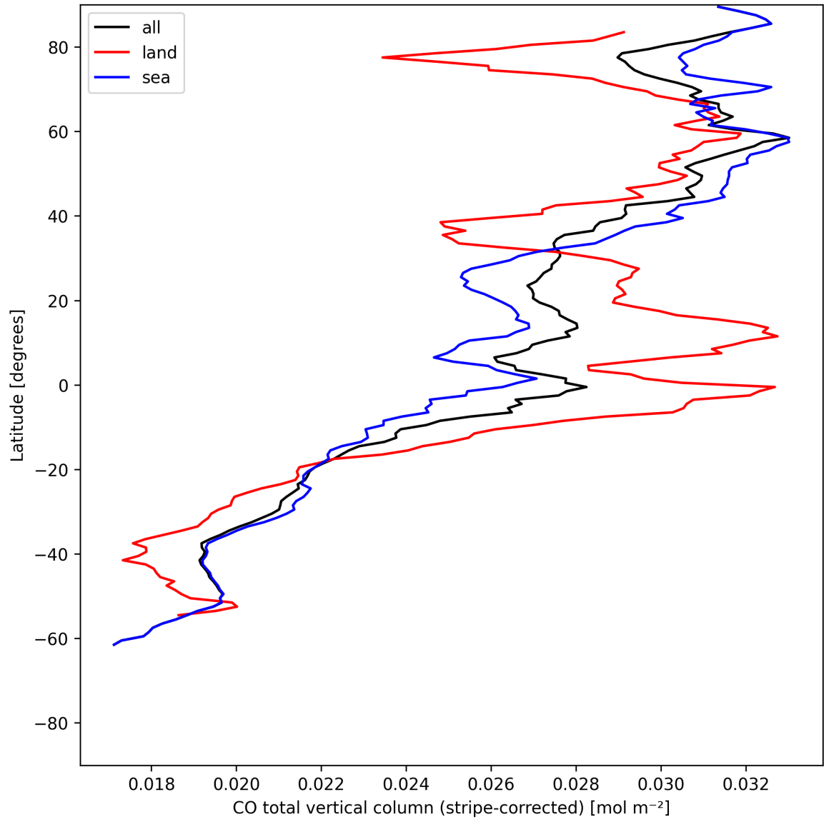
Figure 11: Zonal average of “CO total vertical column (stripe-corrected)” for 2025-06-29 to 2025-07-01.
