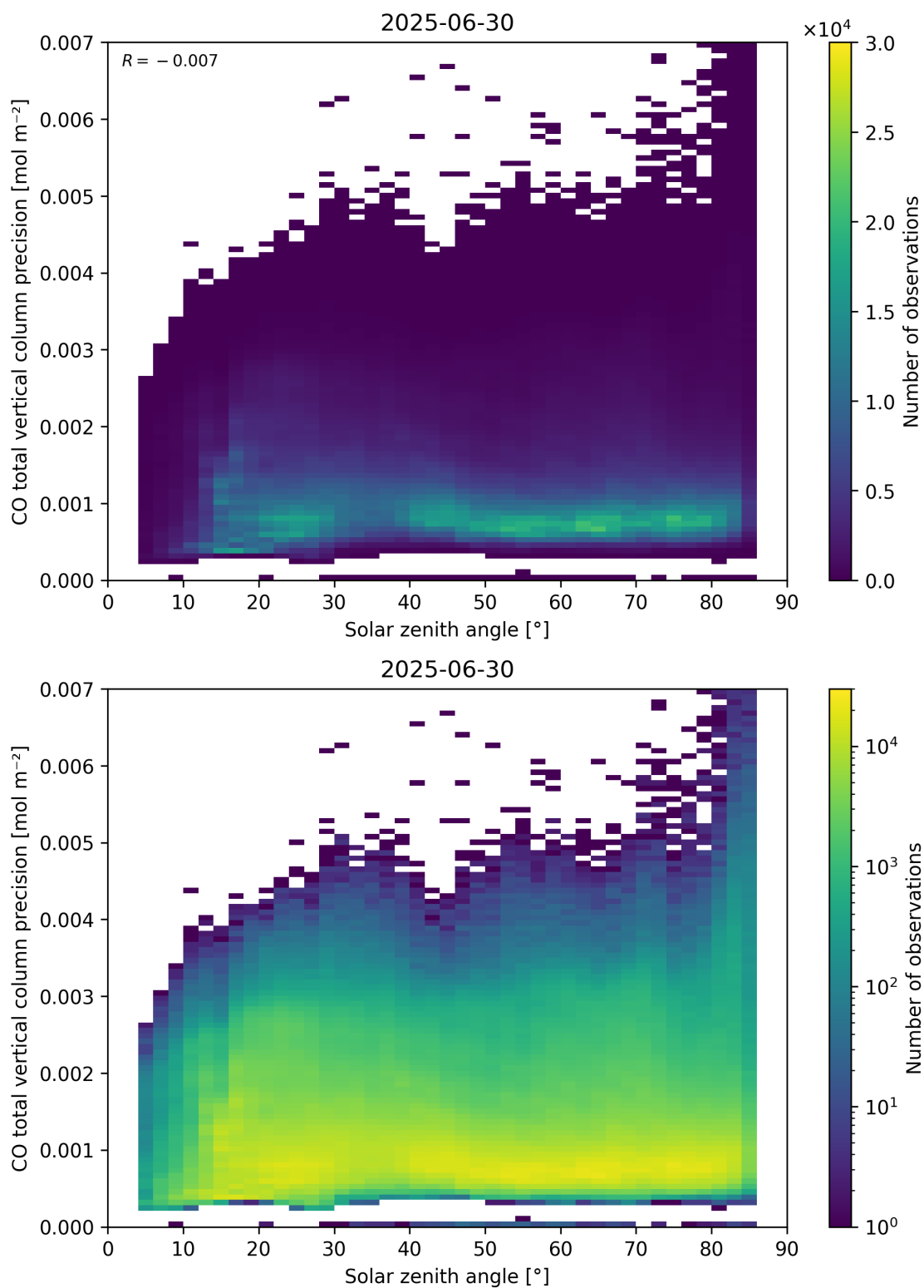
Figure 63: Scatter density plot of “Solar zenith angle” against “CO total vertical column precision” for 2025-06-29 to 2025-07-01.
