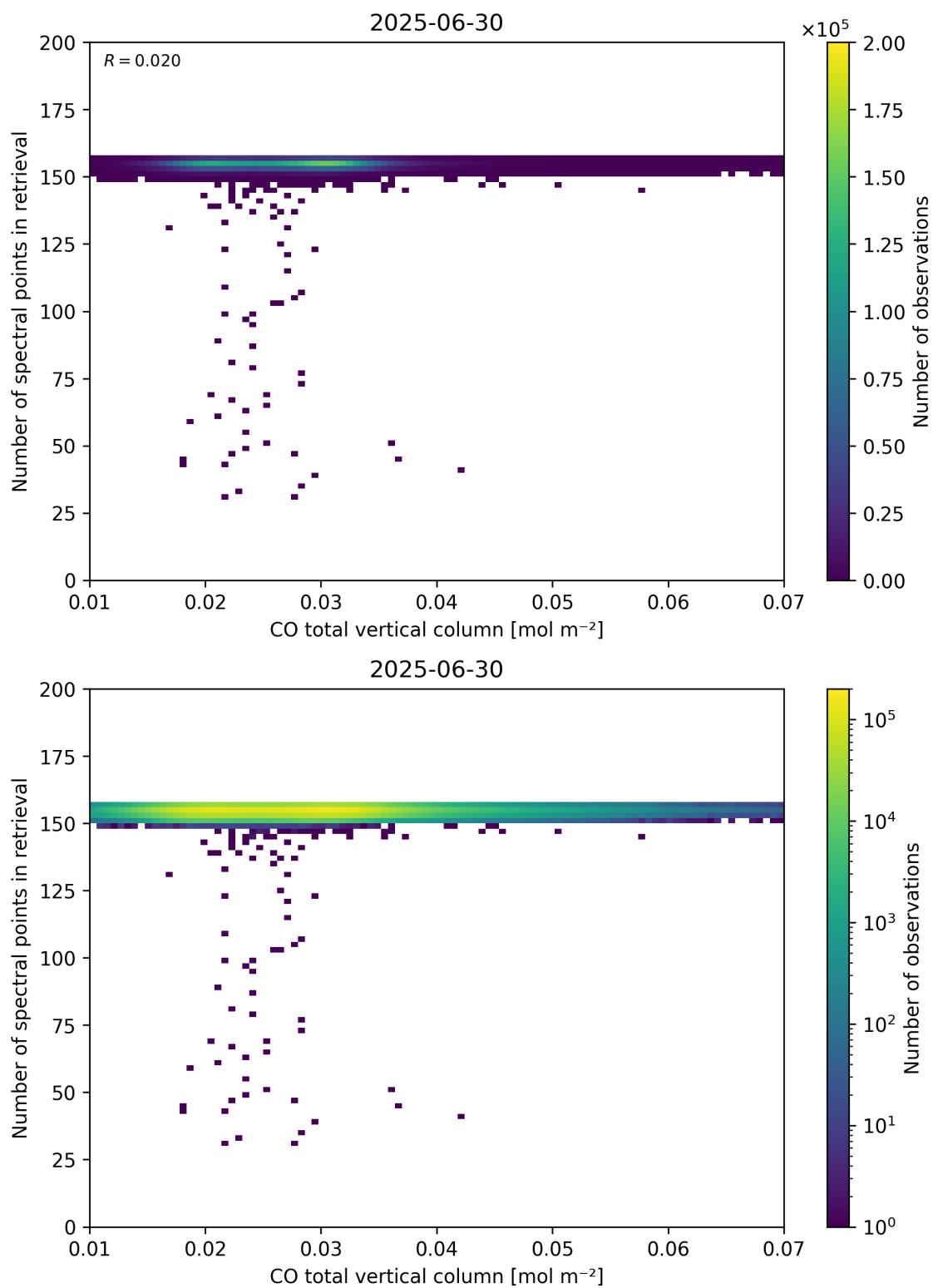
Figure 43: Scatter density plot of “CO total vertical column” against “Number of spectral points in retrieval” for 2025-06-29 to 2025-07-01.
