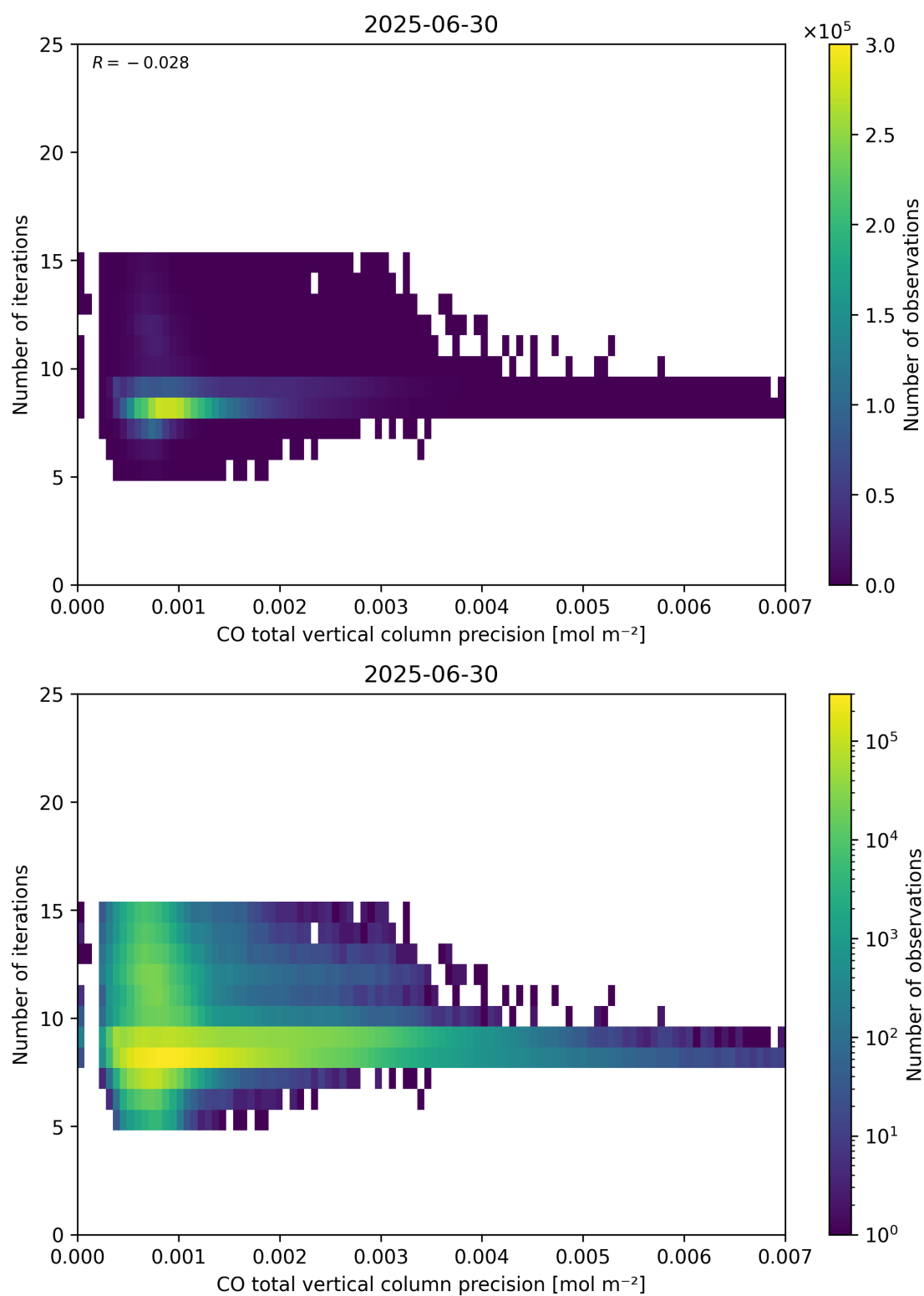
Figure 46: Scatter density plot of “CO total vertical column precision” against “Number of iterations” for 2025-06-29 to 2025-07-01.
