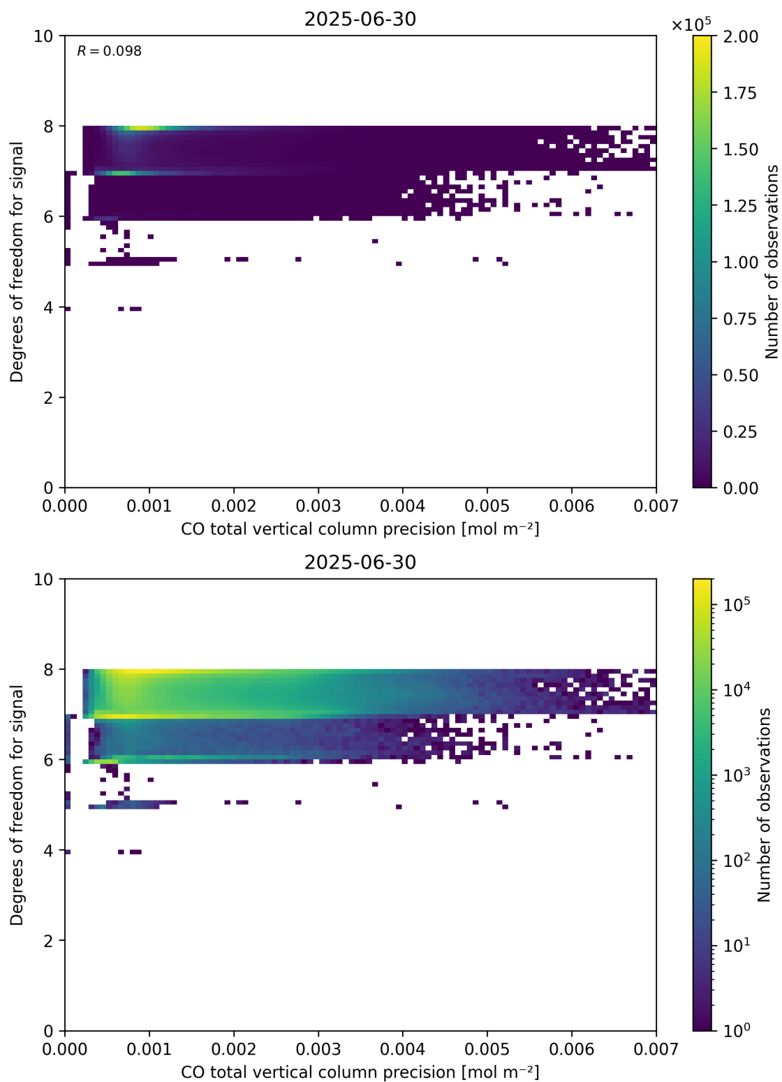
Figure 45: Scatter density plot of “CO total vertical column precision” against “Degrees of freedom for signal” for 2025-06-29 to 2025-07-01.
