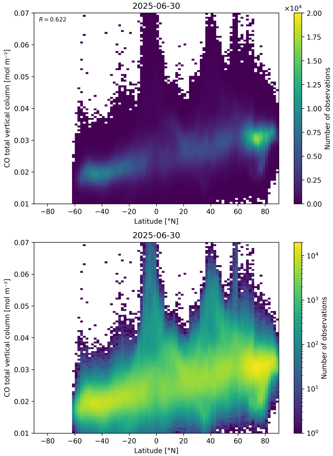
Figure 51: Scatter density plot of “Latitude” against “CO total vertical column” for 2025-06-29 to 2025-07-01.
