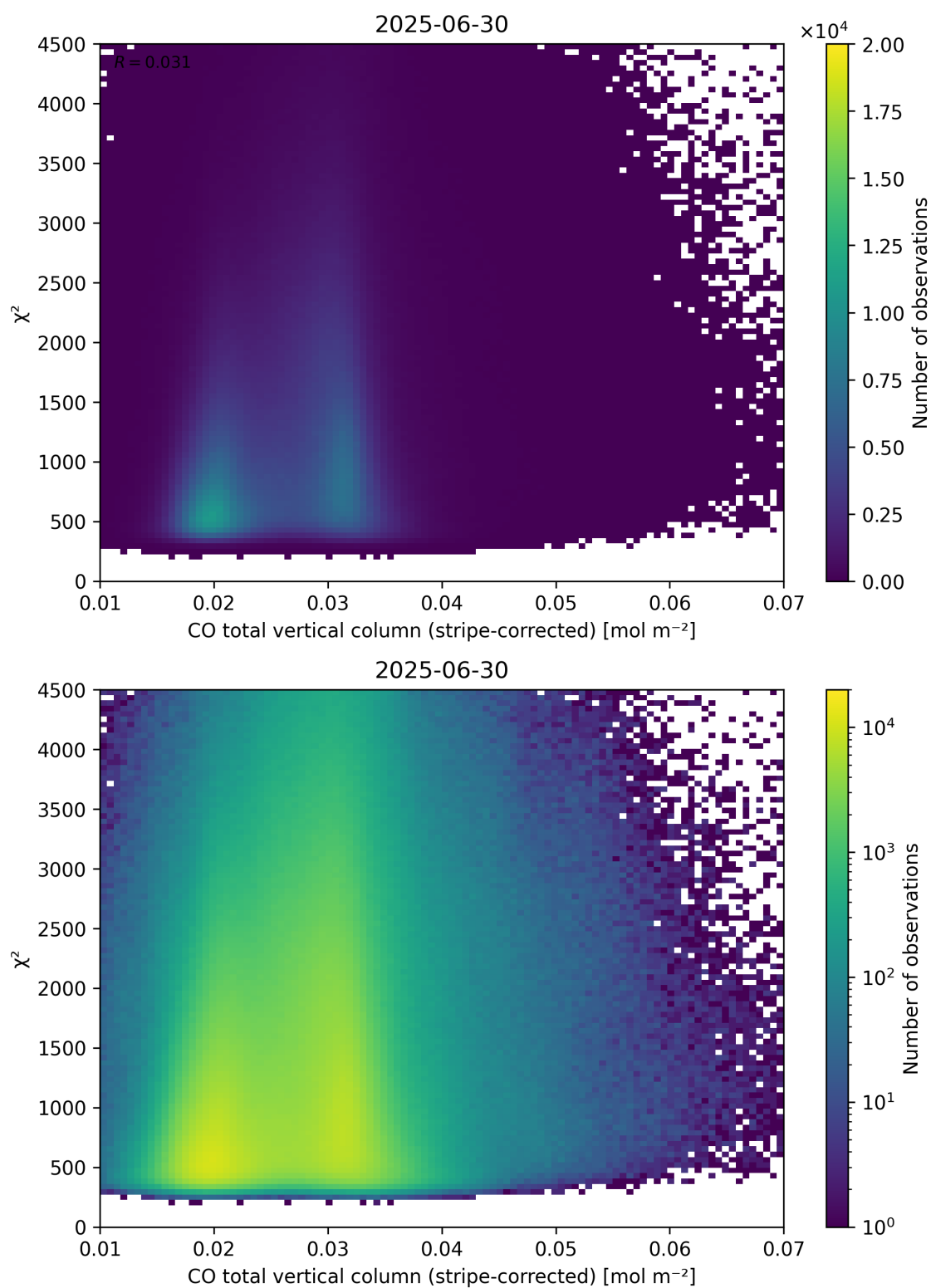
Figure 37: Scatter density plot of “CO total vertical column (stripe-corrected)” against “ \chi^2 ” for 2025-06-29 to 2025-07-01.
