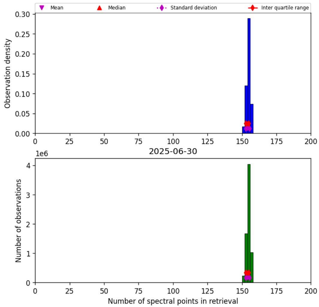
Figure 21: Histogram of “Number of spectral points in retrieval” for 2025-06-29 to 2025-07-01
