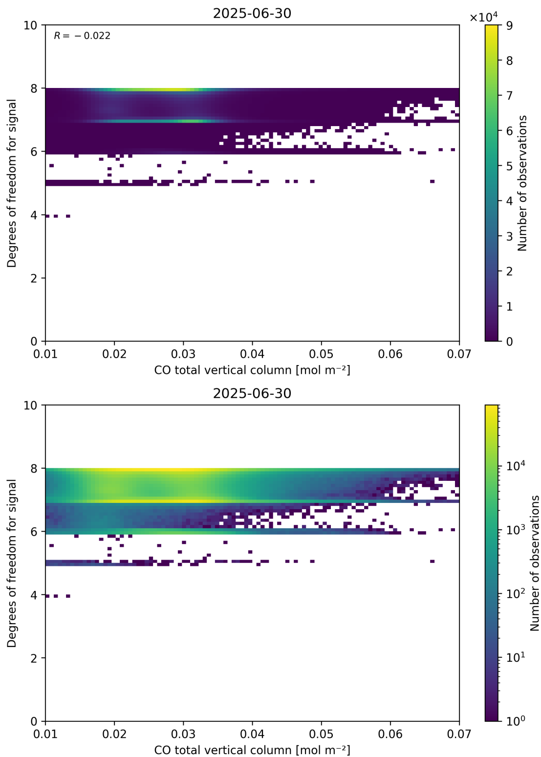
Figure 41: Scatter density plot of “CO total vertical column” against “Degrees of freedom for signal” for 2025-06-29 to 2025-07-01.
