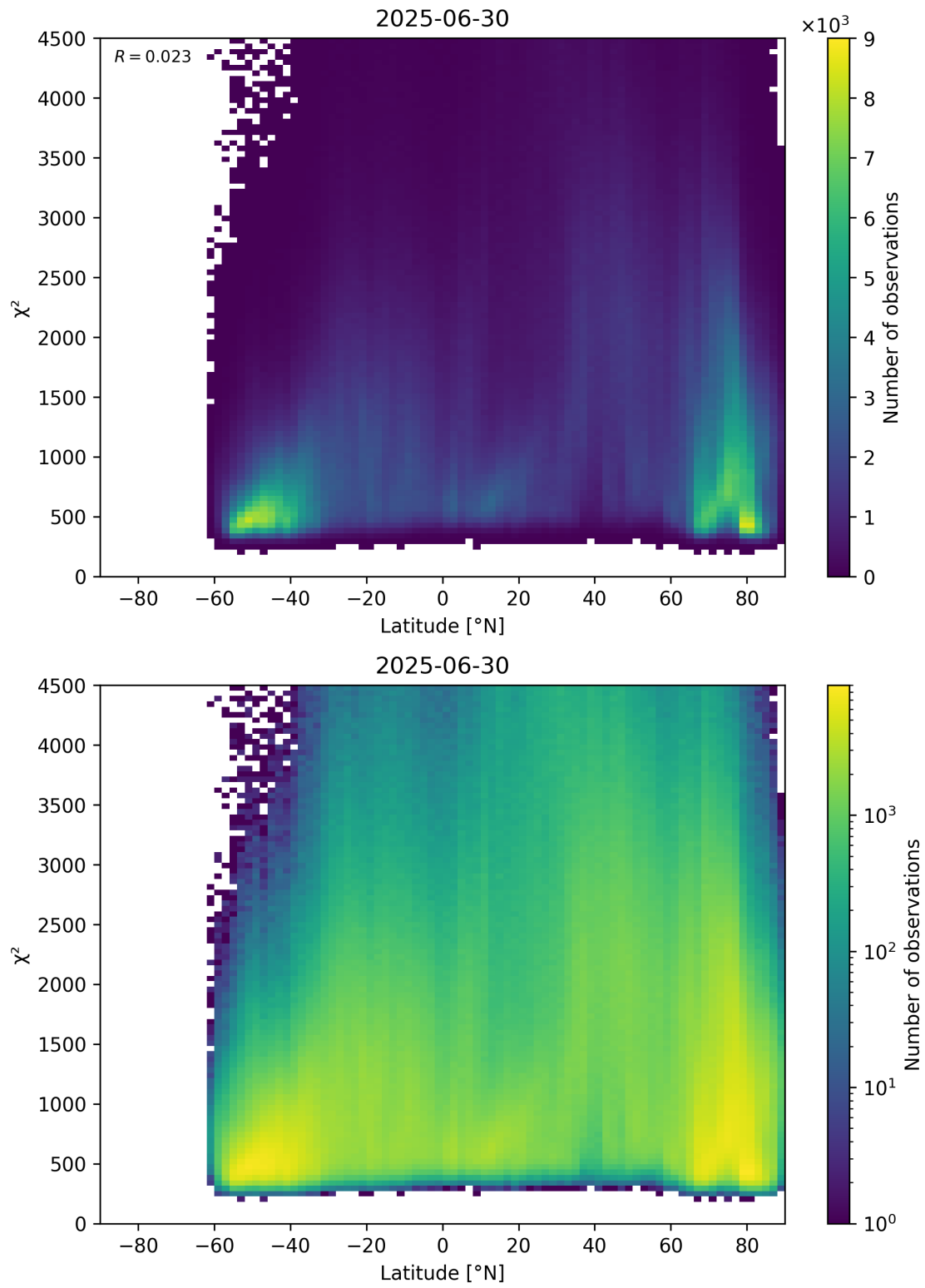
Figure 54: Scatter density plot of “Latitude” against “ \chi^2 ” for 2025-06-29 to 2025-07-01.
