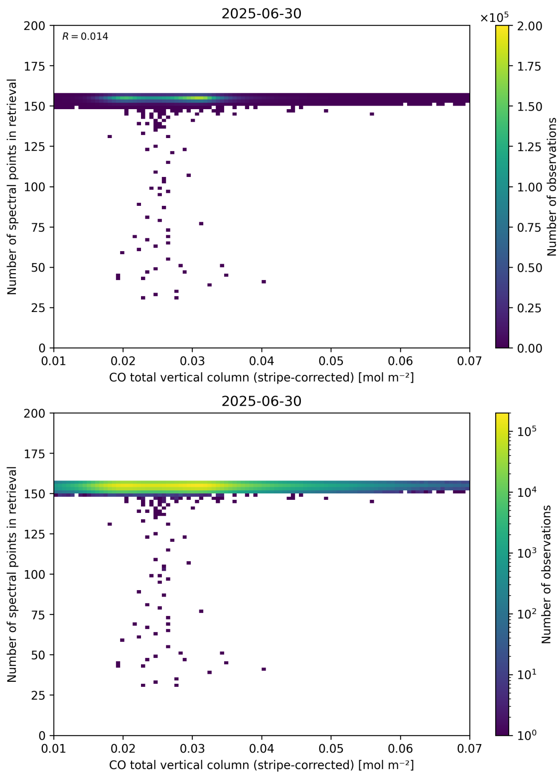
Figure 40: Scatter density plot of “CO total vertical column (stripe-corrected)” against “Number of spectral points in retrieval” for 2025-06-29 to 2025-07-01.
