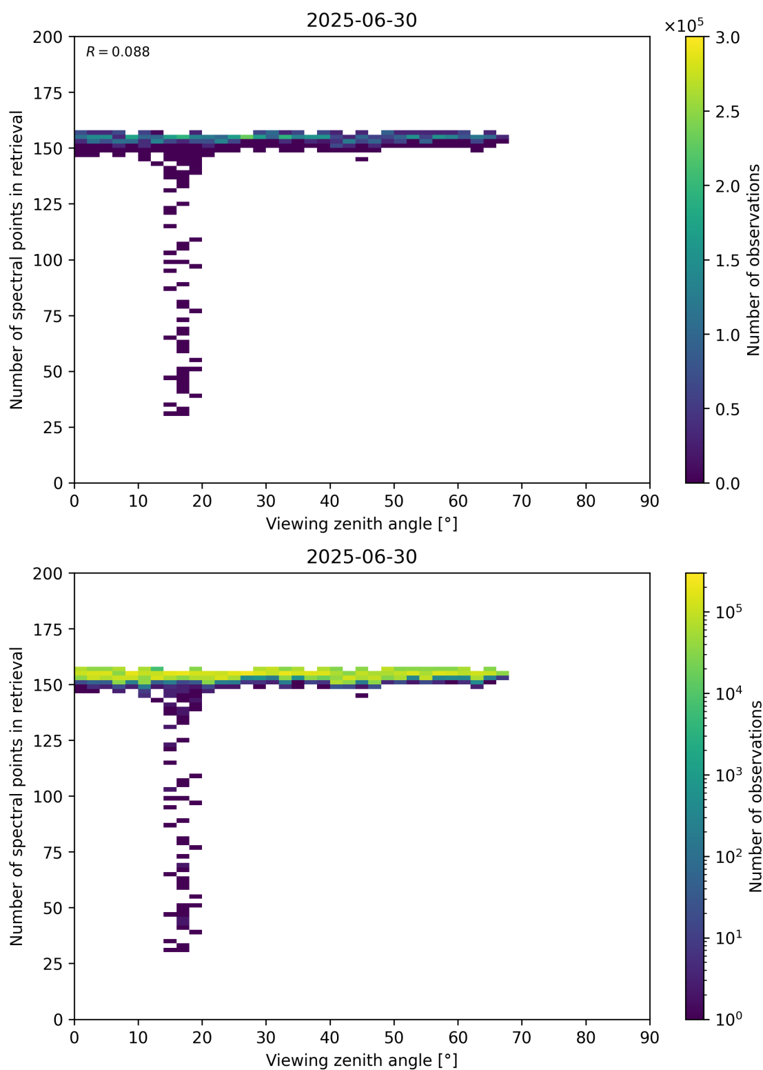
Figure 76: Scatter density plot of “Viewing zenith angle” against “Number of spectral points in retrieval” for 2025-06-29 to 2025-07-01.
