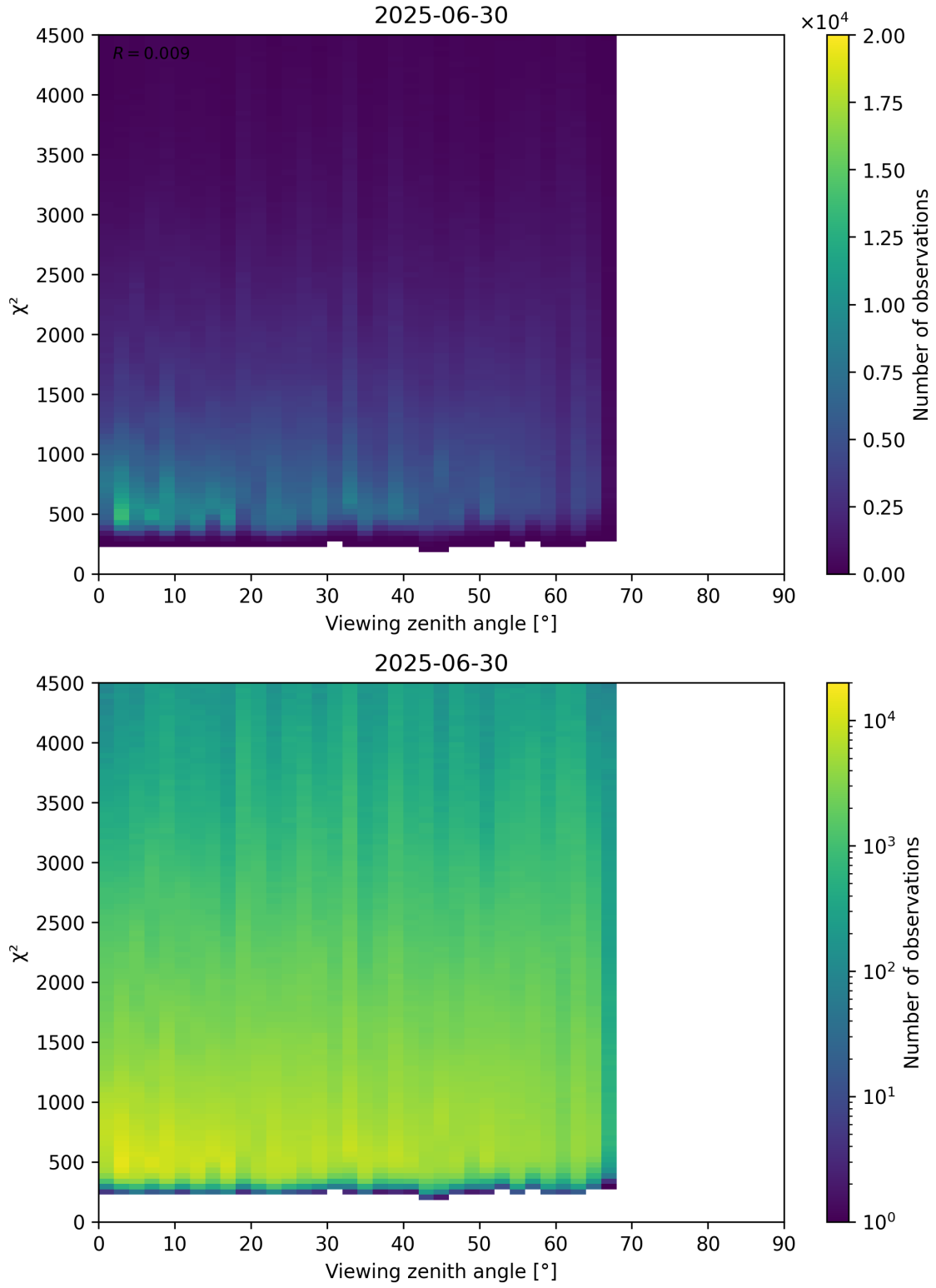
Figure 72: Scatter density plot of “Viewing zenith angle” against “ \chi^2 ” for 2025-06-29 to 2025-07-01.
