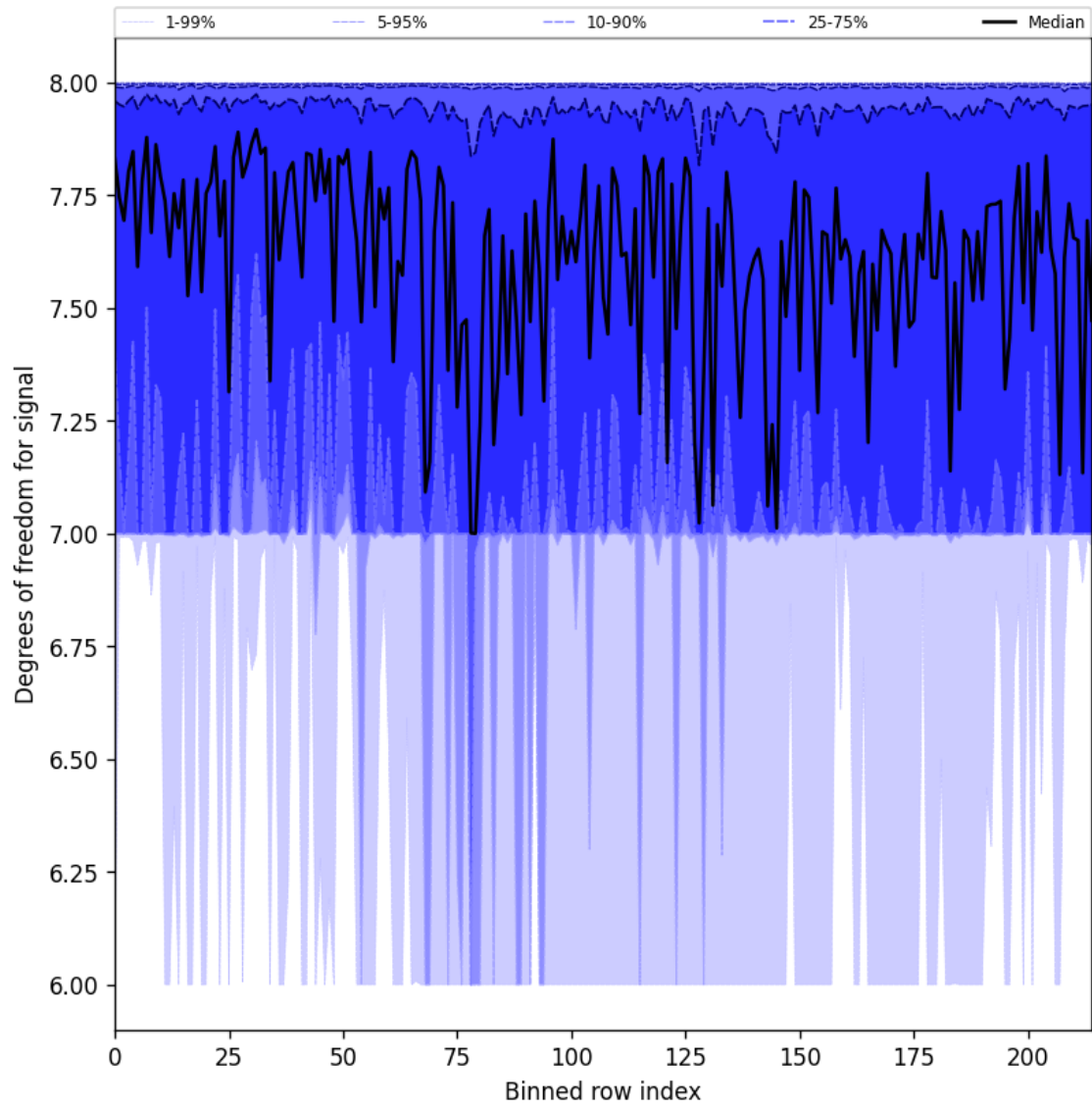
Figure 31: Along track statistics of “Degrees of freedom for signal” for 2025-06-29 to 2025-07-01
