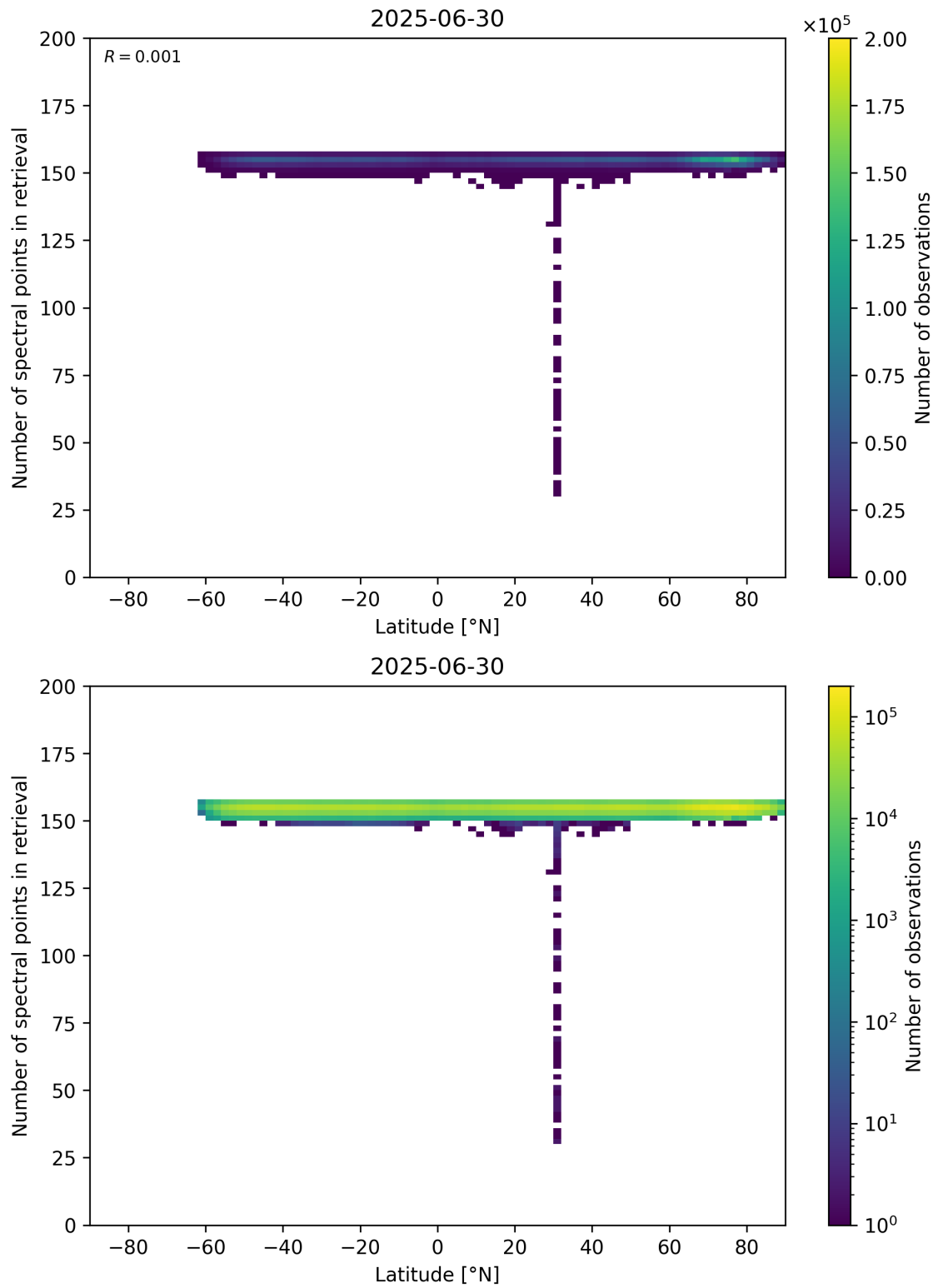
Figure 57: Scatter density plot of “Latitude” against “Number of spectral points in retrieval” for 2025-06-29 to 2025-07-01.
