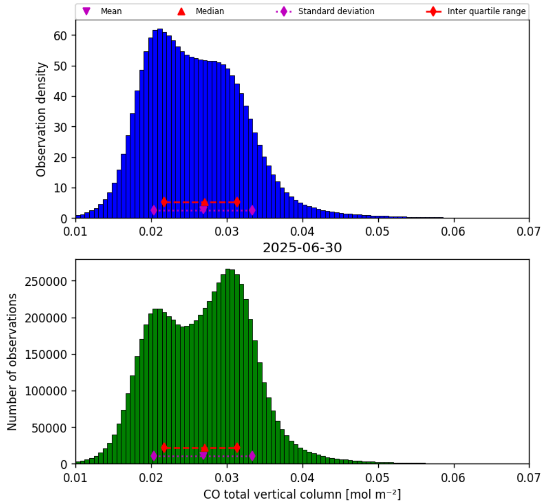
Figure 18: Histogram of “CO total vertical column” for 2025-06-29 to 2025-07-01
