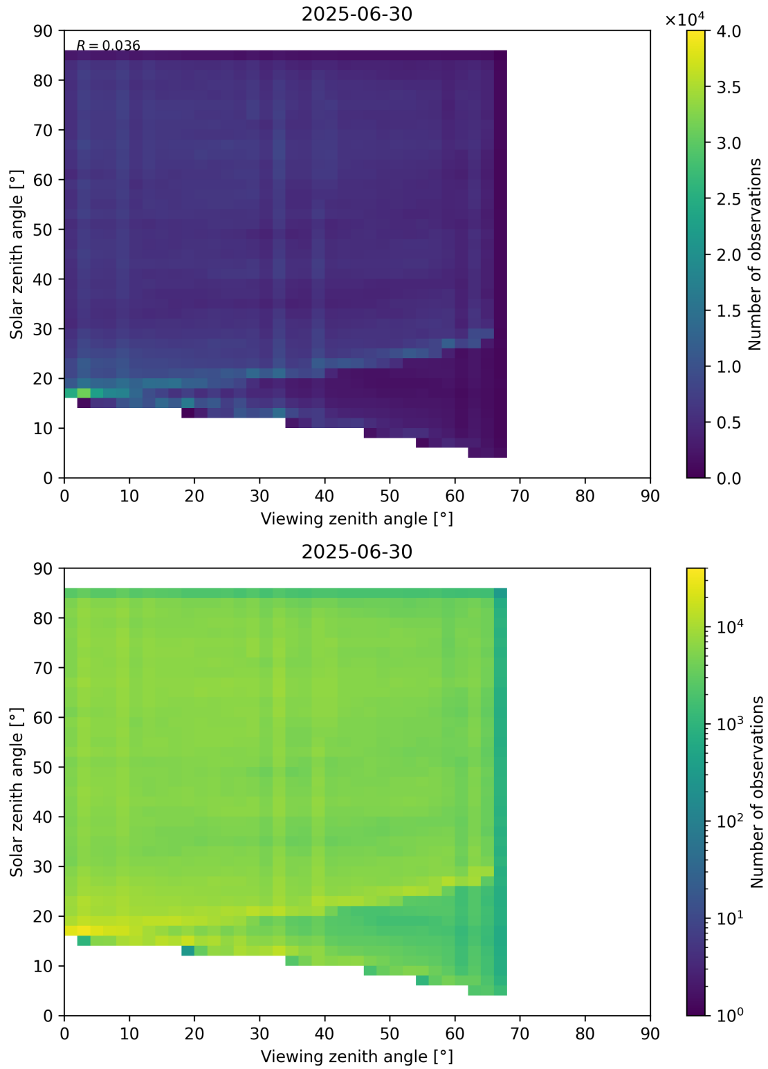
Figure 77: Scatter density plot of “Viewing zenith angle” against “Solar zenith angle” for 2025-06-29 to 2025-07-01.
