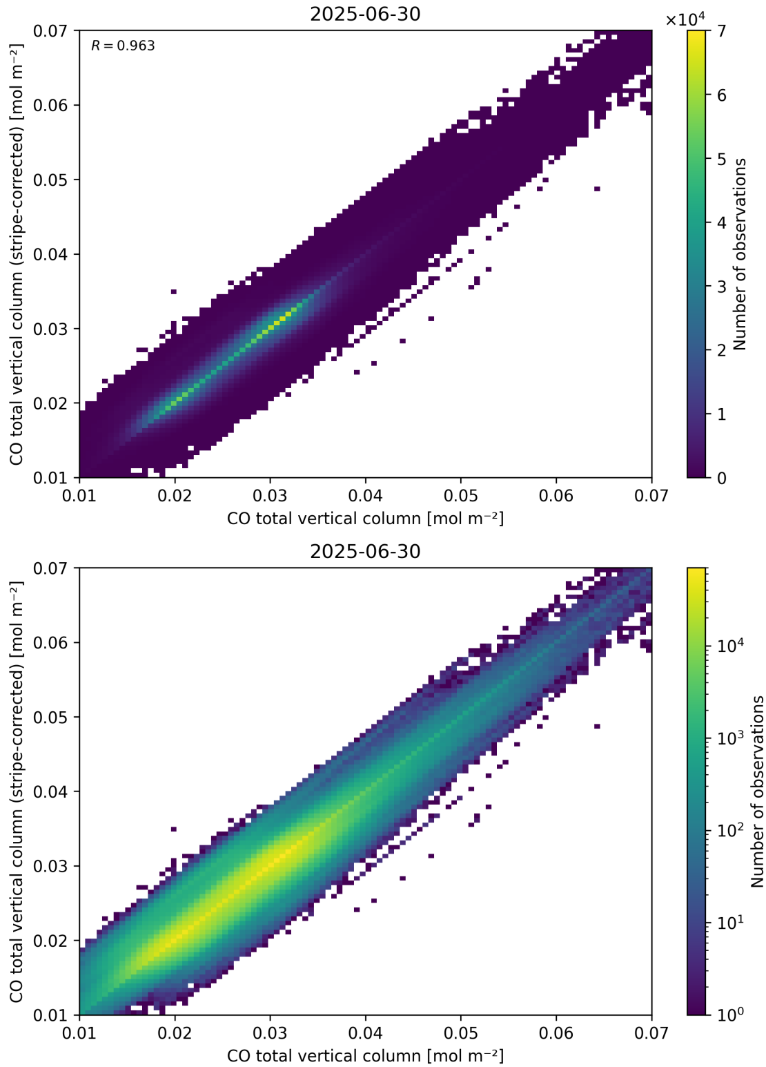
Figure 33: Scatter density plot of “CO total vertical column” against “CO total vertical column (stripe-corrected)” for 2025-06-29 to 2025-07-01.
