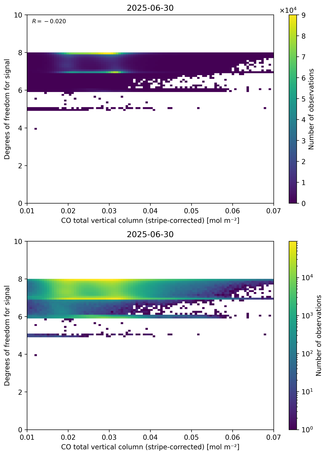
Figure 38: Scatter density plot of “CO total vertical column (stripe-corrected)” against “Degrees of freedom for signal” for 2025-06-29 to 2025-07-01.
