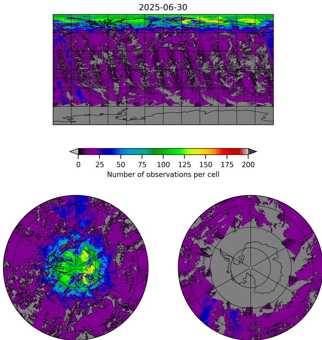
Figure 8: Map of the number of observations for 2025-06-29 to 2025-07-01
