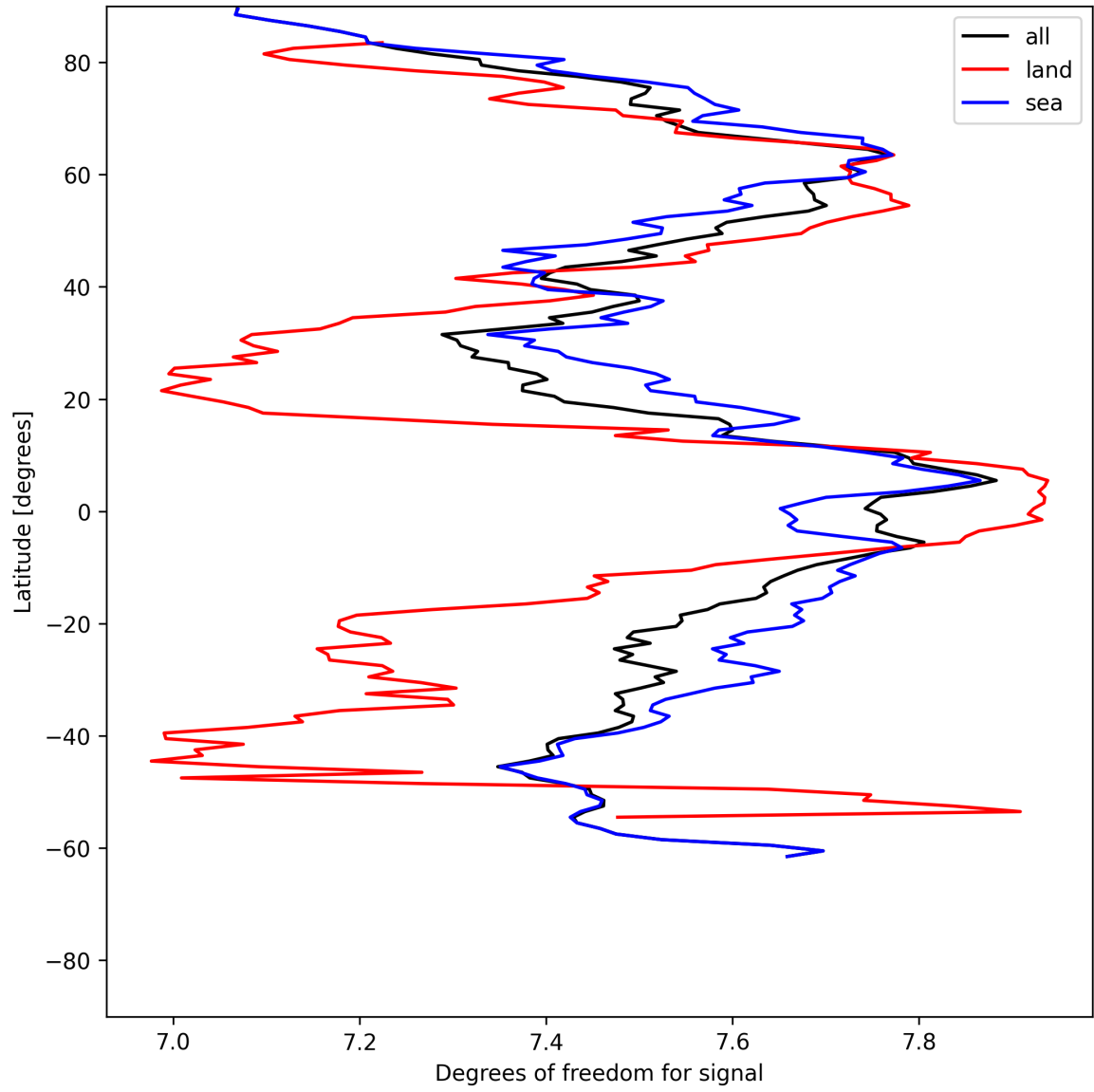
Figure 15: Zonal average of “Degrees of freedom for signal” for 2025-06-29 to 2025-07-01.
