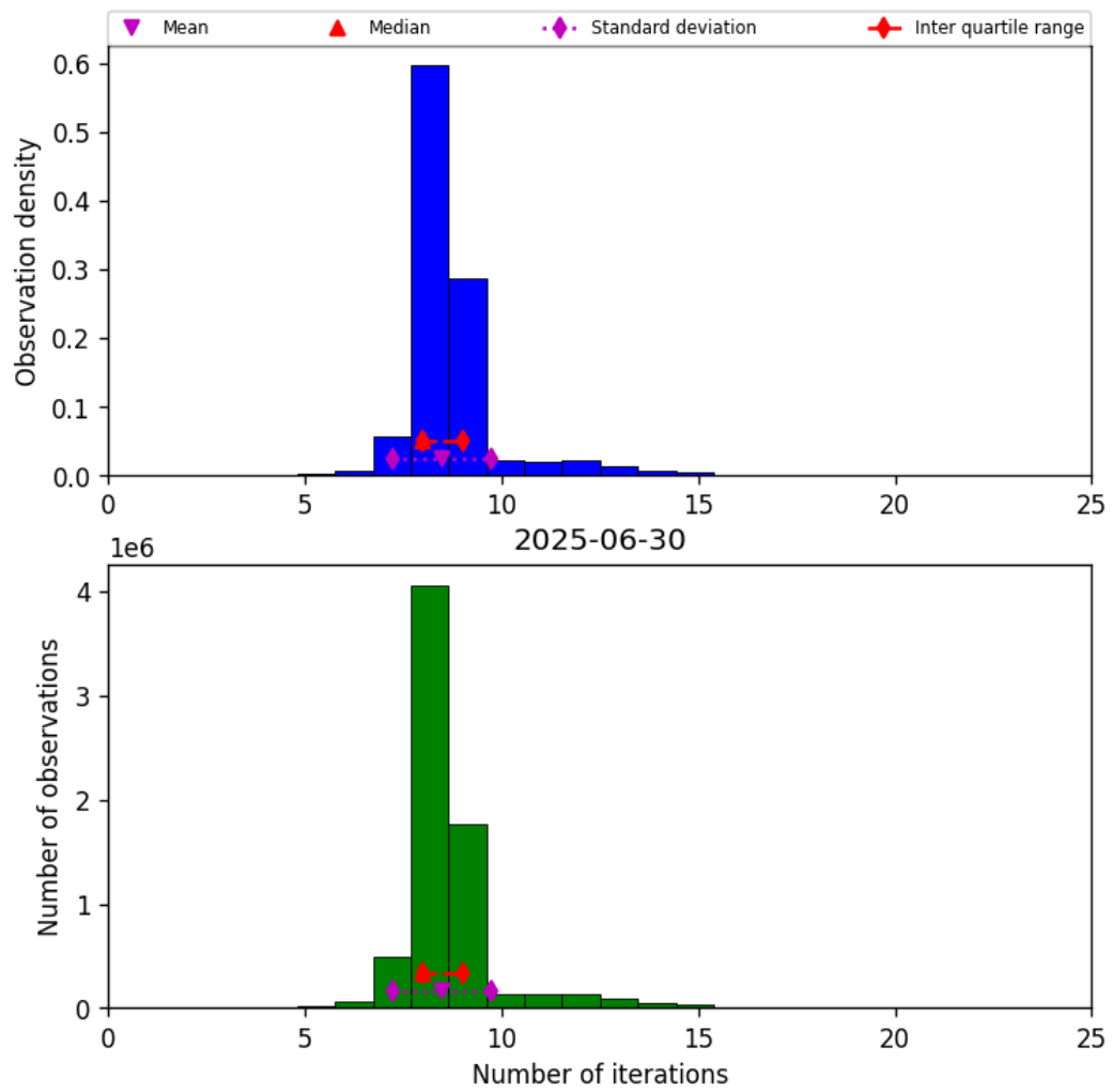
Figure 24: Histogram of “Number of iterations” for 2025-06-29 to 2025-07-01
