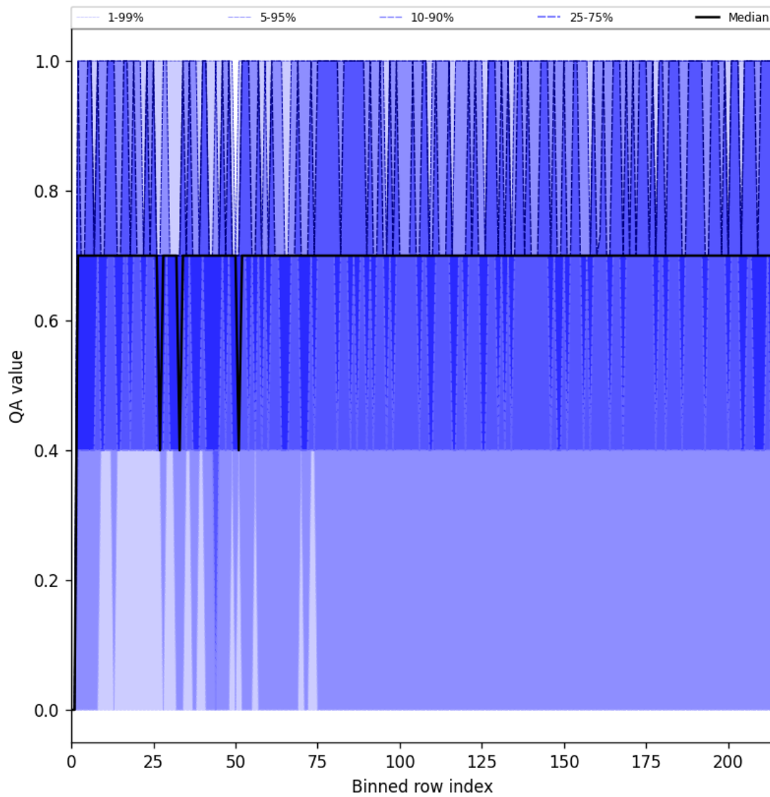
Figure 25: Along track statistics of “QA value” for 2025-06-29 to 2025-07-01
