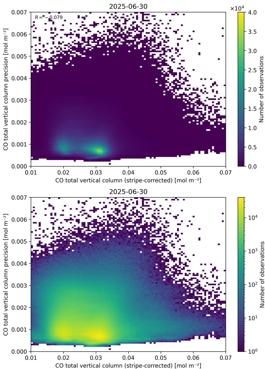
Figure 36: Scatter density plot of “CO total vertical column (stripe-corrected)” against “CO total vertical column precision” for 2025-06-29 to 2025-07-01.
