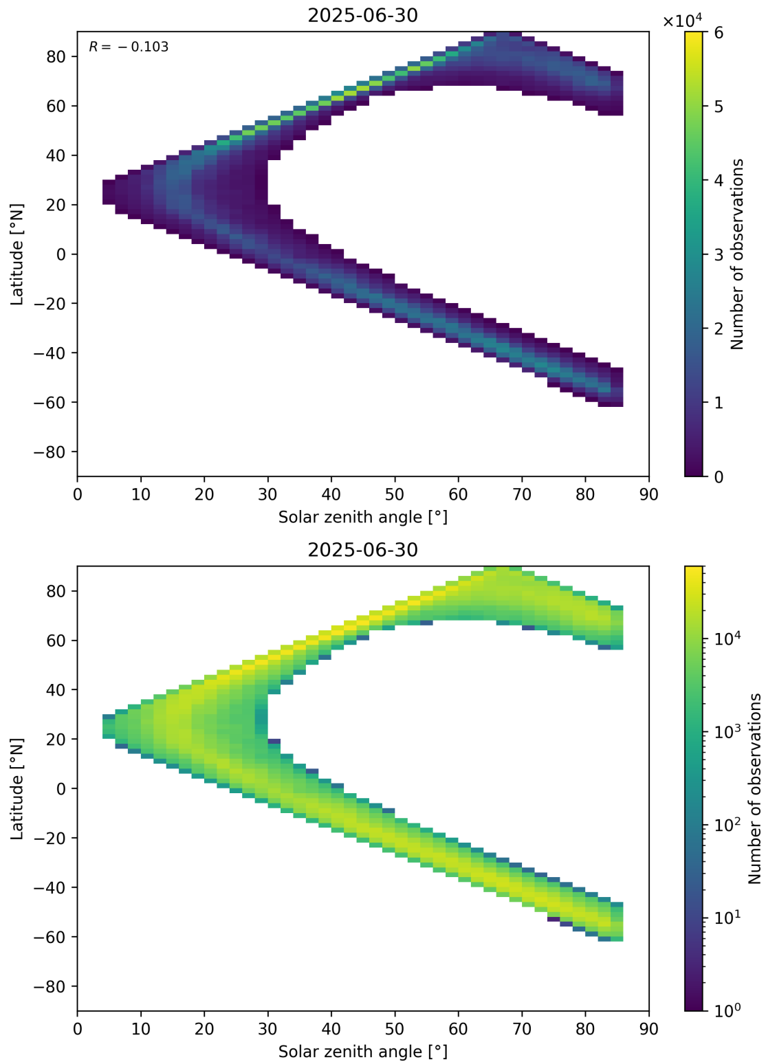
Figure 66: Scatter density plot of “Solar zenith angle” against “Latitude” for 2025-06-29 to 2025-07-01.
