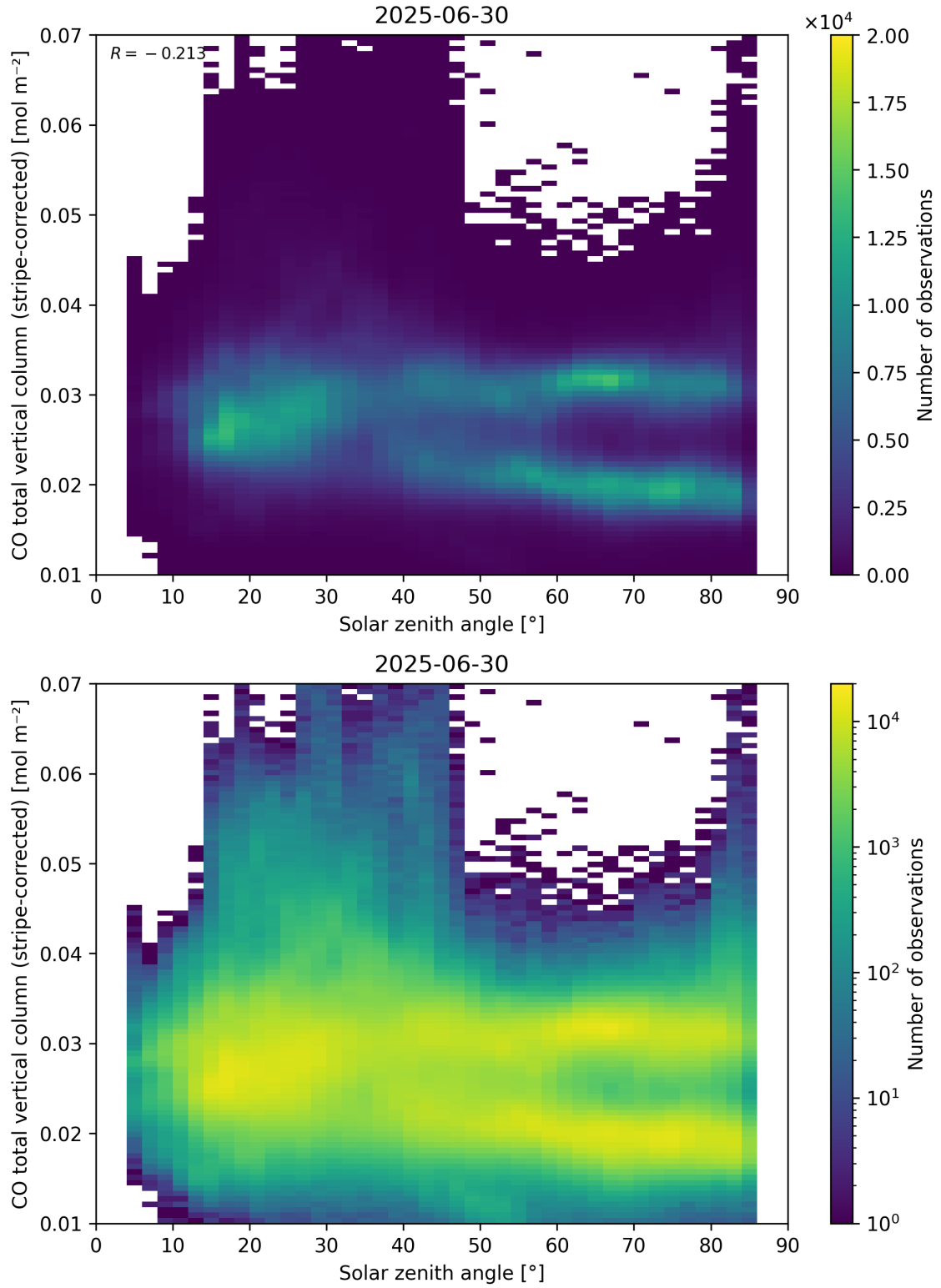
Figure 62: Scatter density plot of “Solar zenith angle” against “CO total vertical column (stripe-corrected)” for 2025-06-29 to 2025-07-01.
