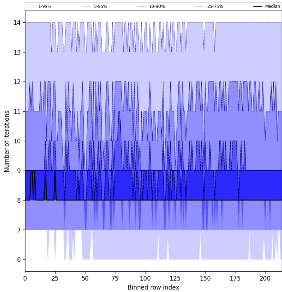
Figure 32: Along track statistics of “Number of iterations” for 2025-06-29 to 2025-07-01
