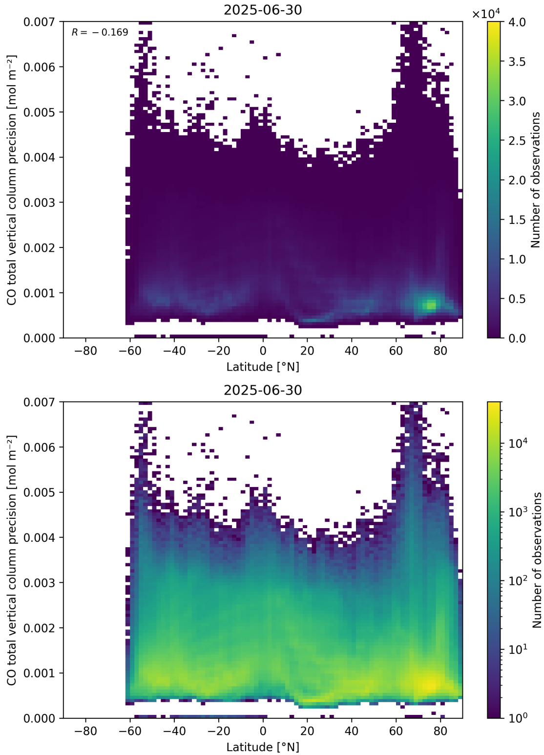
Figure 53: Scatter density plot of “Latitude” against “CO total vertical column precision” for 2025-06-29 to 2025-07-01.
