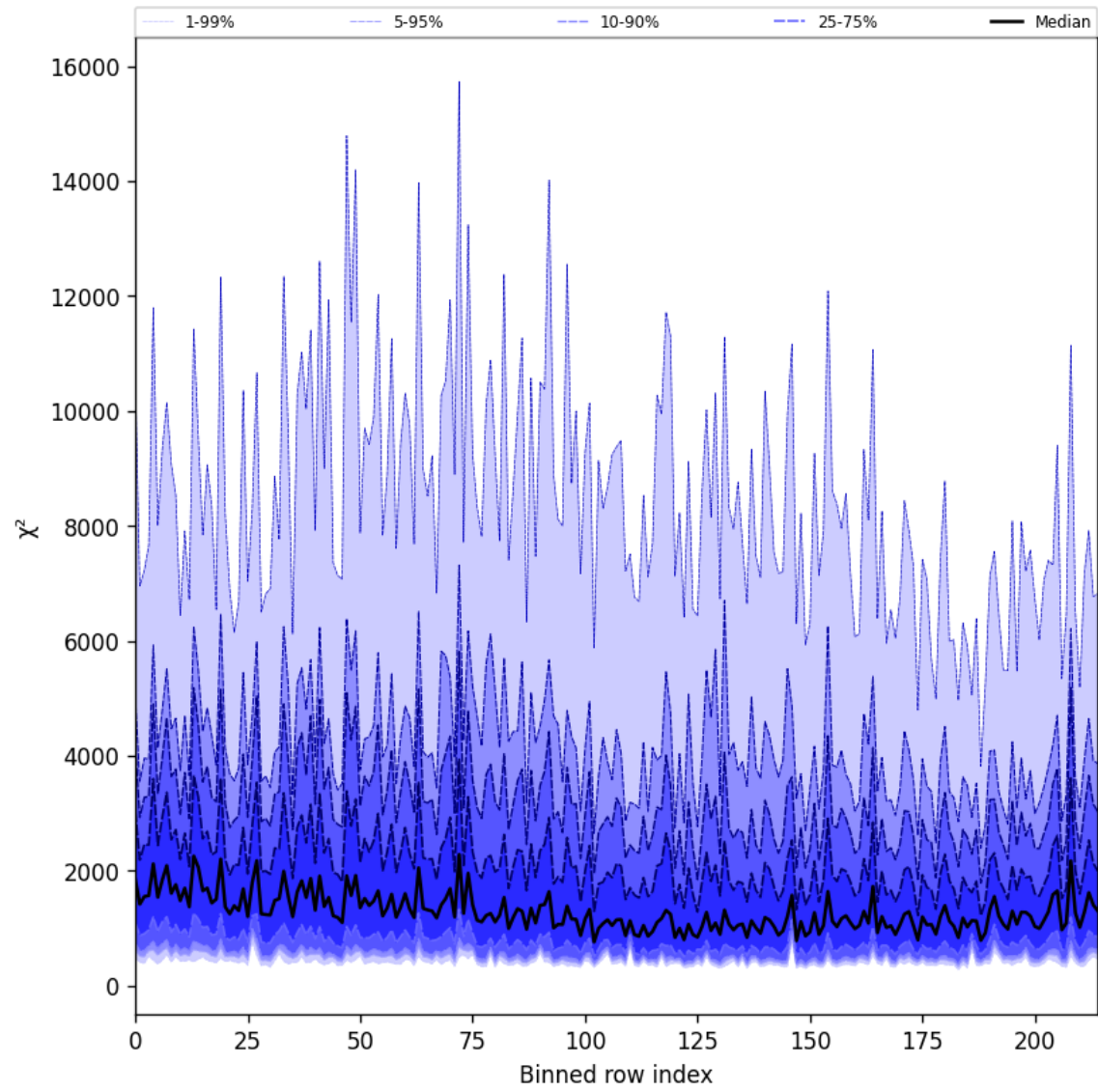
Figure 30: Along track statistics of “ \chi^2 ” for 2025-06-29 to 2025-07-01
