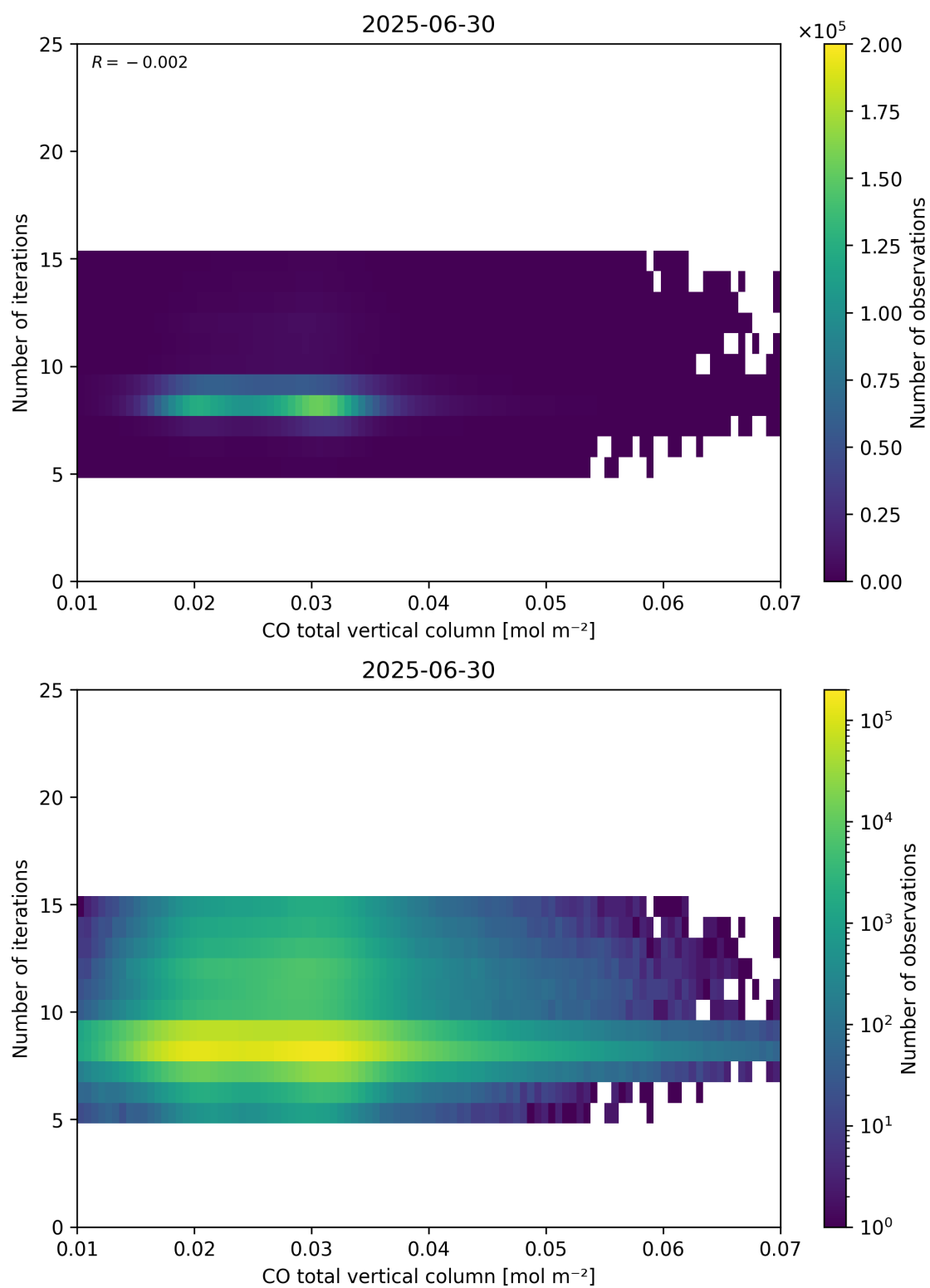
Figure 42: Scatter density plot of “CO total vertical column” against “Number of iterations” for 2025-06-29 to 2025-07-01.
