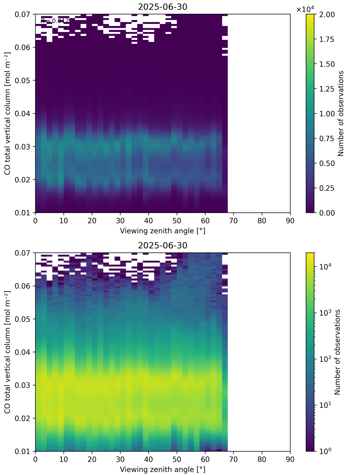
Figure 69: Scatter density plot of “Viewing zenith angle” against “CO total vertical column” for 2025-06-29 to 2025-07-01.
