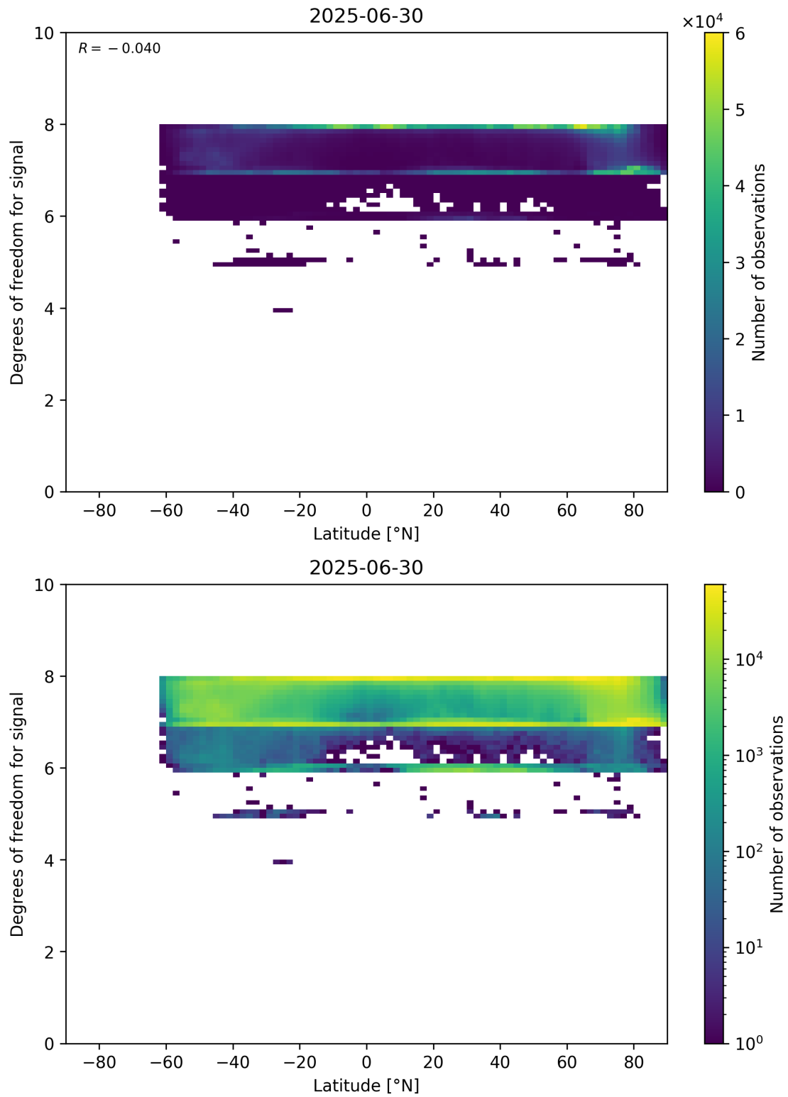
Figure 55: Scatter density plot of “Latitude” against “Degrees of freedom for signal” for 2025-06-29 to 2025-07-01.
