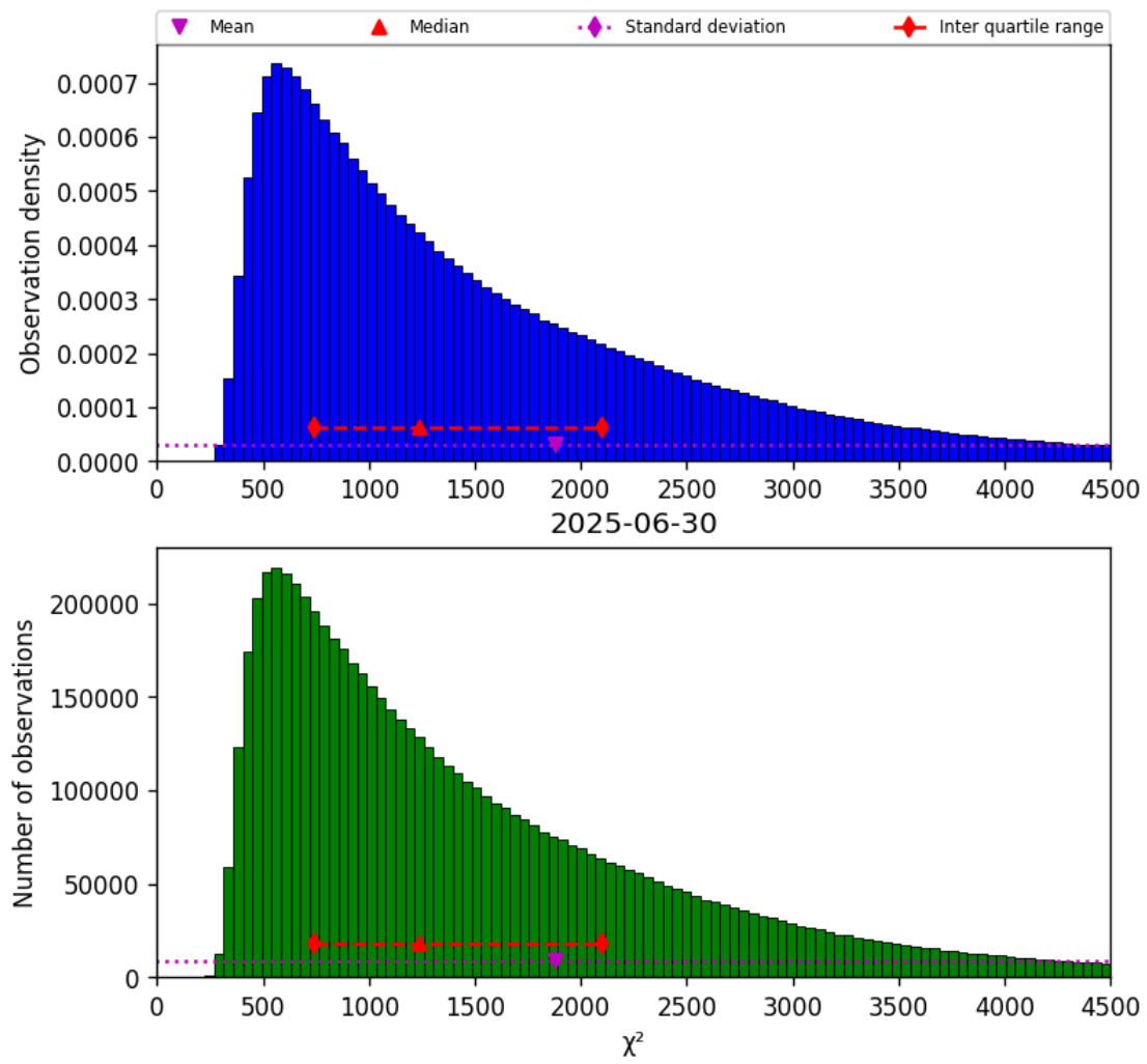
Figure 22: Histogram of “ \chi^2 ” for 2025-06-29 to 2025-07-01
