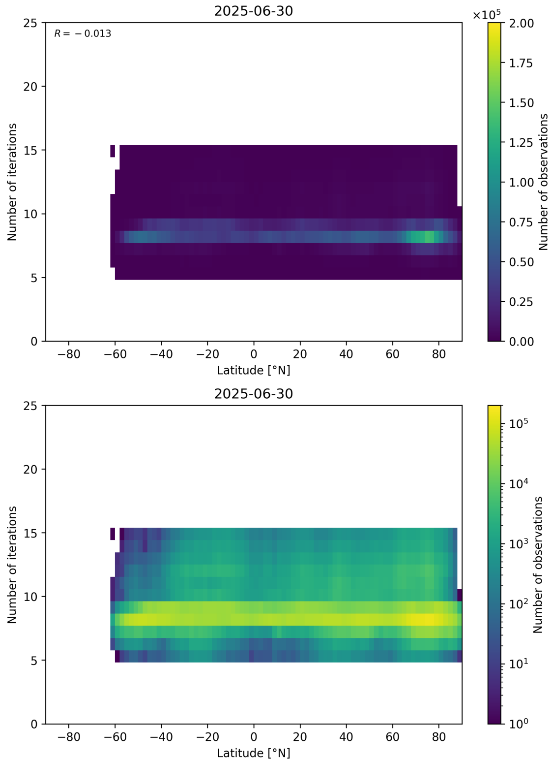
Figure 56: Scatter density plot of “Latitude” against “Number of iterations” for 2025-06-29 to 2025-07-01.
