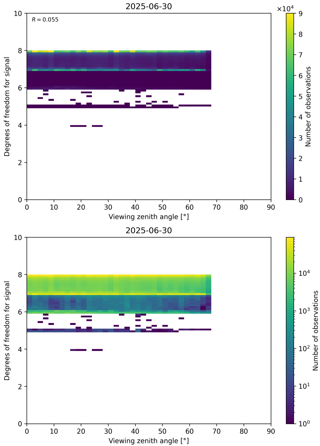
Figure 73: Scatter density plot of “Viewing zenith angle” against “Degrees of freedom for signal” for 2025-06-29 to 2025-07-01.
