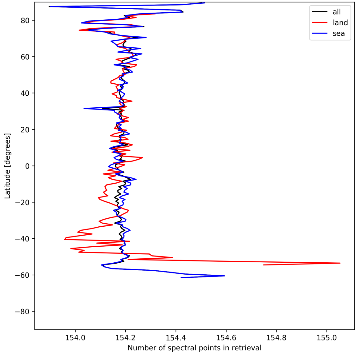
Figure 13: Zonal average of “Number of spectral points in retrieval” for 2025-06-29 to 2025-07-01.
