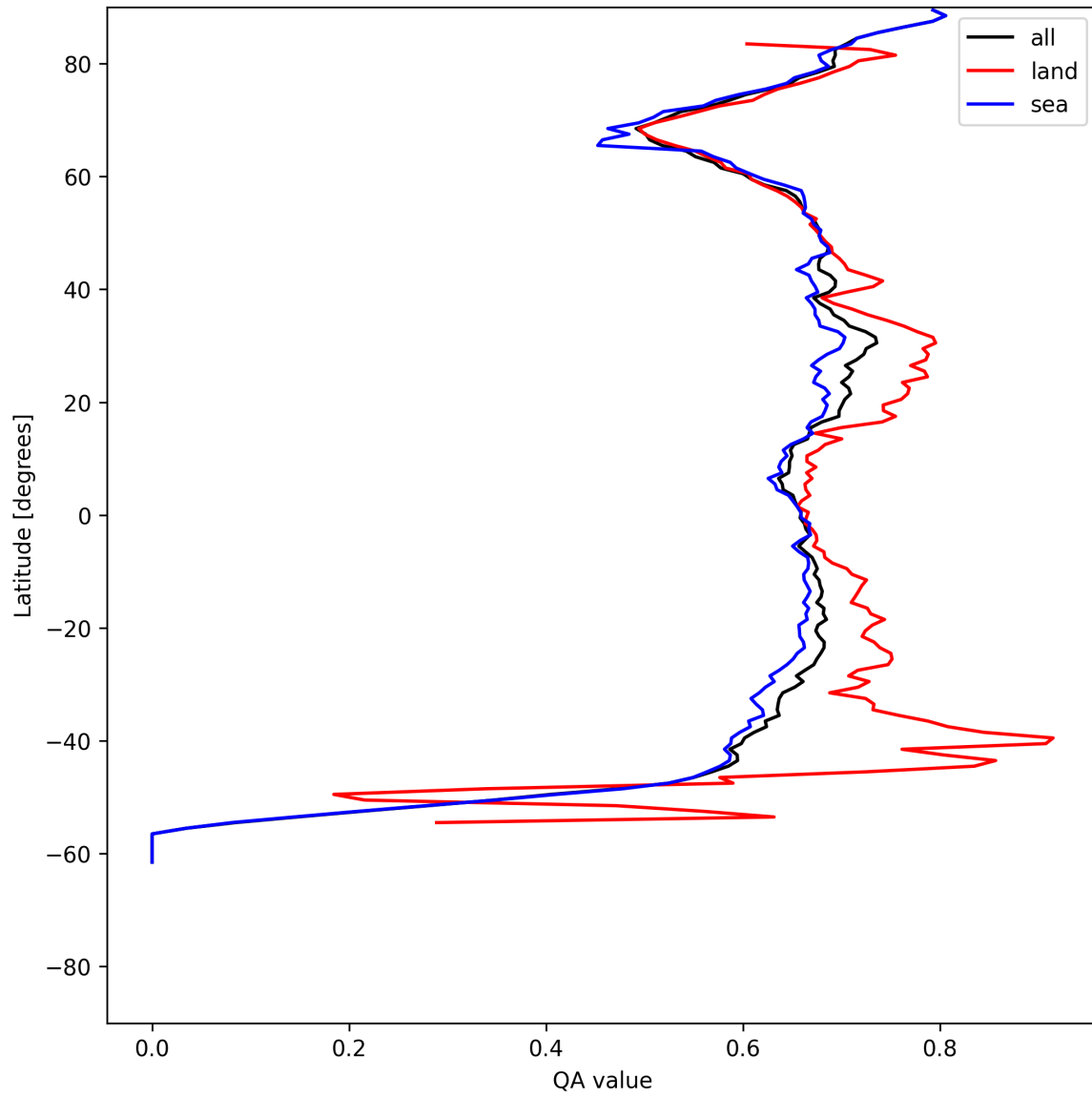
Figure 9: Zonal average of “QA value” for 2025-06-29 to 2025-07-01.
