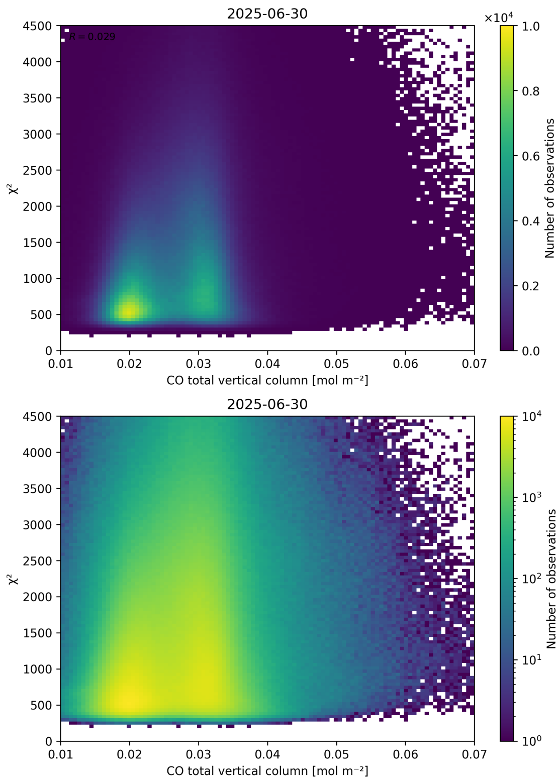
Figure 35: Scatter density plot of “CO total vertical column” against “ \chi^2 ” for 2025-06-29 to 2025-07-01.
