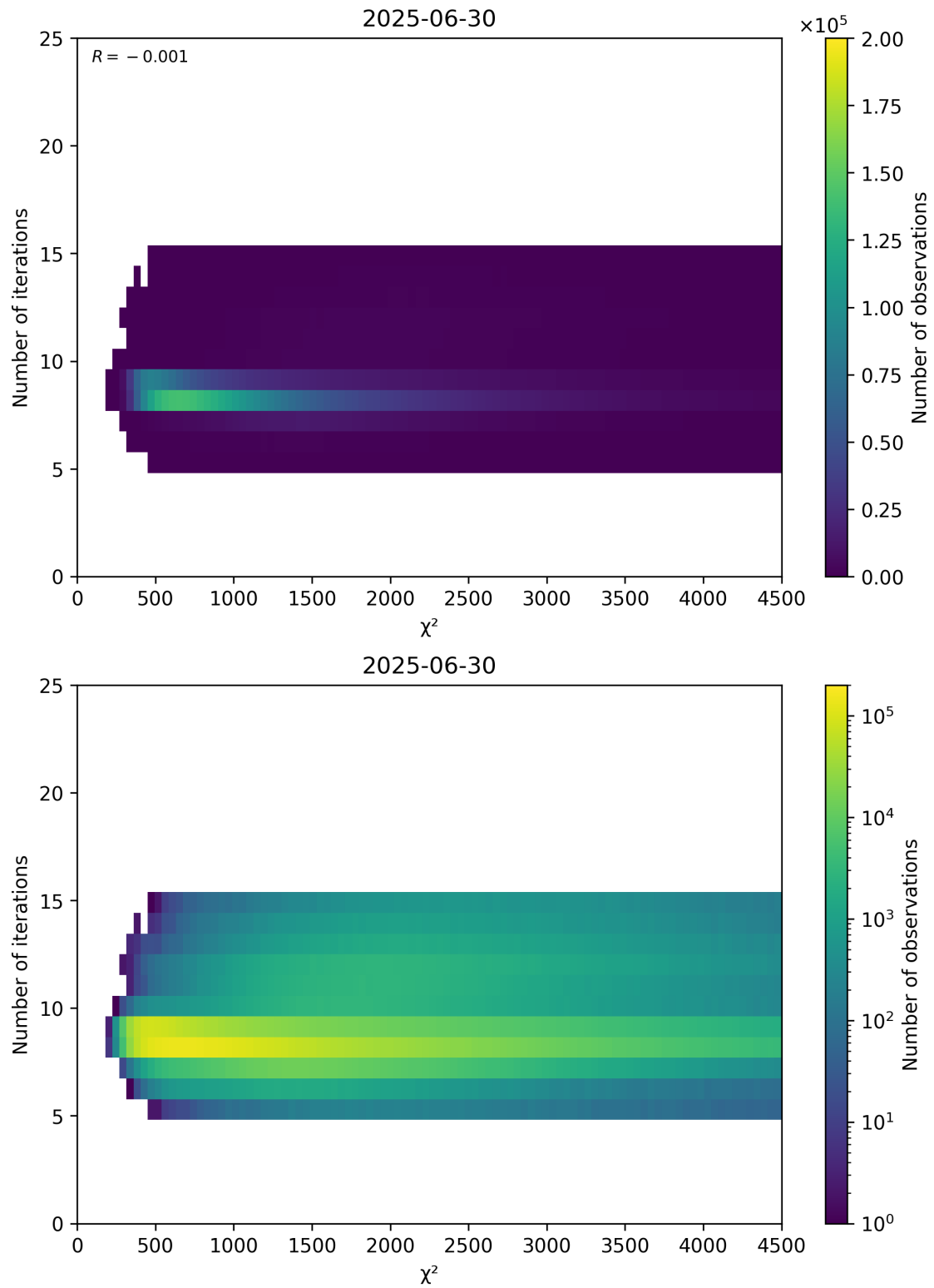
Figure 49: Scatter density plot of “ \chi^2 ” against “Number of iterations” for 2025-06-29 to 2025-07-01.
