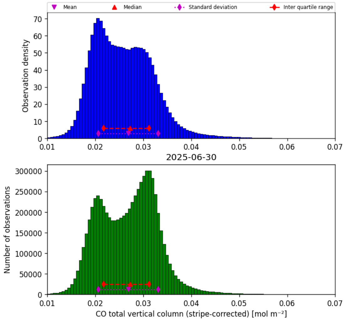
Figure 19: Histogram of “CO total vertical column (stripe-corrected)” for 2025-06-29 to 2025-07-01
