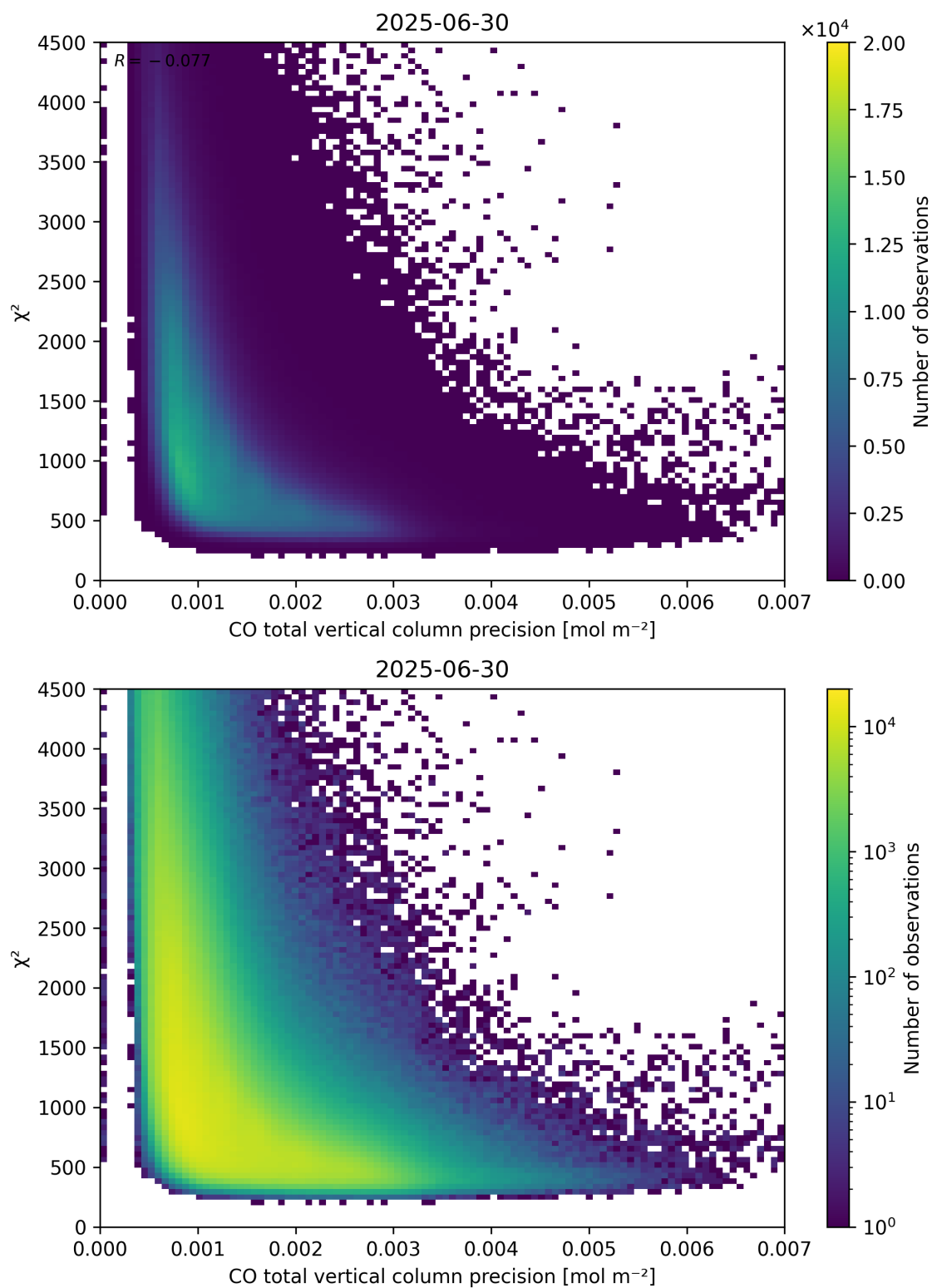
Figure 44: Scatter density plot of “CO total vertical column precision” against “ \chi^2 ” for 2025-06-29 to 2025-07-01.
