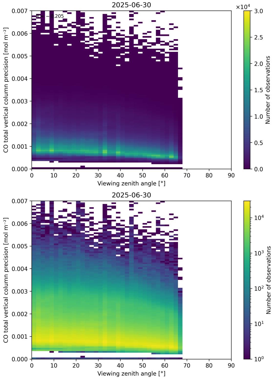
Figure 71: Scatter density plot of “Viewing zenith angle” against “CO total vertical column precision” for 2025-06-29 to 2025-07-01.
