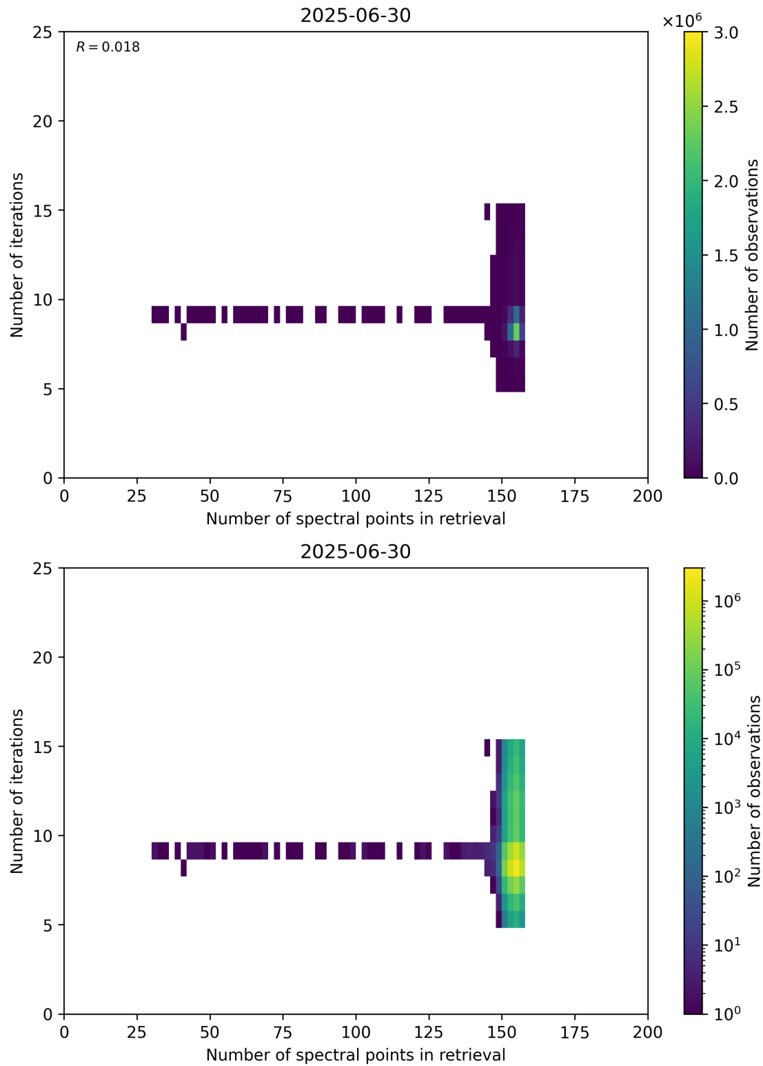
Figure 60: Scatter density plot of “Number of spectral points in retrieval” against “Number of iterations” for 2025-06-29 to 2025-07-01.
