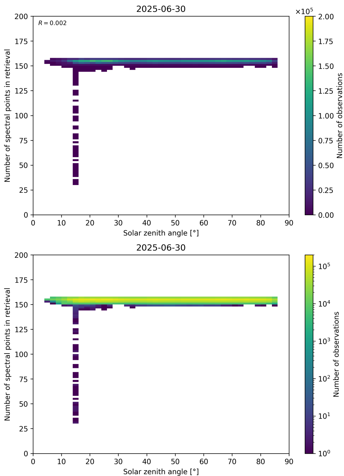
Figure 68: Scatter density plot of “Solar zenith angle” against “Number of spectral points in retrieval” for 2025-06-29 to 2025-07-01.
