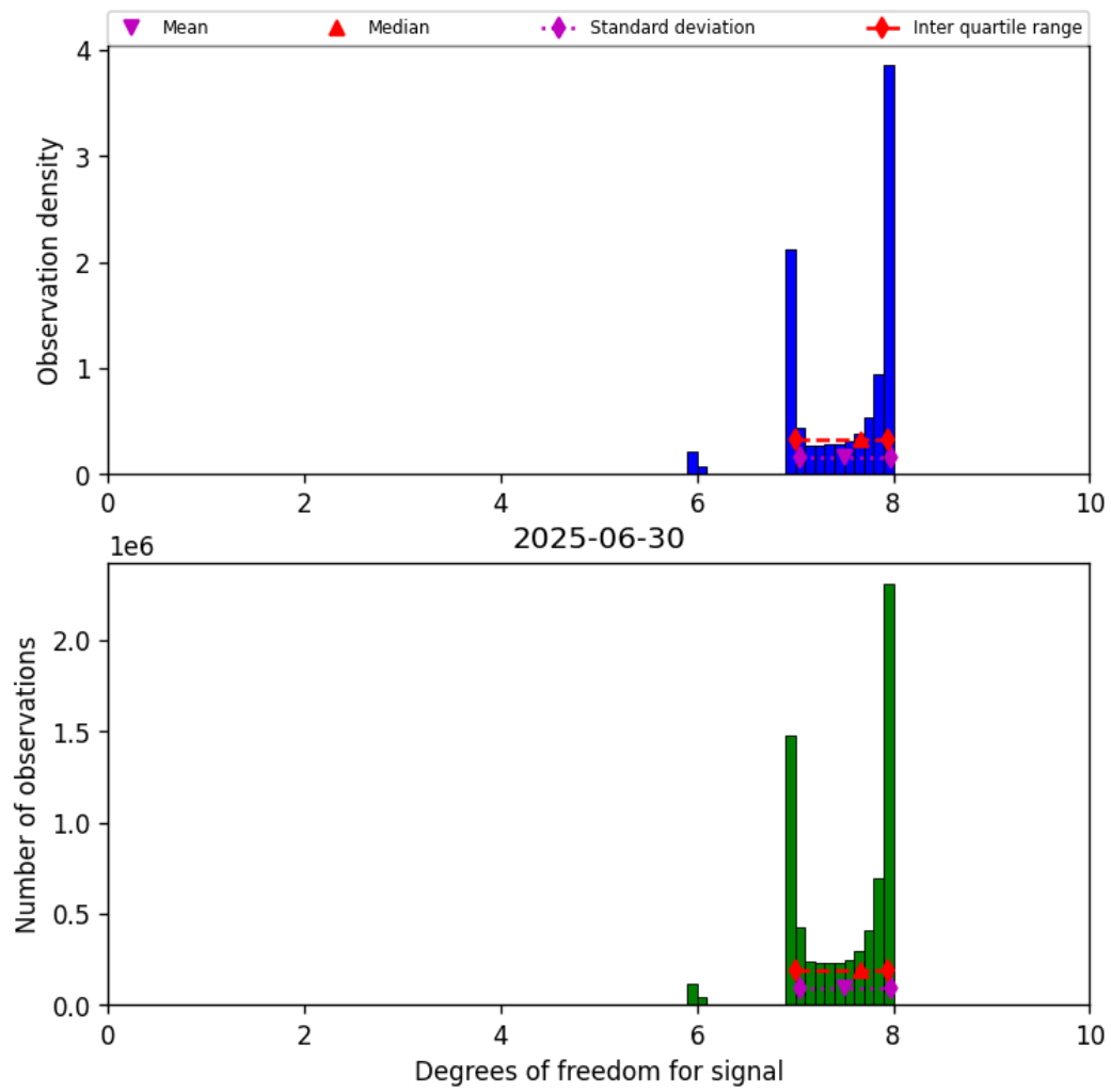
Figure 23: Histogram of “Degrees of freedom for signal” for 2025-06-29 to 2025-07-01
