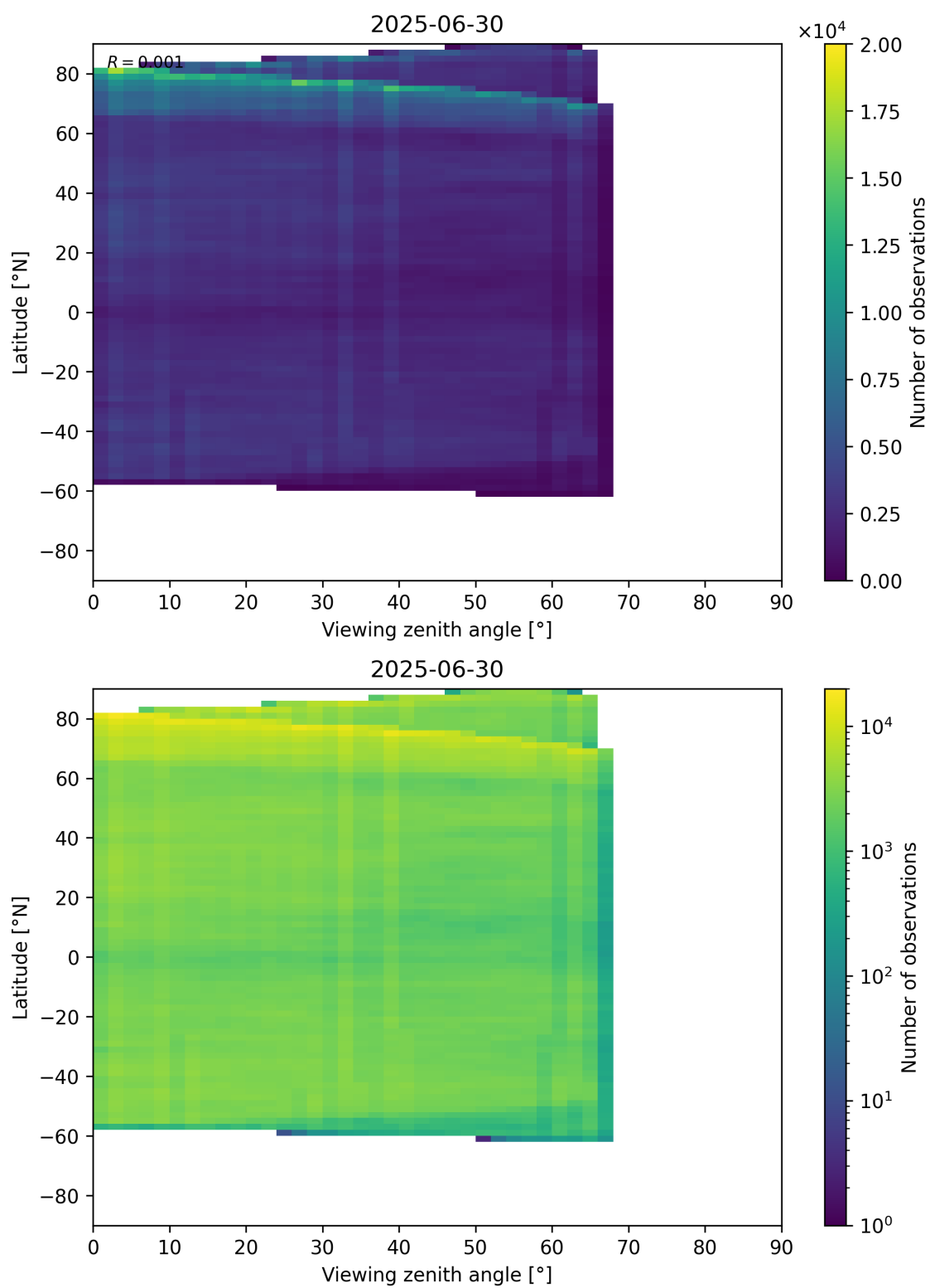
Figure 74: Scatter density plot of “Viewing zenith angle” against “Latitude” for 2025-06-29 to 2025-07-01.
