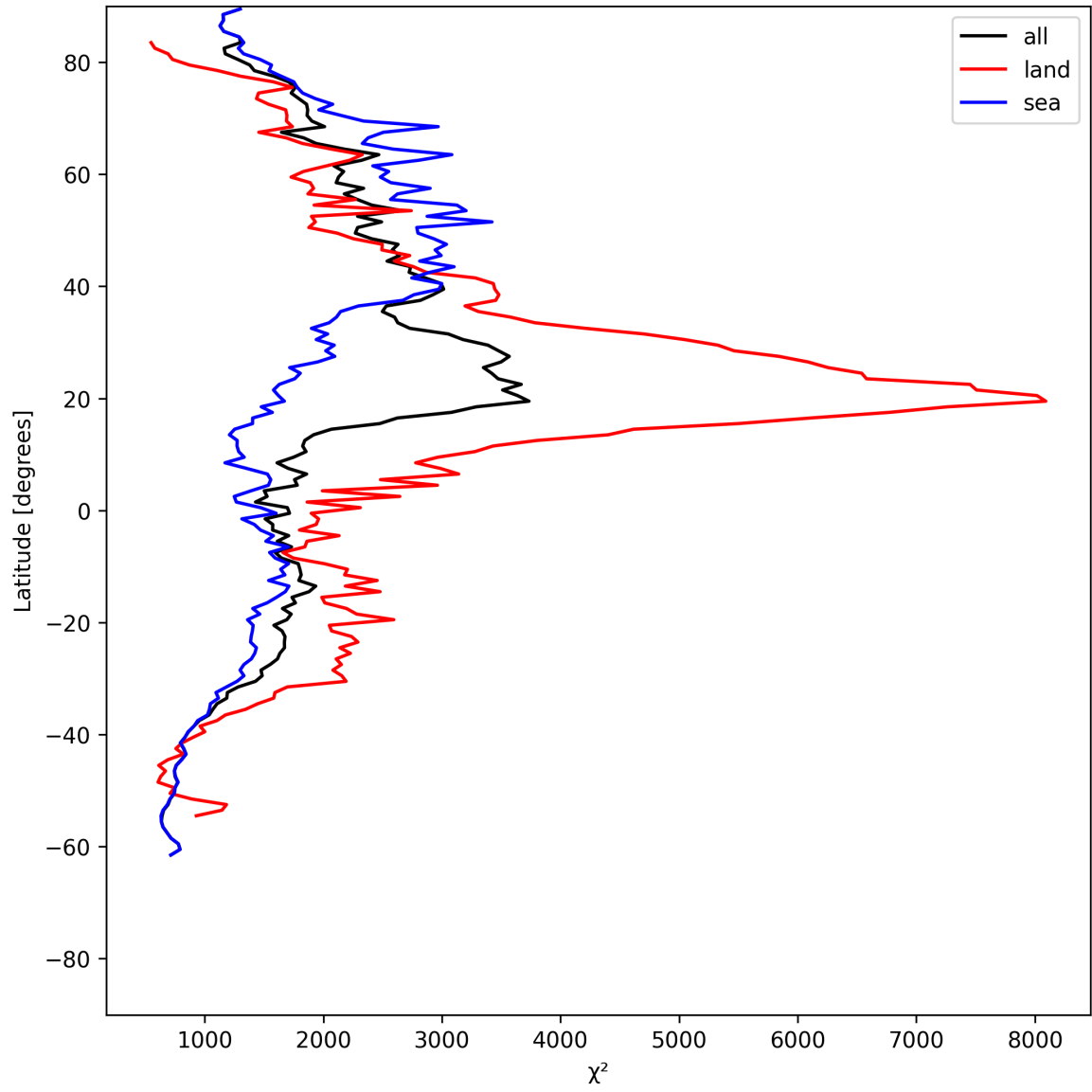
Figure 14: Zonal average of “ \chi^2 ” for 2025-06-29 to 2025-07-01.
