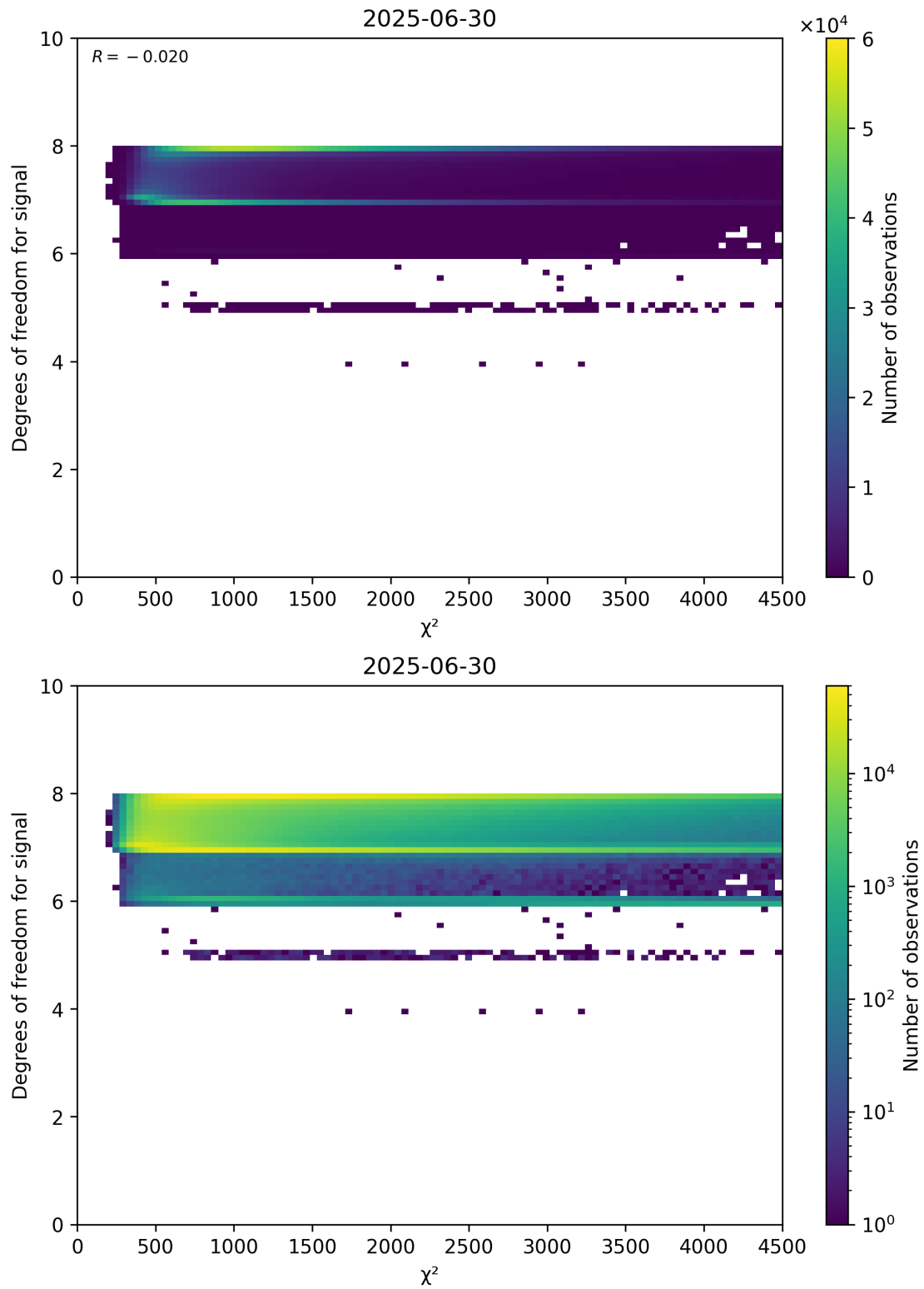
Figure 48: Scatter density plot of “ \chi^2 ” against “Degrees of freedom for signal” for 2025-06-29 to 2025-07-01.
