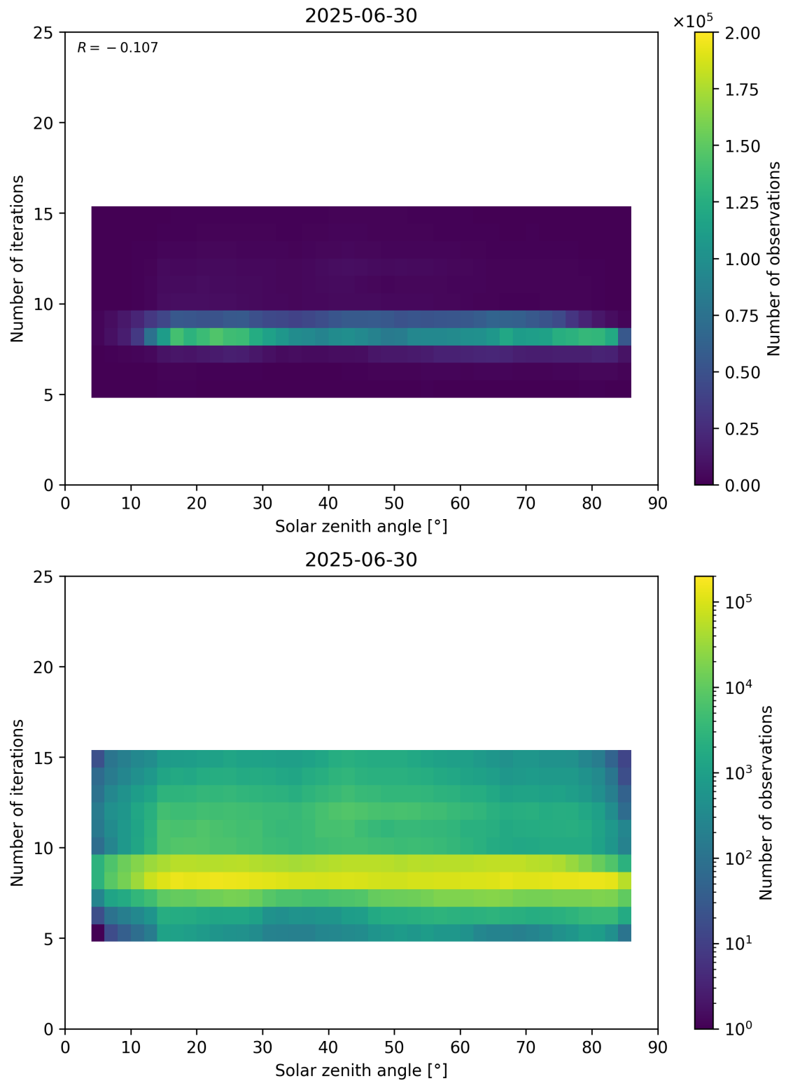
Figure 67: Scatter density plot of “Solar zenith angle” against “Number of iterations” for 2025-06-29 to 2025-07-01.
