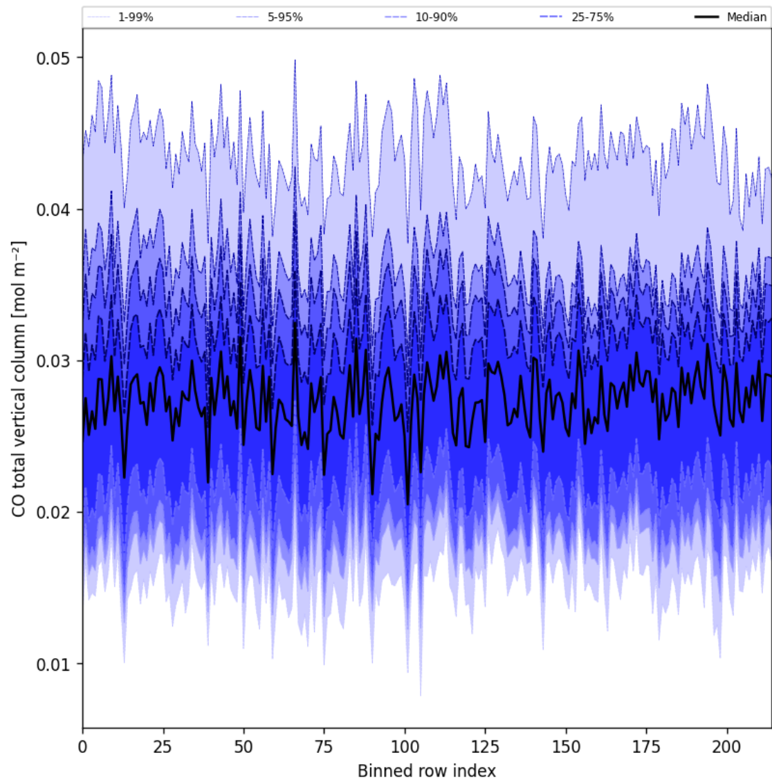
Figure 26: Along track statistics of “CO total vertical column” for 2025-06-29 to 2025-07-01
