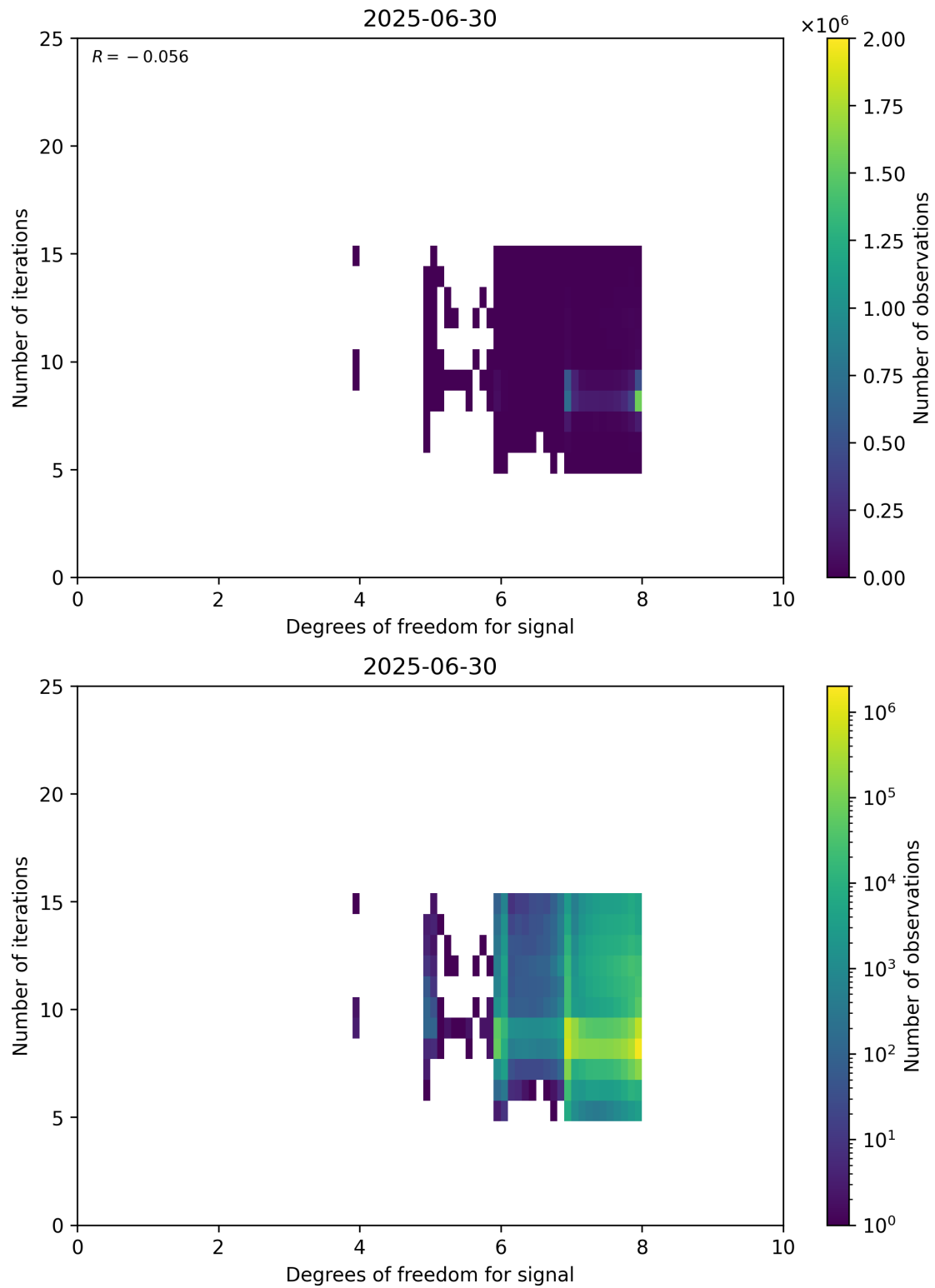
Figure 50: Scatter density plot of “Degrees of freedom for signal” against “Number of iterations” for 2025-06-29 to 2025-07-01.
