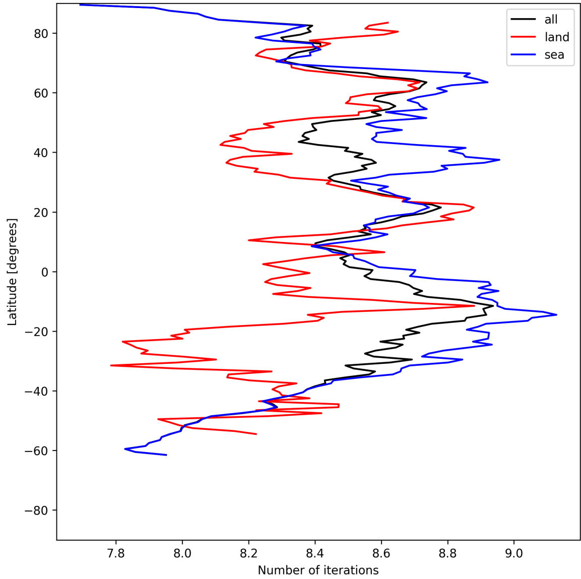
Figure 16: Zonal average of “Number of iterations” for 2025-06-29 to 2025-07-01.
