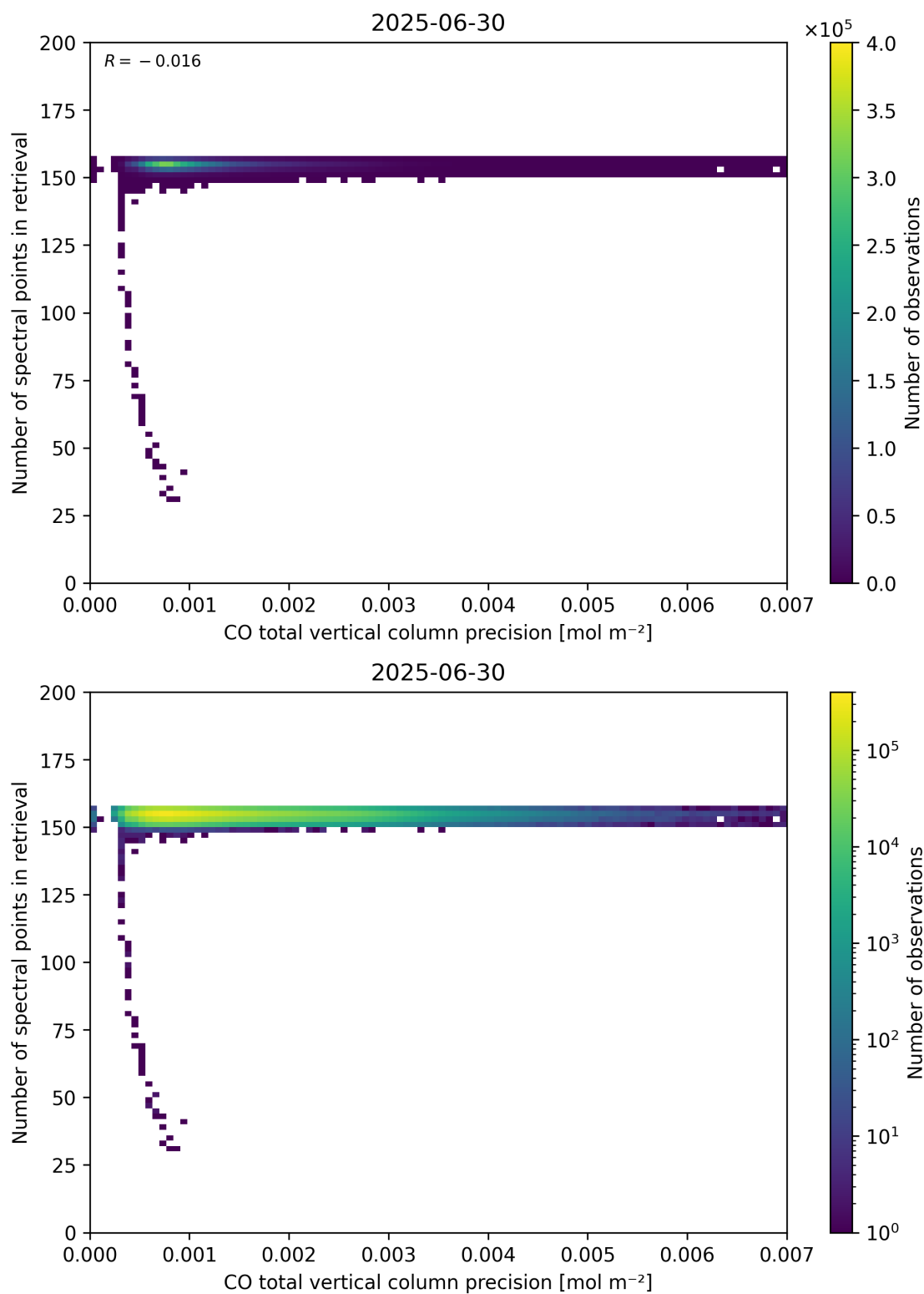
Figure 47: Scatter density plot of “CO total vertical column precision” against “Number of spectral points in retrieval” for 2025-06-29 to 2025-07-01.
