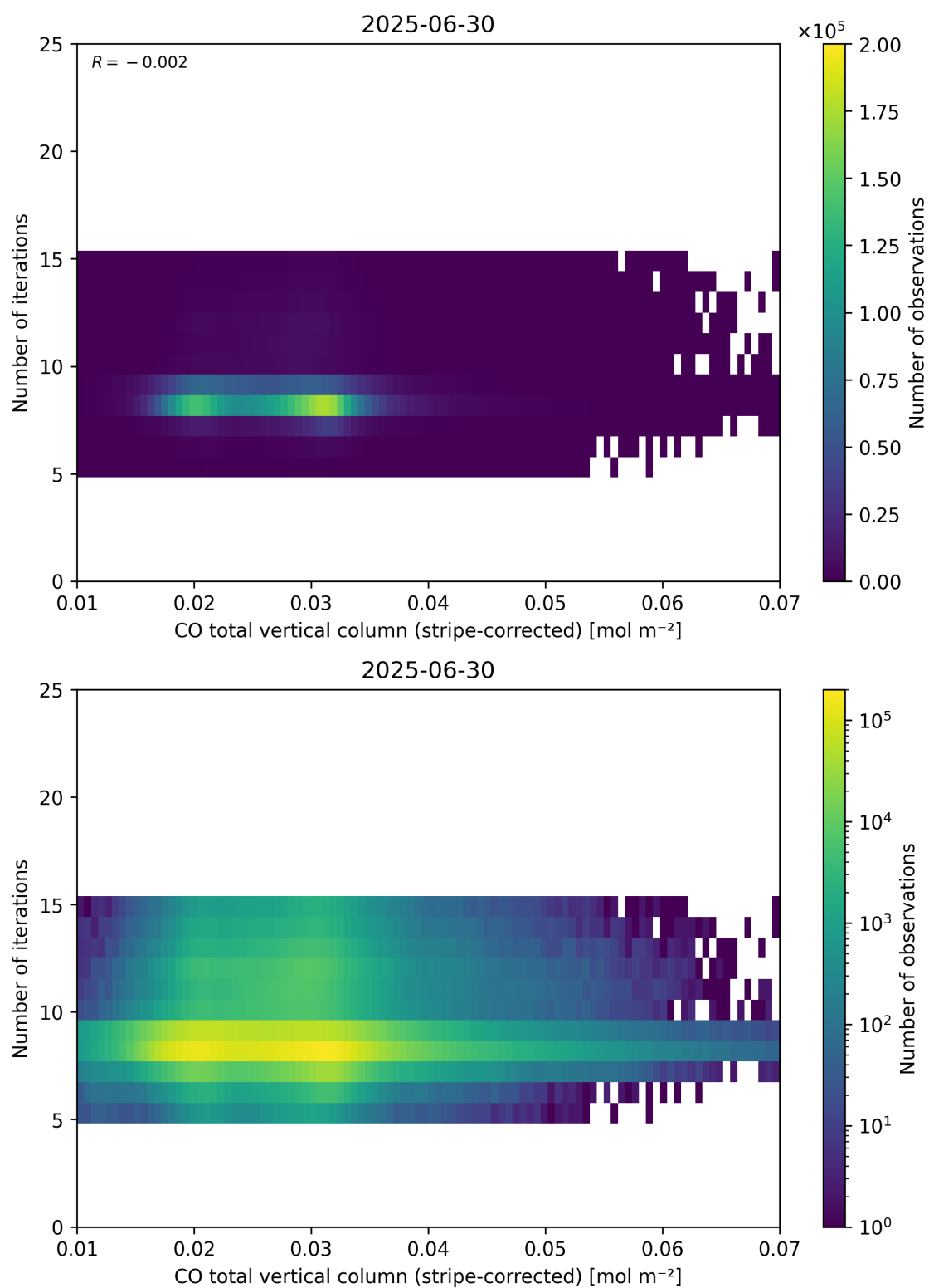
Figure 39: Scatter density plot of “CO total vertical column (stripe-corrected)” against “Number of iterations” for 2025-06-29 to 2025-07-01.
