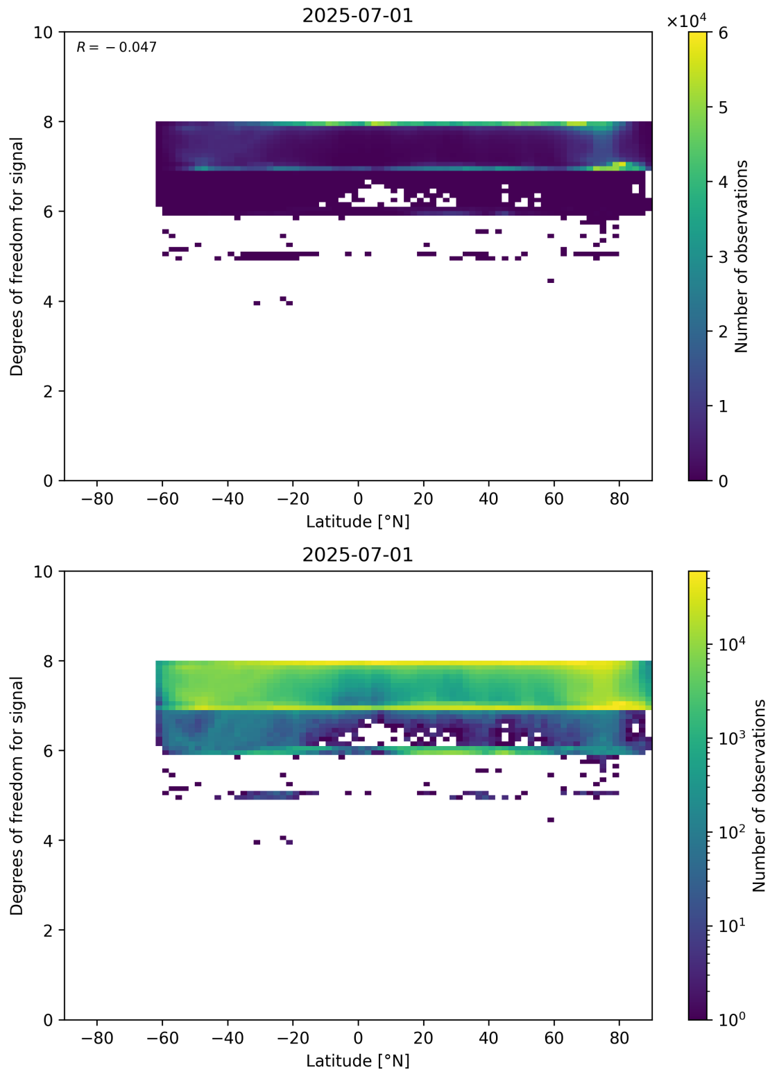
Figure 55: Scatter density plot of “Latitude” against “Degrees of freedom for signal” for 2025-06-30 to 2025-07-02.
