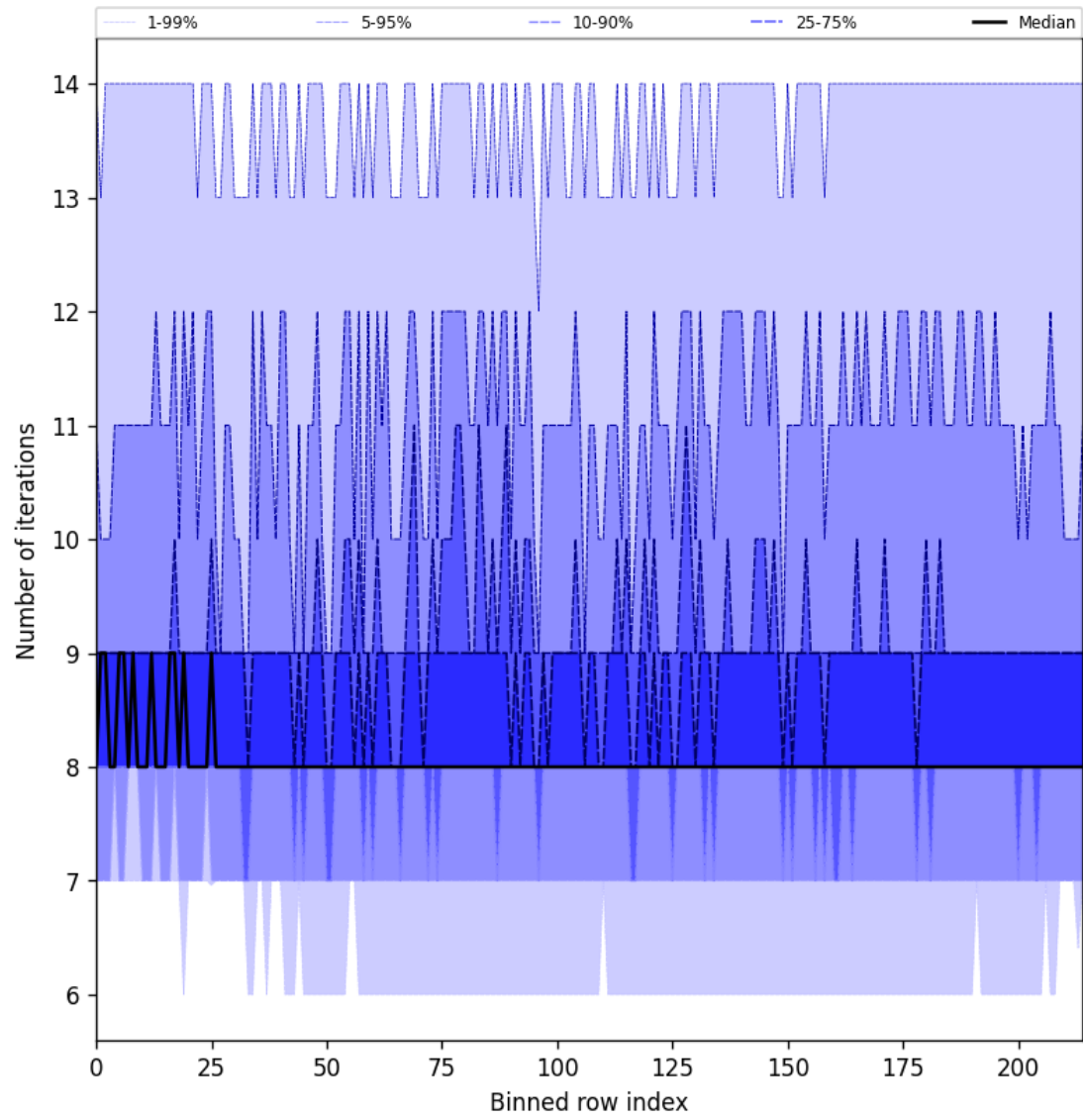
Figure 32: Along track statistics of “Number of iterations” for 2025-06-30 to 2025-07-02
