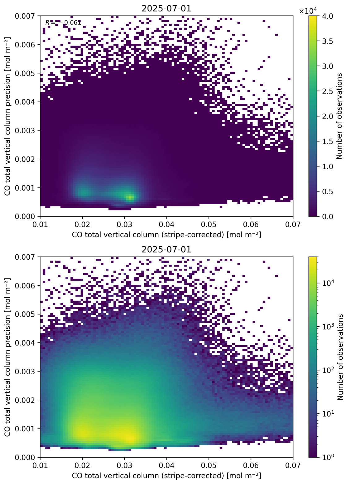
Figure 36: Scatter density plot of “CO total vertical column (stripe-corrected)” against “CO total vertical column precision” for 2025-06-30 to 2025-07-02.
