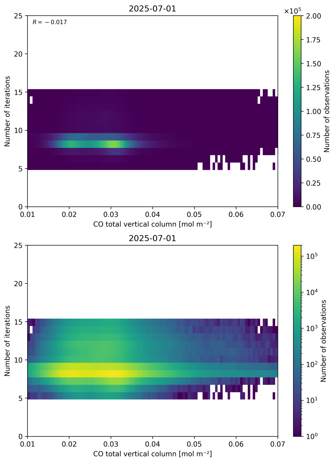
Figure 42: Scatter density plot of “CO total vertical column” against “Number of iterations” for 2025-06-30 to 2025-07-02.
