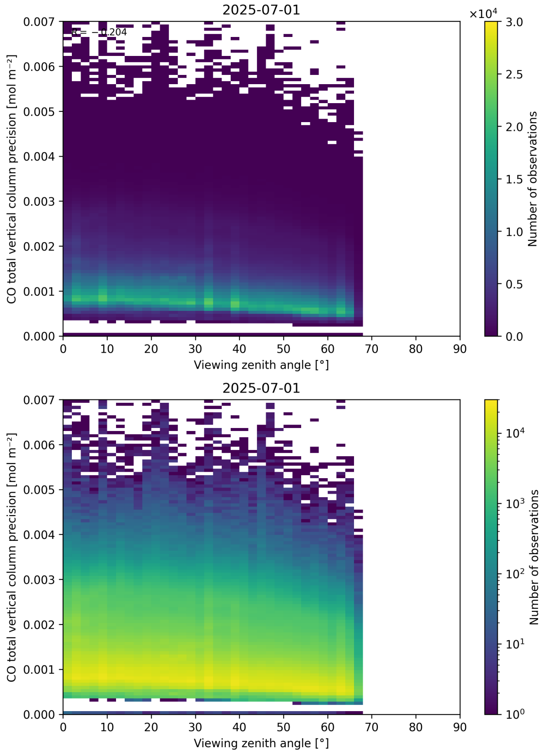
Figure 71: Scatter density plot of “Viewing zenith angle” against “CO total vertical column precision” for 2025-06-30 to 2025-07-02.
