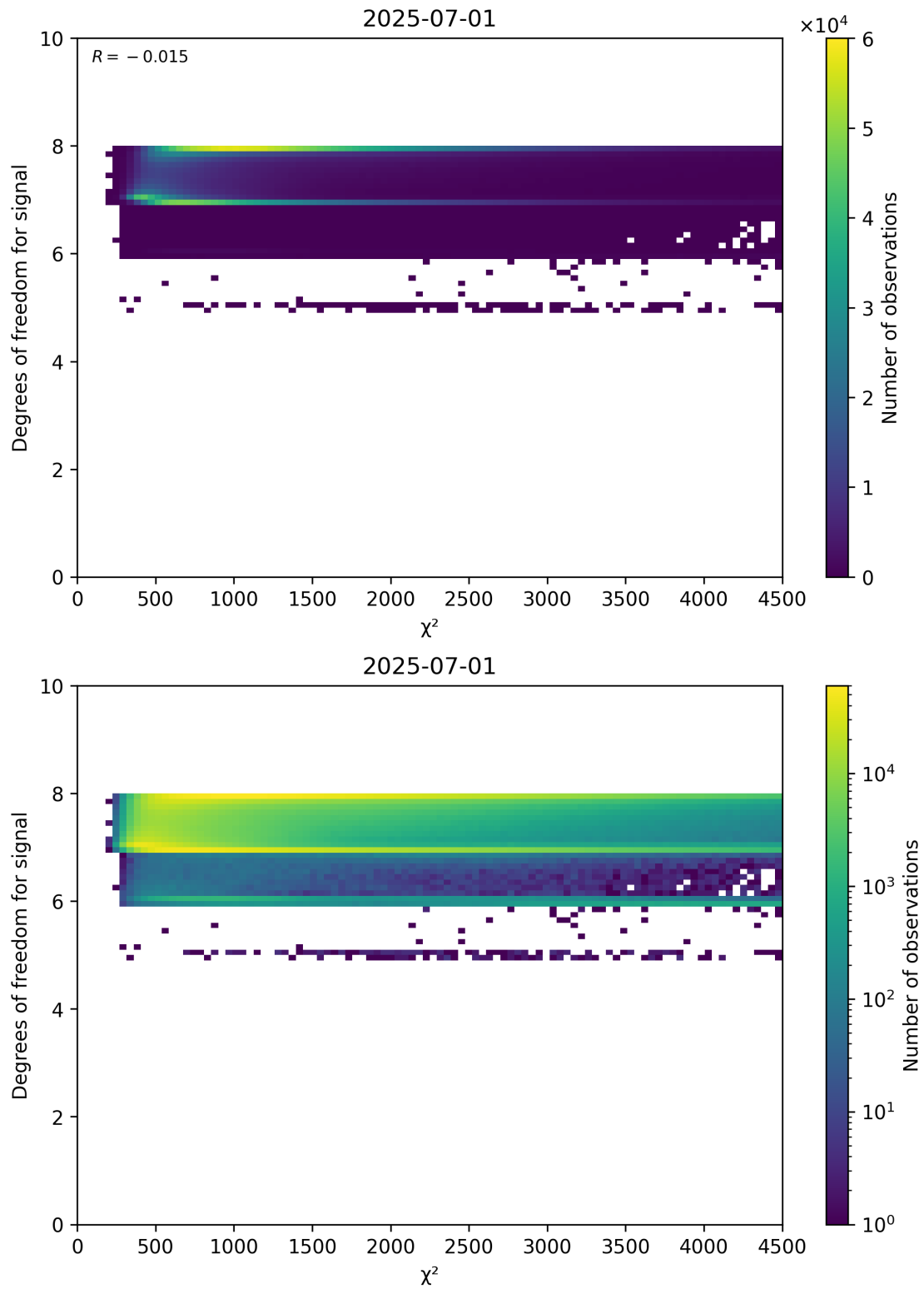
Figure 48: Scatter density plot of “ \chi^2 ” against “Degrees of freedom for signal” for 2025-06-30 to 2025-07-02.
