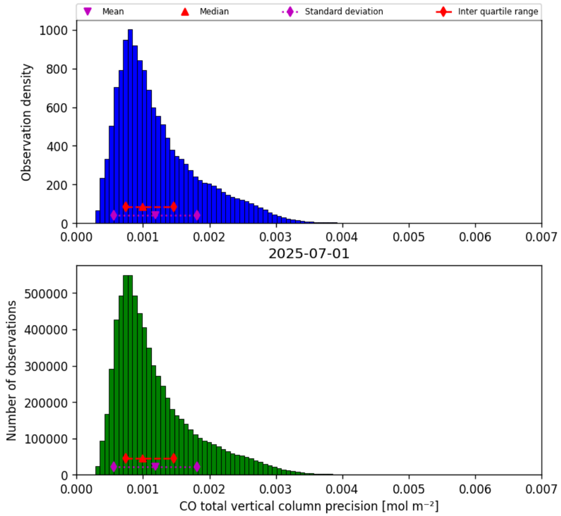
Figure 20: Histogram of “CO total vertical column precision” for 2025-06-30 to 2025-07-02
