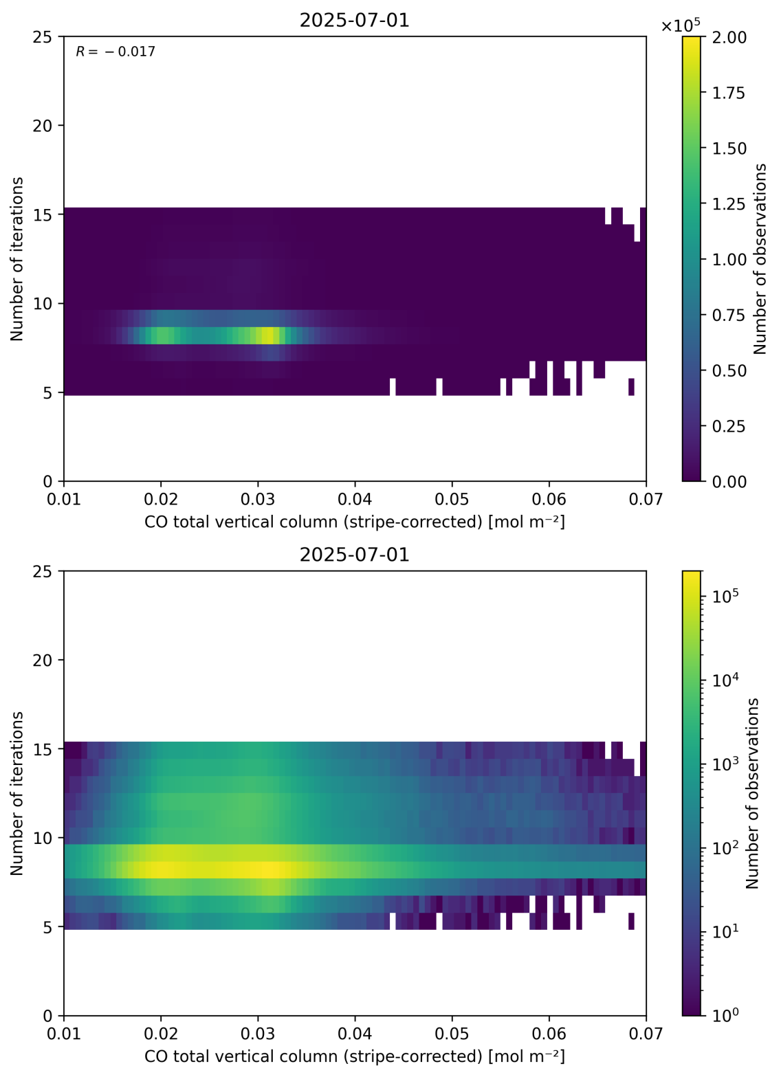
Figure 39: Scatter density plot of “CO total vertical column (stripe-corrected)” against “Number of iterations” for 2025-06-30 to 2025-07-02.
