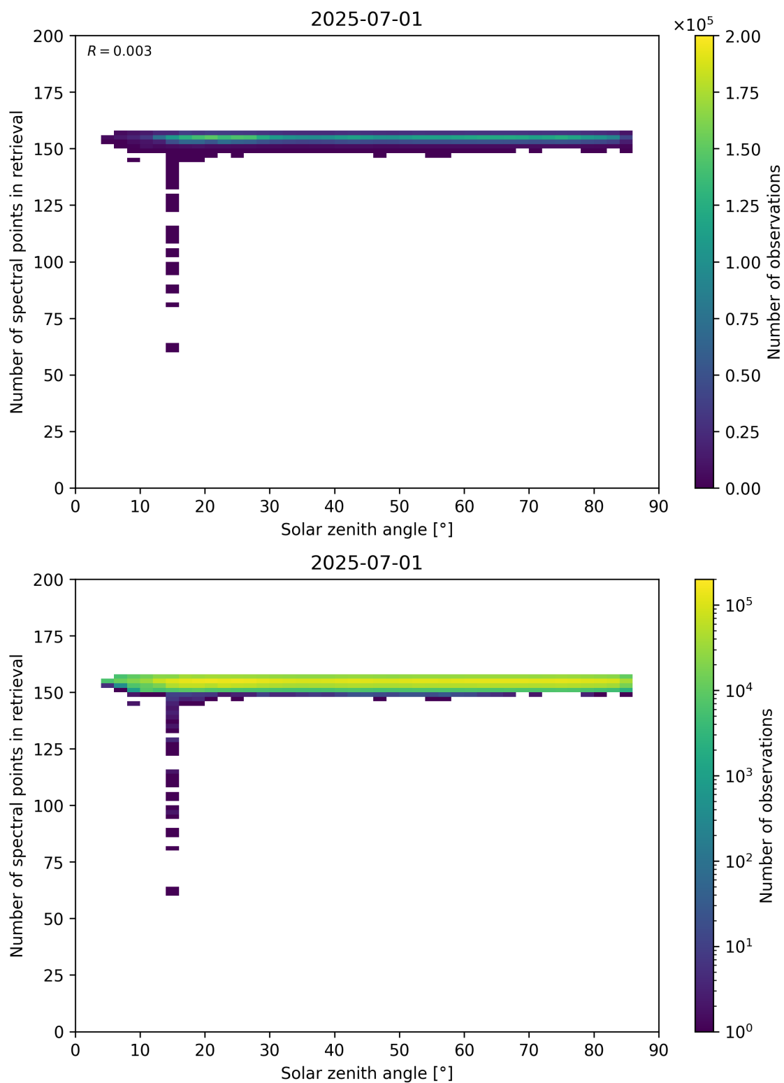
Figure 68: Scatter density plot of “Solar zenith angle” against “Number of spectral points in retrieval” for 2025-06-30 to 2025-07-02.
