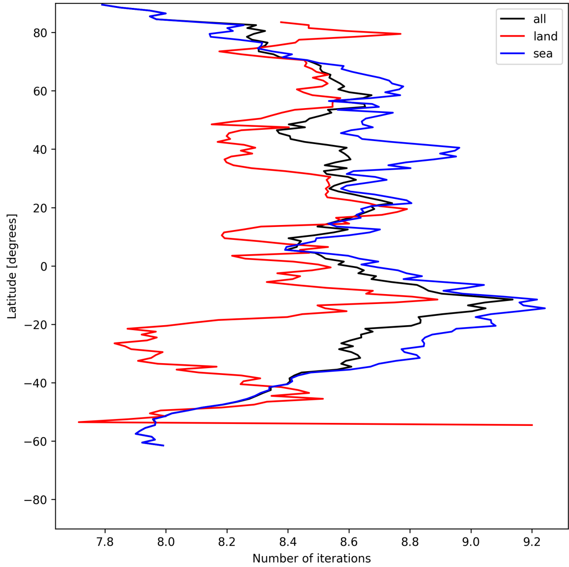
Figure 16: Zonal average of “Number of iterations” for 2025-06-30 to 2025-07-02.
