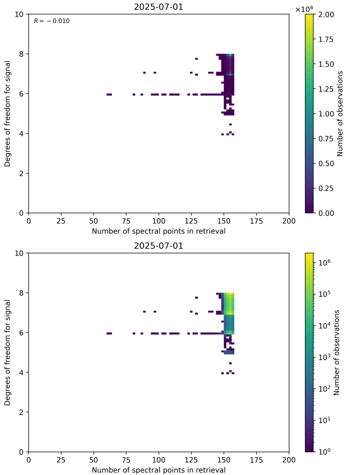
Figure 59: Scatter density plot of “Number of spectral points in retrieval” against “Degrees of freedom for signal” for 2025-06-30 to 2025-07-02.
