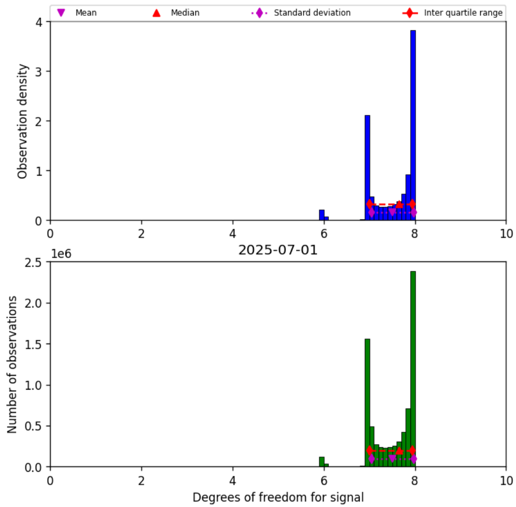
Figure 23: Histogram of “Degrees of freedom for signal” for 2025-06-30 to 2025-07-02
