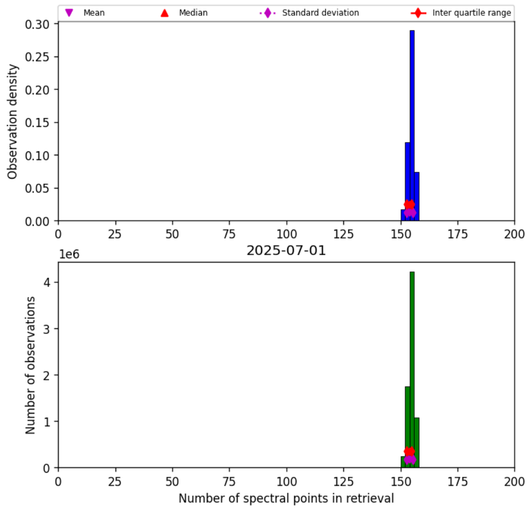
Figure 21: Histogram of “Number of spectral points in retrieval” for 2025-06-30 to 2025-07-02
