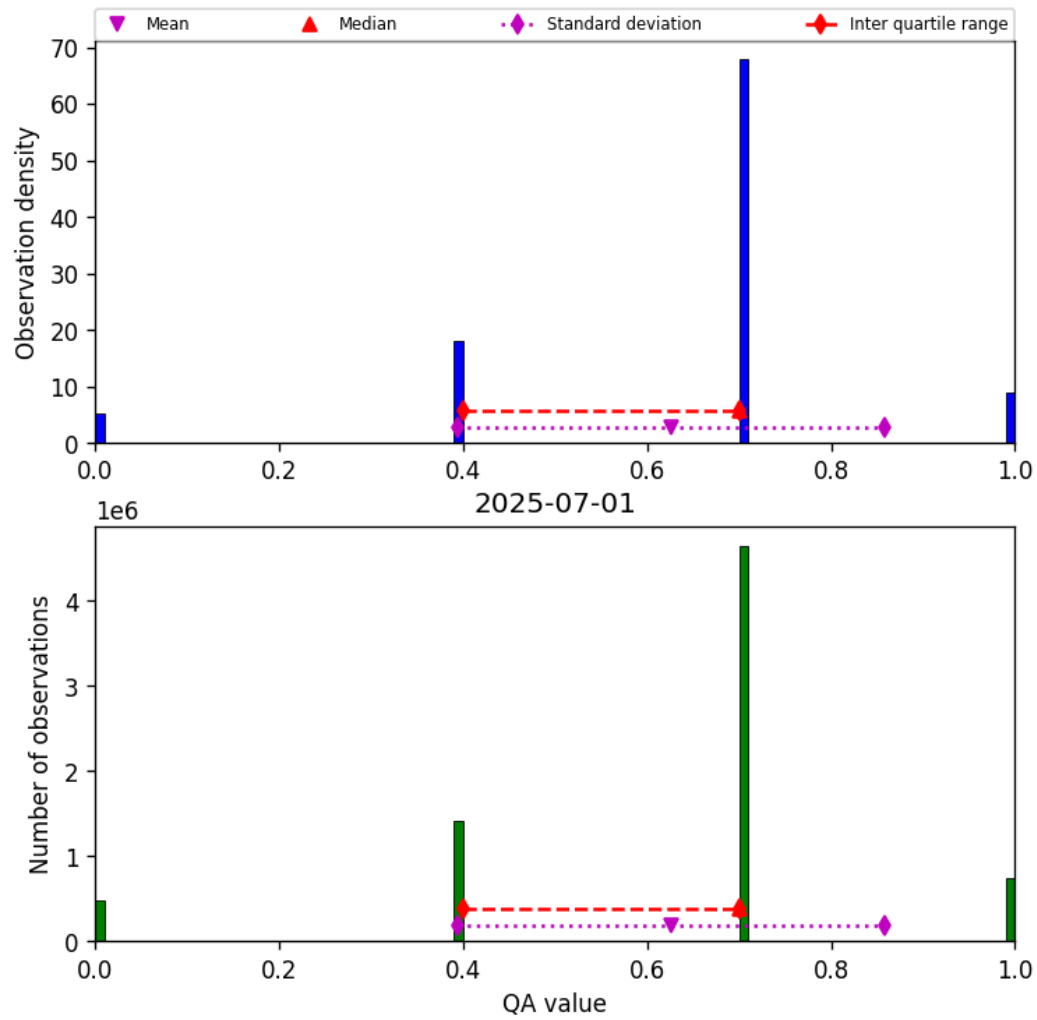
Figure 17: Histogram of “QA value” for 2025-06-30 to 2025-07-02
