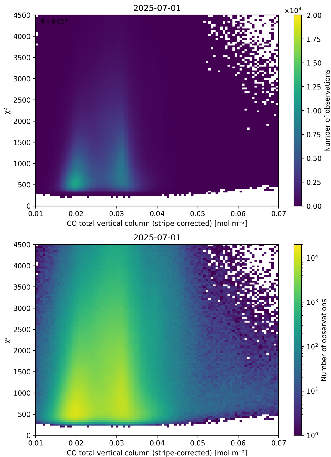
Figure 37: Scatter density plot of “CO total vertical column (stripe-corrected)” against “ \chi^2 ” for 2025-06-30 to 2025-07-02.
