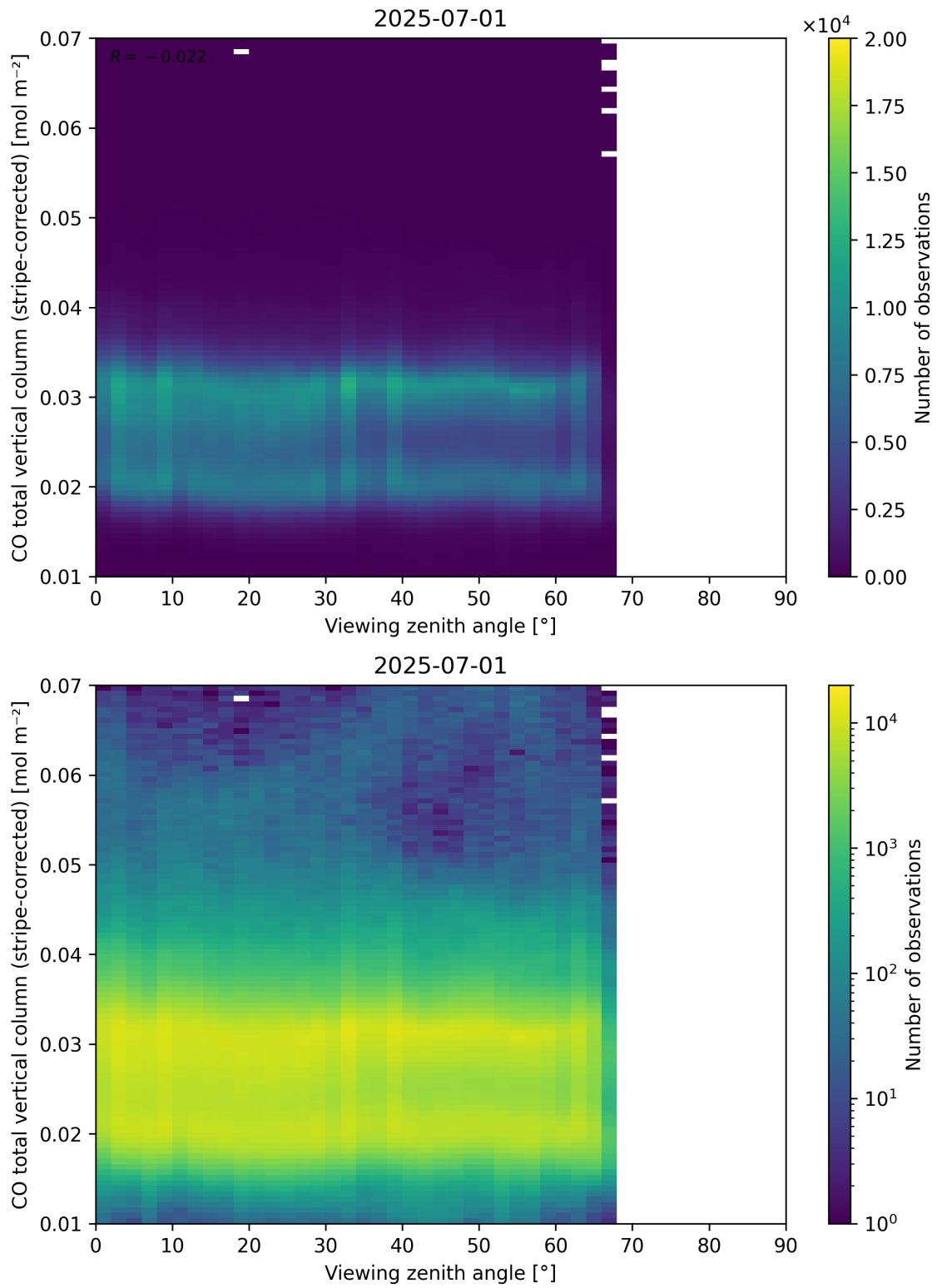
Figure 70: Scatter density plot of “Viewing zenith angle” against “CO total vertical column (stripe-corrected)” for 2025-06-30 to 2025-07-02.
