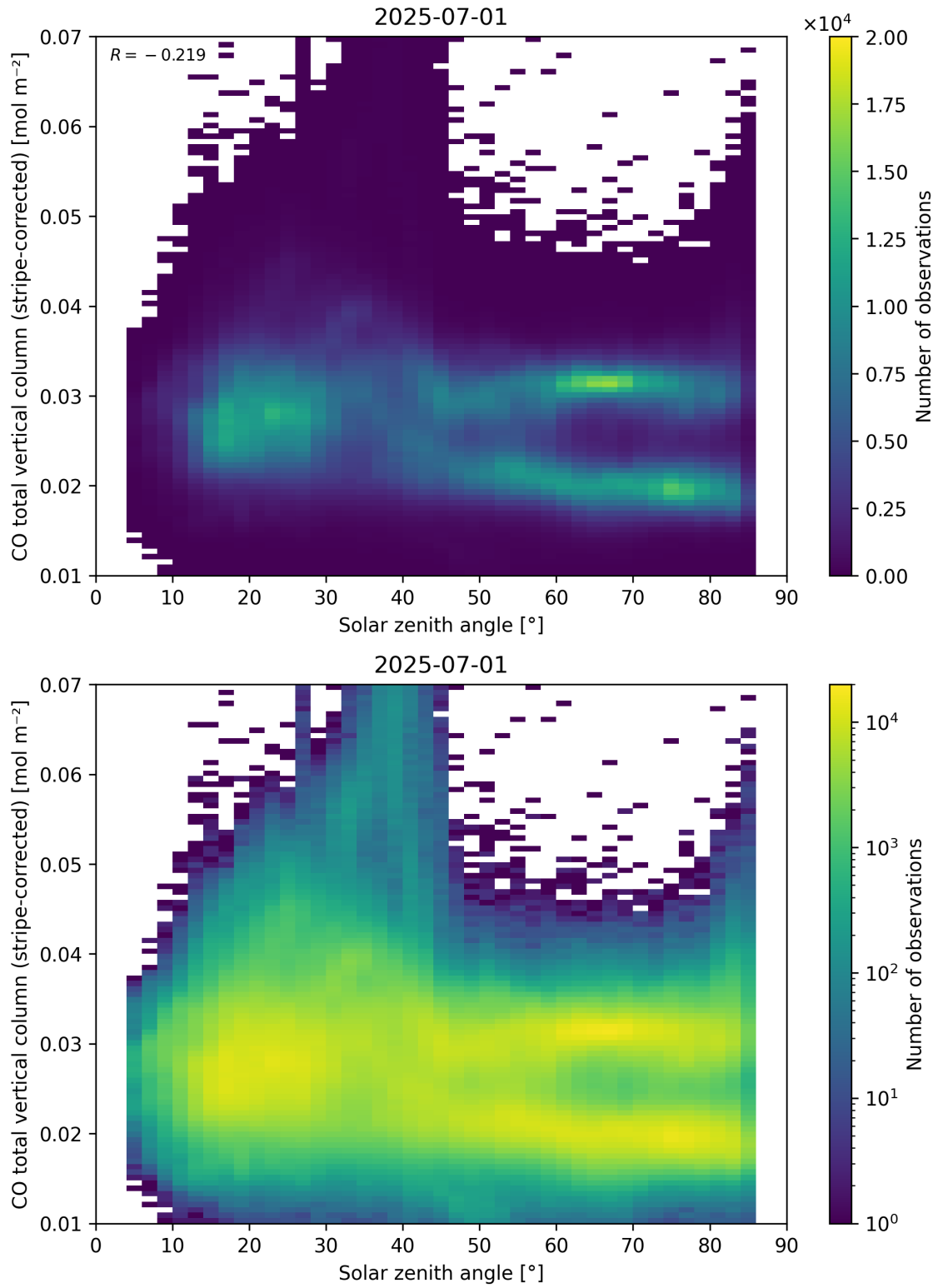
Figure 62: Scatter density plot of “Solar zenith angle” against “CO total vertical column (stripe-corrected)” for 2025-06-30 to 2025-07-02.
