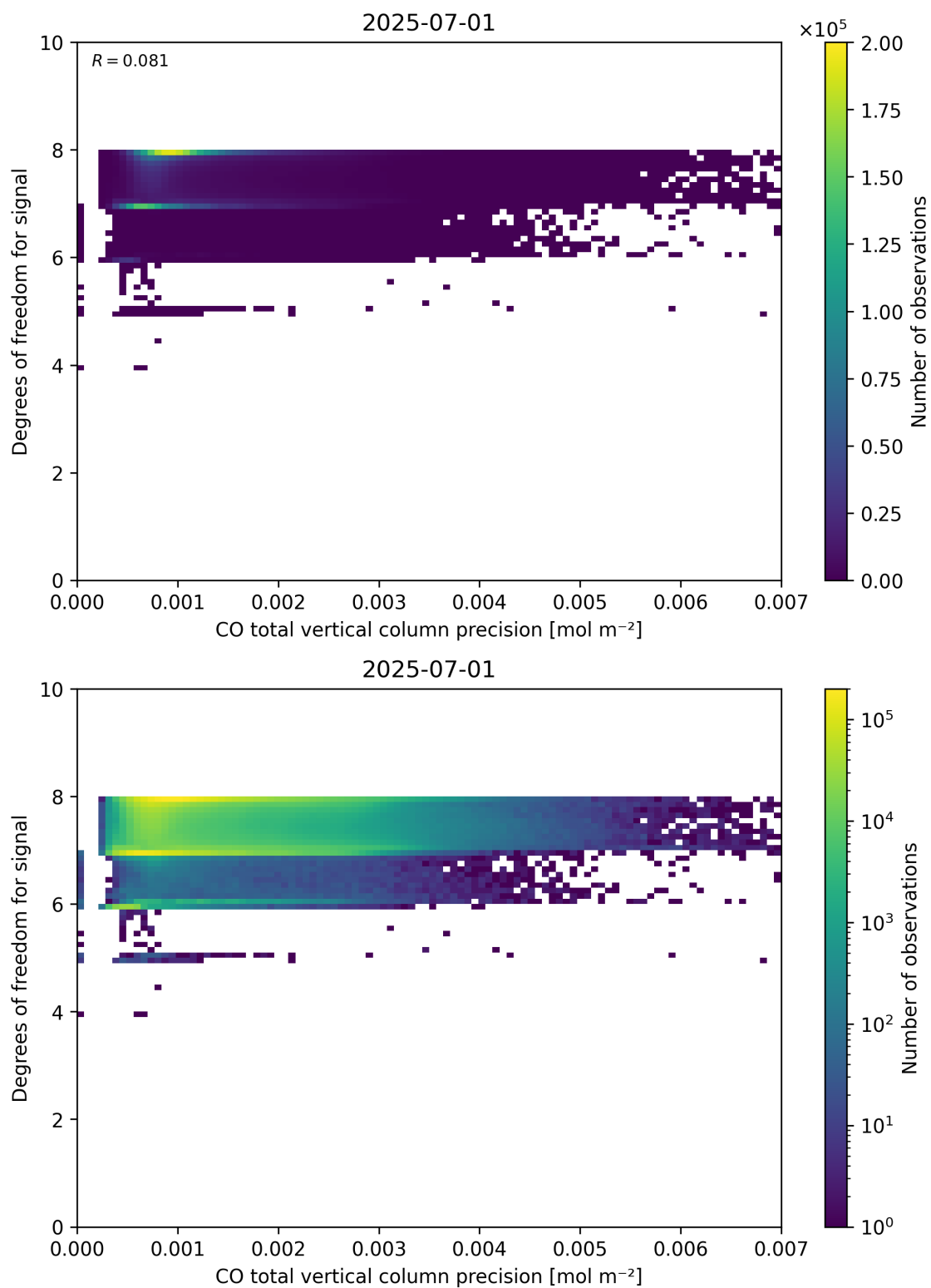
Figure 45: Scatter density plot of “CO total vertical column precision” against “Degrees of freedom for signal” for 2025-06-30 to 2025-07-02.
