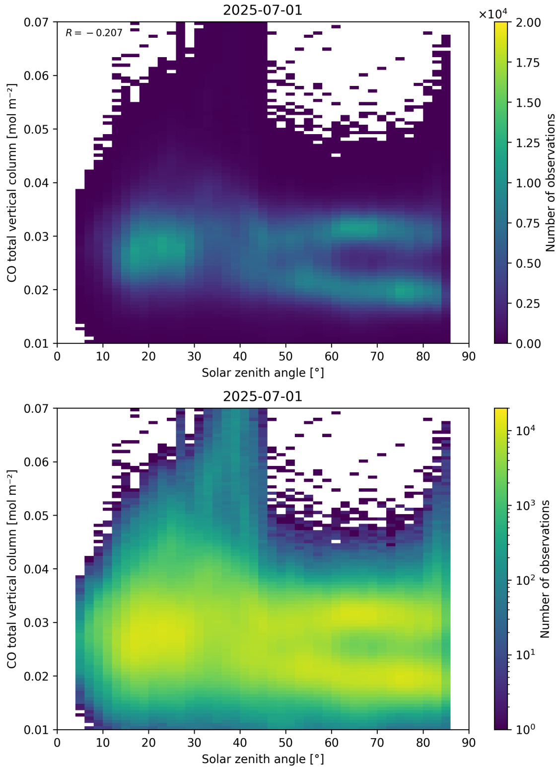
Figure 61: Scatter density plot of “Solar zenith angle” against “CO total vertical column” for 2025-06-30 to 2025-07-02.
