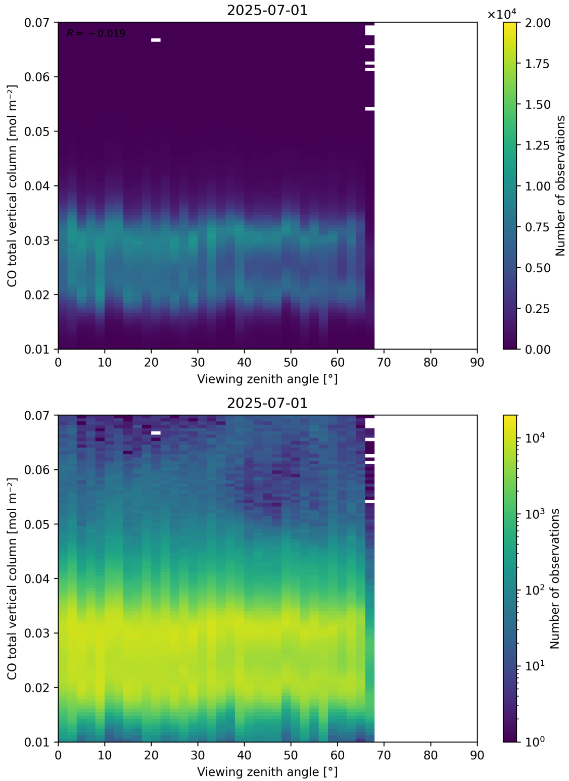
Figure 69: Scatter density plot of “Viewing zenith angle” against “CO total vertical column” for 2025-06-30 to 2025-07-02.
