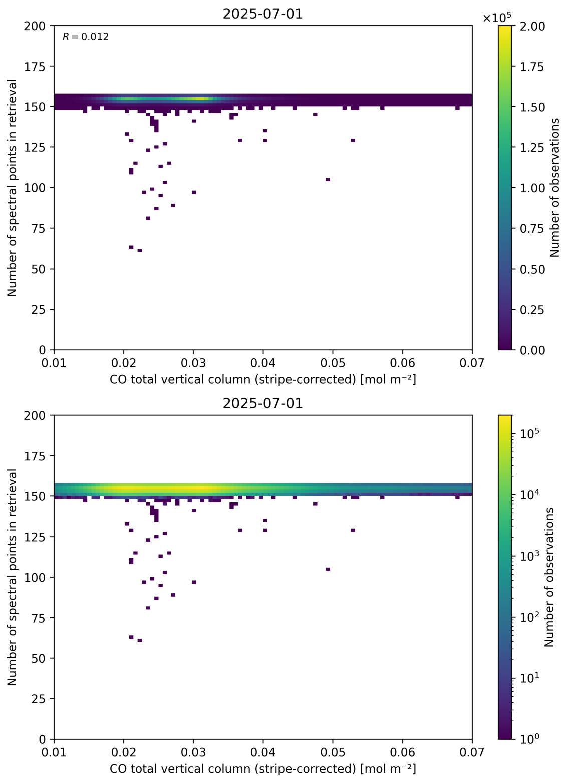
Figure 40: Scatter density plot of “CO total vertical column (stripe-corrected)” against “Number of spectral points in retrieval” for 2025-06-30 to 2025-07-02.
