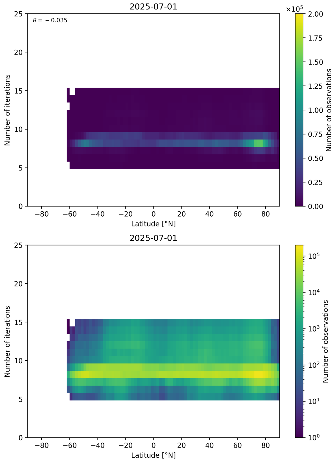
Figure 56: Scatter density plot of “Latitude” against “Number of iterations” for 2025-06-30 to 2025-07-02.
