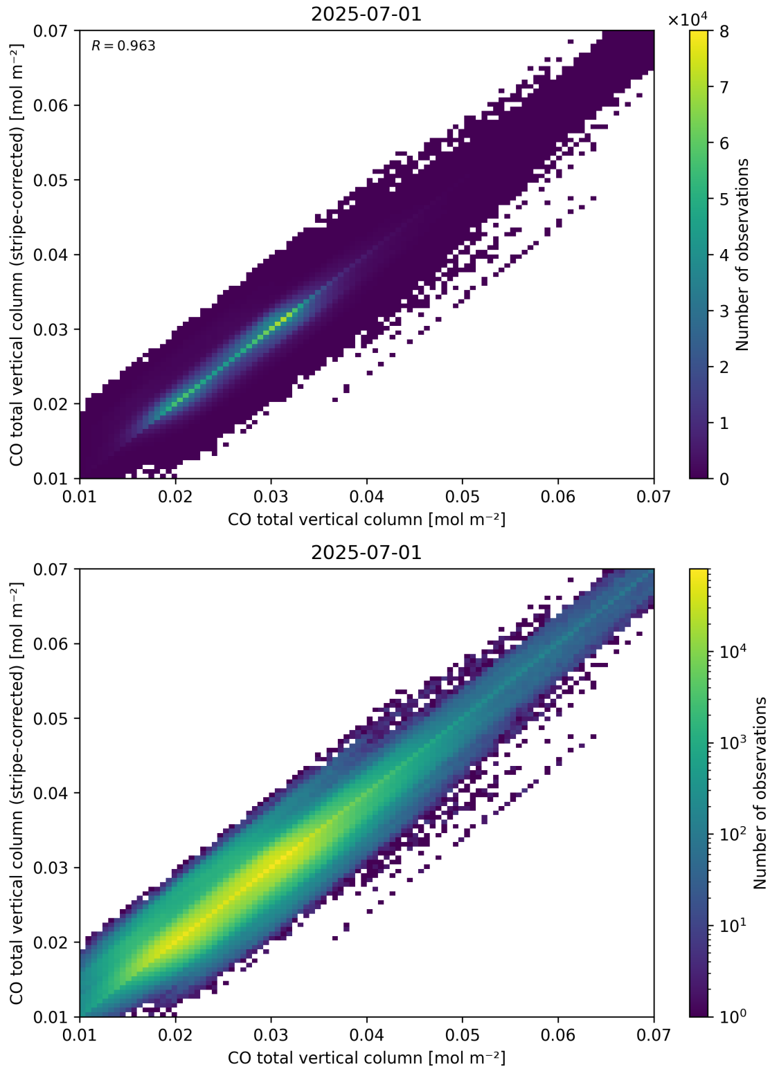
Figure 33: Scatter density plot of “CO total vertical column” against “CO total vertical column (stripe-corrected)” for 2025-06-30 to 2025-07-02.
