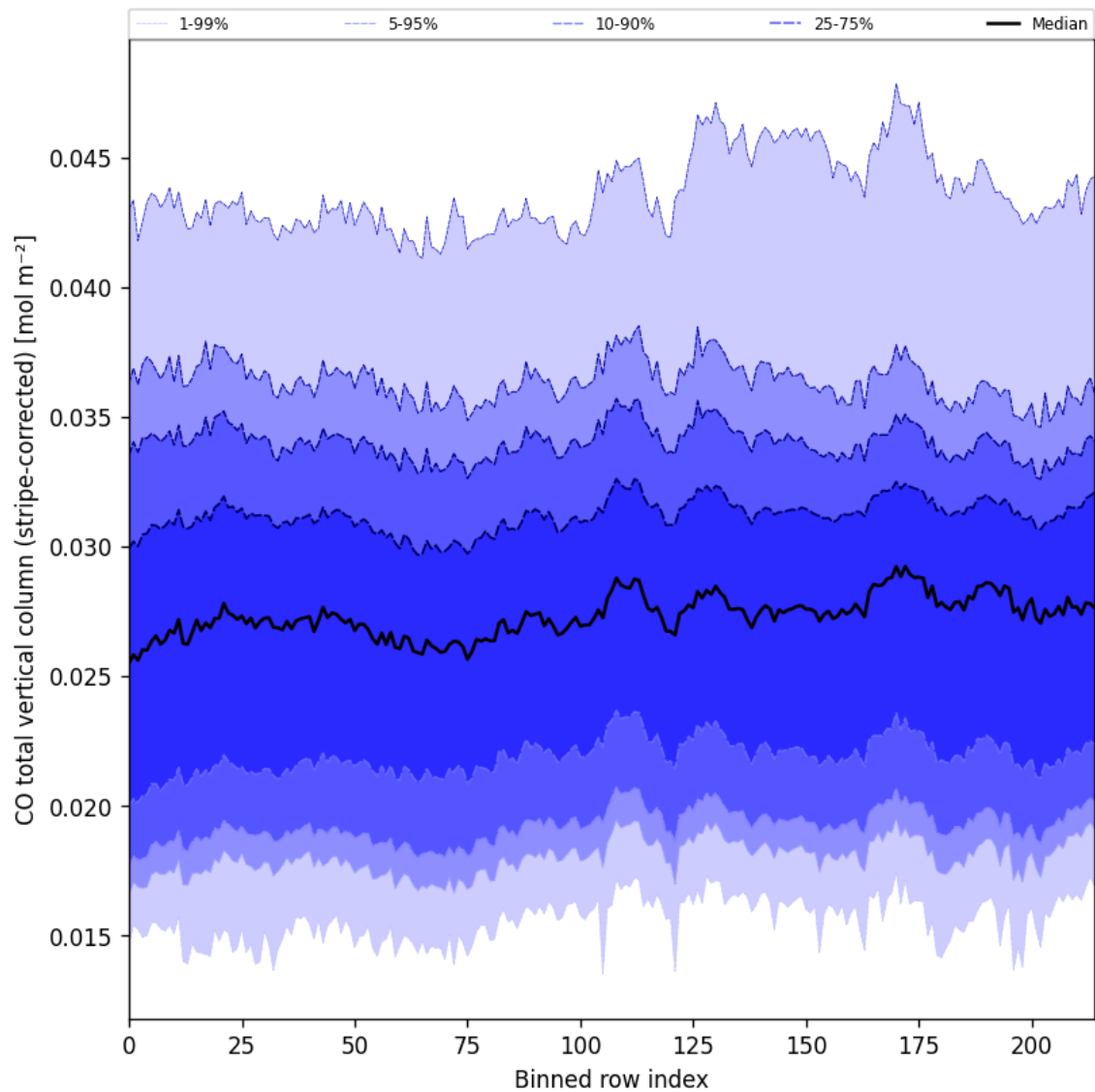
Figure 27: Along track statistics of “CO total vertical column (stripe-corrected)” for 2025-06-30 to 2025-07-02
