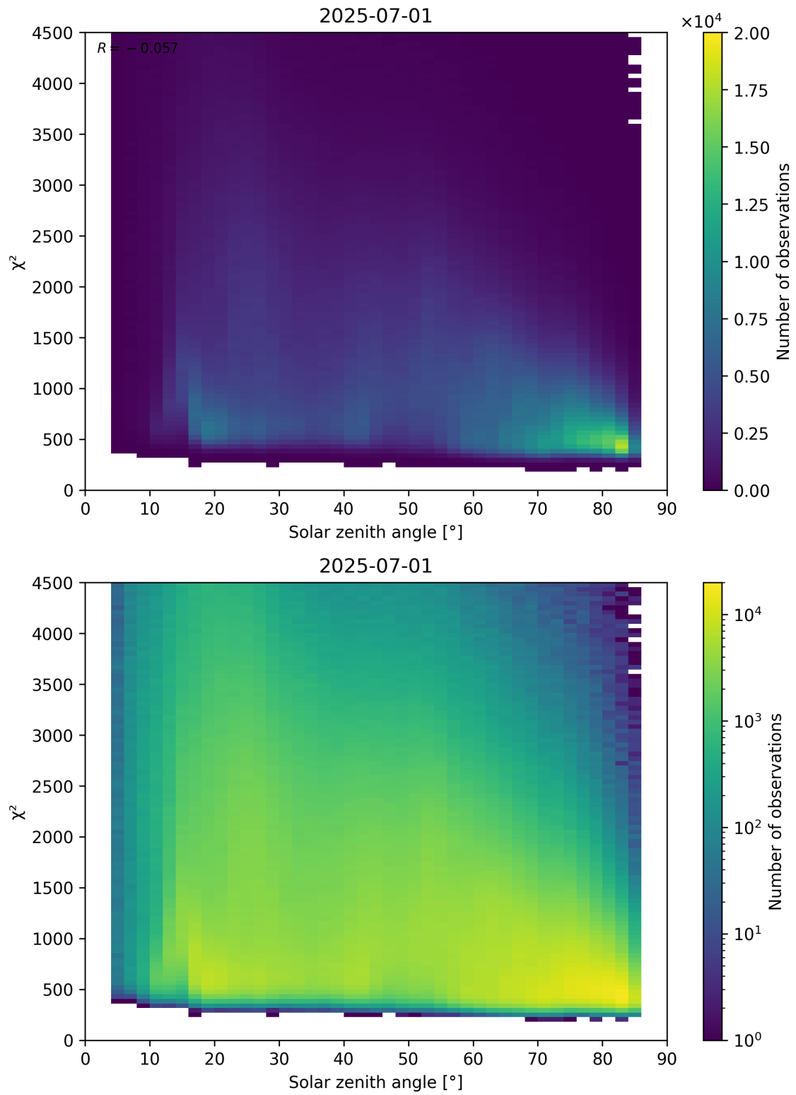
Figure 64: Scatter density plot of “Solar zenith angle” against “ \chi^2 ” for 2025-06-30 to 2025-07-02.
