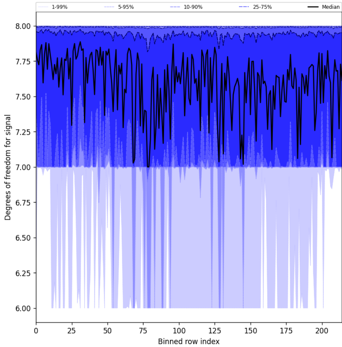
Figure 31: Along track statistics of “Degrees of freedom for signal” for 2025-06-30 to 2025-07-02
