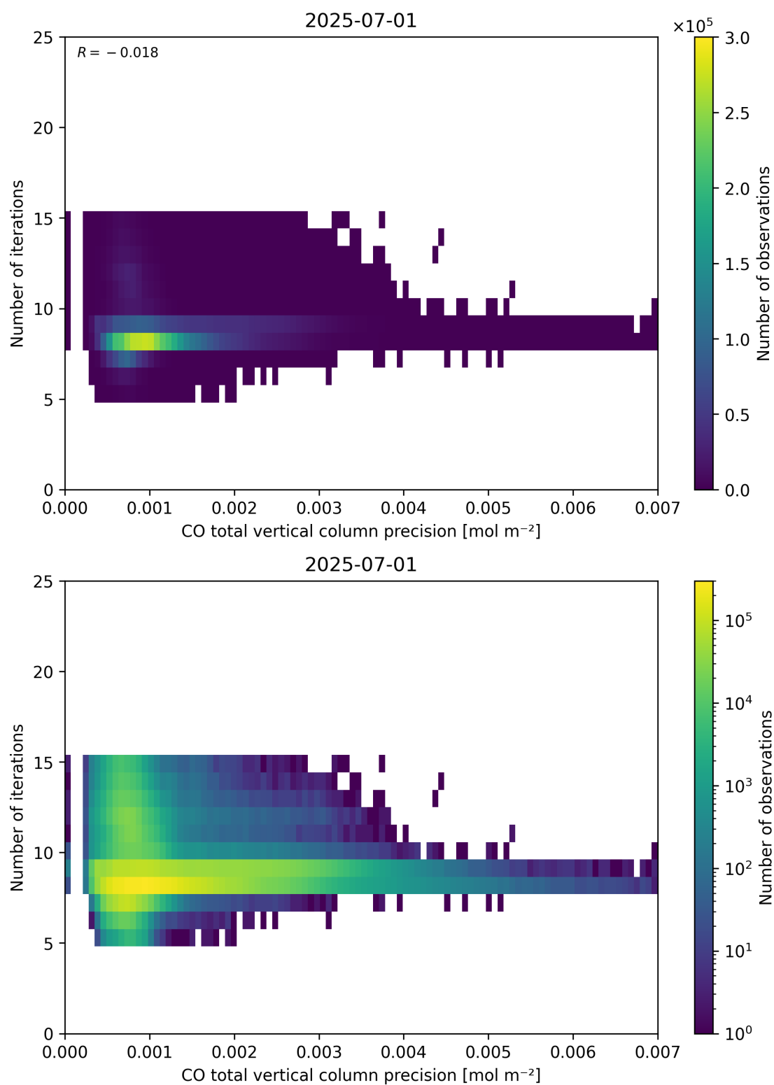
Figure 46: Scatter density plot of “CO total vertical column precision” against “Number of iterations” for 2025-06-30 to 2025-07-02.
