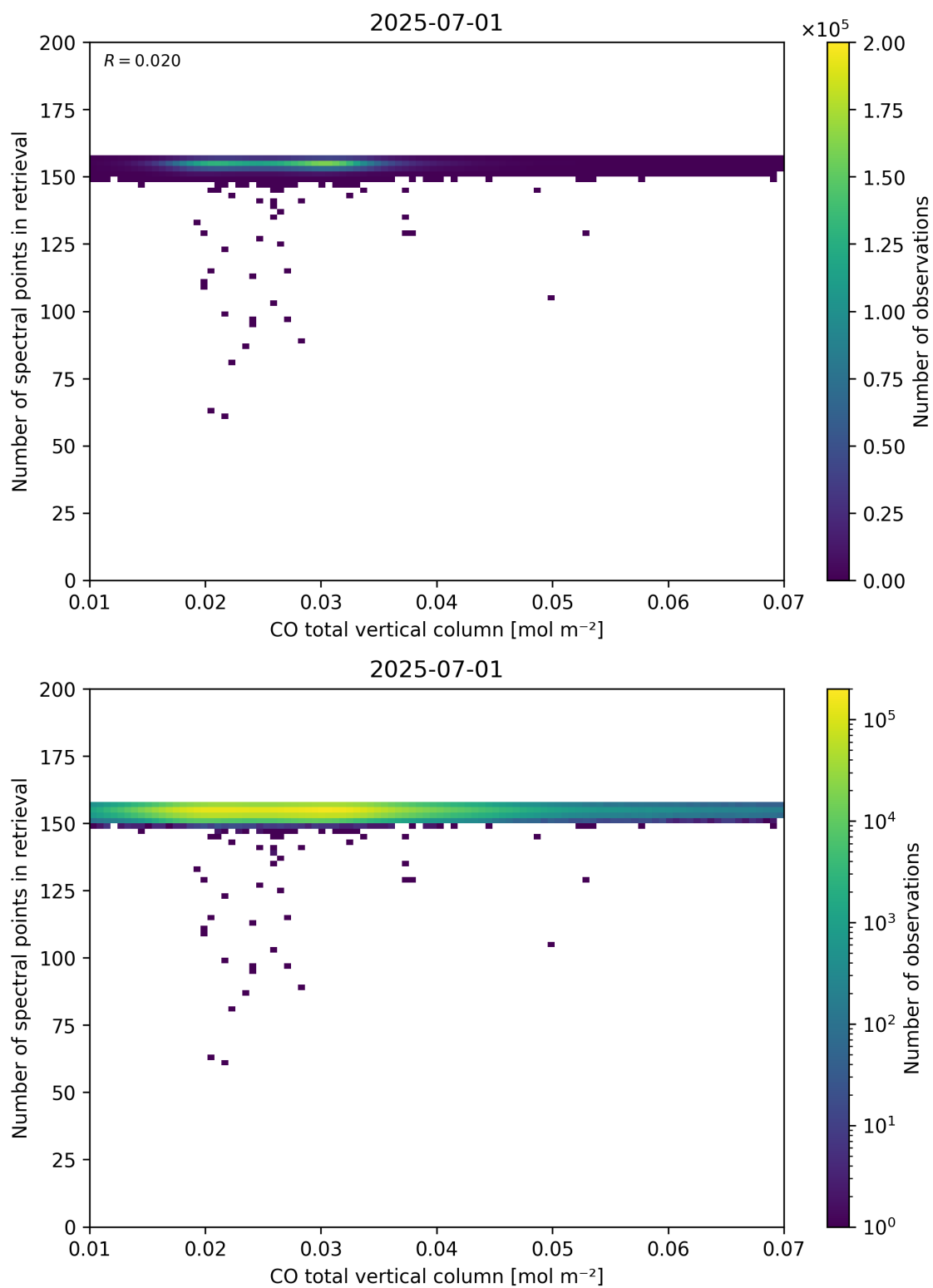
Figure 43: Scatter density plot of “CO total vertical column” against “Number of spectral points in retrieval” for 2025-06-30 to 2025-07-02.
