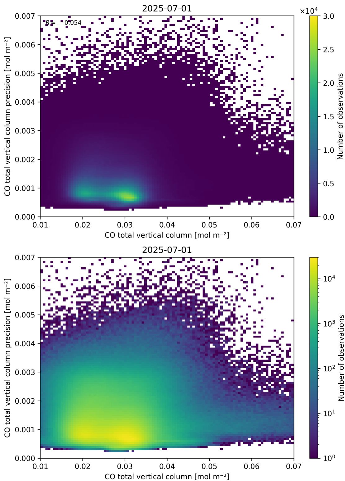
Figure 34: Scatter density plot of “CO total vertical column” against “CO total vertical column precision” for 2025-06-30 to 2025-07-02.
