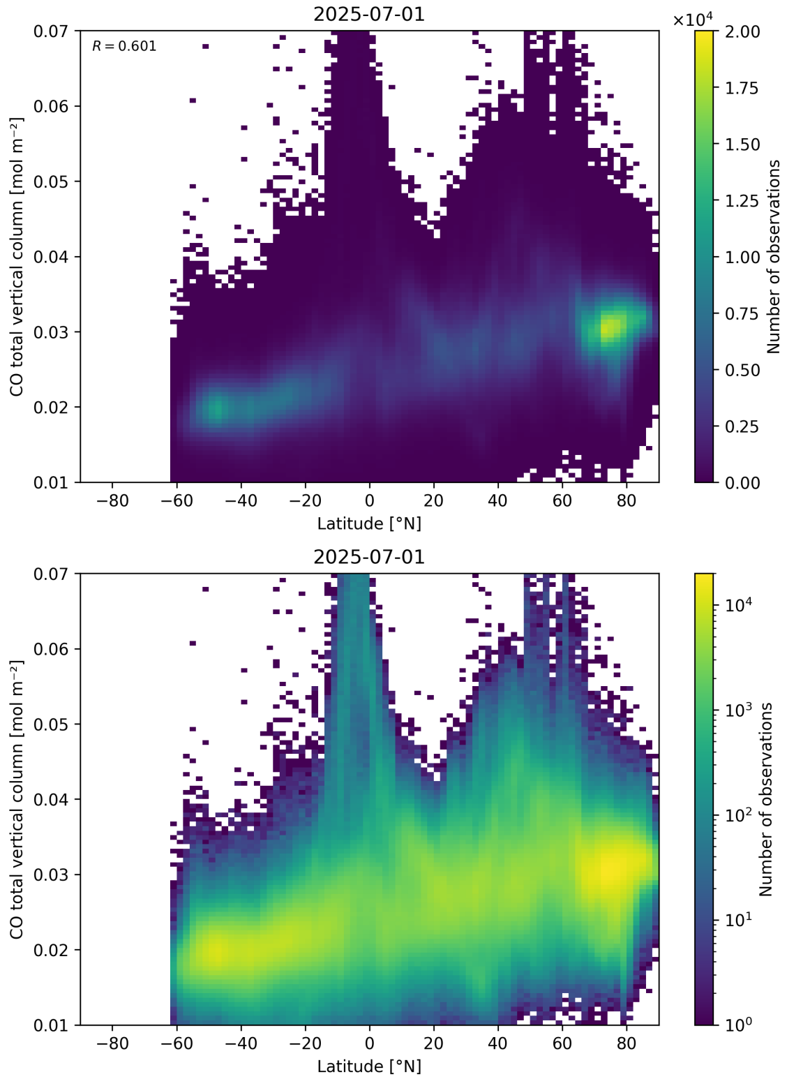
Figure 51: Scatter density plot of “Latitude” against “CO total vertical column” for 2025-06-30 to 2025-07-02.
