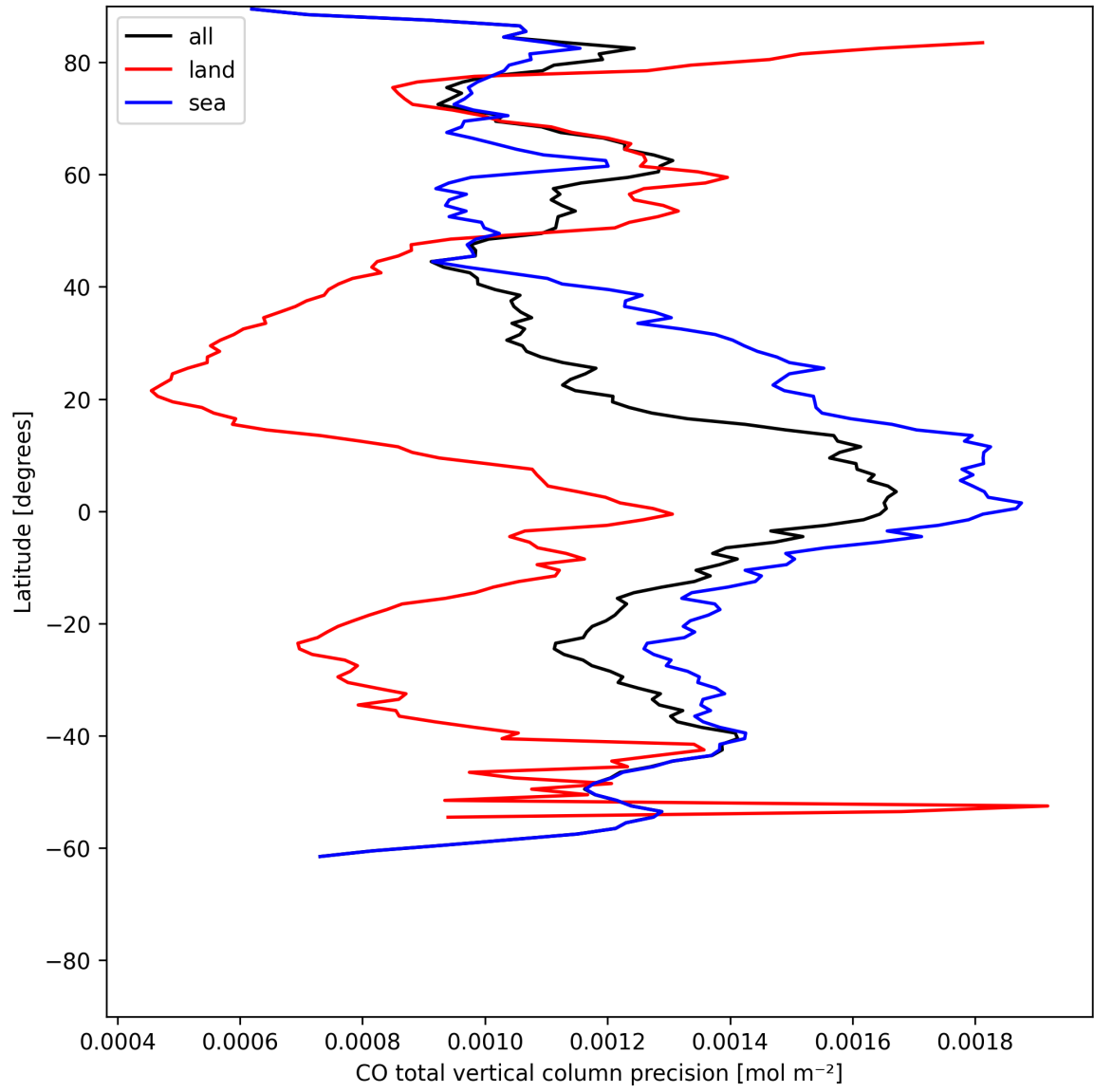
Figure 12: Zonal average of “CO total vertical column precision” for 2025-06-30 to 2025-07-02.
