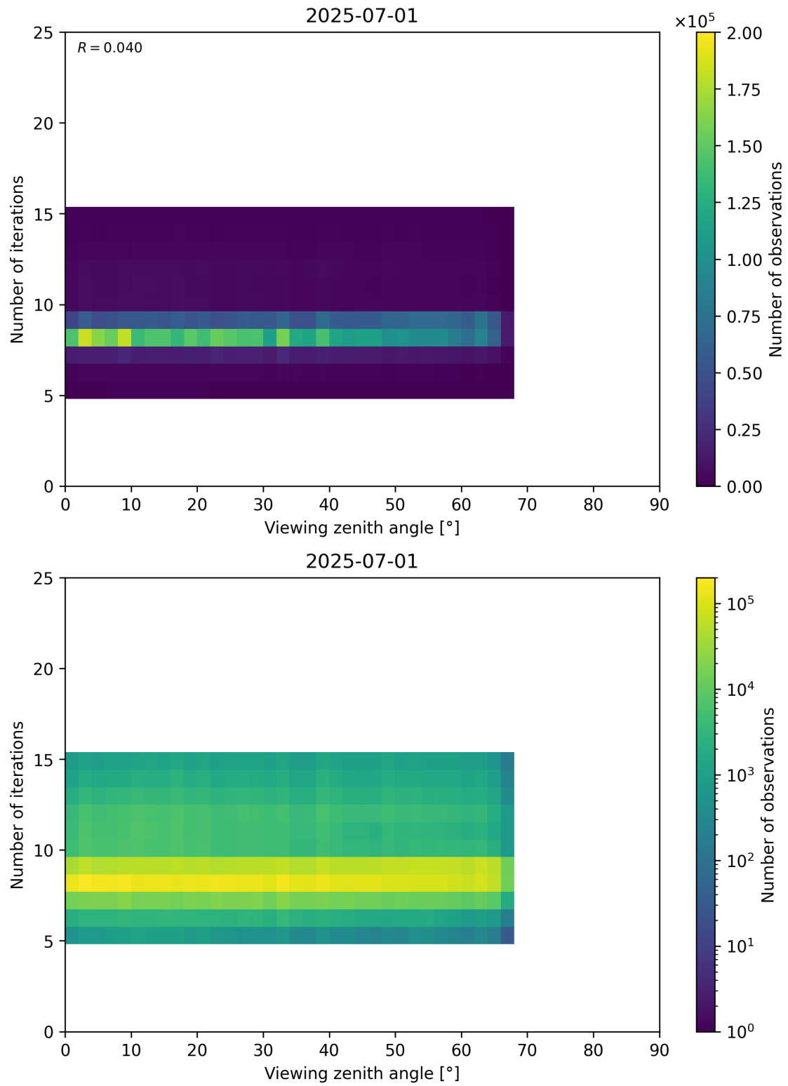
Figure 75: Scatter density plot of “Viewing zenith angle” against “Number of iterations” for 2025-06-30 to 2025-07-02.
