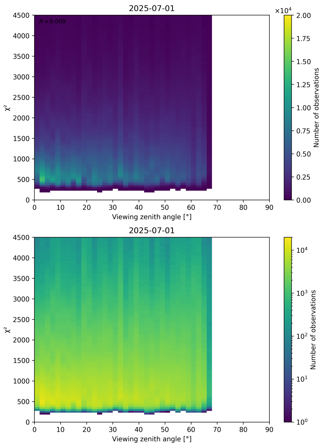
Figure 72: Scatter density plot of “Viewing zenith angle” against “ \chi^2 ” for 2025-06-30 to 2025-07-02.
