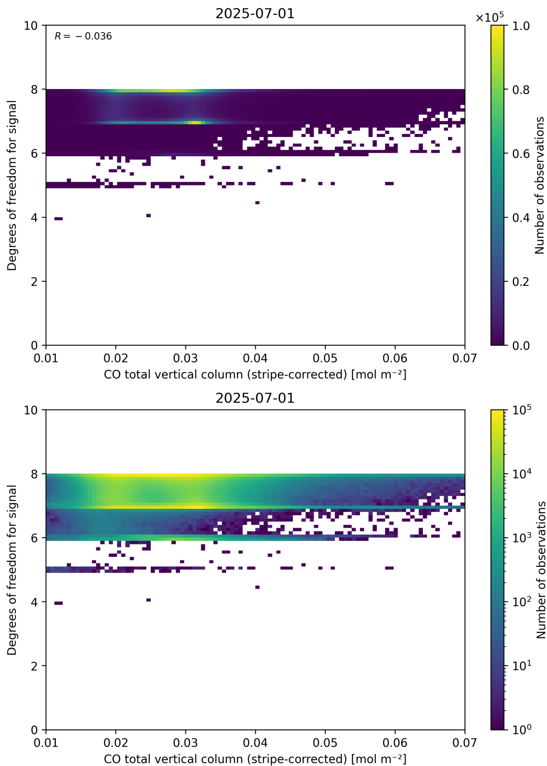
Figure 38: Scatter density plot of “CO total vertical column (stripe-corrected)” against “Degrees of freedom for signal” for 2025-06-30 to 2025-07-02.
