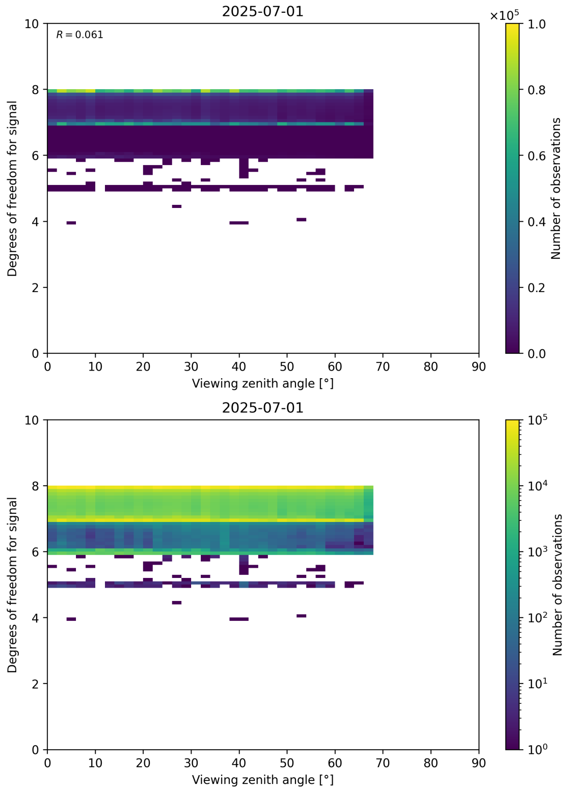
Figure 73: Scatter density plot of “Viewing zenith angle” against “Degrees of freedom for signal” for 2025-06-30 to 2025-07-02.
