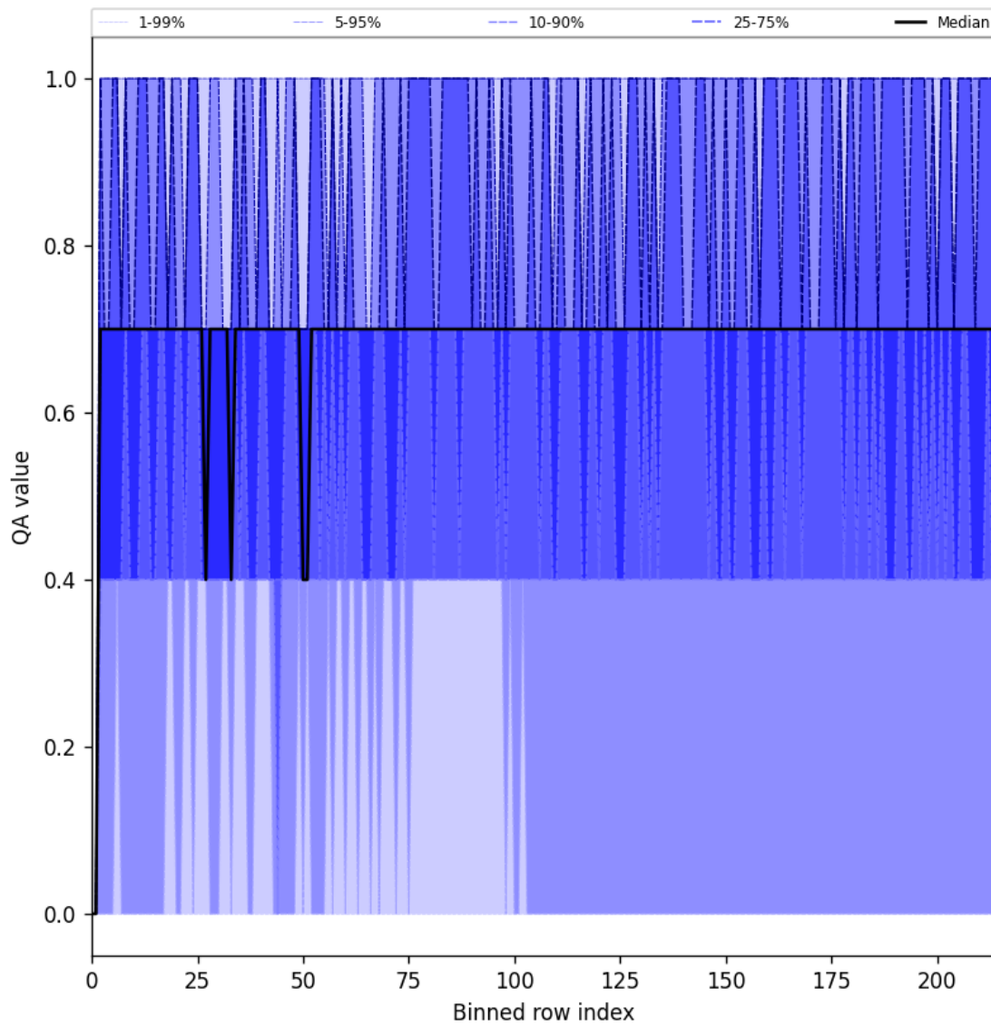
Figure 25: Along track statistics of “QA value” for 2025-06-30 to 2025-07-02
