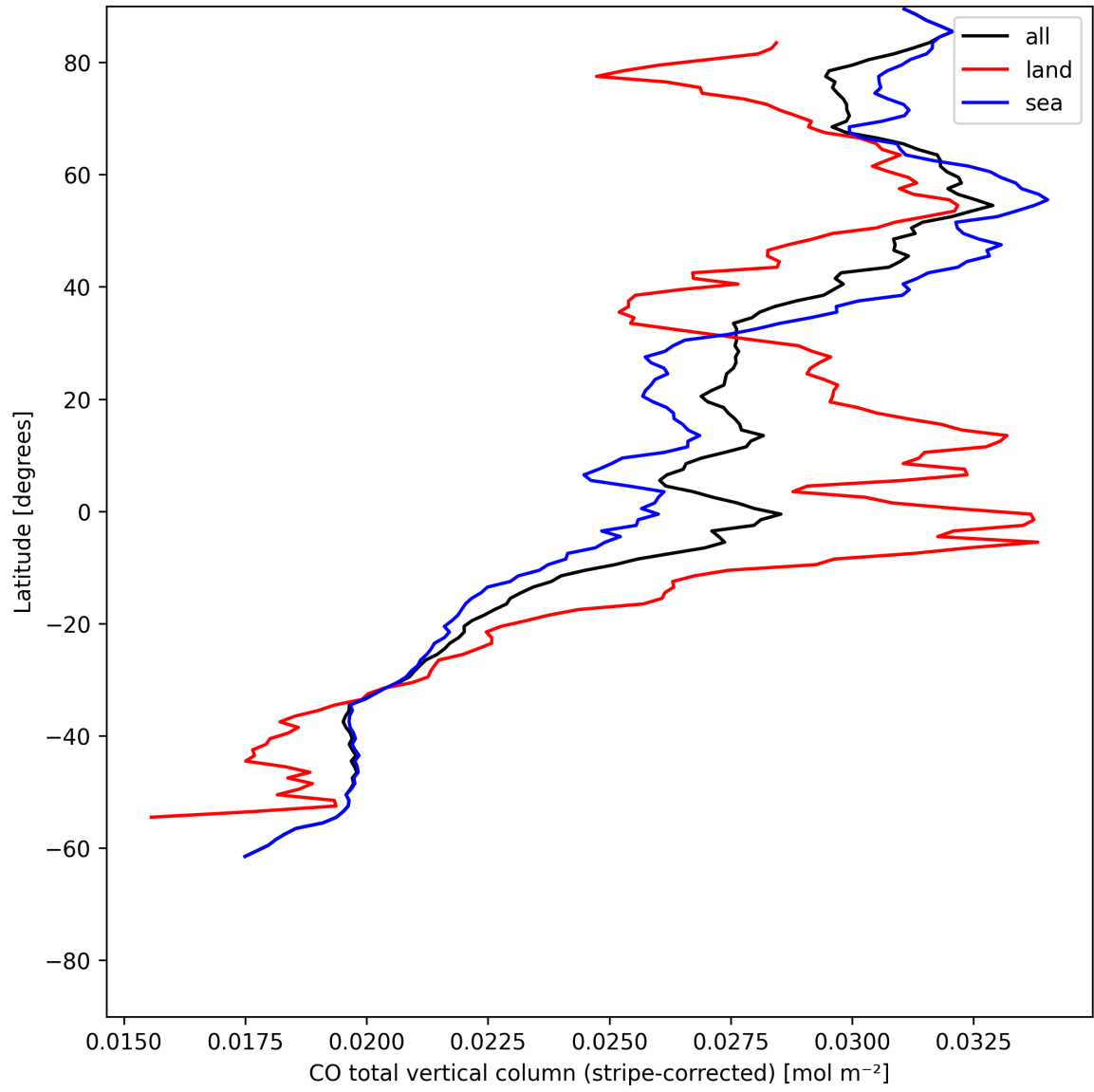
Figure 11: Zonal average of “CO total vertical column (stripe-corrected)” for 2025-06-30 to 2025-07-02.
