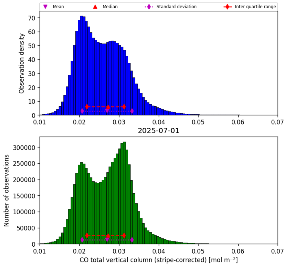
Figure 19: Histogram of “CO total vertical column (stripe-corrected)” for 2025-06-30 to 2025-07-02
