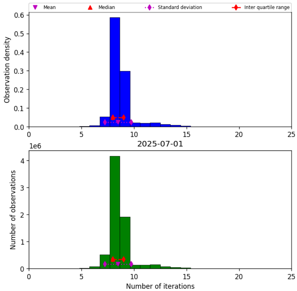
Figure 24: Histogram of “Number of iterations” for 2025-06-30 to 2025-07-02
