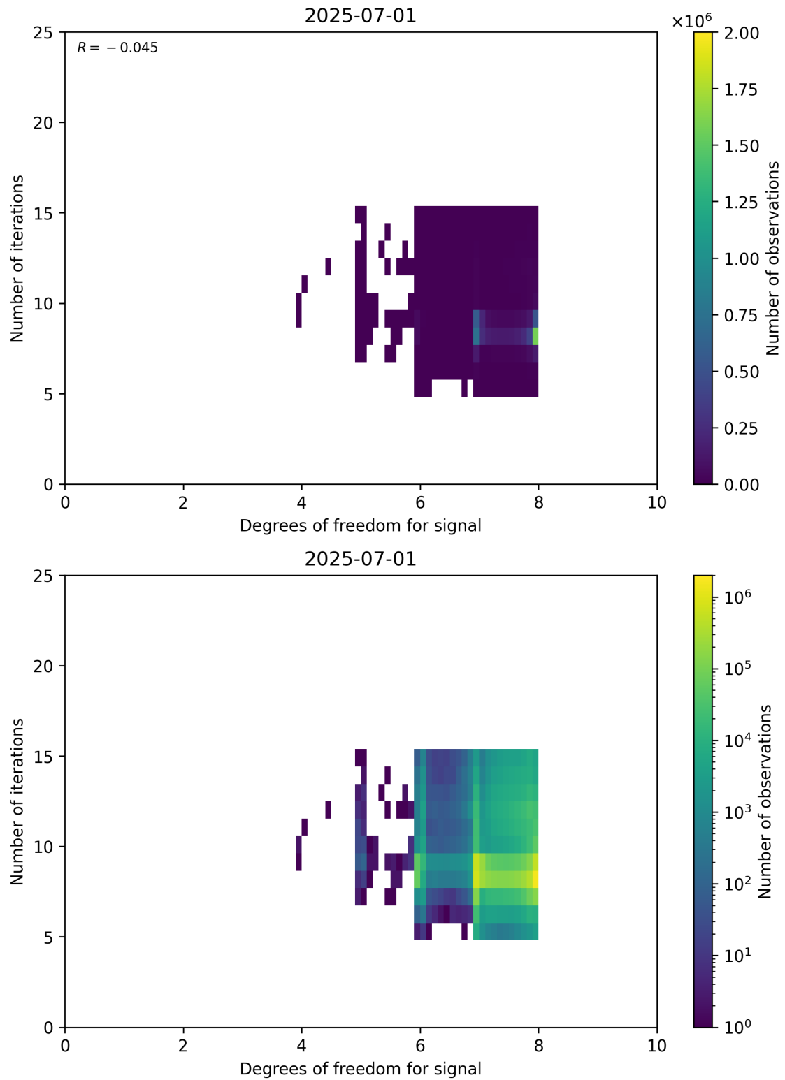
Figure 50: Scatter density plot of “Degrees of freedom for signal” against “Number of iterations” for 2025-06-30 to 2025-07-02.
