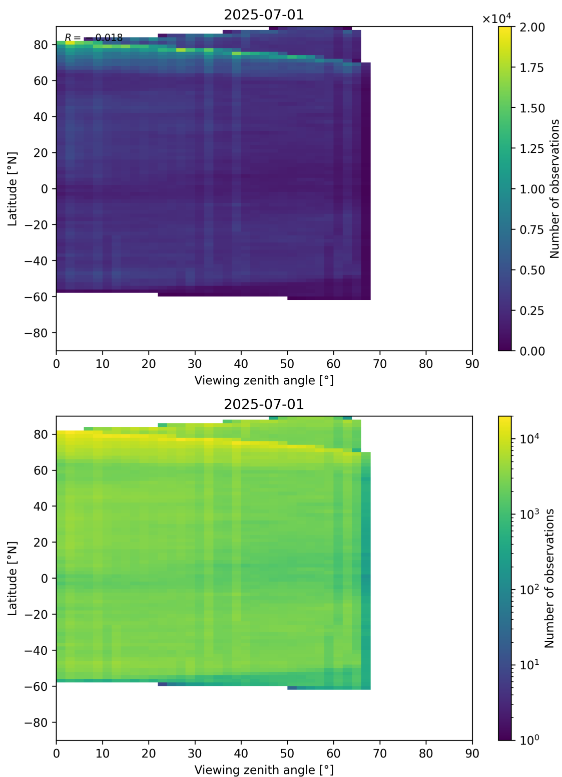
Figure 74: Scatter density plot of “Viewing zenith angle” against “Latitude” for 2025-06-30 to 2025-07-02.
