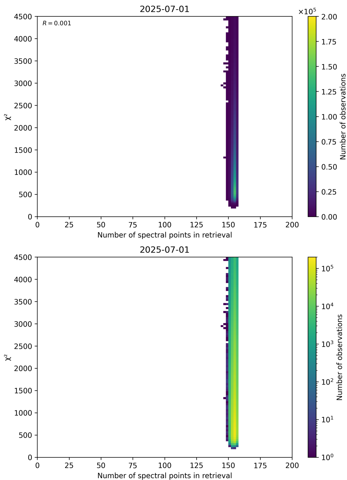
Figure 58: Scatter density plot of “Number of spectral points in retrieval” against “ \chi^2 ” for 2025-06-30 to 2025-07-02.
