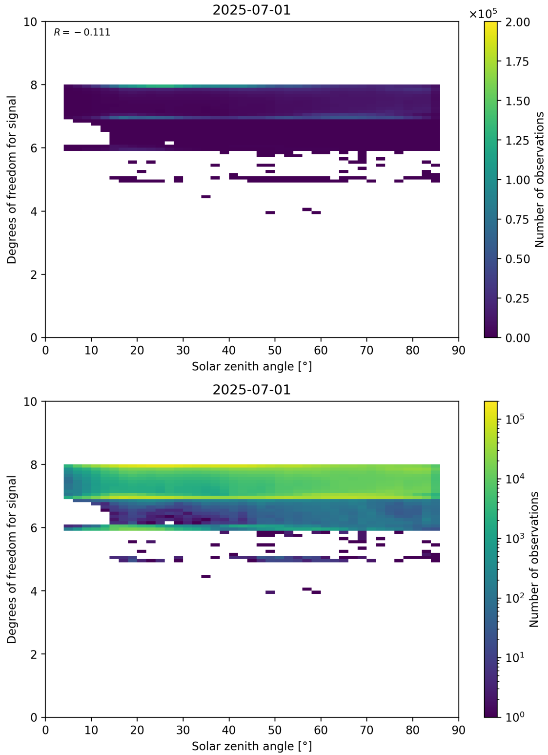
Figure 65: Scatter density plot of “Solar zenith angle” against “Degrees of freedom for signal” for 2025-06-30 to 2025-07-02.
