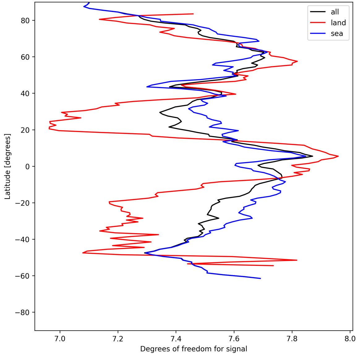
Figure 15: Zonal average of “Degrees of freedom for signal” for 2025-06-30 to 2025-07-02.
