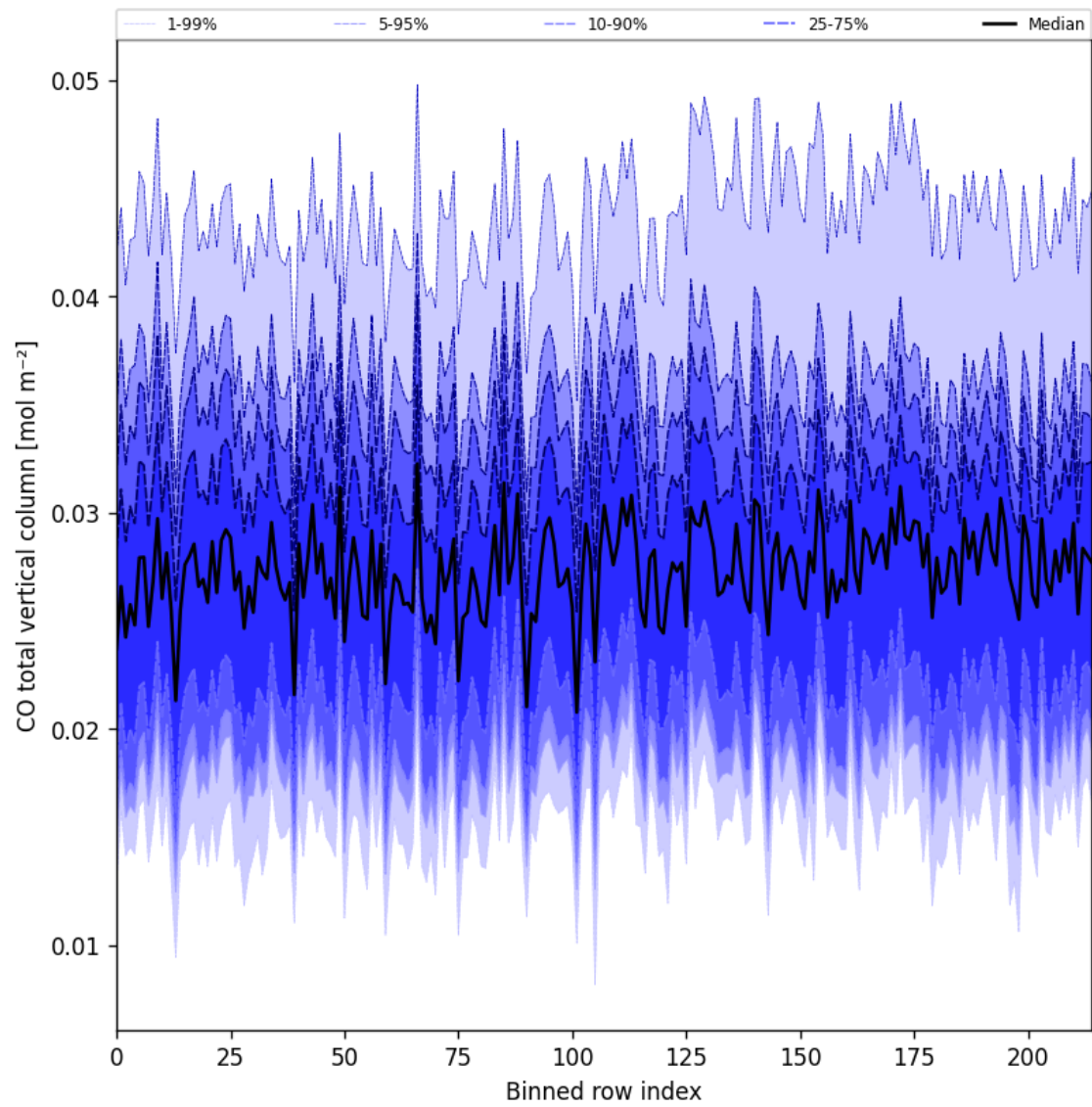
Figure 26: Along track statistics of “CO total vertical column” for 2025-06-30 to 2025-07-02
