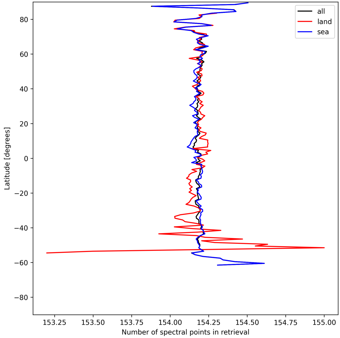
Figure 13: Zonal average of “Number of spectral points in retrieval” for 2025-06-30 to 2025-07-02.
