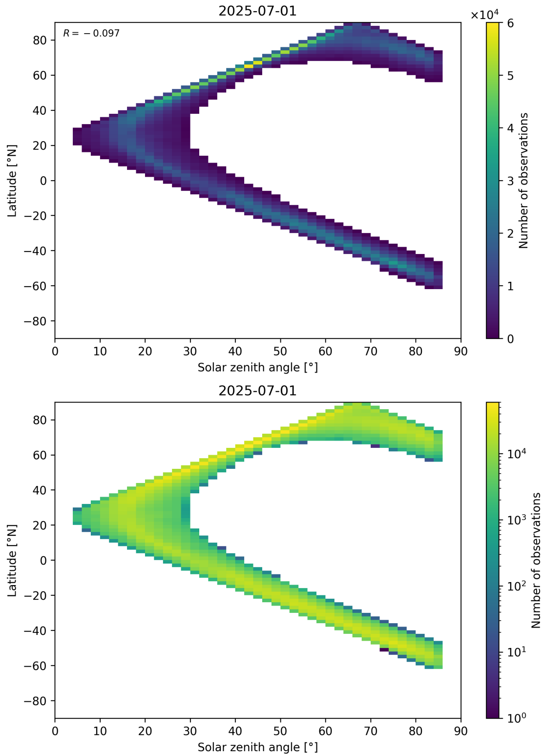
Figure 66: Scatter density plot of “Solar zenith angle” against “Latitude” for 2025-06-30 to 2025-07-02.
