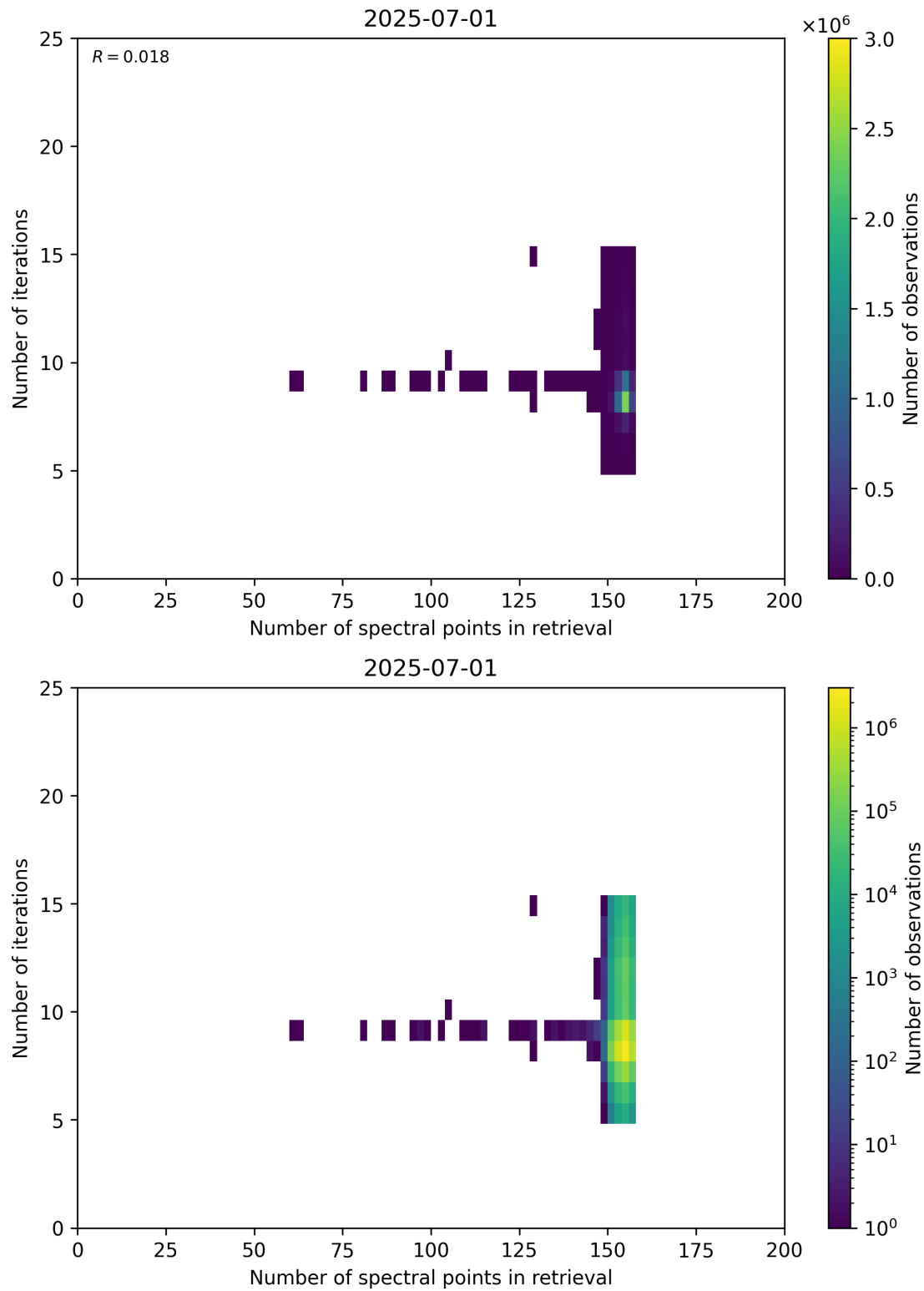
Figure 60: Scatter density plot of “Number of spectral points in retrieval” against “Number of iterations” for 2025-06-30 to 2025-07-02.
