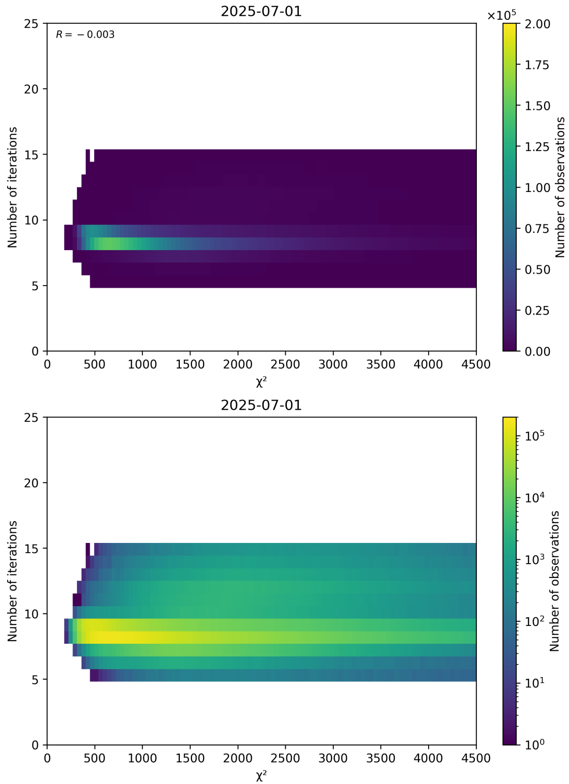
Figure 49: Scatter density plot of “ \chi^2 ” against “Number of iterations” for 2025-06-30 to 2025-07-02.
