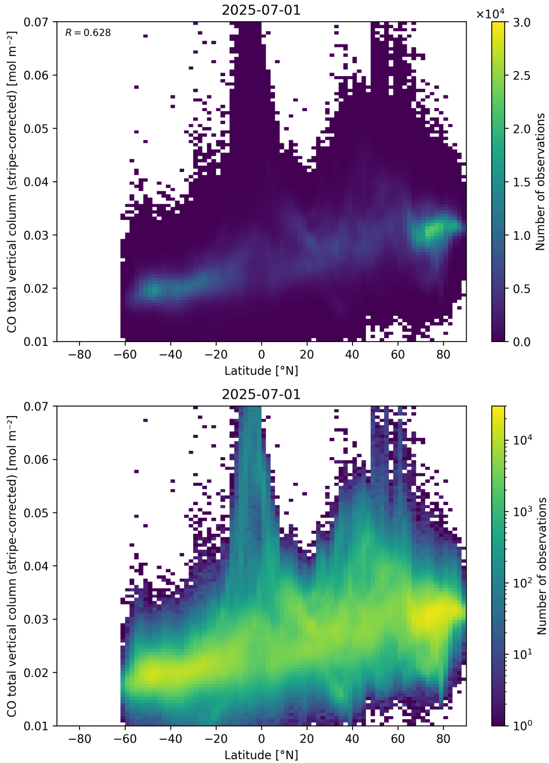
Figure 52: Scatter density plot of “Latitude” against “CO total vertical column (stripe-corrected)” for 2025-06-30 to 2025-07-02.
