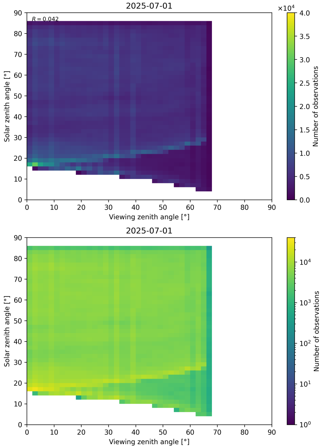
Figure 77: Scatter density plot of “Viewing zenith angle” against “Solar zenith angle” for 2025-06-30 to 2025-07-02.
