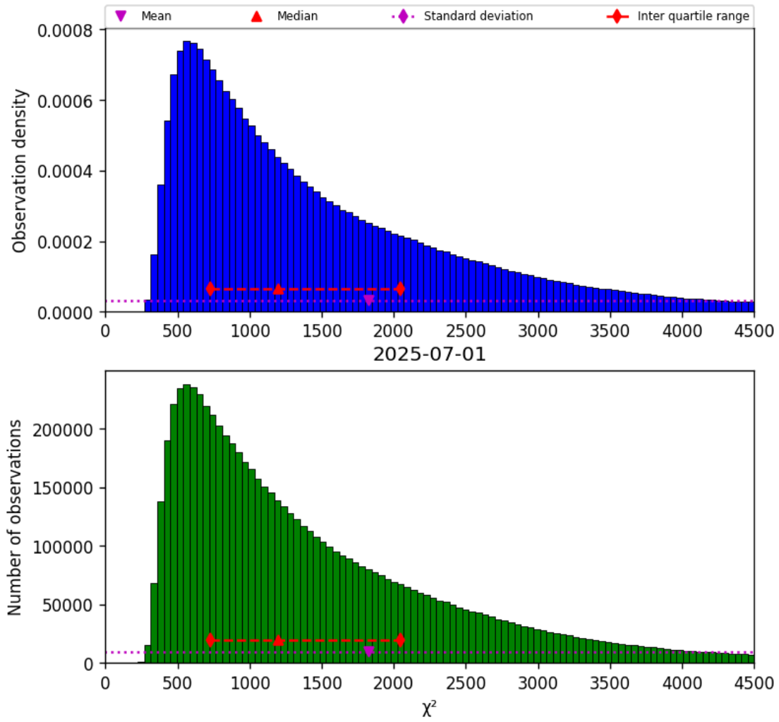
Figure 22: Histogram of “ \chi^2 ” for 2025-06-30 to 2025-07-02
