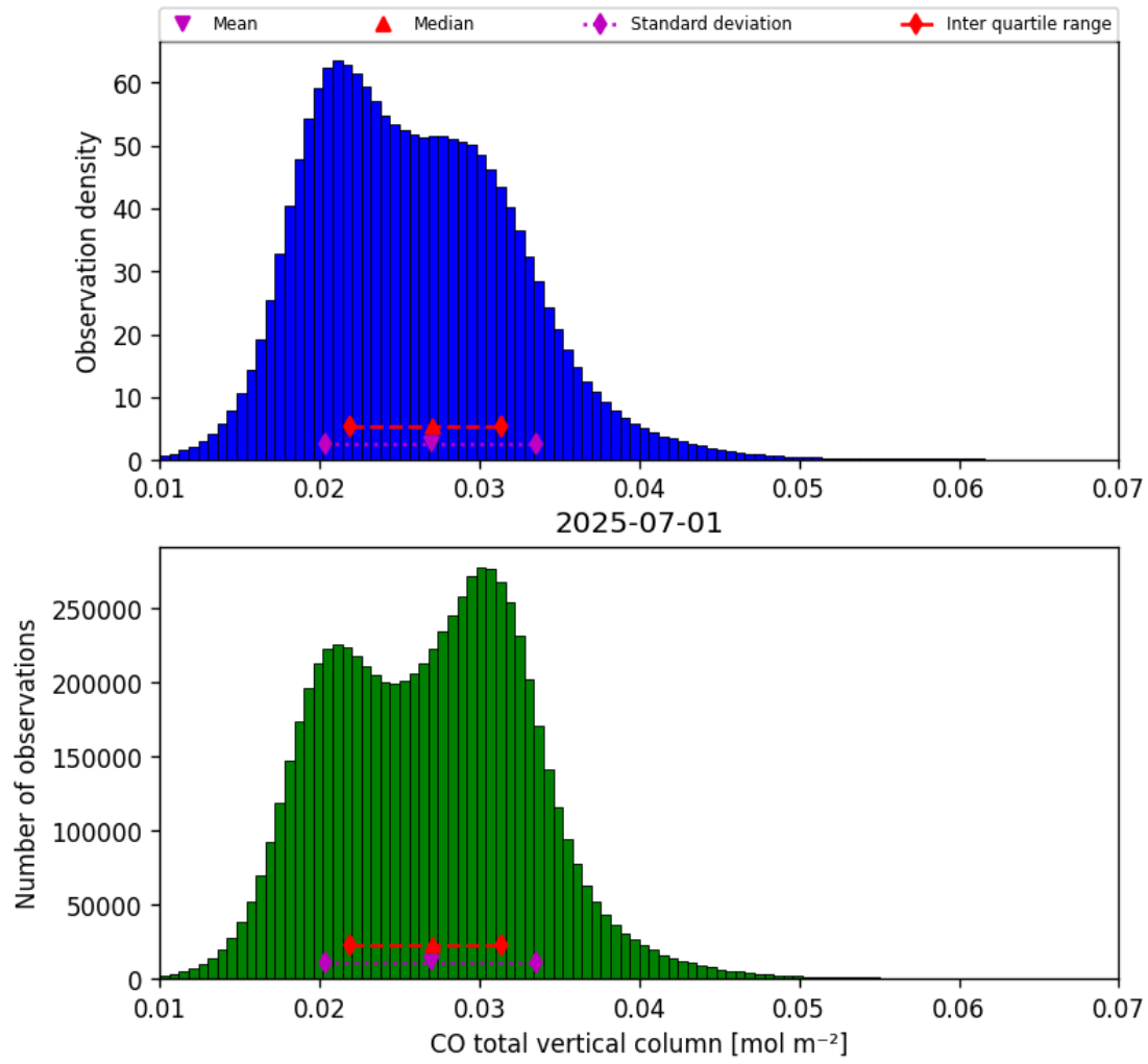
Figure 18: Histogram of “CO total vertical column” for 2025-06-30 to 2025-07-02
