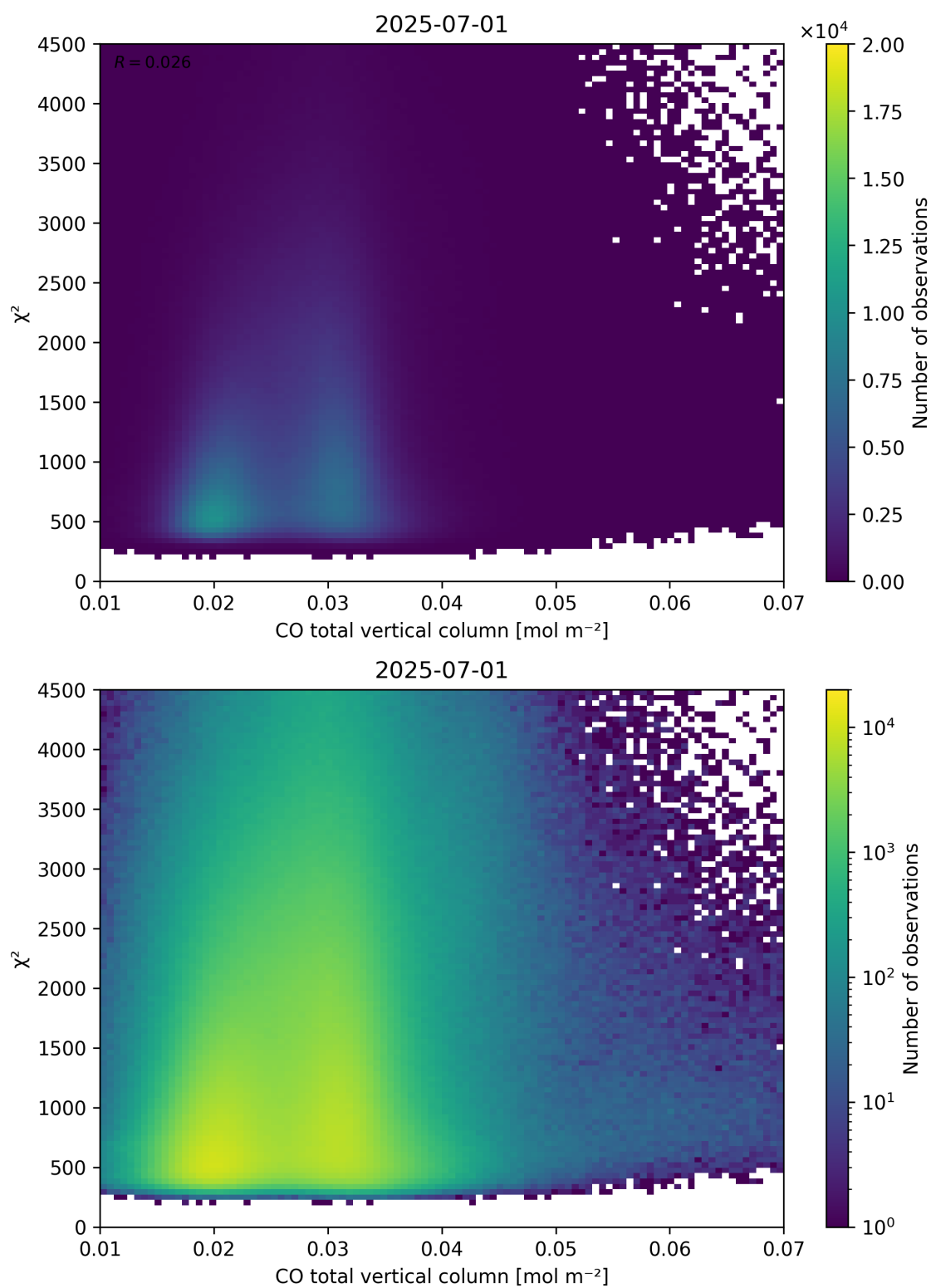
Figure 35: Scatter density plot of “CO total vertical column” against “ \chi^2 ” for 2025-06-30 to 2025-07-02.
