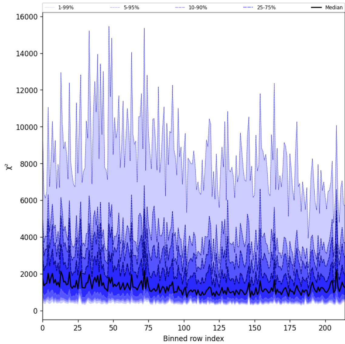
Figure 30: Along track statistics of “ \chi^2 ” for 2025-06-30 to 2025-07-02
