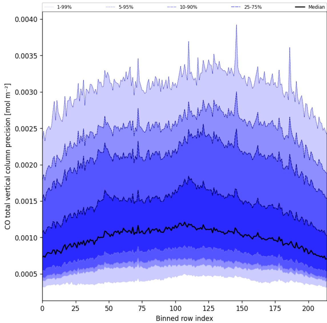
Figure 28: Along track statistics of “CO total vertical column precision” for 2025-06-30 to 2025-07-02
