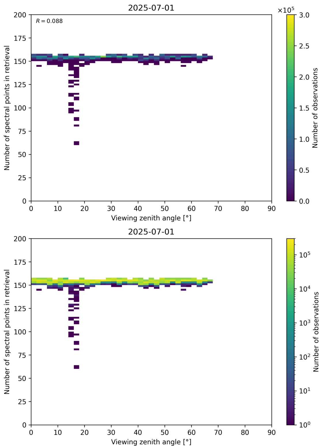
Figure 76: Scatter density plot of “Viewing zenith angle” against “Number of spectral points in retrieval” for 2025-06-30 to 2025-07-02.
