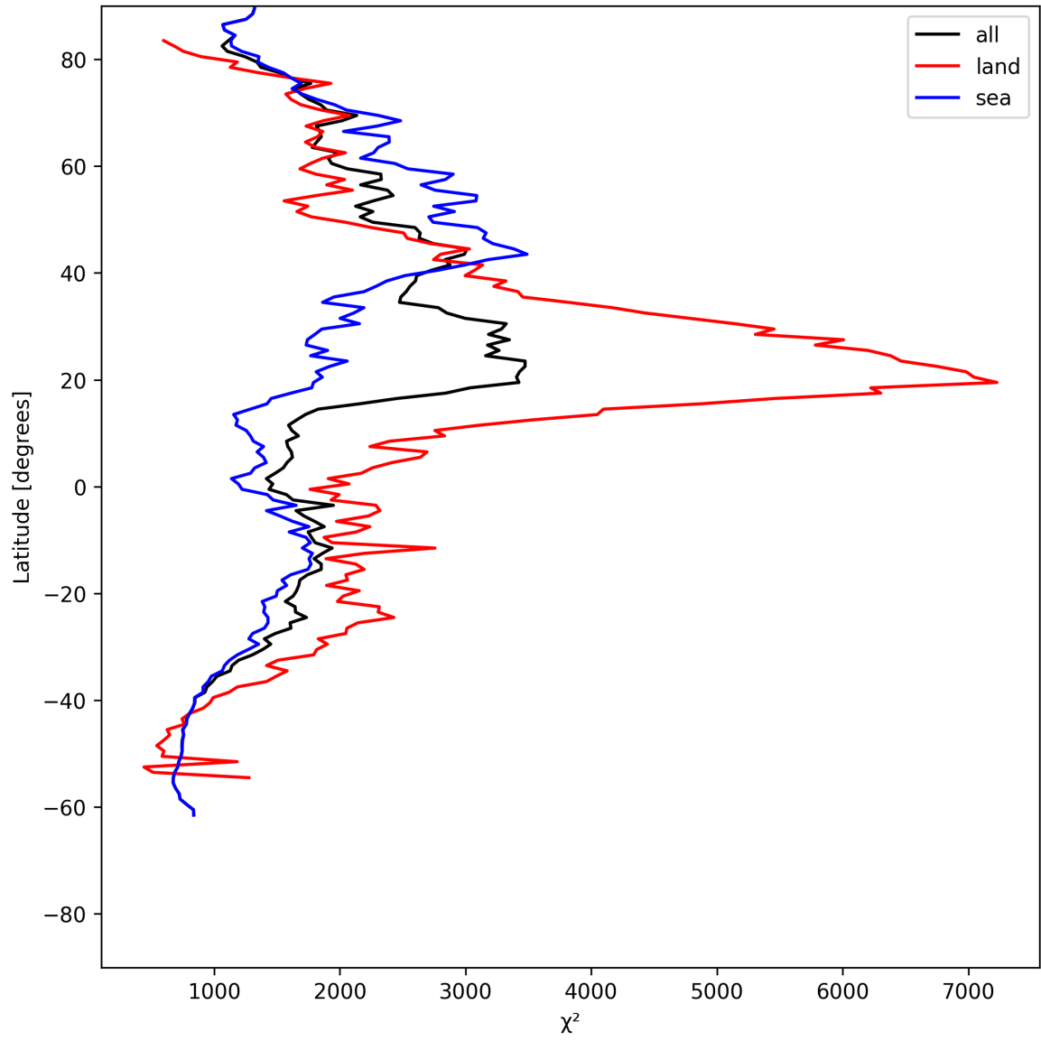
Figure 14: Zonal average of “ \chi^2 ” for 2025-06-30 to 2025-07-02.
