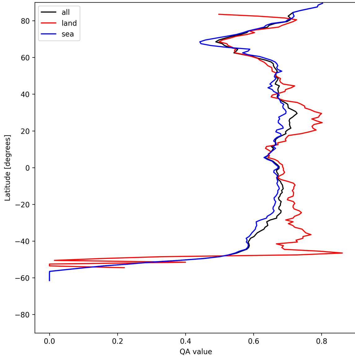
Figure 9: Zonal average of “QA value” for 2025-06-30 to 2025-07-02.
