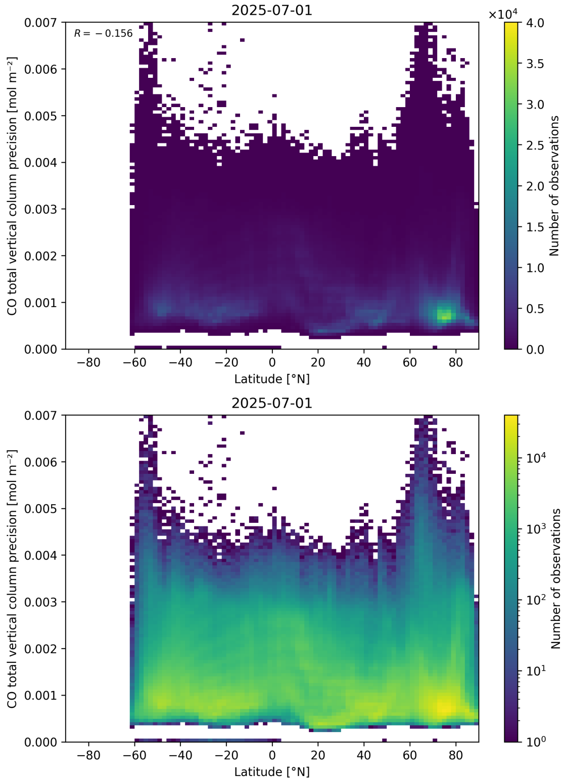
Figure 53: Scatter density plot of “Latitude” against “CO total vertical column precision” for 2025-06-30 to 2025-07-02.
