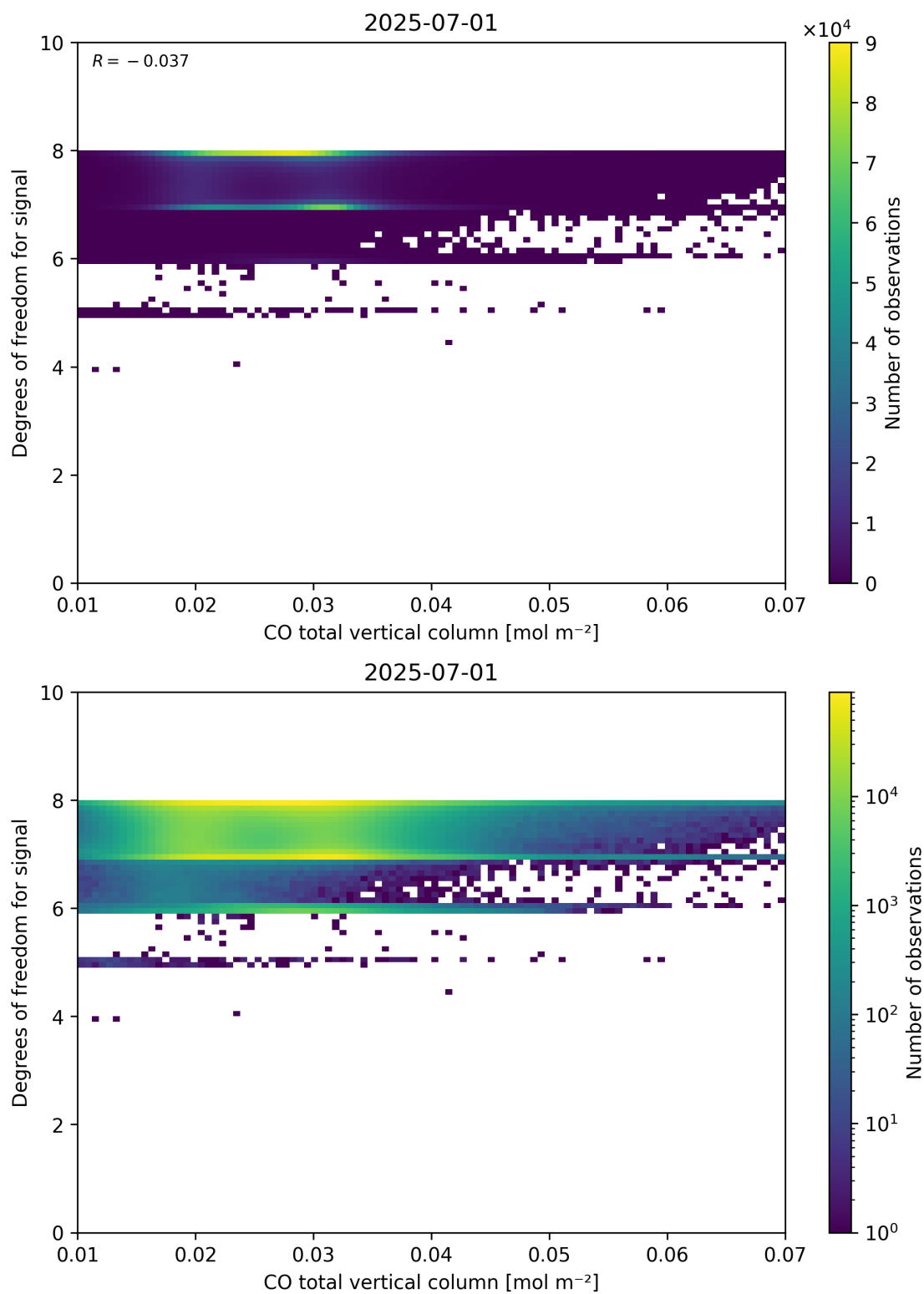
Figure 41: Scatter density plot of “CO total vertical column” against “Degrees of freedom for signal” for 2025-06-30 to 2025-07-02.
