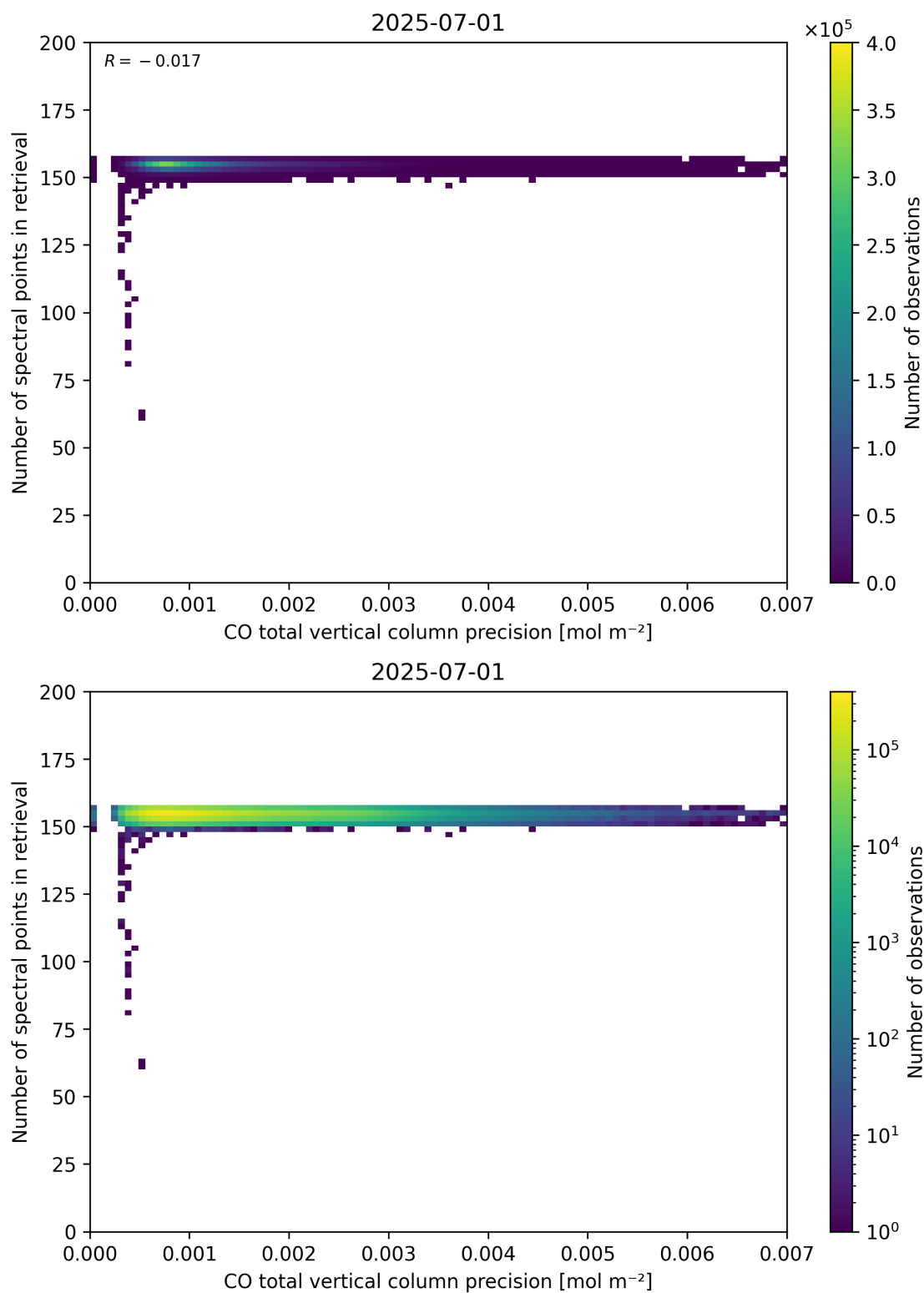
Figure 47: Scatter density plot of “CO total vertical column precision” against “Number of spectral points in retrieval” for 2025-06-30 to 2025-07-02.
