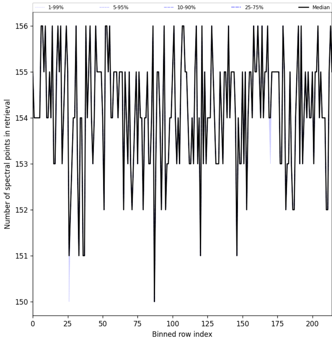
Figure 29: Along track statistics of “Number of spectral points in retrieval” for 2025-06-30 to 2025-07-02
