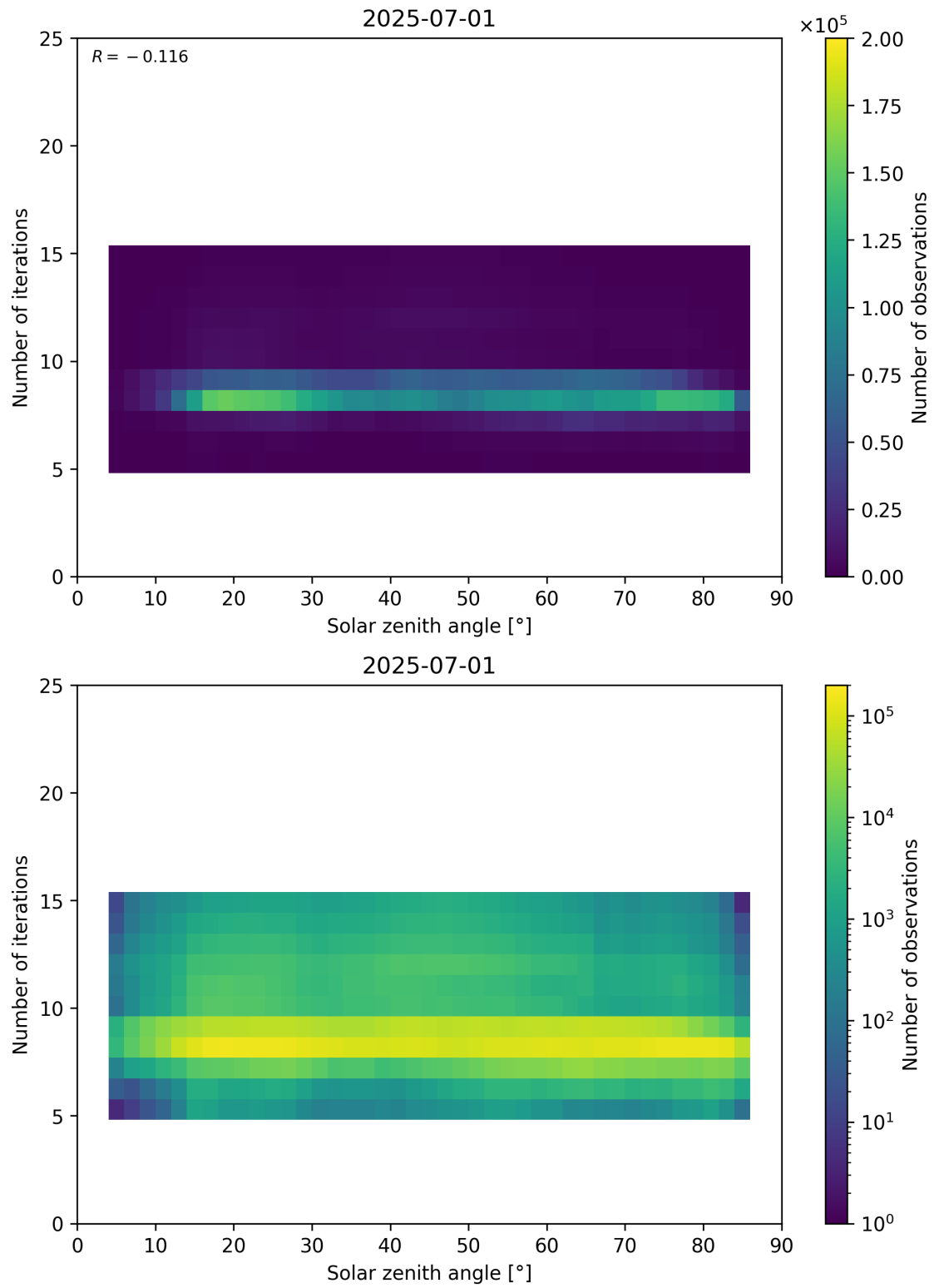
Figure 67: Scatter density plot of “Solar zenith angle” against “Number of iterations” for 2025-06-30 to 2025-07-02.
