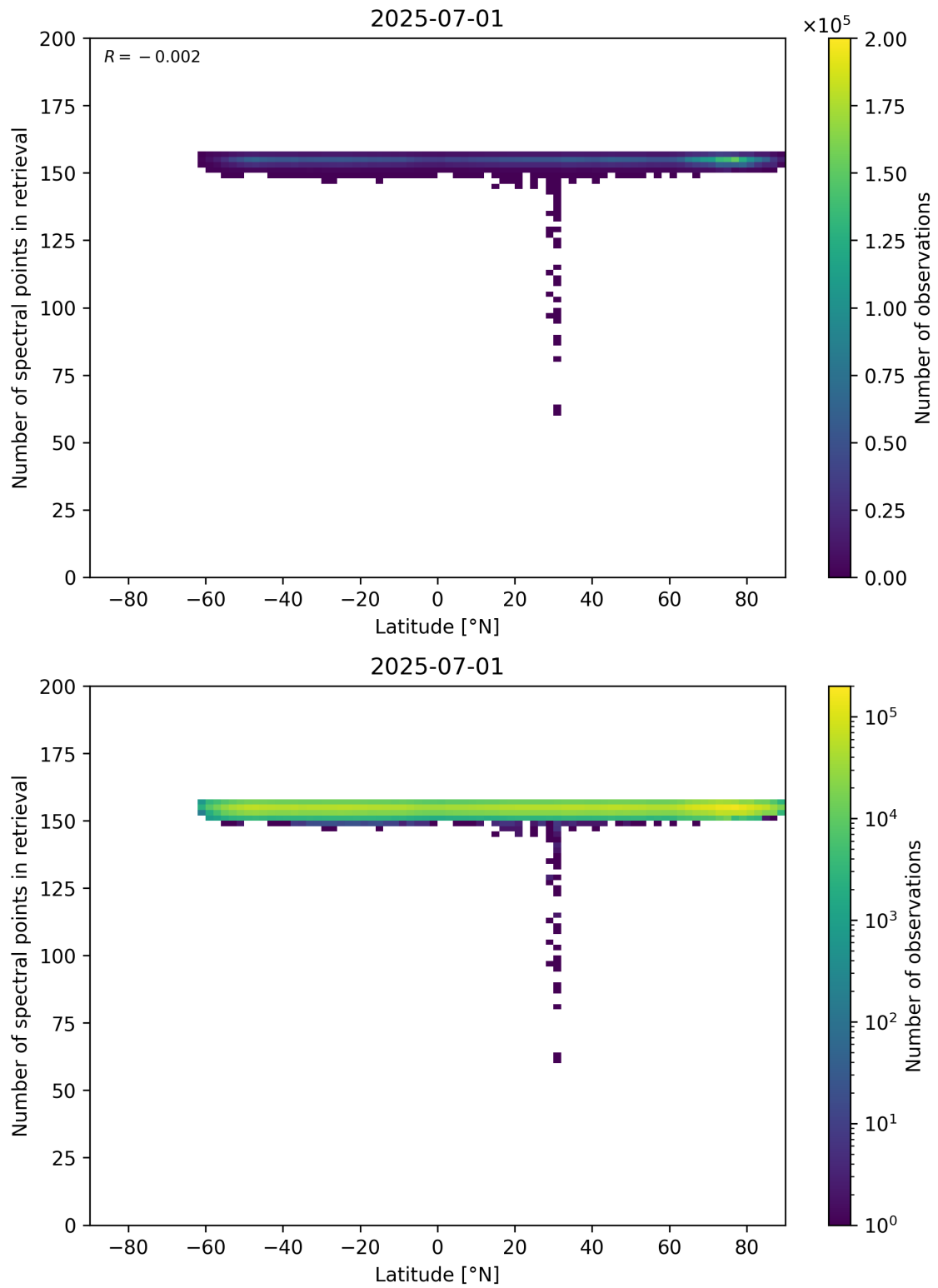
Figure 57: Scatter density plot of “Latitude” against “Number of spectral points in retrieval” for 2025-06-30 to 2025-07-02.
