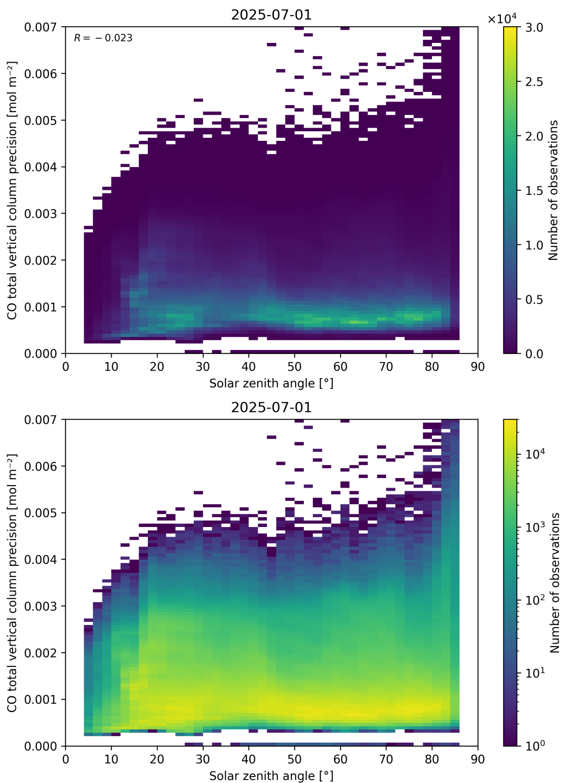
Figure 63: Scatter density plot of “Solar zenith angle” against “CO total vertical column precision” for 2025-06-30 to 2025-07-02.
