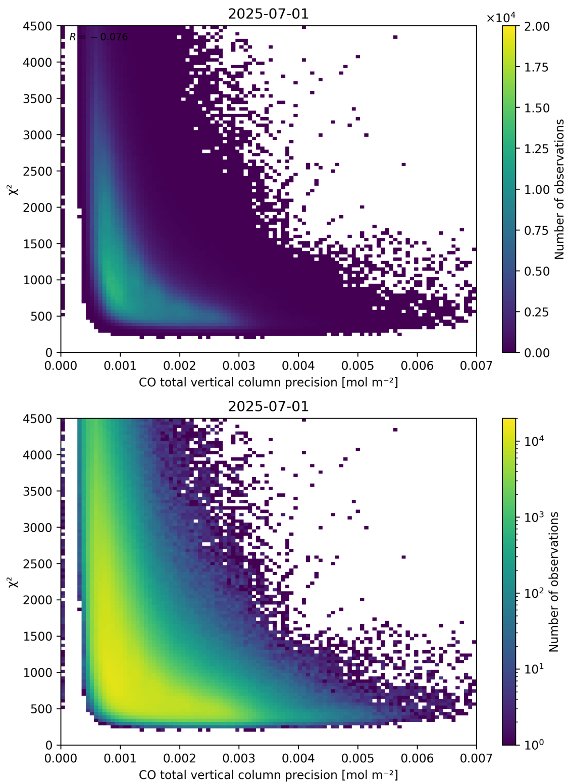
Figure 44: Scatter density plot of “CO total vertical column precision” against “ \chi^2 ” for 2025-06-30 to 2025-07-02.
