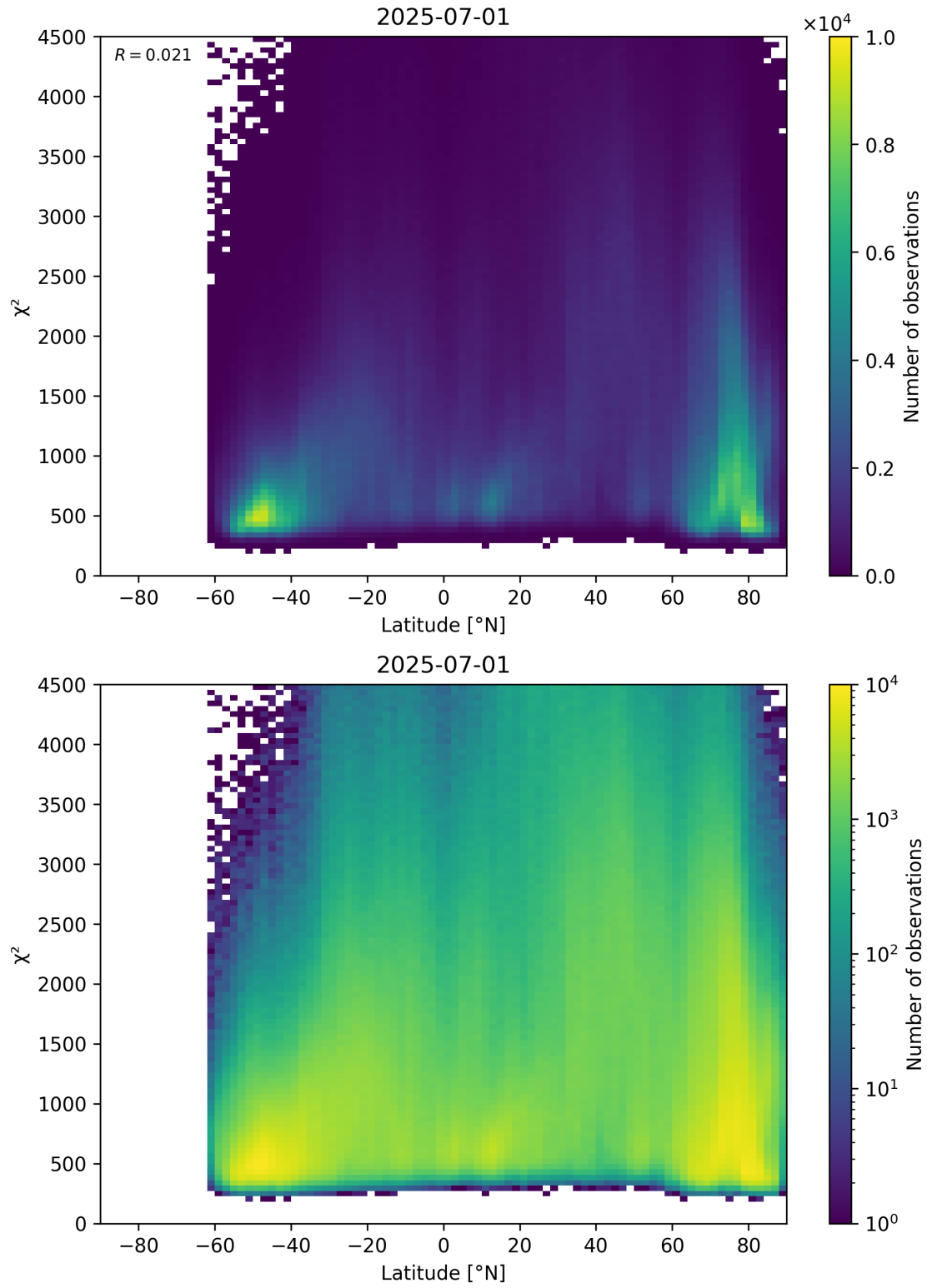
Figure 54: Scatter density plot of “Latitude” against “ \chi^2 ” for 2025-06-30 to 2025-07-02.
