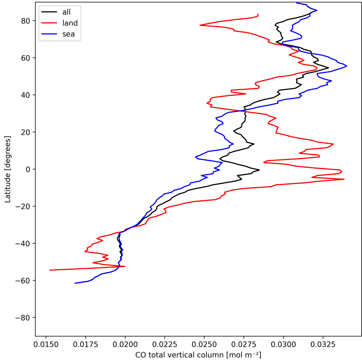
Figure 10: Zonal average of “CO total vertical column” for 2025-06-30 to 2025-07-02.
