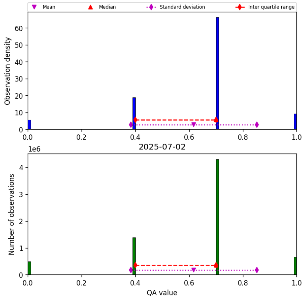
Figure 17: Histogram of “QA value” for 2025-07-02 to 2025-07-03
