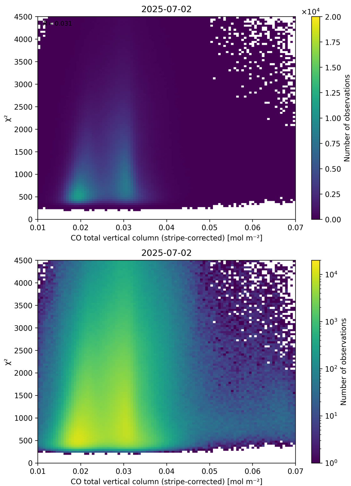
Figure 37: Scatter density plot of “CO total vertical column (stripe-corrected)” against “ \chi^2 ” for 2025-07-02 to 2025-07-03.
