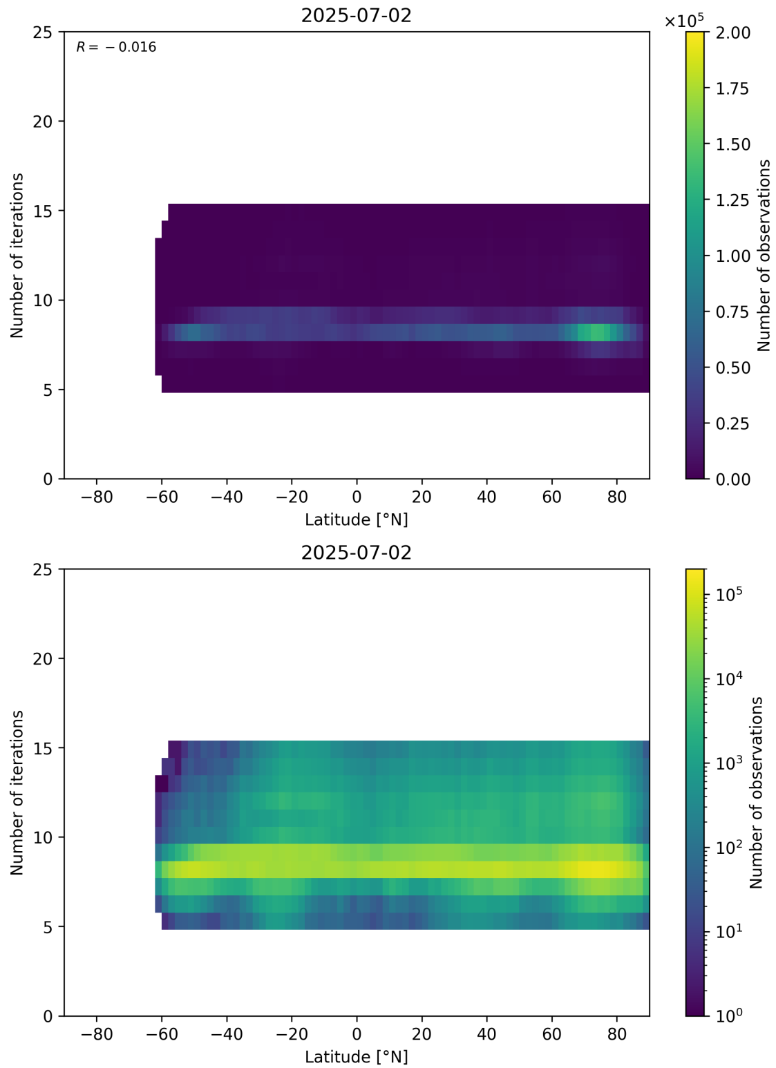
Figure 56: Scatter density plot of “Latitude” against “Number of iterations” for 2025-07-02 to 2025-07-03.
