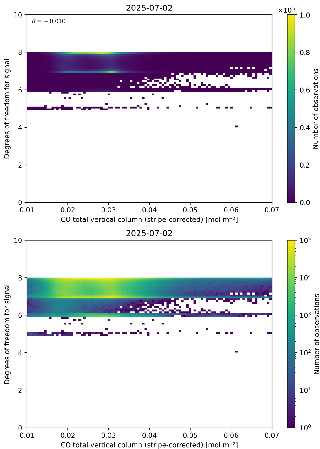
Figure 38: Scatter density plot of “CO total vertical column (stripe-corrected)” against “Degrees of freedom for signal” for 2025-07-02 to 2025-07-03.
