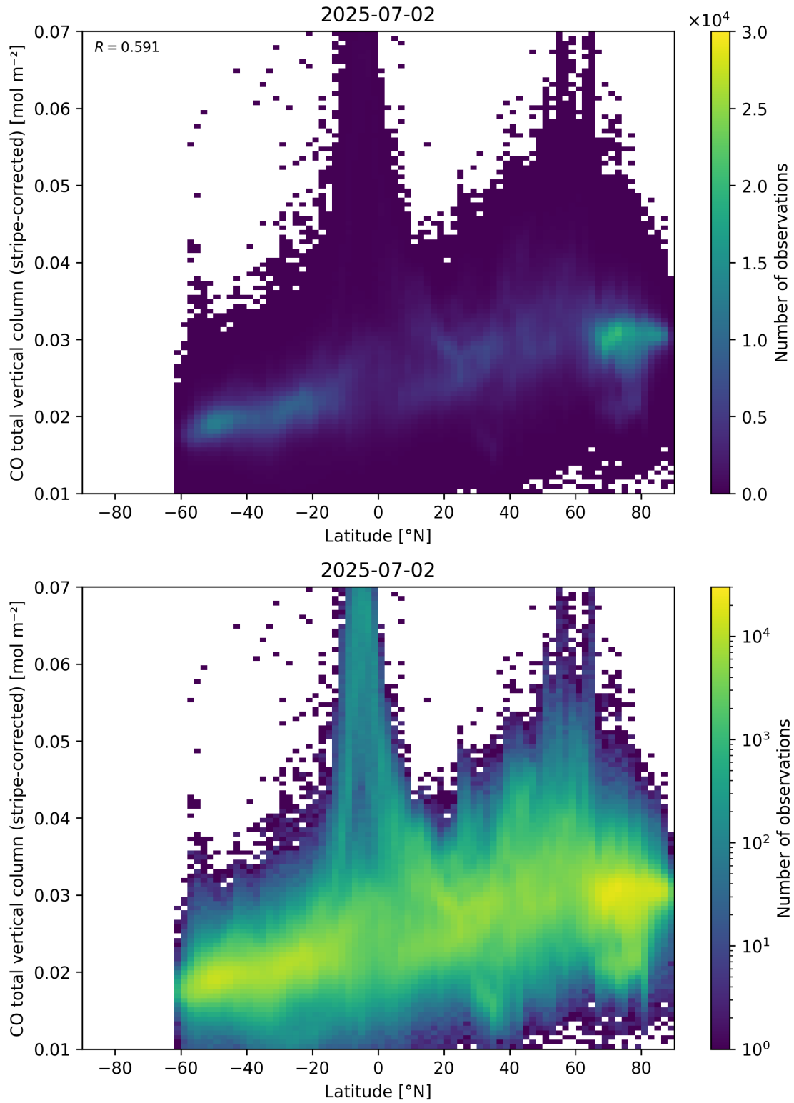
Figure 52: Scatter density plot of “Latitude” against “CO total vertical column (stripe-corrected)” for 2025-07-02 to 2025-07-03.
