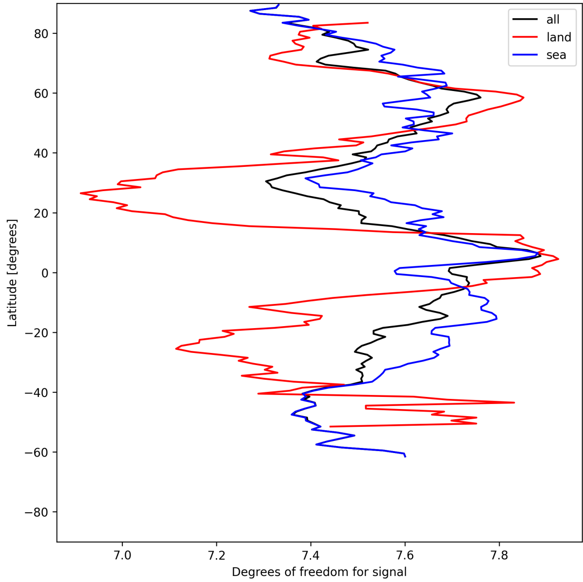
Figure 15: Zonal average of “Degrees of freedom for signal” for 2025-07-02 to 2025-07-03.
