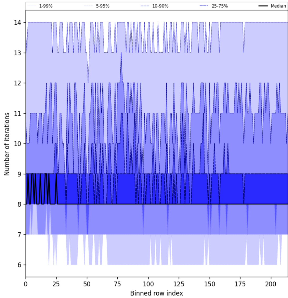
Figure 32: Along track statistics of “Number of iterations” for 2025-07-02 to 2025-07-03
