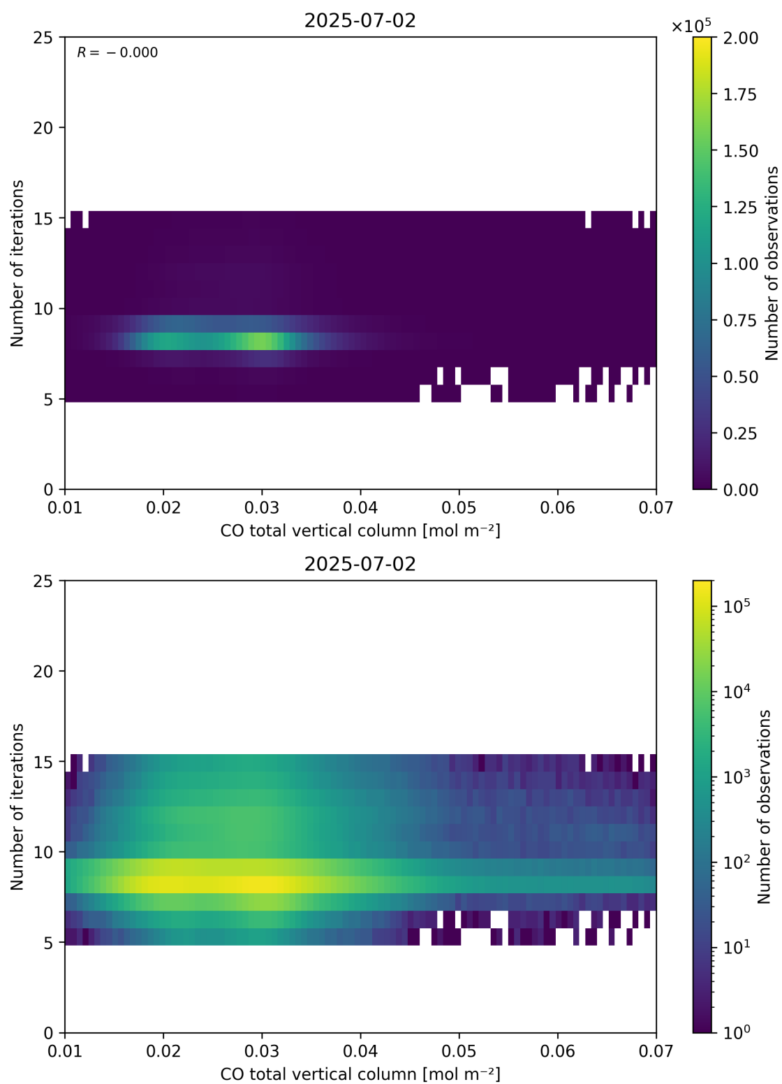
Figure 42: Scatter density plot of “CO total vertical column” against “Number of iterations” for 2025-07-02 to 2025-07-03.
