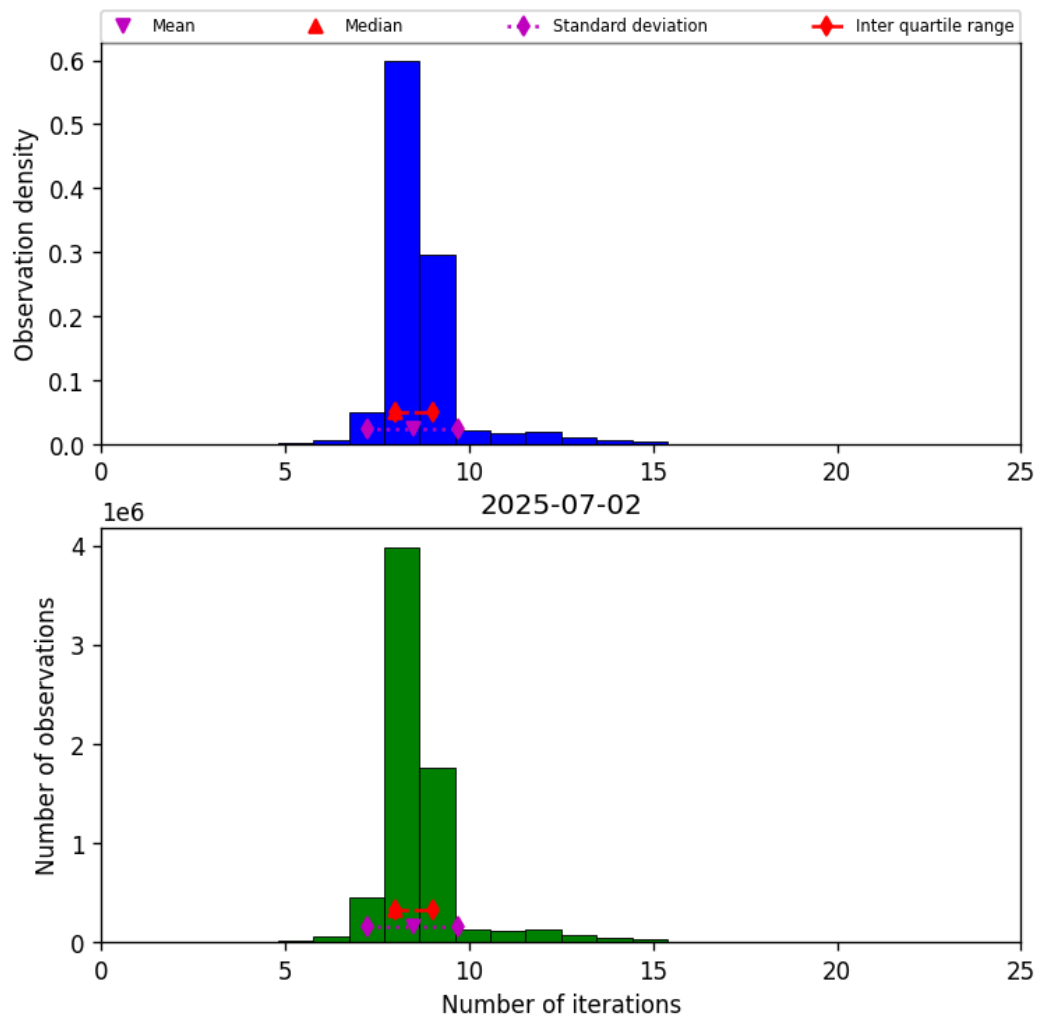
Figure 24: Histogram of “Number of iterations” for 2025-07-02 to 2025-07-03
