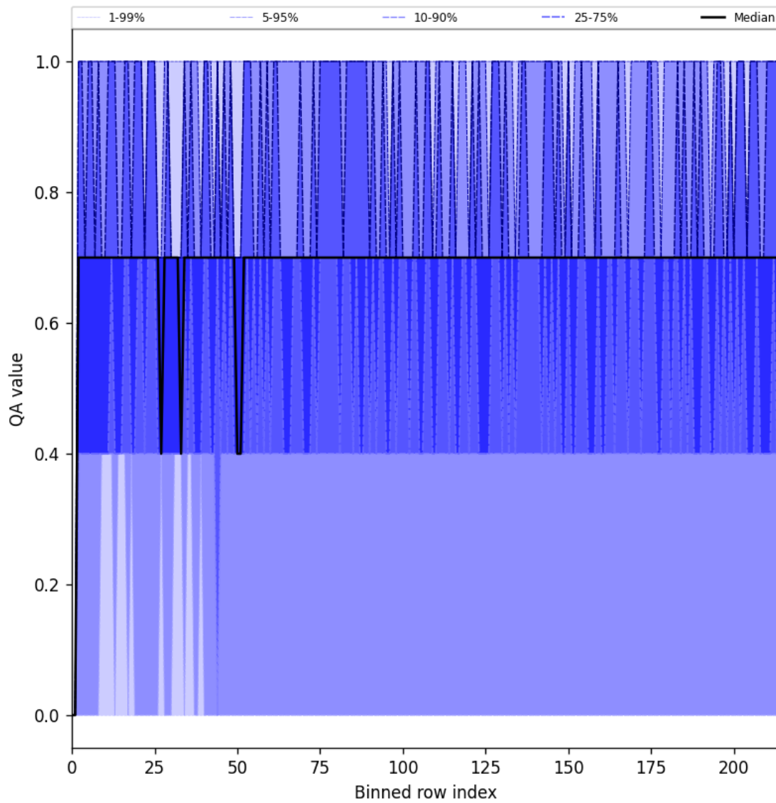
Figure 25: Along track statistics of “QA value” for 2025-07-02 to 2025-07-03
