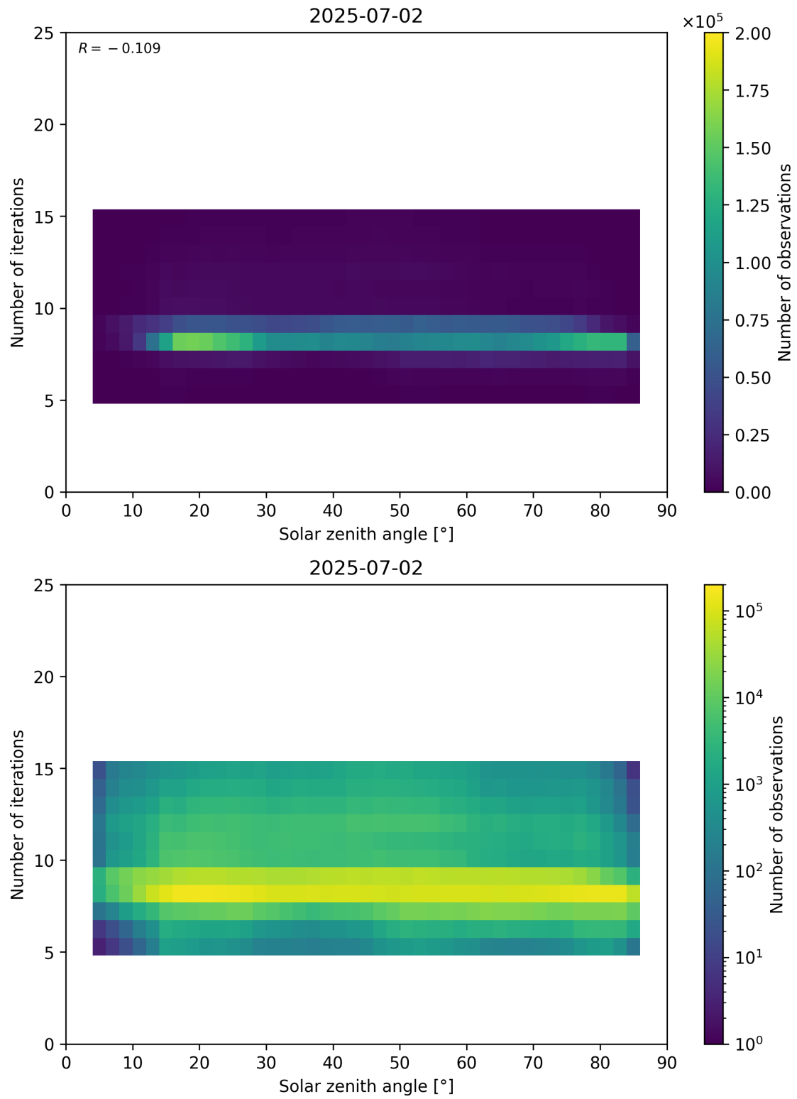
Figure 67: Scatter density plot of “Solar zenith angle” against “Number of iterations” for 2025-07-02 to 2025-07-03.
