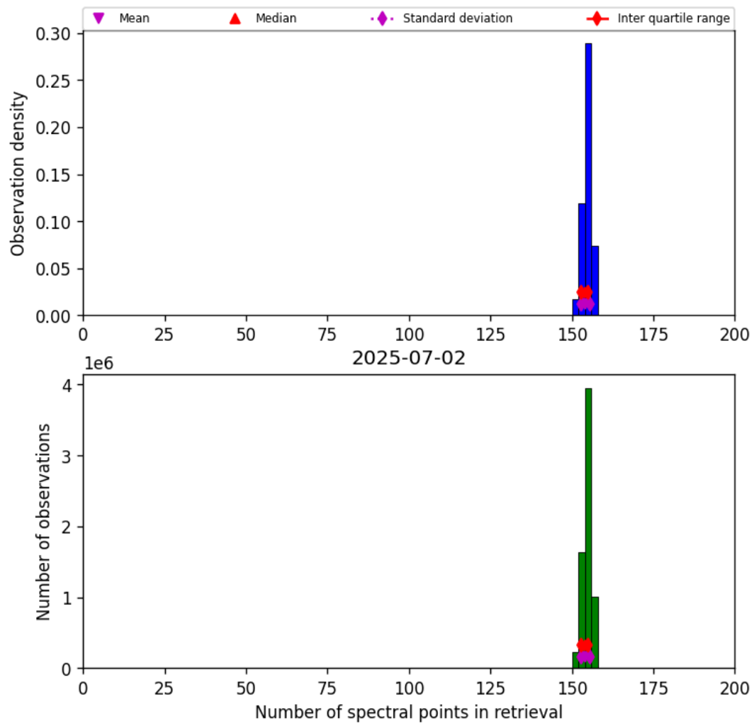
Figure 21: Histogram of “Number of spectral points in retrieval” for 2025-07-02 to 2025-07-03
