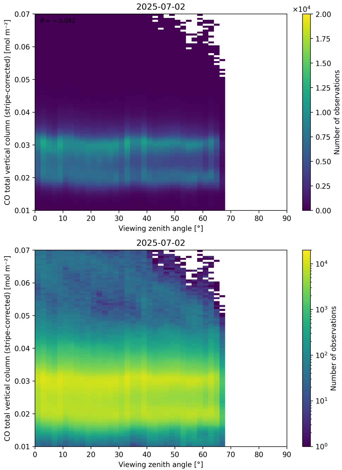
Figure 70: Scatter density plot of “Viewing zenith angle” against “CO total vertical column (stripe-corrected)” for 2025-07-02 to 2025-07-03.
