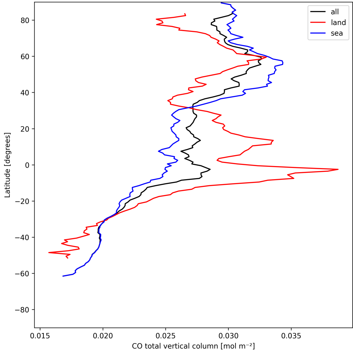
Figure 10: Zonal average of “CO total vertical column” for 2025-07-02 to 2025-07-03.
