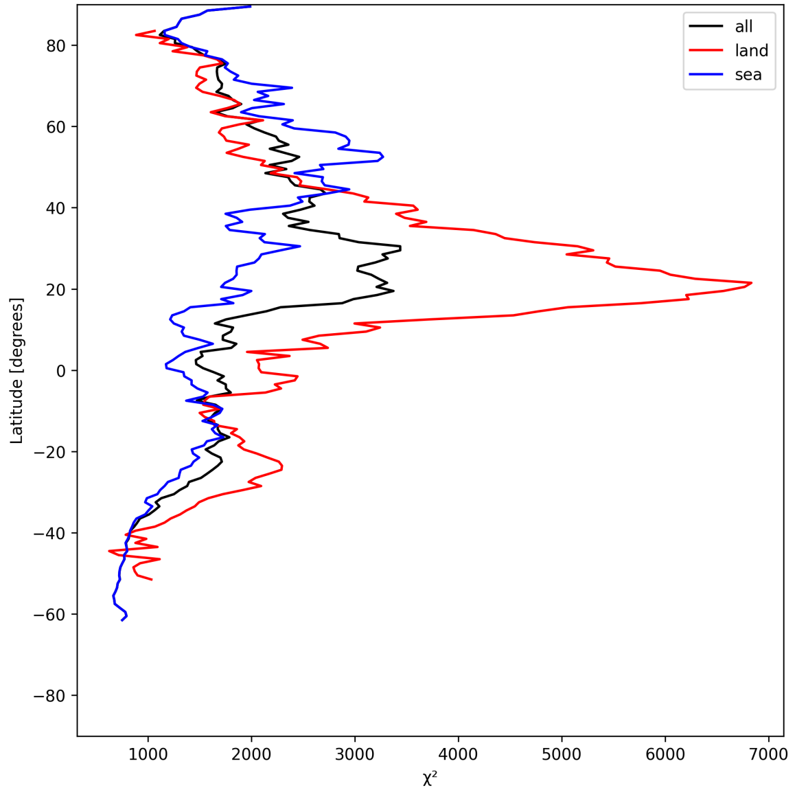
Figure 14: Zonal average of “ \chi^2 ” for 2025-07-02 to 2025-07-03.
