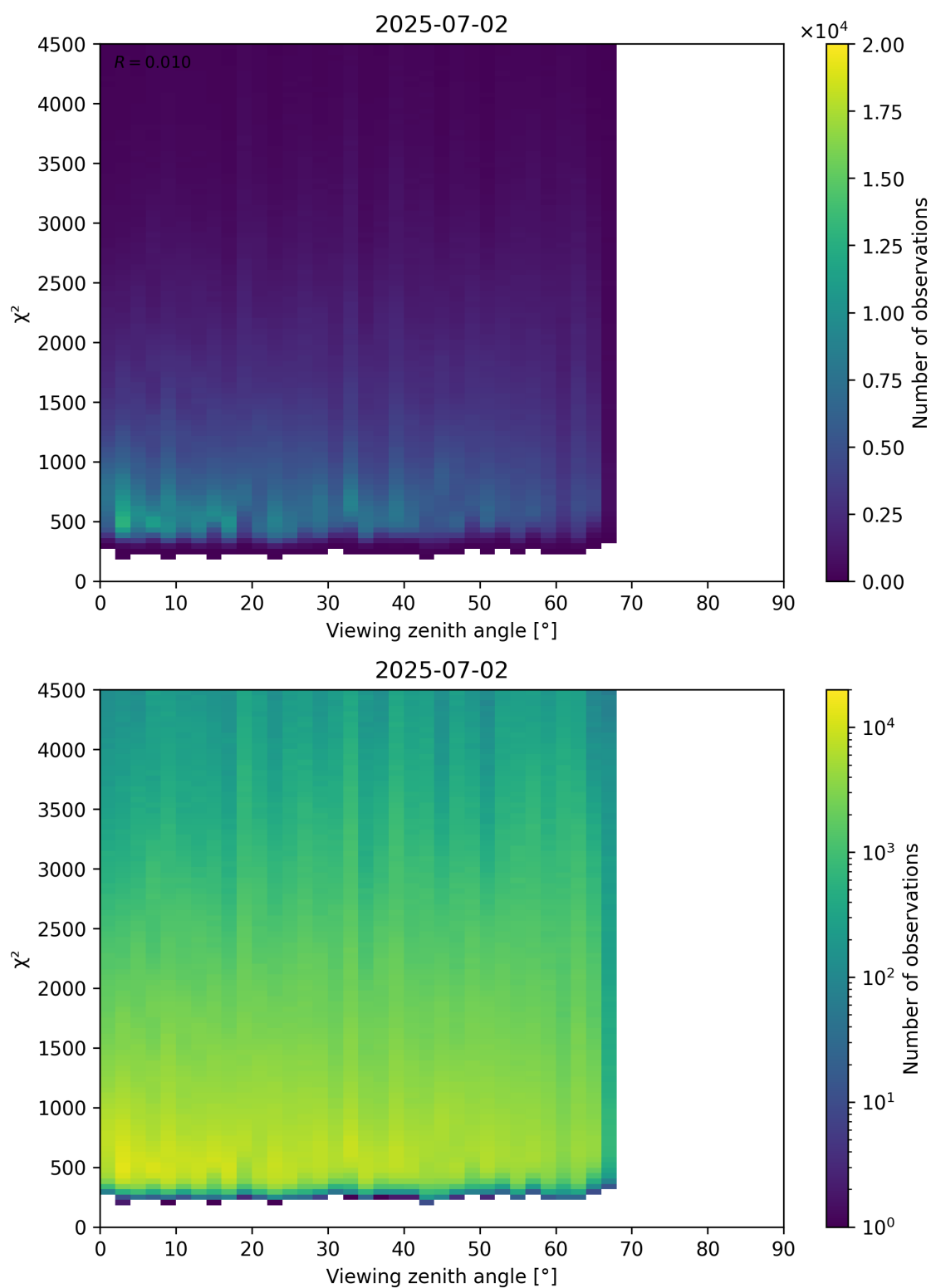
Figure 72: Scatter density plot of “Viewing zenith angle” against “ \chi^2 ” for 2025-07-02 to 2025-07-03.
