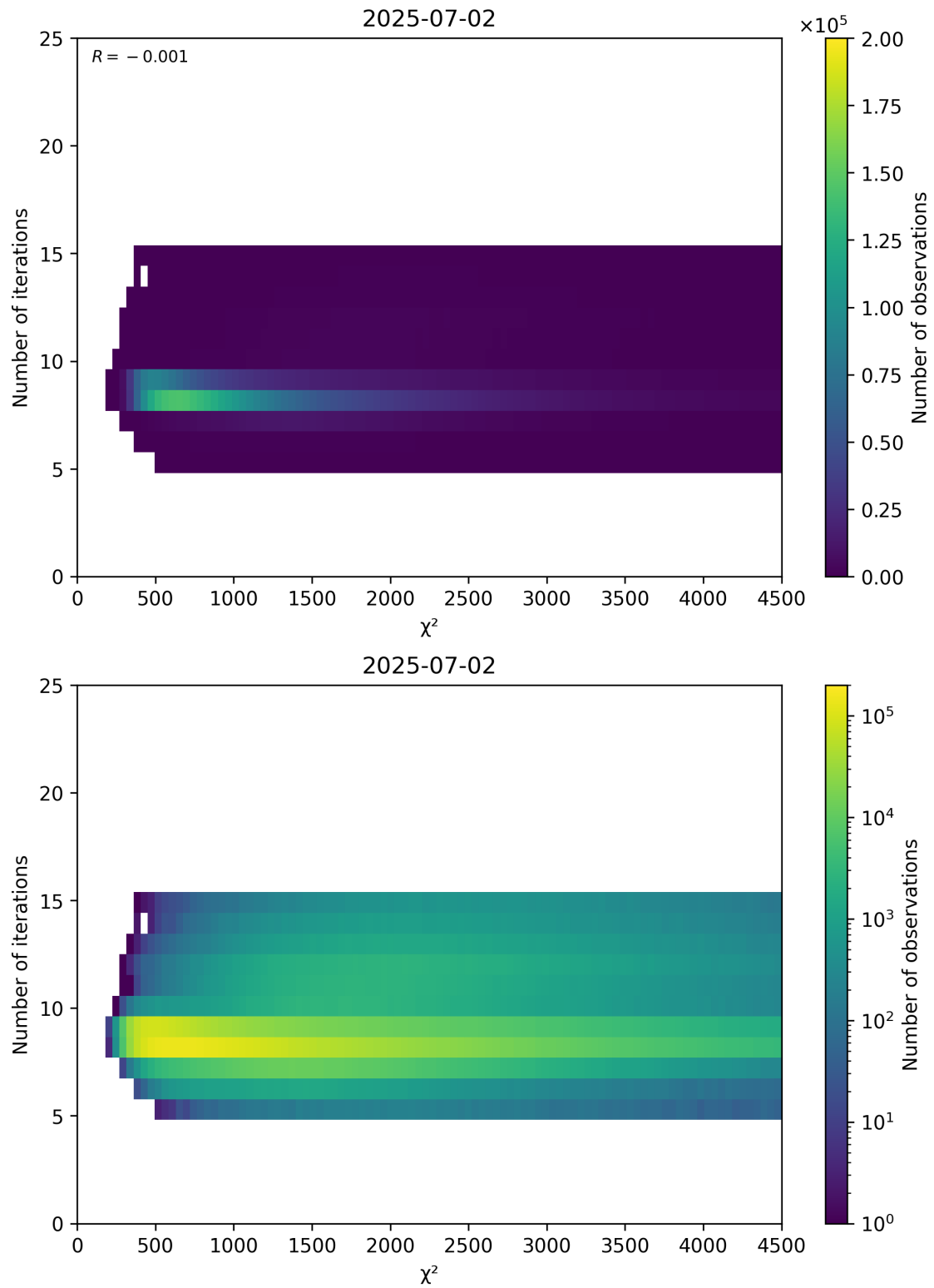
Figure 49: Scatter density plot of “ \chi^2 ” against “Number of iterations” for 2025-07-02 to 2025-07-03.
