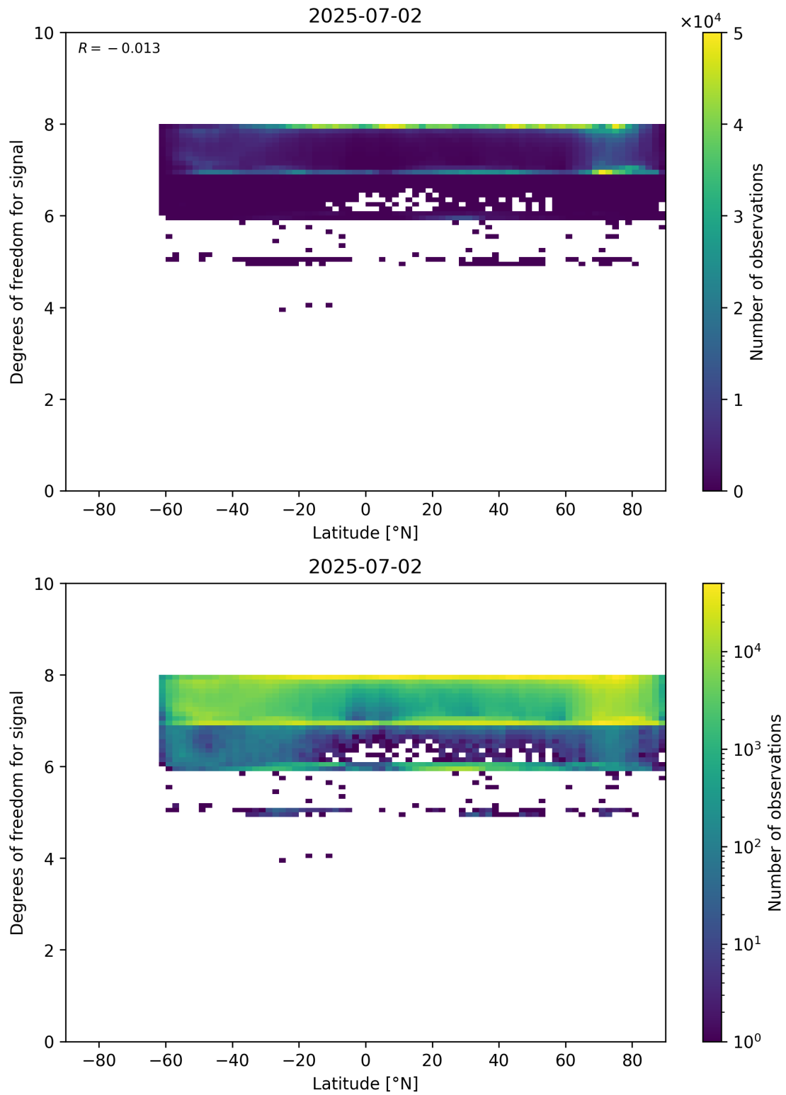
Figure 55: Scatter density plot of “Latitude” against “Degrees of freedom for signal” for 2025-07-02 to 2025-07-03.
