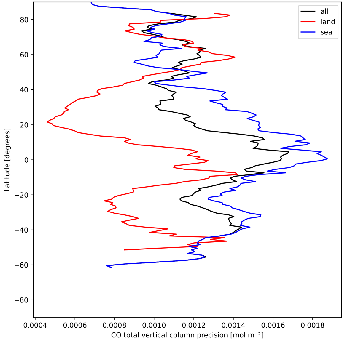
Figure 12: Zonal average of “CO total vertical column precision” for 2025-07-02 to 2025-07-03.
