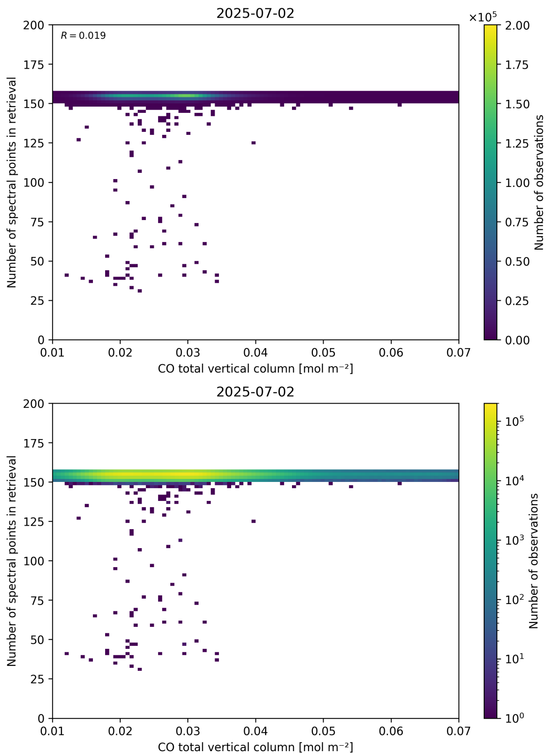
Figure 43: Scatter density plot of “CO total vertical column” against “Number of spectral points in retrieval” for 2025-07-02 to 2025-07-03.
