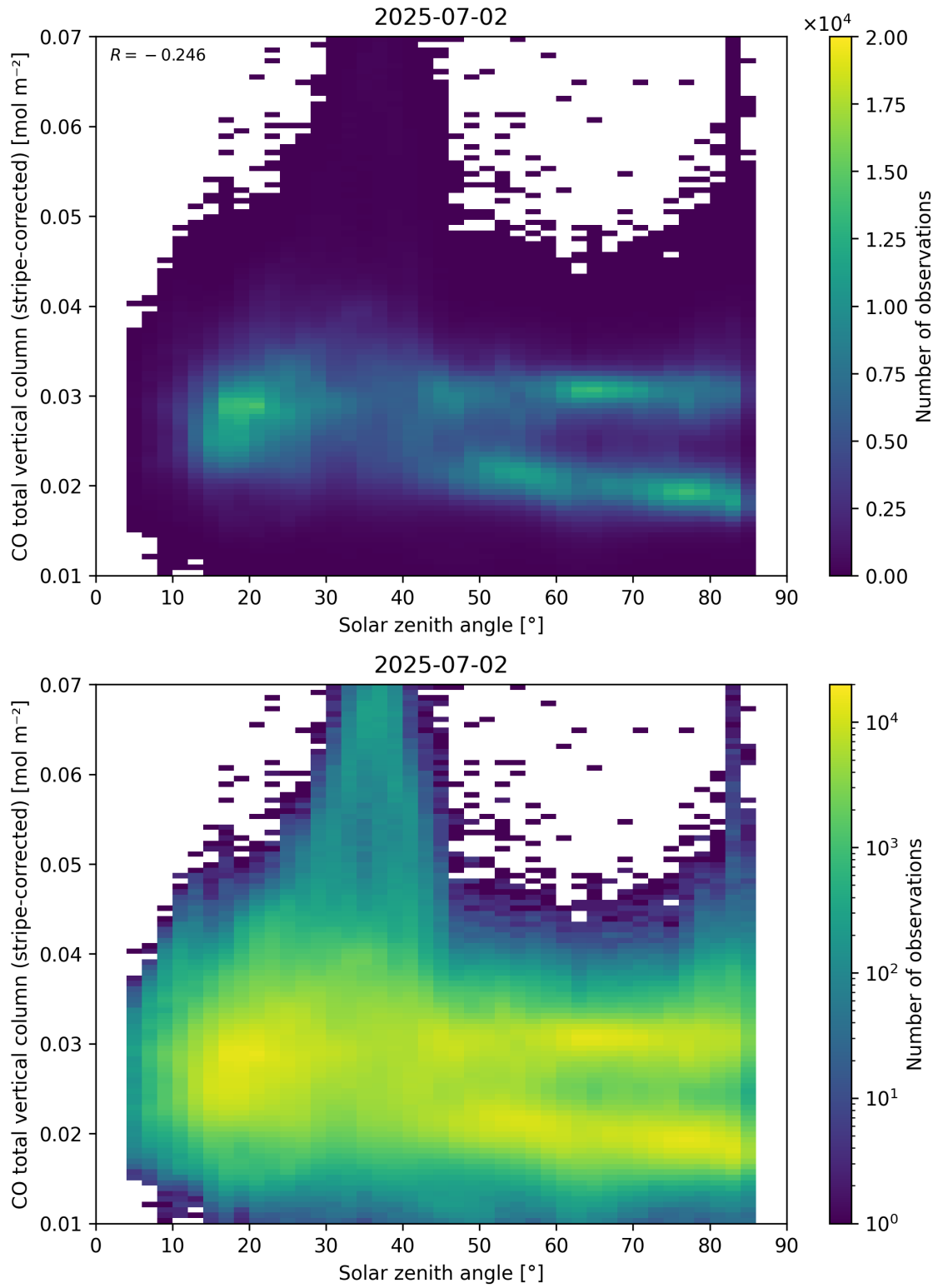
Figure 62: Scatter density plot of “Solar zenith angle” against “CO total vertical column (stripe-corrected)” for 2025-07-02 to 2025-07-03.
