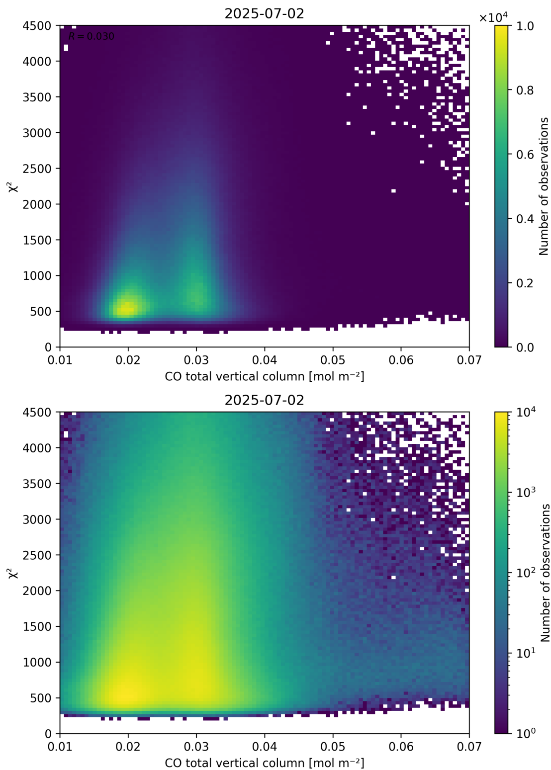
Figure 35: Scatter density plot of “CO total vertical column” against “ \chi^2 ” for 2025-07-02 to 2025-07-03.
