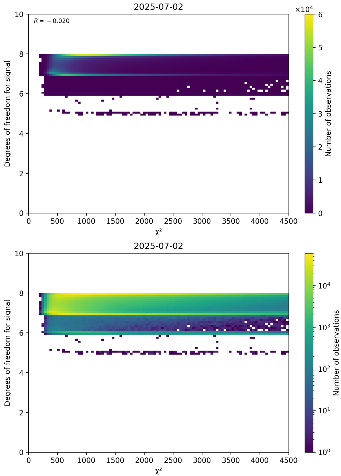
Figure 48: Scatter density plot of “ \chi^2 ” against “Degrees of freedom for signal” for 2025-07-02 to 2025-07-03.
