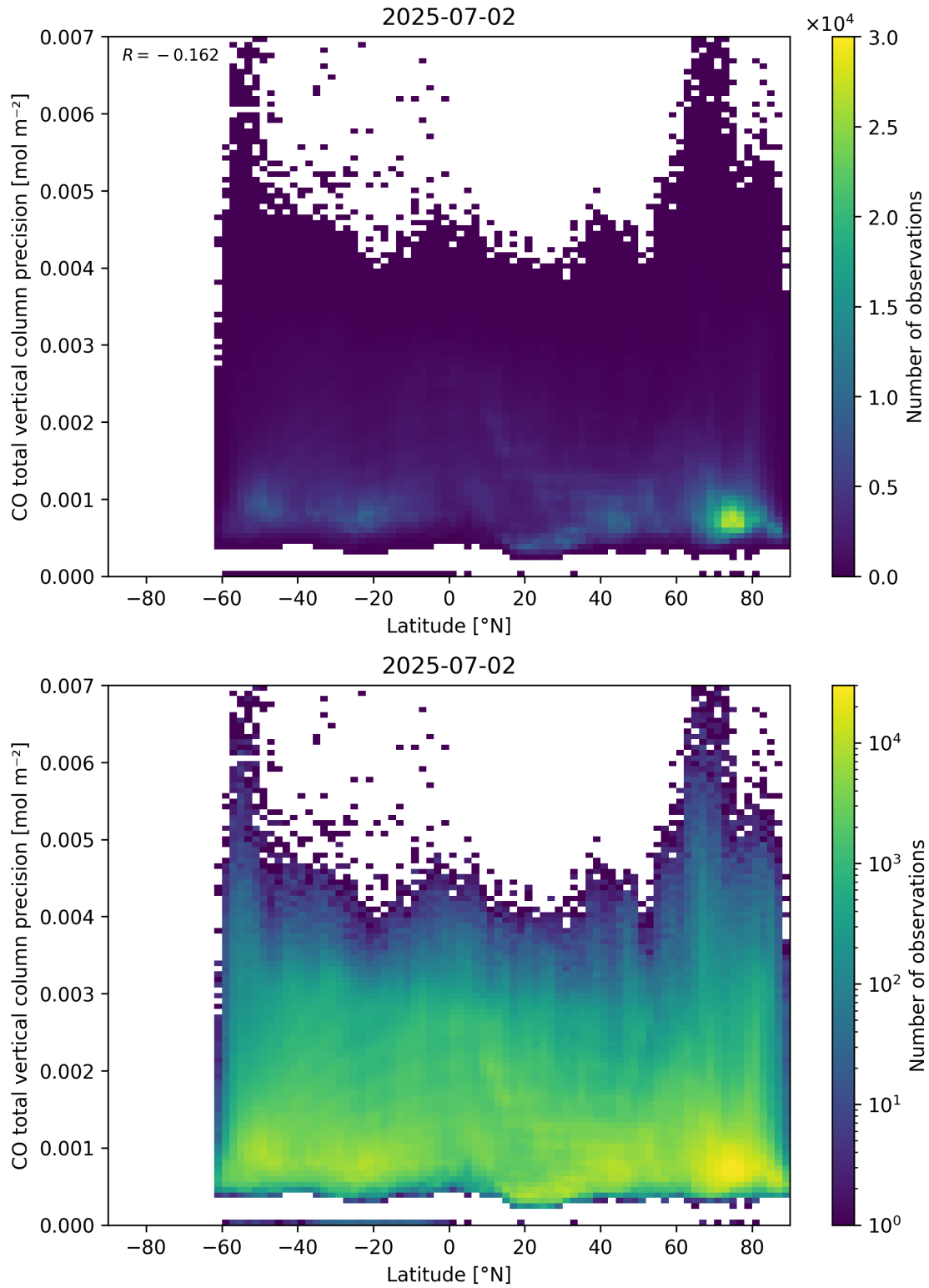
Figure 53: Scatter density plot of “Latitude” against “CO total vertical column precision” for 2025-07-02 to 2025-07-03.
