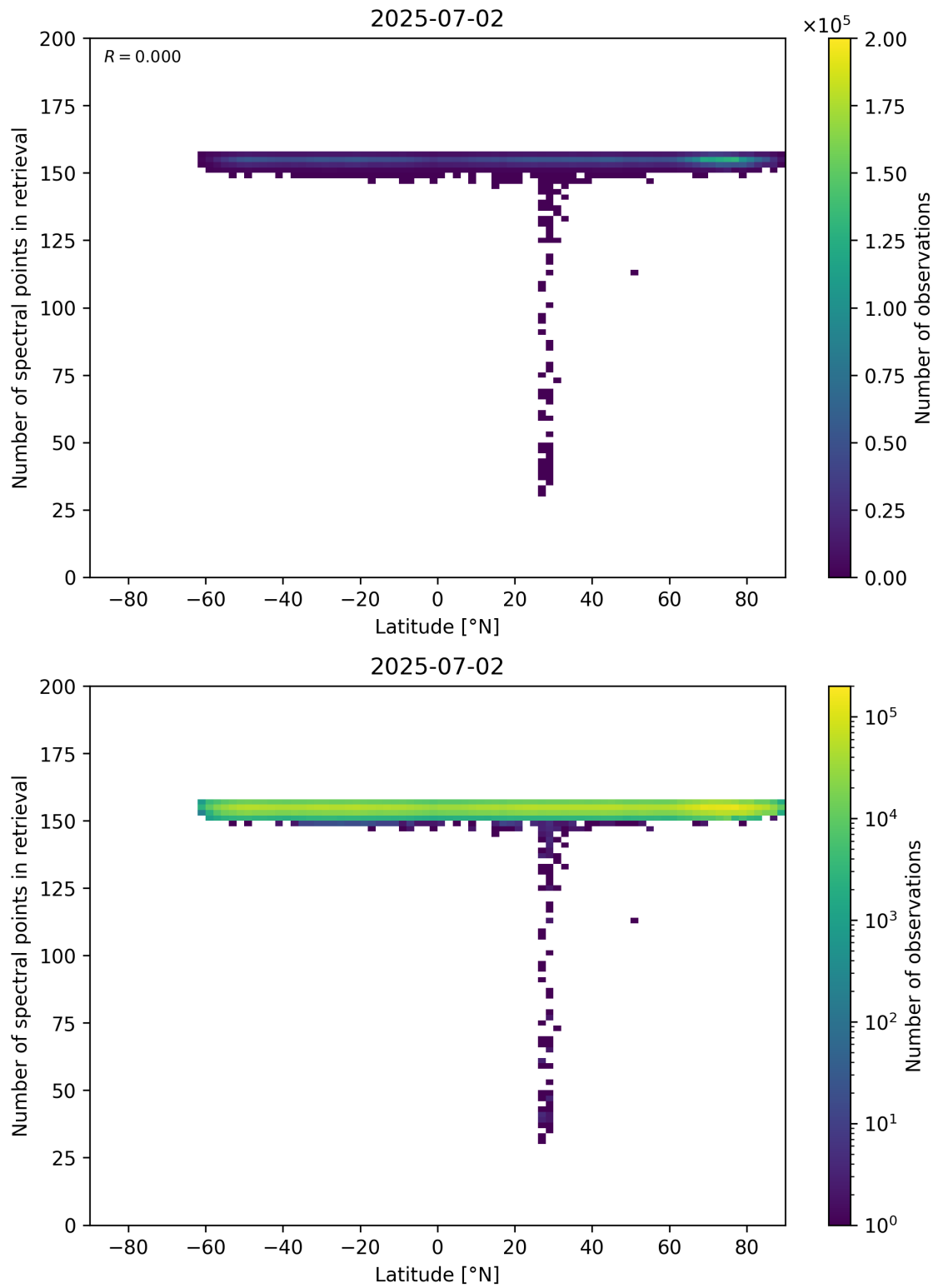
Figure 57: Scatter density plot of “Latitude” against “Number of spectral points in retrieval” for 2025-07-02 to 2025-07-03.
