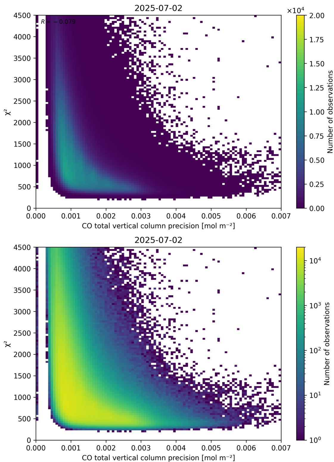
Figure 44: Scatter density plot of “CO total vertical column precision” against “ \chi^2 ” for 2025-07-02 to 2025-07-03.
