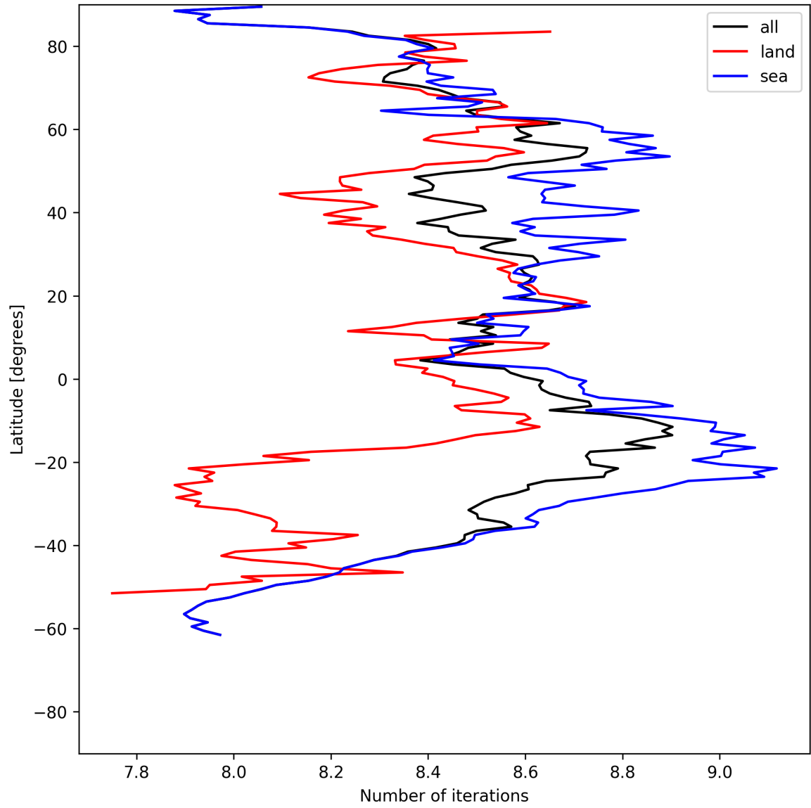
Figure 16: Zonal average of “Number of iterations” for 2025-07-02 to 2025-07-03.
