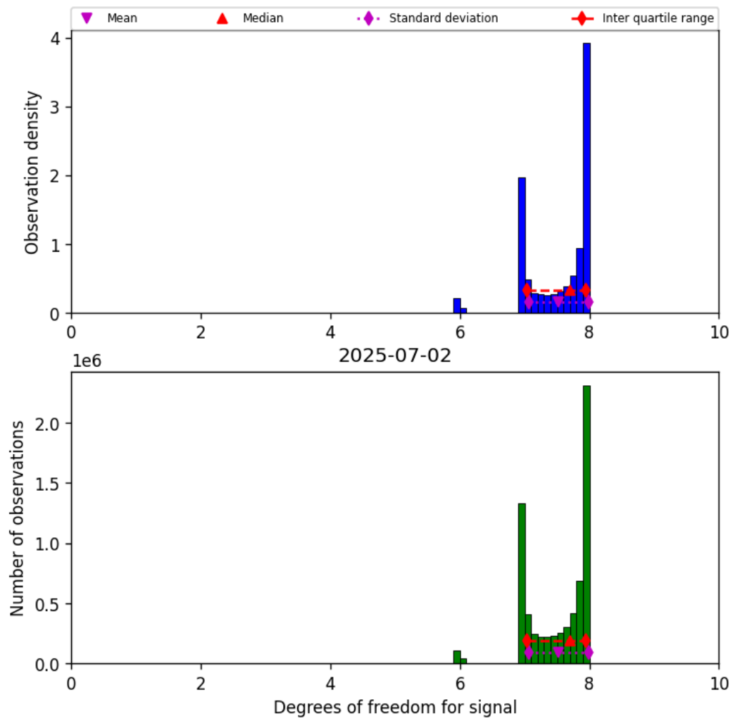
Figure 23: Histogram of “Degrees of freedom for signal” for 2025-07-02 to 2025-07-03
