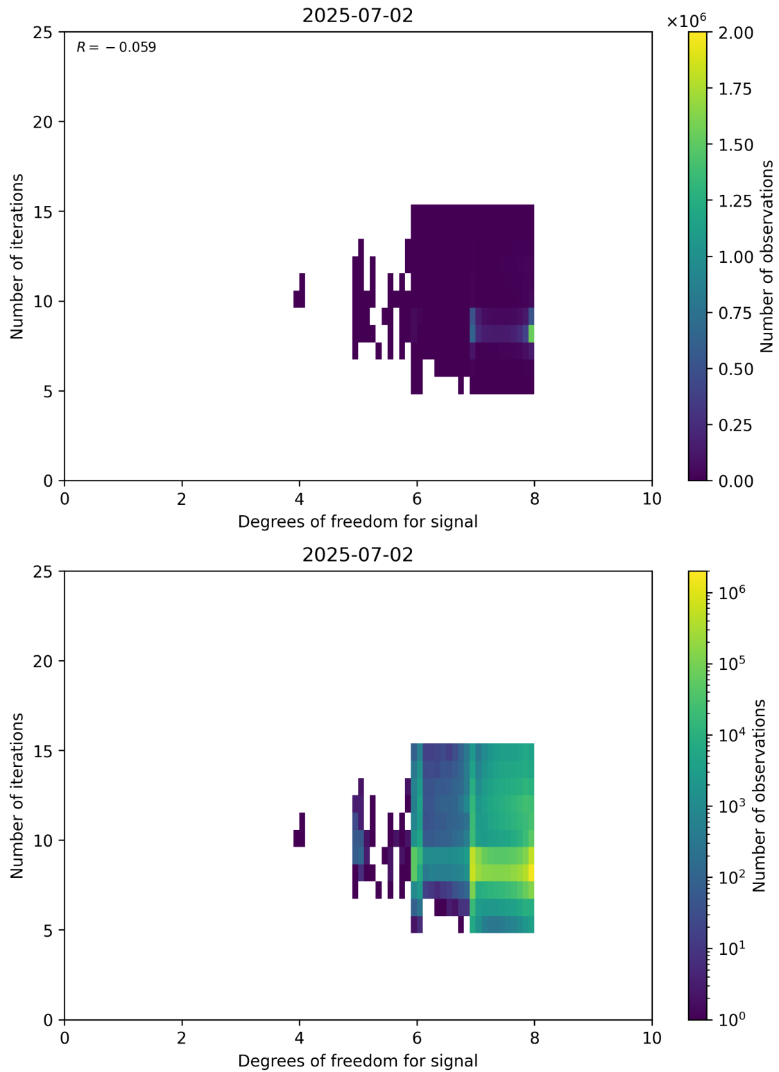
Figure 50: Scatter density plot of “Degrees of freedom for signal” against “Number of iterations” for 2025-07-02 to 2025-07-03.
