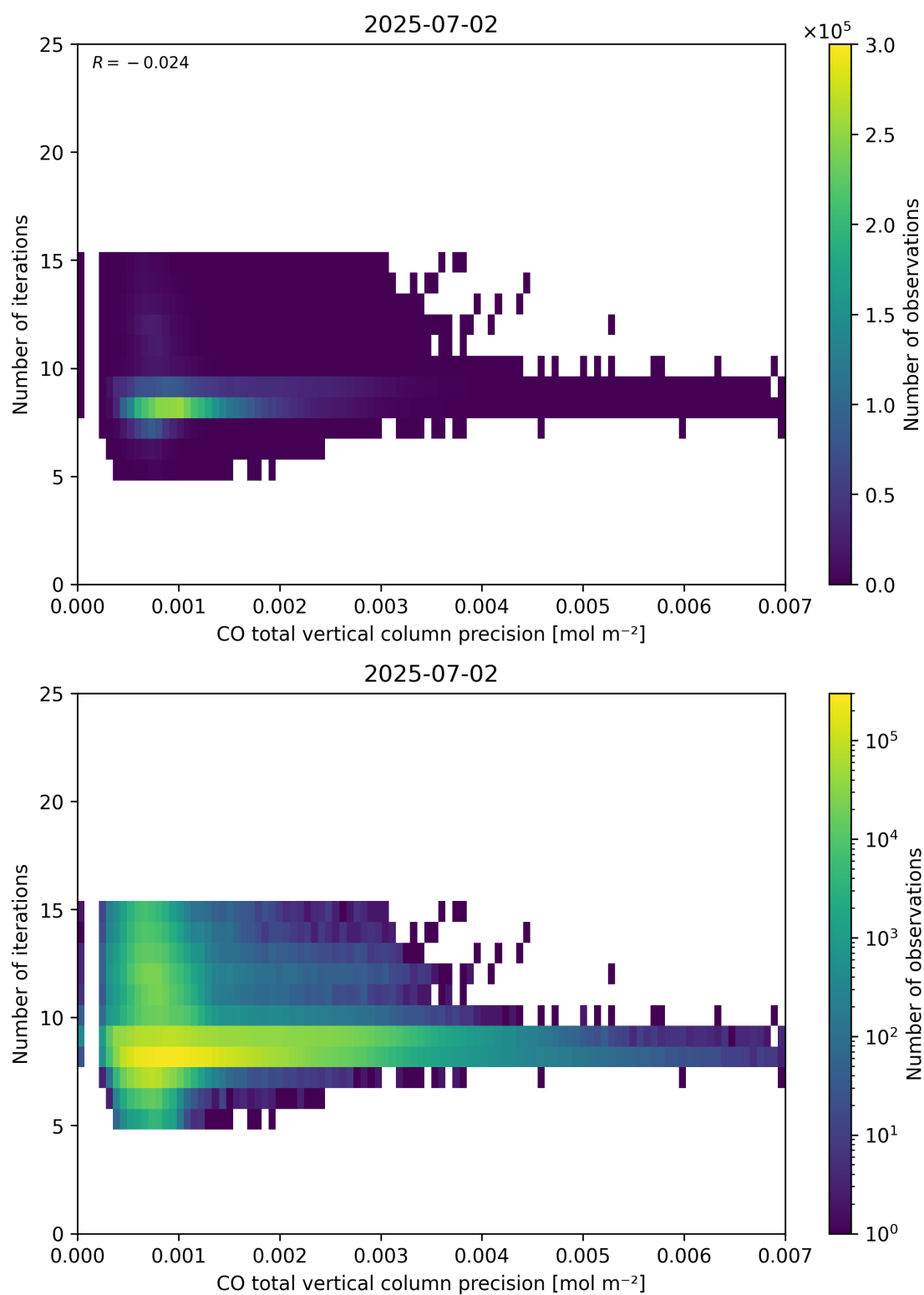
Figure 46: Scatter density plot of “CO total vertical column precision” against “Number of iterations” for 2025-07-02 to 2025-07-03.
