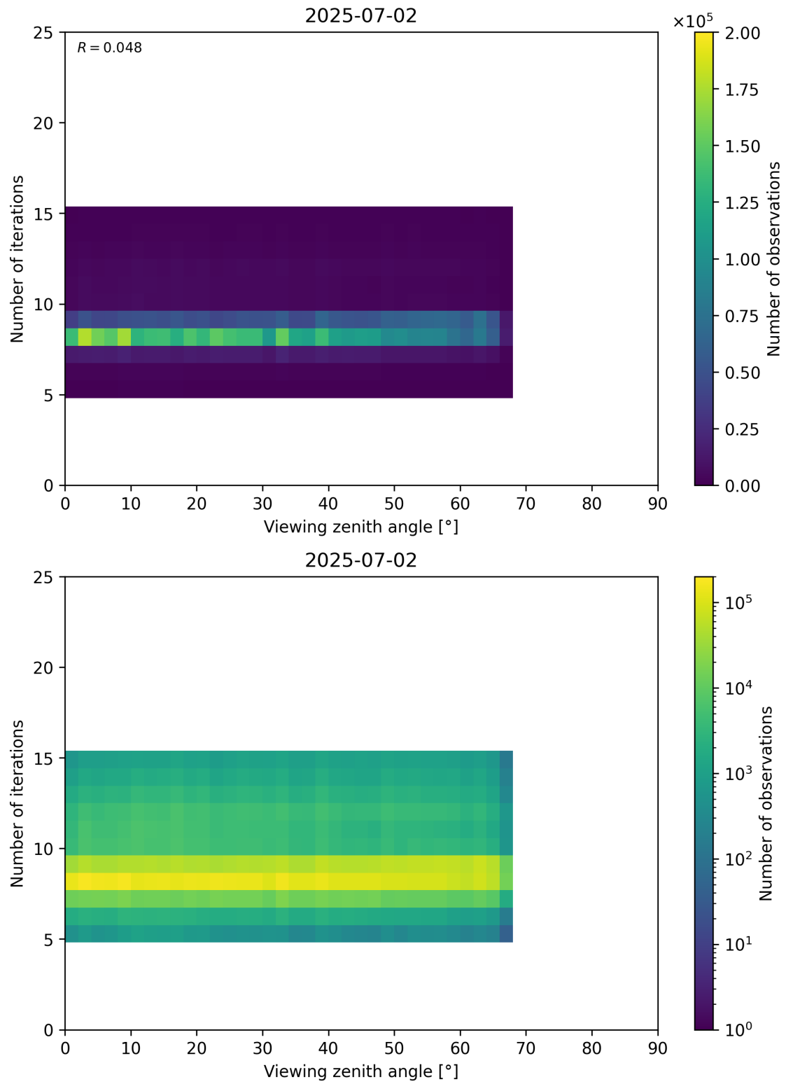
Figure 75: Scatter density plot of “Viewing zenith angle” against “Number of iterations” for 2025-07-02 to 2025-07-03.
