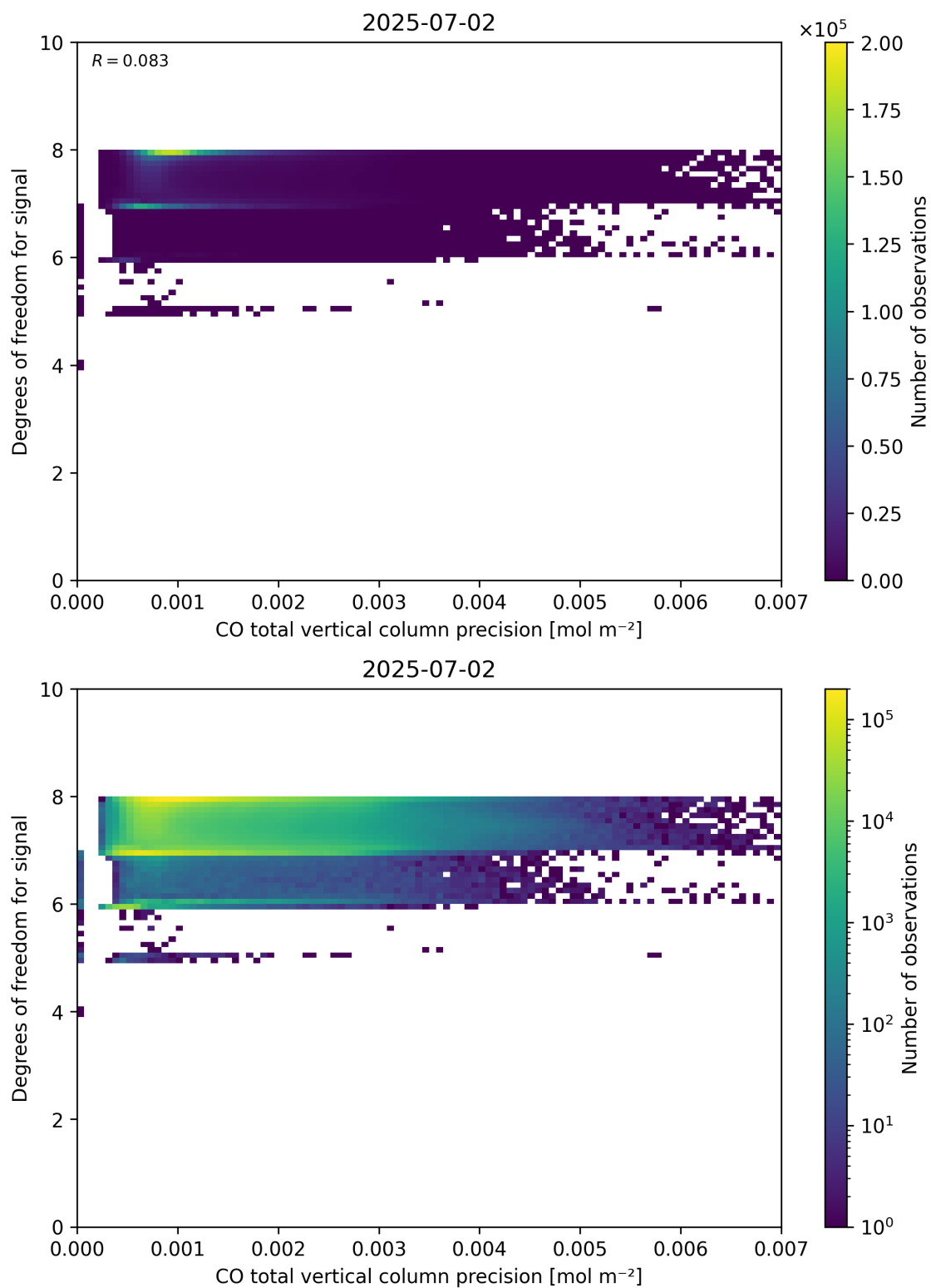
Figure 45: Scatter density plot of “CO total vertical column precision” against “Degrees of freedom for signal” for 2025-07-02 to 2025-07-03.
