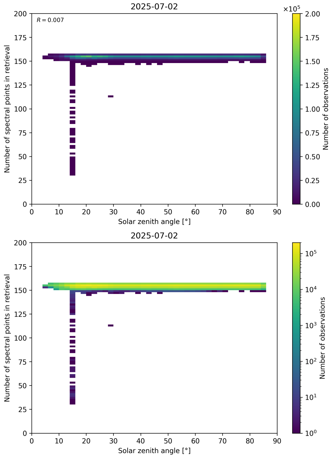
Figure 68: Scatter density plot of “Solar zenith angle” against “Number of spectral points in retrieval” for 2025-07-02 to 2025-07-03.
