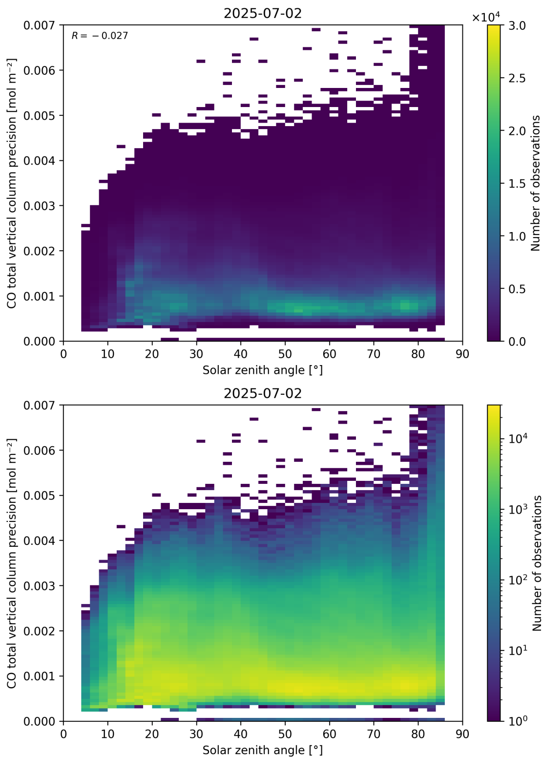
Figure 63: Scatter density plot of “Solar zenith angle” against “CO total vertical column precision” for 2025-07-02 to 2025-07-03.
