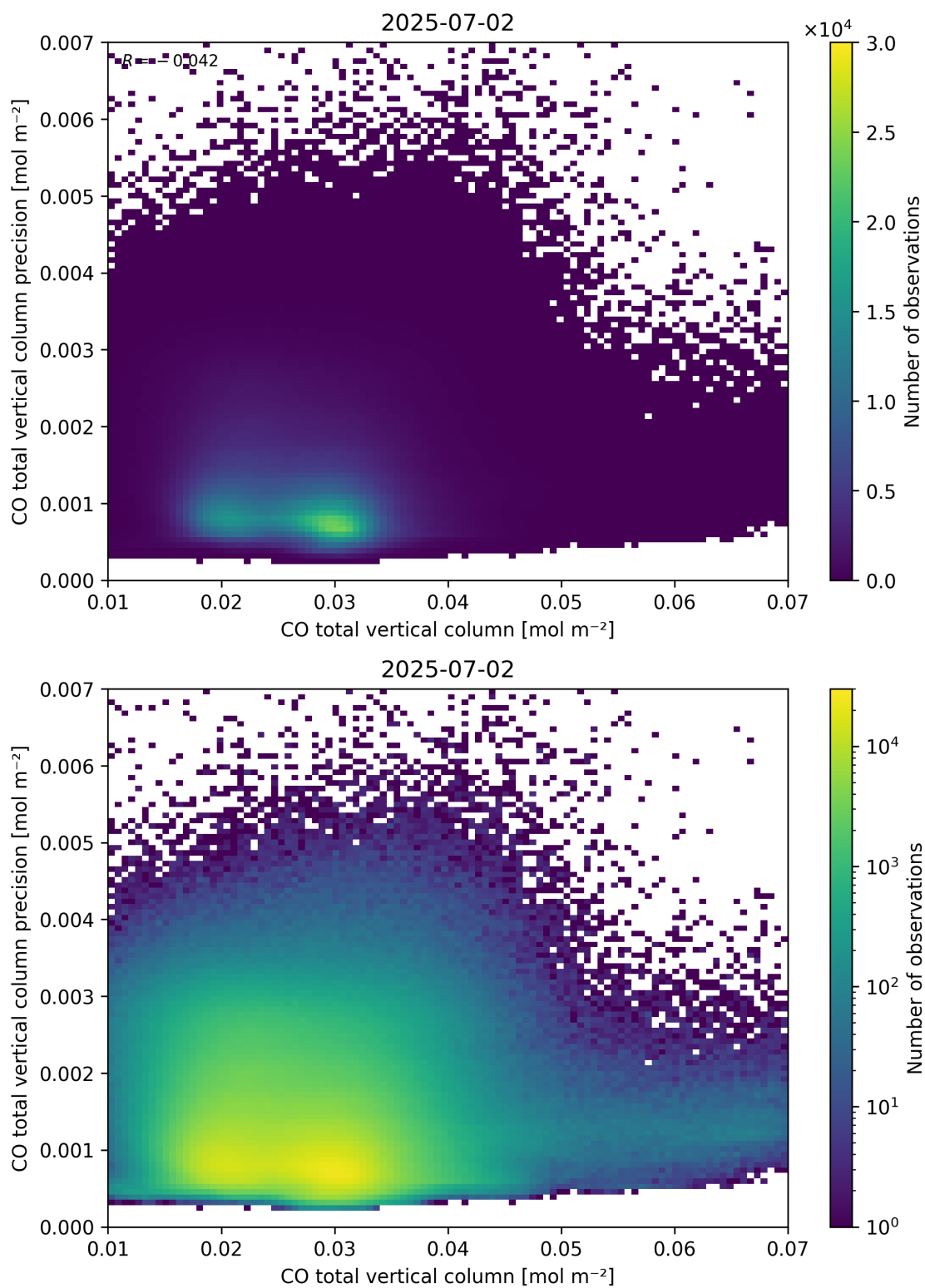
Figure 34: Scatter density plot of “CO total vertical column” against “CO total vertical column precision” for 2025-07-02 to 2025-07-03.
