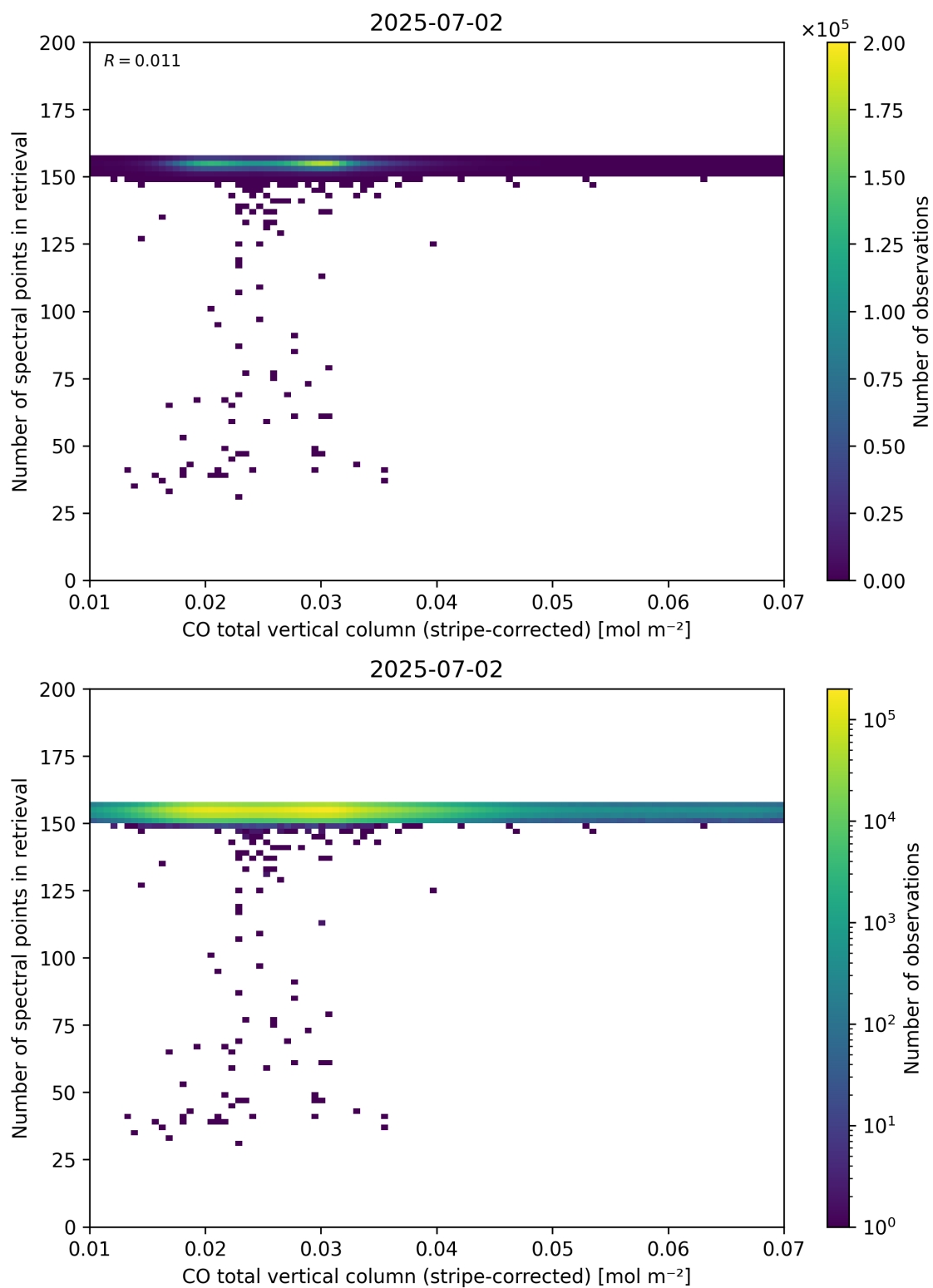
Figure 40: Scatter density plot of “CO total vertical column (stripe-corrected)” against “Number of spectral points in retrieval” for 2025-07-02 to 2025-07-03.
