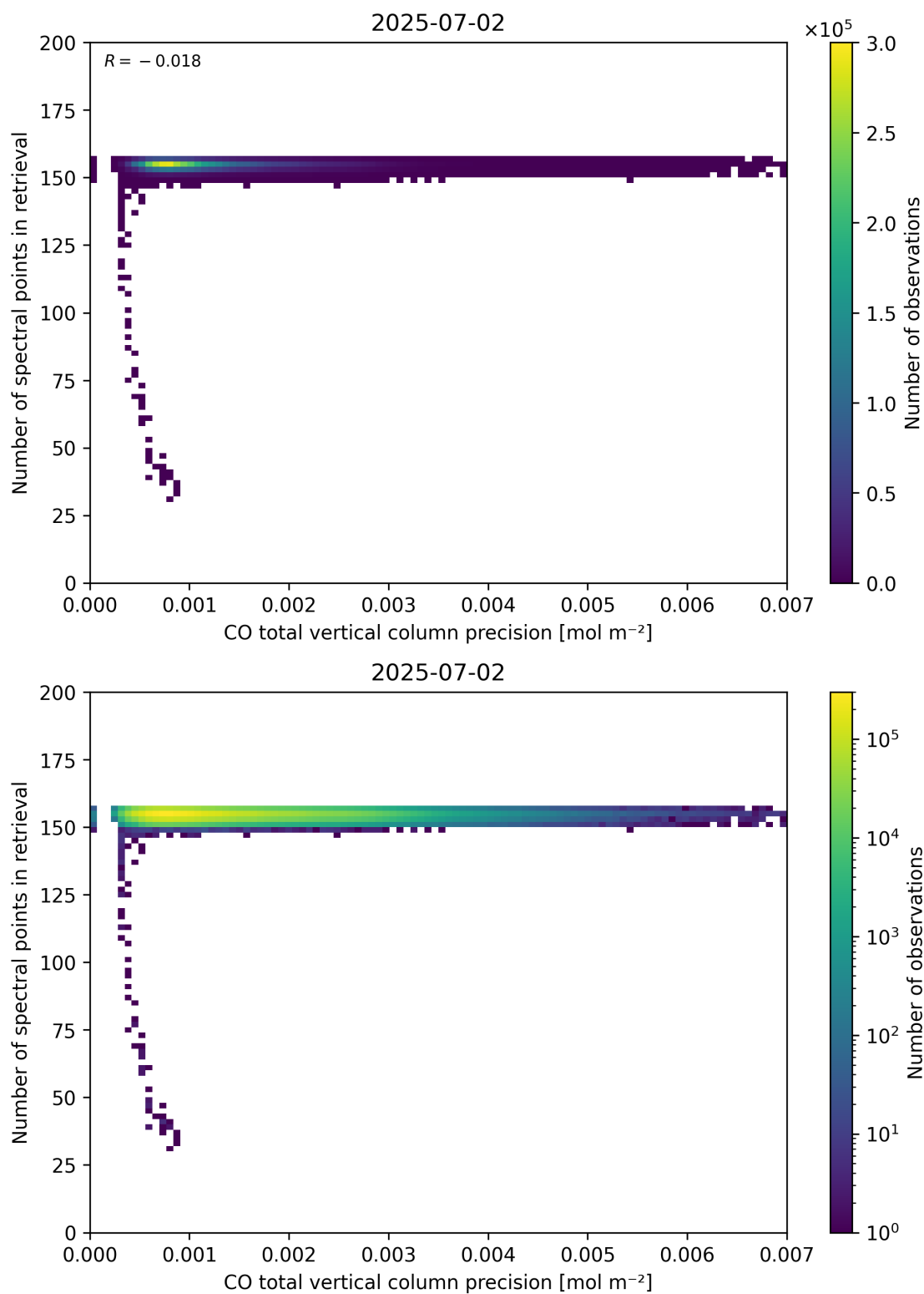
Figure 47: Scatter density plot of “CO total vertical column precision” against “Number of spectral points in retrieval” for 2025-07-02 to 2025-07-03.
