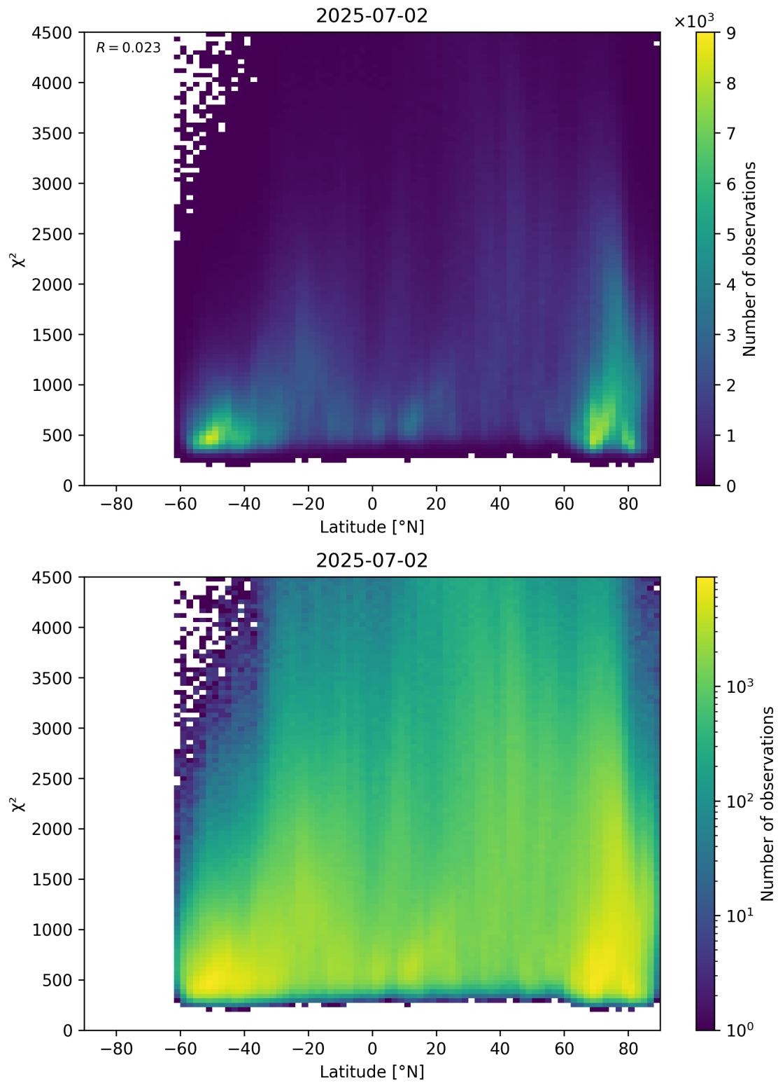
Figure 54: Scatter density plot of “Latitude” against “ \chi^2 ” for 2025-07-02 to 2025-07-03.
