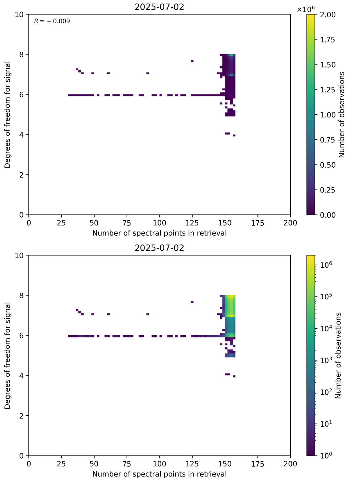
Figure 59: Scatter density plot of “Number of spectral points in retrieval” against “Degrees of freedom for signal” for 2025-07-02 to 2025-07-03.
