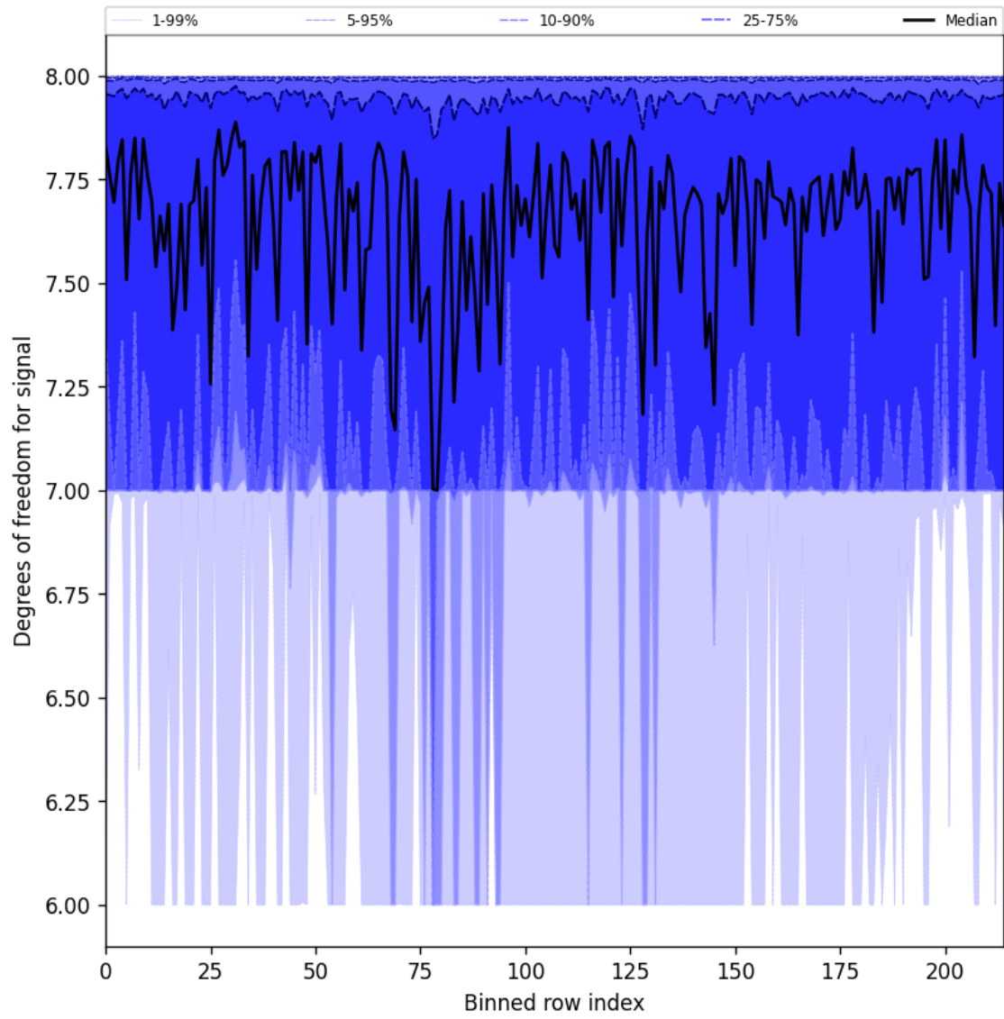
Figure 31: Along track statistics of “Degrees of freedom for signal” for 2025-07-02 to 2025-07-03
