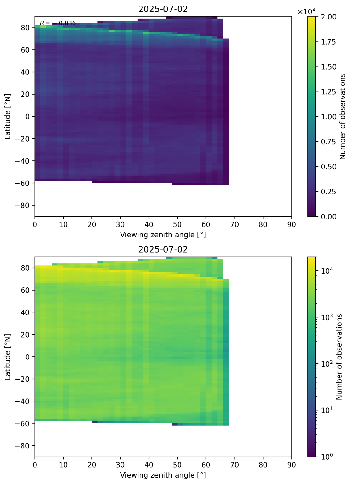
Figure 74: Scatter density plot of “Viewing zenith angle” against “Latitude” for 2025-07-02 to 2025-07-03.
