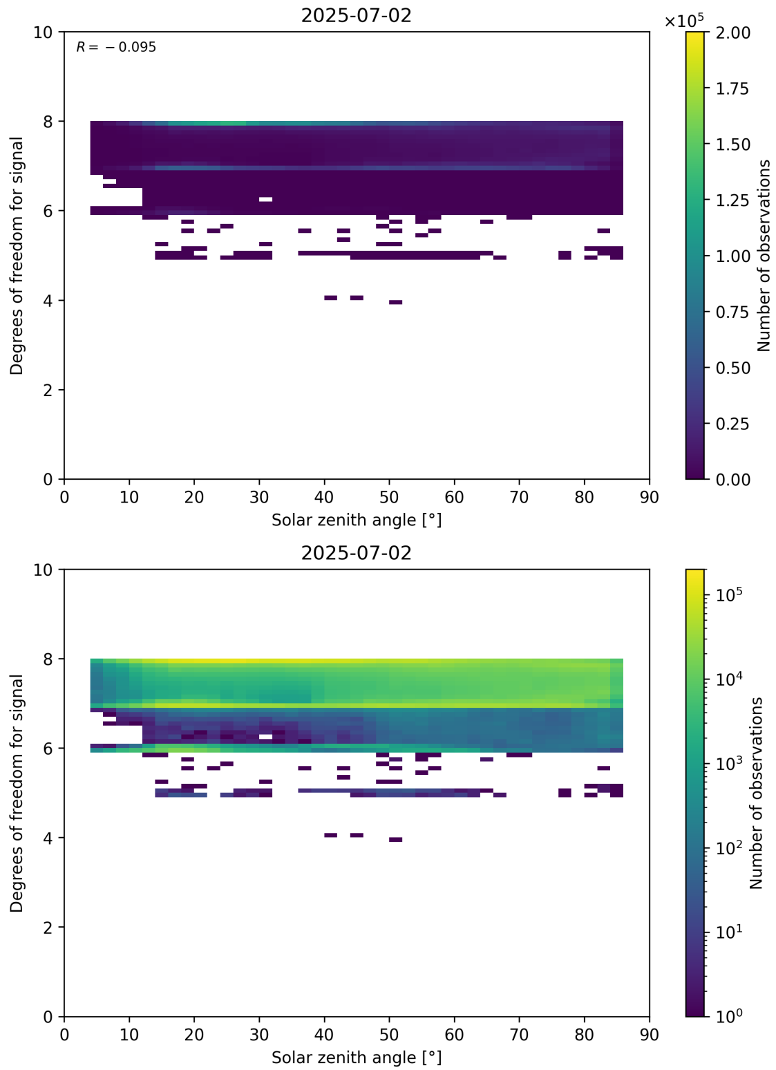
Figure 65: Scatter density plot of “Solar zenith angle” against “Degrees of freedom for signal” for 2025-07-02 to 2025-07-03.
