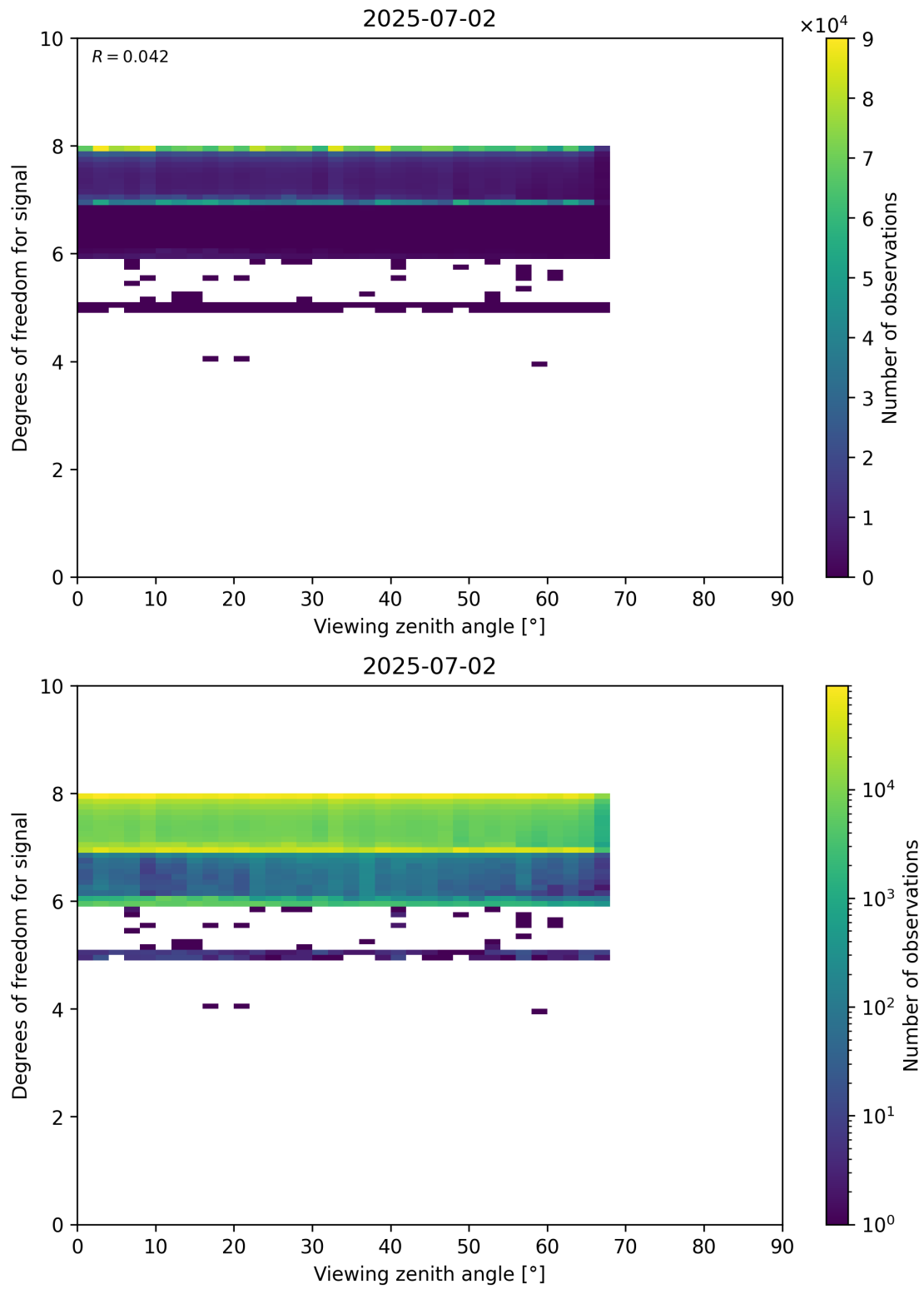
Figure 73: Scatter density plot of “Viewing zenith angle” against “Degrees of freedom for signal” for 2025-07-02 to 2025-07-03.
