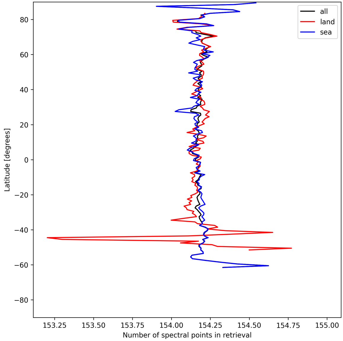
Figure 13: Zonal average of “Number of spectral points in retrieval” for 2025-07-02 to 2025-07-03.
