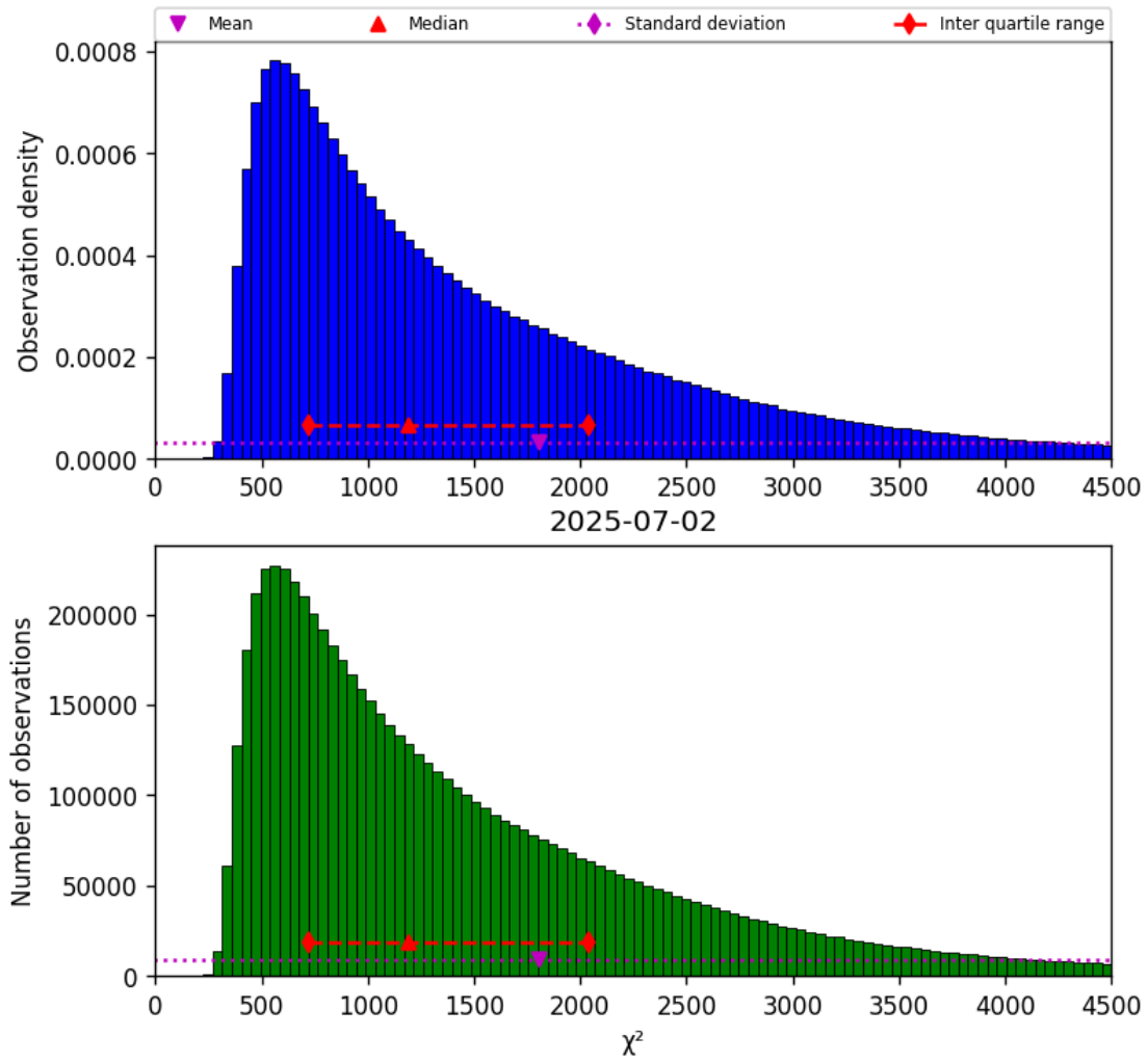
Figure 22: Histogram of " \chi^2 " for 2025-07-02 to 2025-07-03
