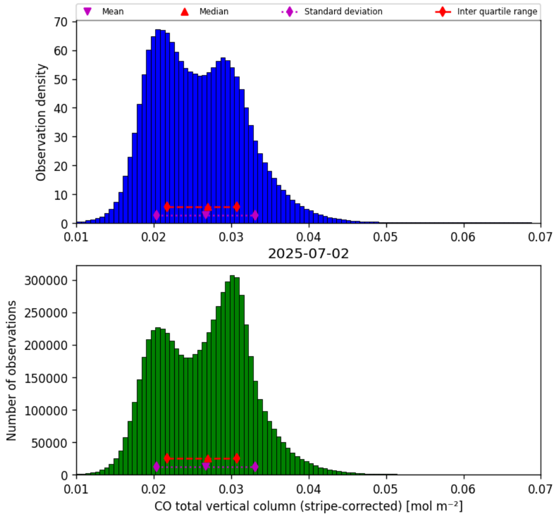
Figure 19: Histogram of “CO total vertical column (stripe-corrected)” for 2025-07-02 to 2025-07-03
