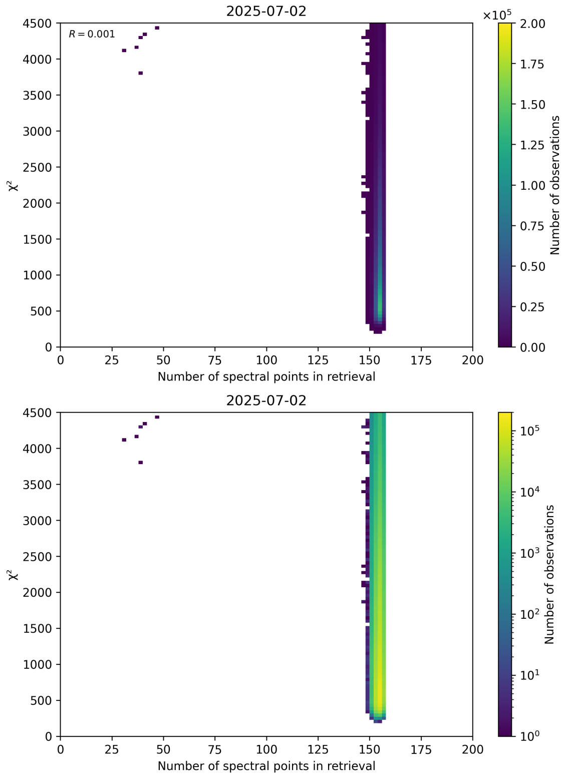
Figure 58: Scatter density plot of “Number of spectral points in retrieval” against “ \chi^2 ” for 2025-07-02 to 2025-07-03.
