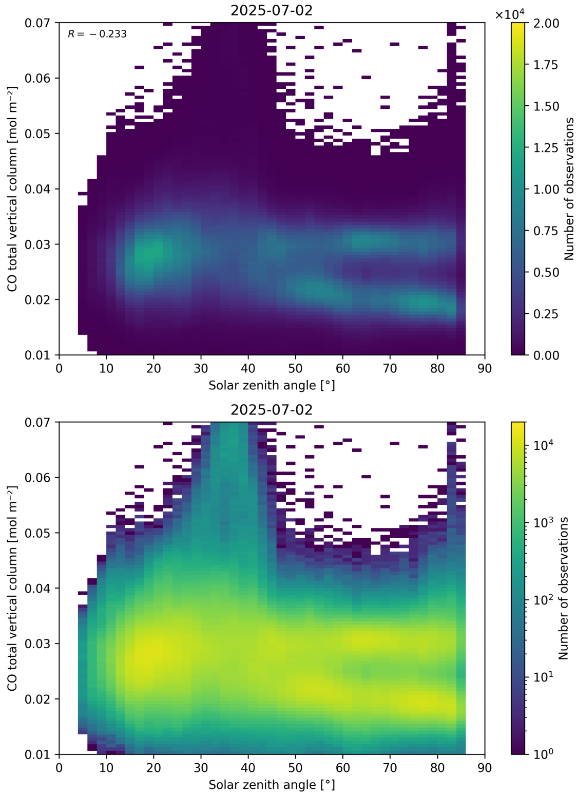
Figure 61: Scatter density plot of “Solar zenith angle” against “CO total vertical column” for 2025-07-02 to 2025-07-03.
