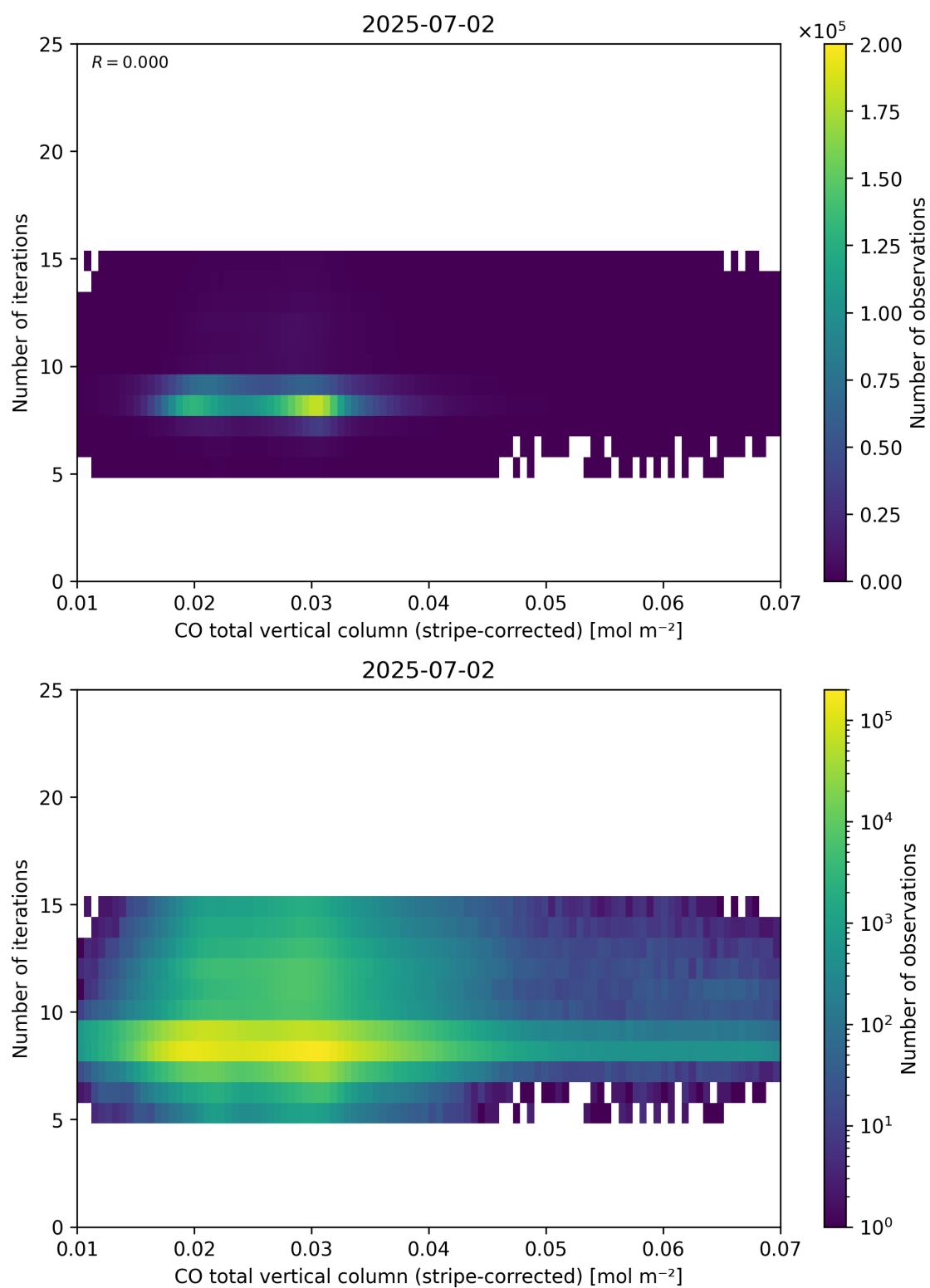
Figure 39: Scatter density plot of “CO total vertical column (stripe-corrected)” against “Number of iterations” for 2025-07-02 to 2025-07-03.
