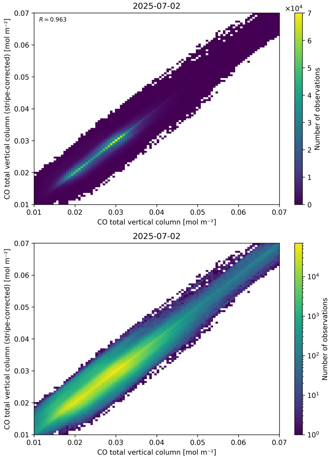
Figure 33: Scatter density plot of “CO total vertical column” against “CO total vertical column (stripe-corrected)” for 2025-07-02 to 2025-07-03.
