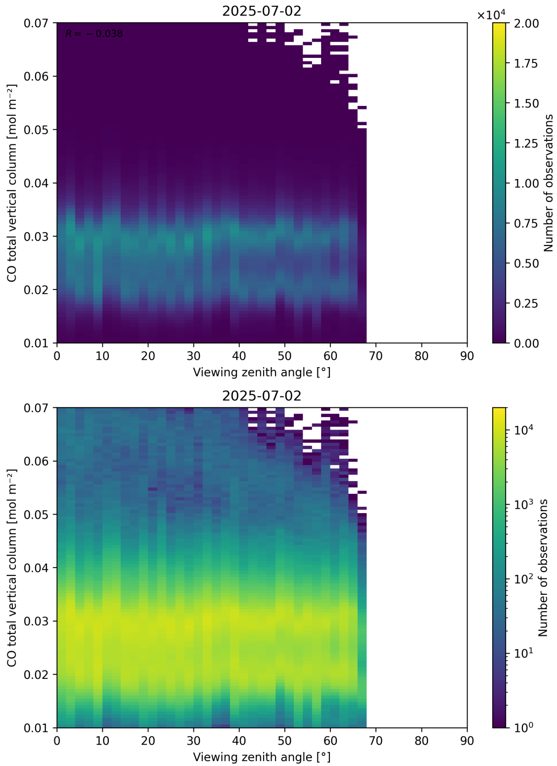
Figure 69: Scatter density plot of “Viewing zenith angle” against “CO total vertical column” for 2025-07-02 to 2025-07-03.
