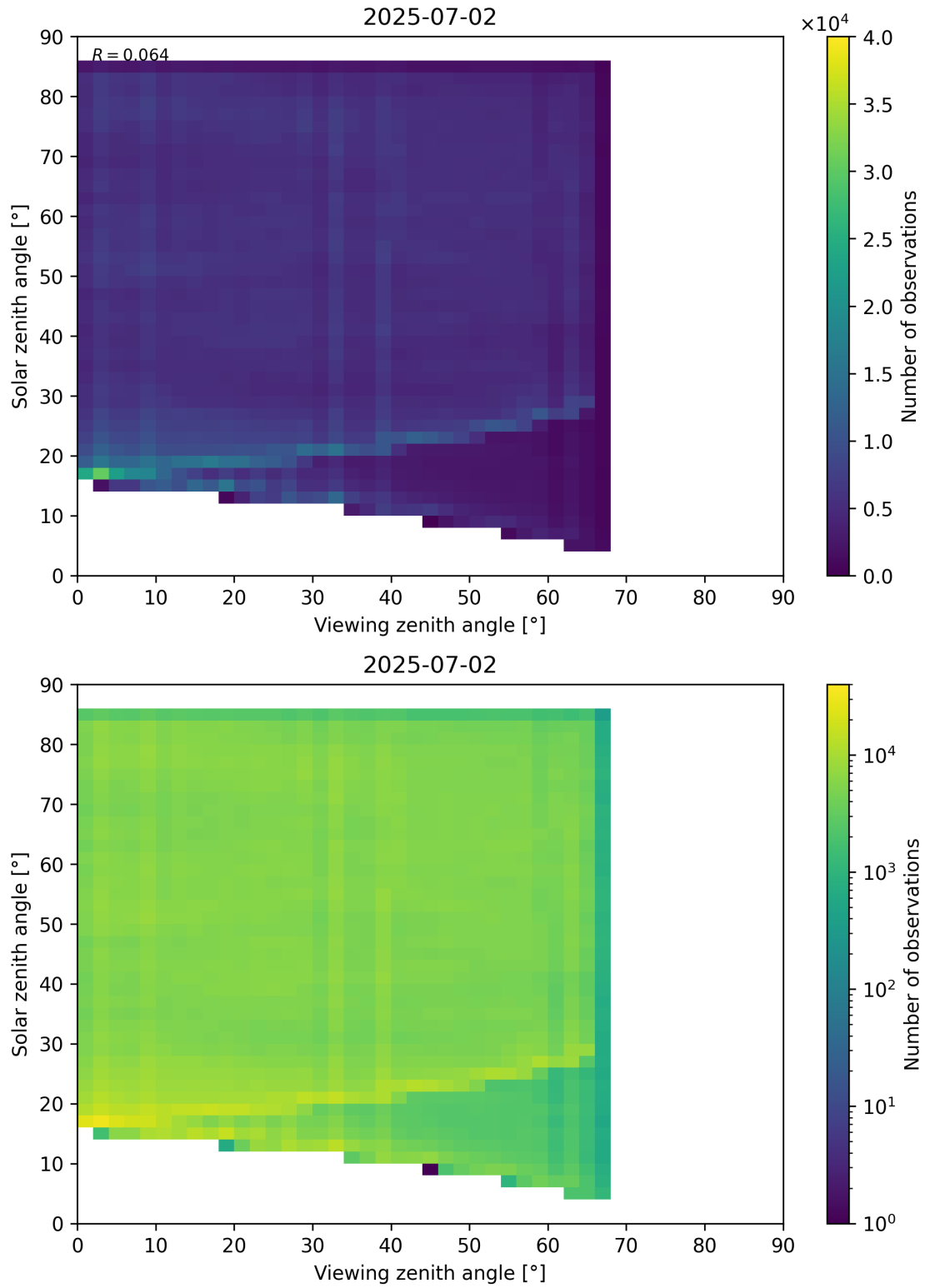
Figure 77: Scatter density plot of “Viewing zenith angle” against “Solar zenith angle” for 2025-07-02 to 2025-07-03.
