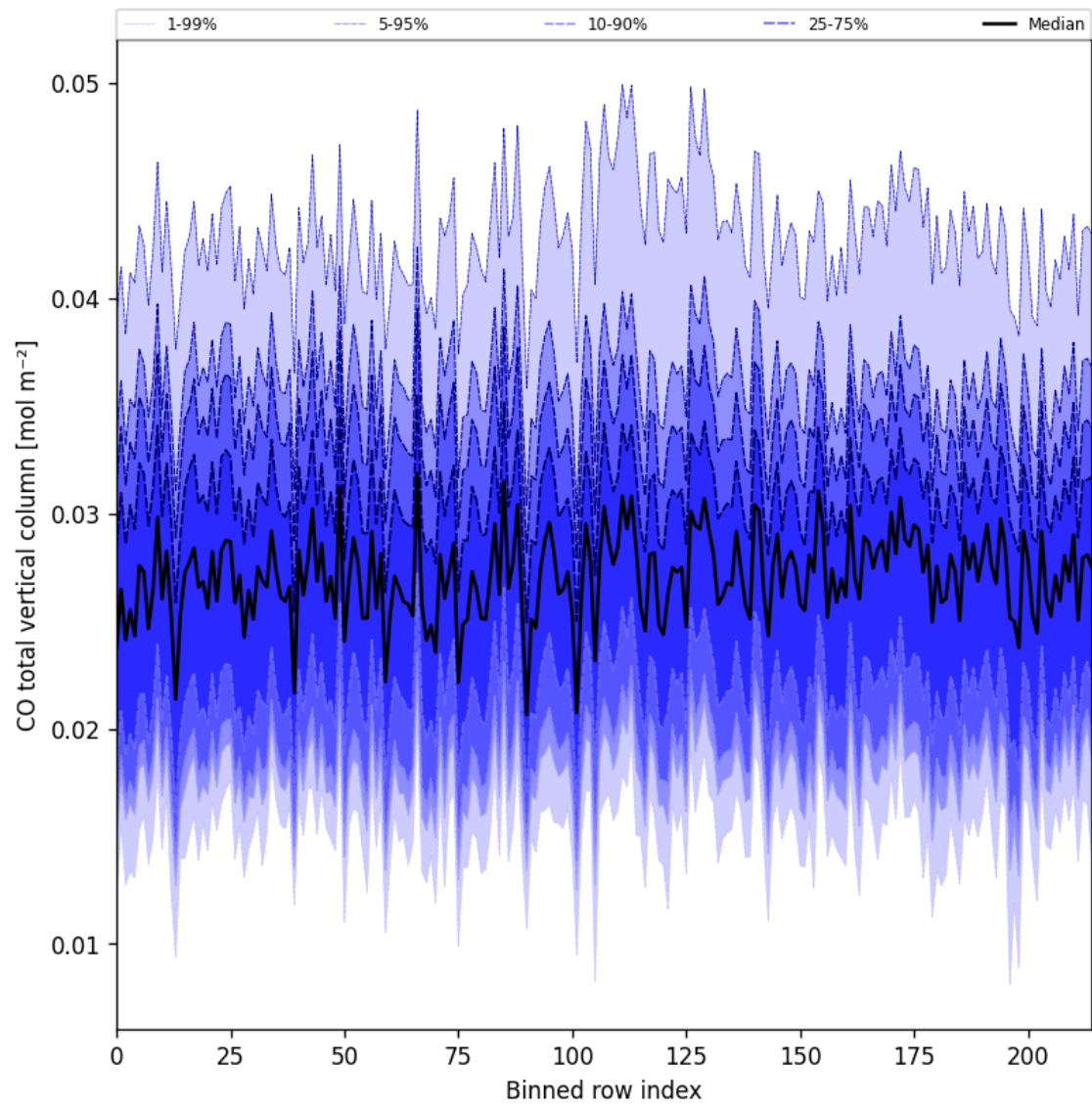
Figure 26: Along track statistics of "CO total vertical column" for 2025-07-02 to 2025-07-03
