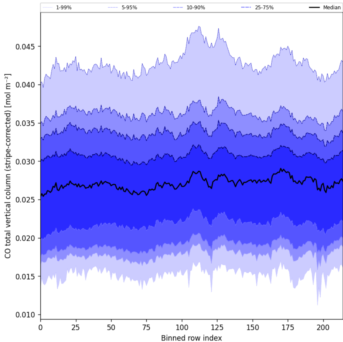
Figure 27: Along track statistics of “CO total vertical column (stripe-corrected)” for 2025-07-02 to 2025-07-03
