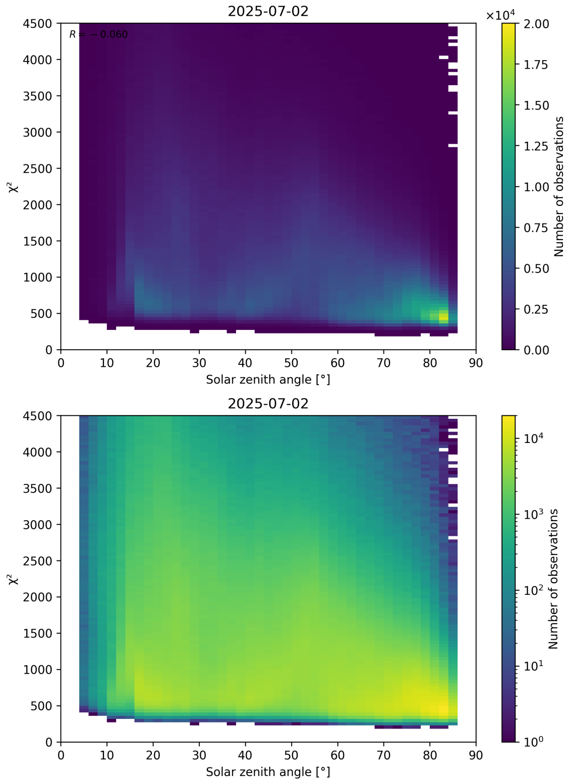
Figure 64: Scatter density plot of “Solar zenith angle” against “ \chi^2 ” for 2025-07-02 to 2025-07-03.
