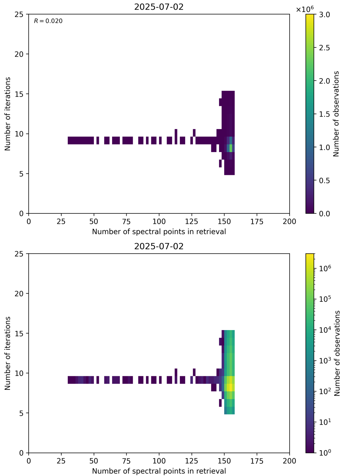
Figure 60: Scatter density plot of “Number of spectral points in retrieval” against “Number of iterations” for 2025-07-02 to 2025-07-03.
