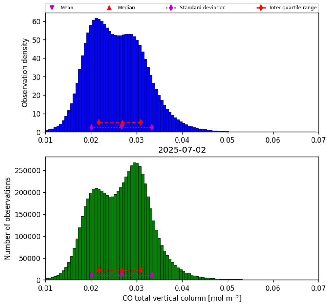
Figure 18: Histogram of “CO total vertical column” for 2025-07-02 to 2025-07-03
