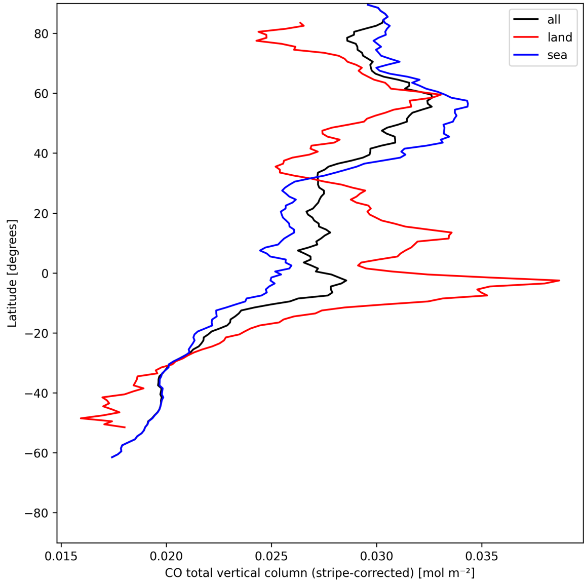
Figure 11: Zonal average of “CO total vertical column (stripe-corrected)” for 2025-07-02 to 2025-07-03.
