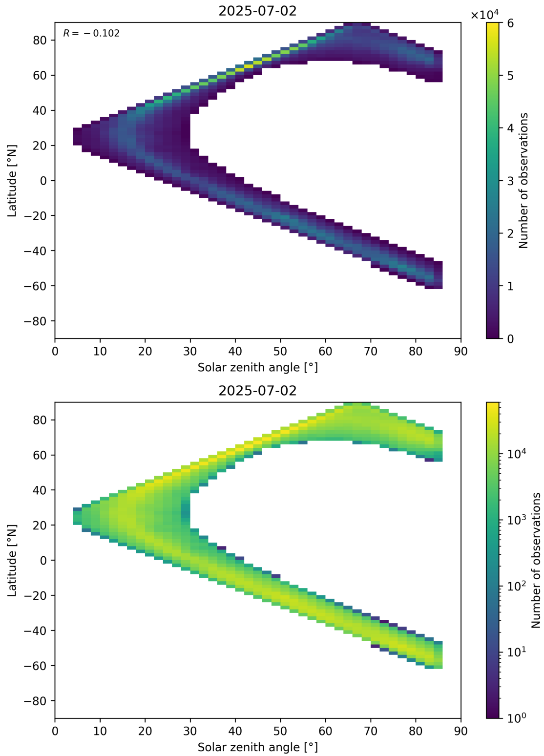
Figure 66: Scatter density plot of “Solar zenith angle” against “Latitude” for 2025-07-02 to 2025-07-03.
