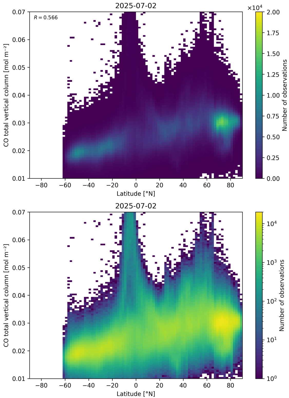
Figure 51: Scatter density plot of “Latitude” against “CO total vertical column” for 2025-07-02 to 2025-07-03.
