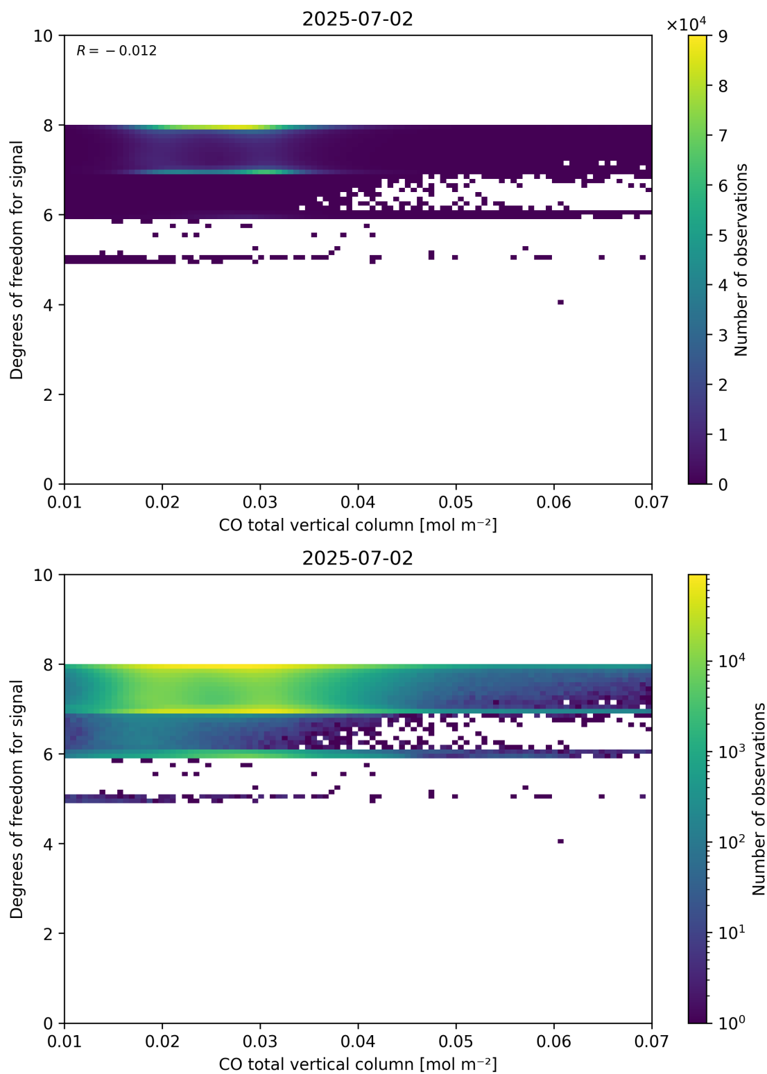
Figure 41: Scatter density plot of “CO total vertical column” against “Degrees of freedom for signal” for 2025-07-02 to 2025-07-03.
