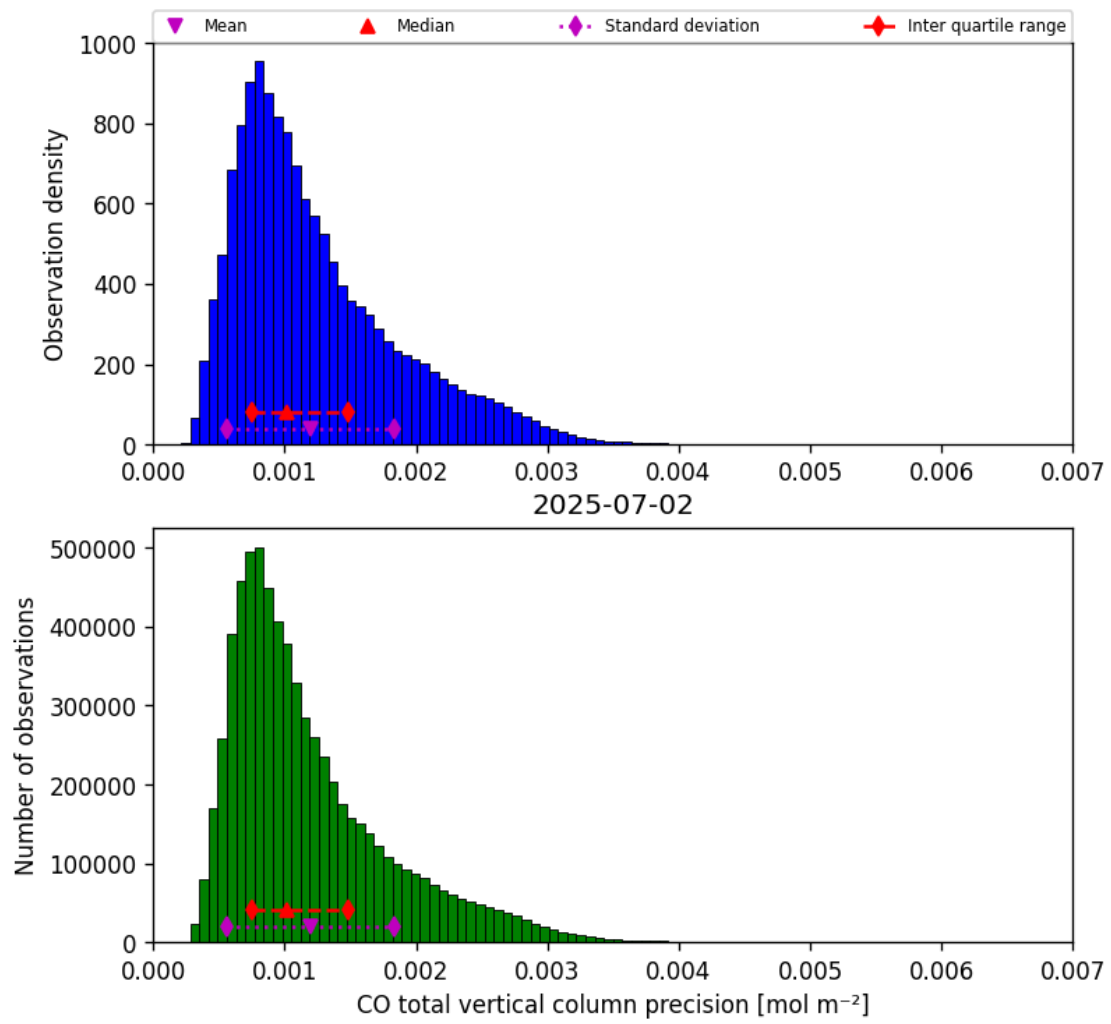
Figure 20: Histogram of “CO total vertical column precision” for 2025-07-02 to 2025-07-03
