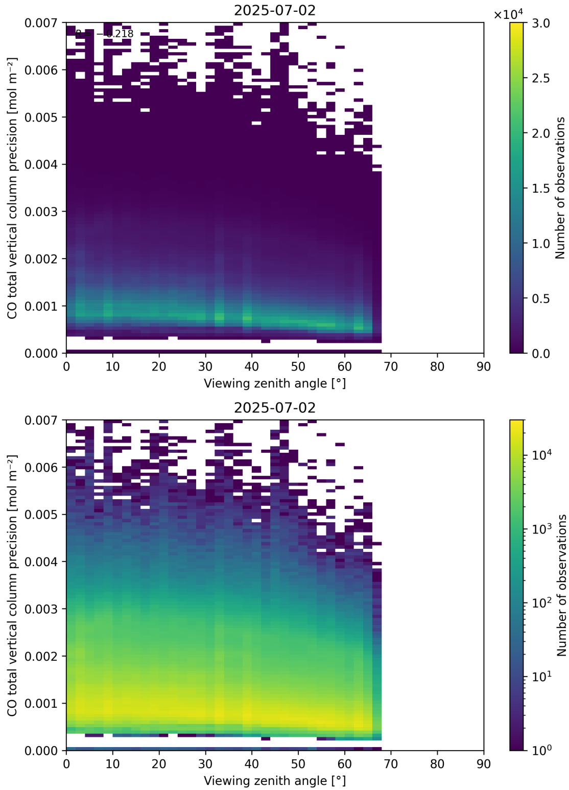
Figure 71: Scatter density plot of “Viewing zenith angle” against “CO total vertical column precision” for 2025-07-02 to 2025-07-03.
