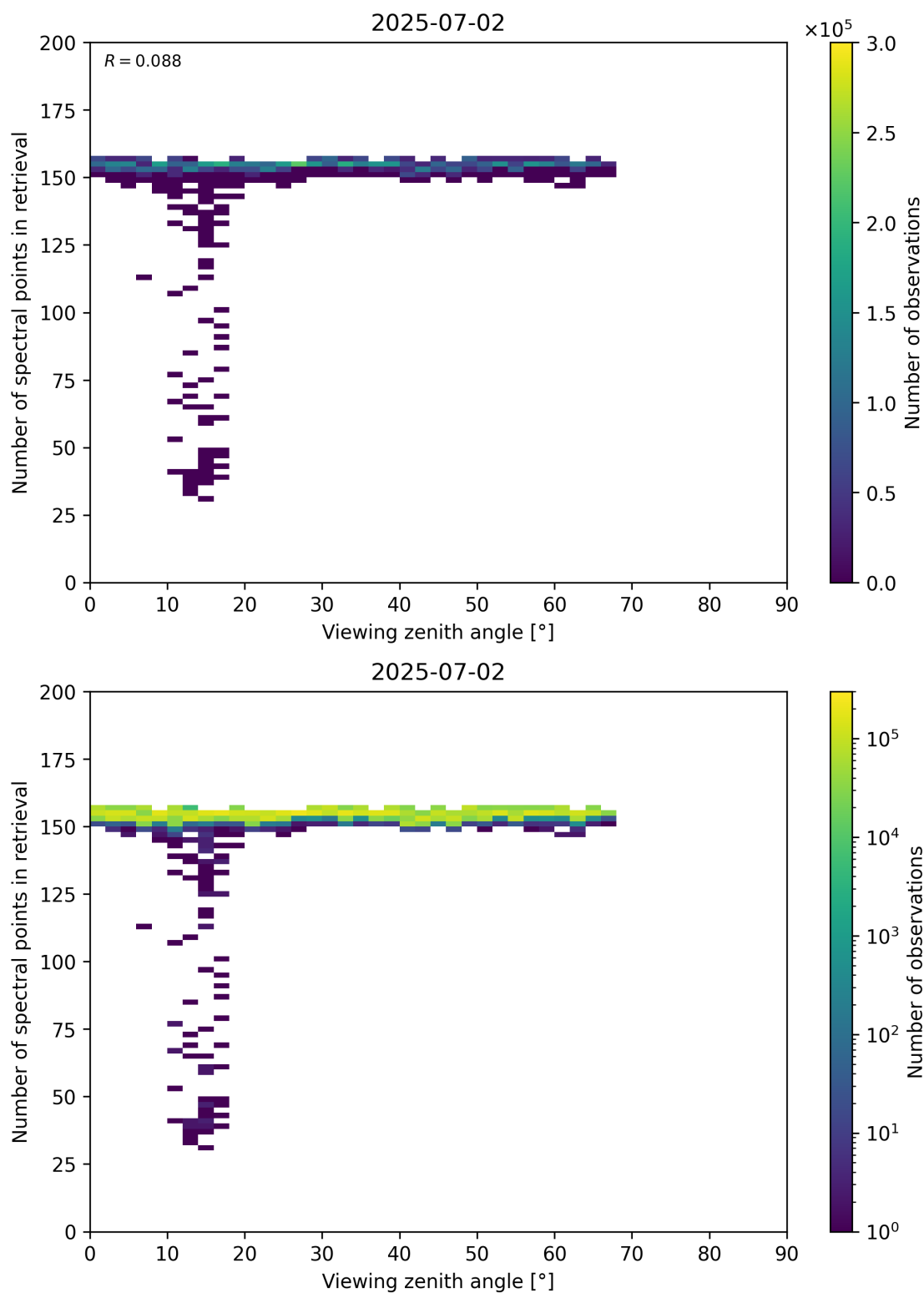
Figure 76: Scatter density plot of “Viewing zenith angle” against “Number of spectral points in retrieval” for 2025-07-02 to 2025-07-03.
