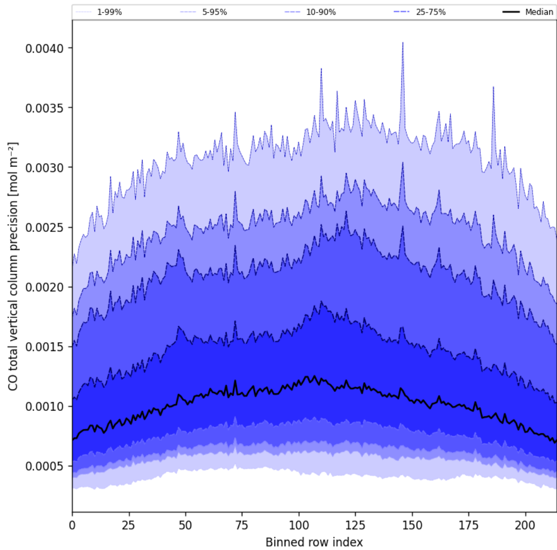
Figure 28: Along track statistics of “CO total vertical column precision” for 2025-07-02 to 2025-07-03
