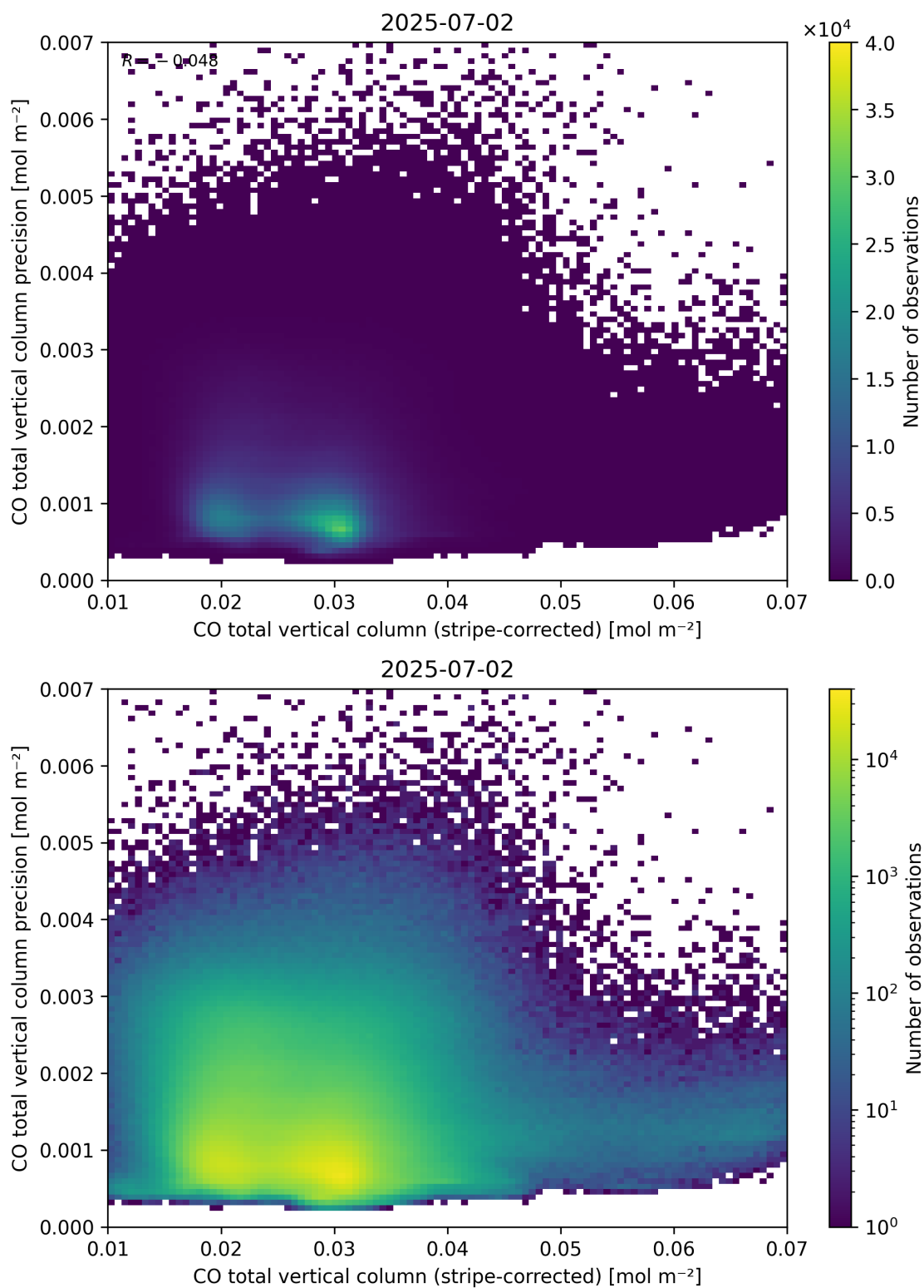
Figure 36: Scatter density plot of “CO total vertical column (stripe-corrected)” against “CO total vertical column precision” for 2025-07-02 to 2025-07-03.
