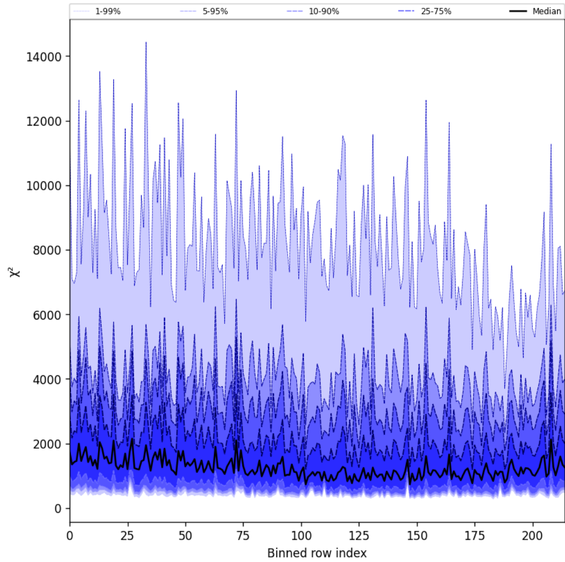
Figure 30: Along track statistics of “ \chi^2 ” for 2025-07-02 to 2025-07-03
