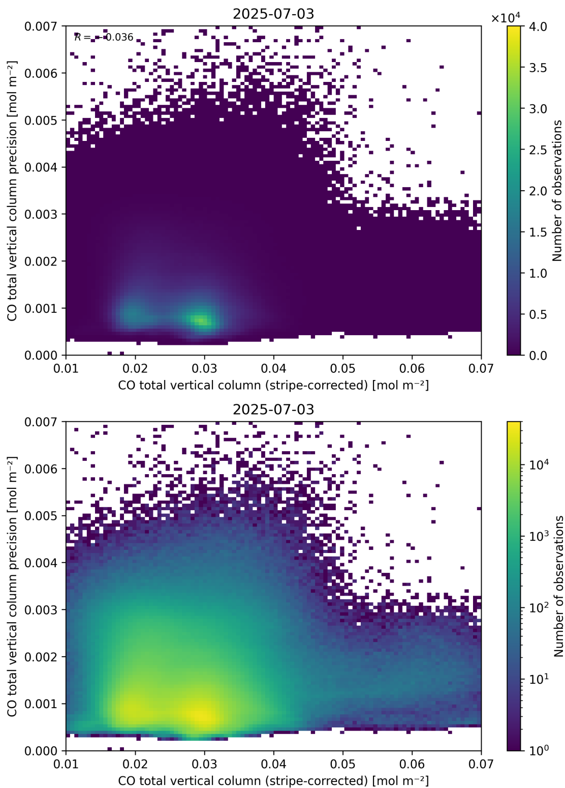
Figure 36: Scatter density plot of “CO total vertical column (stripe-corrected)” against “CO total vertical column precision” for 2025-07-03 to 2025-07-04.
