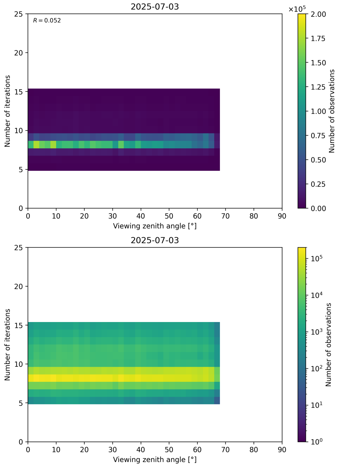
Figure 75: Scatter density plot of “Viewing zenith angle” against “Number of iterations” for 2025-07-03 to 2025-07-04.
