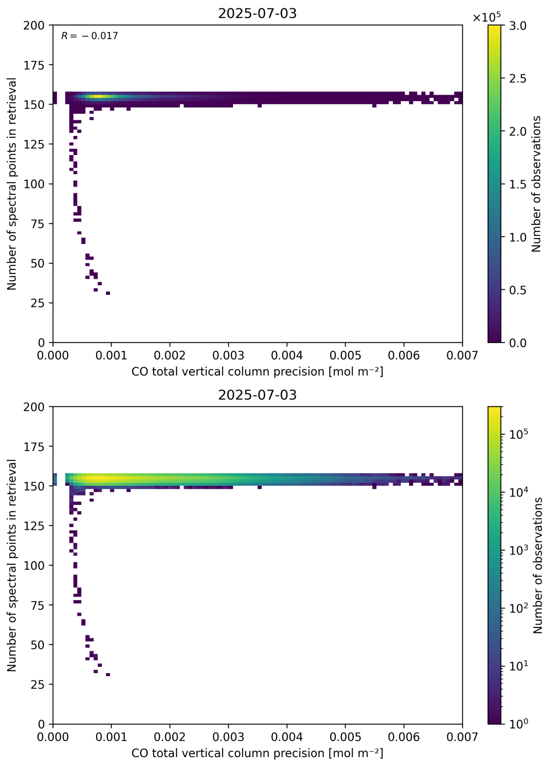
Figure 47: Scatter density plot of “CO total vertical column precision” against “Number of spectral points in retrieval” for 2025-07-03 to 2025-07-04.
