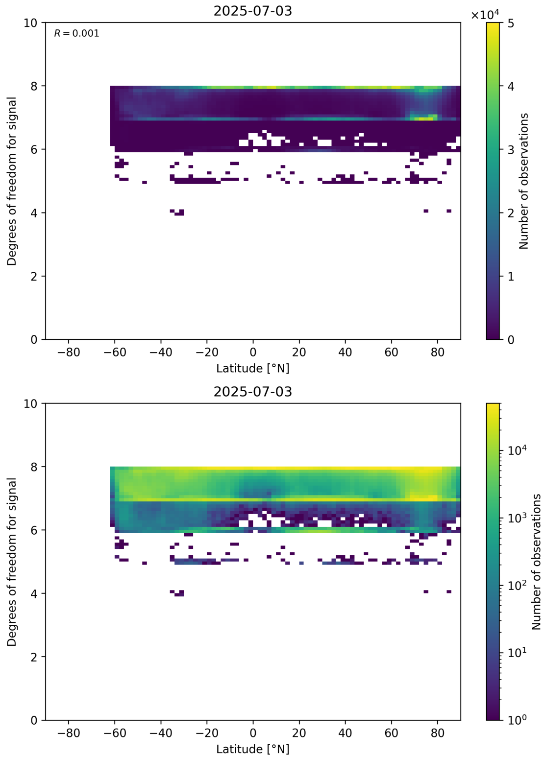
Figure 55: Scatter density plot of “Latitude” against “Degrees of freedom for signal” for 2025-07-03 to 2025-07-04.
