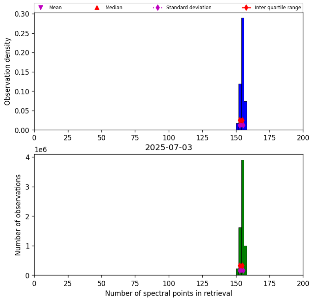
Figure 21: Histogram of “Number of spectral points in retrieval” for 2025-07-03 to 2025-07-04
