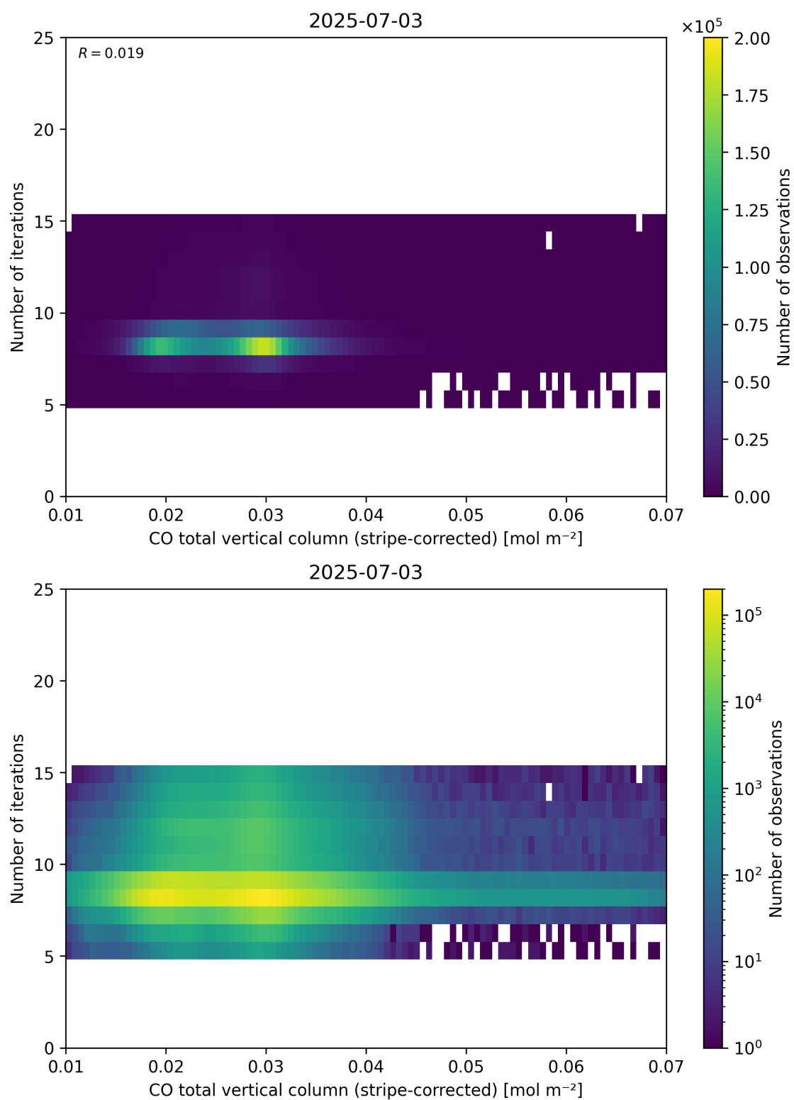
Figure 39: Scatter density plot of “CO total vertical column (stripe-corrected)” against “Number of iterations” for 2025-07-03 to 2025-07-04.
