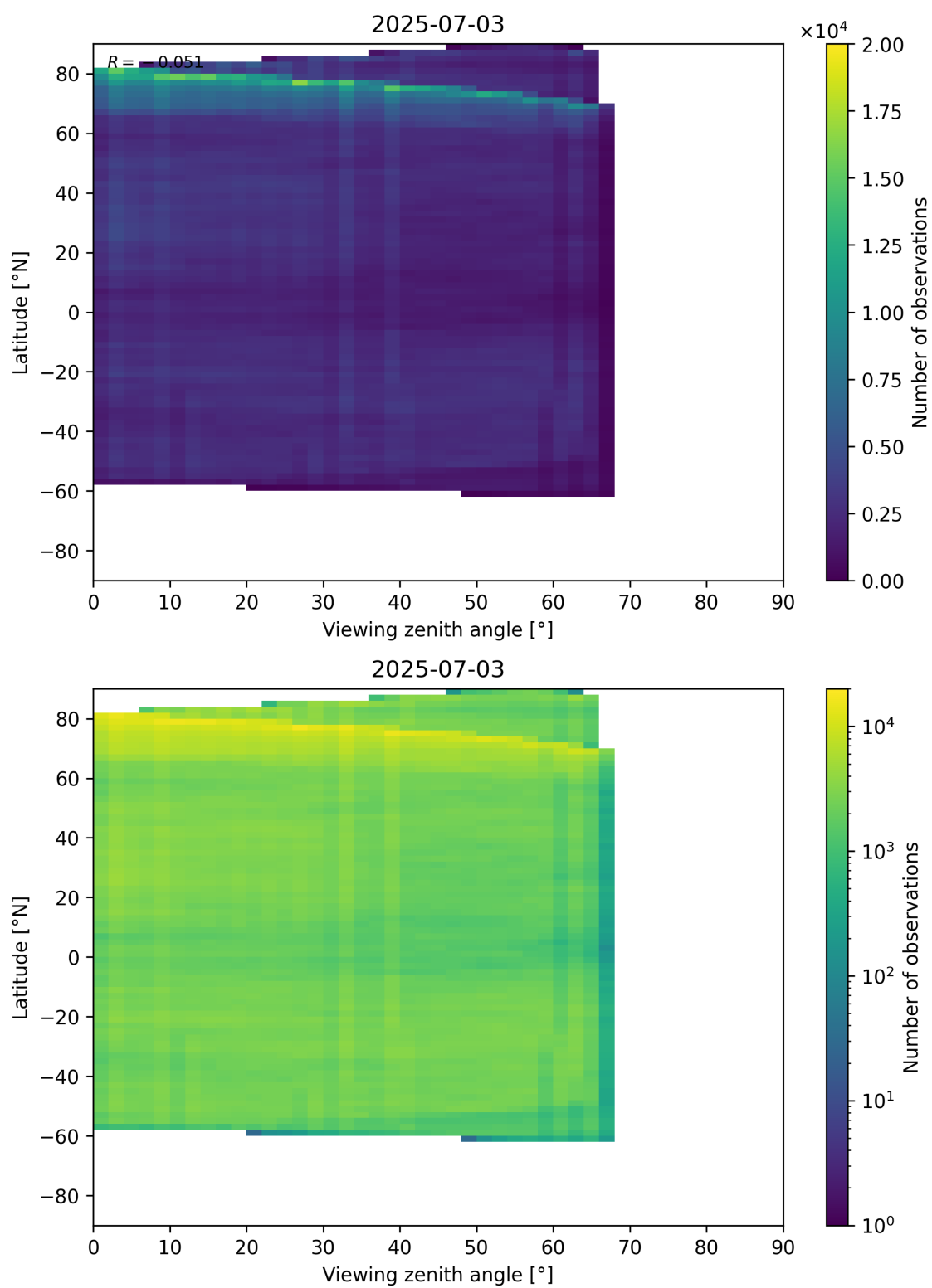
Figure 74: Scatter density plot of “Viewing zenith angle” against “Latitude” for 2025-07-03 to 2025-07-04.
