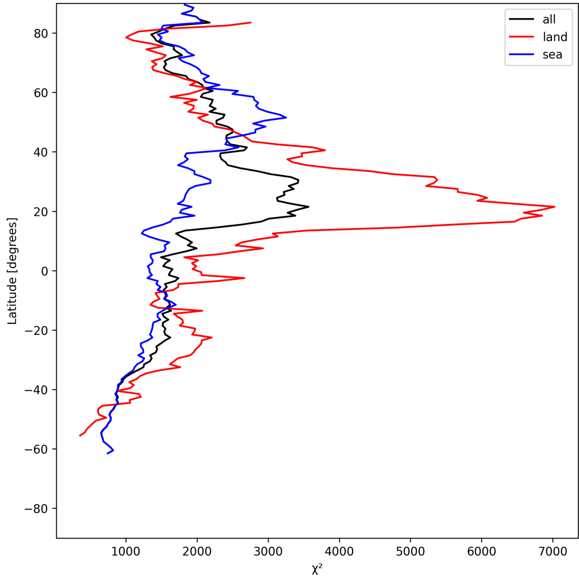
Figure 14: Zonal average of “ \chi^2 ” for 2025-07-03 to 2025-07-04.
