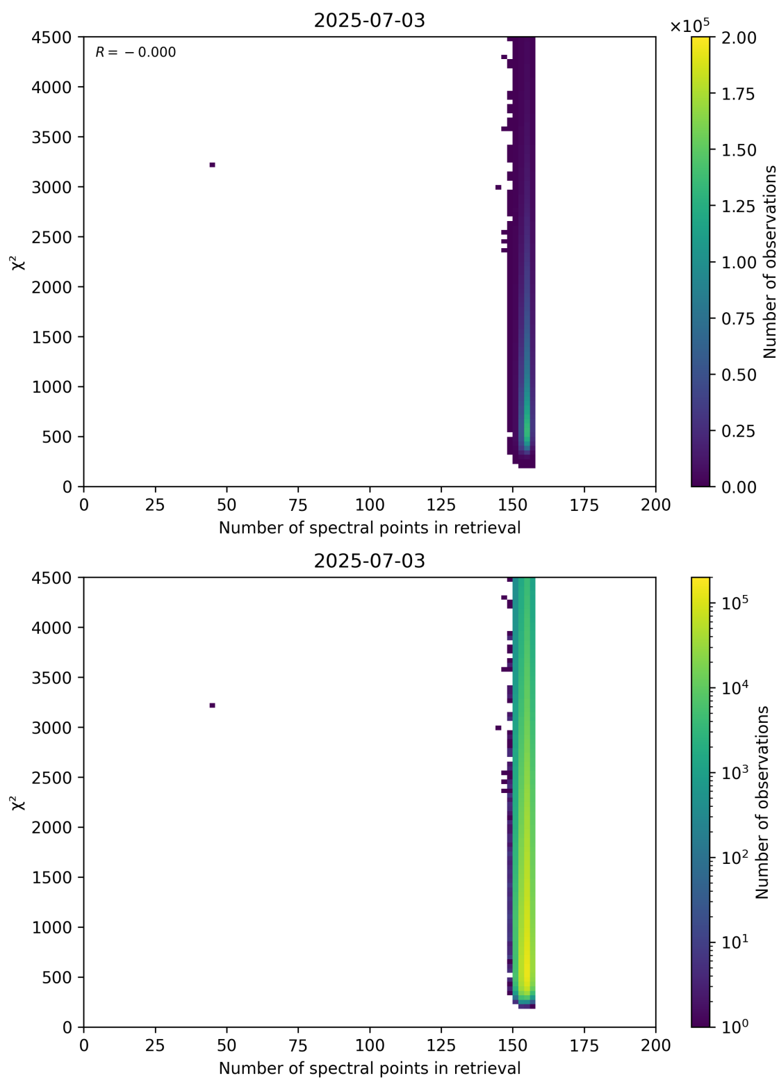
Figure 58: Scatter density plot of “Number of spectral points in retrieval” against “ \chi^2 ” for 2025-07-03 to 2025-07-04.
