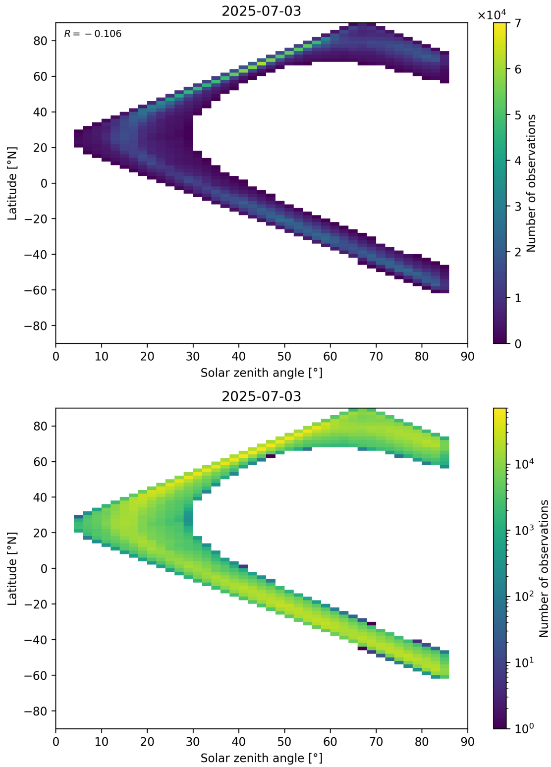
Figure 66: Scatter density plot of “Solar zenith angle” against “Latitude” for 2025-07-03 to 2025-07-04.
