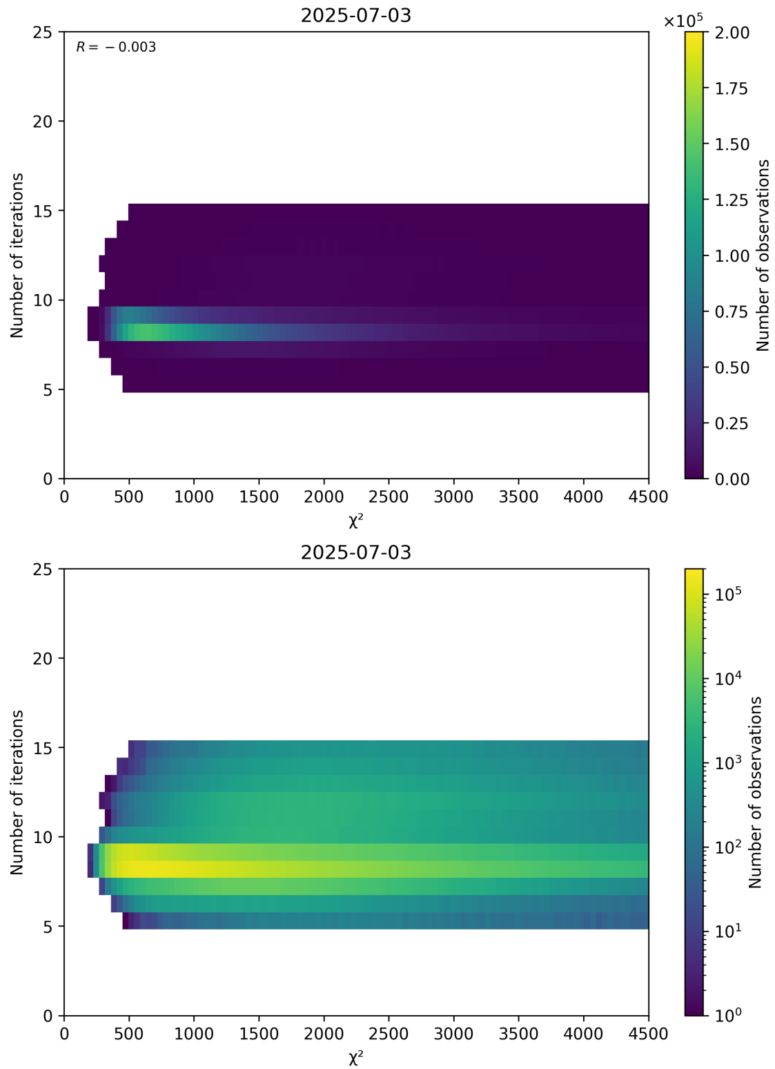
Figure 49: Scatter density plot of “ \chi^2 ” against “Number of iterations” for 2025-07-03 to 2025-07-04.
