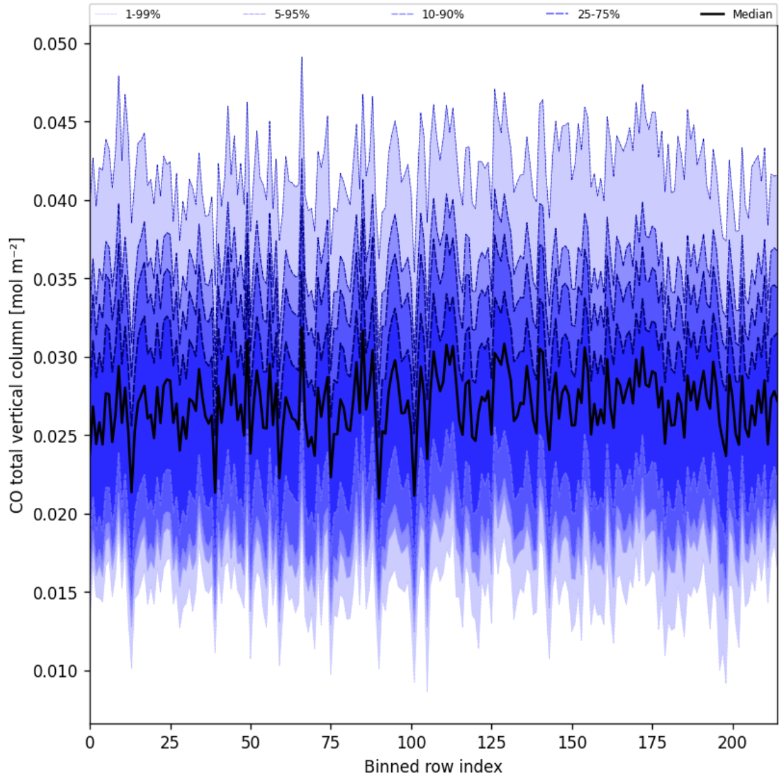
Figure 26: Along track statistics of “CO total vertical column” for 2025-07-03 to 2025-07-04
