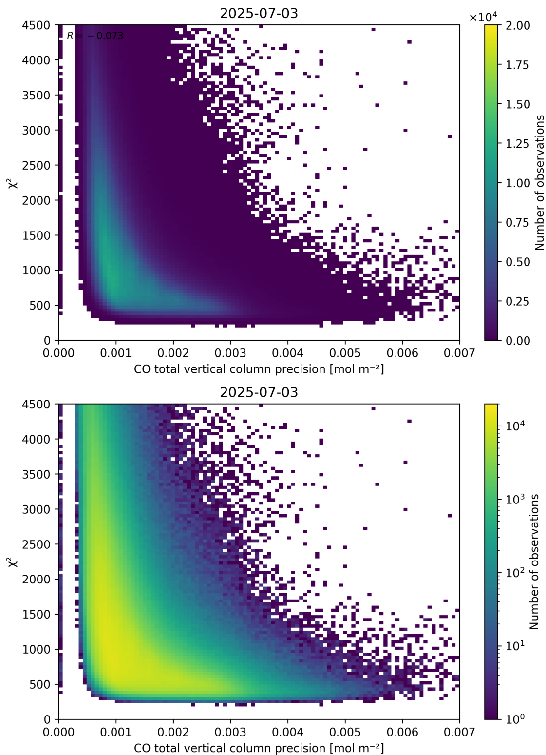
Figure 44: Scatter density plot of “CO total vertical column precision” against “ \chi^2 ” for 2025-07-03 to 2025-07-04.
