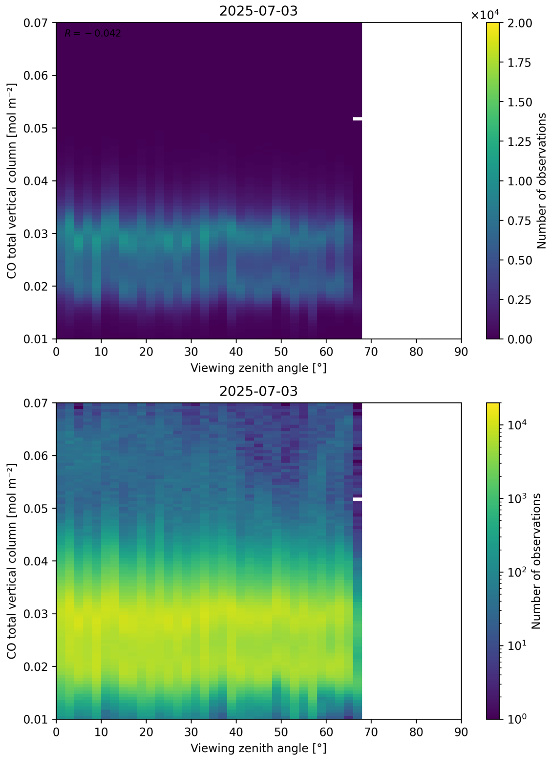
Figure 69: Scatter density plot of “Viewing zenith angle” against “CO total vertical column” for 2025-07-03 to 2025-07-04.
