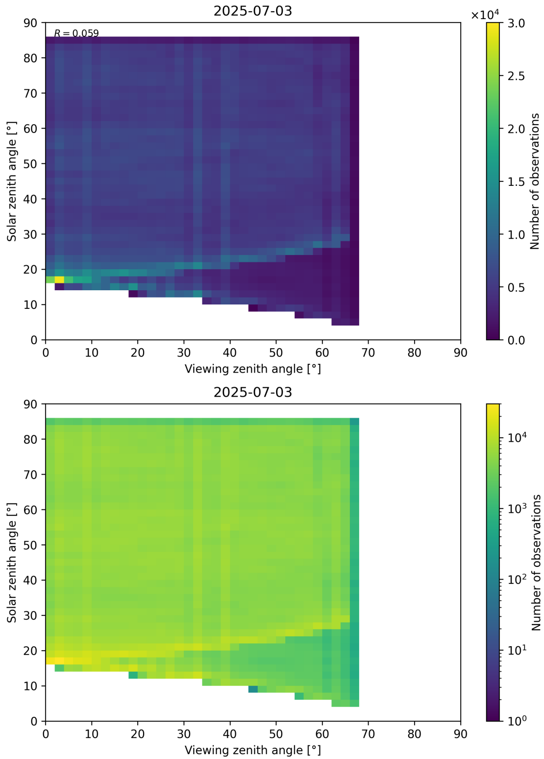
Figure 77: Scatter density plot of “Viewing zenith angle” against “Solar zenith angle” for 2025-07-03 to 2025-07-04.
