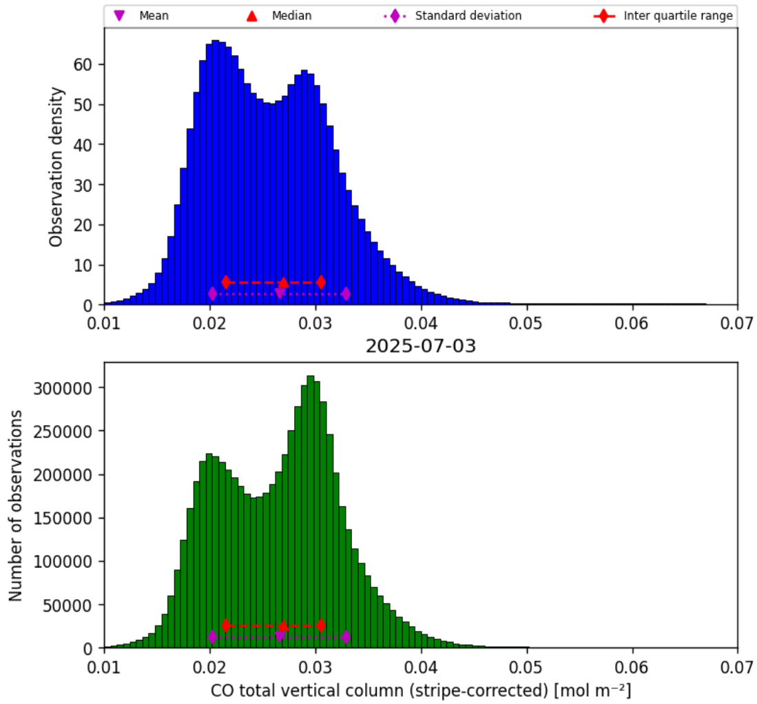
Figure 19: Histogram of “CO total vertical column (stripe-corrected)” for 2025-07-03 to 2025-07-04
