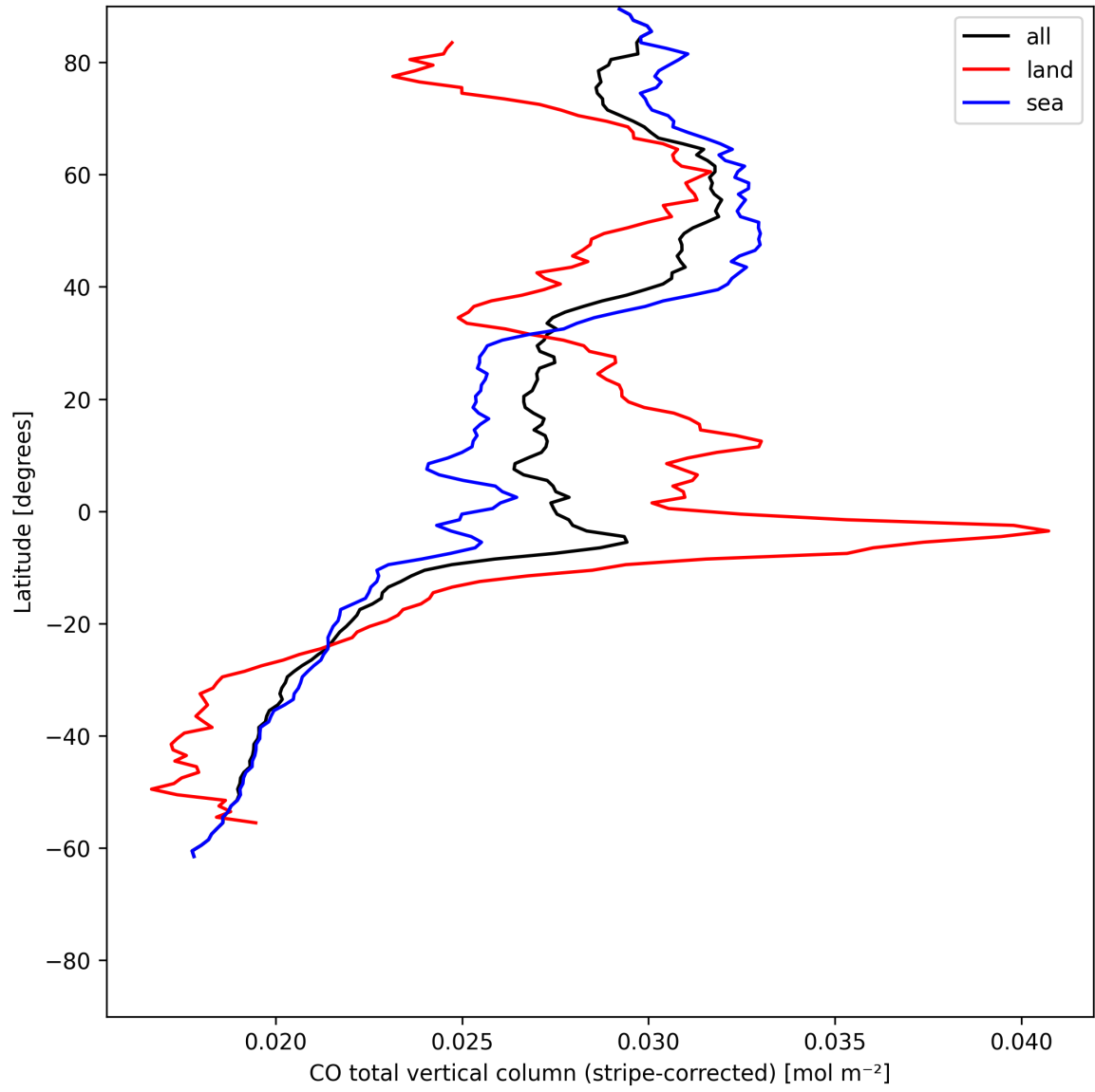
Figure 11: Zonal average of “CO total vertical column (stripe-corrected)” for 2025-07-03 to 2025-07-04.
