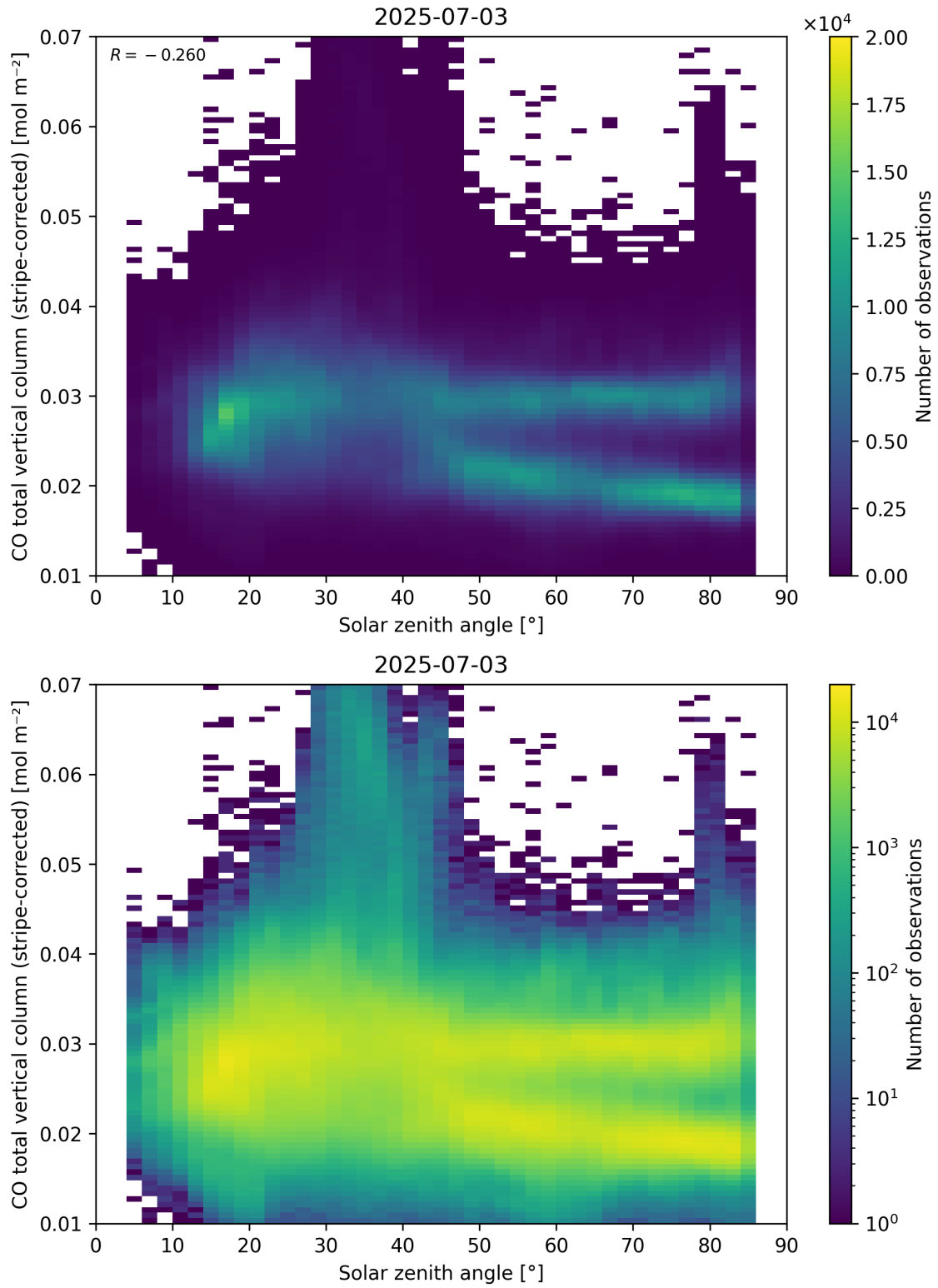
Figure 62: Scatter density plot of “Solar zenith angle” against “CO total vertical column (stripe-corrected)” for 2025-07-03 to 2025-07-04.
