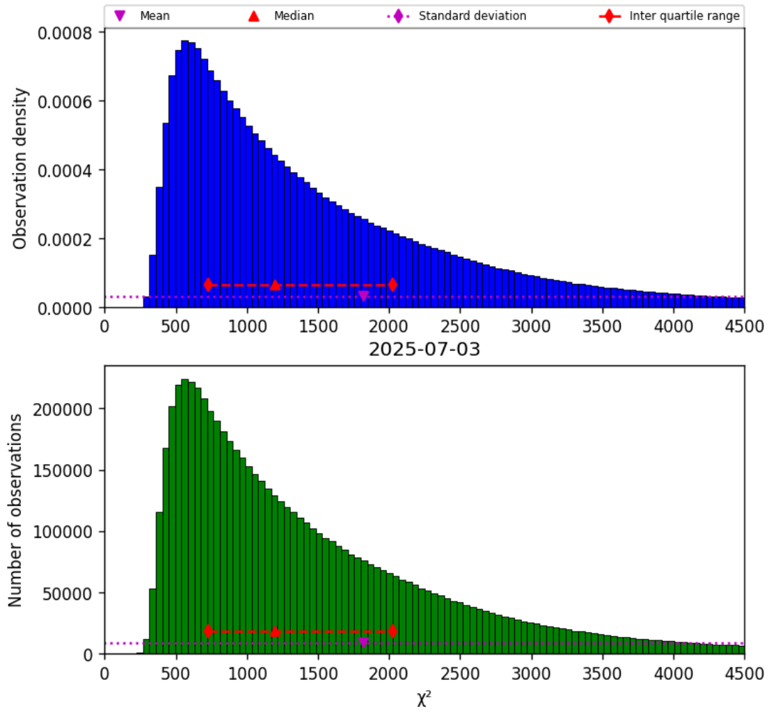
Figure 22: Histogram of “ \chi^2 ” for 2025-07-03 to 2025-07-04
