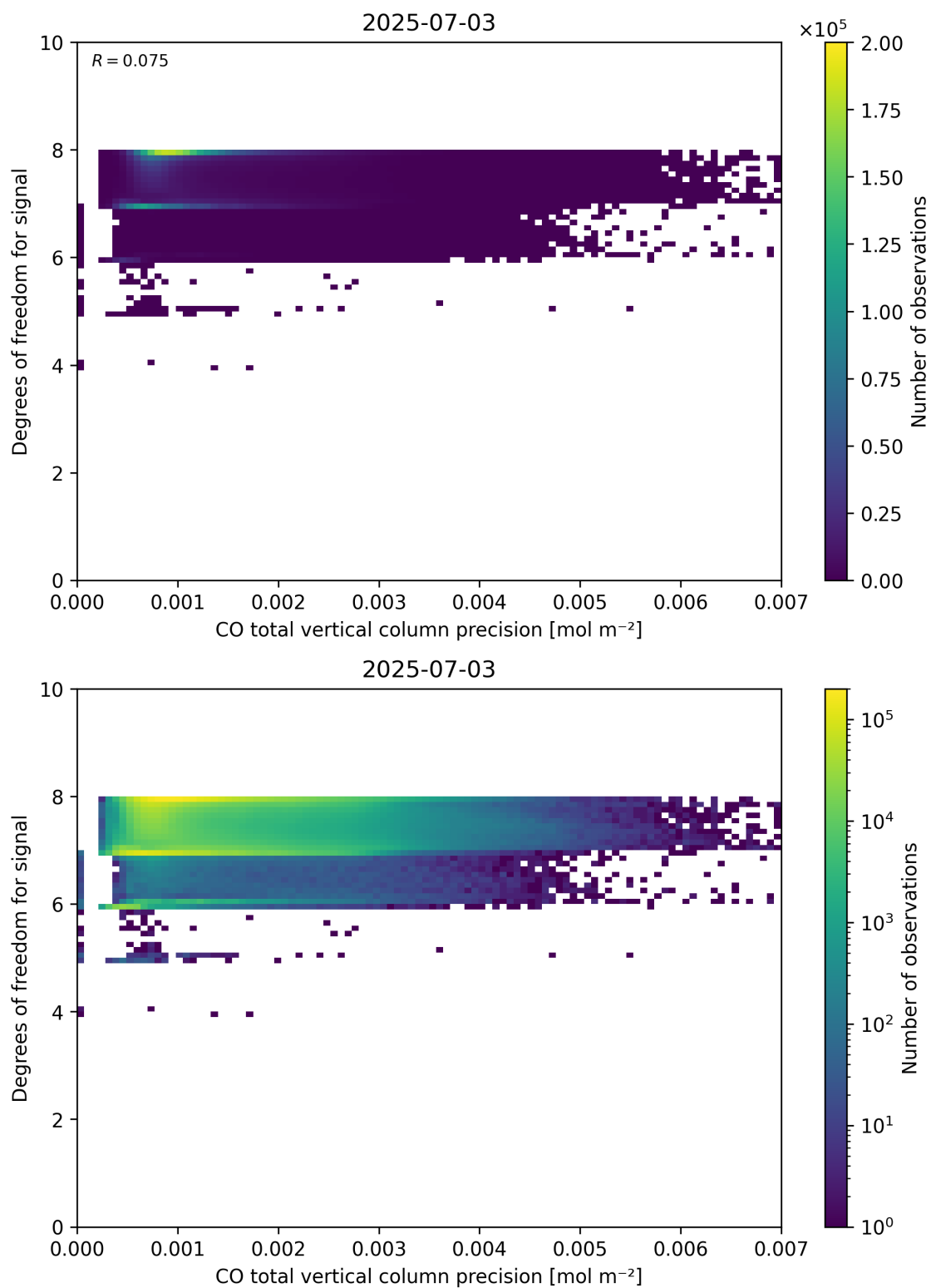
Figure 45: Scatter density plot of “CO total vertical column precision” against “Degrees of freedom for signal” for 2025-07-03 to 2025-07-04.
