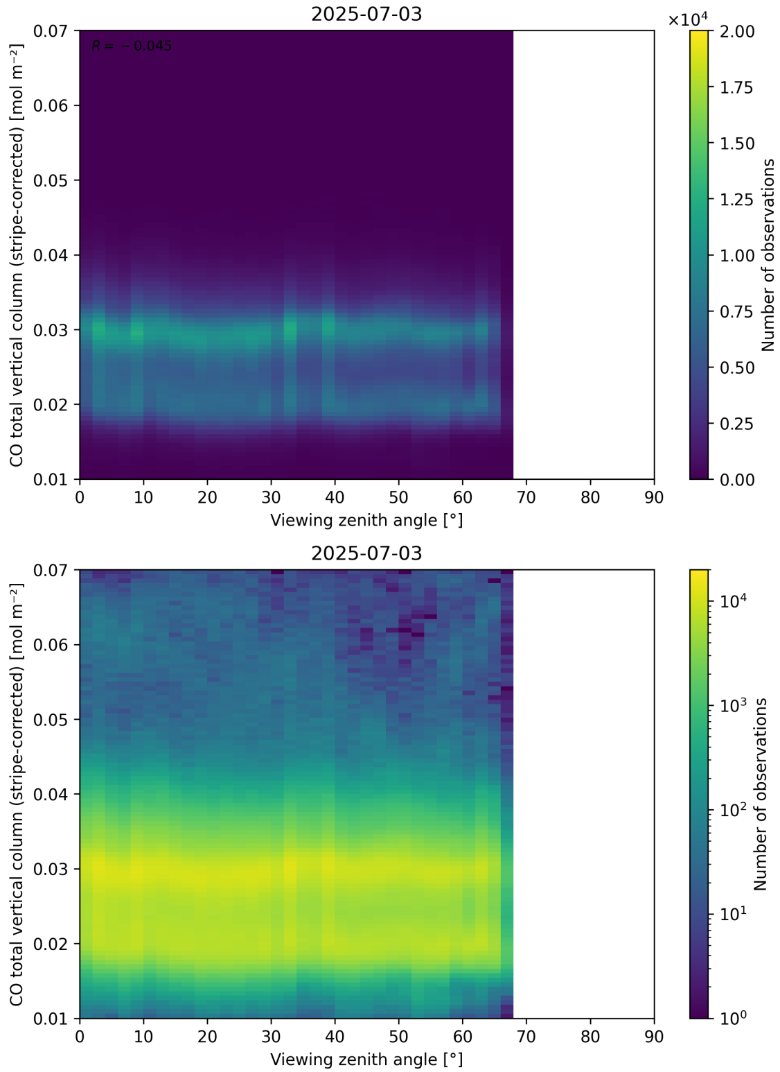
Figure 70: Scatter density plot of “Viewing zenith angle” against “CO total vertical column (stripe-corrected)” for 2025-07-03 to 2025-07-04.
