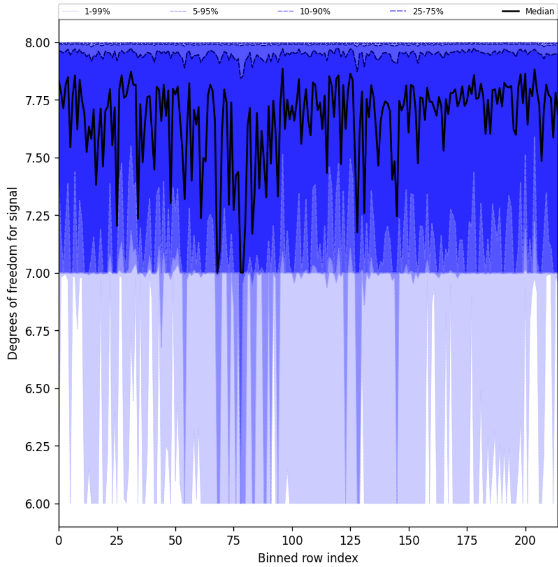
Figure 31: Along track statistics of “Degrees of freedom for signal” for 2025-07-03 to 2025-07-04
