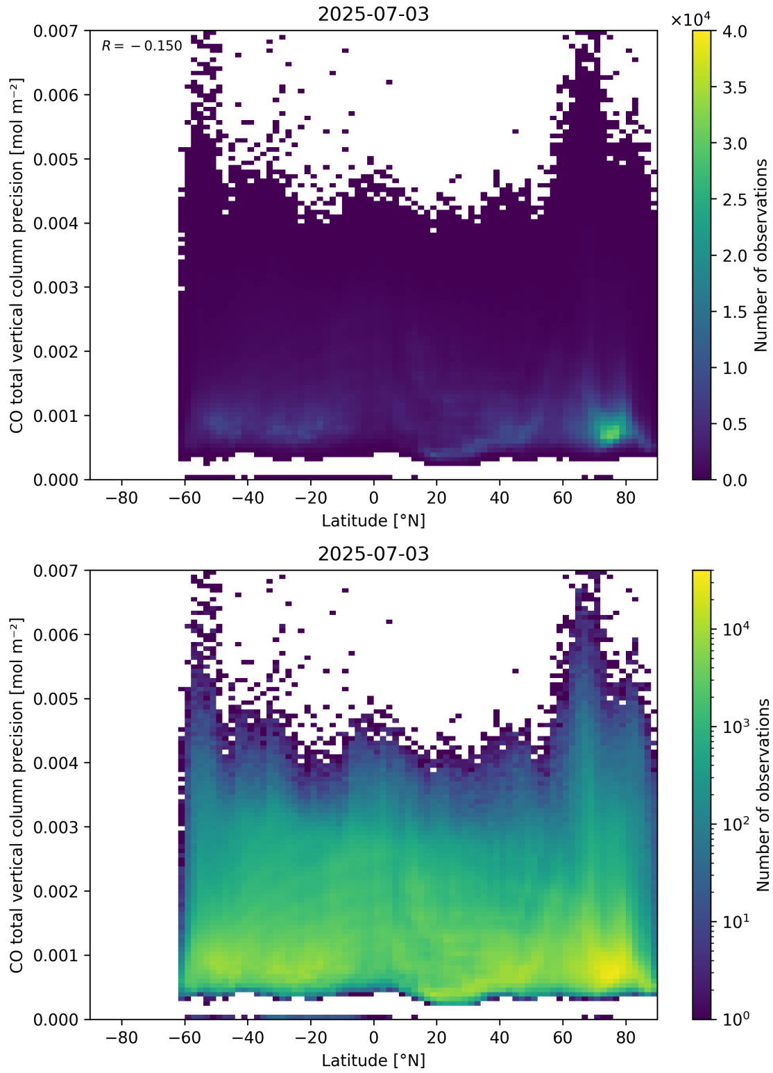
Figure 53: Scatter density plot of “Latitude” against “CO total vertical column precision” for 2025-07-03 to 2025-07-04.
