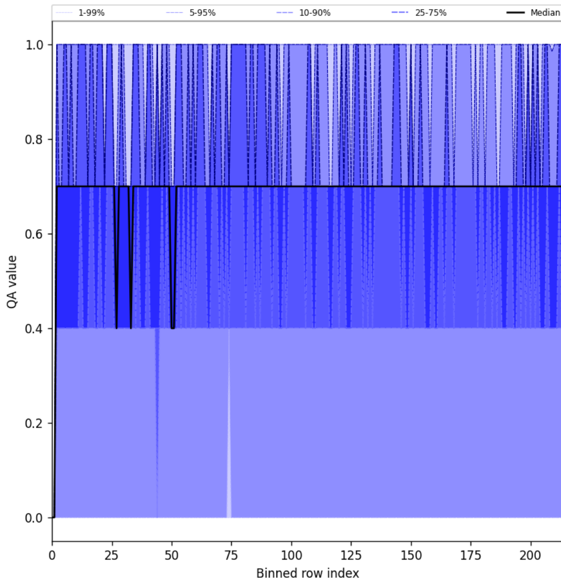
Figure 25: Along track statistics of “QA value” for 2025-07-03 to 2025-07-04
