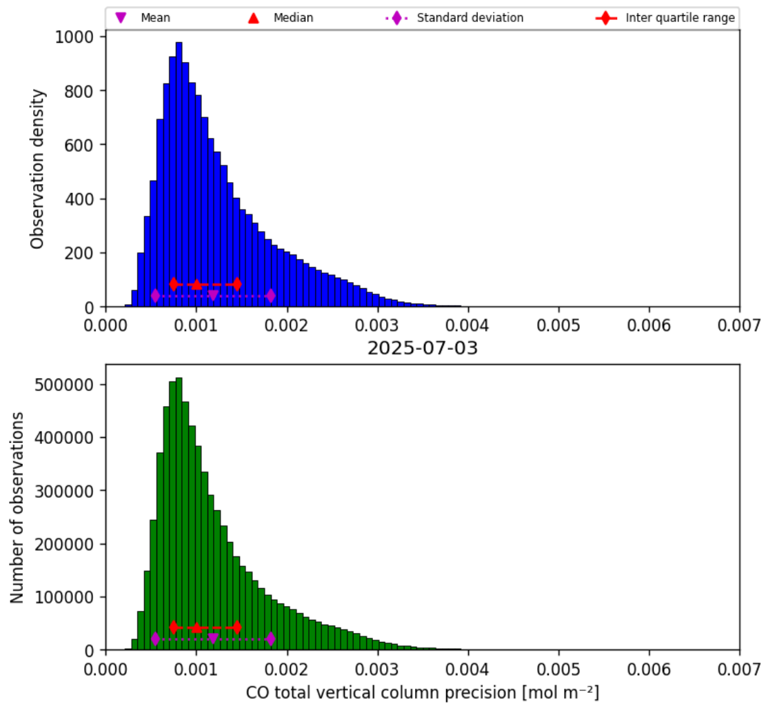
Figure 20: Histogram of “CO total vertical column precision” for 2025-07-03 to 2025-07-04
