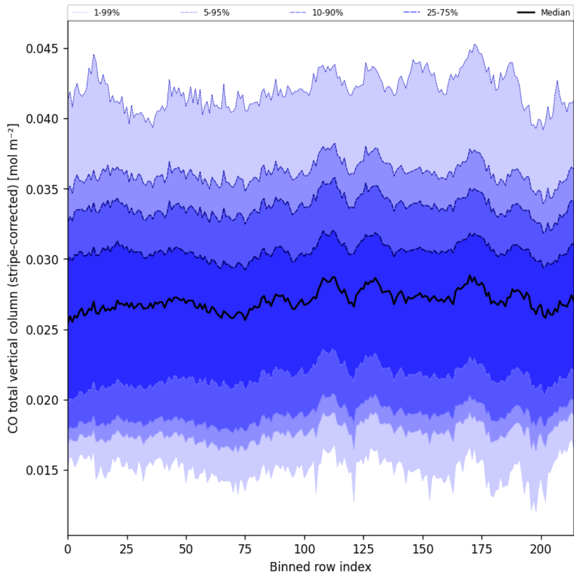
Figure 27: Along track statistics of “CO total vertical column (stripe-corrected)” for 2025-07-03 to 2025-07-04
