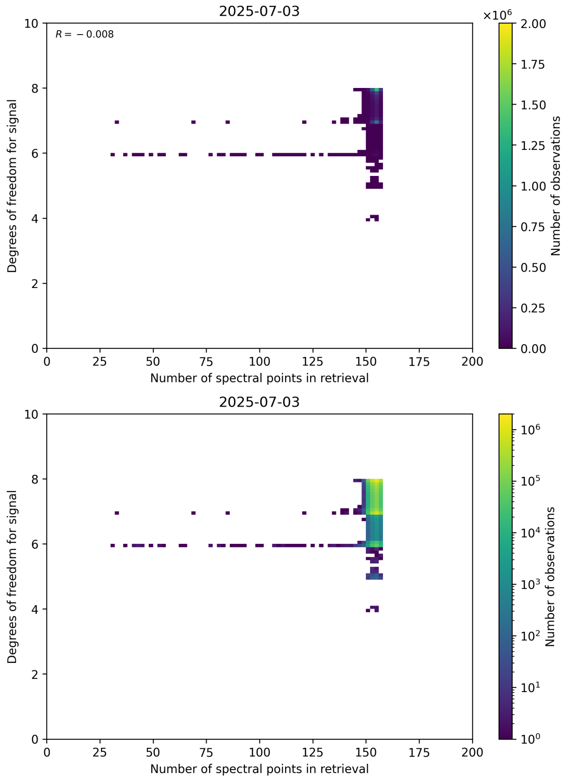
Figure 59: Scatter density plot of “Number of spectral points in retrieval” against “Degrees of freedom for signal” for 2025-07-03 to 2025-07-04.
