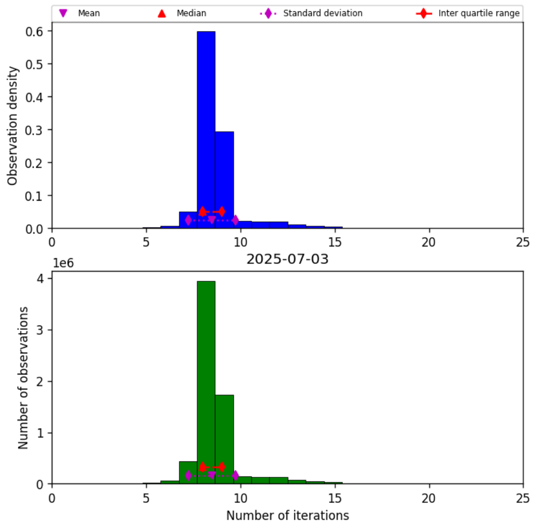
Figure 24: Histogram of “Number of iterations” for 2025-07-03 to 2025-07-04
