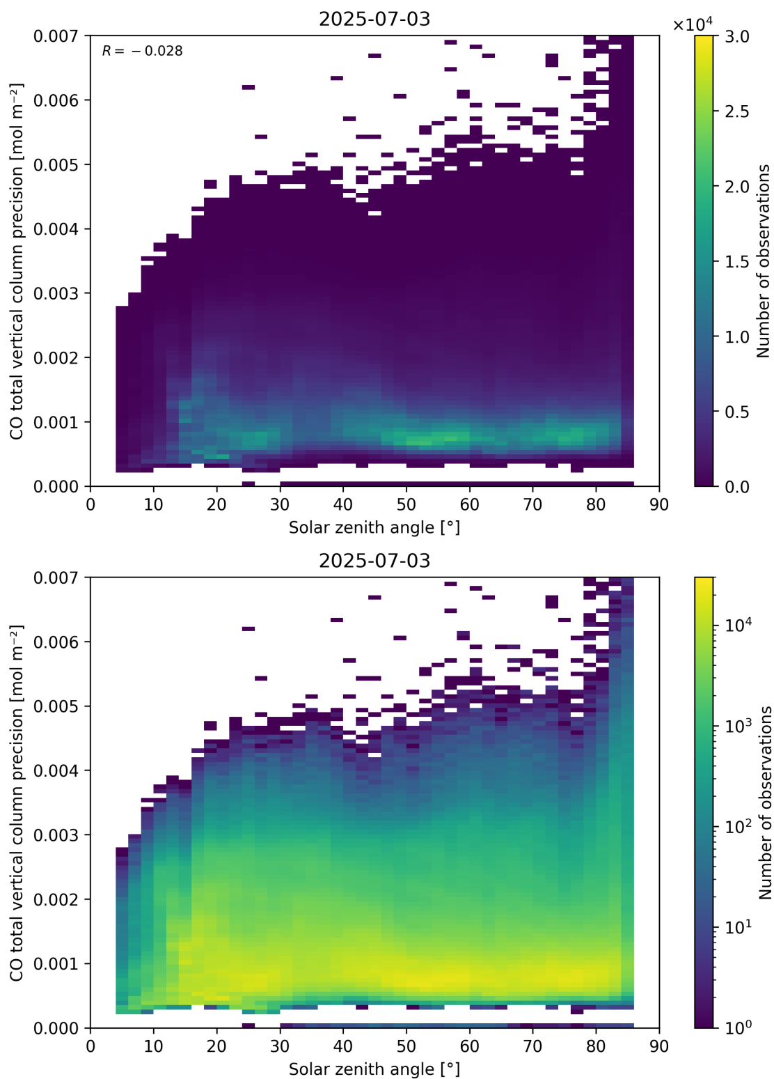
Figure 63: Scatter density plot of “Solar zenith angle” against “CO total vertical column precision” for 2025-07-03 to 2025-07-04.
