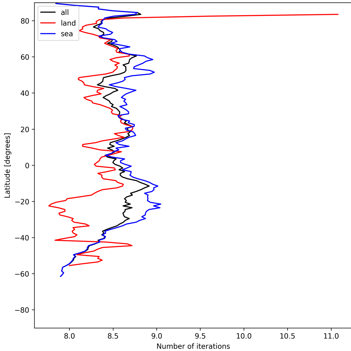
Figure 16: Zonal average of “Number of iterations” for 2025-07-03 to 2025-07-04.
