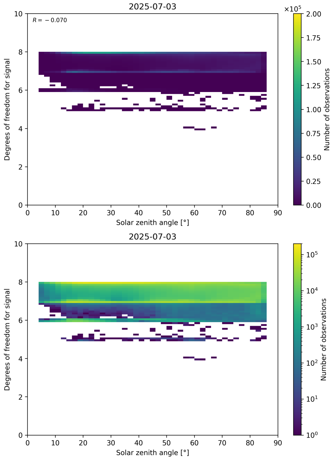
Figure 65: Scatter density plot of “Solar zenith angle” against “Degrees of freedom for signal” for 2025-07-03 to 2025-07-04.
