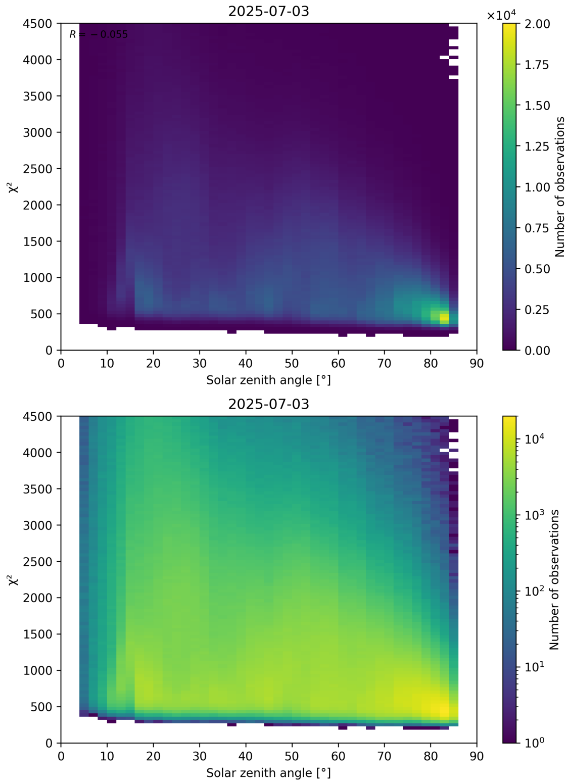
Figure 64: Scatter density plot of “Solar zenith angle” against “ \chi^2 ” for 2025-07-03 to 2025-07-04.
