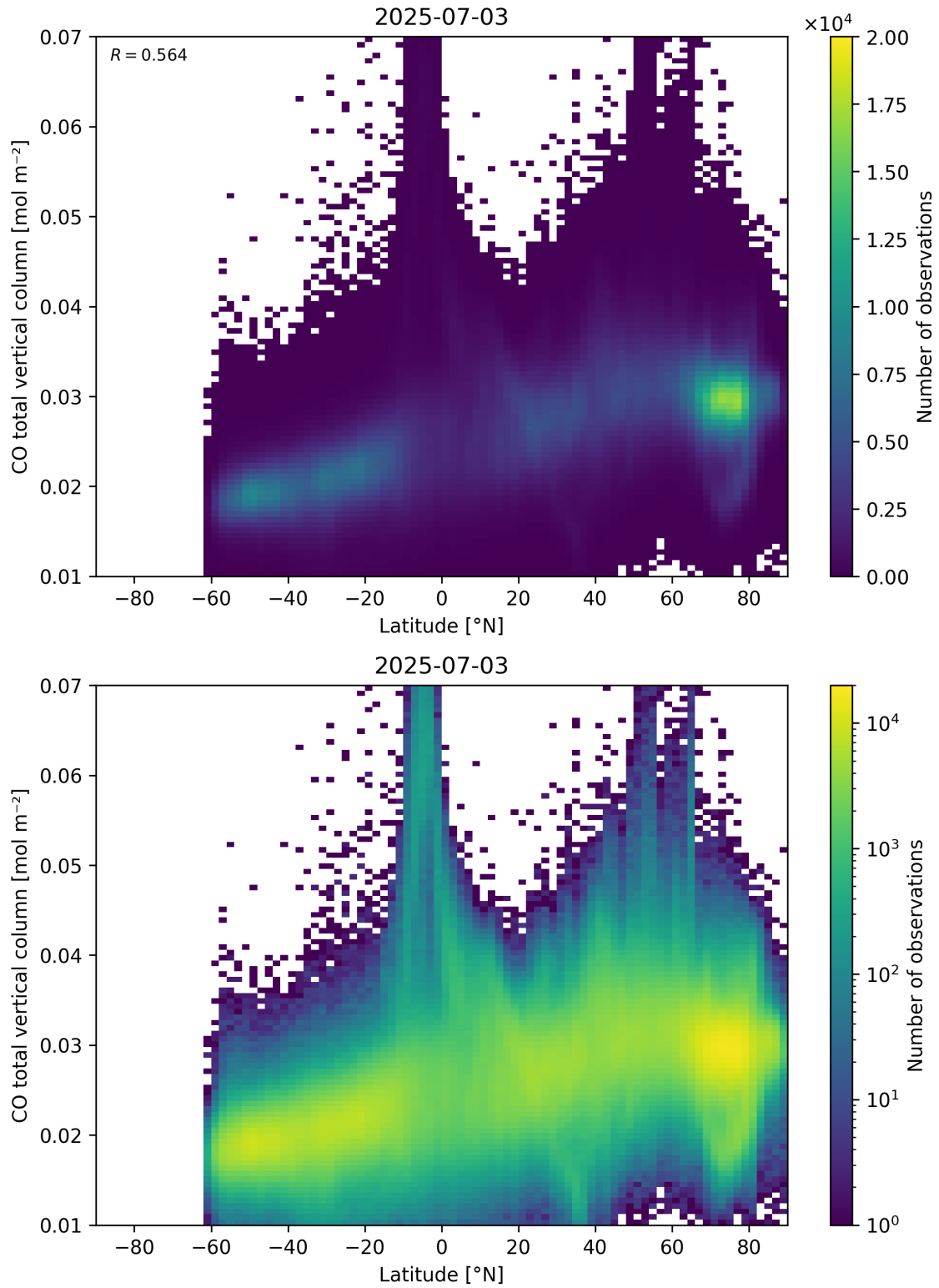
Figure 51: Scatter density plot of “Latitude” against “CO total vertical column” for 2025-07-03 to 2025-07-04.
