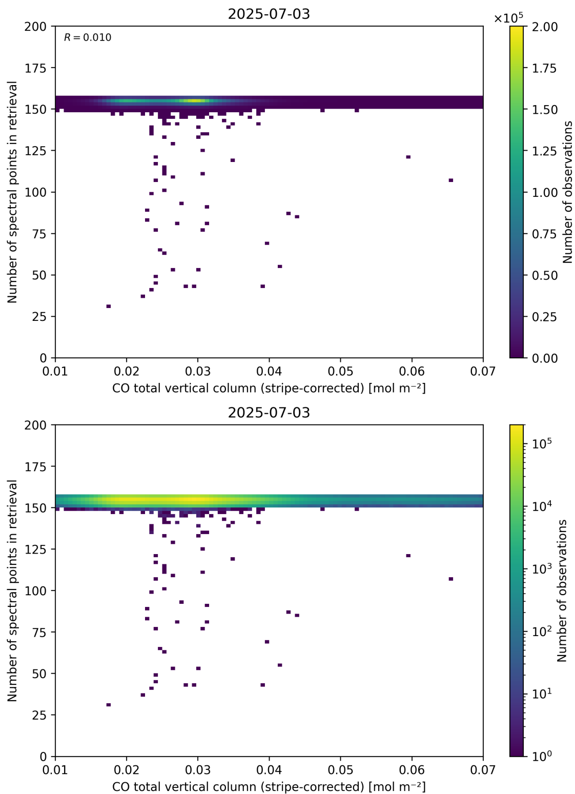
Figure 40: Scatter density plot of “CO total vertical column (stripe-corrected)” against “Number of spectral points in retrieval” for 2025-07-03 to 2025-07-04.
