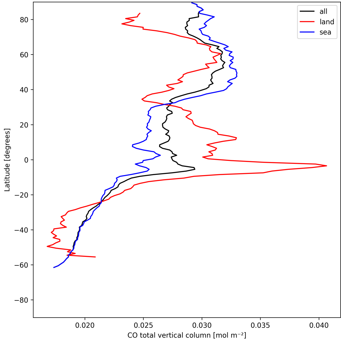
Figure 10: Zonal average of “CO total vertical column” for 2025-07-03 to 2025-07-04.
