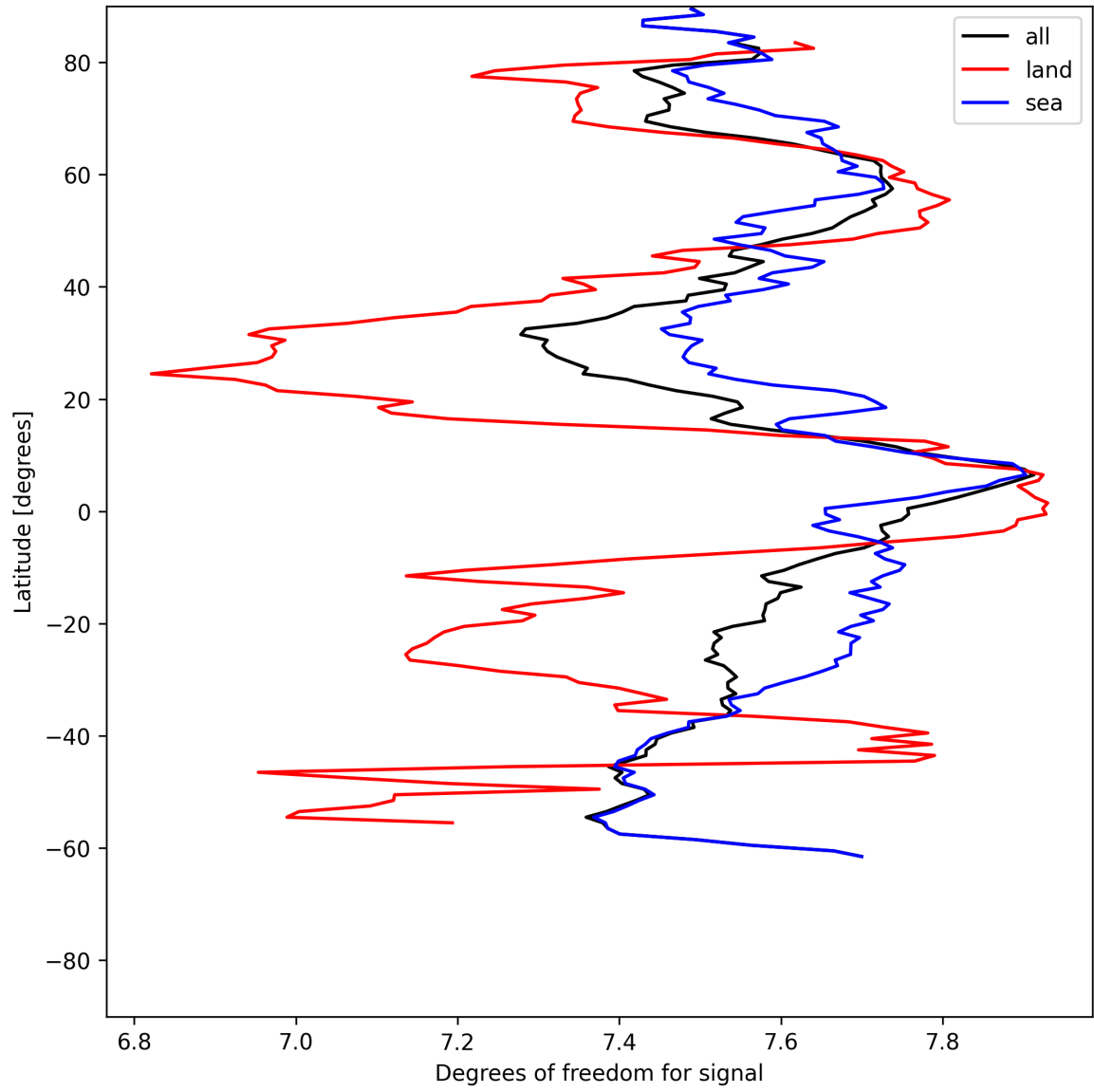
Figure 15: Zonal average of “Degrees of freedom for signal” for 2025-07-03 to 2025-07-04.
