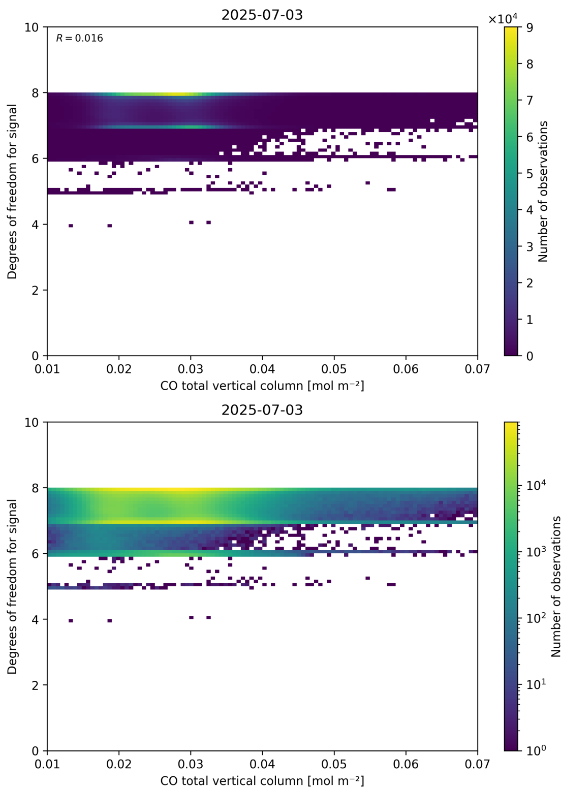
Figure 41: Scatter density plot of “CO total vertical column” against “Degrees of freedom for signal” for 2025-07-03 to 2025-07-04.
