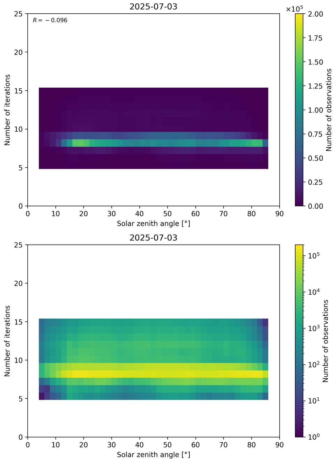
Figure 67: Scatter density plot of “Solar zenith angle” against “Number of iterations” for 2025-07-03 to 2025-07-04.
