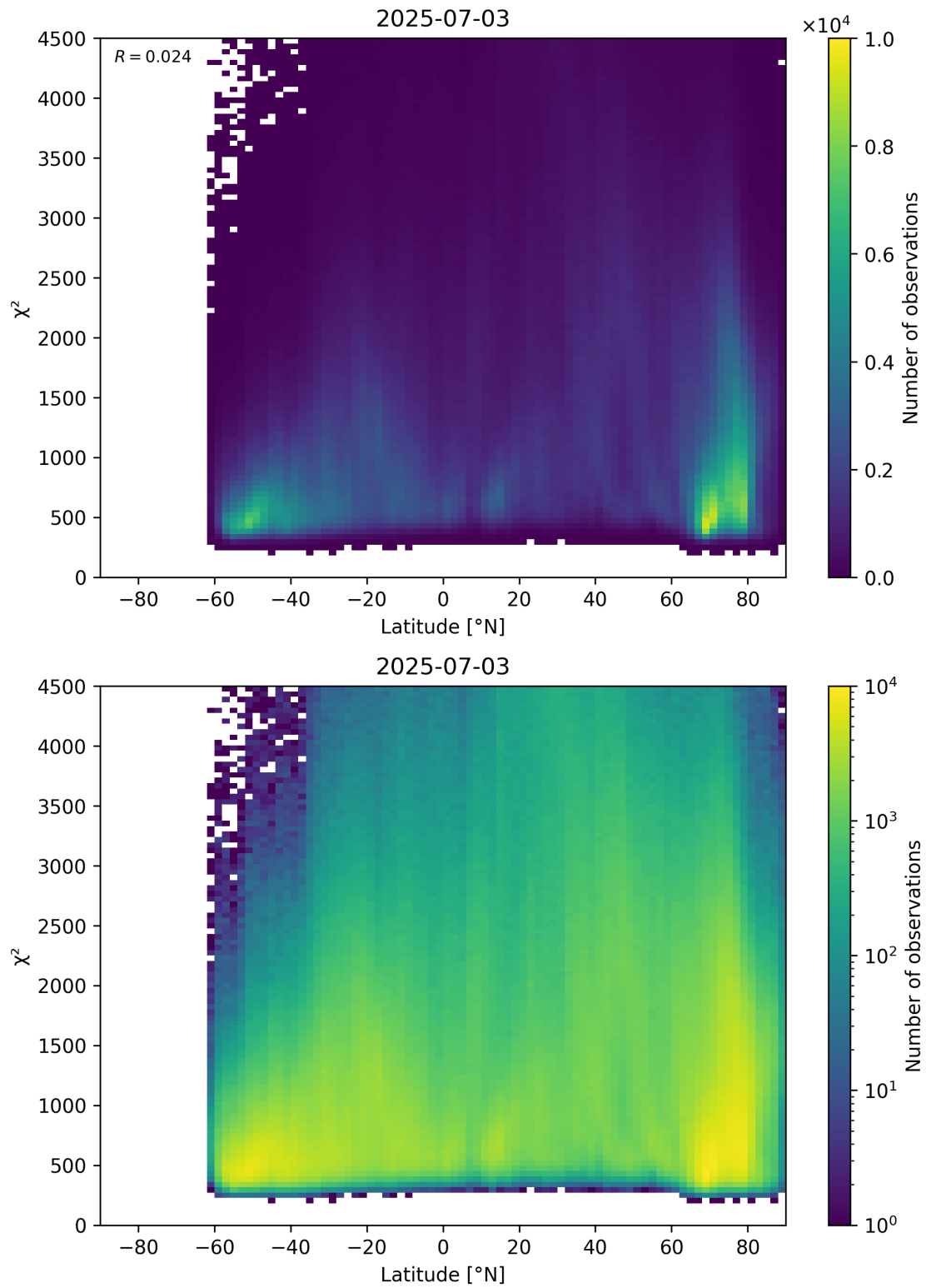
Figure 54: Scatter density plot of “Latitude” against “ \chi^2 ” for 2025-07-03 to 2025-07-04.
