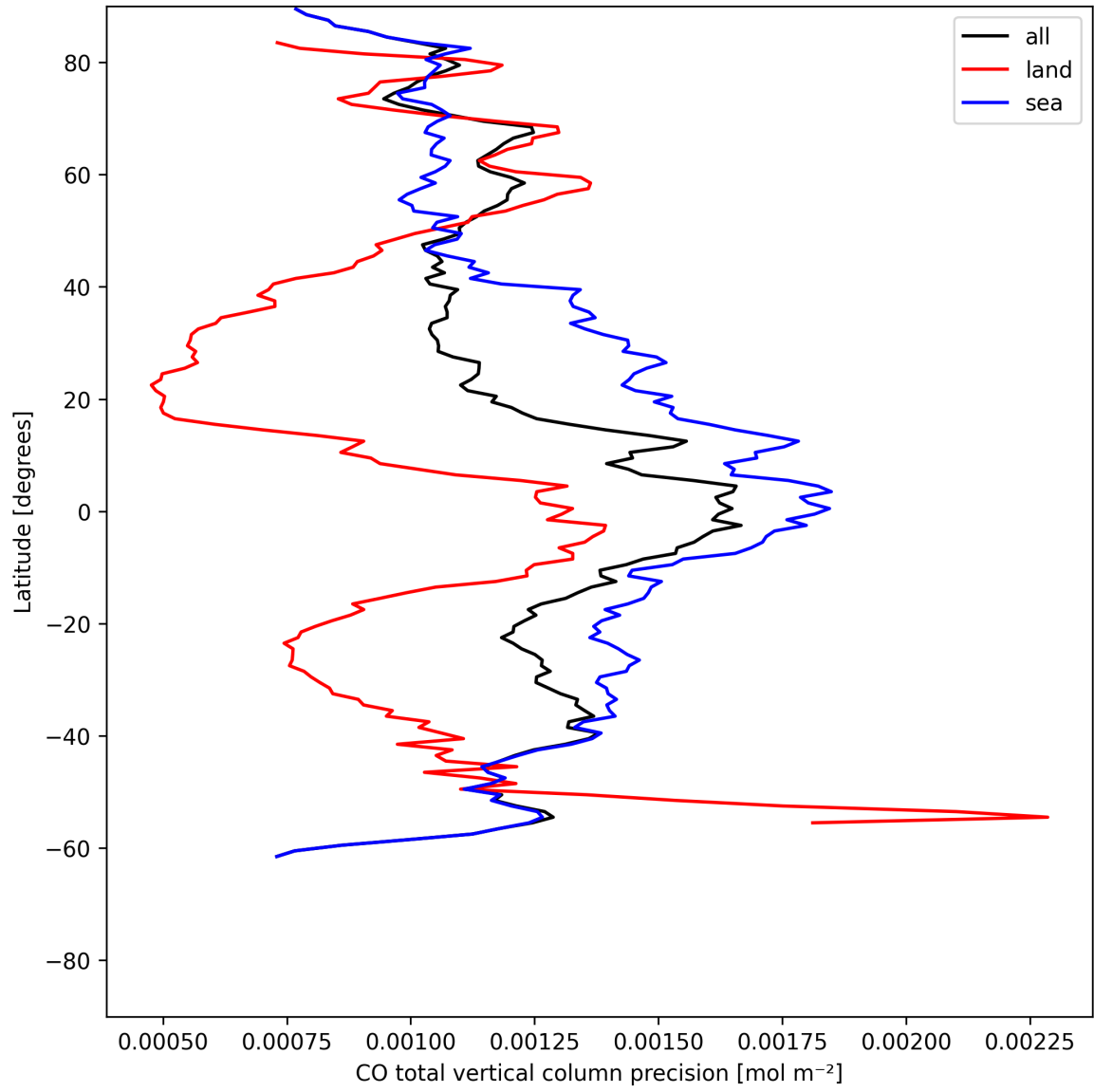
Figure 12: Zonal average of “CO total vertical column precision” for 2025-07-03 to 2025-07-04.
