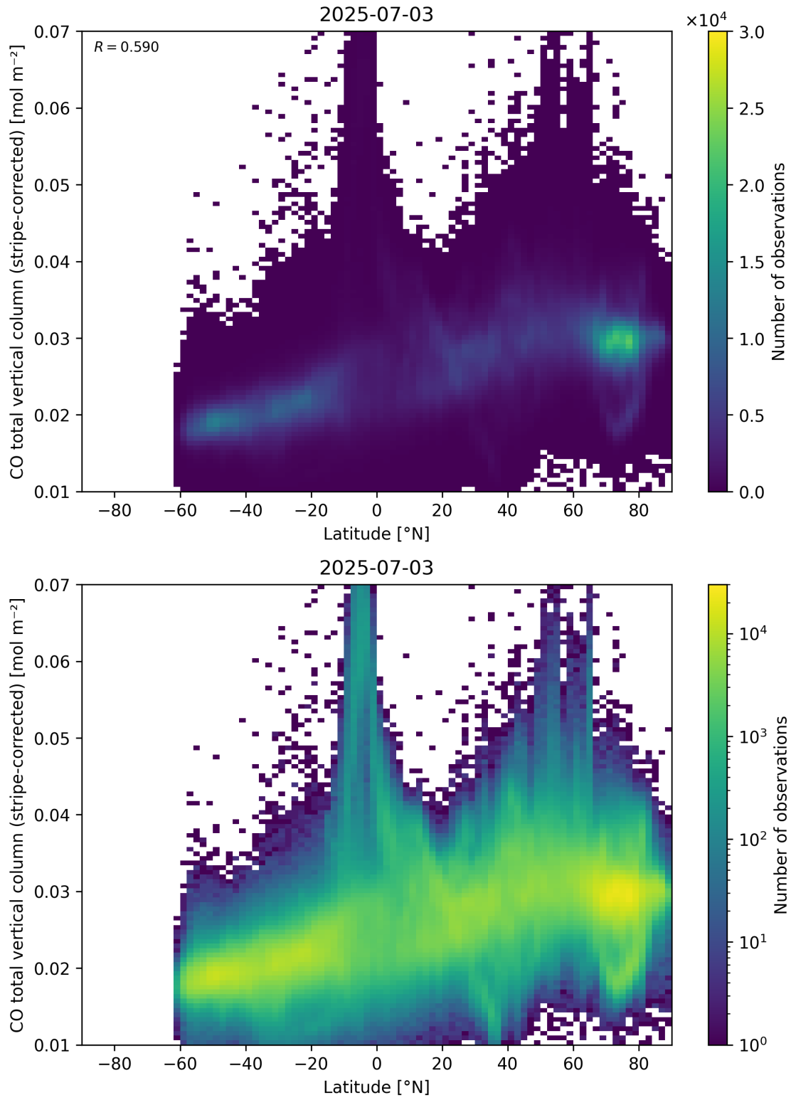
Figure 52: Scatter density plot of “Latitude” against “CO total vertical column (stripe-corrected)” for 2025-07-03 to 2025-07-04.
