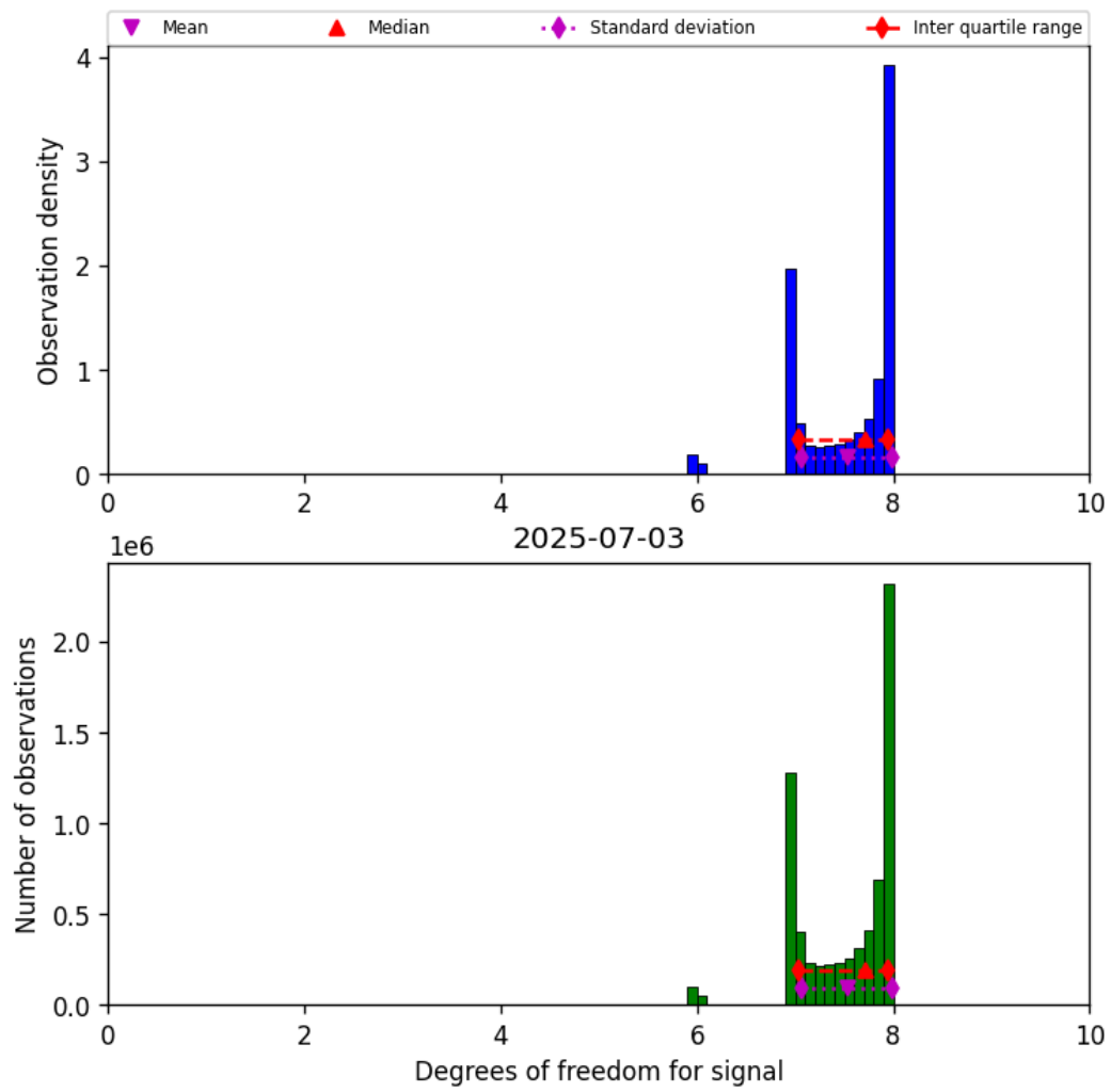
Figure 23: Histogram of “Degrees of freedom for signal” for 2025-07-03 to 2025-07-04
