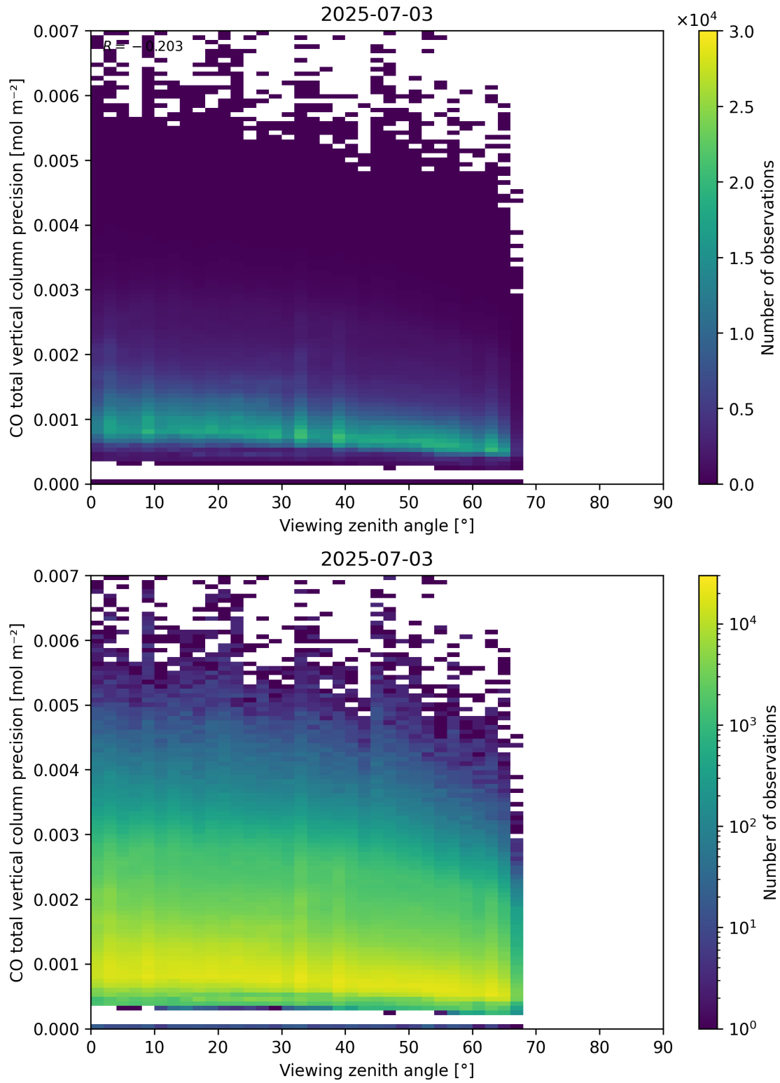
Figure 71: Scatter density plot of “Viewing zenith angle” against “CO total vertical column precision” for 2025-07-03 to 2025-07-04.
