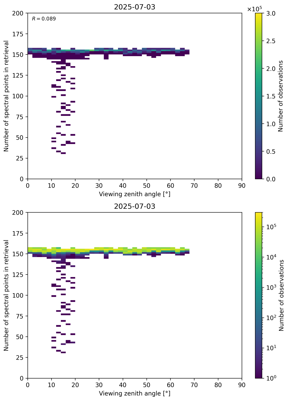
Figure 76: Scatter density plot of “Viewing zenith angle” against “Number of spectral points in retrieval” for 2025-07-03 to 2025-07-04.
