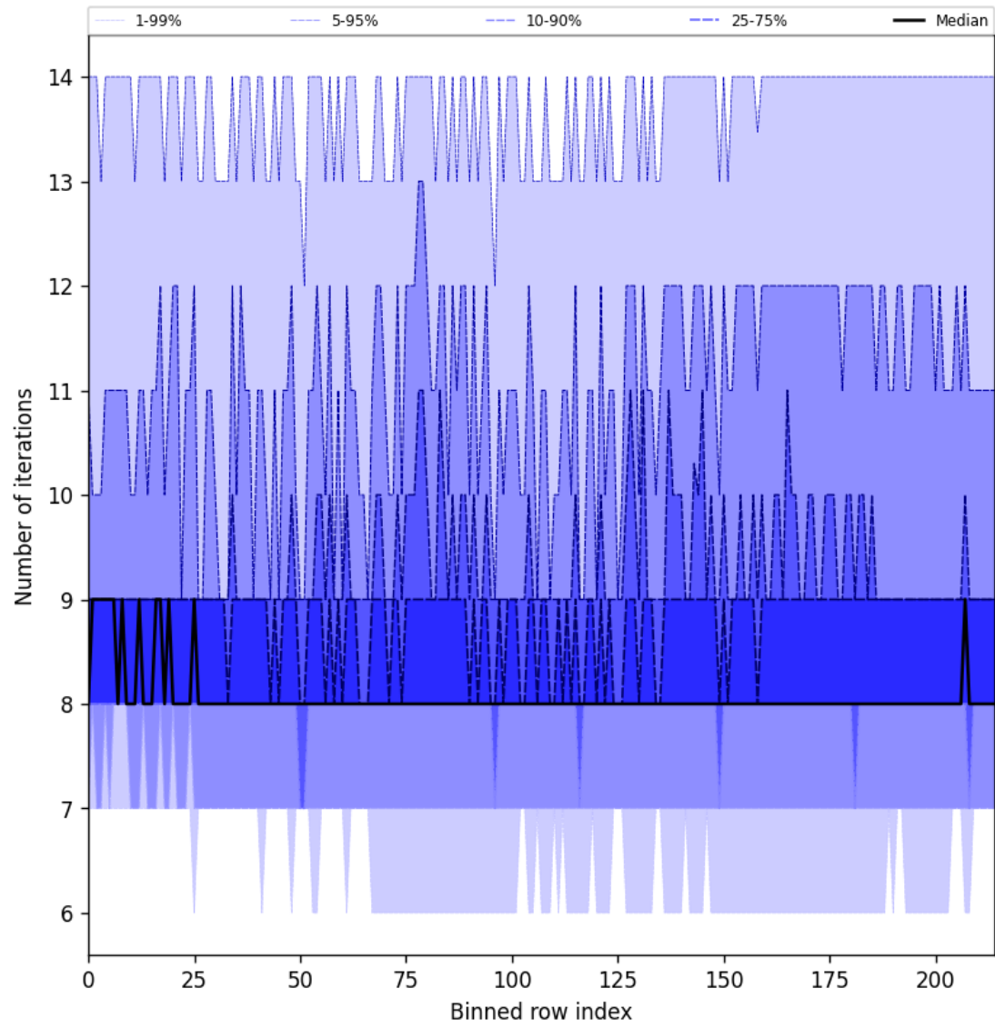
Figure 32: Along track statistics of “Number of iterations” for 2025-07-03 to 2025-07-04
