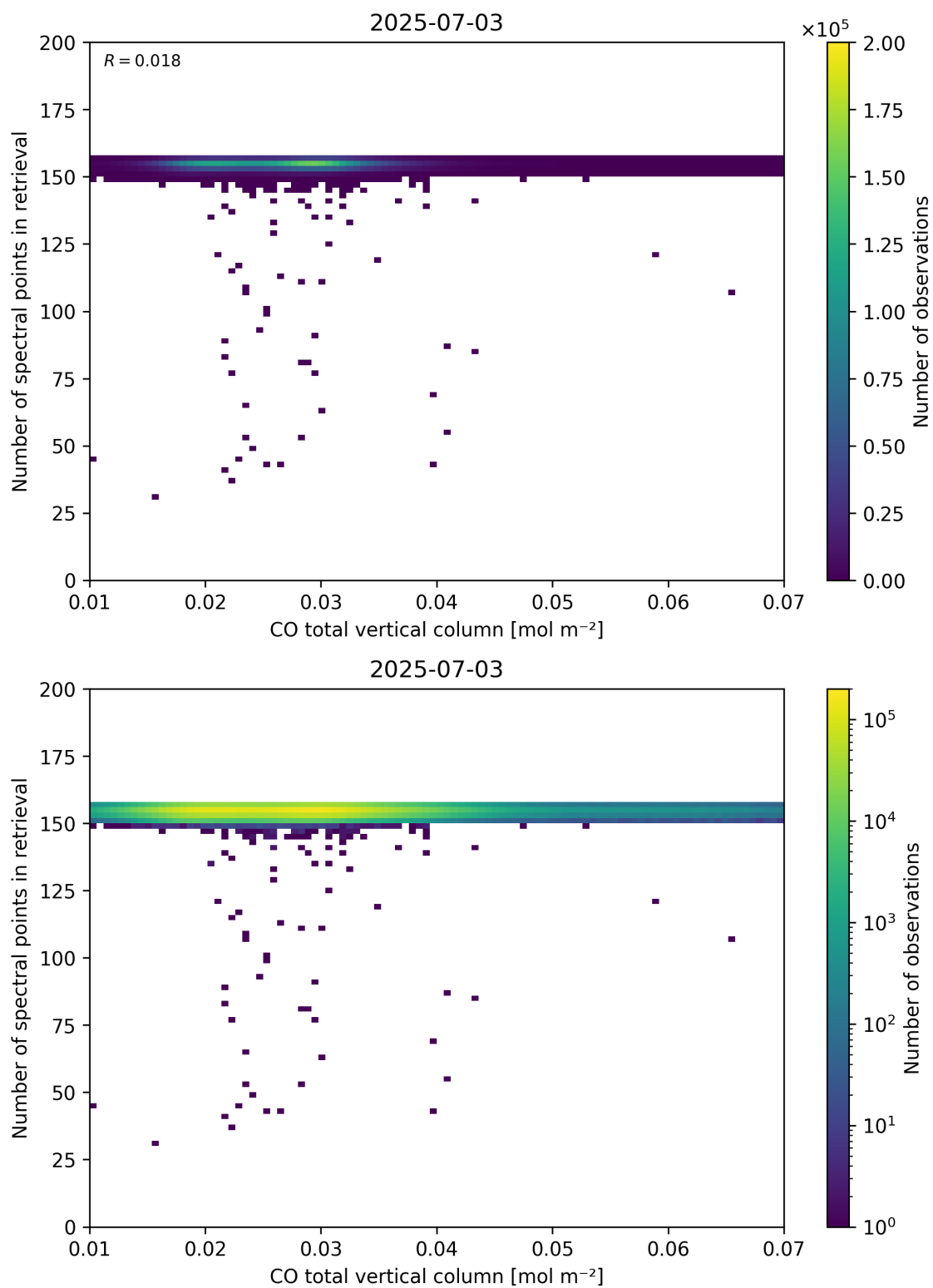
Figure 43: Scatter density plot of “CO total vertical column” against “Number of spectral points in retrieval” for 2025-07-03 to 2025-07-04.
