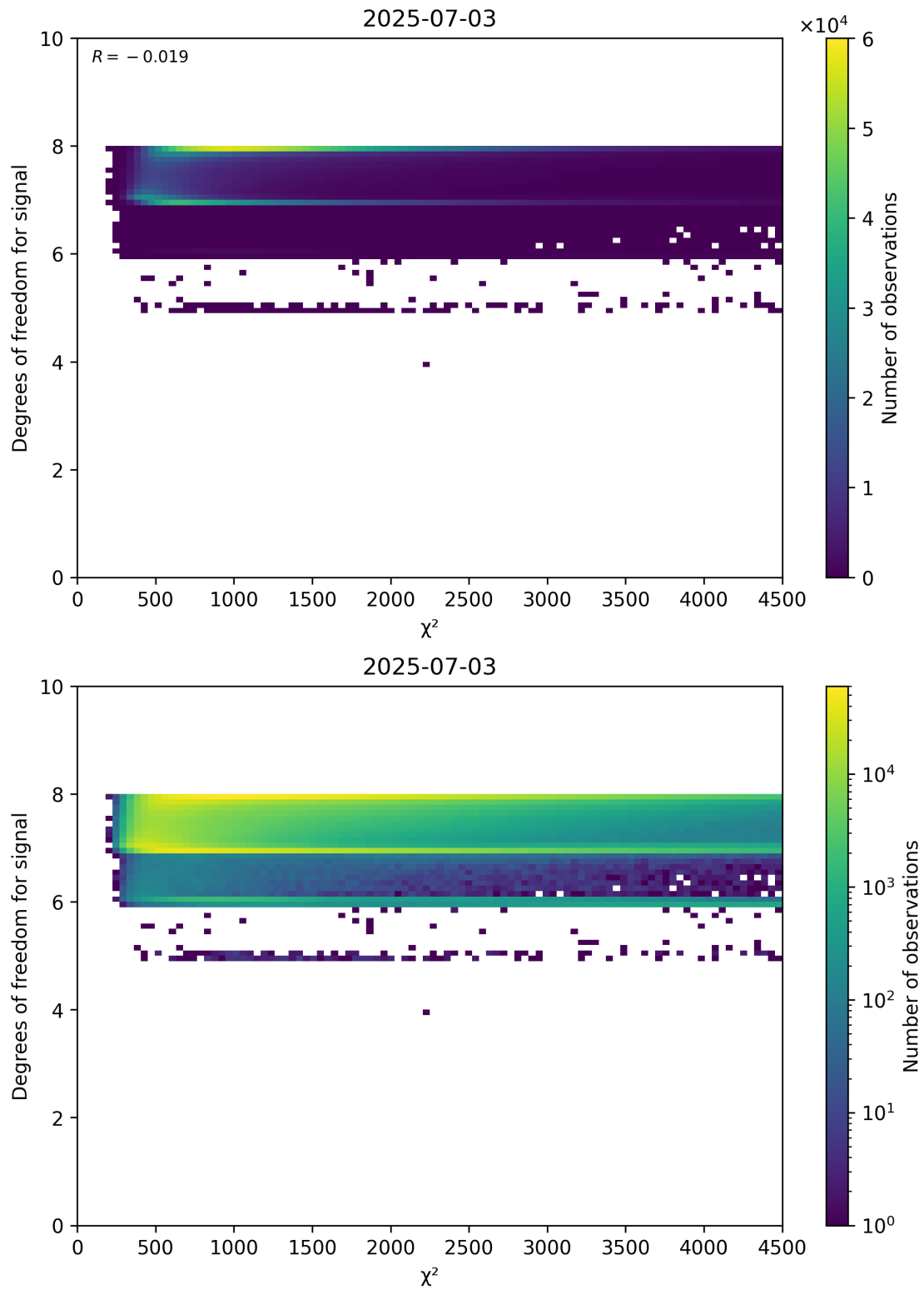
Figure 48: Scatter density plot of " \chi^2 " against "Degrees of freedom for signal" for 2025-07-03 to 2025-07-04.
