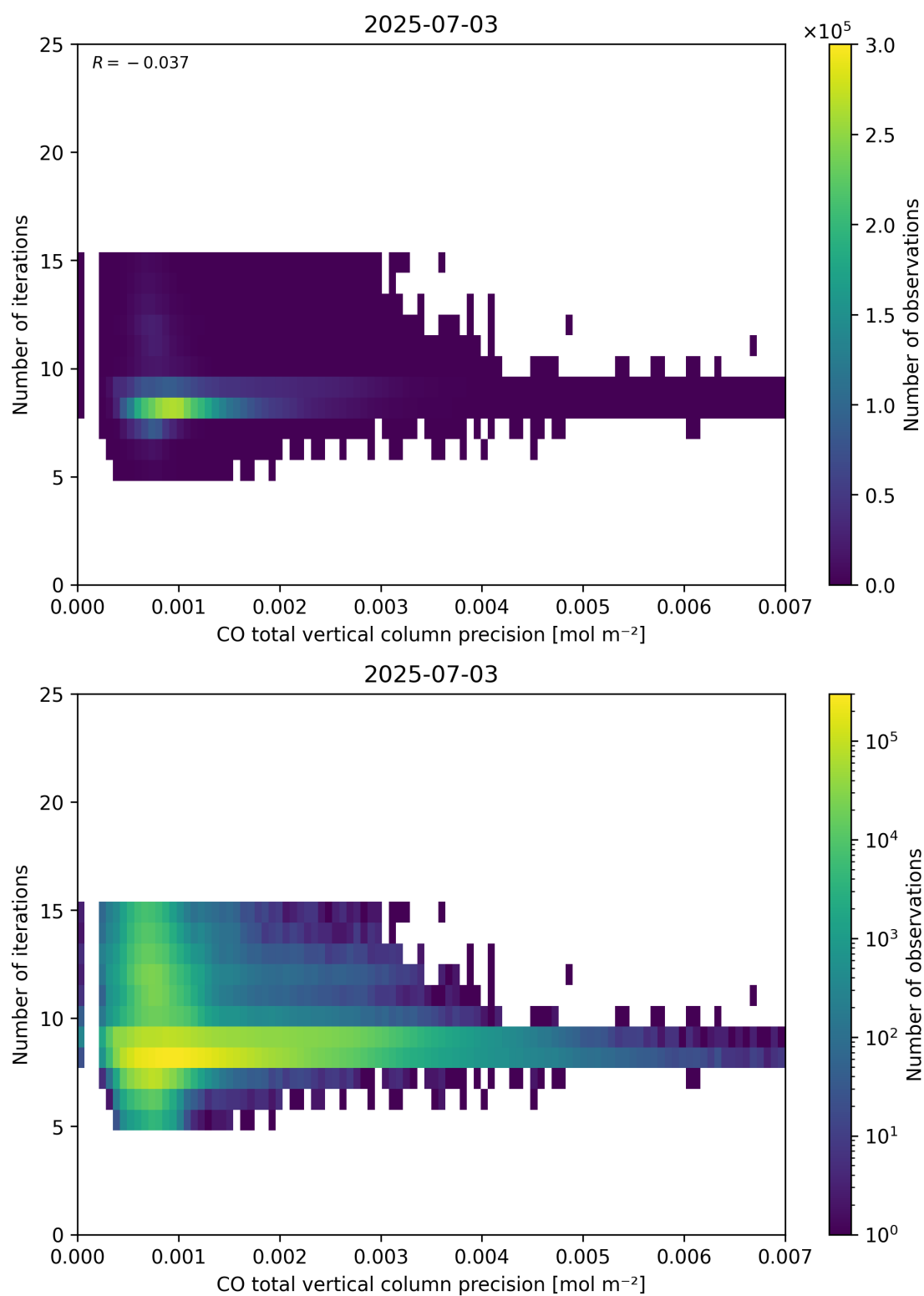
Figure 46: Scatter density plot of “CO total vertical column precision” against “Number of iterations” for 2025-07-03 to 2025-07-04.
