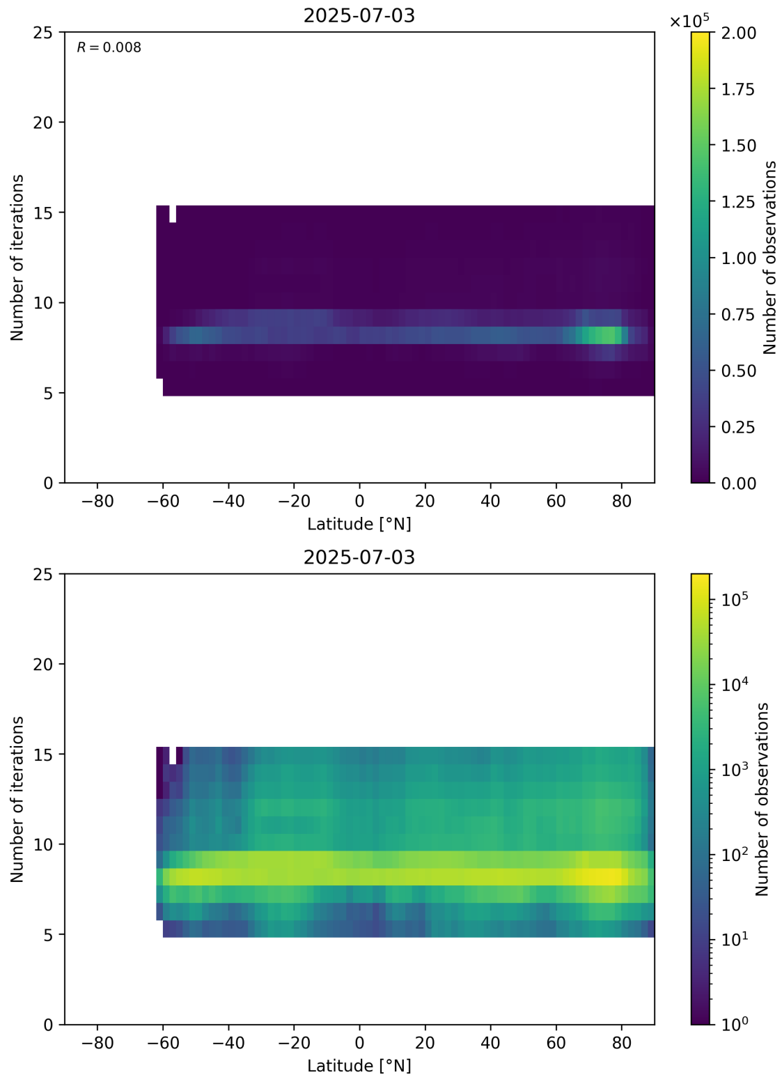
Figure 56: Scatter density plot of “Latitude” against “Number of iterations” for 2025-07-03 to 2025-07-04.
