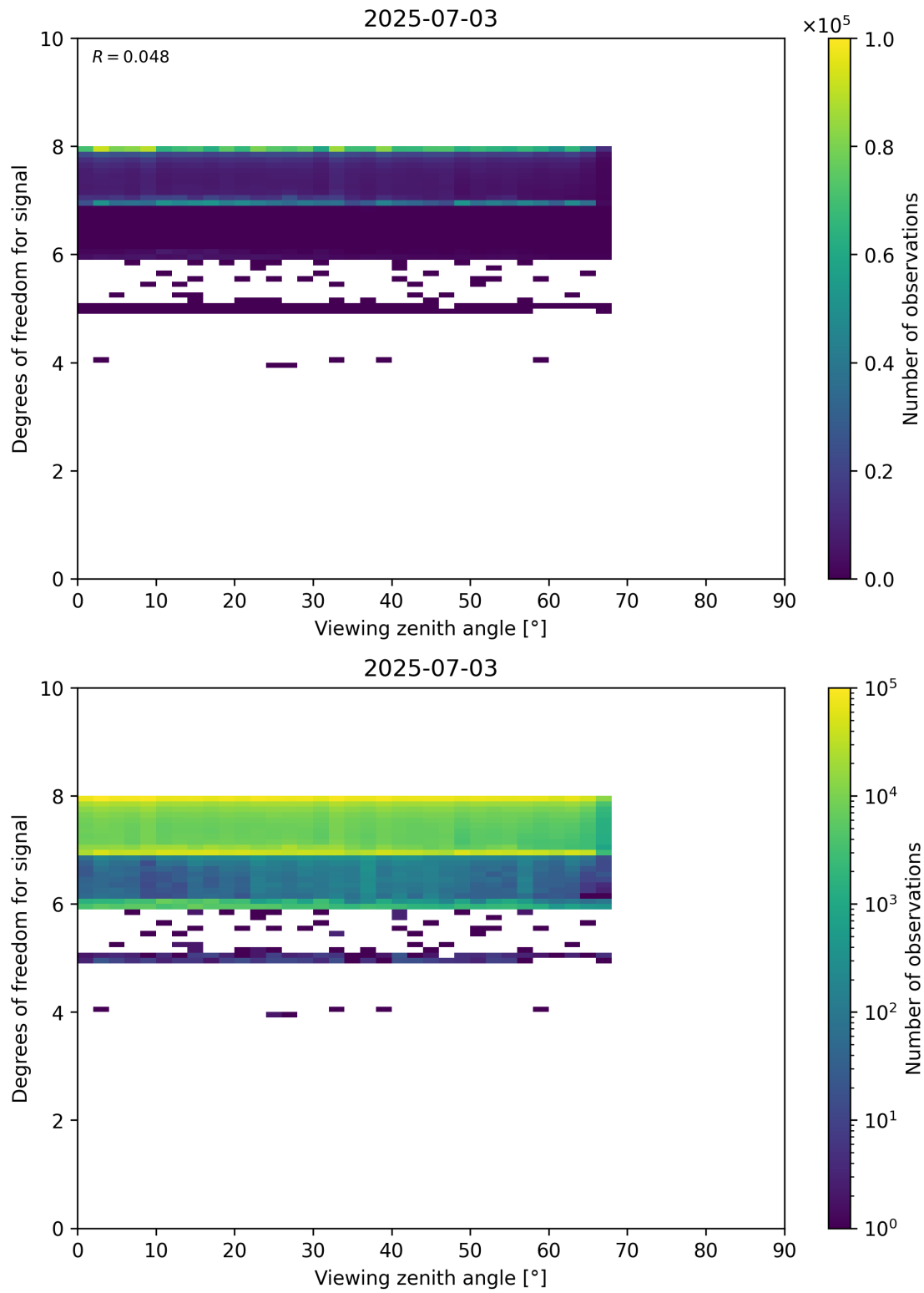
Figure 73: Scatter density plot of “Viewing zenith angle” against “Degrees of freedom for signal” for 2025-07-03 to 2025-07-04.
