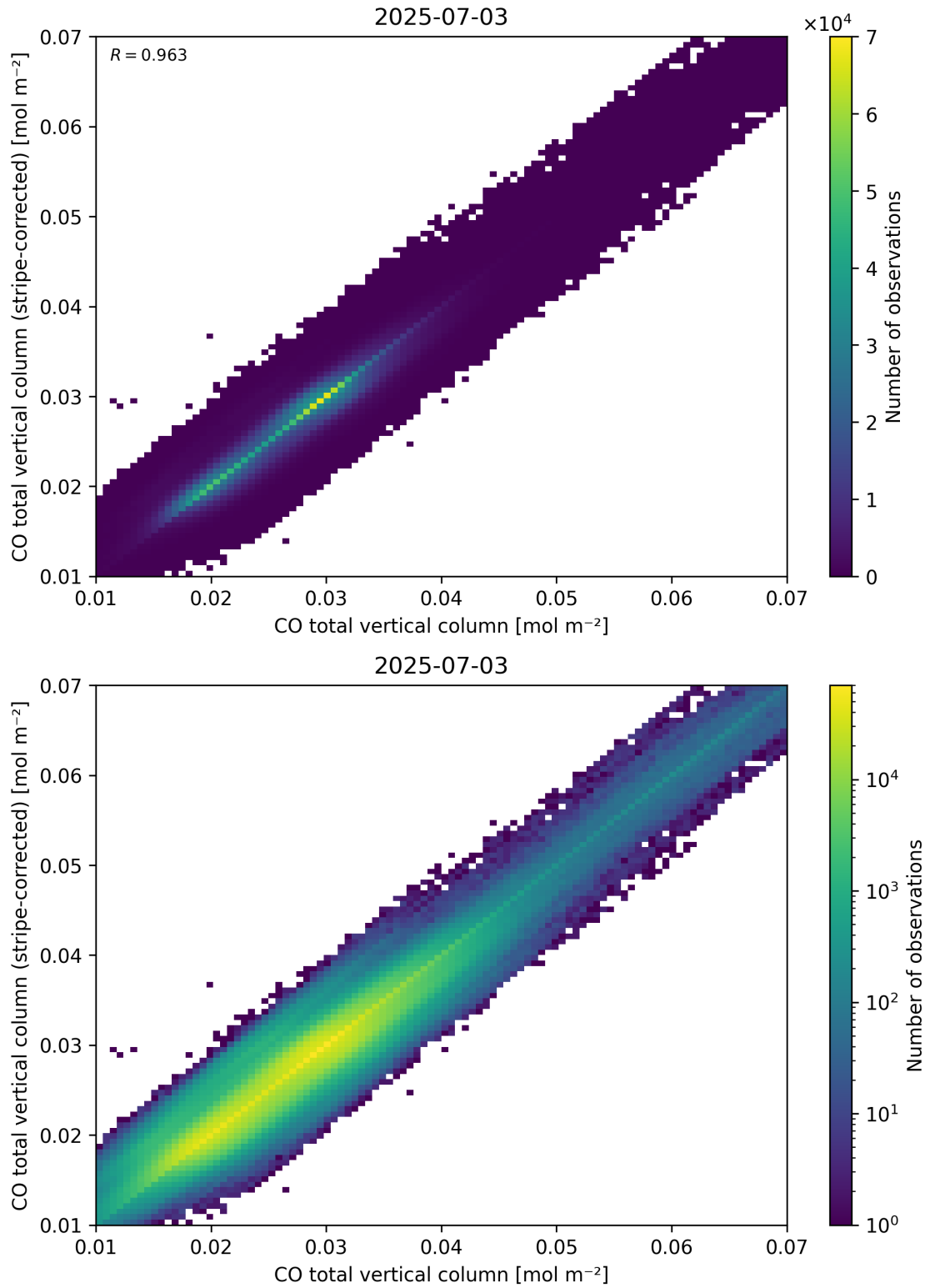
Figure 33: Scatter density plot of “CO total vertical column” against “CO total vertical column (stripe-corrected)” for 2025-07-03 to 2025-07-04.
