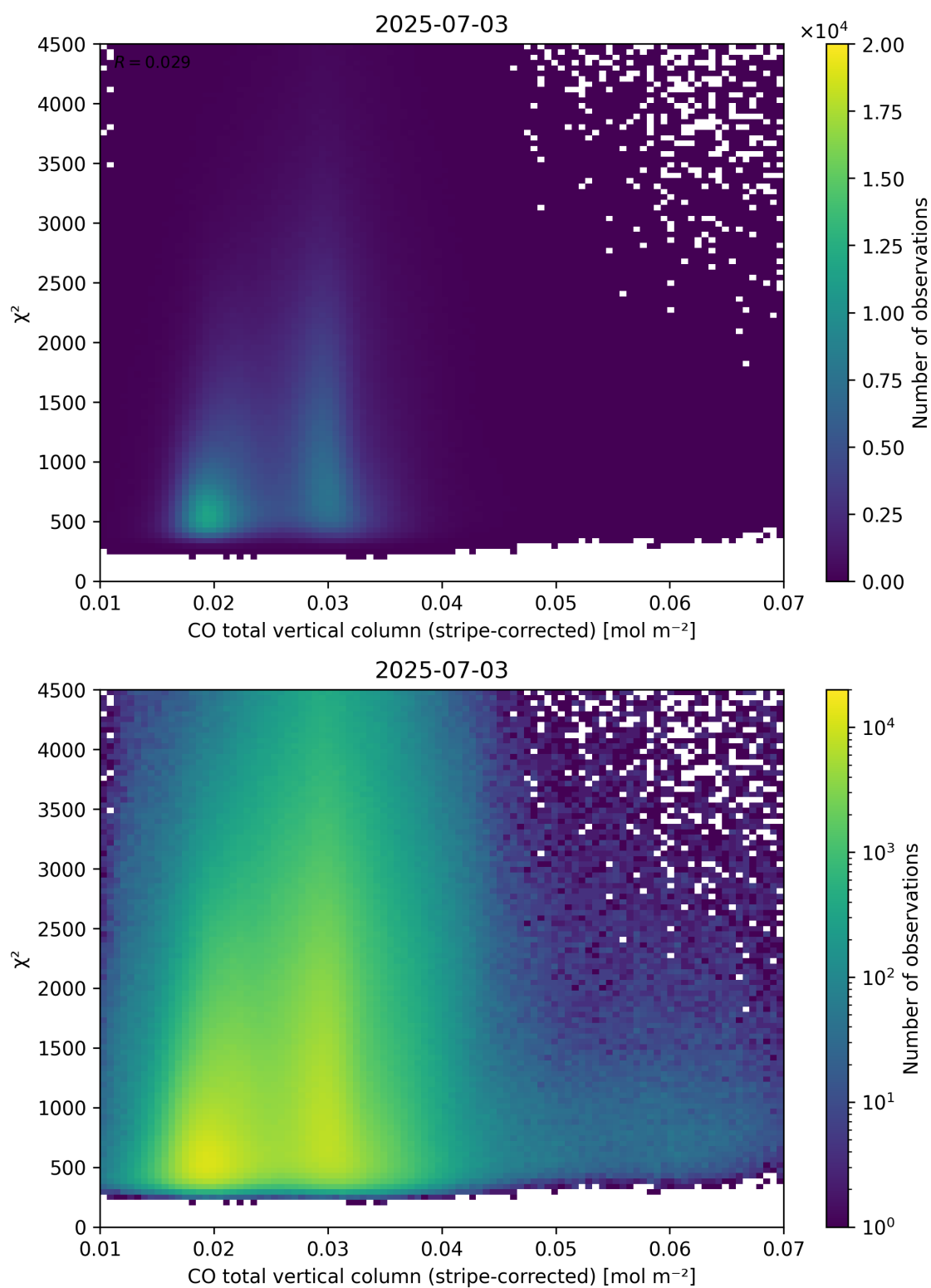
Figure 37: Scatter density plot of “CO total vertical column (stripe-corrected)” against “ \chi^2 ” for 2025-07-03 to 2025-07-04.
