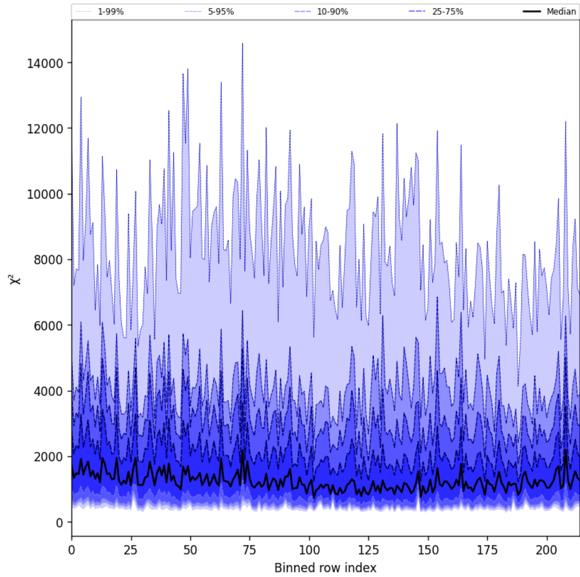
Figure 30: Along track statistics of “ \chi^2 ” for 2025-07-03 to 2025-07-04
