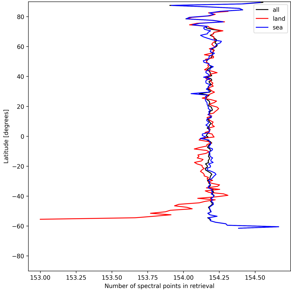
Figure 13: Zonal average of “Number of spectral points in retrieval” for 2025-07-03 to 2025-07-04.
