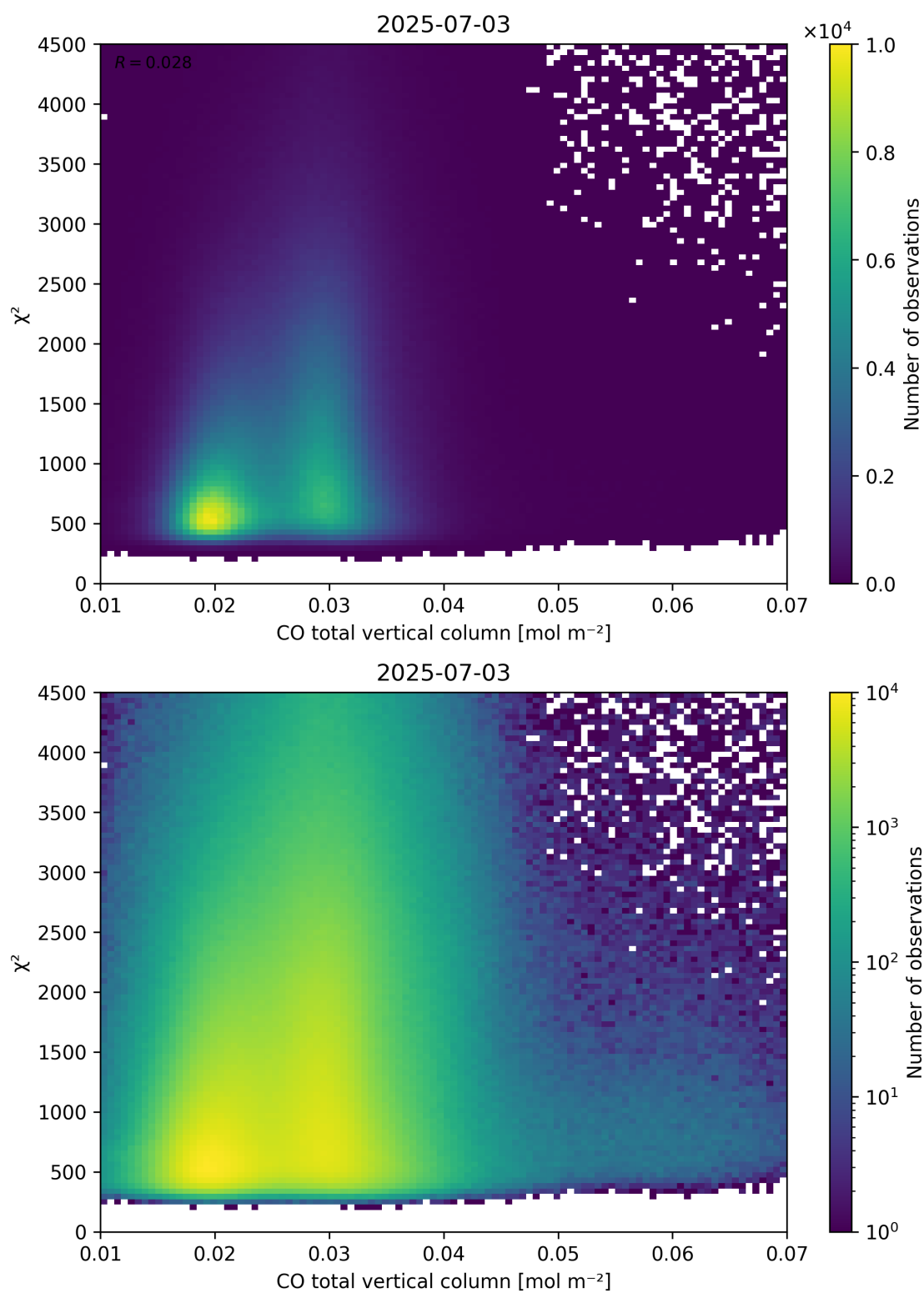
Figure 35: Scatter density plot of “CO total vertical column” against “ \chi^2 ” for 2025-07-03 to 2025-07-04.
