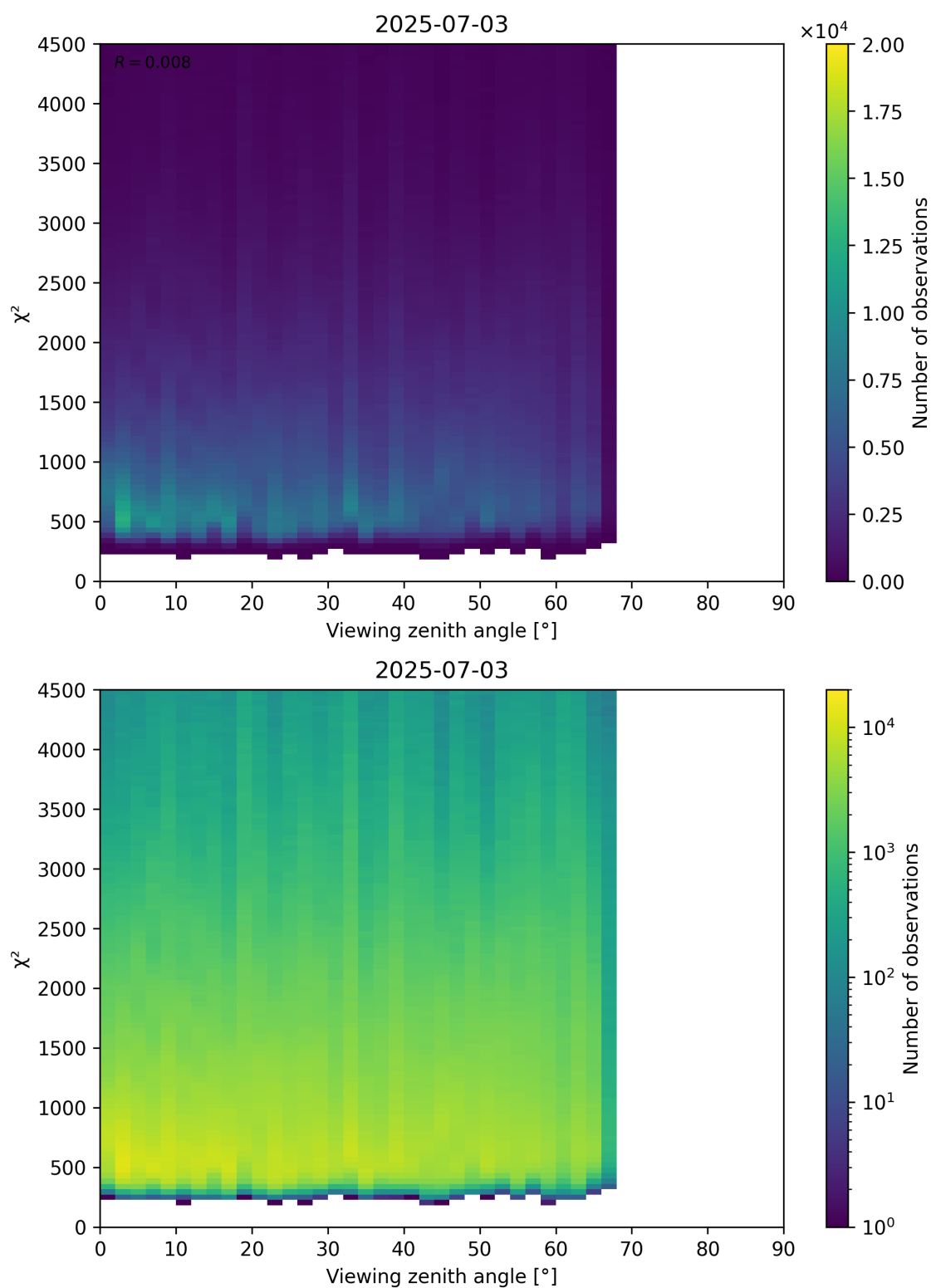
Figure 72: Scatter density plot of “Viewing zenith angle” against “ \chi^2 ” for 2025-07-03 to 2025-07-04.
