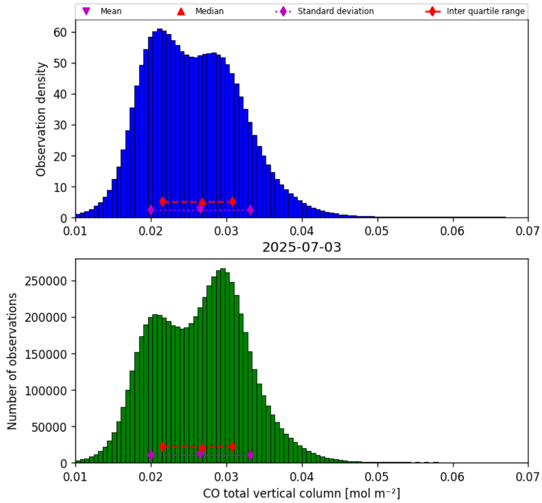
Figure 18: Histogram of “CO total vertical column” for 2025-07-03 to 2025-07-04
