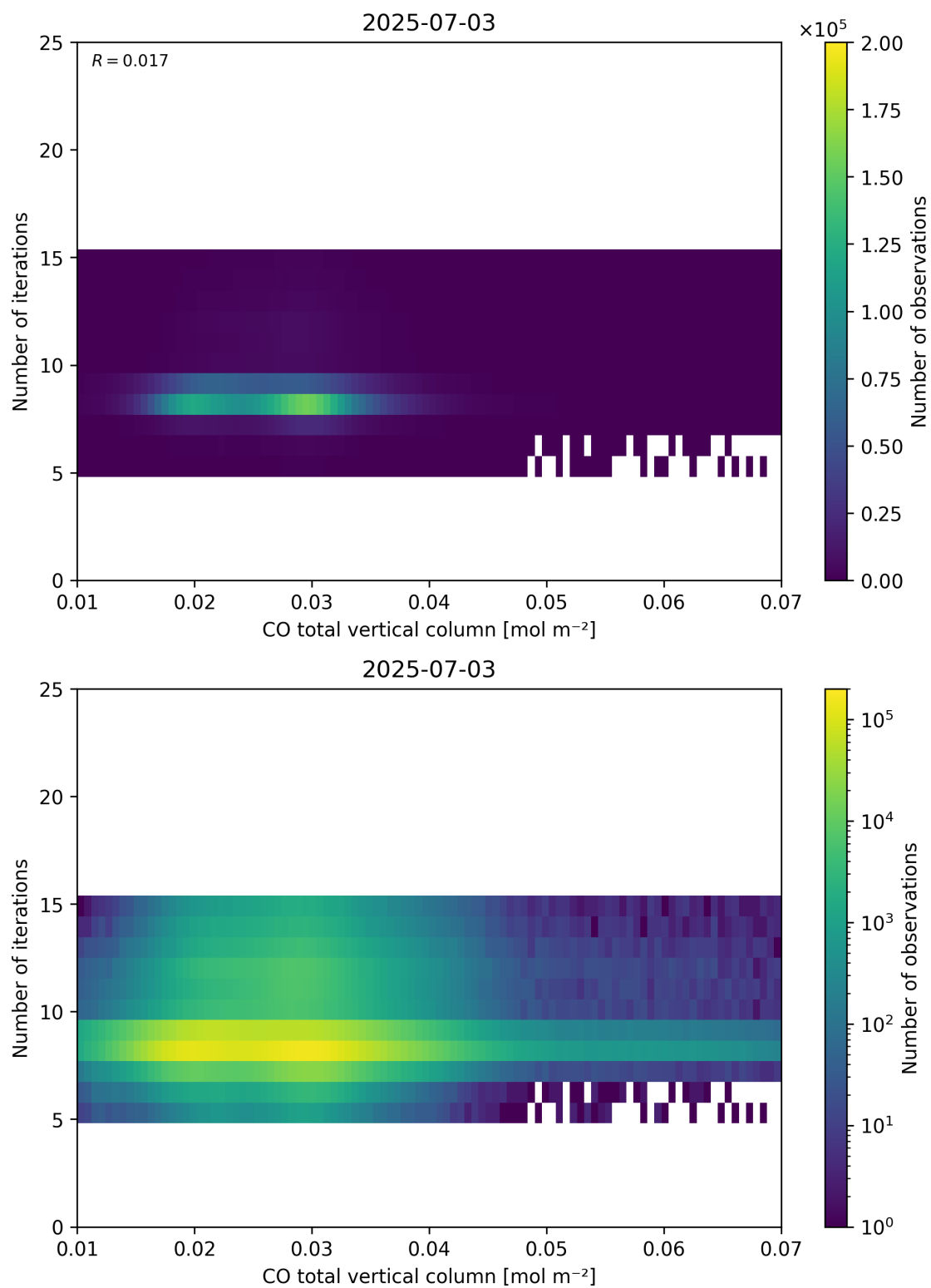
Figure 42: Scatter density plot of “CO total vertical column” against “Number of iterations” for 2025-07-03 to 2025-07-04.
