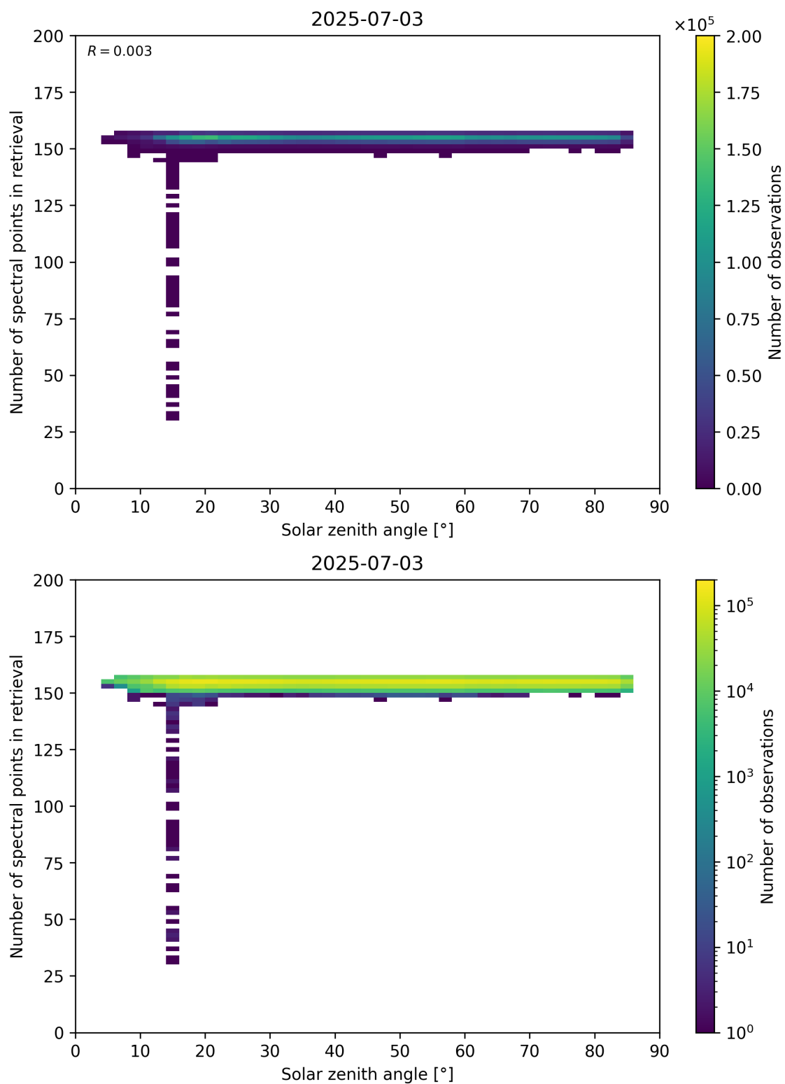
Figure 68: Scatter density plot of “Solar zenith angle” against “Number of spectral points in retrieval” for 2025-07-03 to 2025-07-04.
