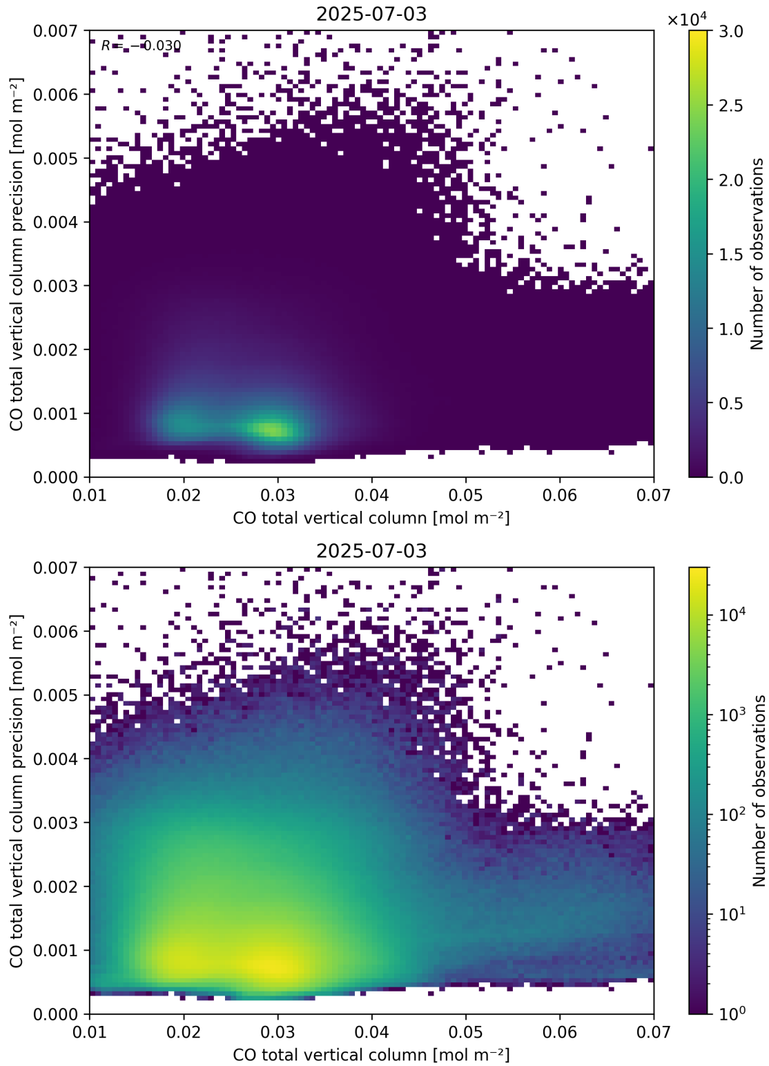
Figure 34: Scatter density plot of “CO total vertical column” against “CO total vertical column precision” for 2025-07-03 to 2025-07-04.
