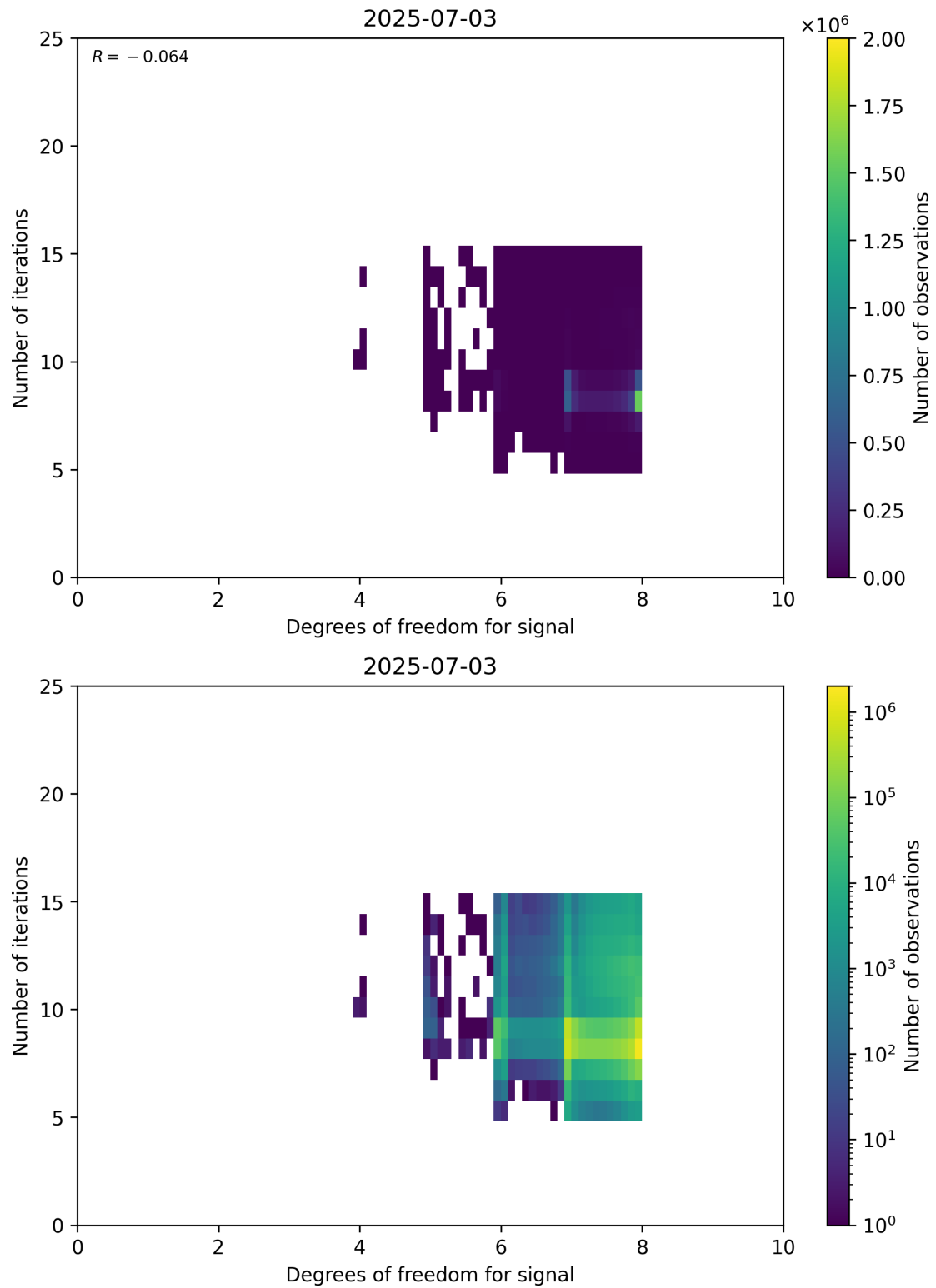
Figure 50: Scatter density plot of “Degrees of freedom for signal” against “Number of iterations” for 2025-07-03 to 2025-07-04.
