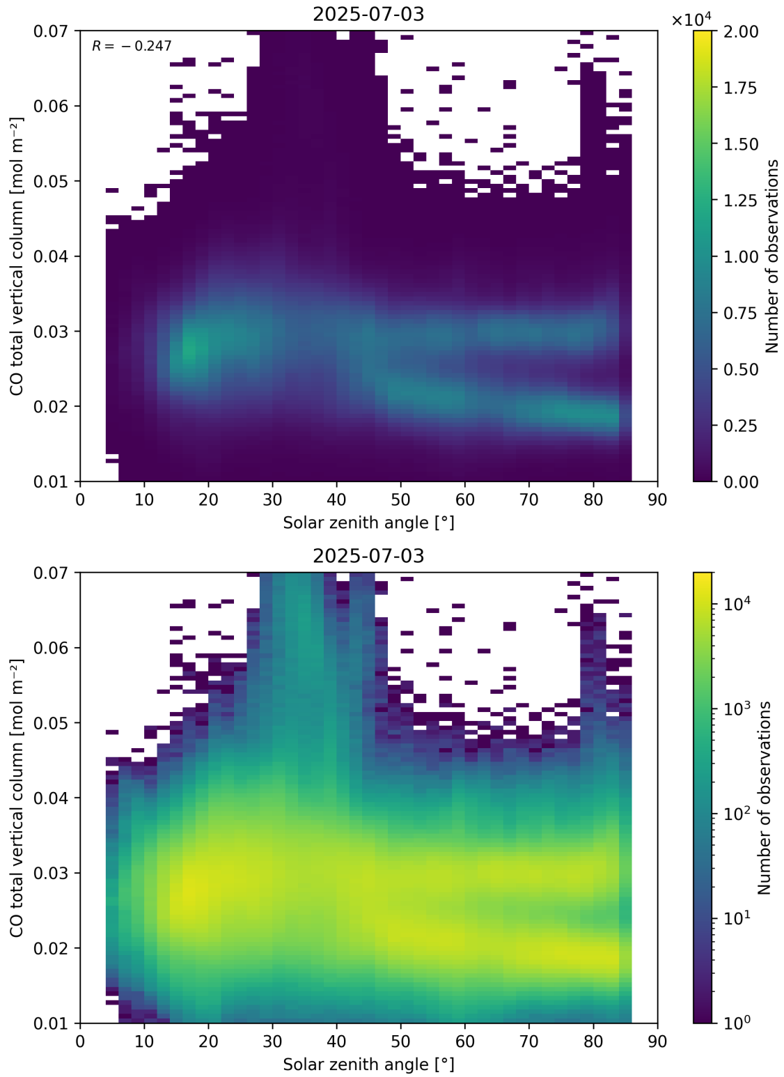
Figure 61: Scatter density plot of “Solar zenith angle” against “CO total vertical column” for 2025-07-03 to 2025-07-04.
