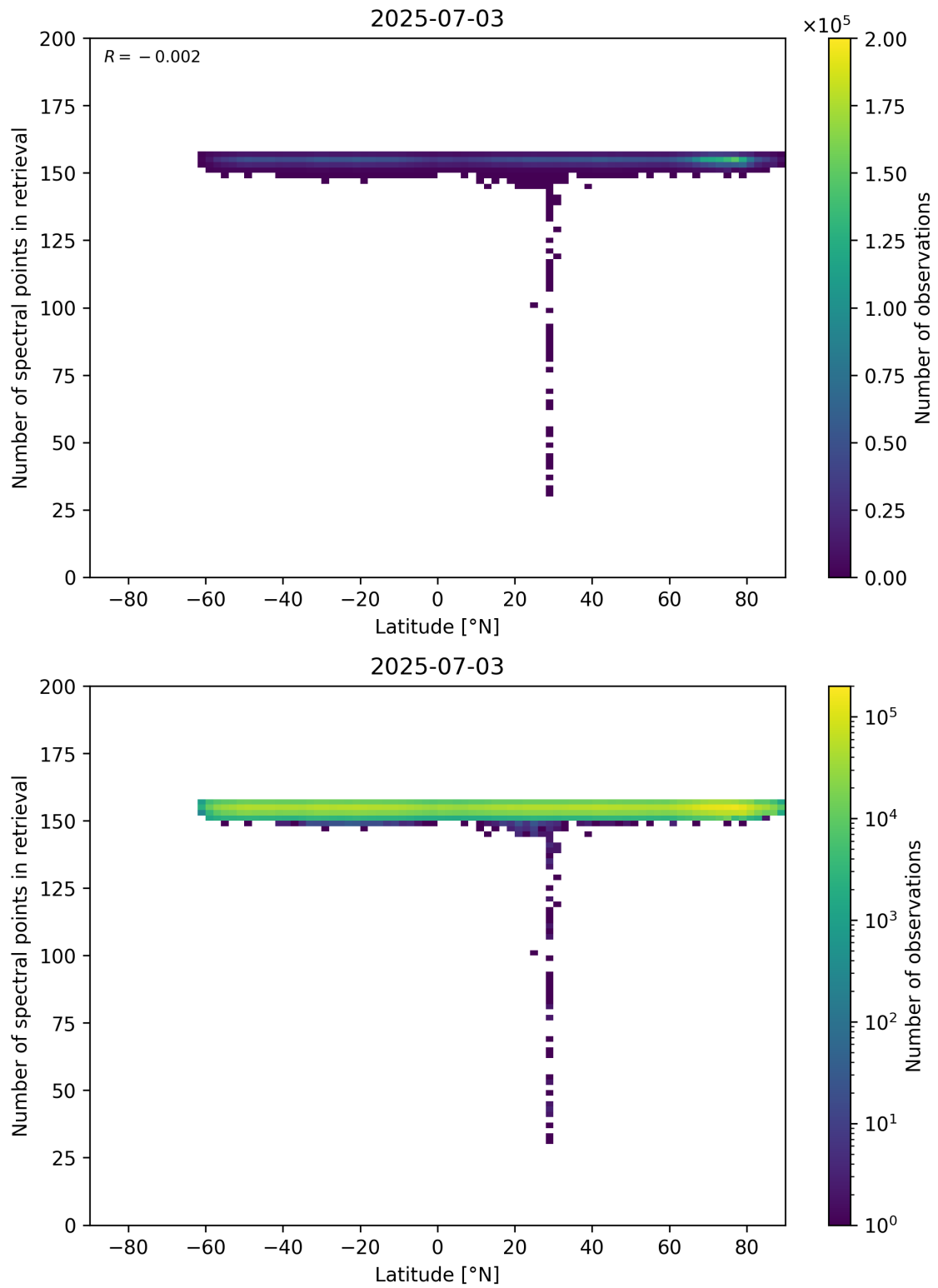
Figure 57: Scatter density plot of “Latitude” against “Number of spectral points in retrieval” for 2025-07-03 to 2025-07-04.
