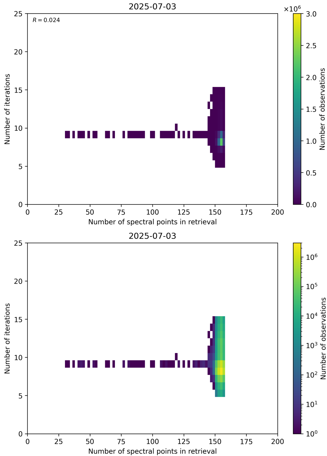
Figure 60: Scatter density plot of “Number of spectral points in retrieval” against “Number of iterations” for 2025-07-03 to 2025-07-04.
