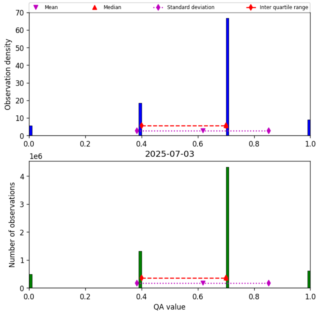
Figure 17: Histogram of “QA value” for 2025-07-03 to 2025-07-04
