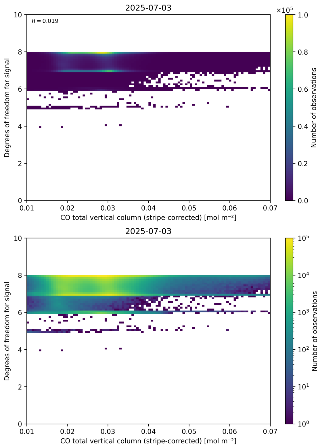
Figure 38: Scatter density plot of “CO total vertical column (stripe-corrected)” against “Degrees of freedom for signal” for 2025-07-03 to 2025-07-04.
