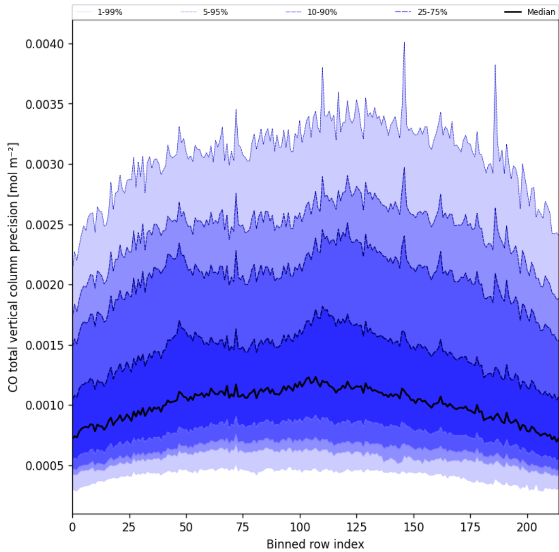
Figure 28: Along track statistics of “CO total vertical column precision” for 2025-07-03 to 2025-07-04
