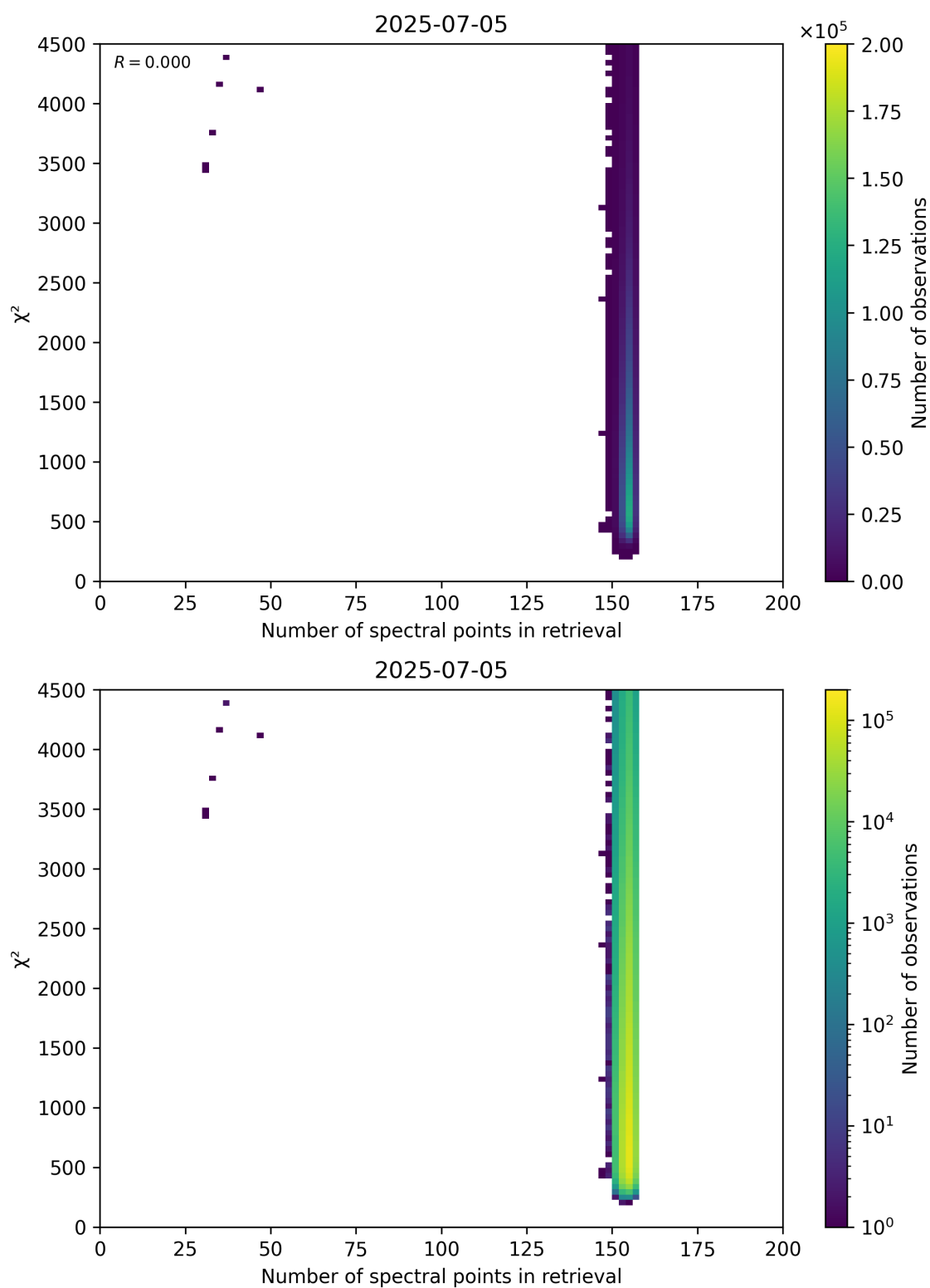
Figure 58: Scatter density plot of “Number of spectral points in retrieval” against “ \chi^2 ” for 2025-07-04 to 2025-07-06.
