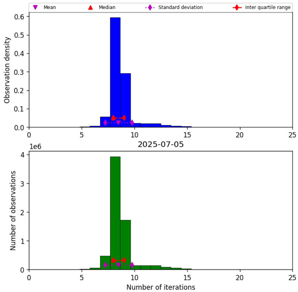
Figure 24: Histogram of “Number of iterations” for 2025-07-04 to 2025-07-06
