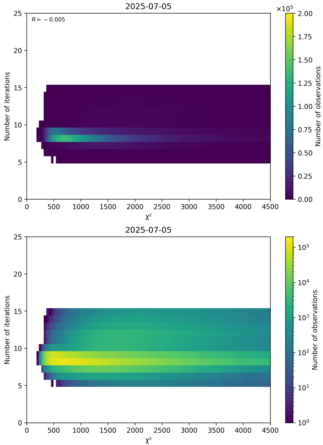
Figure 49: Scatter density plot of “ \chi^2 ” against “Number of iterations” for 2025-07-04 to 2025-07-06.
