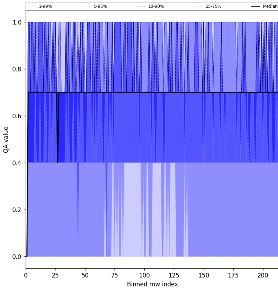
Figure 25: Along track statistics of “QA value” for 2025-07-04 to 2025-07-06
