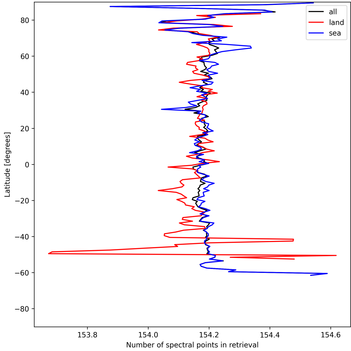
Figure 13: Zonal average of “Number of spectral points in retrieval” for 2025-07-04 to 2025-07-06.
