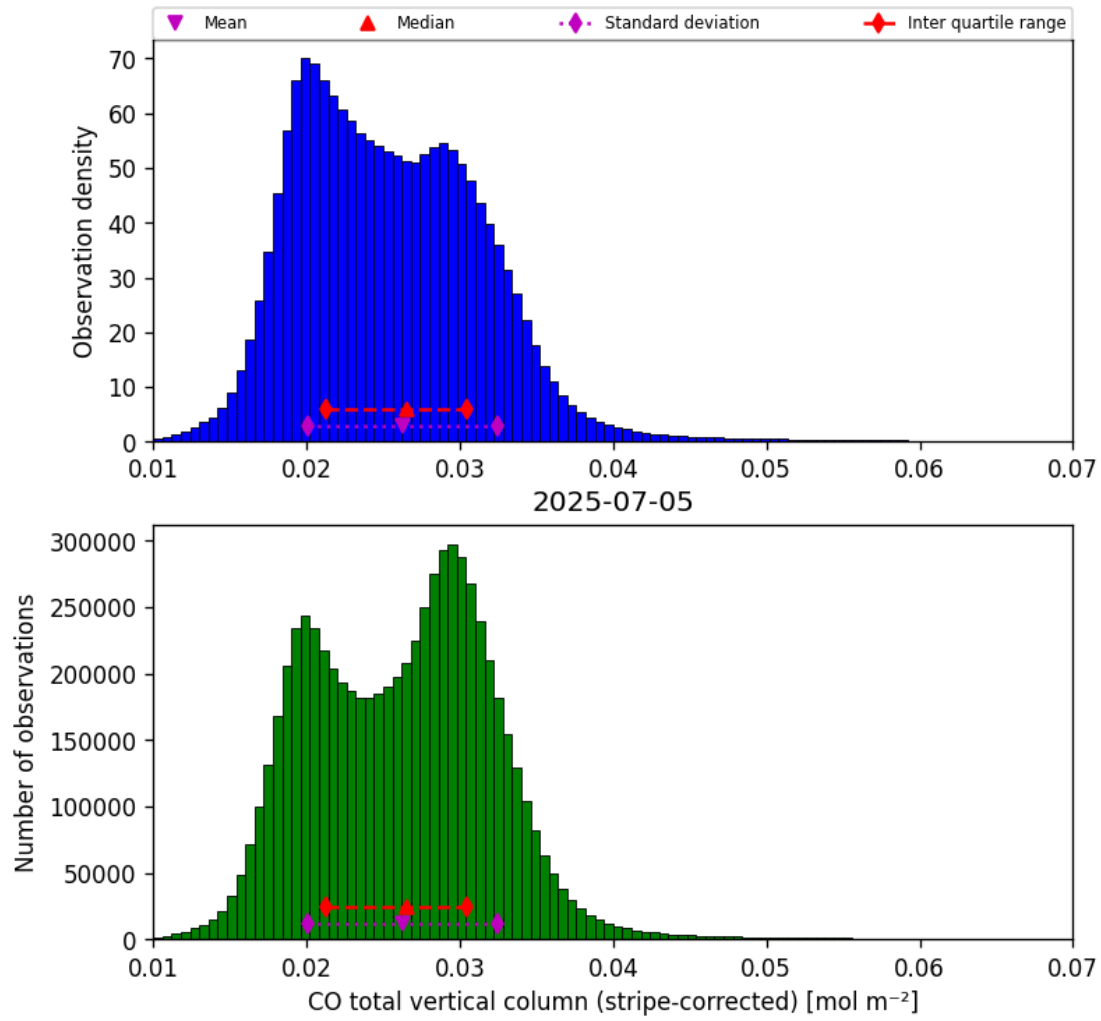
Figure 19: Histogram of “CO total vertical column (stripe-corrected)” for 2025-07-04 to 2025-07-06
