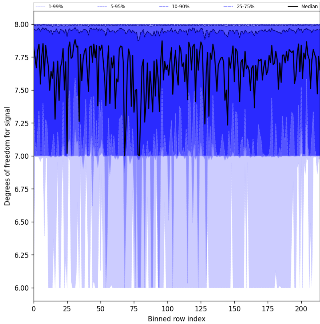
Figure 31: Along track statistics of “Degrees of freedom for signal” for 2025-07-04 to 2025-07-06
