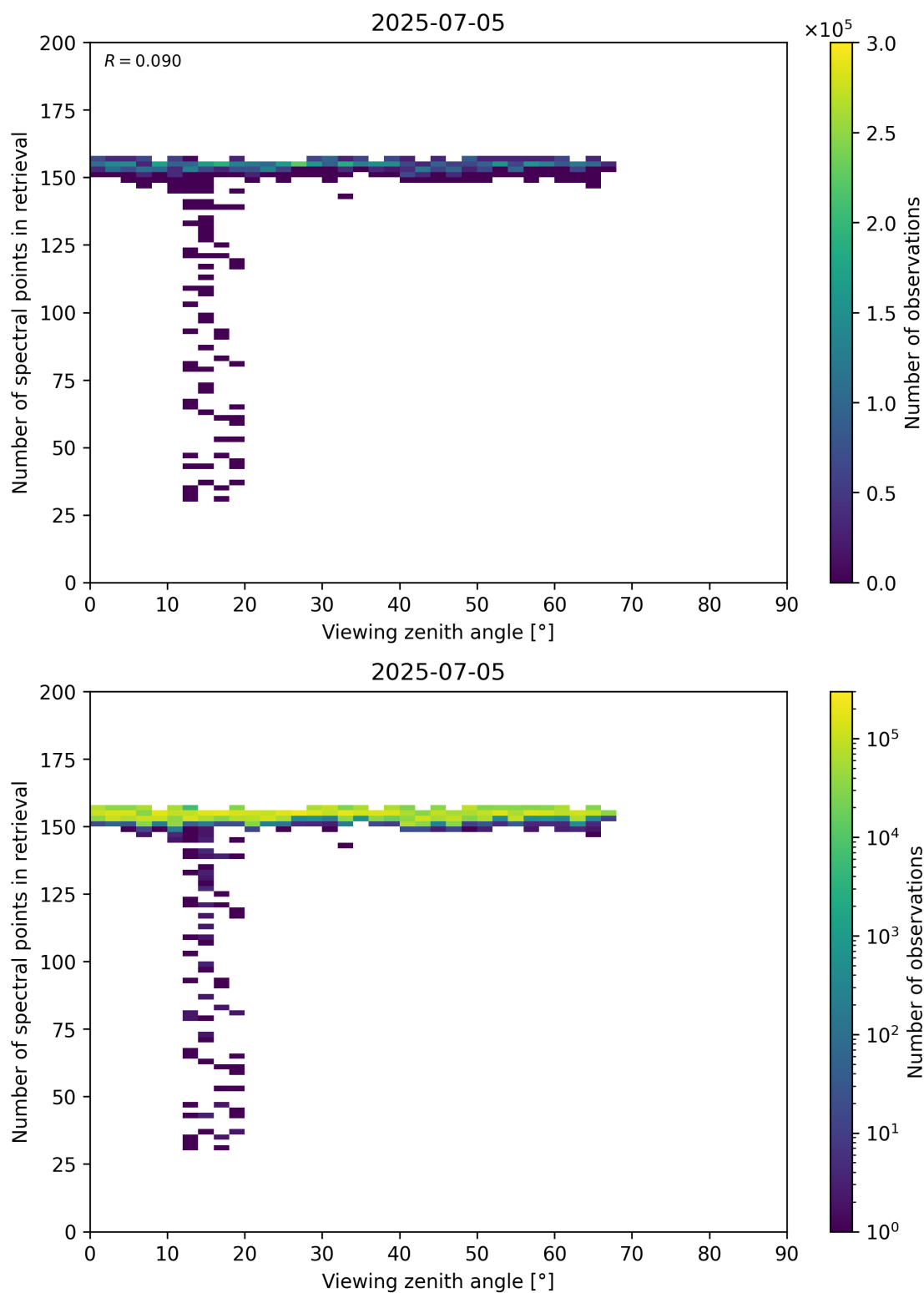
Figure 76: Scatter density plot of “Viewing zenith angle” against “Number of spectral points in retrieval” for 2025-07-04 to 2025-07-06.
