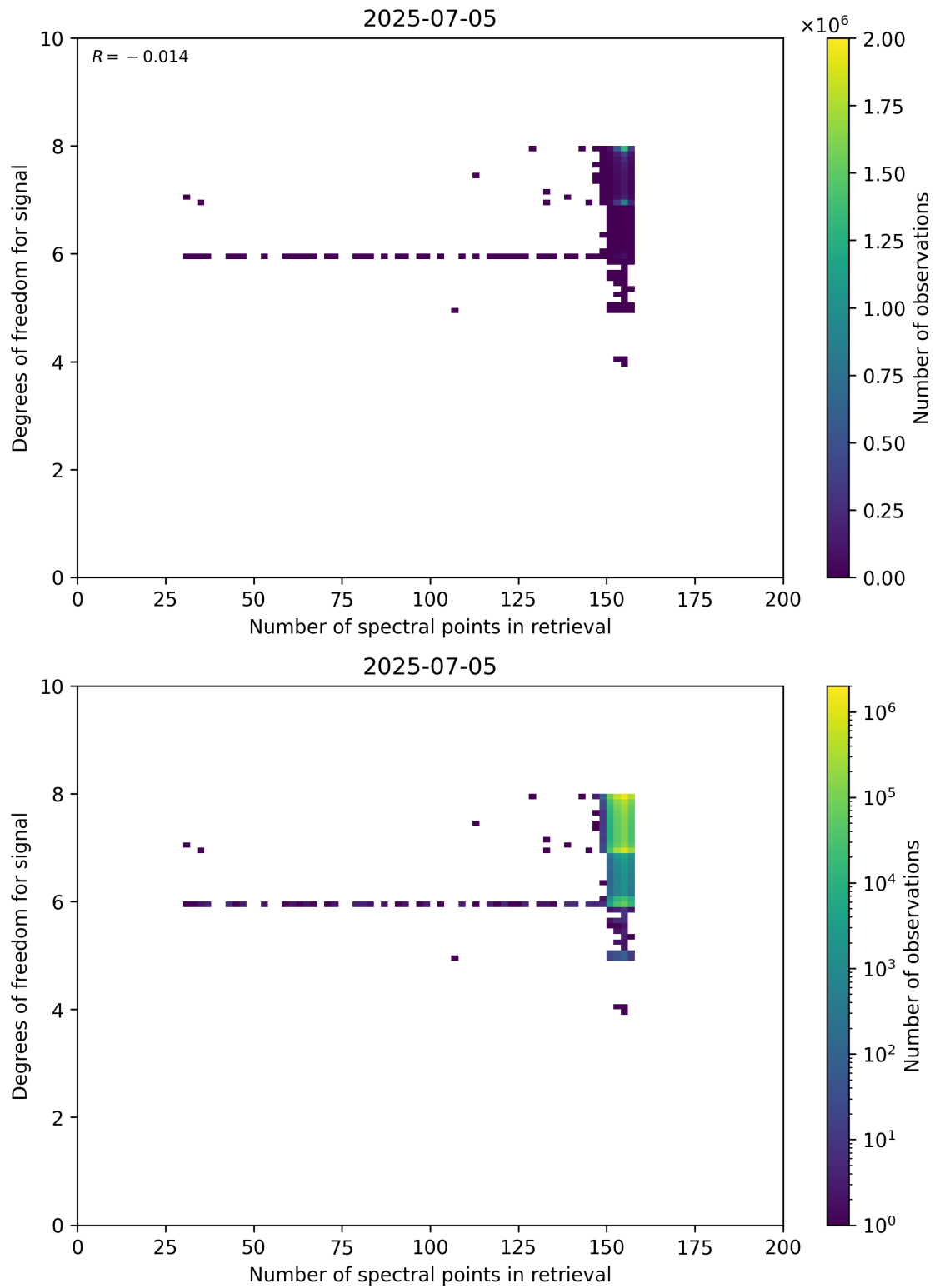
Figure 59: Scatter density plot of “Number of spectral points in retrieval” against “Degrees of freedom for signal” for 2025-07-04 to 2025-07-06.
