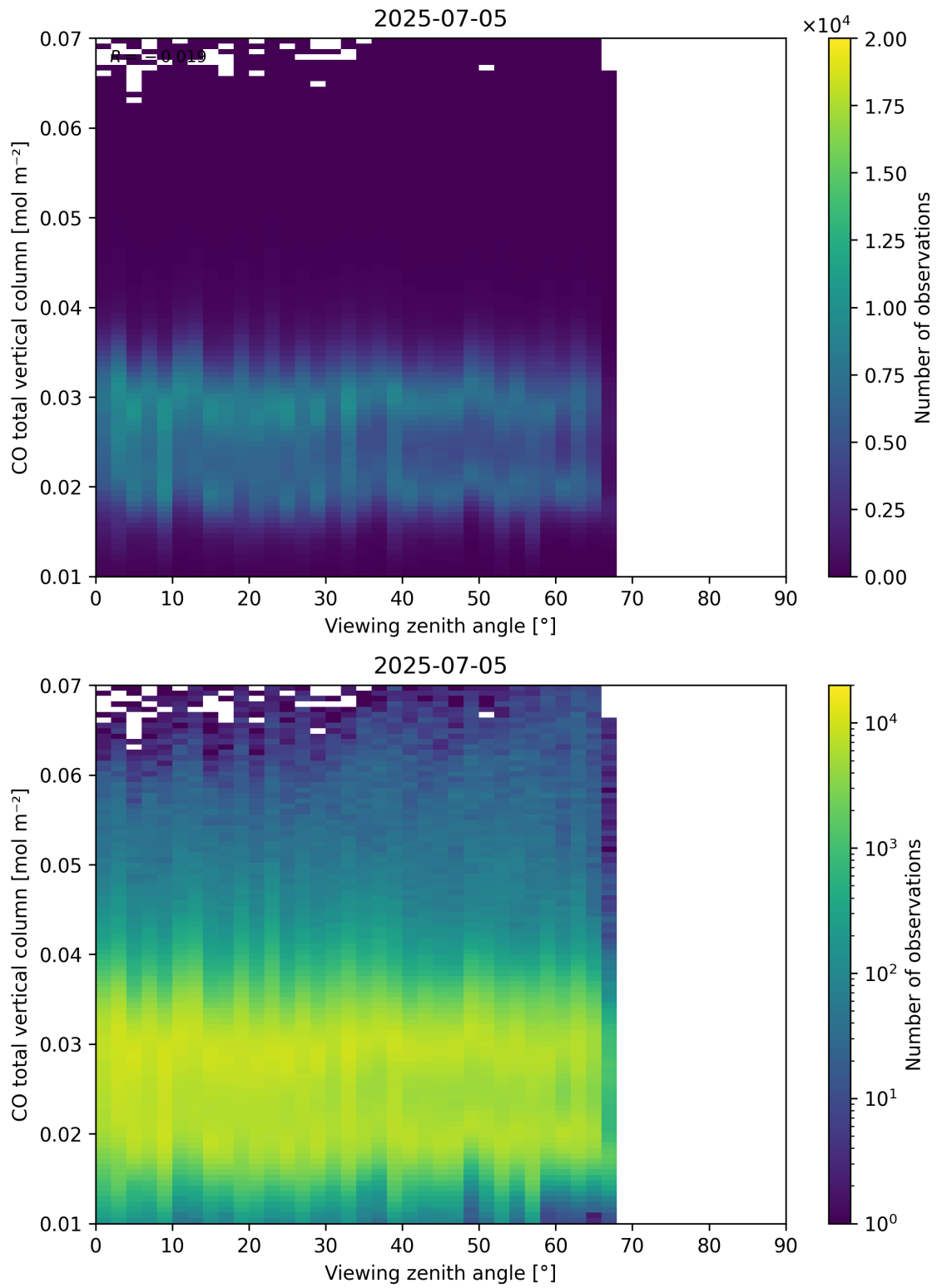
Figure 69: Scatter density plot of “Viewing zenith angle” against “CO total vertical column” for 2025-07-04 to 2025-07-06.
