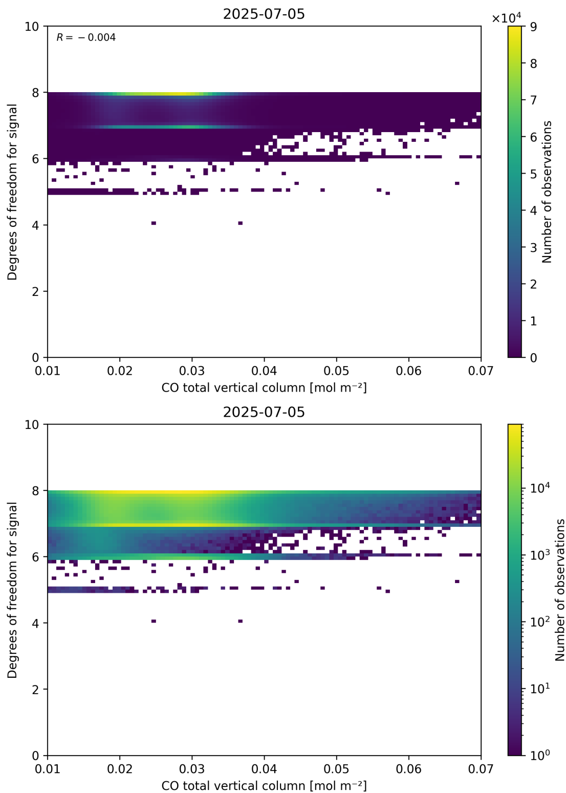
Figure 41: Scatter density plot of “CO total vertical column” against “Degrees of freedom for signal” for 2025-07-04 to 2025-07-06.
