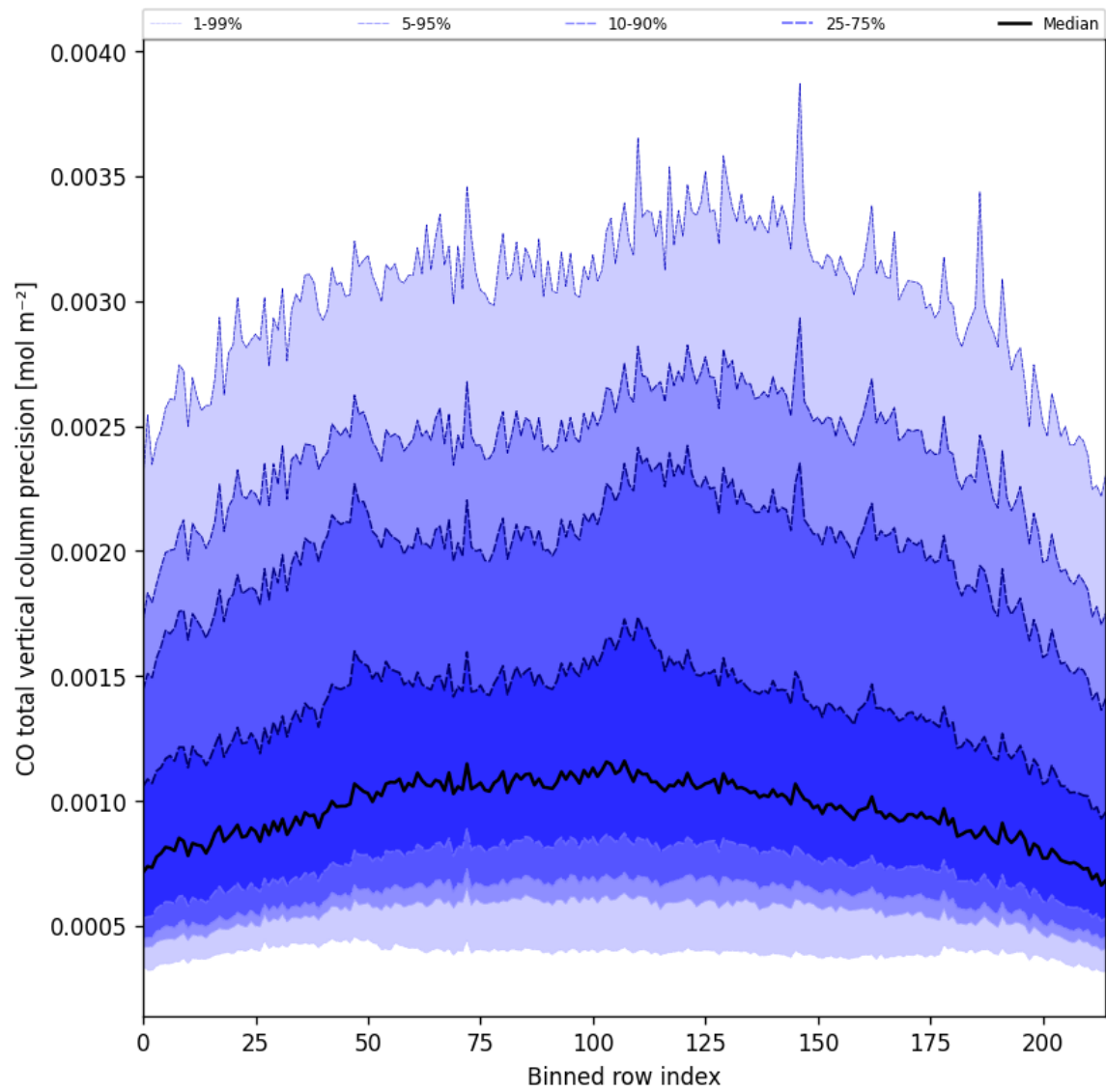
Figure 28: Along track statistics of “CO total vertical column precision” for 2025-07-04 to 2025-07-06
