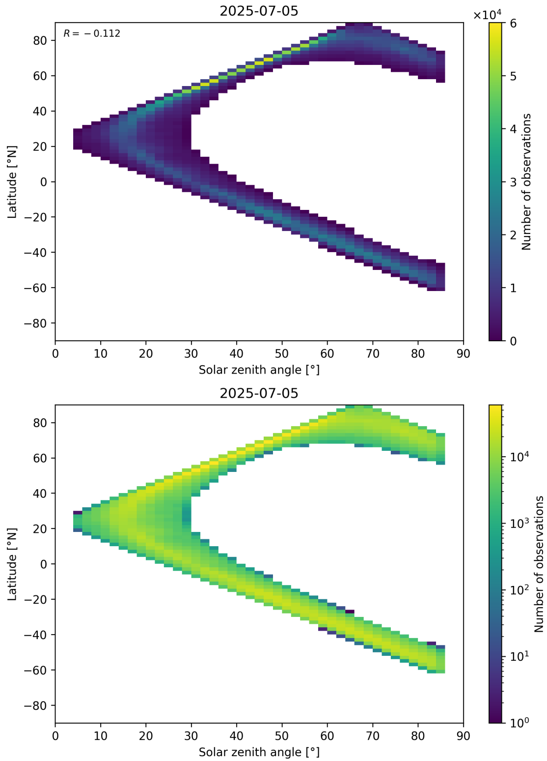
Figure 66: Scatter density plot of “Solar zenith angle” against “Latitude” for 2025-07-04 to 2025-07-06.
