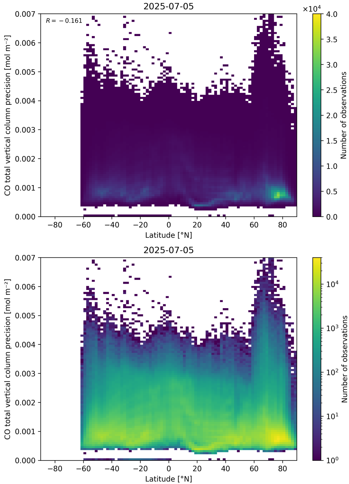
Figure 53: Scatter density plot of “Latitude” against “CO total vertical column precision” for 2025-07-04 to 2025-07-06.
