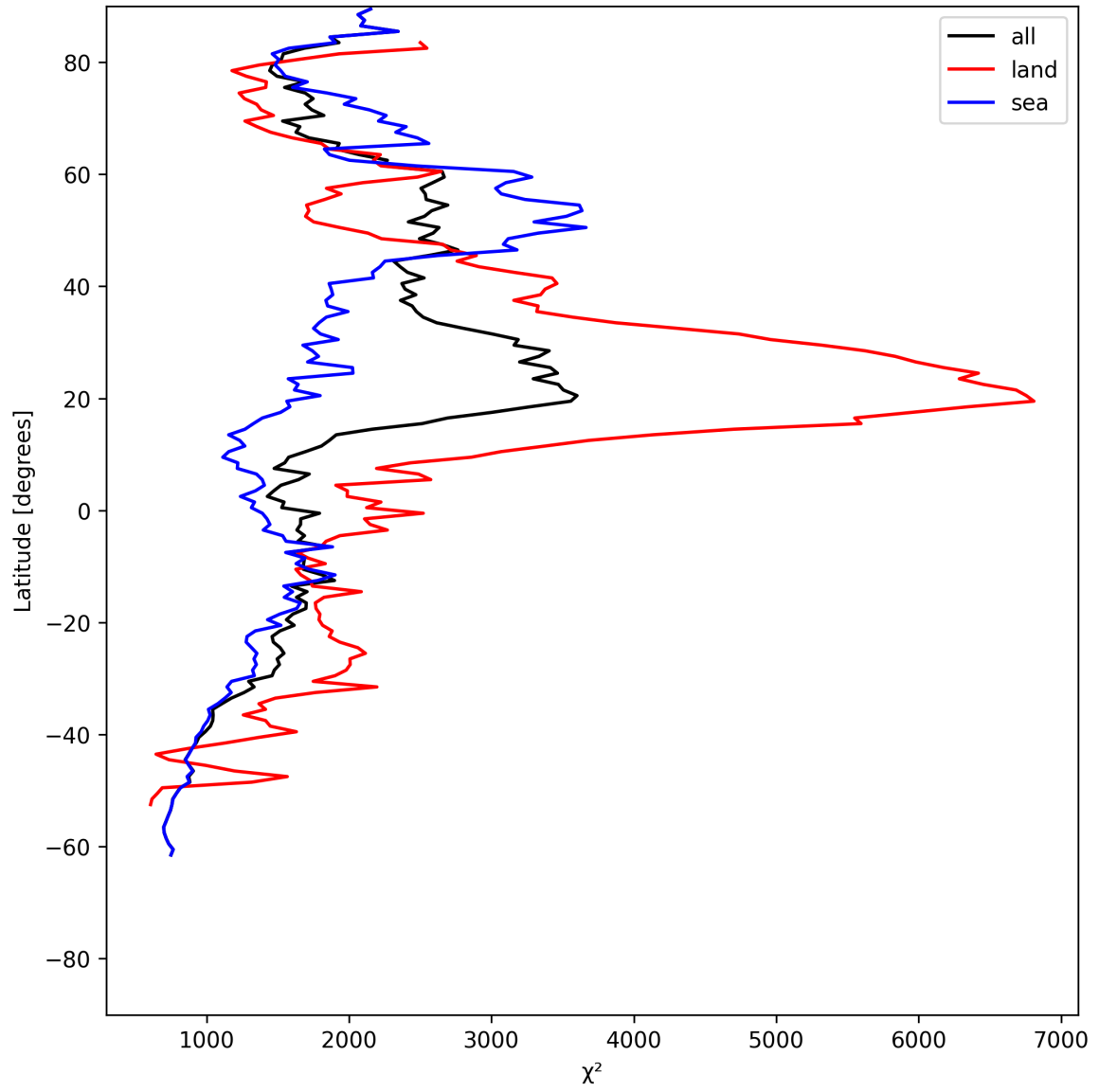
Figure 14: Zonal average of “ \chi^2 ” for 2025-07-04 to 2025-07-06.
