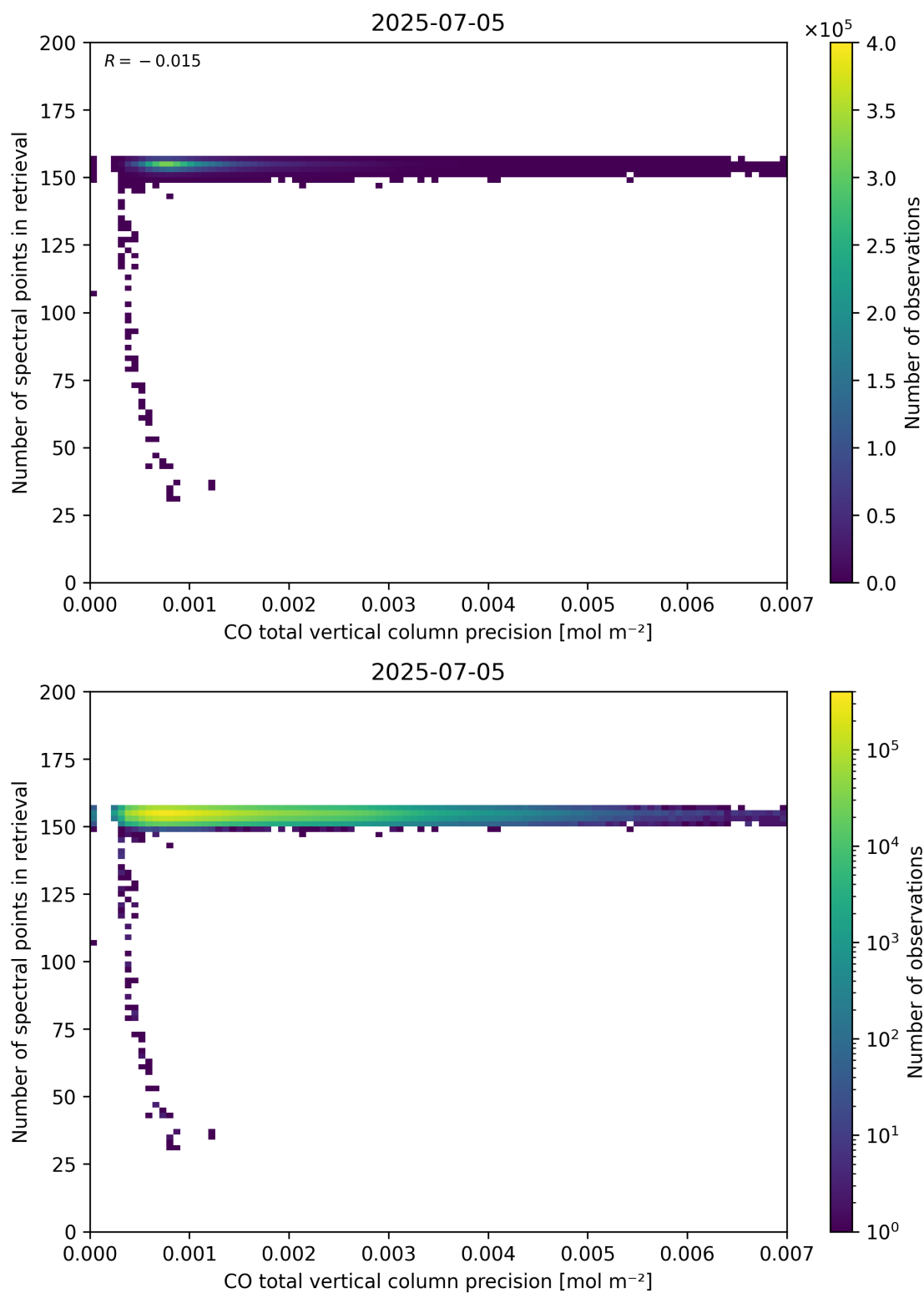
Figure 47: Scatter density plot of “CO total vertical column precision” against “Number of spectral points in retrieval” for 2025-07-04 to 2025-07-06.
