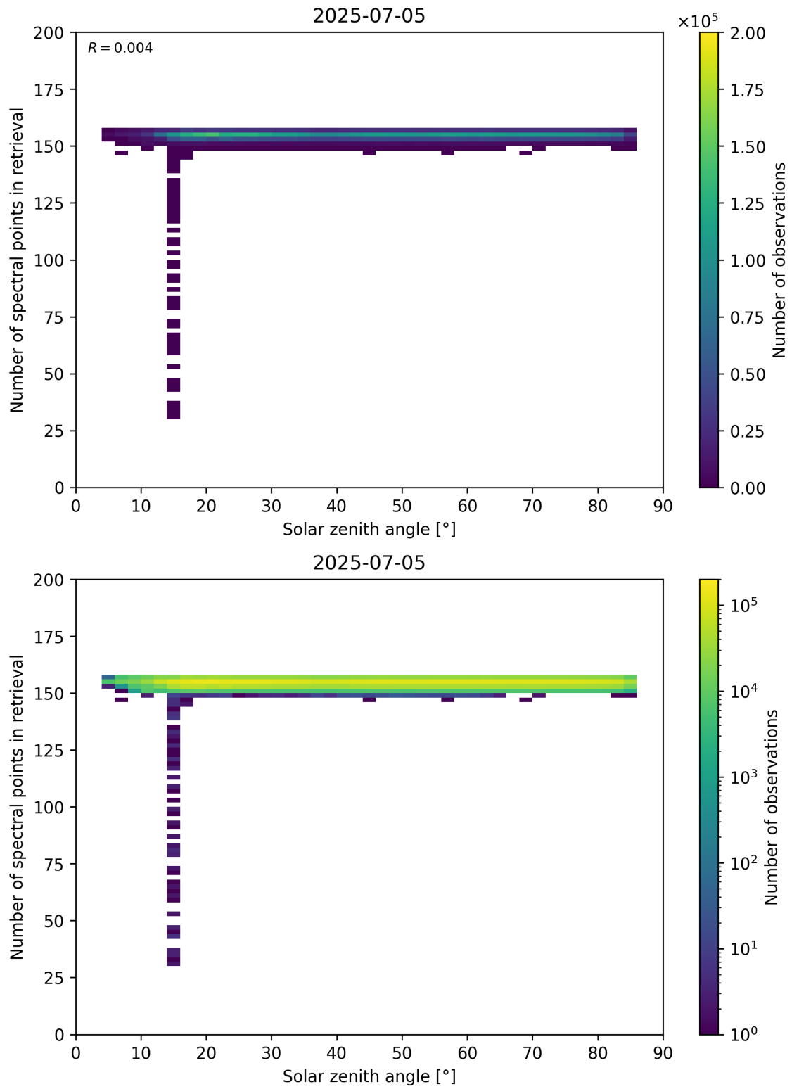
Figure 68: Scatter density plot of “Solar zenith angle” against “Number of spectral points in retrieval” for 2025-07-04 to 2025-07-06.
