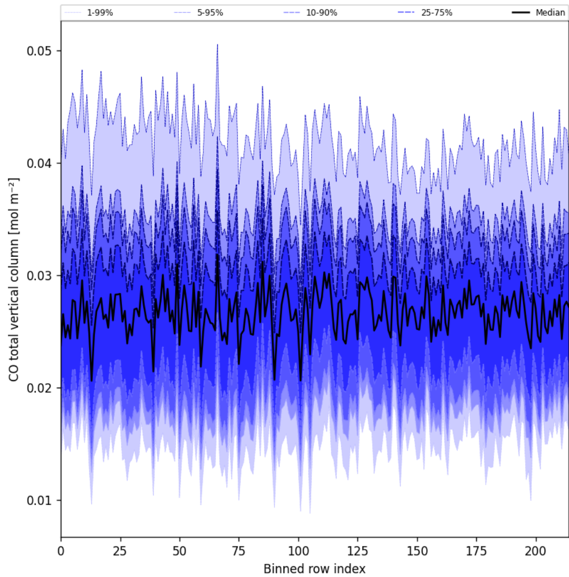
Figure 26: Along track statistics of “CO total vertical column” for 2025-07-04 to 2025-07-06
