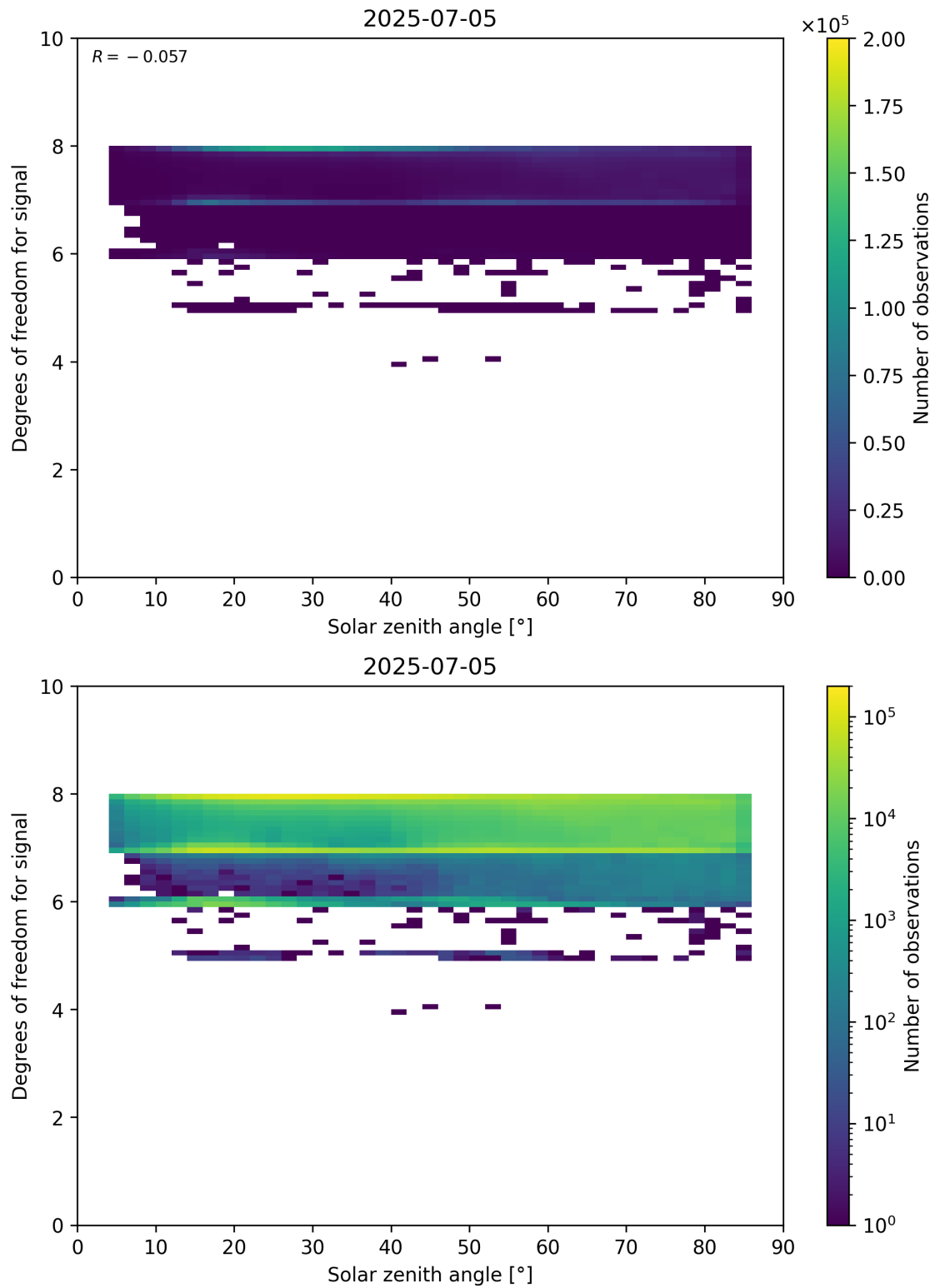
Figure 65: Scatter density plot of “Solar zenith angle” against “Degrees of freedom for signal” for 2025-07-04 to 2025-07-06.
