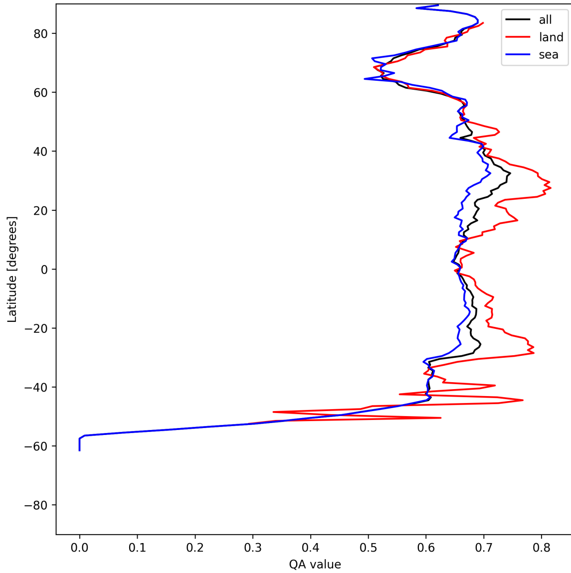
Figure 9: Zonal average of “QA value” for 2025-07-04 to 2025-07-06.
