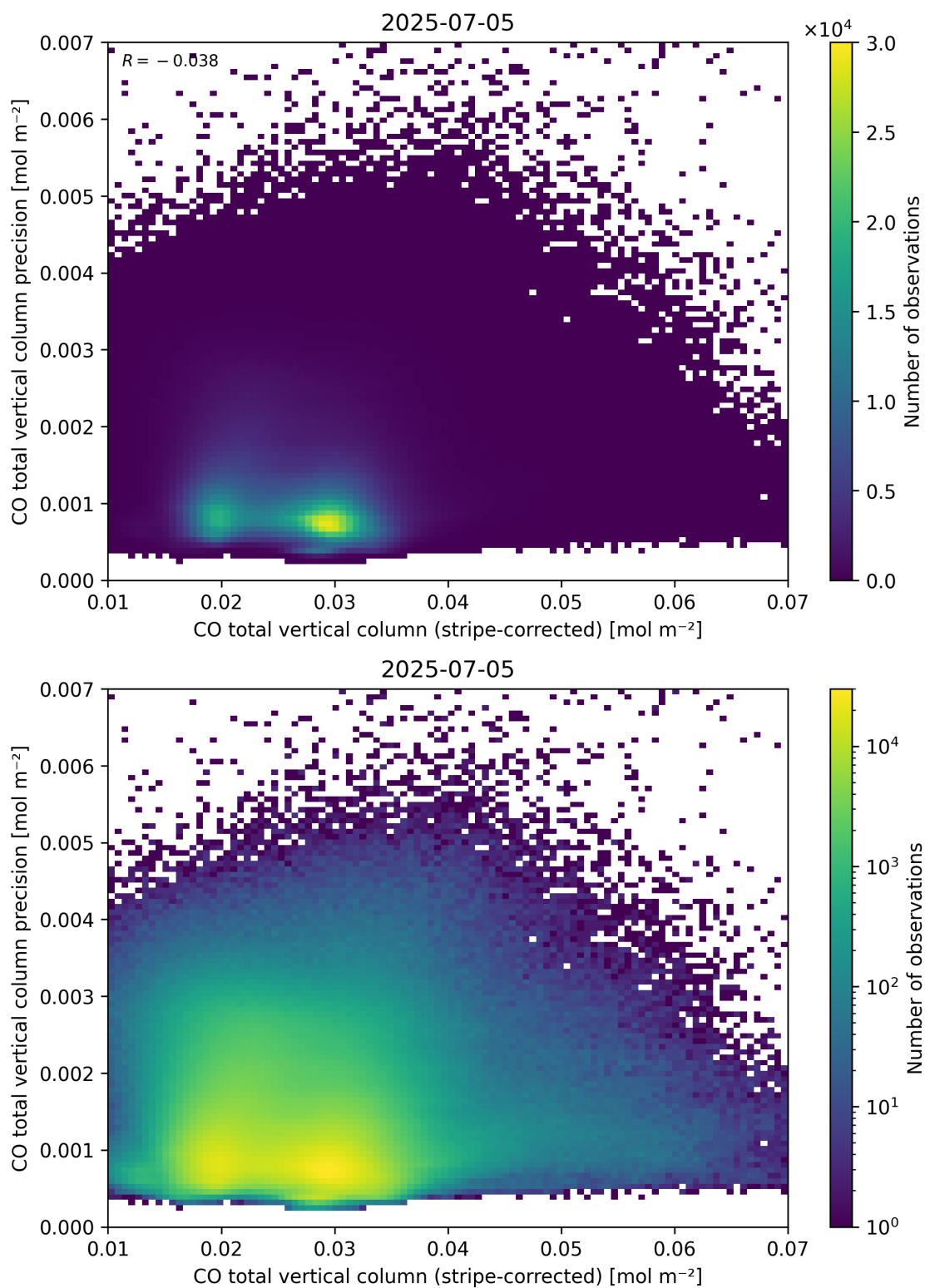
Figure 36: Scatter density plot of “CO total vertical column (stripe-corrected)” against “CO total vertical column precision” for 2025-07-04 to 2025-07-06.
