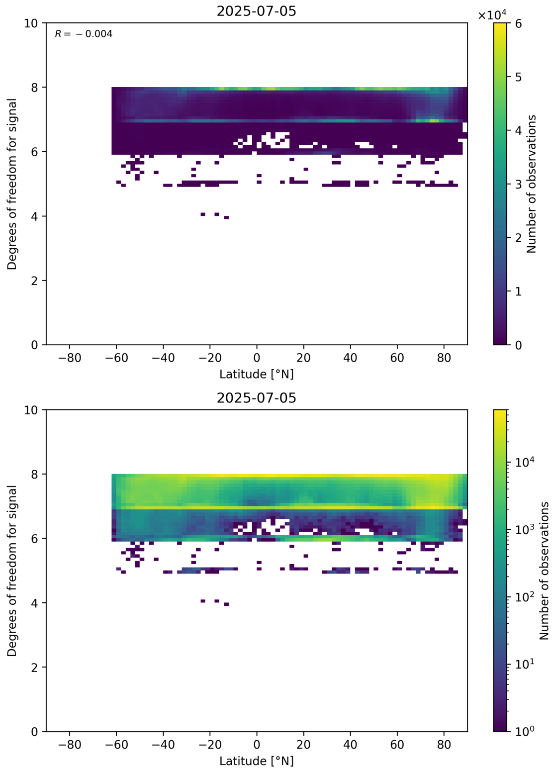
Figure 55: Scatter density plot of “Latitude” against “Degrees of freedom for signal” for 2025-07-04 to 2025-07-06.
