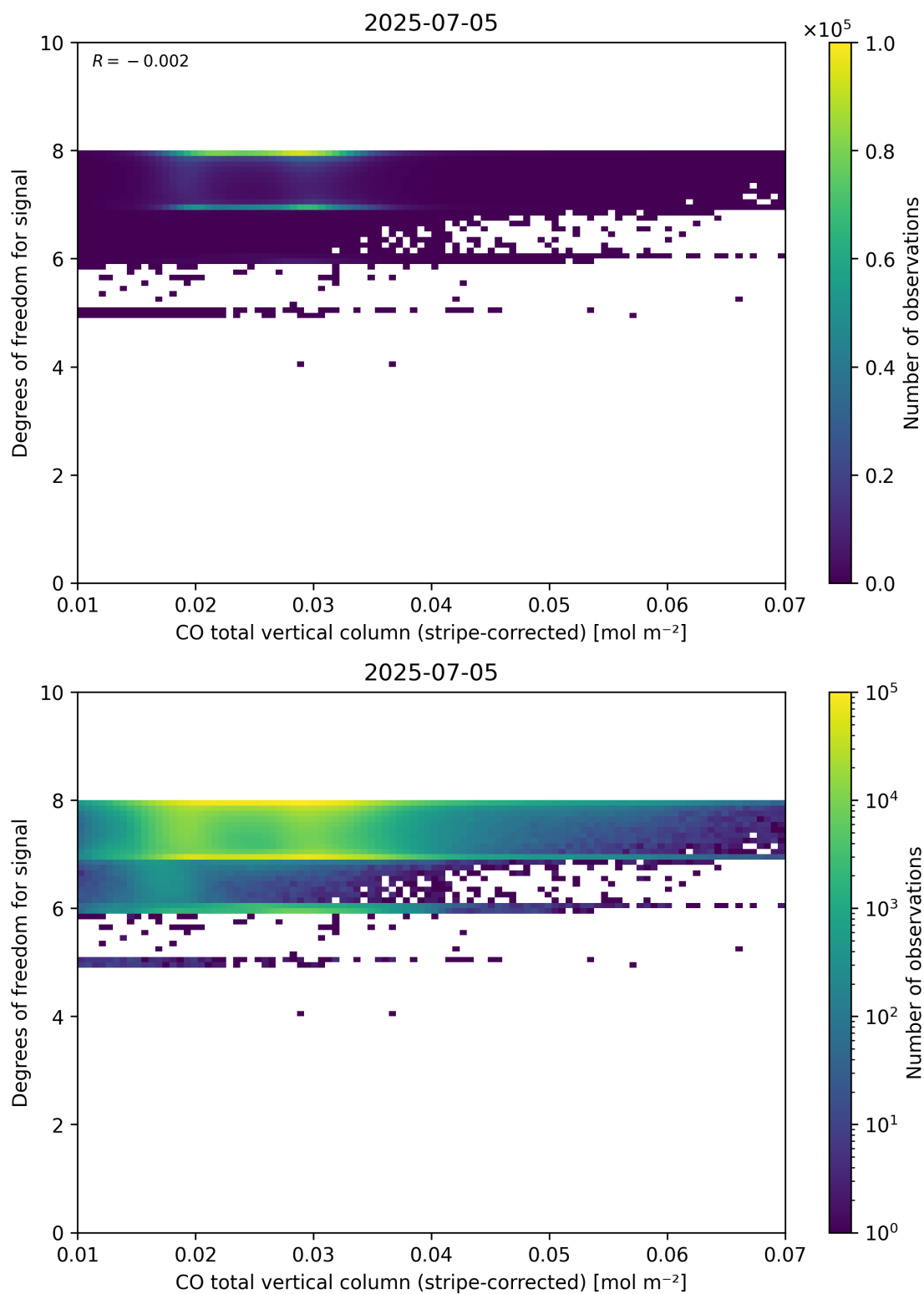
Figure 38: Scatter density plot of “CO total vertical column (stripe-corrected)” against “Degrees of freedom for signal” for 2025-07-04 to 2025-07-06.
