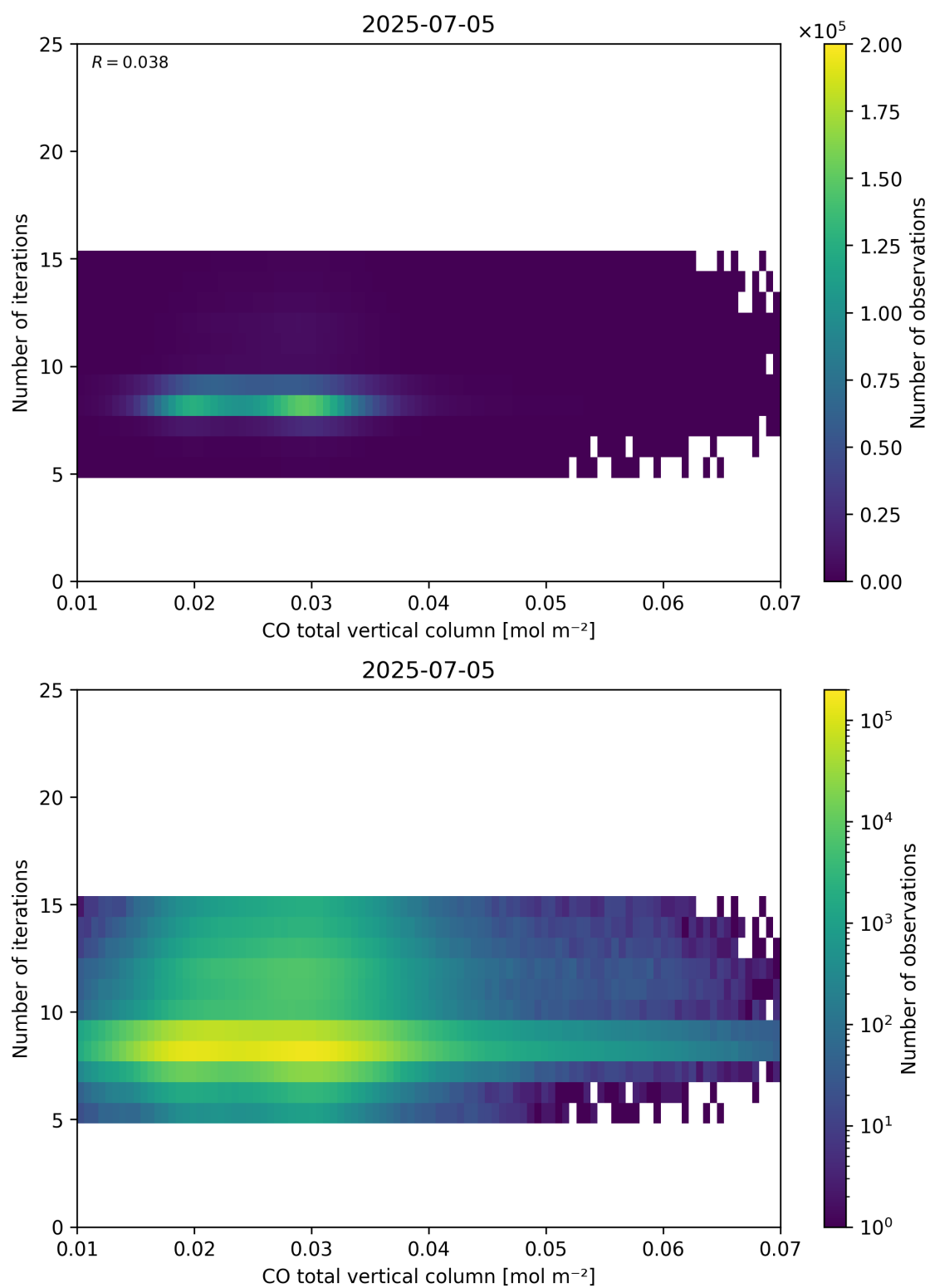
Figure 42: Scatter density plot of “CO total vertical column” against “Number of iterations” for 2025-07-04 to 2025-07-06.
