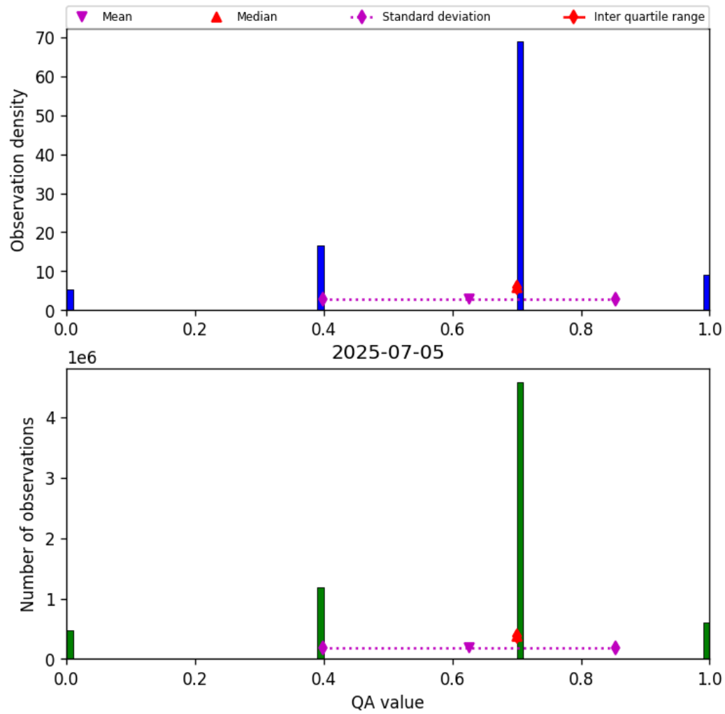
Figure 17: Histogram of “QA value” for 2025-07-04 to 2025-07-06
