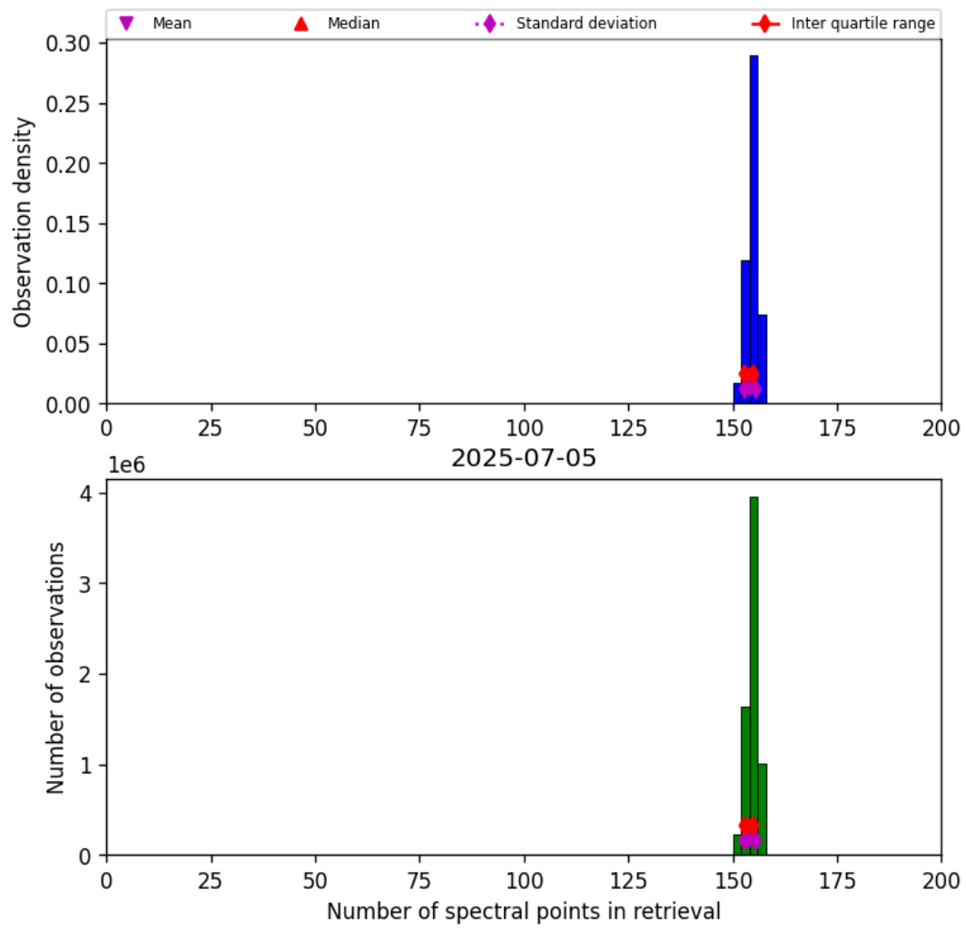
Figure 21: Histogram of “Number of spectral points in retrieval” for 2025-07-04 to 2025-07-06
