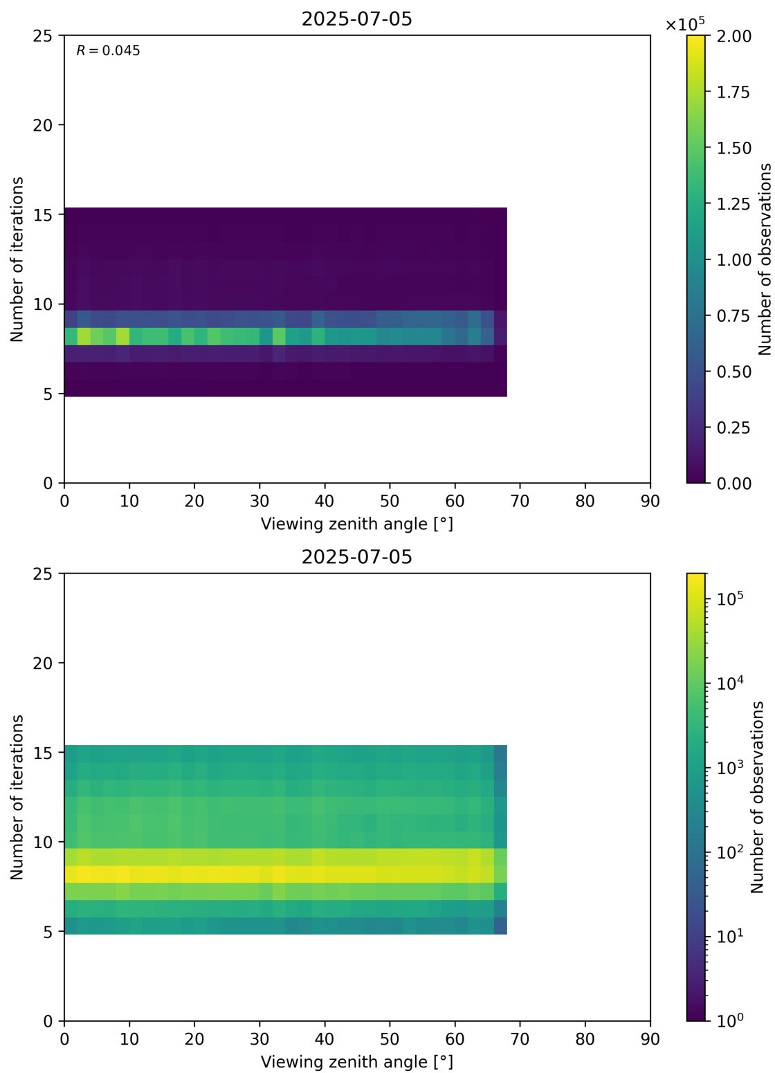
Figure 75: Scatter density plot of “Viewing zenith angle” against “Number of iterations” for 2025-07-04 to 2025-07-06.
