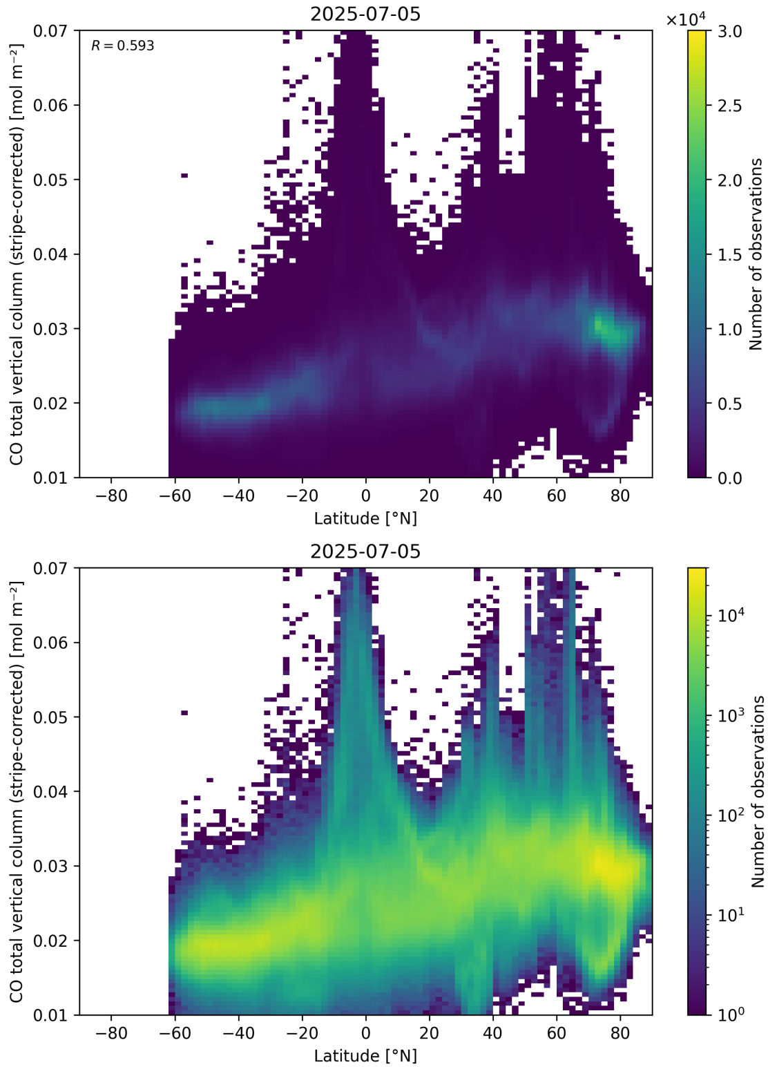
Figure 52: Scatter density plot of “Latitude” against “CO total vertical column (stripe-corrected)” for 2025-07-04 to 2025-07-06.
