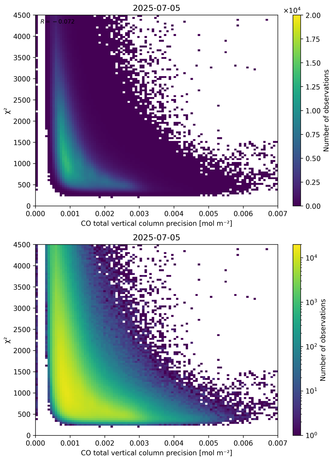
Figure 44: Scatter density plot of “CO total vertical column precision” against “ \chi^2 ” for 2025-07-04 to 2025-07-06.
