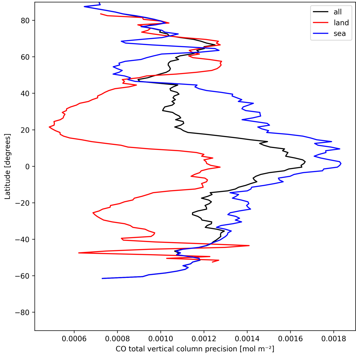
Figure 12: Zonal average of "CO total vertical column precision" for 2025-07-04 to 2025-07-06.
