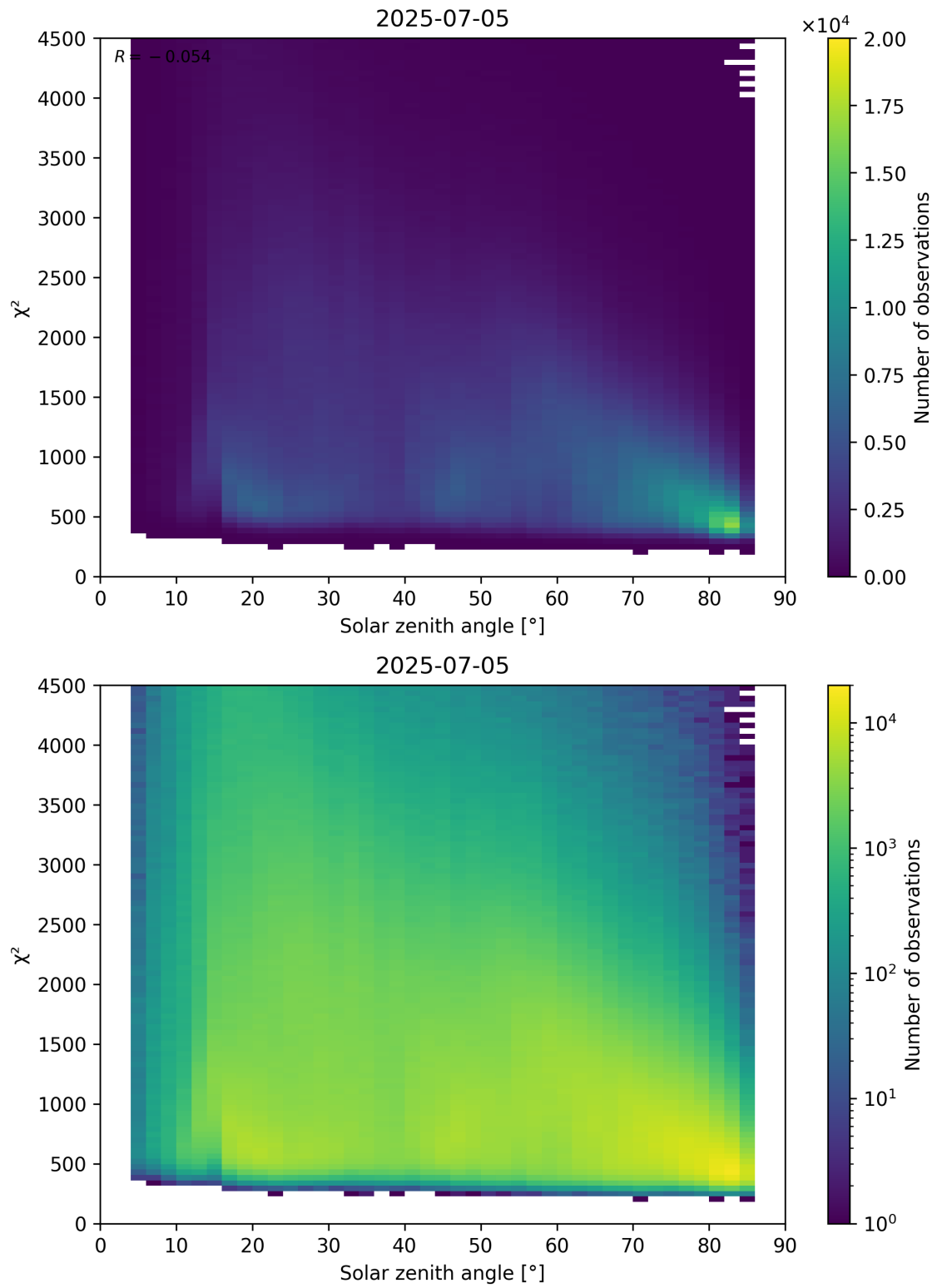
Figure 64: Scatter density plot of “Solar zenith angle” against “ \chi^2 ” for 2025-07-04 to 2025-07-06.
