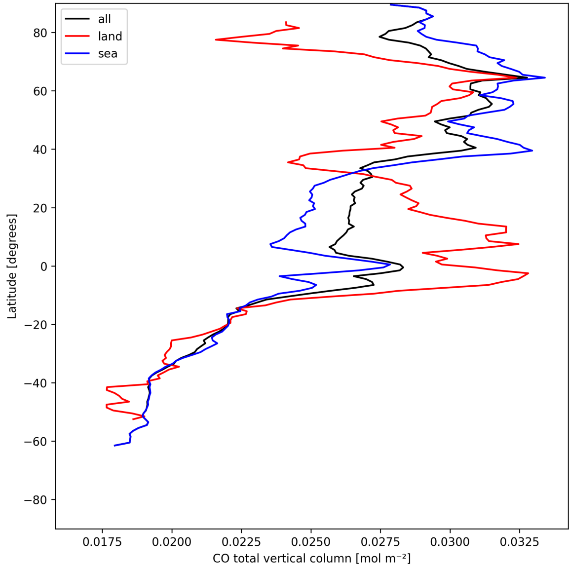
Figure 10: Zonal average of “CO total vertical column” for 2025-07-04 to 2025-07-06.
