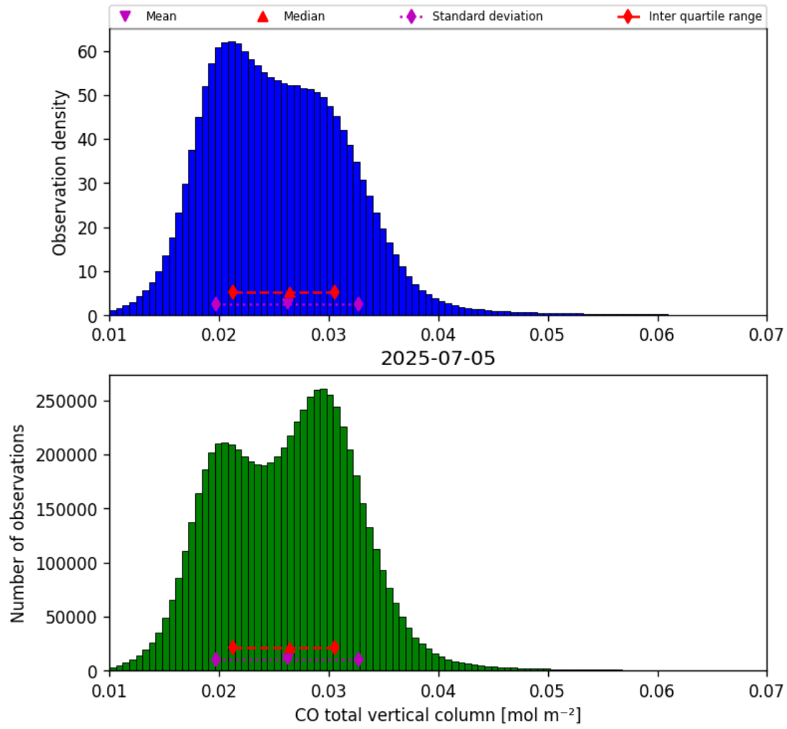
Figure 18: Histogram of “CO total vertical column” for 2025-07-04 to 2025-07-06
