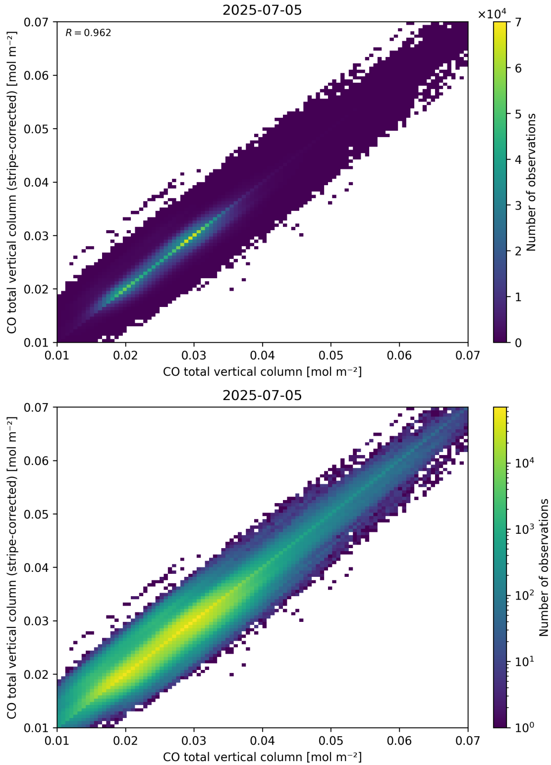
Figure 33: Scatter density plot of “CO total vertical column” against “CO total vertical column (stripe-corrected)” for 2025-07-04 to 2025-07-06.
