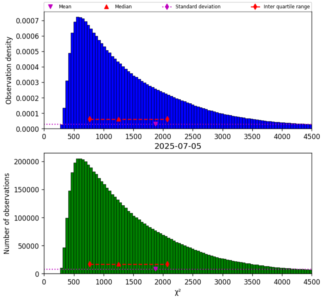
Figure 22: Histogram of “ \chi^2 ” for 2025-07-04 to 2025-07-06
