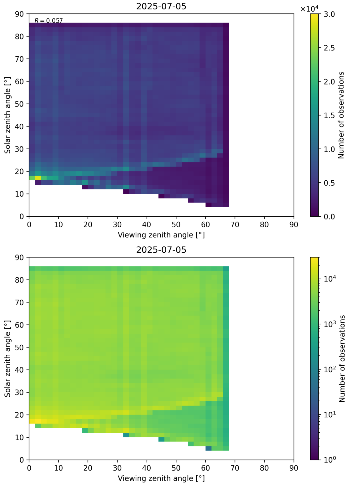
Figure 77: Scatter density plot of “Viewing zenith angle” against “Solar zenith angle” for 2025-07-04 to 2025-07-06.
