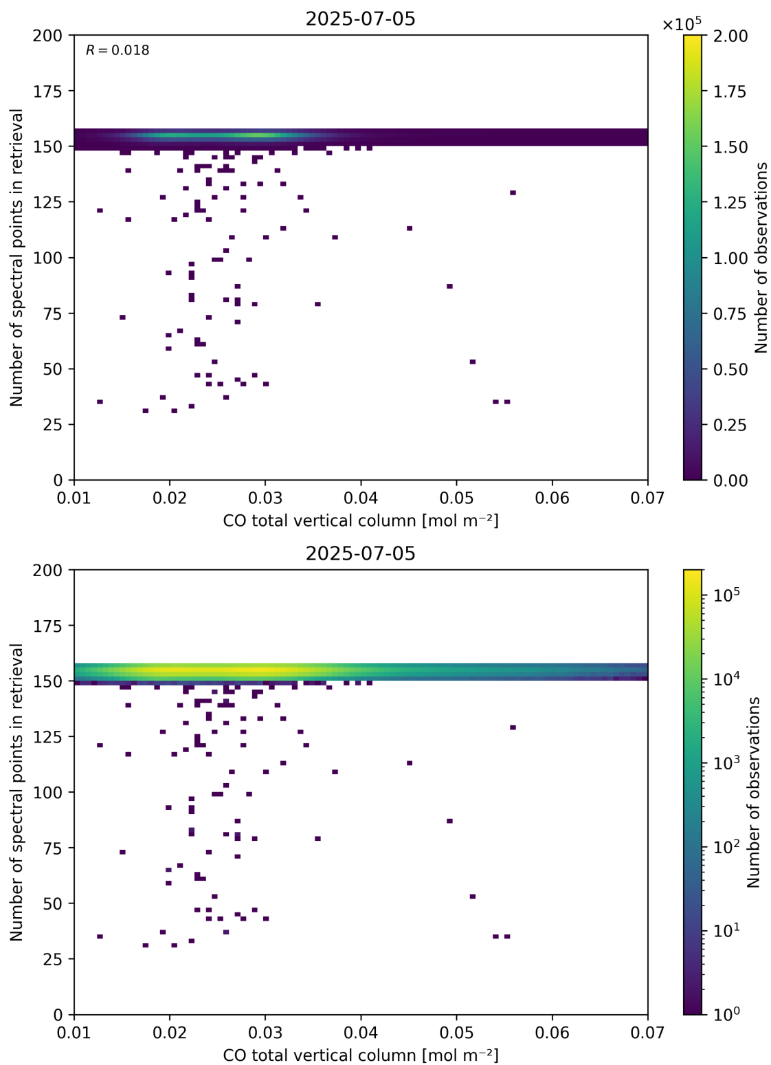
Figure 43: Scatter density plot of “CO total vertical column” against “Number of spectral points in retrieval” for 2025-07-04 to 2025-07-06.
