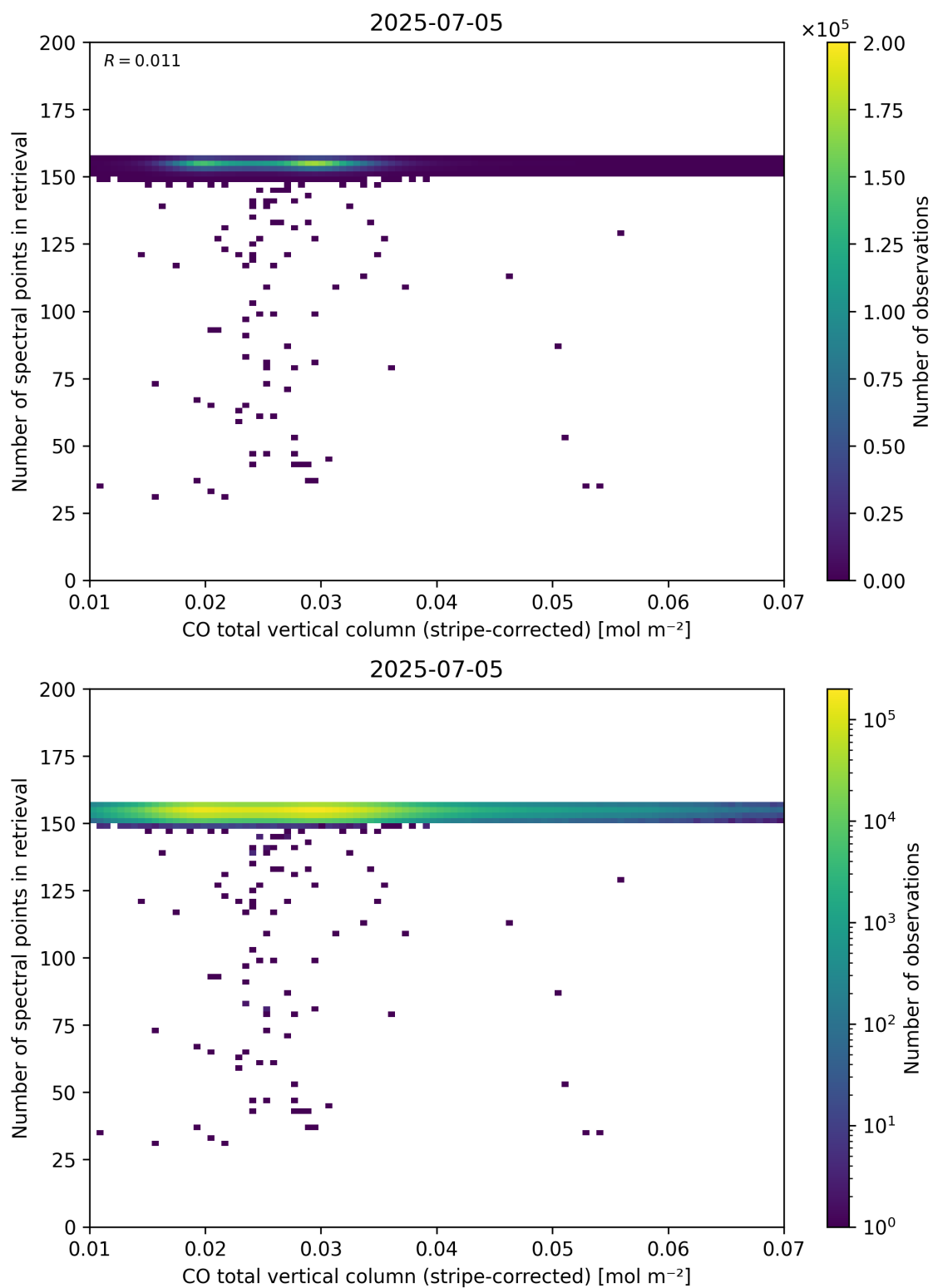
Figure 40: Scatter density plot of “CO total vertical column (stripe-corrected)” against “Number of spectral points in retrieval” for 2025-07-04 to 2025-07-06.
