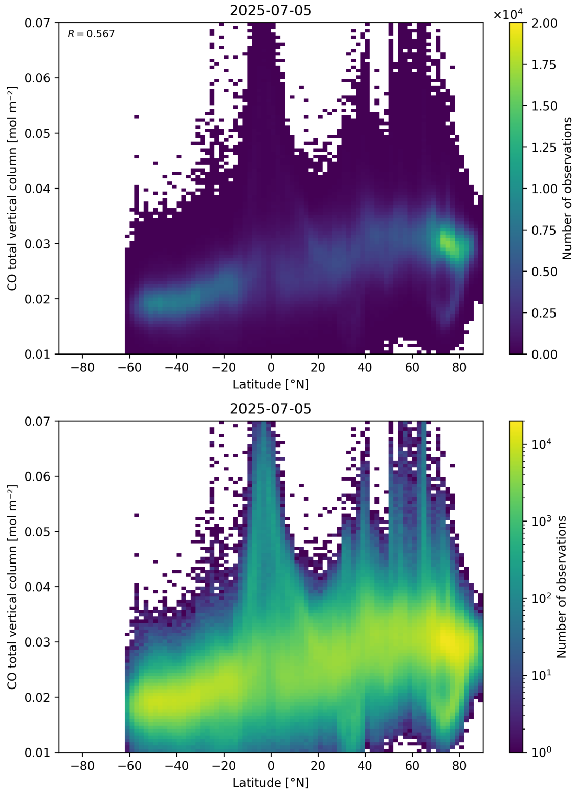
Figure 51: Scatter density plot of “Latitude” against “CO total vertical column” for 2025-07-04 to 2025-07-06.
