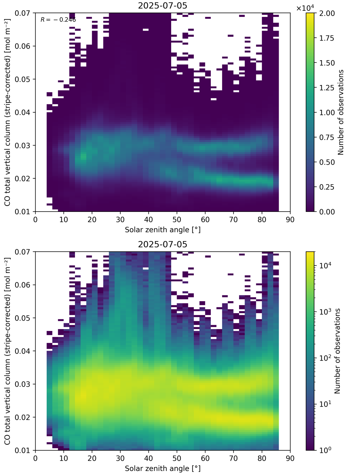
Figure 62: Scatter density plot of “Solar zenith angle” against “CO total vertical column (stripe-corrected)” for 2025-07-04 to 2025-07-06.
