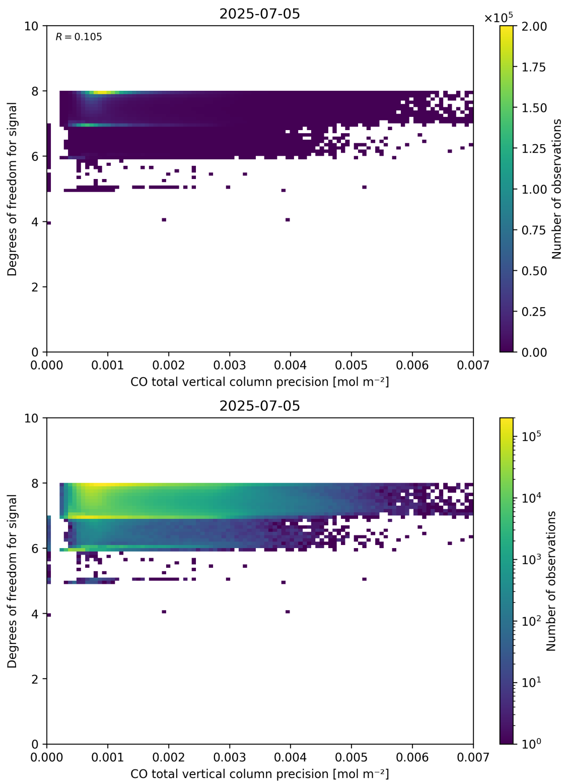
Figure 45: Scatter density plot of “CO total vertical column precision” against “Degrees of freedom for signal” for 2025-07-04 to 2025-07-06.
