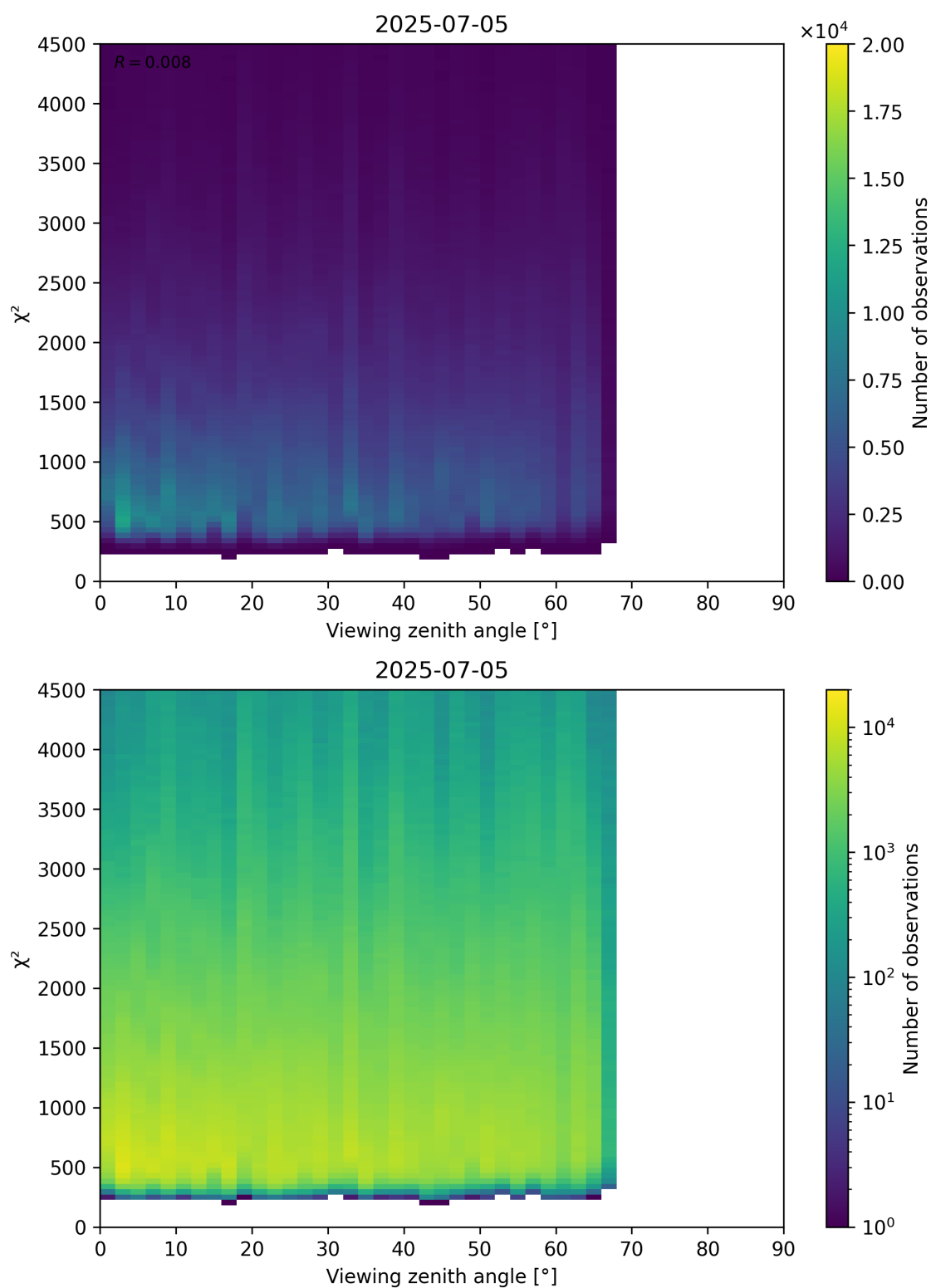
Figure 72: Scatter density plot of “Viewing zenith angle” against “ \chi^2 ” for 2025-07-04 to 2025-07-06.
