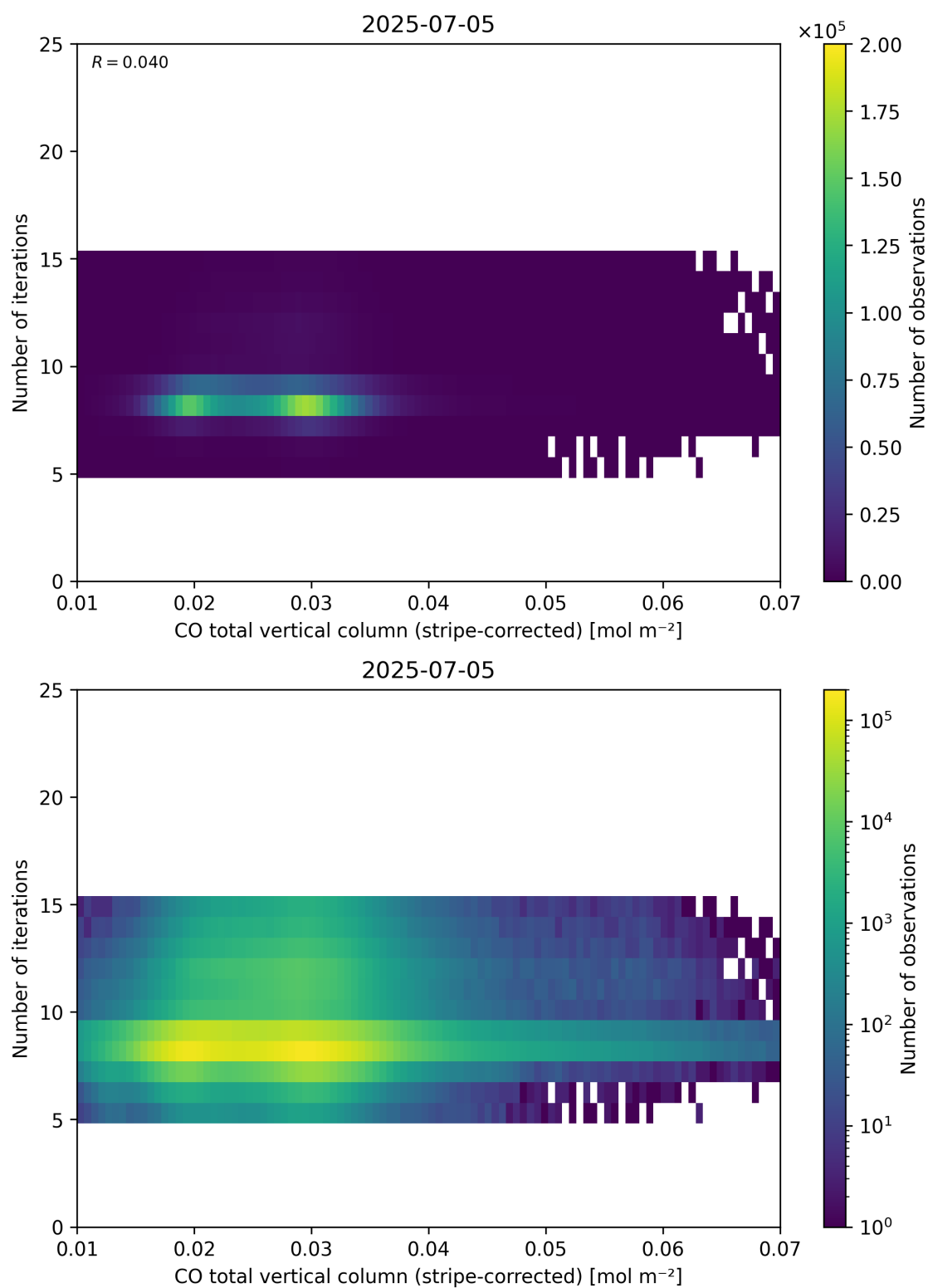
Figure 39: Scatter density plot of “CO total vertical column (stripe-corrected)” against “Number of iterations” for 2025-07-04 to 2025-07-06.
