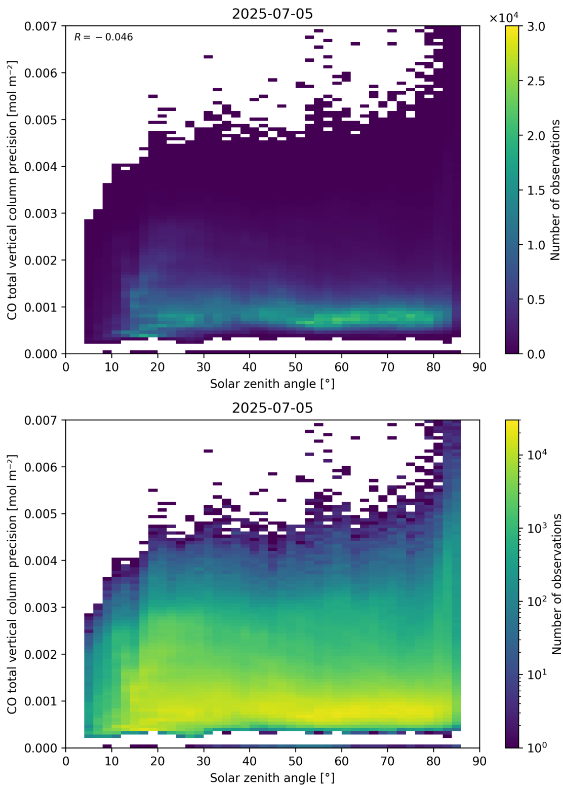
Figure 63: Scatter density plot of “Solar zenith angle” against “CO total vertical column precision” for 2025-07-04 to 2025-07-06.
