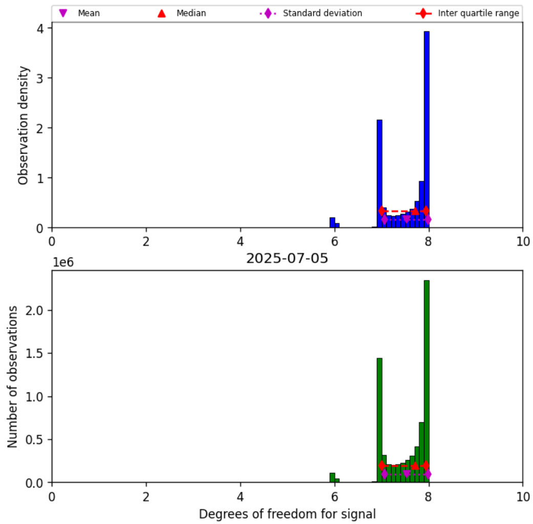
Figure 23: Histogram of “Degrees of freedom for signal” for 2025-07-04 to 2025-07-06
