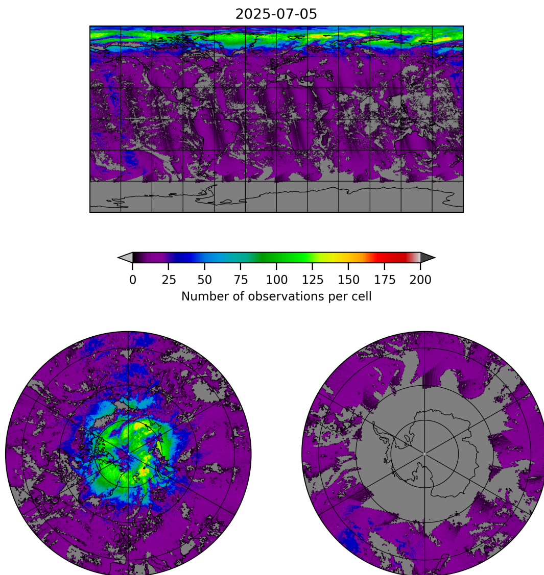
Figure 8: Map of the number of observations for 2025-07-04 to 2025-07-06
