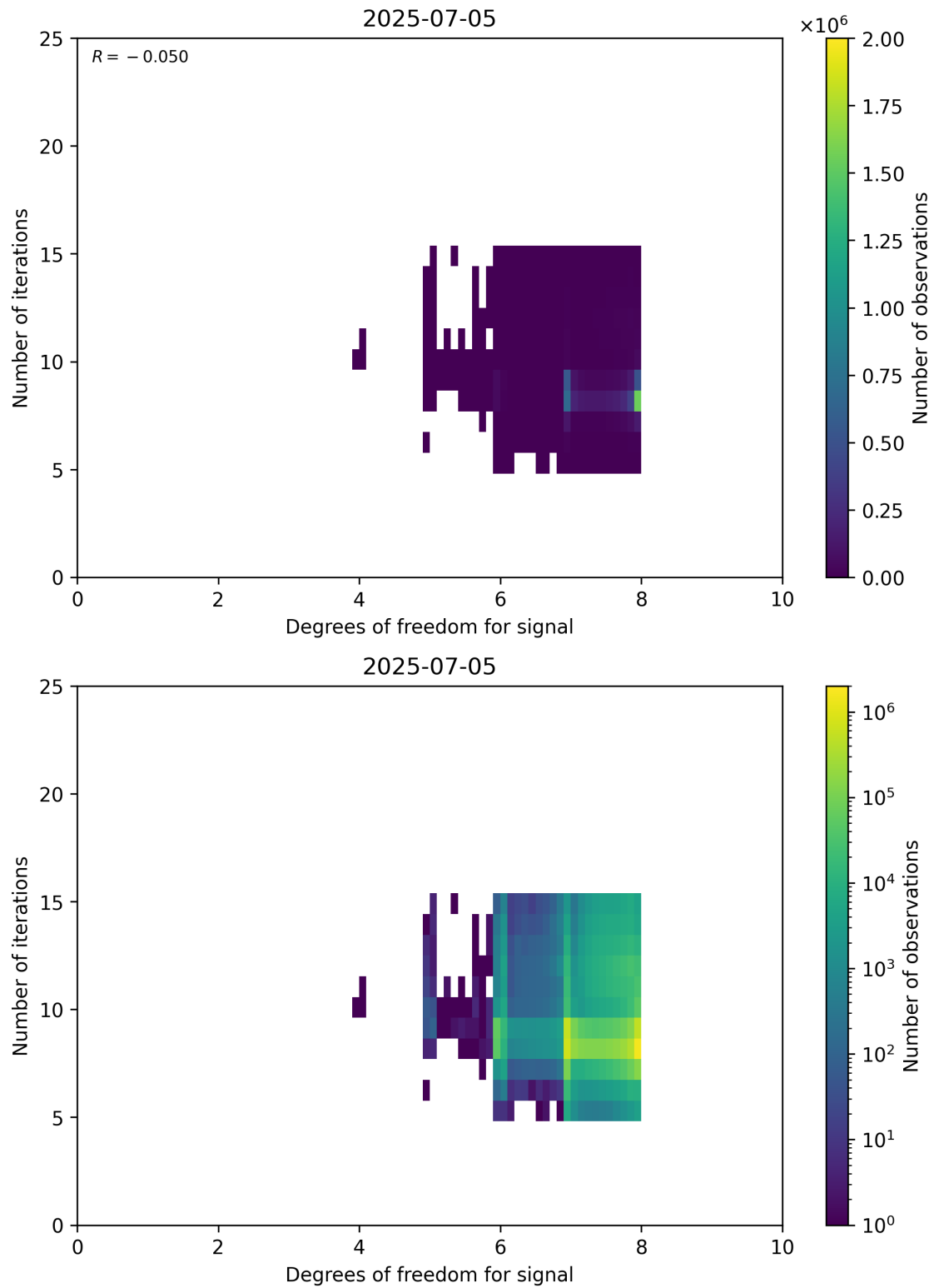
Figure 50: Scatter density plot of “Degrees of freedom for signal” against “Number of iterations” for 2025-07-04 to 2025-07-06.
