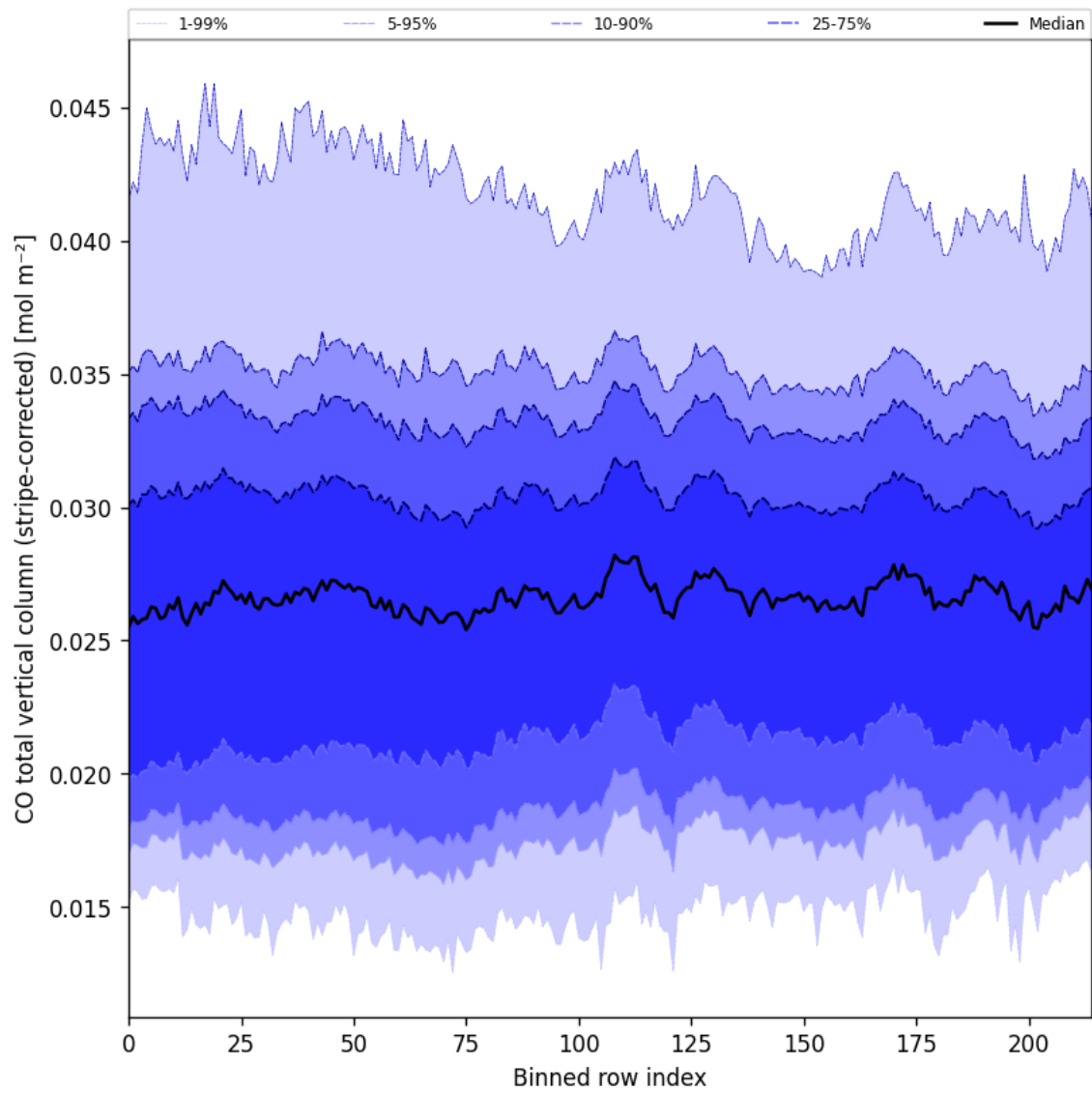
Figure 27: Along track statistics of “CO total vertical column (stripe-corrected)” for 2025-07-04 to 2025-07-06
