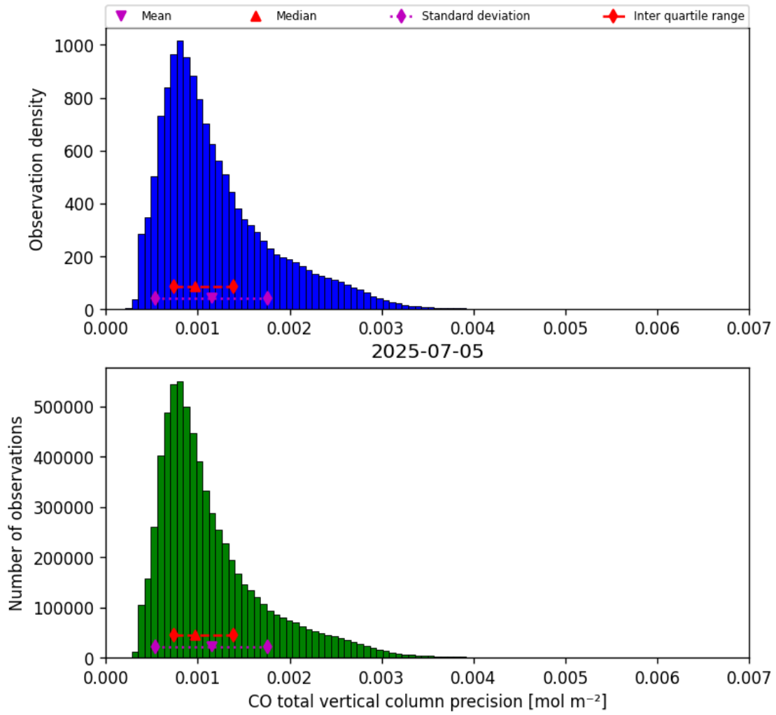
Figure 20: Histogram of “CO total vertical column precision” for 2025-07-04 to 2025-07-06
