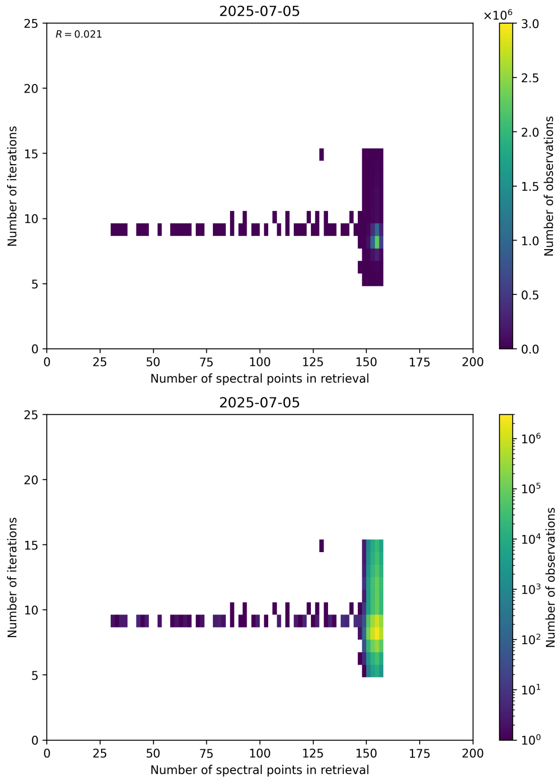
Figure 60: Scatter density plot of “Number of spectral points in retrieval” against “Number of iterations” for 2025-07-04 to 2025-07-06.
