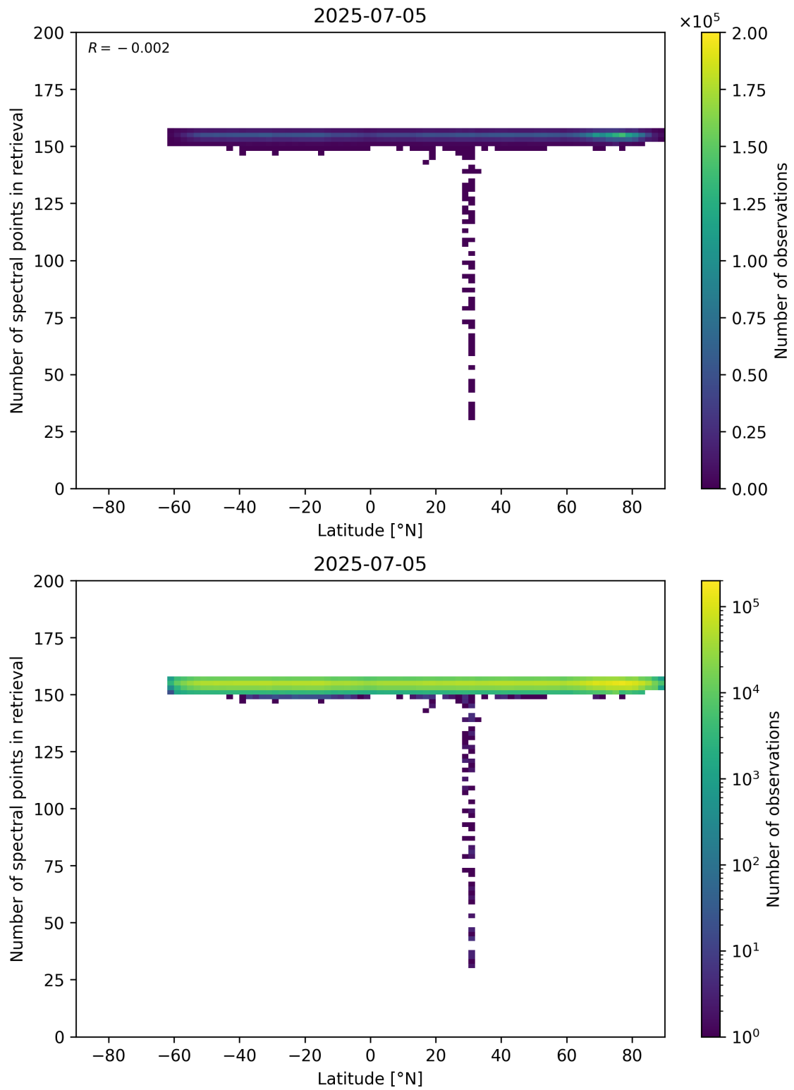
Figure 57: Scatter density plot of “Latitude” against “Number of spectral points in retrieval” for 2025-07-04 to 2025-07-06.
