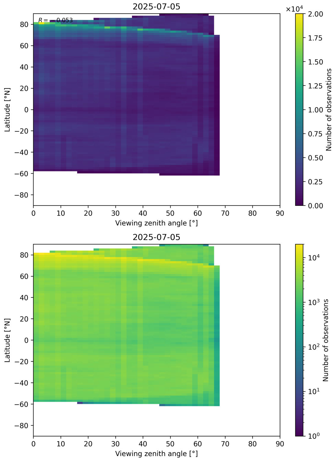
Figure 74: Scatter density plot of “Viewing zenith angle” against “Latitude” for 2025-07-04 to 2025-07-06.
