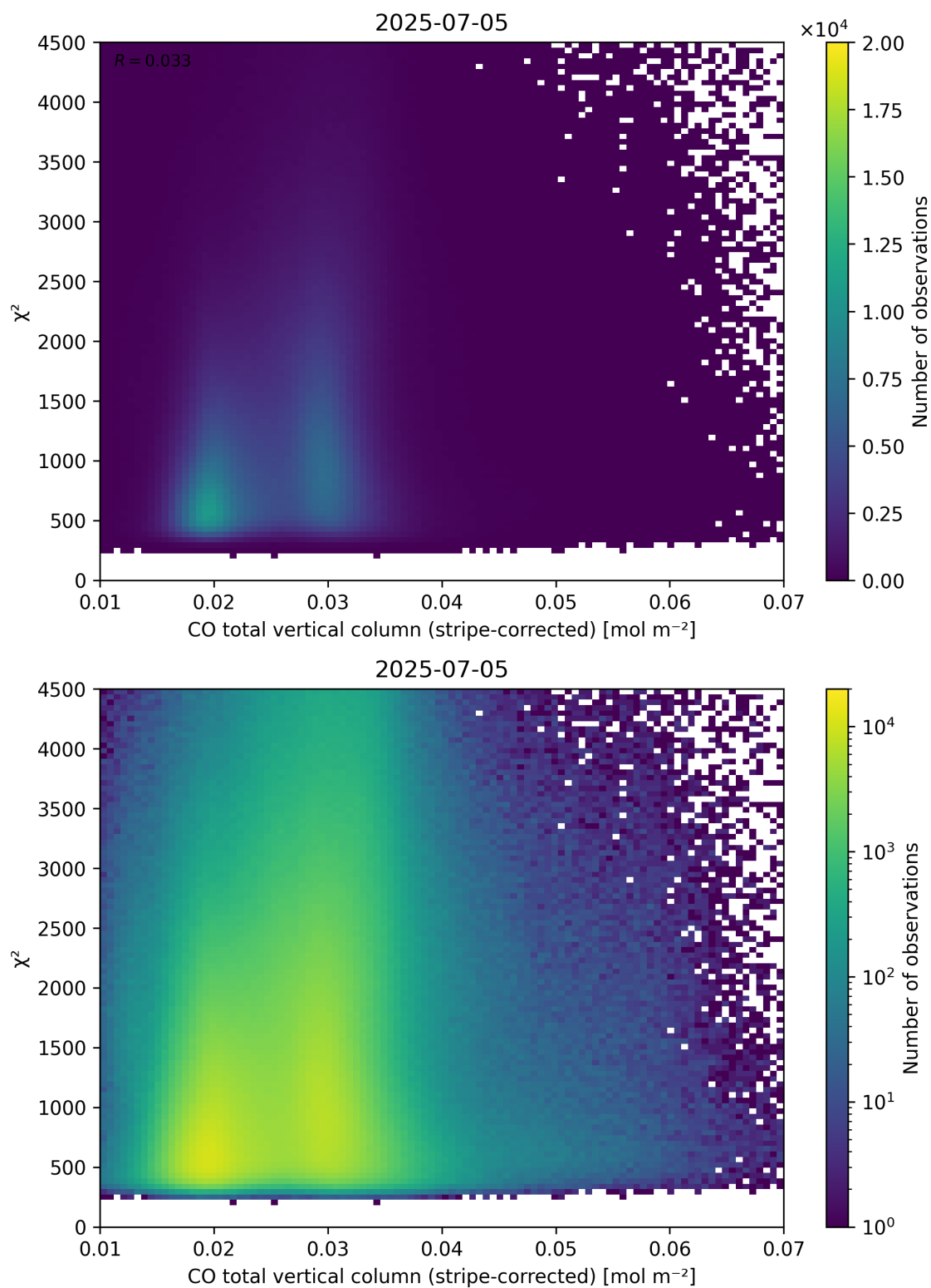
Figure 37: Scatter density plot of “CO total vertical column (stripe-corrected)” against “ \chi^2 ” for 2025-07-04 to 2025-07-06.
