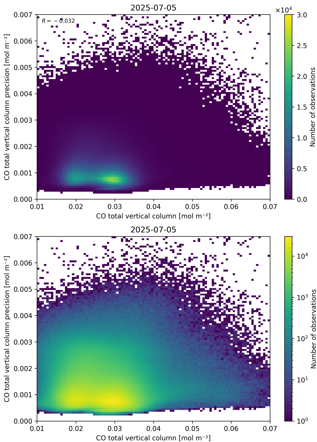
Figure 34: Scatter density plot of “CO total vertical column” against “CO total vertical column precision” for 2025-07-04 to 2025-07-06.
