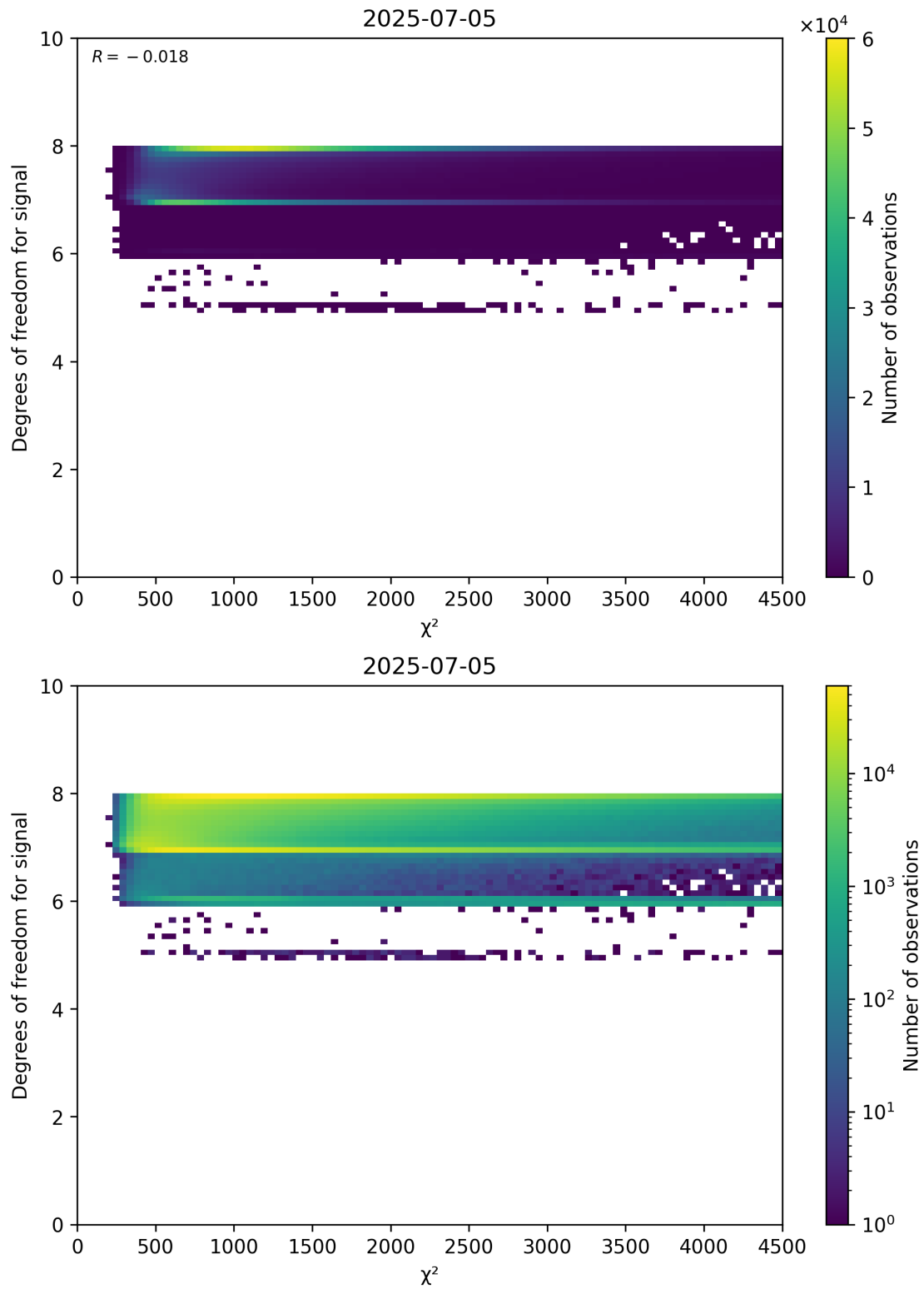
Figure 48: Scatter density plot of “ \chi^2 ” against “Degrees of freedom for signal” for 2025-07-04 to 2025-07-06.
