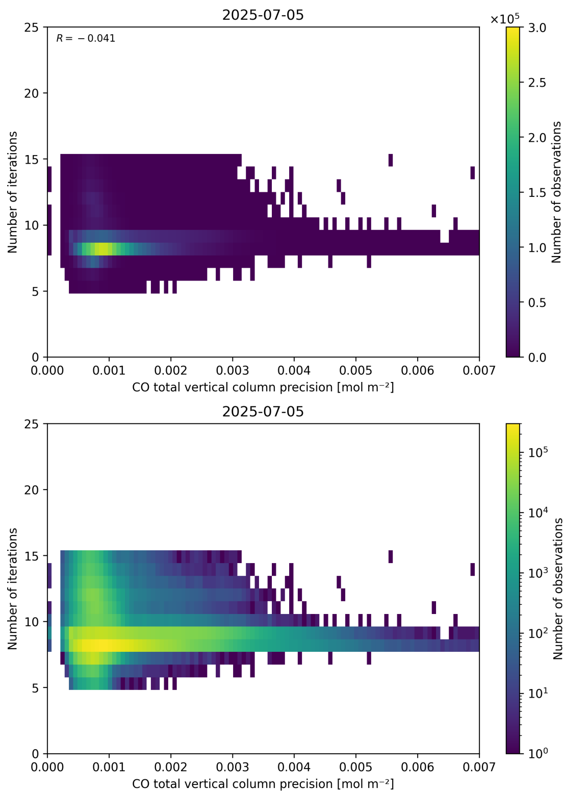
Figure 46: Scatter density plot of “CO total vertical column precision” against “Number of iterations” for 2025-07-04 to 2025-07-06.
