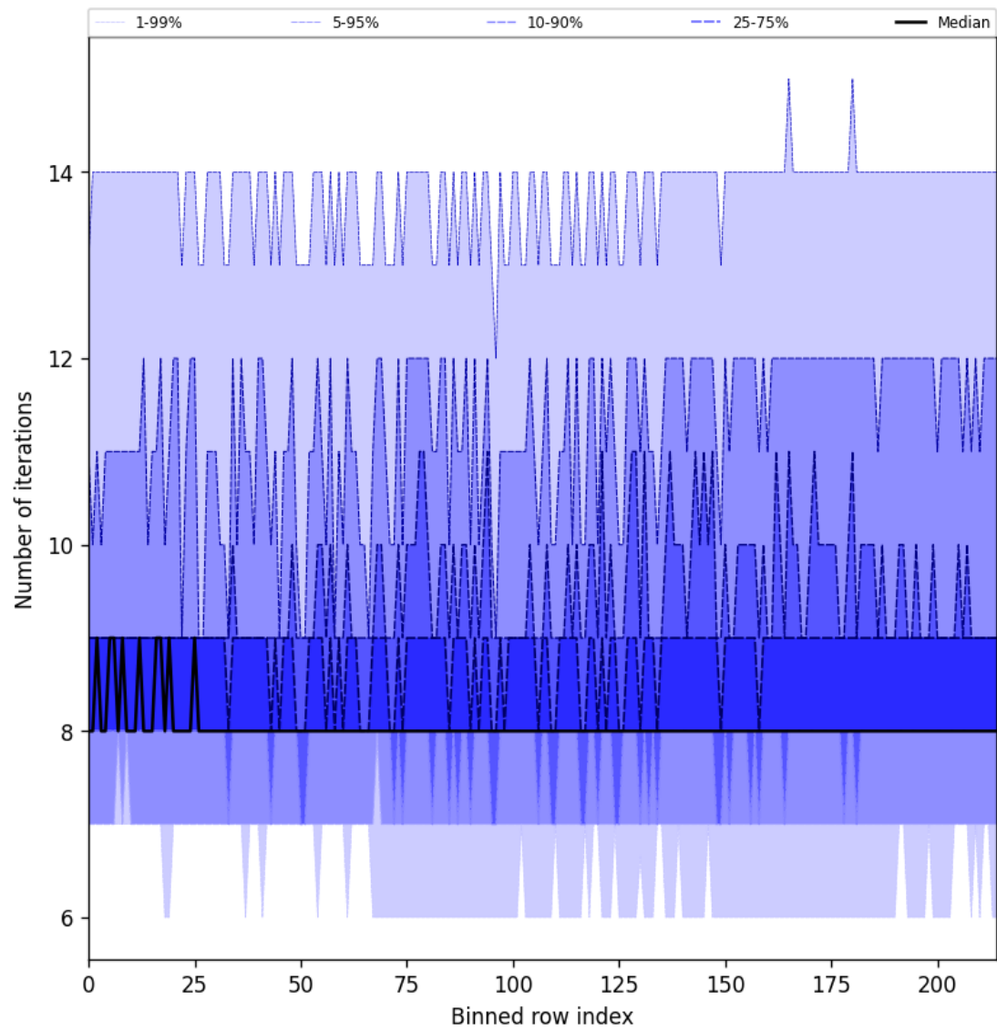
Figure 32: Along track statistics of “Number of iterations” for 2025-07-04 to 2025-07-06
