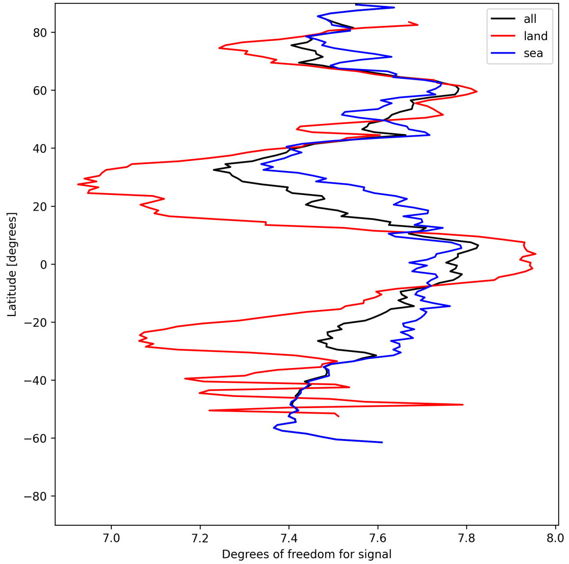
Figure 15: Zonal average of “Degrees of freedom for signal” for 2025-07-04 to 2025-07-06.
