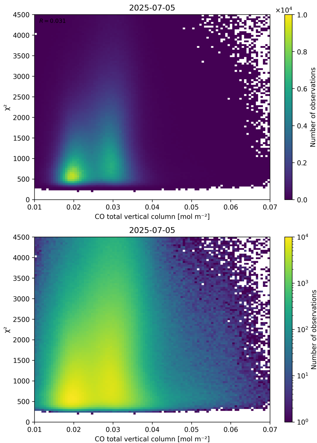
Figure 35: Scatter density plot of “CO total vertical column” against “ \chi^2 ” for 2025-07-04 to 2025-07-06.
