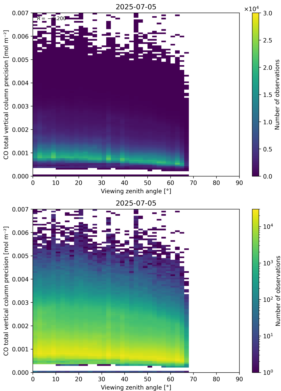
Figure 71: Scatter density plot of “Viewing zenith angle” against “CO total vertical column precision” for 2025-07-04 to 2025-07-06.
