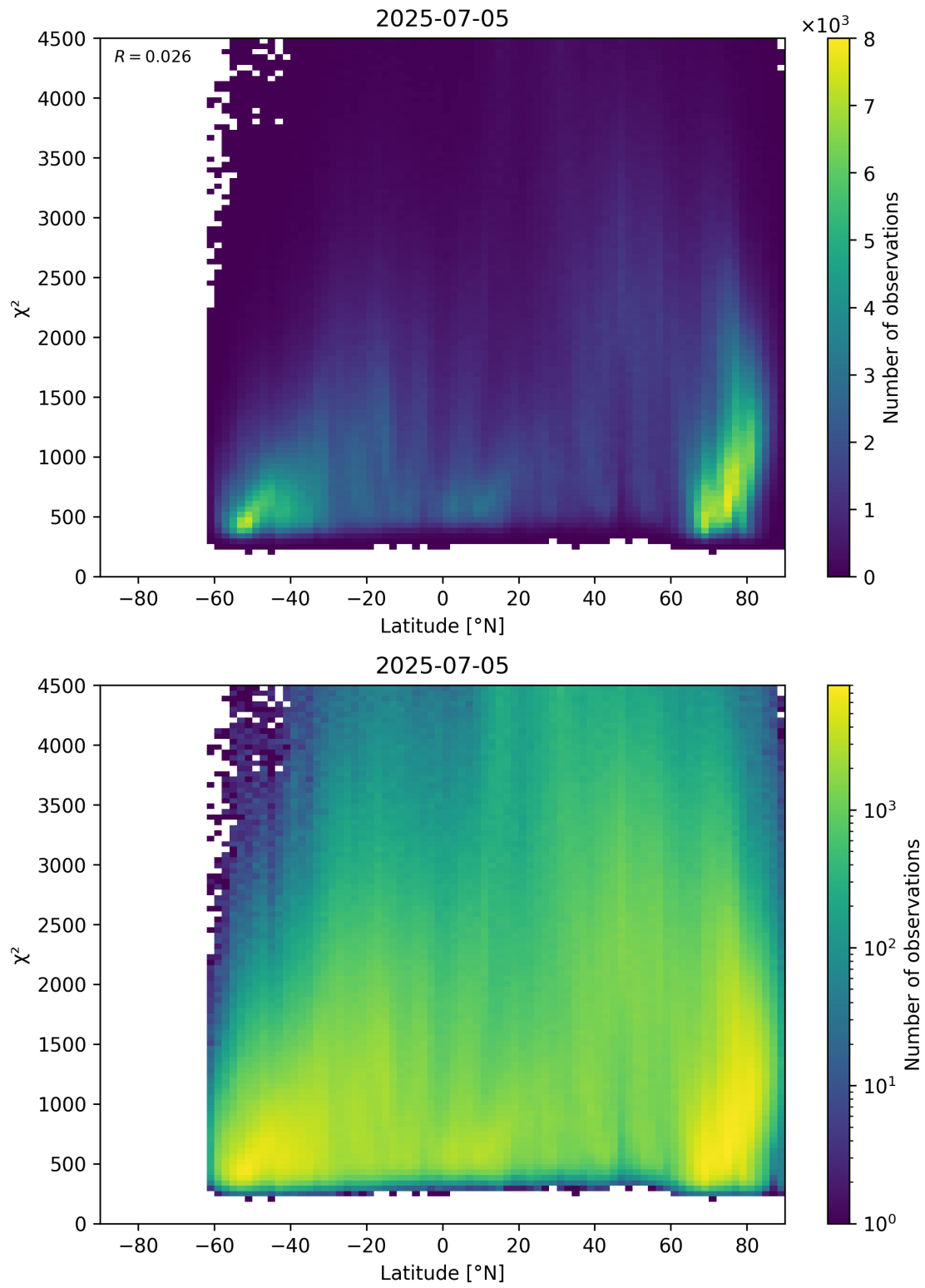
Figure 54: Scatter density plot of “Latitude” against “ \chi^2 ” for 2025-07-04 to 2025-07-06.
