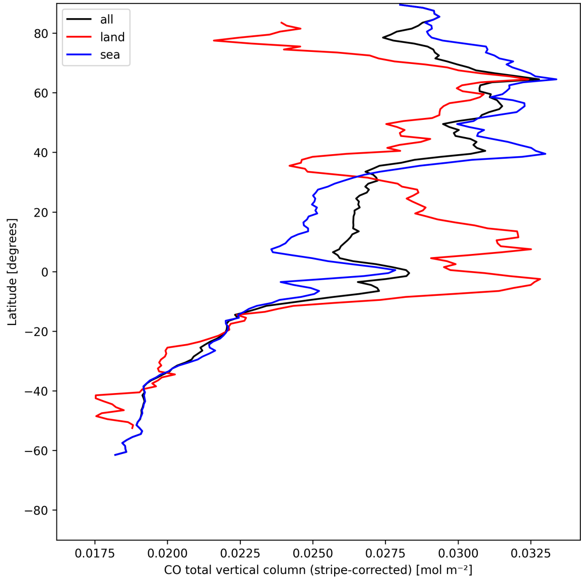
Figure 11: Zonal average of “CO total vertical column (stripe-corrected)” for 2025-07-04 to 2025-07-06.
