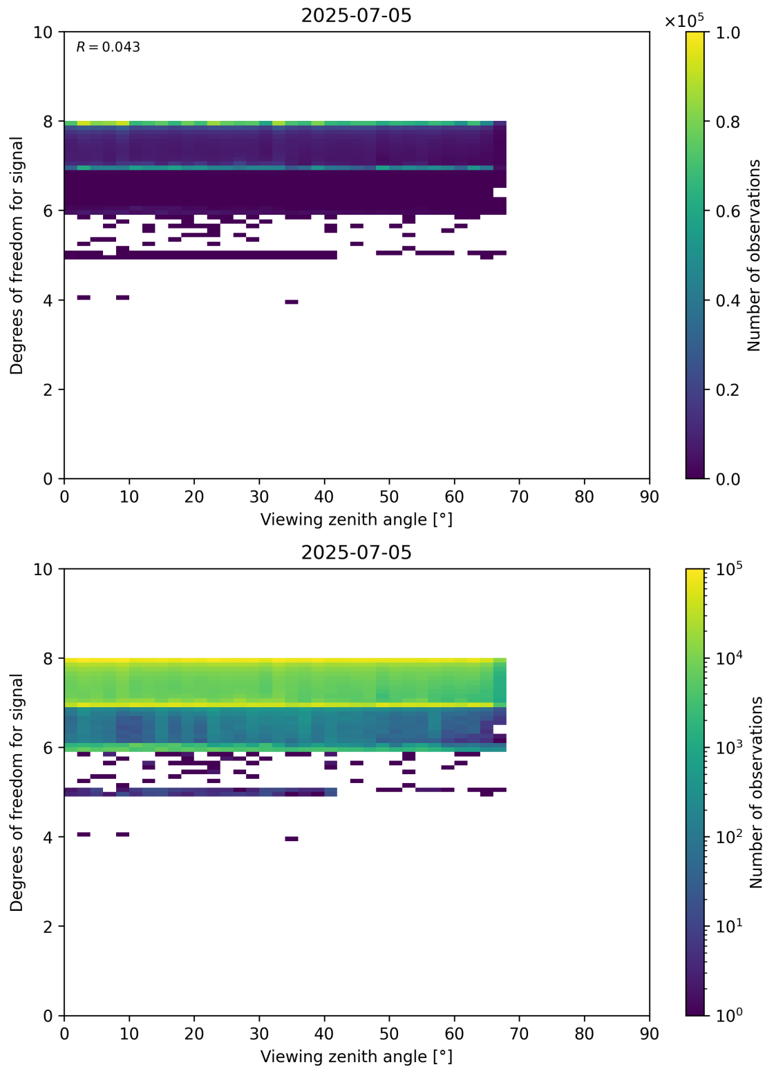
Figure 73: Scatter density plot of “Viewing zenith angle” against “Degrees of freedom for signal” for 2025-07-04 to 2025-07-06.
