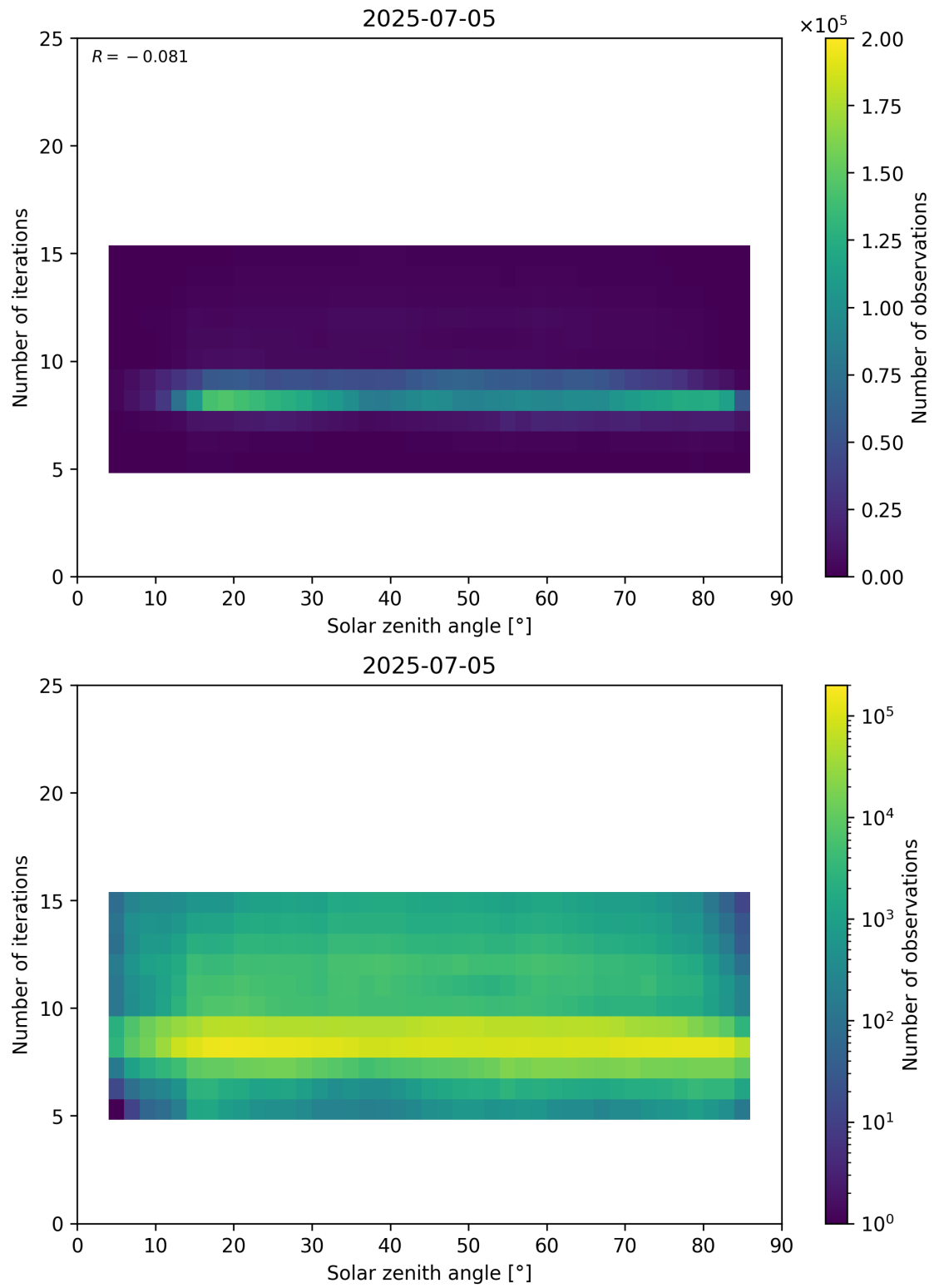
Figure 67: Scatter density plot of “Solar zenith angle” against “Number of iterations” for 2025-07-04 to 2025-07-06.
