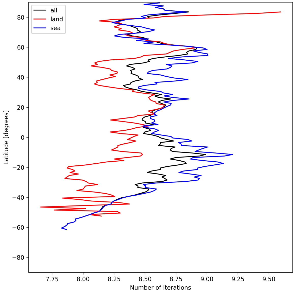
Figure 16: Zonal average of “Number of iterations” for 2025-07-04 to 2025-07-06.
