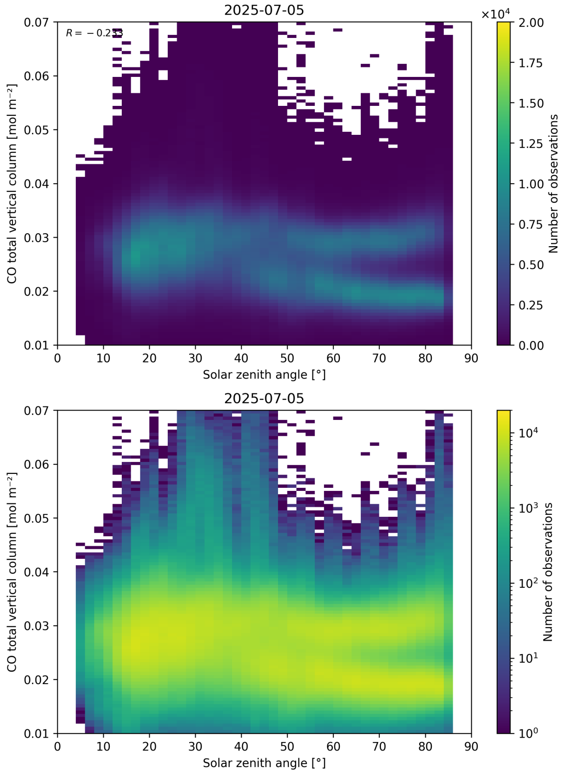
Figure 61: Scatter density plot of “Solar zenith angle” against “CO total vertical column” for 2025-07-04 to 2025-07-06.
