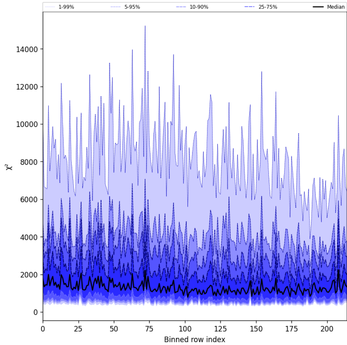
Figure 30: Along track statistics of “ \chi^2 ” for 2025-07-04 to 2025-07-06
