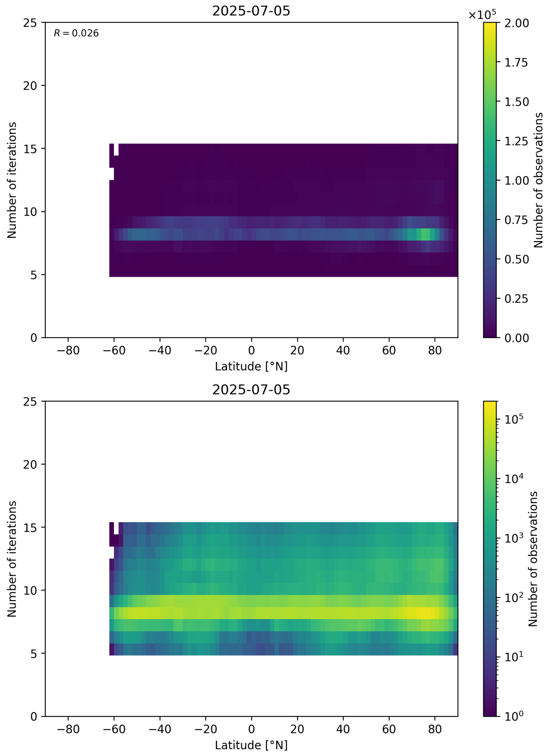
Figure 56: Scatter density plot of “Latitude” against “Number of iterations” for 2025-07-04 to 2025-07-06.
