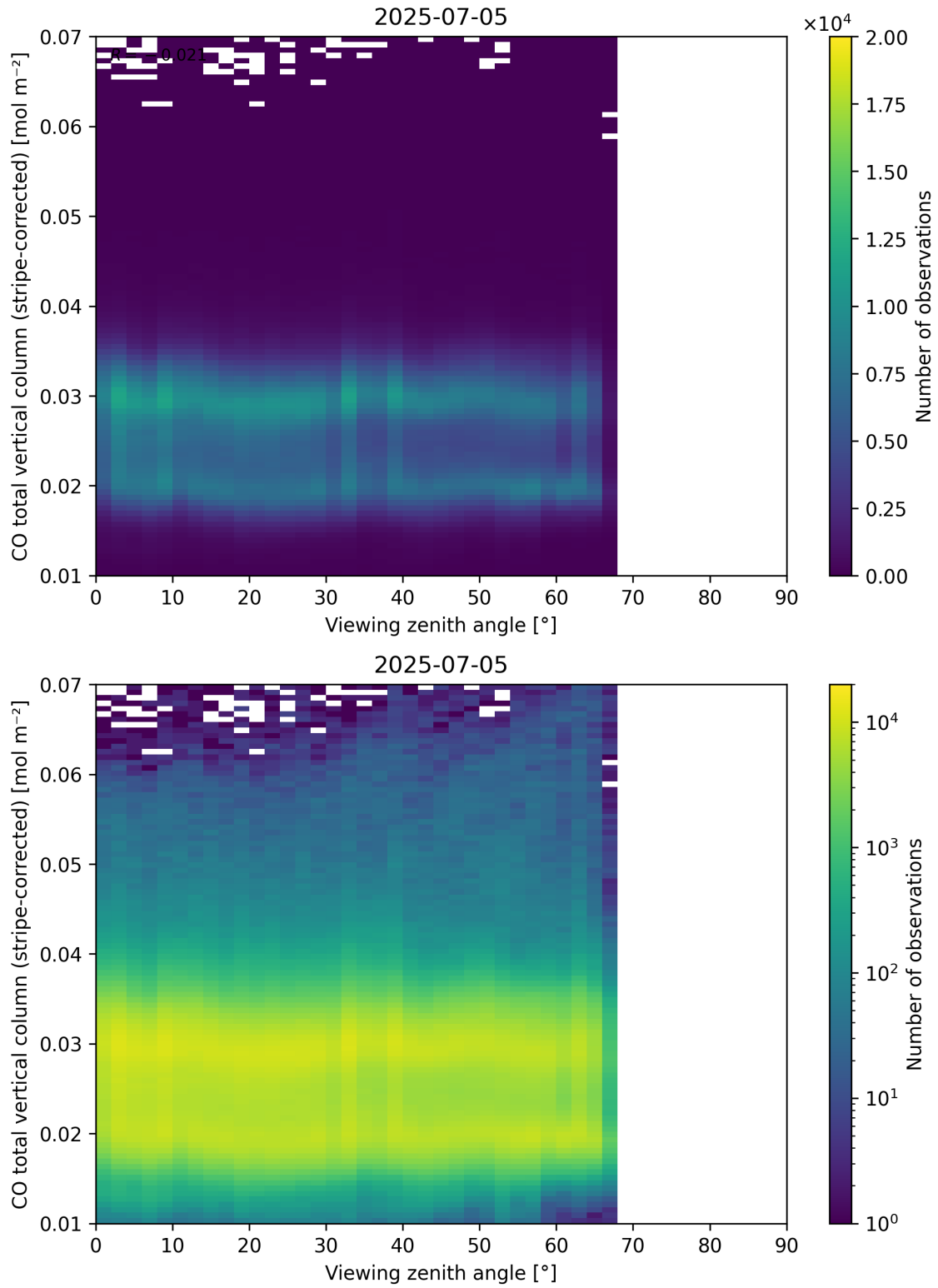
Figure 70: Scatter density plot of “Viewing zenith angle” against “CO total vertical column (stripe-corrected)” for 2025-07-04 to 2025-07-06.
