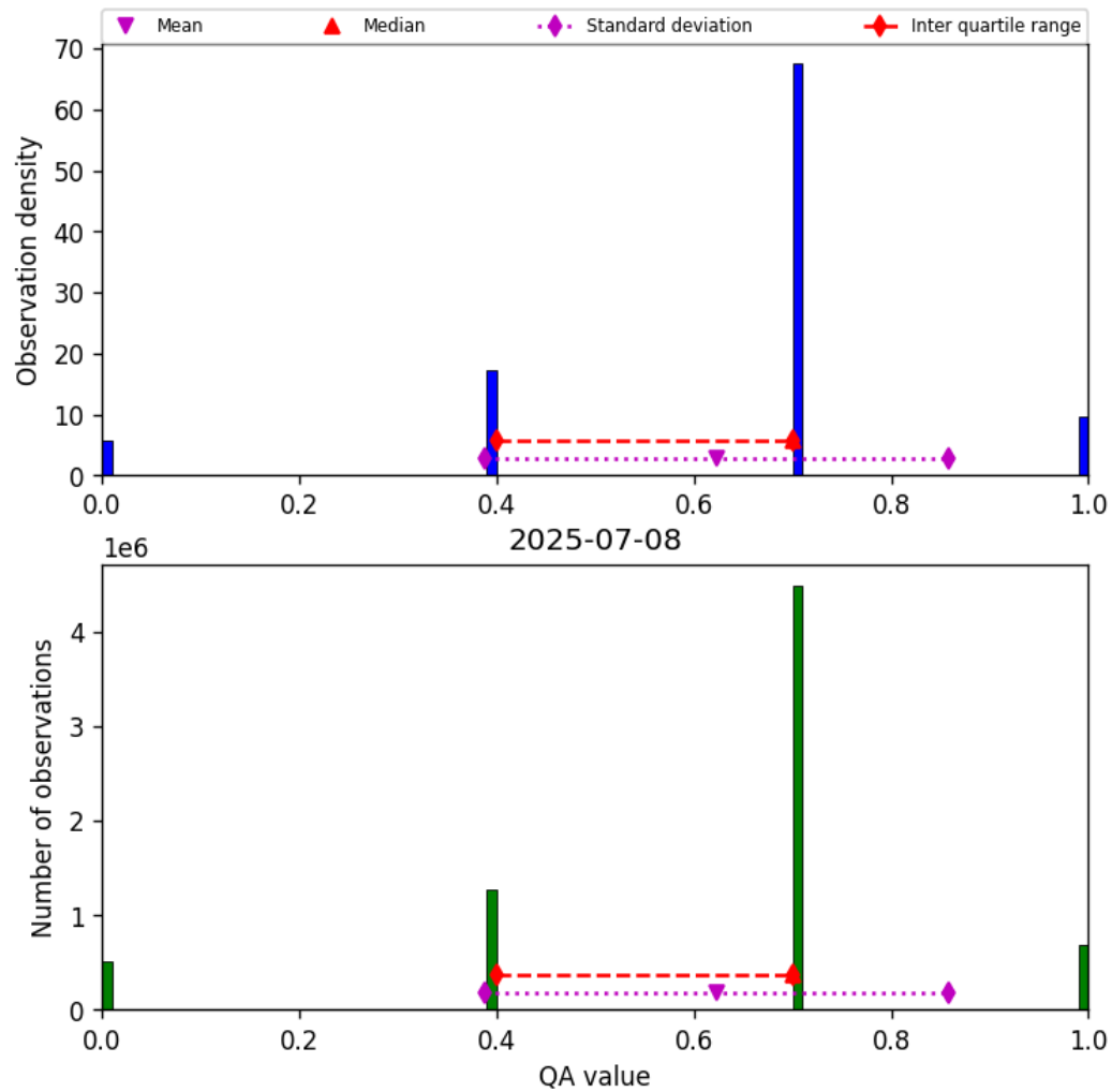
Figure 17: Histogram of “QA value” for 2025-07-08 to 2025-07-09
