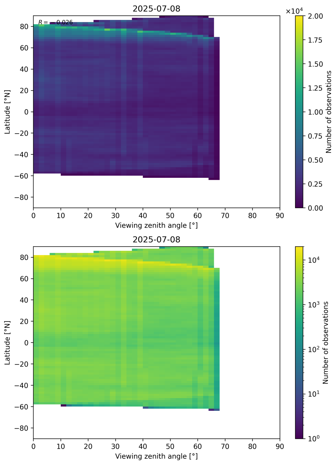
Figure 74: Scatter density plot of “Viewing zenith angle” against “Latitude” for 2025-07-08 to 2025-07-09.
