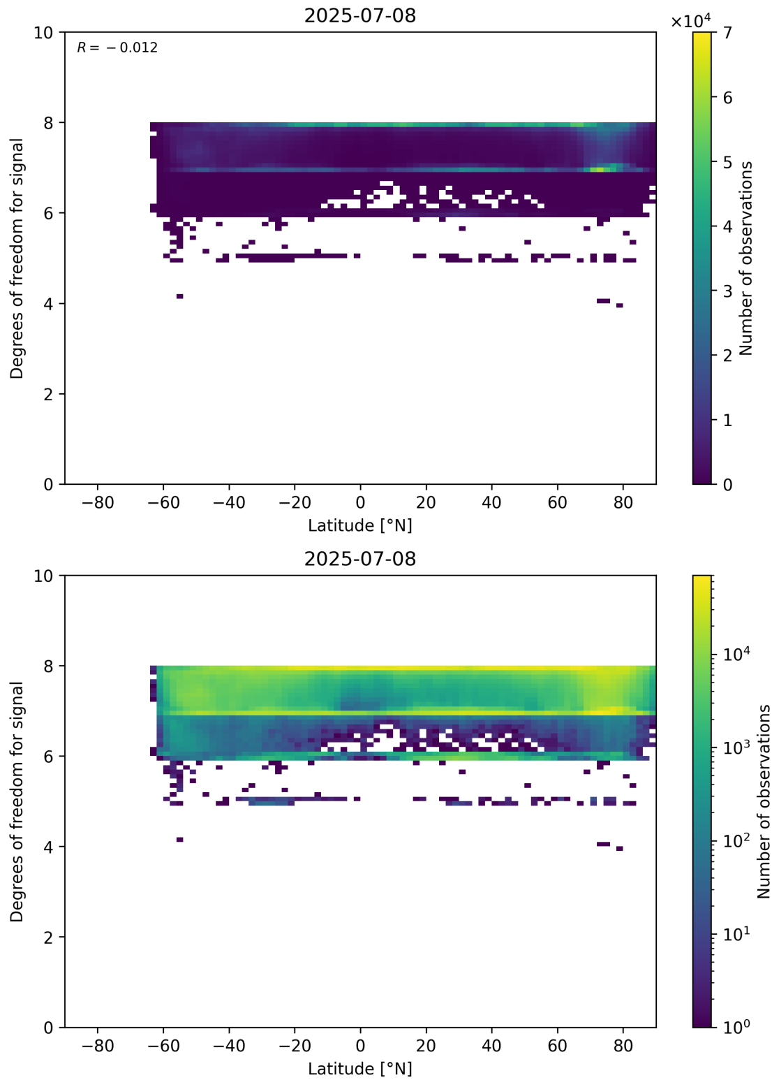
Figure 55: Scatter density plot of “Latitude” against “Degrees of freedom for signal” for 2025-07-08 to 2025-07-09.
