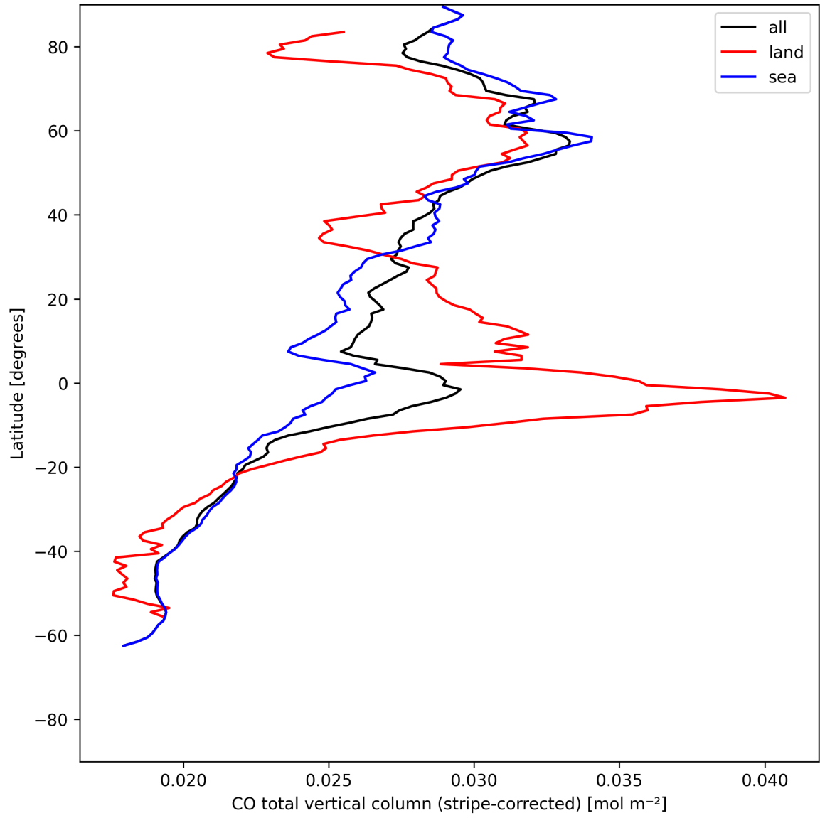
Figure 11: Zonal average of “CO total vertical column (stripe-corrected)” for 2025-07-08 to 2025-07-09.
