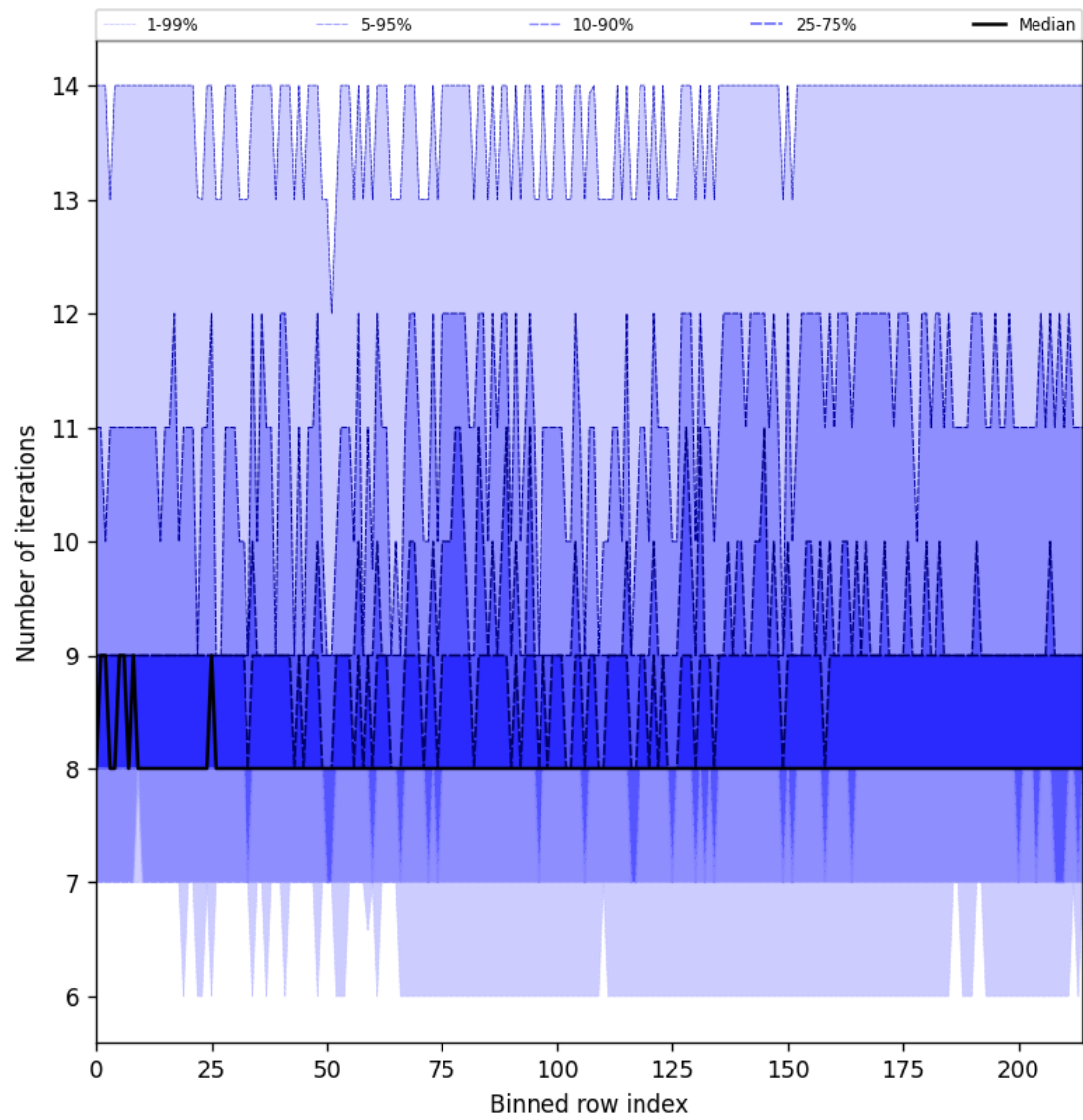
Figure 32: Along track statistics of “Number of iterations” for 2025-07-08 to 2025-07-09
