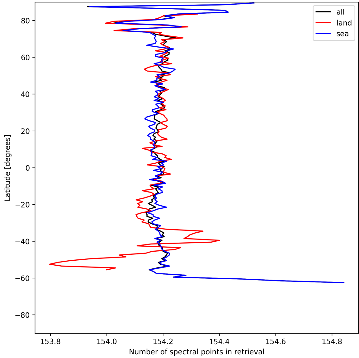
Figure 13: Zonal average of “Number of spectral points in retrieval” for 2025-07-08 to 2025-07-09.
