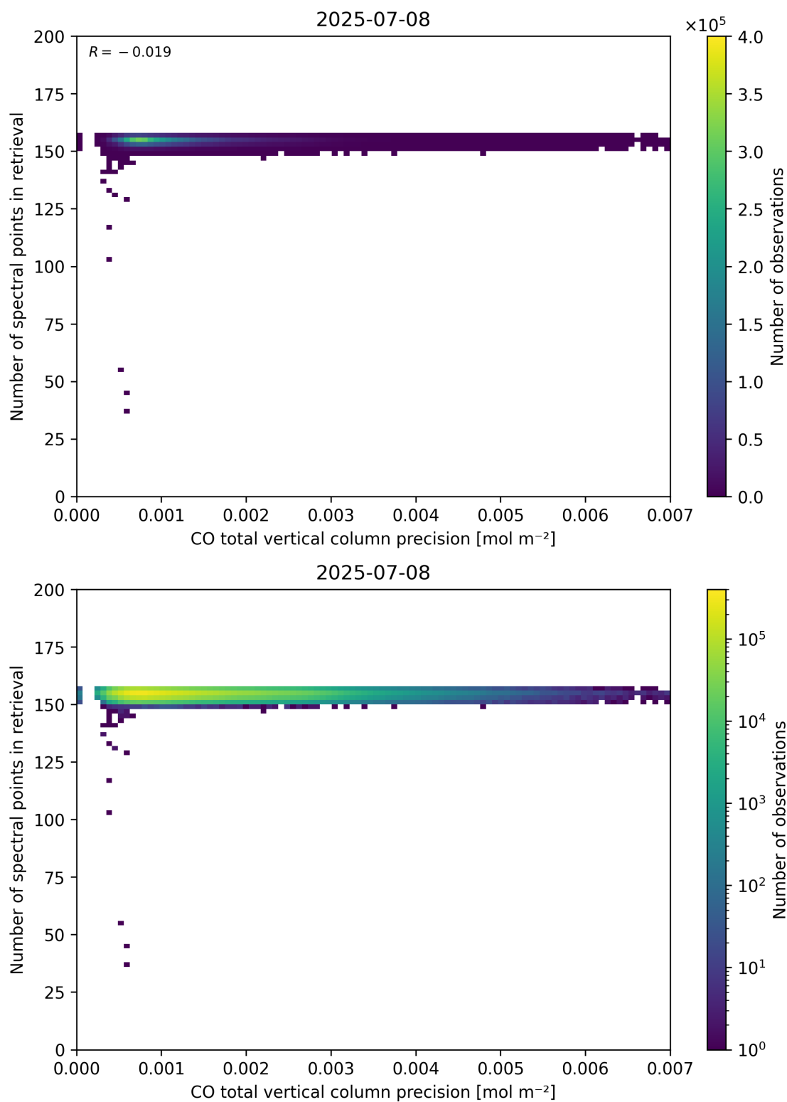
Figure 47: Scatter density plot of “CO total vertical column precision” against “Number of spectral points in retrieval” for 2025-07-08 to 2025-07-09.
