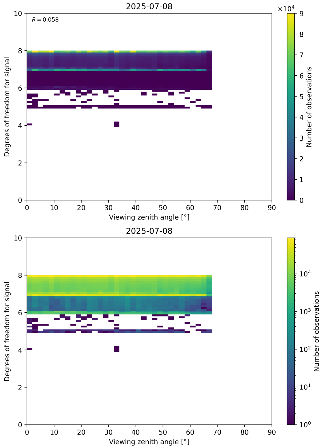
Figure 73: Scatter density plot of “Viewing zenith angle” against “Degrees of freedom for signal” for 2025-07-08 to 2025-07-09.
