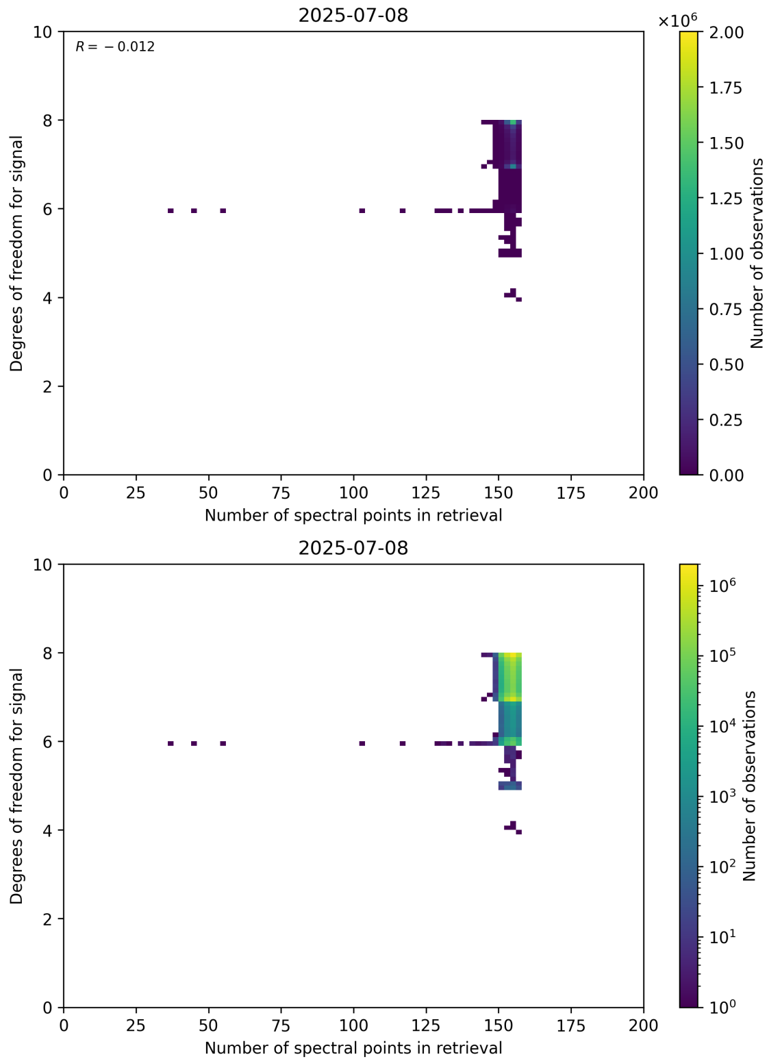
Figure 59: Scatter density plot of “Number of spectral points in retrieval” against “Degrees of freedom for signal” for 2025-07-08 to 2025-07-09.
