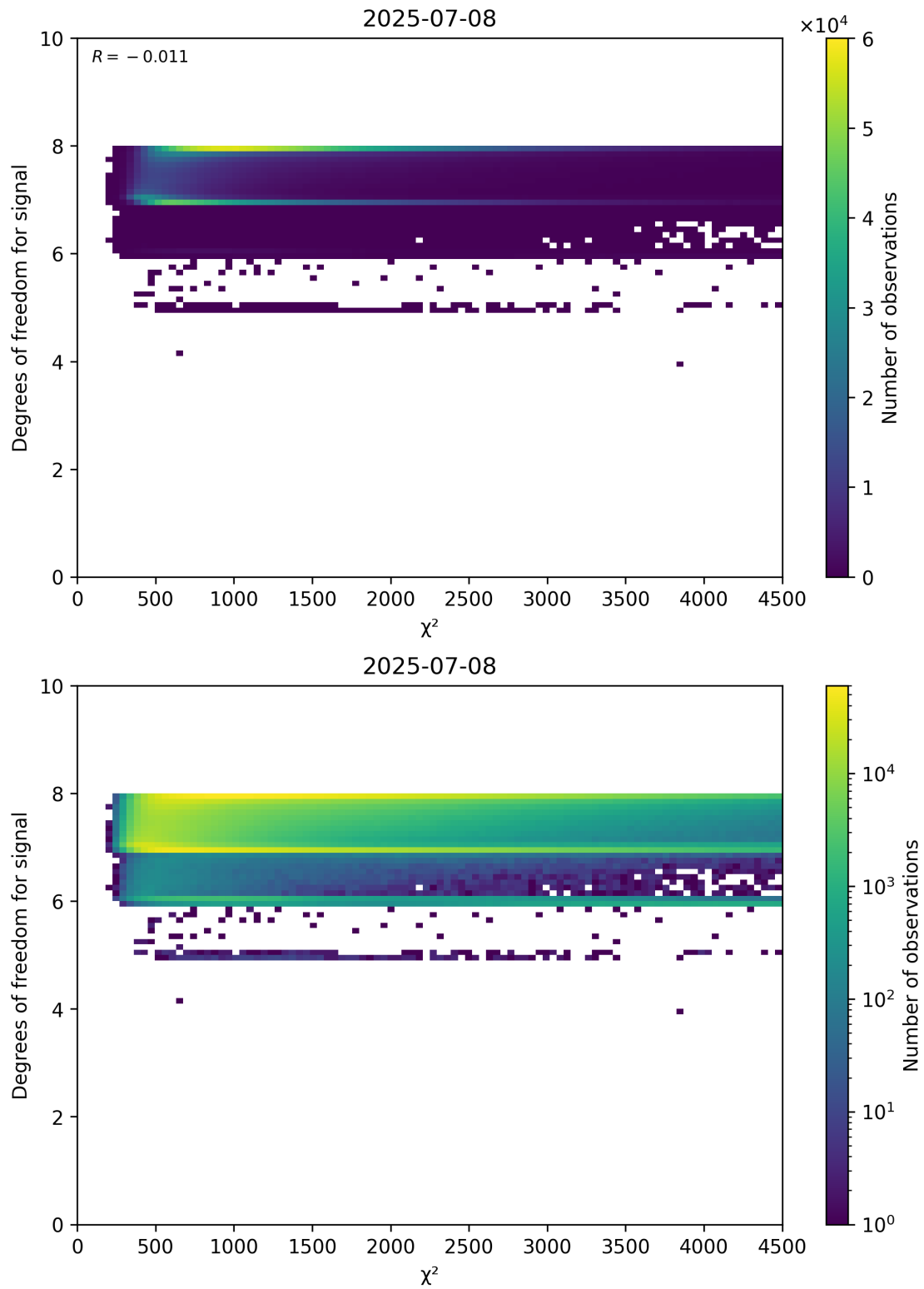
Figure 48: Scatter density plot of “ \chi^2 ” against “Degrees of freedom for signal” for 2025-07-08 to 2025-07-09.
