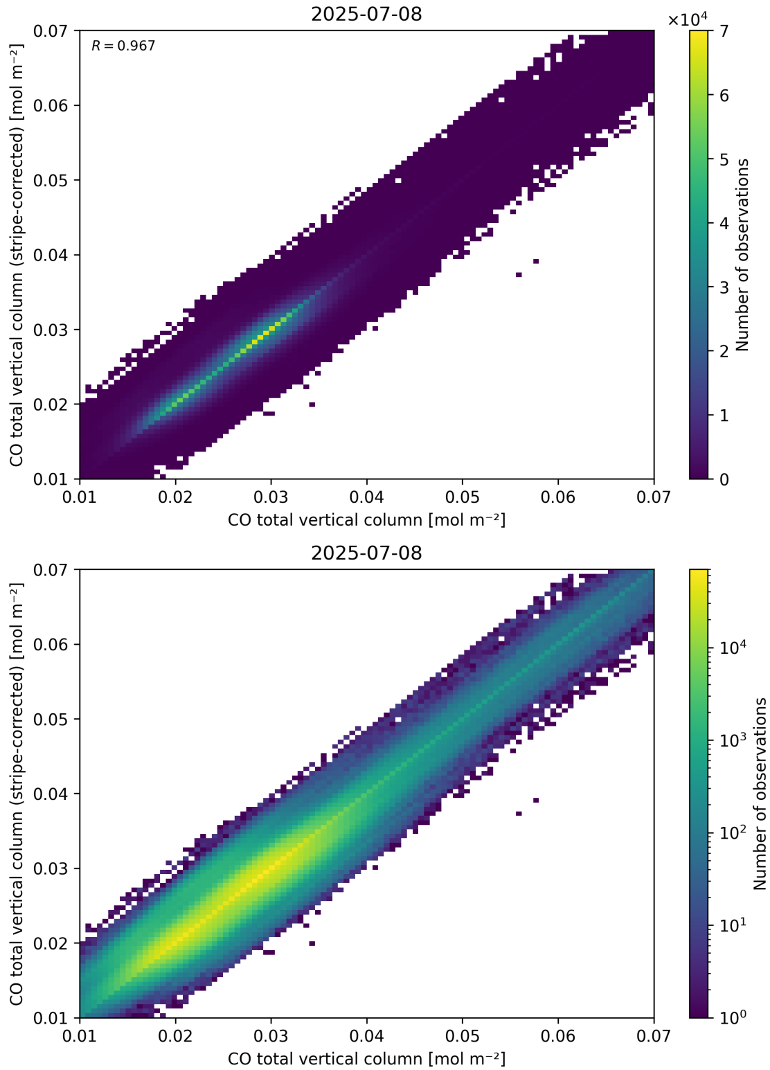
Figure 33: Scatter density plot of “CO total vertical column” against “CO total vertical column (stripe-corrected)” for 2025-07-08 to 2025-07-09.
