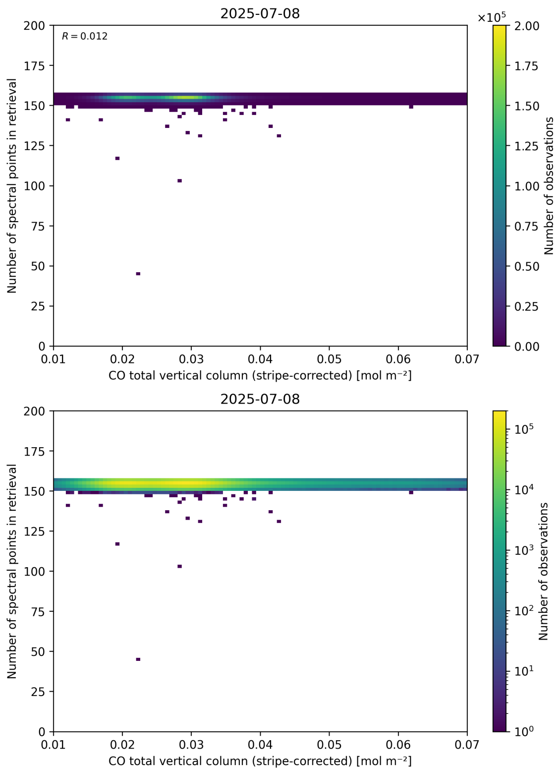
Figure 40: Scatter density plot of “CO total vertical column (stripe-corrected)” against “Number of spectral points in retrieval” for 2025-07-08 to 2025-07-09.
