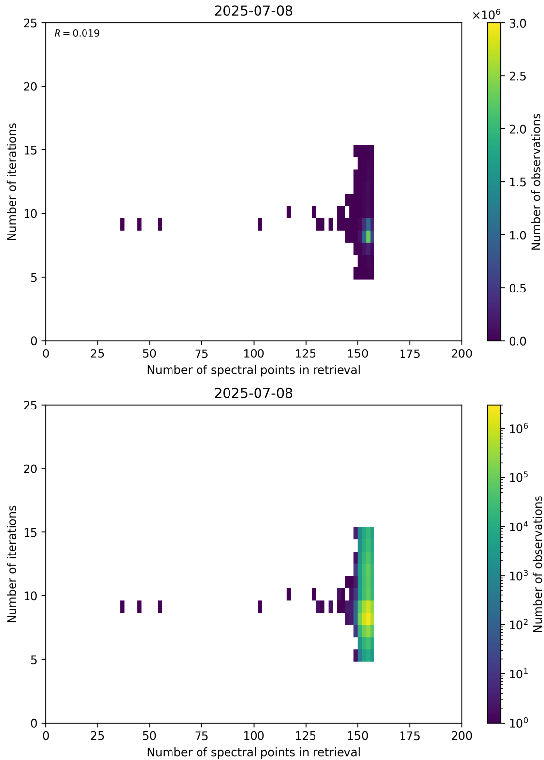
Figure 60: Scatter density plot of “Number of spectral points in retrieval” against “Number of iterations” for 2025-07-08 to 2025-07-09.
