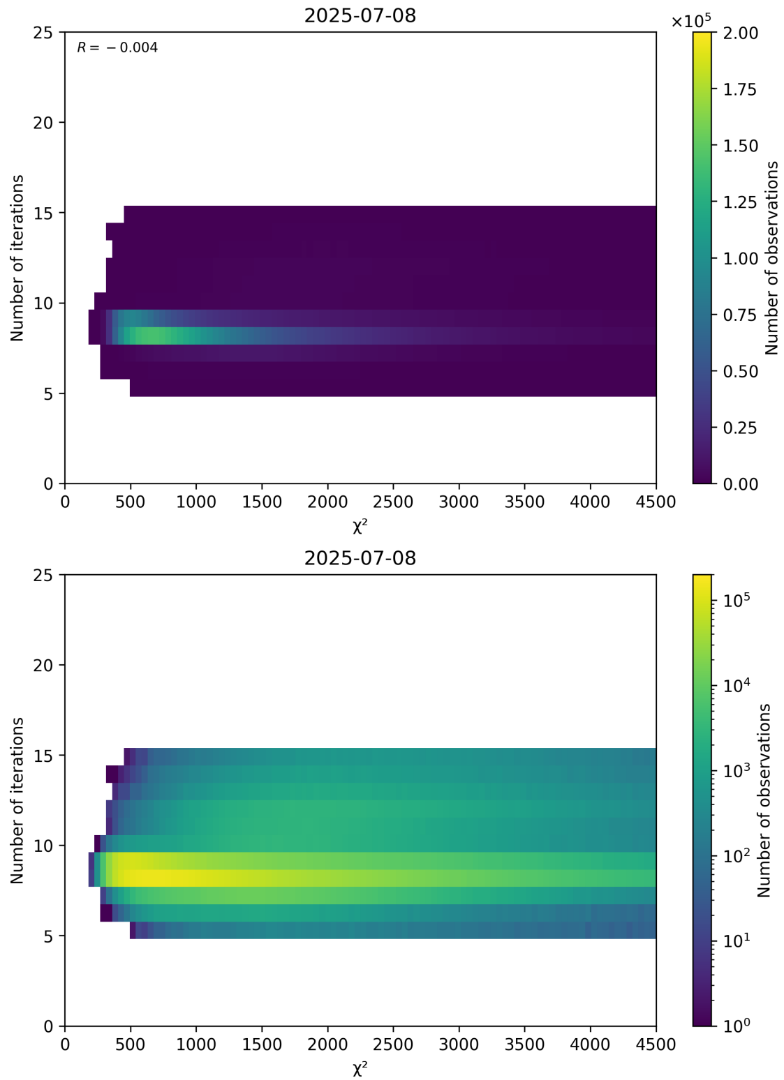
Figure 49: Scatter density plot of “ \chi^2 ” against “Number of iterations” for 2025-07-08 to 2025-07-09.
