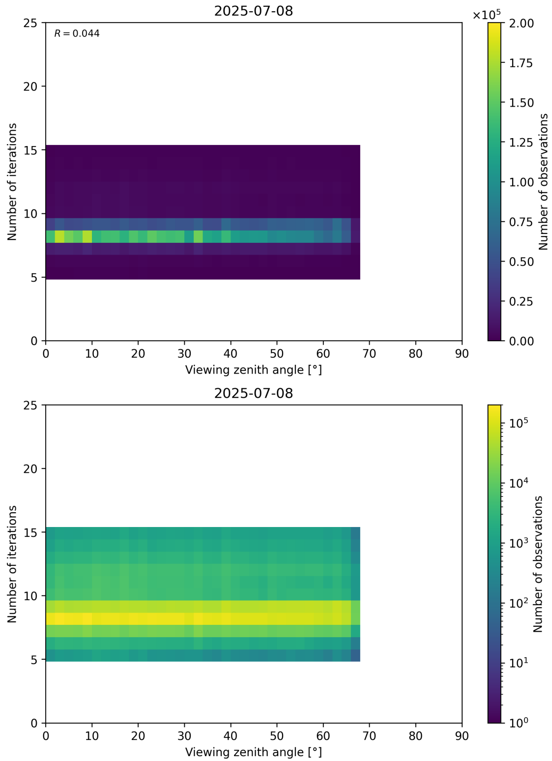
Figure 75: Scatter density plot of “Viewing zenith angle” against “Number of iterations” for 2025-07-08 to 2025-07-09.
