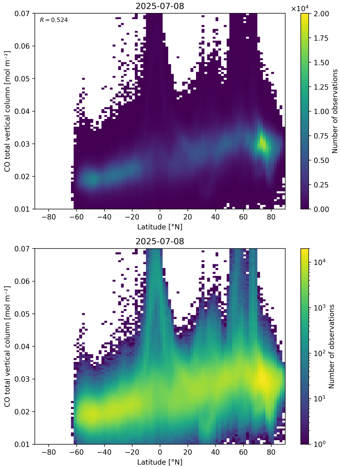
Figure 51: Scatter density plot of “Latitude” against “CO total vertical column” for 2025-07-08 to 2025-07-09.
