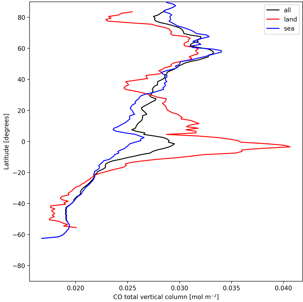
Figure 10: Zonal average of “CO total vertical column” for 2025-07-08 to 2025-07-09.
