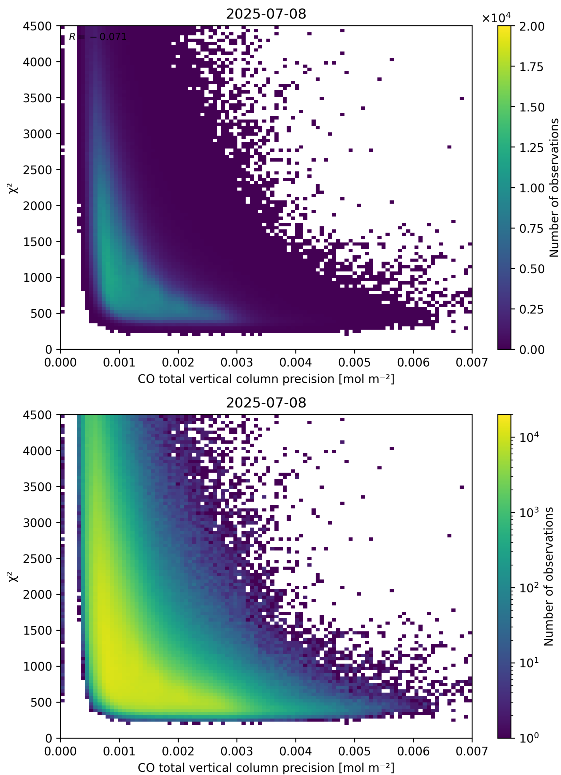
Figure 44: Scatter density plot of “CO total vertical column precision” against “ \chi^2 ” for 2025-07-08 to 2025-07-09.
