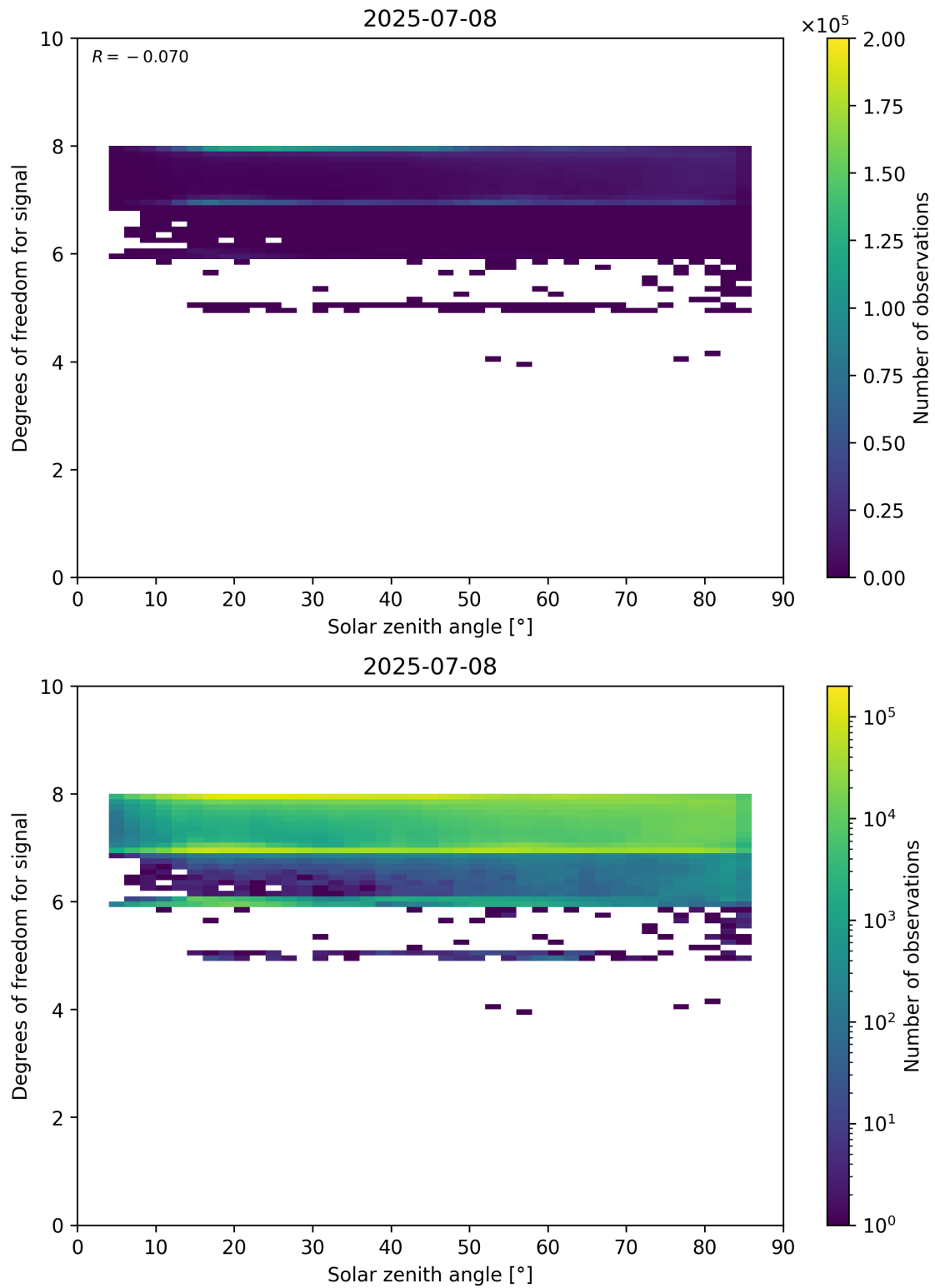
Figure 65: Scatter density plot of “Solar zenith angle” against “Degrees of freedom for signal” for 2025-07-08 to 2025-07-09.
