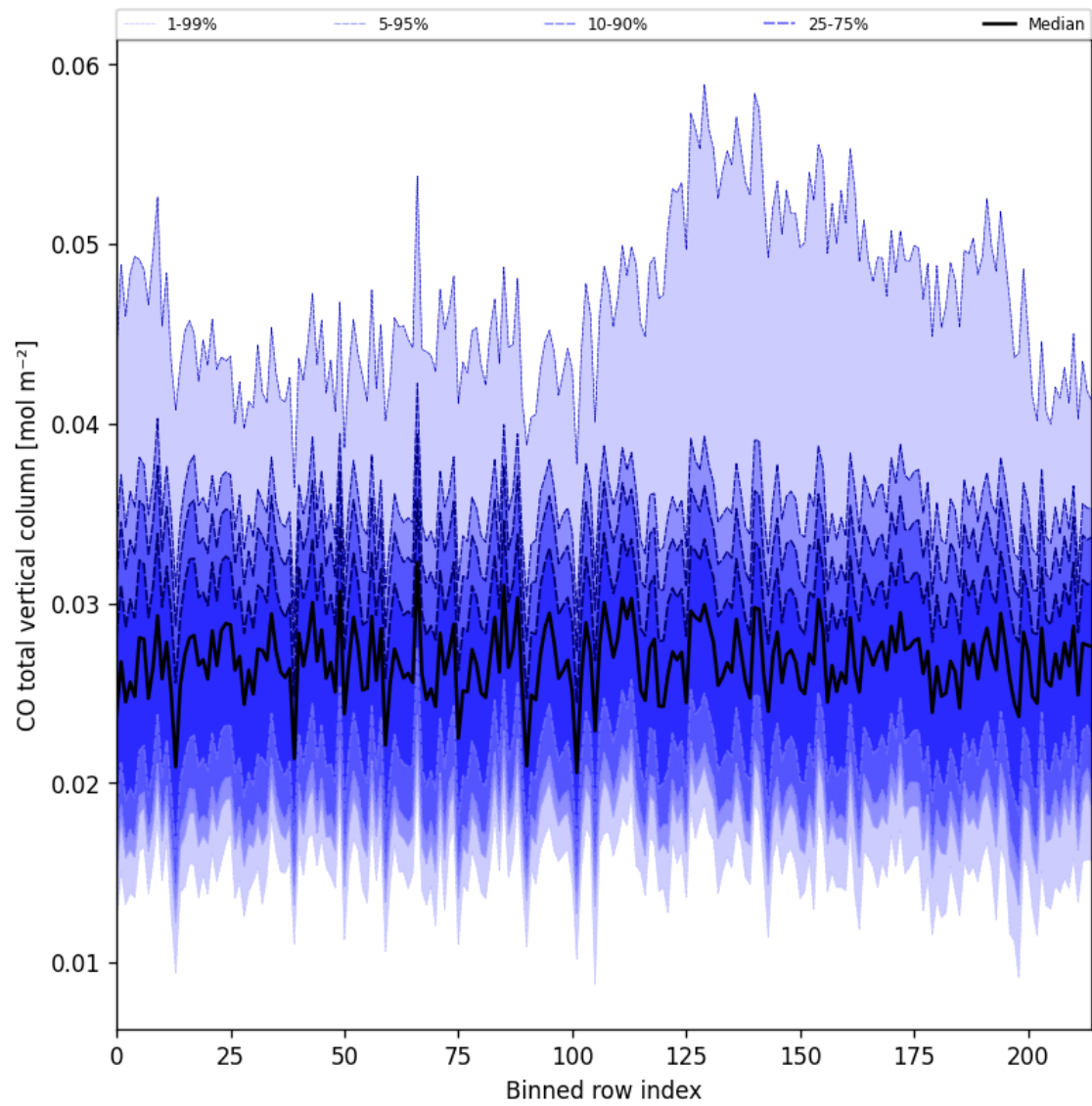
Figure 26: Along track statistics of “CO total vertical column” for 2025-07-08 to 2025-07-09
