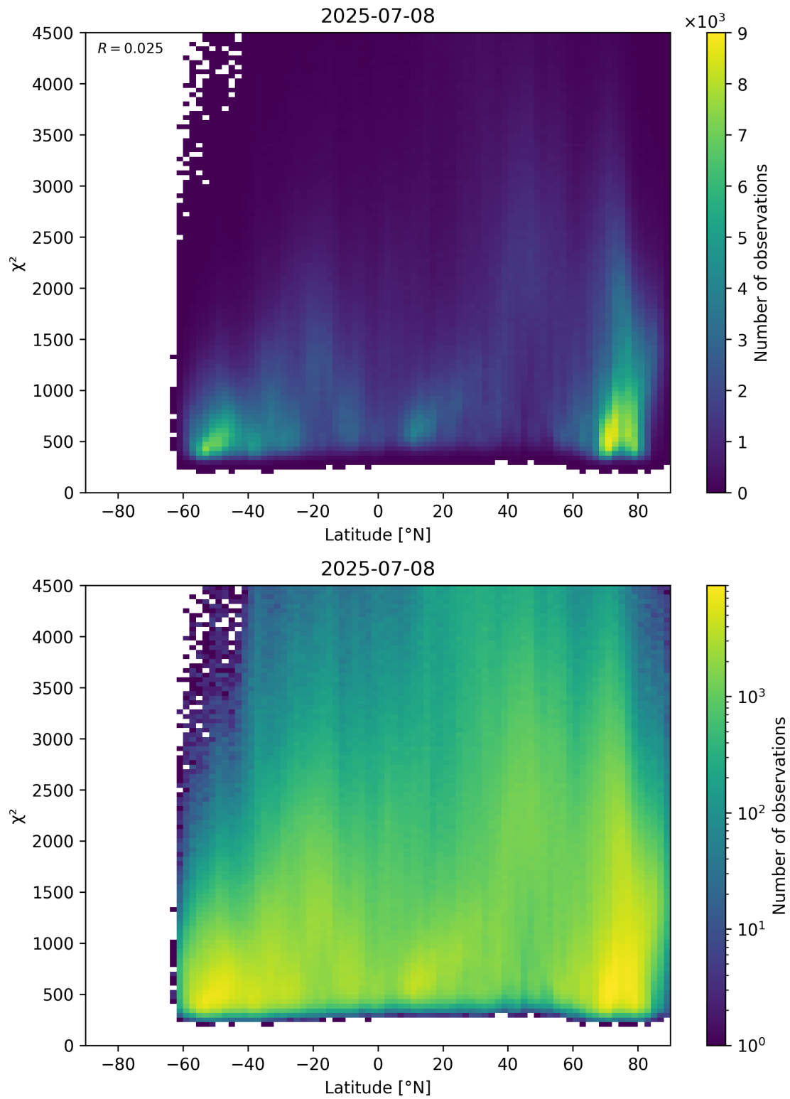
Figure 54: Scatter density plot of “Latitude” against “ \chi^2 ” for 2025-07-08 to 2025-07-09.
