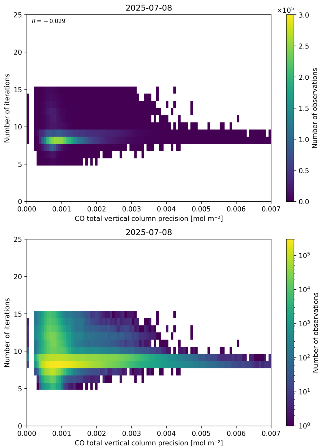
Figure 46: Scatter density plot of “CO total vertical column precision” against “Number of iterations” for 2025-07-08 to 2025-07-09.
