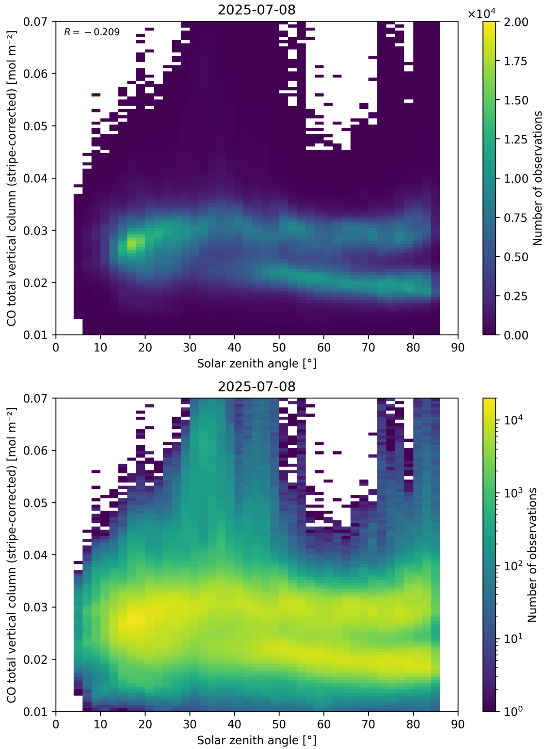
Figure 62: Scatter density plot of “Solar zenith angle” against “CO total vertical column (stripe-corrected)” for 2025-07-08 to 2025-07-09.
