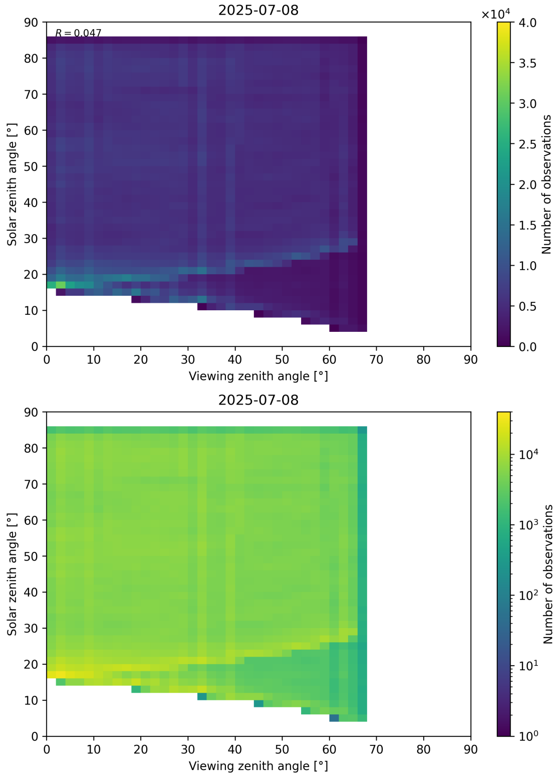
Figure 77: Scatter density plot of “Viewing zenith angle” against “Solar zenith angle” for 2025-07-08 to 2025-07-09.
