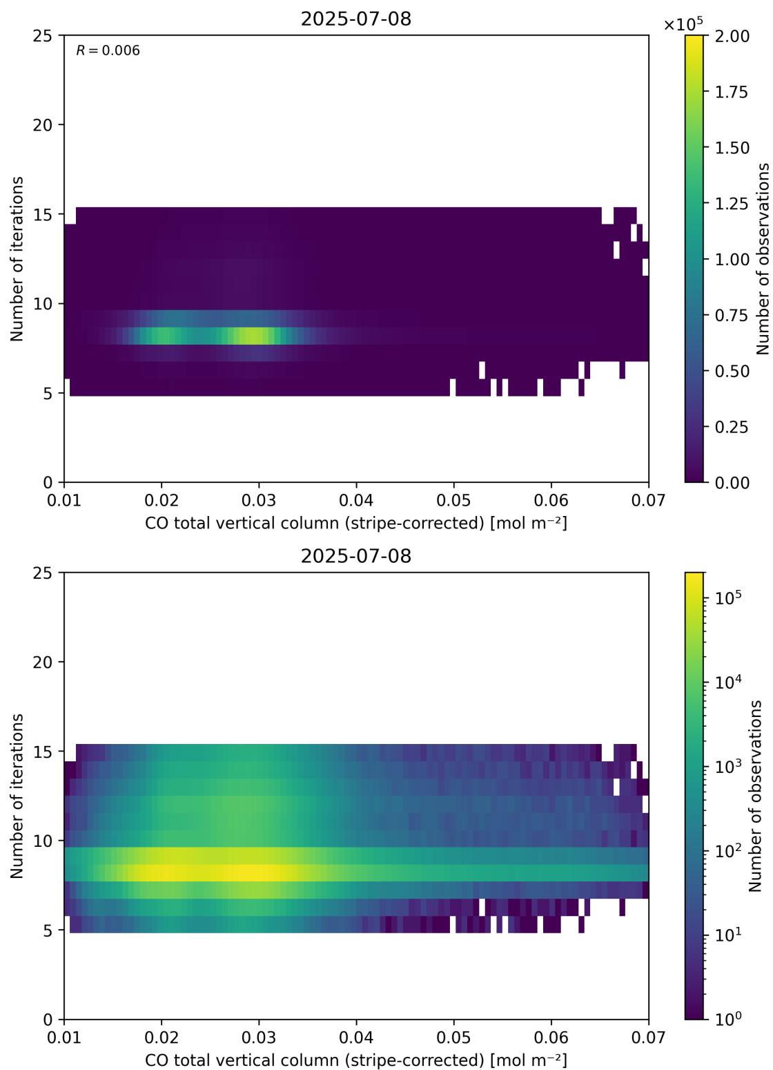
Figure 39: Scatter density plot of “CO total vertical column (stripe-corrected)” against “Number of iterations” for 2025-07-08 to 2025-07-09.
