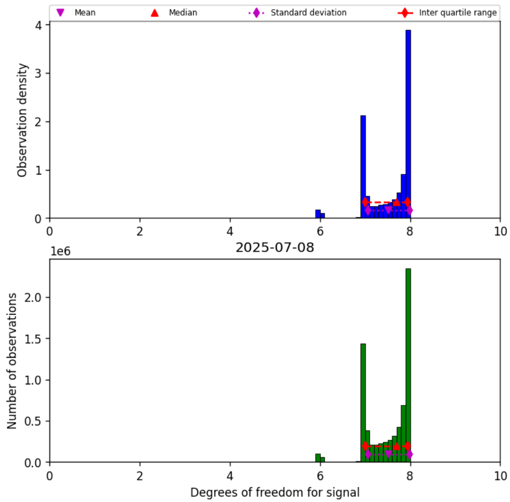
Figure 23: Histogram of “Degrees of freedom for signal” for 2025-07-08 to 2025-07-09
