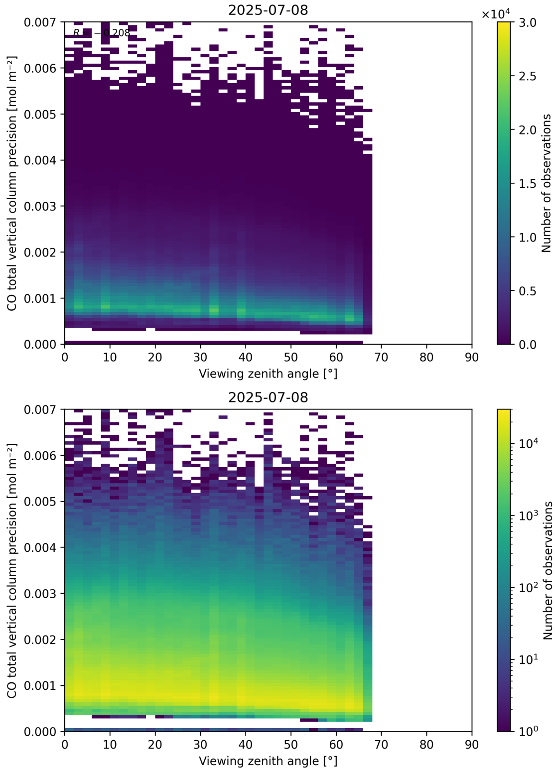
Figure 71: Scatter density plot of “Viewing zenith angle” against “CO total vertical column precision” for 2025-07-08 to 2025-07-09.
