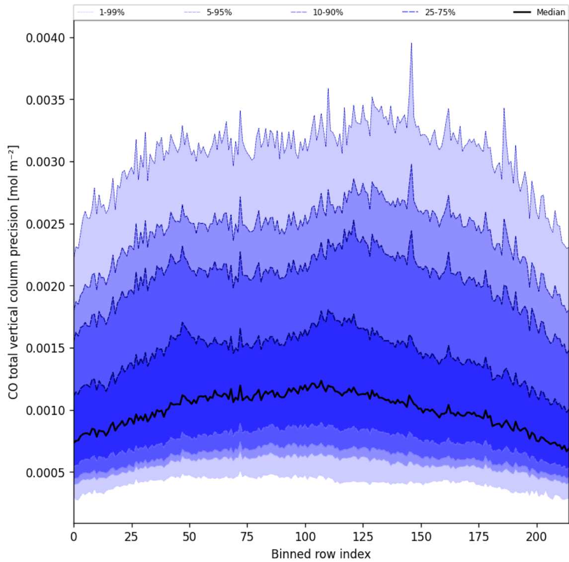
Figure 28: Along track statistics of “CO total vertical column precision” for 2025-07-08 to 2025-07-09
