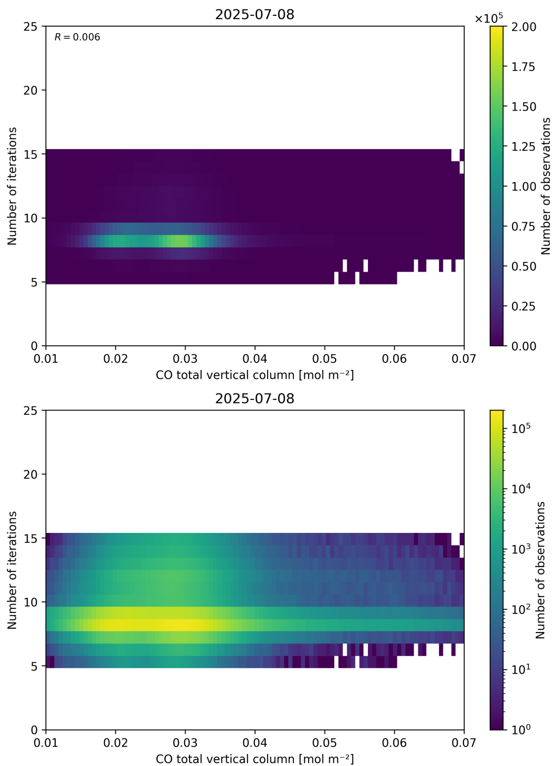
Figure 42: Scatter density plot of “CO total vertical column” against “Number of iterations” for 2025-07-08 to 2025-07-09.
