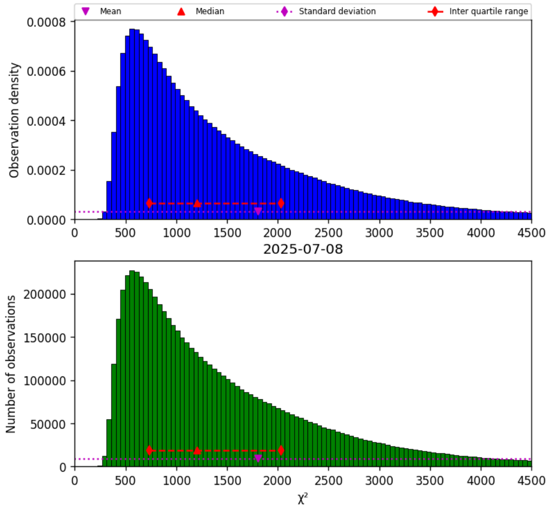
Figure 22: Histogram of " \chi^2 " for 2025-07-08 to 2025-07-09
