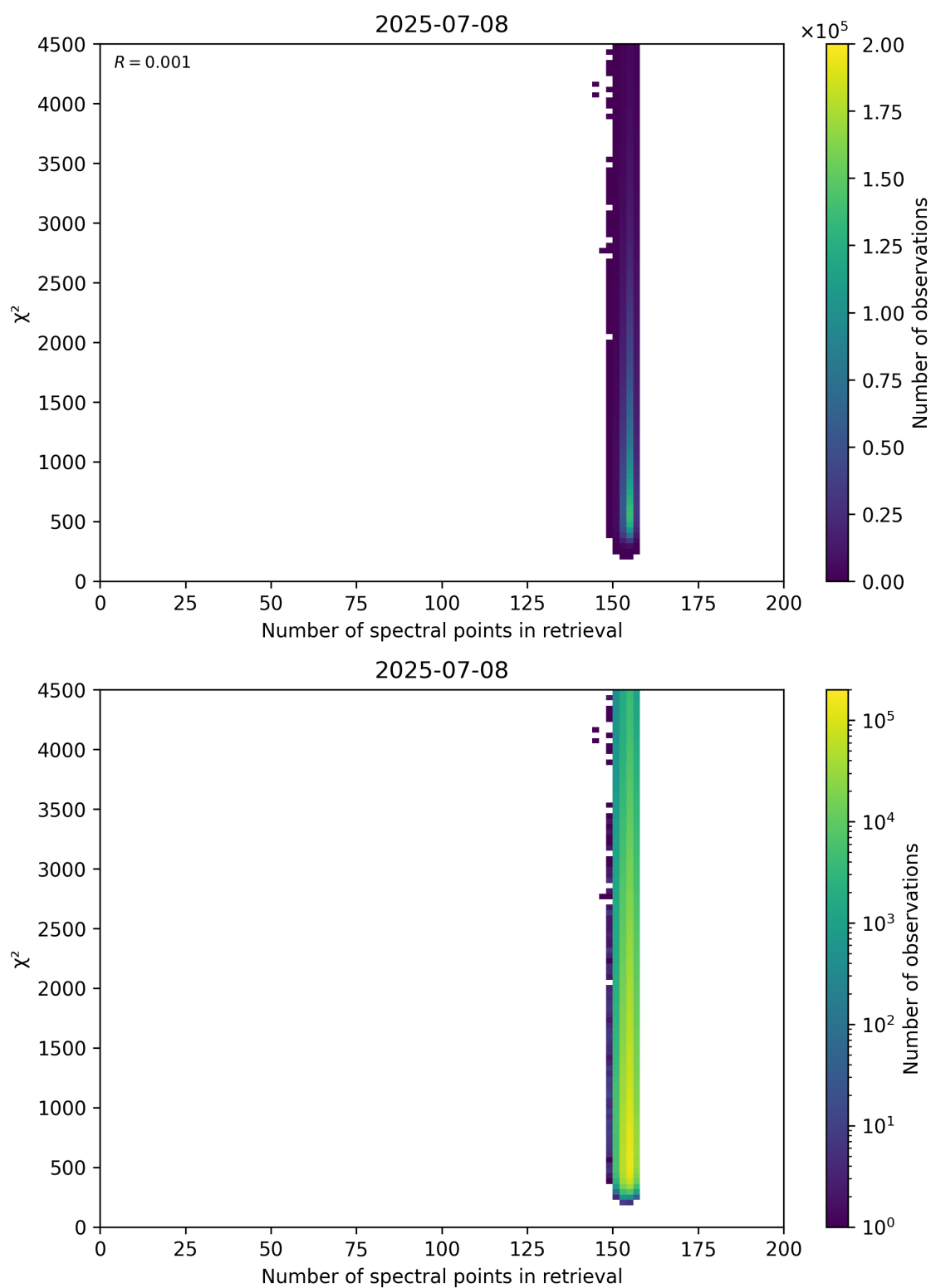
Figure 58: Scatter density plot of “Number of spectral points in retrieval” against “ \chi^2 ” for 2025-07-08 to 2025-07-09.
