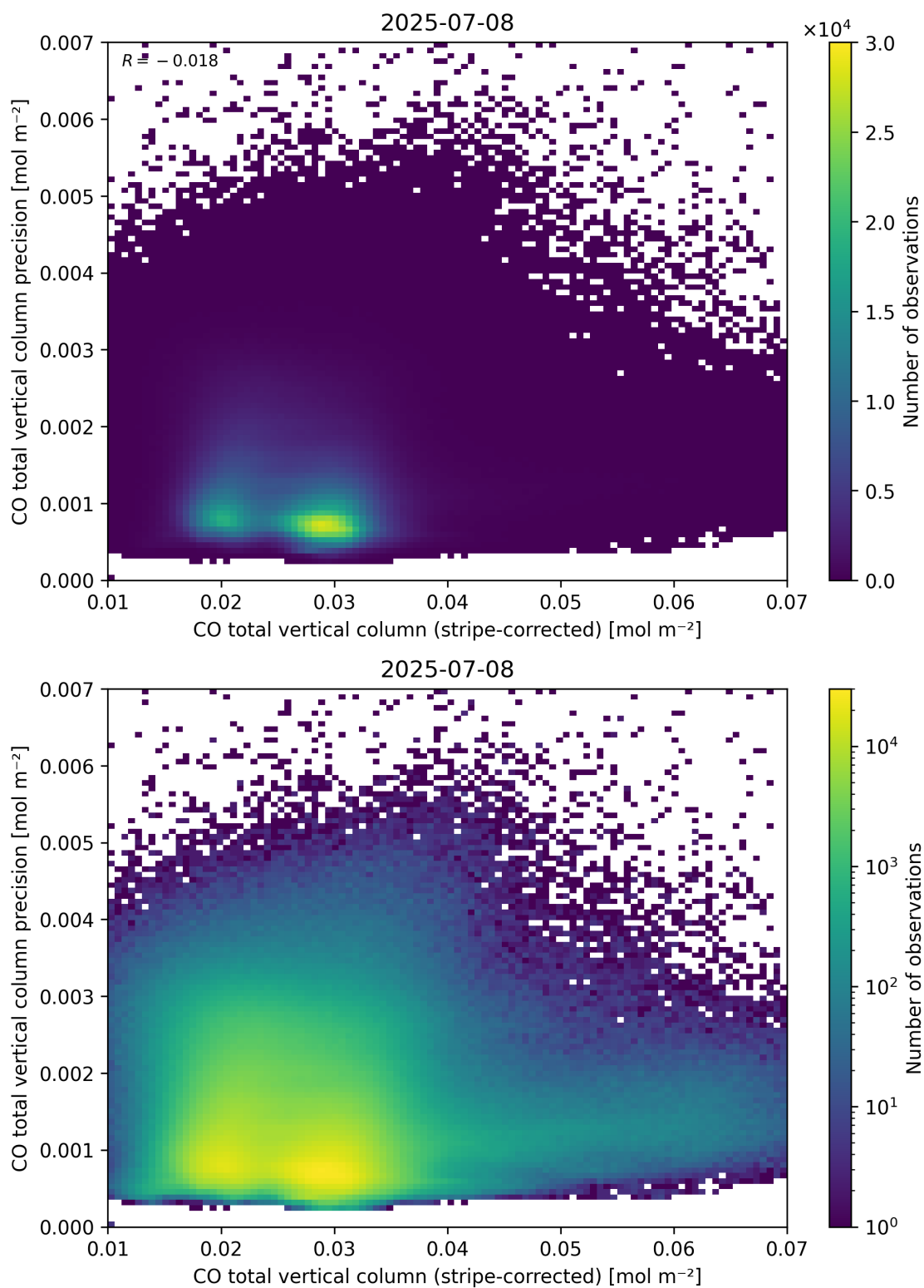
Figure 36: Scatter density plot of “CO total vertical column (stripe-corrected)” against “CO total vertical column precision” for 2025-07-08 to 2025-07-09.
