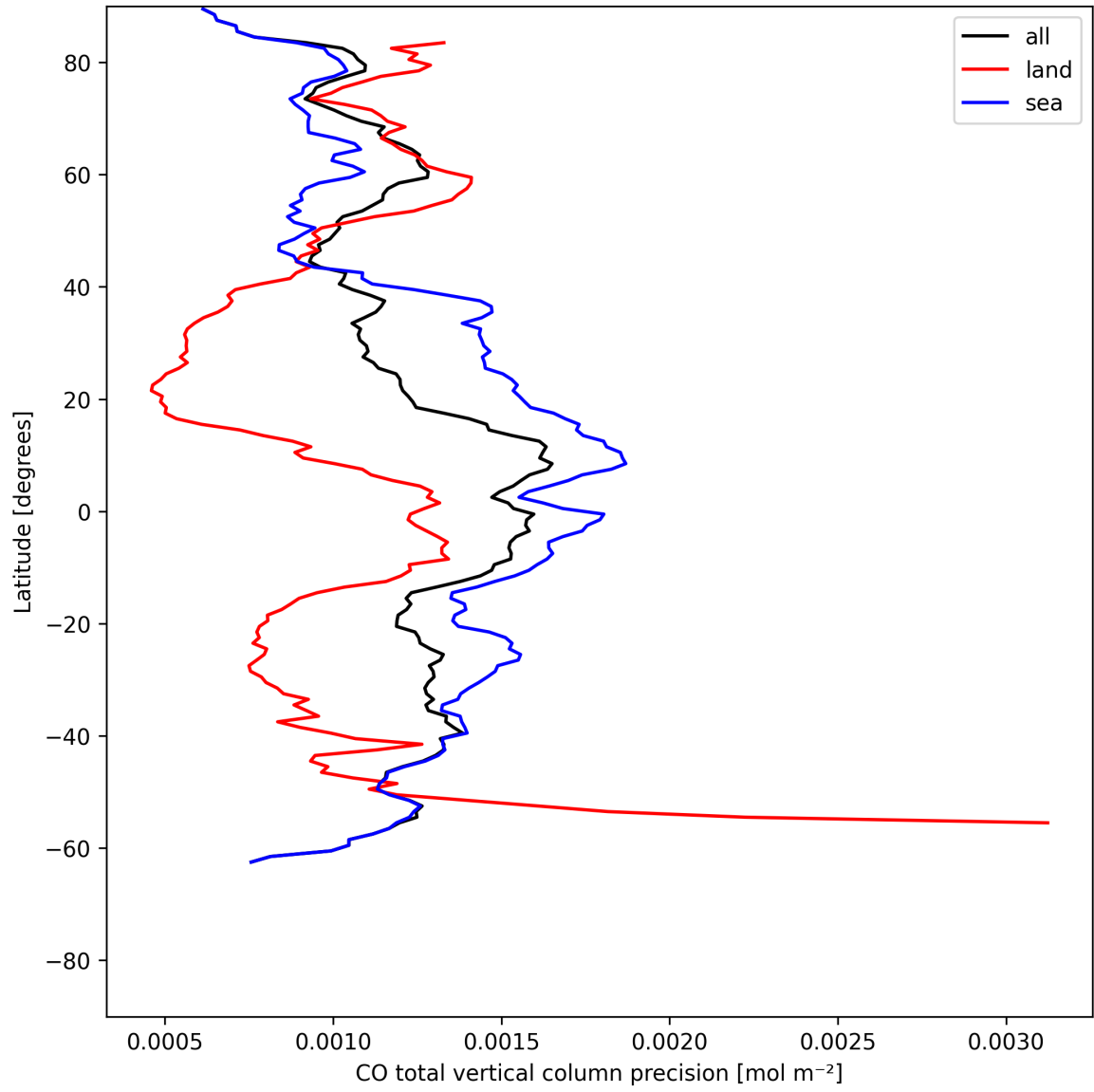
Figure 12: Zonal average of “CO total vertical column precision” for 2025-07-08 to 2025-07-09.
