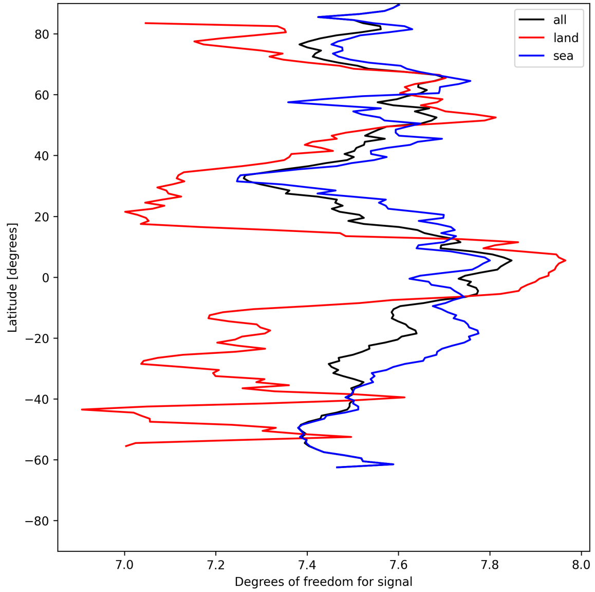
Figure 15: Zonal average of “Degrees of freedom for signal” for 2025-07-08 to 2025-07-09.
