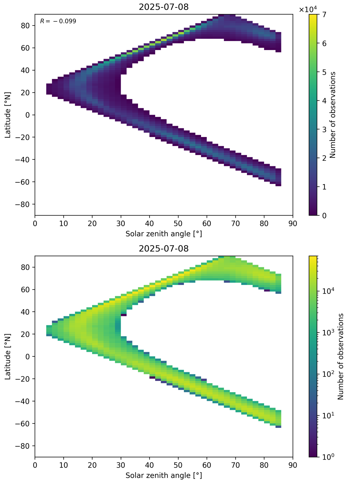
Figure 66: Scatter density plot of “Solar zenith angle” against “Latitude” for 2025-07-08 to 2025-07-09.
