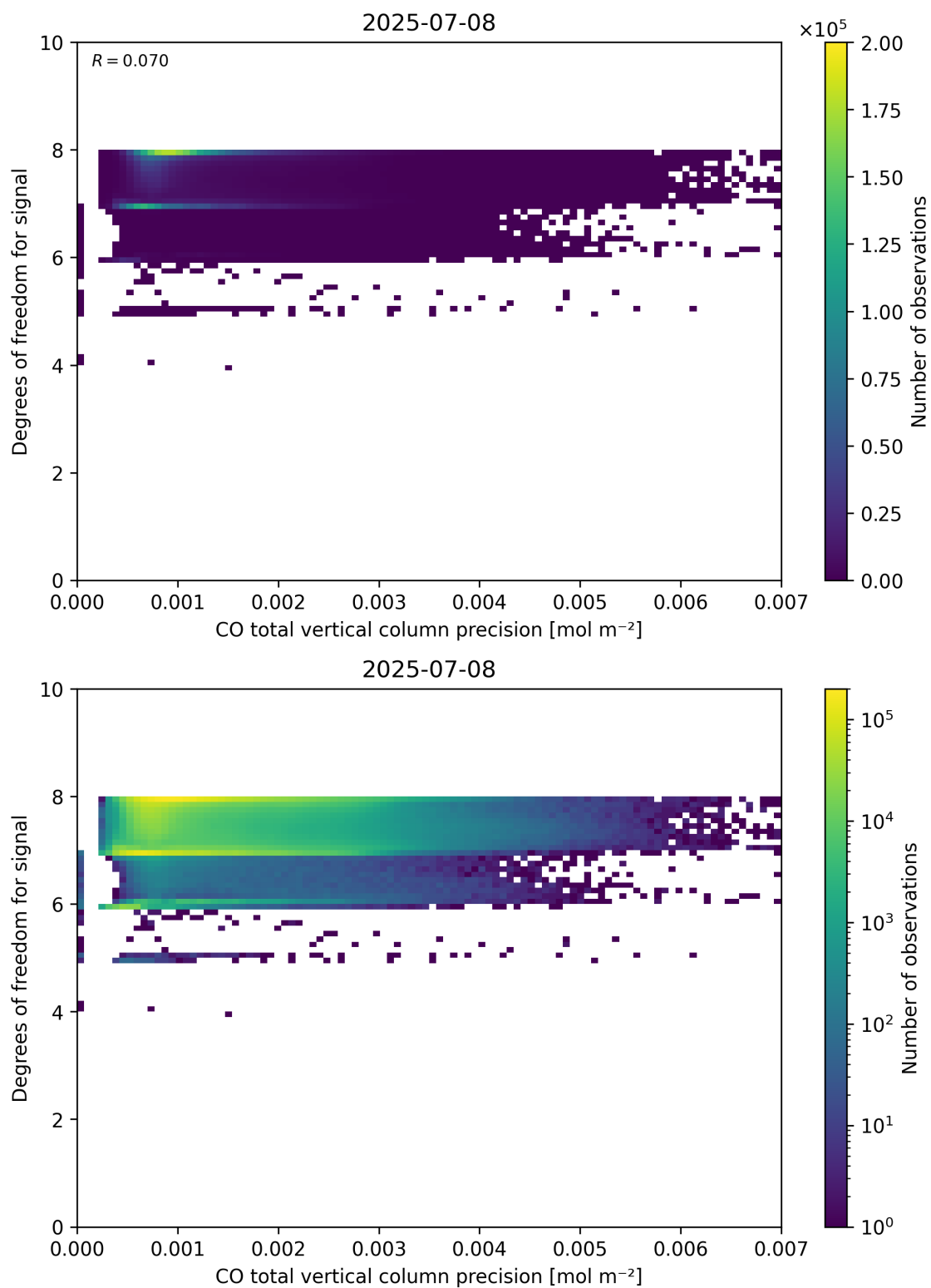
Figure 45: Scatter density plot of “CO total vertical column precision” against “Degrees of freedom for signal” for 2025-07-08 to 2025-07-09.
