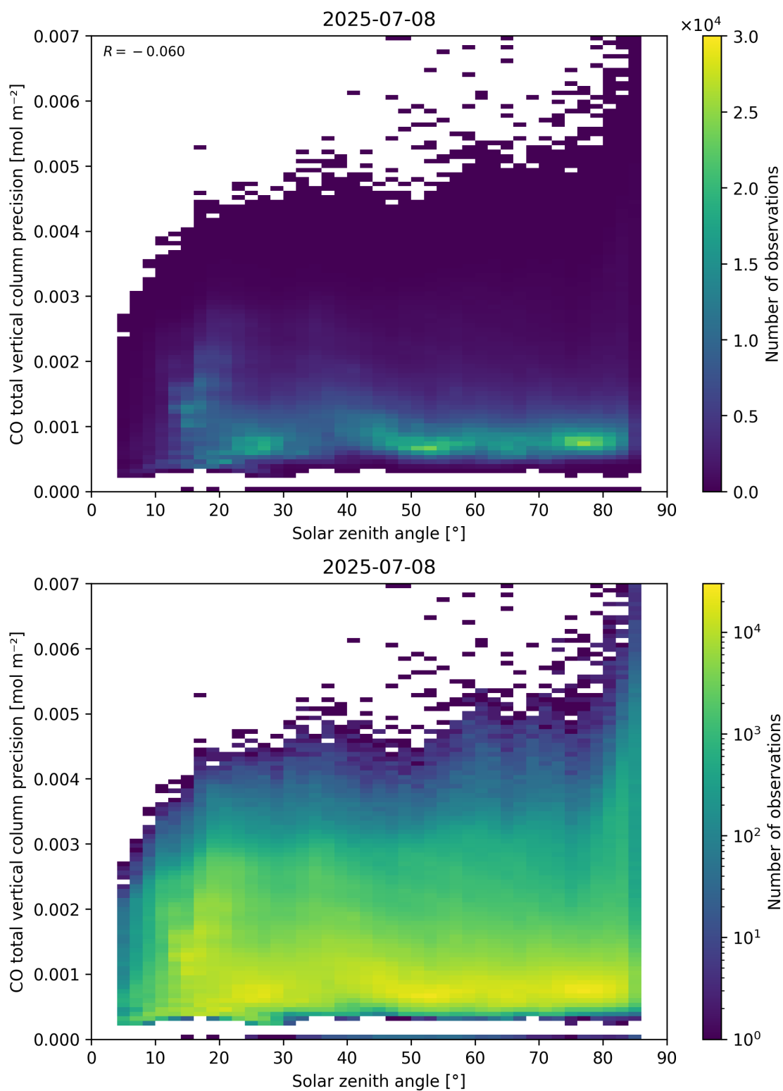
Figure 63: Scatter density plot of “Solar zenith angle” against “CO total vertical column precision” for 2025-07-08 to 2025-07-09.
