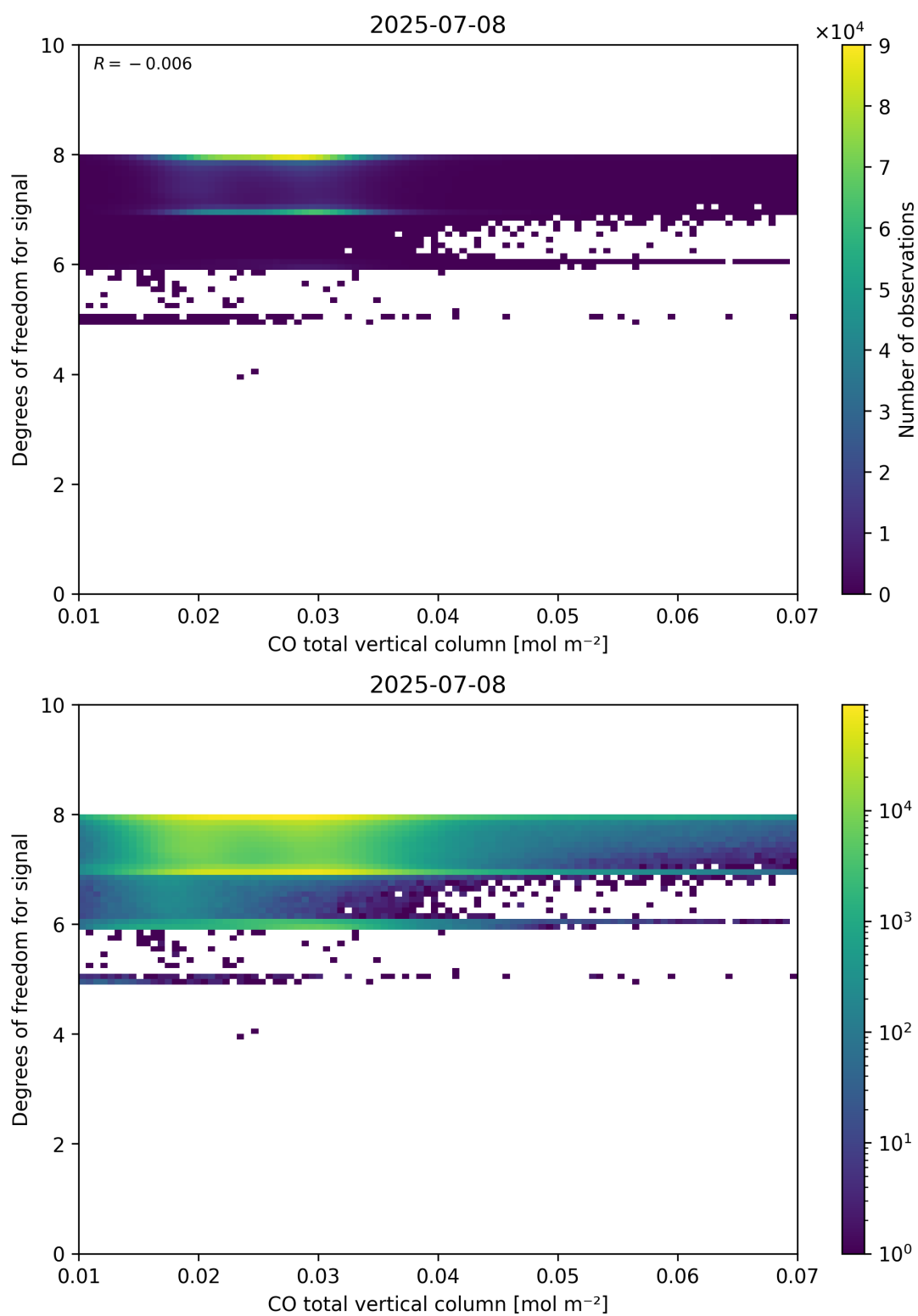
Figure 41: Scatter density plot of “CO total vertical column” against “Degrees of freedom for signal” for 2025-07-08 to 2025-07-09.
