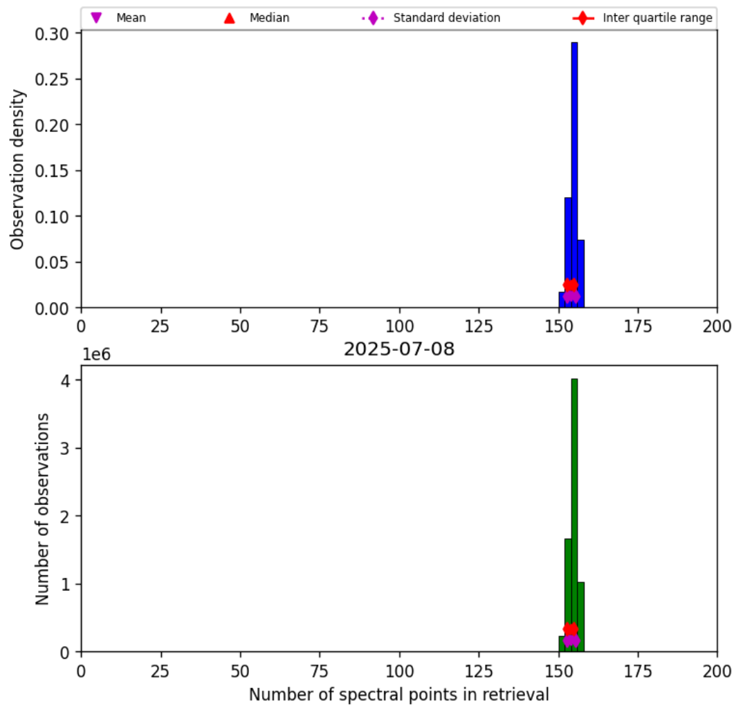
Figure 21: Histogram of “Number of spectral points in retrieval” for 2025-07-08 to 2025-07-09
