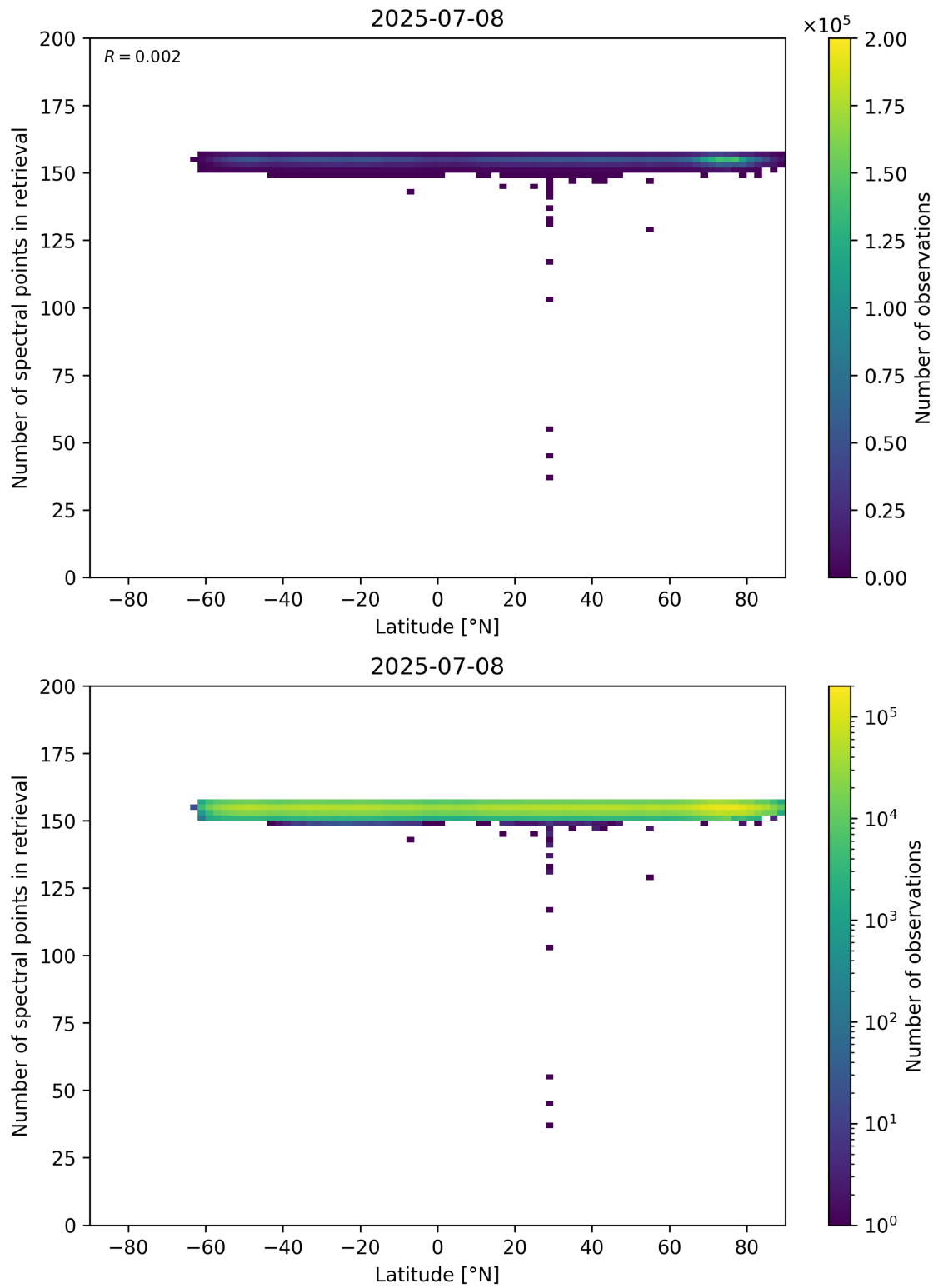
Figure 57: Scatter density plot of “Latitude” against “Number of spectral points in retrieval” for 2025-07-08 to 2025-07-09.
