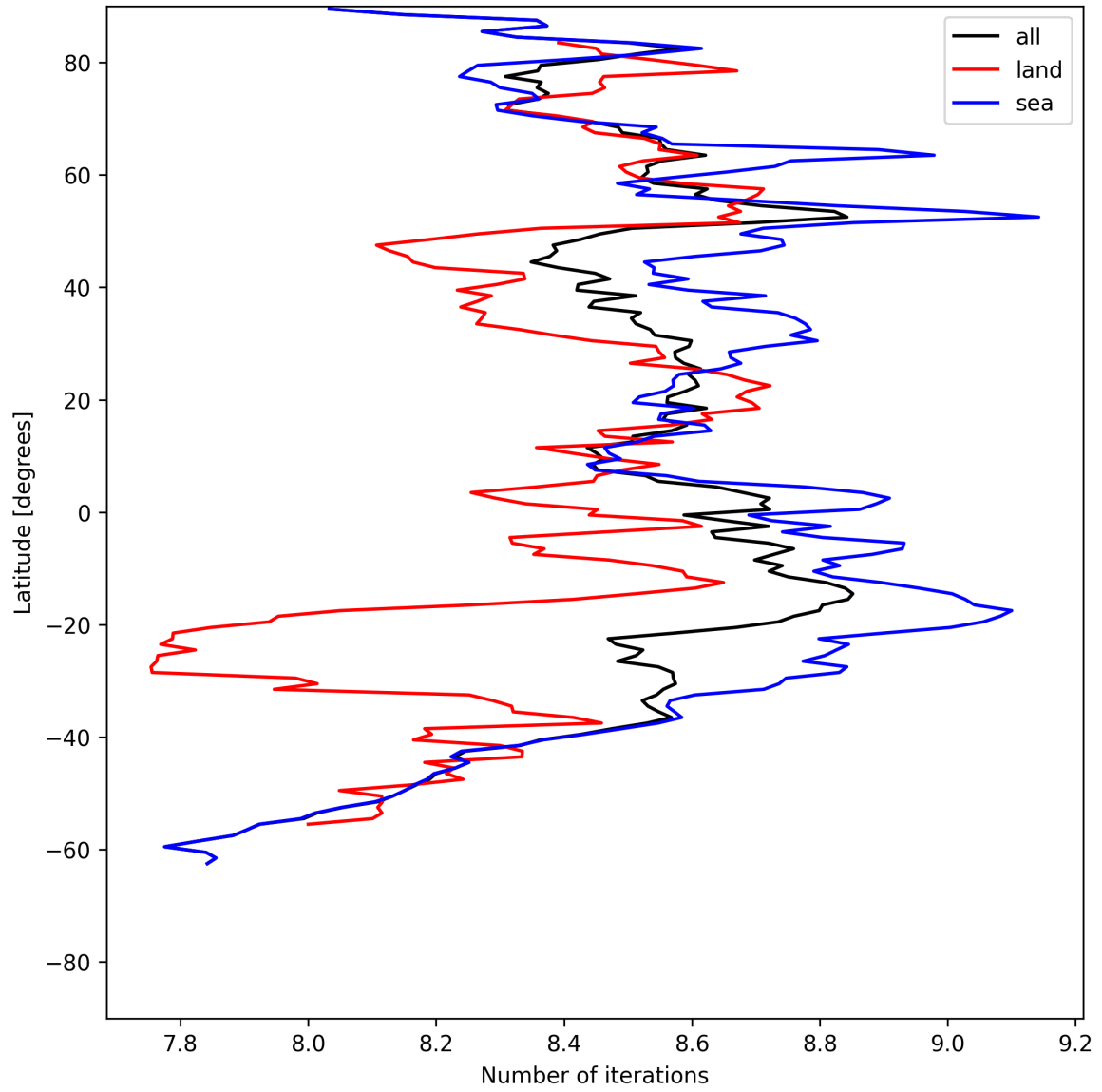
Figure 16: Zonal average of “Number of iterations” for 2025-07-08 to 2025-07-09.
