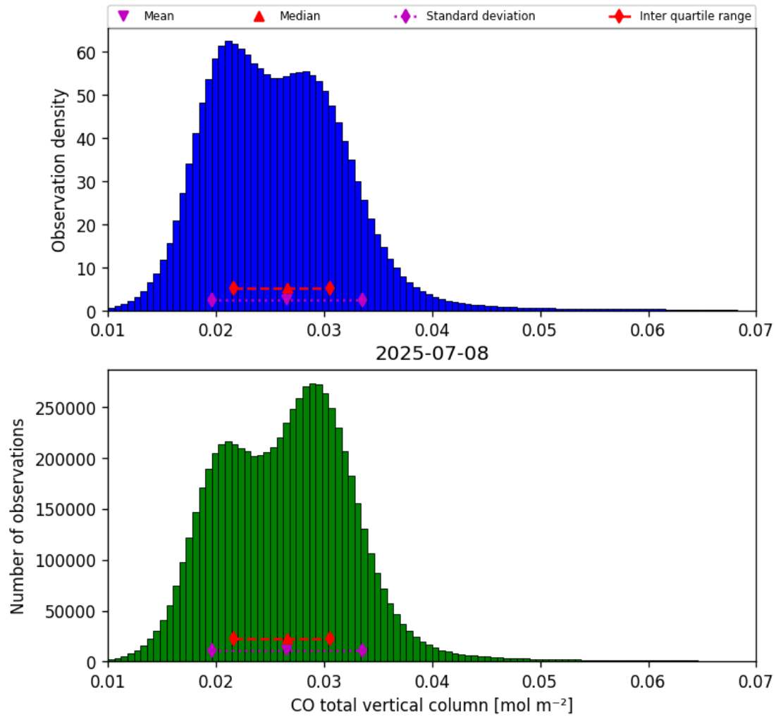
Figure 18: Histogram of “CO total vertical column” for 2025-07-08 to 2025-07-09
