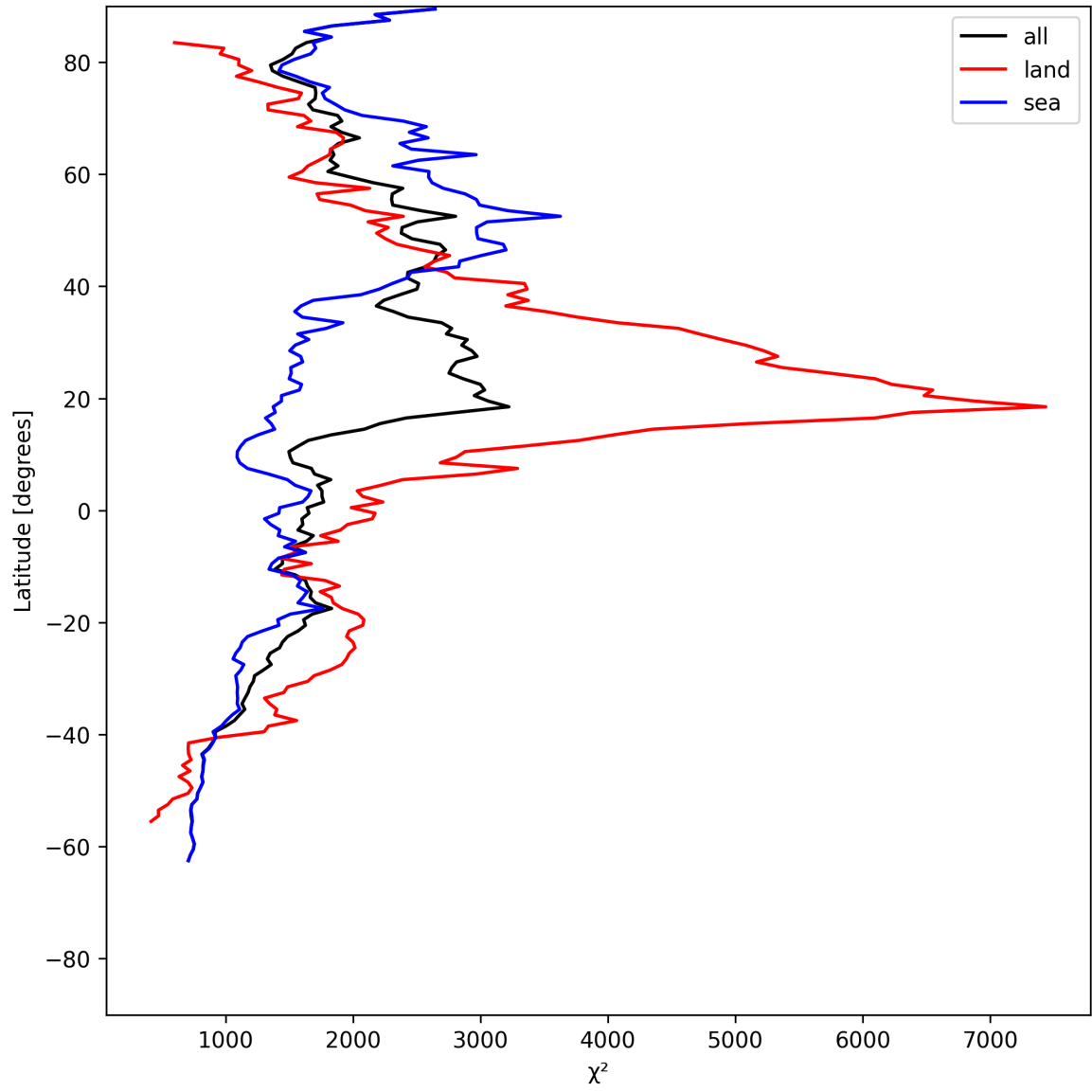
Figure 14: Zonal average of “ \chi^2 ” for 2025-07-08 to 2025-07-09.
