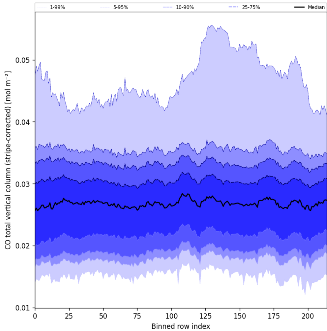
Figure 27: Along track statistics of “CO total vertical column (stripe-corrected)” for 2025-07-08 to 2025-07-09
