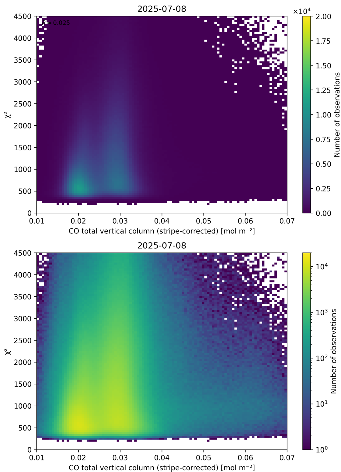
Figure 37: Scatter density plot of “CO total vertical column (stripe-corrected)” against “ \chi^2 ” for 2025-07-08 to 2025-07-09.
