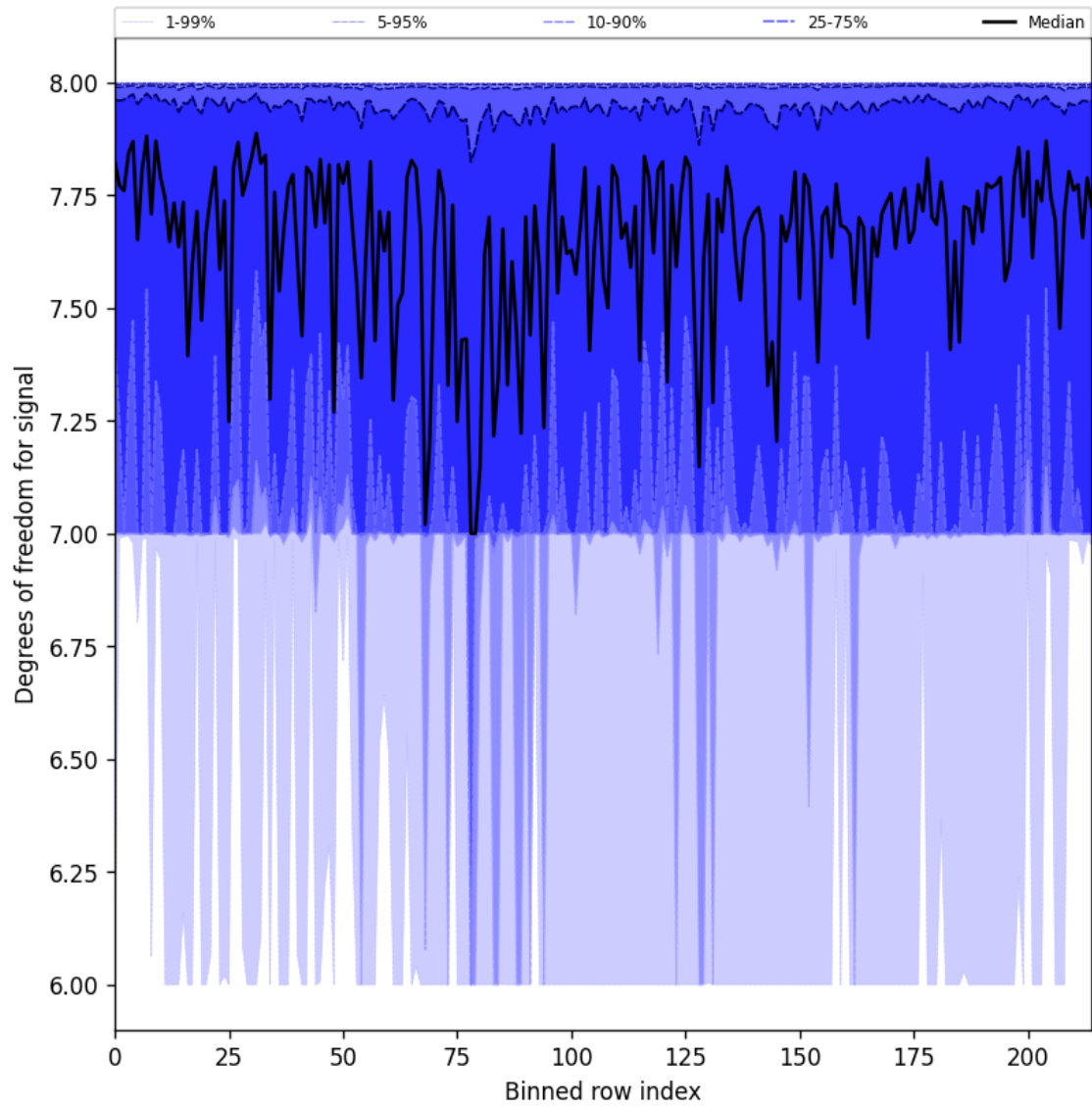
Figure 31: Along track statistics of “Degrees of freedom for signal” for 2025-07-08 to 2025-07-09
