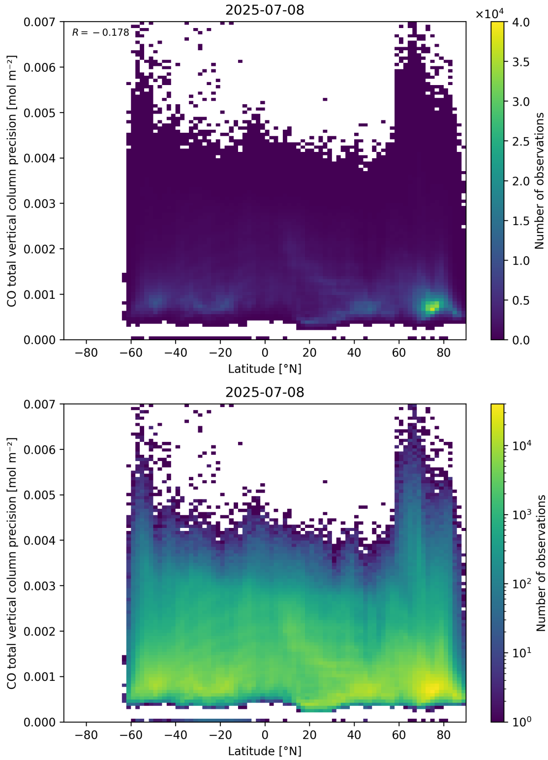
Figure 53: Scatter density plot of “Latitude” against “CO total vertical column precision” for 2025-07-08 to 2025-07-09.
