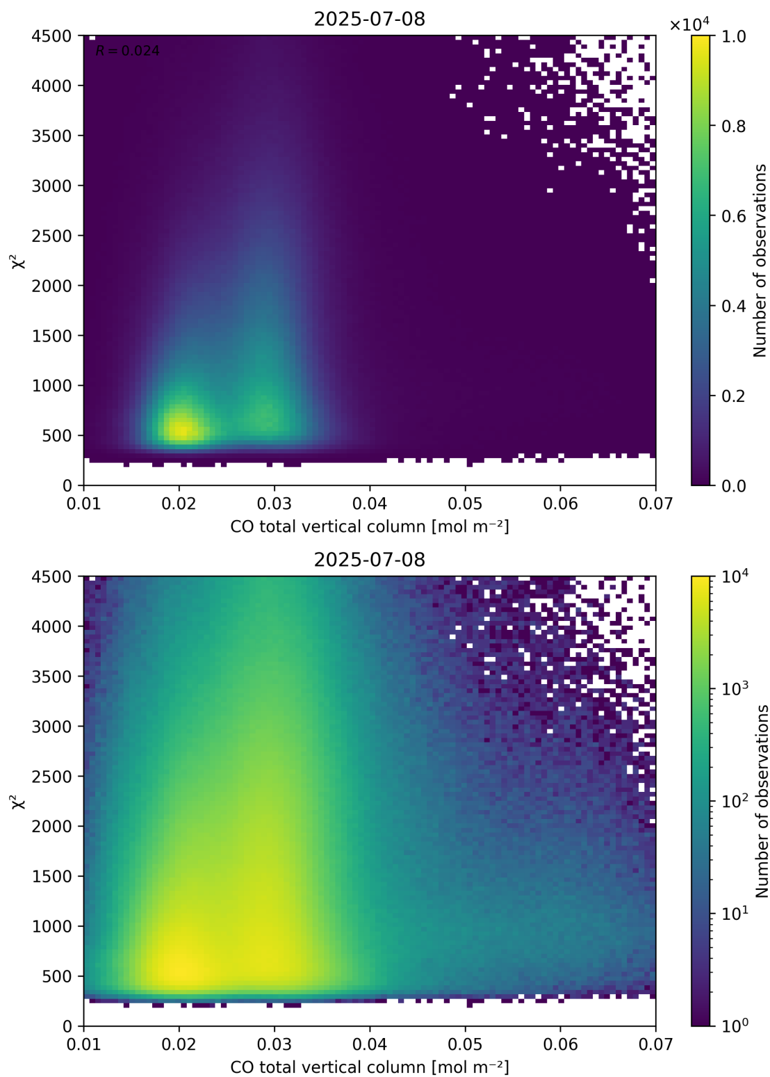
Figure 35: Scatter density plot of “CO total vertical column” against “ \chi^2 ” for 2025-07-08 to 2025-07-09.
