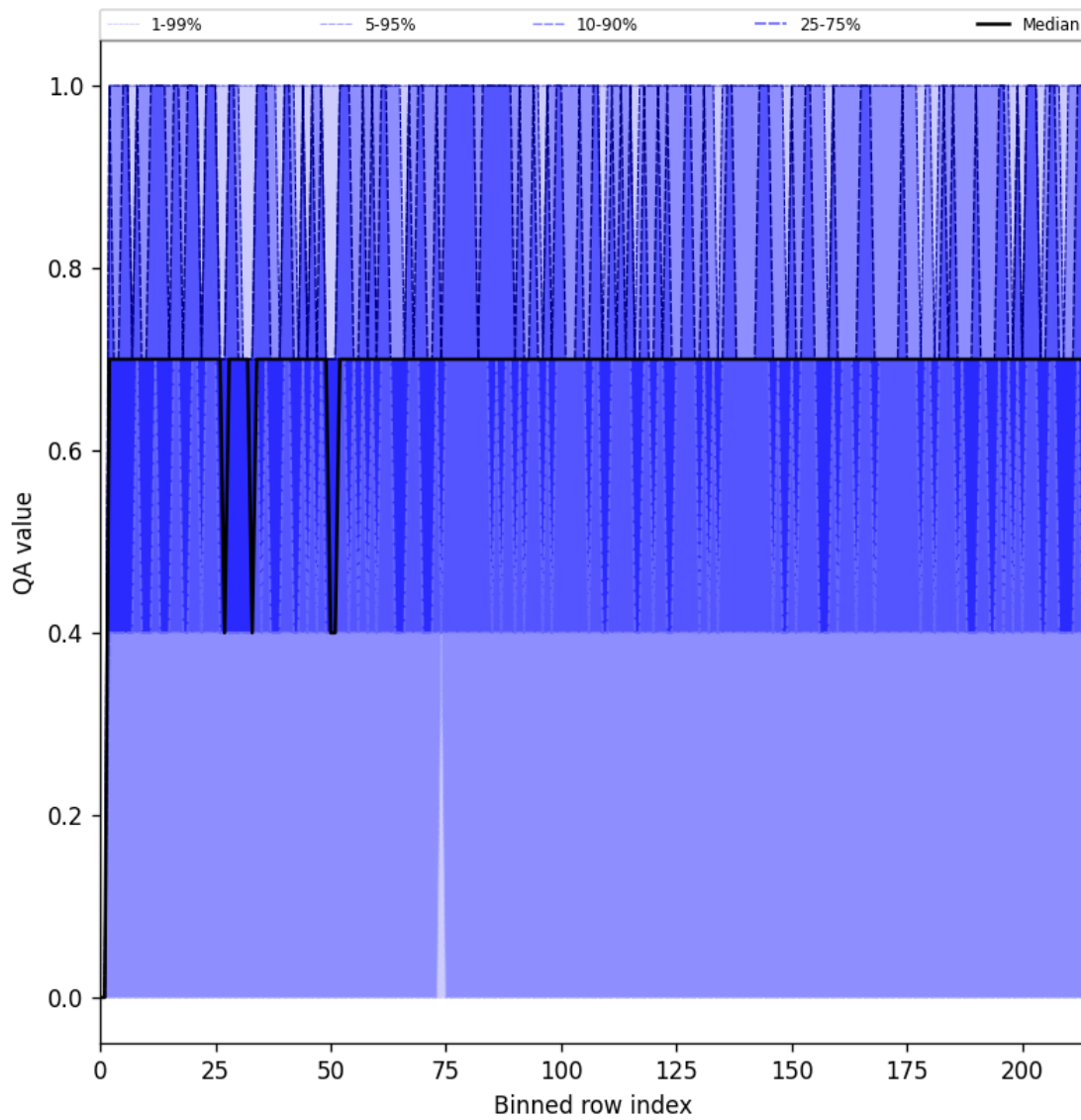
Figure 25: Along track statistics of “QA value” for 2025-07-08 to 2025-07-09
