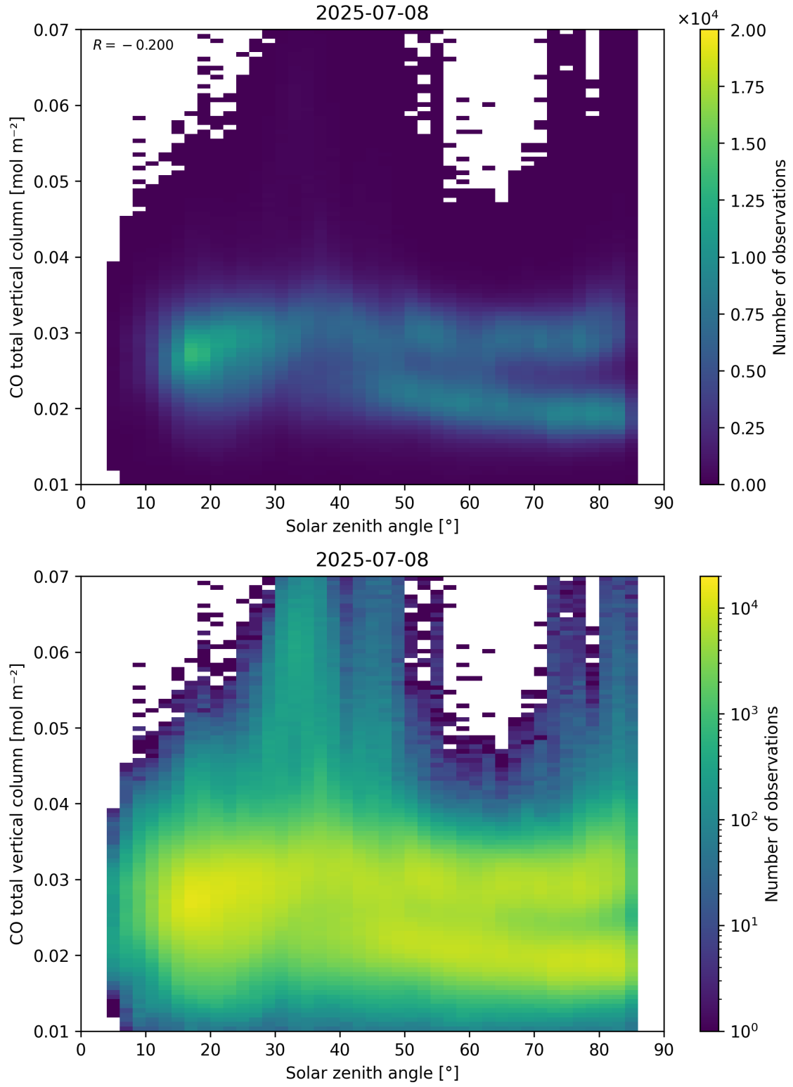
Figure 61: Scatter density plot of “Solar zenith angle” against “CO total vertical column” for 2025-07-08 to 2025-07-09.
