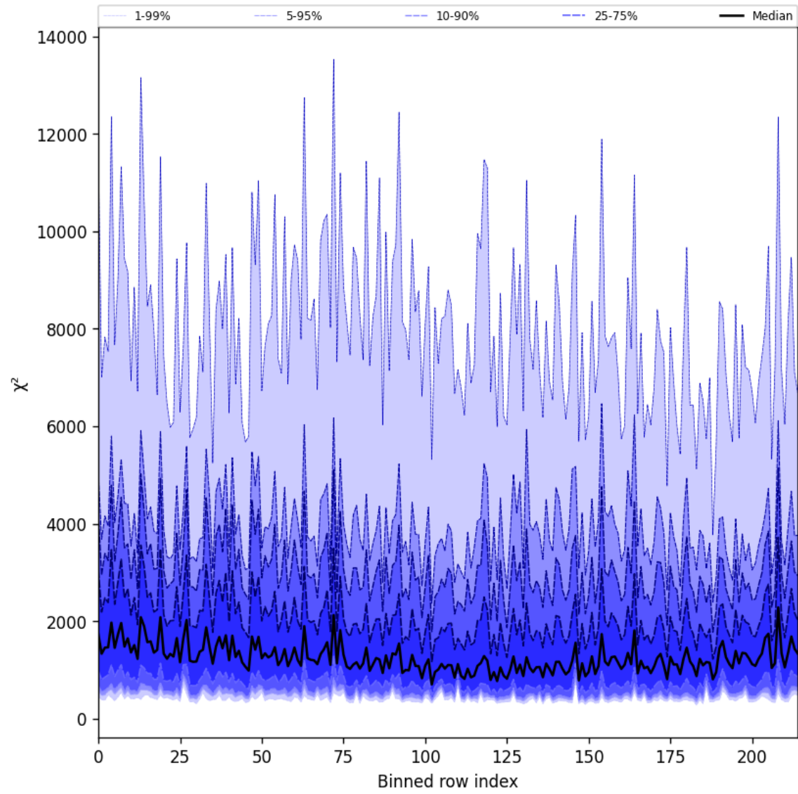
Figure 30: Along track statistics of “ \chi^2 ” for 2025-07-08 to 2025-07-09
