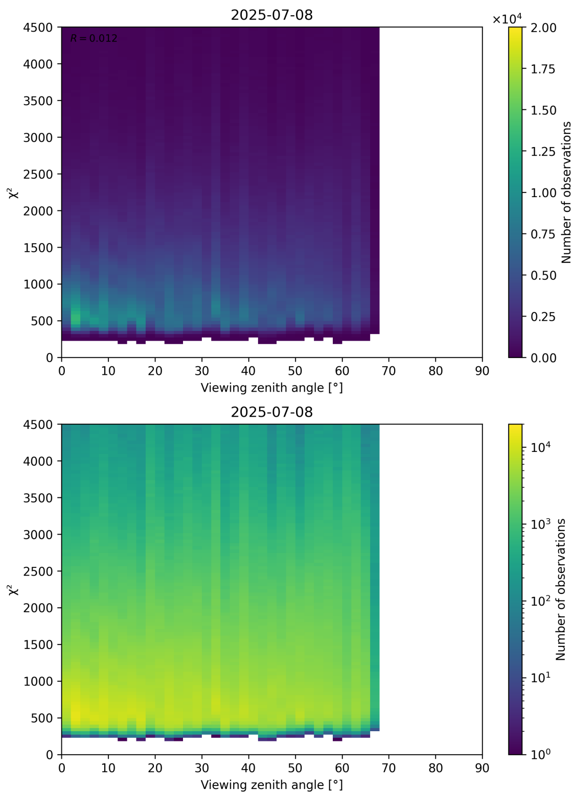
Figure 72: Scatter density plot of “Viewing zenith angle” against “ \chi^2 ” for 2025-07-08 to 2025-07-09.
