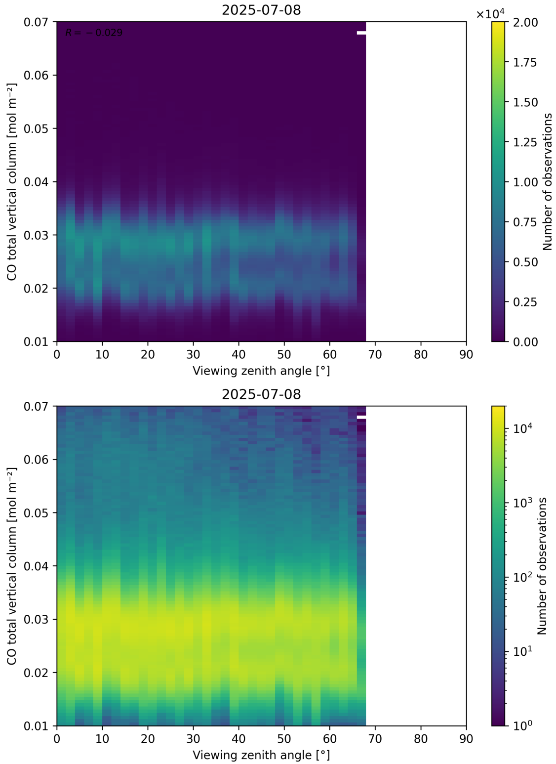
Figure 69: Scatter density plot of “Viewing zenith angle” against “CO total vertical column” for 2025-07-08 to 2025-07-09.
