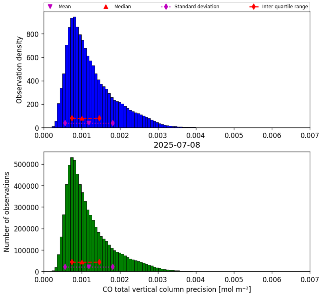
Figure 20: Histogram of “CO total vertical column precision” for 2025-07-08 to 2025-07-09
