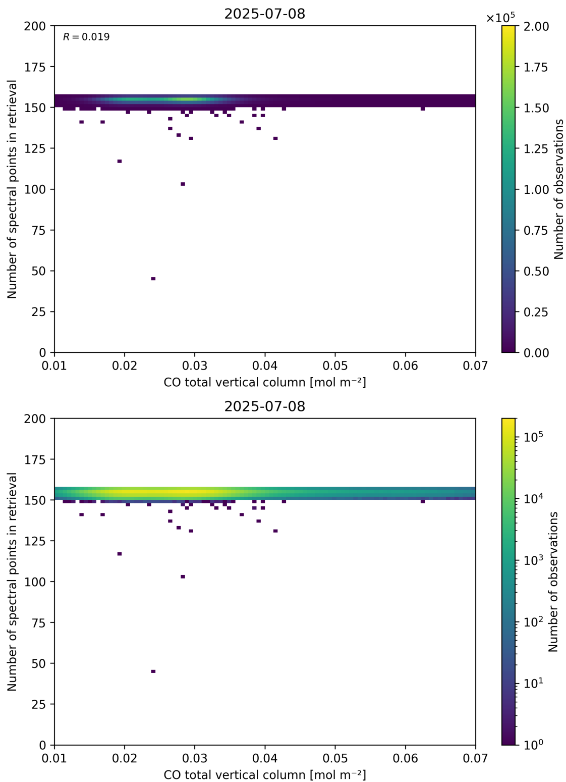
Figure 43: Scatter density plot of “CO total vertical column” against “Number of spectral points in retrieval” for 2025-07-08 to 2025-07-09.
