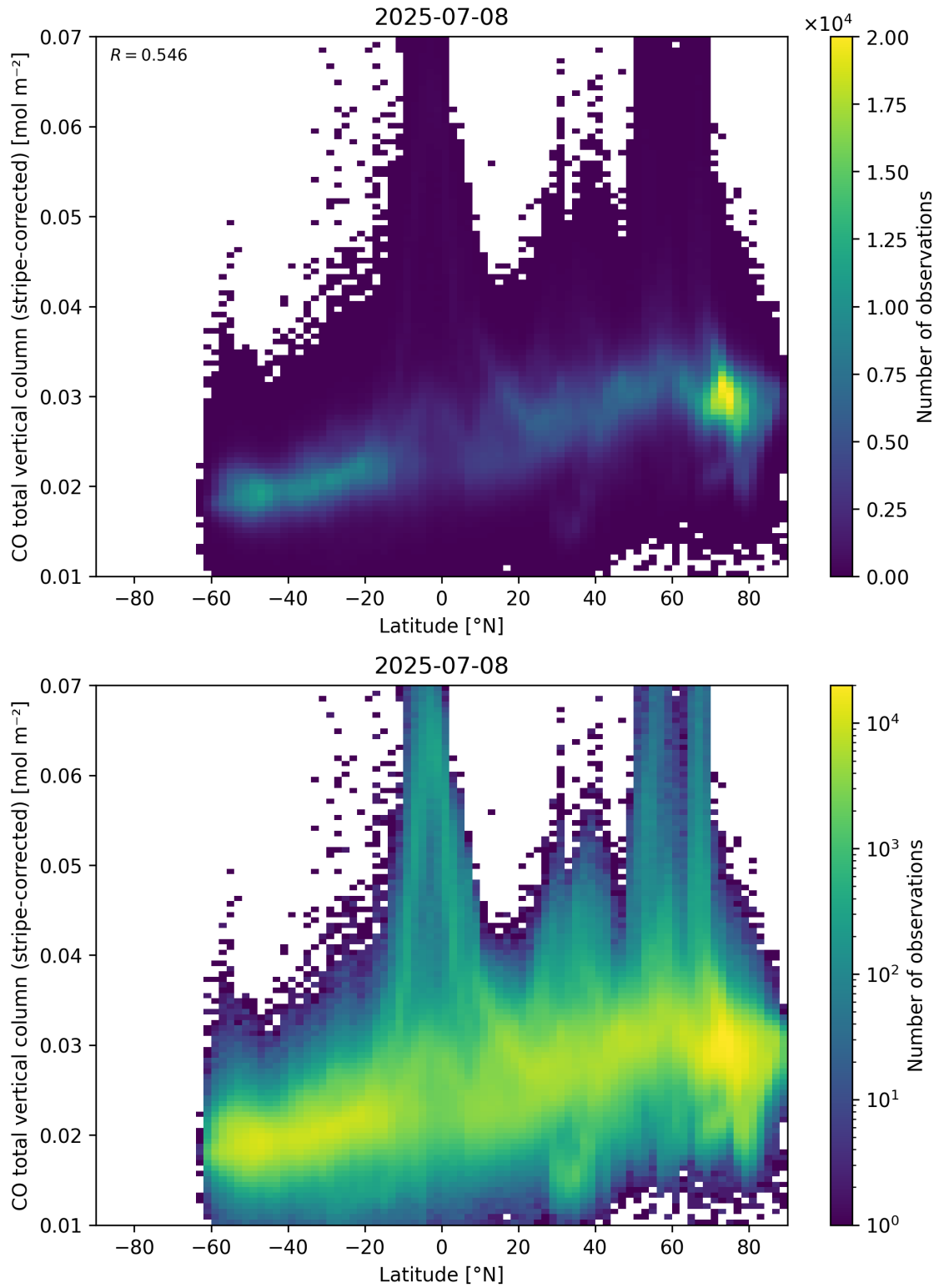
Figure 52: Scatter density plot of “Latitude” against “CO total vertical column (stripe-corrected)” for 2025-07-08 to 2025-07-09.
