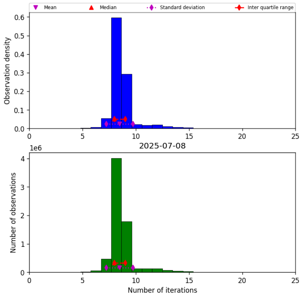
Figure 24: Histogram of “Number of iterations” for 2025-07-08 to 2025-07-09
