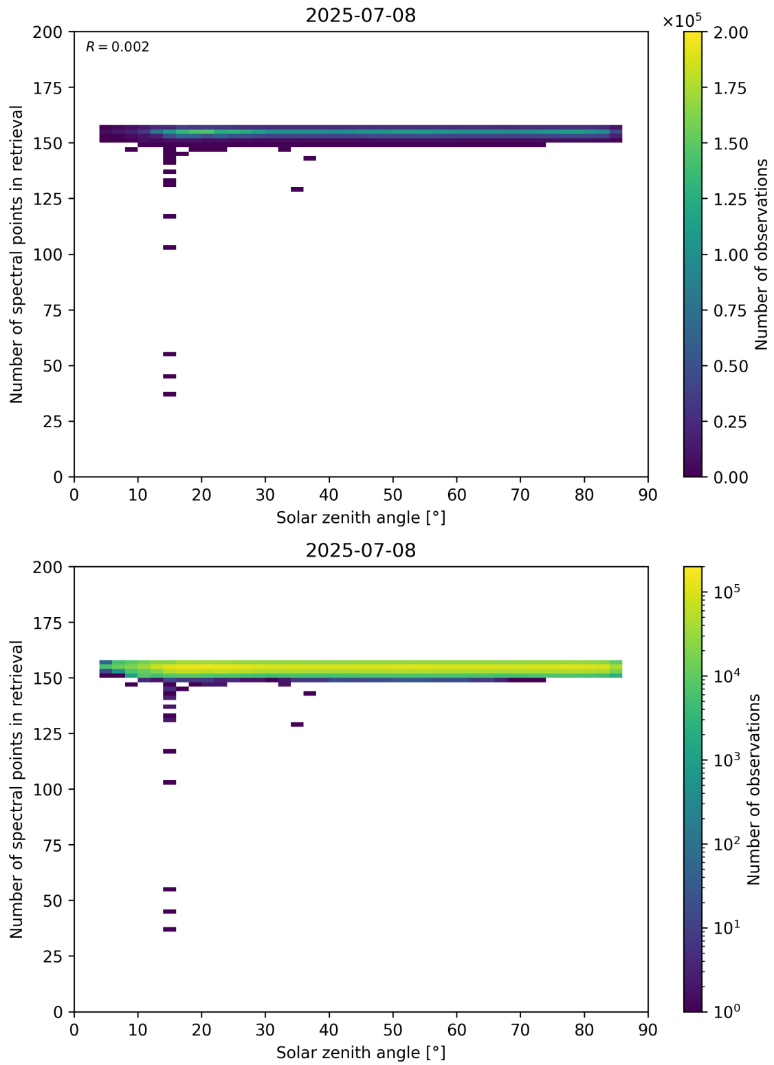
Figure 68: Scatter density plot of “Solar zenith angle” against “Number of spectral points in retrieval” for 2025-07-08 to 2025-07-09.
