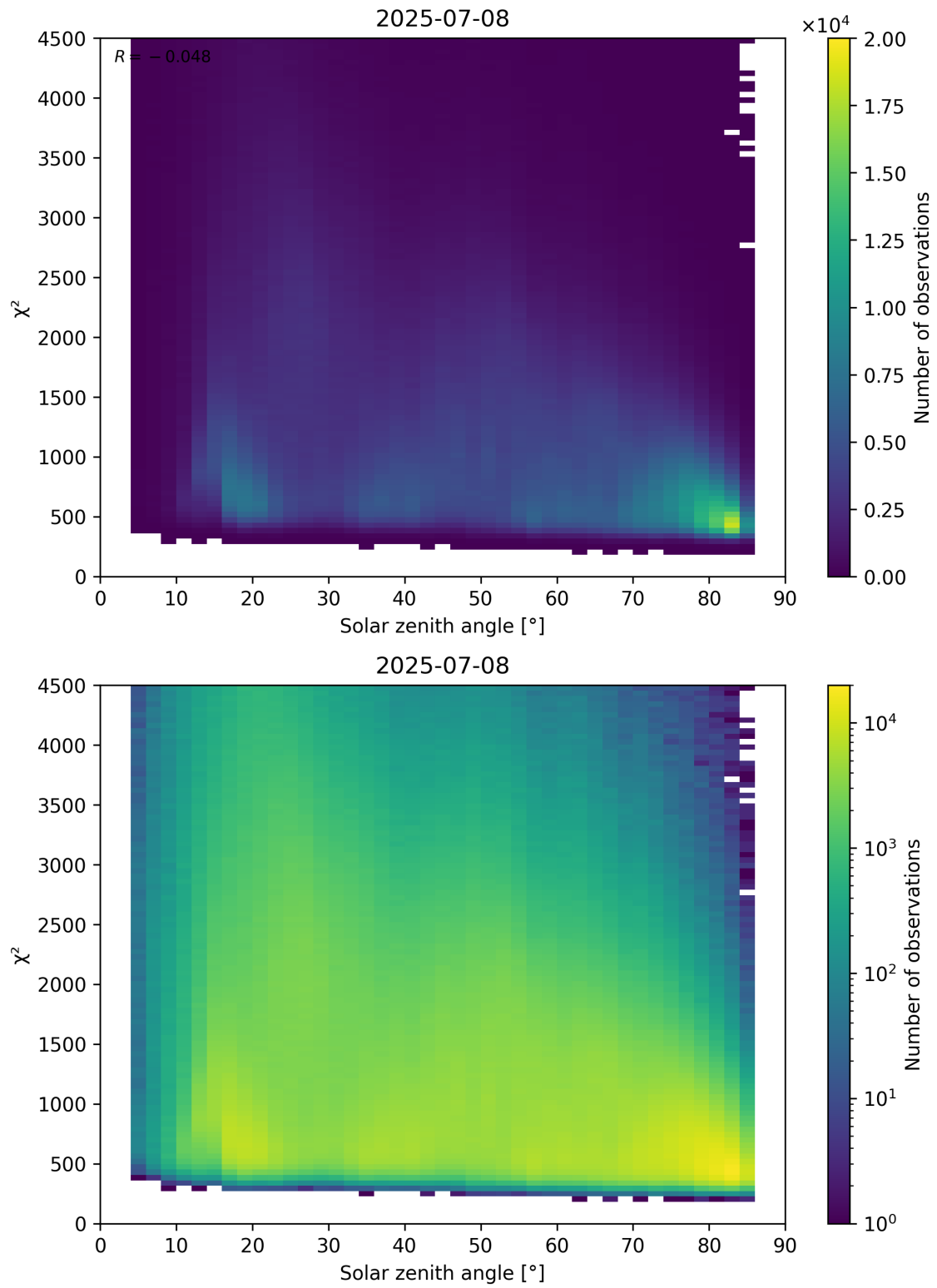
Figure 64: Scatter density plot of “Solar zenith angle” against “ \chi^2 ” for 2025-07-08 to 2025-07-09.
