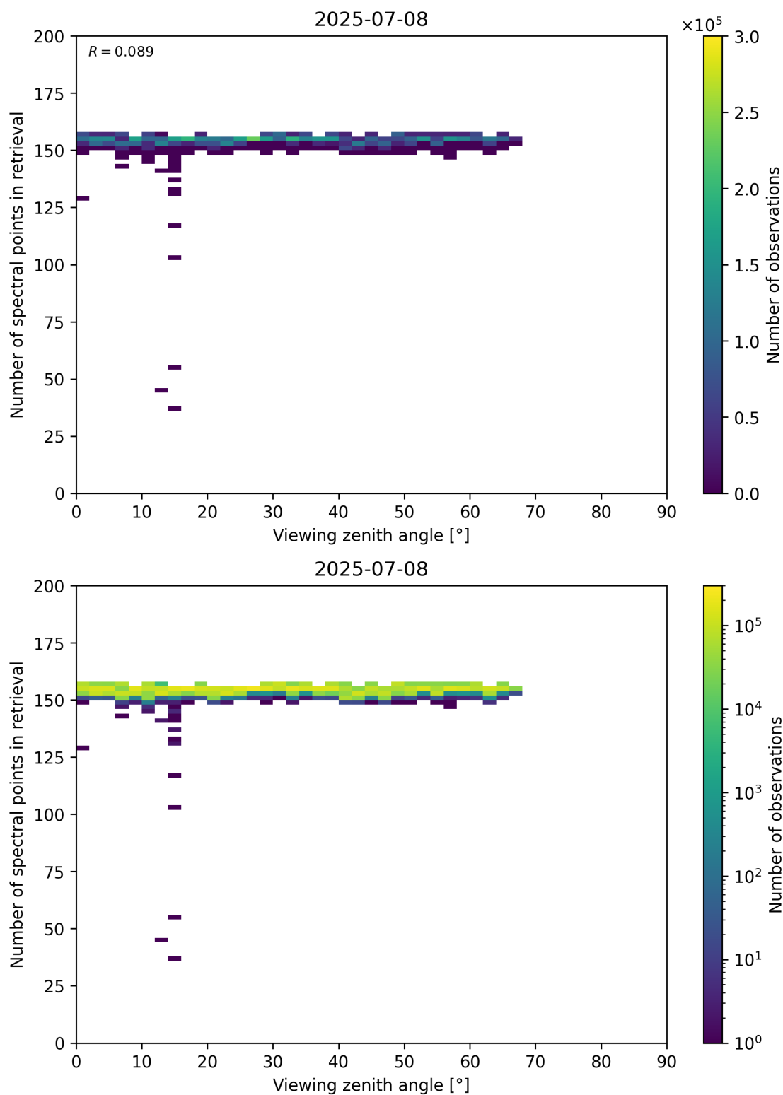
Figure 76: Scatter density plot of “Viewing zenith angle” against “Number of spectral points in retrieval” for 2025-07-08 to 2025-07-09.
