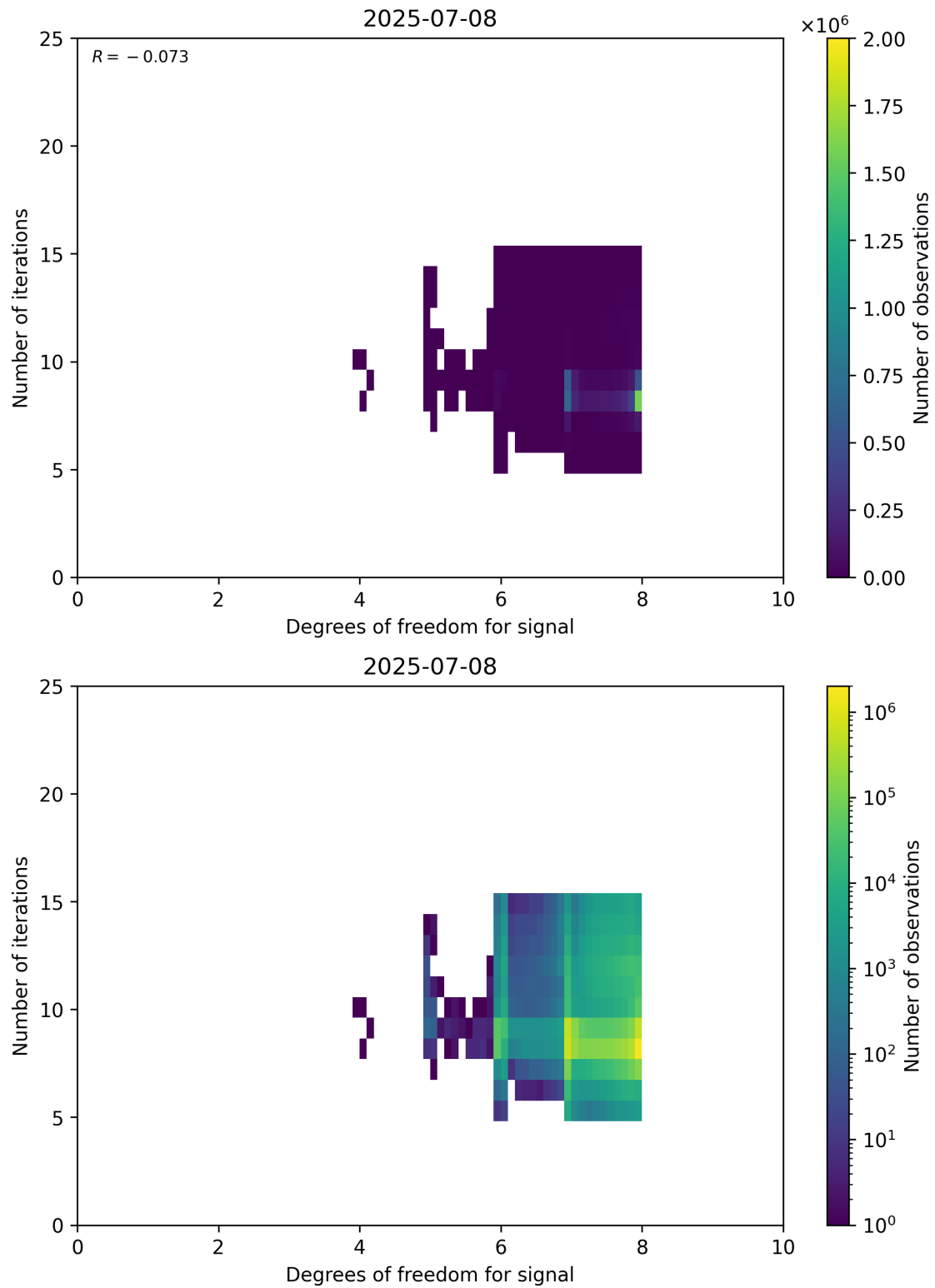
Figure 50: Scatter density plot of “Degrees of freedom for signal” against “Number of iterations” for 2025-07-08 to 2025-07-09.
