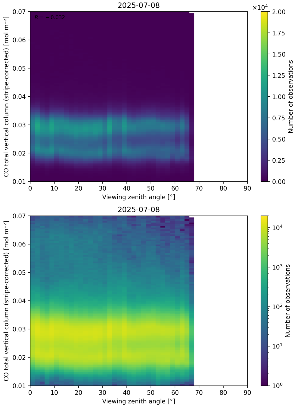
Figure 70: Scatter density plot of “Viewing zenith angle” against “CO total vertical column (stripe-corrected)” for 2025-07-08 to 2025-07-09.
