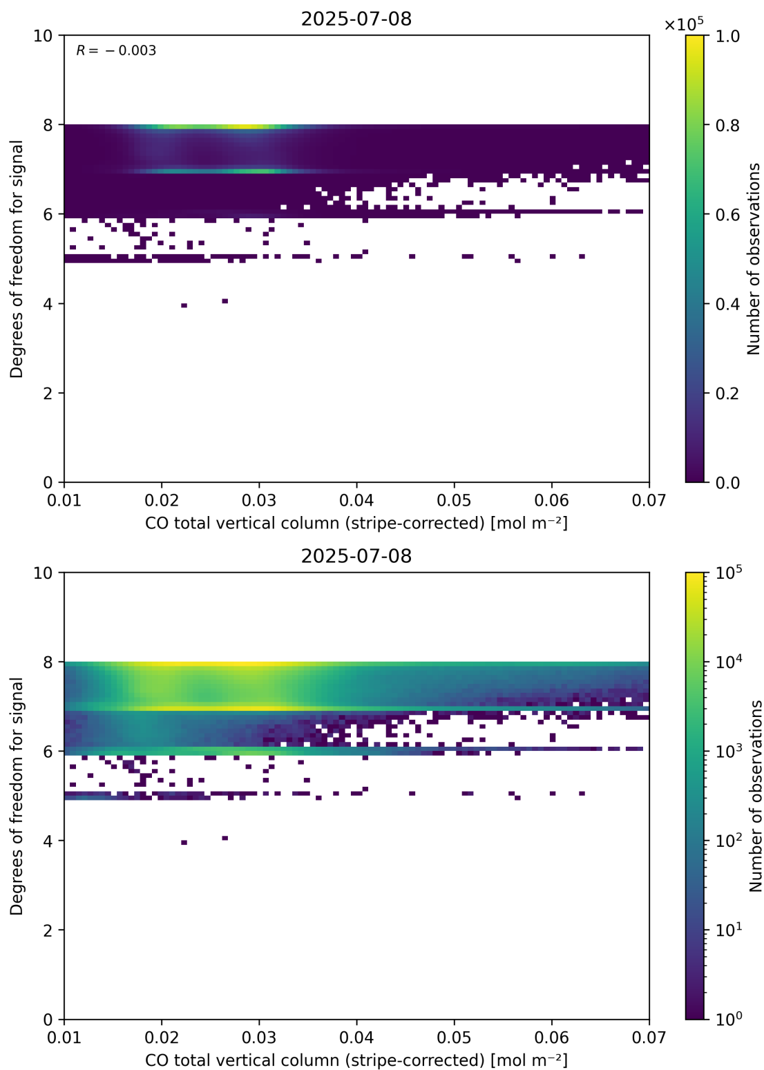
Figure 38: Scatter density plot of “CO total vertical column (stripe-corrected)” against “Degrees of freedom for signal” for 2025-07-08 to 2025-07-09.
