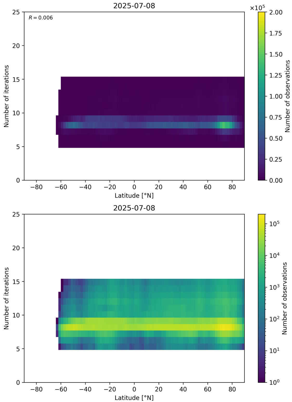
Figure 56: Scatter density plot of “Latitude” against “Number of iterations” for 2025-07-08 to 2025-07-09.
