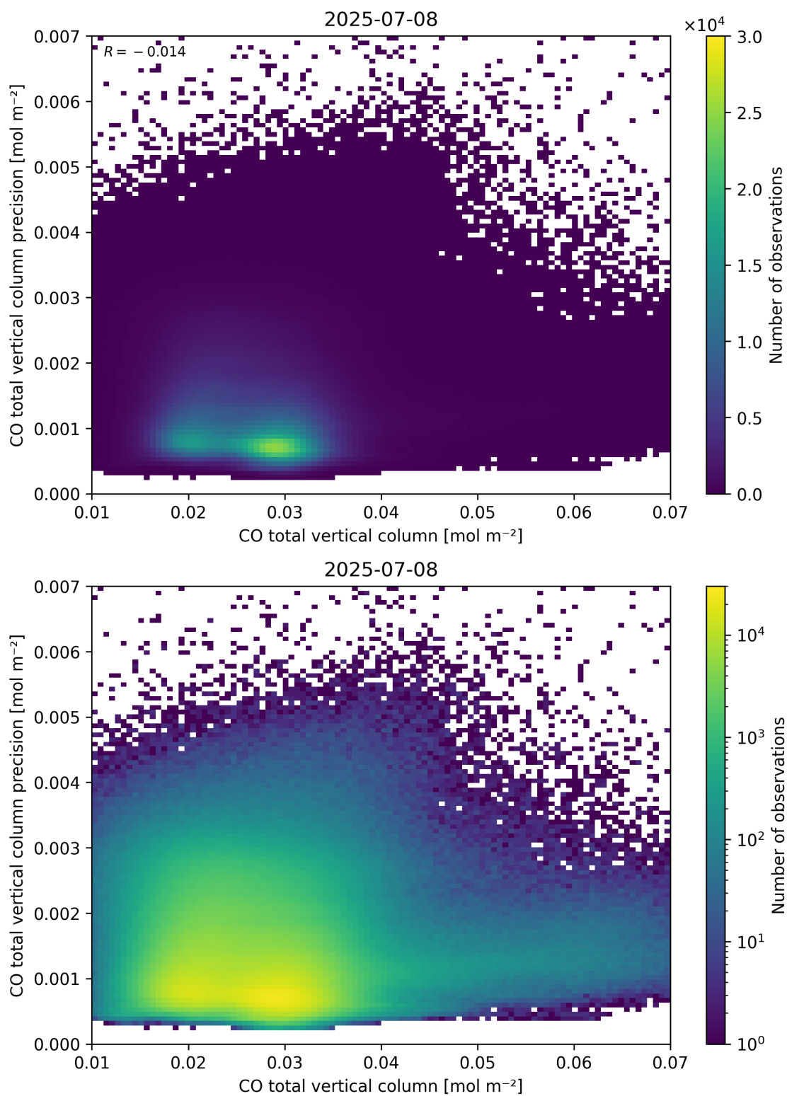
Figure 34: Scatter density plot of “CO total vertical column” against “CO total vertical column precision” for 2025-07-08 to 2025-07-09.
