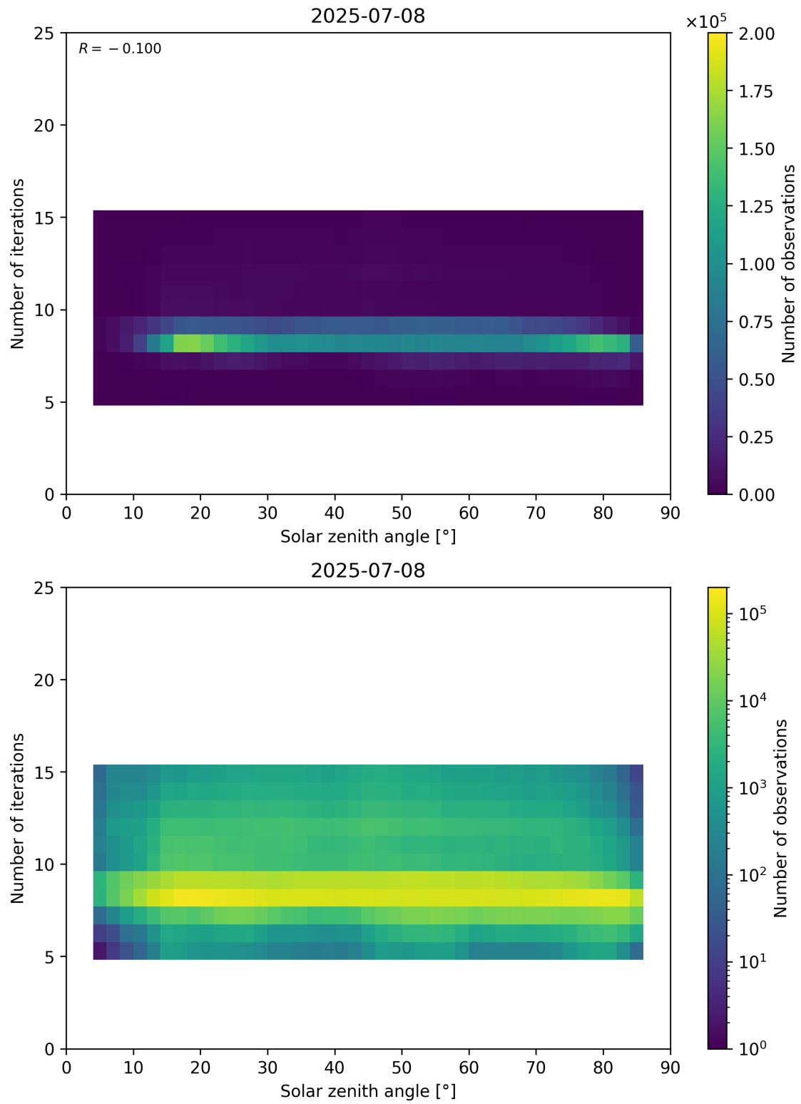
Figure 67: Scatter density plot of “Solar zenith angle” against “Number of iterations” for 2025-07-08 to 2025-07-09.
