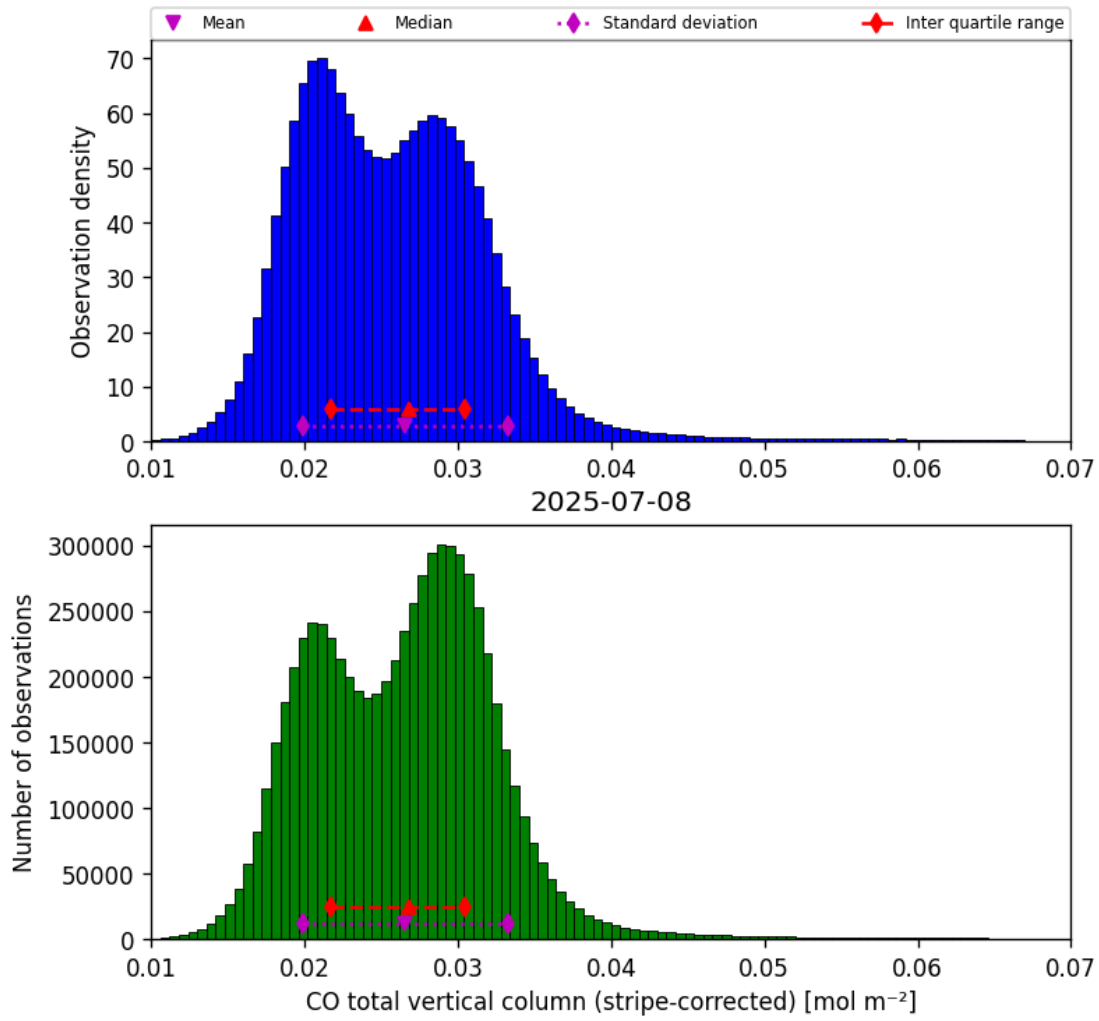
Figure 19: Histogram of “CO total vertical column (stripe-corrected)” for 2025-07-08 to 2025-07-09
