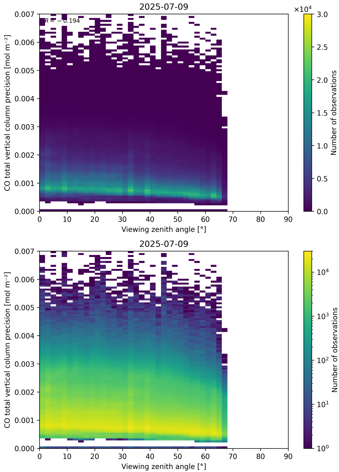
Figure 71: Scatter density plot of “Viewing zenith angle” against “CO total vertical column precision” for 2025-07-08 to 2025-07-10.
