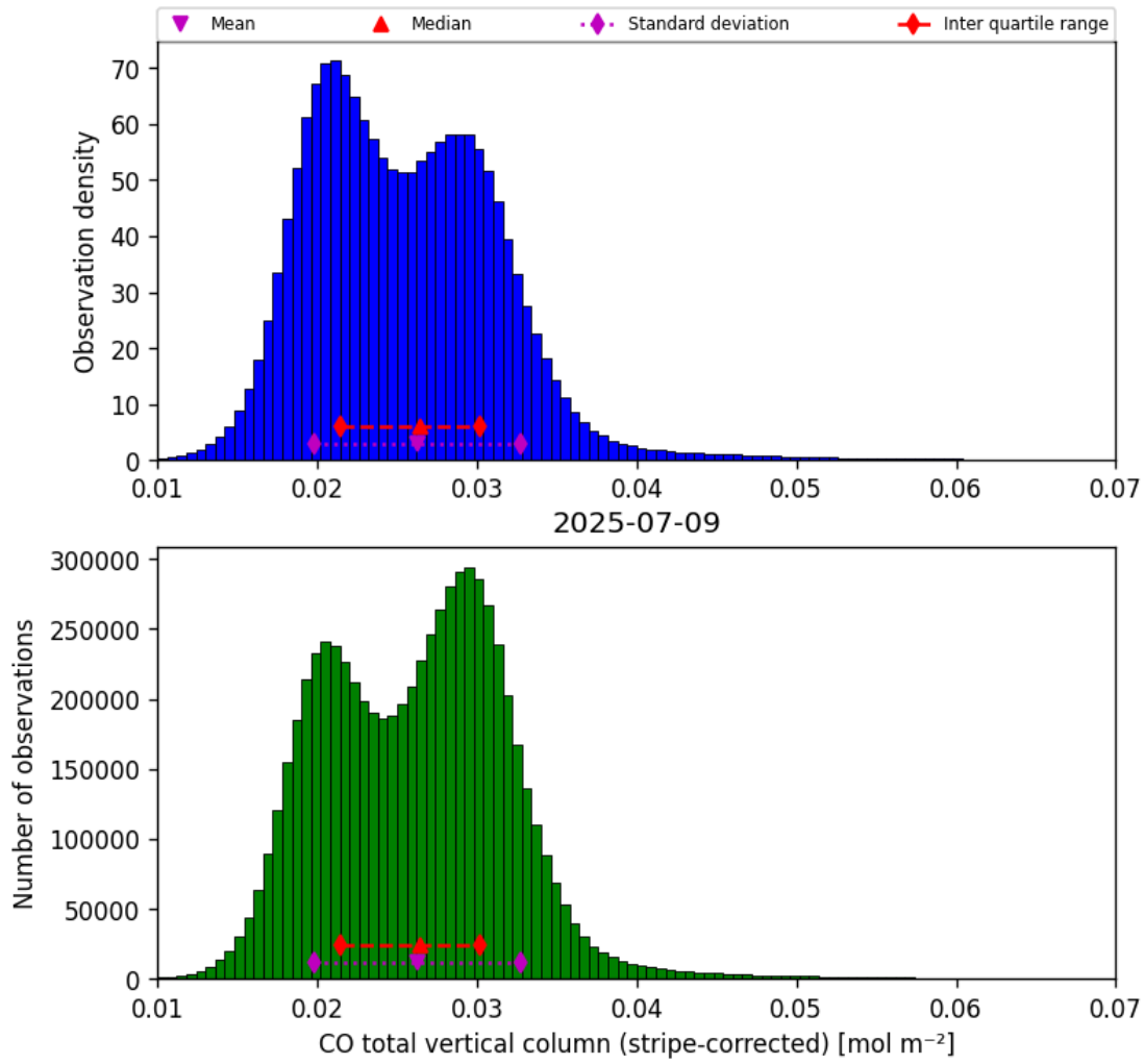
Figure 19: Histogram of “CO total vertical column (stripe-corrected)” for 2025-07-08 to 2025-07-10
