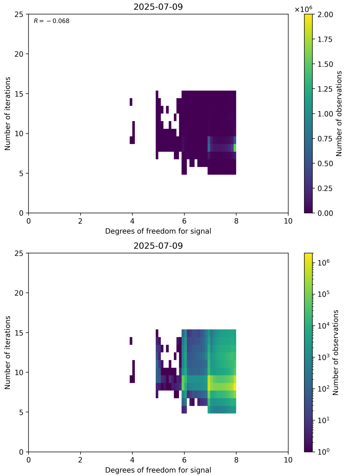
Figure 50: Scatter density plot of “Degrees of freedom for signal” against “Number of iterations” for 2025-07-08 to 2025-07-10.
