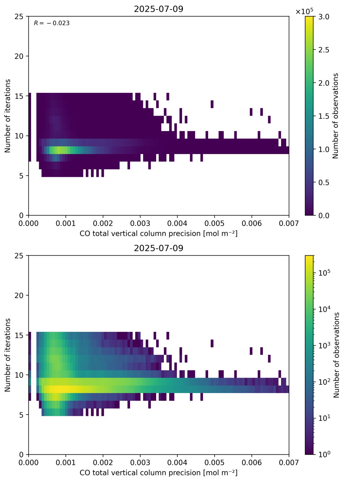
Figure 46: Scatter density plot of “CO total vertical column precision” against “Number of iterations” for 2025-07-08 to 2025-07-10.
