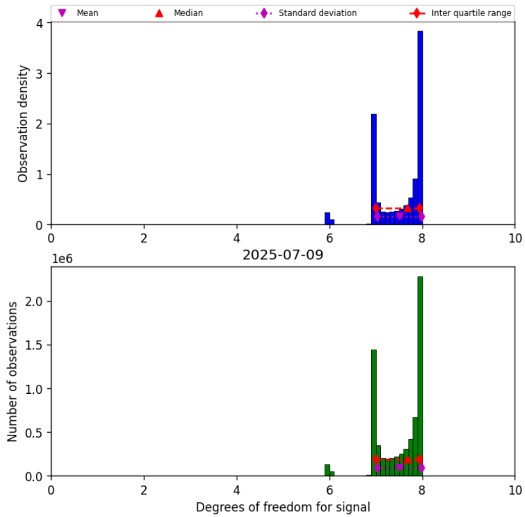
Figure 23: Histogram of “Degrees of freedom for signal” for 2025-07-08 to 2025-07-10
