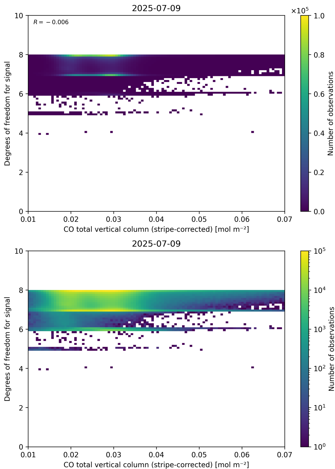
Figure 38: Scatter density plot of “CO total vertical column (stripe-corrected)” against “Degrees of freedom for signal” for 2025-07-08 to 2025-07-10.
