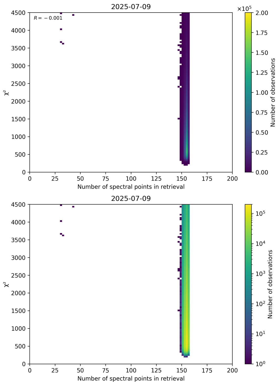
Figure 58: Scatter density plot of “Number of spectral points in retrieval” against “ \chi^2 ” for 2025-07-08 to 2025-07-10.
