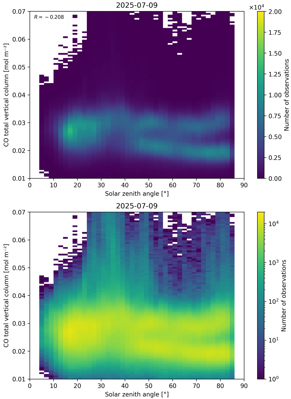
Figure 61: Scatter density plot of “Solar zenith angle” against “CO total vertical column” for 2025-07-08 to 2025-07-10.
