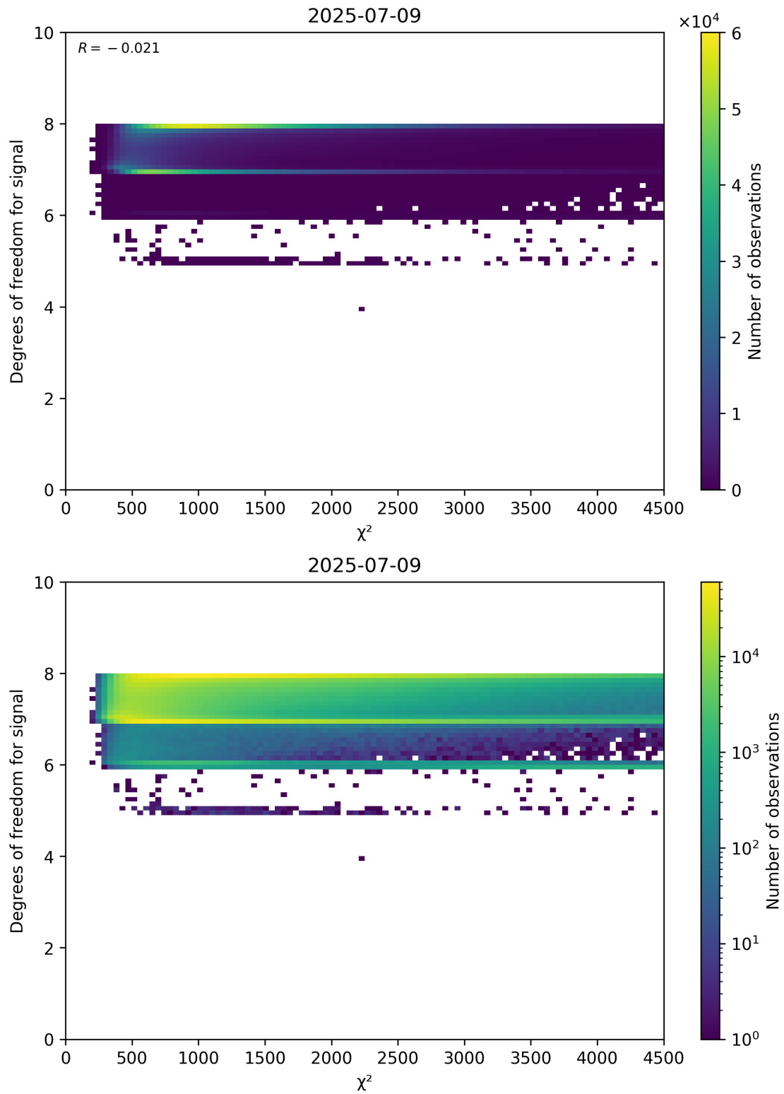
Figure 48: Scatter density plot of “ \chi^2 ” against “Degrees of freedom for signal” for 2025-07-08 to 2025-07-10.
