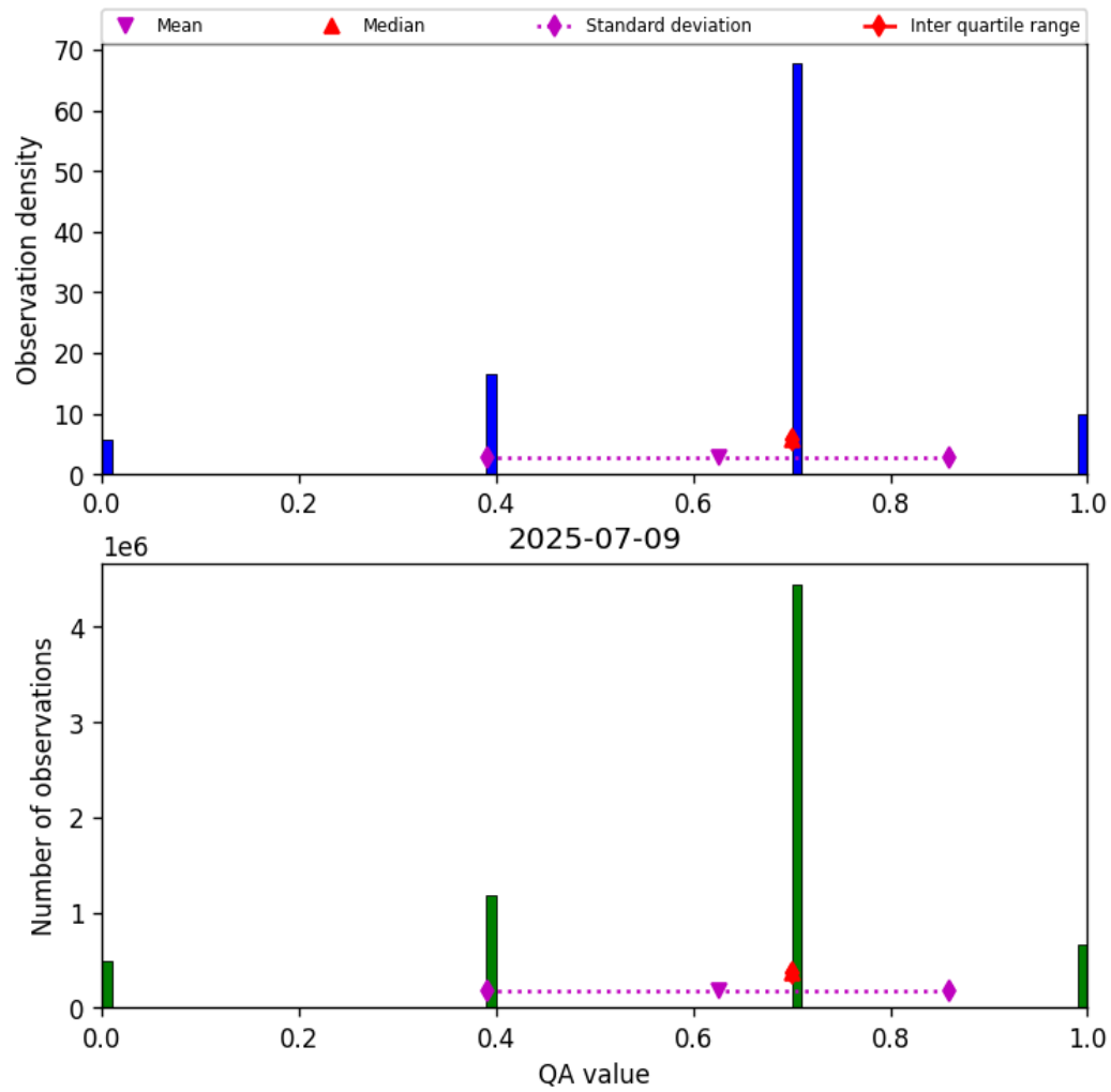
Figure 17: Histogram of “QA value” for 2025-07-08 to 2025-07-10
