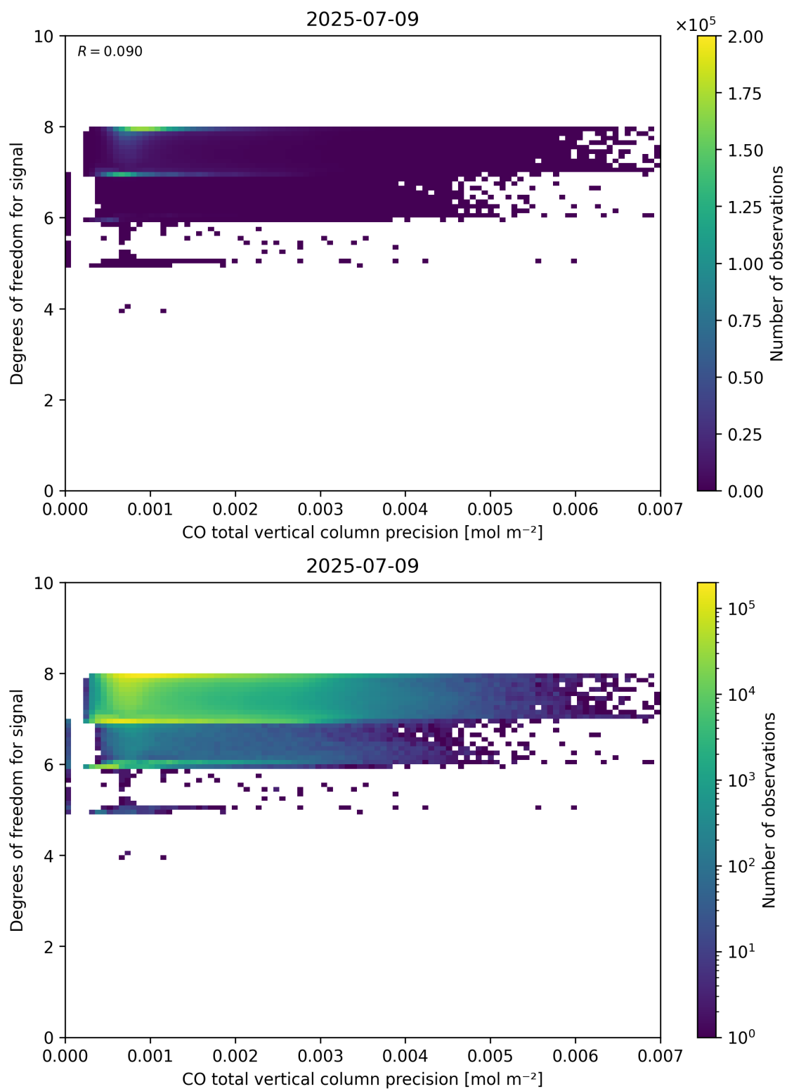
Figure 45: Scatter density plot of “CO total vertical column precision” against “Degrees of freedom for signal” for 2025-07-08 to 2025-07-10.
