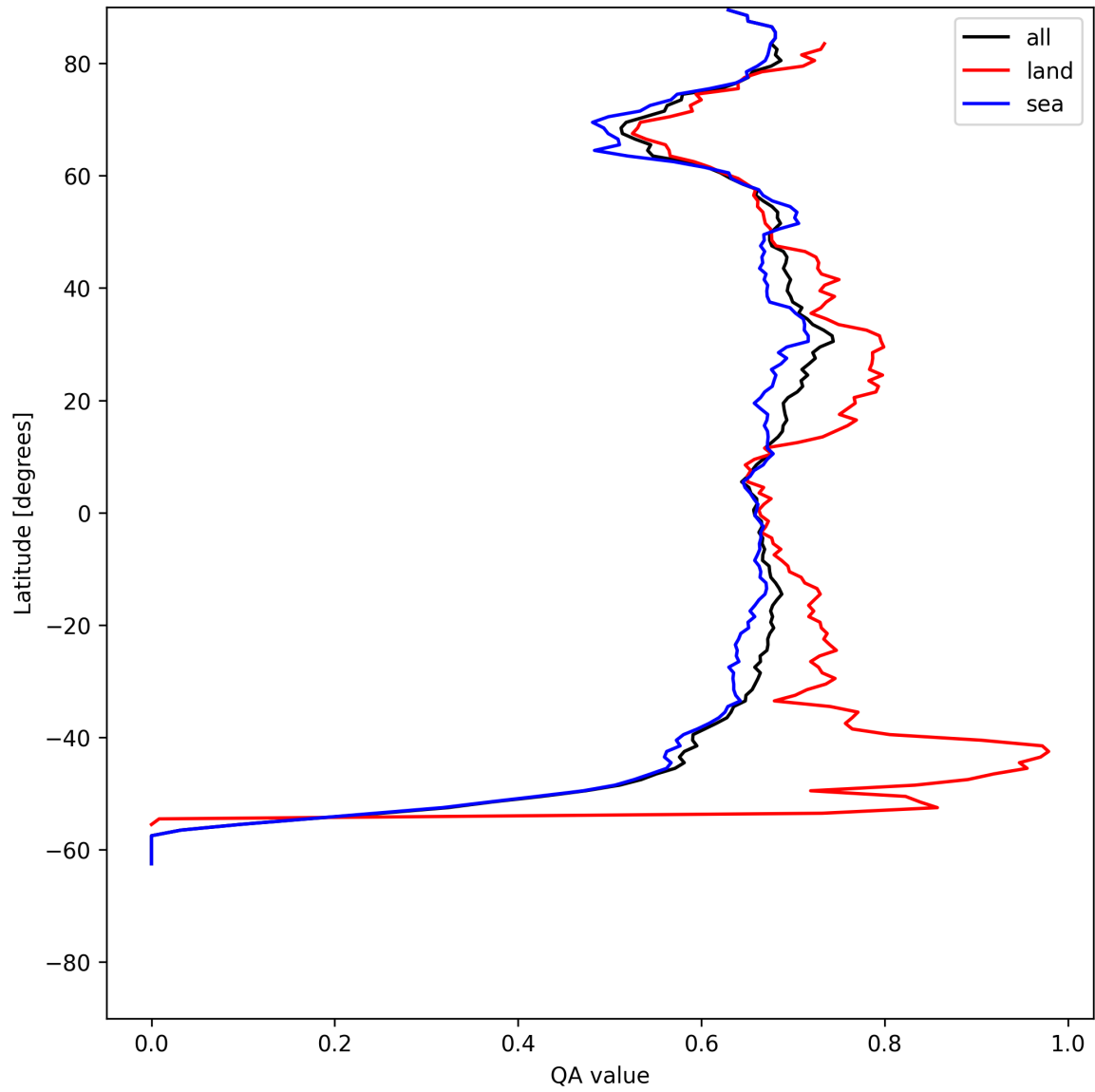
Figure 9: Zonal average of “QA value” for 2025-07-08 to 2025-07-10.
