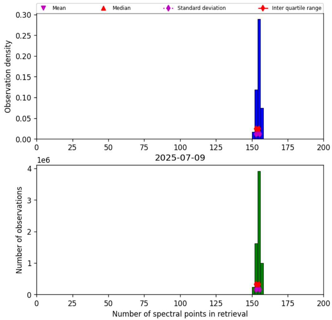
Figure 21: Histogram of “Number of spectral points in retrieval” for 2025-07-08 to 2025-07-10
