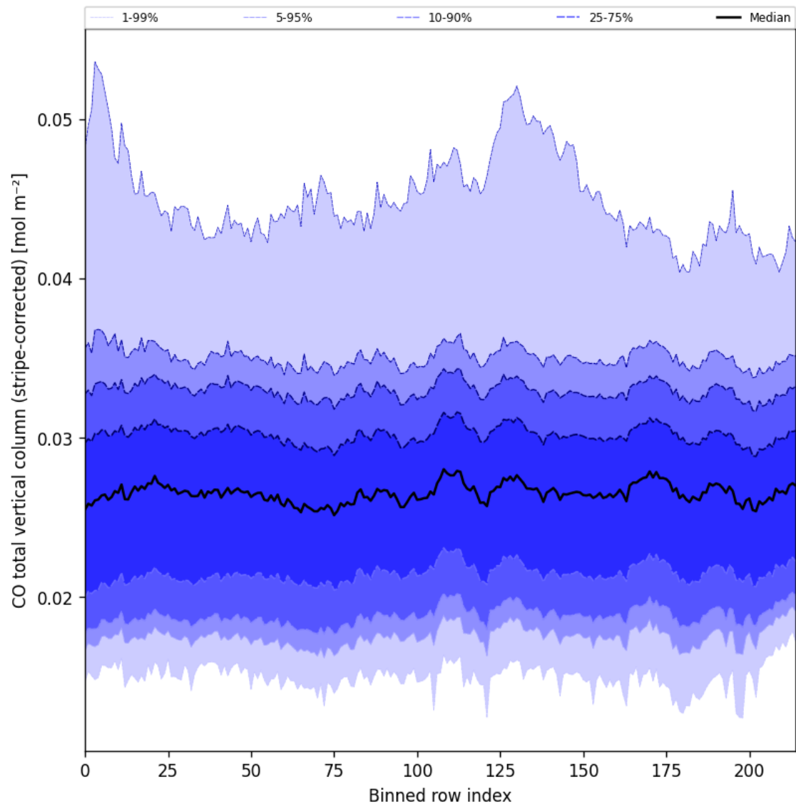
Figure 27: Along track statistics of “CO total vertical column (stripe-corrected)” for 2025-07-08 to 2025-07-10
