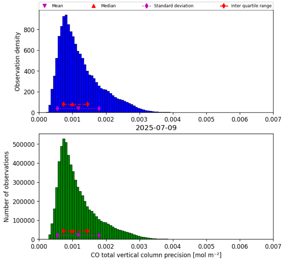
Figure 20: Histogram of “CO total vertical column precision” for 2025-07-08 to 2025-07-10
