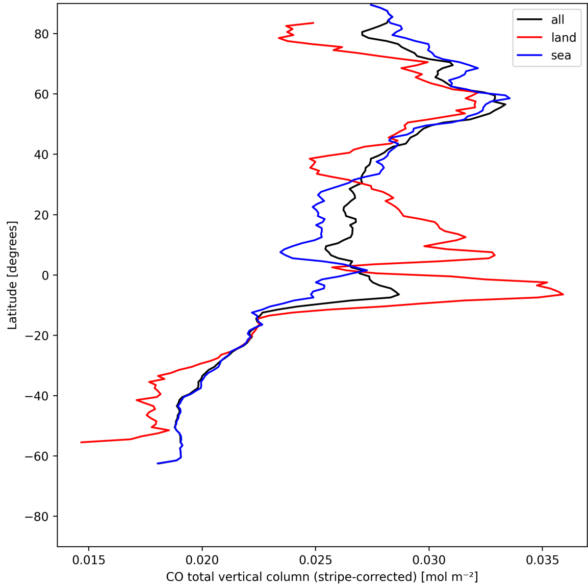
Figure 11: Zonal average of “CO total vertical column (stripe-corrected)” for 2025-07-08 to 2025-07-10.
