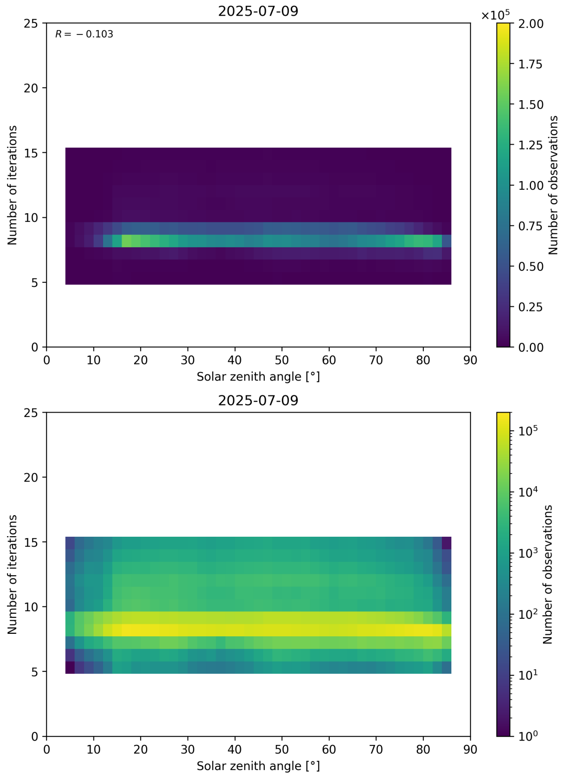
Figure 67: Scatter density plot of “Solar zenith angle” against “Number of iterations” for 2025-07-08 to 2025-07-10.
