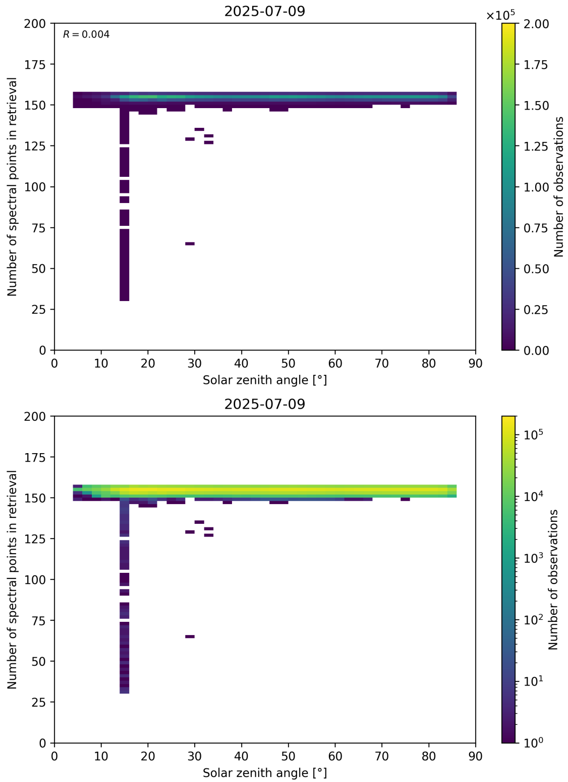
Figure 68: Scatter density plot of “Solar zenith angle” against “Number of spectral points in retrieval” for 2025-07-08 to 2025-07-10.
