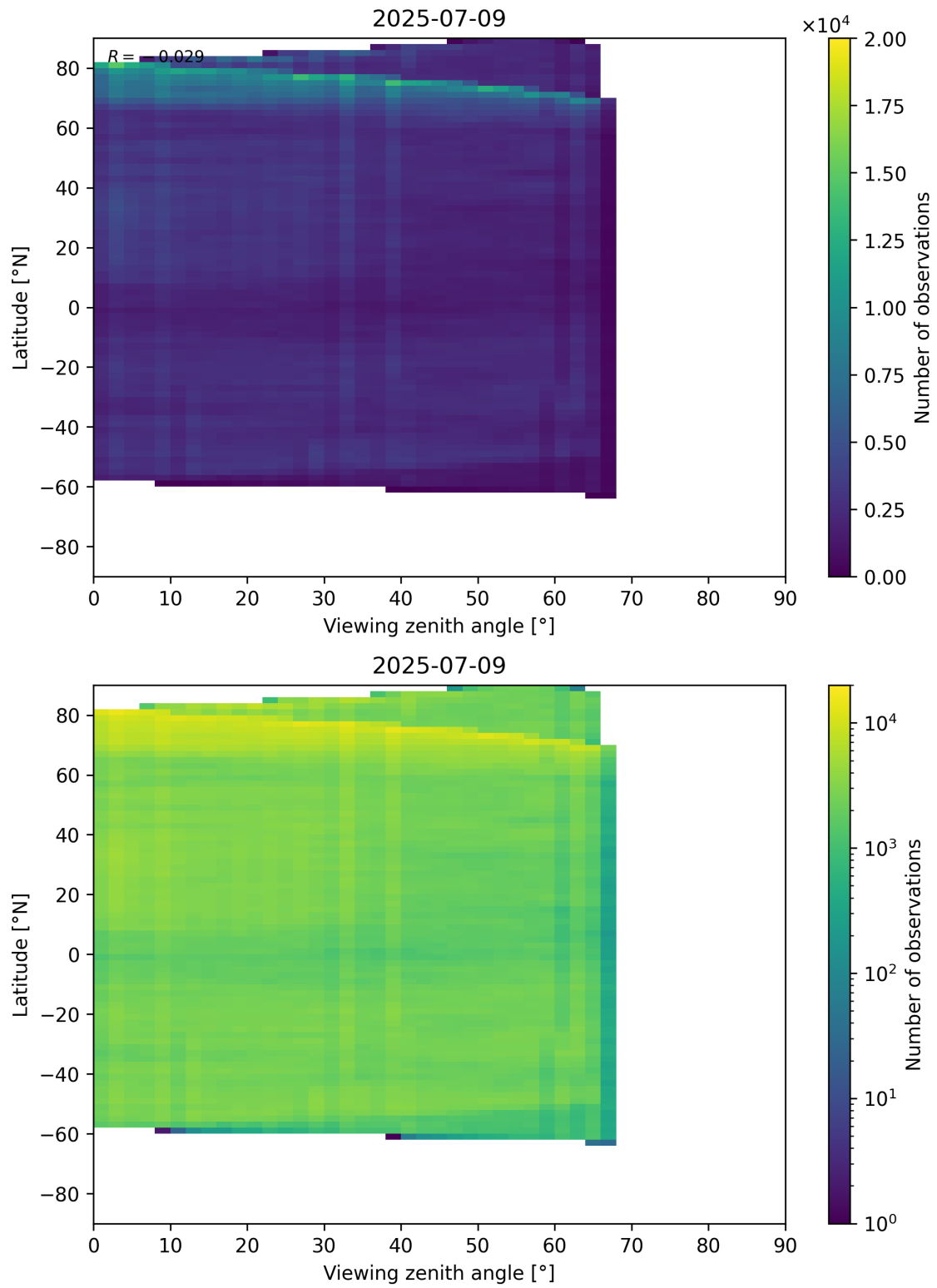
Figure 74: Scatter density plot of “Viewing zenith angle” against “Latitude” for 2025-07-08 to 2025-07-10.
