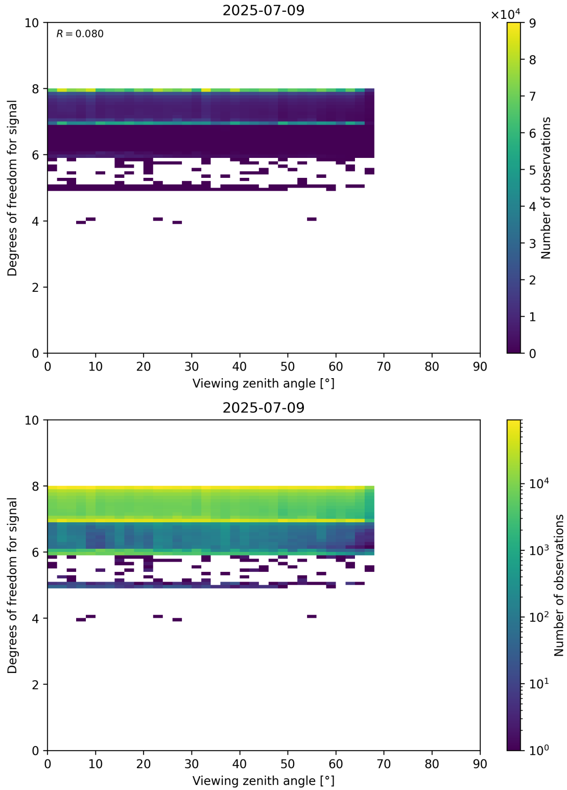
Figure 73: Scatter density plot of “Viewing zenith angle” against “Degrees of freedom for signal” for 2025-07-08 to 2025-07-10.
