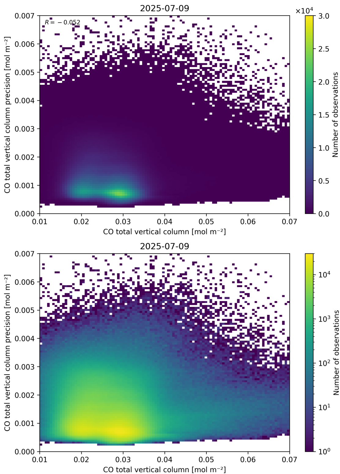
Figure 34: Scatter density plot of “CO total vertical column” against “CO total vertical column precision” for 2025-07-08 to 2025-07-10.
