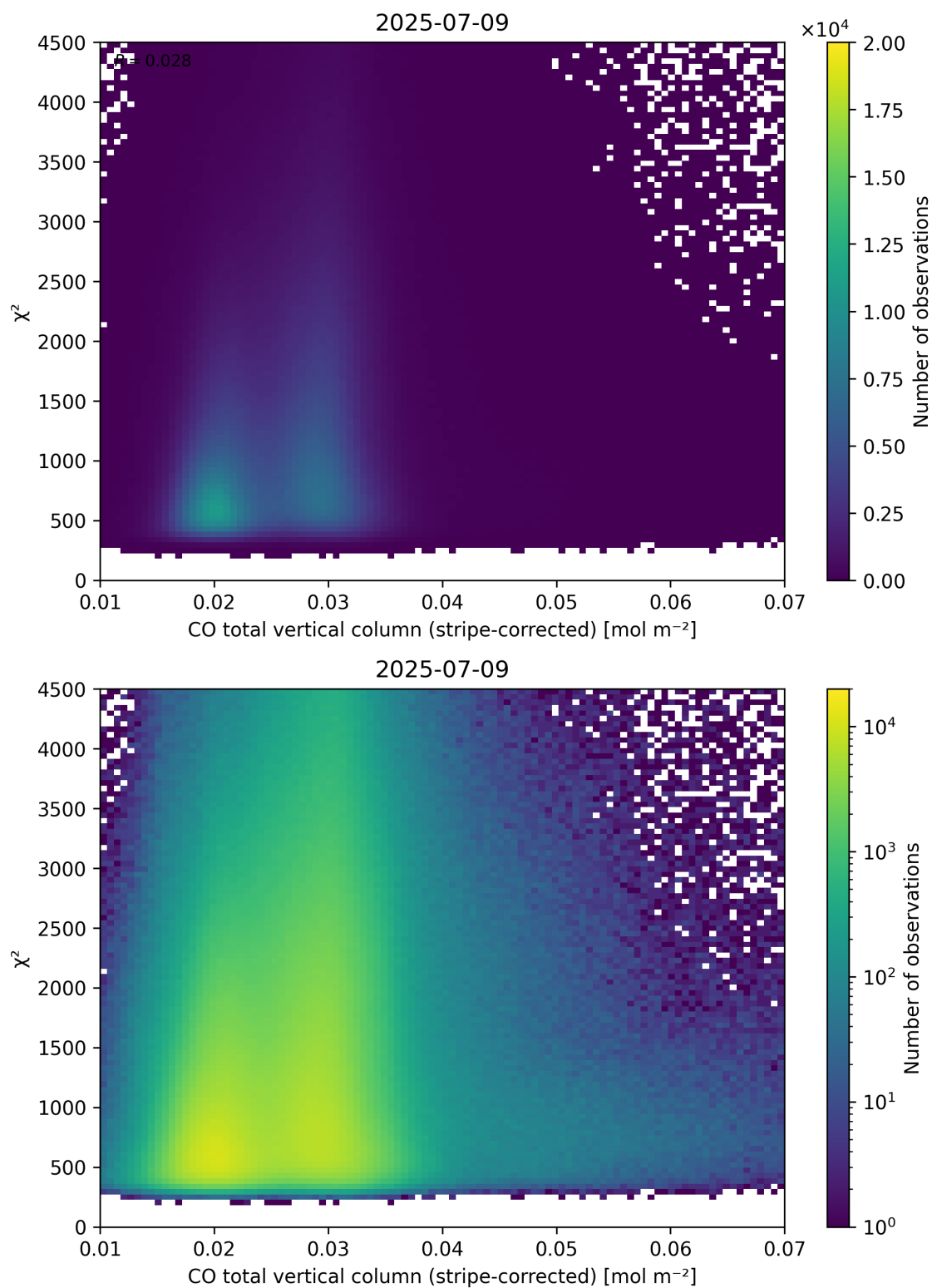
Figure 37: Scatter density plot of “CO total vertical column (stripe-corrected)” against “ \chi^2 ” for 2025-07-08 to 2025-07-10.
