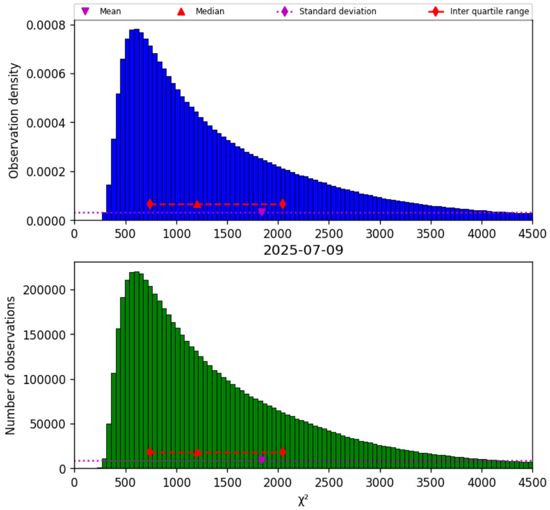
Figure 22: Histogram of " \chi^2 " for 2025-07-08 to 2025-07-10
