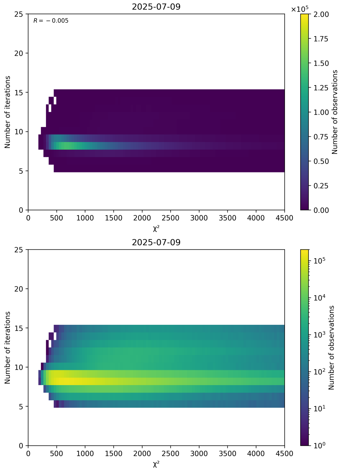
Figure 49: Scatter density plot of “ \chi^2 ” against “Number of iterations” for 2025-07-08 to 2025-07-10.
