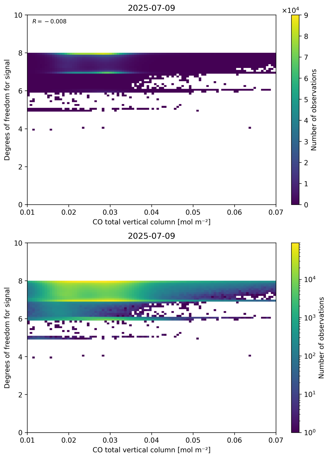
Figure 41: Scatter density plot of “CO total vertical column” against “Degrees of freedom for signal” for 2025-07-08 to 2025-07-10.
