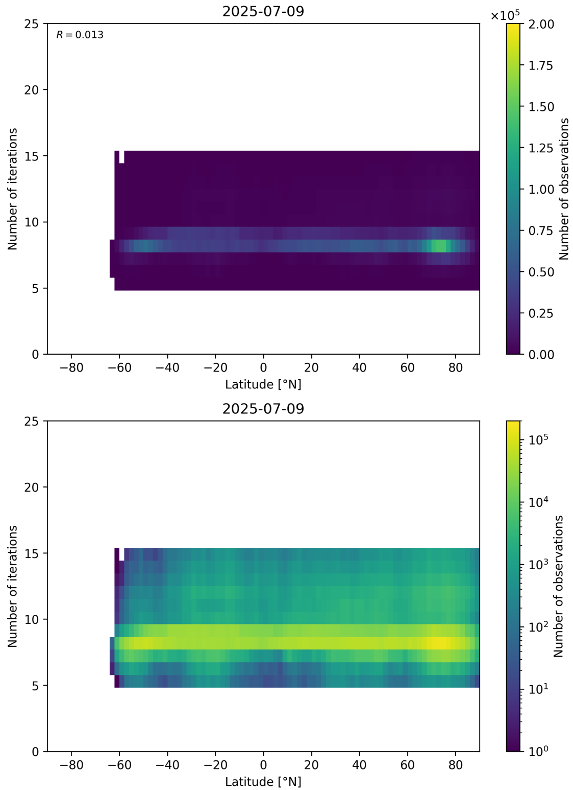
Figure 56: Scatter density plot of “Latitude” against “Number of iterations” for 2025-07-08 to 2025-07-10.
