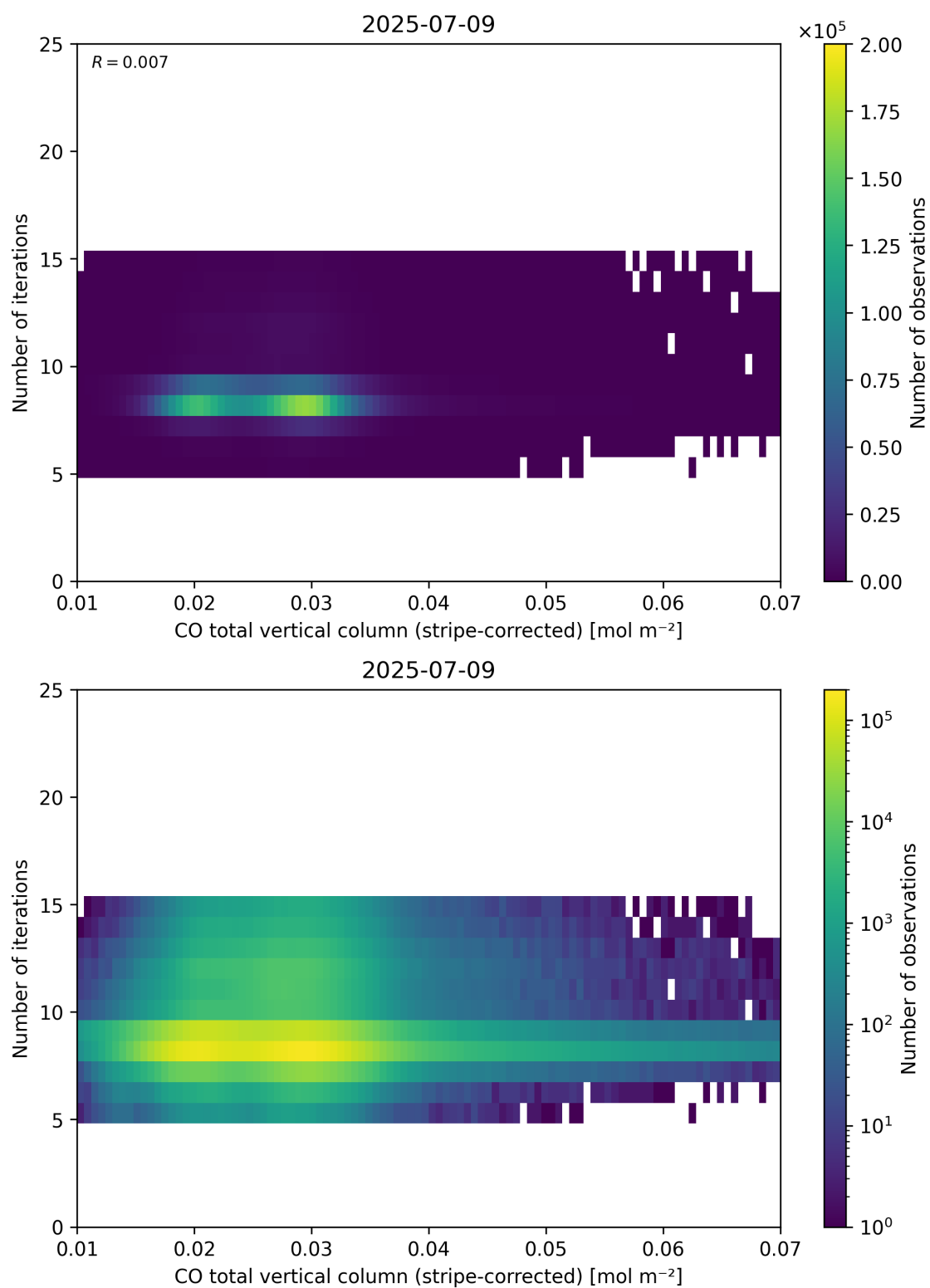
Figure 39: Scatter density plot of “CO total vertical column (stripe-corrected)” against “Number of iterations” for 2025-07-08 to 2025-07-10.
