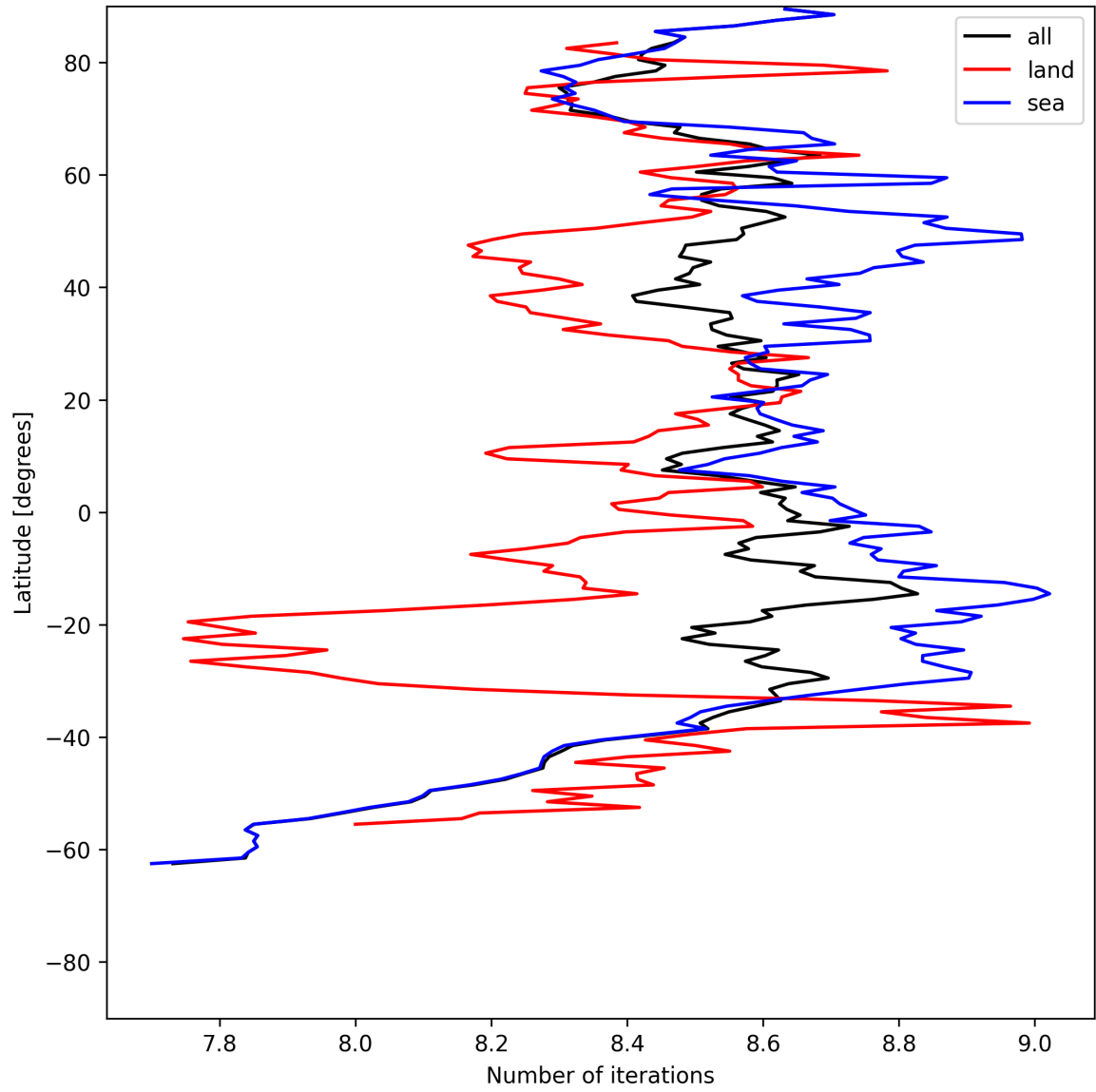
Figure 16: Zonal average of “Number of iterations” for 2025-07-08 to 2025-07-10.
