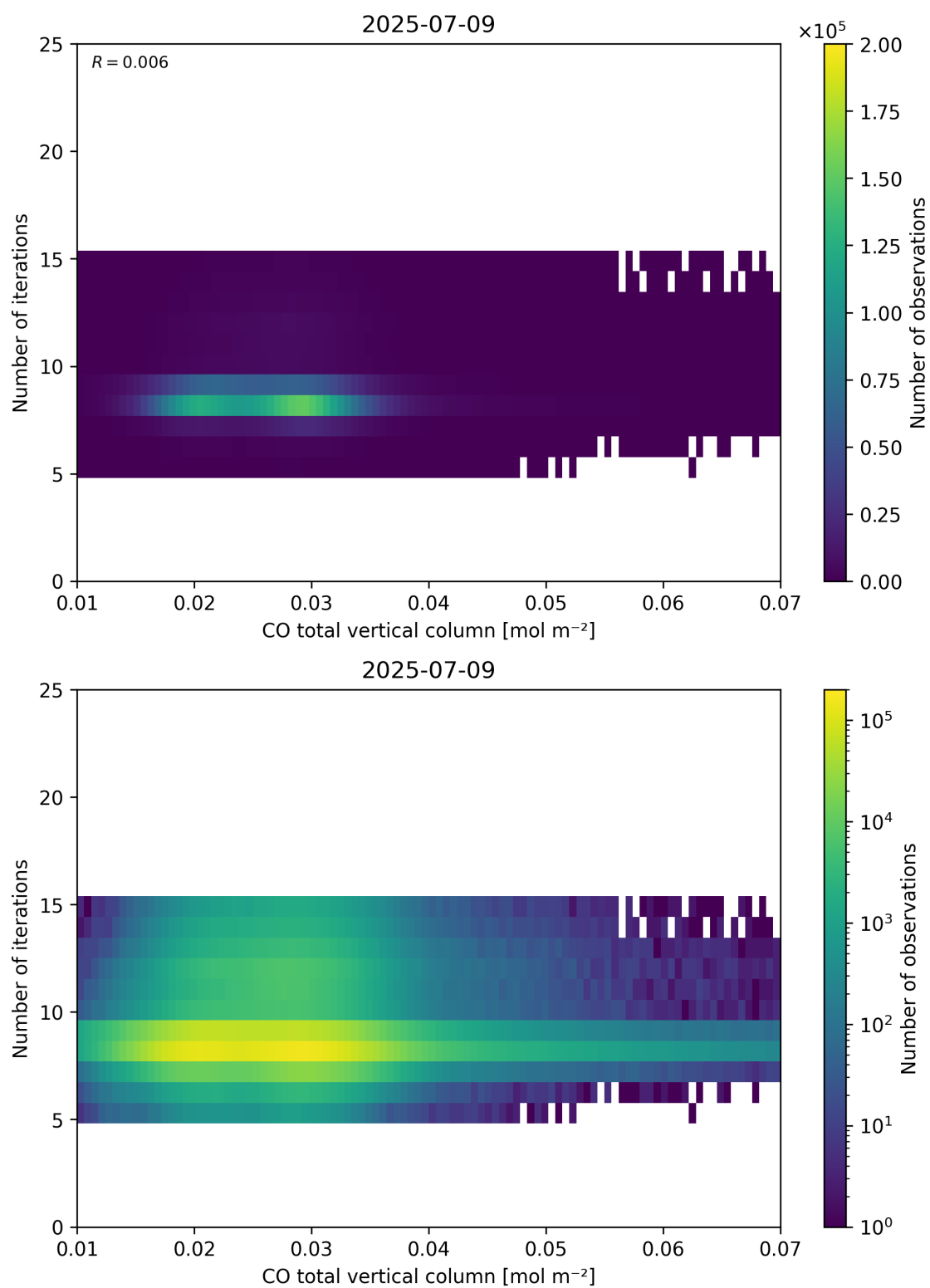
Figure 42: Scatter density plot of “CO total vertical column” against “Number of iterations” for 2025-07-08 to 2025-07-10.
