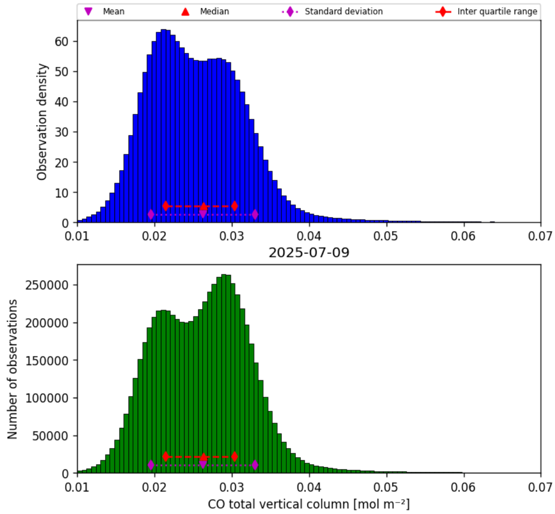
Figure 18: Histogram of “CO total vertical column” for 2025-07-08 to 2025-07-10
