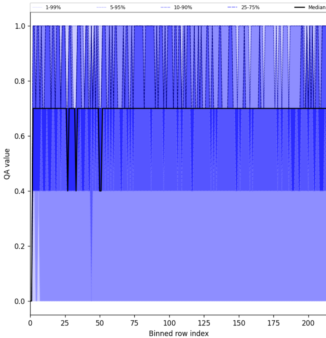
Figure 25: Along track statistics of “QA value” for 2025-07-08 to 2025-07-10
