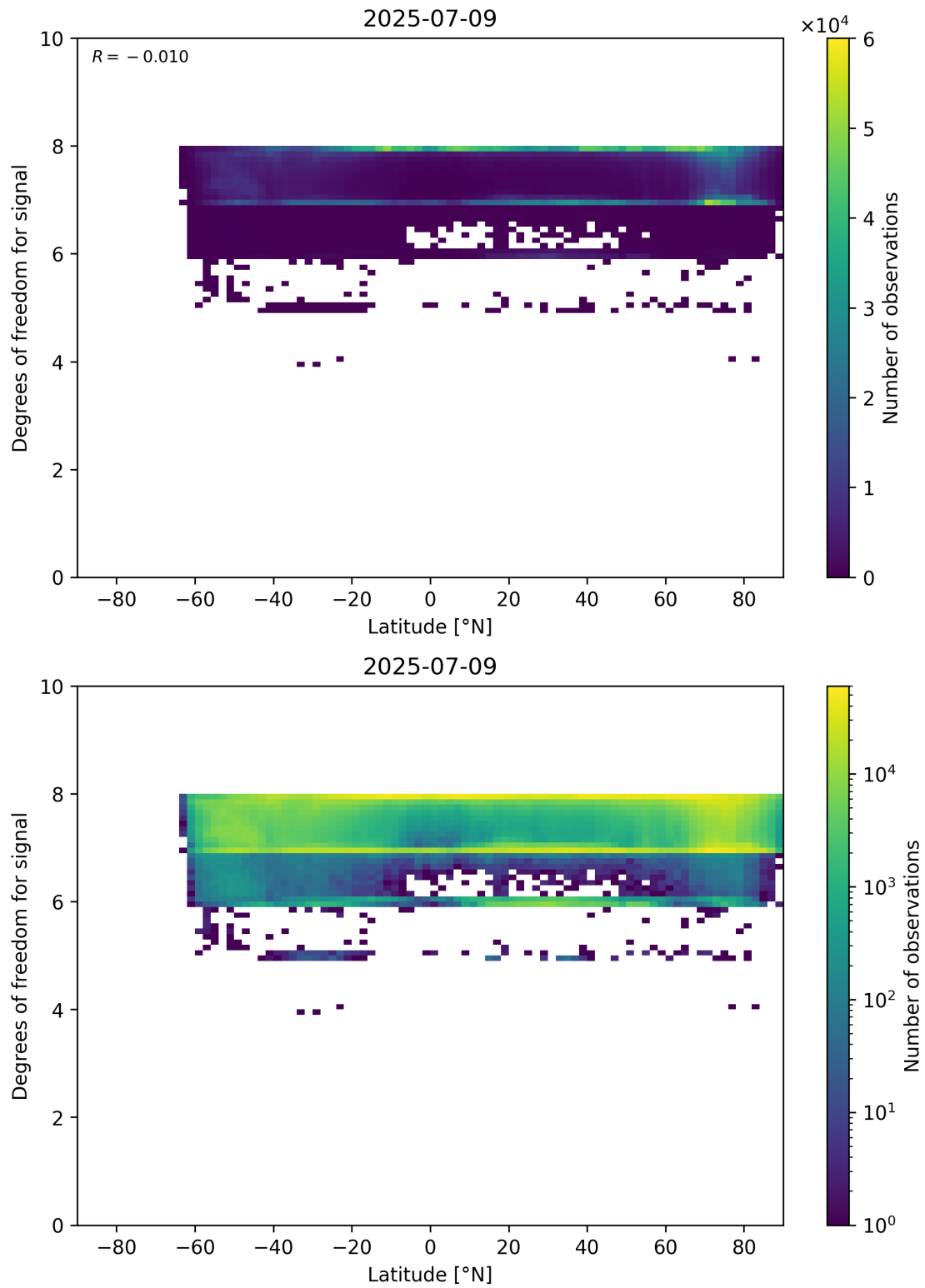
Figure 55: Scatter density plot of “Latitude” against “Degrees of freedom for signal” for 2025-07-08 to 2025-07-10.
