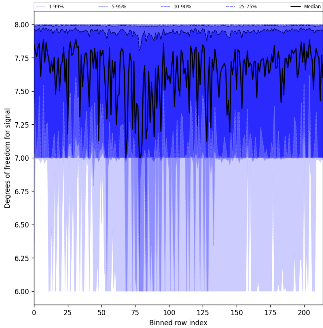
Figure 31: Along track statistics of “Degrees of freedom for signal” for 2025-07-08 to 2025-07-10
