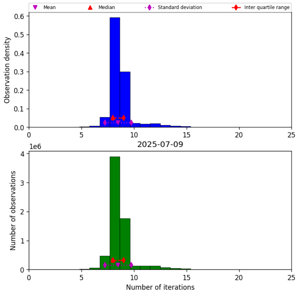
Figure 24: Histogram of “Number of iterations” for 2025-07-08 to 2025-07-10
