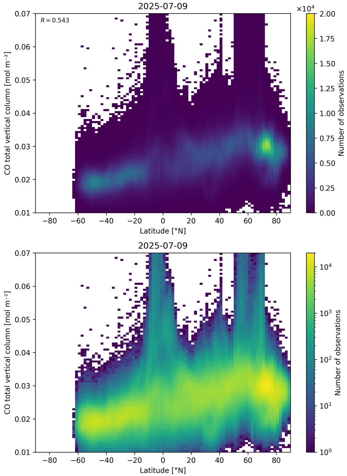
Figure 51: Scatter density plot of “Latitude” against “CO total vertical column” for 2025-07-08 to 2025-07-10.
