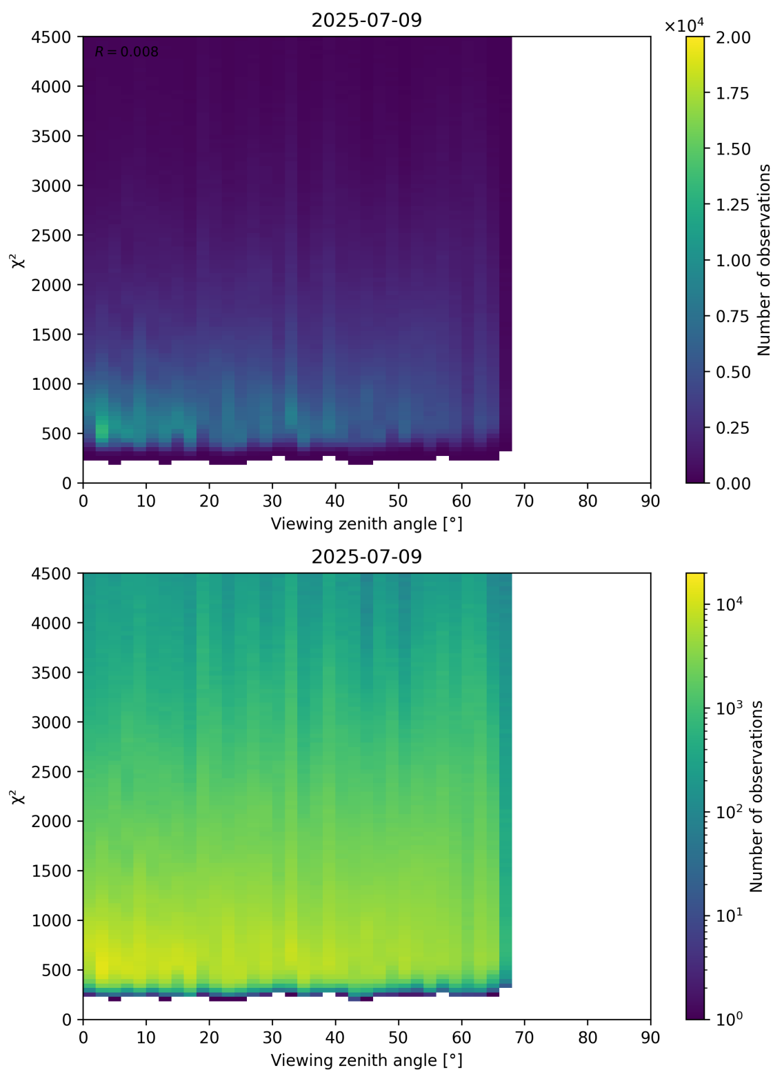
Figure 72: Scatter density plot of “Viewing zenith angle” against “ \chi^2 ” for 2025-07-08 to 2025-07-10.
