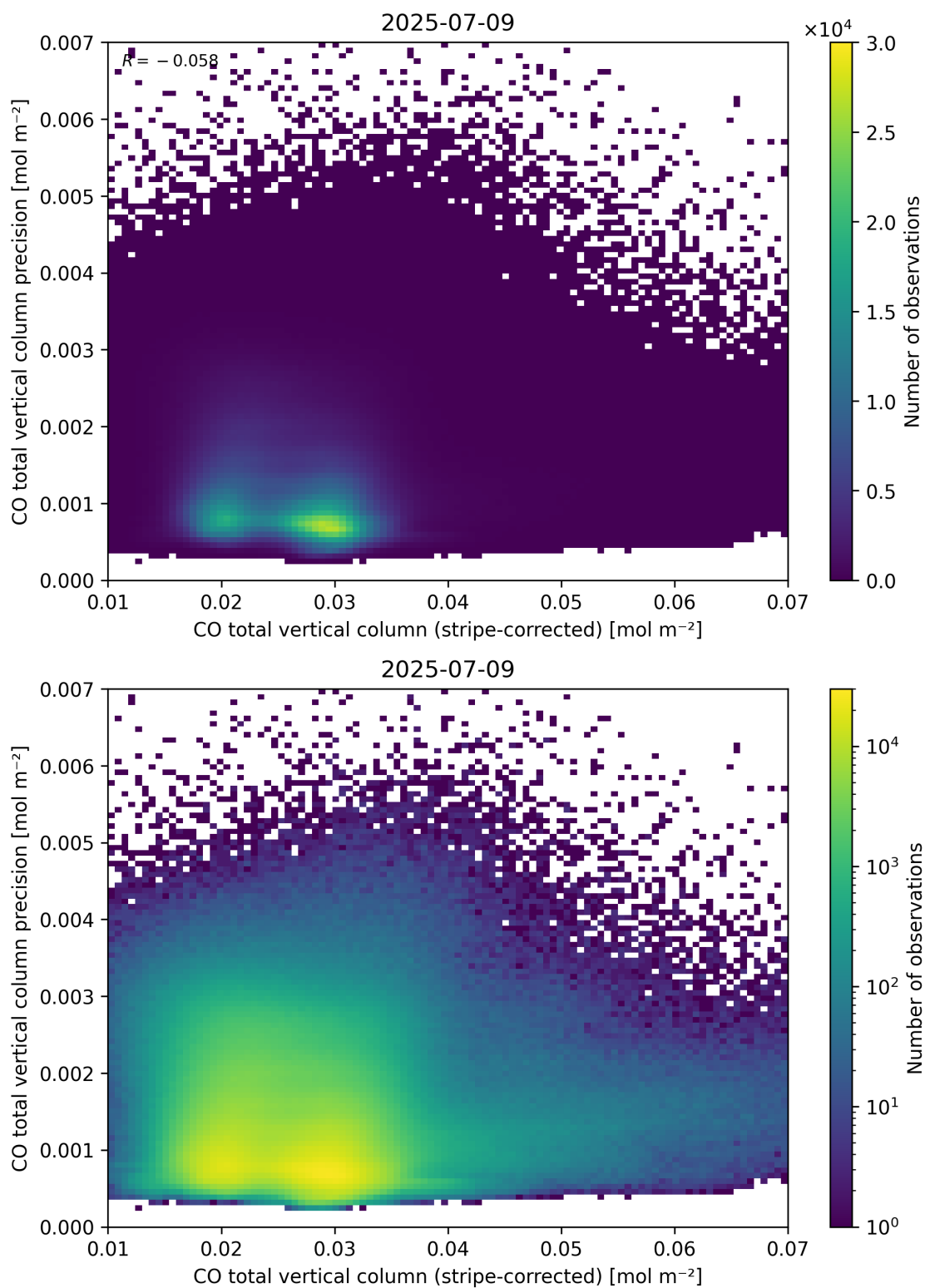
Figure 36: Scatter density plot of “CO total vertical column (stripe-corrected)” against “CO total vertical column precision” for 2025-07-08 to 2025-07-10.
