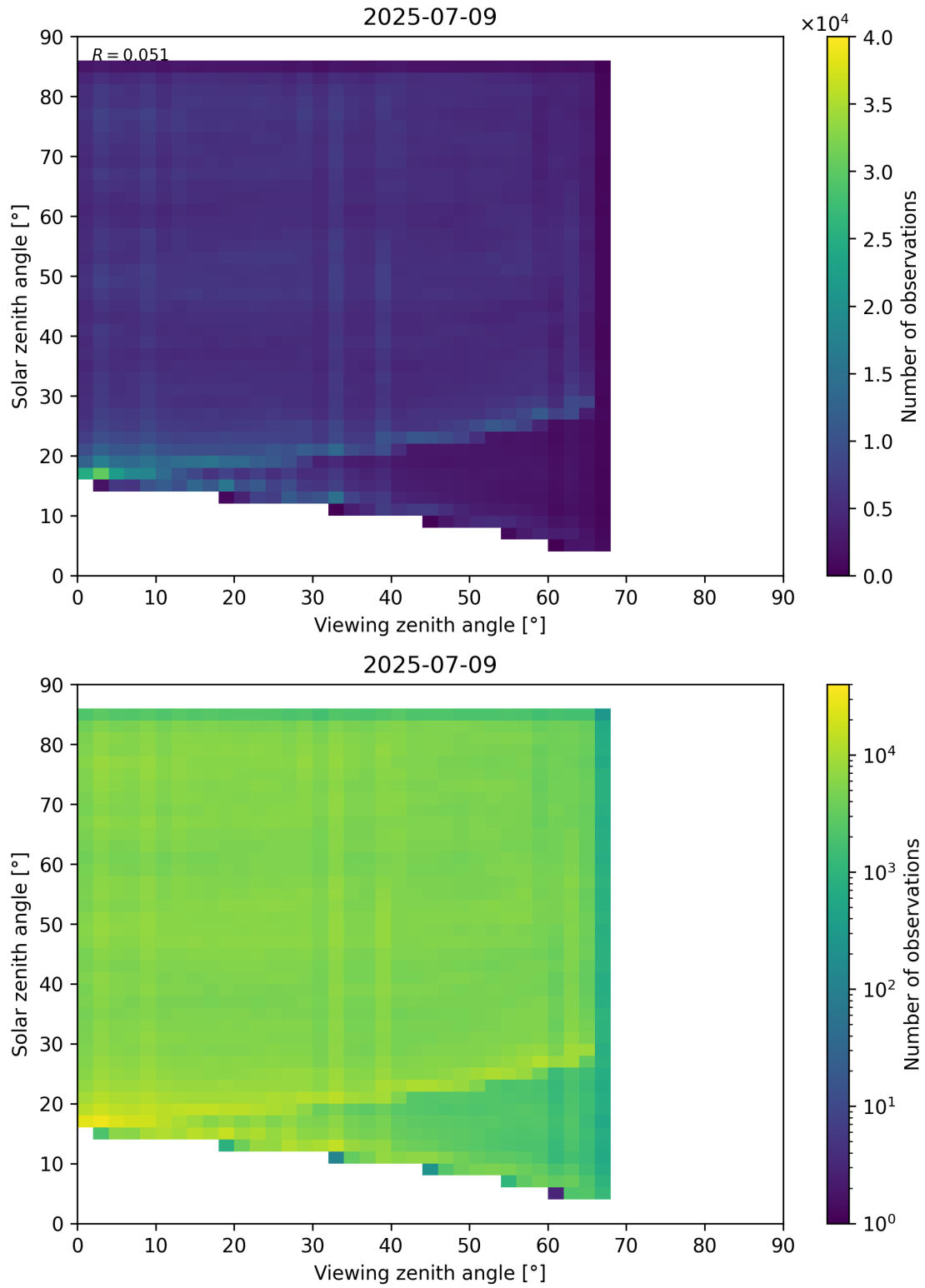
Figure 77: Scatter density plot of “Viewing zenith angle” against “Solar zenith angle” for 2025-07-08 to 2025-07-10.
