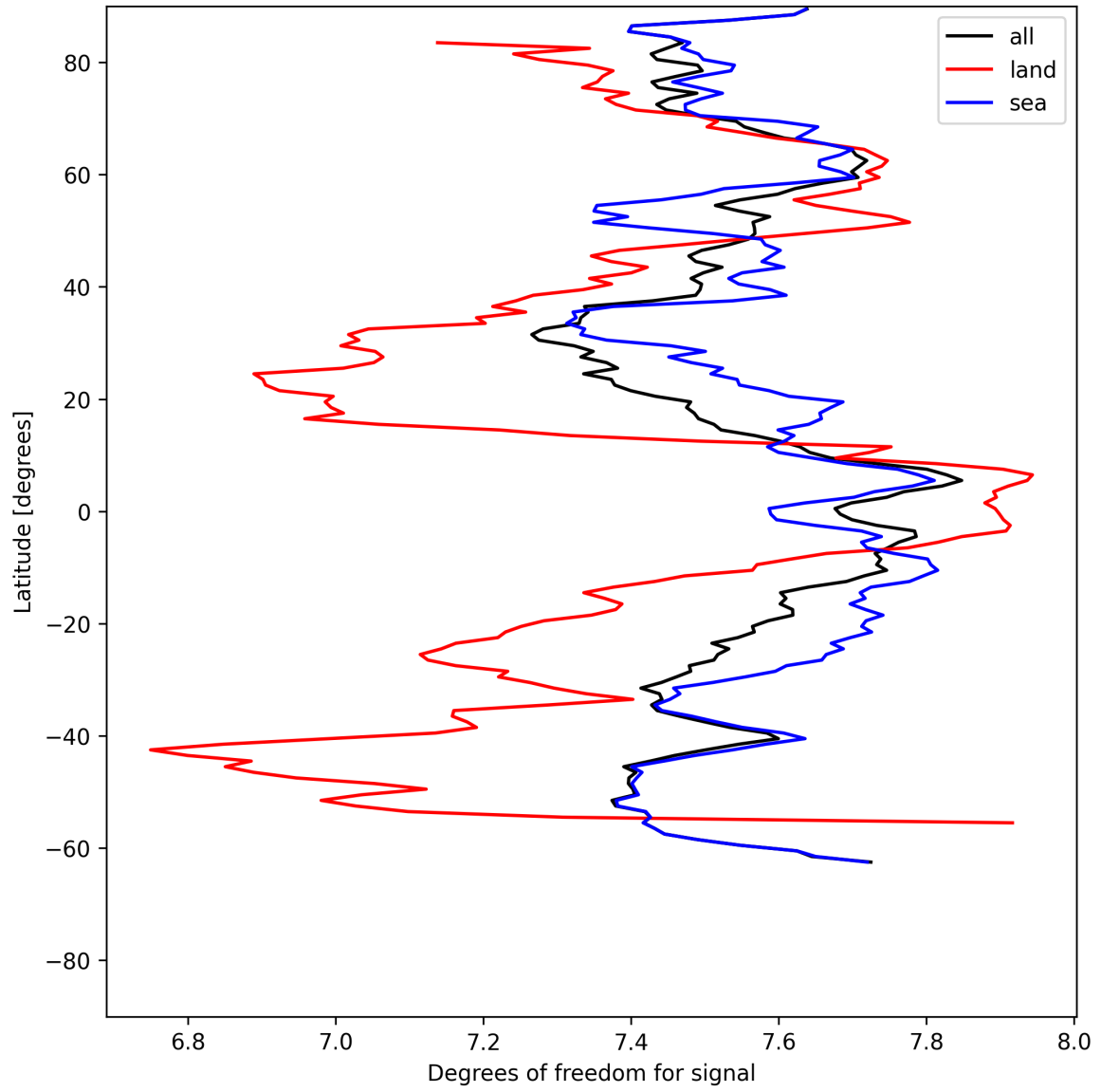
Figure 15: Zonal average of “Degrees of freedom for signal” for 2025-07-08 to 2025-07-10.
