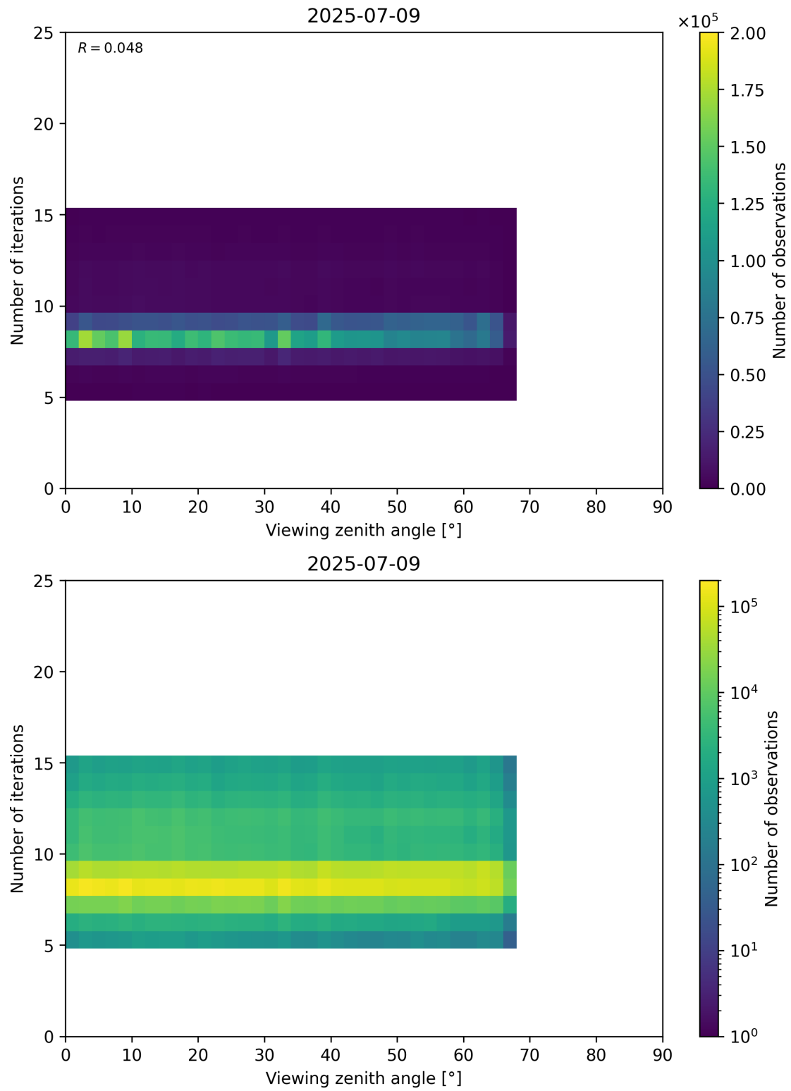
Figure 75: Scatter density plot of “Viewing zenith angle” against “Number of iterations” for 2025-07-08 to 2025-07-10.
