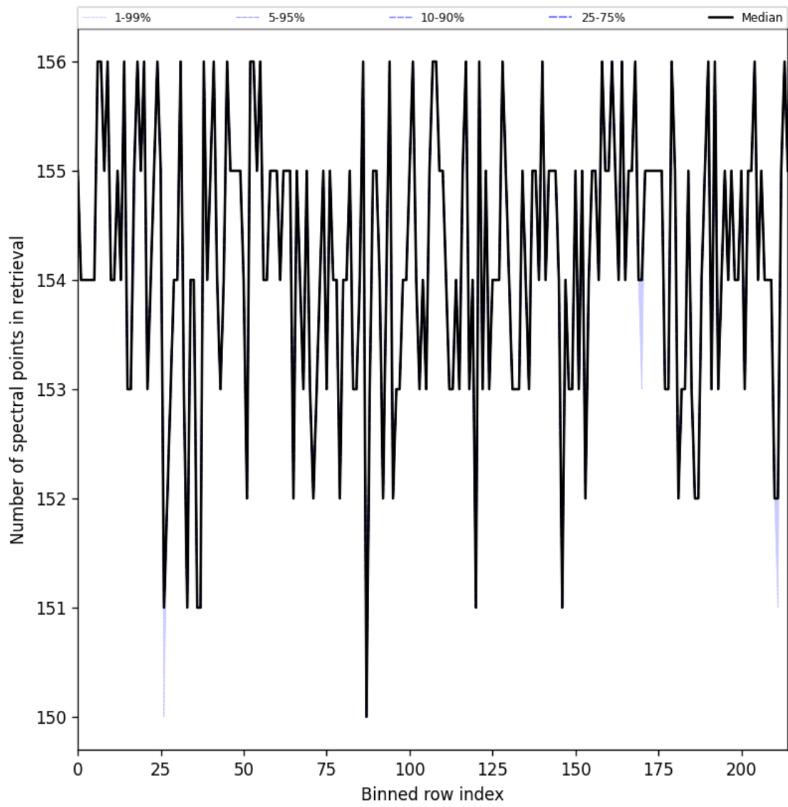
Figure 29: Along track statistics of “Number of spectral points in retrieval” for 2025-07-08 to 2025-07-10
