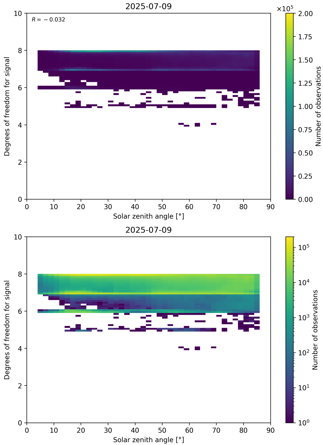
Figure 65: Scatter density plot of “Solar zenith angle” against “Degrees of freedom for signal” for 2025-07-08 to 2025-07-10.
