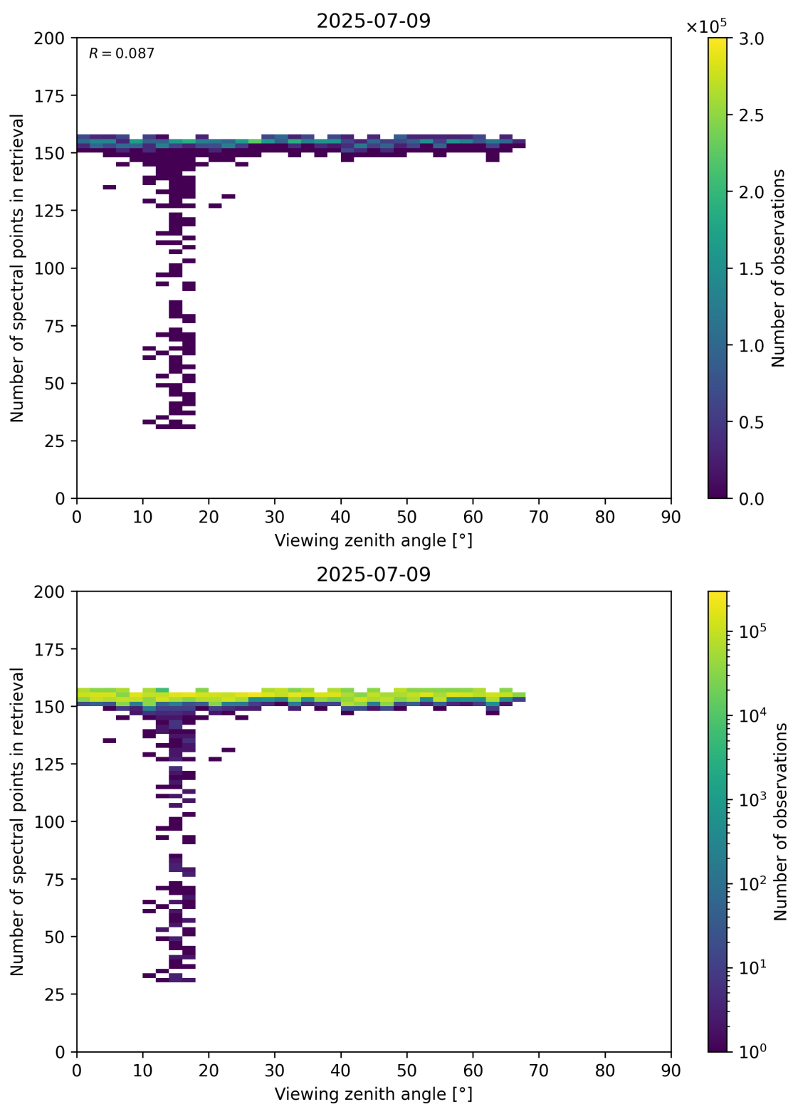
Figure 76: Scatter density plot of “Viewing zenith angle” against “Number of spectral points in retrieval” for 2025-07-08 to 2025-07-10.
