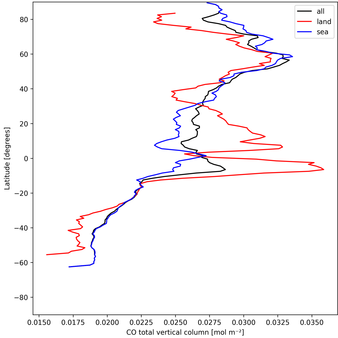
Figure 10: Zonal average of “CO total vertical column” for 2025-07-08 to 2025-07-10.
