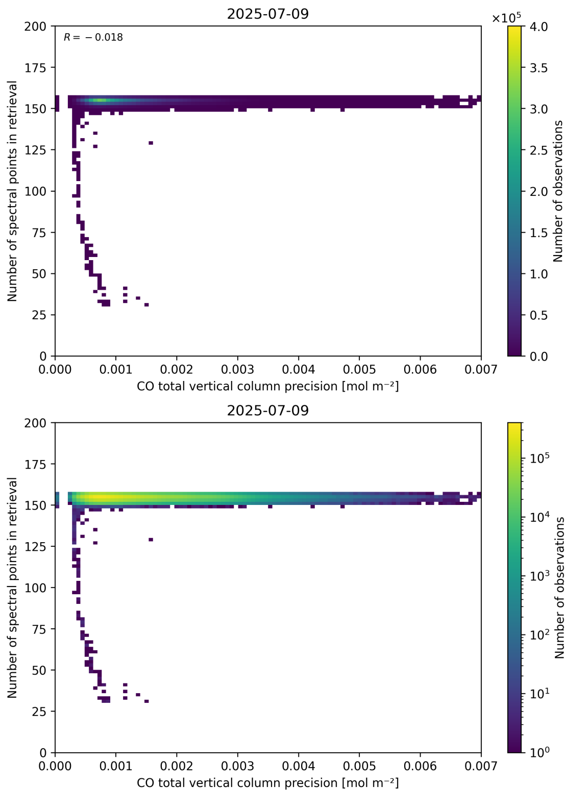
Figure 47: Scatter density plot of “CO total vertical column precision” against “Number of spectral points in retrieval” for 2025-07-08 to 2025-07-10.
