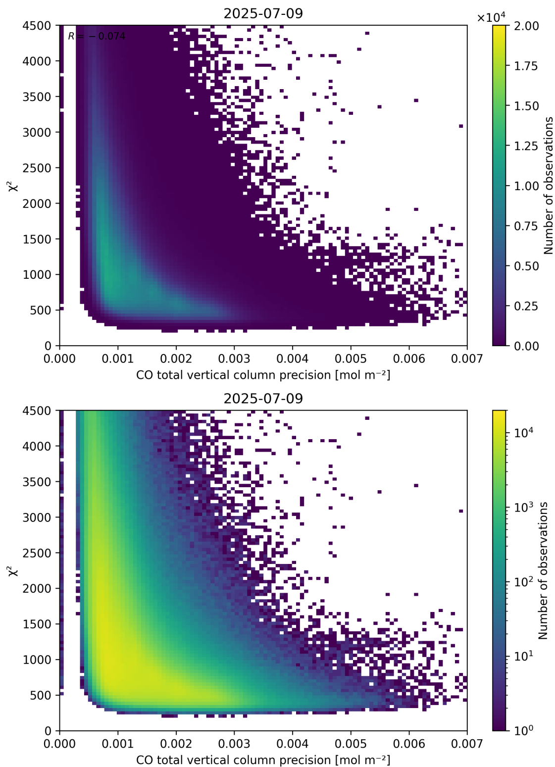
Figure 44: Scatter density plot of “CO total vertical column precision” against “ \chi^2 ” for 2025-07-08 to 2025-07-10.
