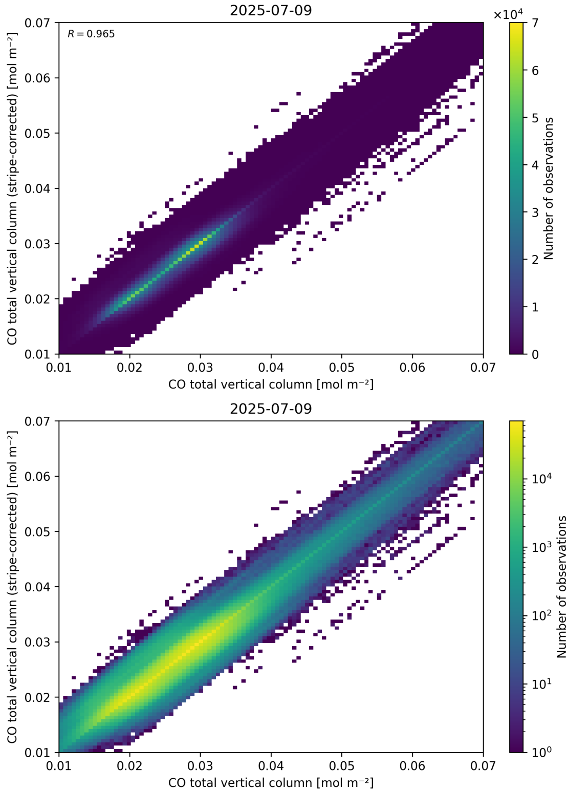
Figure 33: Scatter density plot of “CO total vertical column” against “CO total vertical column (stripe-corrected)” for 2025-07-08 to 2025-07-10.
