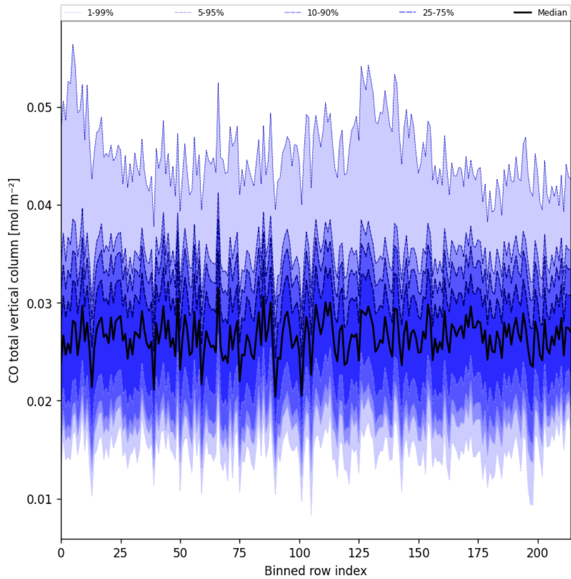
Figure 26: Along track statistics of “CO total vertical column” for 2025-07-08 to 2025-07-10
