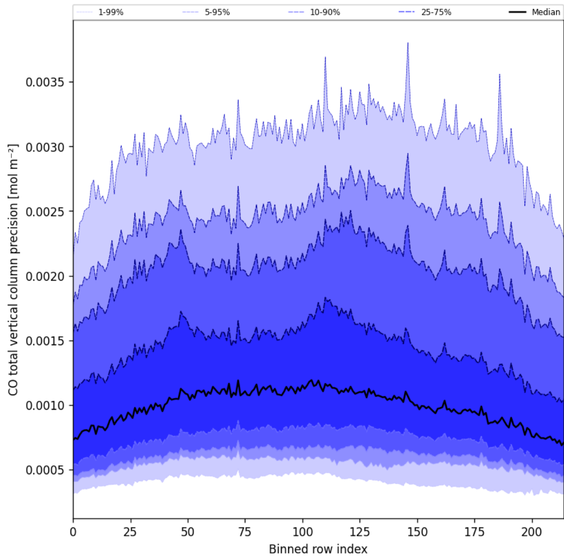
Figure 28: Along track statistics of “CO total vertical column precision” for 2025-07-08 to 2025-07-10
