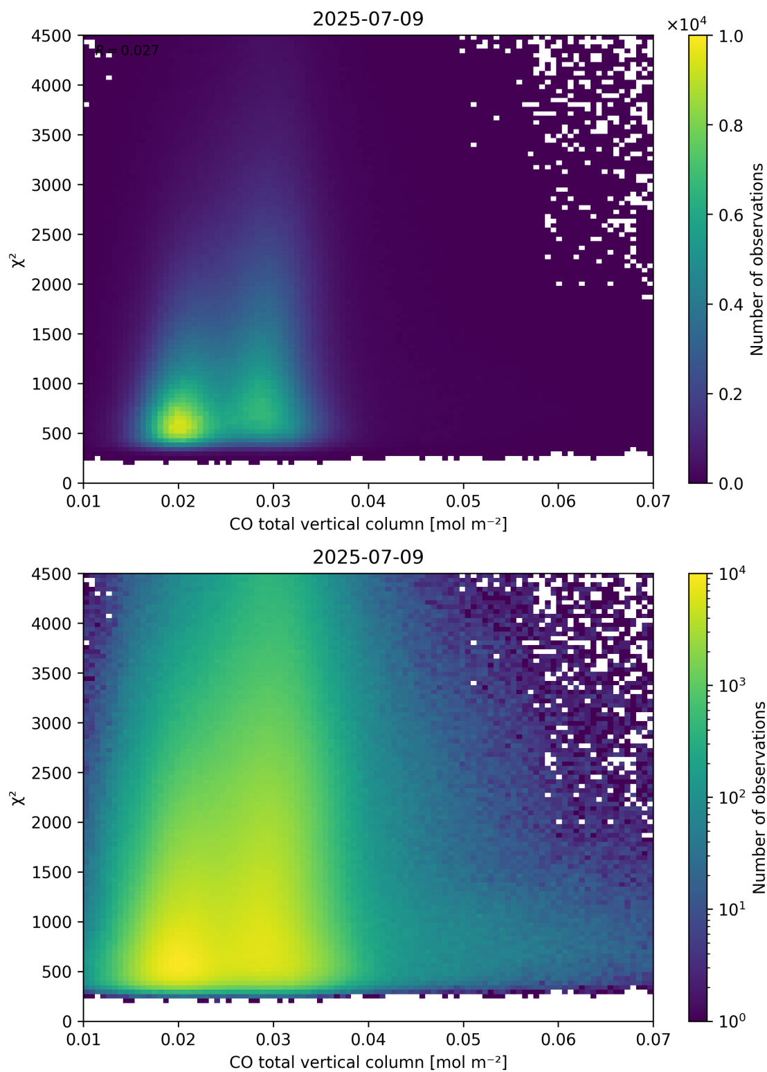
Figure 35: Scatter density plot of “CO total vertical column” against “ \chi^2 ” for 2025-07-08 to 2025-07-10.
