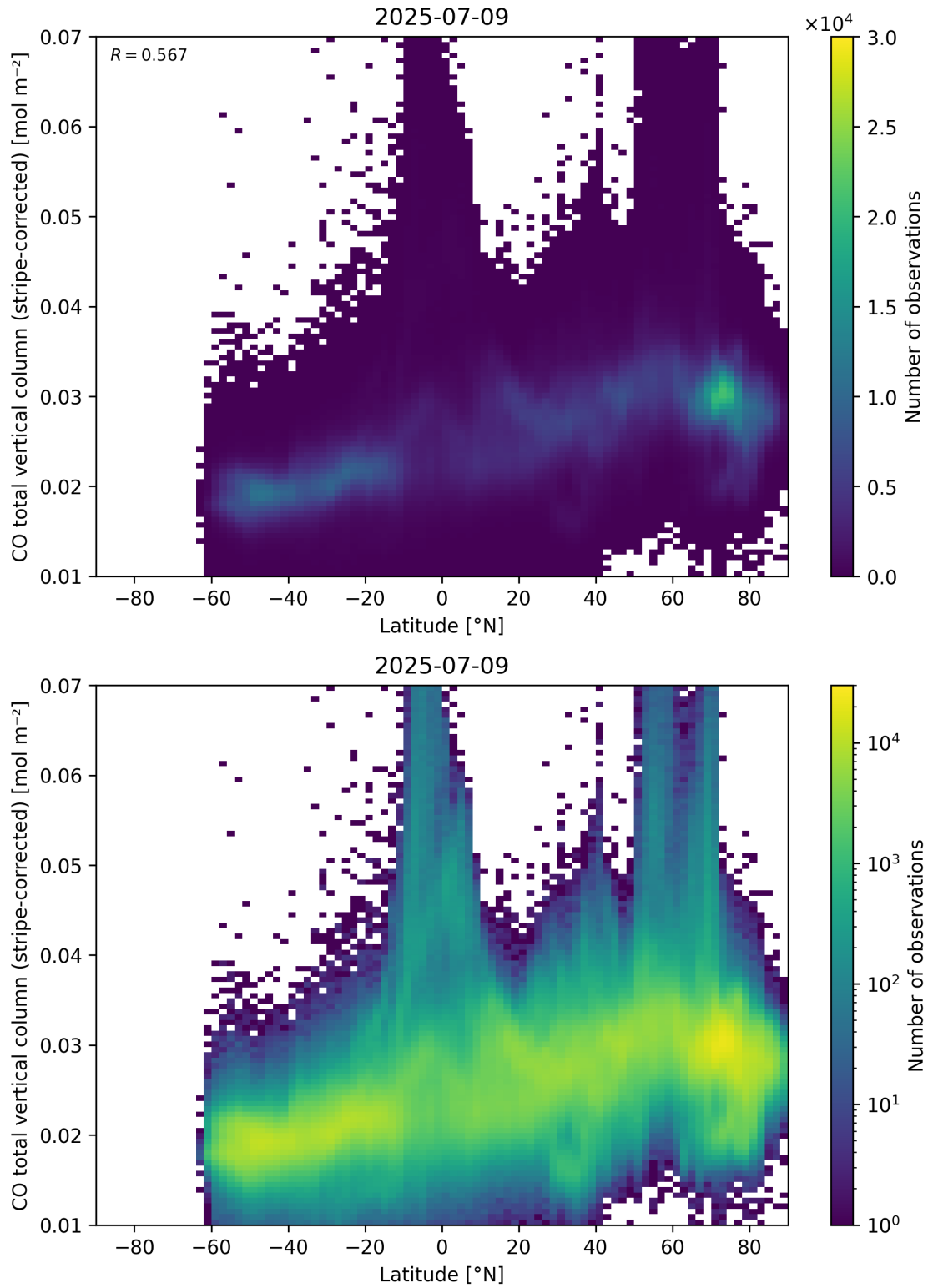
Figure 52: Scatter density plot of “Latitude” against “CO total vertical column (stripe-corrected)” for 2025-07-08 to 2025-07-10.
