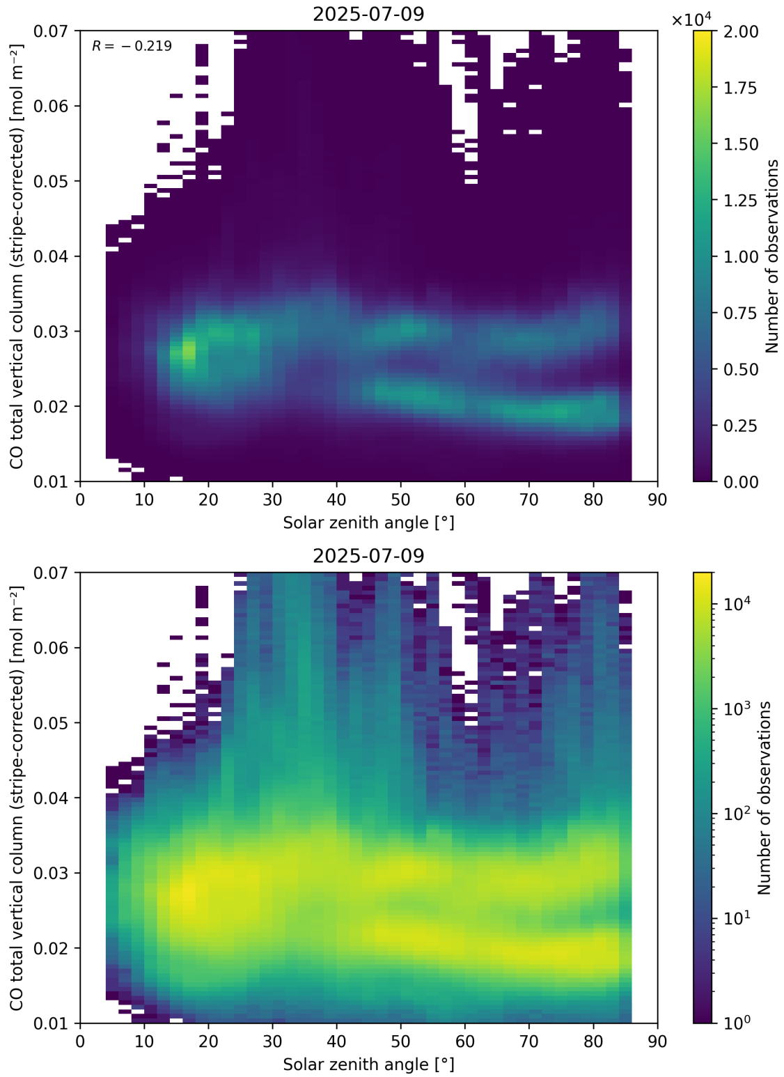
Figure 62: Scatter density plot of “Solar zenith angle” against “CO total vertical column (stripe-corrected)” for 2025-07-08 to 2025-07-10.
