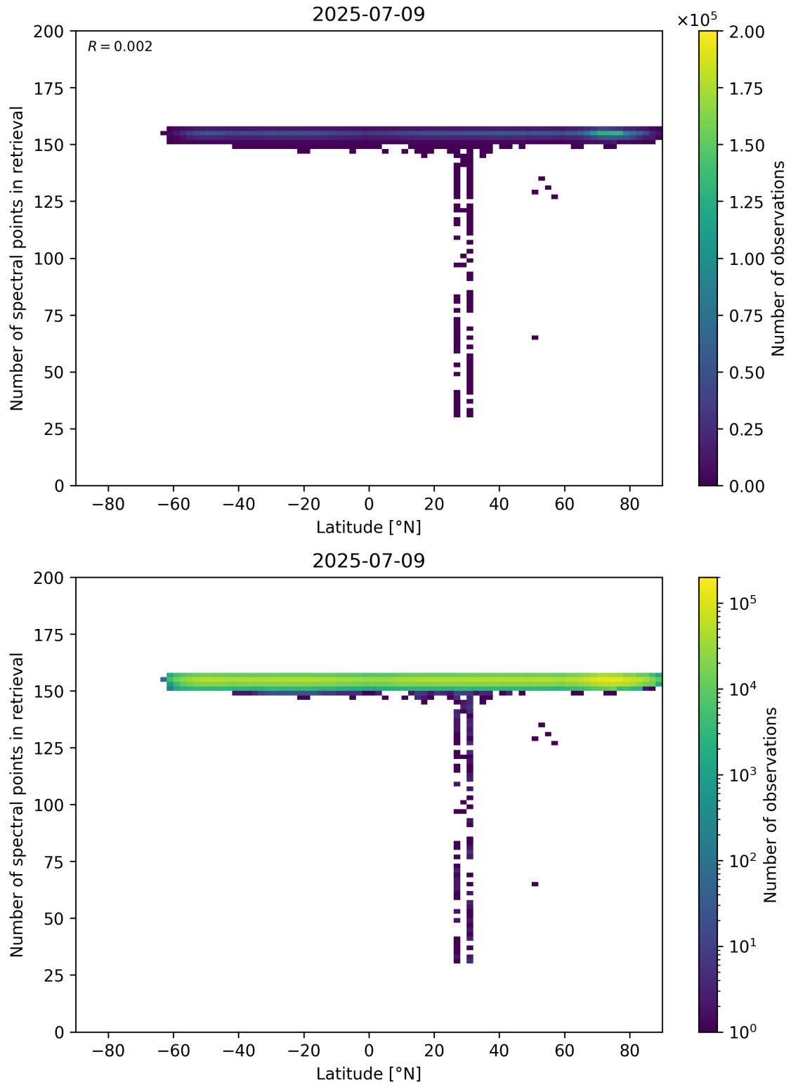
Figure 57: Scatter density plot of “Latitude” against “Number of spectral points in retrieval” for 2025-07-08 to 2025-07-10.
