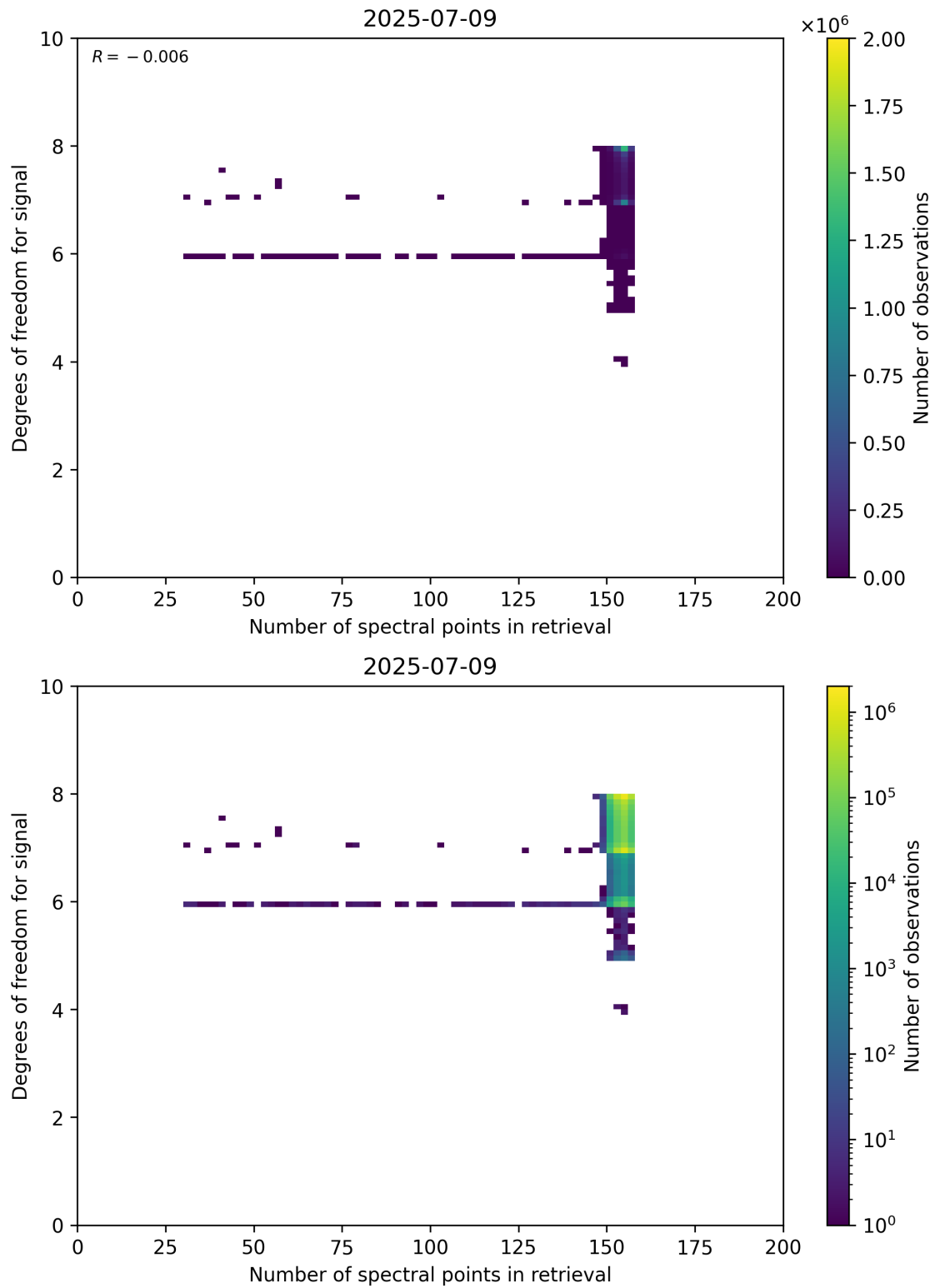
Figure 59: Scatter density plot of “Number of spectral points in retrieval” against “Degrees of freedom for signal” for 2025-07-08 to 2025-07-10.
