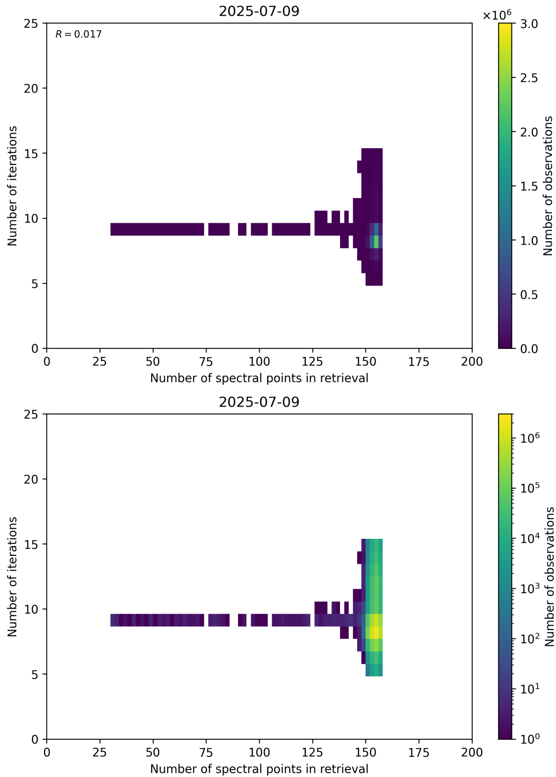
Figure 60: Scatter density plot of “Number of spectral points in retrieval” against “Number of iterations” for 2025-07-08 to 2025-07-10.
