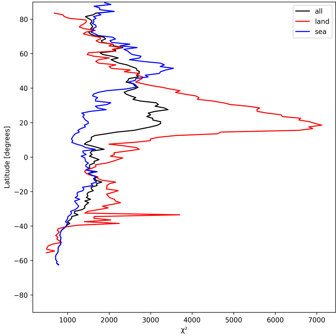
Figure 14: Zonal average of “ \chi^2 ” for 2025-07-08 to 2025-07-10.
