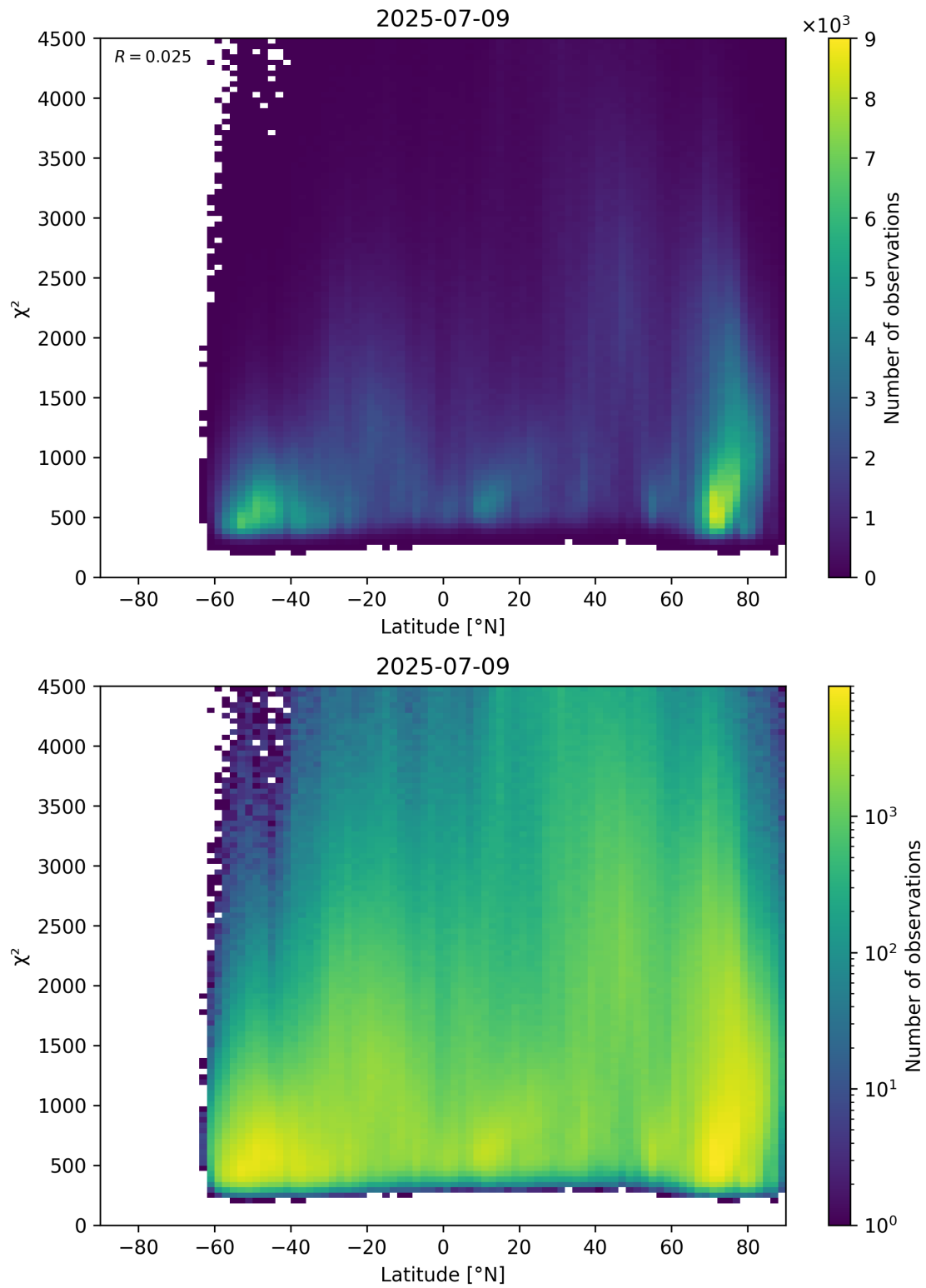
Figure 54: Scatter density plot of “Latitude” against “ \chi^2 ” for 2025-07-08 to 2025-07-10.
