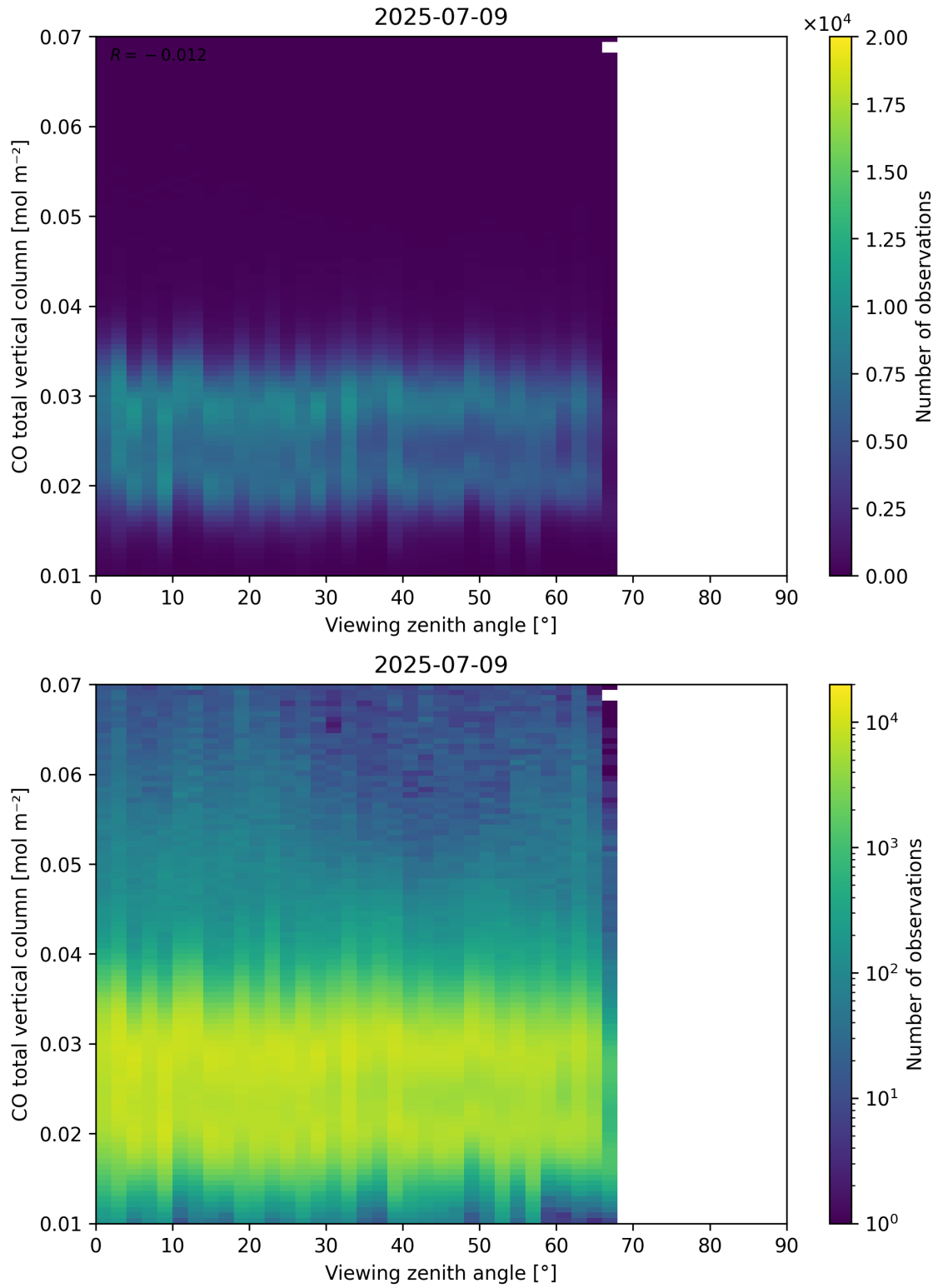
Figure 69: Scatter density plot of “Viewing zenith angle” against “CO total vertical column” for 2025-07-08 to 2025-07-10.
