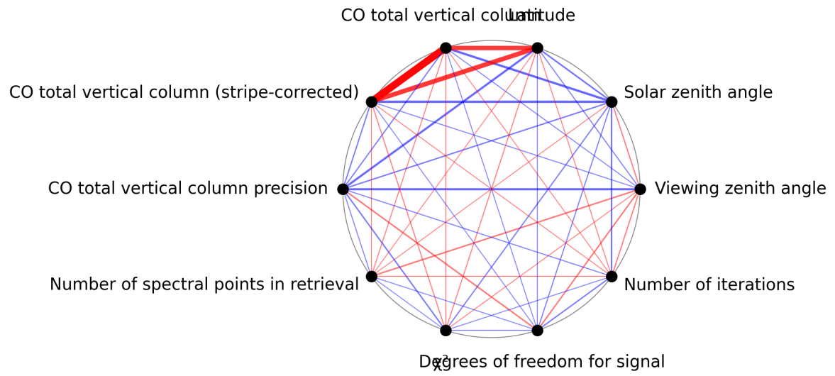
Figure 1: Map of correlation graph for 2025-07-08 to 2025-07-10.
