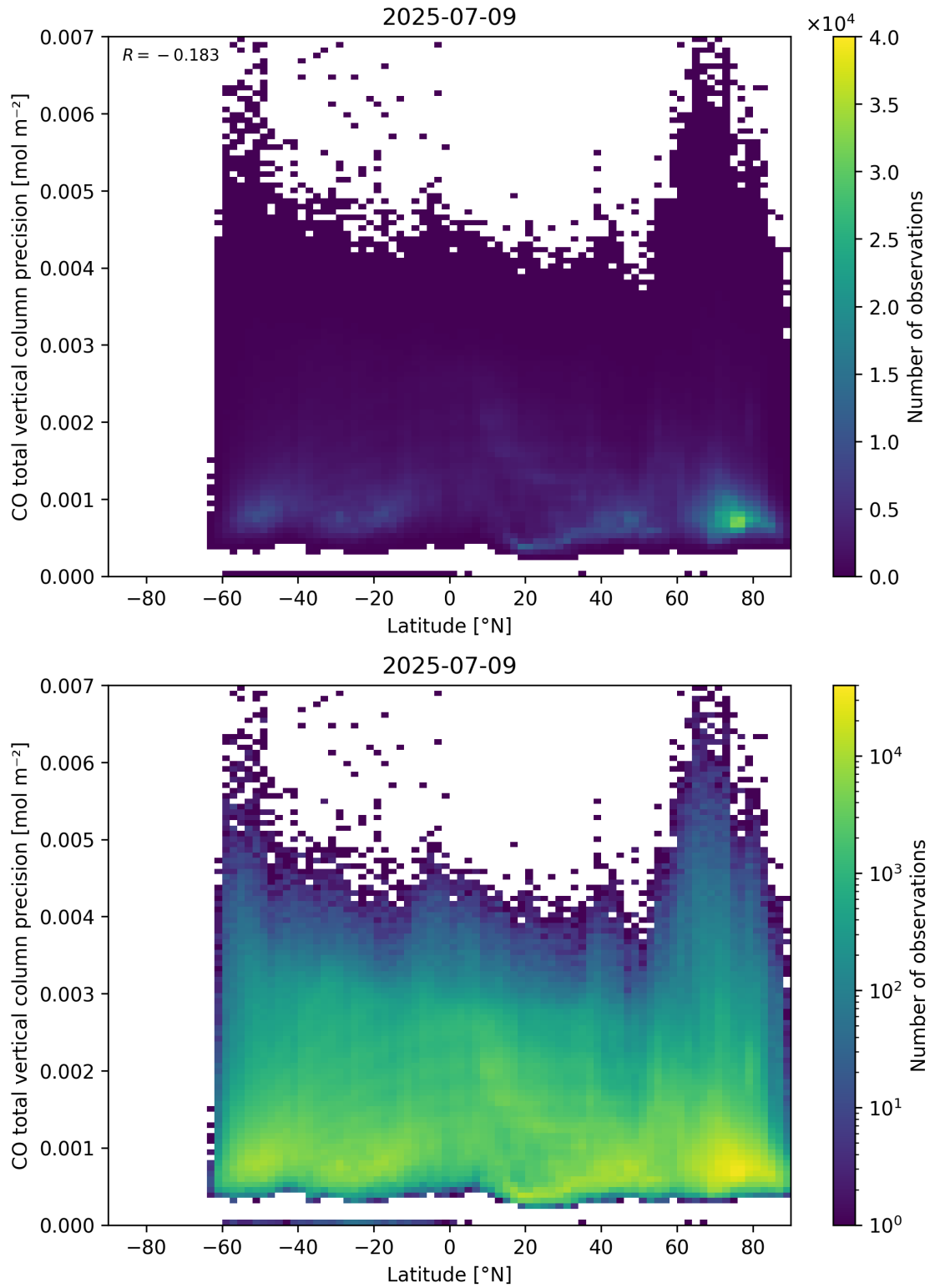
Figure 53: Scatter density plot of “Latitude” against “CO total vertical column precision” for 2025-07-08 to 2025-07-10.
