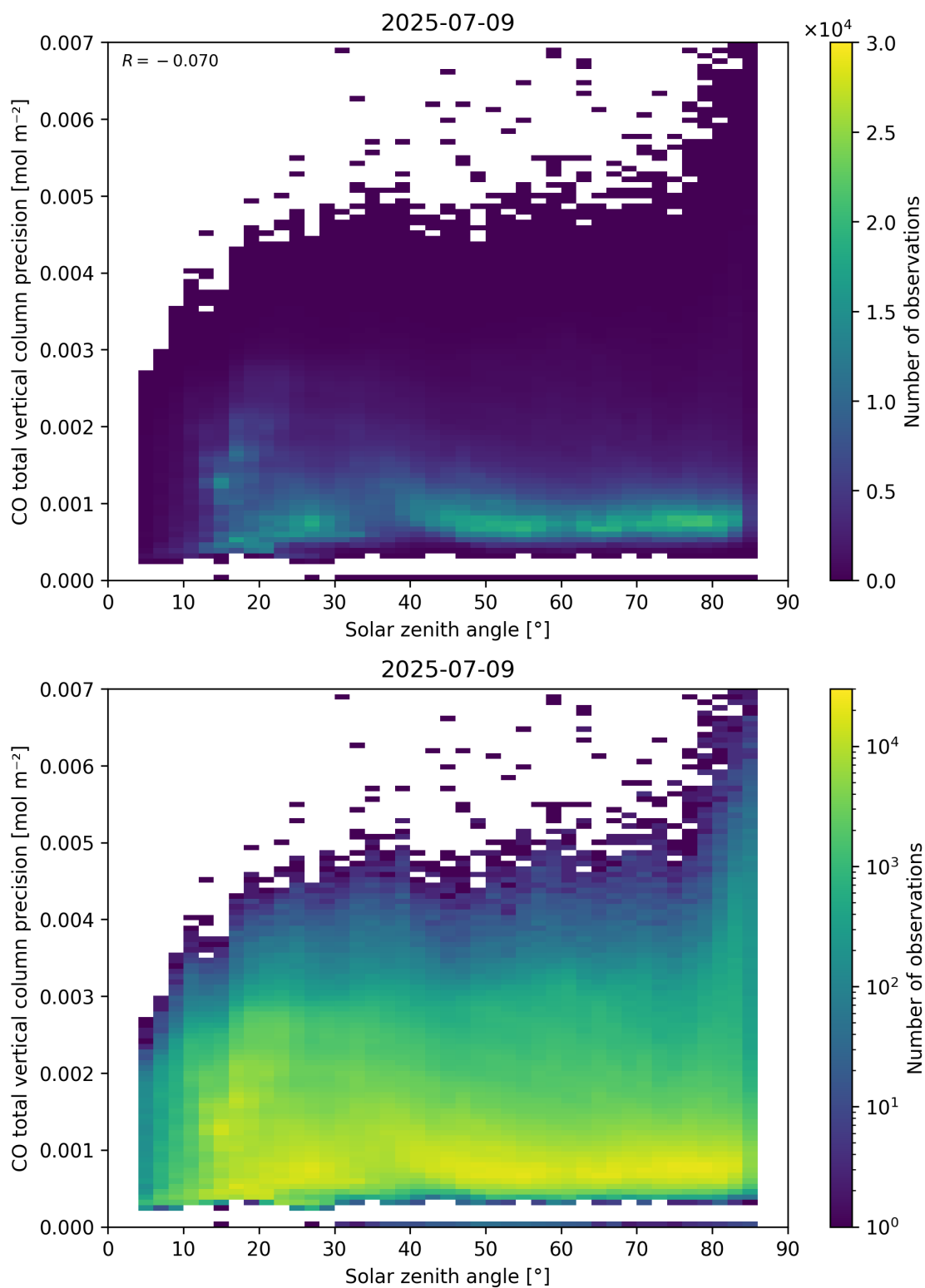
Figure 63: Scatter density plot of “Solar zenith angle” against “CO total vertical column precision” for 2025-07-08 to 2025-07-10.
