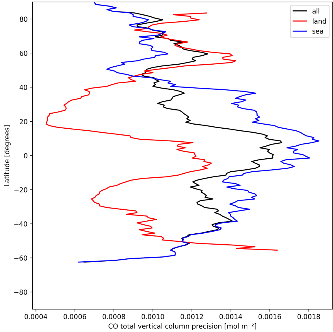
Figure 12: Zonal average of “CO total vertical column precision” for 2025-07-08 to 2025-07-10.
