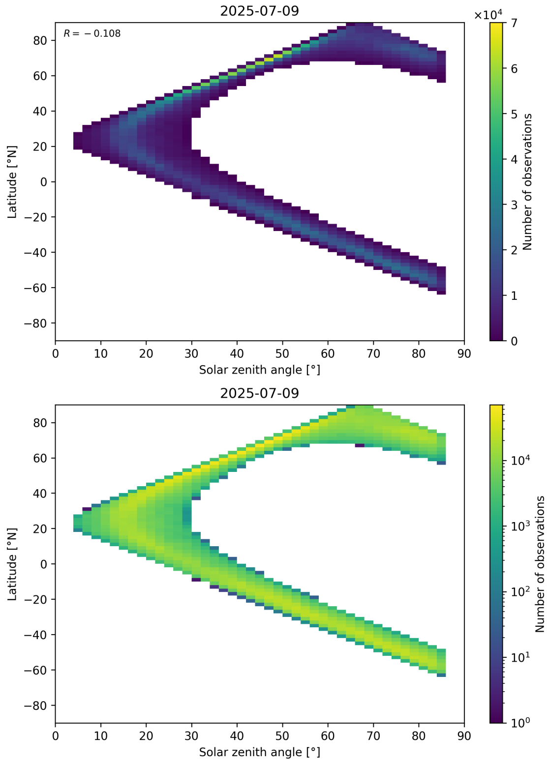
Figure 66: Scatter density plot of “Solar zenith angle” against “Latitude” for 2025-07-08 to 2025-07-10.
