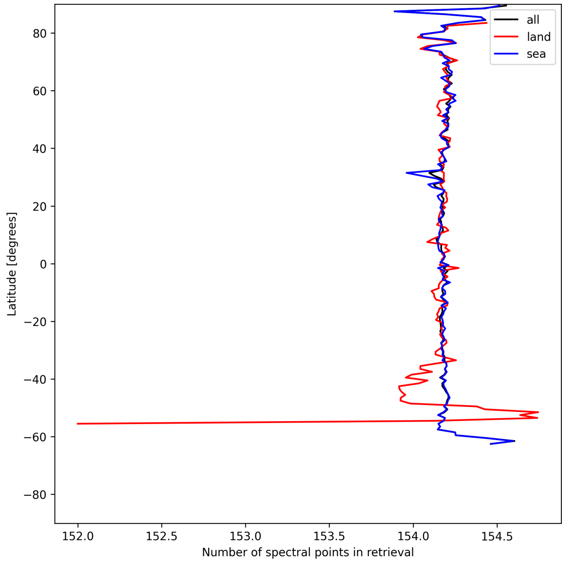
Figure 13: Zonal average of “Number of spectral points in retrieval” for 2025-07-08 to 2025-07-10.
