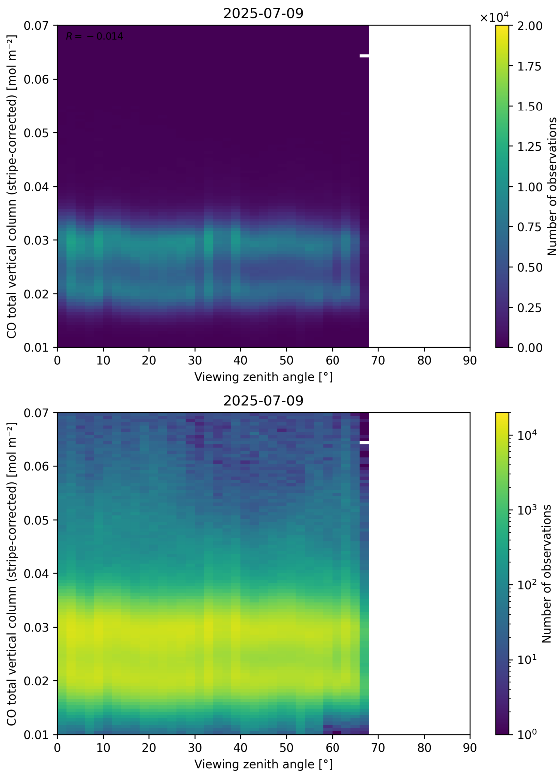
Figure 70: Scatter density plot of “Viewing zenith angle” against “CO total vertical column (stripe-corrected)” for 2025-07-08 to 2025-07-10.
