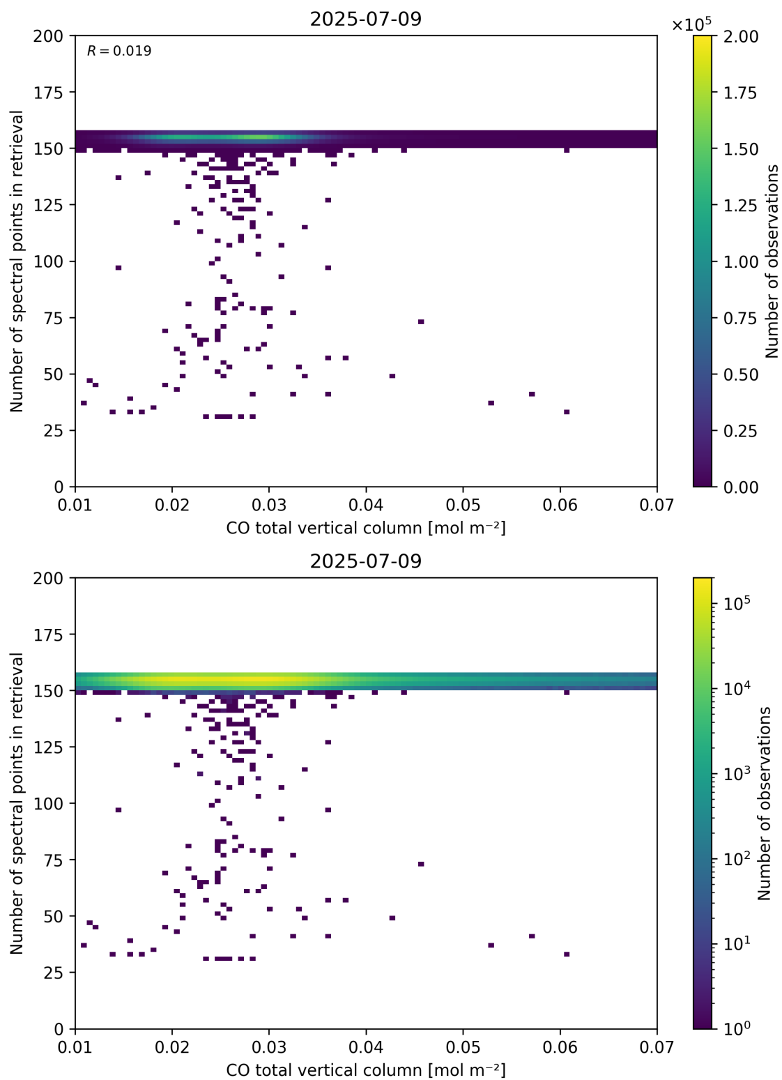
Figure 43: Scatter density plot of “CO total vertical column” against “Number of spectral points in retrieval” for 2025-07-08 to 2025-07-10.
