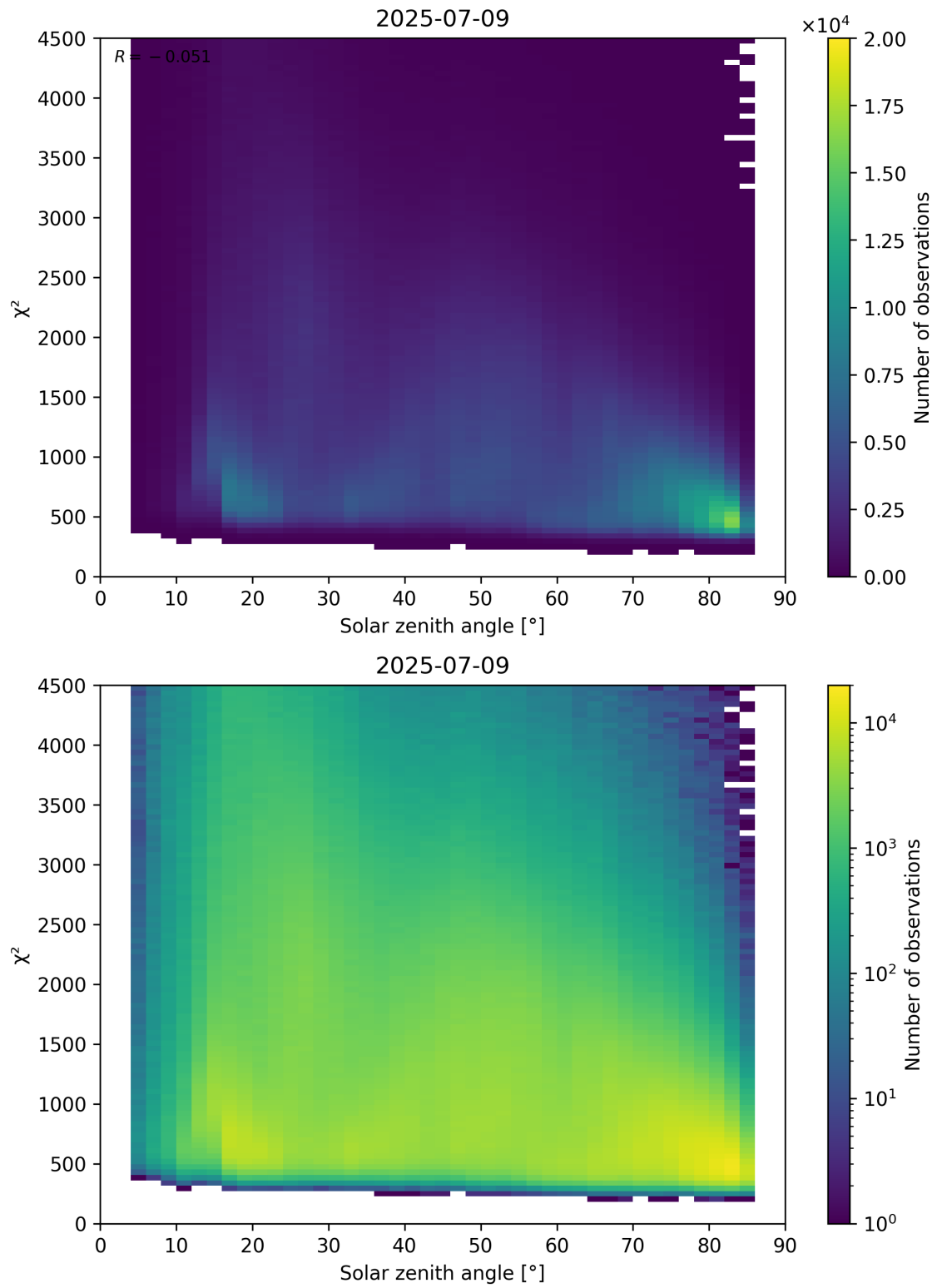
Figure 64: Scatter density plot of “Solar zenith angle” against “ \chi^2 ” for 2025-07-08 to 2025-07-10.
