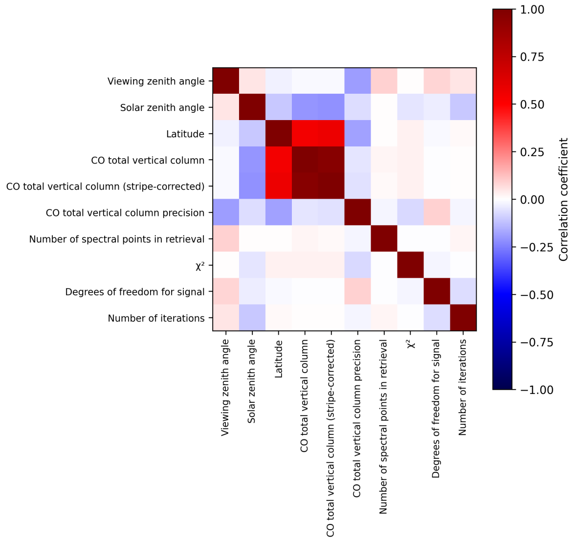
Figure 2: Map of correlation matrix for 2025-07-08 to 2025-07-10.
