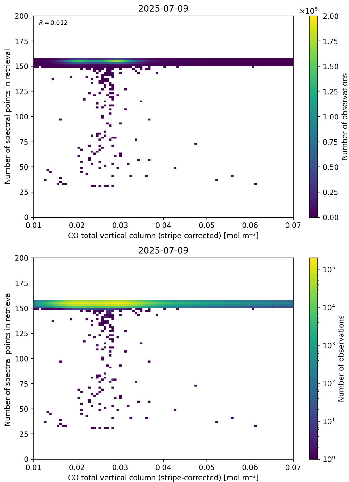
Figure 40: Scatter density plot of “CO total vertical column (stripe-corrected)” against “Number of spectral points in retrieval” for 2025-07-08 to 2025-07-10.
