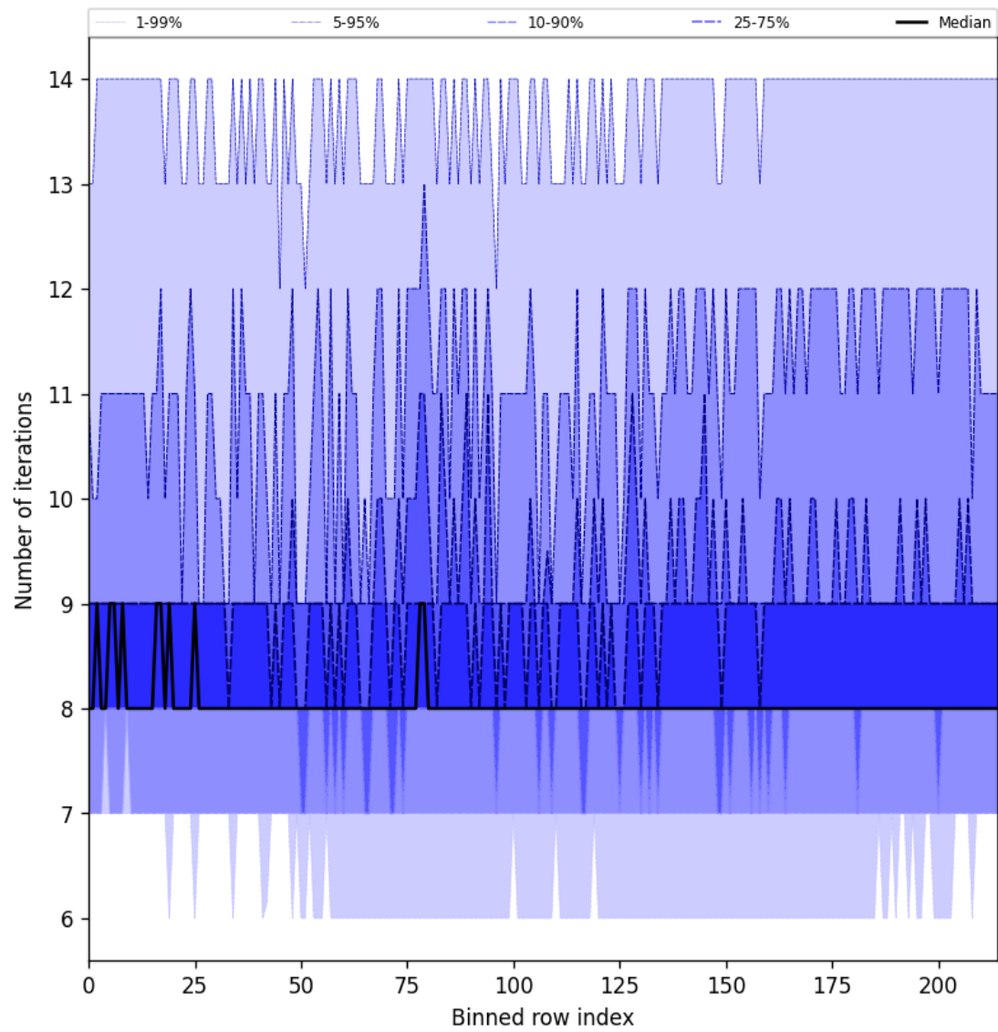
Figure 32: Along track statistics of “Number of iterations” for 2025-07-08 to 2025-07-10
