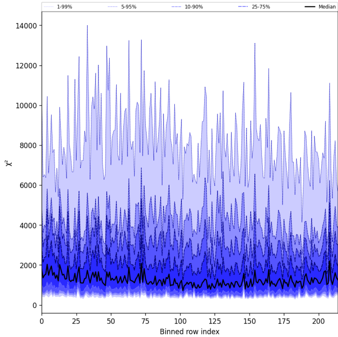
Figure 30: Along track statistics of “ \chi^2 ” for 2025-07-08 to 2025-07-10
