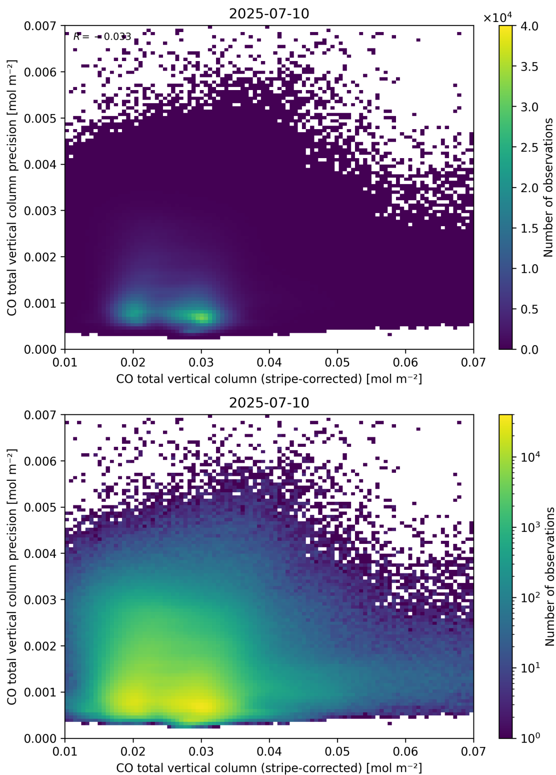
Figure 36: Scatter density plot of “CO total vertical column (stripe-corrected)” against “CO total vertical column precision” for 2025-07-09 to 2025-07-11.
