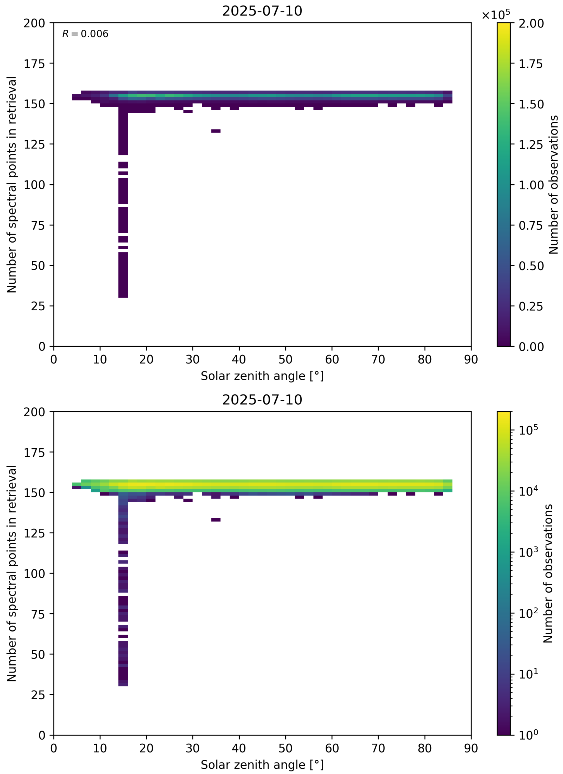
Figure 68: Scatter density plot of “Solar zenith angle” against “Number of spectral points in retrieval” for 2025-07-09 to 2025-07-11.
