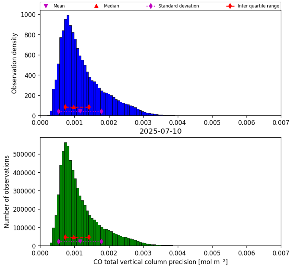
Figure 20: Histogram of “CO total vertical column precision” for 2025-07-09 to 2025-07-11
