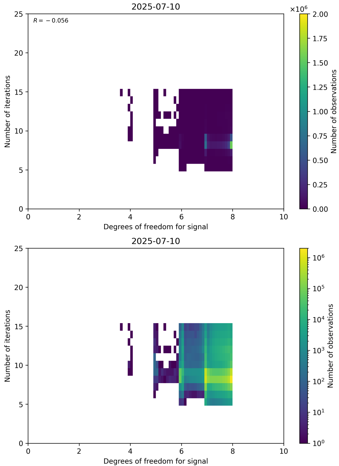
Figure 50: Scatter density plot of “Degrees of freedom for signal” against “Number of iterations” for 2025-07-09 to 2025-07-11.
