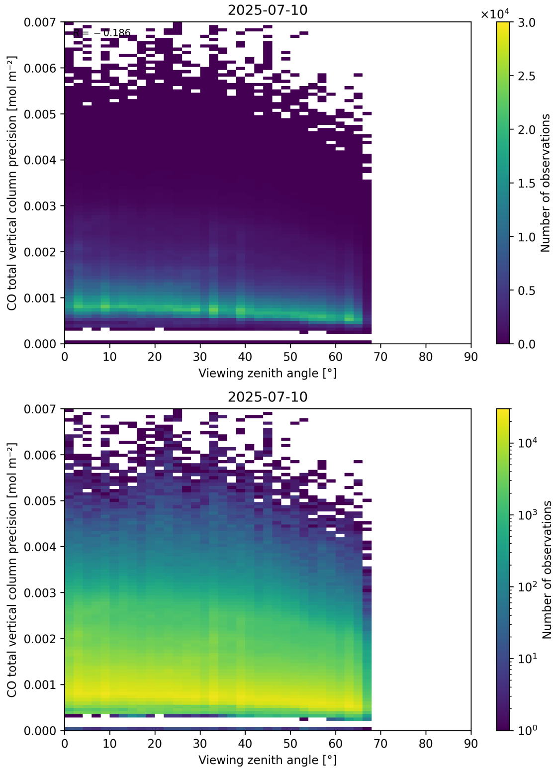
Figure 71: Scatter density plot of “Viewing zenith angle” against “CO total vertical column precision” for 2025-07-09 to 2025-07-11.
