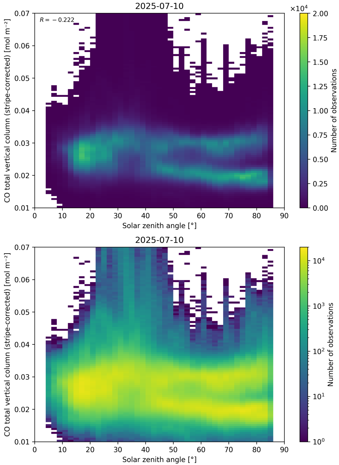
Figure 62: Scatter density plot of “Solar zenith angle” against “CO total vertical column (stripe-corrected)” for 2025-07-09 to 2025-07-11.
