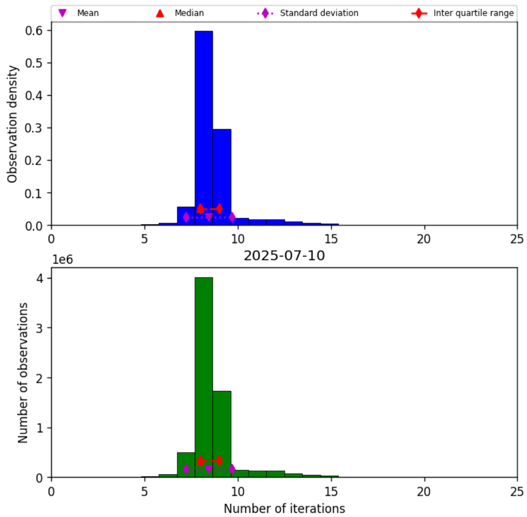
Figure 24: Histogram of “Number of iterations” for 2025-07-09 to 2025-07-11
