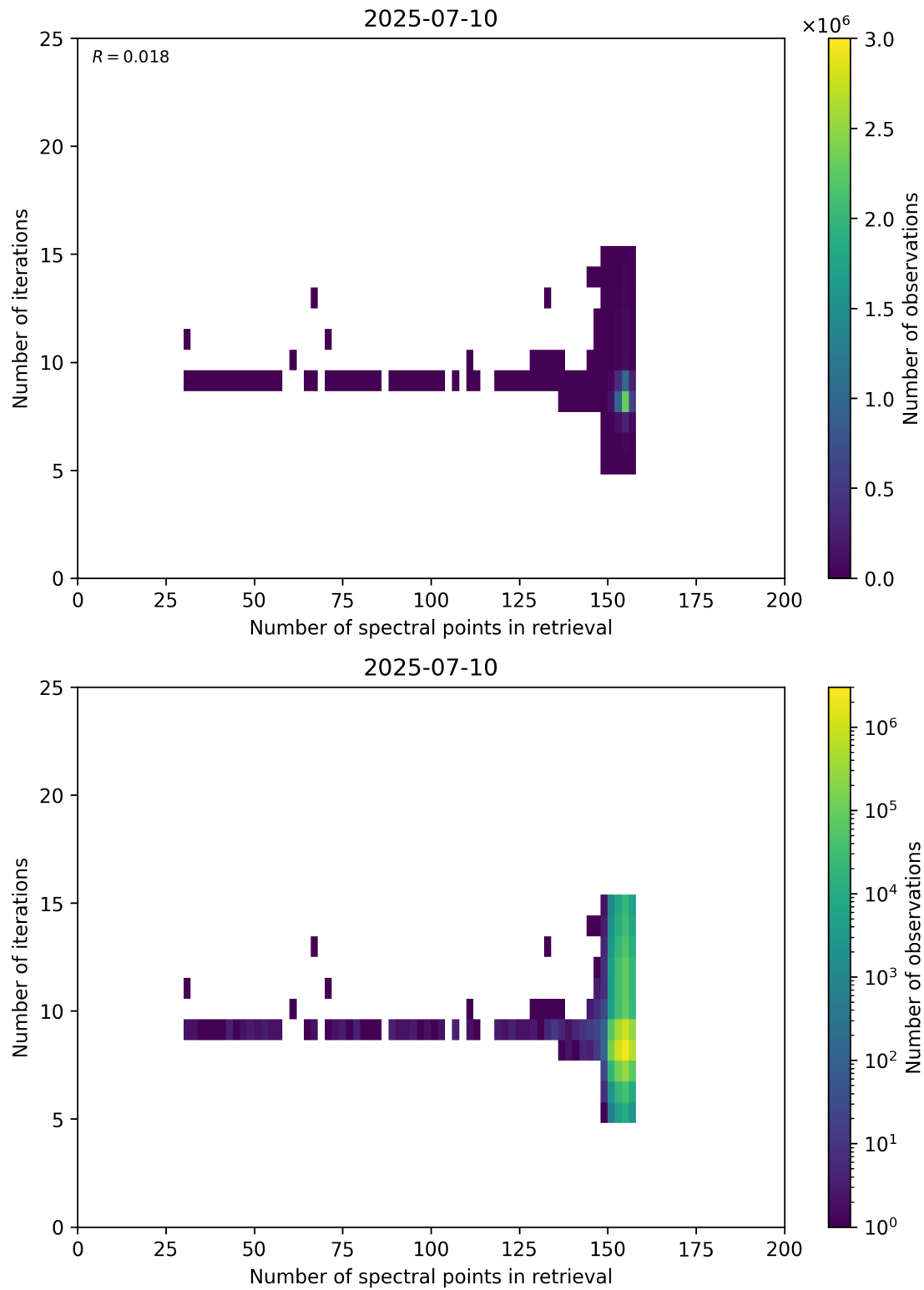
Figure 60: Scatter density plot of “Number of spectral points in retrieval” against “Number of iterations” for 2025-07-09 to 2025-07-11.
