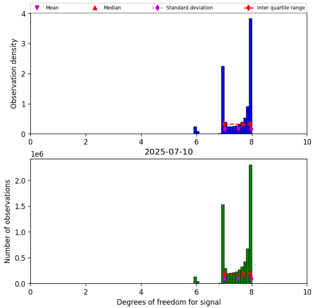
Figure 23: Histogram of “Degrees of freedom for signal” for 2025-07-09 to 2025-07-11
