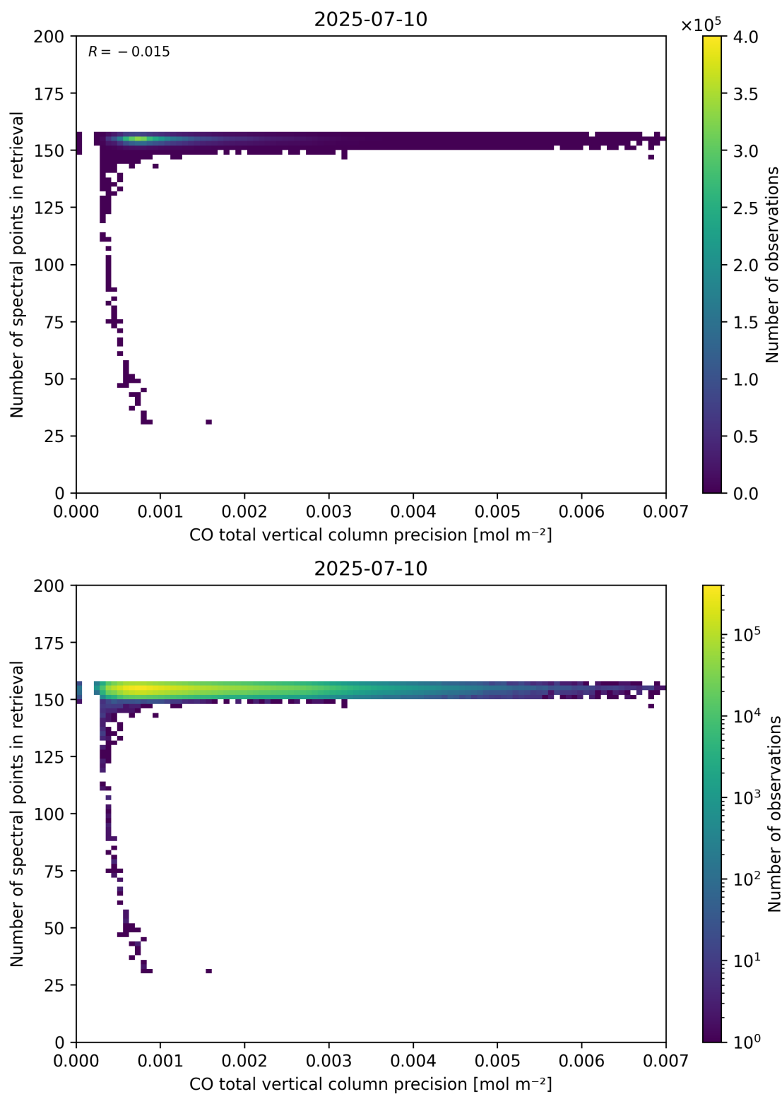
Figure 47: Scatter density plot of “CO total vertical column precision” against “Number of spectral points in retrieval” for 2025-07-09 to 2025-07-11.
