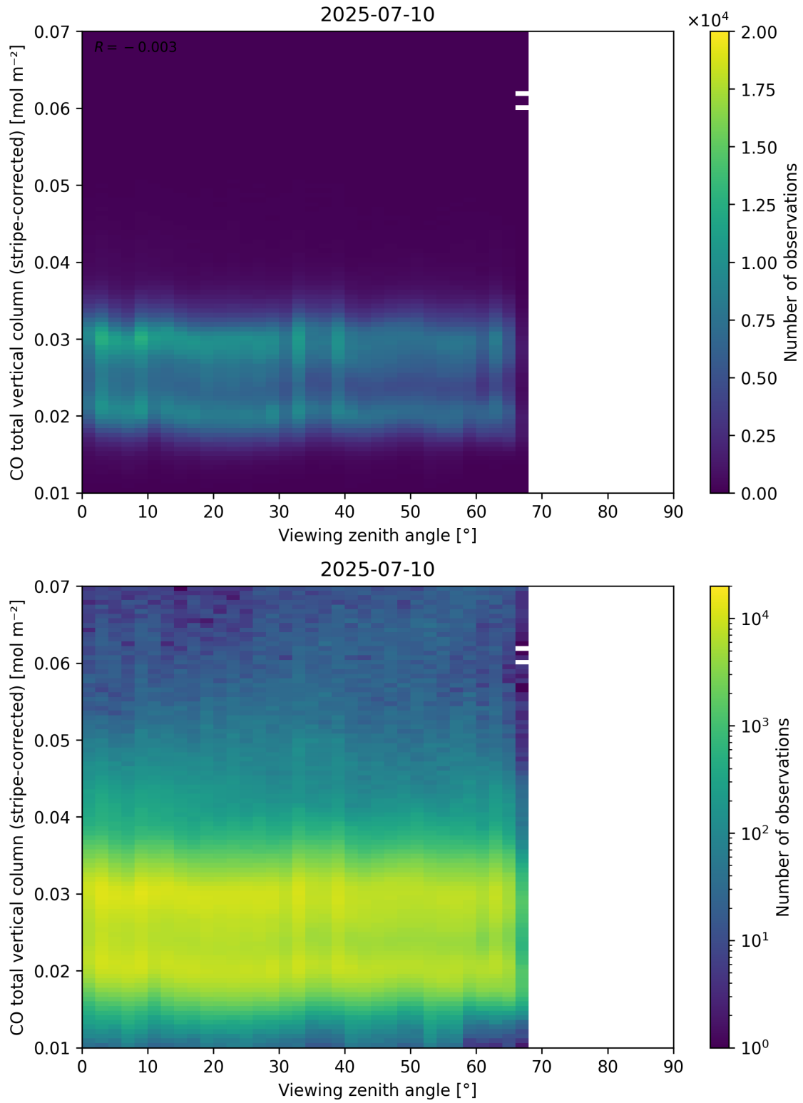
Figure 70: Scatter density plot of “Viewing zenith angle” against “CO total vertical column (stripe-corrected)” for 2025-07-09 to 2025-07-11.
