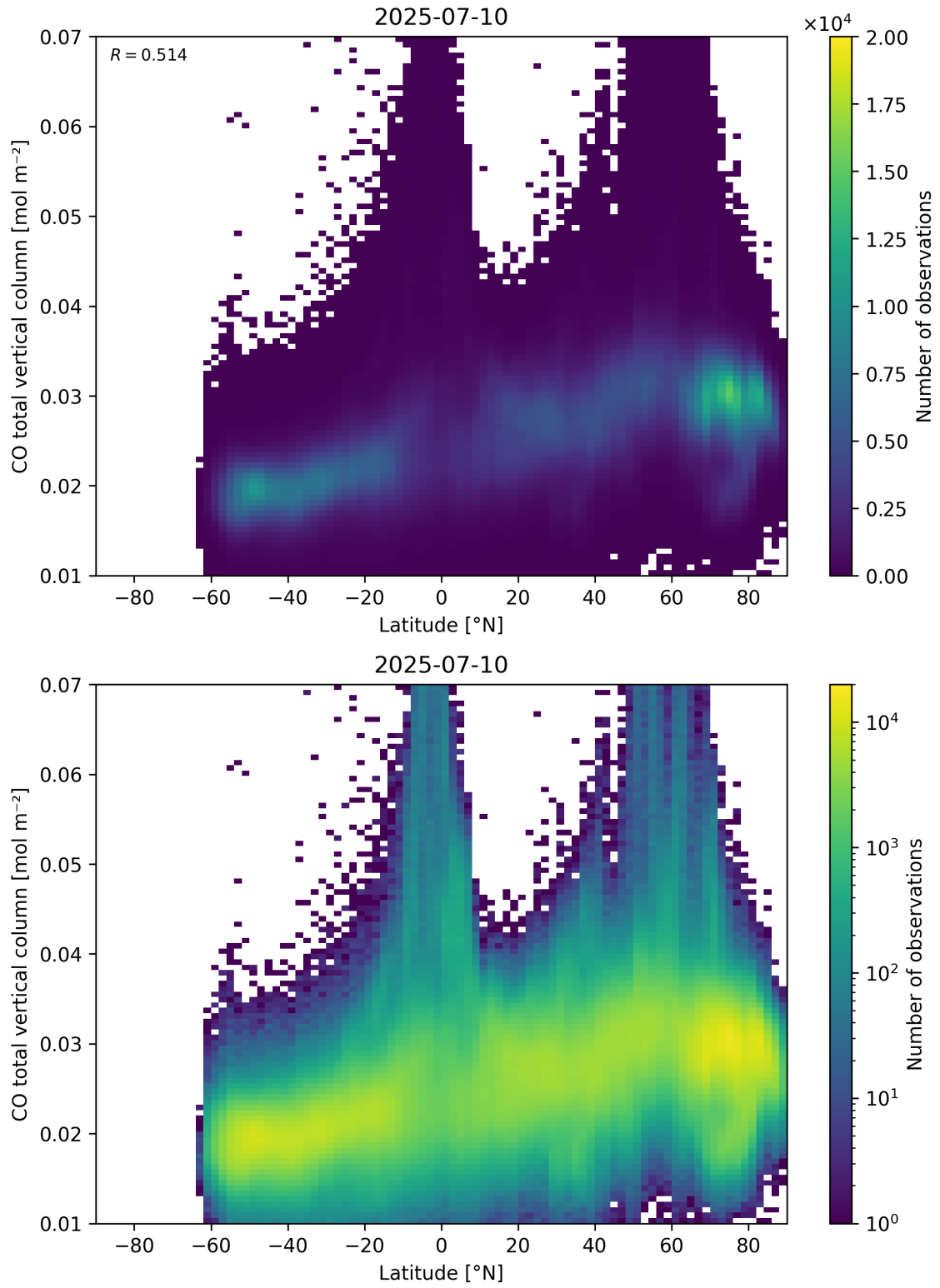
Figure 51: Scatter density plot of “Latitude” against “CO total vertical column” for 2025-07-09 to 2025-07-11.
