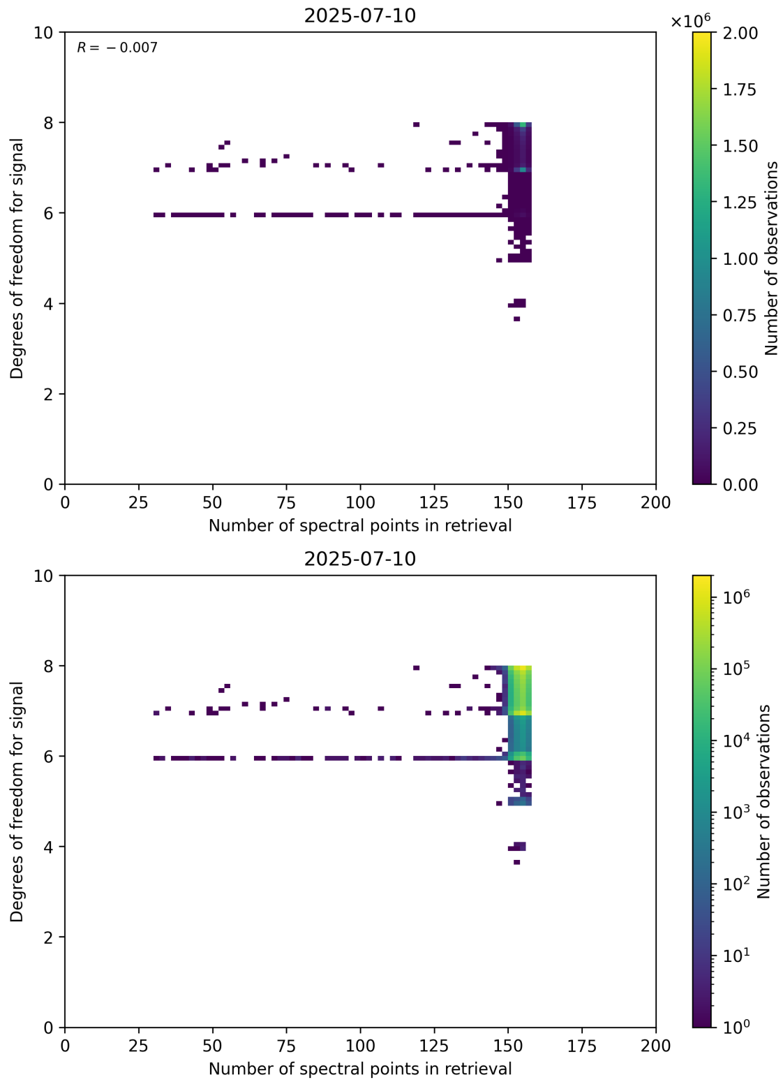
Figure 59: Scatter density plot of “Number of spectral points in retrieval” against “Degrees of freedom for signal” for 2025-07-09 to 2025-07-11.
