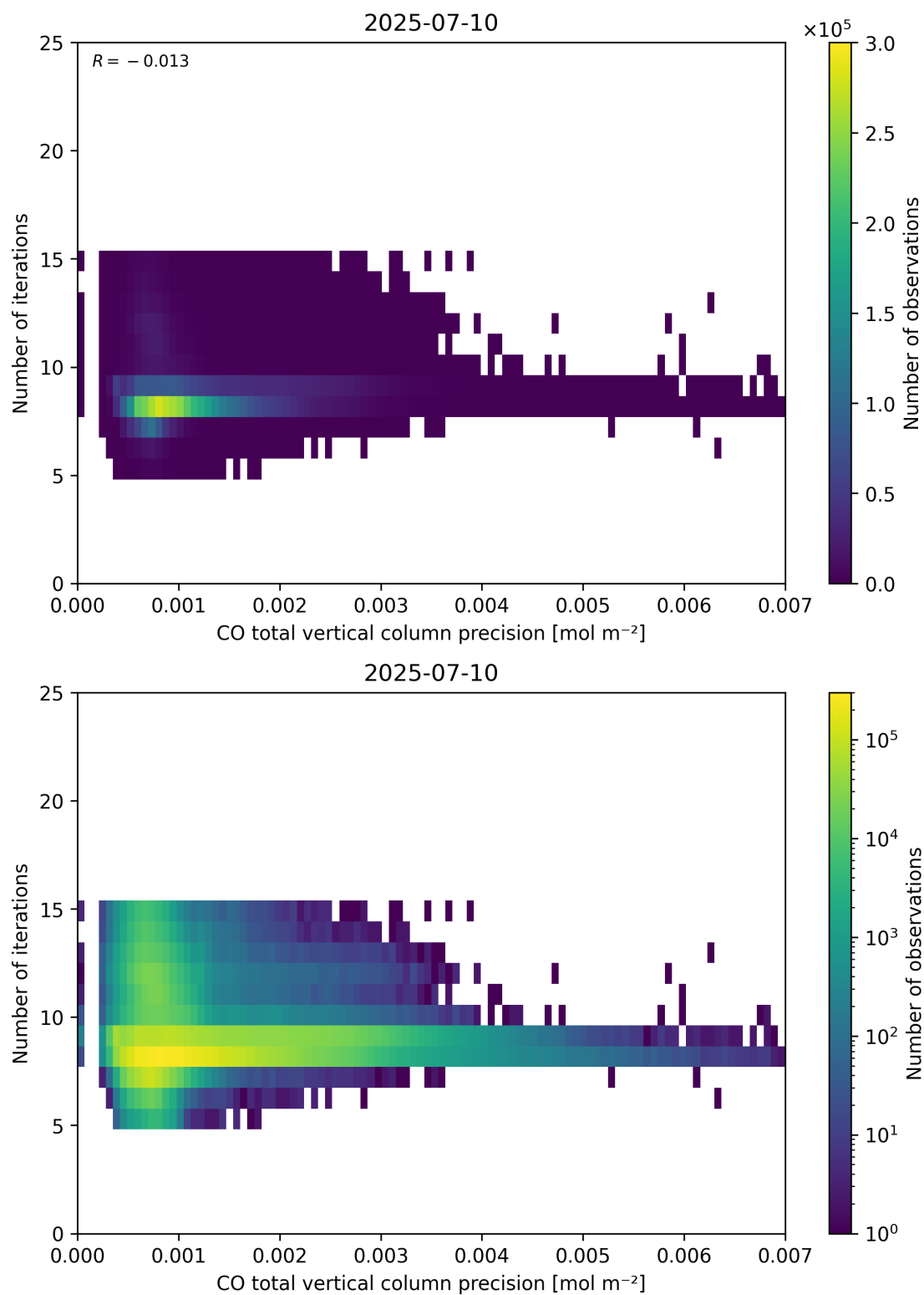
Figure 46: Scatter density plot of “CO total vertical column precision” against “Number of iterations” for 2025-07-09 to 2025-07-11.
