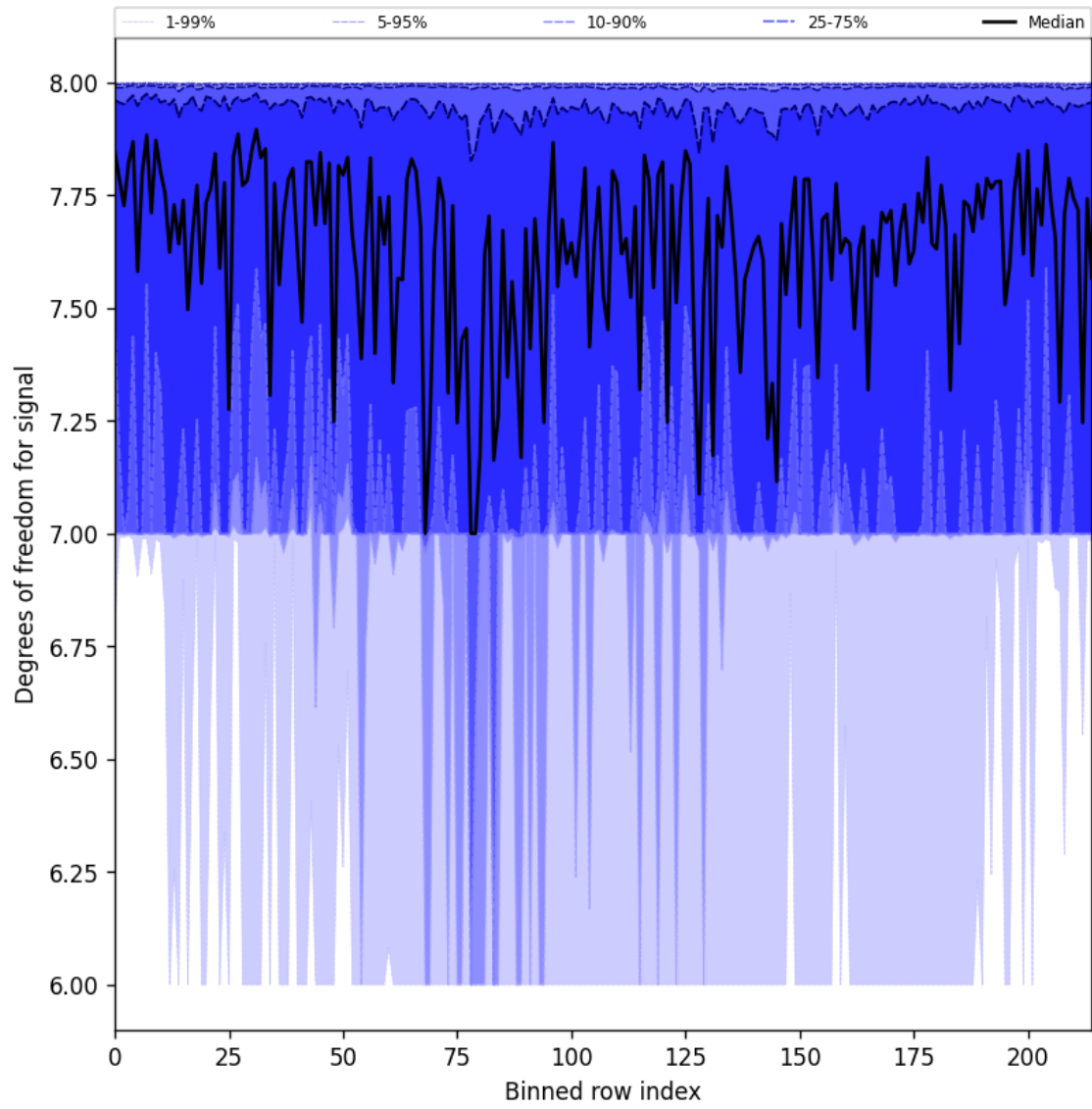
Figure 31: Along track statistics of “Degrees of freedom for signal” for 2025-07-09 to 2025-07-11
