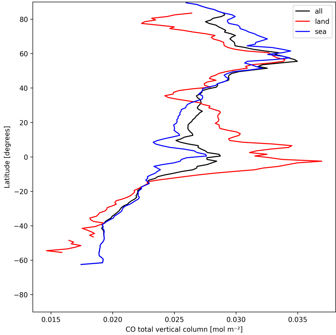
Figure 10: Zonal average of “CO total vertical column” for 2025-07-09 to 2025-07-11.
