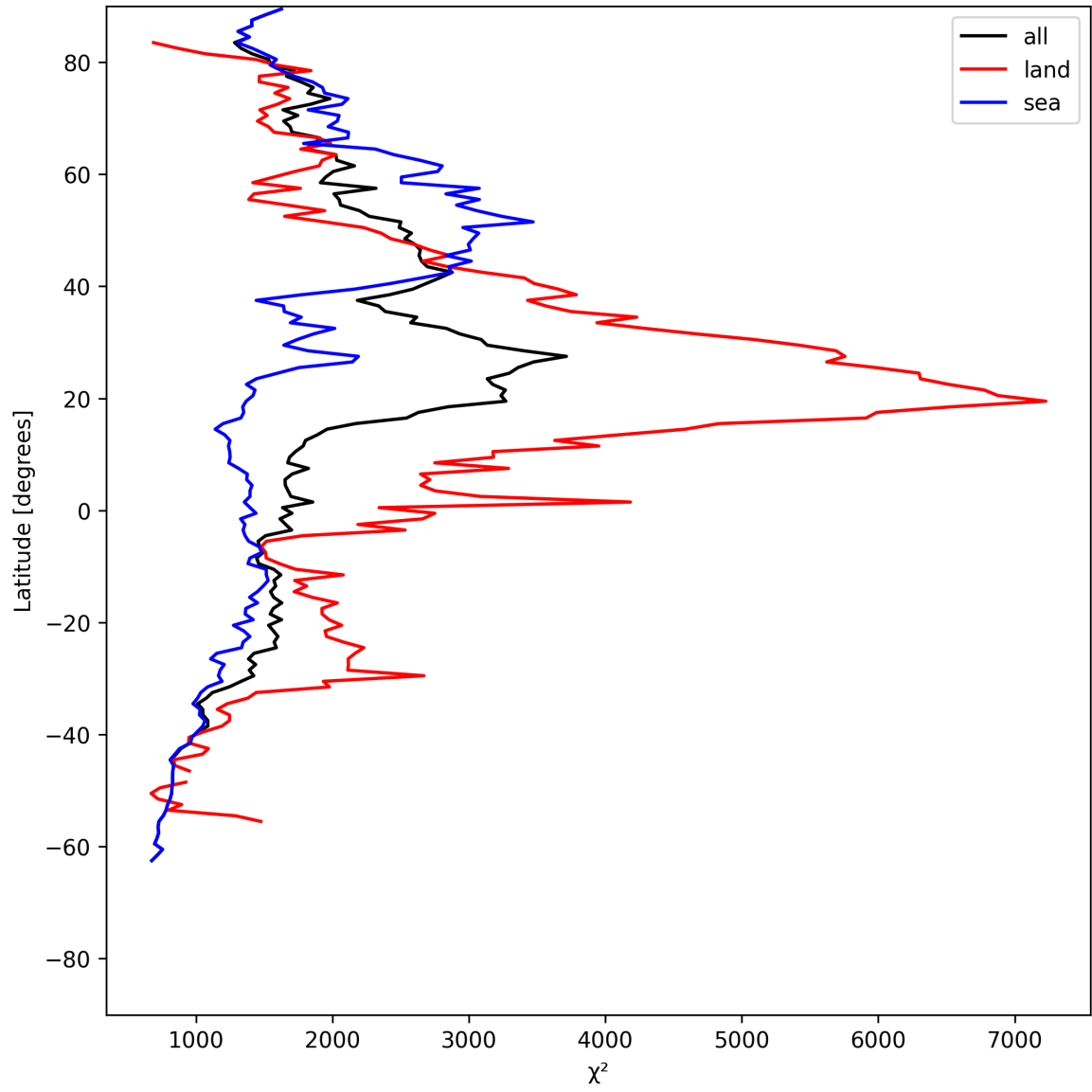
Figure 14: Zonal average of “ \chi^2 ” for 2025-07-09 to 2025-07-11.
