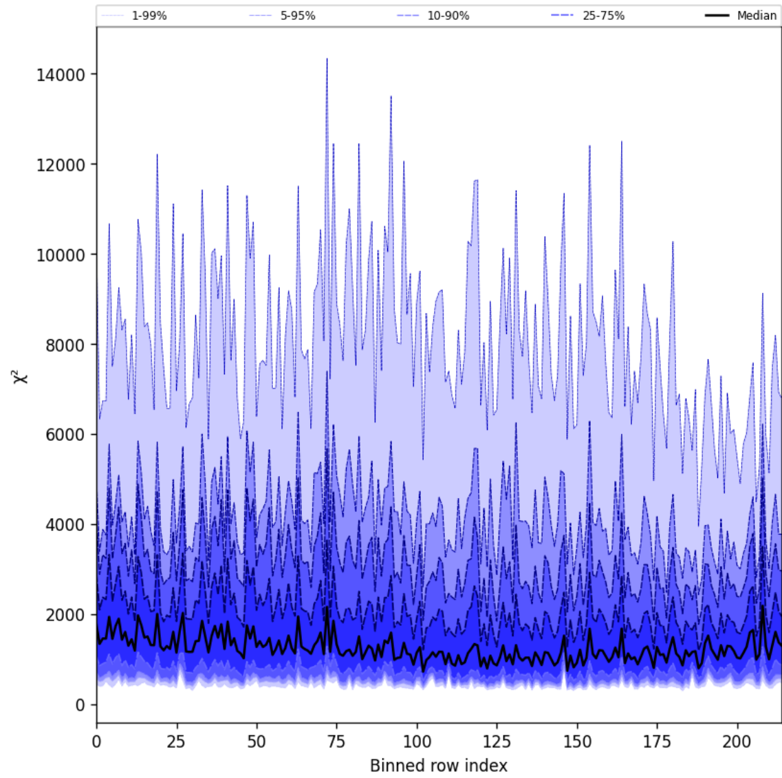
Figure 30: Along track statistics of “ \chi^2 ” for 2025-07-09 to 2025-07-11
