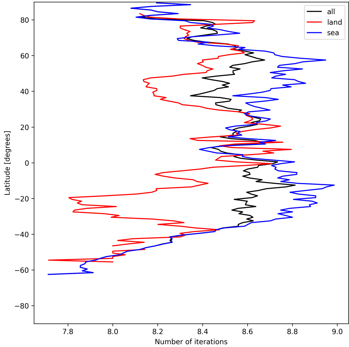
Figure 16: Zonal average of “Number of iterations” for 2025-07-09 to 2025-07-11.
