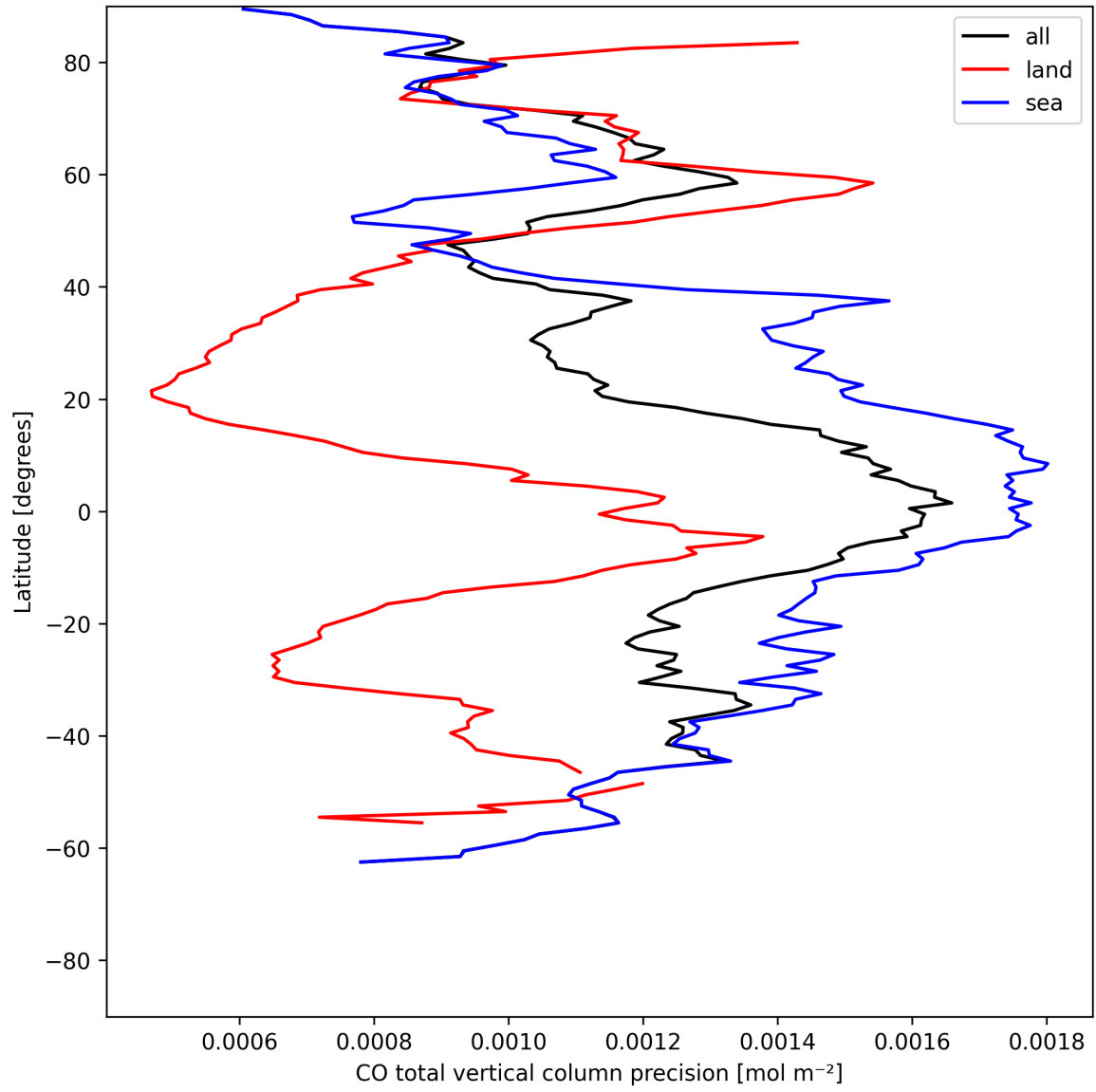
Figure 12: Zonal average of “CO total vertical column precision” for 2025-07-09 to 2025-07-11.
