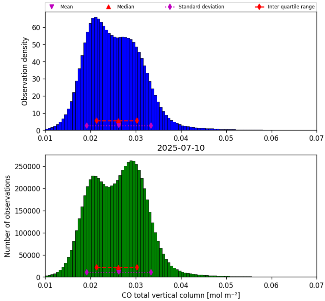
Figure 18: Histogram of “CO total vertical column” for 2025-07-09 to 2025-07-11
