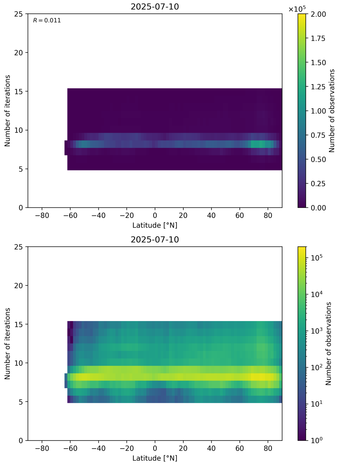
Figure 56: Scatter density plot of “Latitude” against “Number of iterations” for 2025-07-09 to 2025-07-11.
