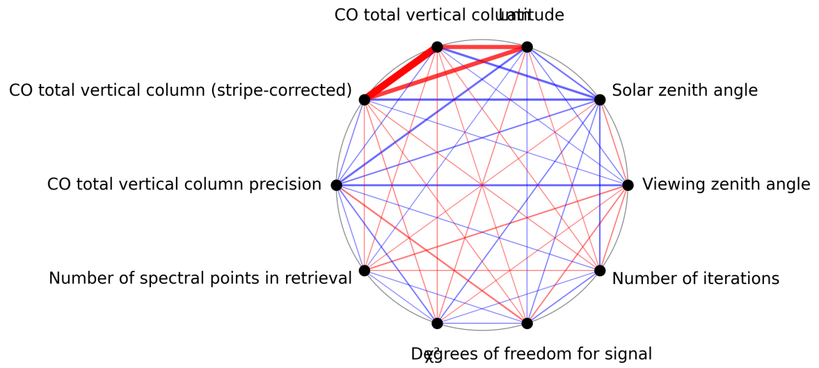
Figure 1: Map of correlation graph for 2025-07-09 to 2025-07-11.
