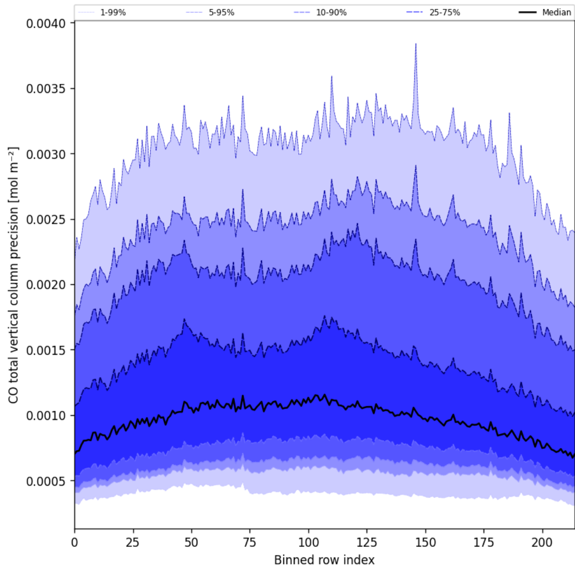
Figure 28: Along track statistics of “CO total vertical column precision” for 2025-07-09 to 2025-07-11
