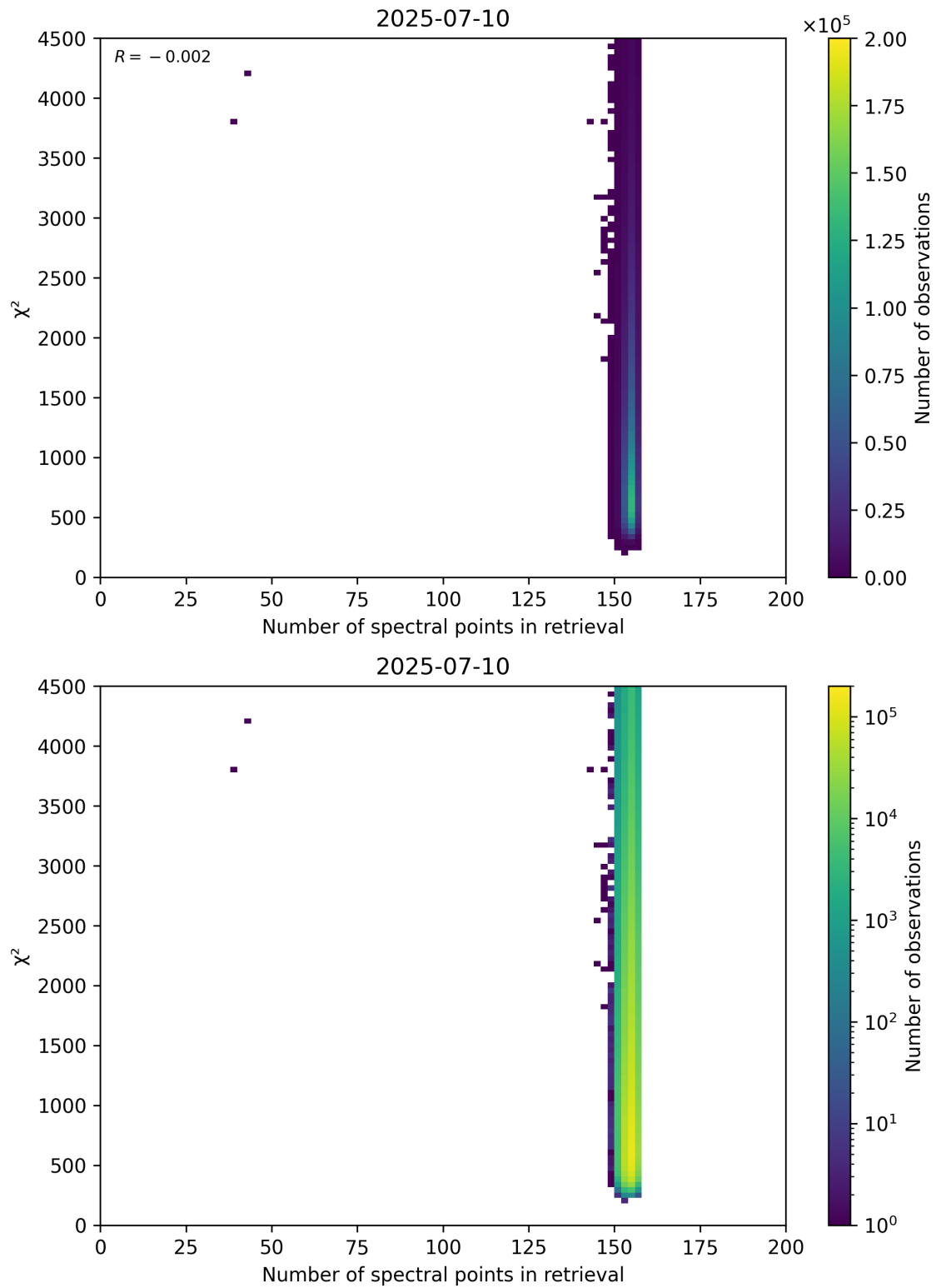
Figure 58: Scatter density plot of “Number of spectral points in retrieval” against “ \chi^2 ” for 2025-07-09 to 2025-07-11.
