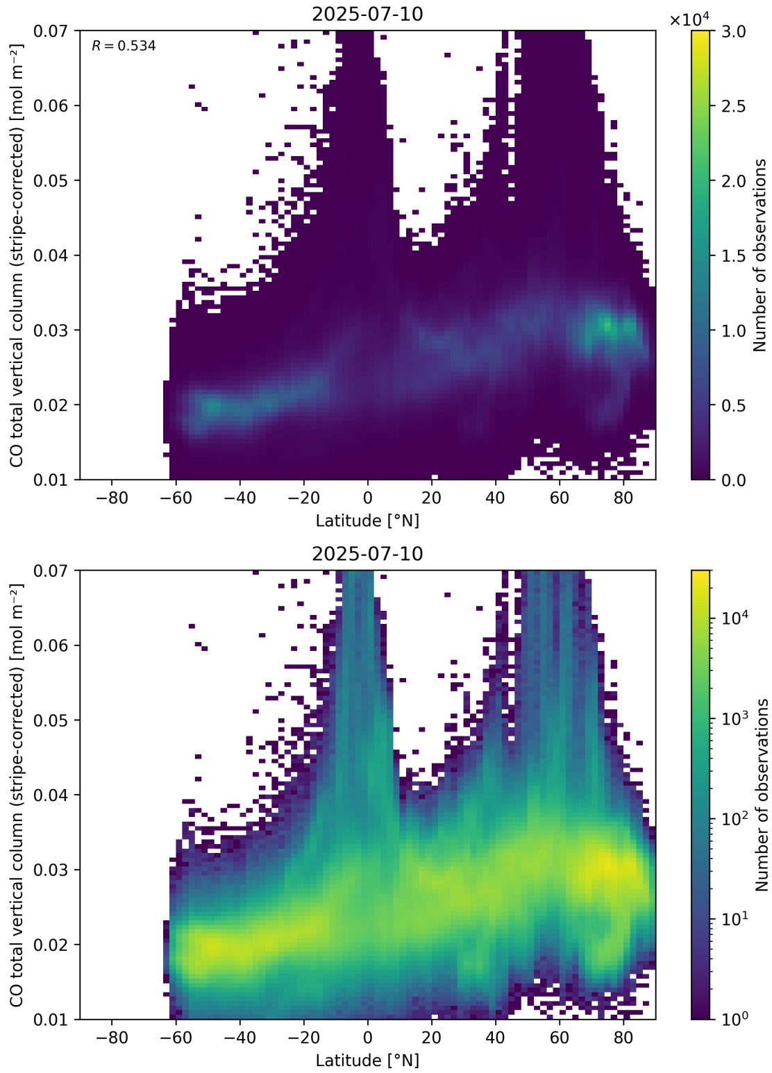
Figure 52: Scatter density plot of “Latitude” against “CO total vertical column (stripe-corrected)” for 2025-07-09 to 2025-07-11.
