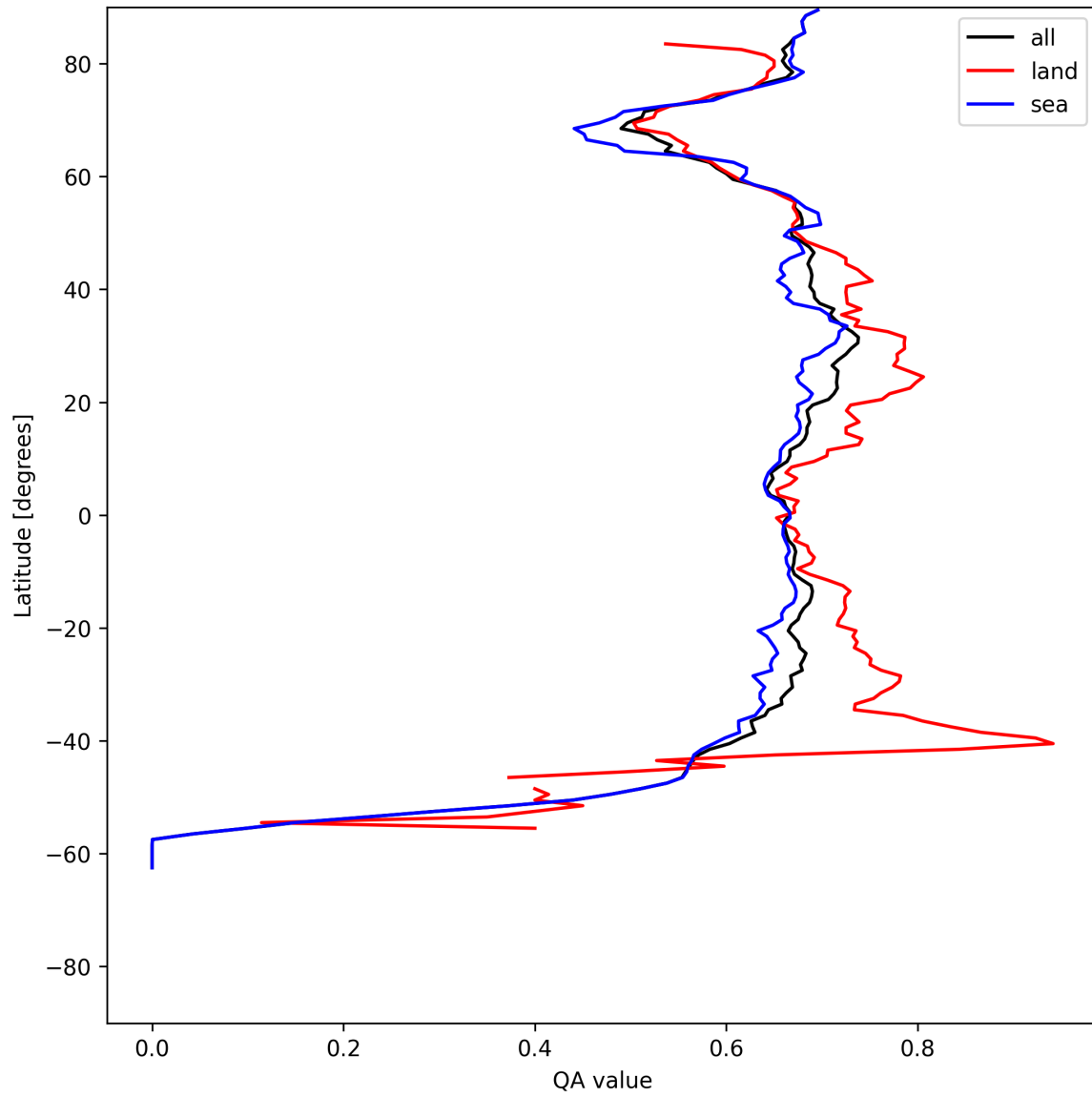
Figure 9: Zonal average of “QA value” for 2025-07-09 to 2025-07-11.
