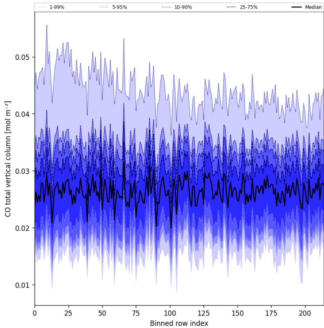
Figure 26: Along track statistics of “CO total vertical column” for 2025-07-09 to 2025-07-11
