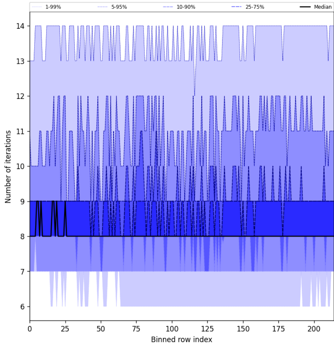
Figure 32: Along track statistics of “Number of iterations” for 2025-07-09 to 2025-07-11
