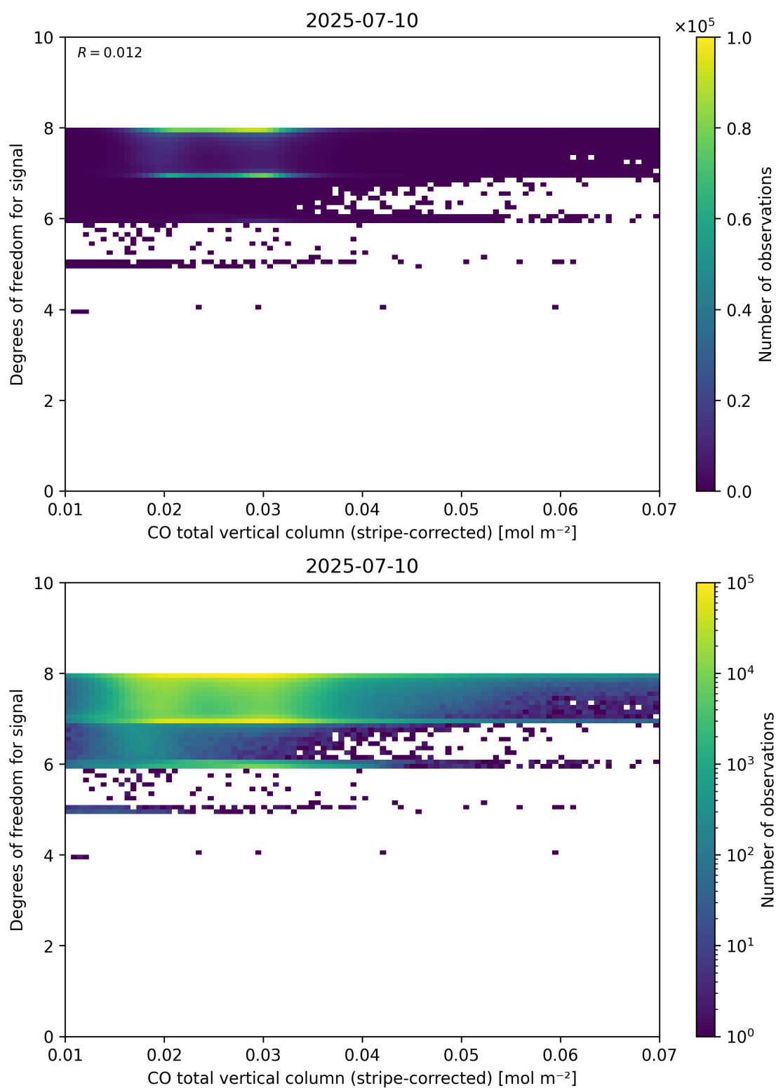
Figure 38: Scatter density plot of “CO total vertical column (stripe-corrected)” against “Degrees of freedom for signal” for 2025-07-09 to 2025-07-11.
