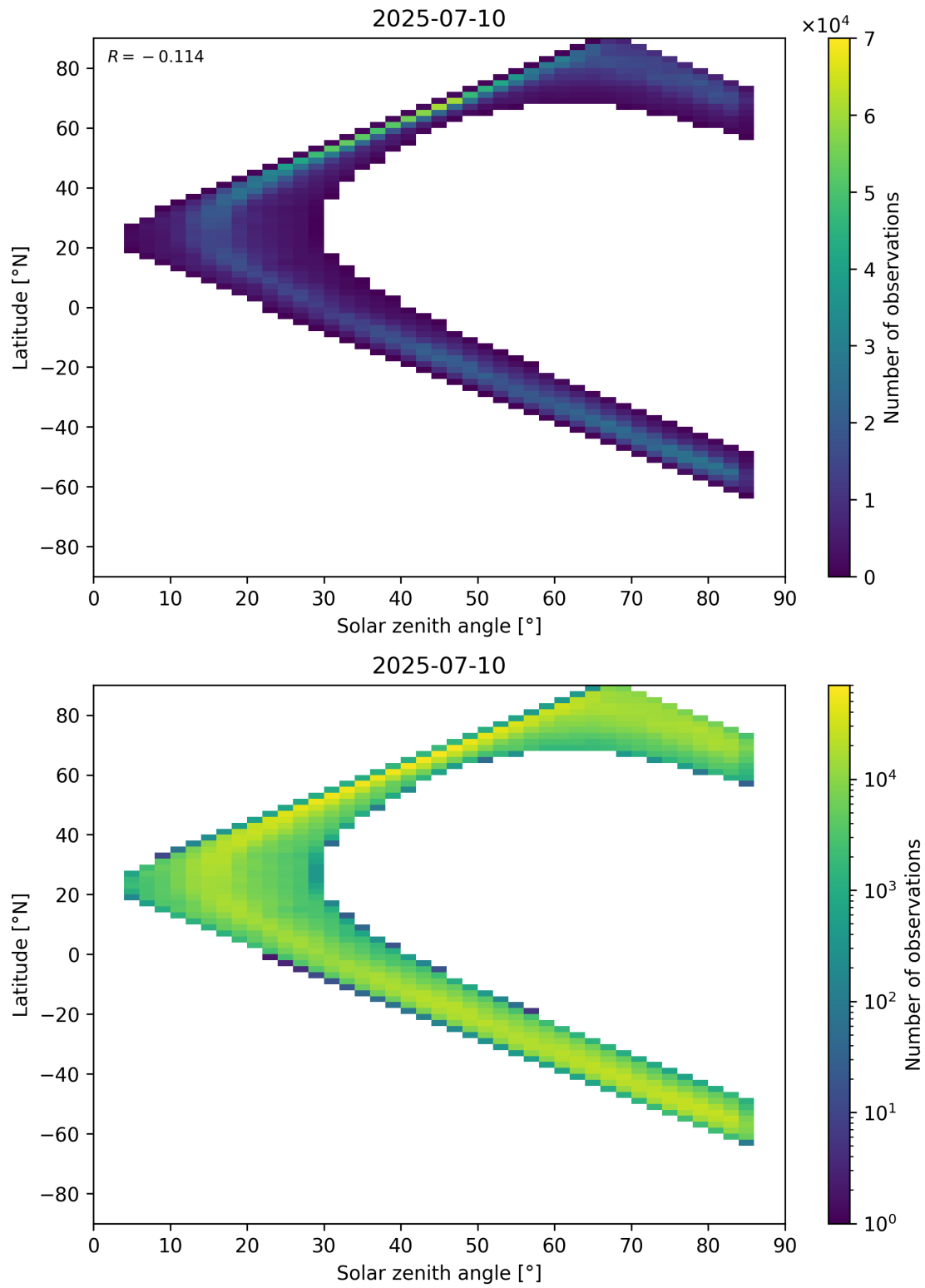
Figure 66: Scatter density plot of “Solar zenith angle” against “Latitude” for 2025-07-09 to 2025-07-11.
