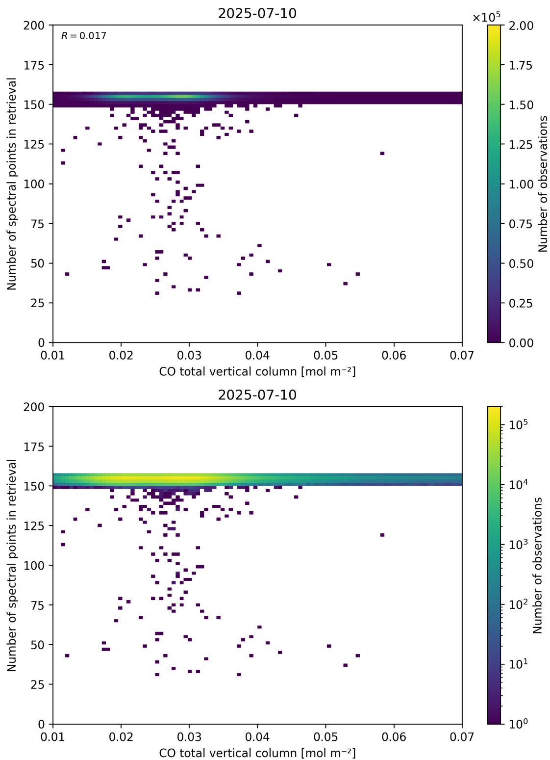
Figure 43: Scatter density plot of “CO total vertical column” against “Number of spectral points in retrieval” for 2025-07-09 to 2025-07-11.
