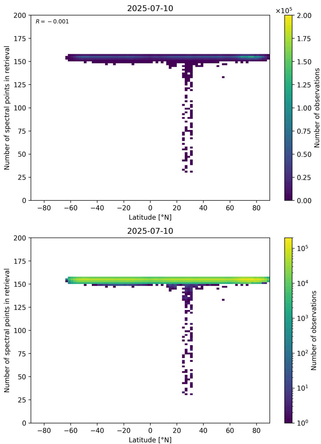
Figure 57: Scatter density plot of “Latitude” against “Number of spectral points in retrieval” for 2025-07-09 to 2025-07-11.
