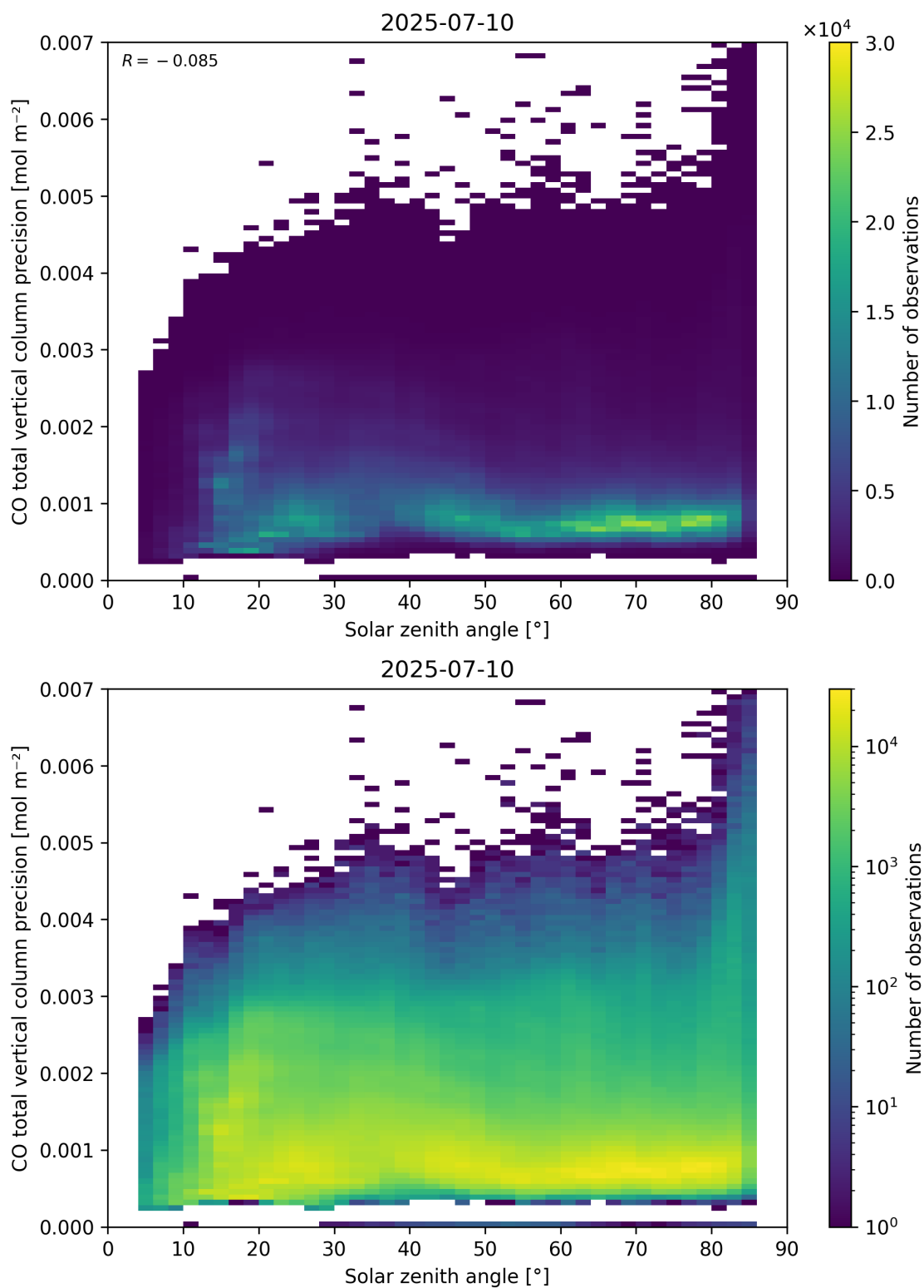
Figure 63: Scatter density plot of “Solar zenith angle” against “CO total vertical column precision” for 2025-07-09 to 2025-07-11.
