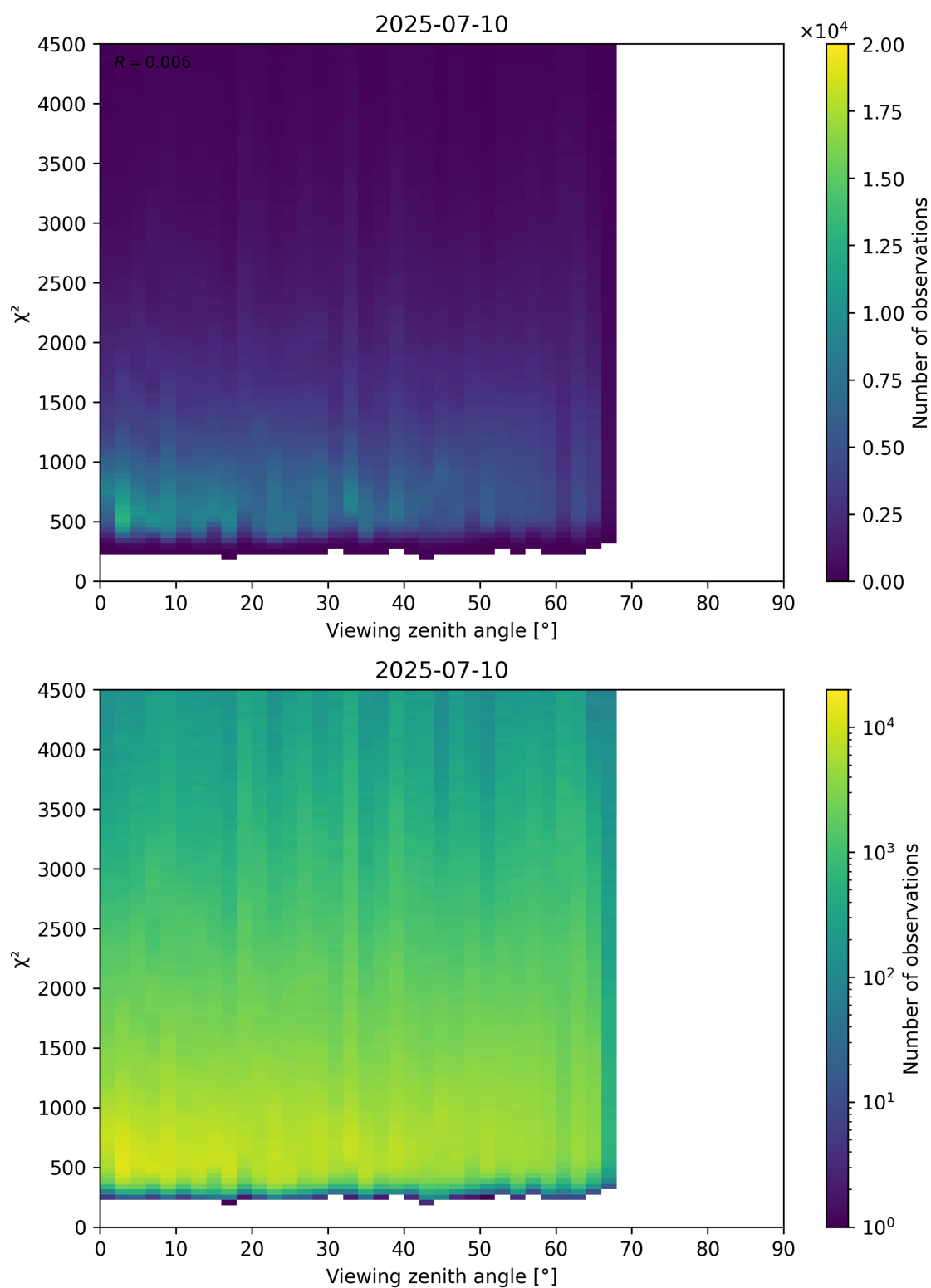
Figure 72: Scatter density plot of “Viewing zenith angle” against “ \chi^2 ” for 2025-07-09 to 2025-07-11.
