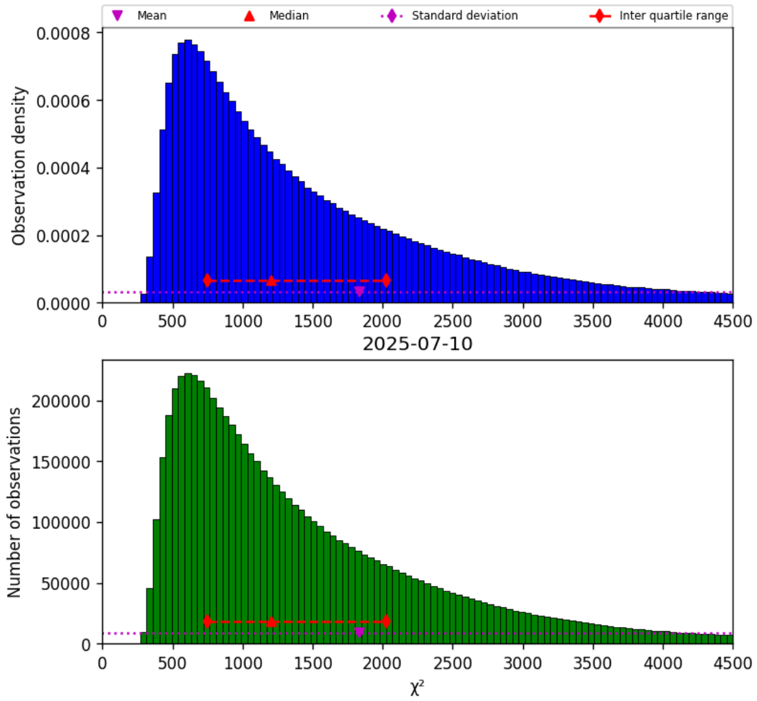
Figure 22: Histogram of “ \chi^2 ” for 2025-07-09 to 2025-07-11
