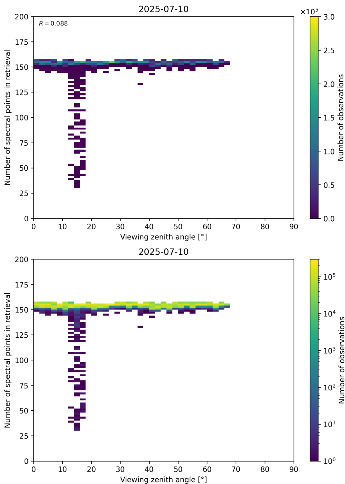
Figure 76: Scatter density plot of “Viewing zenith angle” against “Number of spectral points in retrieval” for 2025-07-09 to 2025-07-11.
