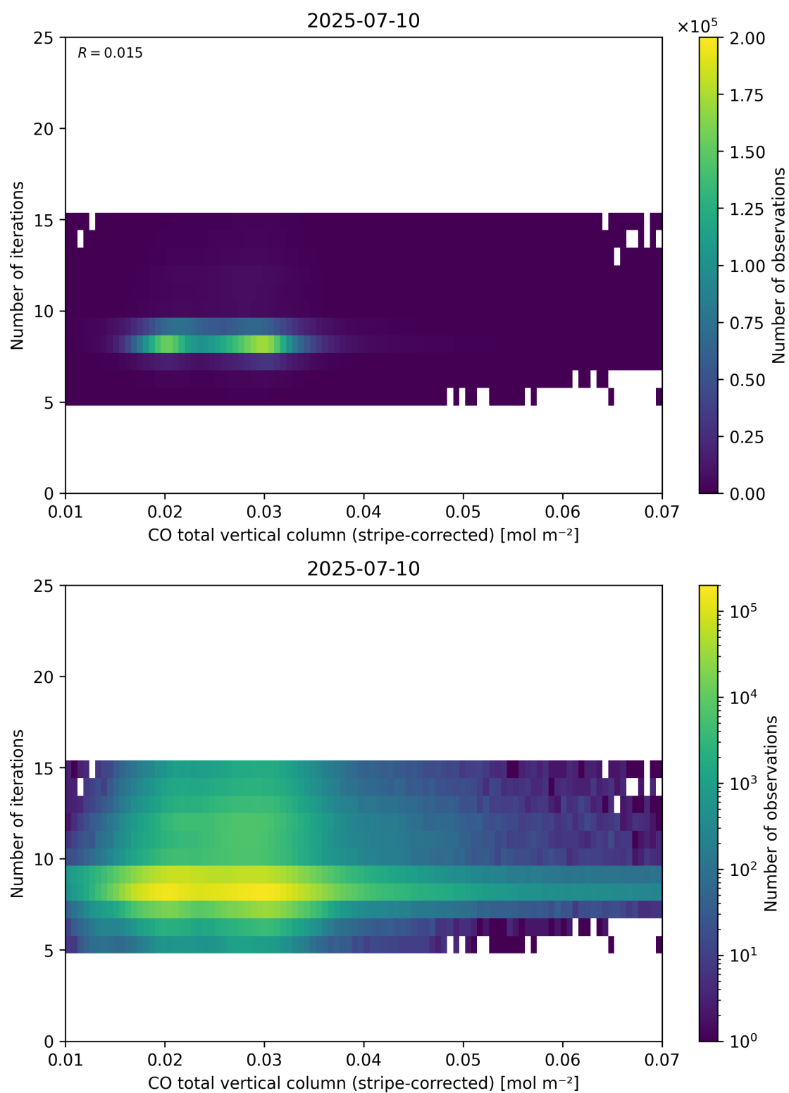
Figure 39: Scatter density plot of “CO total vertical column (stripe-corrected)” against “Number of iterations” for 2025-07-09 to 2025-07-11.
