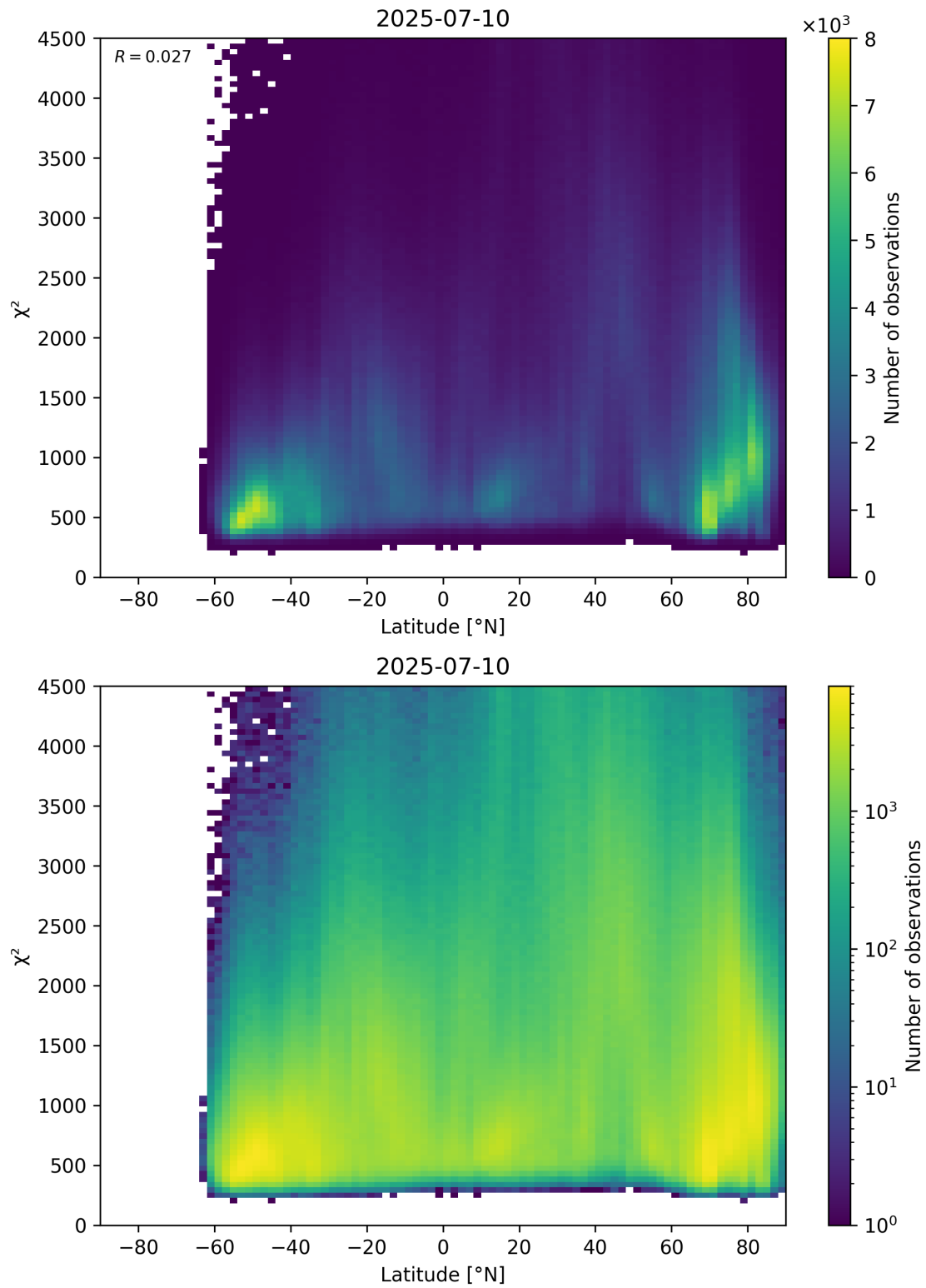
Figure 54: Scatter density plot of “Latitude” against “ \chi^2 ” for 2025-07-09 to 2025-07-11.
