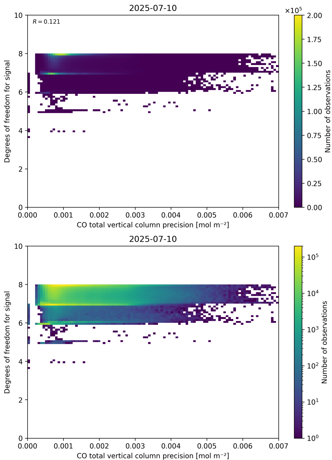
Figure 45: Scatter density plot of “CO total vertical column precision” against “Degrees of freedom for signal” for 2025-07-09 to 2025-07-11.
