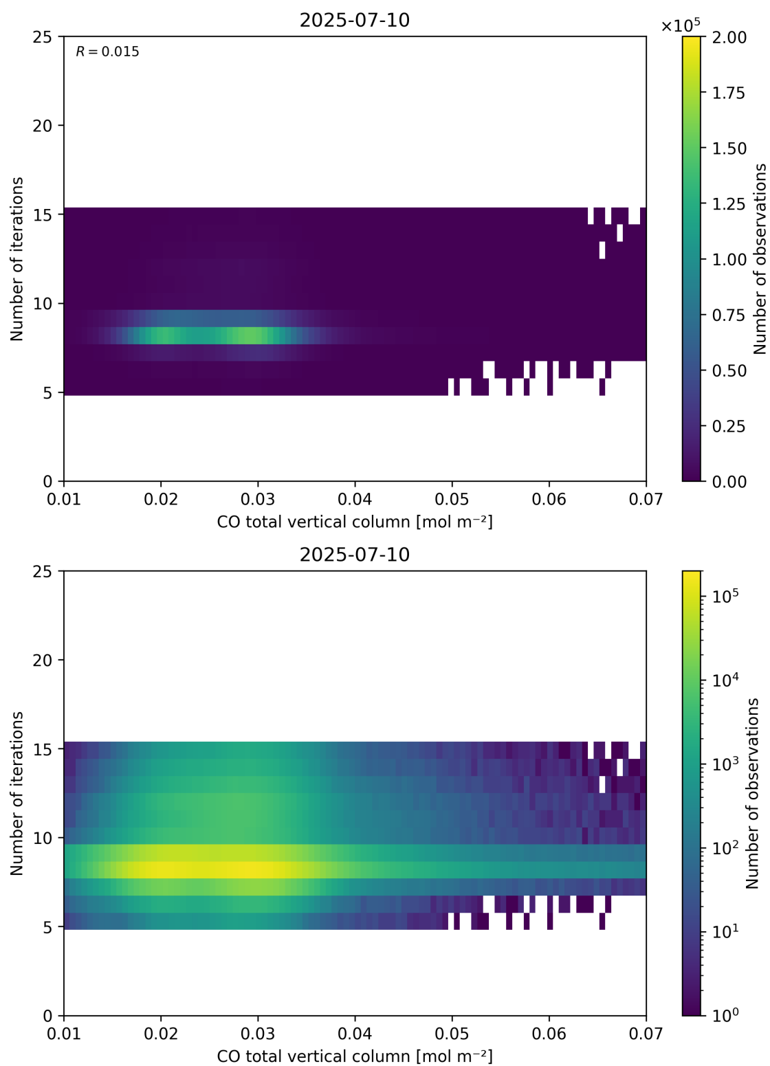
Figure 42: Scatter density plot of “CO total vertical column” against “Number of iterations” for 2025-07-09 to 2025-07-11.
