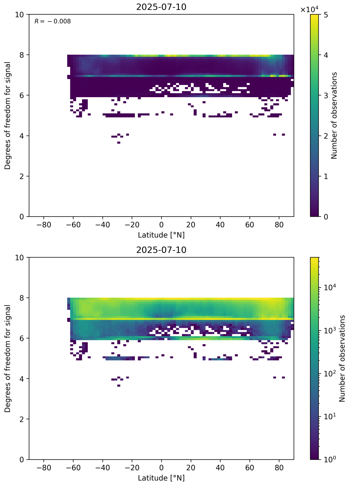
Figure 55: Scatter density plot of “Latitude” against “Degrees of freedom for signal” for 2025-07-09 to 2025-07-11.
