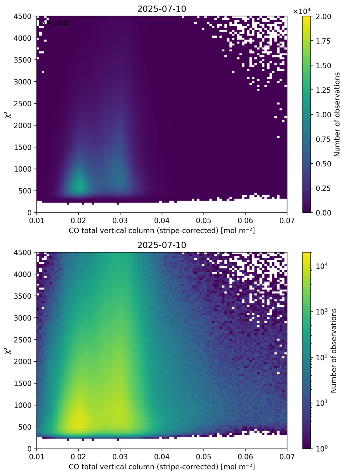
Figure 37: Scatter density plot of “CO total vertical column (stripe-corrected)” against “ \chi^2 ” for 2025-07-09 to 2025-07-11.
