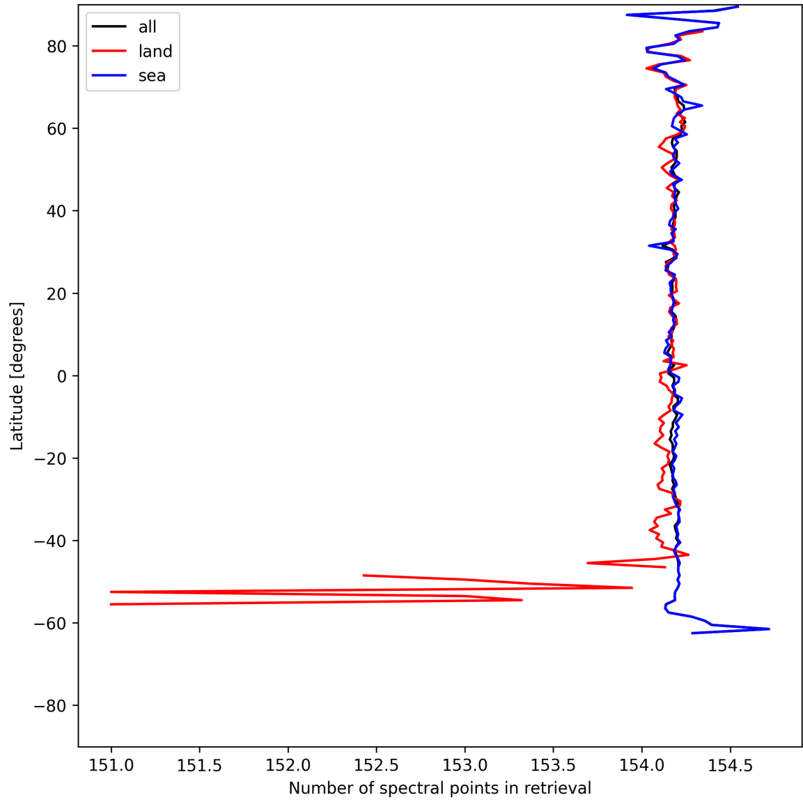
Figure 13: Zonal average of “Number of spectral points in retrieval” for 2025-07-09 to 2025-07-11.
