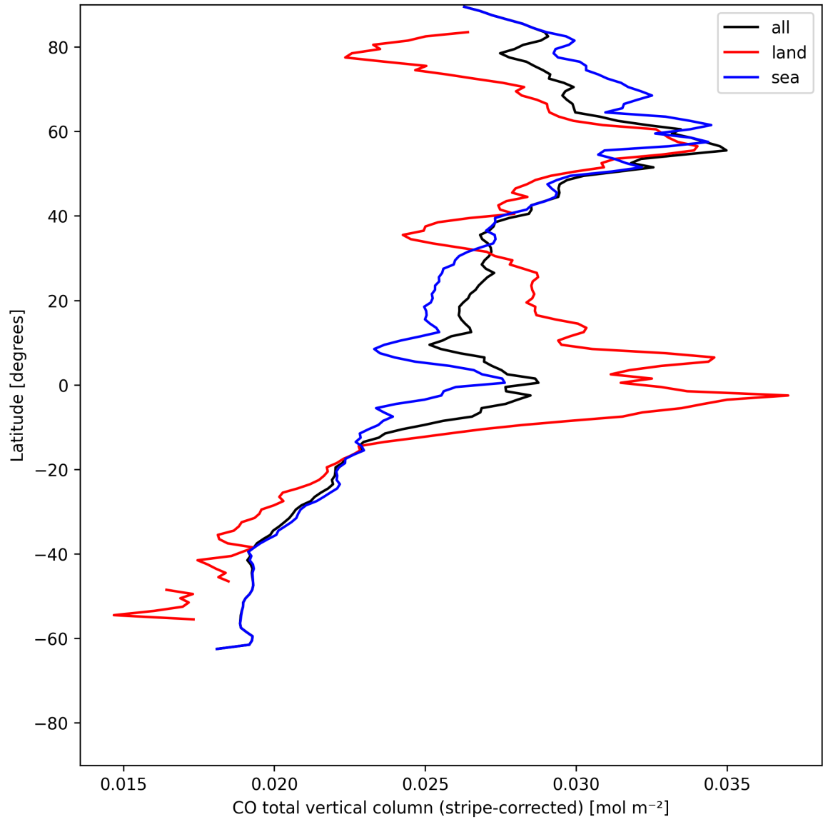
Figure 11: Zonal average of “CO total vertical column (stripe-corrected)” for 2025-07-09 to 2025-07-11.
