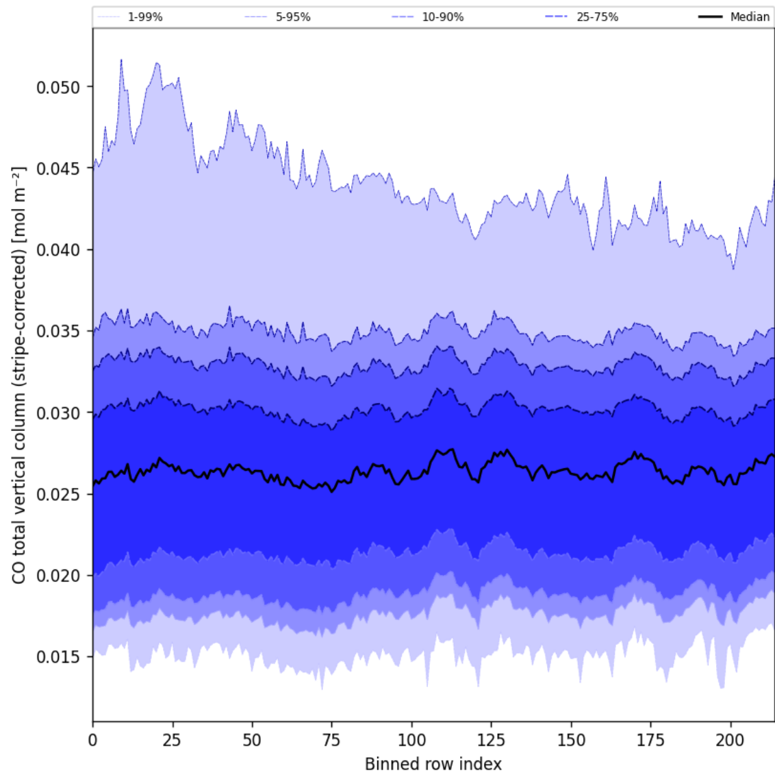
Figure 27: Along track statistics of “CO total vertical column (stripe-corrected)” for 2025-07-09 to 2025-07-11
