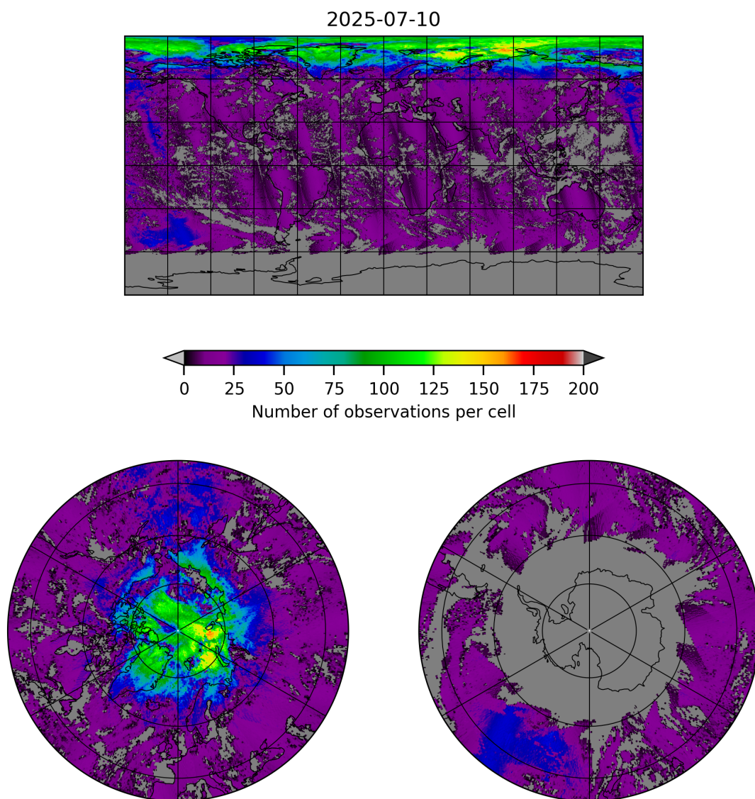
Figure 8: Map of the number of observations for 2025-07-09 to 2025-07-11
