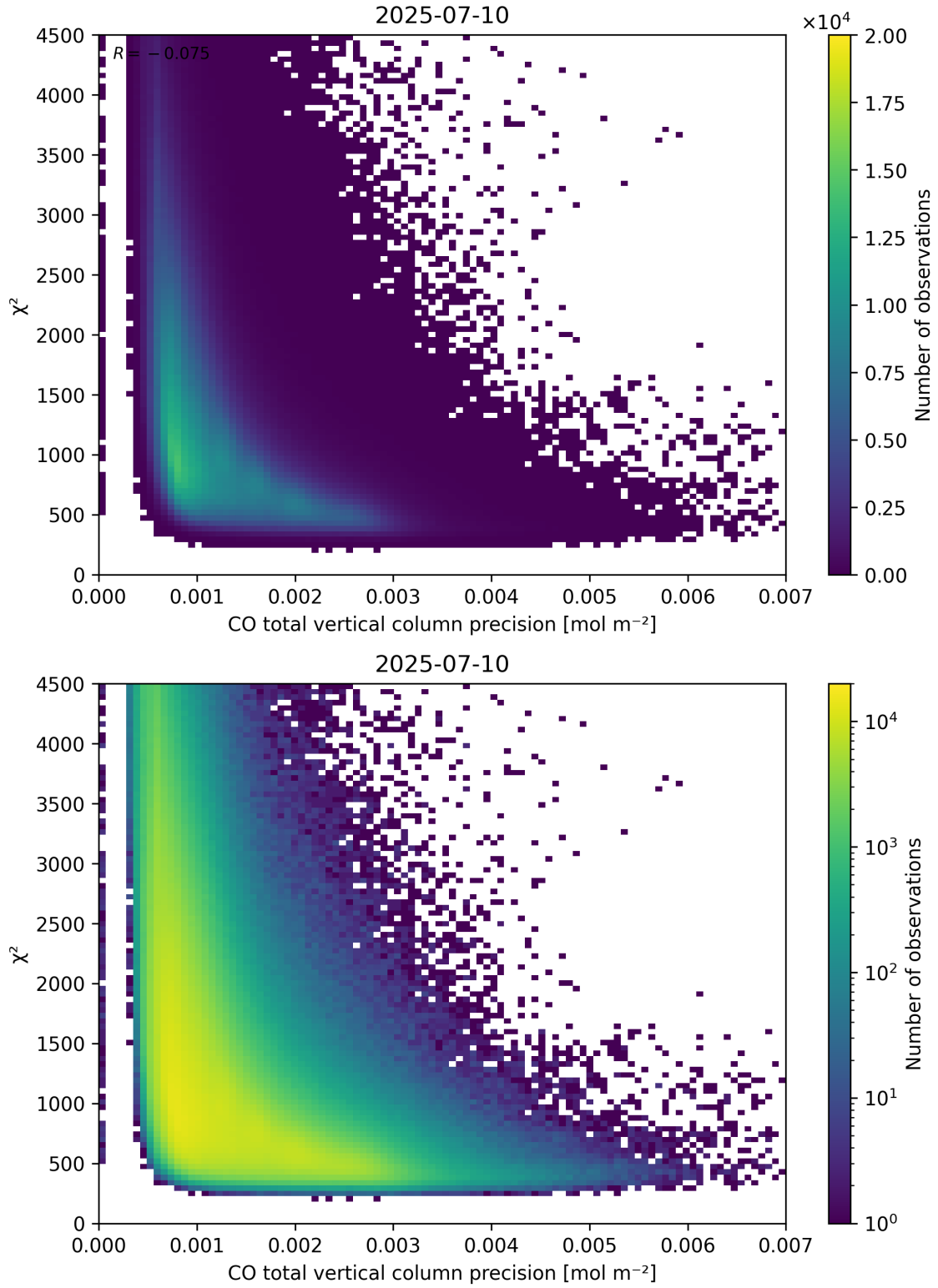
Figure 44: Scatter density plot of “CO total vertical column precision” against “ \chi^2 ” for 2025-07-09 to 2025-07-11.
