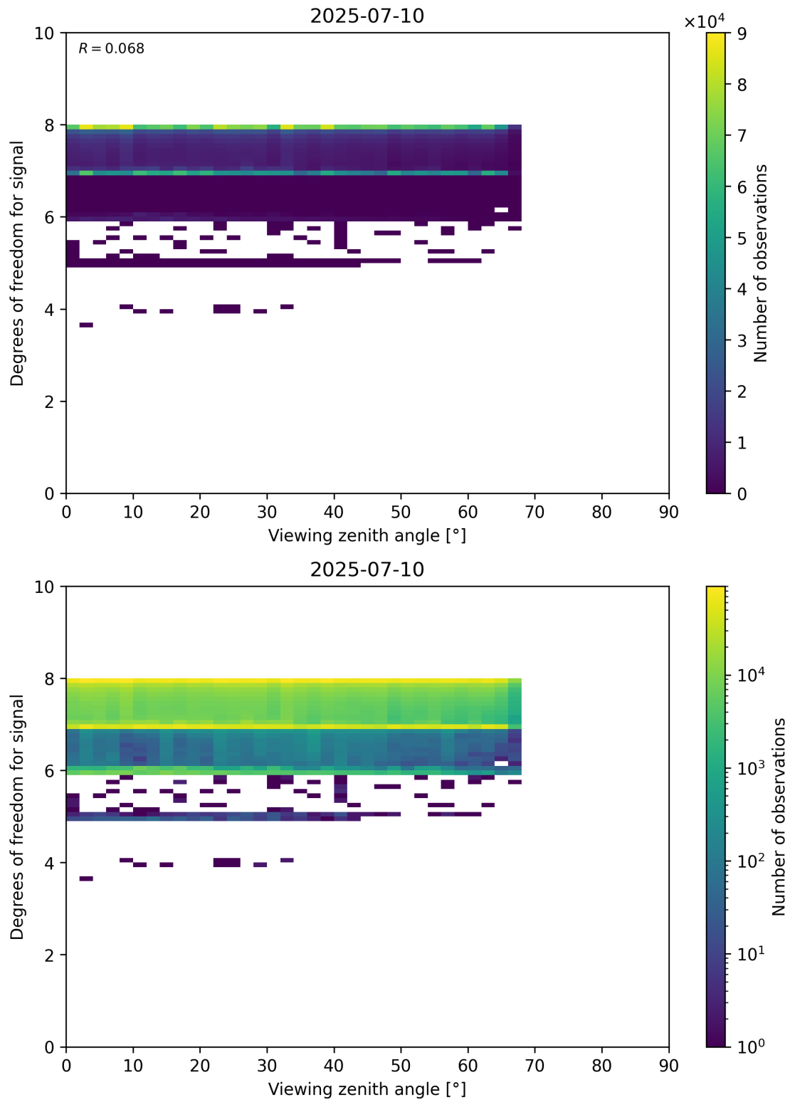
Figure 73: Scatter density plot of “Viewing zenith angle” against “Degrees of freedom for signal” for 2025-07-09 to 2025-07-11.
