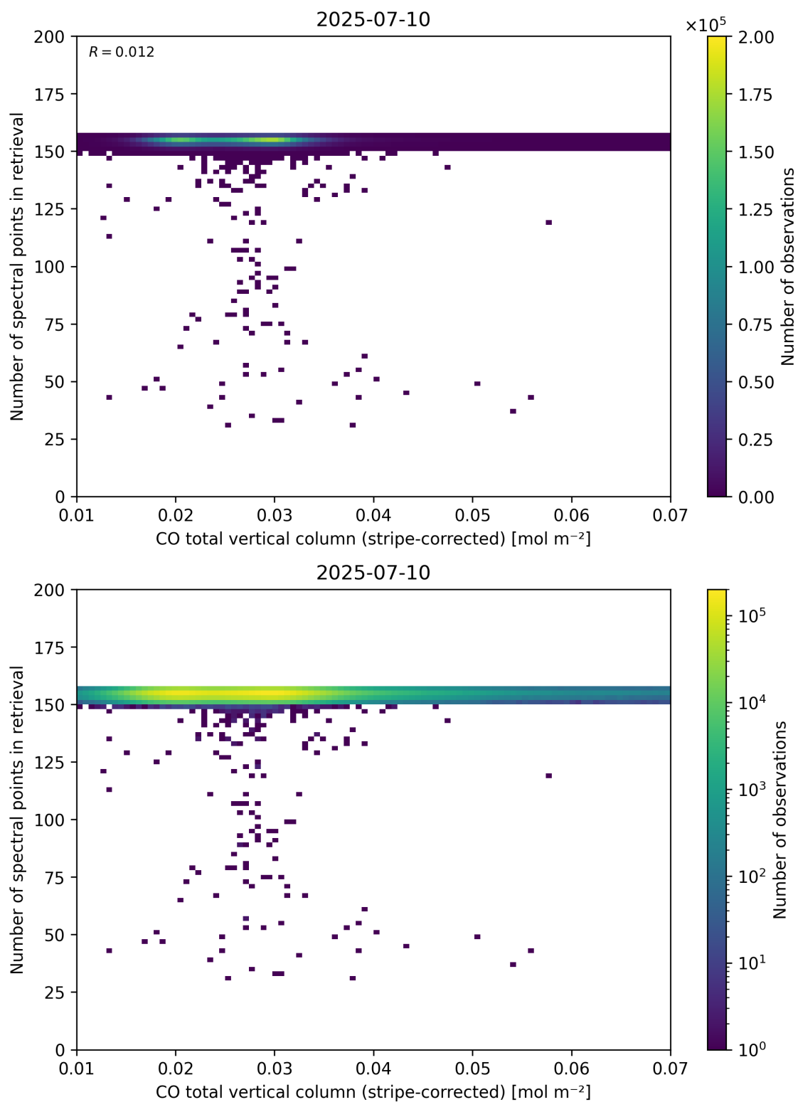
Figure 40: Scatter density plot of “CO total vertical column (stripe-corrected)” against “Number of spectral points in retrieval” for 2025-07-09 to 2025-07-11.
