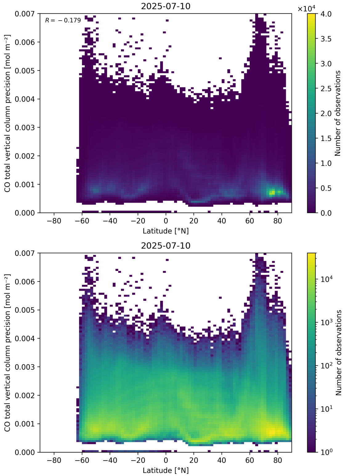
Figure 53: Scatter density plot of “Latitude” against “CO total vertical column precision” for 2025-07-09 to 2025-07-11.
