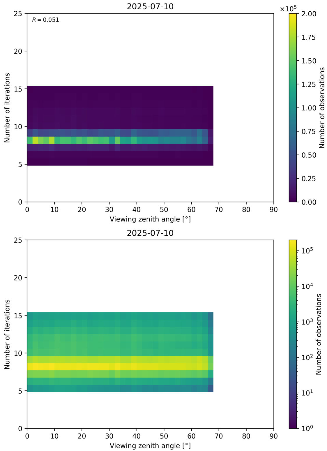
Figure 75: Scatter density plot of “Viewing zenith angle” against “Number of iterations” for 2025-07-09 to 2025-07-11.
