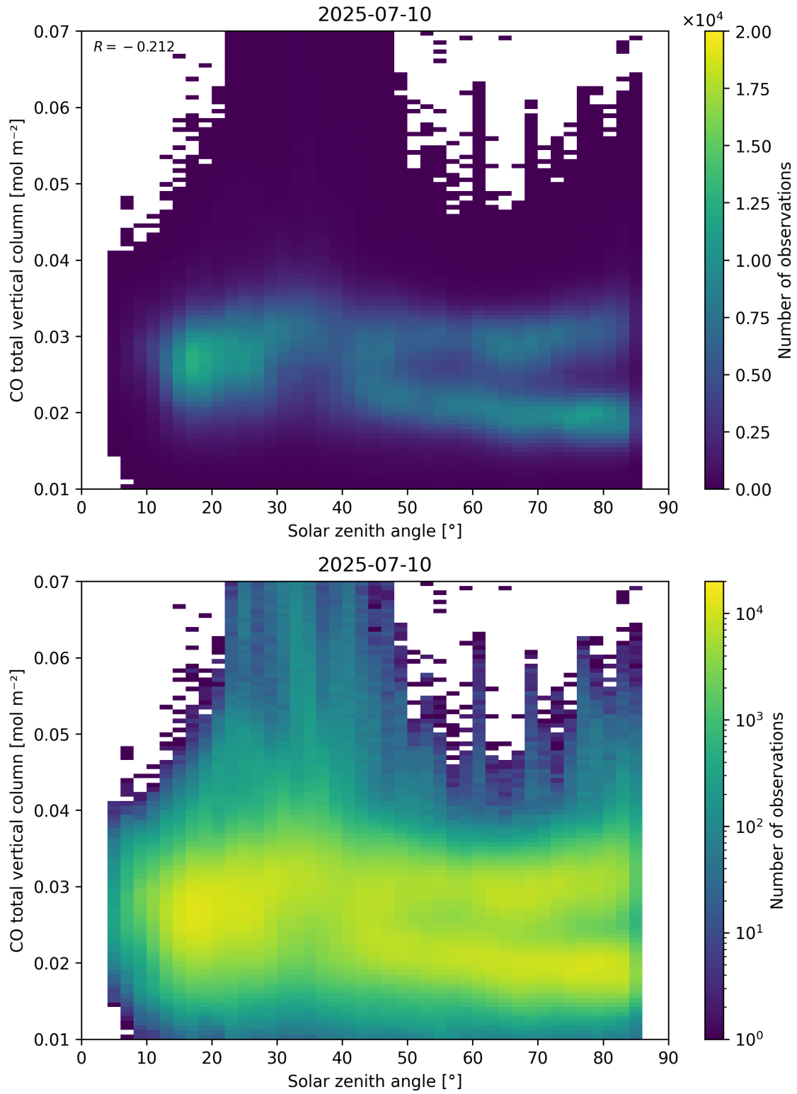
Figure 61: Scatter density plot of “Solar zenith angle” against “CO total vertical column” for 2025-07-09 to 2025-07-11.
