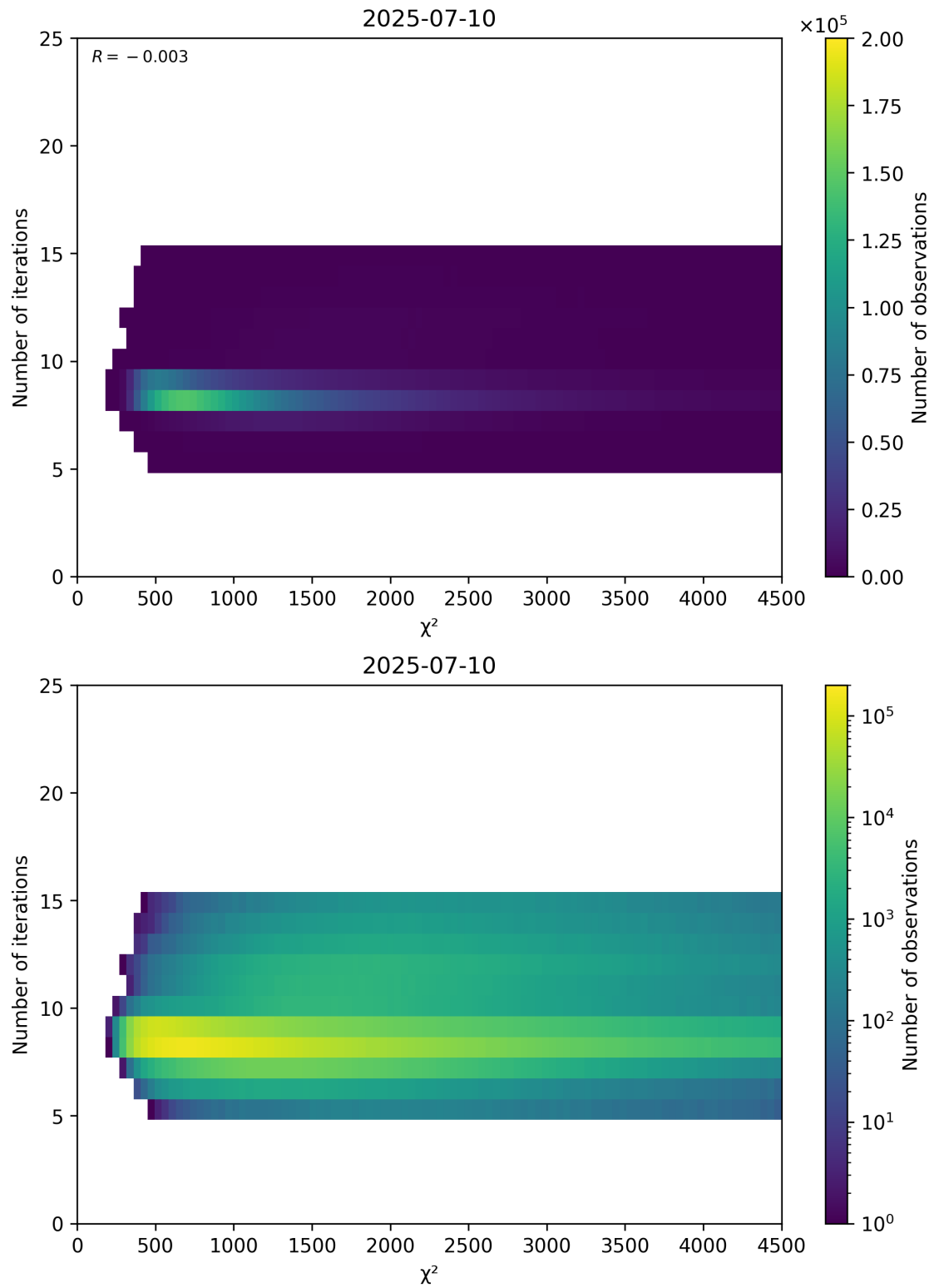
Figure 49: Scatter density plot of “ \chi^2 ” against “Number of iterations” for 2025-07-09 to 2025-07-11.
