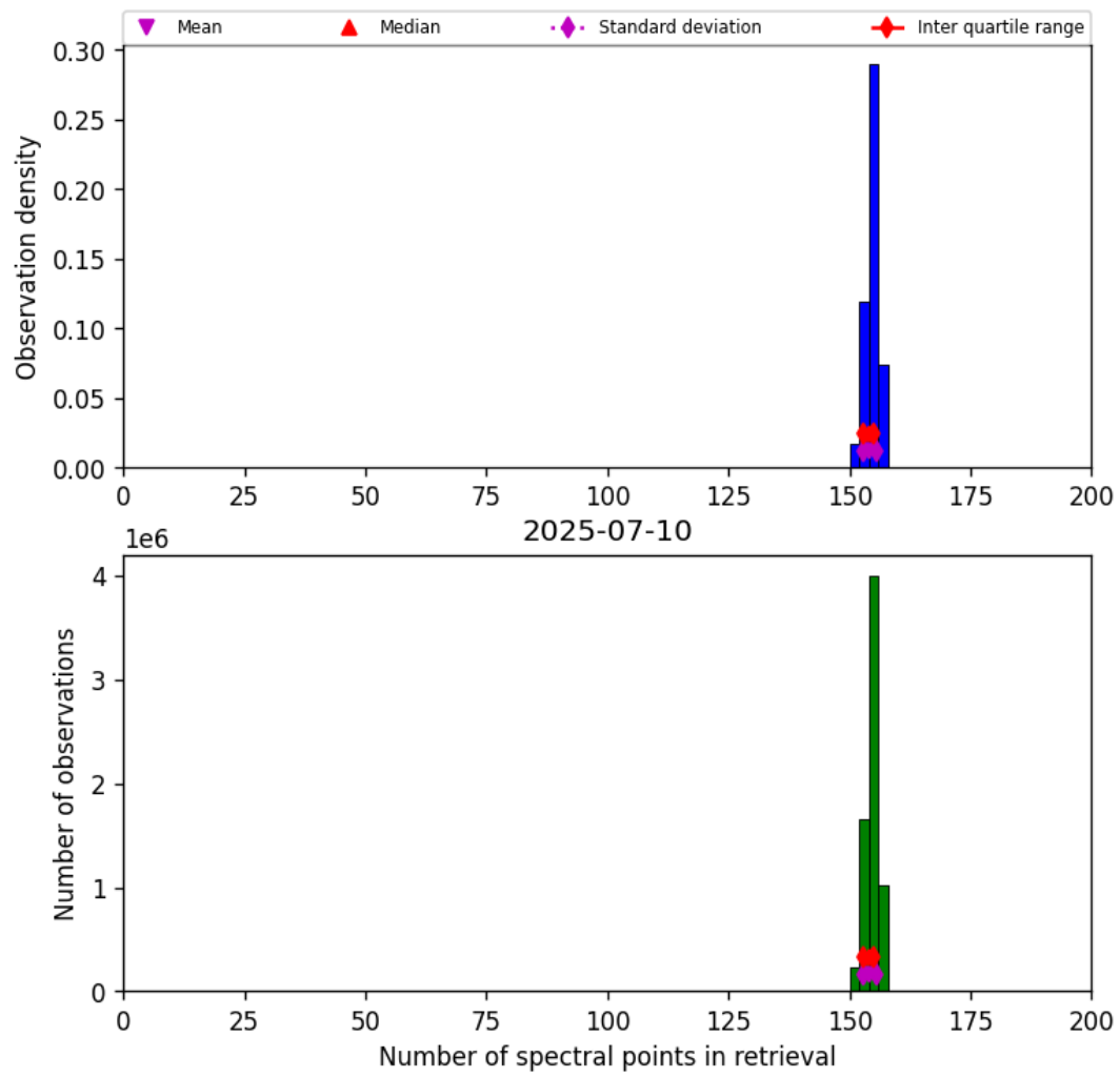
Figure 21: Histogram of “Number of spectral points in retrieval” for 2025-07-09 to 2025-07-11
