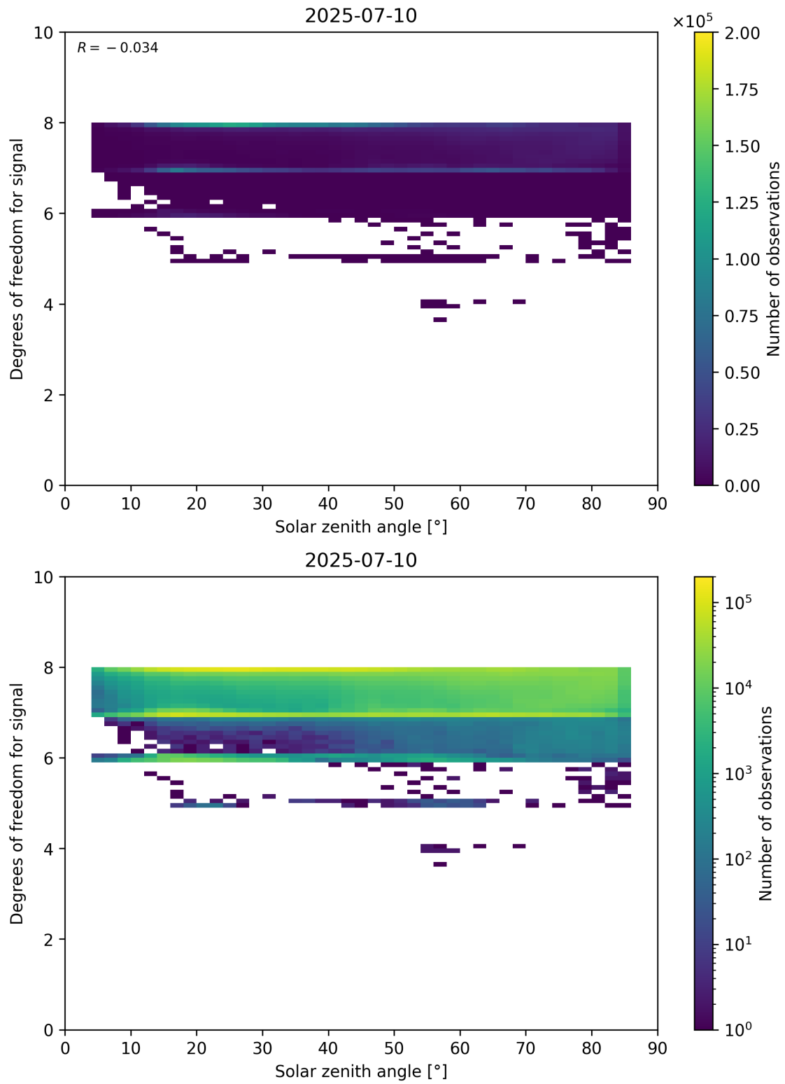
Figure 65: Scatter density plot of “Solar zenith angle” against “Degrees of freedom for signal” for 2025-07-09 to 2025-07-11.
