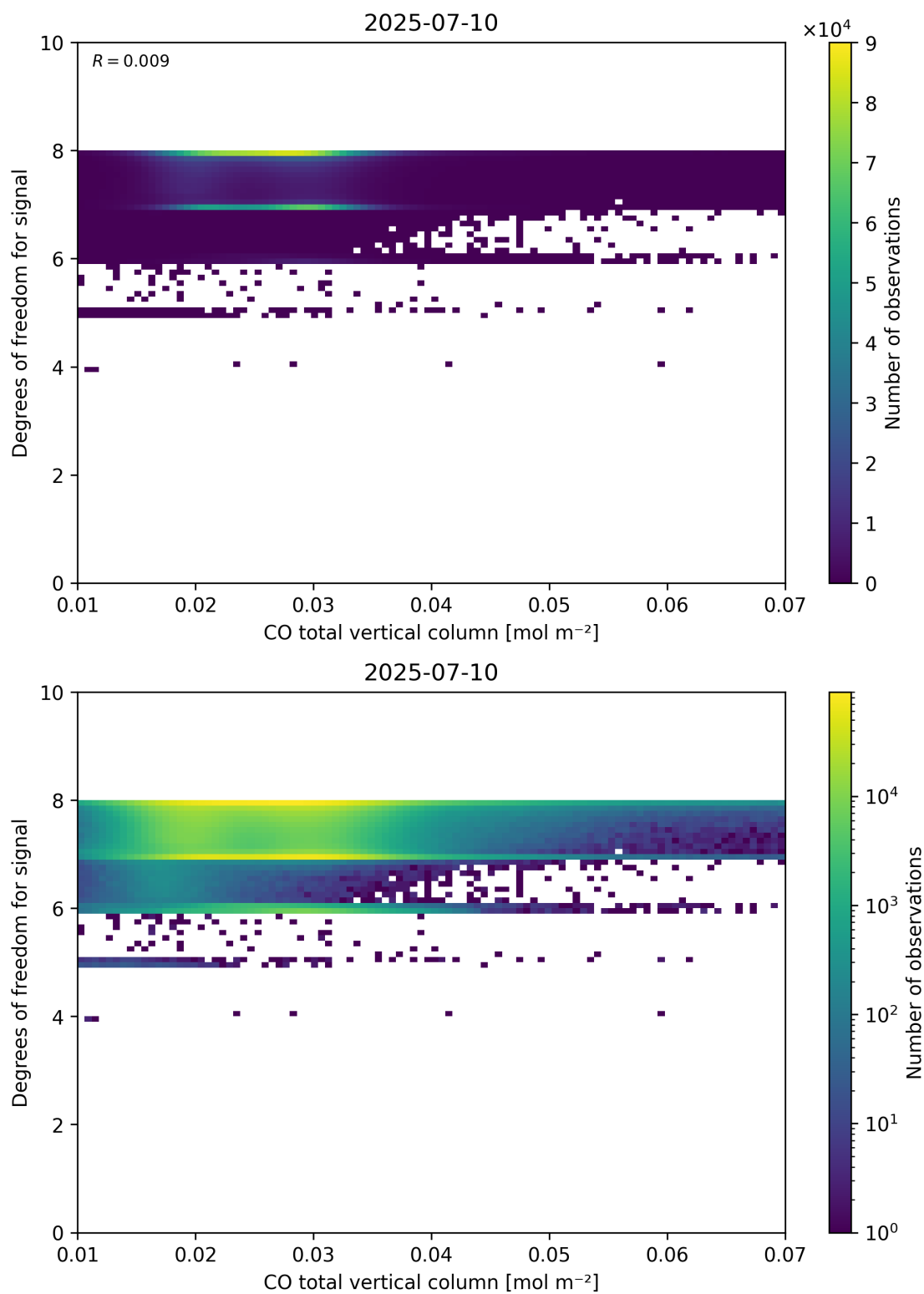
Figure 41: Scatter density plot of “CO total vertical column” against “Degrees of freedom for signal” for 2025-07-09 to 2025-07-11.
