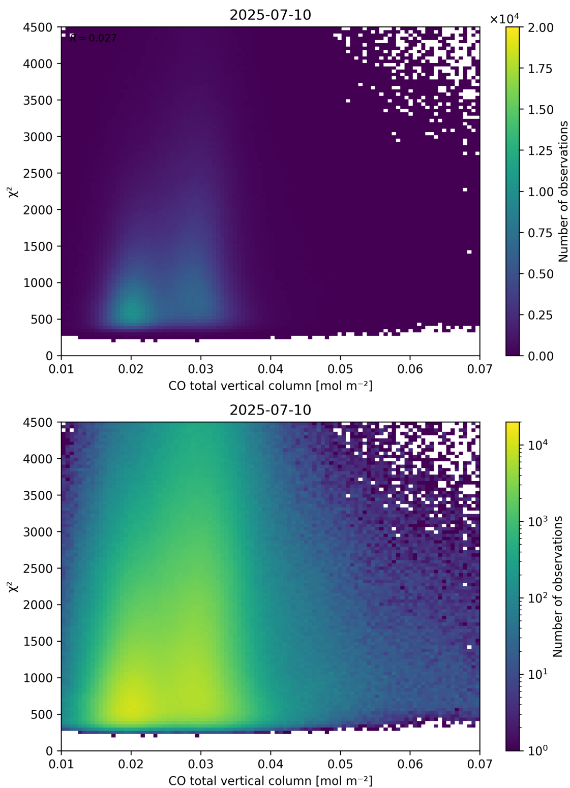
Figure 35: Scatter density plot of “CO total vertical column” against “ \chi^2 ” for 2025-07-09 to 2025-07-11.
