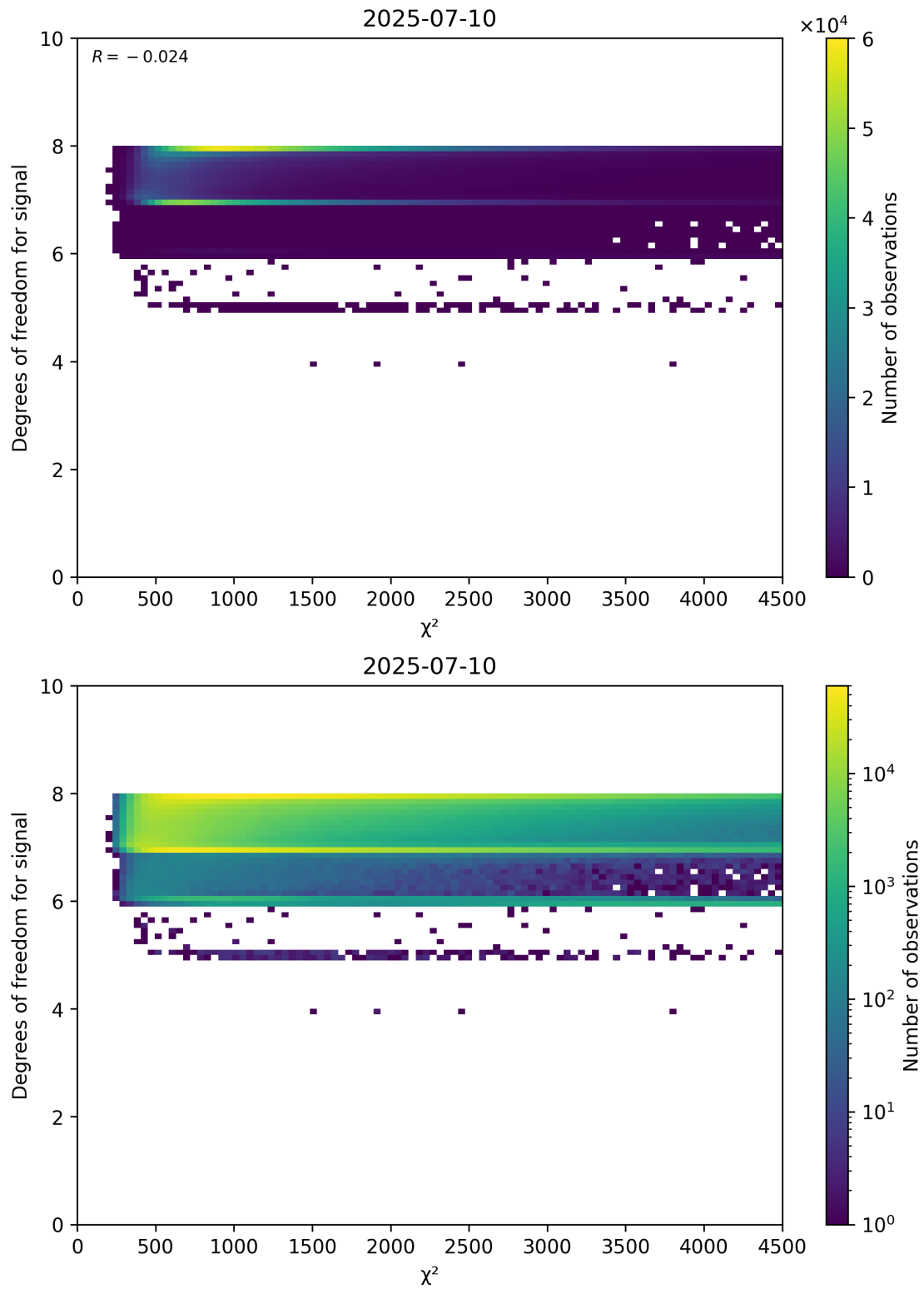
Figure 48: Scatter density plot of “ \chi^2 ” against “Degrees of freedom for signal” for 2025-07-09 to 2025-07-11.
