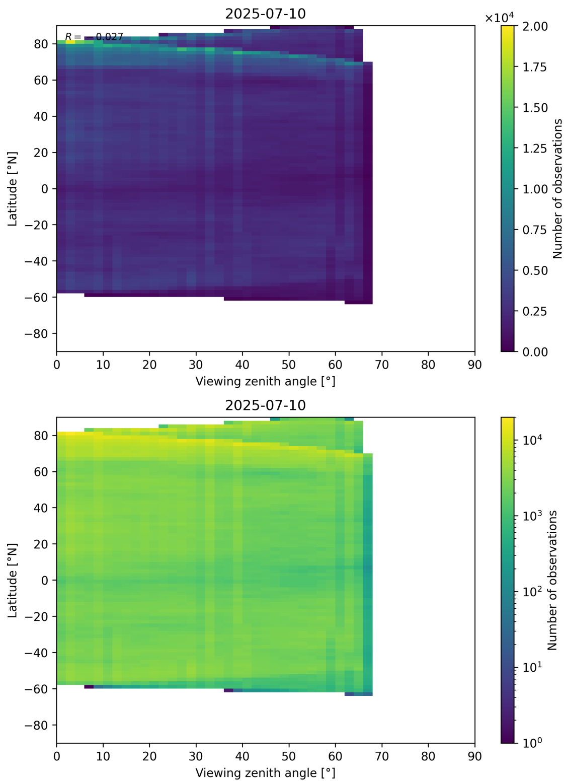
Figure 74: Scatter density plot of “Viewing zenith angle” against “Latitude” for 2025-07-09 to 2025-07-11.
