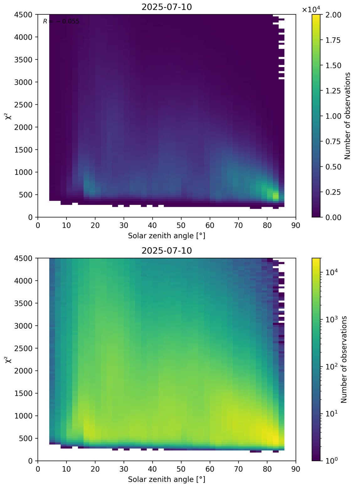
Figure 64: Scatter density plot of “Solar zenith angle” against “ \chi^2 ” for 2025-07-09 to 2025-07-11.
