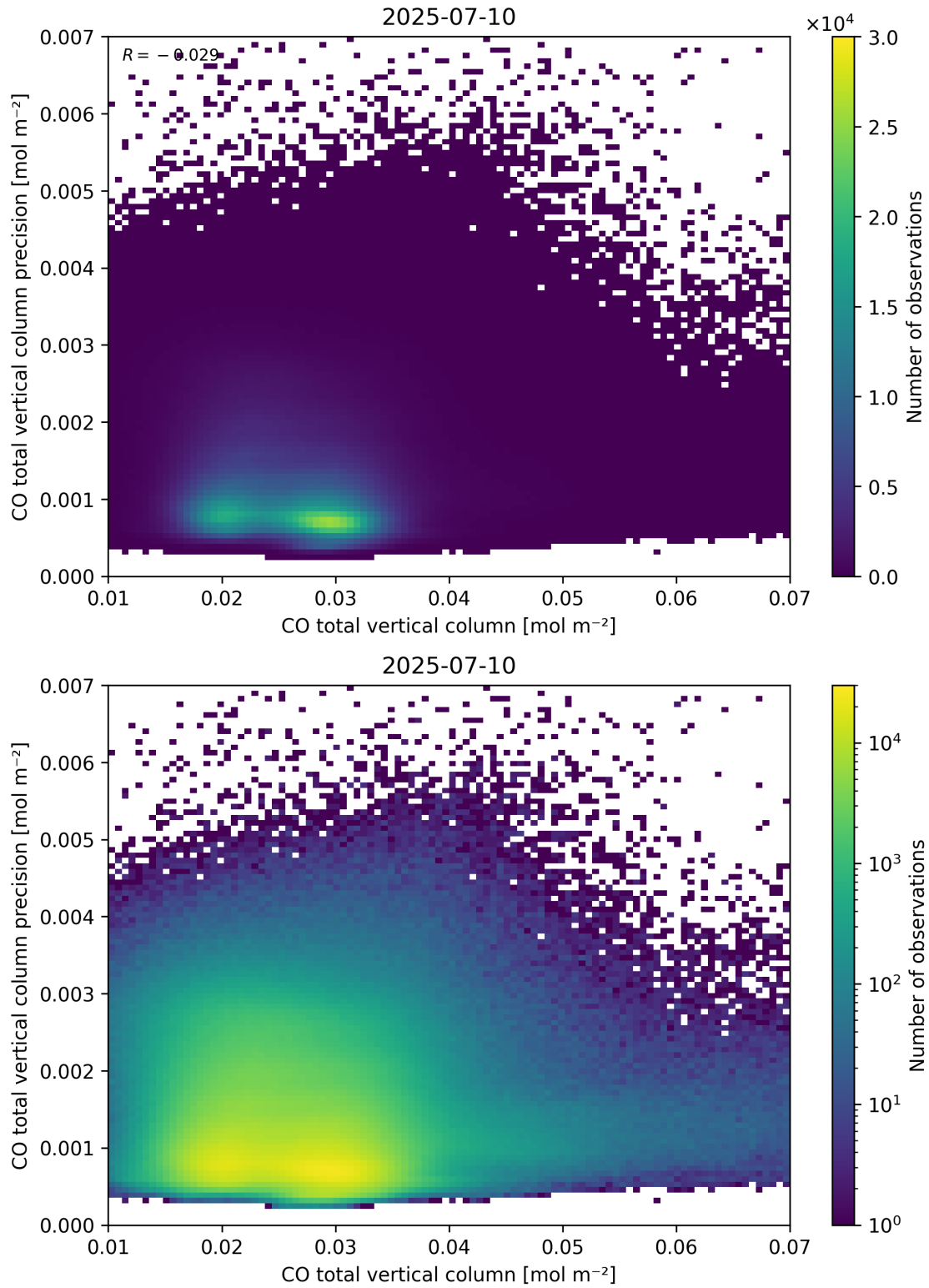
Figure 34: Scatter density plot of “CO total vertical column” against “CO total vertical column precision” for 2025-07-09 to 2025-07-11.
