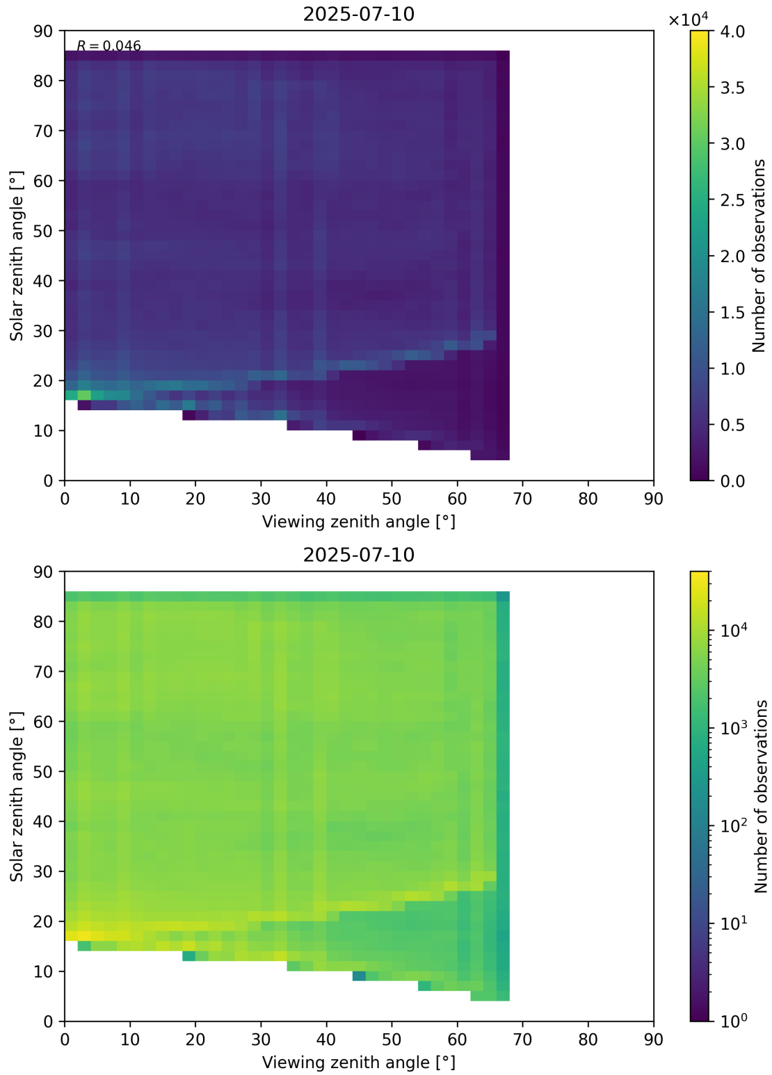
Figure 77: Scatter density plot of “Viewing zenith angle” against “Solar zenith angle” for 2025-07-09 to 2025-07-11.
