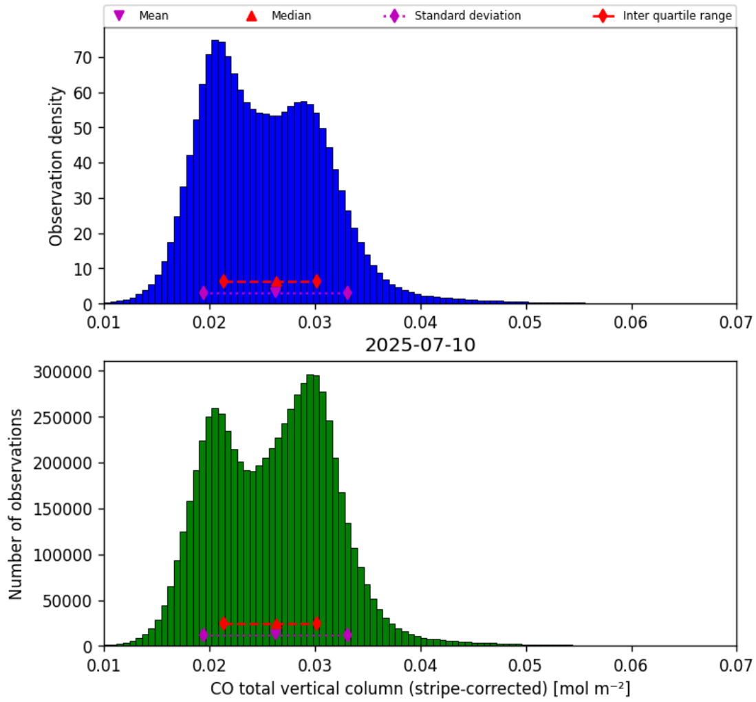
Figure 19: Histogram of “CO total vertical column (stripe-corrected)” for 2025-07-09 to 2025-07-11
