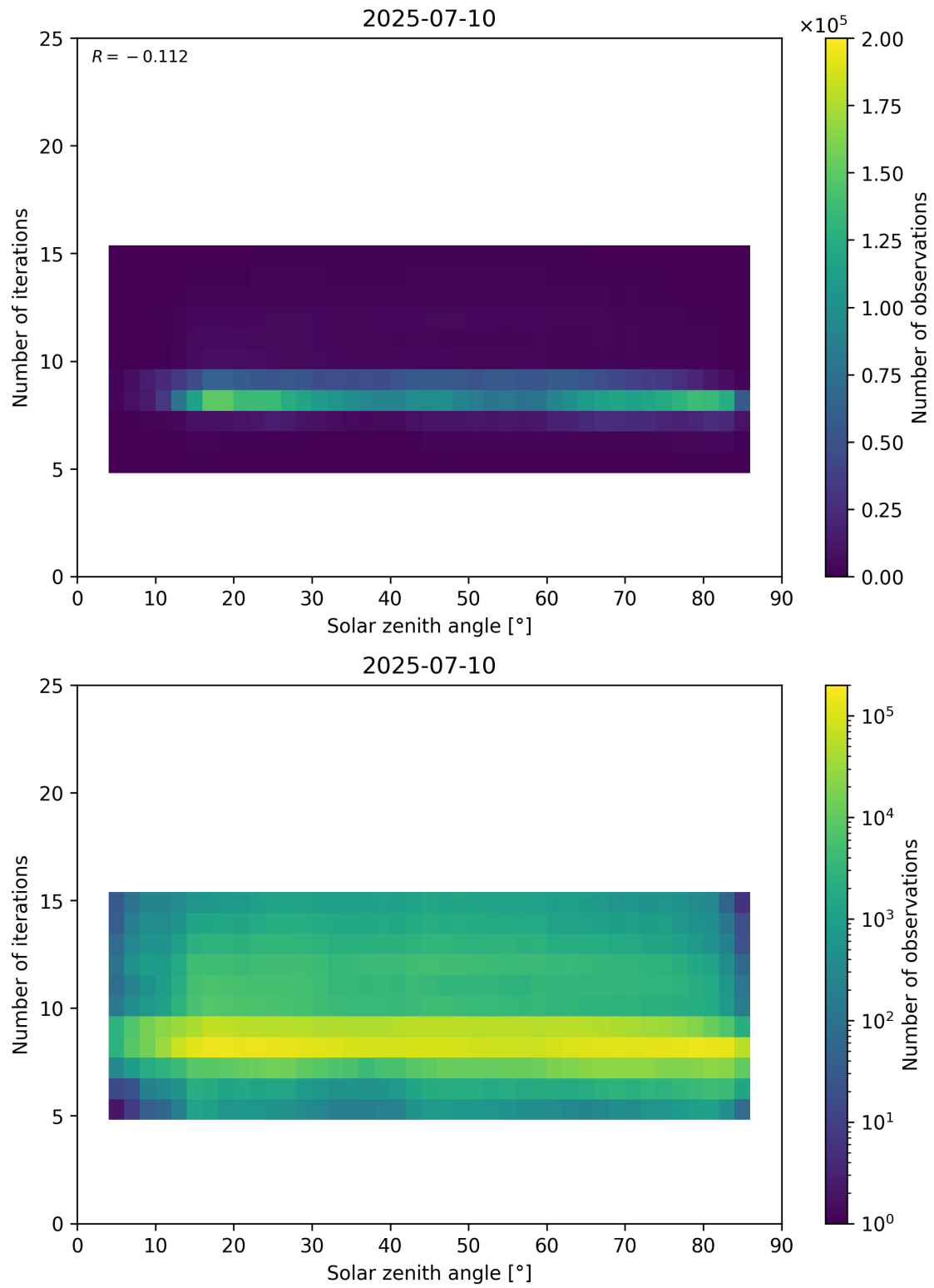
Figure 67: Scatter density plot of “Solar zenith angle” against “Number of iterations” for 2025-07-09 to 2025-07-11.
