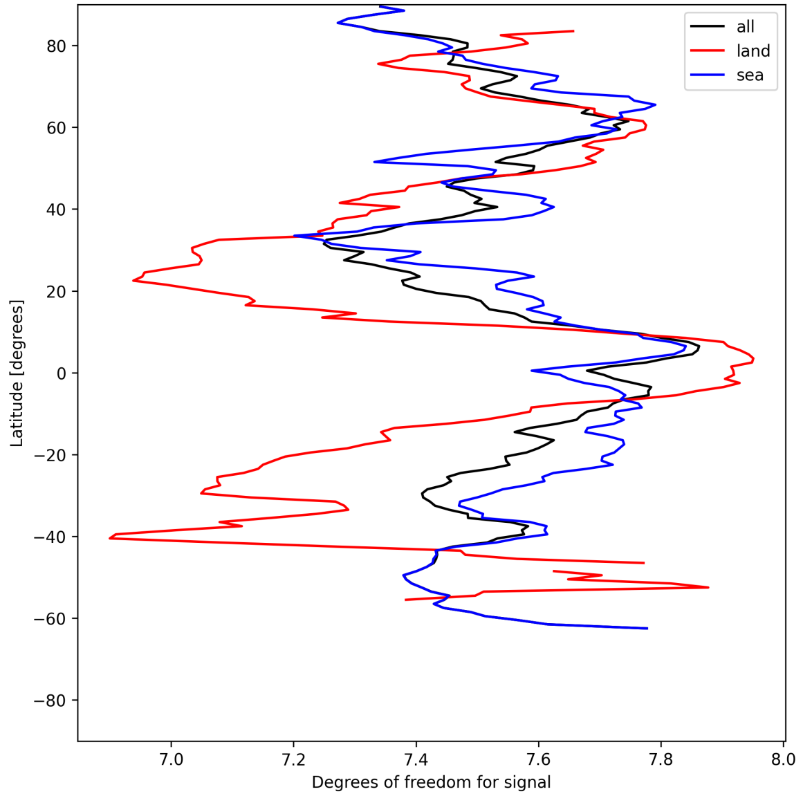
Figure 15: Zonal average of “Degrees of freedom for signal” for 2025-07-09 to 2025-07-11.
