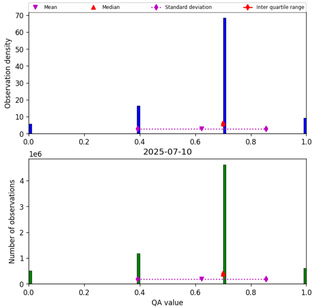
Figure 17: Histogram of “QA value” for 2025-07-09 to 2025-07-11
