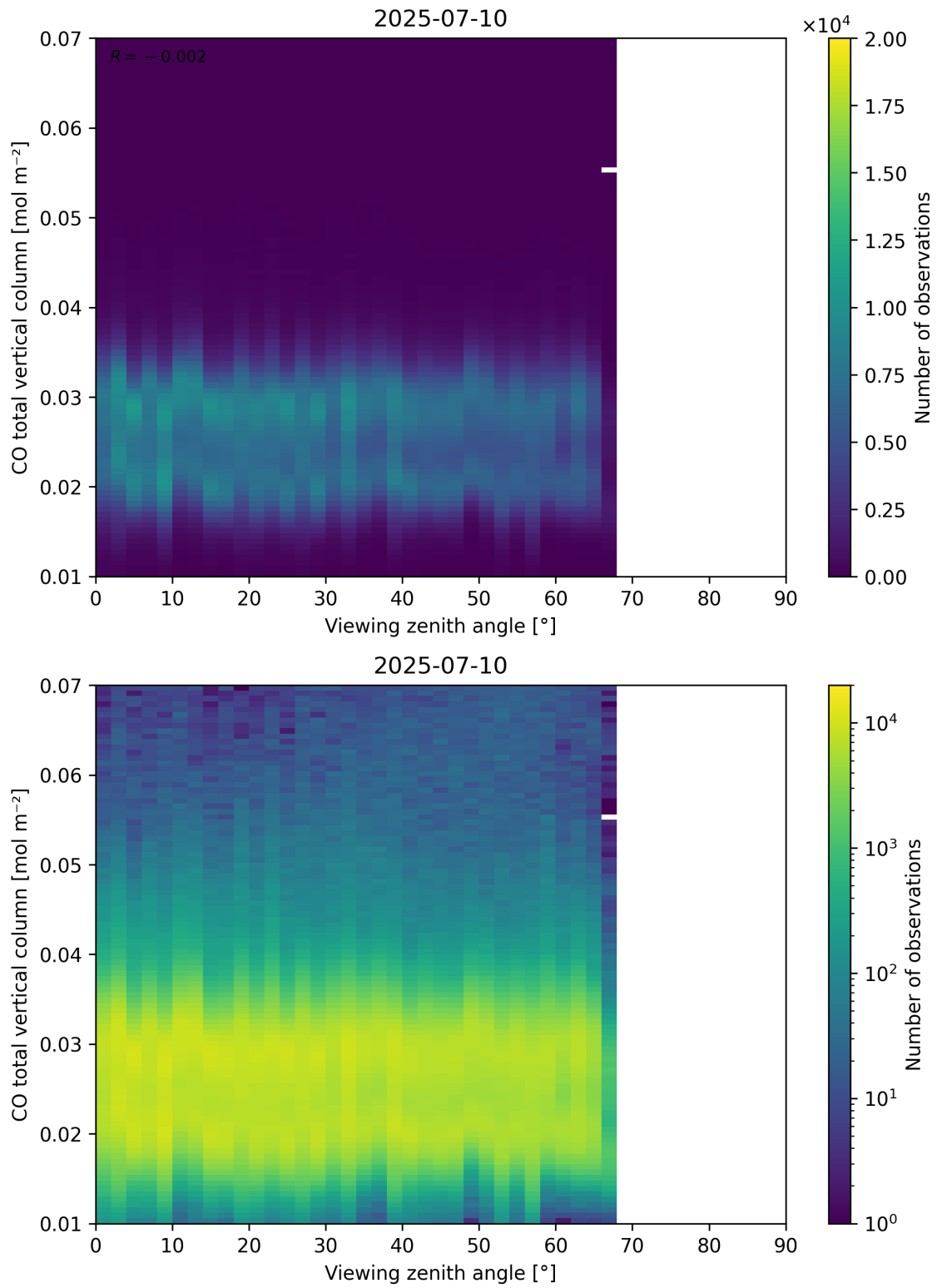
Figure 69: Scatter density plot of “Viewing zenith angle” against “CO total vertical column” for 2025-07-09 to 2025-07-11.
