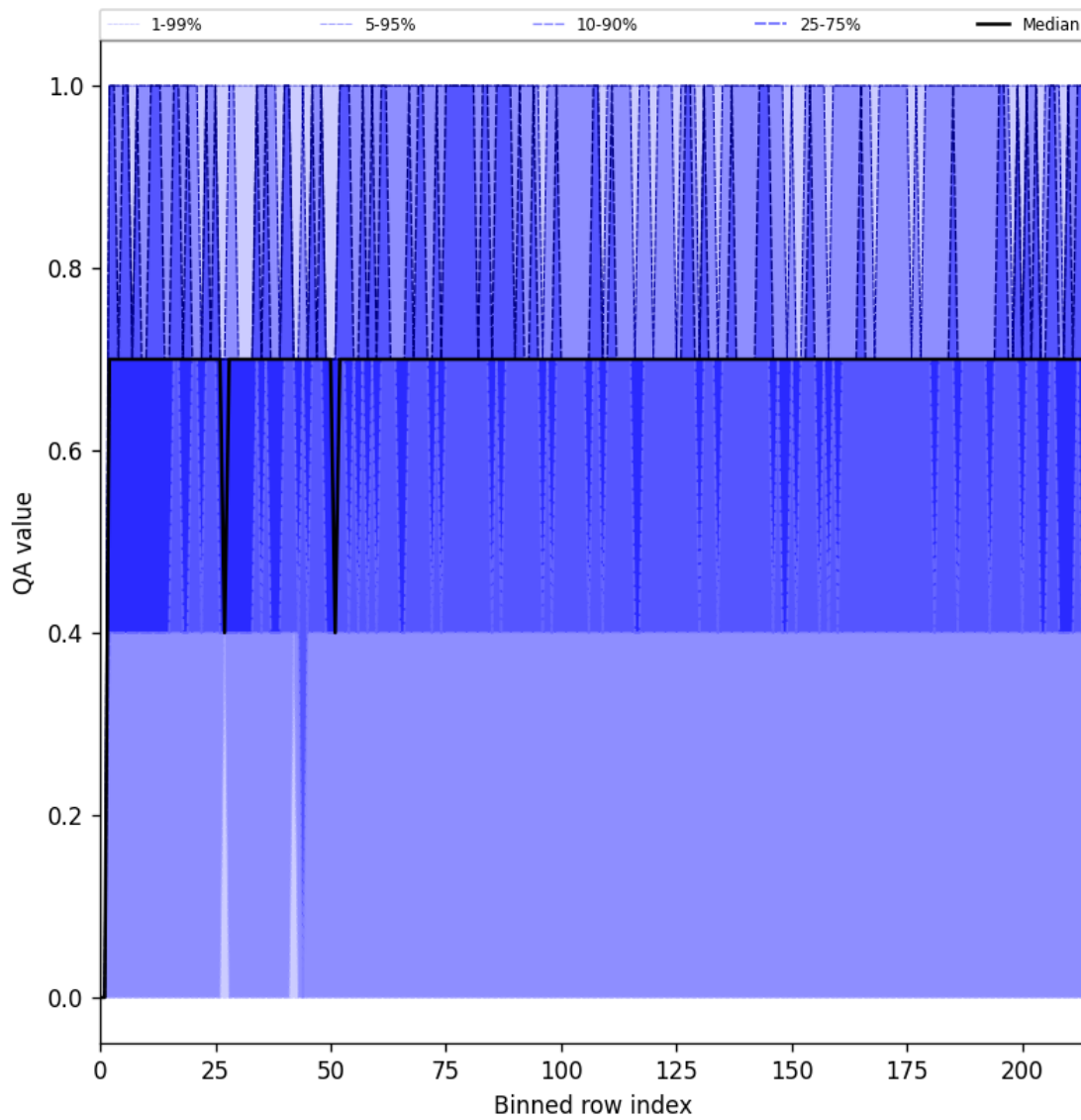
Figure 25: Along track statistics of “QA value” for 2025-07-09 to 2025-07-11
