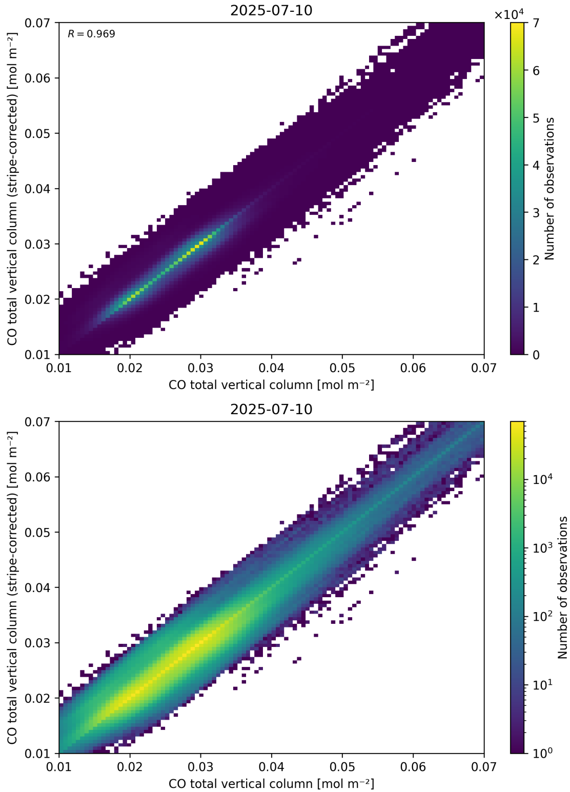
Figure 33: Scatter density plot of “CO total vertical column” against “CO total vertical column (stripe-corrected)” for 2025-07-09 to 2025-07-11.
