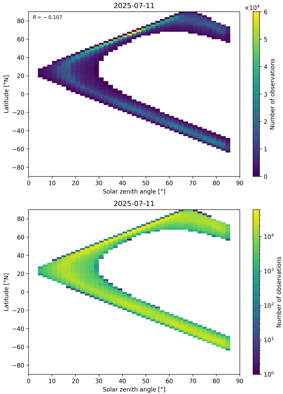
Figure 66: Scatter density plot of “Solar zenith angle” against “Latitude” for 2025-07-10 to 2025-07-12.
