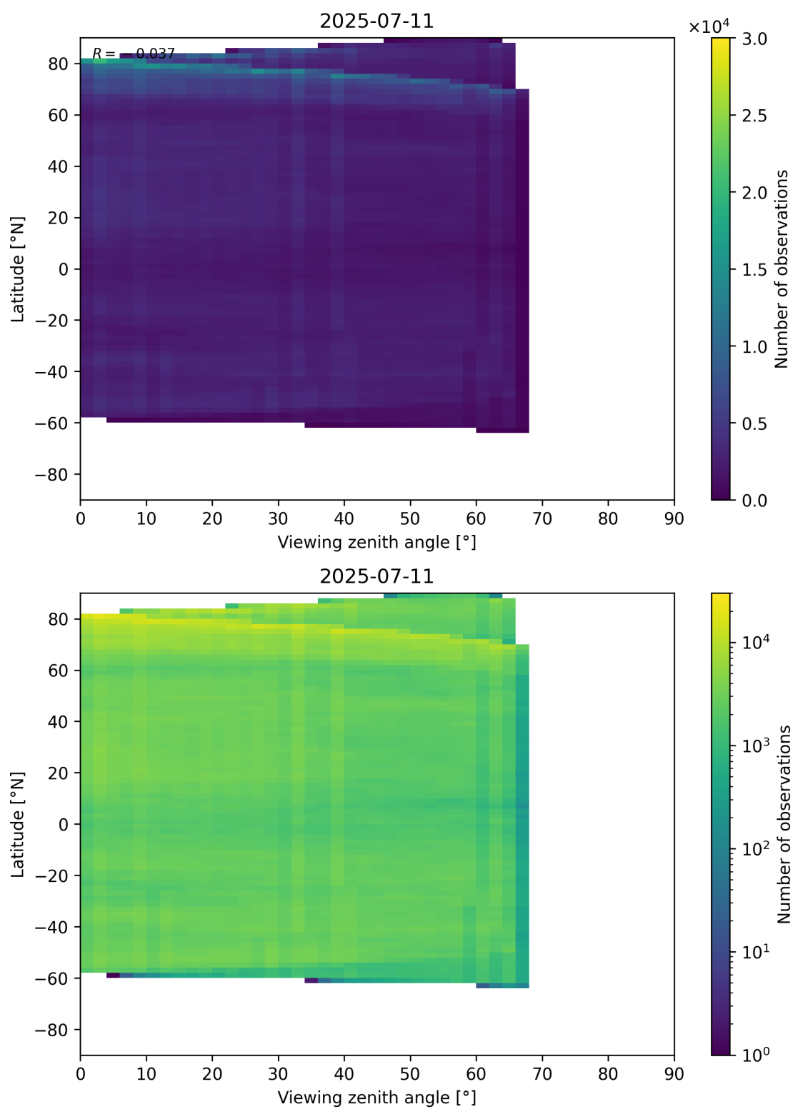
Figure 74: Scatter density plot of “Viewing zenith angle” against “Latitude” for 2025-07-10 to 2025-07-12.
