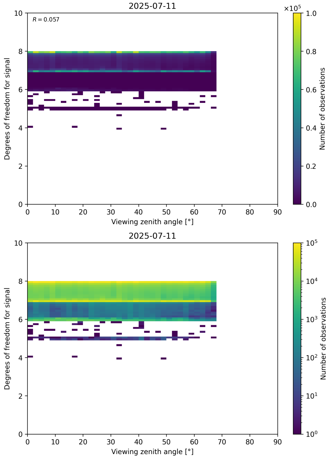
Figure 73: Scatter density plot of “Viewing zenith angle” against “Degrees of freedom for signal” for 2025-07-10 to 2025-07-12.
