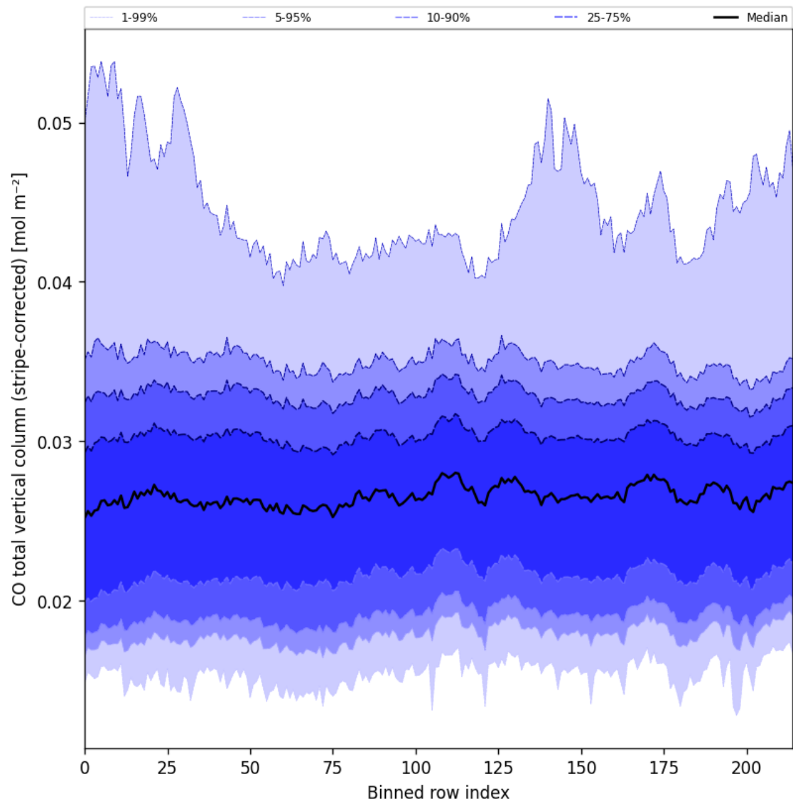
Figure 27: Along track statistics of “CO total vertical column (stripe-corrected)” for 2025-07-10 to 2025-07-12
