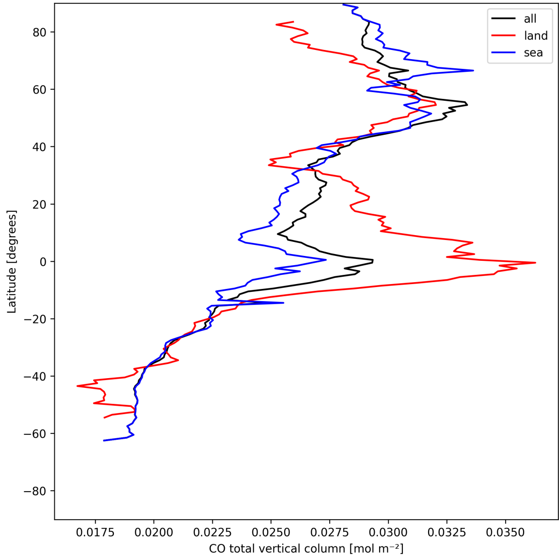
Figure 10: Zonal average of “CO total vertical column” for 2025-07-10 to 2025-07-12.
