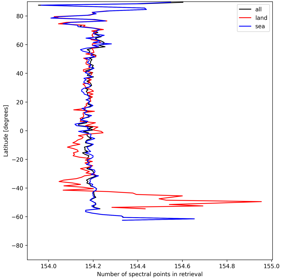
Figure 13: Zonal average of “Number of spectral points in retrieval” for 2025-07-10 to 2025-07-12.
