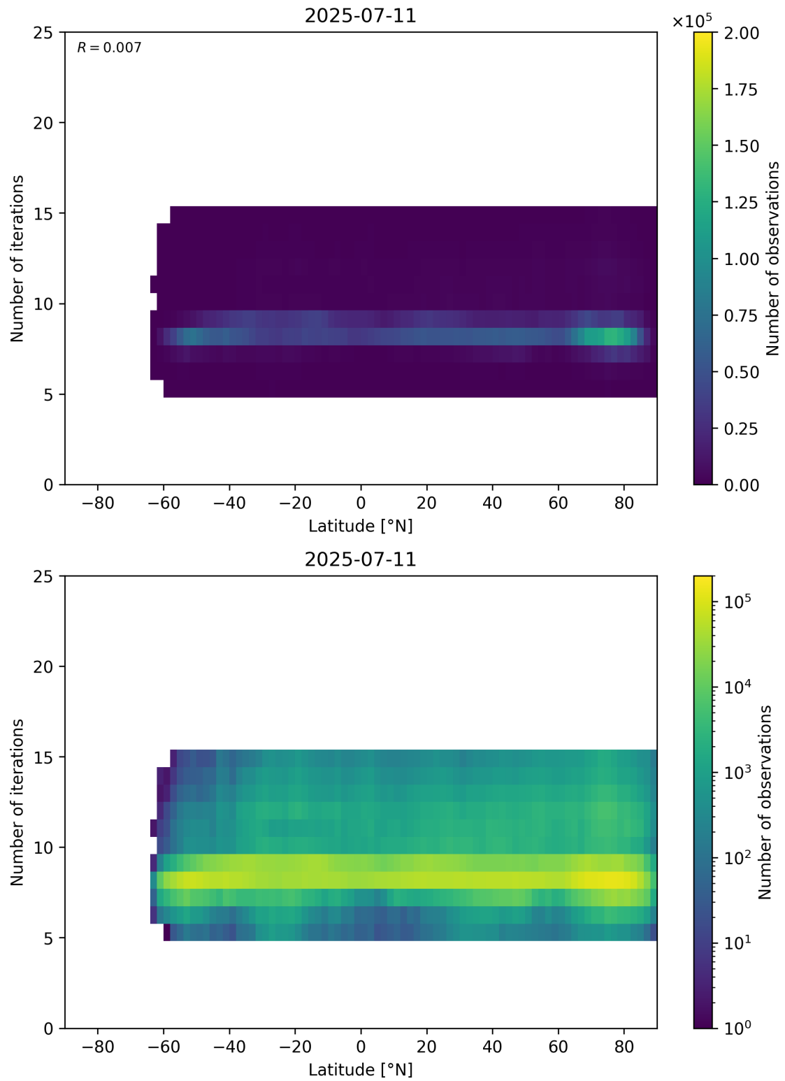
Figure 56: Scatter density plot of “Latitude” against “Number of iterations” for 2025-07-10 to 2025-07-12.
