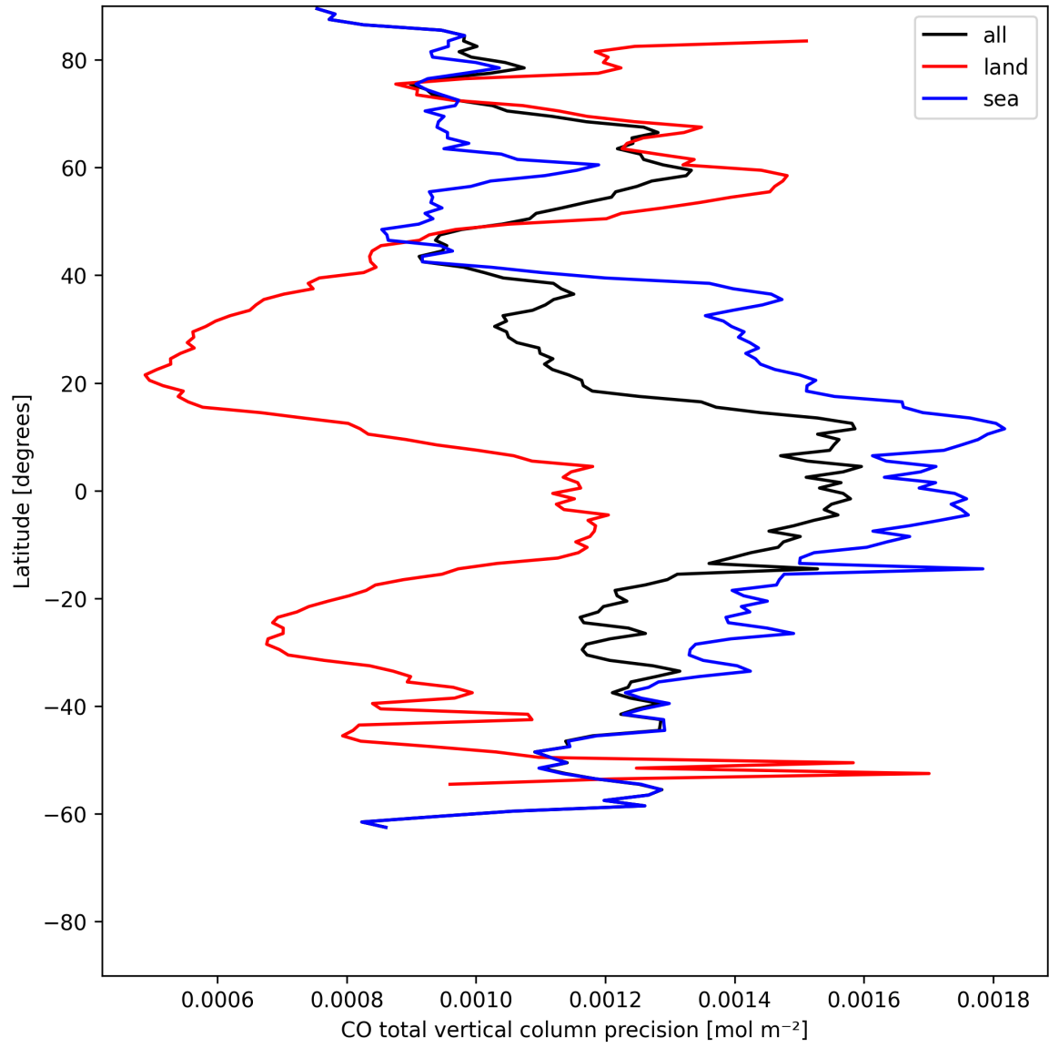
Figure 12: Zonal average of “CO total vertical column precision” for 2025-07-10 to 2025-07-12.
