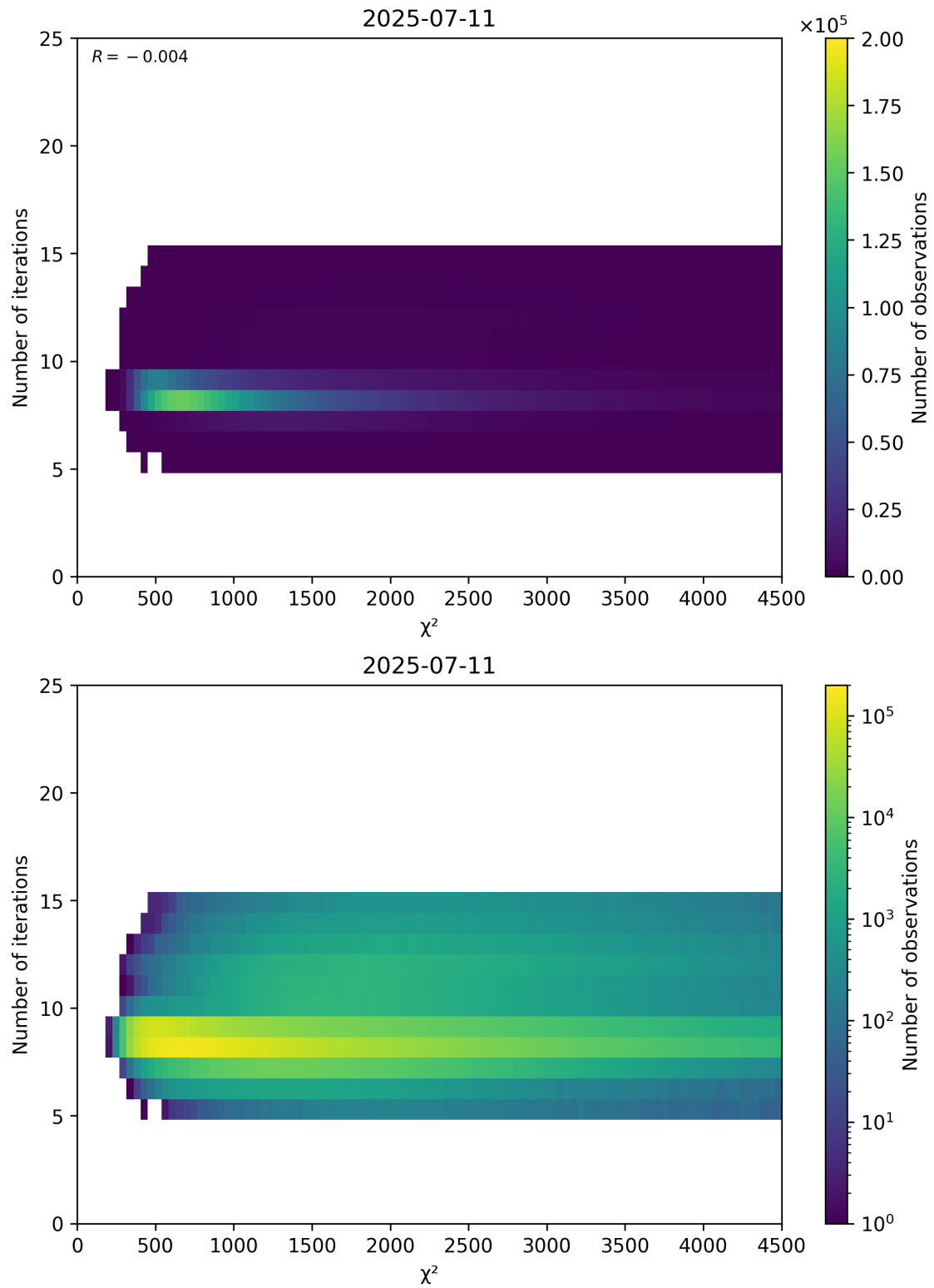
Figure 49: Scatter density plot of “ \chi^2 ” against “Number of iterations” for 2025-07-10 to 2025-07-12.
