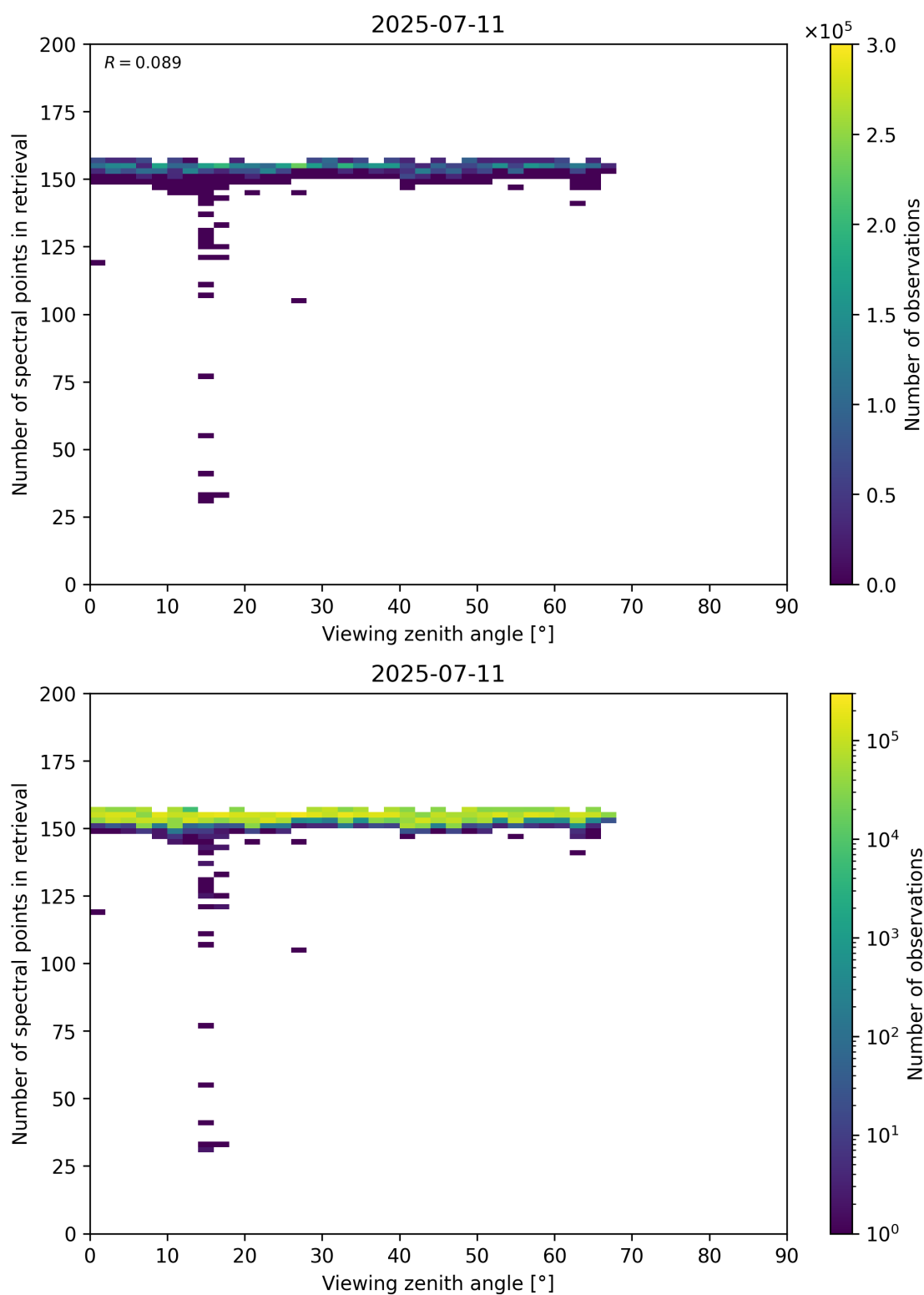
Figure 76: Scatter density plot of “Viewing zenith angle” against “Number of spectral points in retrieval” for 2025-07-10 to 2025-07-12.
