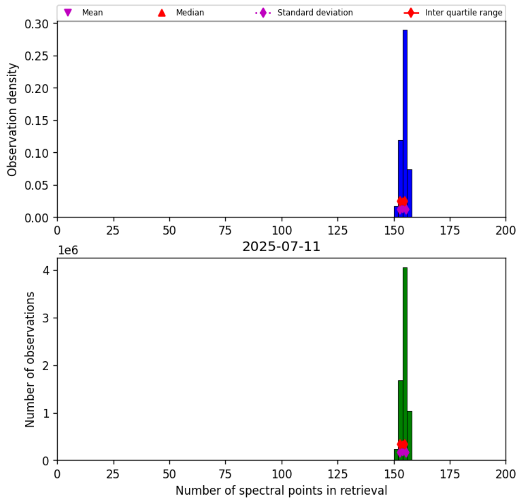
Figure 21: Histogram of “Number of spectral points in retrieval” for 2025-07-10 to 2025-07-12
