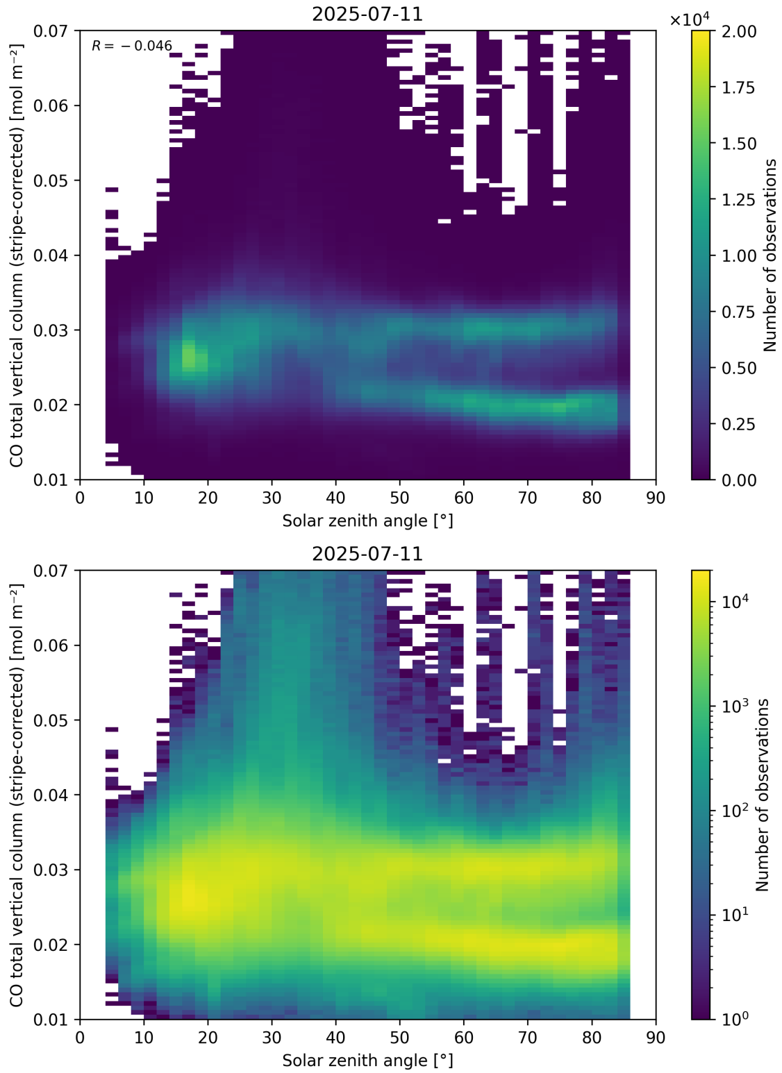
Figure 62: Scatter density plot of “Solar zenith angle” against “CO total vertical column (stripe-corrected)” for 2025-07-10 to 2025-07-12.
