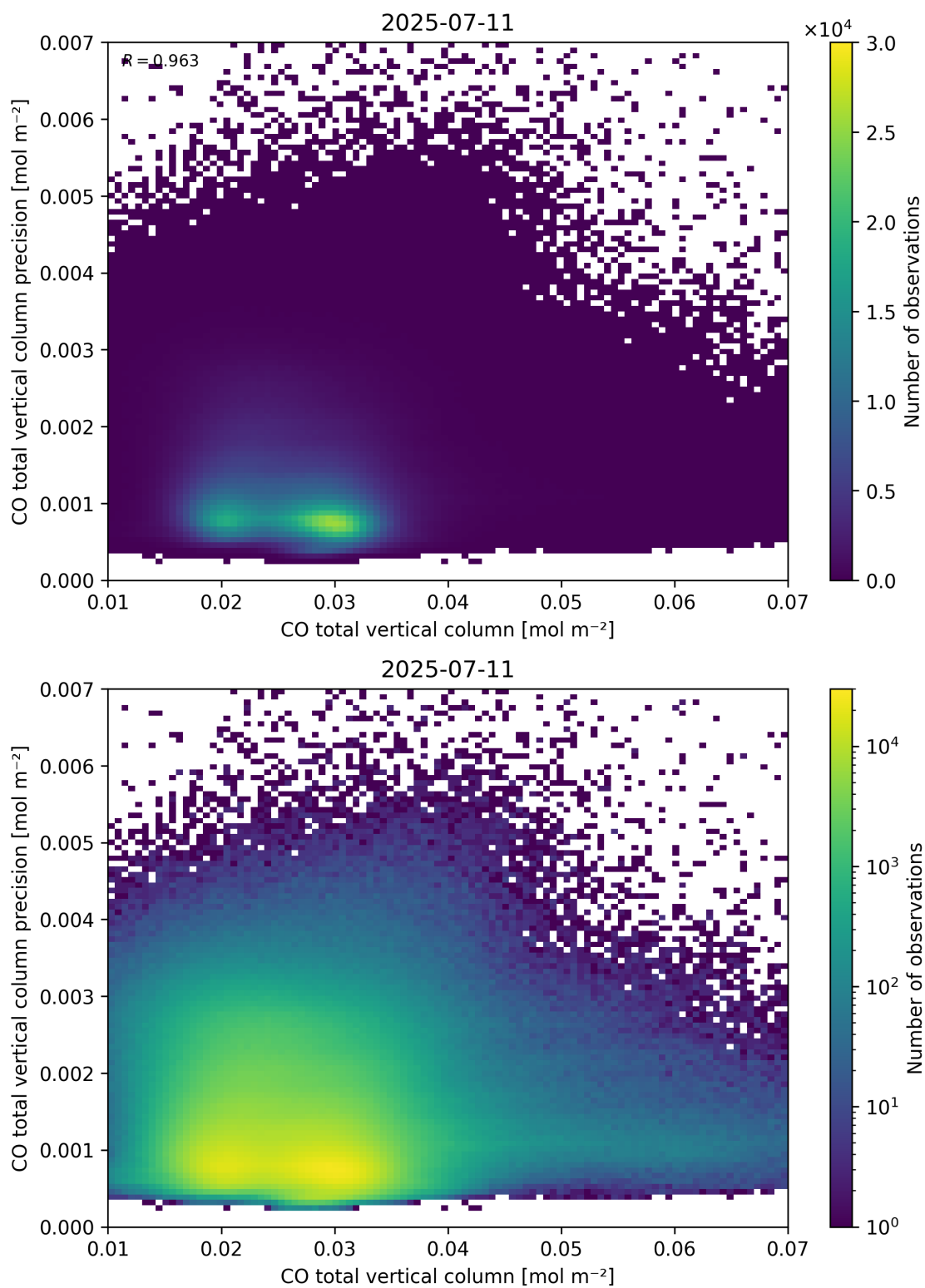
Figure 34: Scatter density plot of “CO total vertical column” against “CO total vertical column precision” for 2025-07-10 to 2025-07-12.
