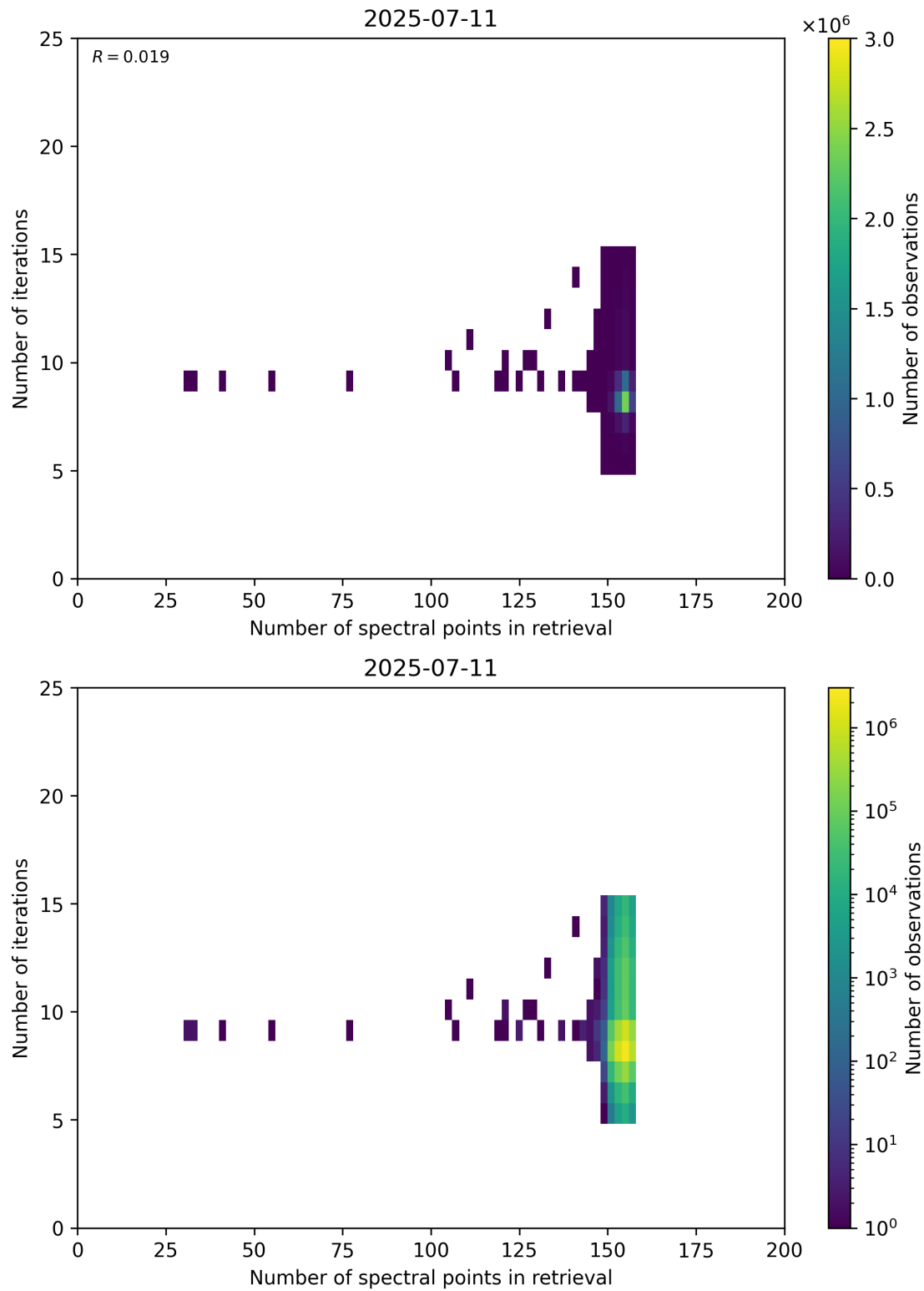
Figure 60: Scatter density plot of “Number of spectral points in retrieval” against “Number of iterations” for 2025-07-10 to 2025-07-12.
