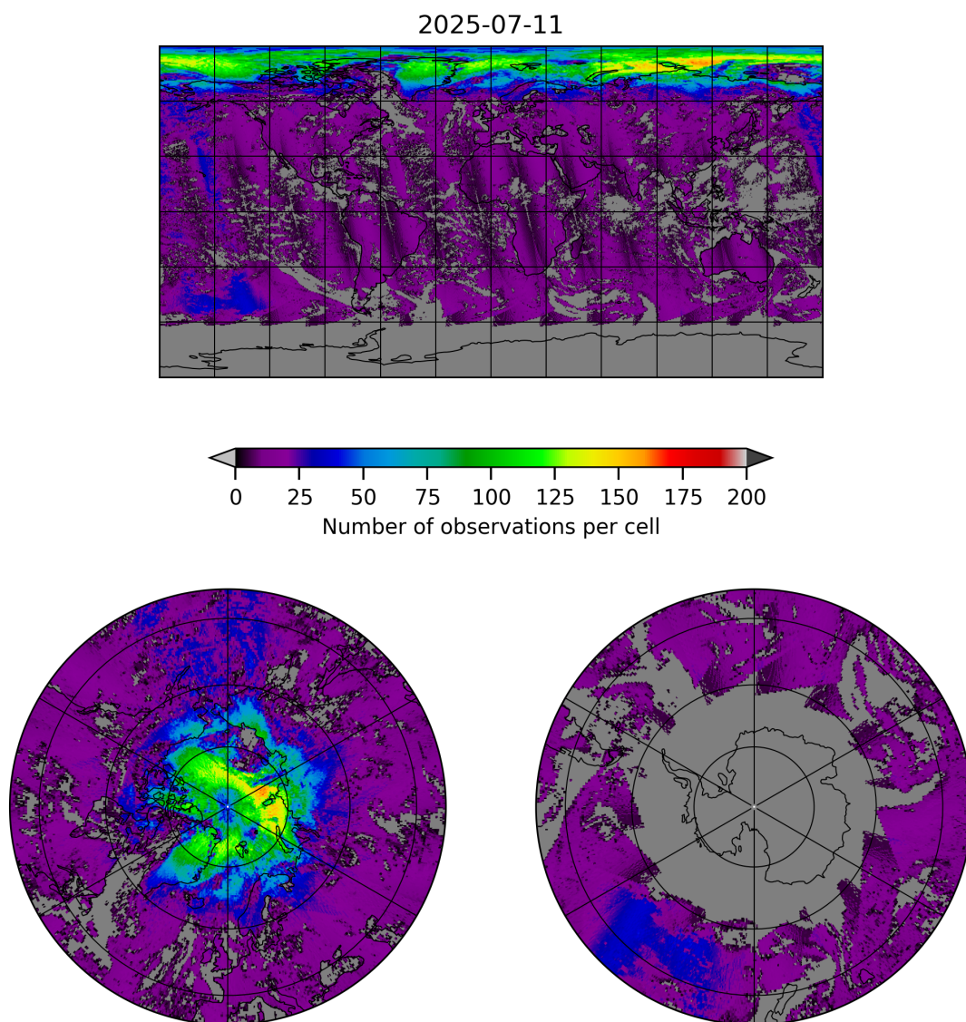
Figure 8: Map of the number of observations for 2025-07-10 to 2025-07-12
