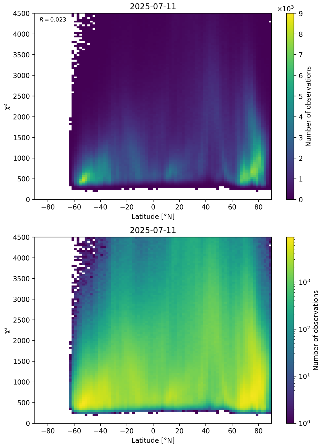
Figure 54: Scatter density plot of “Latitude” against “ \chi^2 ” for 2025-07-10 to 2025-07-12.
