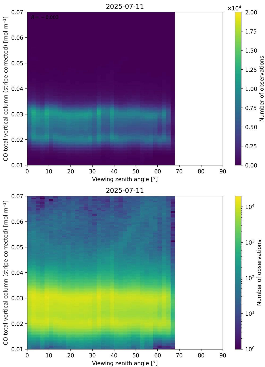
Figure 70: Scatter density plot of “Viewing zenith angle” against “CO total vertical column (stripe-corrected)” for 2025-07-10 to 2025-07-12.
