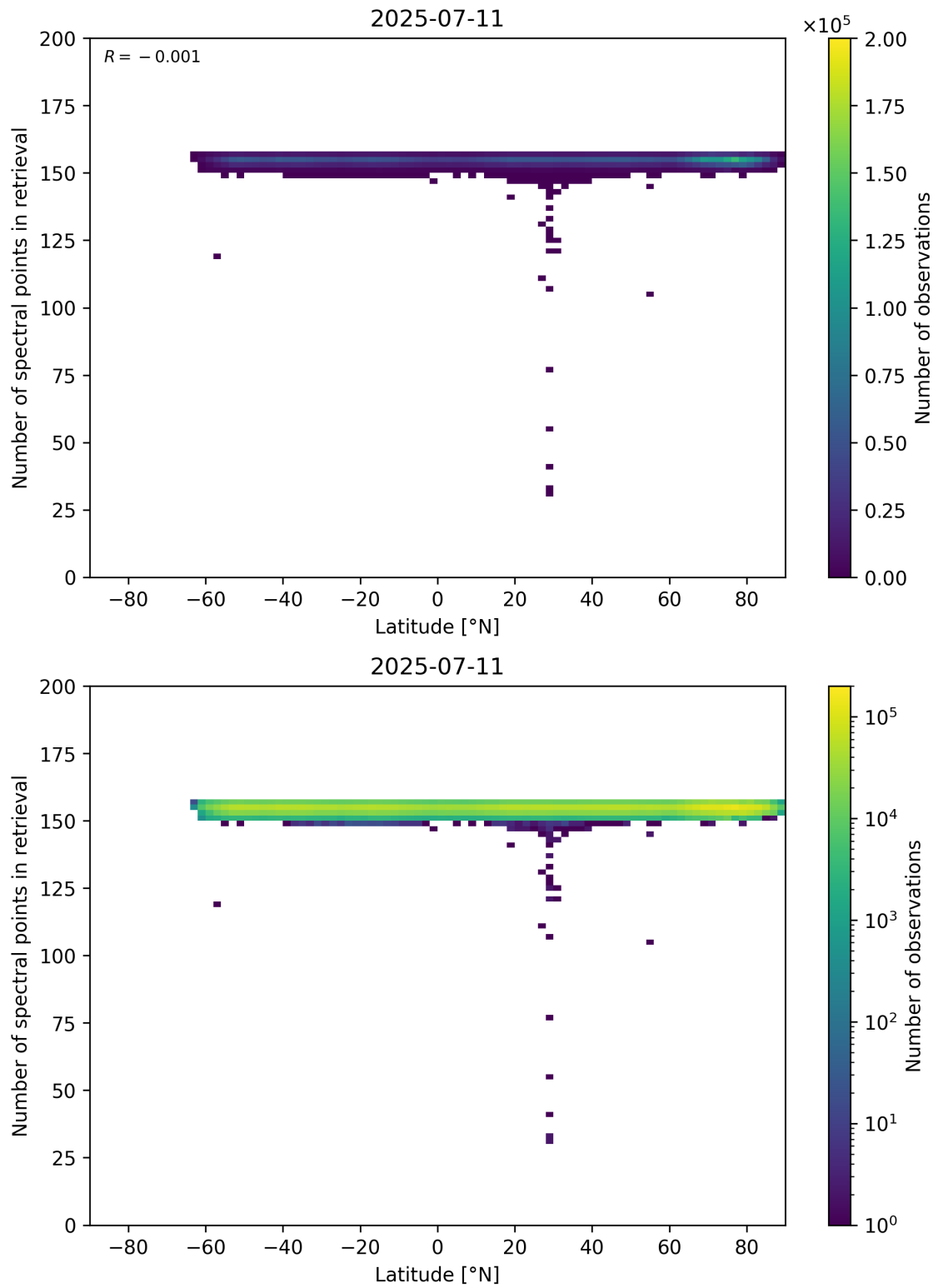
Figure 57: Scatter density plot of “Latitude” against “Number of spectral points in retrieval” for 2025-07-10 to 2025-07-12.
