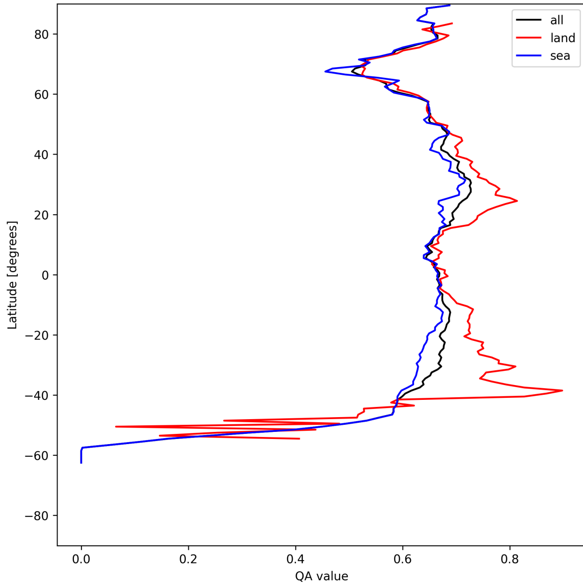
Figure 9: Zonal average of “QA value” for 2025-07-10 to 2025-07-12.
