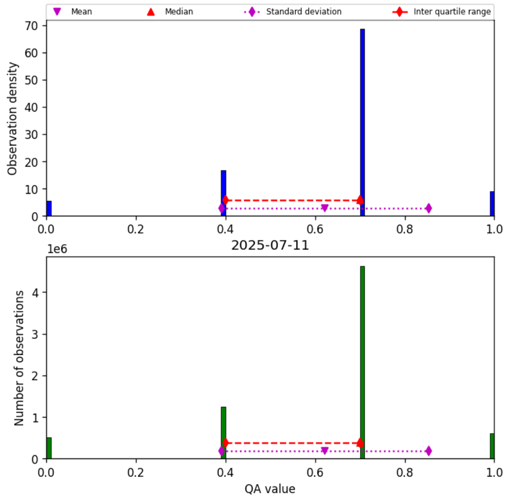
Figure 17: Histogram of “QA value” for 2025-07-10 to 2025-07-12
