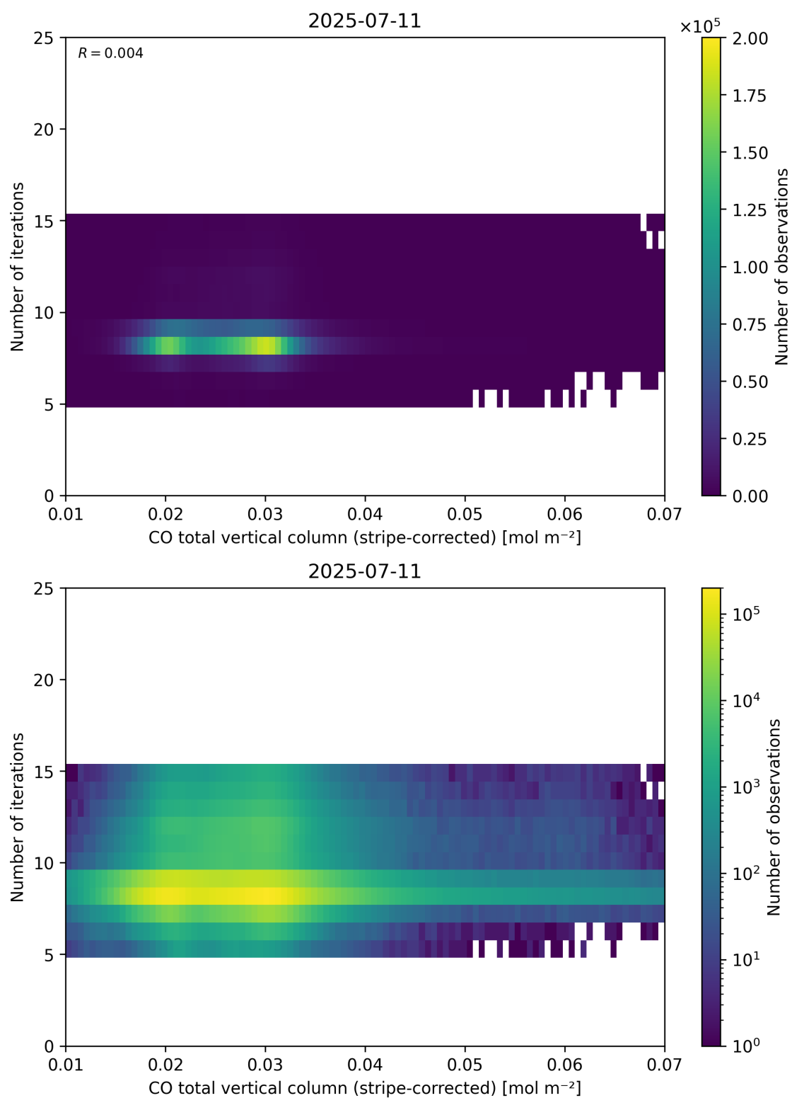
Figure 39: Scatter density plot of “CO total vertical column (stripe-corrected)” against “Number of iterations” for 2025-07-10 to 2025-07-12.
