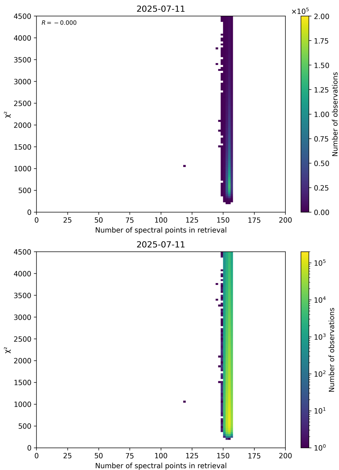
Figure 58: Scatter density plot of “Number of spectral points in retrieval” against “ \chi^2 ” for 2025-07-10 to 2025-07-12.
