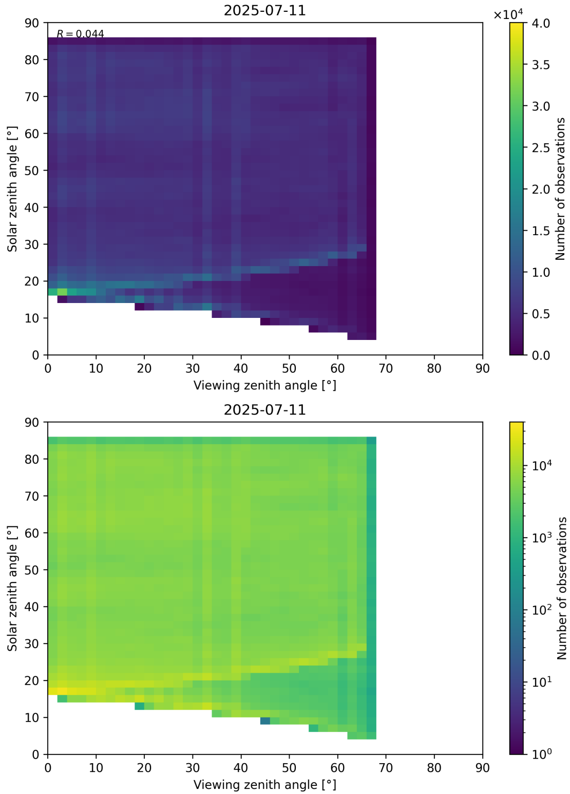
Figure 77: Scatter density plot of “Viewing zenith angle” against “Solar zenith angle” for 2025-07-10 to 2025-07-12.
