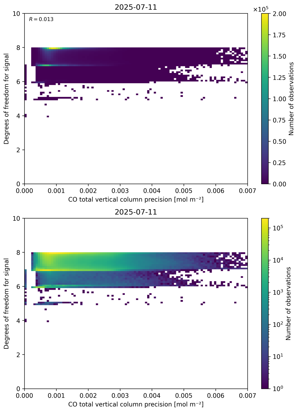
Figure 45: Scatter density plot of “CO total vertical column precision” against “Degrees of freedom for signal” for 2025-07-10 to 2025-07-12.
