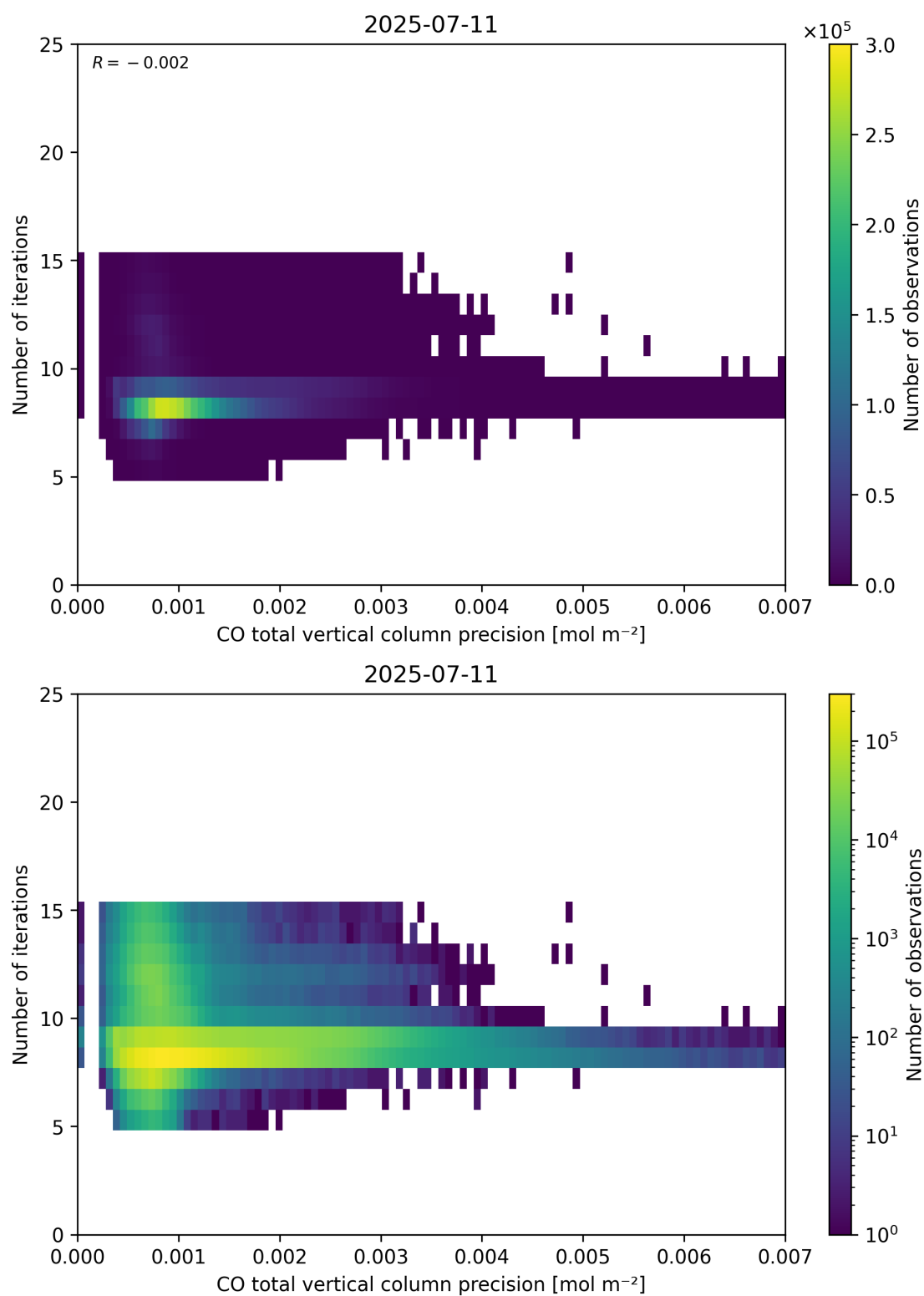
Figure 46: Scatter density plot of “CO total vertical column precision” against “Number of iterations” for 2025-07-10 to 2025-07-12.
