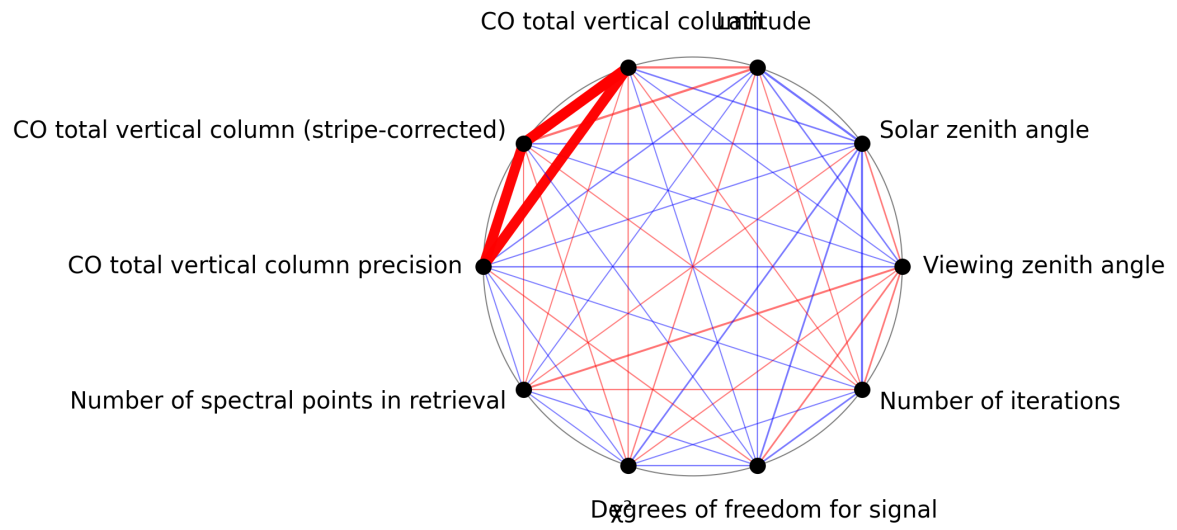
Figure 1: Map of correlation graph for 2025-07-10 to 2025-07-12.
