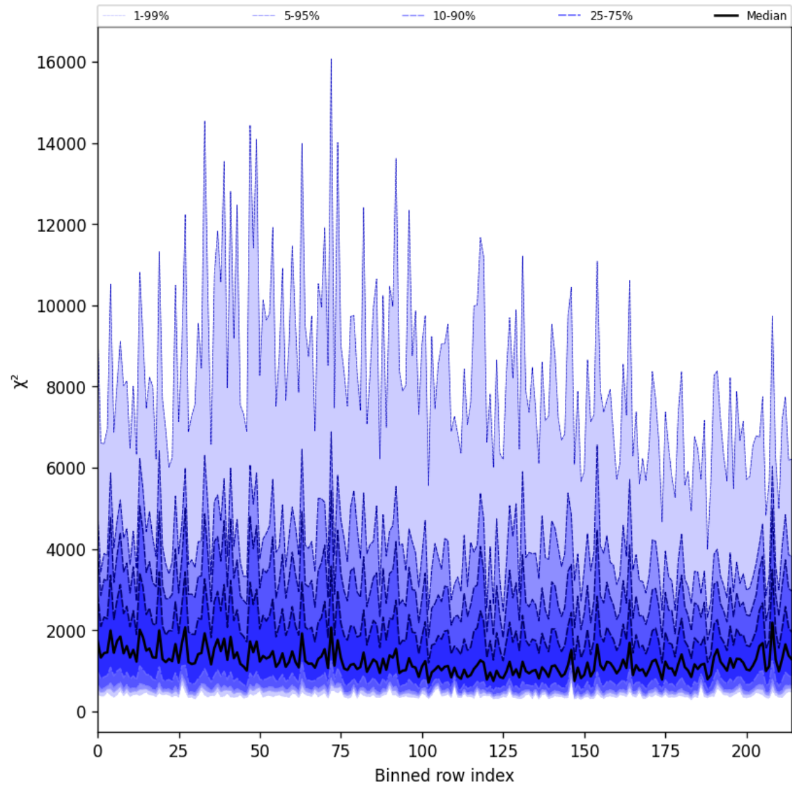
Figure 30: Along track statistics of “ \chi^2 ” for 2025-07-10 to 2025-07-12
