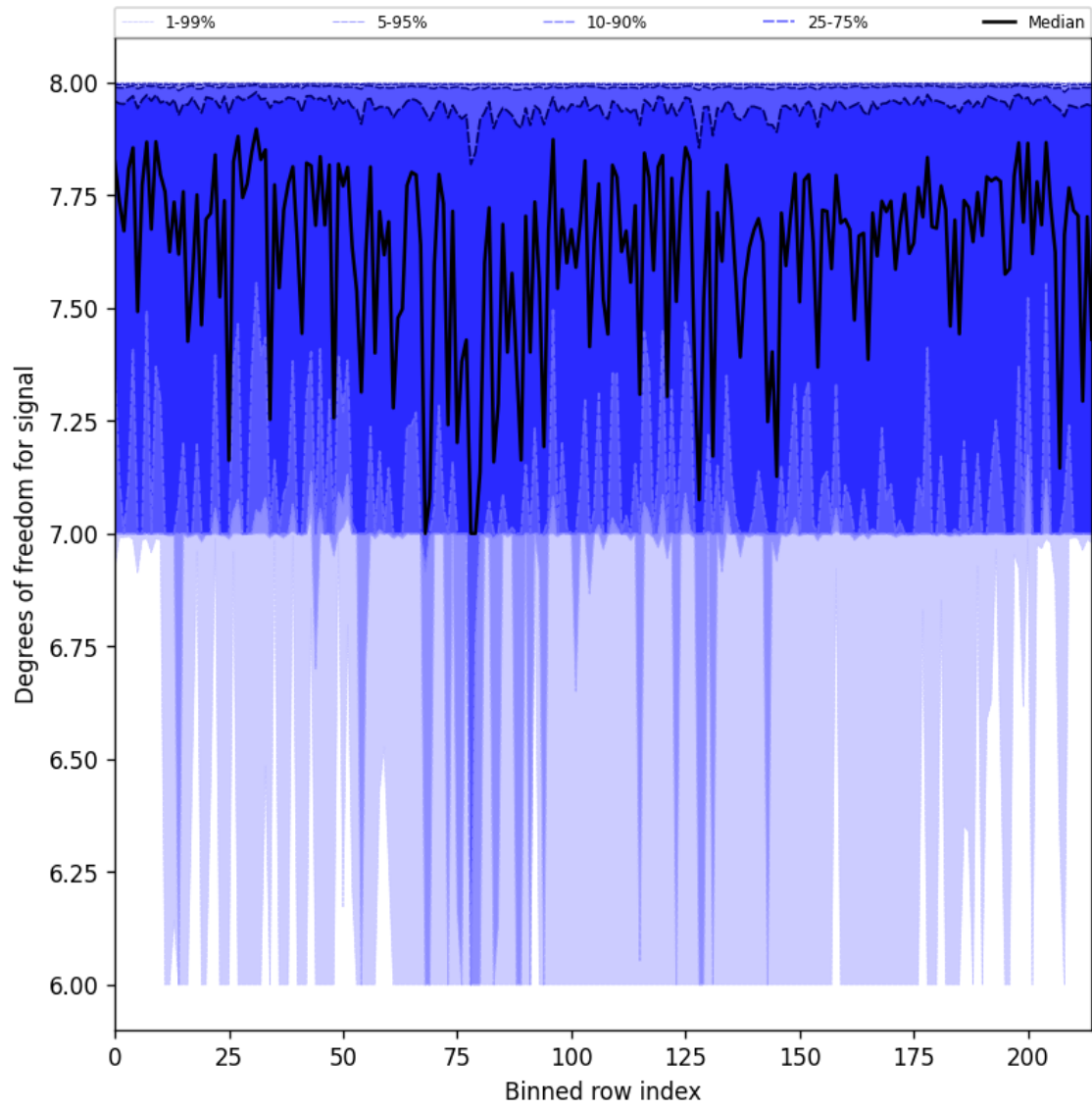
Figure 31: Along track statistics of “Degrees of freedom for signal” for 2025-07-10 to 2025-07-12
