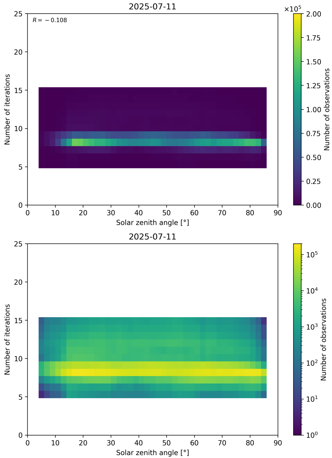
Figure 67: Scatter density plot of “Solar zenith angle” against “Number of iterations” for 2025-07-10 to 2025-07-12.
