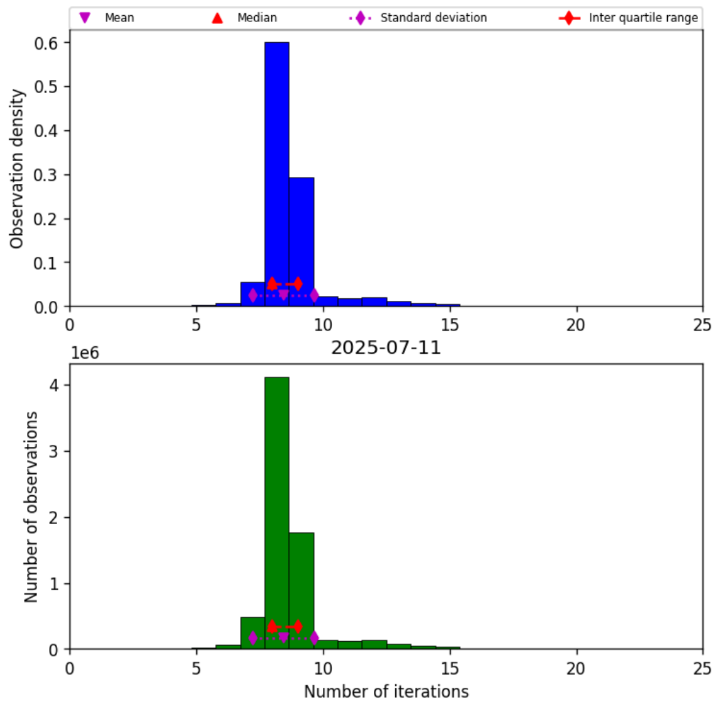
Figure 24: Histogram of “Number of iterations” for 2025-07-10 to 2025-07-12
