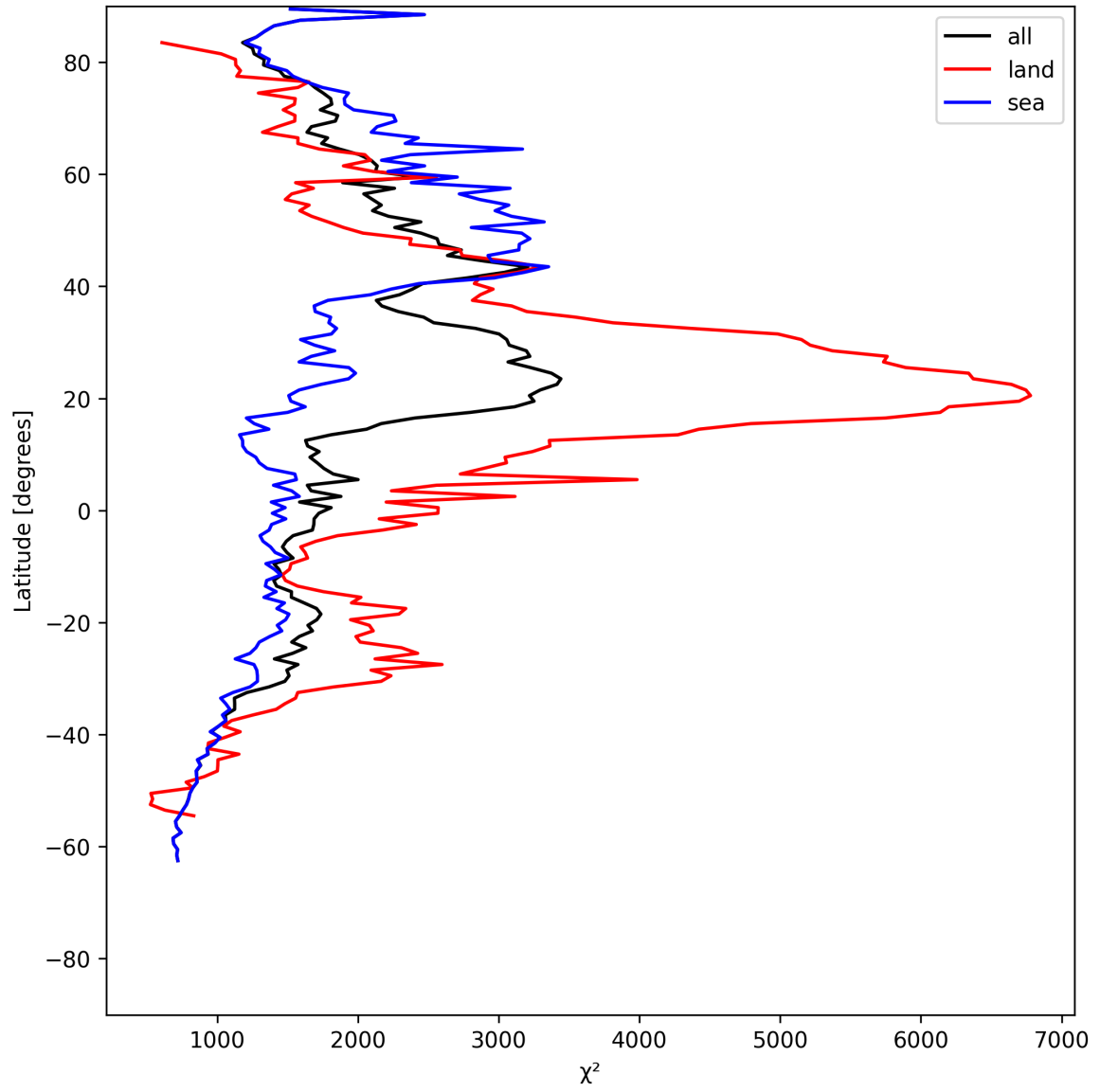
Figure 14: Zonal average of “ \chi^2 ” for 2025-07-10 to 2025-07-12.
