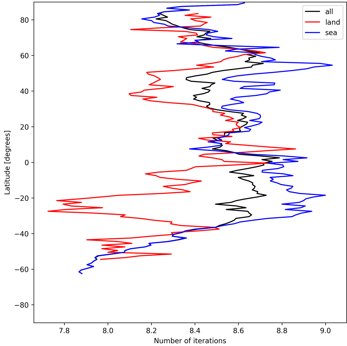
Figure 16: Zonal average of “Number of iterations” for 2025-07-10 to 2025-07-12.
