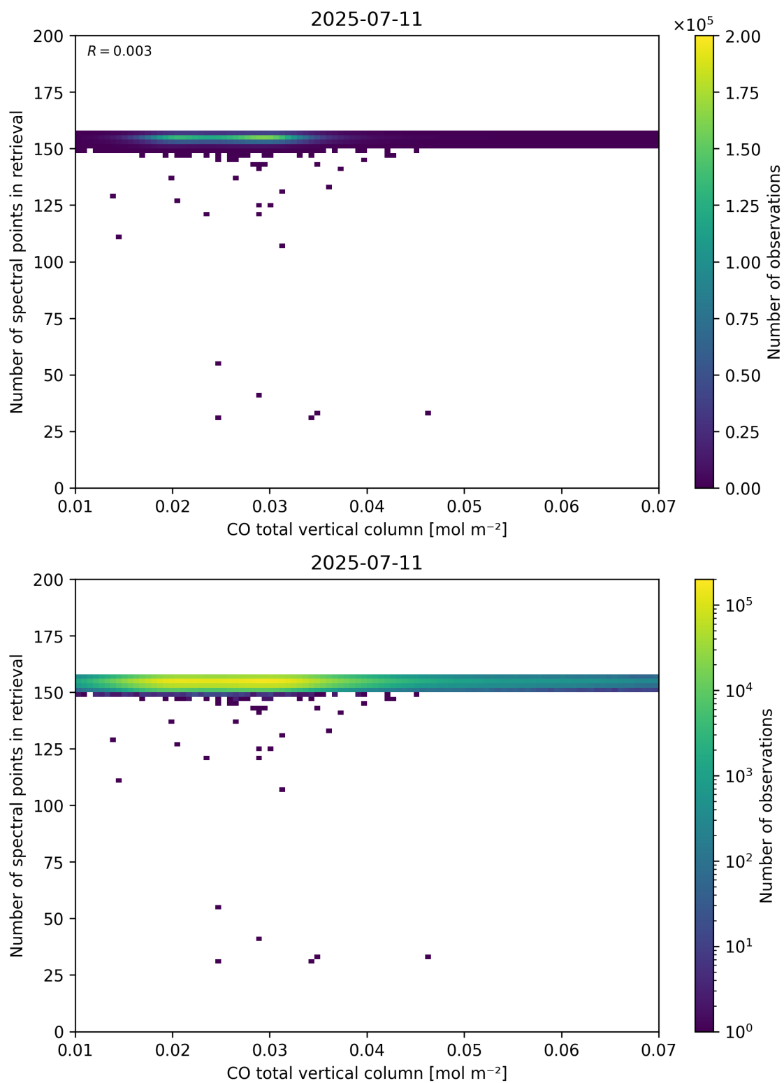
Figure 43: Scatter density plot of “CO total vertical column” against “Number of spectral points in retrieval” for 2025-07-10 to 2025-07-12.
