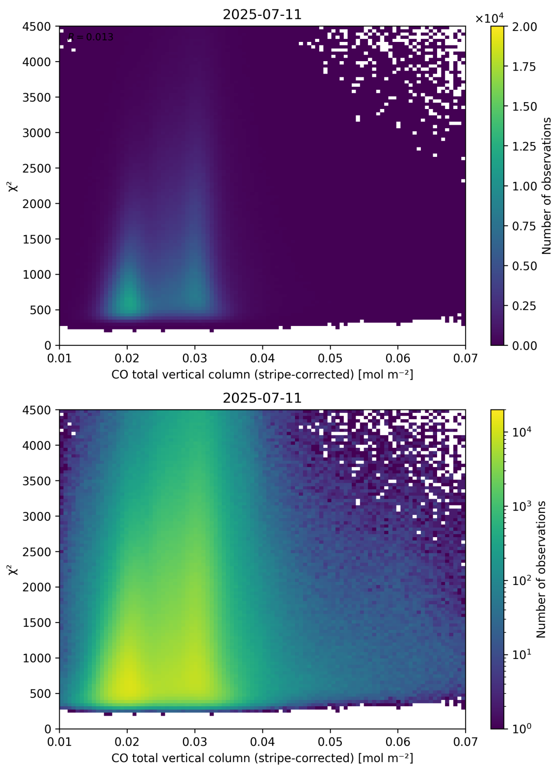
Figure 37: Scatter density plot of “CO total vertical column (stripe-corrected)” against “ \chi^2 ” for 2025-07-10 to 2025-07-12.
