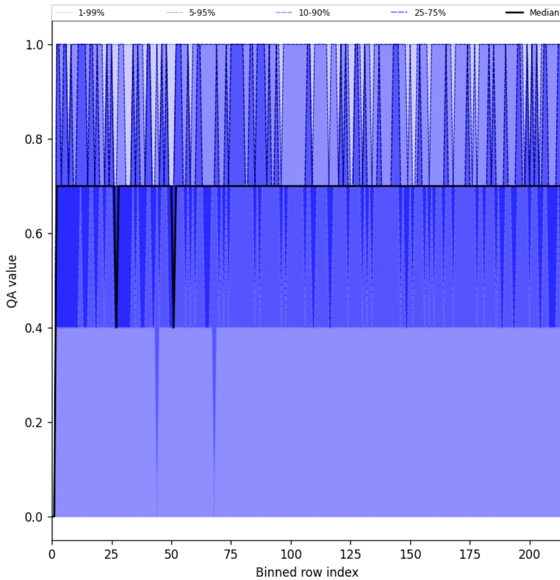
Figure 25: Along track statistics of “QA value” for 2025-07-10 to 2025-07-12
