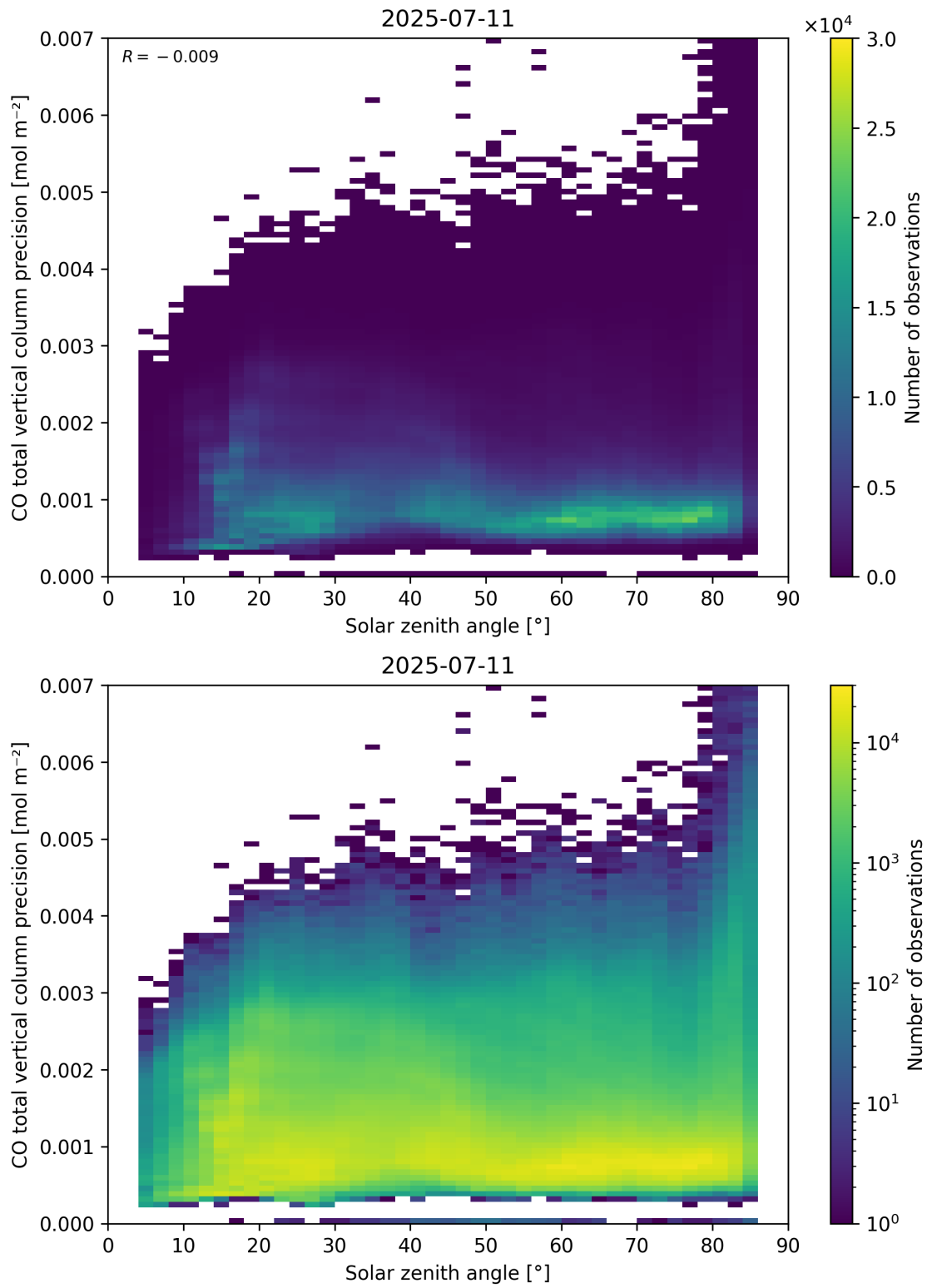
Figure 63: Scatter density plot of “Solar zenith angle” against “CO total vertical column precision” for 2025-07-10 to 2025-07-12.
