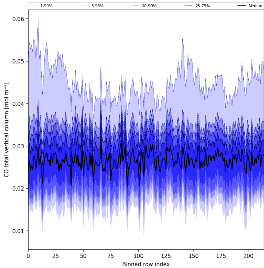
Figure 26: Along track statistics of “CO total vertical column” for 2025-07-10 to 2025-07-12
