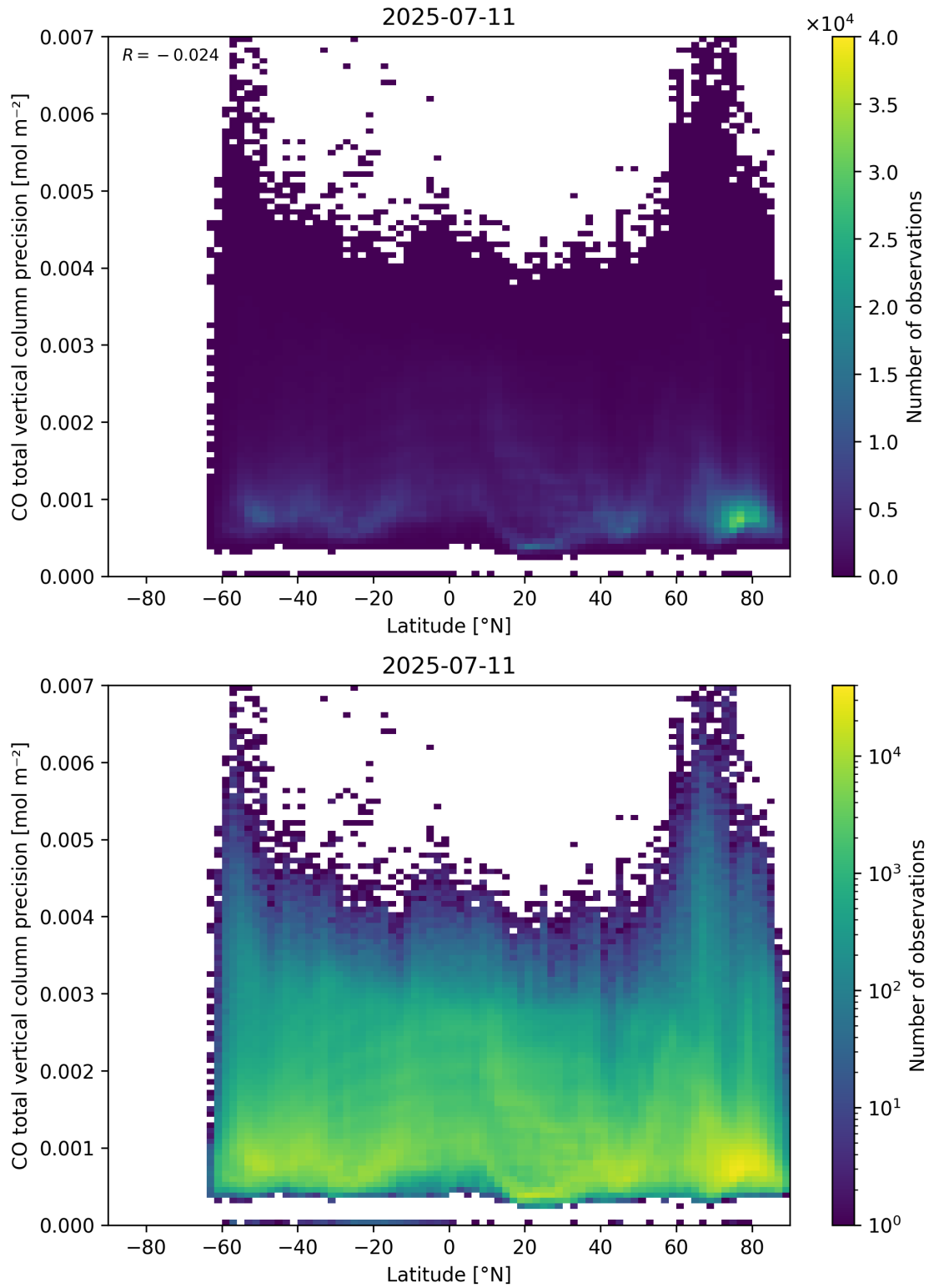
Figure 53: Scatter density plot of “Latitude” against “CO total vertical column precision” for 2025-07-10 to 2025-07-12.
