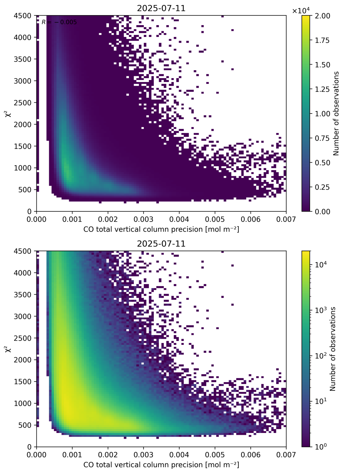
Figure 44: Scatter density plot of “CO total vertical column precision” against “ \chi^2 ” for 2025-07-10 to 2025-07-12.
