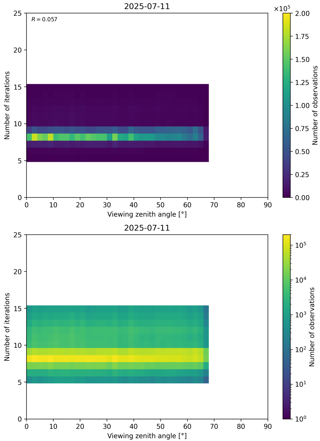
Figure 75: Scatter density plot of “Viewing zenith angle” against “Number of iterations” for 2025-07-10 to 2025-07-12.
