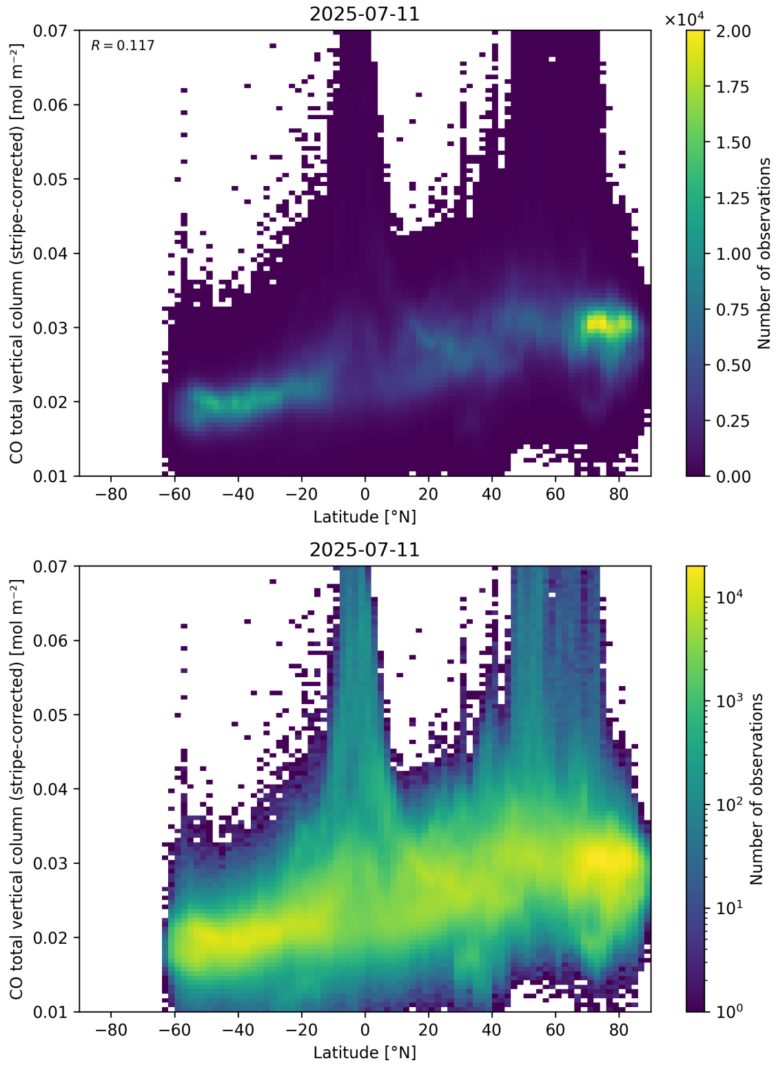
Figure 52: Scatter density plot of “Latitude” against “CO total vertical column (stripe-corrected)” for 2025-07-10 to 2025-07-12.
