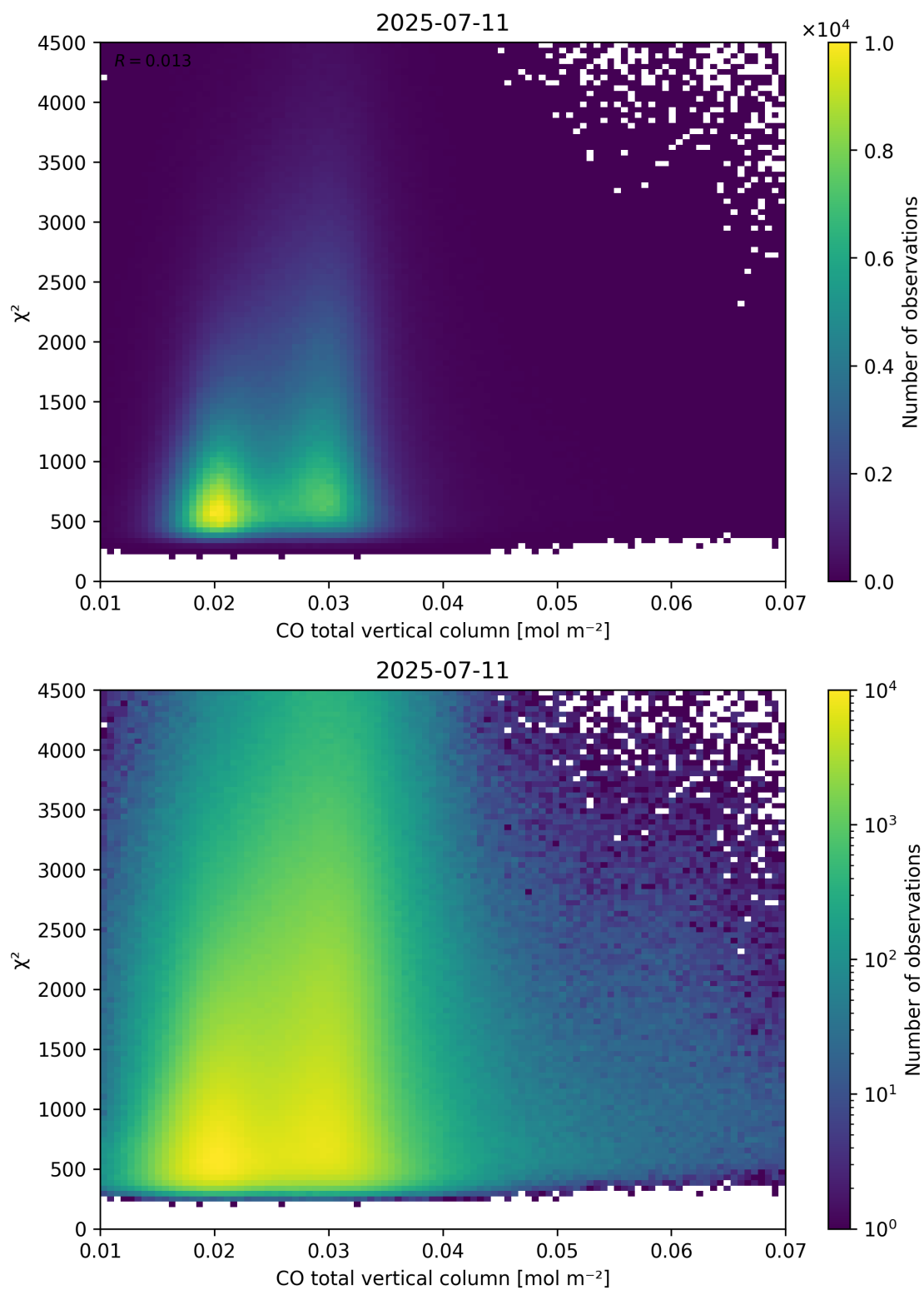
Figure 35: Scatter density plot of “CO total vertical column” against “ \chi^2 ” for 2025-07-10 to 2025-07-12.
