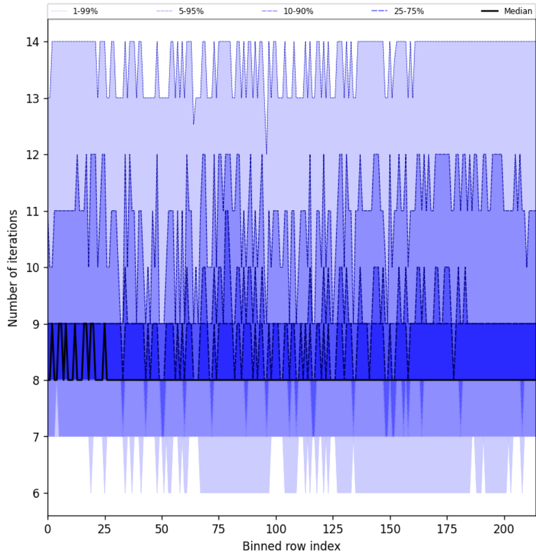
Figure 32: Along track statistics of “Number of iterations” for 2025-07-10 to 2025-07-12
