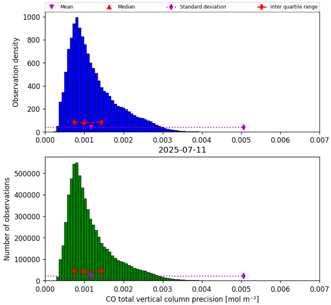
Figure 20: Histogram of “CO total vertical column precision” for 2025-07-10 to 2025-07-12
