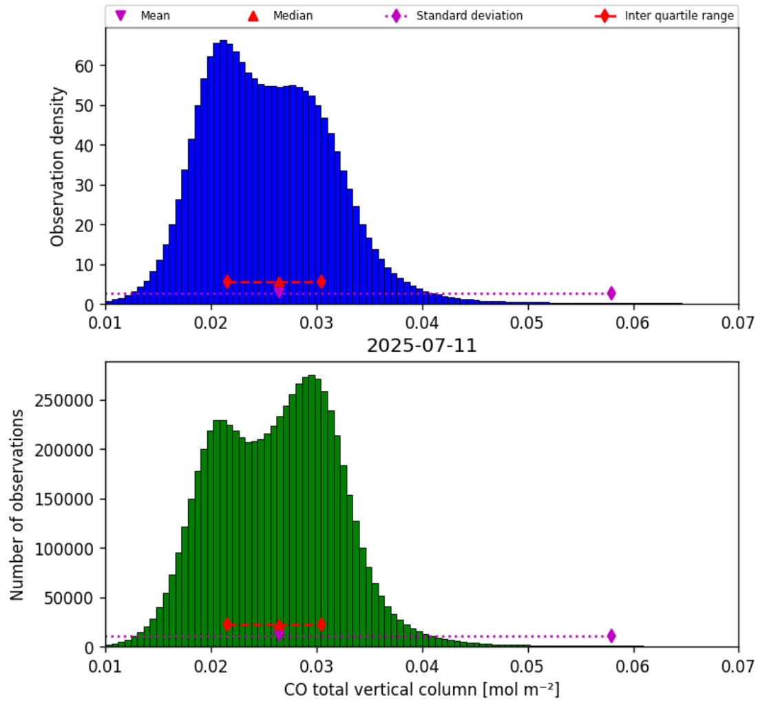
Figure 18: Histogram of “CO total vertical column” for 2025-07-10 to 2025-07-12
