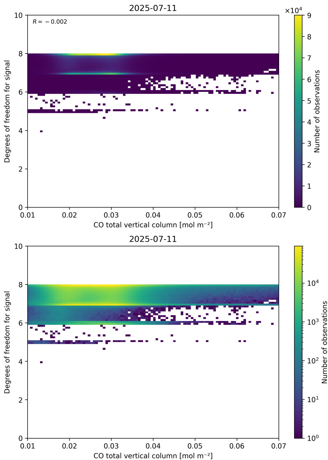
Figure 41: Scatter density plot of “CO total vertical column” against “Degrees of freedom for signal” for 2025-07-10 to 2025-07-12.
