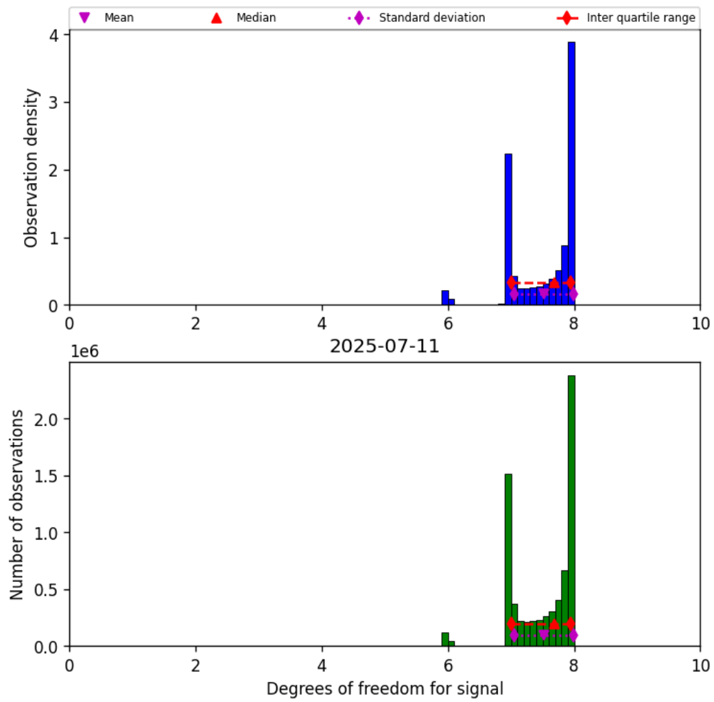
Figure 23: Histogram of “Degrees of freedom for signal” for 2025-07-10 to 2025-07-12
