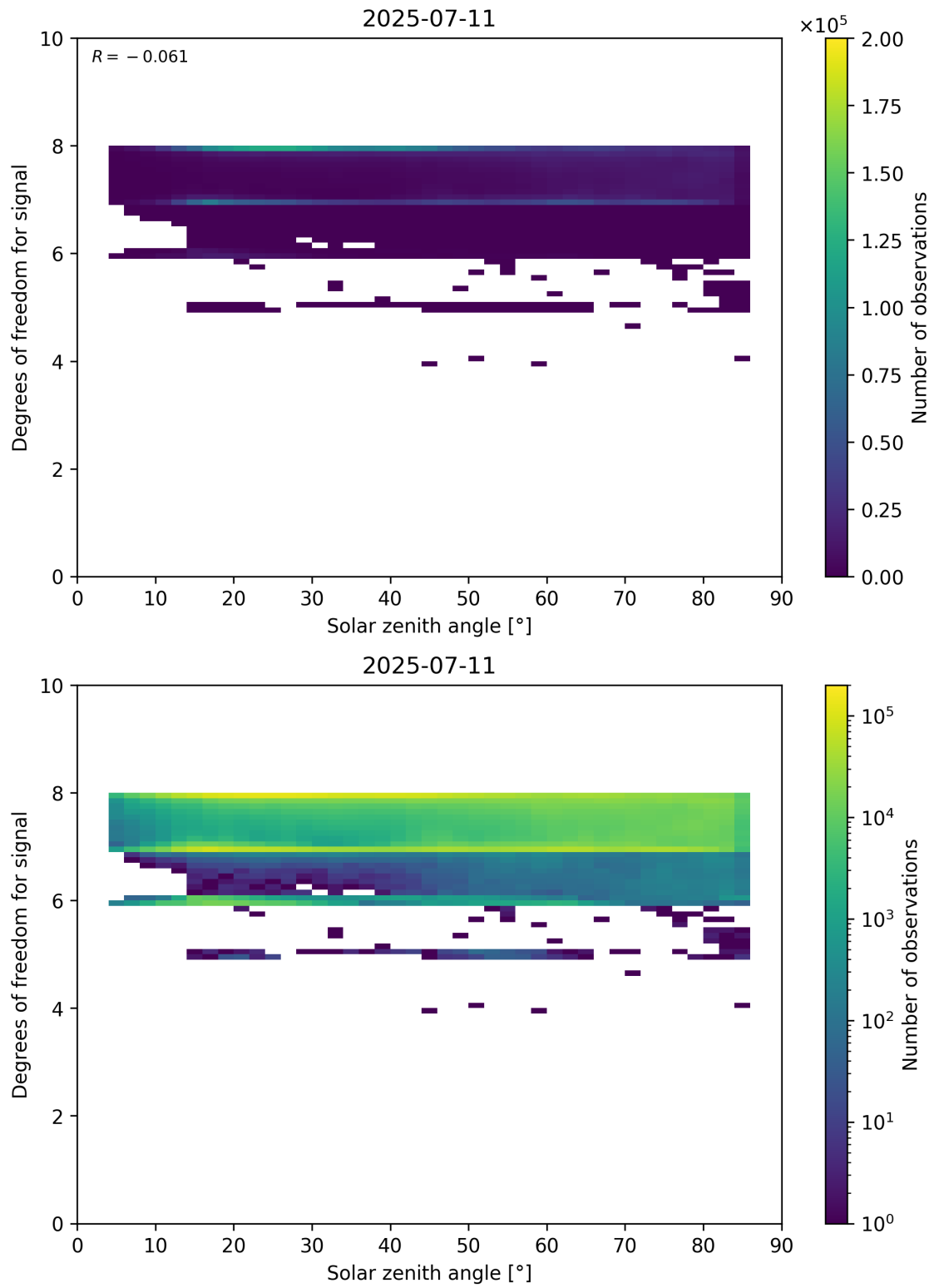
Figure 65: Scatter density plot of “Solar zenith angle” against “Degrees of freedom for signal” for 2025-07-10 to 2025-07-12.
