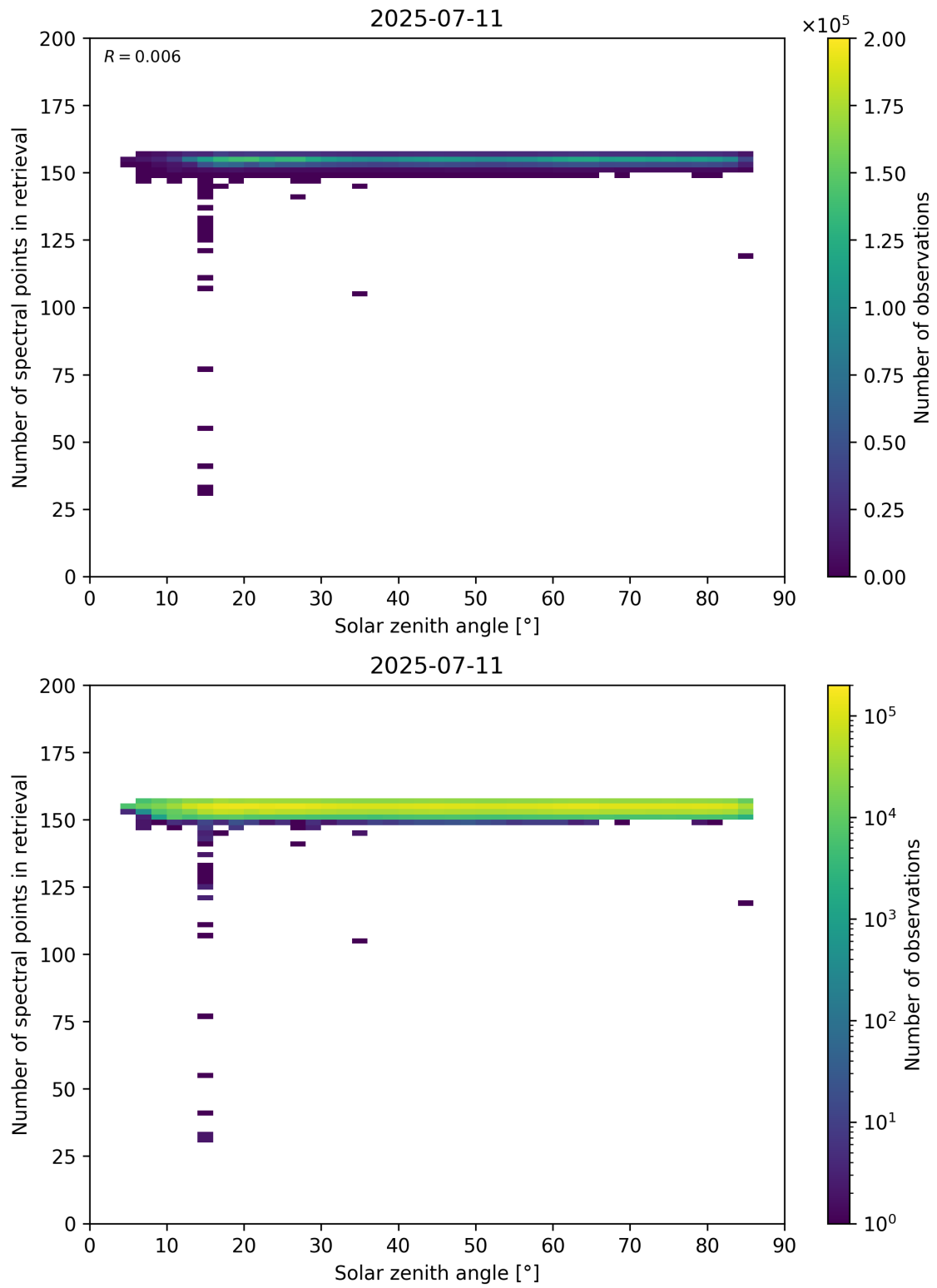
Figure 68: Scatter density plot of “Solar zenith angle” against “Number of spectral points in retrieval” for 2025-07-10 to 2025-07-12.
