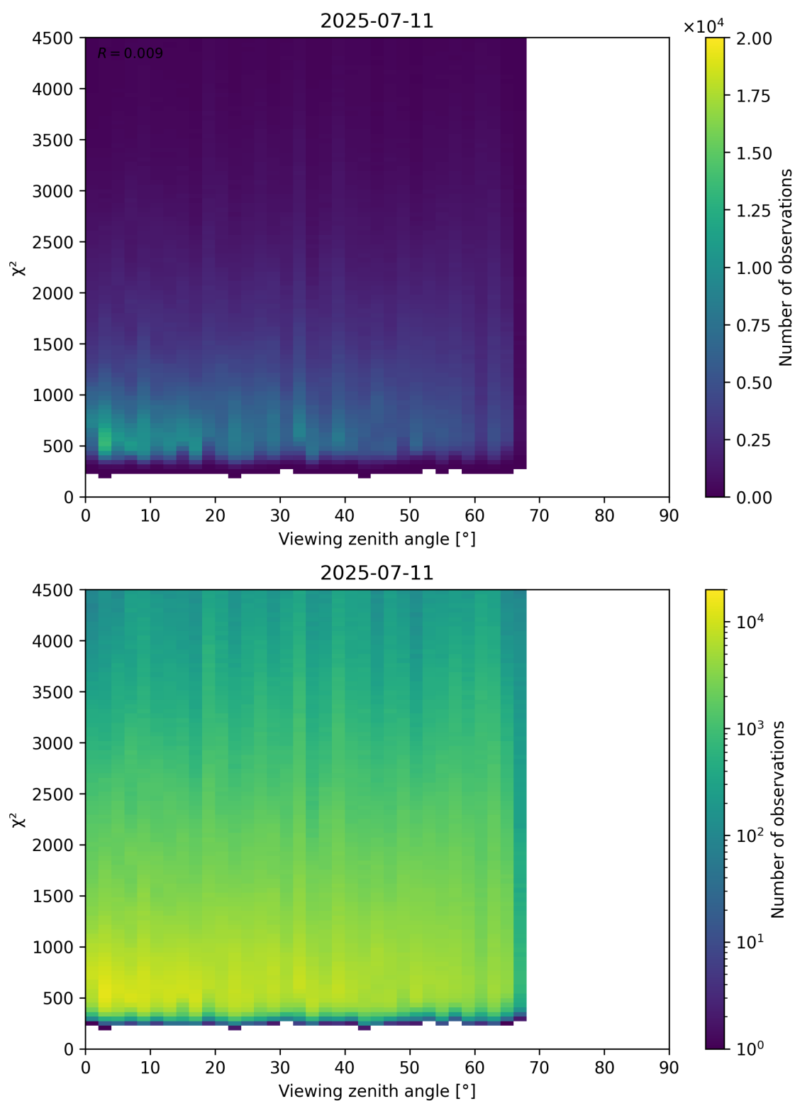
Figure 72: Scatter density plot of “Viewing zenith angle” against “ \chi^2 ” for 2025-07-10 to 2025-07-12.
