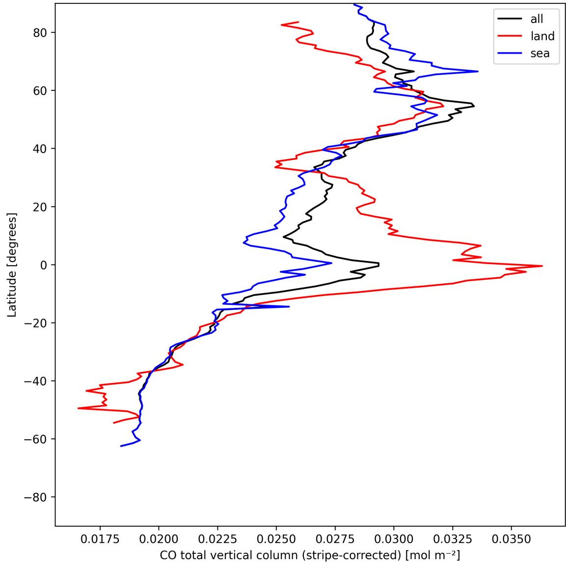
Figure 11: Zonal average of “CO total vertical column (stripe-corrected)” for 2025-07-10 to 2025-07-12.
