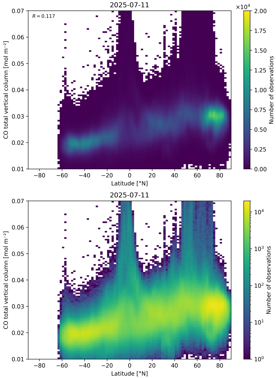
Figure 51: Scatter density plot of “Latitude” against “CO total vertical column” for 2025-07-10 to 2025-07-12.
