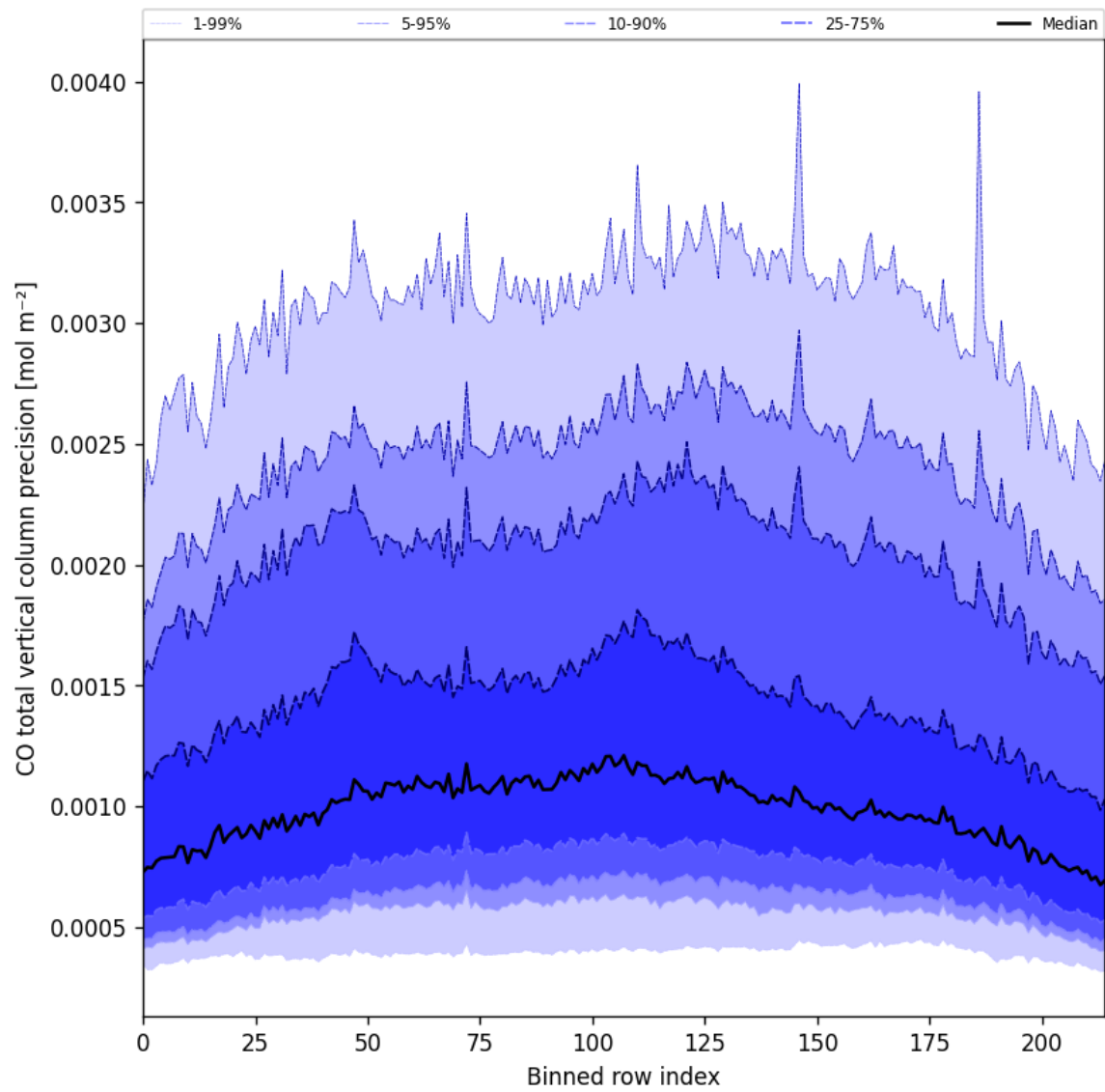
Figure 28: Along track statistics of “CO total vertical column precision” for 2025-07-10 to 2025-07-12
