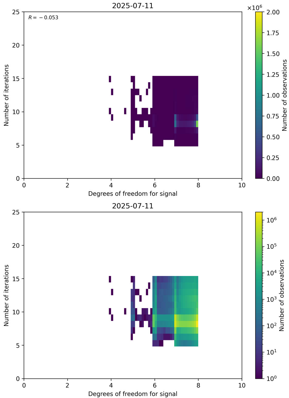
Figure 50: Scatter density plot of “Degrees of freedom for signal” against “Number of iterations” for 2025-07-10 to 2025-07-12.
