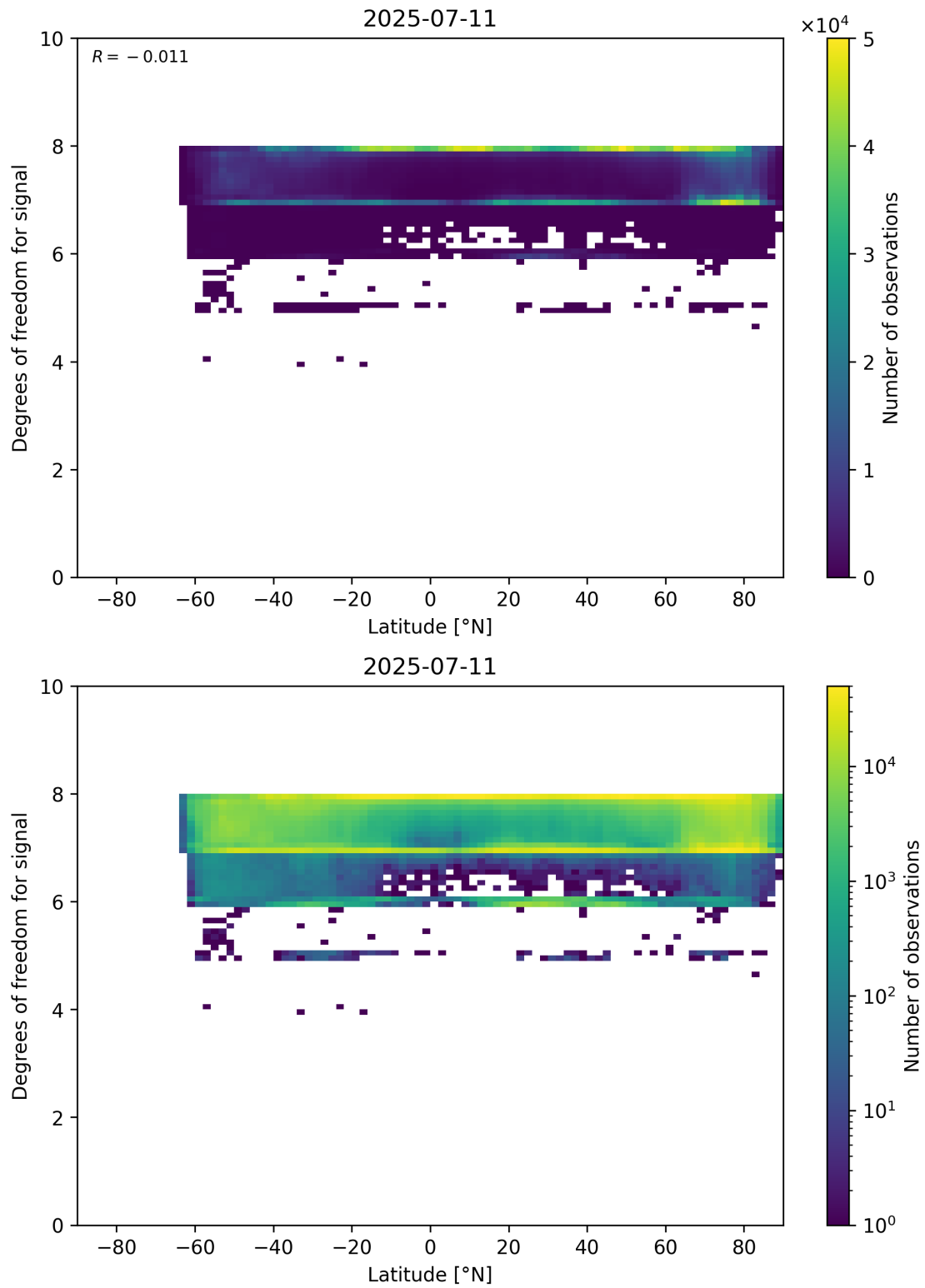
Figure 55: Scatter density plot of “Latitude” against “Degrees of freedom for signal” for 2025-07-10 to 2025-07-12.
