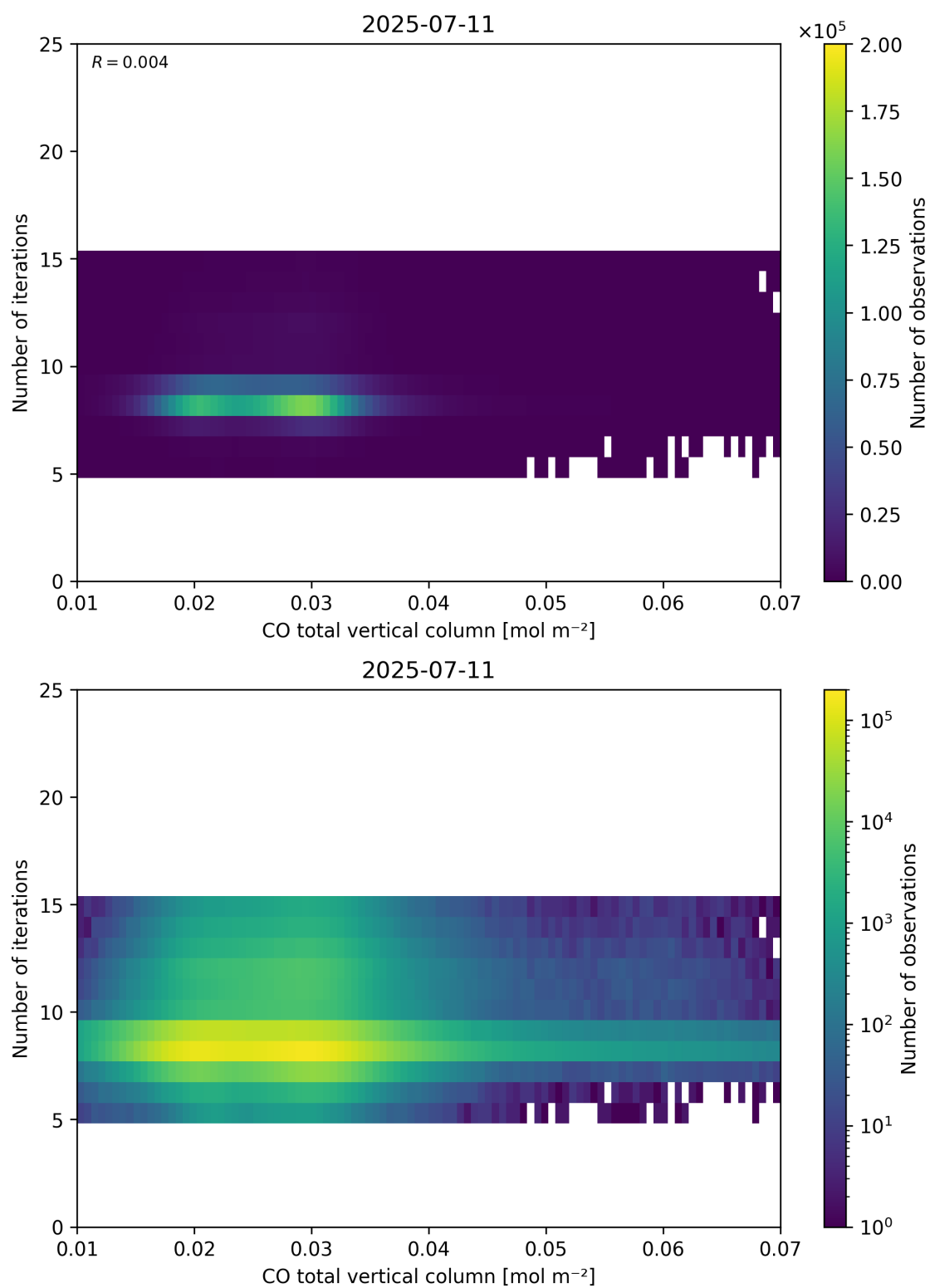
Figure 42: Scatter density plot of “CO total vertical column” against “Number of iterations” for 2025-07-10 to 2025-07-12.
