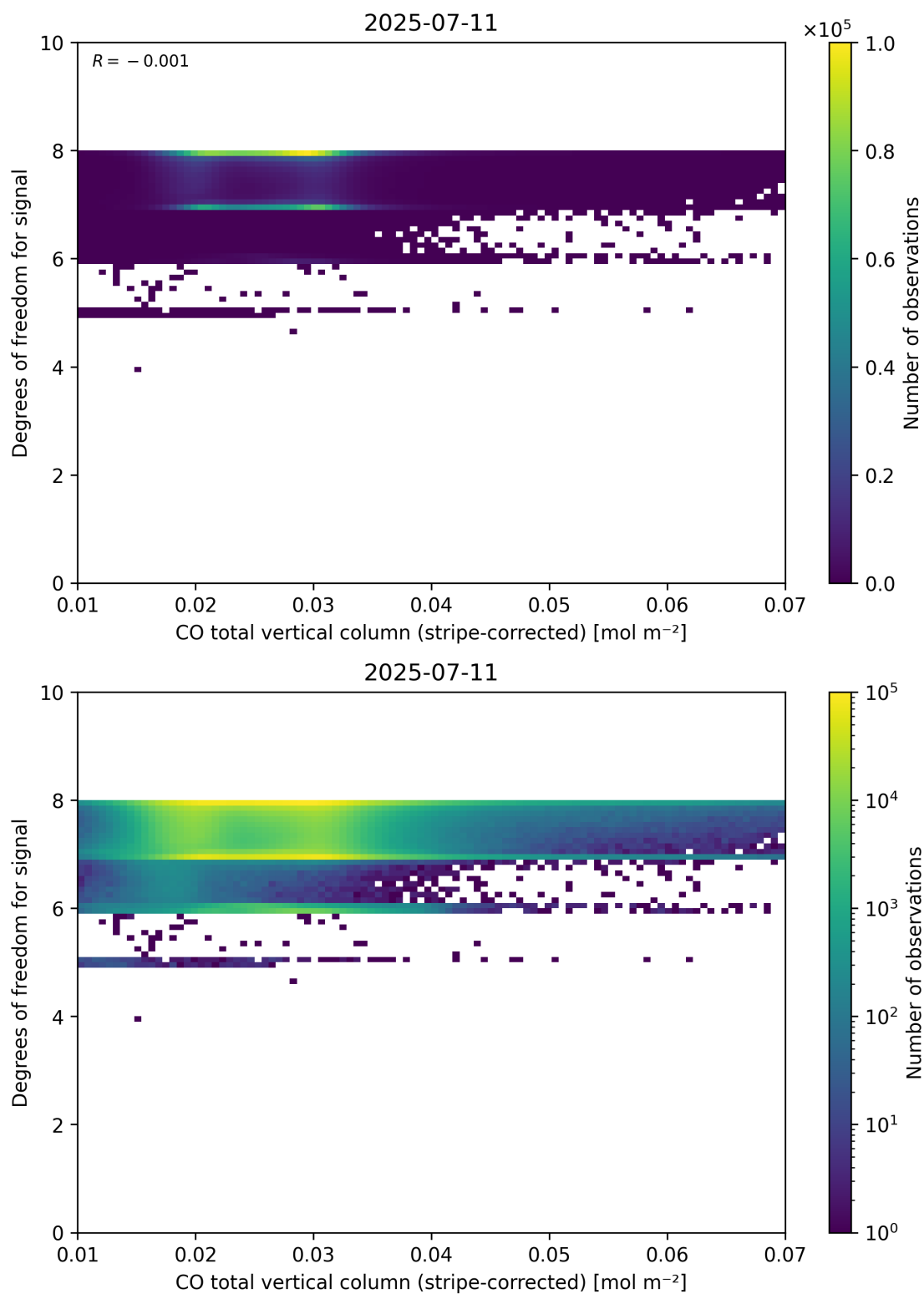
Figure 38: Scatter density plot of “CO total vertical column (stripe-corrected)” against “Degrees of freedom for signal” for 2025-07-10 to 2025-07-12.
