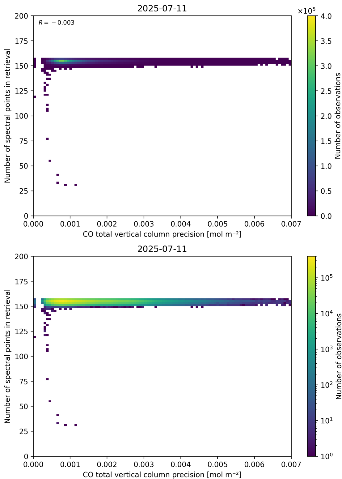
Figure 47: Scatter density plot of “CO total vertical column precision” against “Number of spectral points in retrieval” for 2025-07-10 to 2025-07-12.
