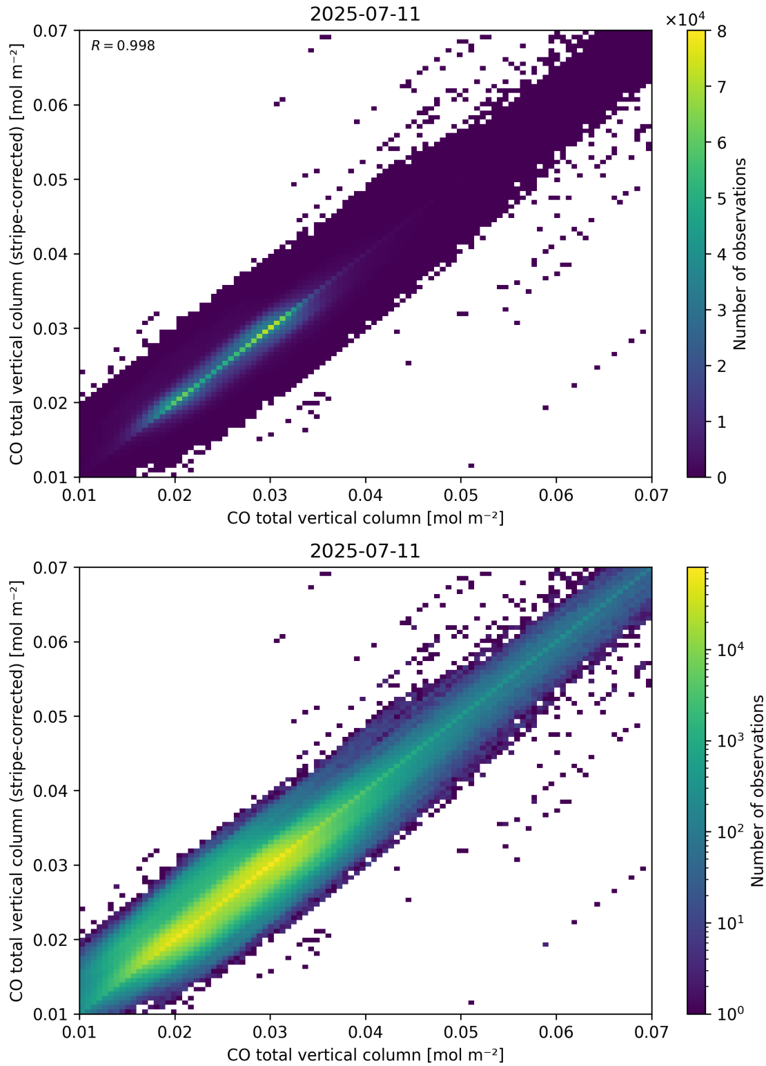
Figure 33: Scatter density plot of “CO total vertical column” against “CO total vertical column (stripe-corrected)” for 2025-07-10 to 2025-07-12.
