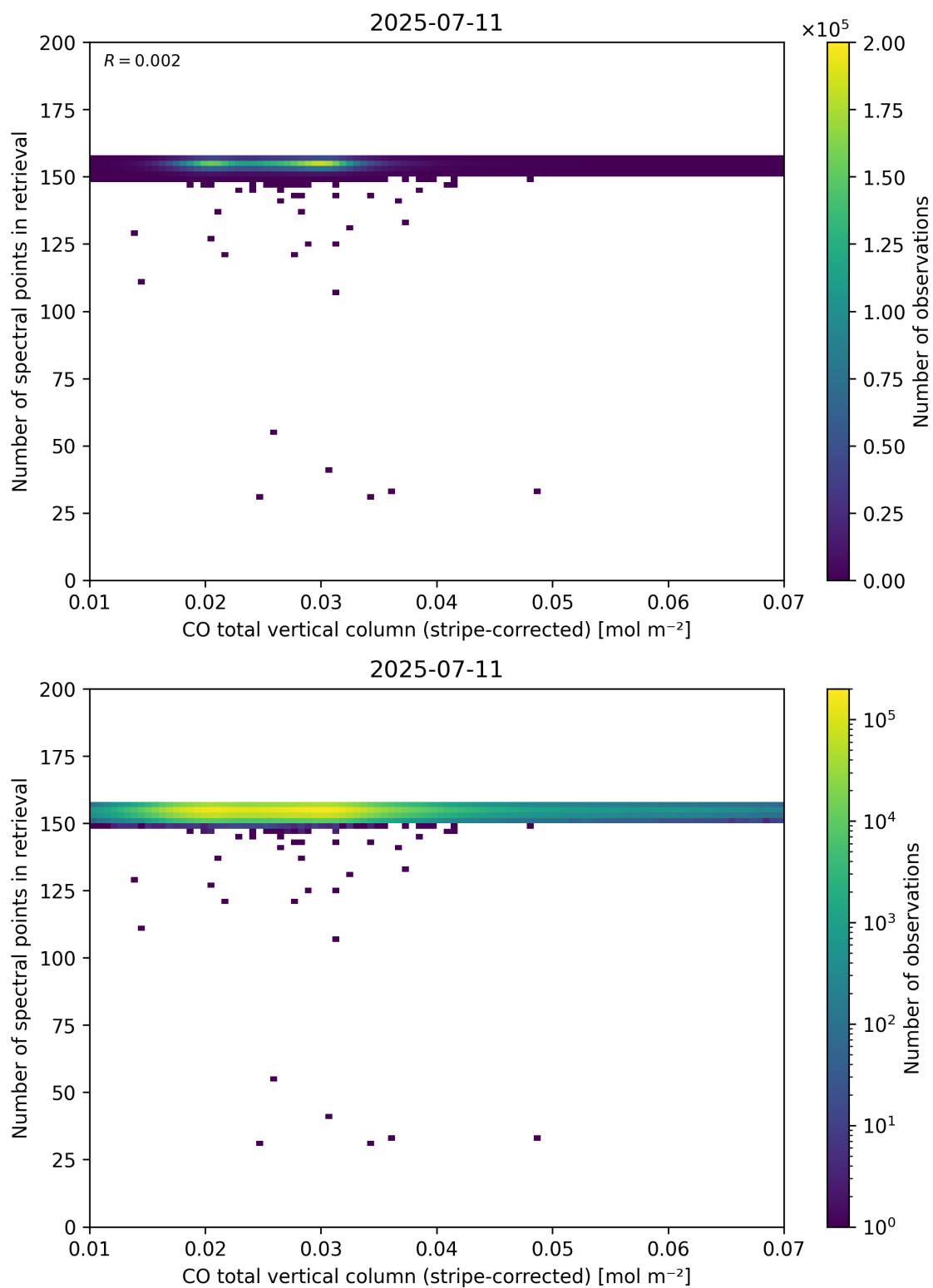
Figure 40: Scatter density plot of “CO total vertical column (stripe-corrected)” against “Number of spectral points in retrieval” for 2025-07-10 to 2025-07-12.
