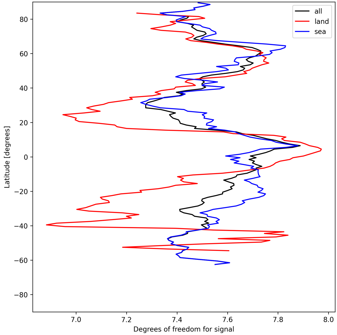
Figure 15: Zonal average of “Degrees of freedom for signal” for 2025-07-10 to 2025-07-12.
