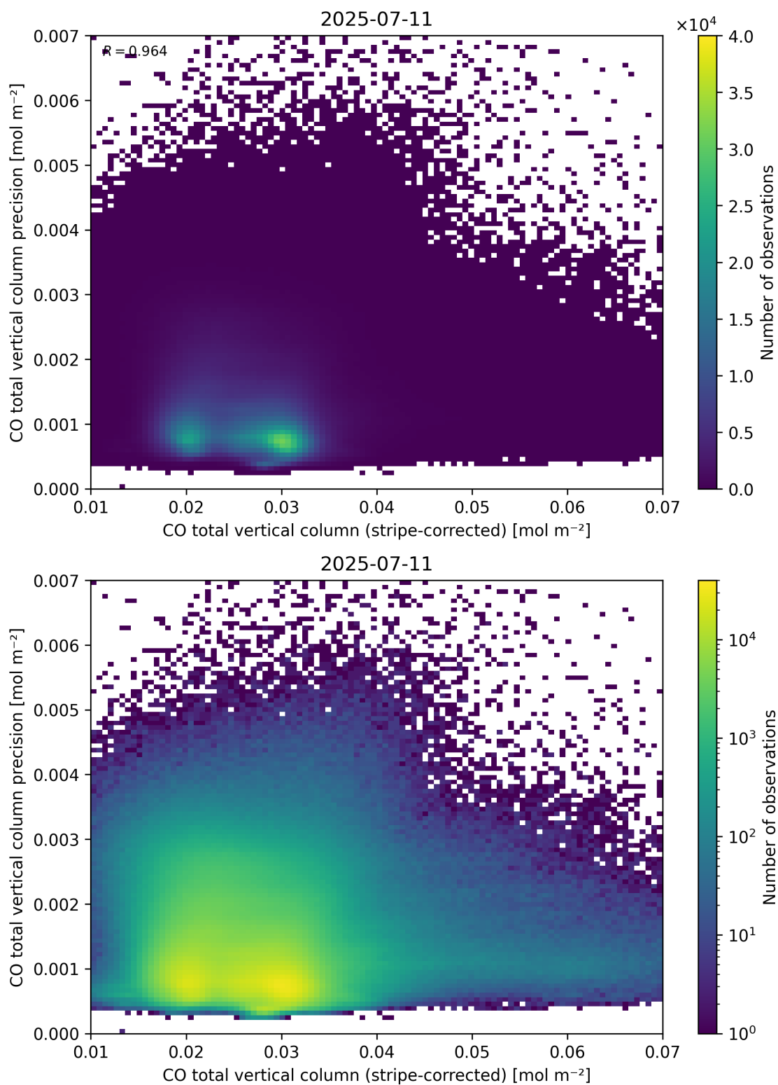
Figure 36: Scatter density plot of “CO total vertical column (stripe-corrected)” against “CO total vertical column precision” for 2025-07-10 to 2025-07-12.
