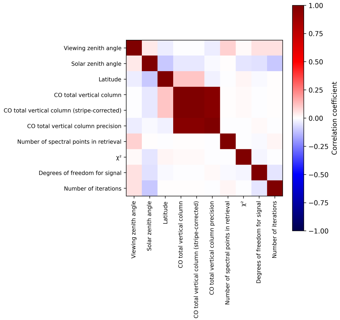
Figure 2: Map of correlation matrix for 2025-07-10 to 2025-07-12.
