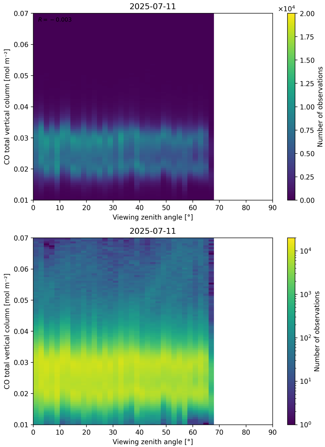
Figure 69: Scatter density plot of “Viewing zenith angle” against “CO total vertical column” for 2025-07-10 to 2025-07-12.
