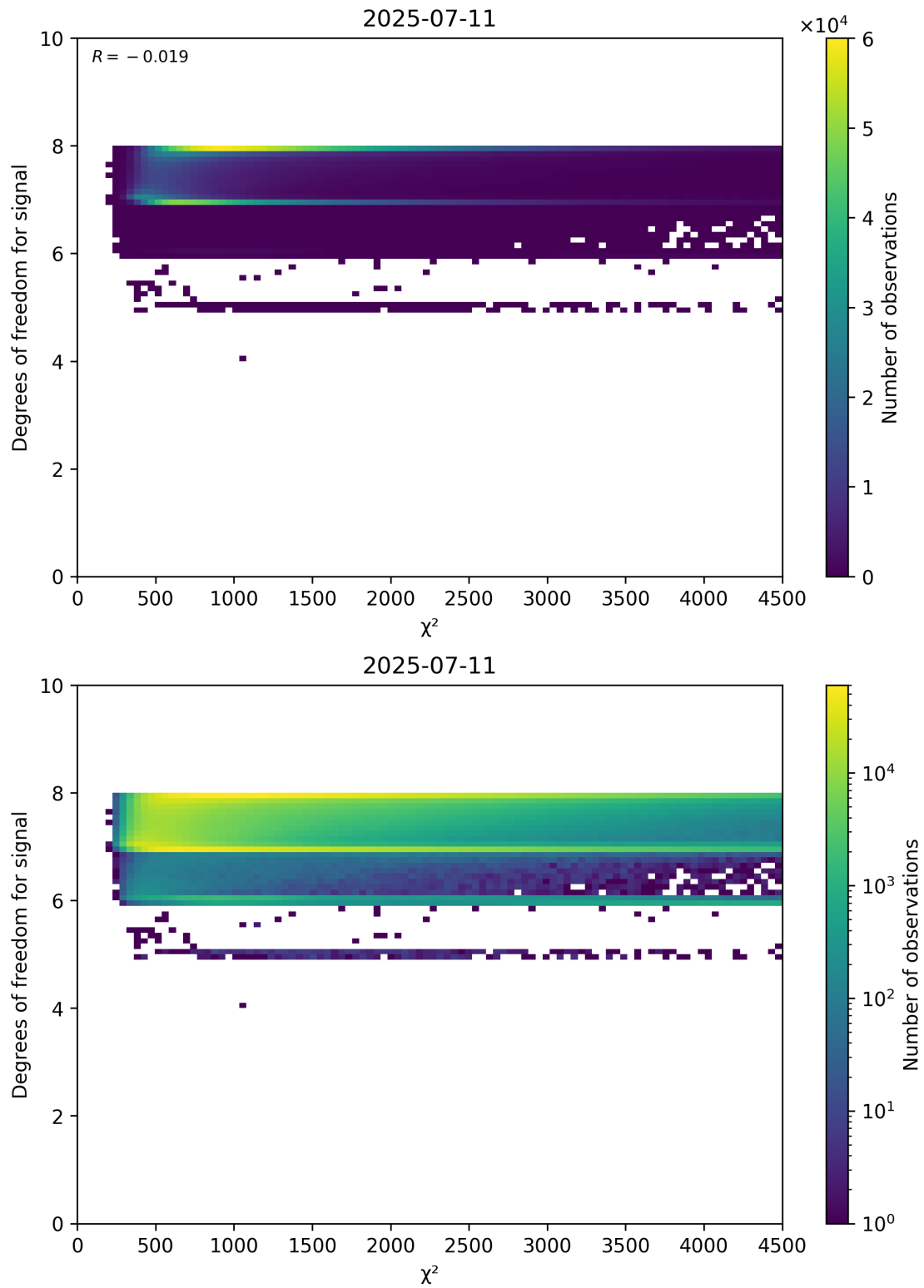
Figure 48: Scatter density plot of “ \chi^2 ” against “Degrees of freedom for signal” for 2025-07-10 to 2025-07-12.
