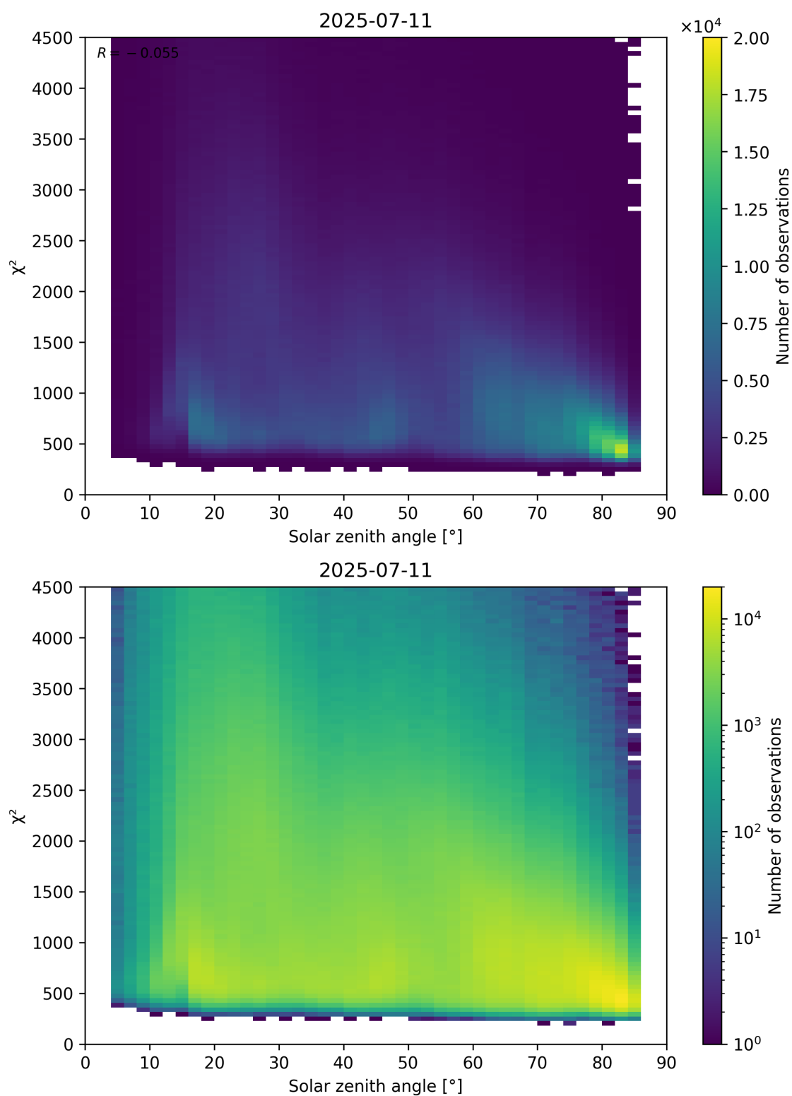
Figure 64: Scatter density plot of “Solar zenith angle” against “ \chi^2 ” for 2025-07-10 to 2025-07-12.
