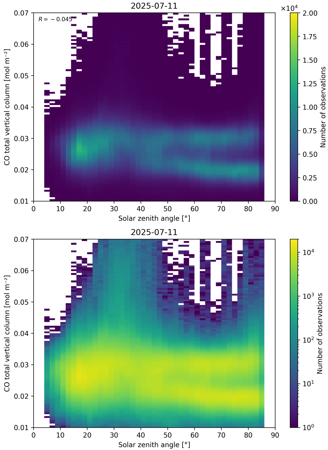
Figure 61: Scatter density plot of “Solar zenith angle” against “CO total vertical column” for 2025-07-10 to 2025-07-12.
