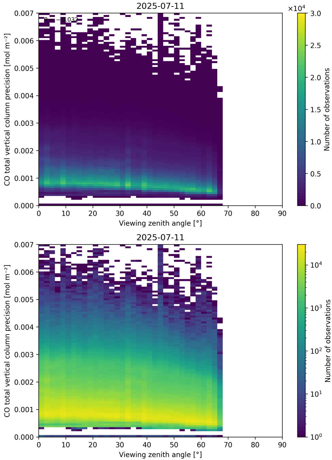
Figure 71: Scatter density plot of “Viewing zenith angle” against “CO total vertical column precision” for 2025-07-10 to 2025-07-12.
