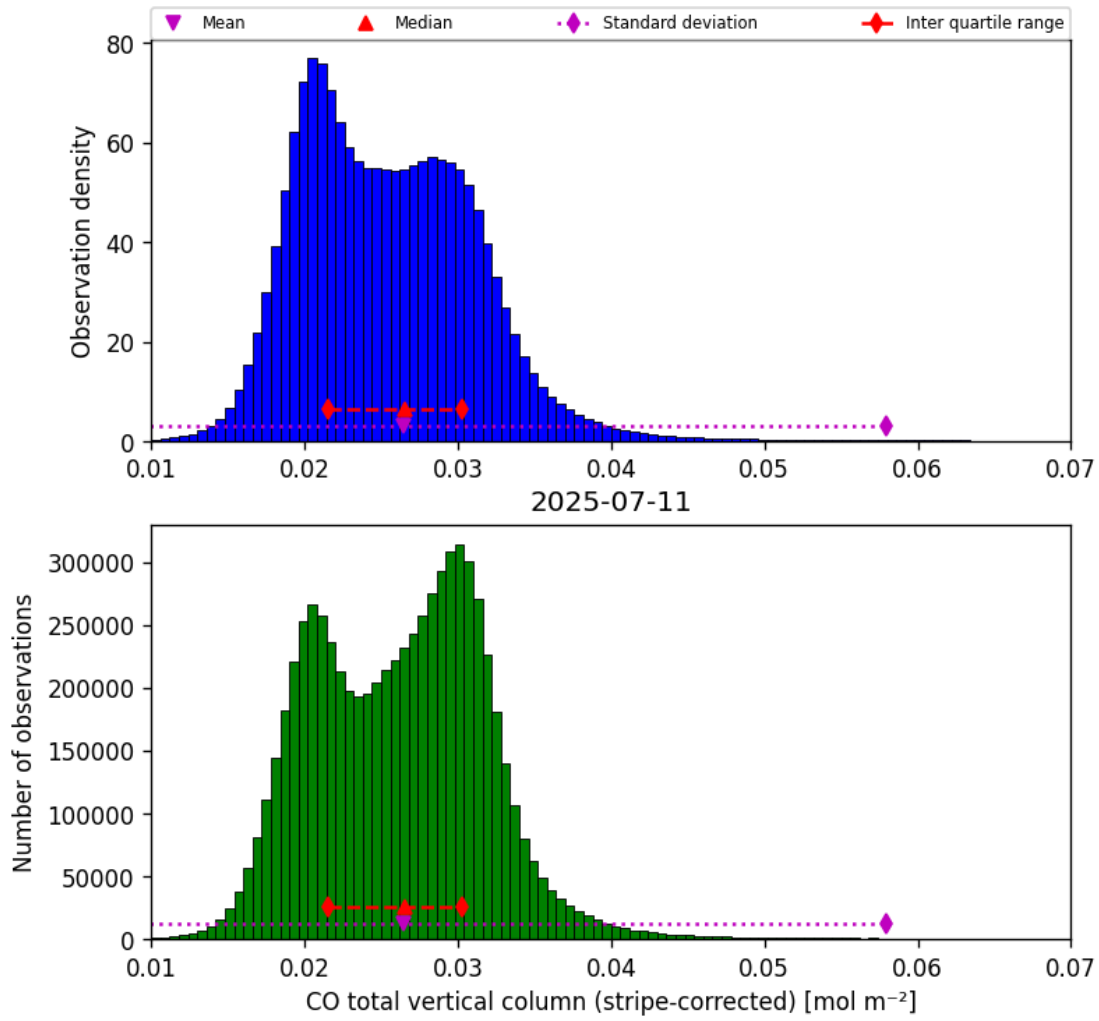
Figure 19: Histogram of “CO total vertical column (stripe-corrected)” for 2025-07-10 to 2025-07-12
