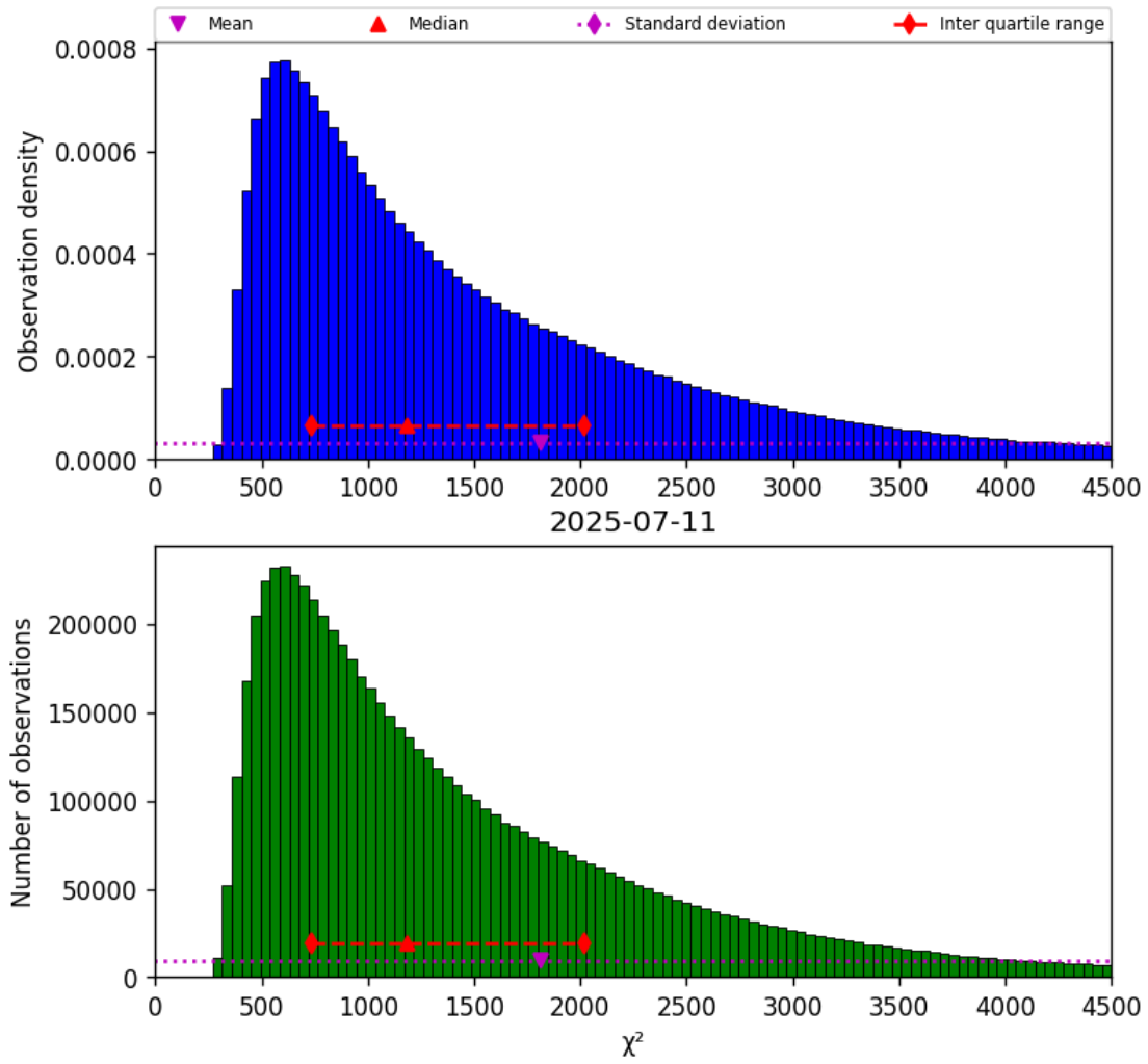
Figure 22: Histogram of “ \chi^2 ” for 2025-07-10 to 2025-07-12
