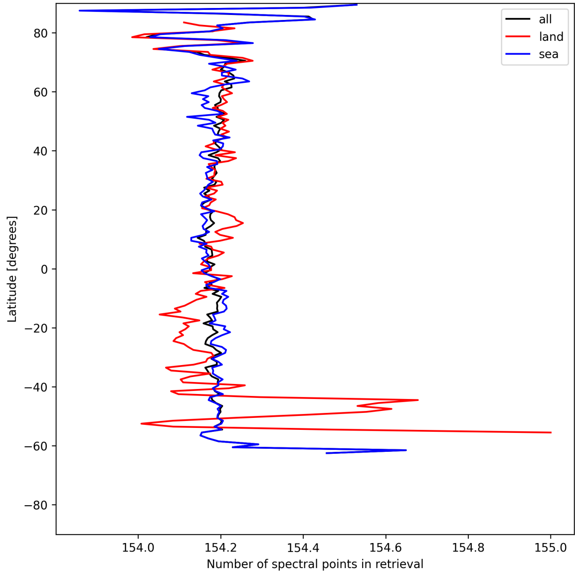
Figure 13: Zonal average of “Number of spectral points in retrieval” for 2025-07-11 to 2025-07-13.
