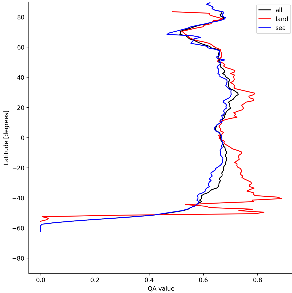
Figure 9: Zonal average of “QA value” for 2025-07-11 to 2025-07-13.
