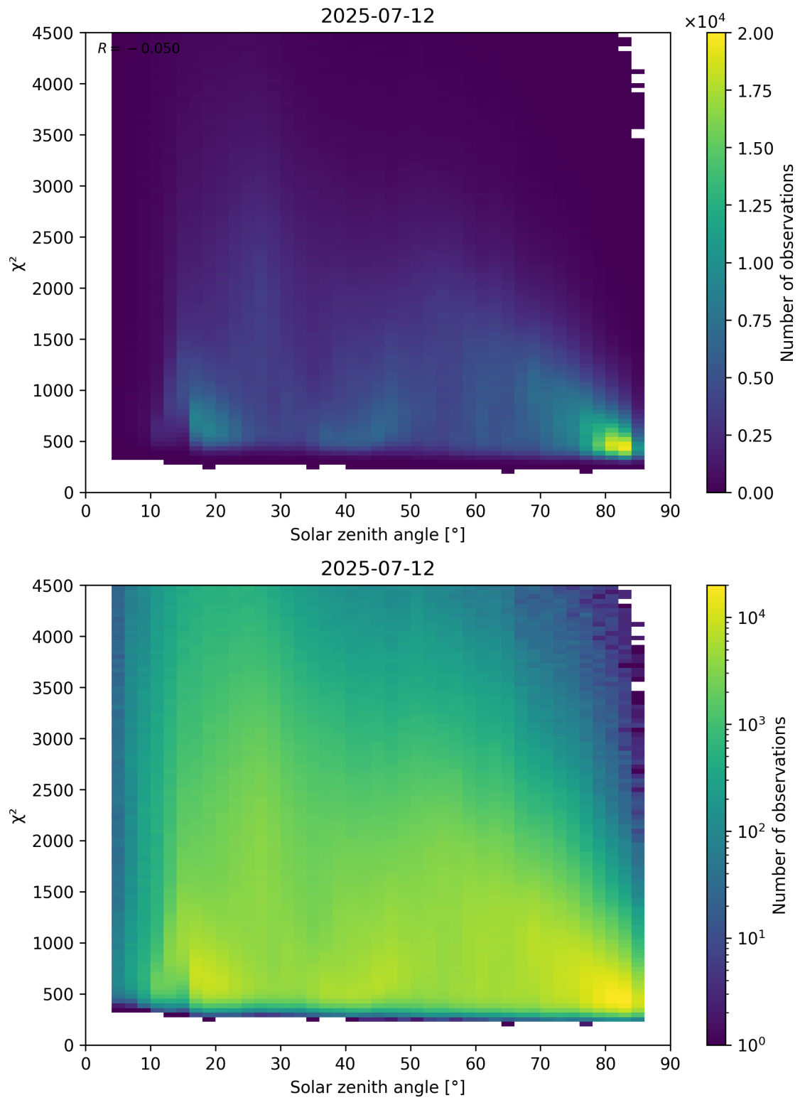
Figure 64: Scatter density plot of “Solar zenith angle” against “ \chi^2 ” for 2025-07-11 to 2025-07-13.
