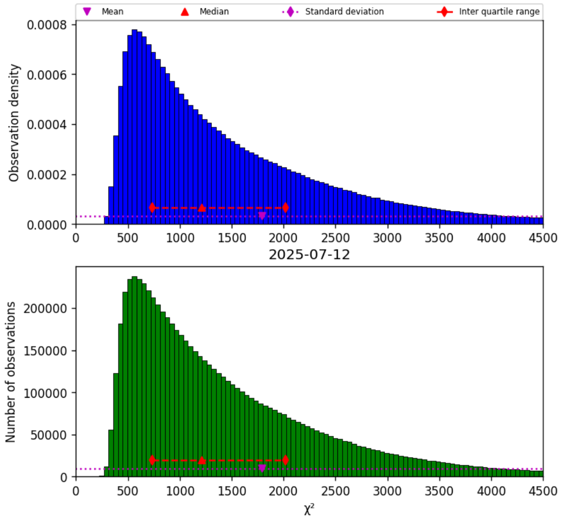
Figure 22: Histogram of “ \chi^2 ” for 2025-07-11 to 2025-07-13
