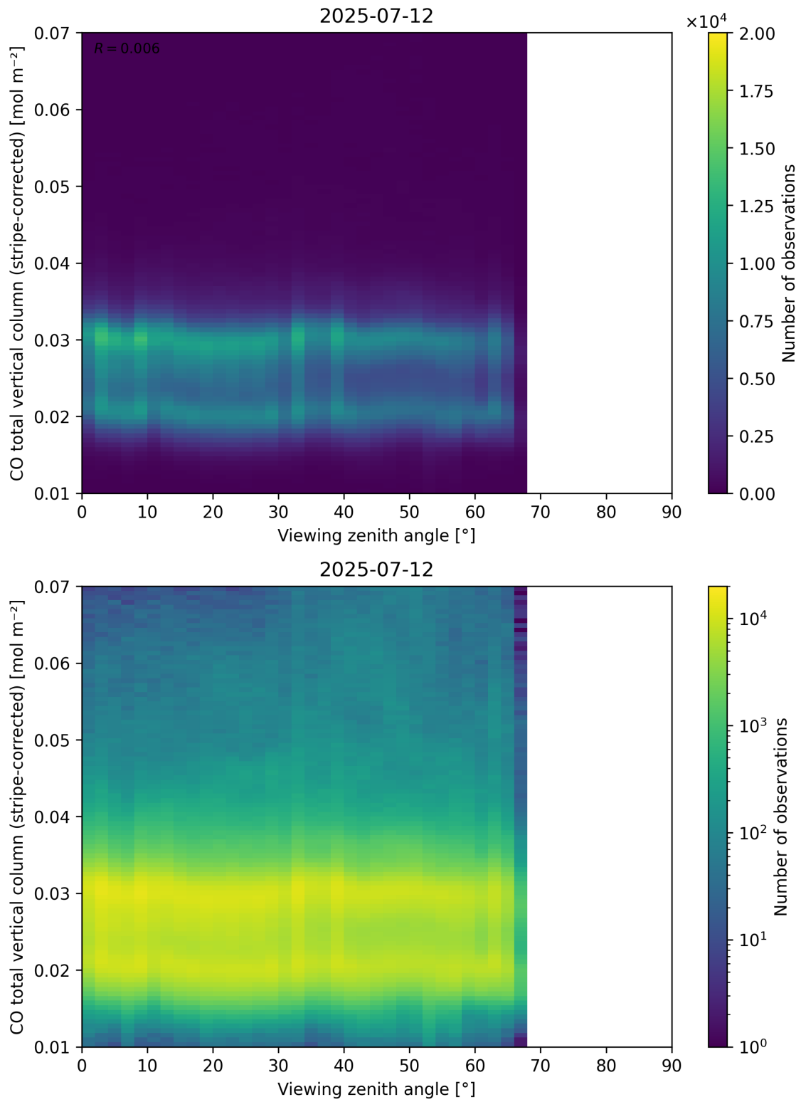
Figure 70: Scatter density plot of “Viewing zenith angle” against “CO total vertical column (stripe-corrected)” for 2025-07-11 to 2025-07-13.
