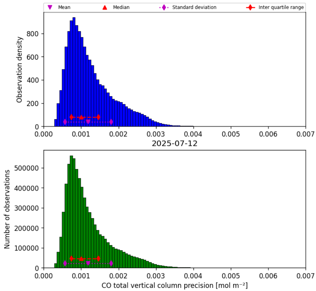
Figure 20: Histogram of “CO total vertical column precision” for 2025-07-11 to 2025-07-13
