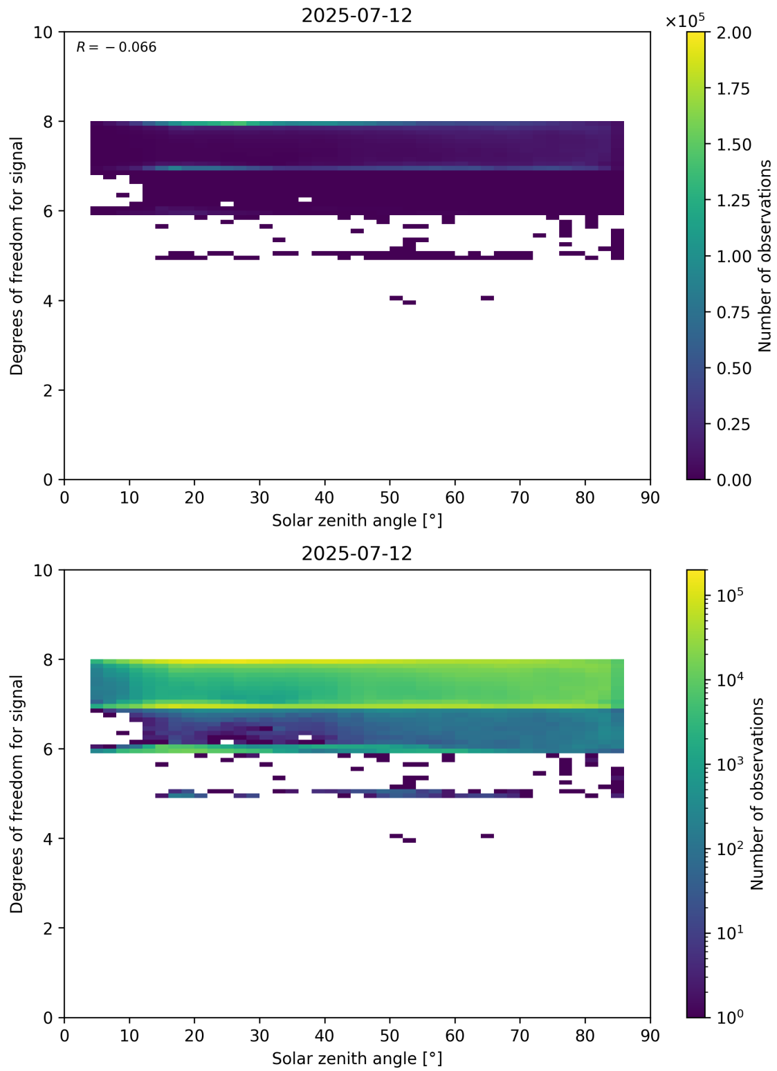
Figure 65: Scatter density plot of “Solar zenith angle” against “Degrees of freedom for signal” for 2025-07-11 to 2025-07-13.
