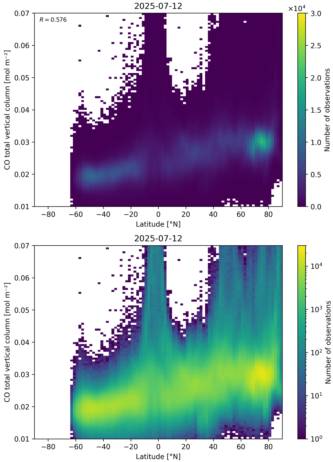
Figure 51: Scatter density plot of “Latitude” against “CO total vertical column” for 2025-07-11 to 2025-07-13.
