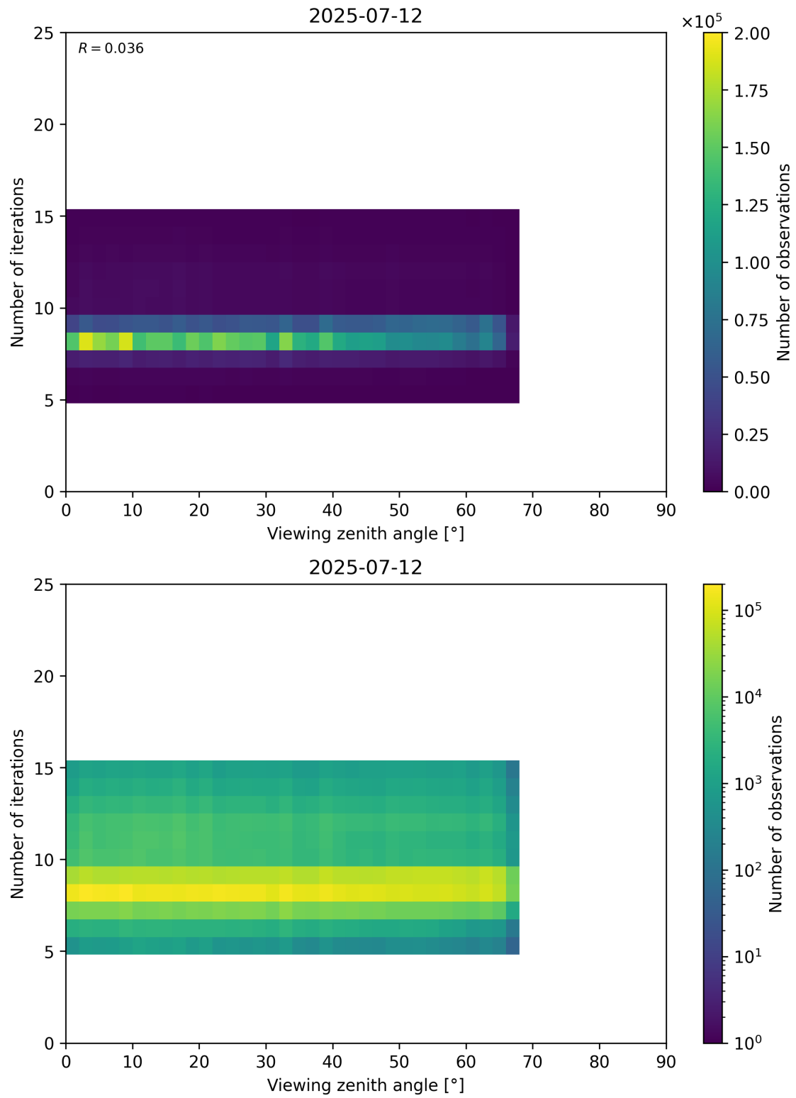
Figure 75: Scatter density plot of “Viewing zenith angle” against “Number of iterations” for 2025-07-11 to 2025-07-13.
