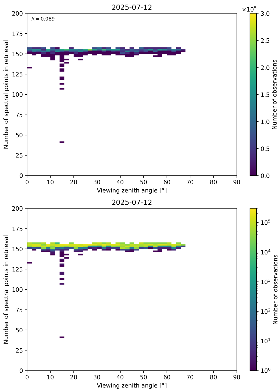
Figure 76: Scatter density plot of “Viewing zenith angle” against “Number of spectral points in retrieval” for 2025-07-11 to 2025-07-13.
