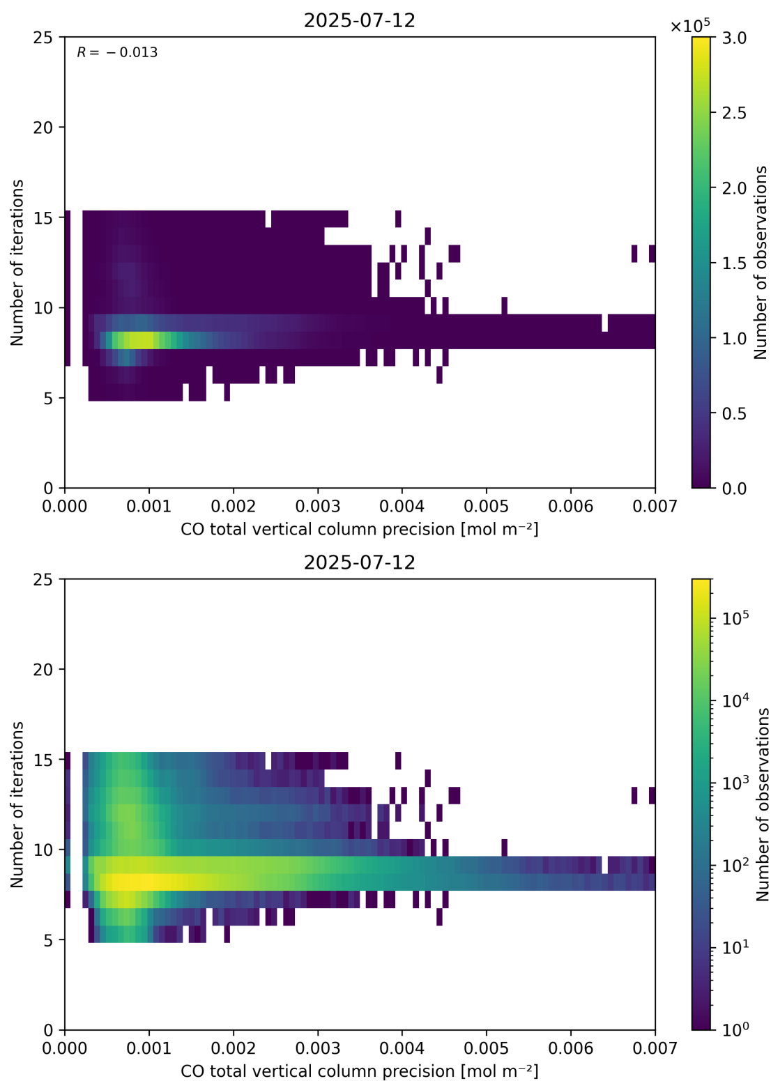
Figure 46: Scatter density plot of “CO total vertical column precision” against “Number of iterations” for 2025-07-11 to 2025-07-13.
