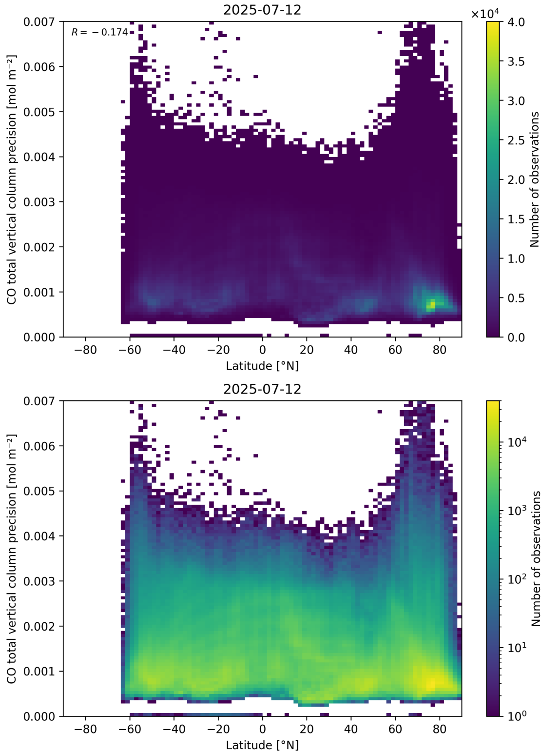
Figure 53: Scatter density plot of “Latitude” against “CO total vertical column precision” for 2025-07-11 to 2025-07-13.
