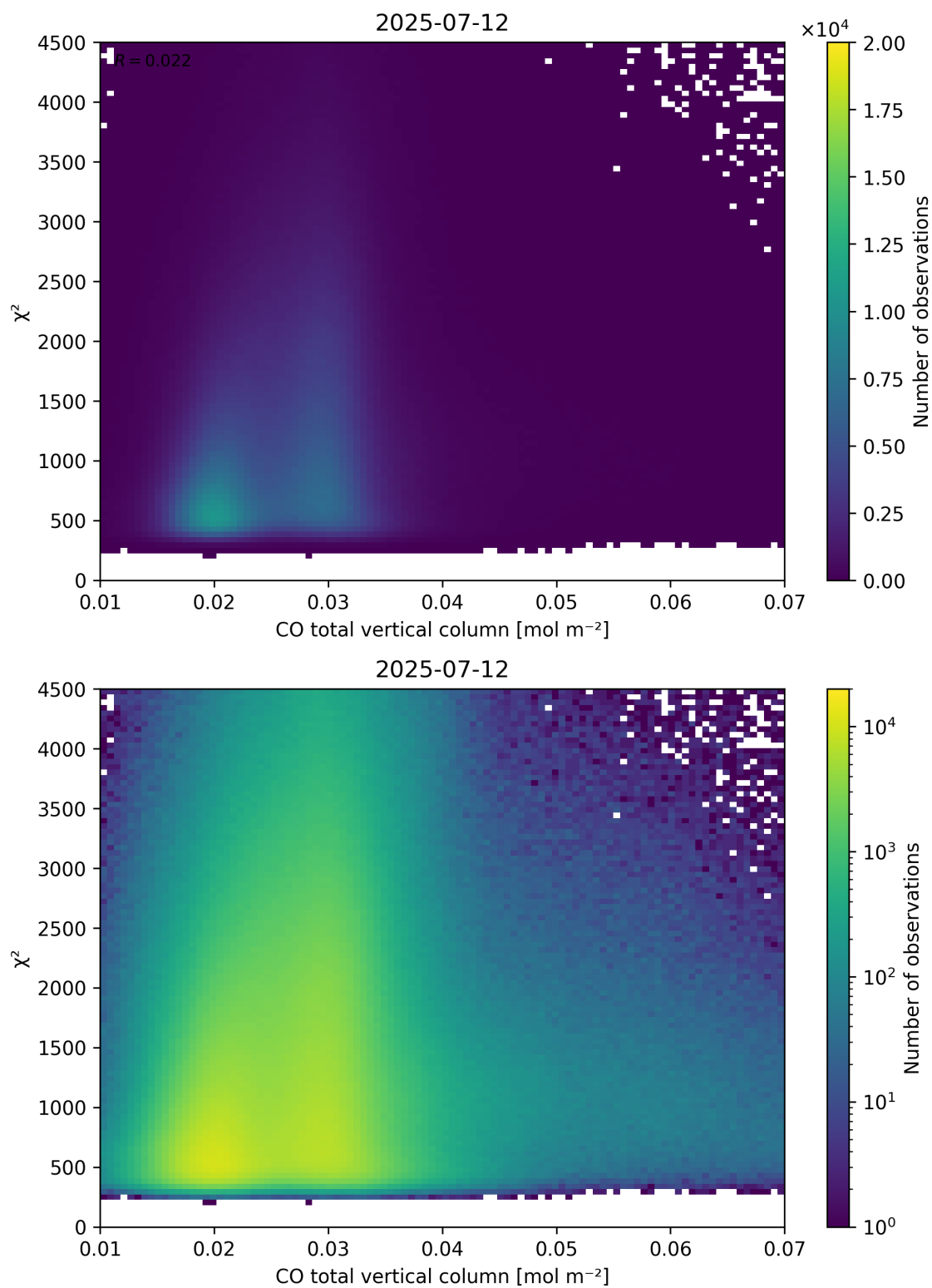
Figure 35: Scatter density plot of “CO total vertical column” against “ \chi^2 ” for 2025-07-11 to 2025-07-13.
