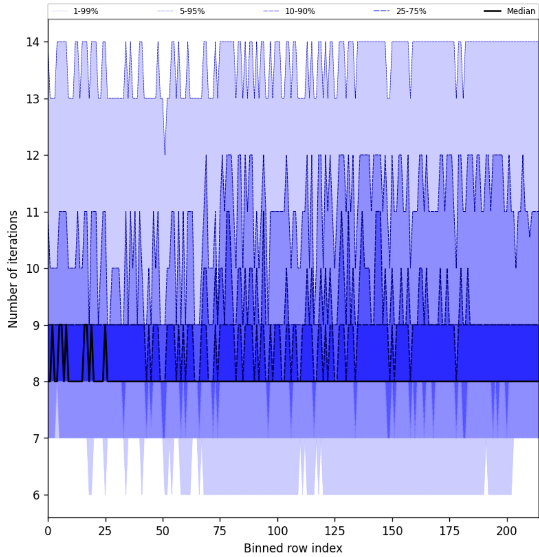
Figure 32: Along track statistics of “Number of iterations” for 2025-07-11 to 2025-07-13
