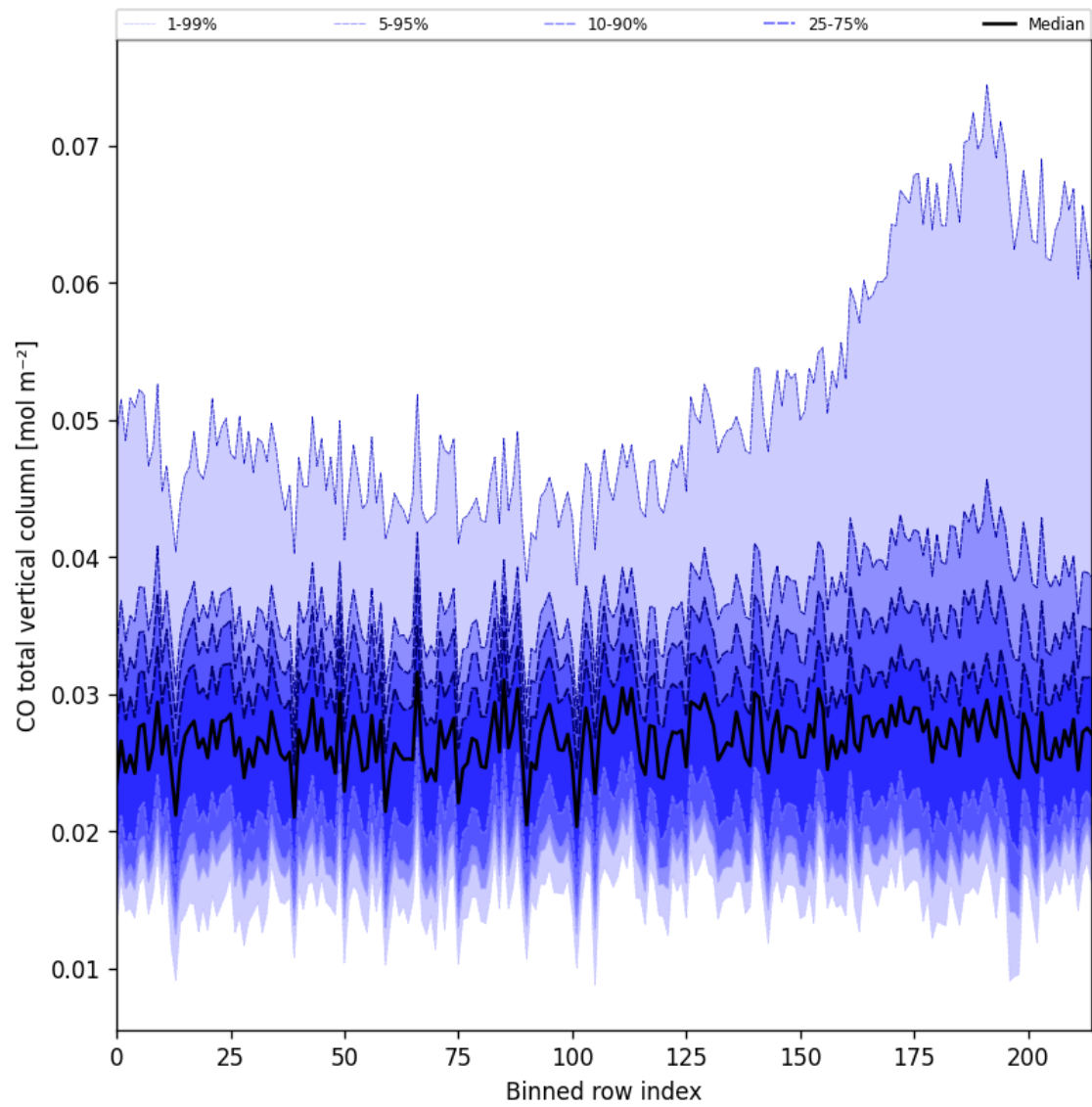
Figure 26: Along track statistics of “CO total vertical column” for 2025-07-11 to 2025-07-13
