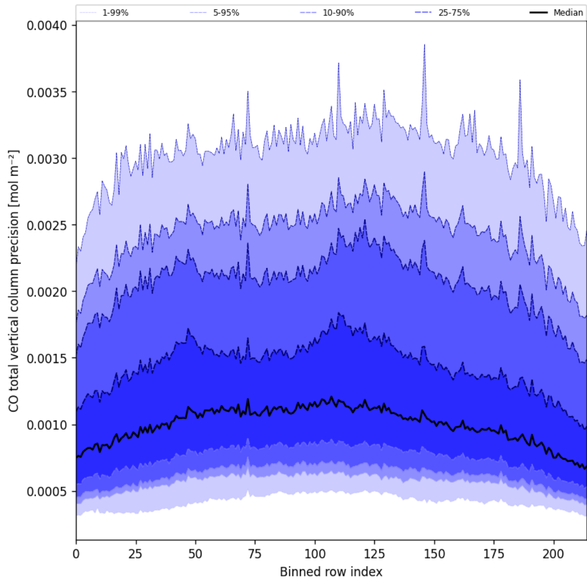
Figure 28: Along track statistics of “CO total vertical column precision” for 2025-07-11 to 2025-07-13
