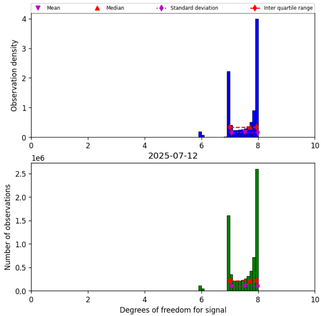
Figure 23: Histogram of “Degrees of freedom for signal” for 2025-07-11 to 2025-07-13
