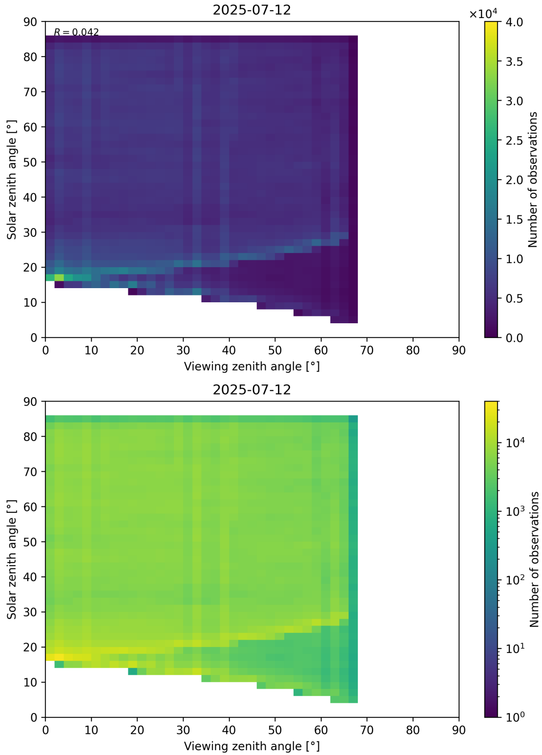
Figure 77: Scatter density plot of “Viewing zenith angle” against “Solar zenith angle” for 2025-07-11 to 2025-07-13.
