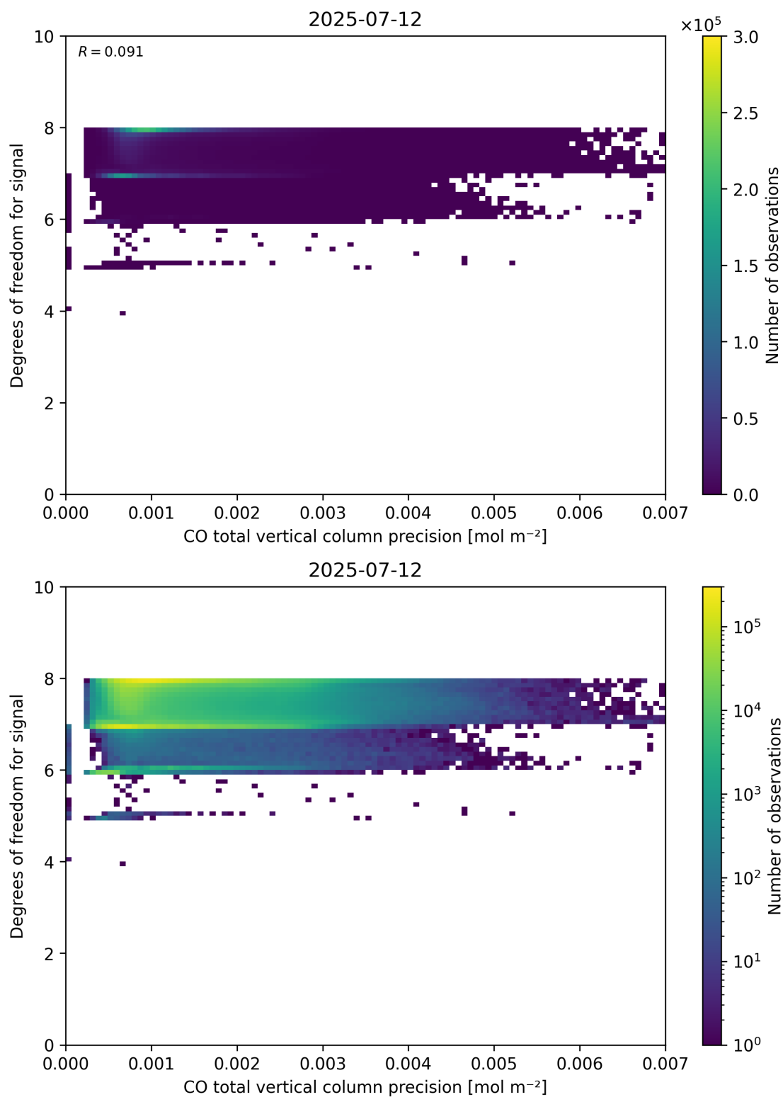
Figure 45: Scatter density plot of “CO total vertical column precision” against “Degrees of freedom for signal” for 2025-07-11 to 2025-07-13.
