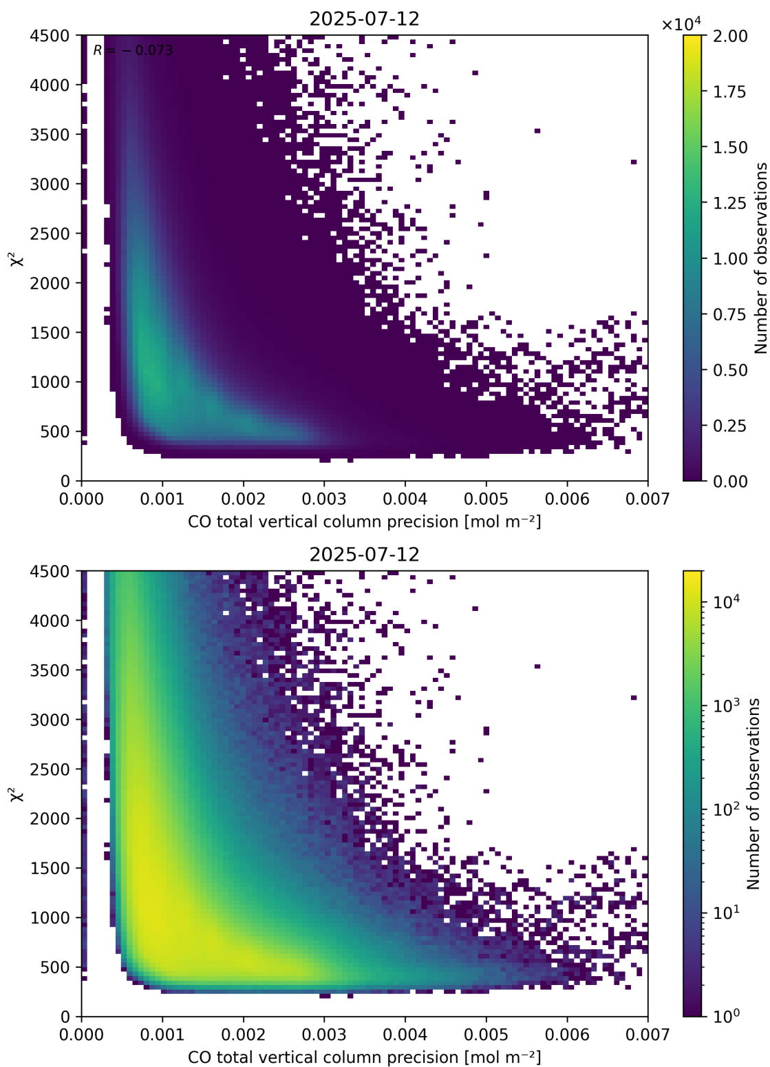
Figure 44: Scatter density plot of “CO total vertical column precision” against “ \chi^2 ” for 2025-07-11 to 2025-07-13.
