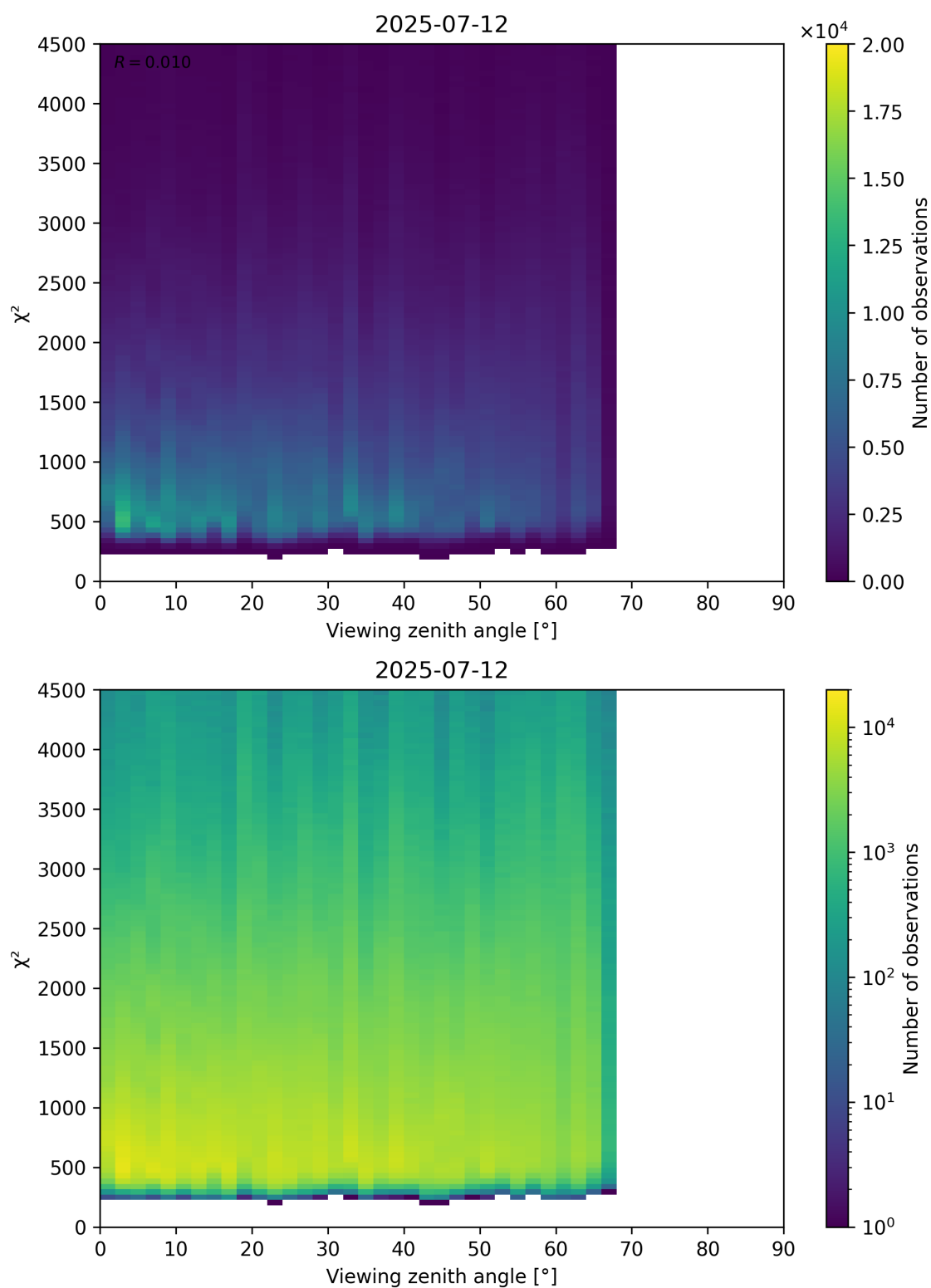
Figure 72: Scatter density plot of “Viewing zenith angle” against “ \chi^2 ” for 2025-07-11 to 2025-07-13.
