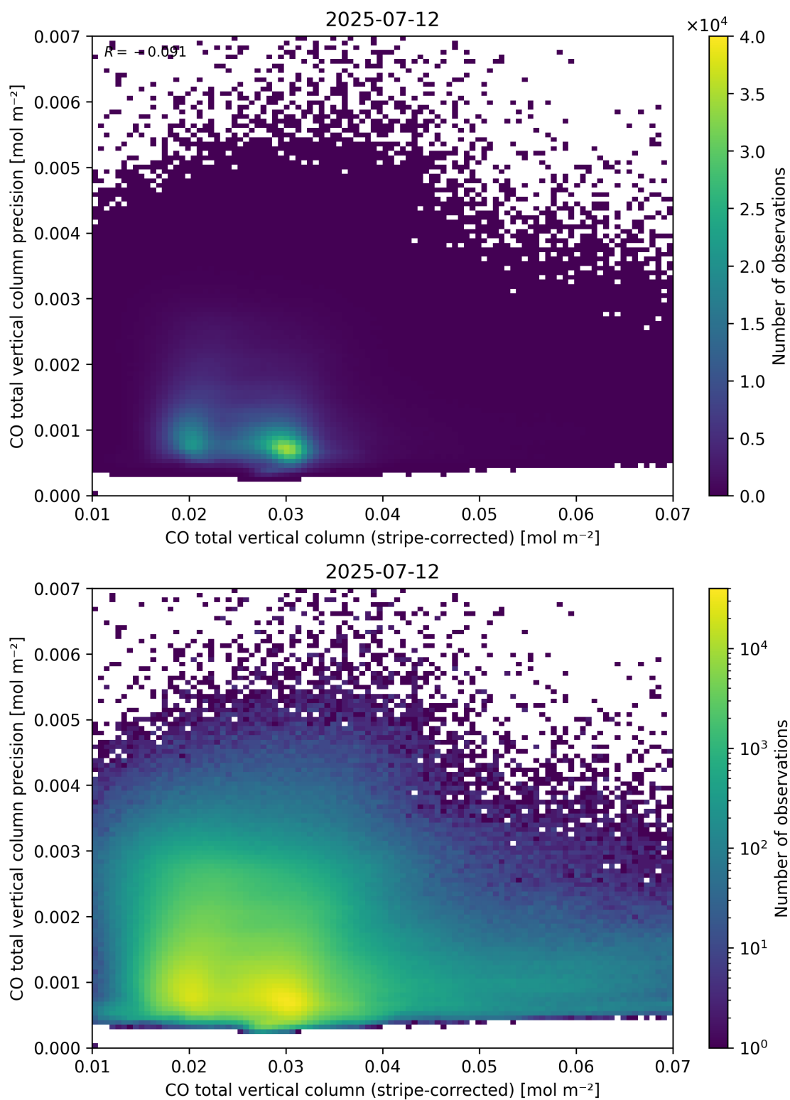
Figure 36: Scatter density plot of “CO total vertical column (stripe-corrected)” against “CO total vertical column precision” for 2025-07-11 to 2025-07-13.
