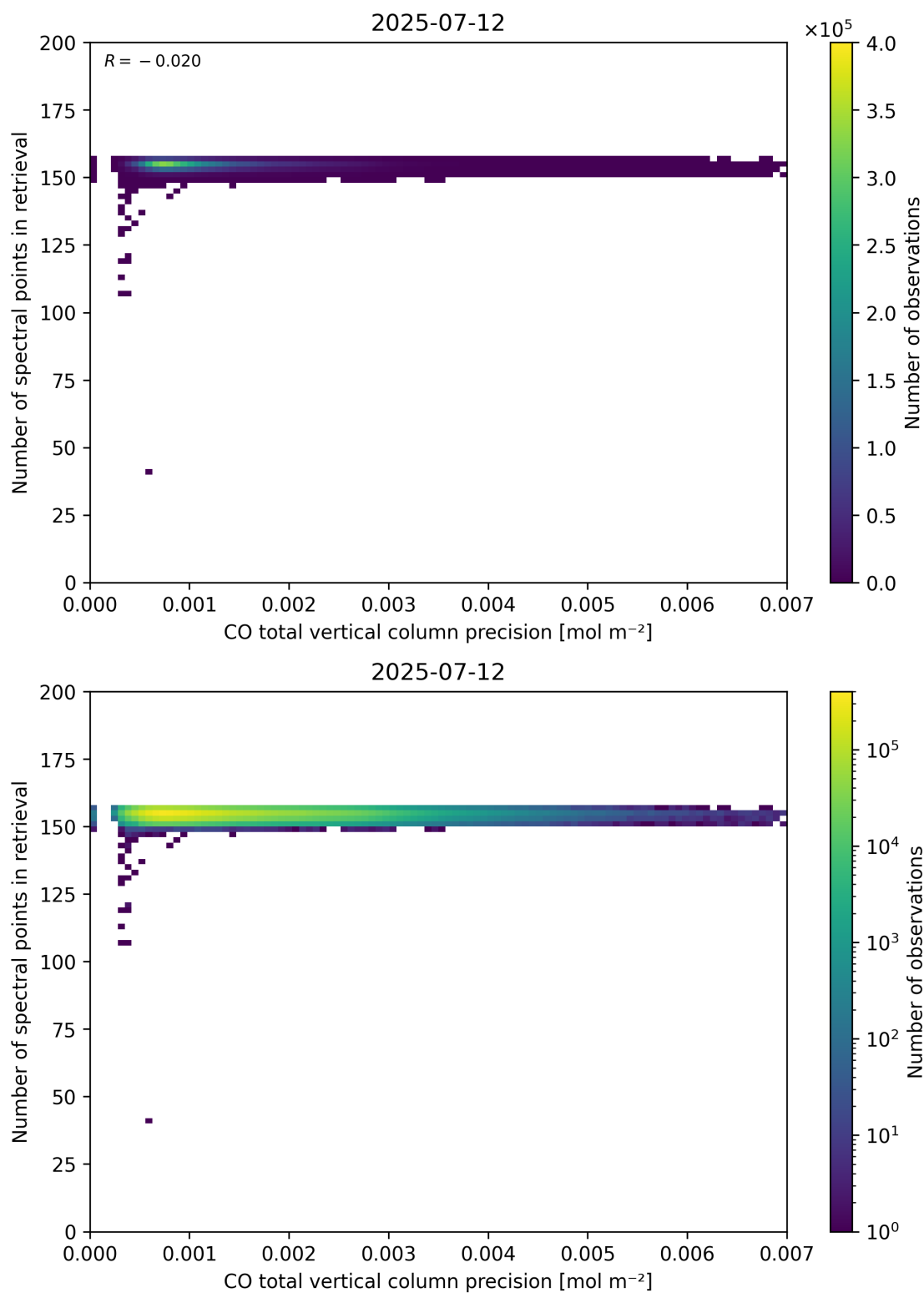
Figure 47: Scatter density plot of “CO total vertical column precision” against “Number of spectral points in retrieval” for 2025-07-11 to 2025-07-13.
