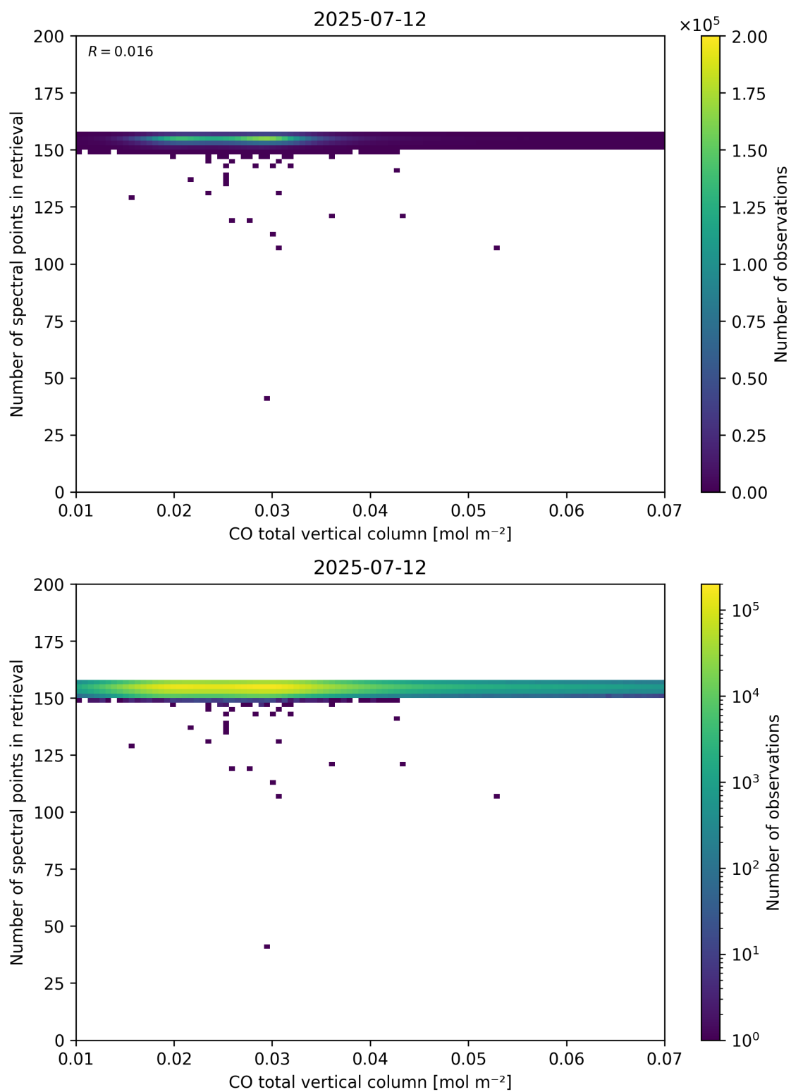
Figure 43: Scatter density plot of “CO total vertical column” against “Number of spectral points in retrieval” for 2025-07-11 to 2025-07-13.
