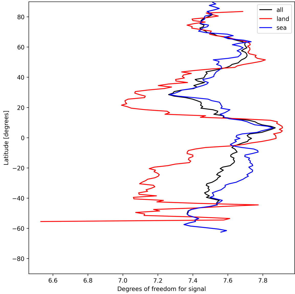
Figure 15: Zonal average of “Degrees of freedom for signal” for 2025-07-11 to 2025-07-13.
