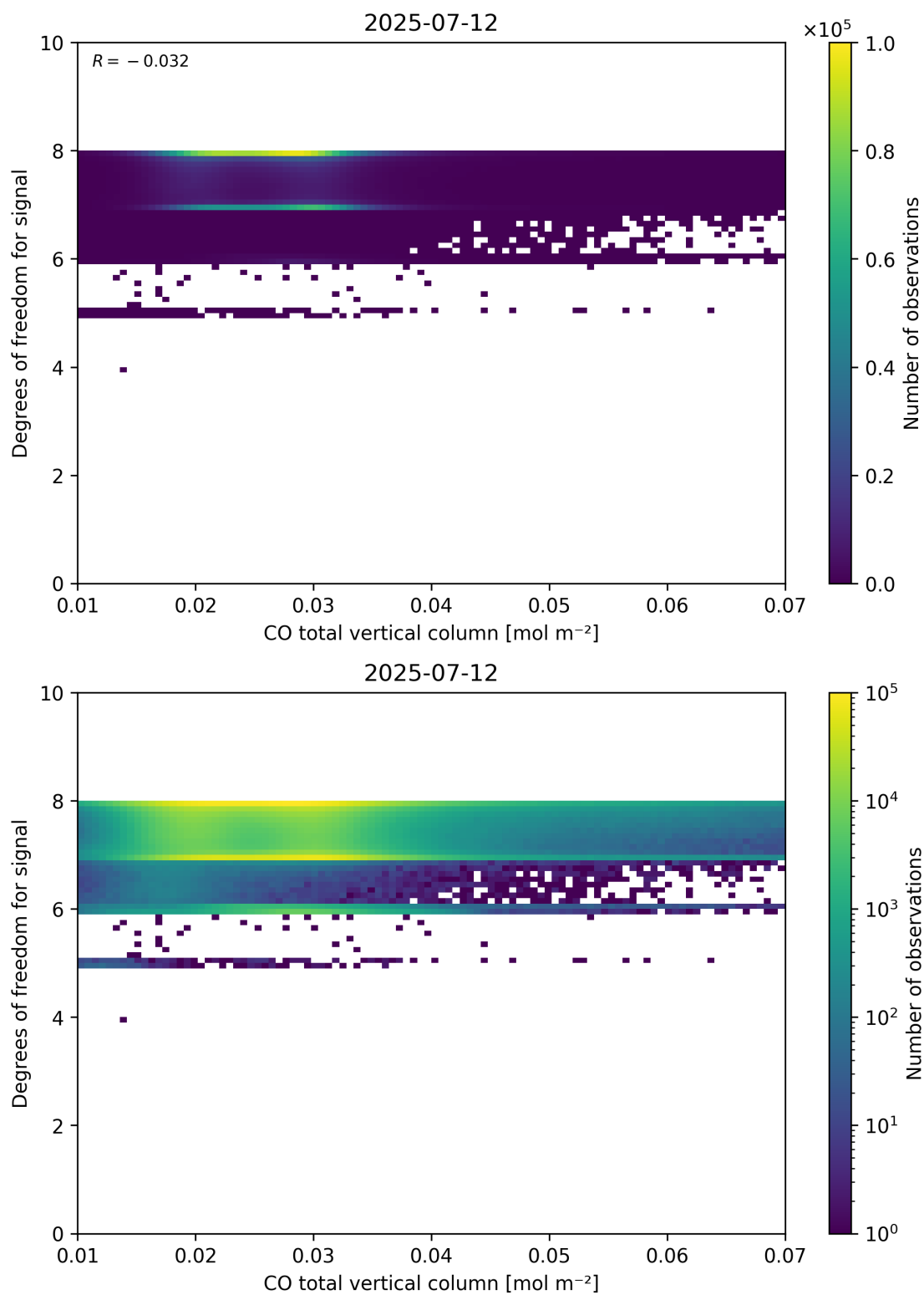
Figure 41: Scatter density plot of “CO total vertical column” against “Degrees of freedom for signal” for 2025-07-11 to 2025-07-13.
