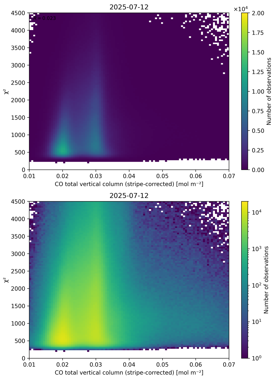
Figure 37: Scatter density plot of “CO total vertical column (stripe-corrected)” against “ \chi^2 ” for 2025-07-11 to 2025-07-13.
