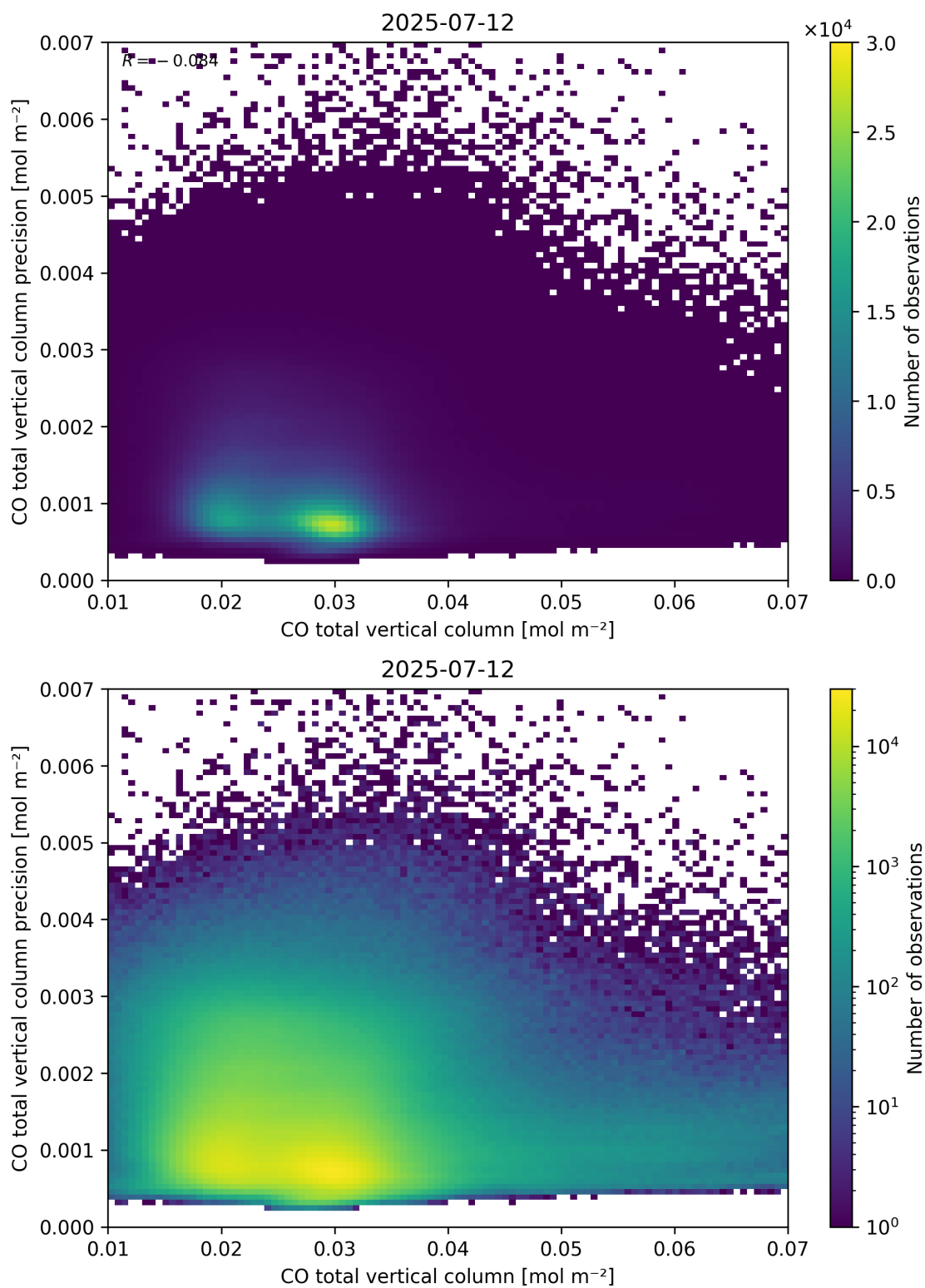
Figure 34: Scatter density plot of “CO total vertical column” against “CO total vertical column precision” for 2025-07-11 to 2025-07-13.
