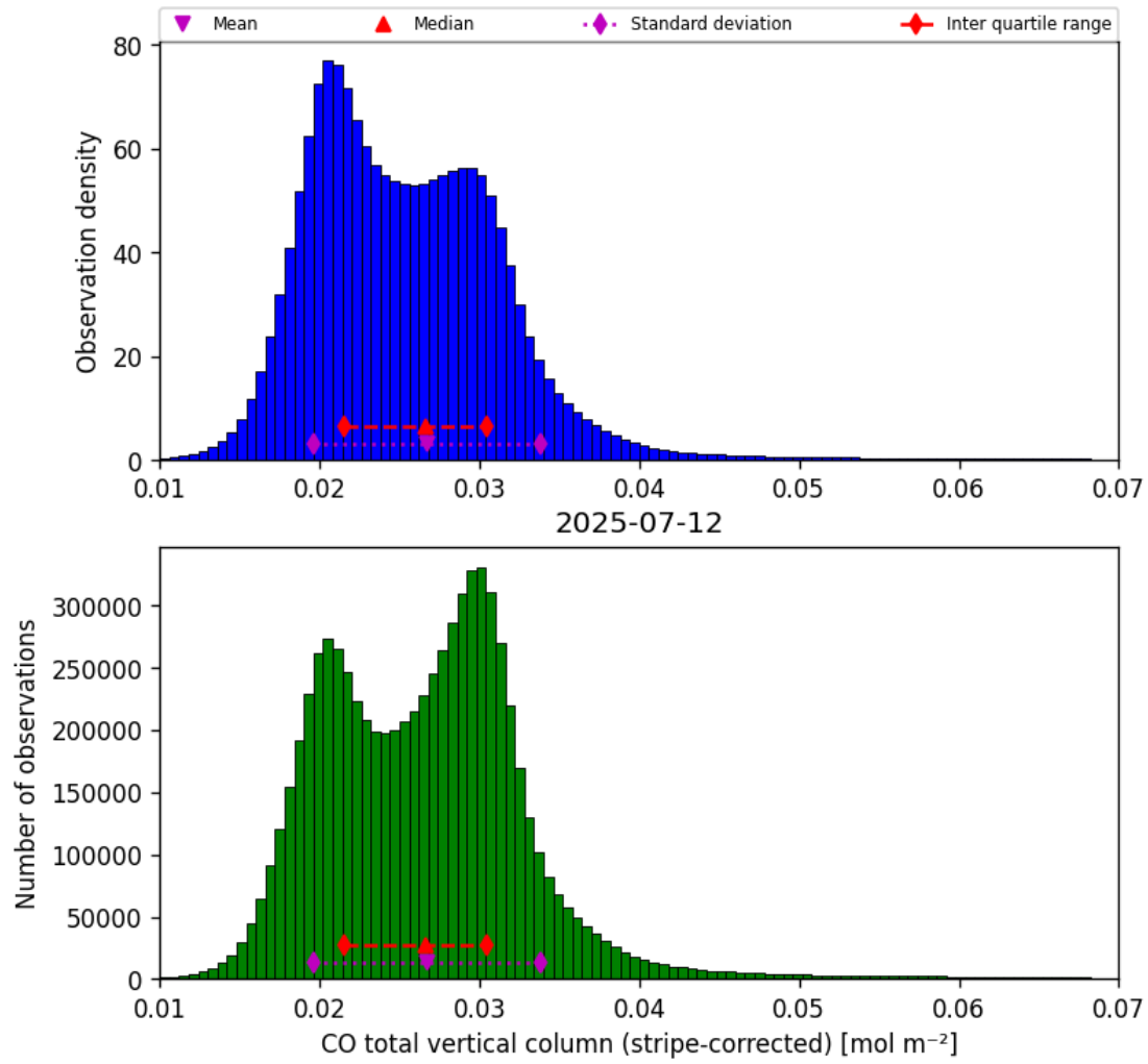
Figure 19: Histogram of “CO total vertical column (stripe-corrected)” for 2025-07-11 to 2025-07-13
