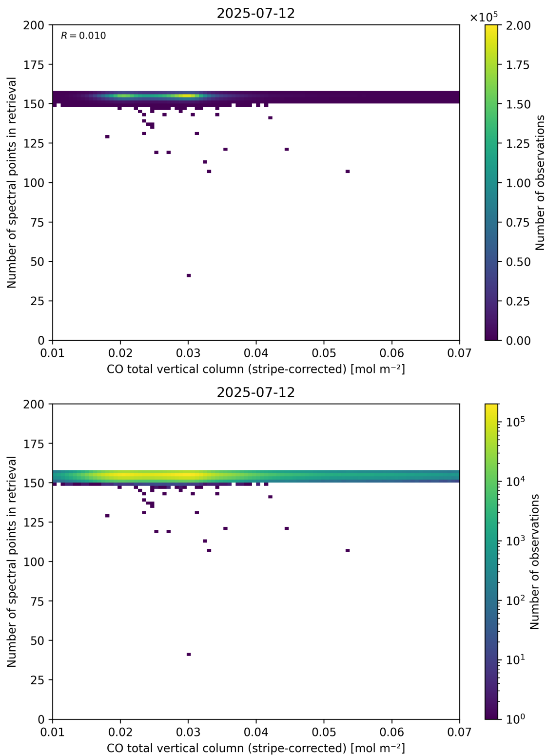
Figure 40: Scatter density plot of “CO total vertical column (stripe-corrected)” against “Number of spectral points in retrieval” for 2025-07-11 to 2025-07-13.
