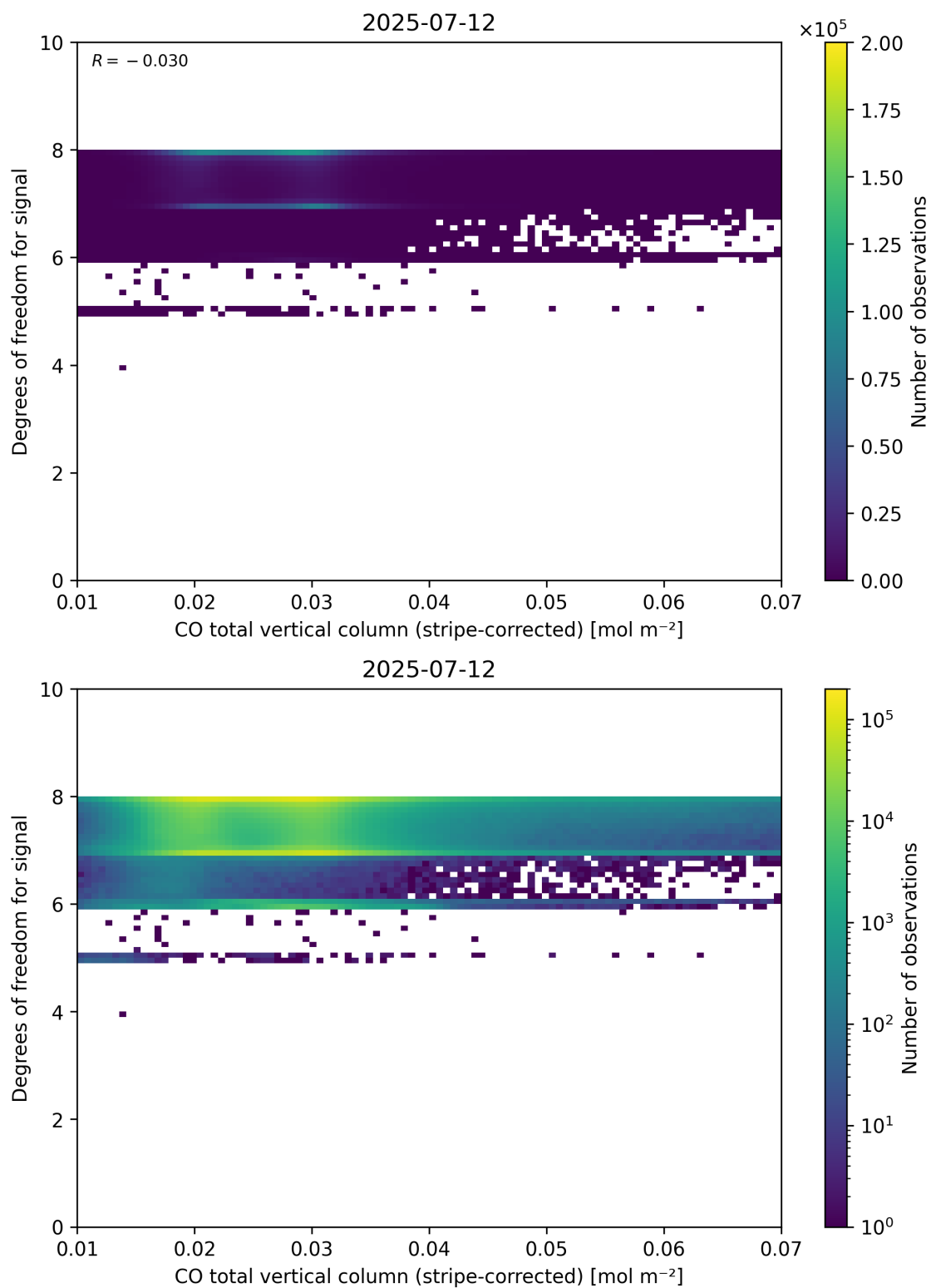
Figure 38: Scatter density plot of “CO total vertical column (stripe-corrected)” against “Degrees of freedom for signal” for 2025-07-11 to 2025-07-13.
