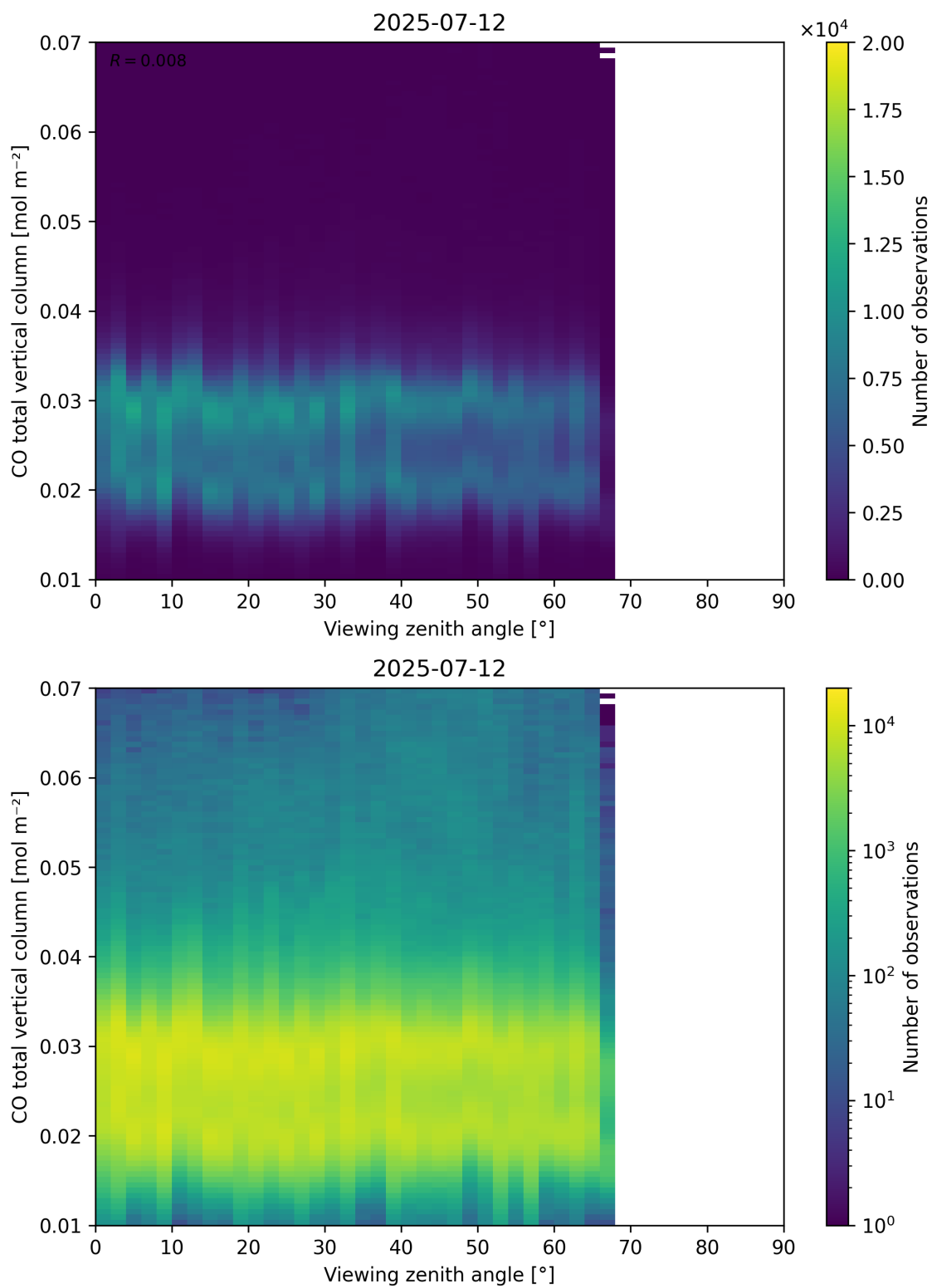
Figure 69: Scatter density plot of “Viewing zenith angle” against “CO total vertical column” for 2025-07-11 to 2025-07-13.
