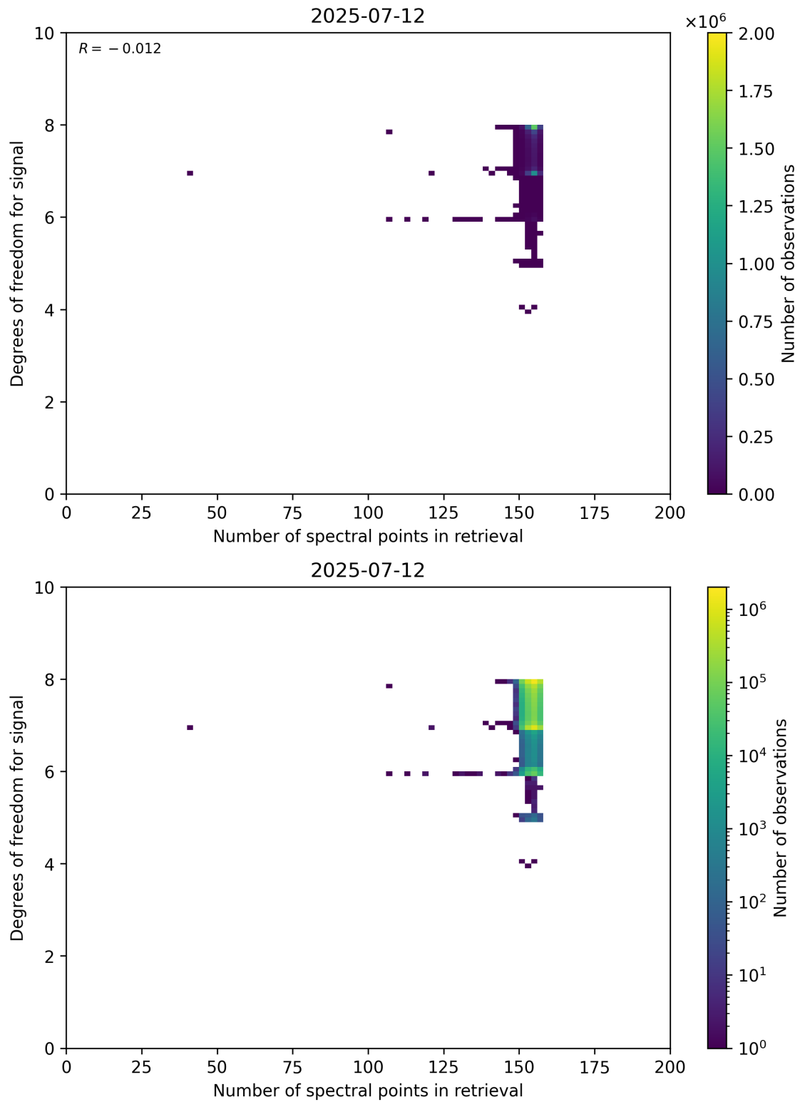
Figure 59: Scatter density plot of “Number of spectral points in retrieval” against “Degrees of freedom for signal” for 2025-07-11 to 2025-07-13.
