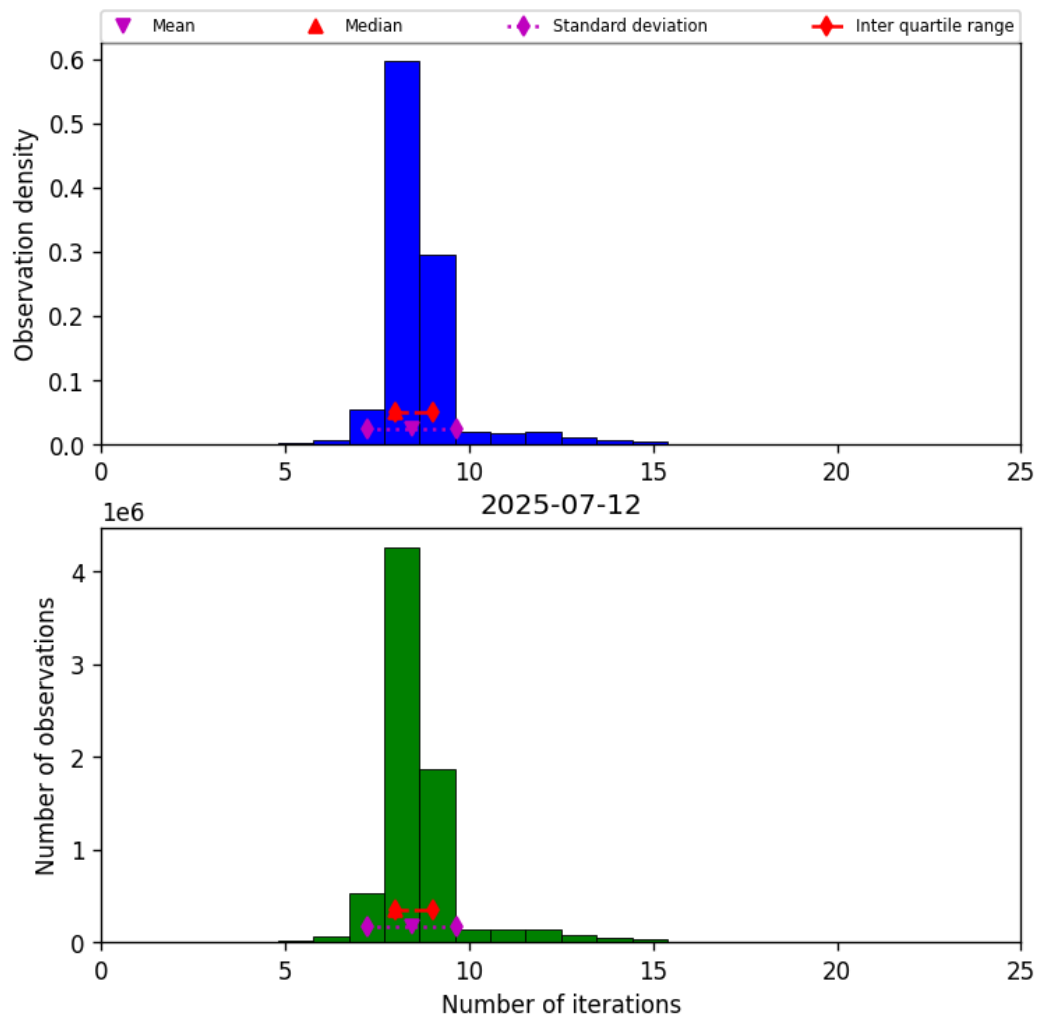
Figure 24: Histogram of “Number of iterations” for 2025-07-11 to 2025-07-13
