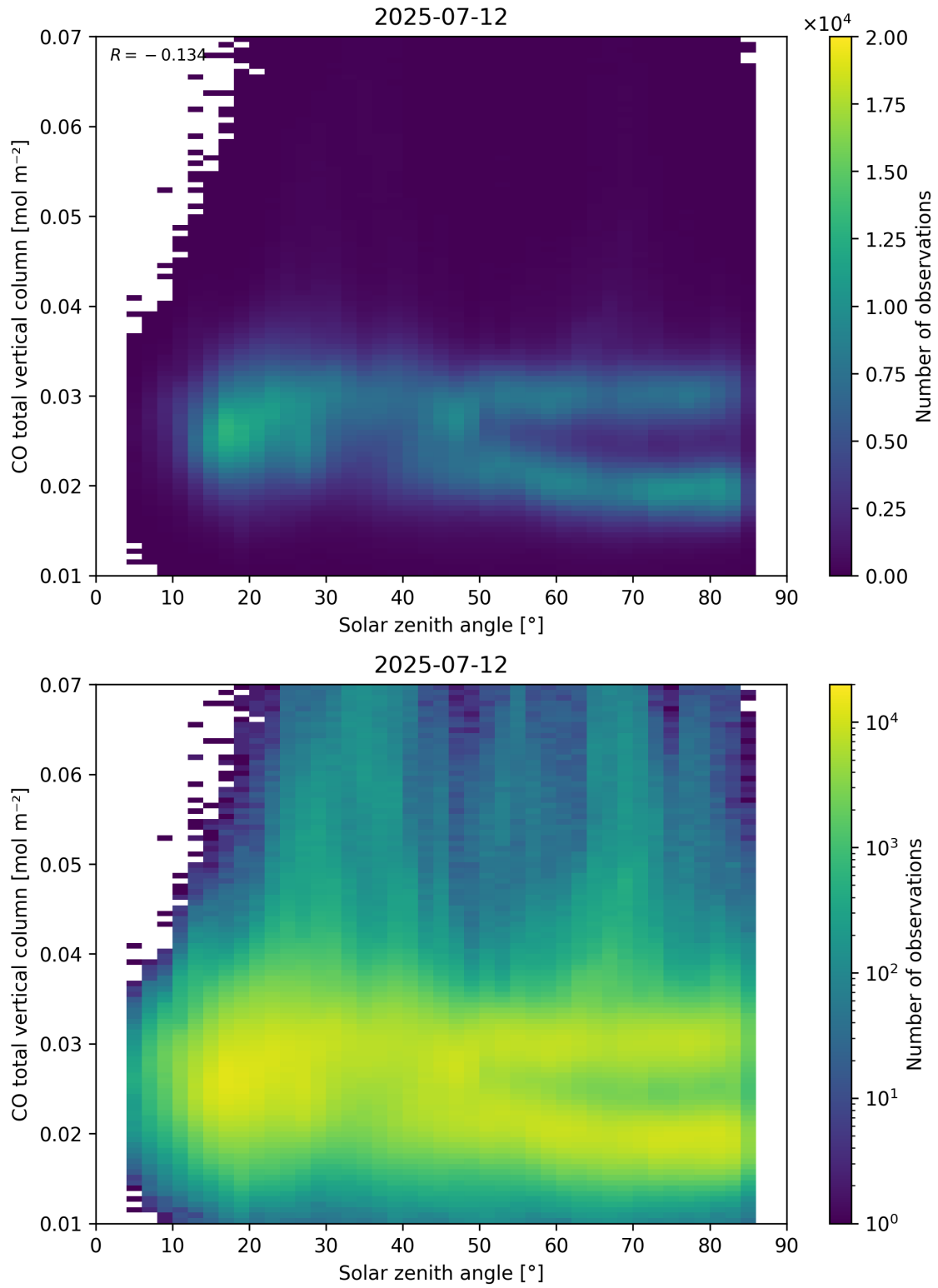
Figure 61: Scatter density plot of “Solar zenith angle” against “CO total vertical column” for 2025-07-11 to 2025-07-13.
