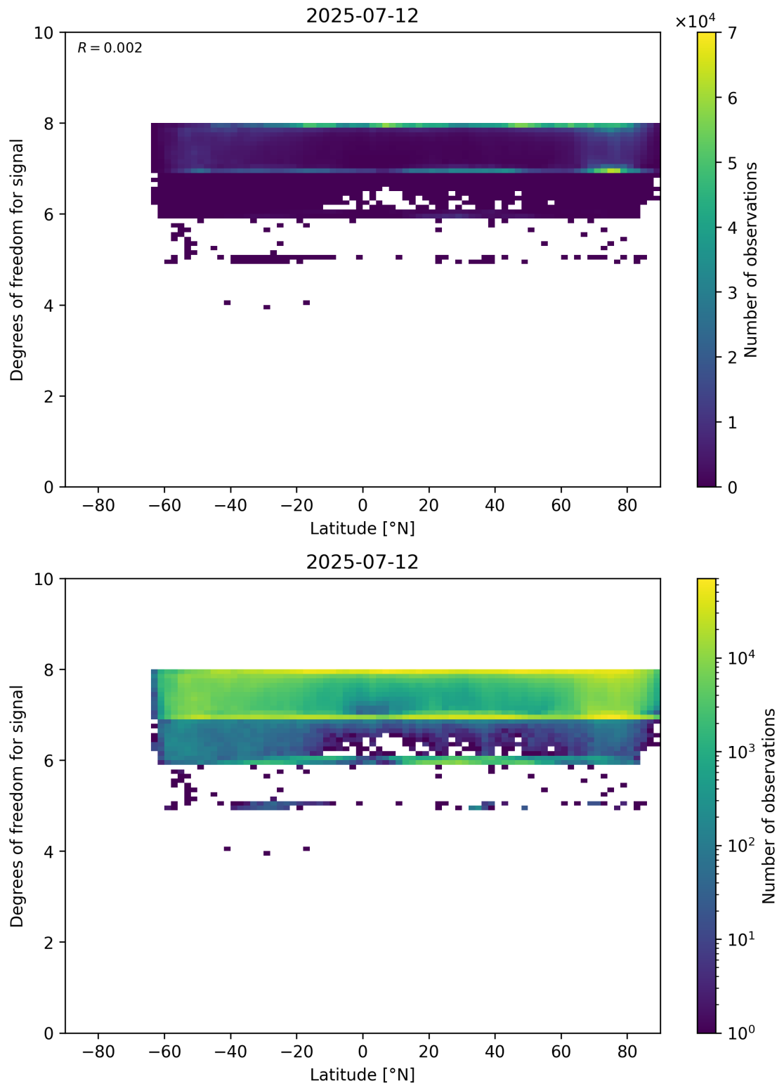
Figure 55: Scatter density plot of “Latitude” against “Degrees of freedom for signal” for 2025-07-11 to 2025-07-13.
