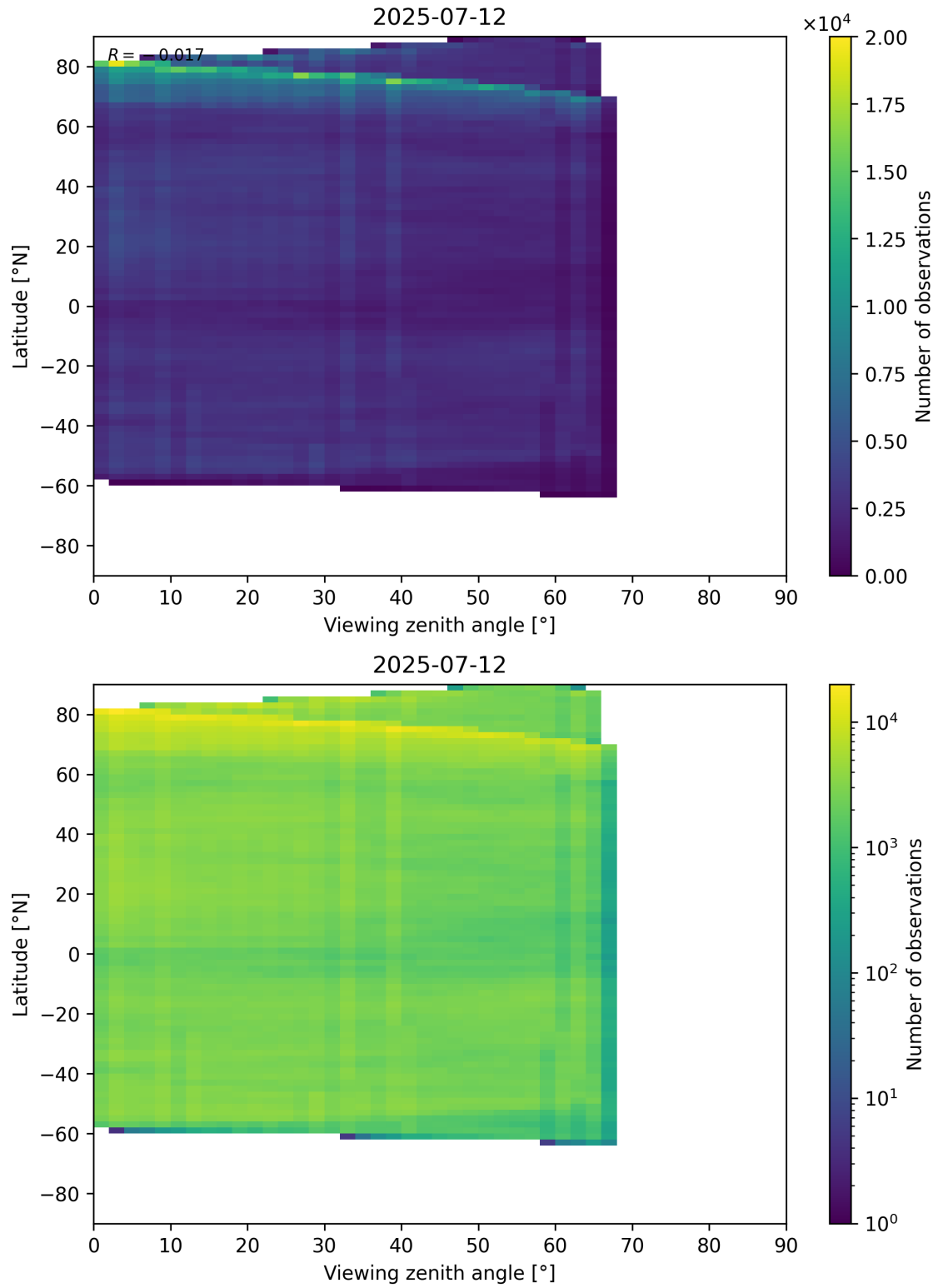
Figure 74: Scatter density plot of “Viewing zenith angle” against “Latitude” for 2025-07-11 to 2025-07-13.
