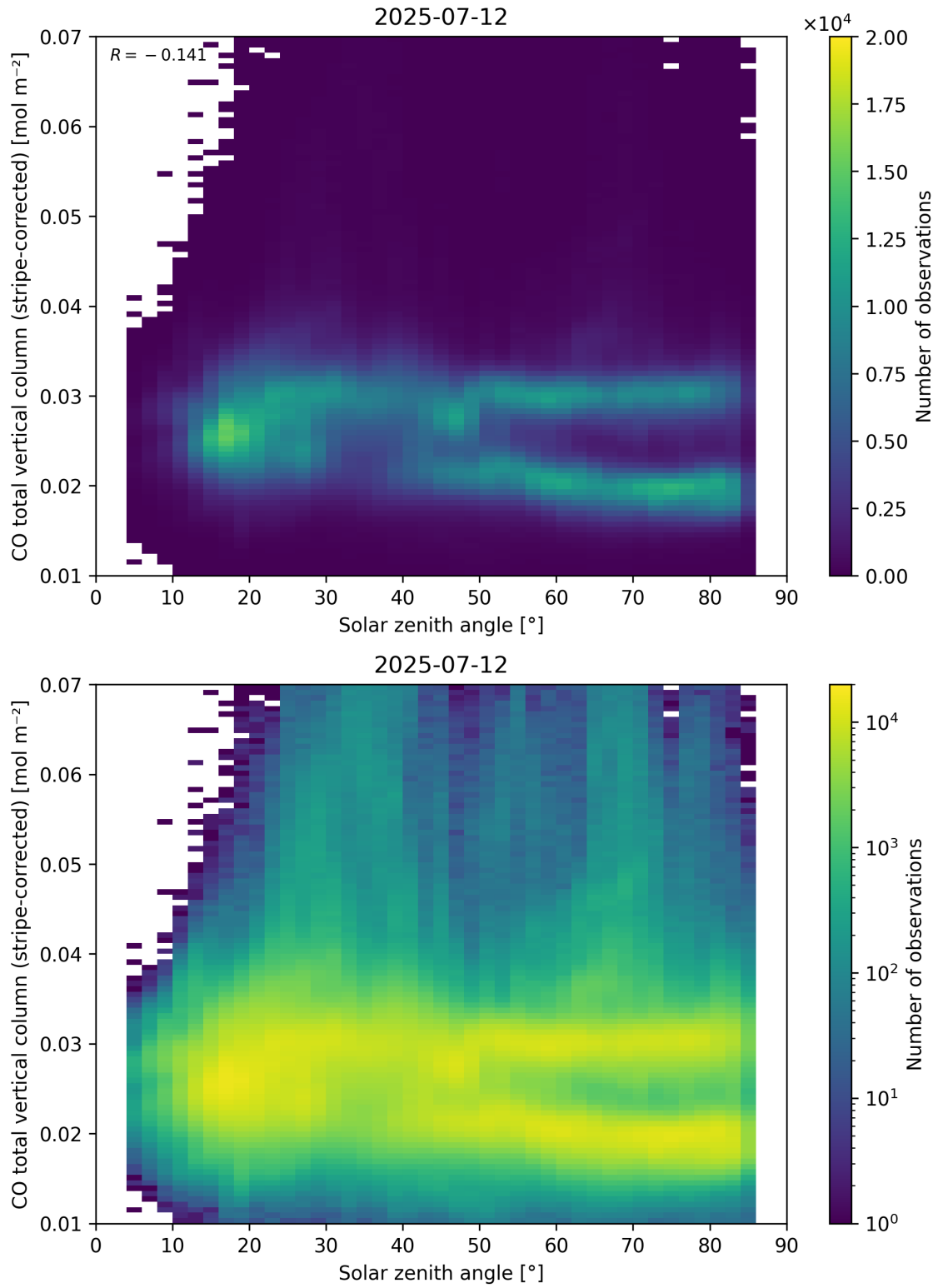
Figure 62: Scatter density plot of “Solar zenith angle” against “CO total vertical column (stripe-corrected)” for 2025-07-11 to 2025-07-13.
