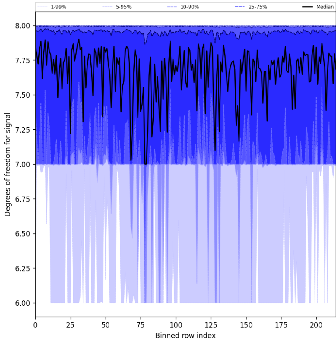
Figure 31: Along track statistics of “Degrees of freedom for signal” for 2025-07-11 to 2025-07-13
