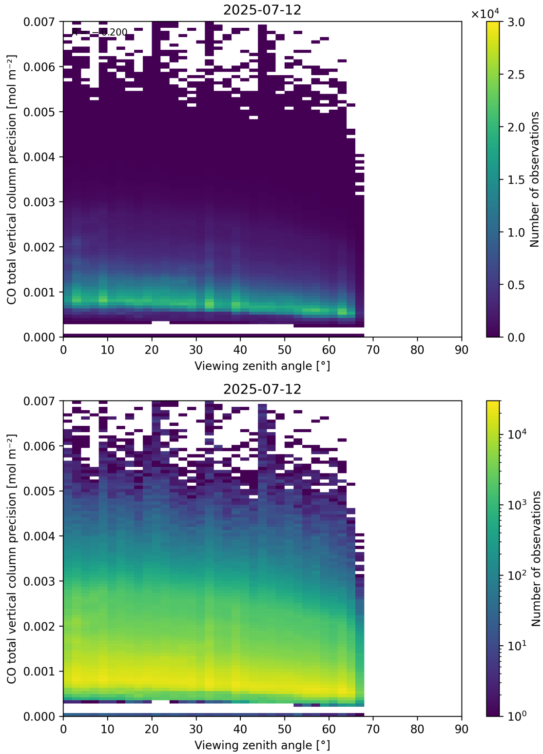
Figure 71: Scatter density plot of “Viewing zenith angle” against “CO total vertical column precision” for 2025-07-11 to 2025-07-13.
