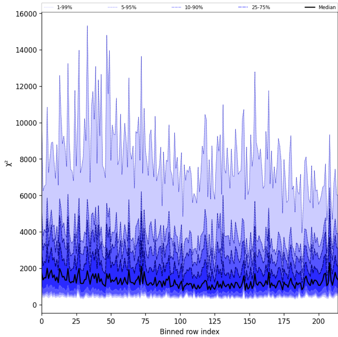
Figure 30: Along track statistics of “ \chi^2 ” for 2025-07-11 to 2025-07-13
