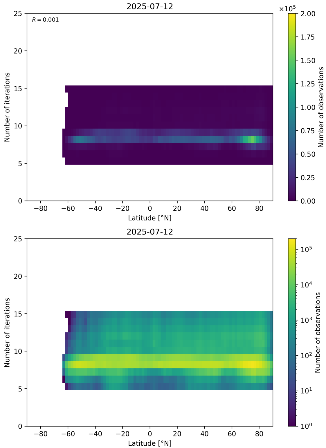
Figure 56: Scatter density plot of “Latitude” against “Number of iterations” for 2025-07-11 to 2025-07-13.
