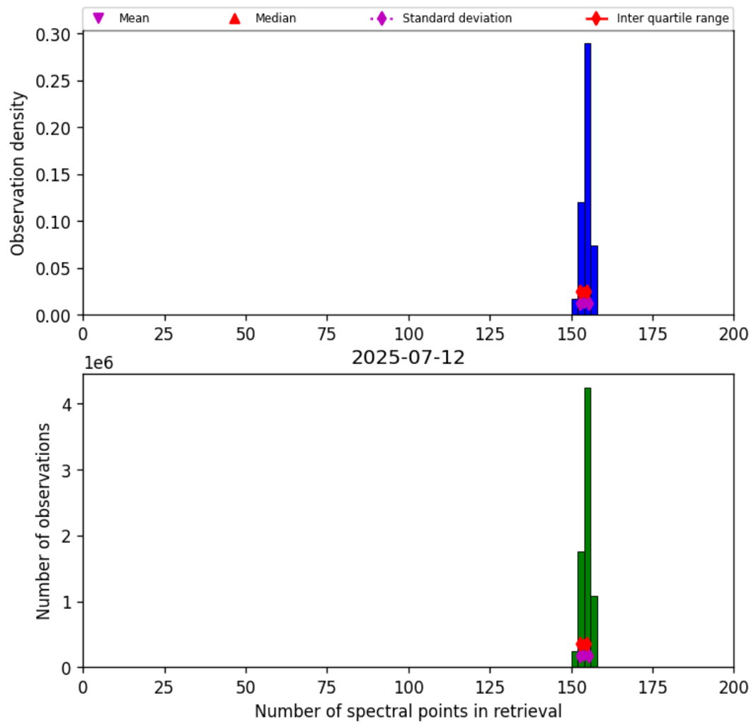
Figure 21: Histogram of “Number of spectral points in retrieval” for 2025-07-11 to 2025-07-13
