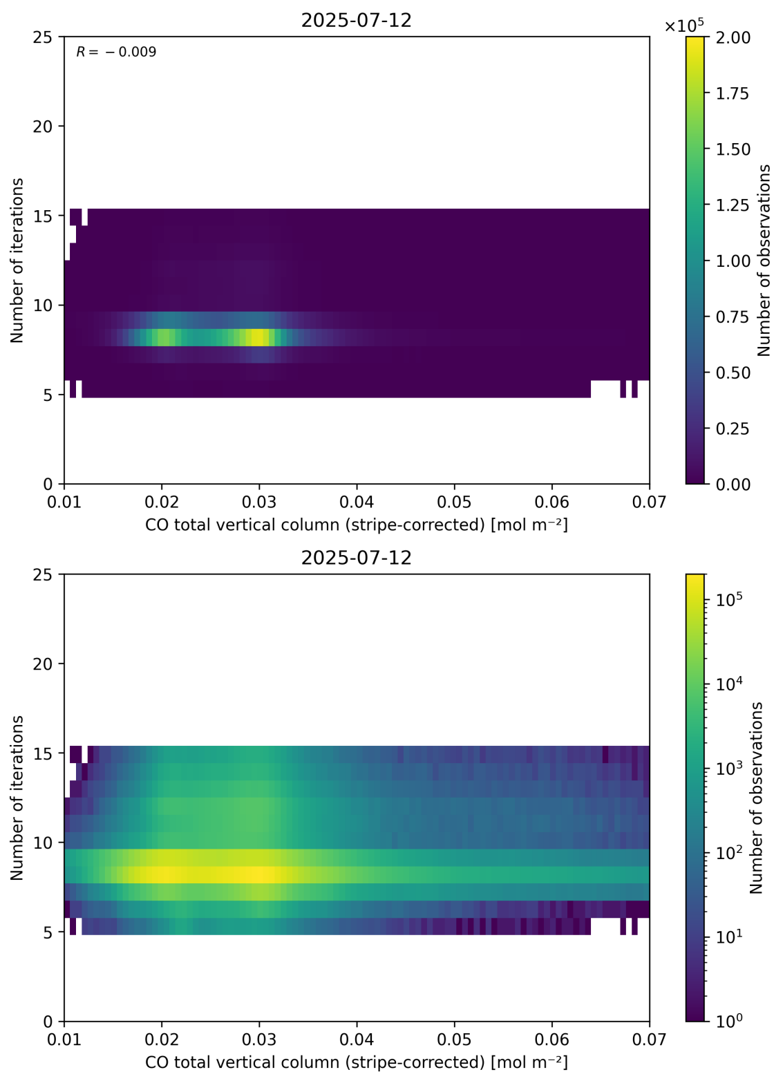
Figure 39: Scatter density plot of “CO total vertical column (stripe-corrected)” against “Number of iterations” for 2025-07-11 to 2025-07-13.
