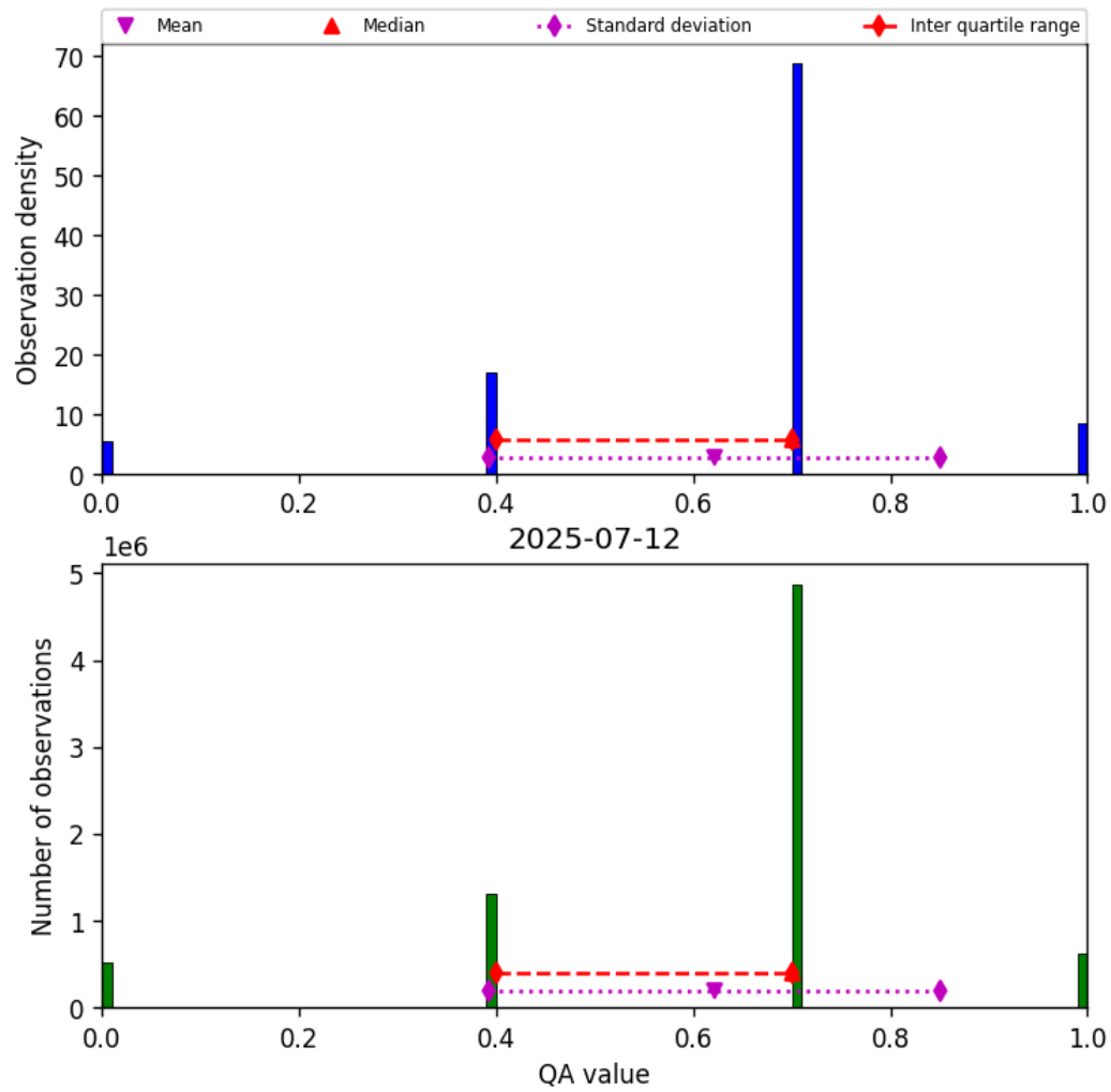
Figure 17: Histogram of “QA value” for 2025-07-11 to 2025-07-13
