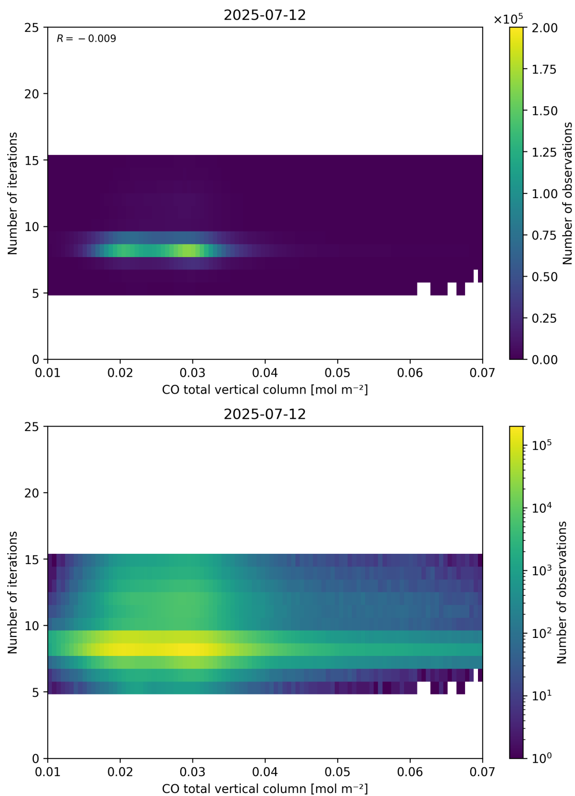
Figure 42: Scatter density plot of “CO total vertical column” against “Number of iterations” for 2025-07-11 to 2025-07-13.
