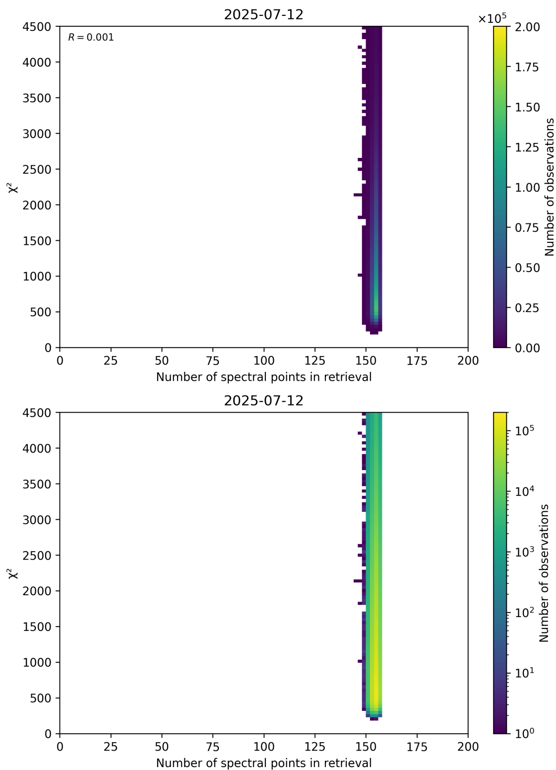
Figure 58: Scatter density plot of “Number of spectral points in retrieval” against “ \chi^2 ” for 2025-07-11 to 2025-07-13.
