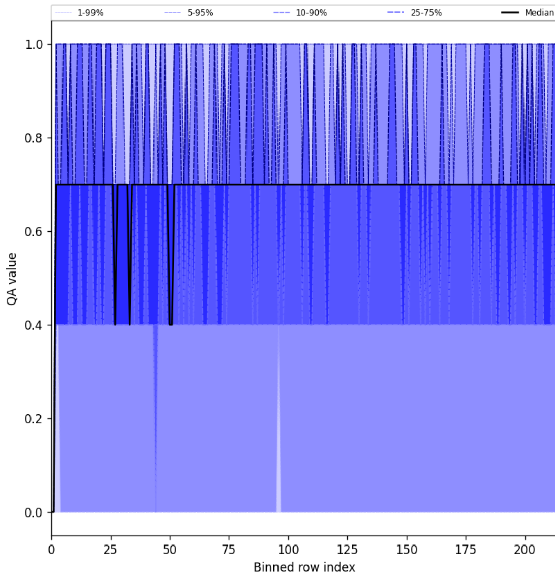
Figure 25: Along track statistics of “QA value” for 2025-07-11 to 2025-07-13
