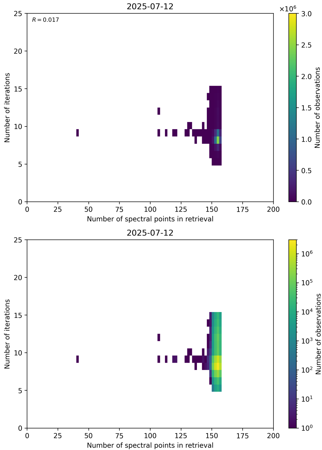
Figure 60: Scatter density plot of “Number of spectral points in retrieval” against “Number of iterations” for 2025-07-11 to 2025-07-13.
