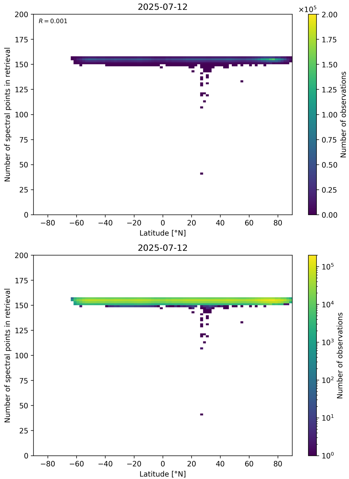
Figure 57: Scatter density plot of “Latitude” against “Number of spectral points in retrieval” for 2025-07-11 to 2025-07-13.
