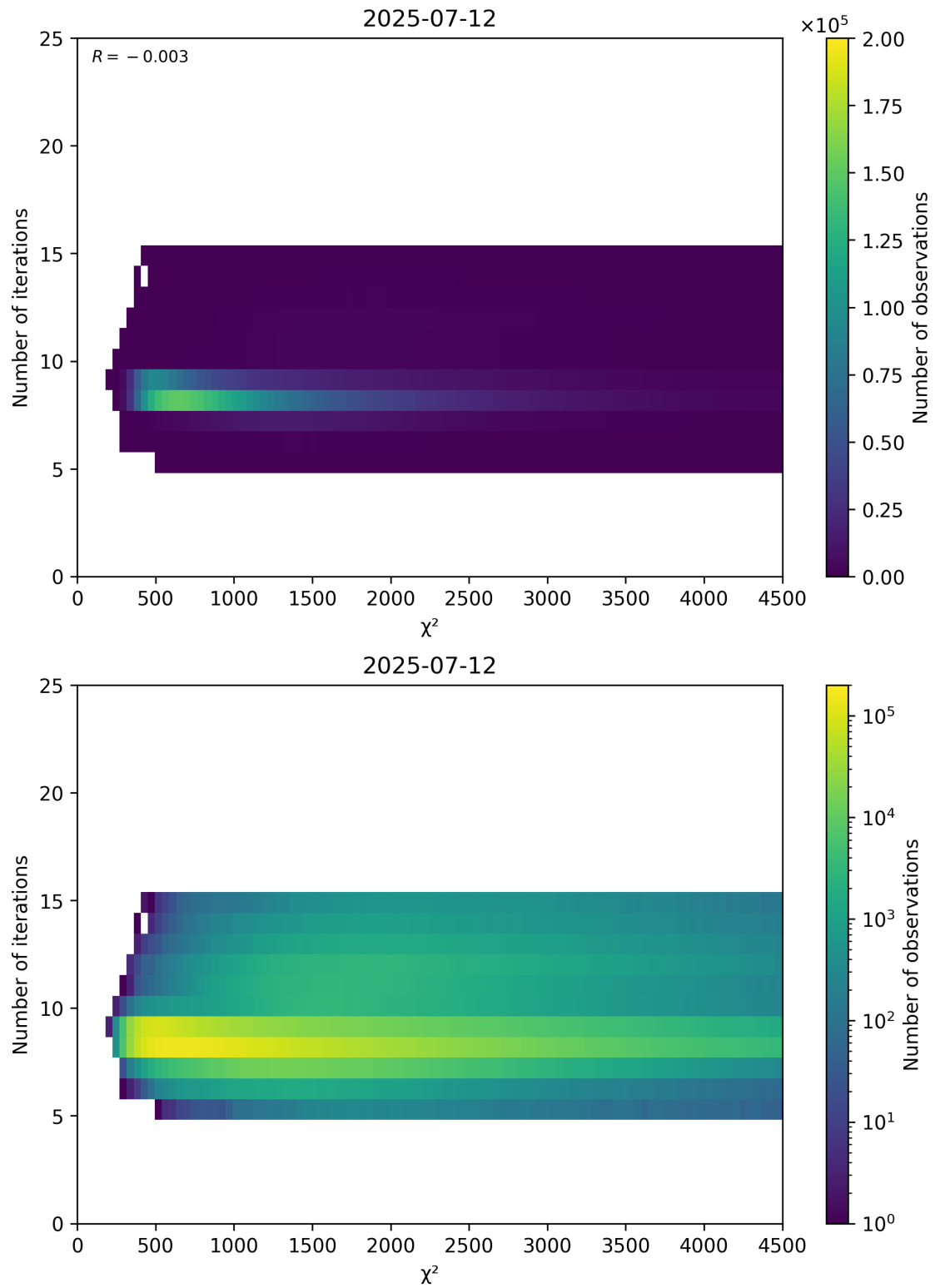
Figure 49: Scatter density plot of “ \chi^2 ” against “Number of iterations” for 2025-07-11 to 2025-07-13.
