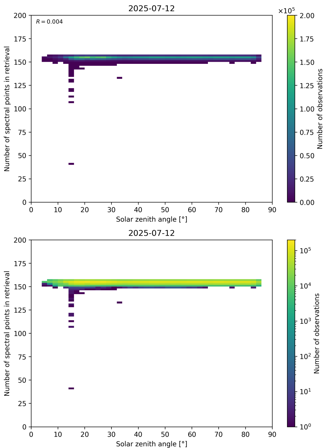
Figure 68: Scatter density plot of “Solar zenith angle” against “Number of spectral points in retrieval” for 2025-07-11 to 2025-07-13.
