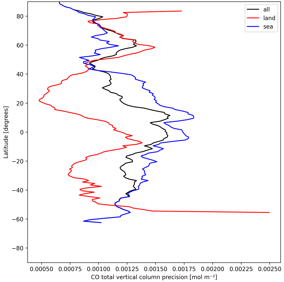
Figure 12: Zonal average of “CO total vertical column precision” for 2025-07-11 to 2025-07-13.
