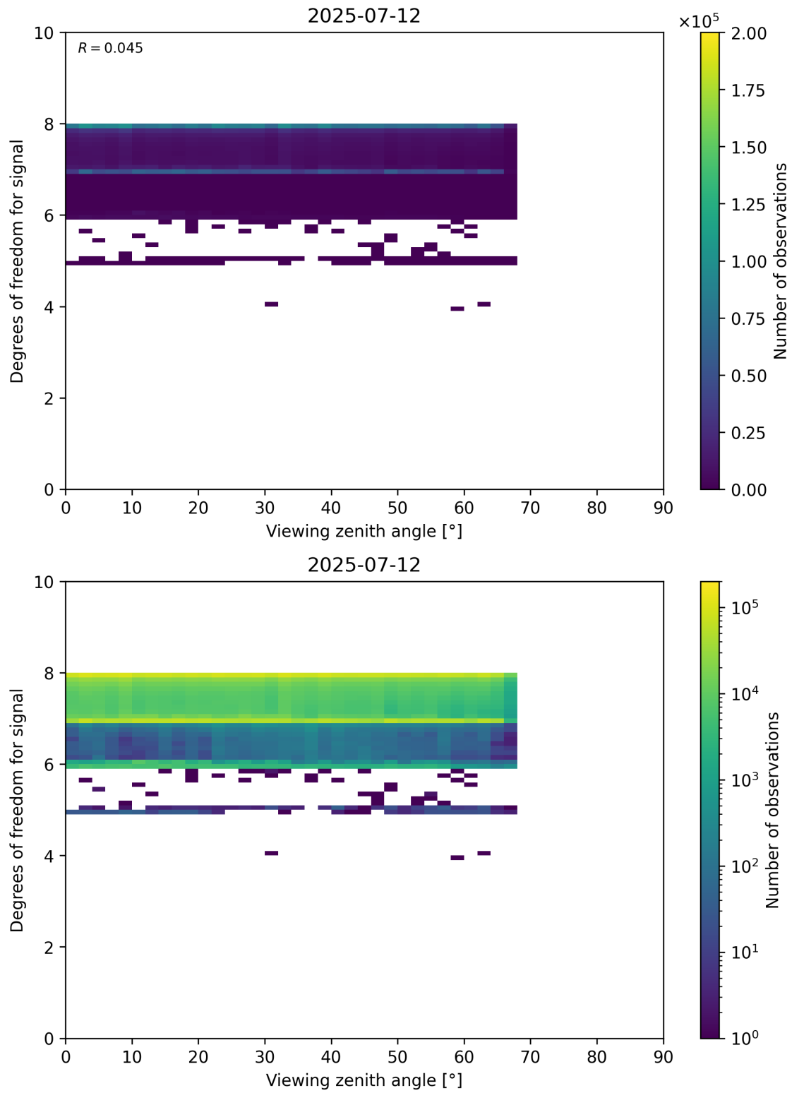
Figure 73: Scatter density plot of “Viewing zenith angle” against “Degrees of freedom for signal” for 2025-07-11 to 2025-07-13.
