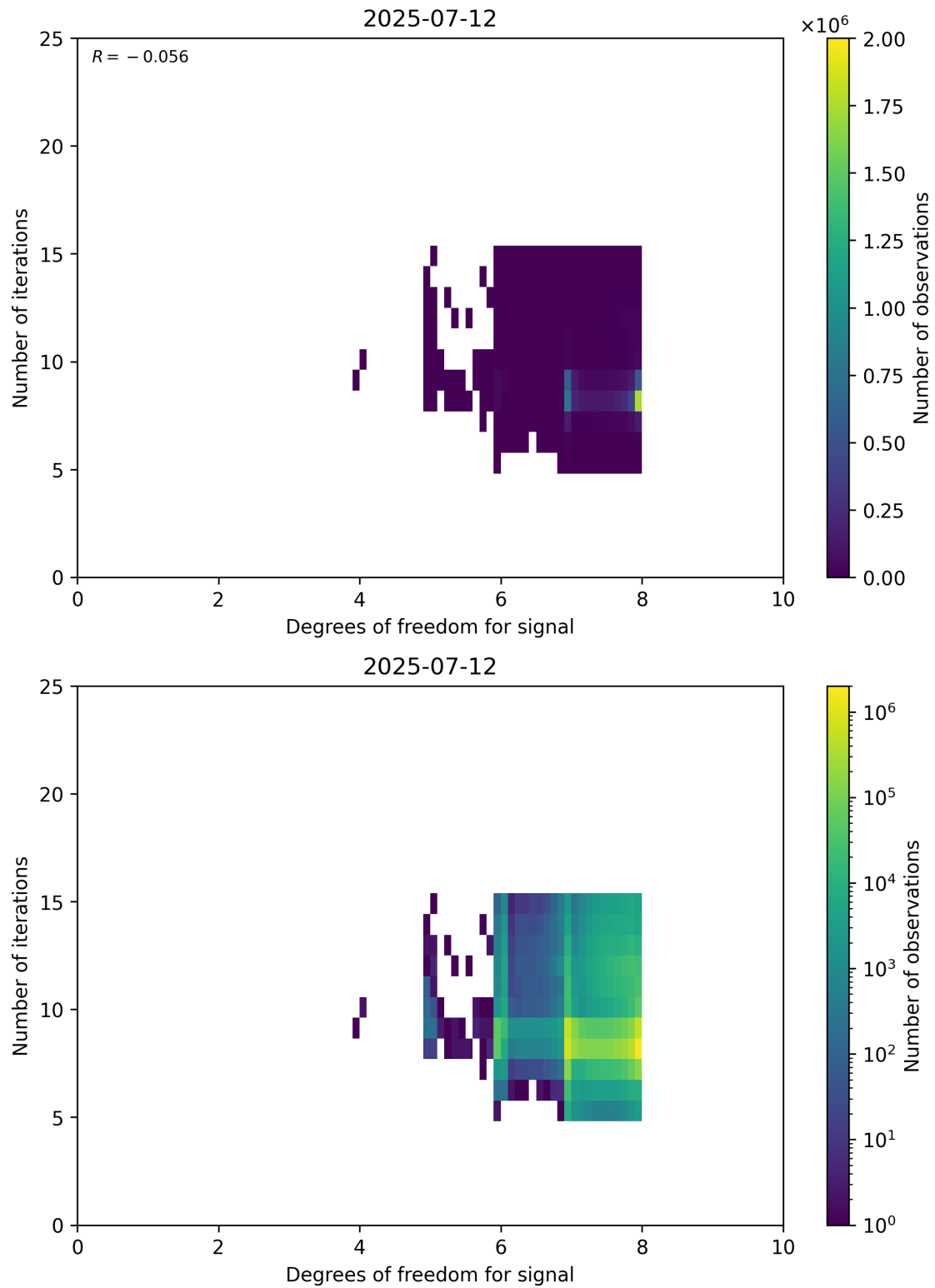
Figure 50: Scatter density plot of “Degrees of freedom for signal” against “Number of iterations” for 2025-07-11 to 2025-07-13.
