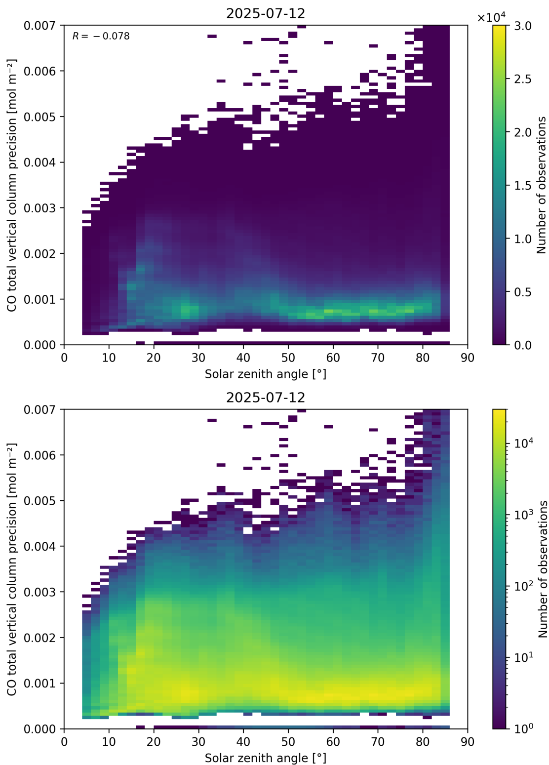
Figure 63: Scatter density plot of “Solar zenith angle” against “CO total vertical column precision” for 2025-07-11 to 2025-07-13.
