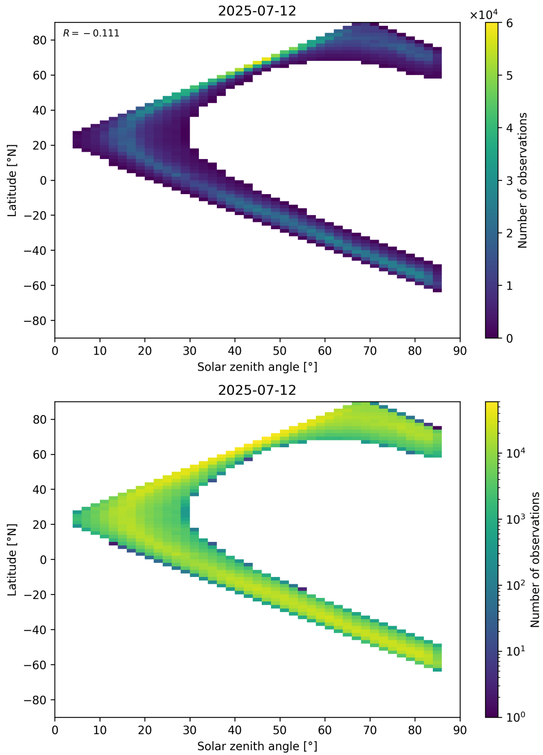
Figure 66: Scatter density plot of “Solar zenith angle” against “Latitude” for 2025-07-11 to 2025-07-13.
