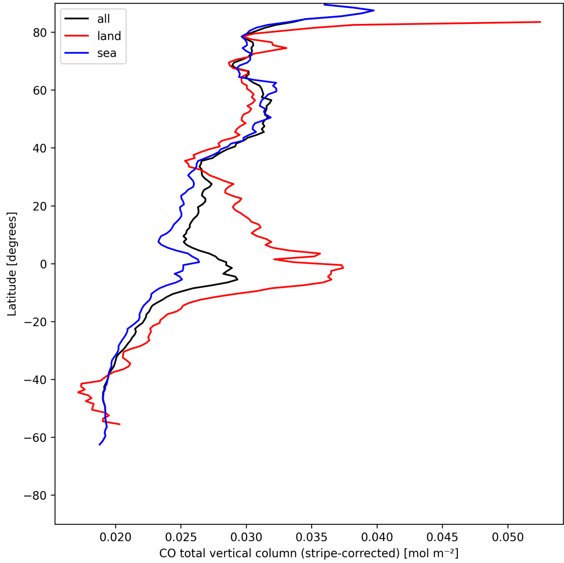
Figure 11: Zonal average of “CO total vertical column (stripe-corrected)” for 2025-07-11 to 2025-07-13.
