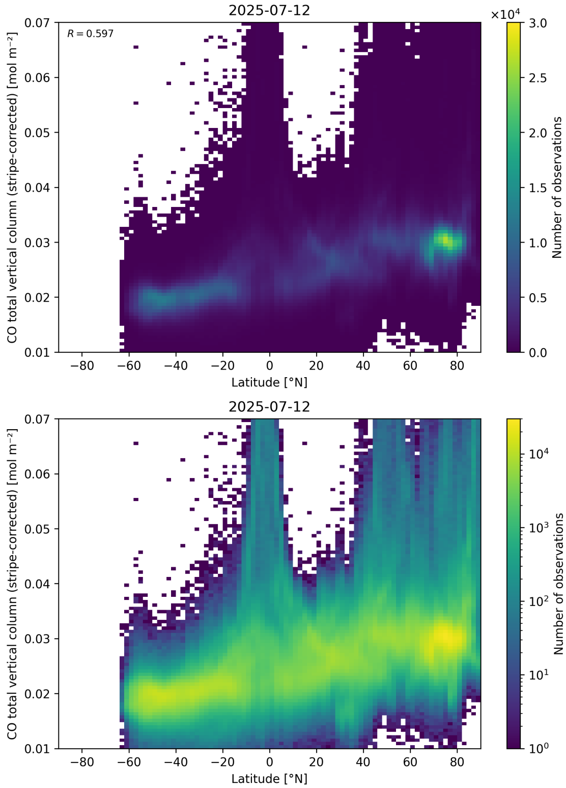
Figure 52: Scatter density plot of “Latitude” against “CO total vertical column (stripe-corrected)” for 2025-07-11 to 2025-07-13.
