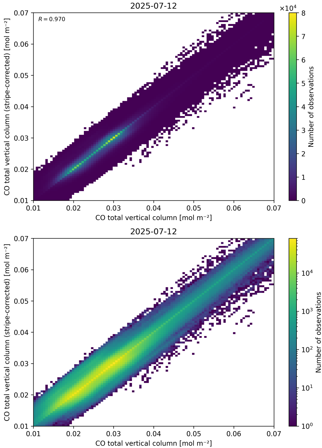
Figure 33: Scatter density plot of “CO total vertical column” against “CO total vertical column (stripe-corrected)” for 2025-07-11 to 2025-07-13.
