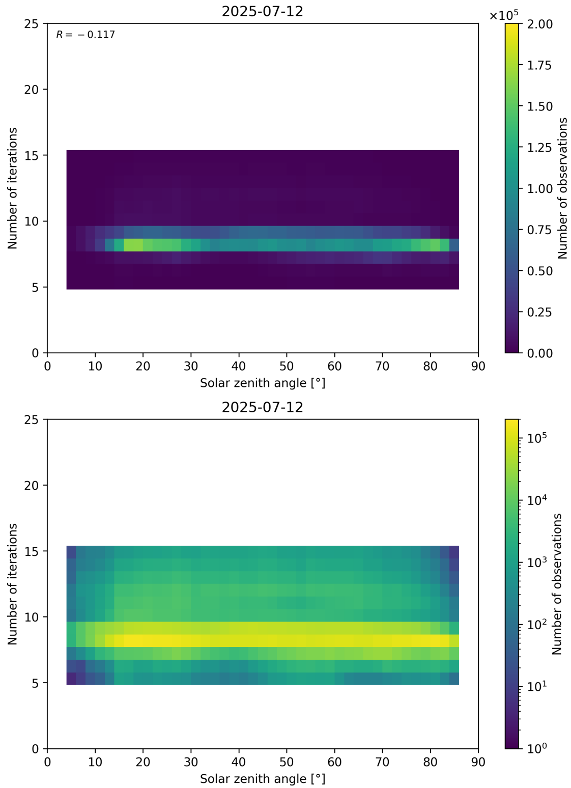
Figure 67: Scatter density plot of “Solar zenith angle” against “Number of iterations” for 2025-07-11 to 2025-07-13.
