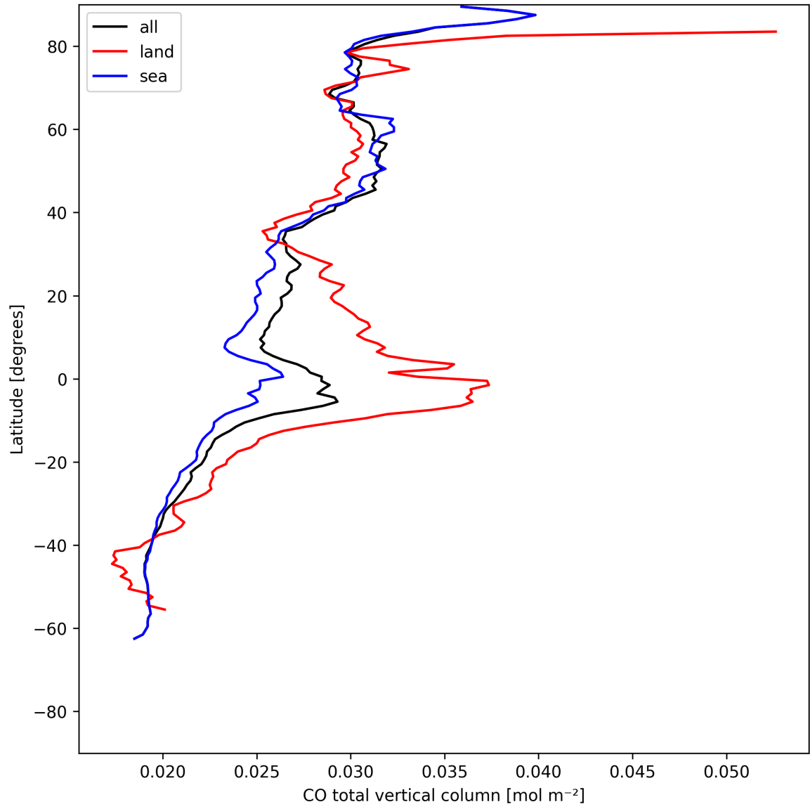
Figure 10: Zonal average of “CO total vertical column” for 2025-07-11 to 2025-07-13.
