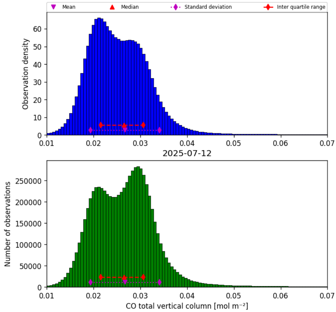
Figure 18: Histogram of “CO total vertical column” for 2025-07-11 to 2025-07-13
