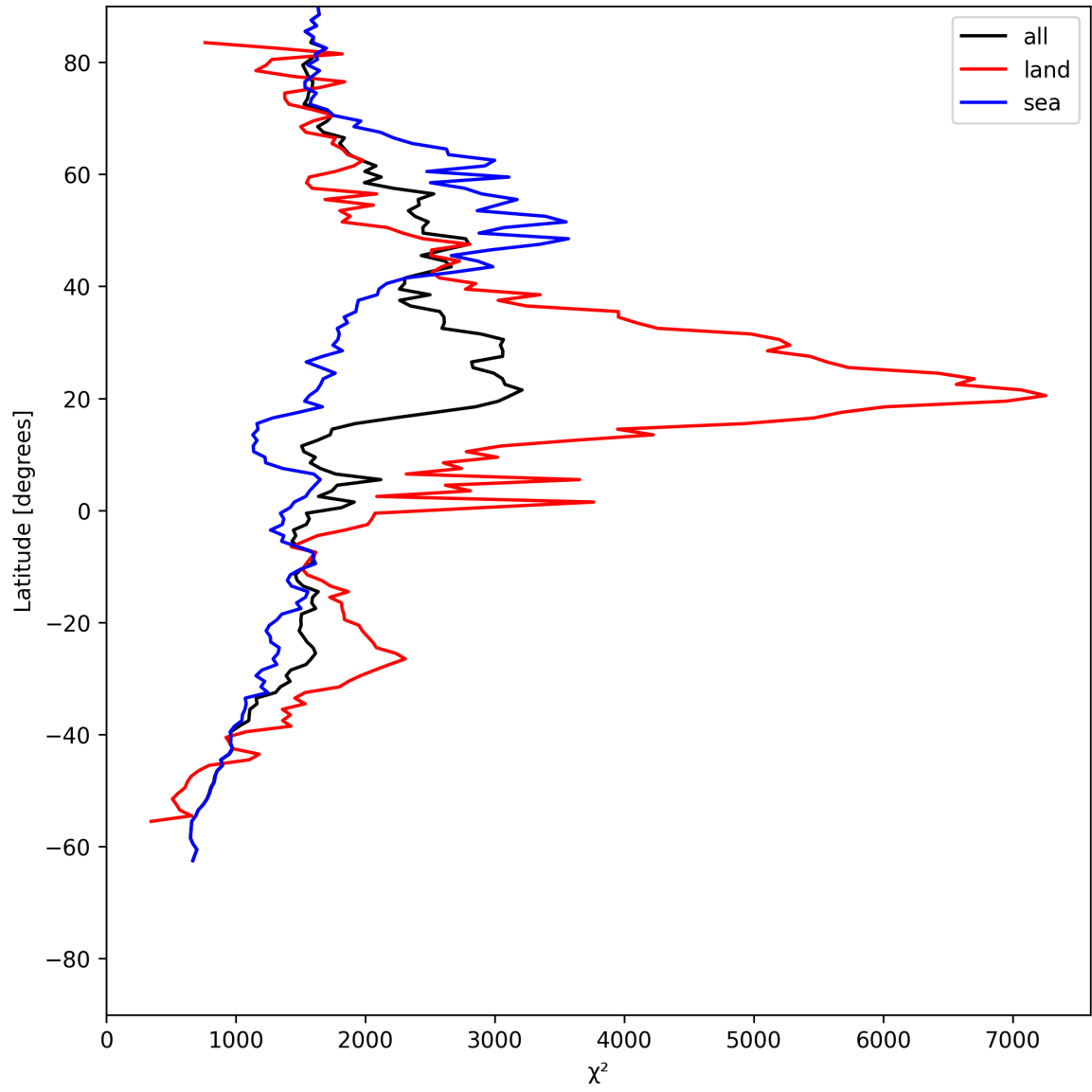
Figure 14: Zonal average of “ \chi^2 ” for 2025-07-11 to 2025-07-13.
