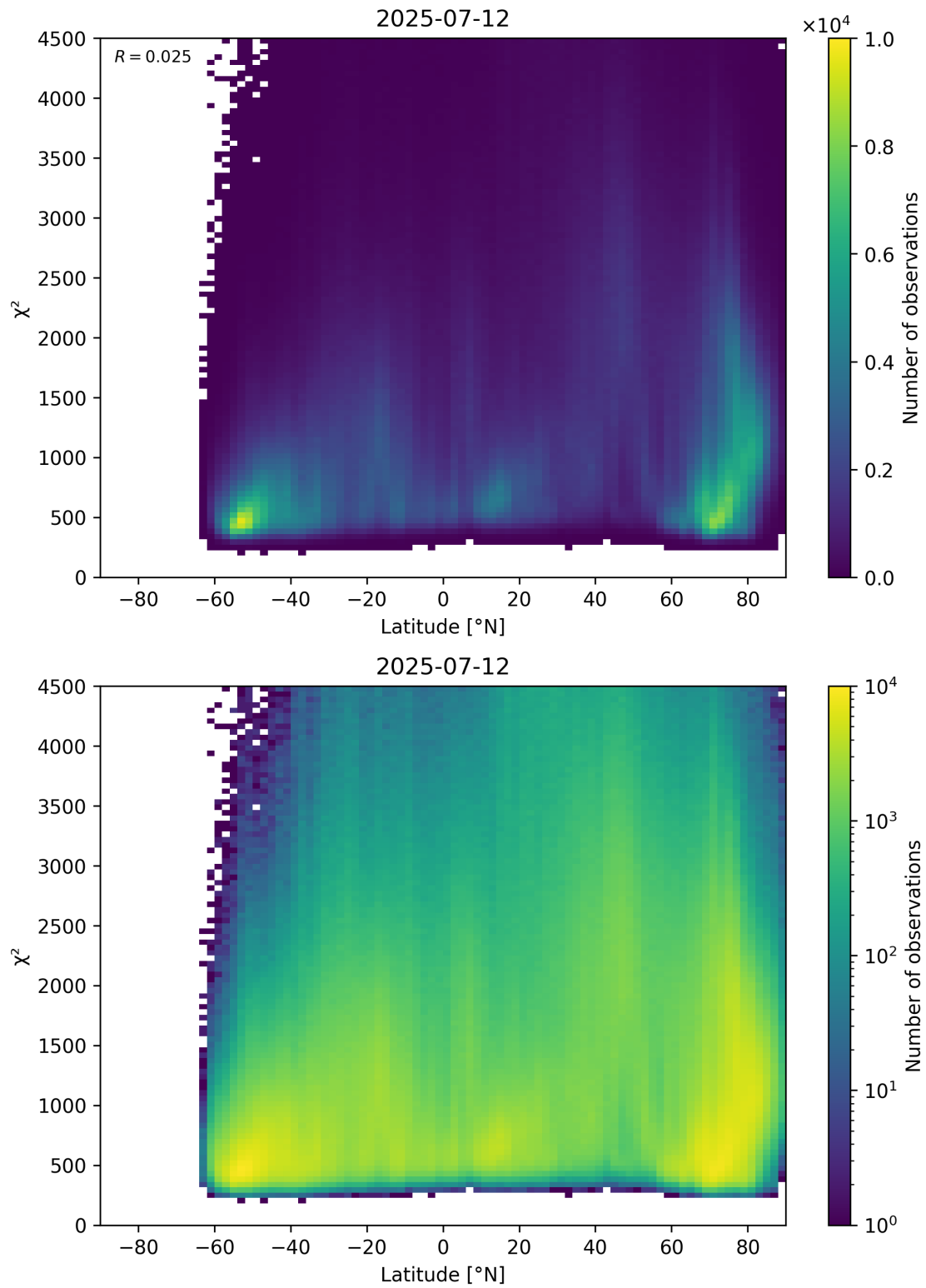
Figure 54: Scatter density plot of “Latitude” against “ \chi^2 ” for 2025-07-11 to 2025-07-13.
