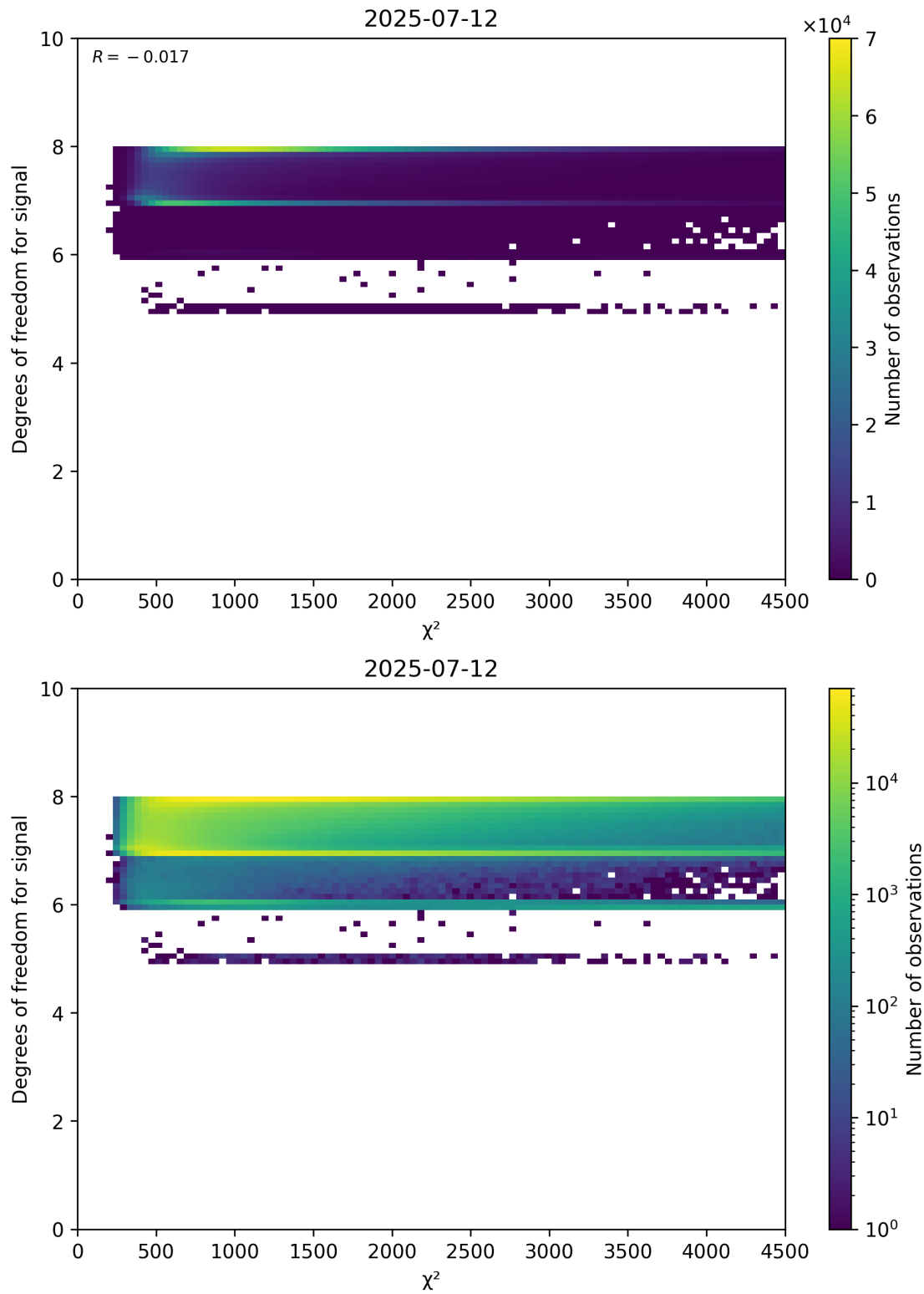
Figure 48: Scatter density plot of “ \chi^2 ” against “Degrees of freedom for signal” for 2025-07-11 to 2025-07-13.
