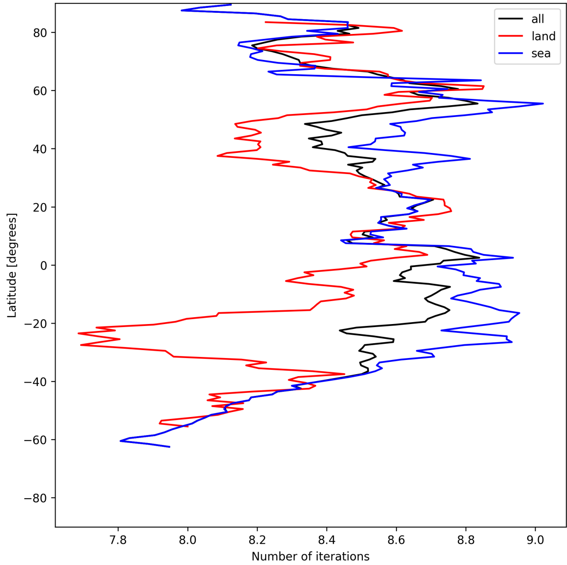
Figure 16: Zonal average of “Number of iterations” for 2025-07-11 to 2025-07-13.
