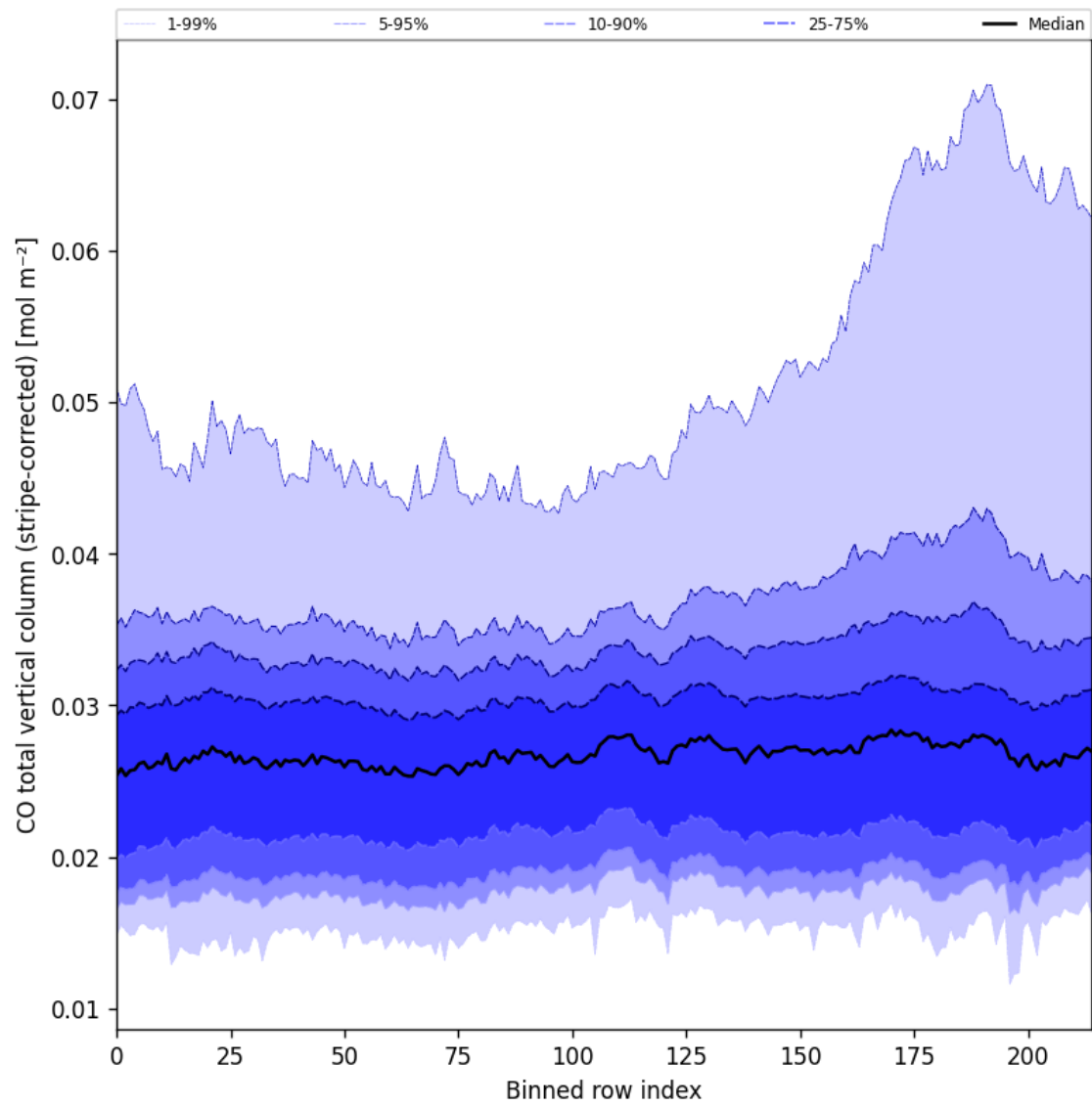
Figure 27: Along track statistics of “CO total vertical column (stripe-corrected)” for 2025-07-11 to 2025-07-13
