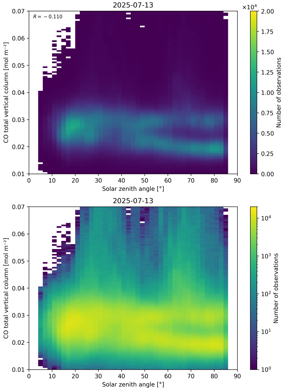
Figure 61: Scatter density plot of “Solar zenith angle” against “CO total vertical column” for 2025-07-13 to 2025-07-14.
