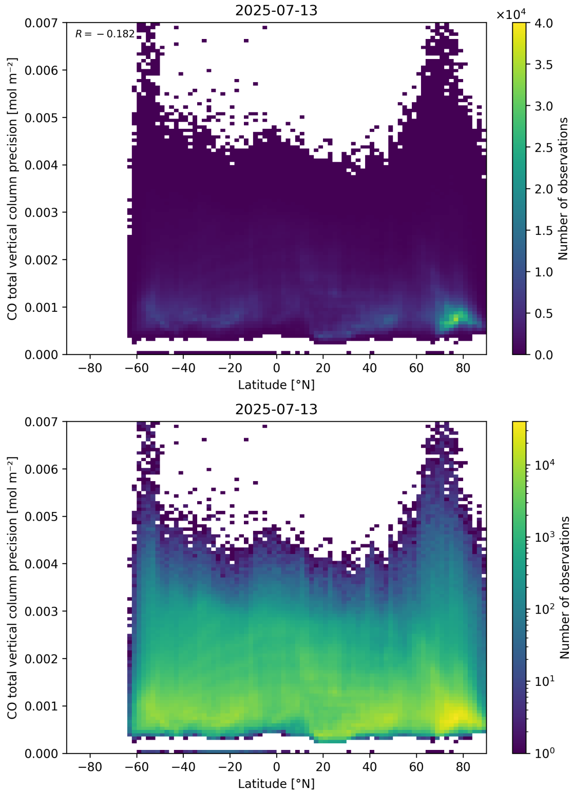
Figure 53: Scatter density plot of “Latitude” against “CO total vertical column precision” for 2025-07-13 to 2025-07-14.
