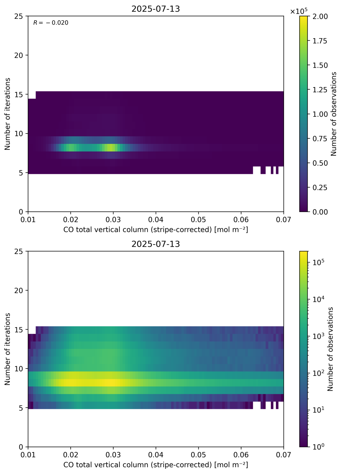
Figure 39: Scatter density plot of “CO total vertical column (stripe-corrected)” against “Number of iterations” for 2025-07-13 to 2025-07-14.
