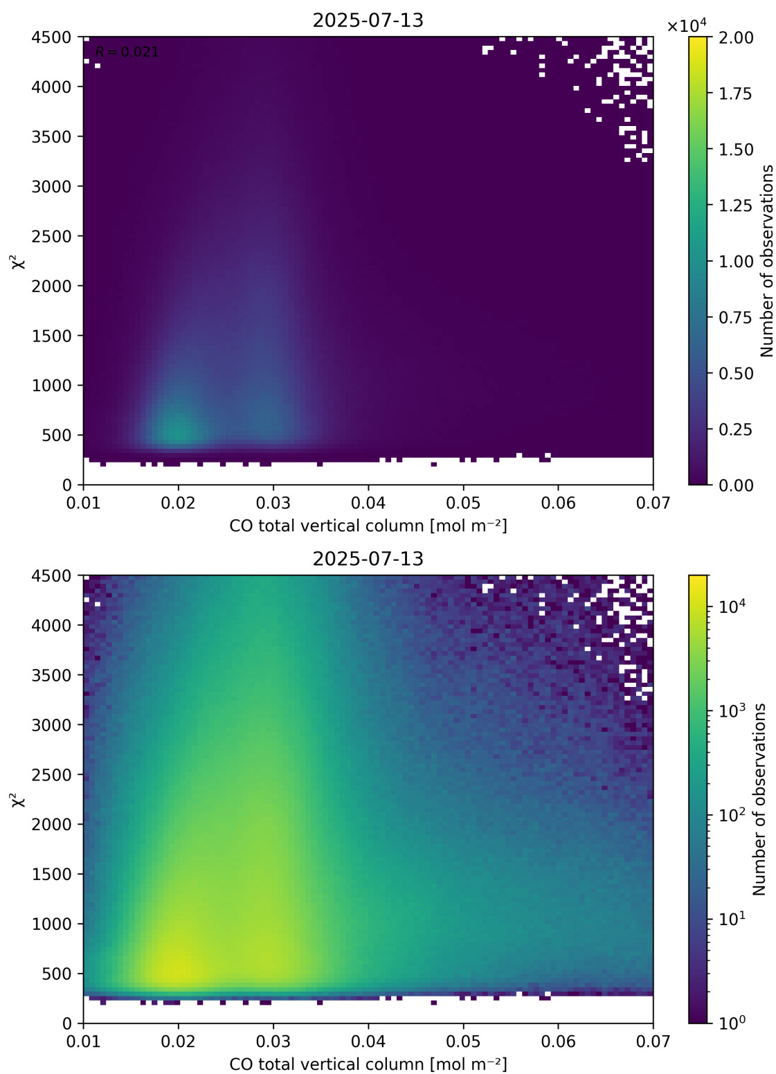
Figure 35: Scatter density plot of “CO total vertical column” against “ \chi^2 ” for 2025-07-13 to 2025-07-14.
