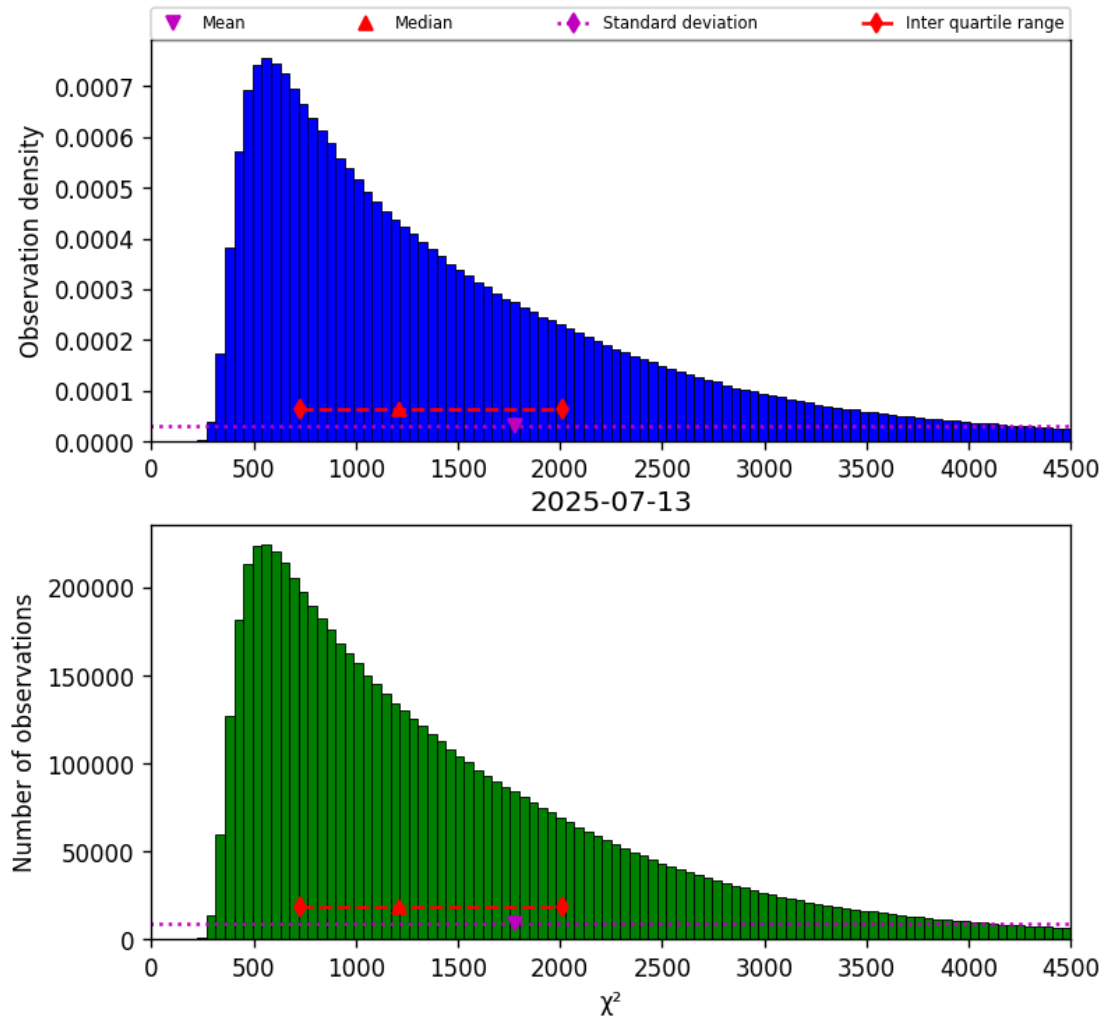
Figure 22: Histogram of “ \chi^2 ” for 2025-07-13 to 2025-07-14
