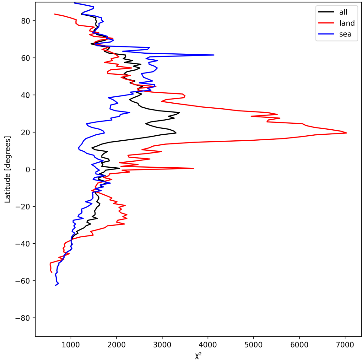
Figure 14: Zonal average of “ \chi^2 ” for 2025-07-13 to 2025-07-14.
