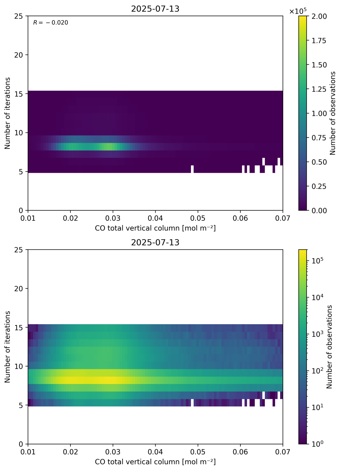
Figure 42: Scatter density plot of “CO total vertical column” against “Number of iterations” for 2025-07-13 to 2025-07-14.
