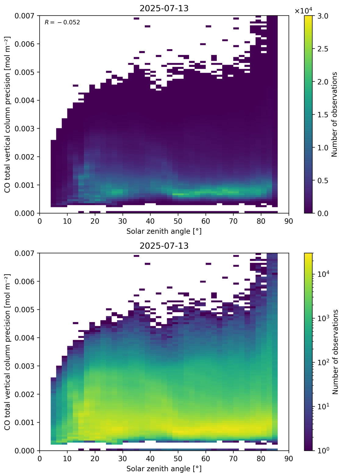
Figure 63: Scatter density plot of “Solar zenith angle” against “CO total vertical column precision” for 2025-07-13 to 2025-07-14.
