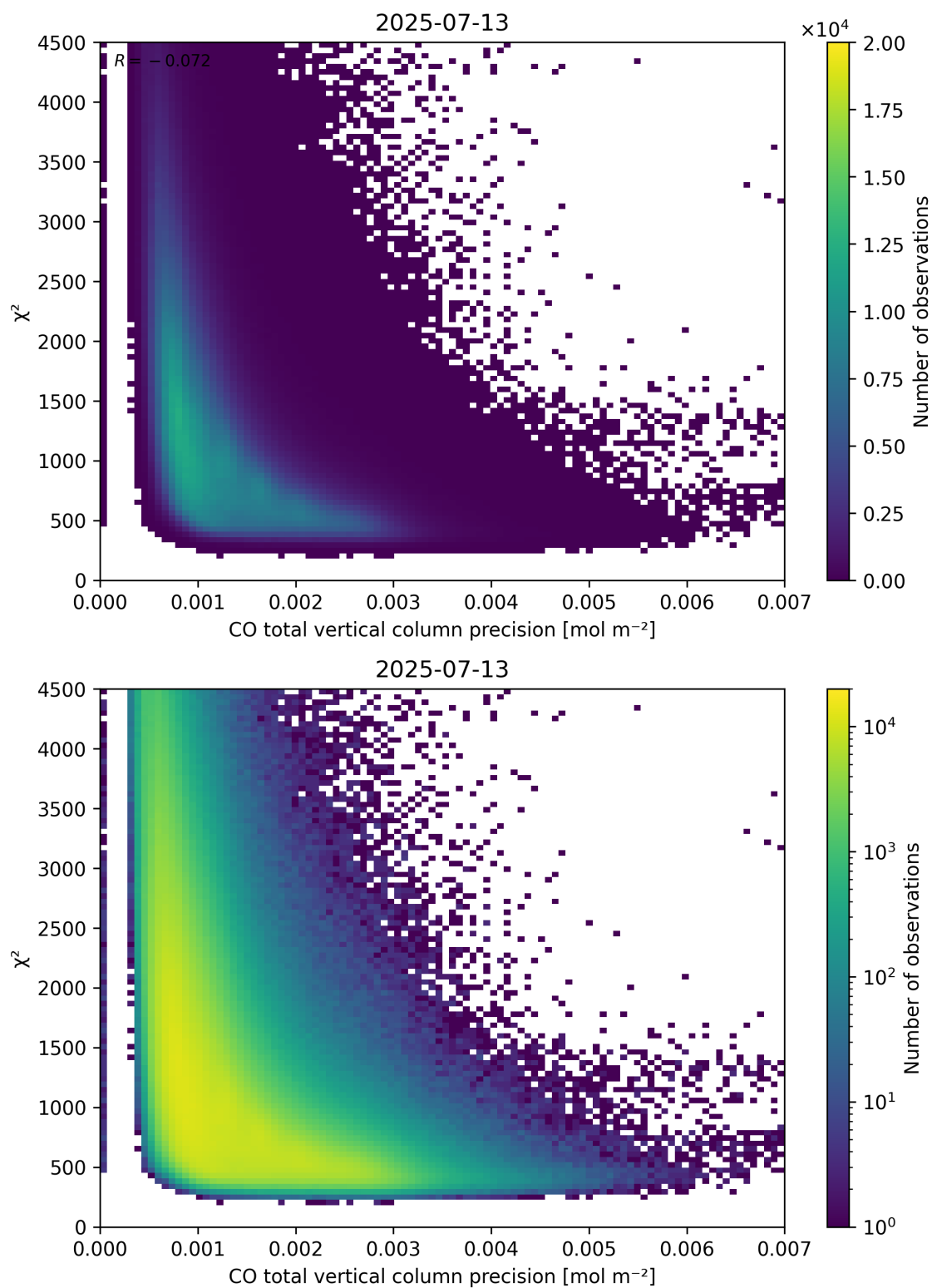
Figure 44: Scatter density plot of “CO total vertical column precision” against “ \chi^2 ” for 2025-07-13 to 2025-07-14.
