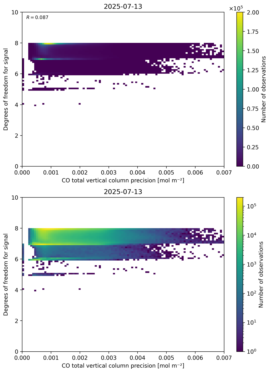
Figure 45: Scatter density plot of “CO total vertical column precision” against “Degrees of freedom for signal” for 2025-07-13 to 2025-07-14.
