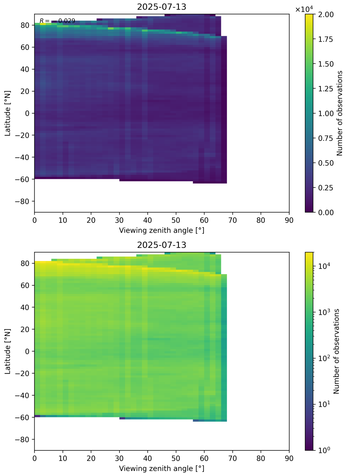
Figure 74: Scatter density plot of “Viewing zenith angle” against “Latitude” for 2025-07-13 to 2025-07-14.
