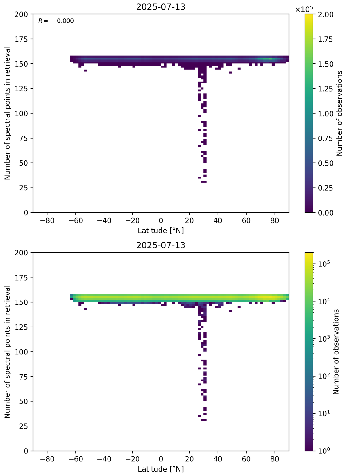
Figure 57: Scatter density plot of “Latitude” against “Number of spectral points in retrieval” for 2025-07-13 to 2025-07-14.
