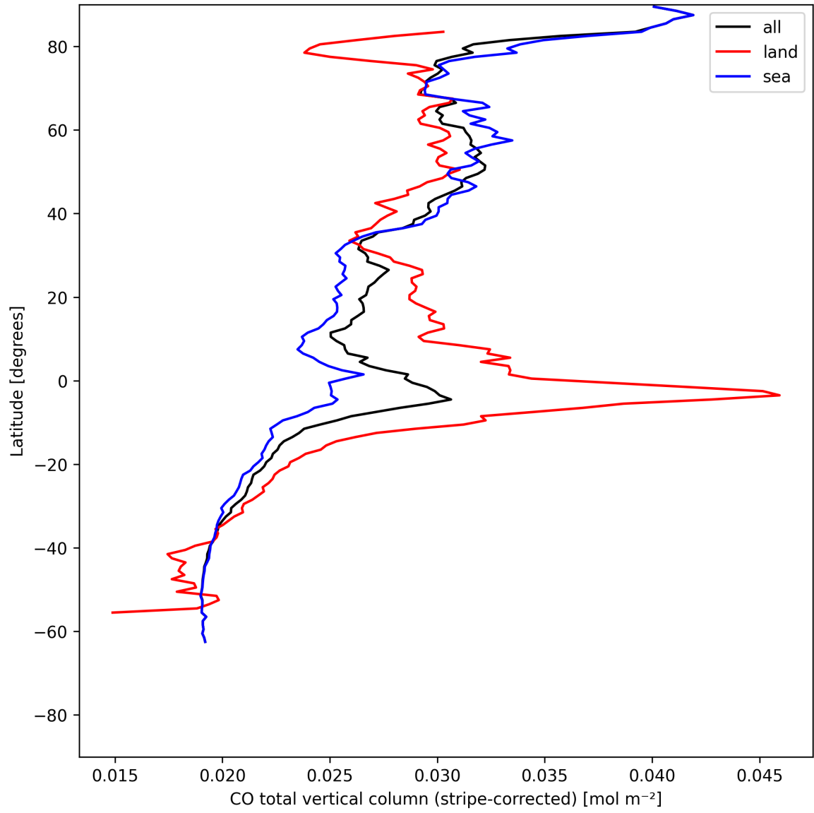
Figure 11: Zonal average of “CO total vertical column (stripe-corrected)” for 2025-07-13 to 2025-07-14.
