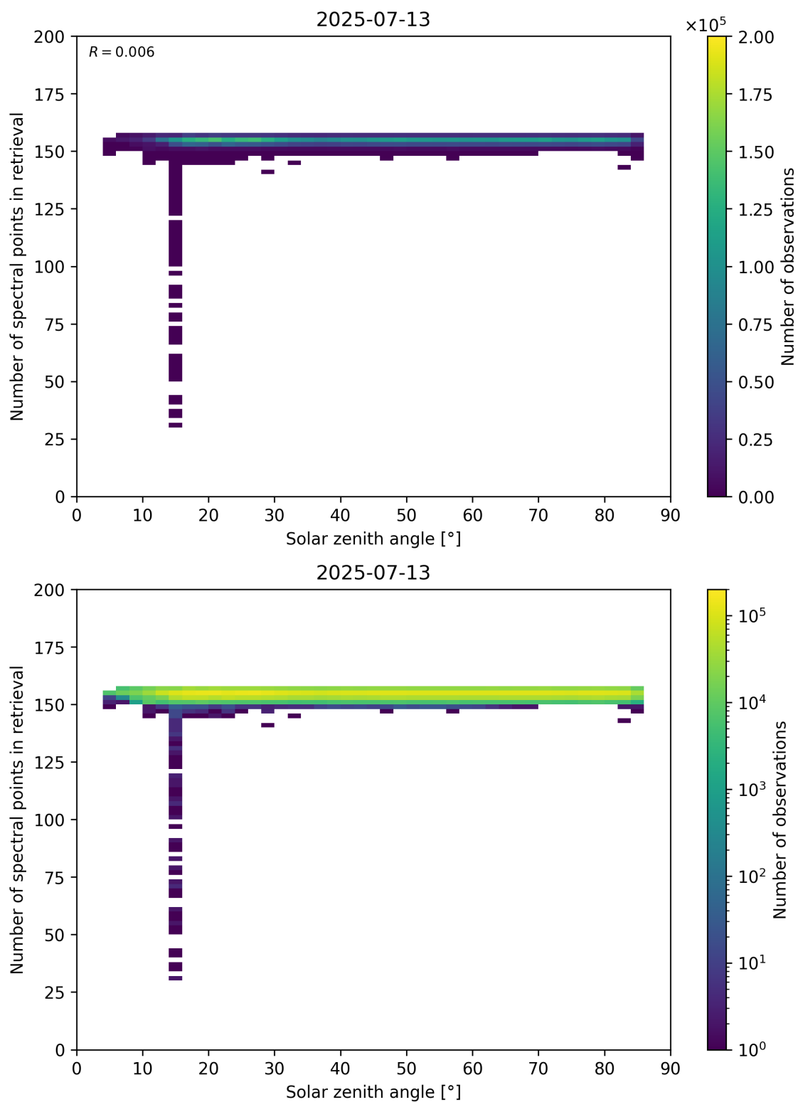
Figure 68: Scatter density plot of “Solar zenith angle” against “Number of spectral points in retrieval” for 2025-07-13 to 2025-07-14.
