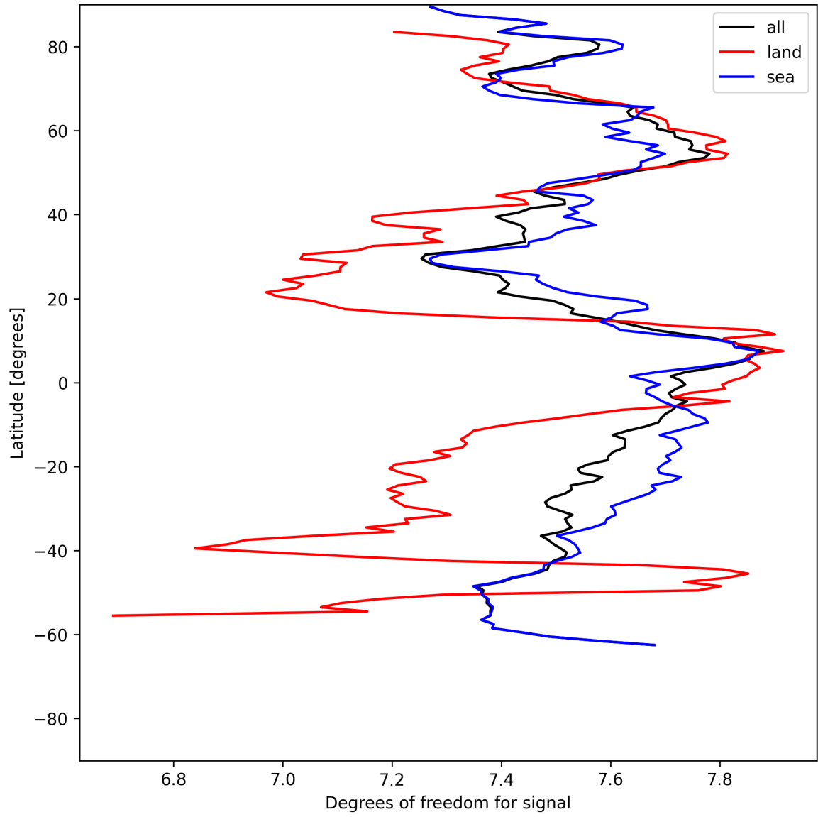
Figure 15: Zonal average of “Degrees of freedom for signal” for 2025-07-13 to 2025-07-14.
