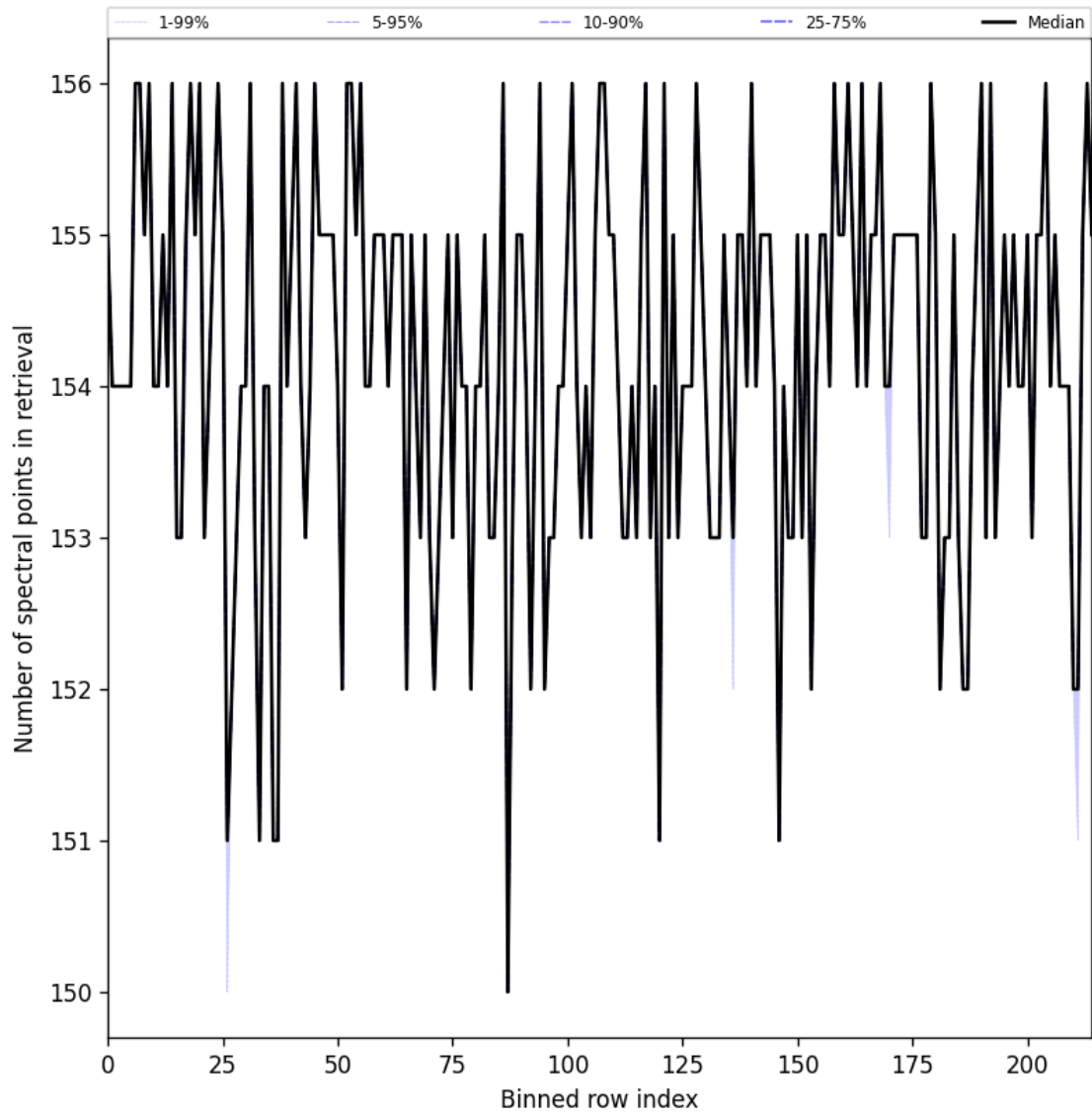
Figure 29: Along track statistics of “Number of spectral points in retrieval” for 2025-07-13 to 2025-07-14
