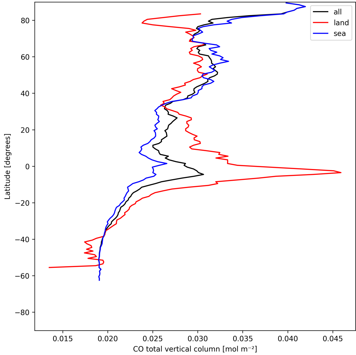
Figure 10: Zonal average of “CO total vertical column” for 2025-07-13 to 2025-07-14.
