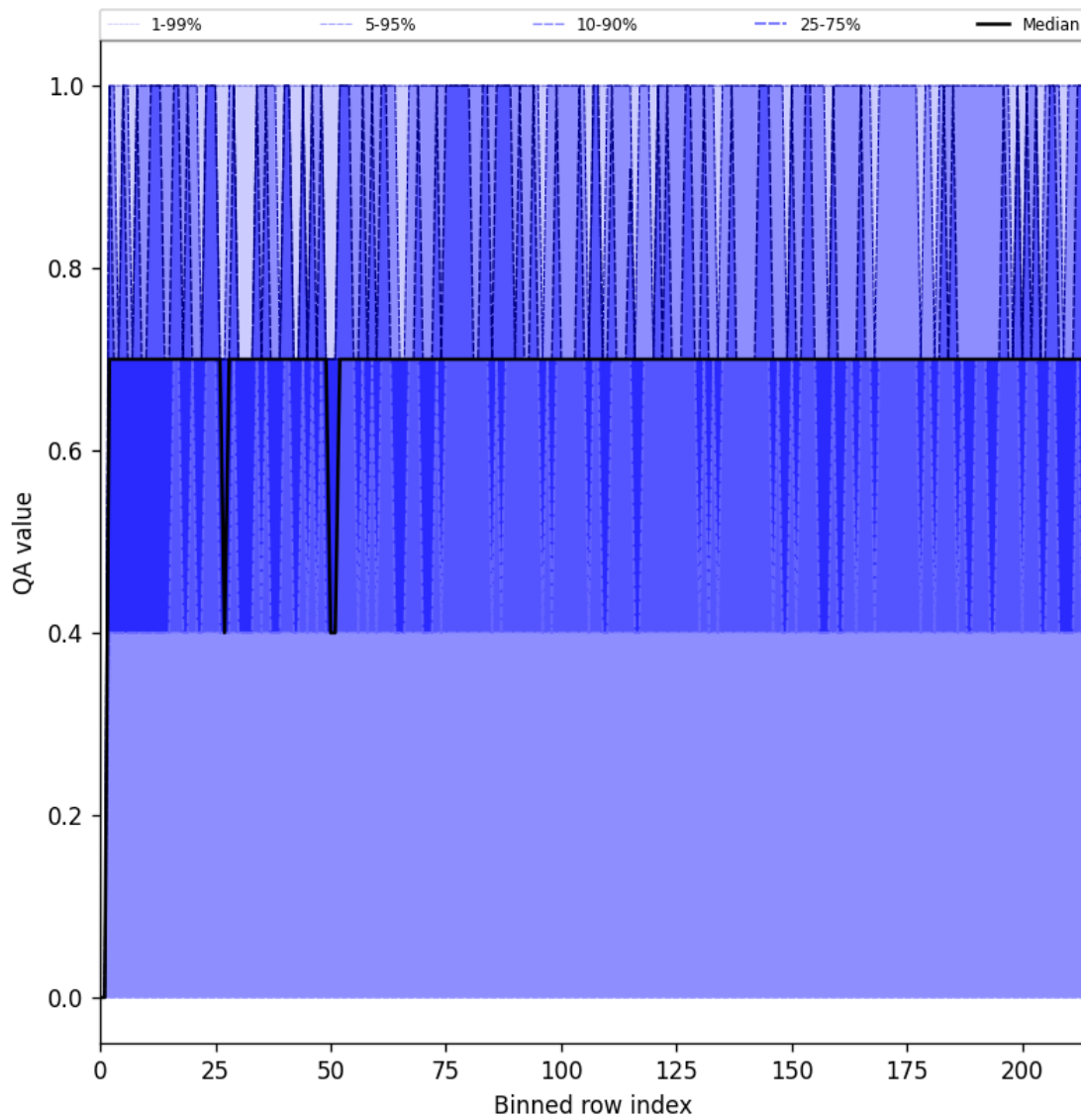
Figure 25: Along track statistics of “QA value” for 2025-07-13 to 2025-07-14
