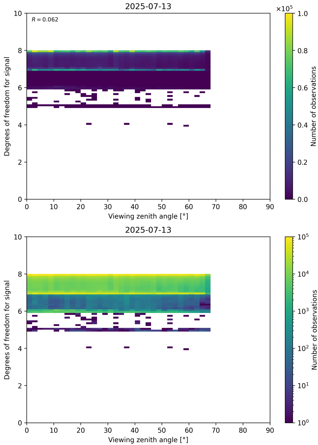
Figure 73: Scatter density plot of “Viewing zenith angle” against “Degrees of freedom for signal” for 2025-07-13 to 2025-07-14.
