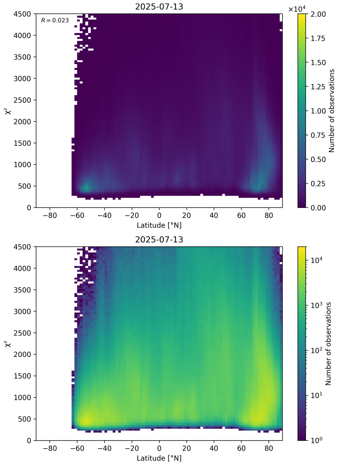
Figure 54: Scatter density plot of “Latitude” against “ \chi^2 ” for 2025-07-13 to 2025-07-14.
