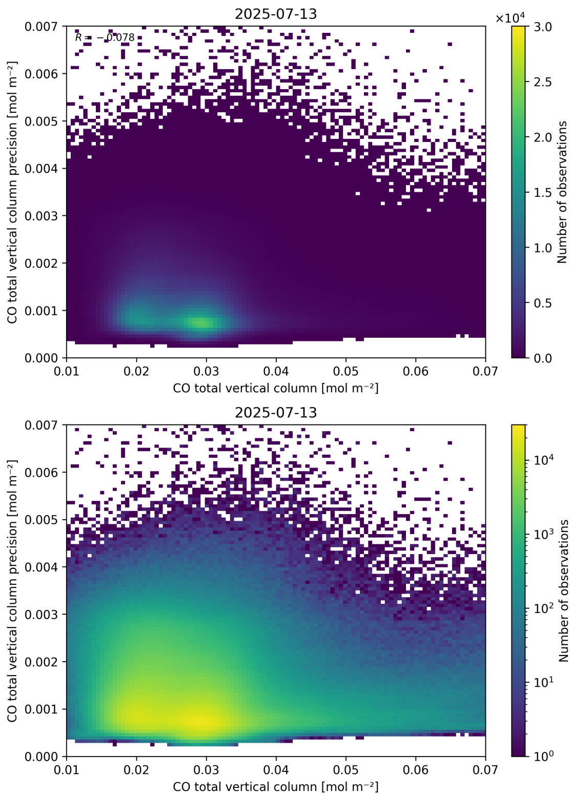
Figure 34: Scatter density plot of “CO total vertical column” against “CO total vertical column precision” for 2025-07-13 to 2025-07-14.
