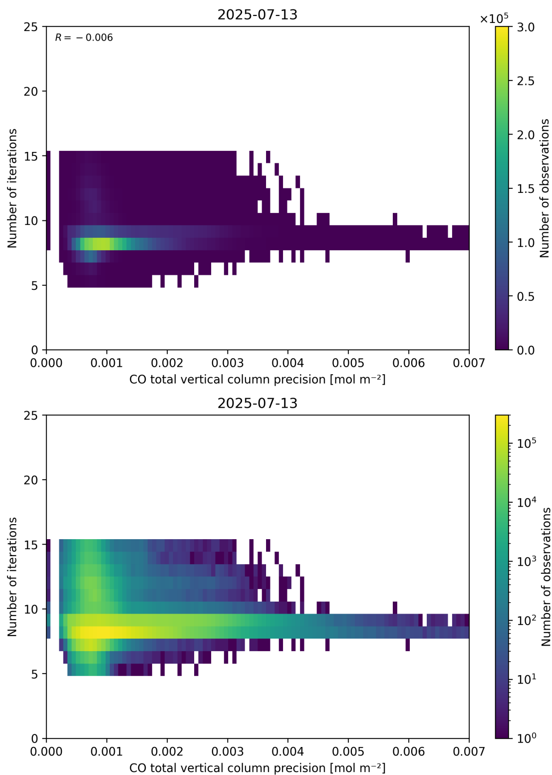
Figure 46: Scatter density plot of “CO total vertical column precision” against “Number of iterations” for 2025-07-13 to 2025-07-14.
