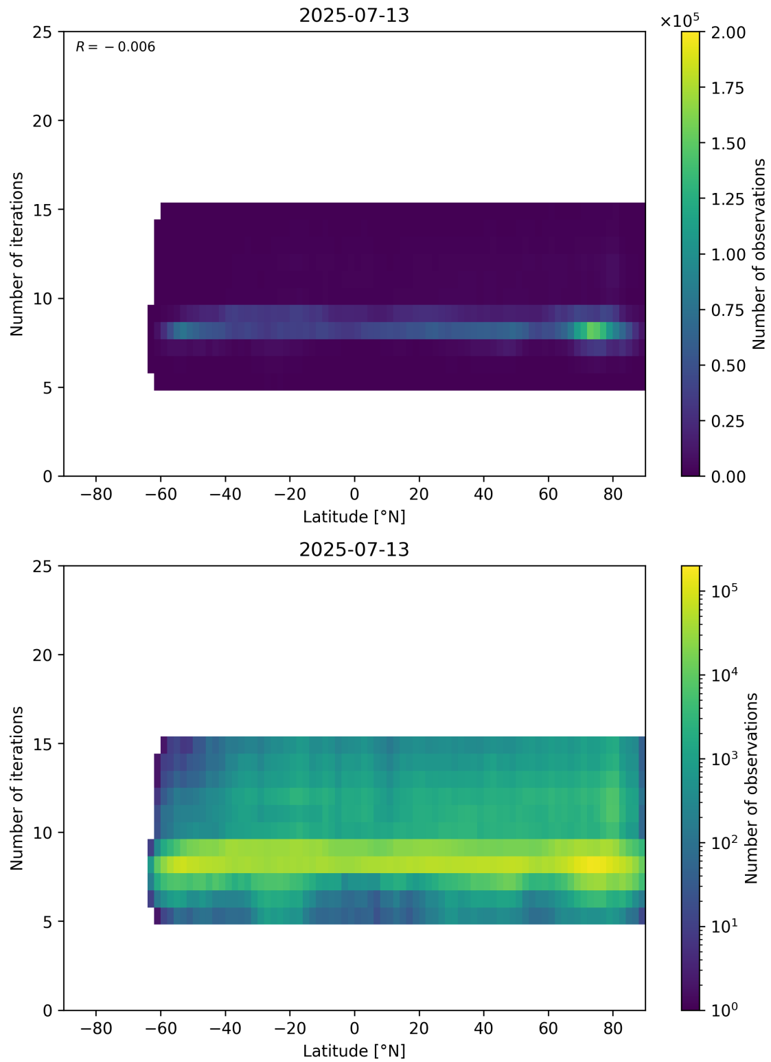
Figure 56: Scatter density plot of “Latitude” against “Number of iterations” for 2025-07-13 to 2025-07-14.
