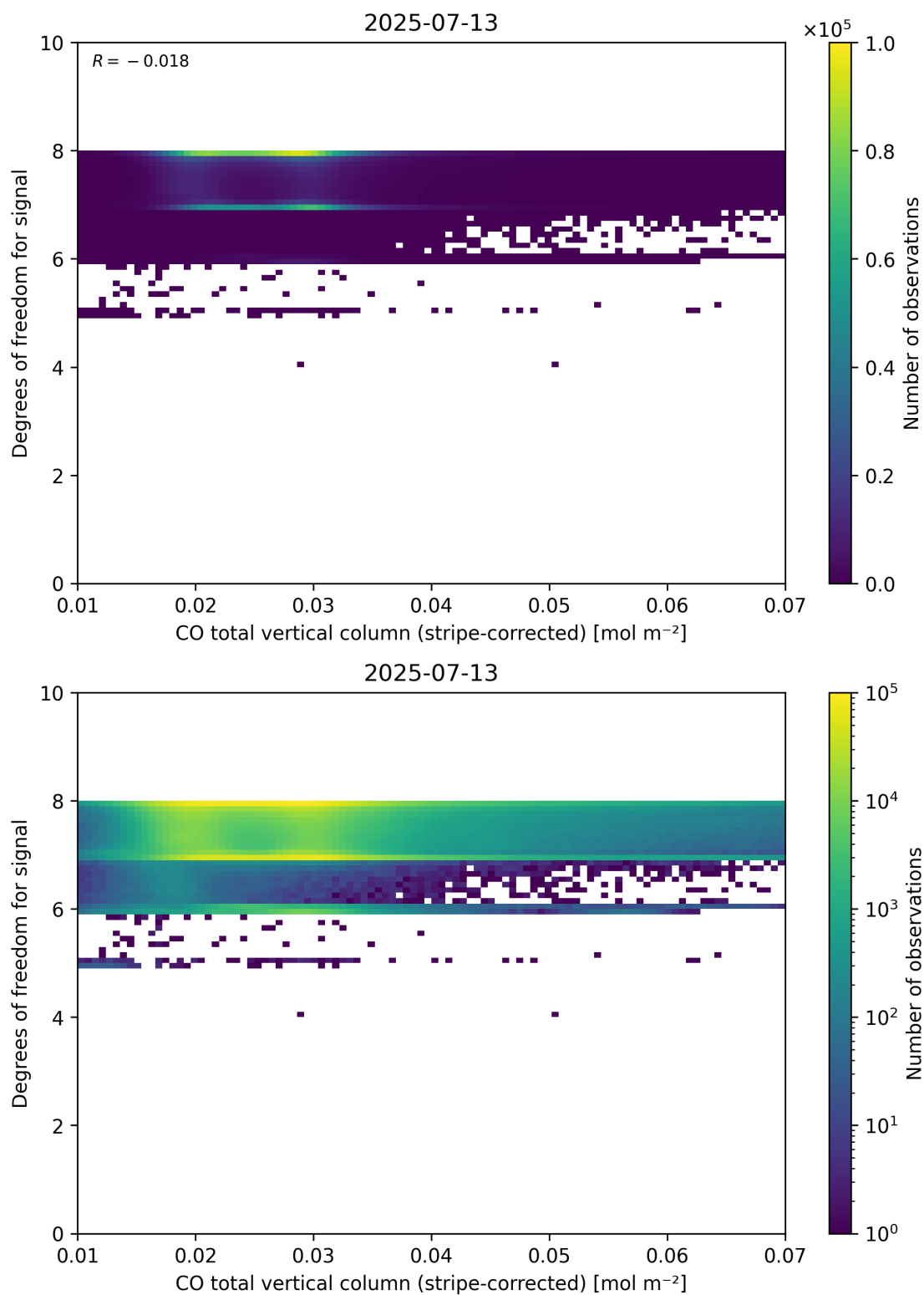
Figure 38: Scatter density plot of “CO total vertical column (stripe-corrected)” against “Degrees of freedom for signal” for 2025-07-13 to 2025-07-14.
