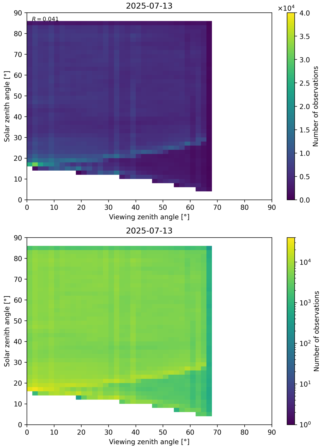
Figure 77: Scatter density plot of “Viewing zenith angle” against “Solar zenith angle” for 2025-07-13 to 2025-07-14.
