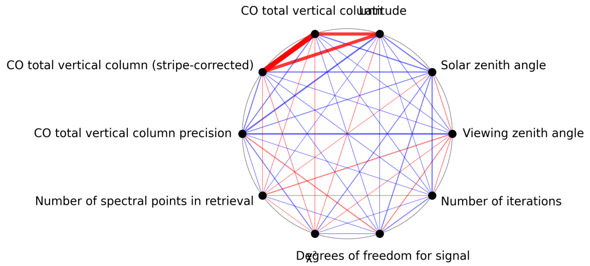
Figure 1: Map of correlation graph for 2025-07-13 to 2025-07-14.
