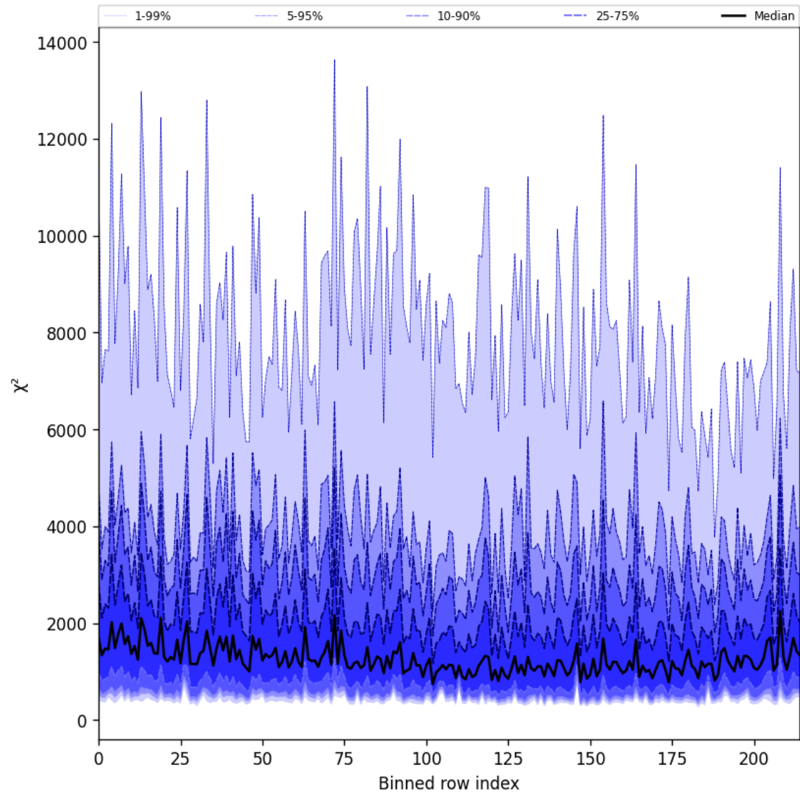
Figure 30: Along track statistics of “ \chi^2 ” for 2025-07-13 to 2025-07-14
