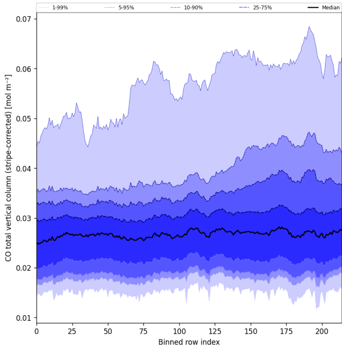
Figure 27: Along track statistics of “CO total vertical column (stripe-corrected)” for 2025-07-13 to 2025-07-14
