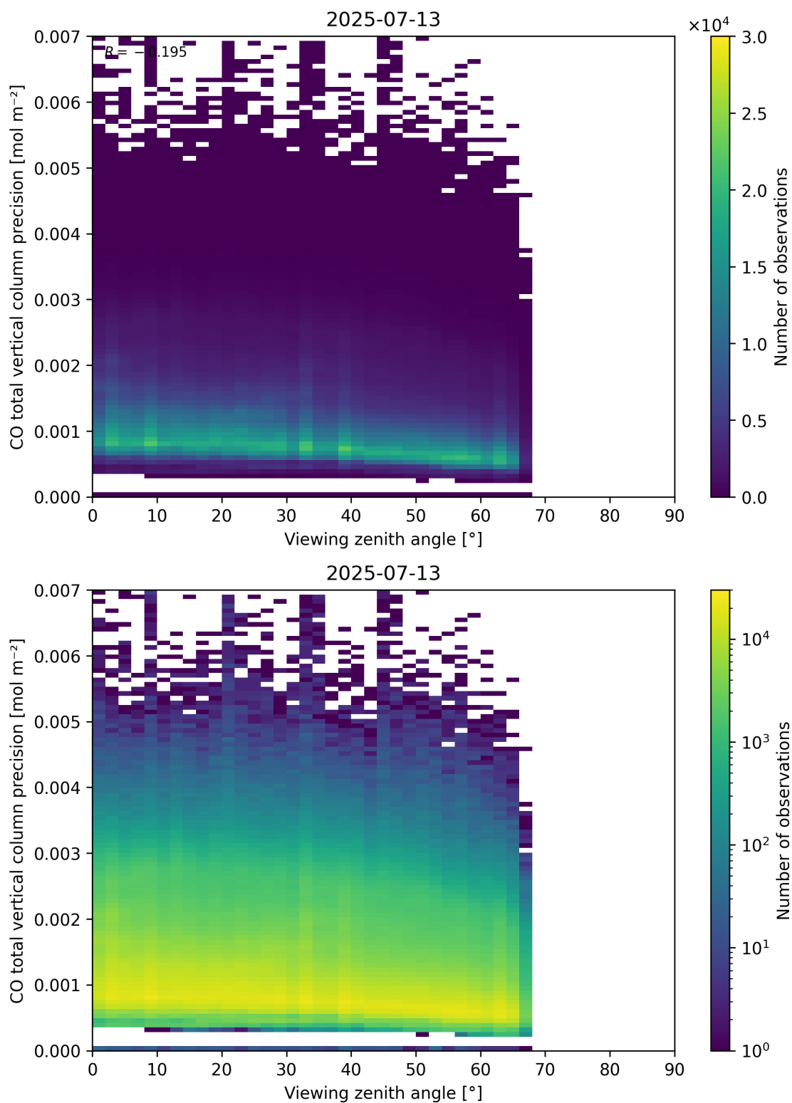
Figure 71: Scatter density plot of “Viewing zenith angle” against “CO total vertical column precision” for 2025-07-13 to 2025-07-14.
