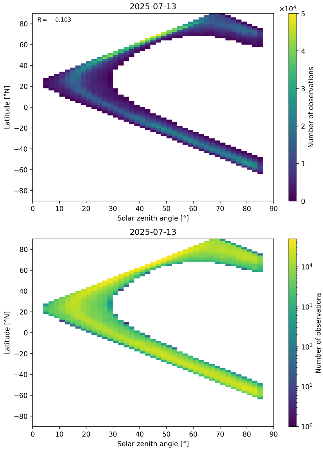
Figure 66: Scatter density plot of “Solar zenith angle” against “Latitude” for 2025-07-13 to 2025-07-14.
