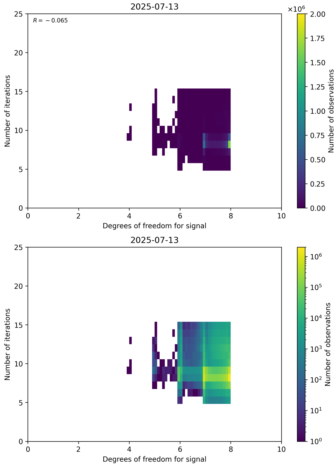
Figure 50: Scatter density plot of “Degrees of freedom for signal” against “Number of iterations” for 2025-07-13 to 2025-07-14.
