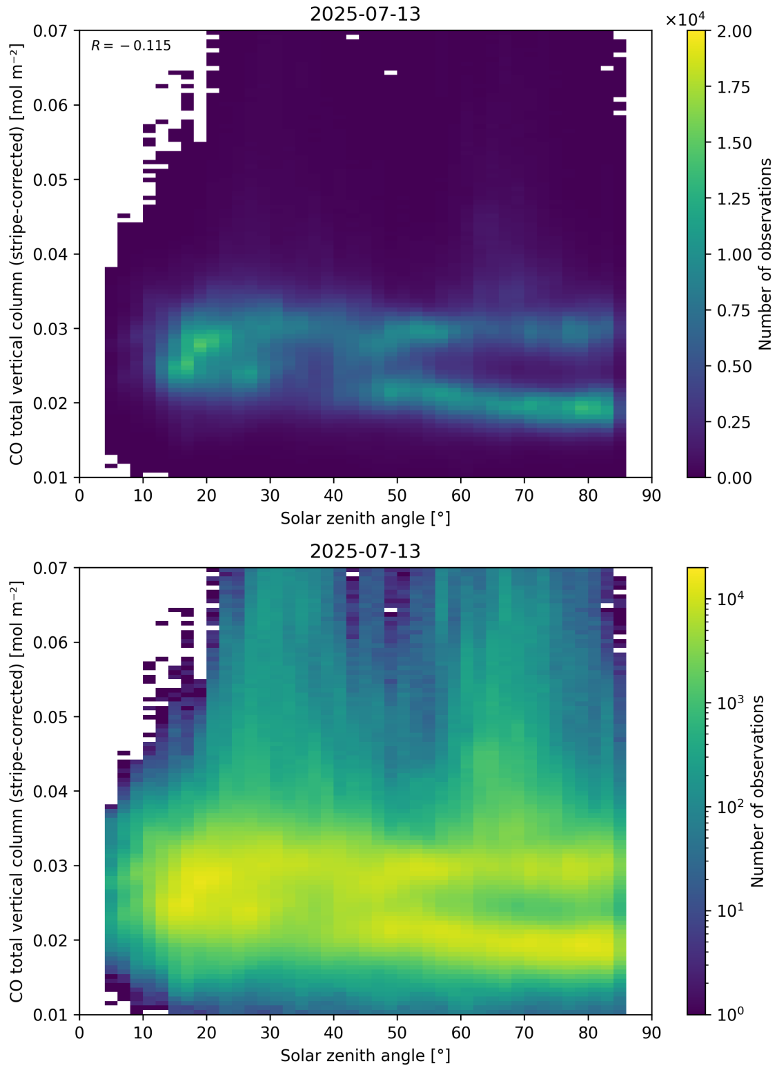
Figure 62: Scatter density plot of “Solar zenith angle” against “CO total vertical column (stripe-corrected)” for 2025-07-13 to 2025-07-14.
