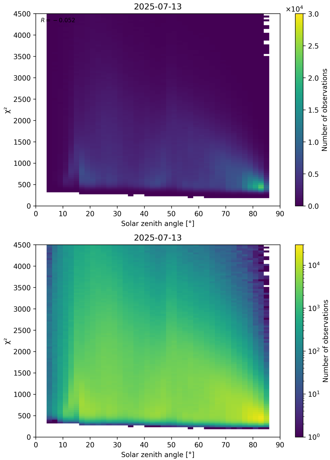
Figure 64: Scatter density plot of “Solar zenith angle” against “ \chi^2 ” for 2025-07-13 to 2025-07-14.
