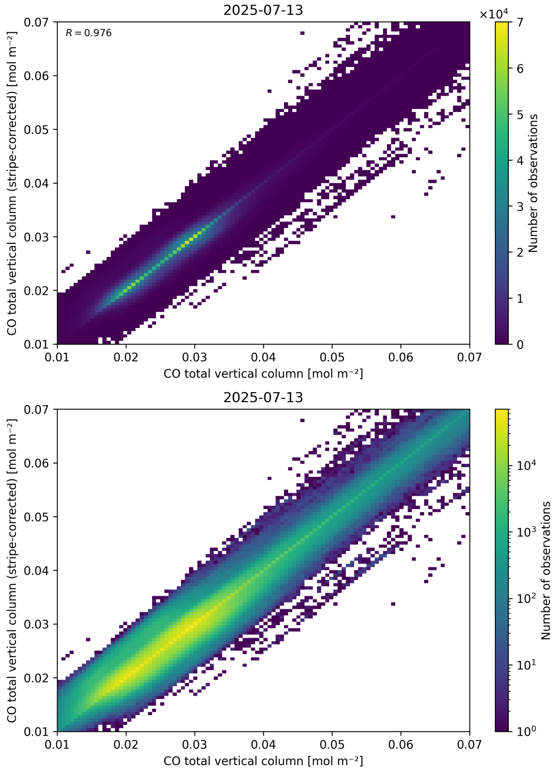
Figure 33: Scatter density plot of “CO total vertical column” against “CO total vertical column (stripe-corrected)” for 2025-07-13 to 2025-07-14.
