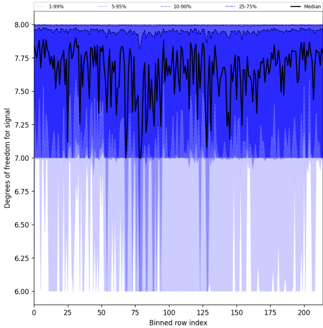
Figure 31: Along track statistics of “Degrees of freedom for signal” for 2025-07-13 to 2025-07-14
