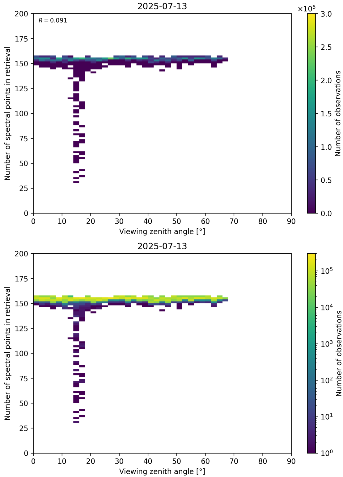
Figure 76: Scatter density plot of “Viewing zenith angle” against “Number of spectral points in retrieval” for 2025-07-13 to 2025-07-14.
