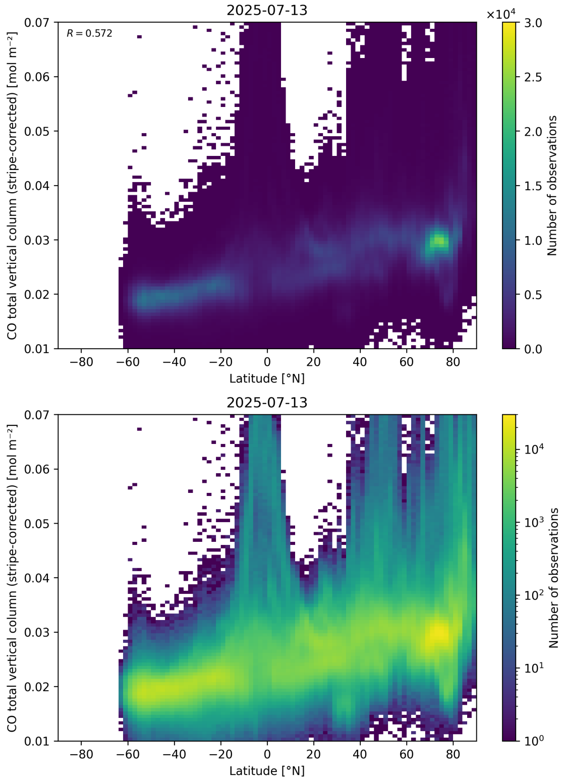
Figure 52: Scatter density plot of “Latitude” against “CO total vertical column (stripe-corrected)” for 2025-07-13 to 2025-07-14.
