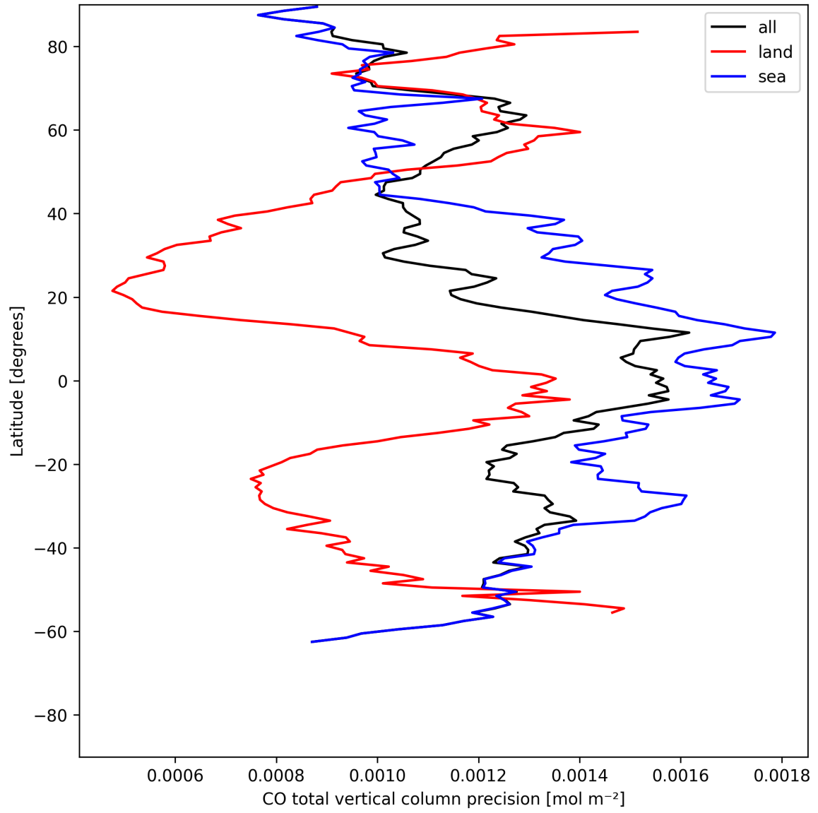
Figure 12: Zonal average of “CO total vertical column precision” for 2025-07-13 to 2025-07-14.
