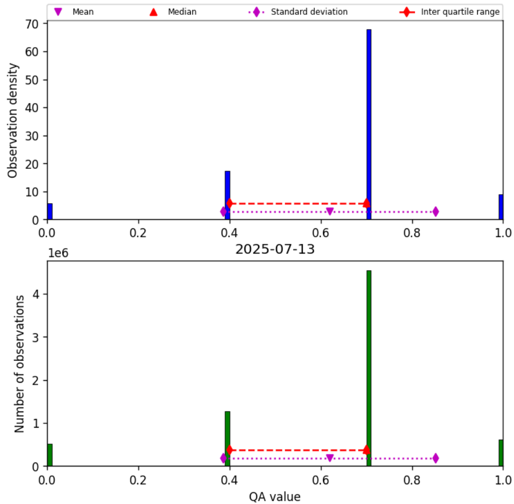
Figure 17: Histogram of “QA value” for 2025-07-13 to 2025-07-14
