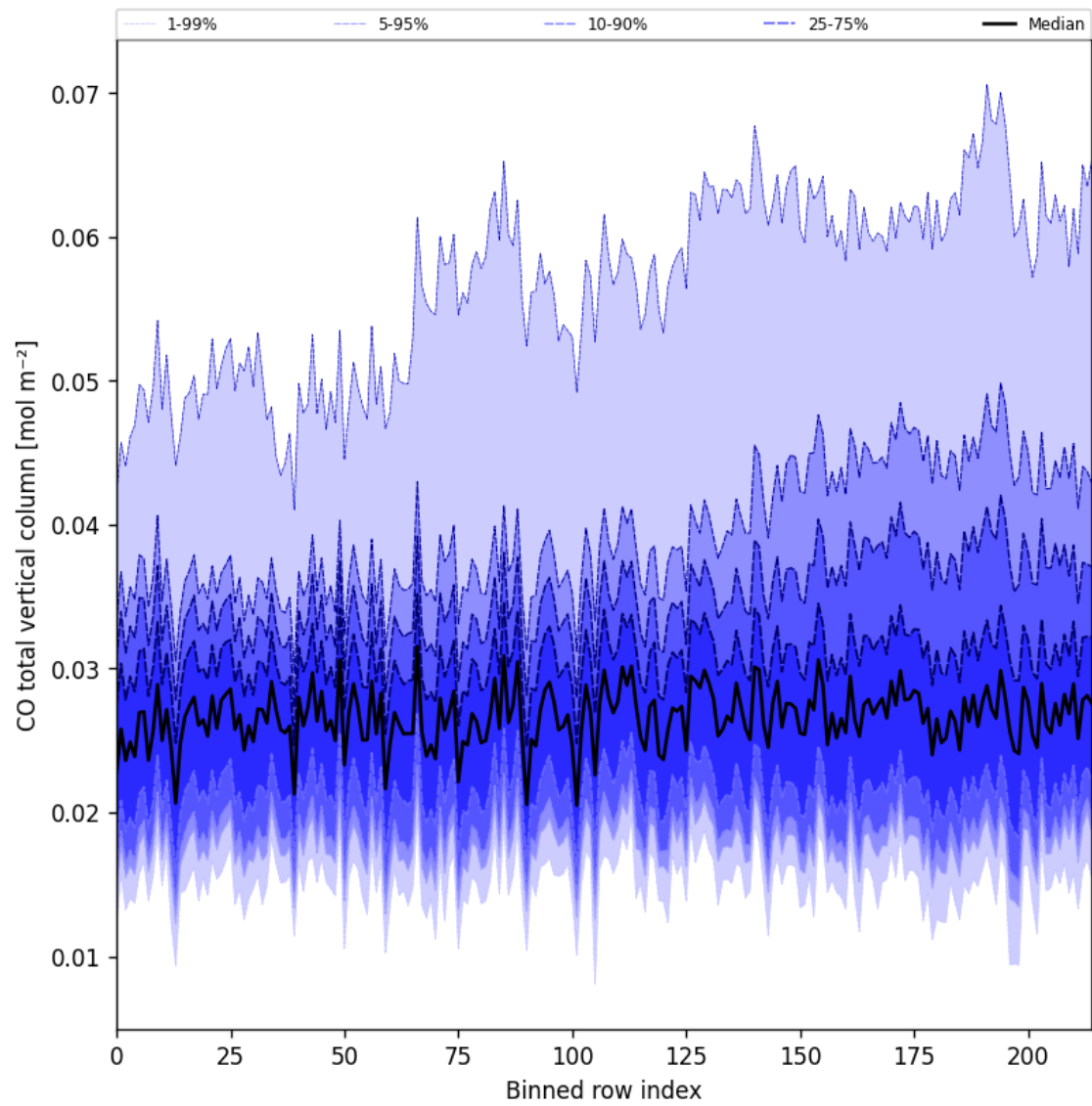
Figure 26: Along track statistics of “CO total vertical column” for 2025-07-13 to 2025-07-14
