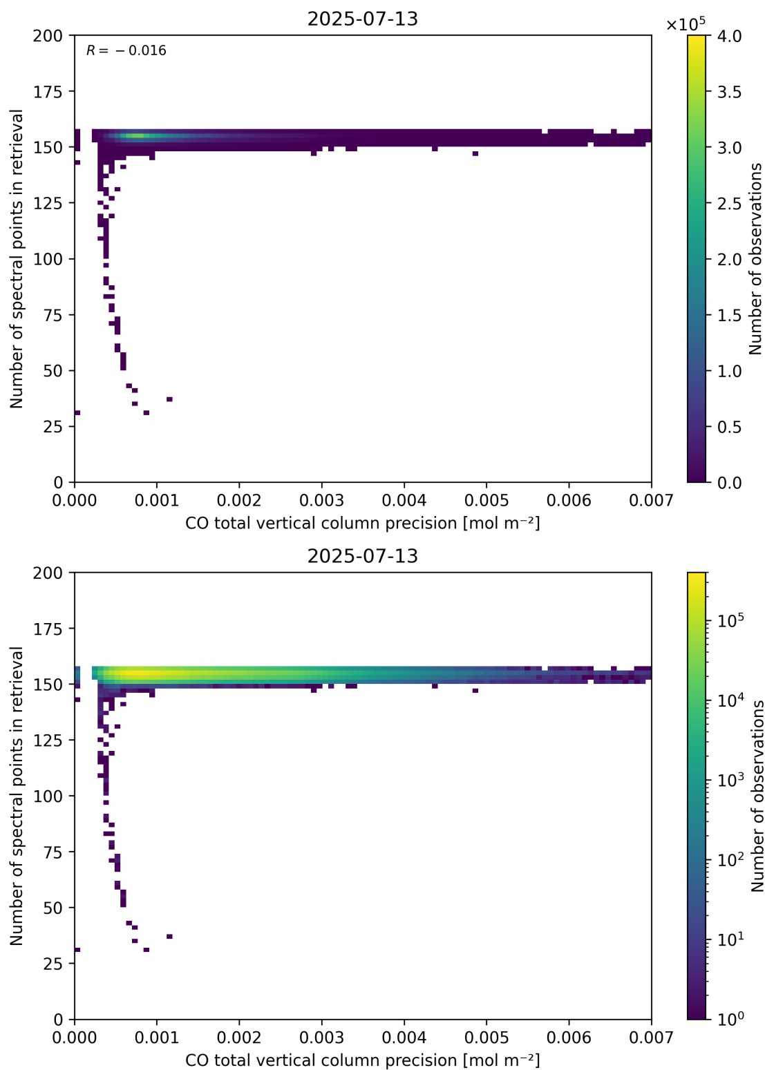
Figure 47: Scatter density plot of “CO total vertical column precision” against “Number of spectral points in retrieval” for 2025-07-13 to 2025-07-14.
