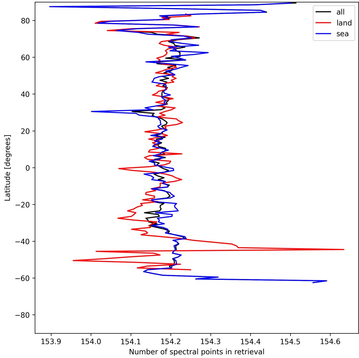
Figure 13: Zonal average of “Number of spectral points in retrieval” for 2025-07-13 to 2025-07-14.
