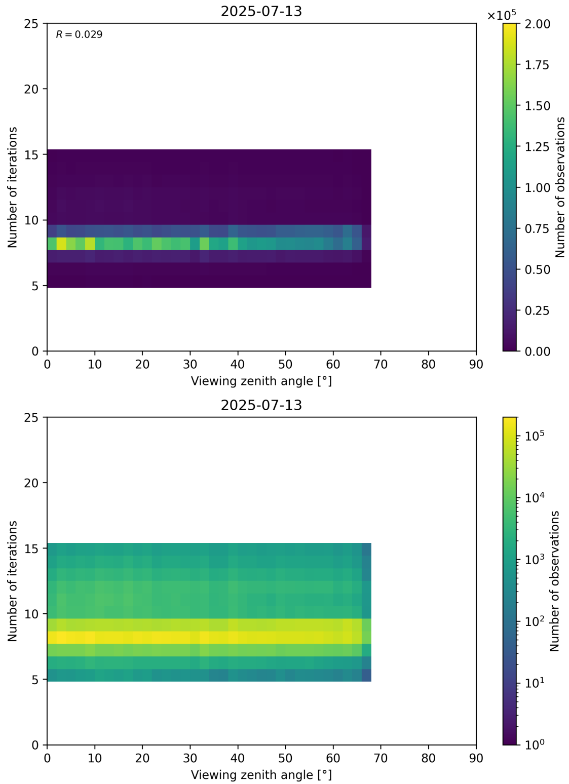
Figure 75: Scatter density plot of “Viewing zenith angle” against “Number of iterations” for 2025-07-13 to 2025-07-14.
