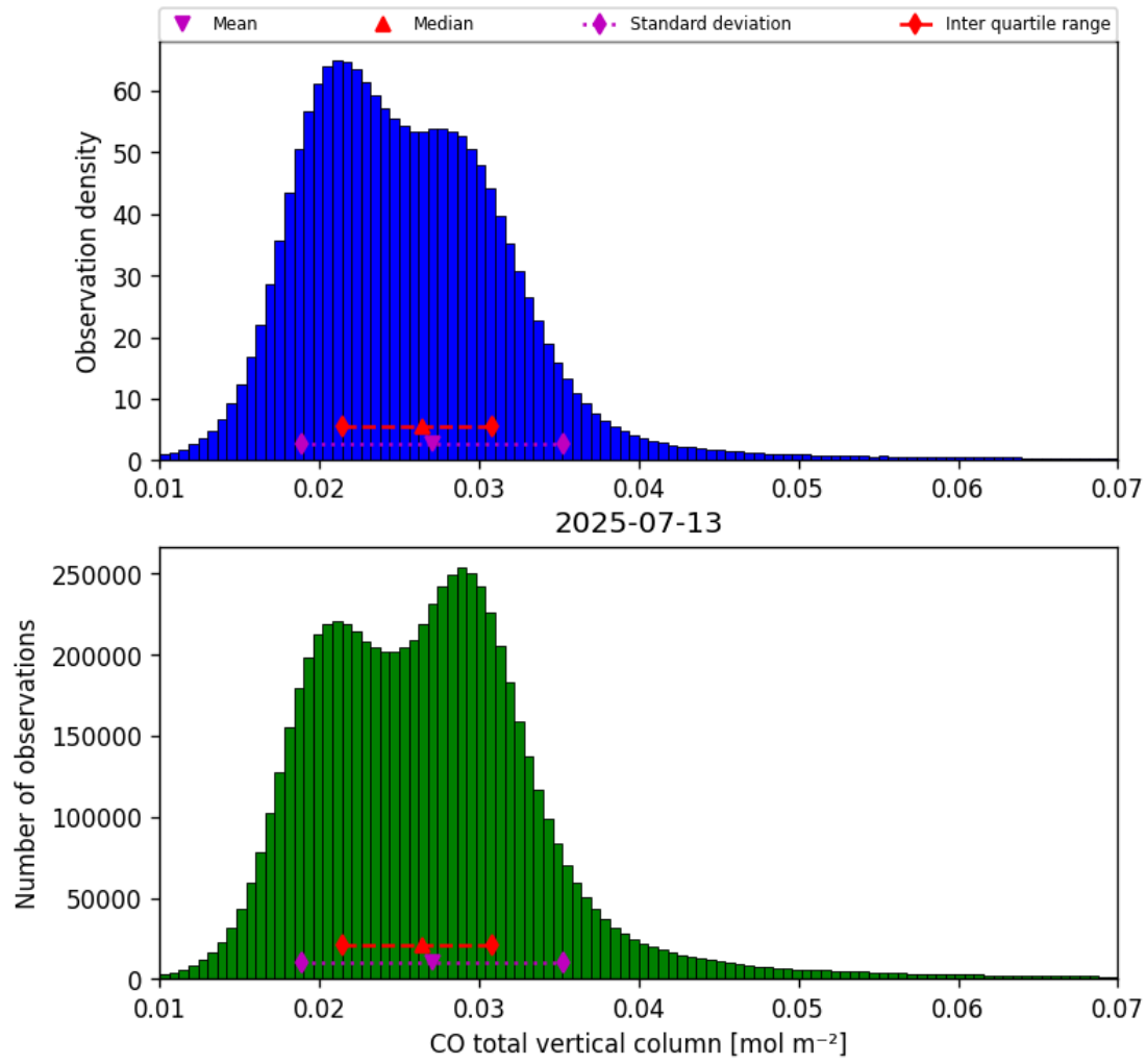
Figure 18: Histogram of “CO total vertical column” for 2025-07-13 to 2025-07-14
