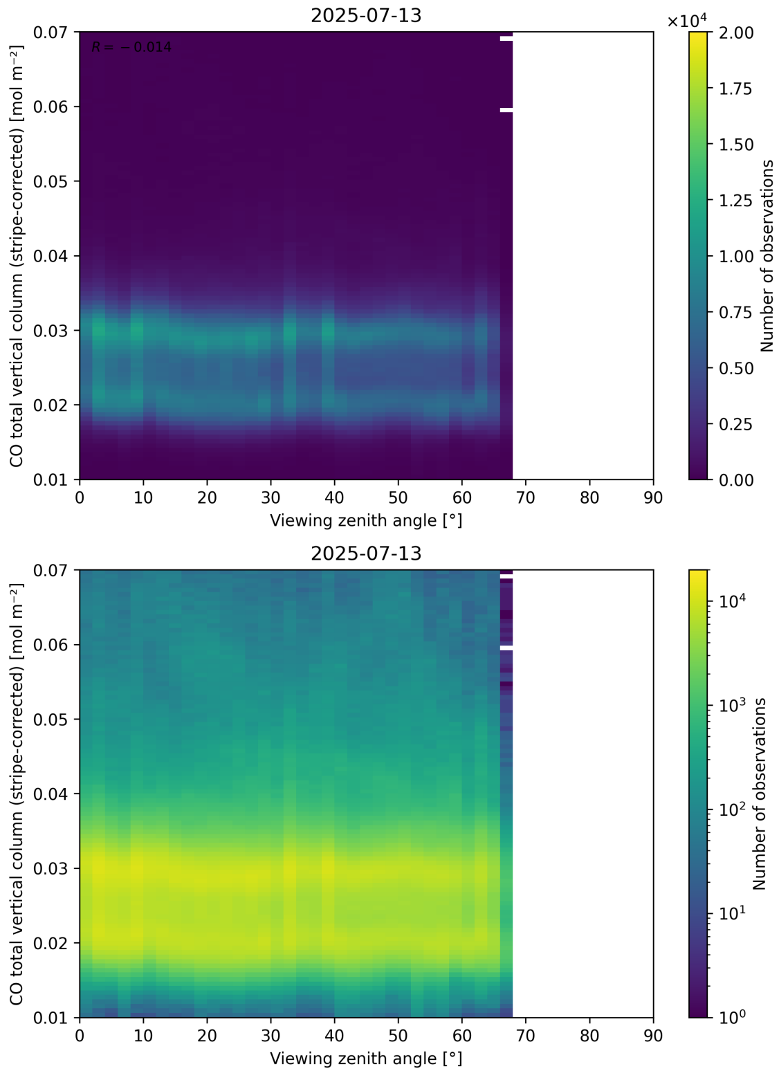
Figure 70: Scatter density plot of “Viewing zenith angle” against “CO total vertical column (stripe-corrected)” for 2025-07-13 to 2025-07-14.
