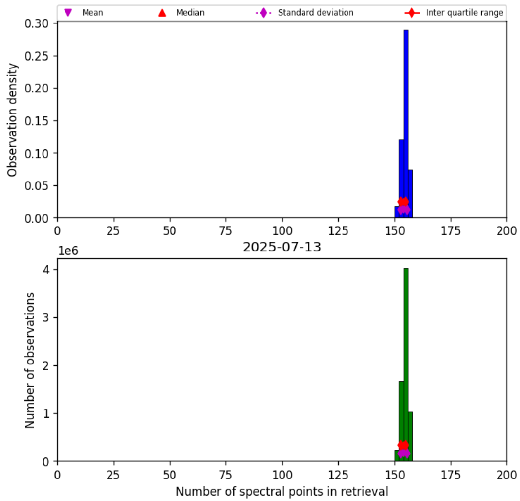
Figure 21: Histogram of “Number of spectral points in retrieval” for 2025-07-13 to 2025-07-14
