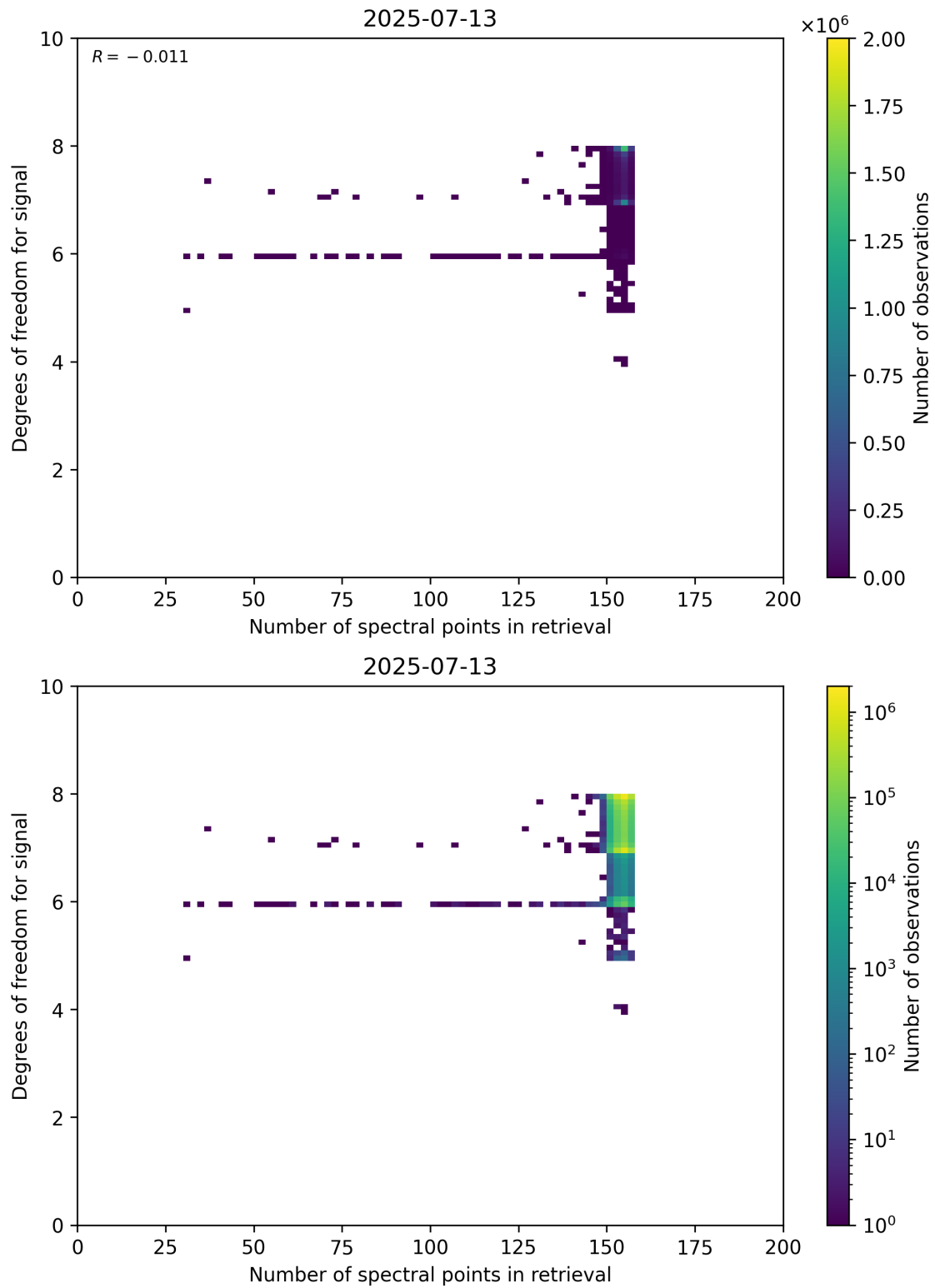
Figure 59: Scatter density plot of “Number of spectral points in retrieval” against “Degrees of freedom for signal” for 2025-07-13 to 2025-07-14.
