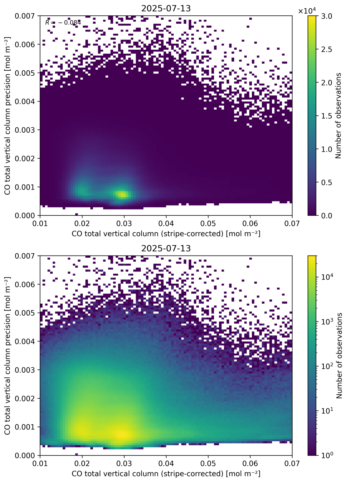
Figure 36: Scatter density plot of “CO total vertical column (stripe-corrected)” against “CO total vertical column precision” for 2025-07-13 to 2025-07-14.
