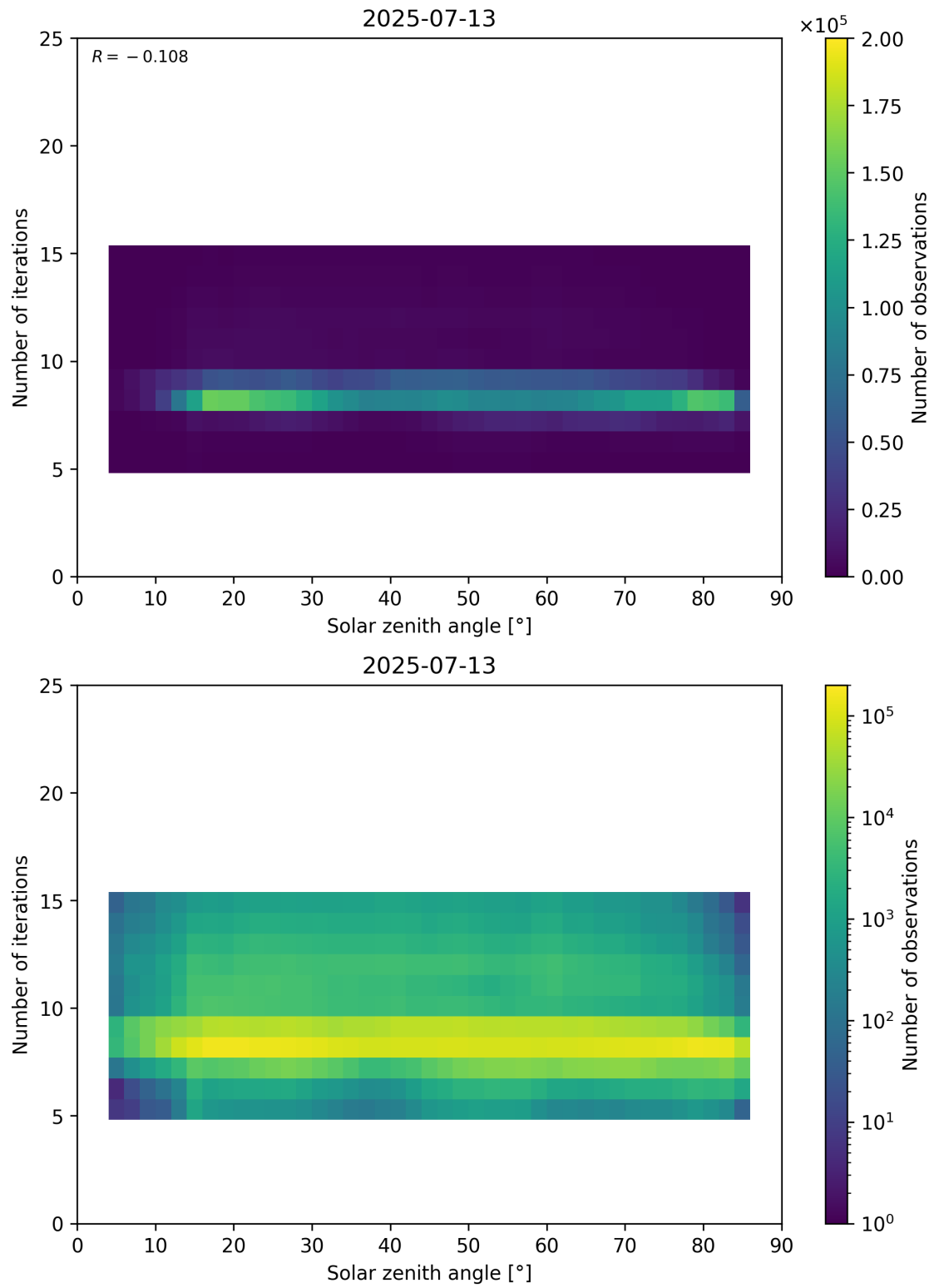
Figure 67: Scatter density plot of “Solar zenith angle” against “Number of iterations” for 2025-07-13 to 2025-07-14.
