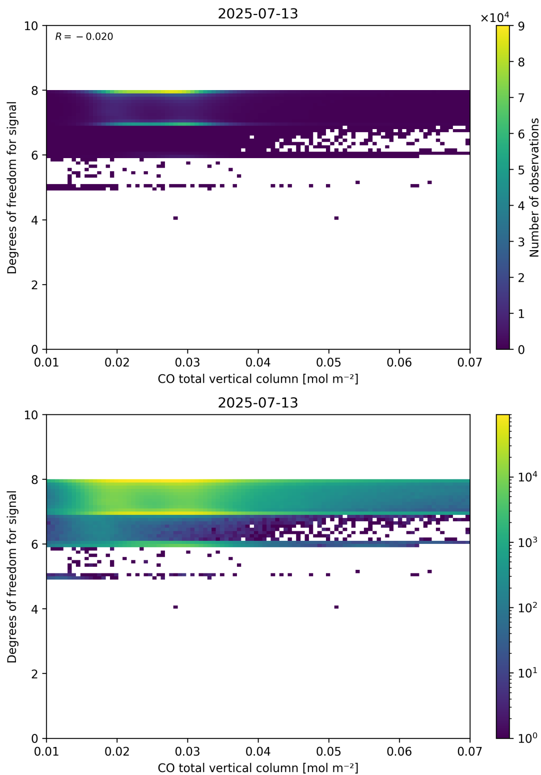
Figure 41: Scatter density plot of “CO total vertical column” against “Degrees of freedom for signal” for 2025-07-13 to 2025-07-14.
