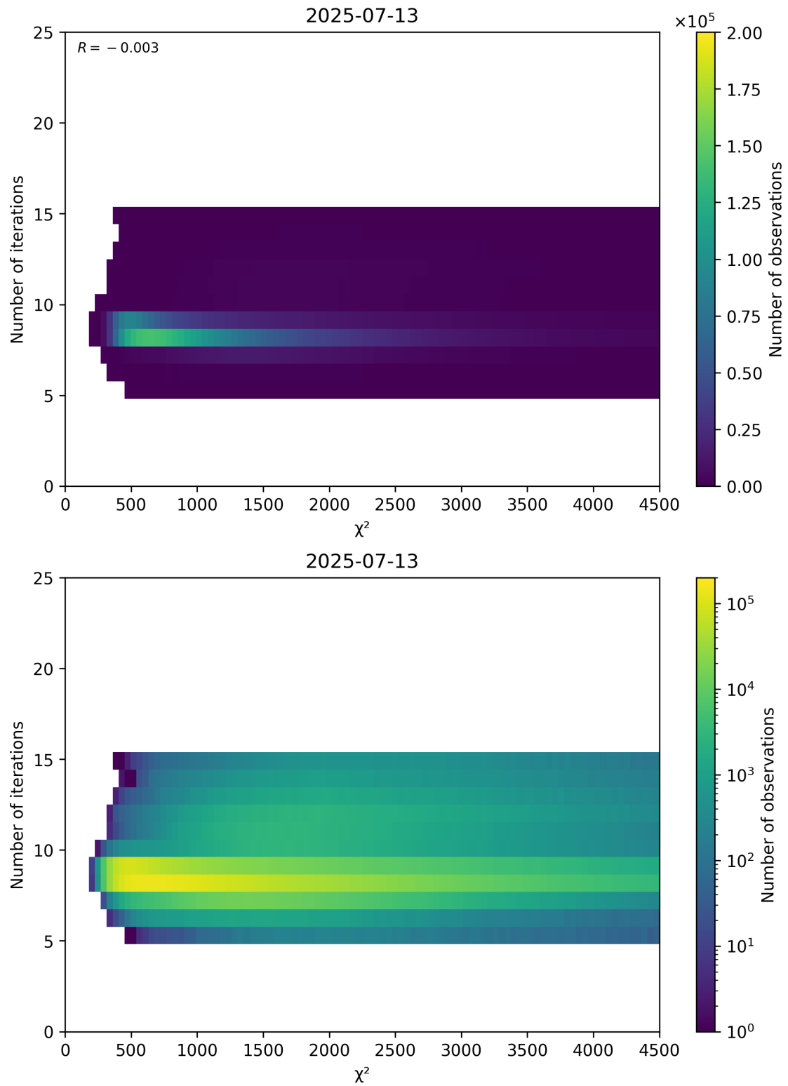
Figure 49: Scatter density plot of “ \chi^2 ” against “Number of iterations” for 2025-07-13 to 2025-07-14.
