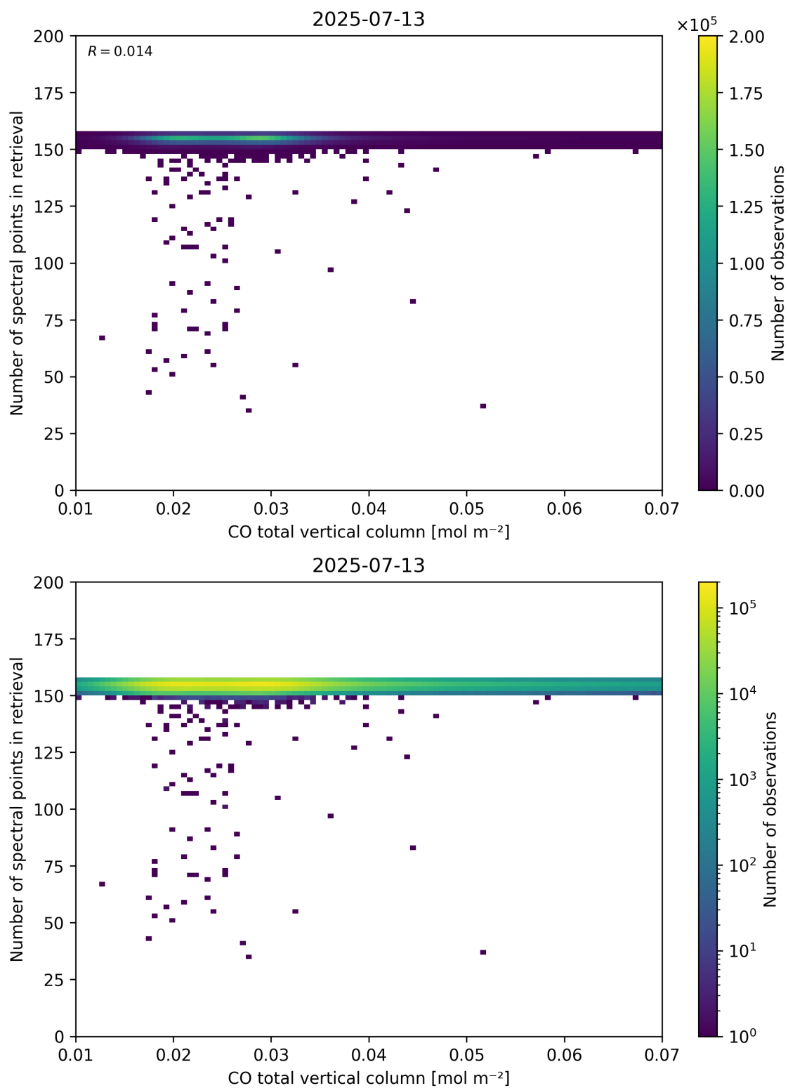
Figure 43: Scatter density plot of “CO total vertical column” against “Number of spectral points in retrieval” for 2025-07-13 to 2025-07-14.
