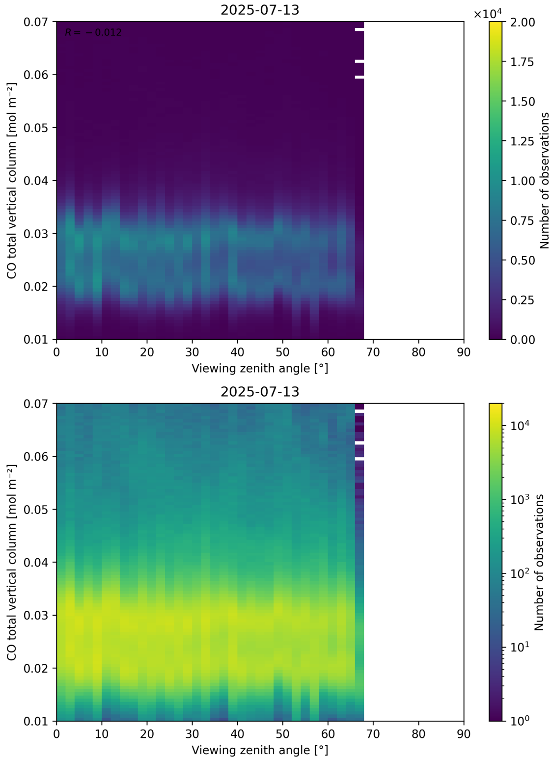
Figure 69: Scatter density plot of “Viewing zenith angle” against “CO total vertical column” for 2025-07-13 to 2025-07-14.
