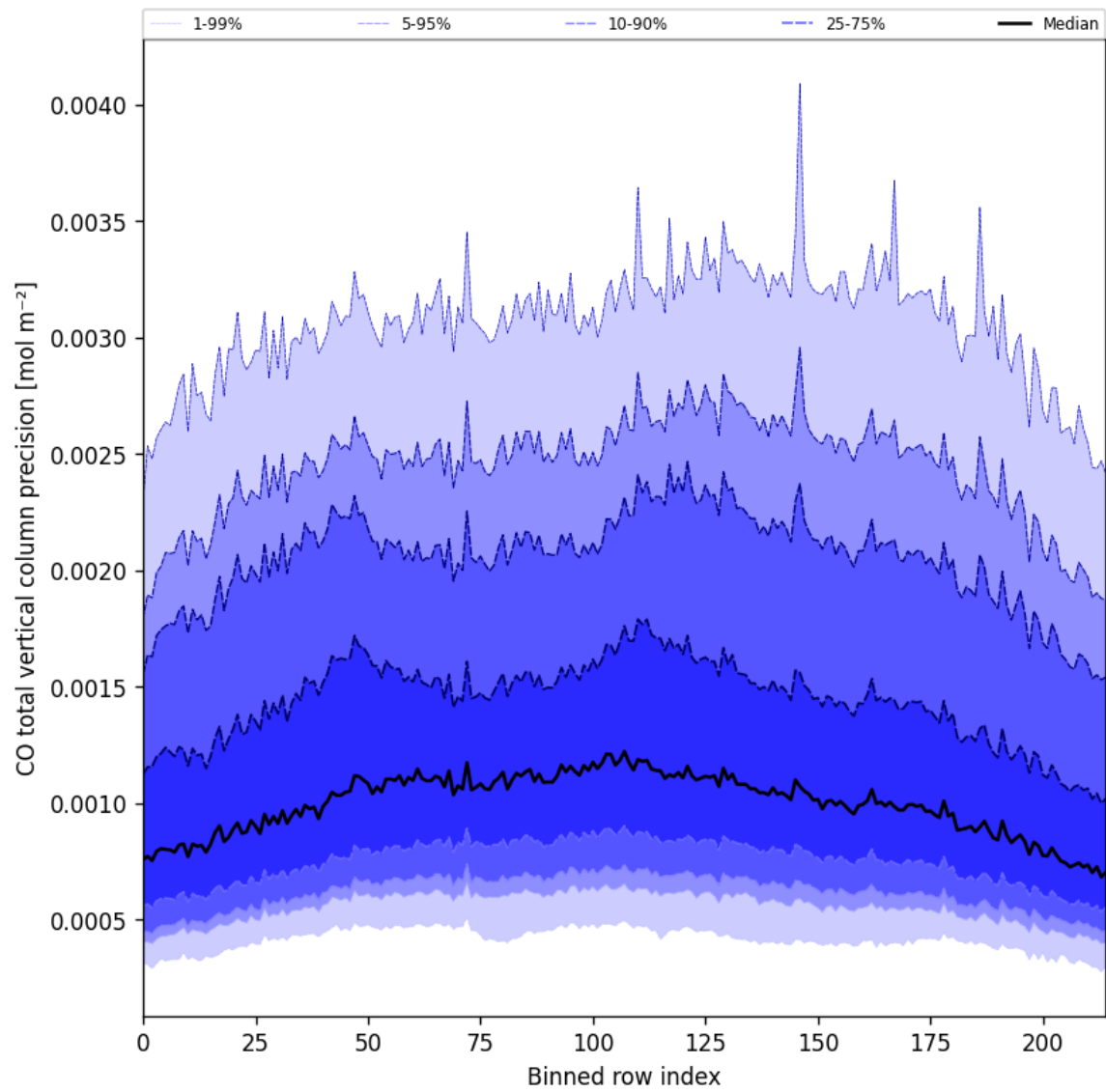
Figure 28: Along track statistics of “CO total vertical column precision” for 2025-07-13 to 2025-07-14
