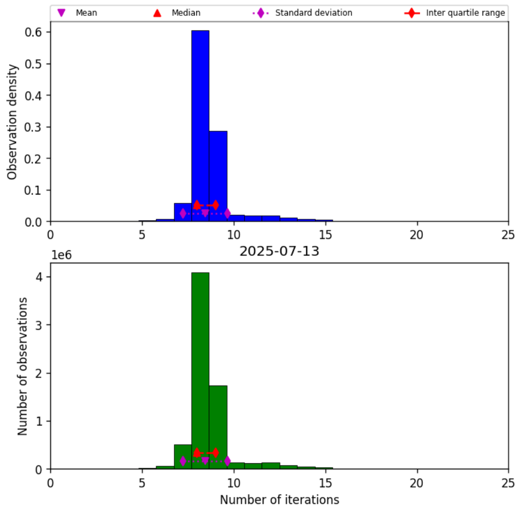
Figure 24: Histogram of “Number of iterations” for 2025-07-13 to 2025-07-14
