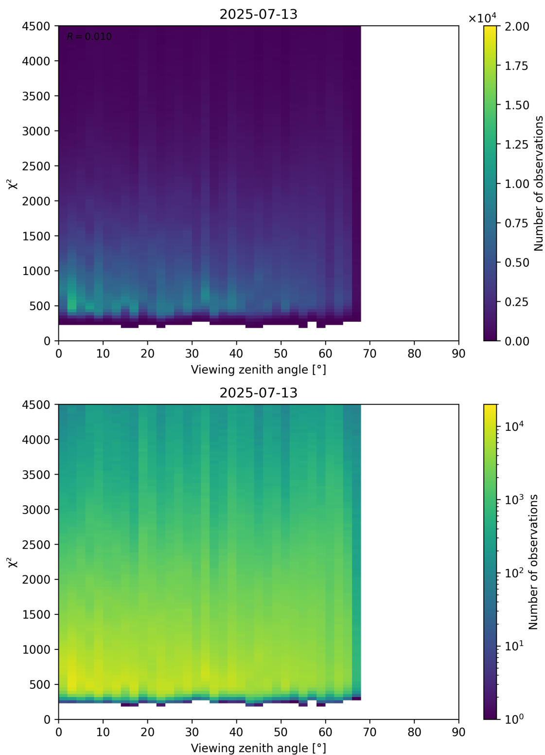
Figure 72: Scatter density plot of “Viewing zenith angle” against “ \chi^2 ” for 2025-07-13 to 2025-07-14.
