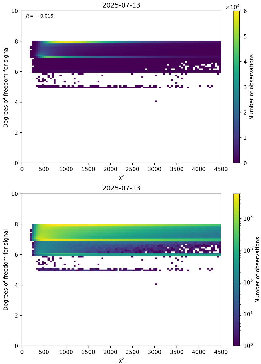
Figure 48: Scatter density plot of “ \chi^2 ” against “Degrees of freedom for signal” for 2025-07-13 to 2025-07-14.
