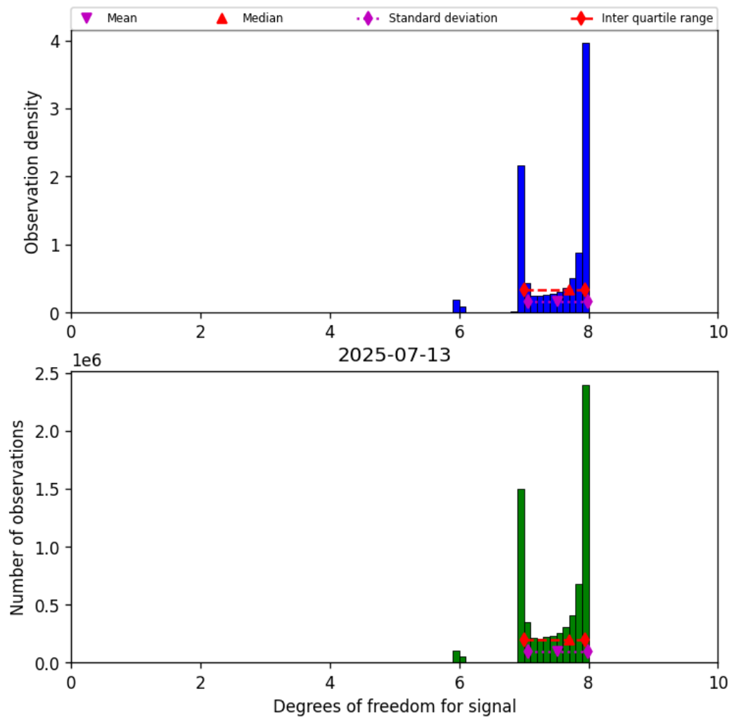
Figure 23: Histogram of “Degrees of freedom for signal” for 2025-07-13 to 2025-07-14
