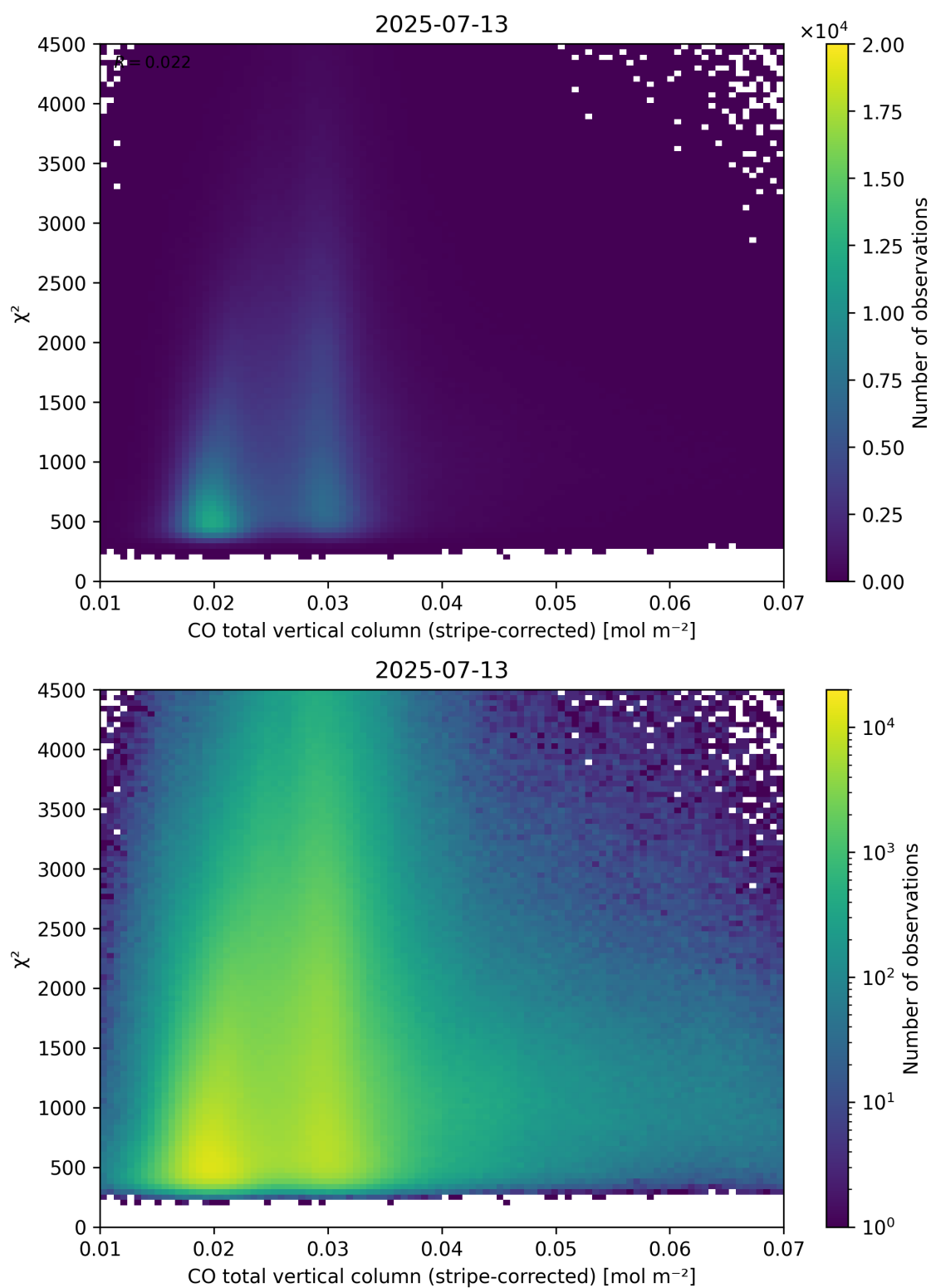
Figure 37: Scatter density plot of “CO total vertical column (stripe-corrected)” against “ \chi^2 ” for 2025-07-13 to 2025-07-14.
