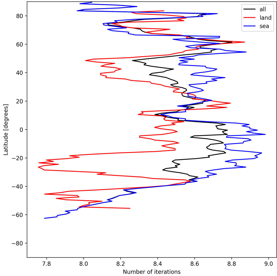
Figure 16: Zonal average of “Number of iterations” for 2025-07-13 to 2025-07-14.
