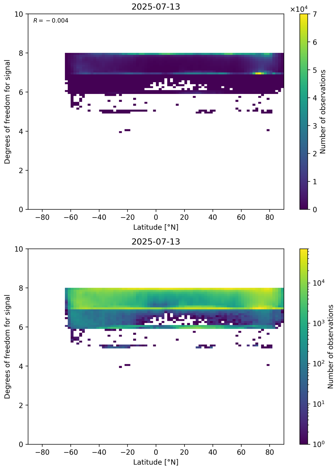
Figure 55: Scatter density plot of “Latitude” against “Degrees of freedom for signal” for 2025-07-13 to 2025-07-14.
