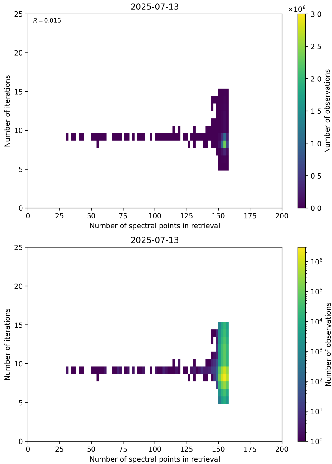
Figure 60: Scatter density plot of “Number of spectral points in retrieval” against “Number of iterations” for 2025-07-13 to 2025-07-14.
