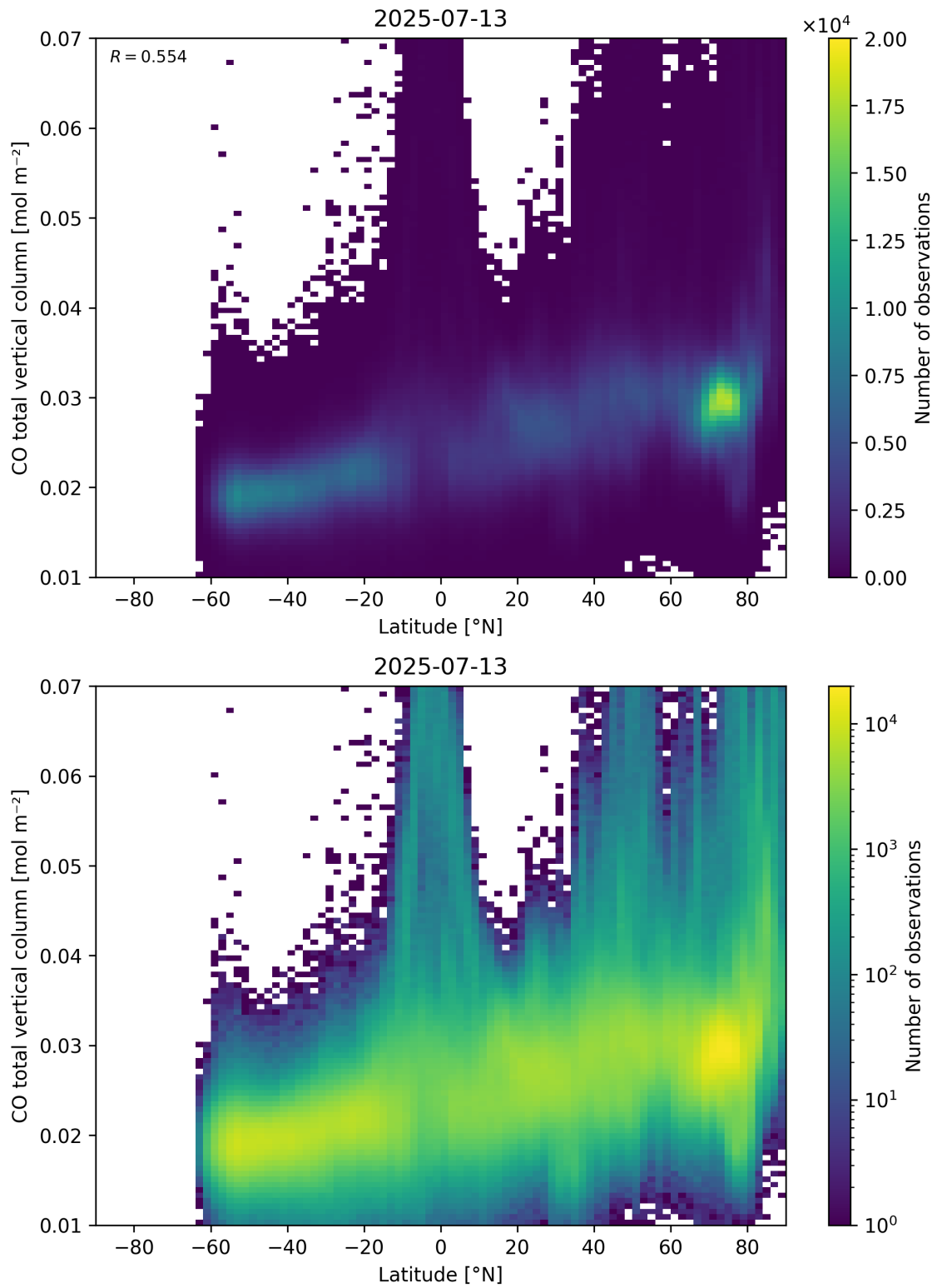
Figure 51: Scatter density plot of “Latitude” against “CO total vertical column” for 2025-07-13 to 2025-07-14.
