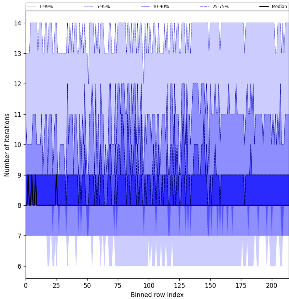
Figure 32: Along track statistics of “Number of iterations” for 2025-07-13 to 2025-07-14
