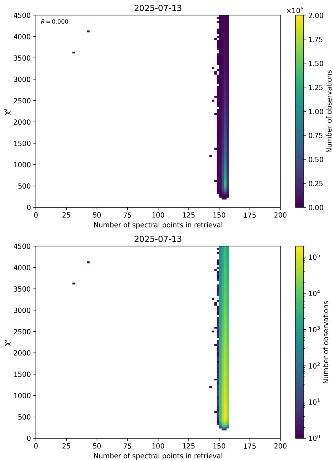
Figure 58: Scatter density plot of “Number of spectral points in retrieval” against “ \chi^2 ” for 2025-07-13 to 2025-07-14.
