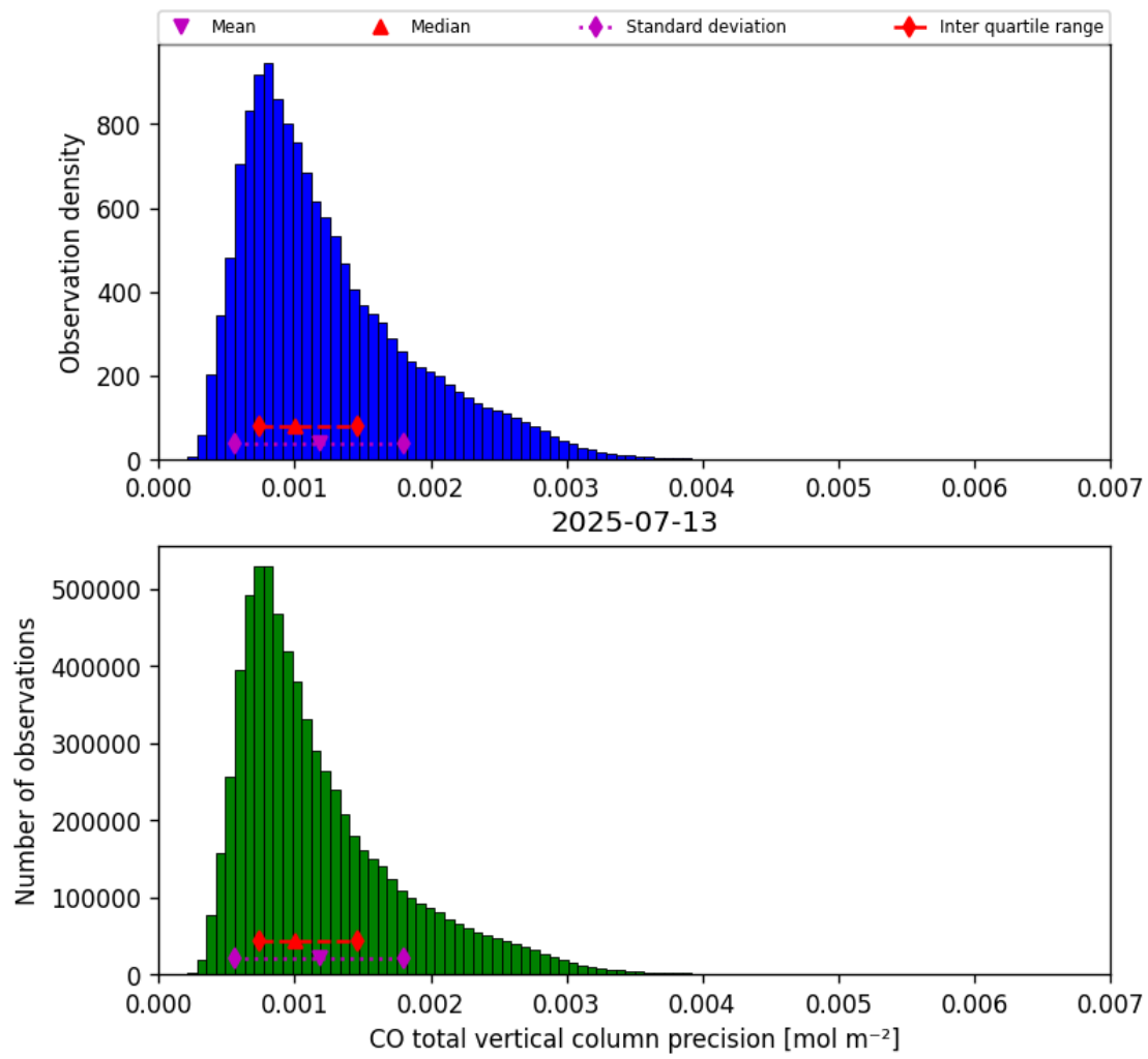
Figure 20: Histogram of “CO total vertical column precision” for 2025-07-13 to 2025-07-14
