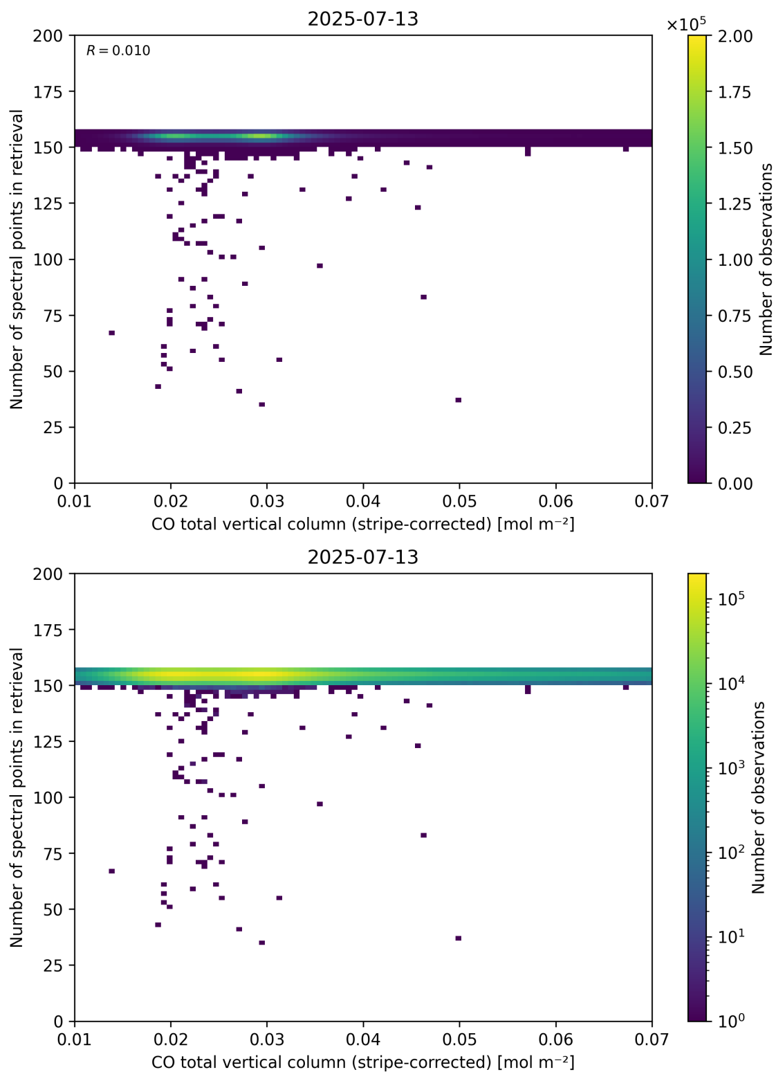
Figure 40: Scatter density plot of “CO total vertical column (stripe-corrected)” against “Number of spectral points in retrieval” for 2025-07-13 to 2025-07-14.
