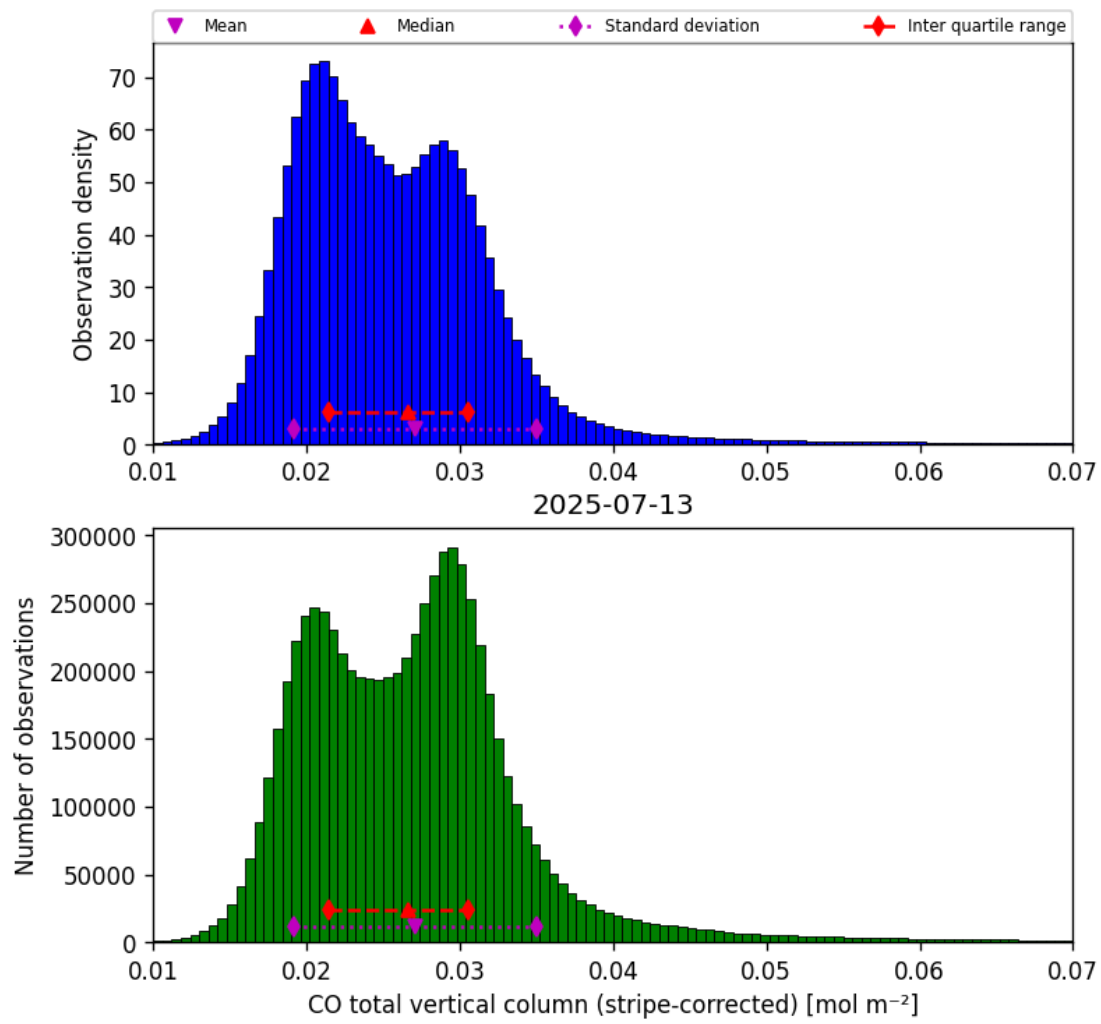
Figure 19: Histogram of “CO total vertical column (stripe-corrected)” for 2025-07-13 to 2025-07-14
