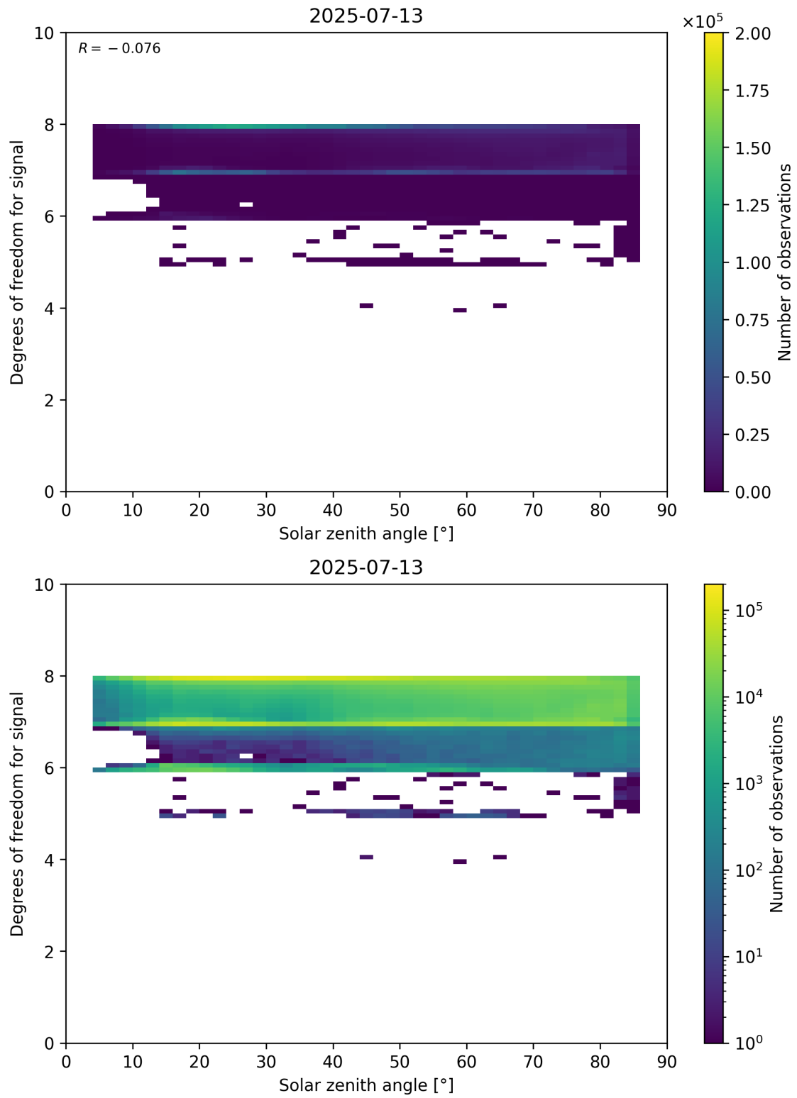
Figure 65: Scatter density plot of “Solar zenith angle” against “Degrees of freedom for signal” for 2025-07-13 to 2025-07-14.
