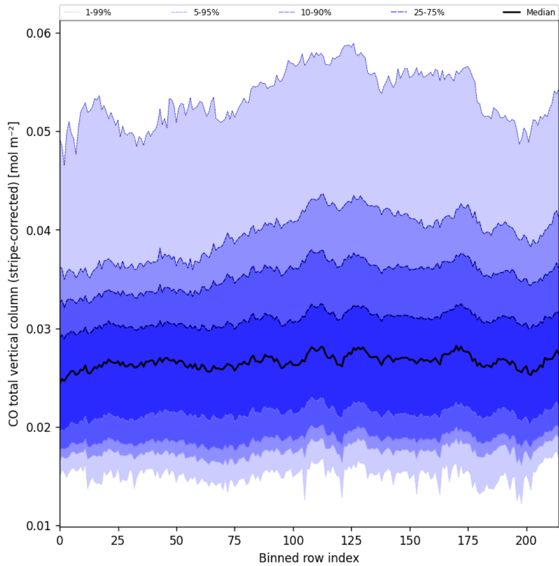
Figure 27: Along track statistics of “CO total vertical column (stripe-corrected)” for 2025-07-13 to 2025-07-15
