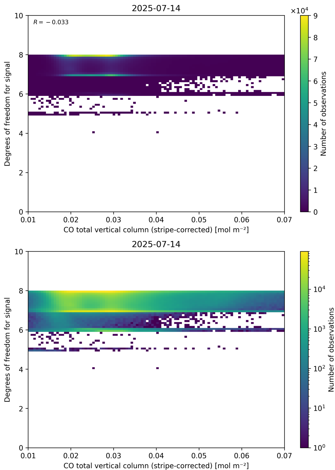
Figure 38: Scatter density plot of “CO total vertical column (stripe-corrected)” against “Degrees of freedom for signal” for 2025-07-13 to 2025-07-15.
