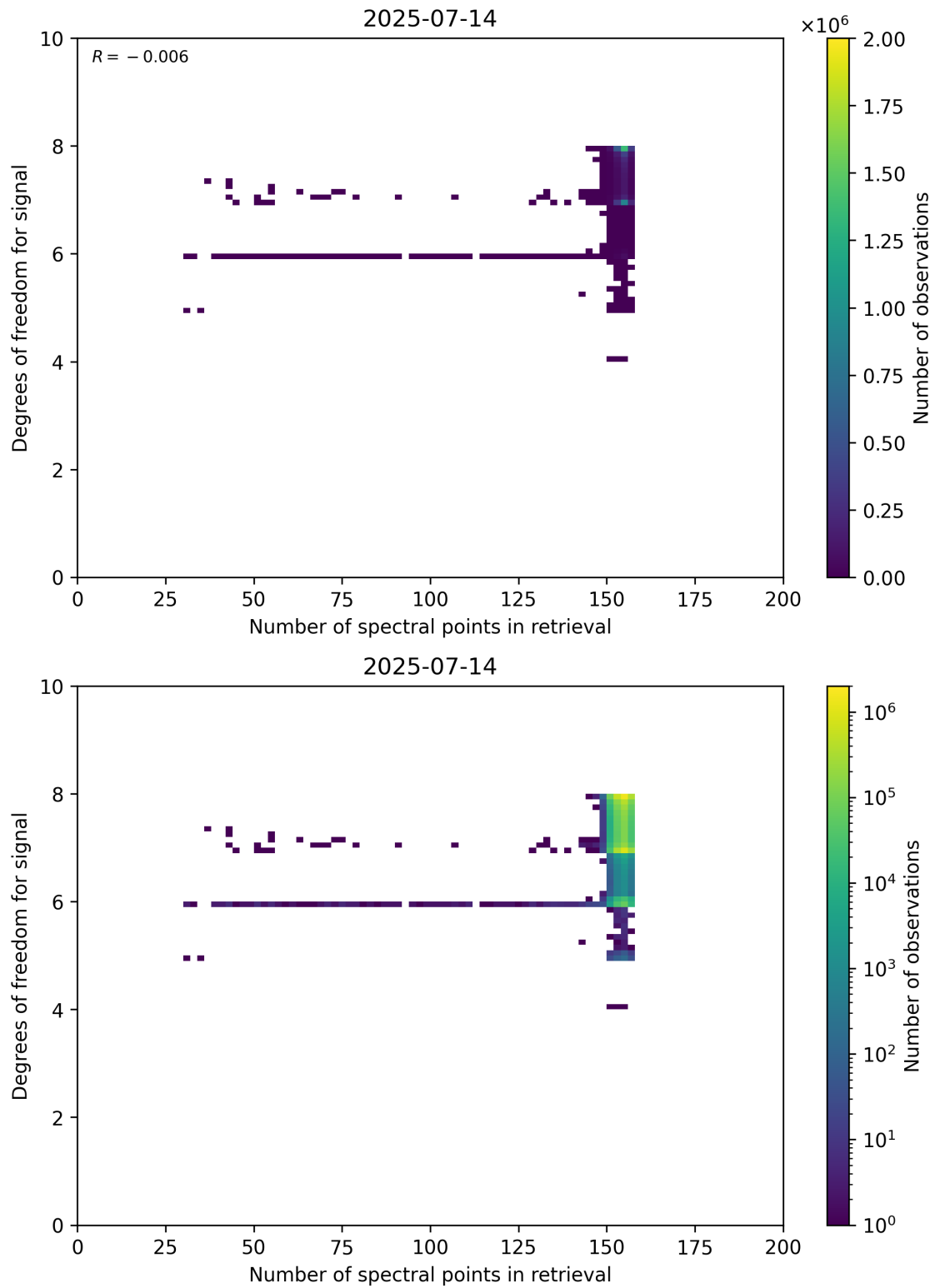
Figure 59: Scatter density plot of “Number of spectral points in retrieval” against “Degrees of freedom for signal” for 2025-07-13 to 2025-07-15.
