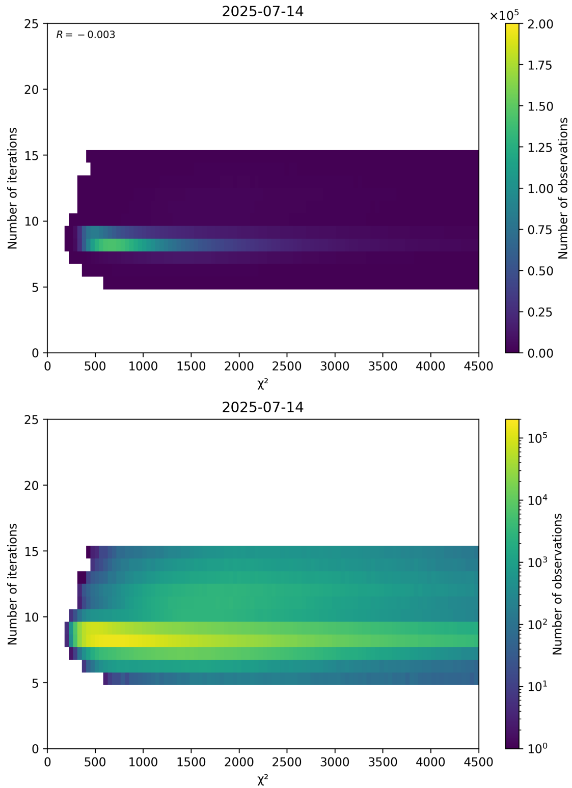
Figure 49: Scatter density plot of “ \chi^2 ” against “Number of iterations” for 2025-07-13 to 2025-07-15.
