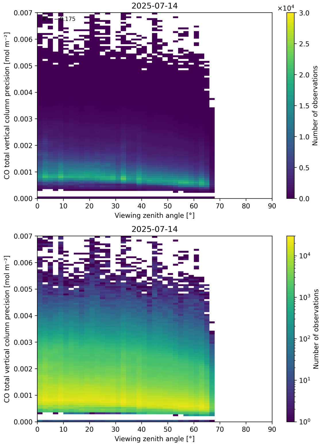
Figure 71: Scatter density plot of “Viewing zenith angle” against “CO total vertical column precision” for 2025-07-13 to 2025-07-15.
