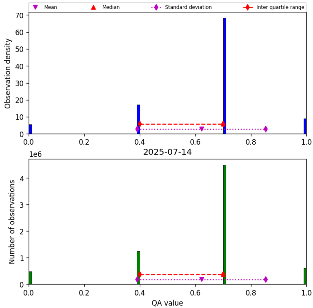
Figure 17: Histogram of “QA value” for 2025-07-13 to 2025-07-15
