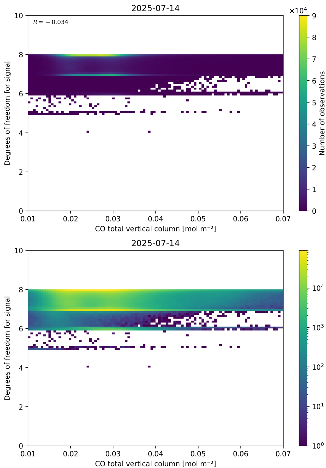
Figure 41: Scatter density plot of “CO total vertical column” against “Degrees of freedom for signal” for 2025-07-13 to 2025-07-15.
