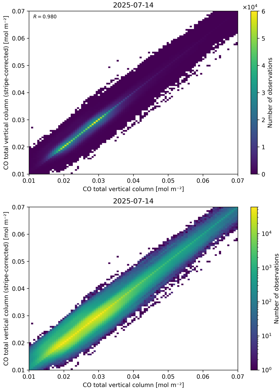
Figure 33: Scatter density plot of “CO total vertical column” against “CO total vertical column (stripe-corrected)” for 2025-07-13 to 2025-07-15.
