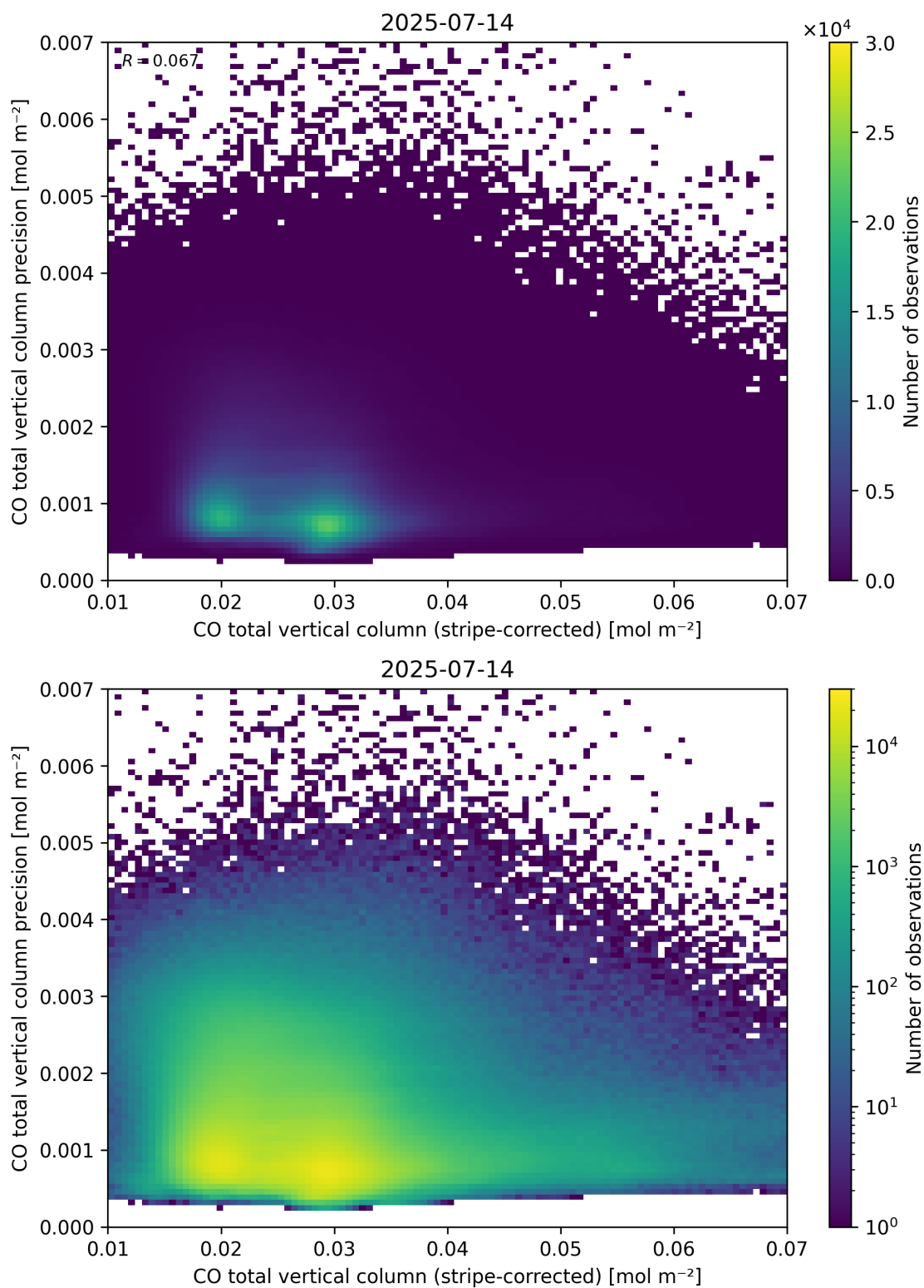
Figure 36: Scatter density plot of “CO total vertical column (stripe-corrected)” against “CO total vertical column precision” for 2025-07-13 to 2025-07-15.
