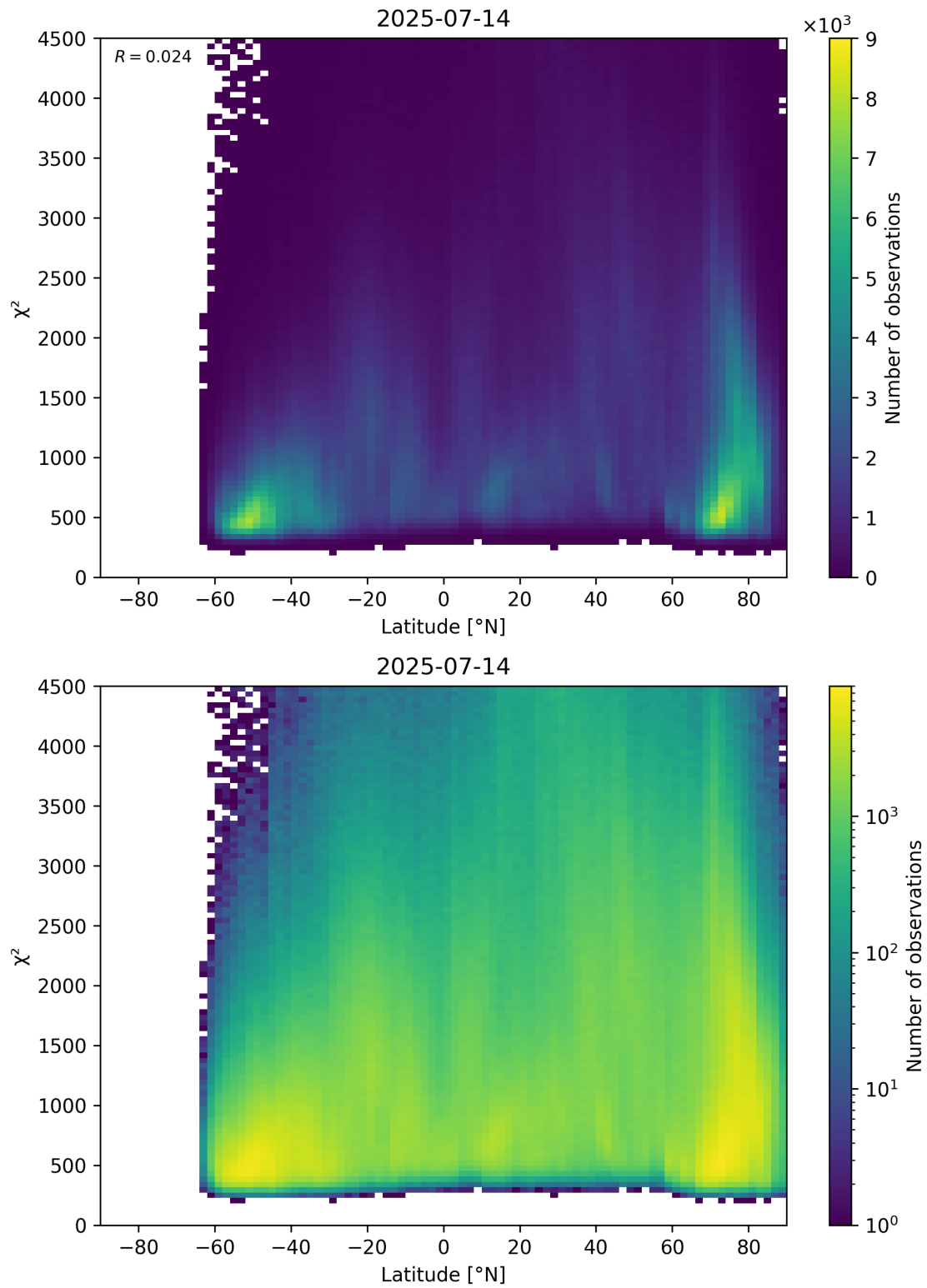
Figure 54: Scatter density plot of “Latitude” against “ \chi^2 ” for 2025-07-13 to 2025-07-15.
