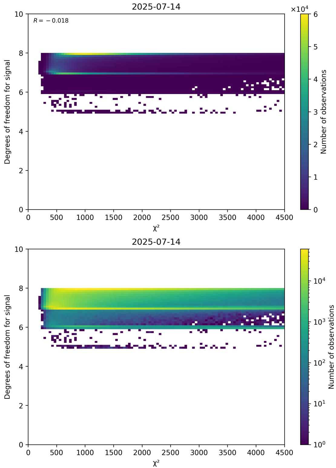
Figure 48: Scatter density plot of " \chi^2 " against "Degrees of freedom for signal" for 2025-07-13 to 2025-07-15.
