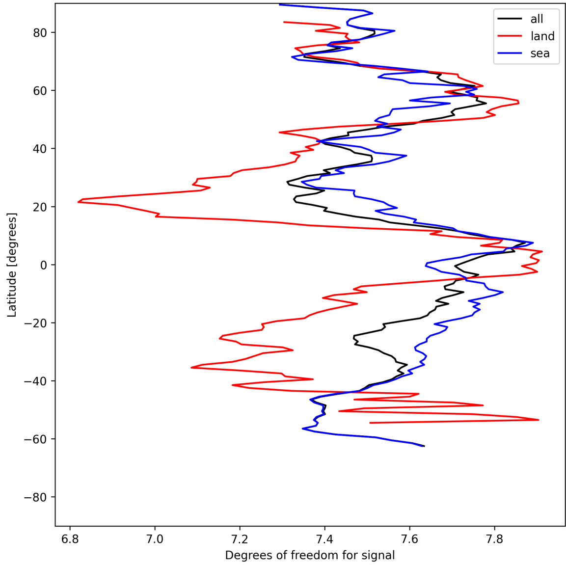
Figure 15: Zonal average of “Degrees of freedom for signal” for 2025-07-13 to 2025-07-15.
