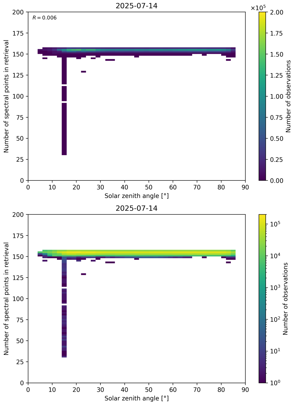
Figure 68: Scatter density plot of “Solar zenith angle” against “Number of spectral points in retrieval” for 2025-07-13 to 2025-07-15.
