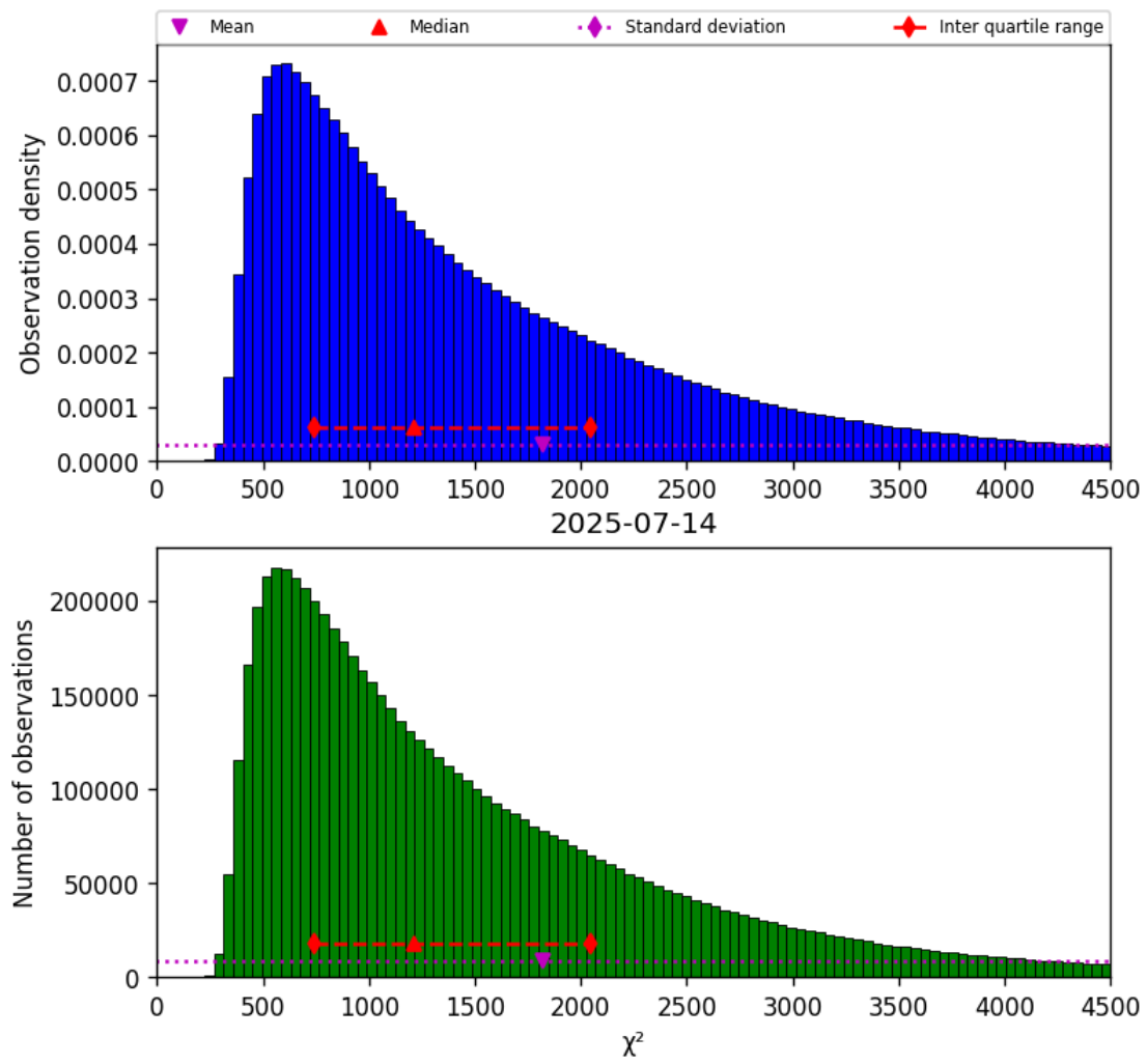
Figure 22: Histogram of “ \chi^2 ” for 2025-07-13 to 2025-07-15
