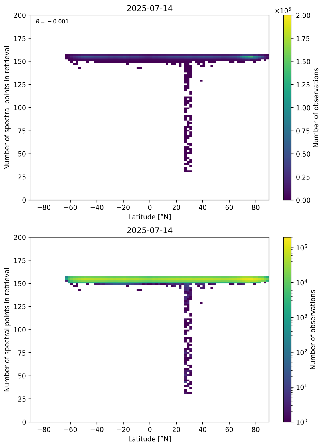
Figure 57: Scatter density plot of “Latitude” against “Number of spectral points in retrieval” for 2025-07-13 to 2025-07-15.
