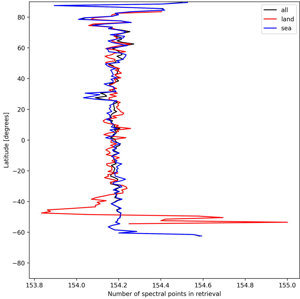
Figure 13: Zonal average of “Number of spectral points in retrieval” for 2025-07-13 to 2025-07-15.
