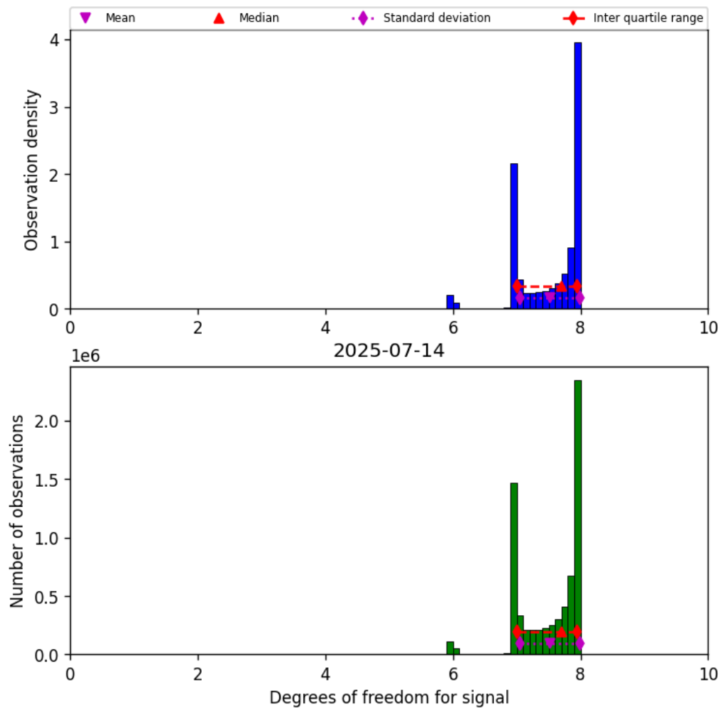
Figure 23: Histogram of “Degrees of freedom for signal” for 2025-07-13 to 2025-07-15
