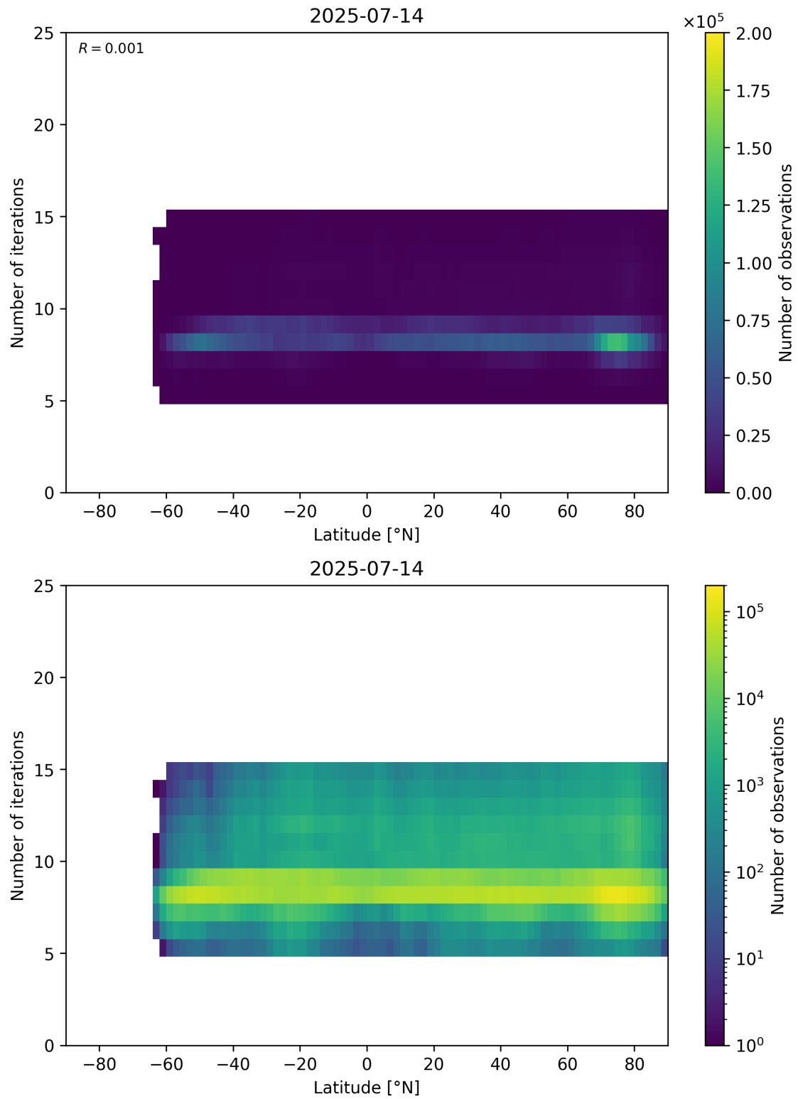
Figure 56: Scatter density plot of “Latitude” against “Number of iterations” for 2025-07-13 to 2025-07-15.
