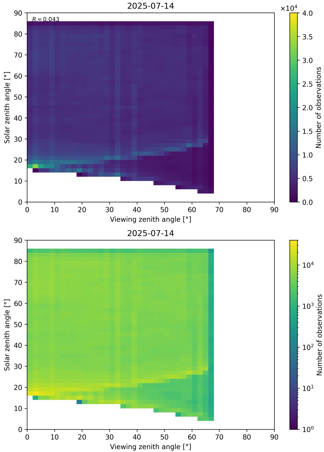
Figure 77: Scatter density plot of “Viewing zenith angle” against “Solar zenith angle” for 2025-07-13 to 2025-07-15.
