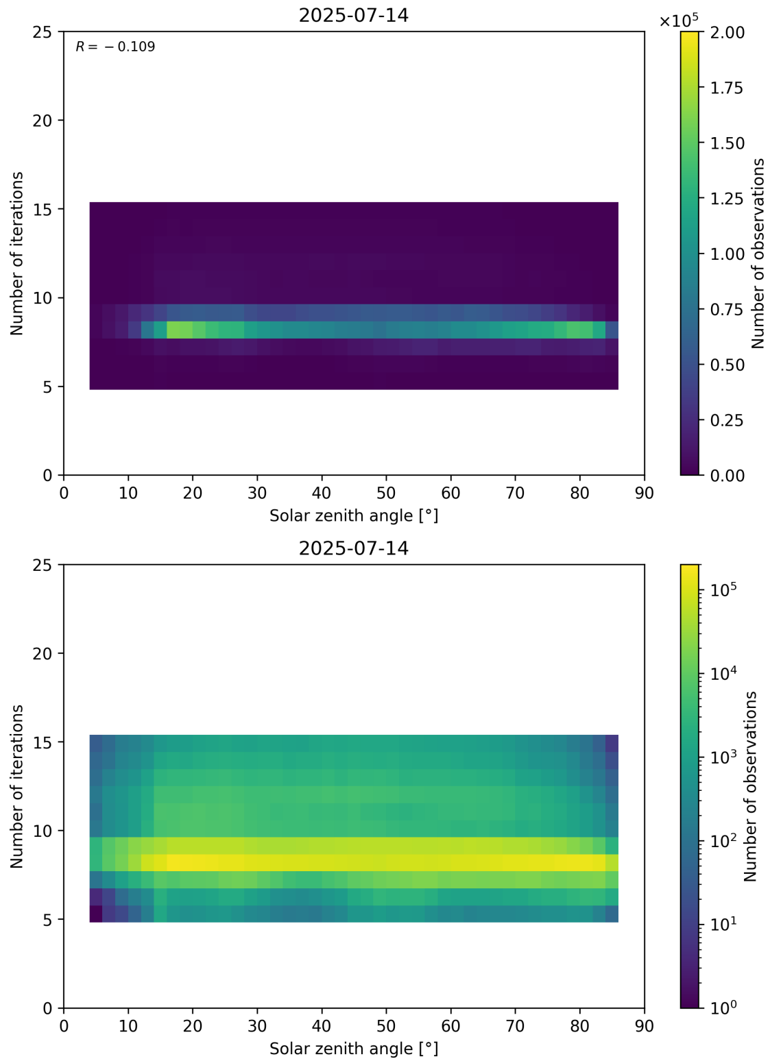
Figure 67: Scatter density plot of “Solar zenith angle” against “Number of iterations” for 2025-07-13 to 2025-07-15.
