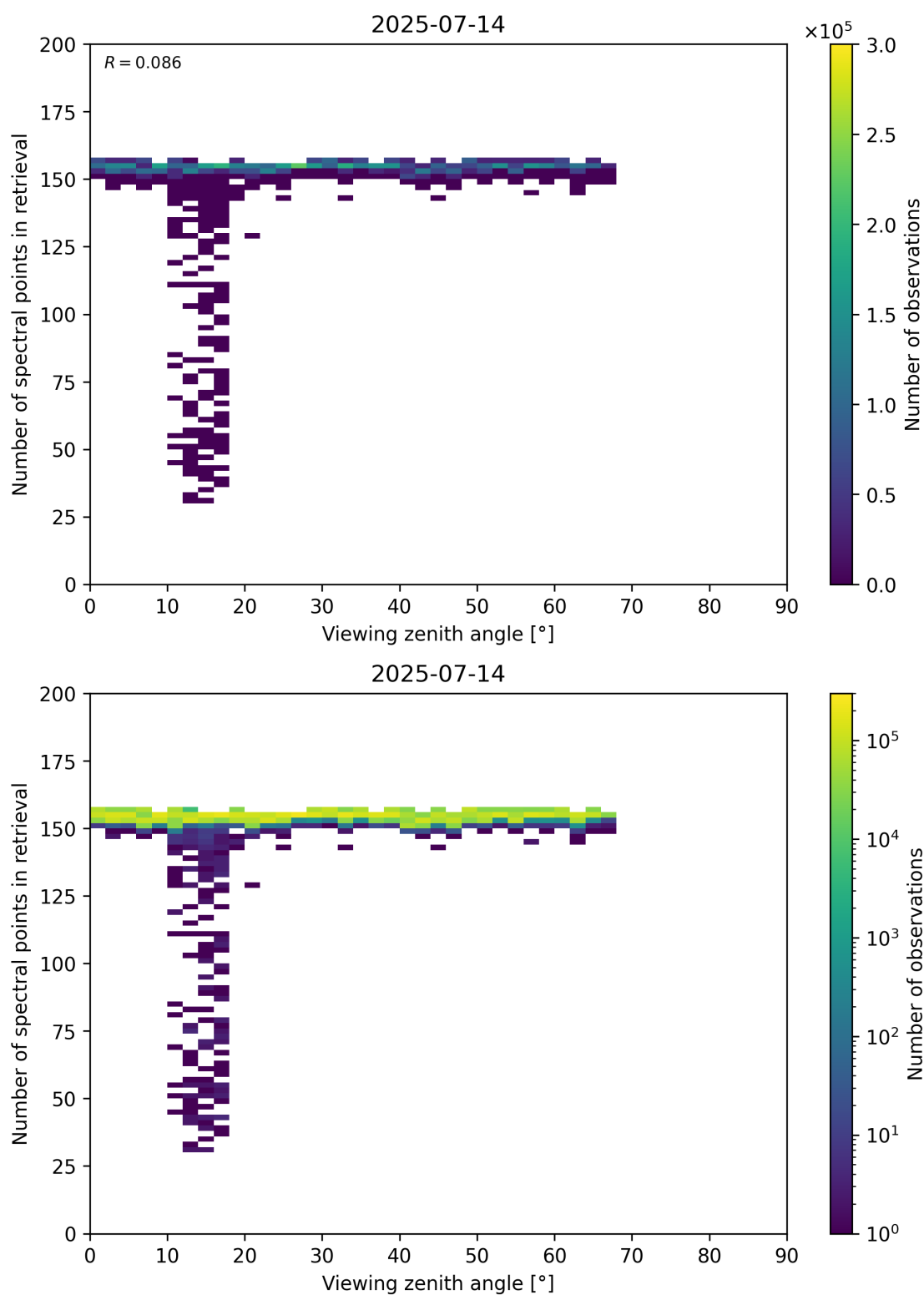
Figure 76: Scatter density plot of “Viewing zenith angle” against “Number of spectral points in retrieval” for 2025-07-13 to 2025-07-15.
