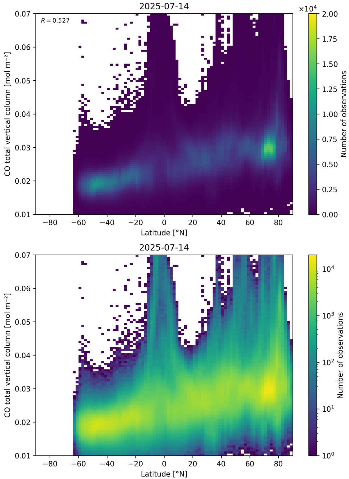
Figure 51: Scatter density plot of “Latitude” against “CO total vertical column” for 2025-07-13 to 2025-07-15.
