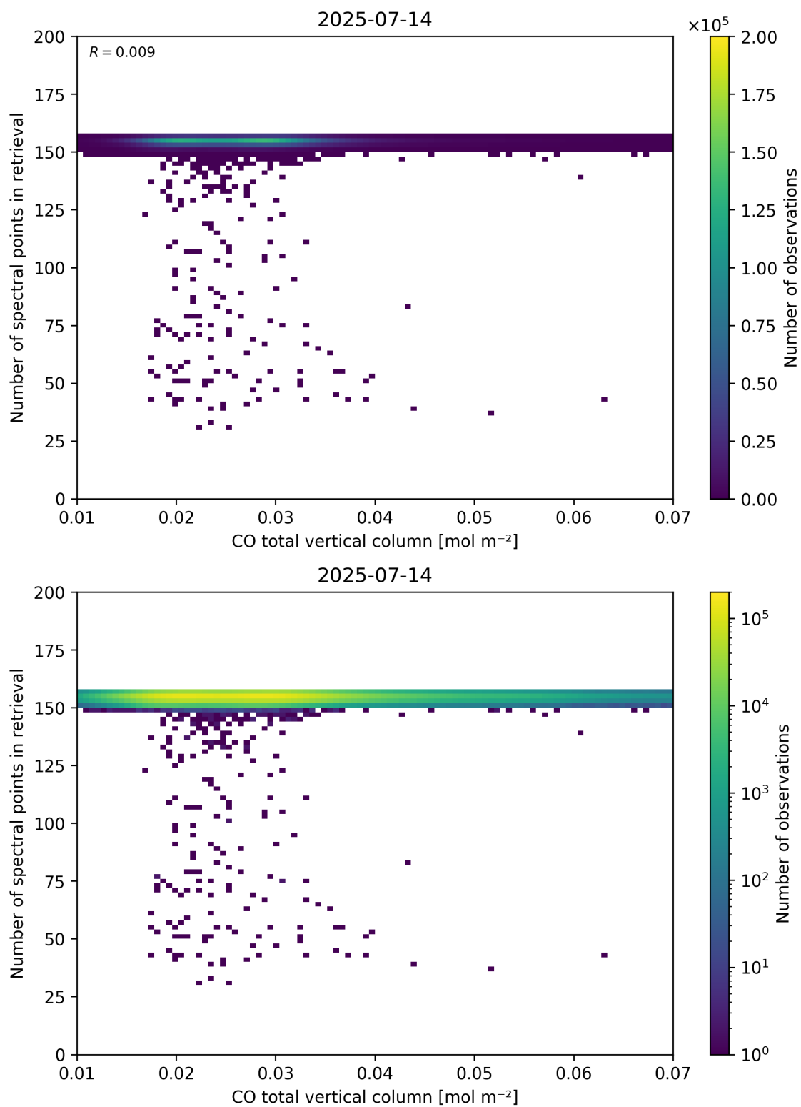
Figure 43: Scatter density plot of “CO total vertical column” against “Number of spectral points in retrieval” for 2025-07-13 to 2025-07-15.
