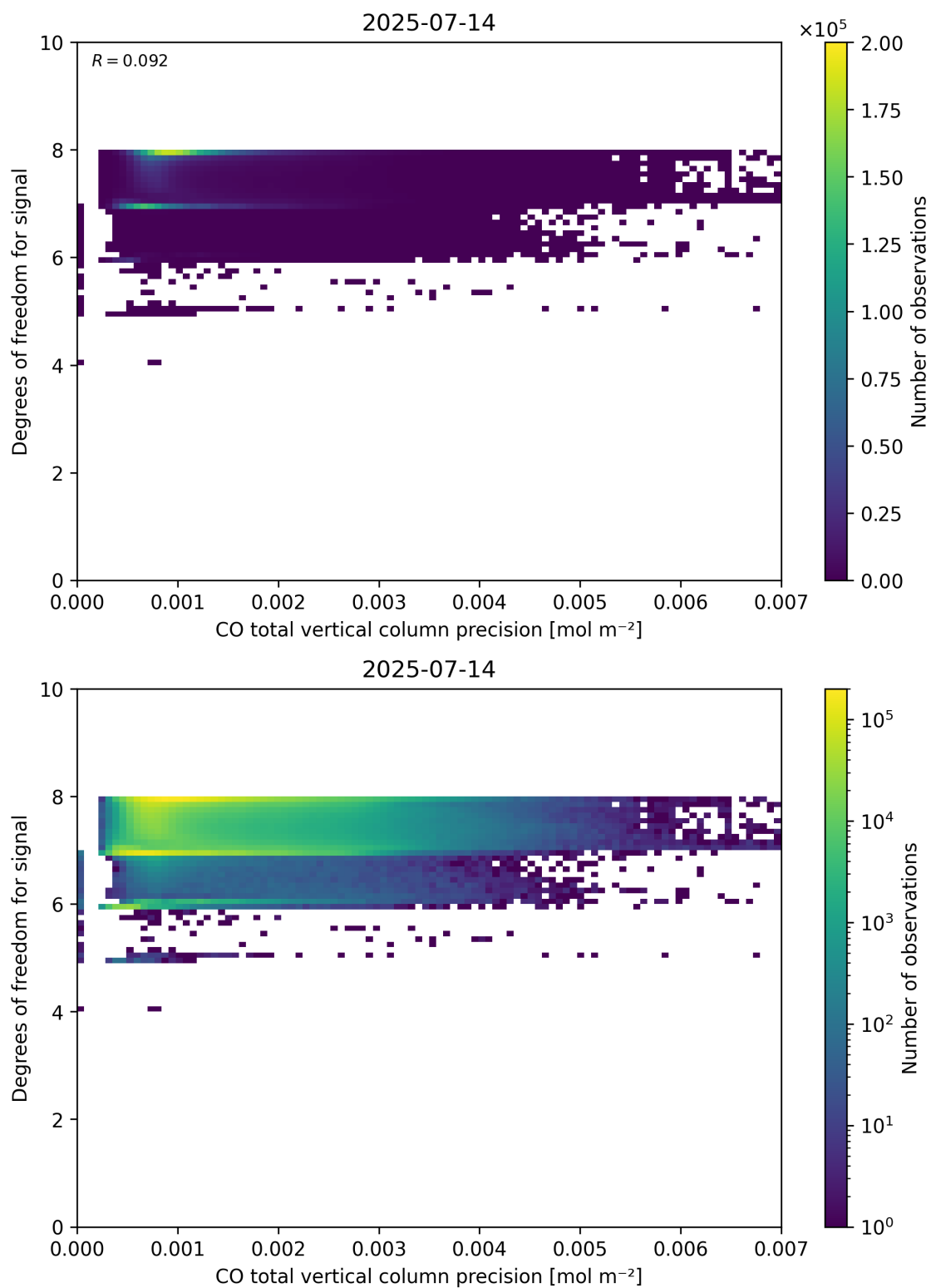
Figure 45: Scatter density plot of “CO total vertical column precision” against “Degrees of freedom for signal” for 2025-07-13 to 2025-07-15.
