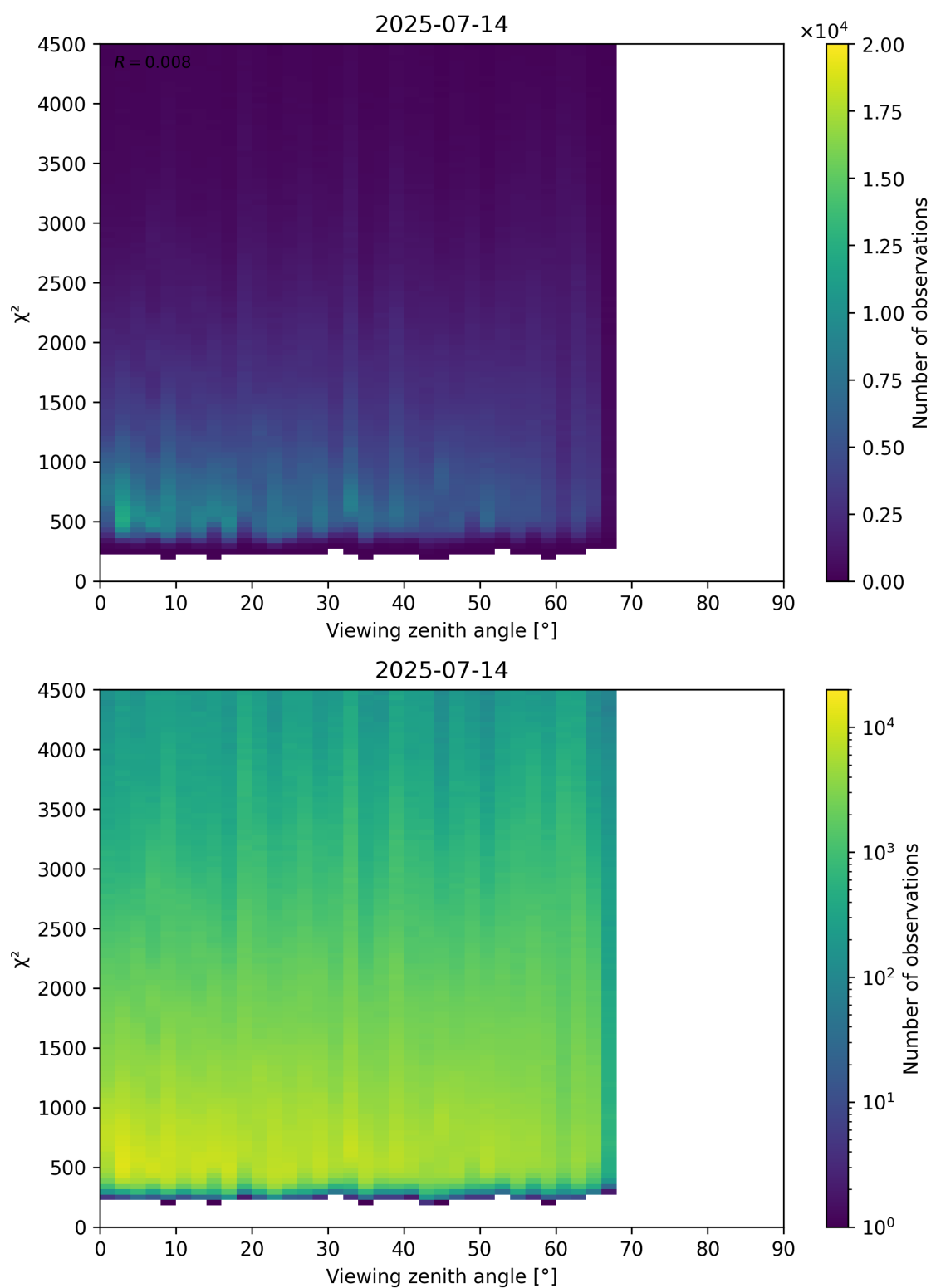
Figure 72: Scatter density plot of “Viewing zenith angle” against “ \chi^2 ” for 2025-07-13 to 2025-07-15.
