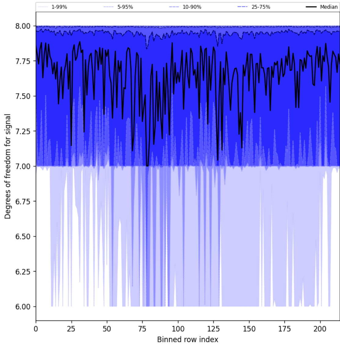
Figure 31: Along track statistics of “Degrees of freedom for signal” for 2025-07-13 to 2025-07-15
