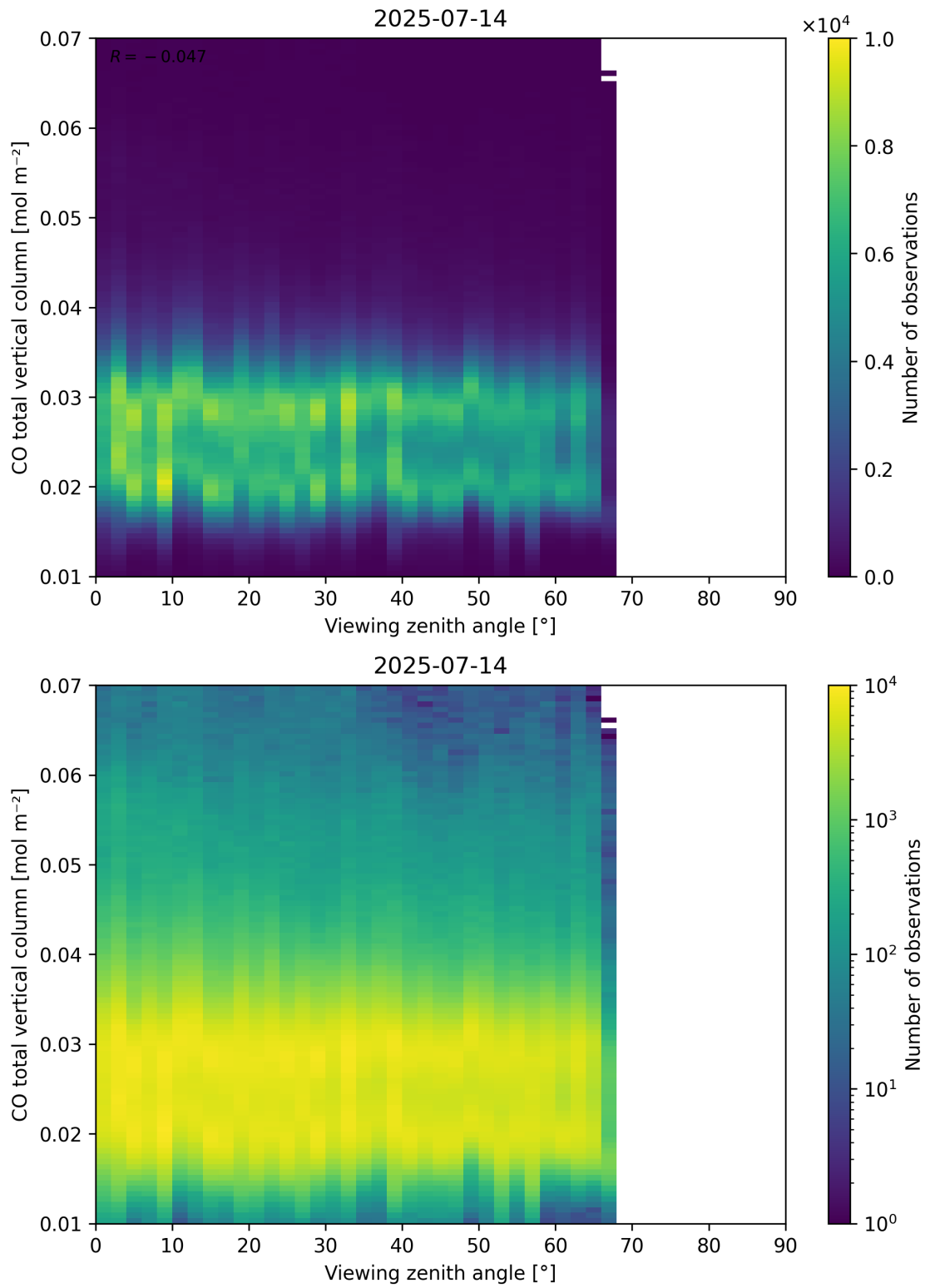
Figure 69: Scatter density plot of “Viewing zenith angle” against “CO total vertical column” for 2025-07-13 to 2025-07-15.
