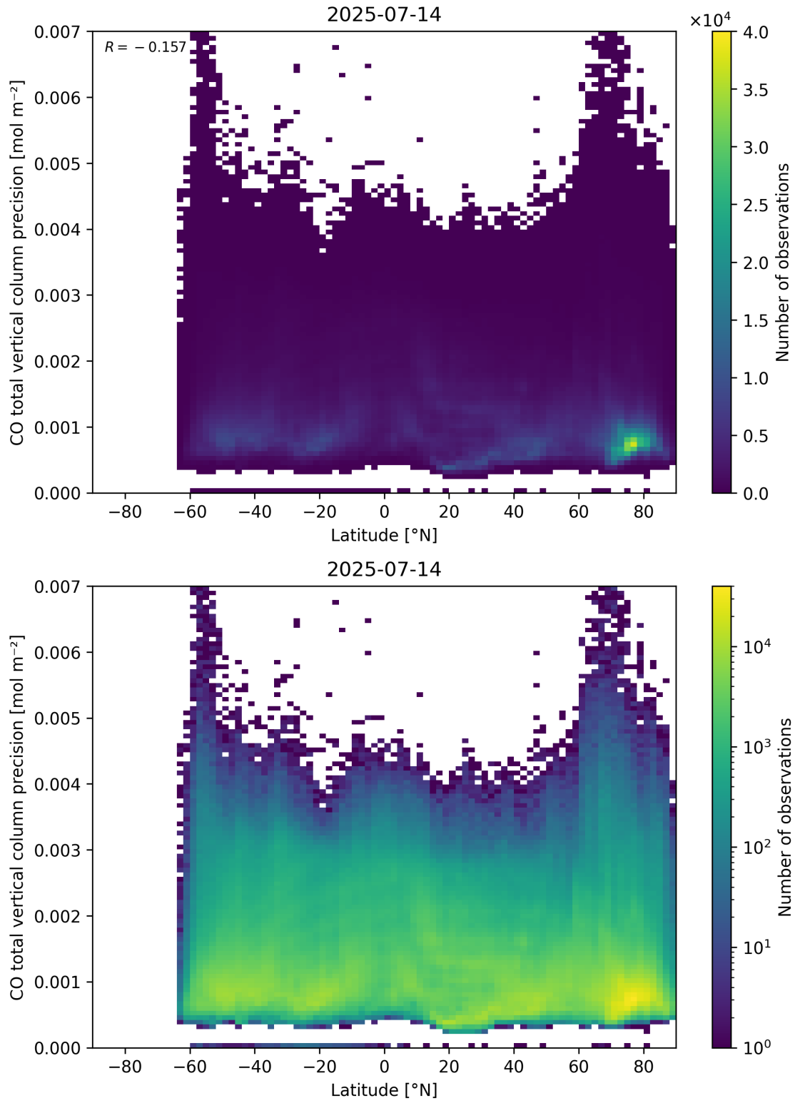
Figure 53: Scatter density plot of “Latitude” against “CO total vertical column precision” for 2025-07-13 to 2025-07-15.
