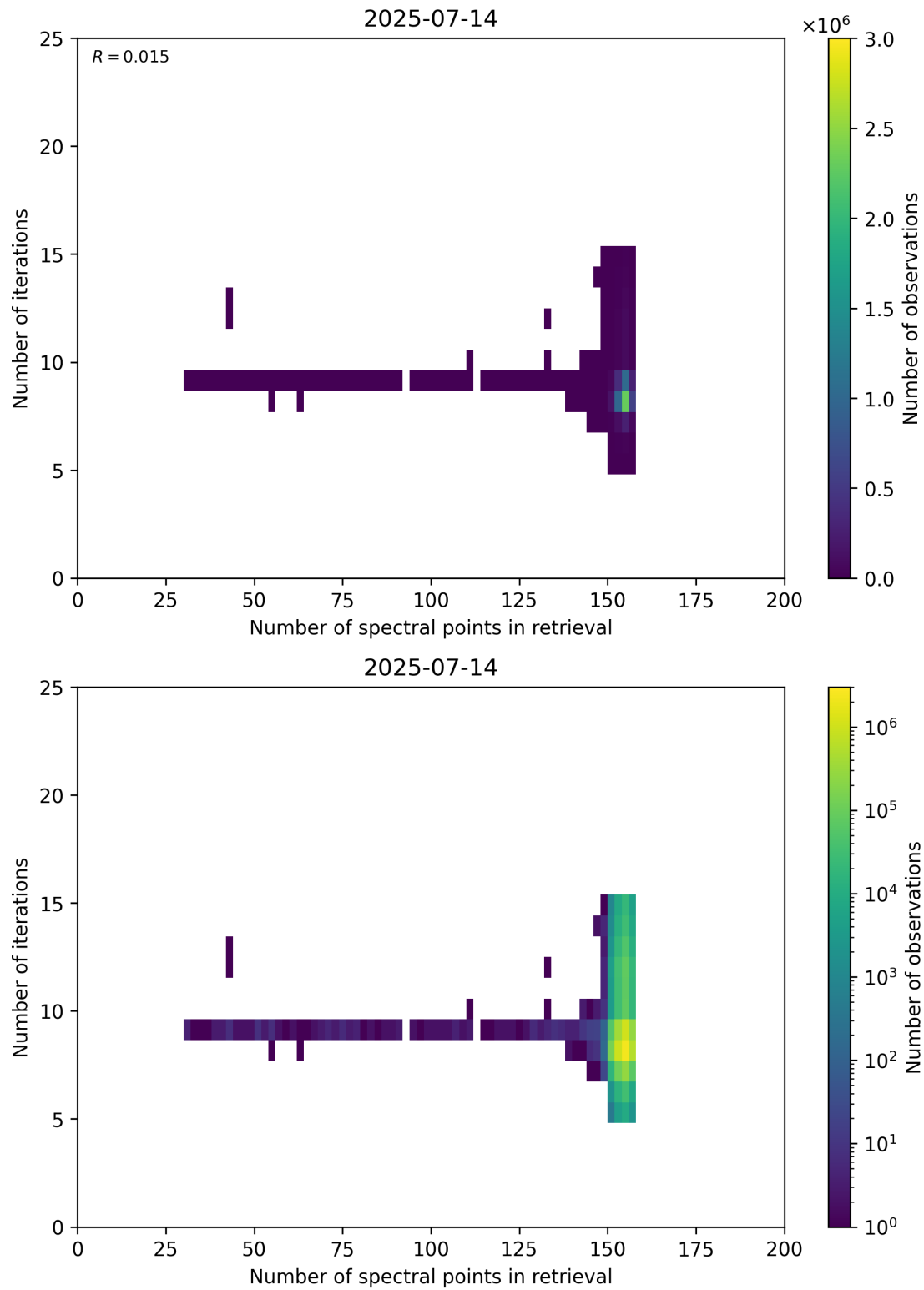
Figure 60: Scatter density plot of “Number of spectral points in retrieval” against “Number of iterations” for 2025-07-13 to 2025-07-15.
