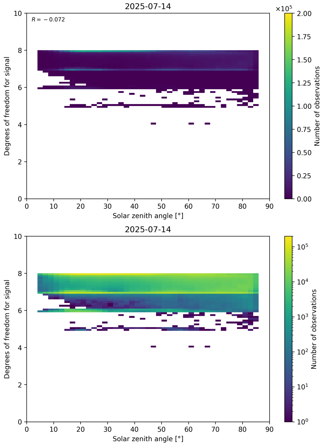
Figure 65: Scatter density plot of “Solar zenith angle” against “Degrees of freedom for signal” for 2025-07-13 to 2025-07-15.
