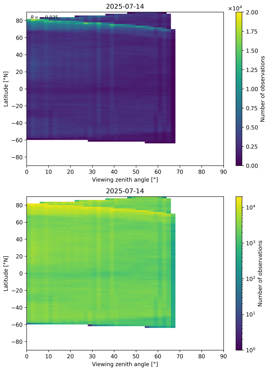
Figure 74: Scatter density plot of “Viewing zenith angle” against “Latitude” for 2025-07-13 to 2025-07-15.
