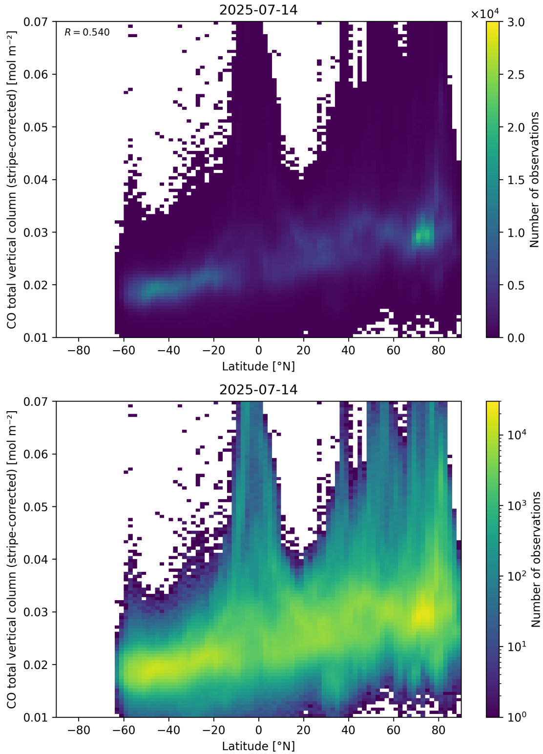
Figure 52: Scatter density plot of “Latitude” against “CO total vertical column (stripe-corrected)” for 2025-07-13 to 2025-07-15.
