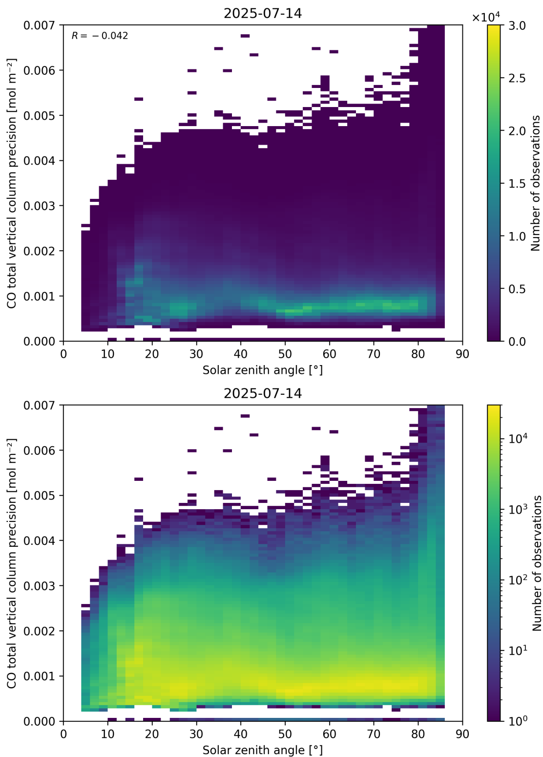
Figure 63: Scatter density plot of “Solar zenith angle” against “CO total vertical column precision” for 2025-07-13 to 2025-07-15.
