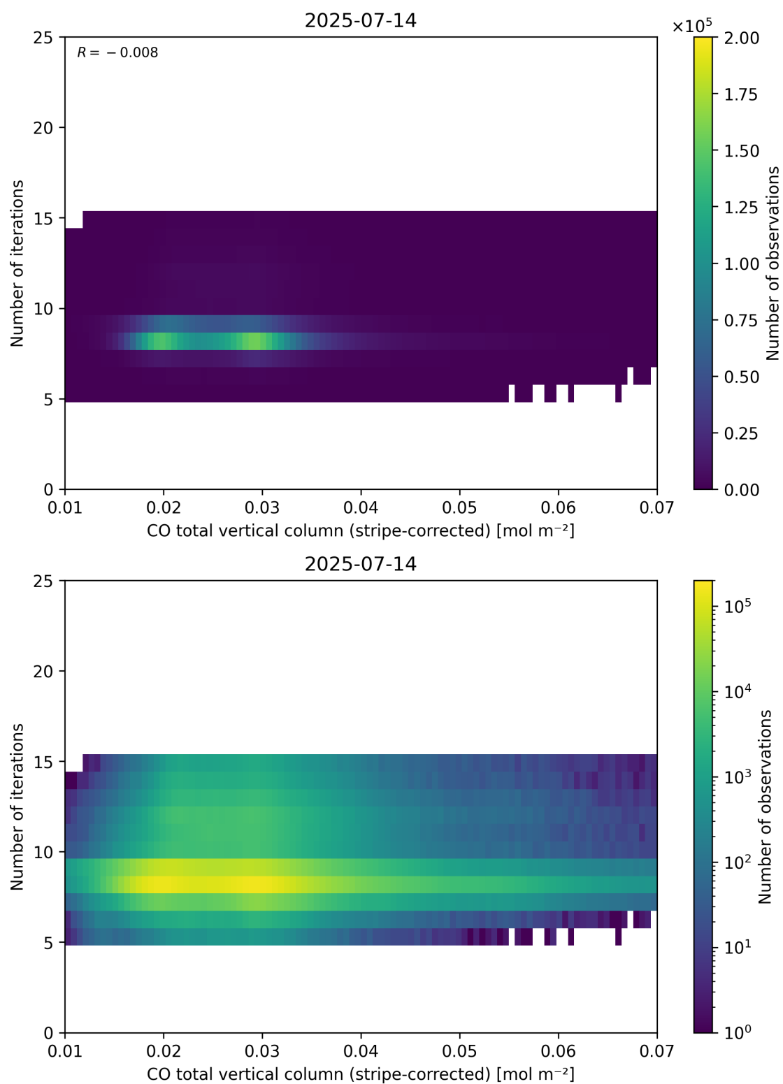
Figure 39: Scatter density plot of “CO total vertical column (stripe-corrected)” against “Number of iterations” for 2025-07-13 to 2025-07-15.
