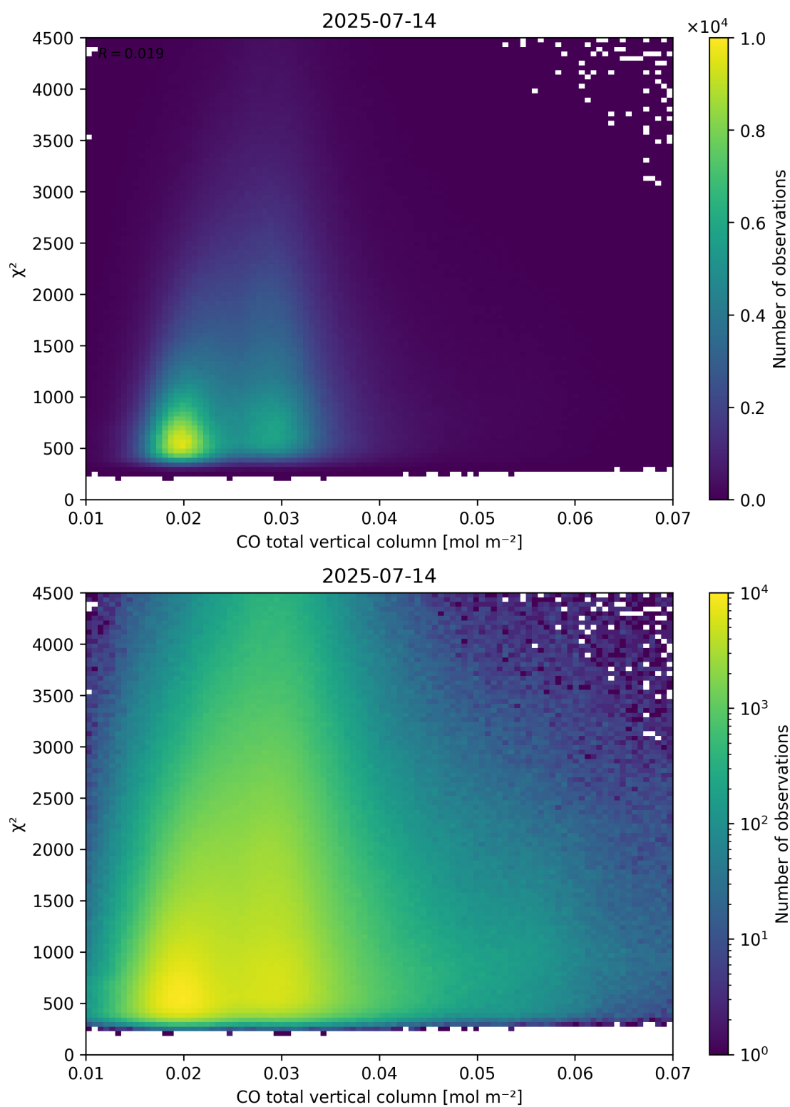
Figure 35: Scatter density plot of “CO total vertical column” against “ \chi^2 ” for 2025-07-13 to 2025-07-15.
