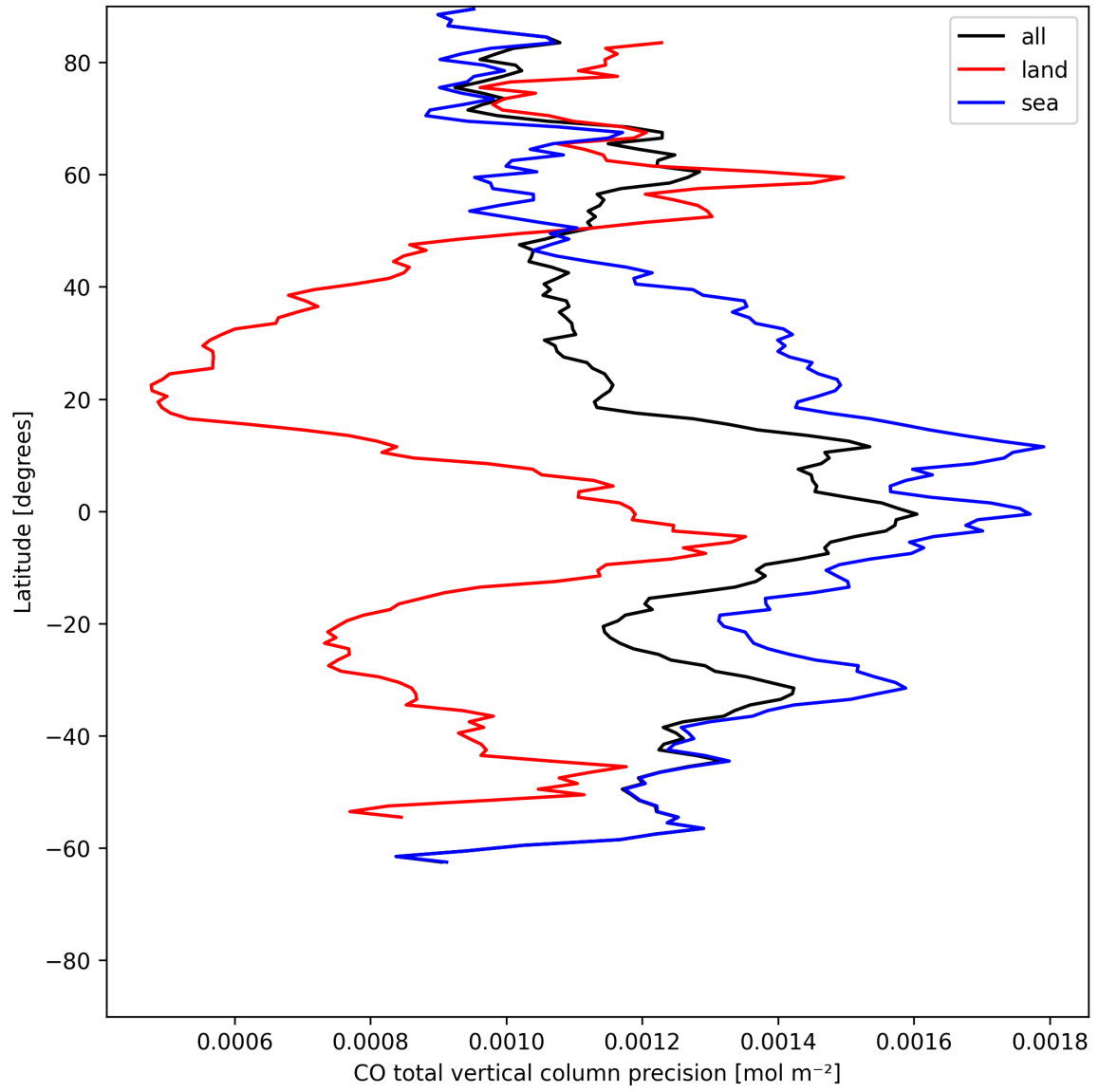
Figure 12: Zonal average of “CO total vertical column precision” for 2025-07-13 to 2025-07-15.
