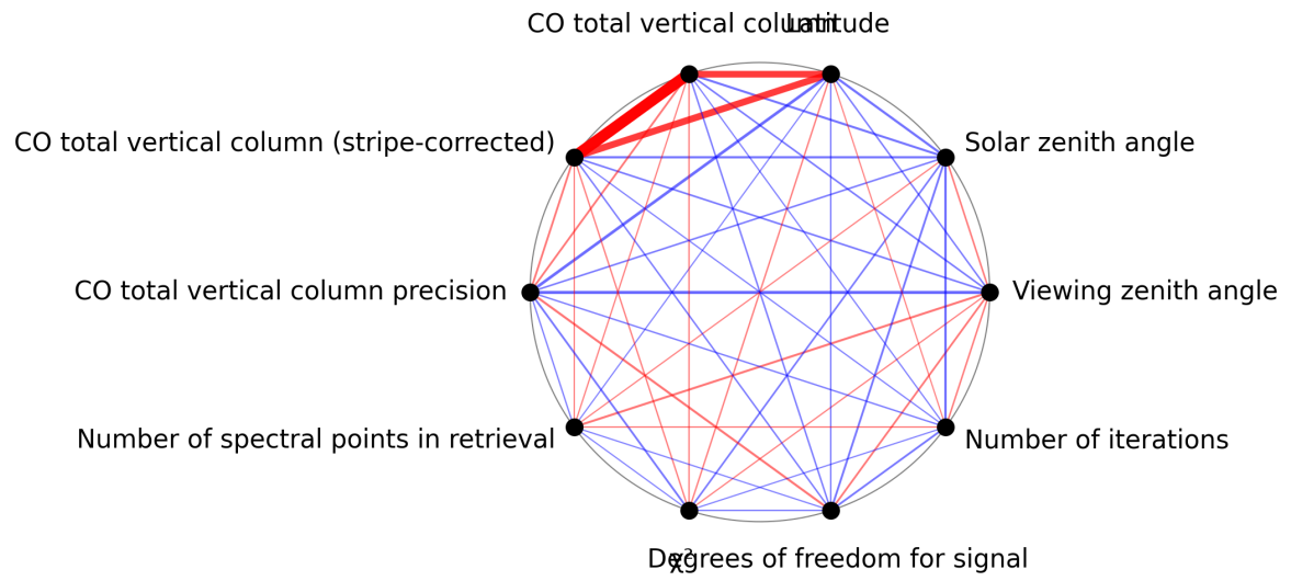
Figure 1: Map of correlation graph for 2025-07-13 to 2025-07-15.
