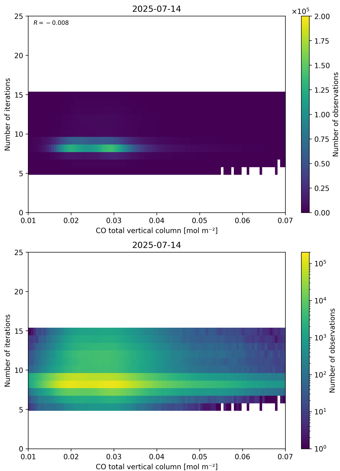
Figure 42: Scatter density plot of “CO total vertical column” against “Number of iterations” for 2025-07-13 to 2025-07-15.
