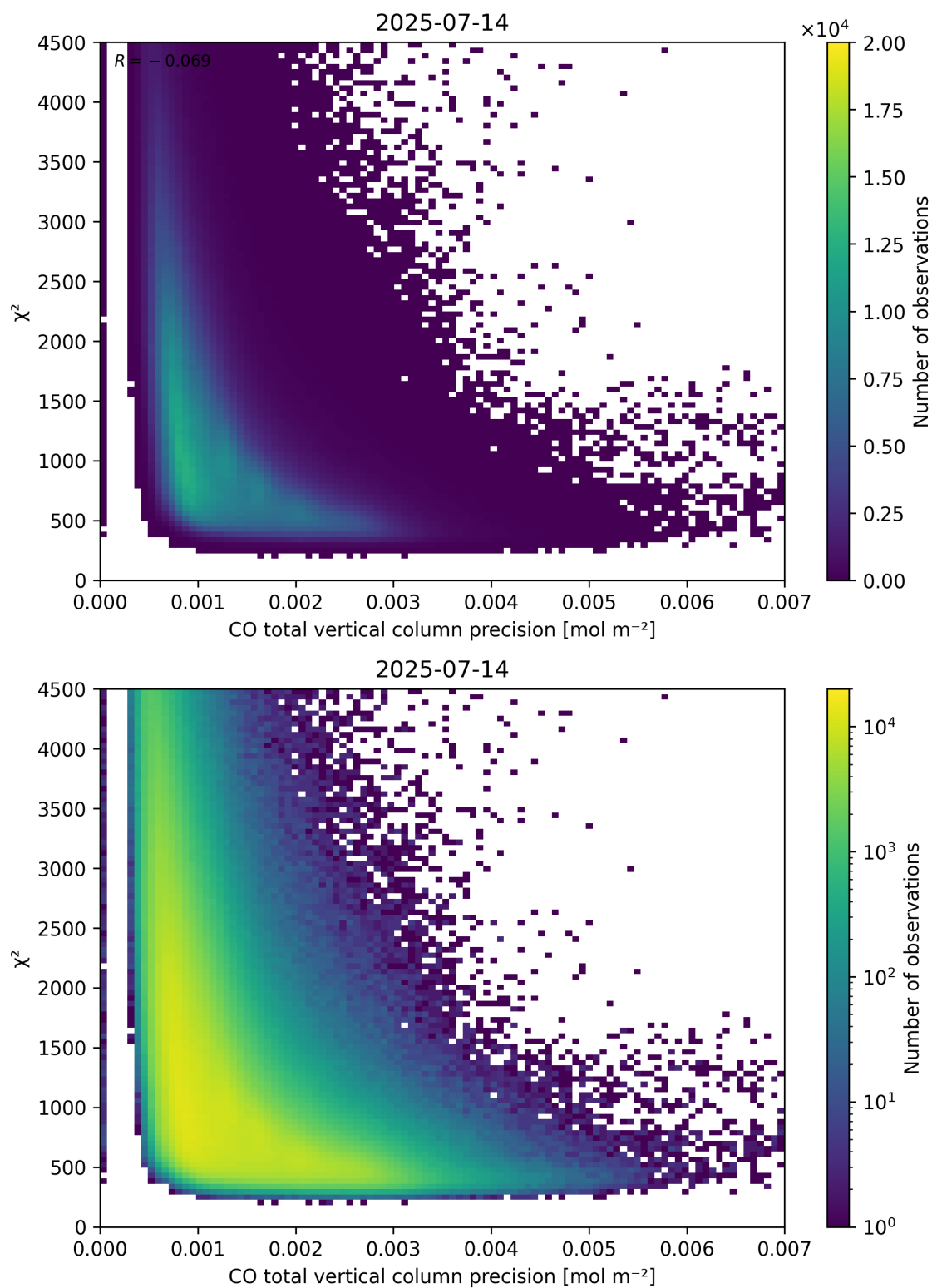
Figure 44: Scatter density plot of “CO total vertical column precision” against “ \chi^2 ” for 2025-07-13 to 2025-07-15.
