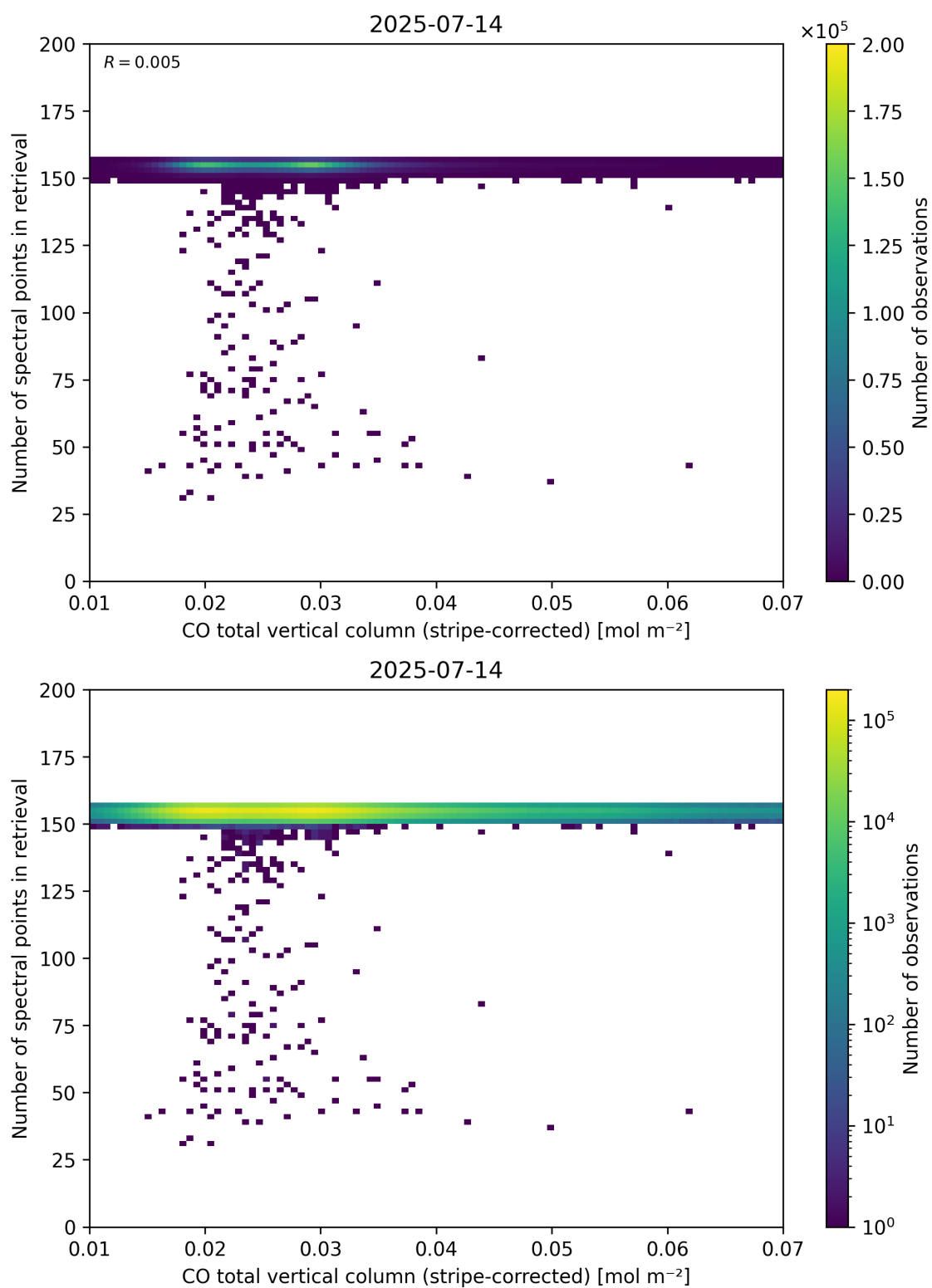
Figure 40: Scatter density plot of “CO total vertical column (stripe-corrected)” against “Number of spectral points in retrieval” for 2025-07-13 to 2025-07-15.
