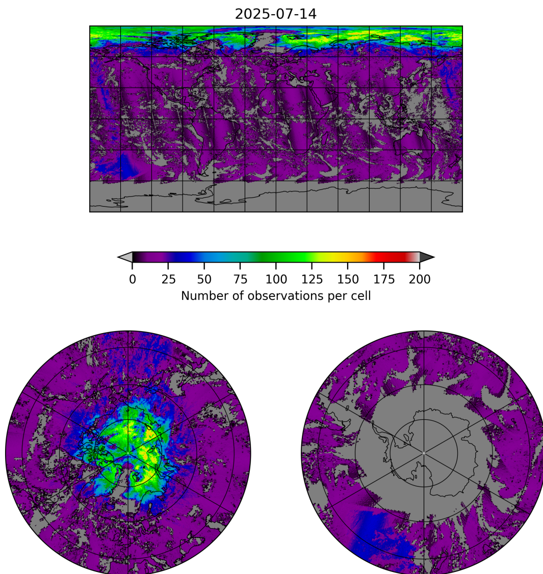
Figure 8: Map of the number of observations for 2025-07-13 to 2025-07-15
