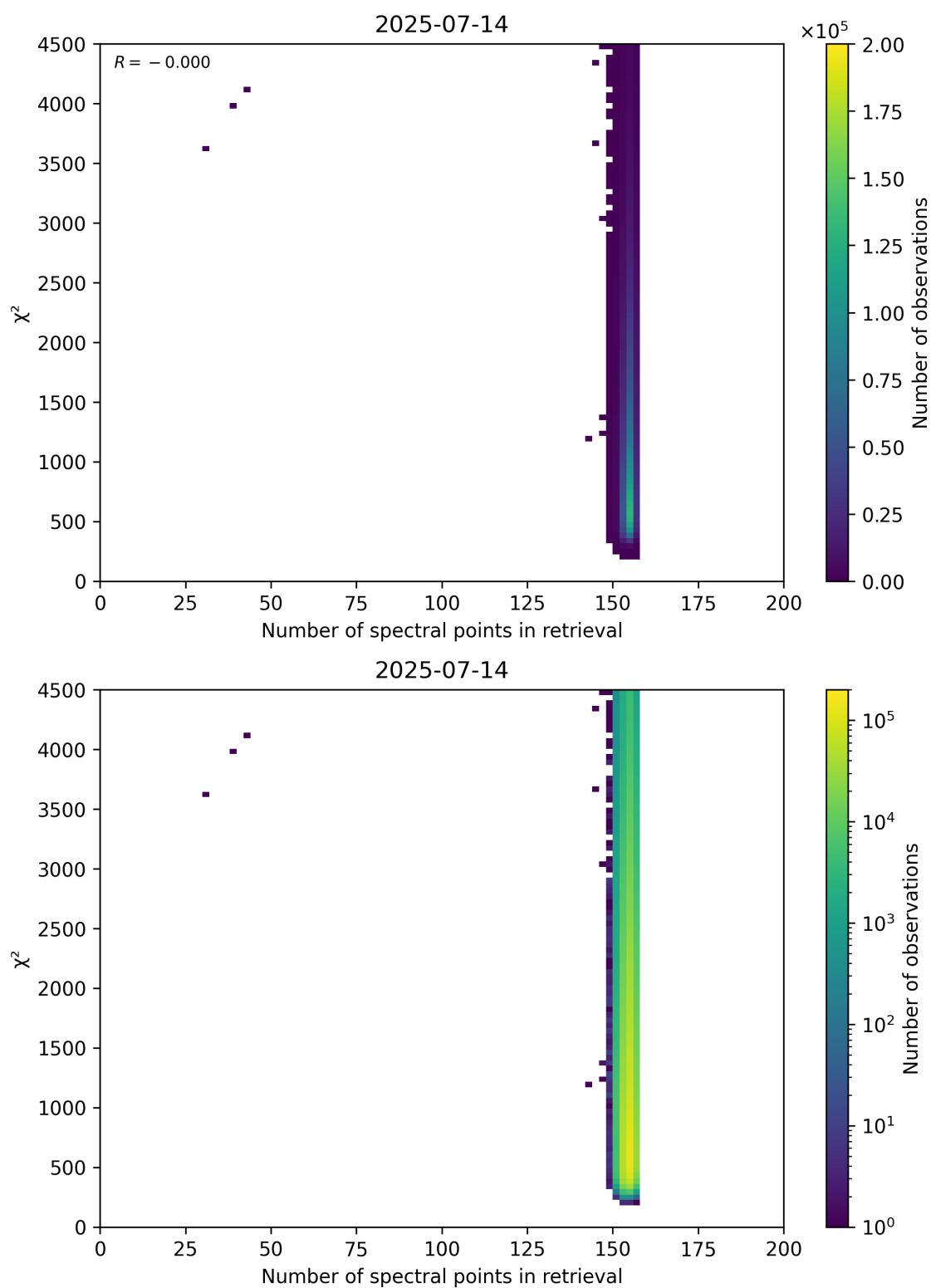
Figure 58: Scatter density plot of “Number of spectral points in retrieval” against “ \chi^2 ” for 2025-07-13 to 2025-07-15.
