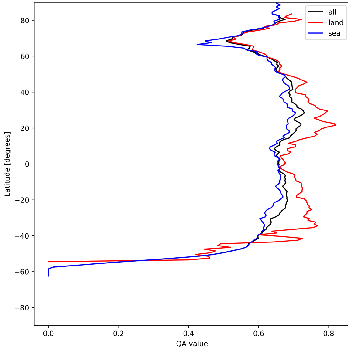
Figure 9: Zonal average of “QA value” for 2025-07-13 to 2025-07-15.
