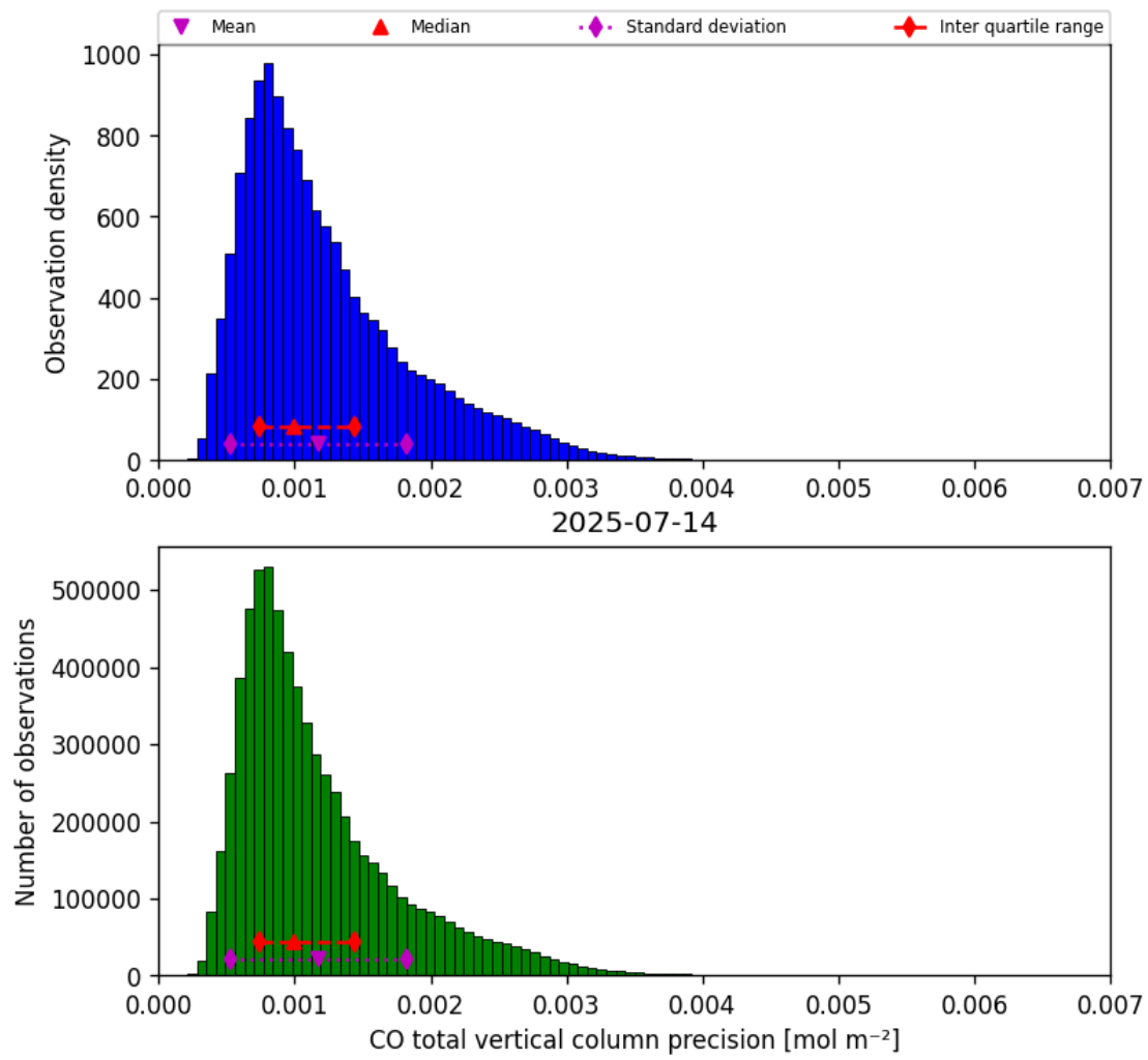
Figure 20: Histogram of “CO total vertical column precision” for 2025-07-13 to 2025-07-15
