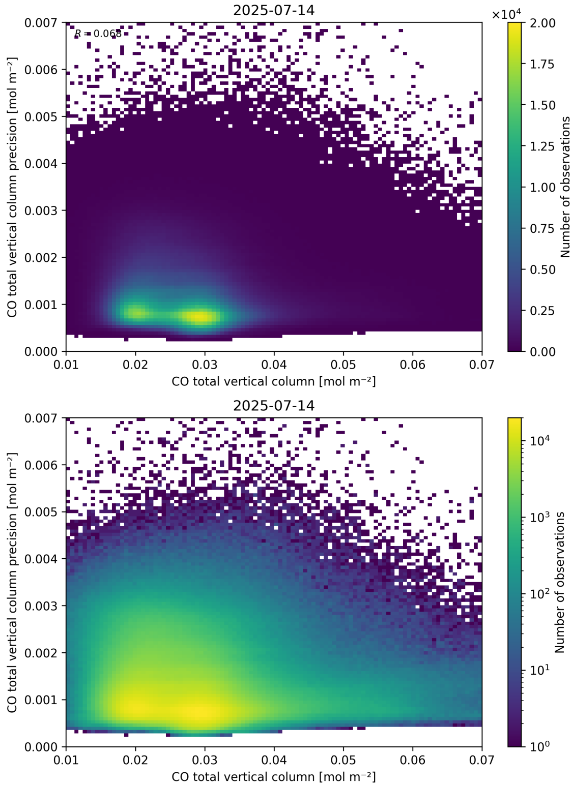
Figure 34: Scatter density plot of “CO total vertical column” against “CO total vertical column precision” for 2025-07-13 to 2025-07-15.
