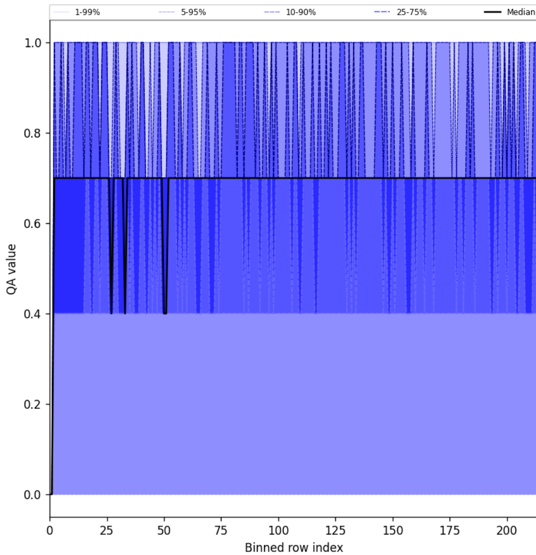
Figure 25: Along track statistics of “QA value” for 2025-07-13 to 2025-07-15
