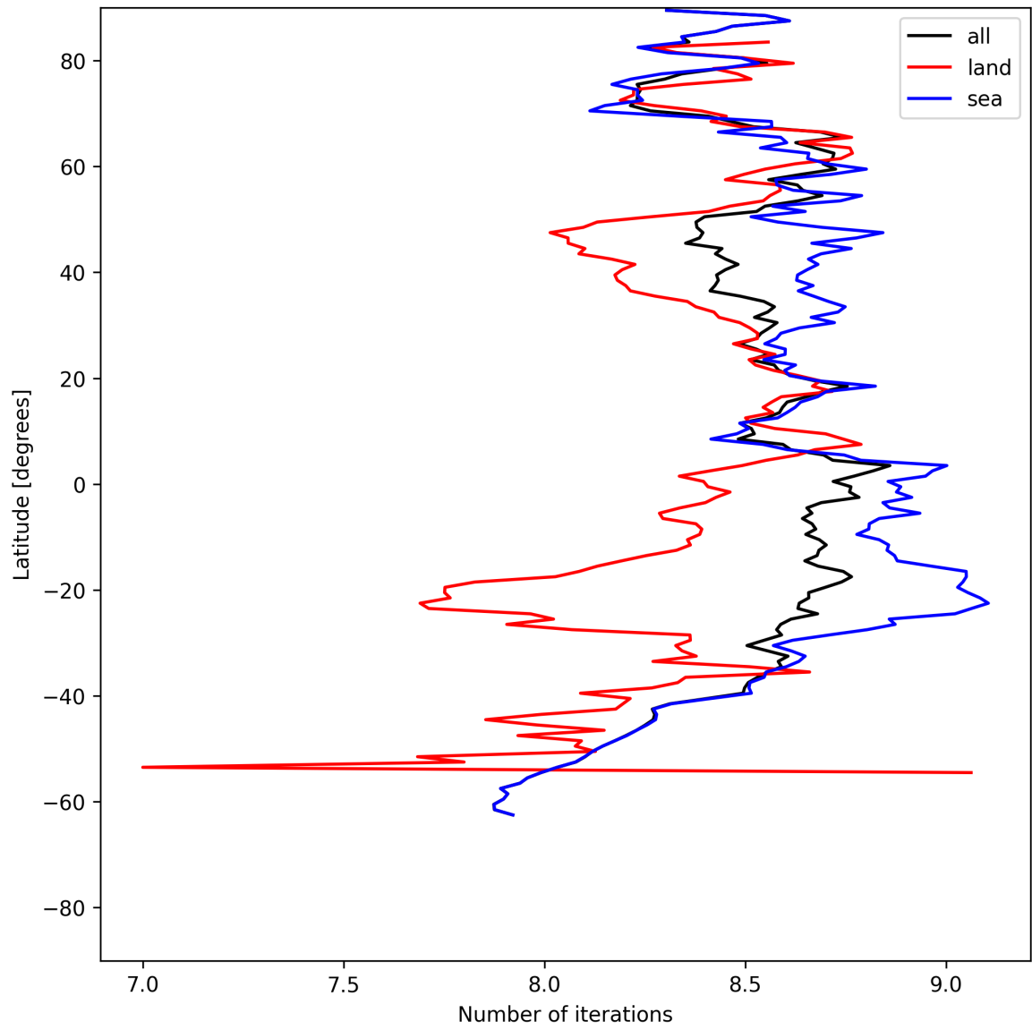
Figure 16: Zonal average of “Number of iterations” for 2025-07-13 to 2025-07-15.
