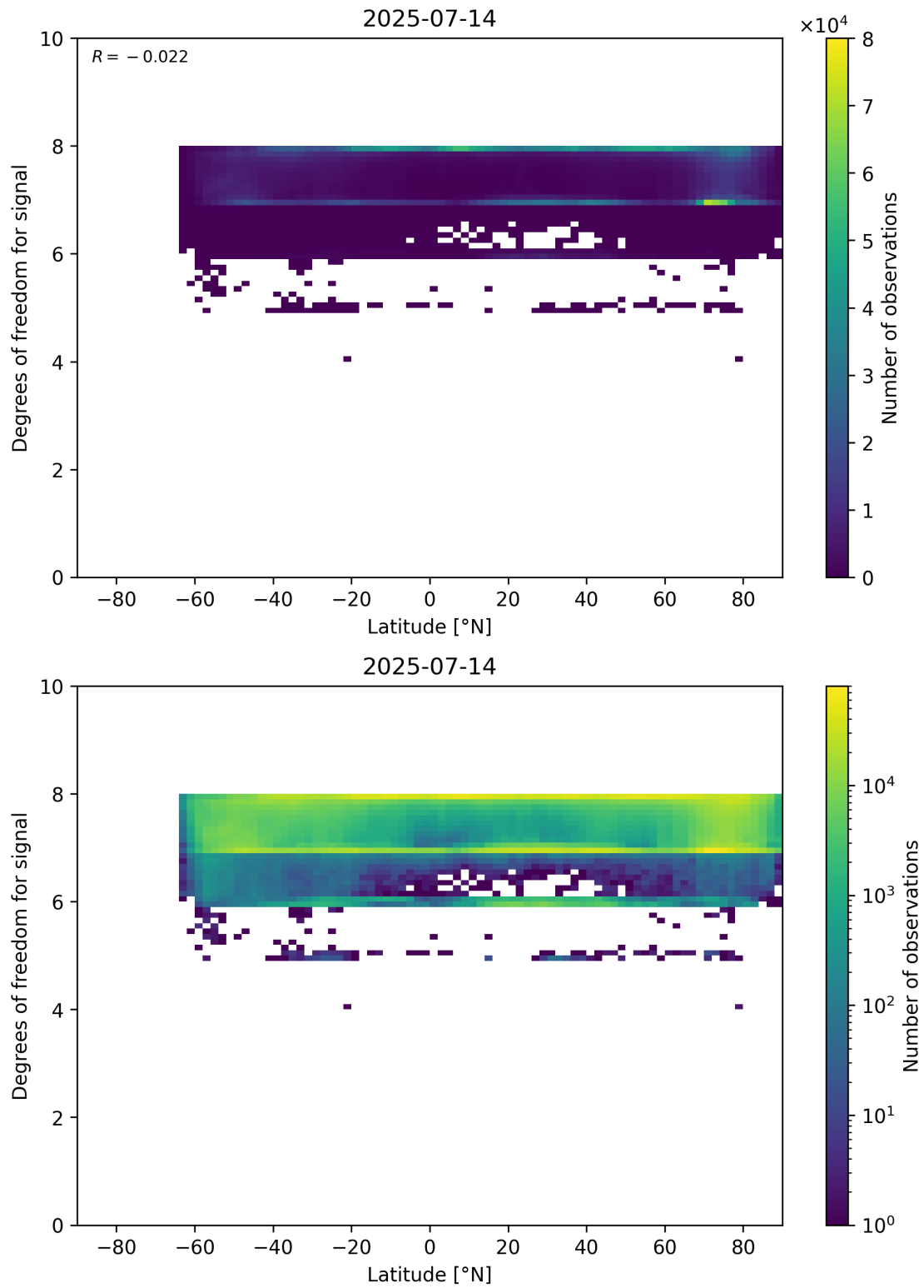
Figure 55: Scatter density plot of “Latitude” against “Degrees of freedom for signal” for 2025-07-13 to 2025-07-15.
