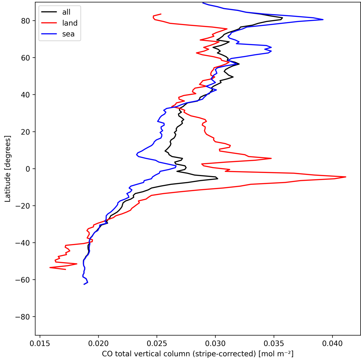
Figure 11: Zonal average of “CO total vertical column (stripe-corrected)” for 2025-07-13 to 2025-07-15.
