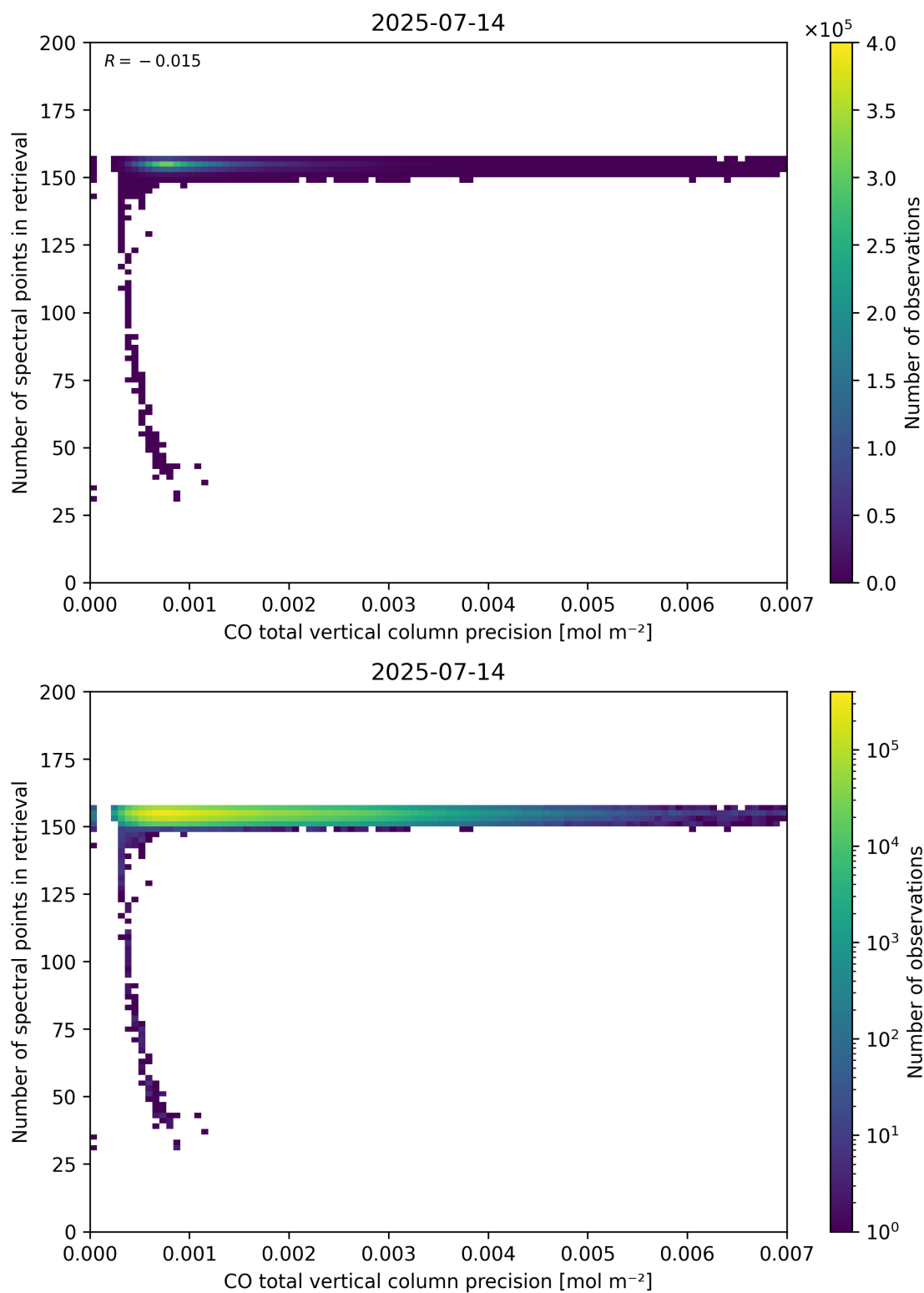
Figure 47: Scatter density plot of “CO total vertical column precision” against “Number of spectral points in retrieval” for 2025-07-13 to 2025-07-15.
