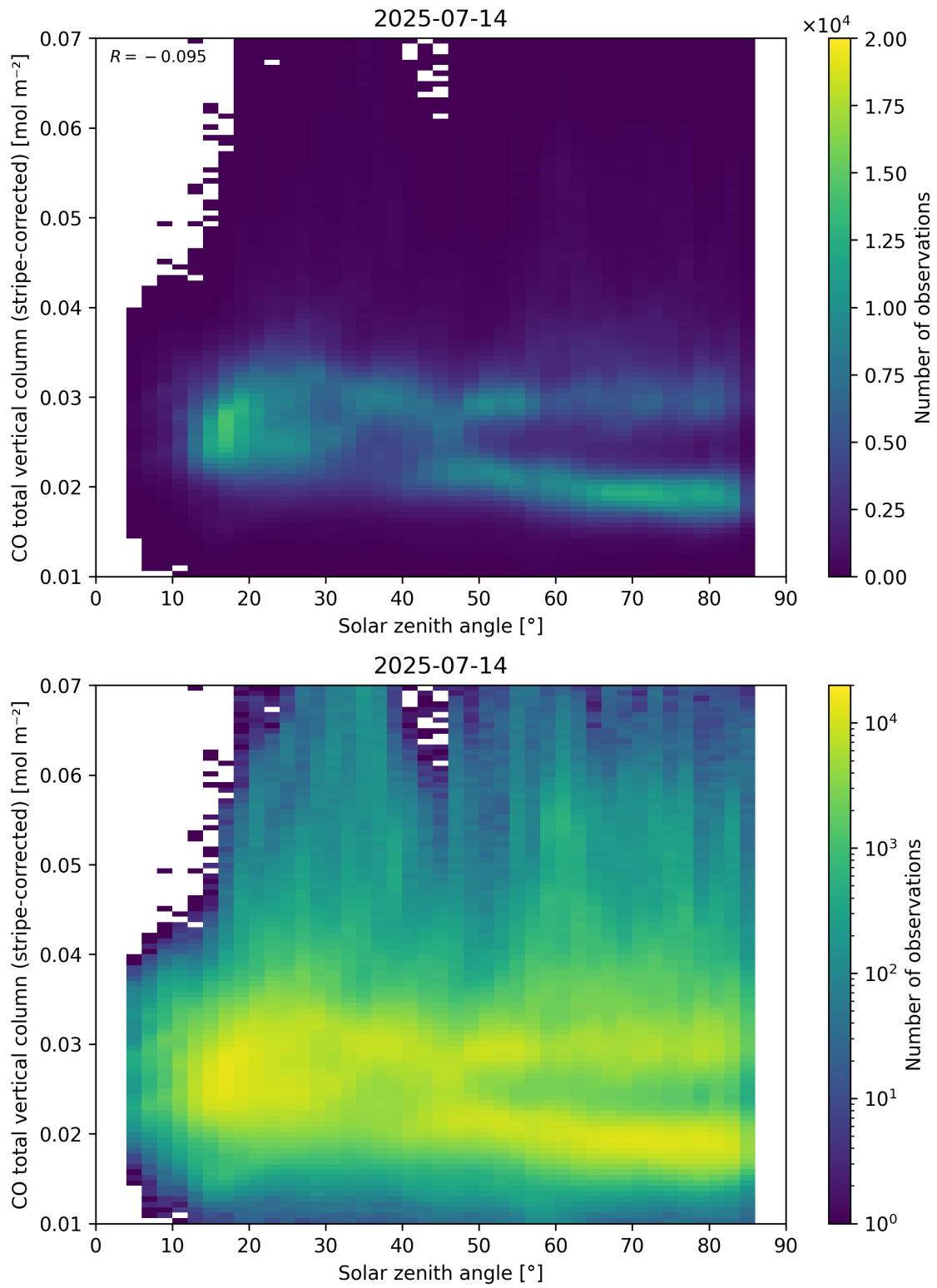
Figure 62: Scatter density plot of “Solar zenith angle” against “CO total vertical column (stripe-corrected)” for 2025-07-13 to 2025-07-15.
