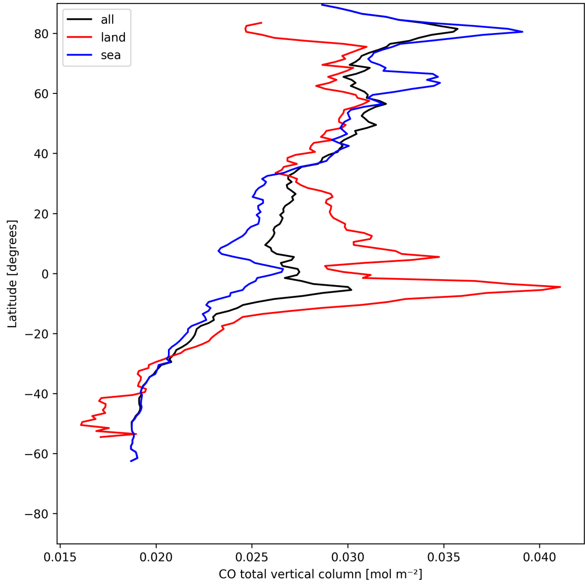
Figure 10: Zonal average of “CO total vertical column” for 2025-07-13 to 2025-07-15.
