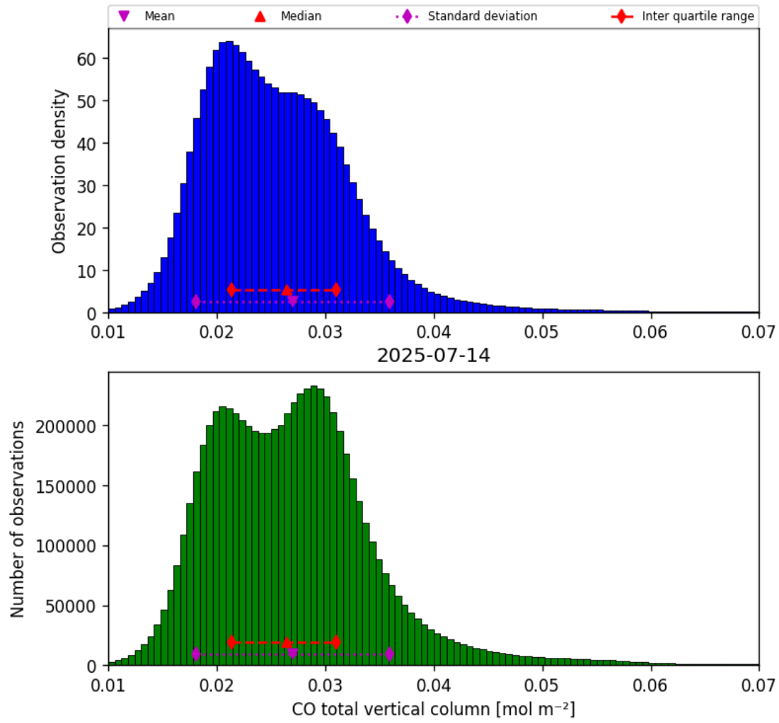
Figure 18: Histogram of “CO total vertical column” for 2025-07-13 to 2025-07-15
