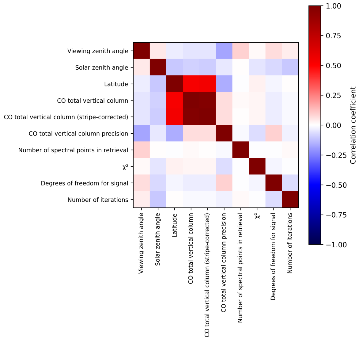
Figure 2: Map of correlation matrix for 2025-07-13 to 2025-07-15.
