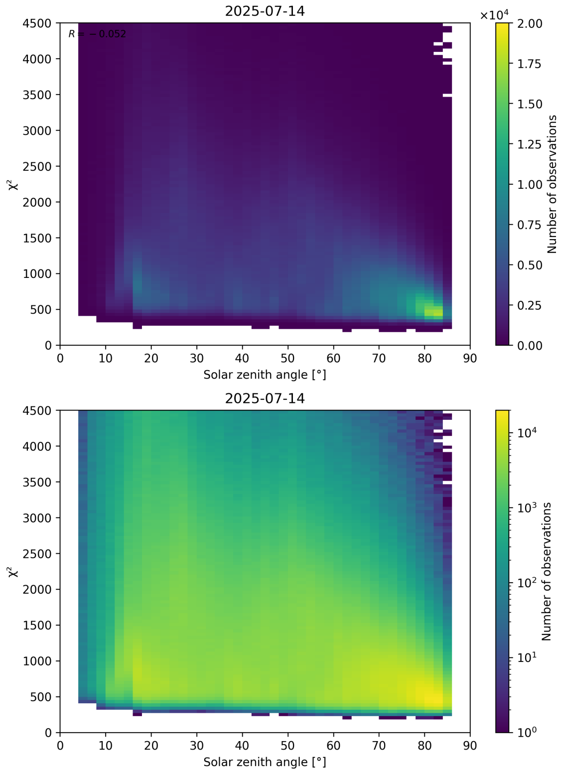
Figure 64: Scatter density plot of “Solar zenith angle” against “ \chi^2 ” for 2025-07-13 to 2025-07-15.
