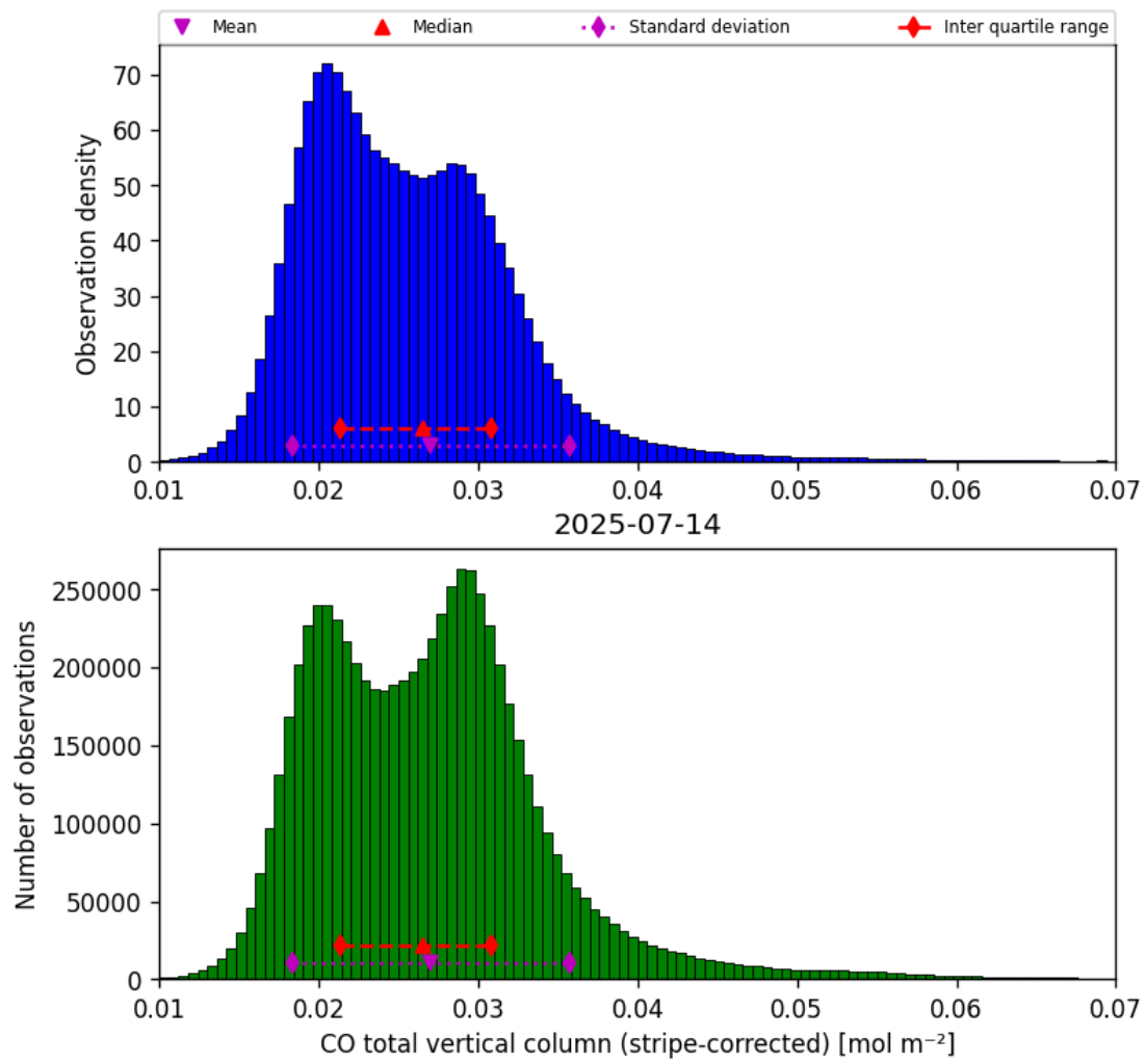
Figure 19: Histogram of “CO total vertical column (stripe-corrected)” for 2025-07-13 to 2025-07-15
