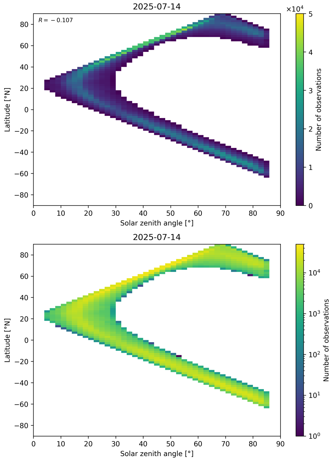
Figure 66: Scatter density plot of “Solar zenith angle” against “Latitude” for 2025-07-13 to 2025-07-15.
