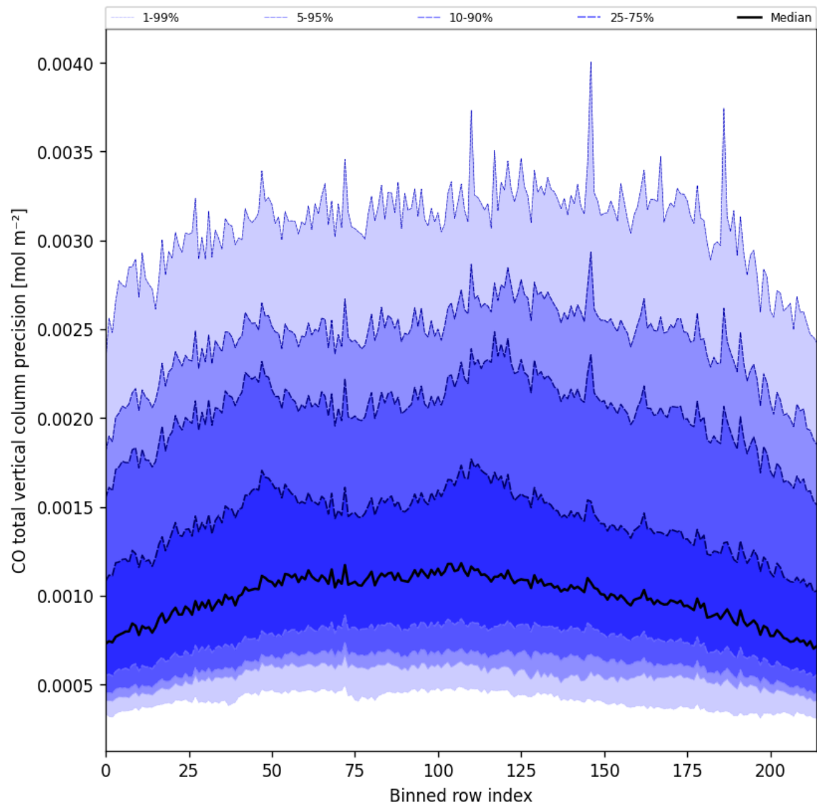
Figure 28: Along track statistics of “CO total vertical column precision” for 2025-07-13 to 2025-07-15
