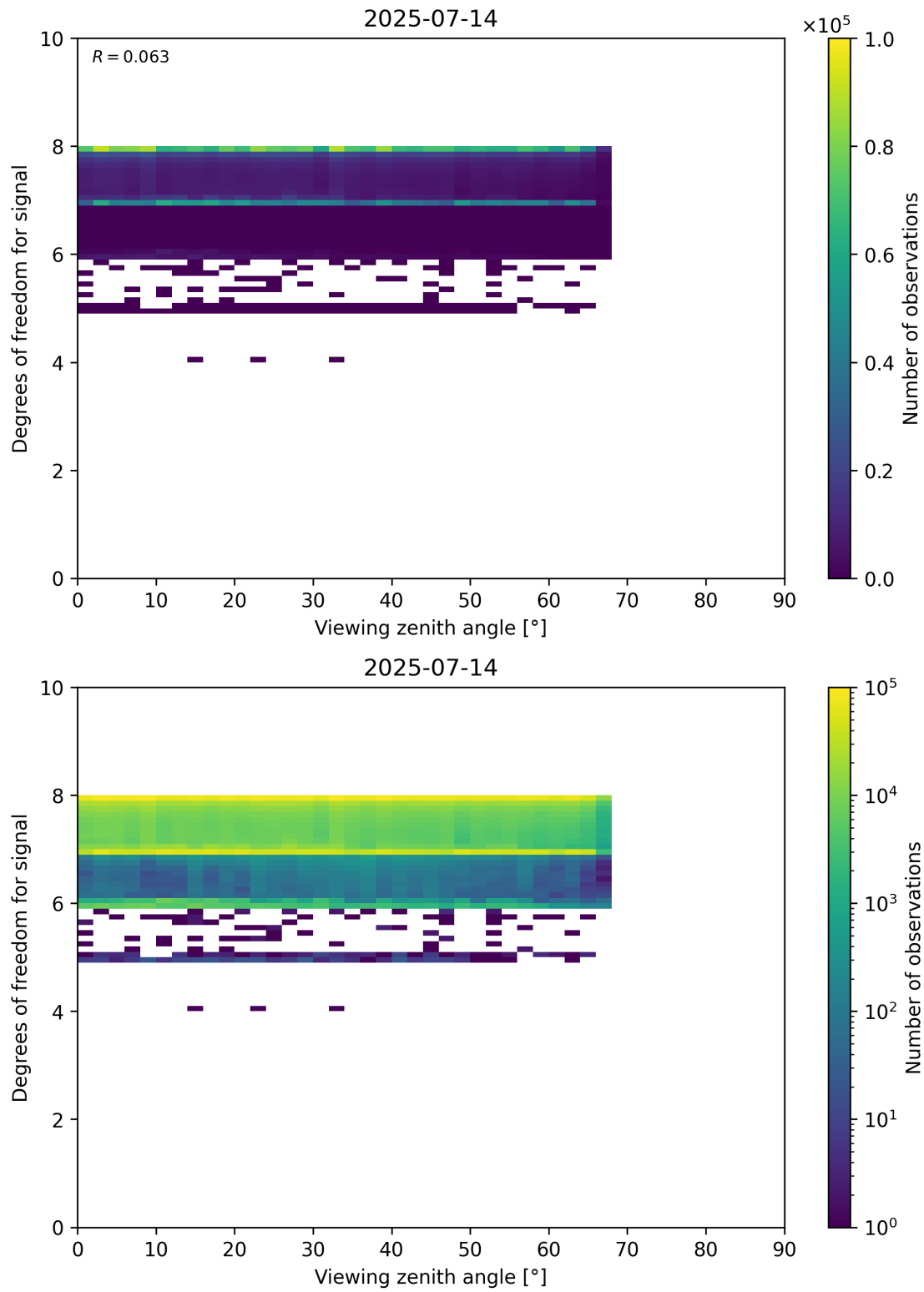
Figure 73: Scatter density plot of “Viewing zenith angle” against “Degrees of freedom for signal” for 2025-07-13 to 2025-07-15.
