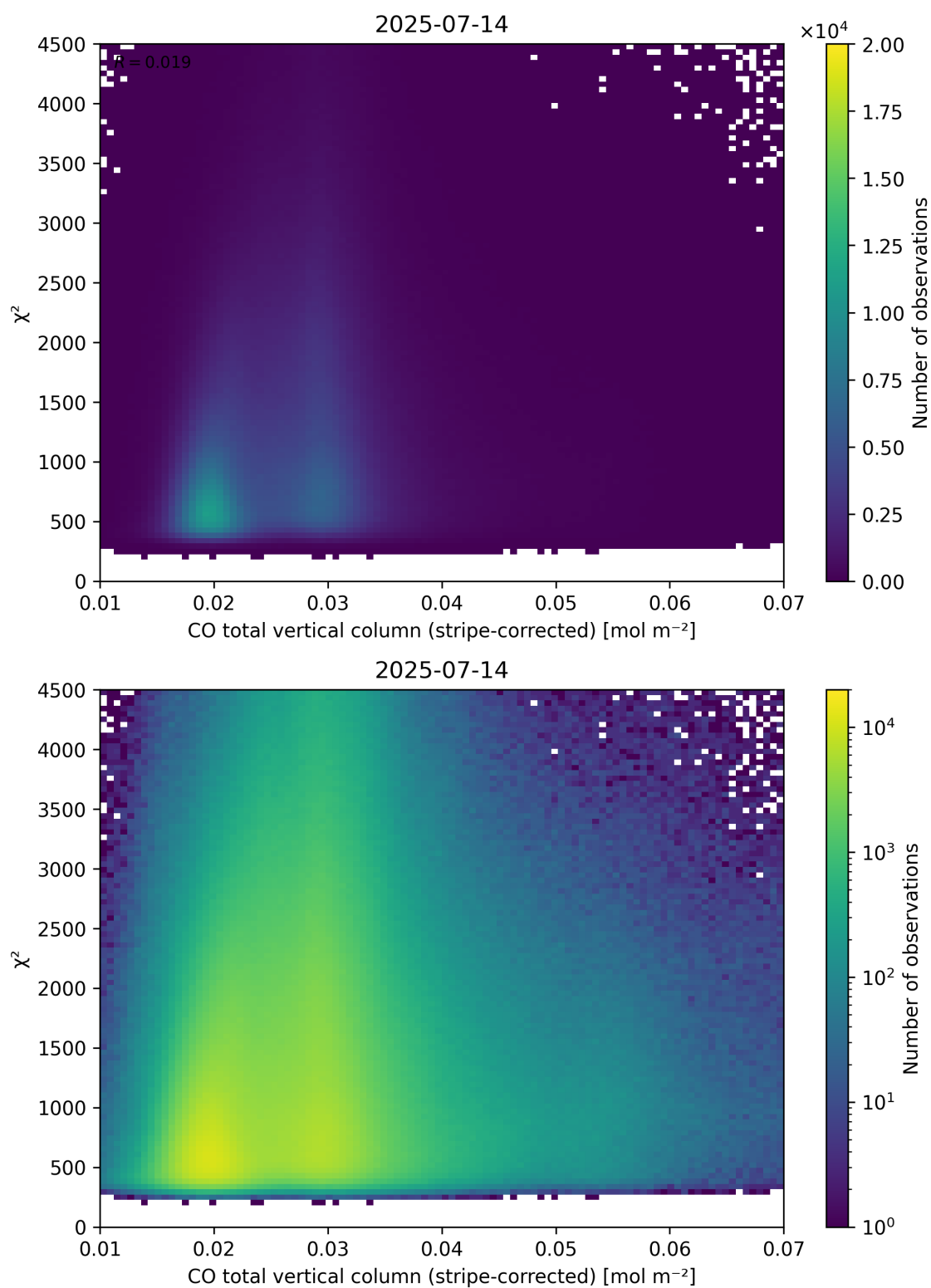
Figure 37: Scatter density plot of “CO total vertical column (stripe-corrected)” against “ \chi^2 ” for 2025-07-13 to 2025-07-15.
