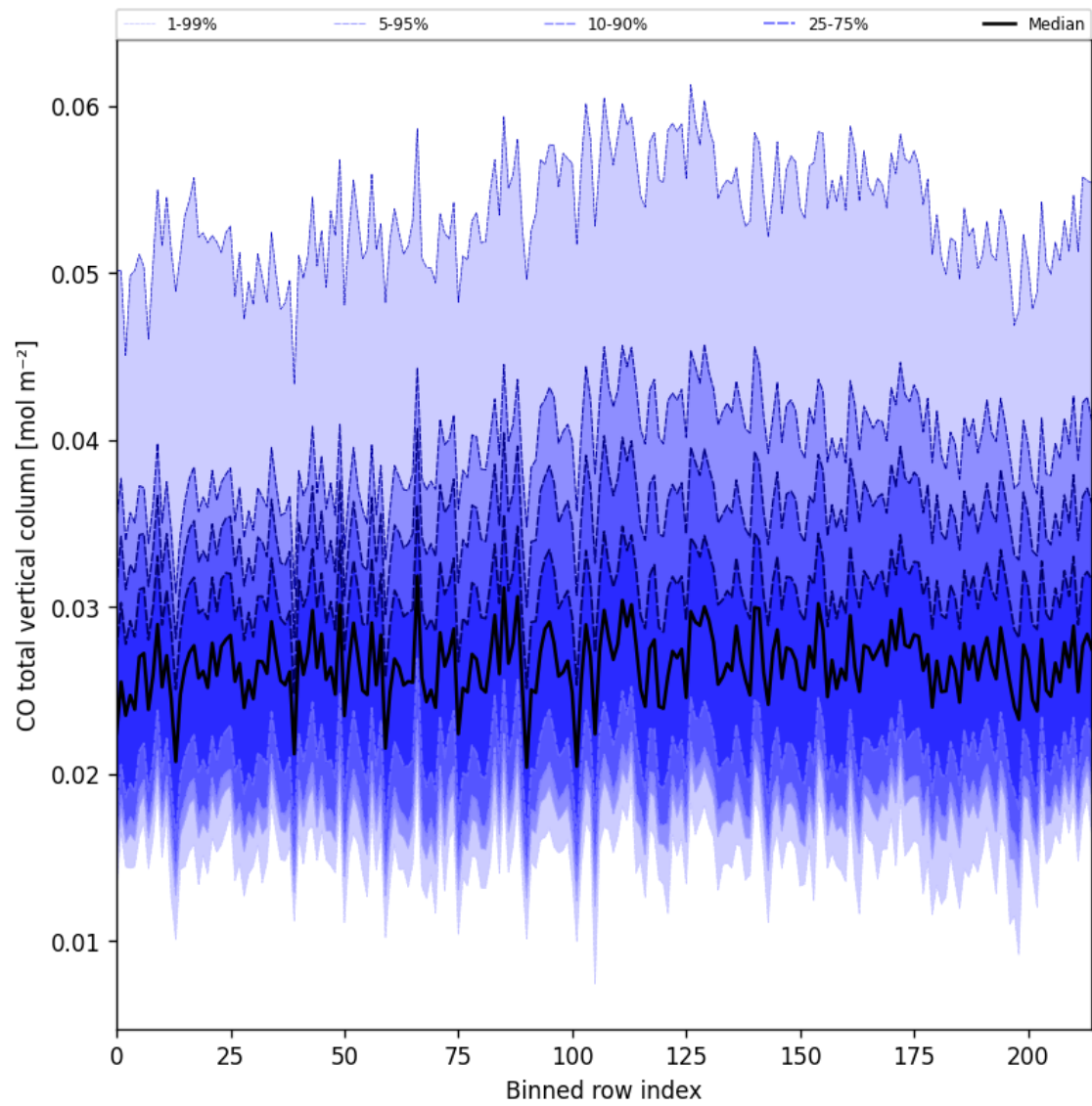
Figure 26: Along track statistics of “CO total vertical column” for 2025-07-13 to 2025-07-15
