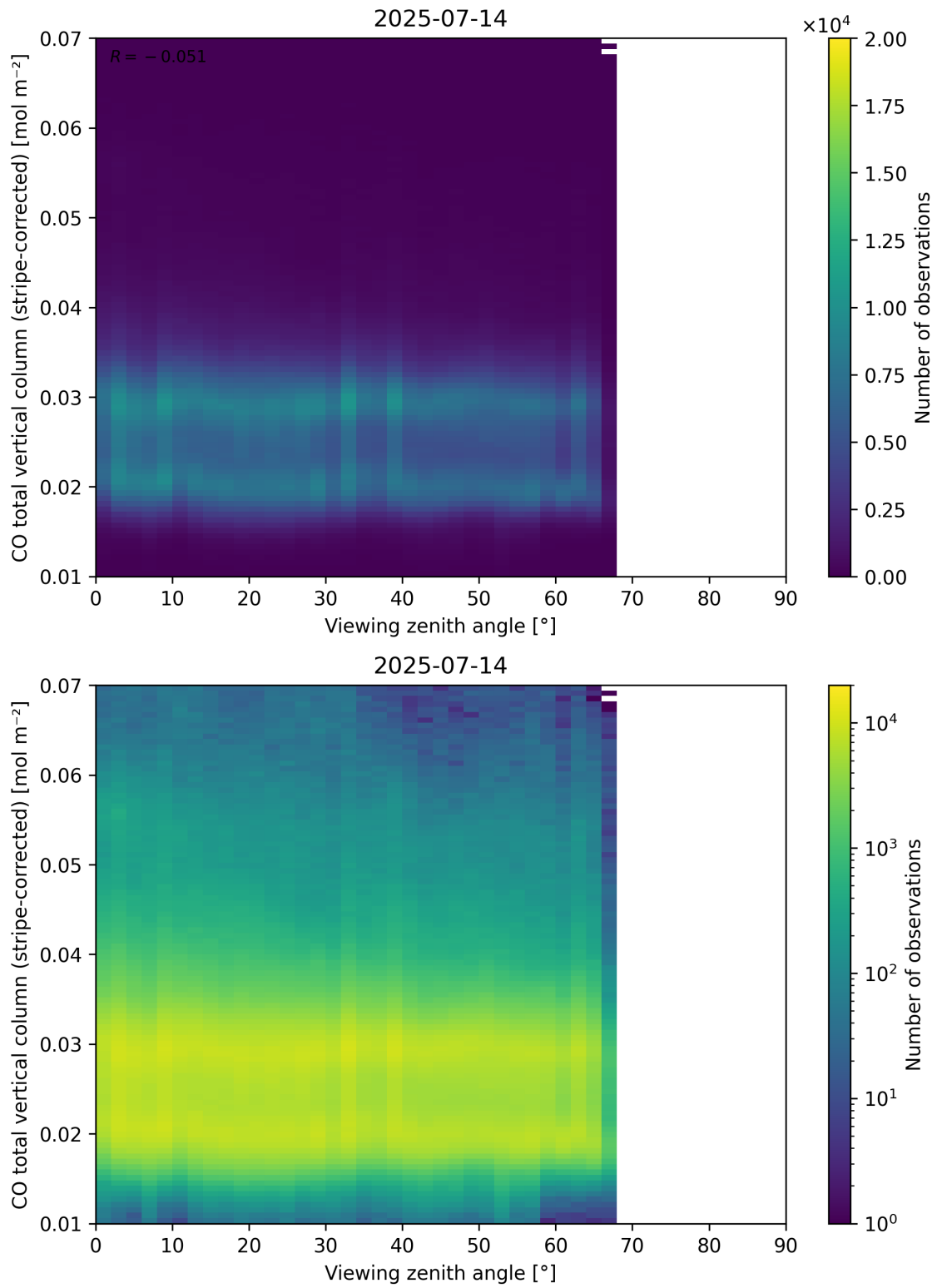
Figure 70: Scatter density plot of “Viewing zenith angle” against “CO total vertical column (stripe-corrected)” for 2025-07-13 to 2025-07-15.
