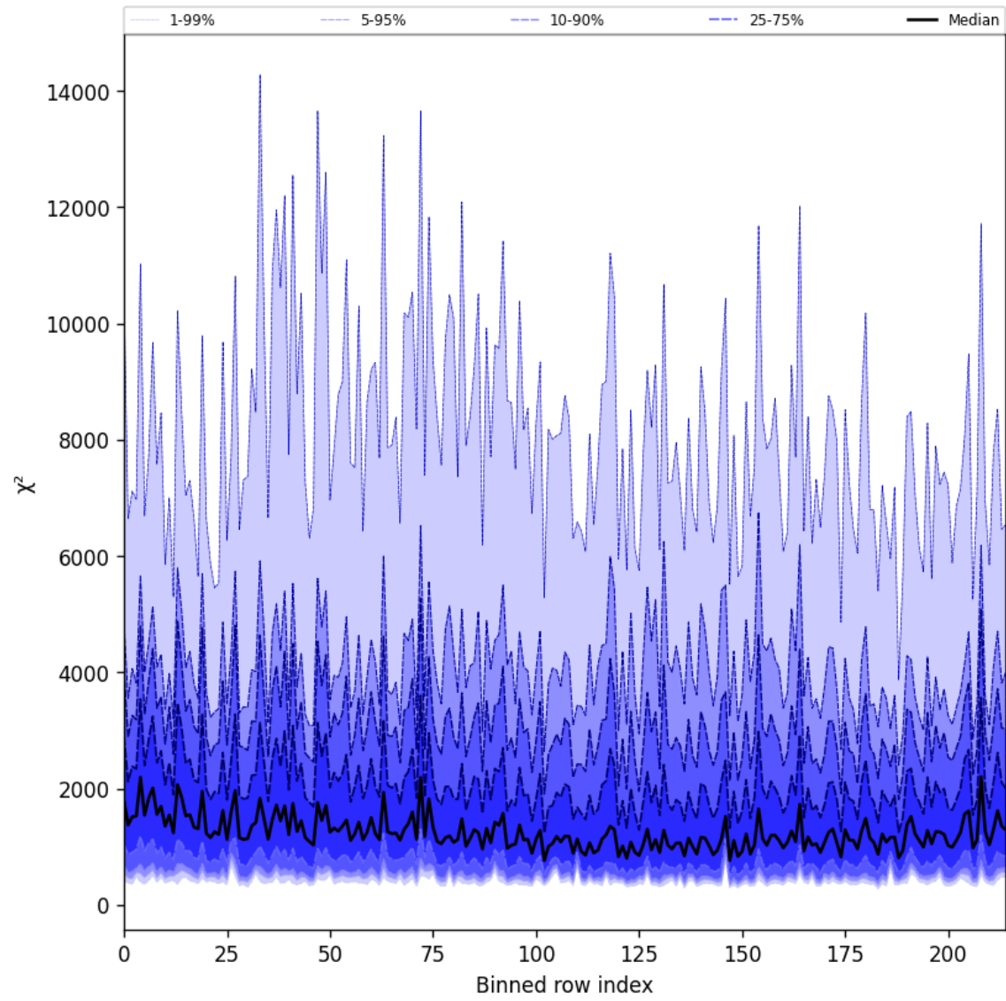
Figure 30: Along track statistics of “ \chi^2 ” for 2025-07-13 to 2025-07-15
