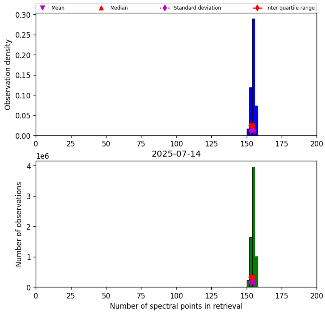
Figure 21: Histogram of “Number of spectral points in retrieval” for 2025-07-13 to 2025-07-15
