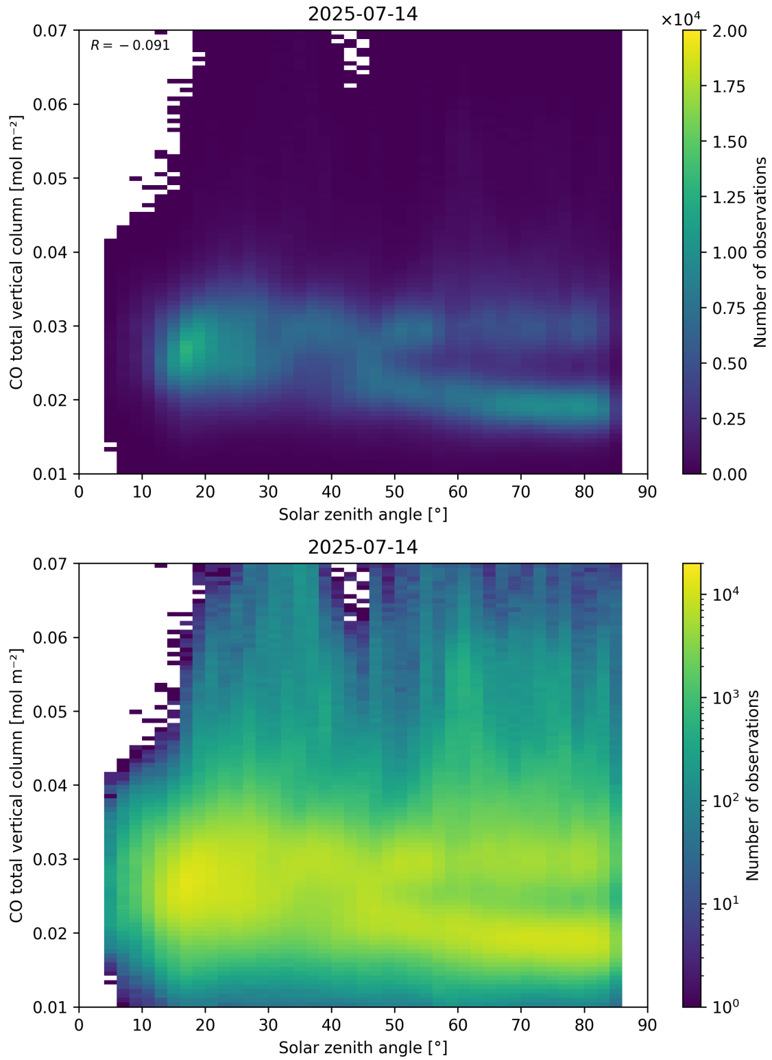
Figure 61: Scatter density plot of “Solar zenith angle” against “CO total vertical column” for 2025-07-13 to 2025-07-15.
