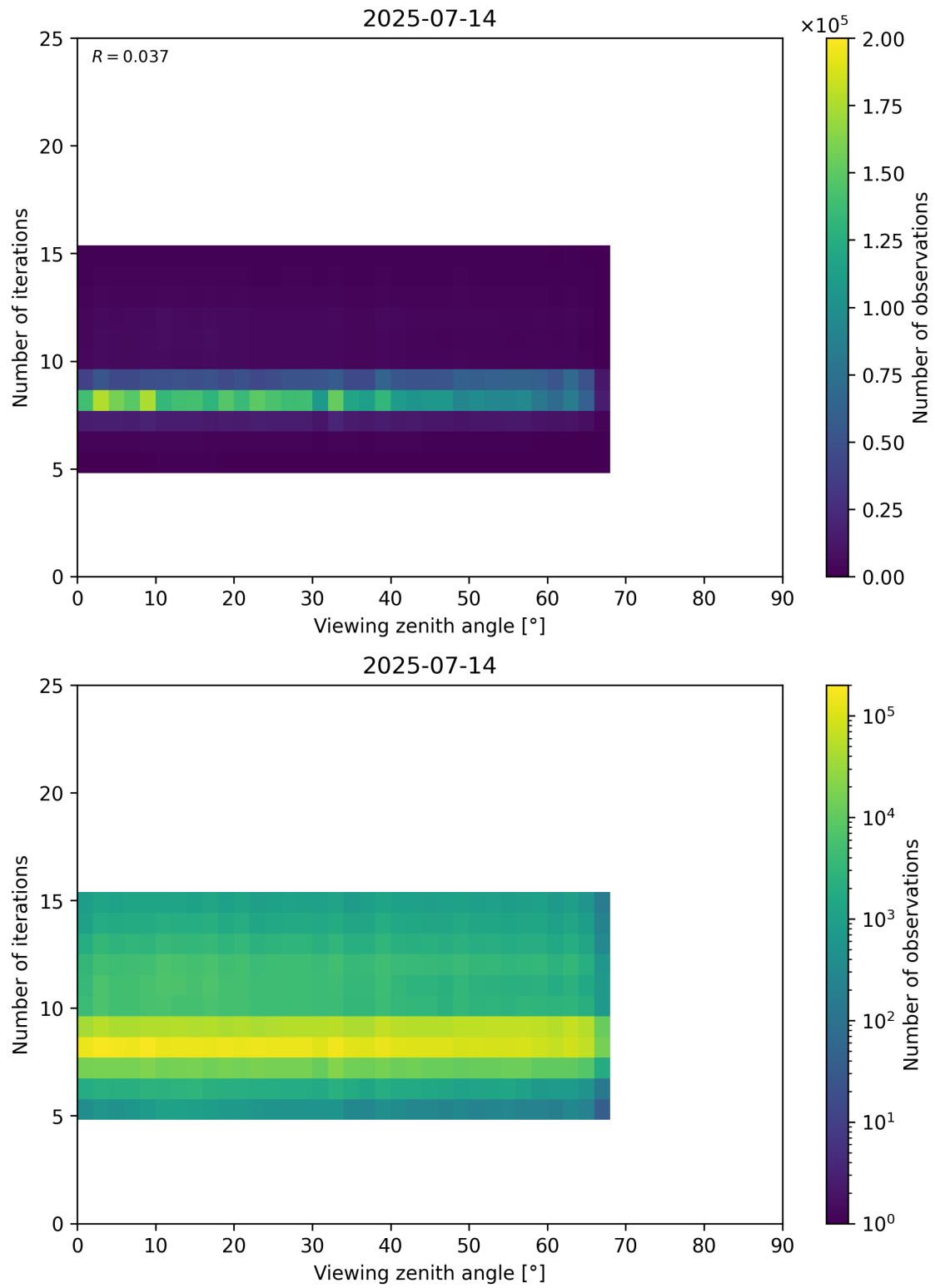
Figure 75: Scatter density plot of “Viewing zenith angle” against “Number of iterations” for 2025-07-13 to 2025-07-15.
