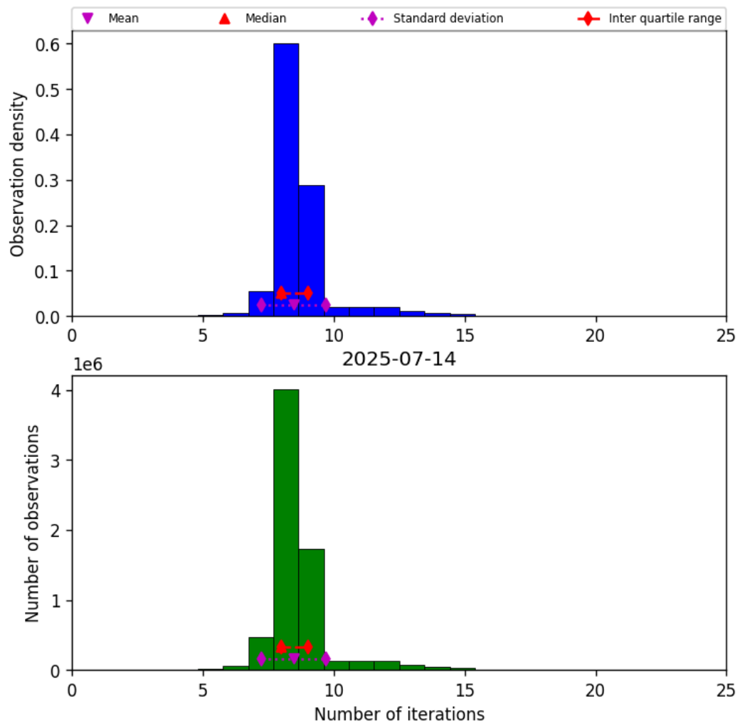
Figure 24: Histogram of “Number of iterations” for 2025-07-13 to 2025-07-15
