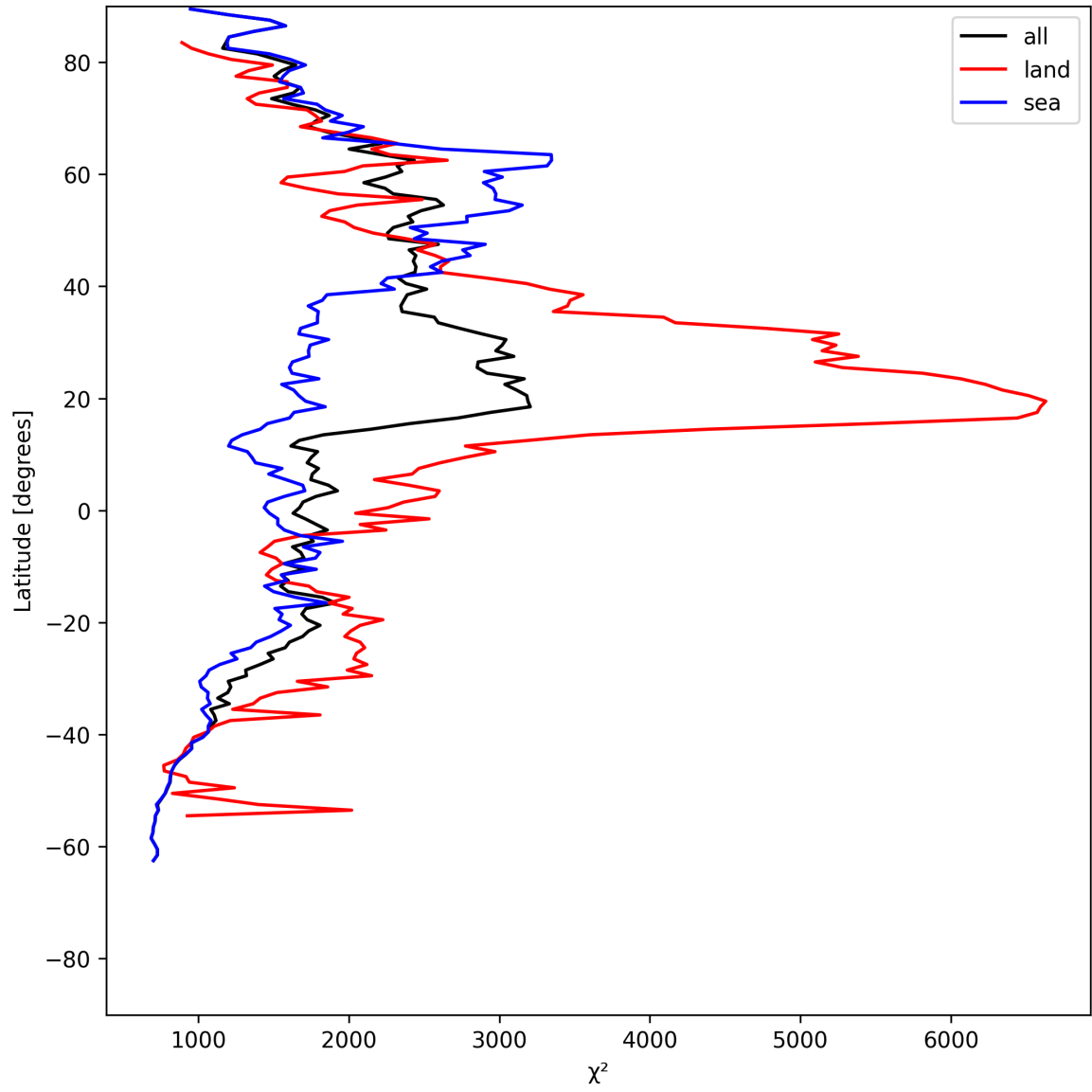
Figure 14: Zonal average of “ \chi^2 ” for 2025-07-13 to 2025-07-15.
