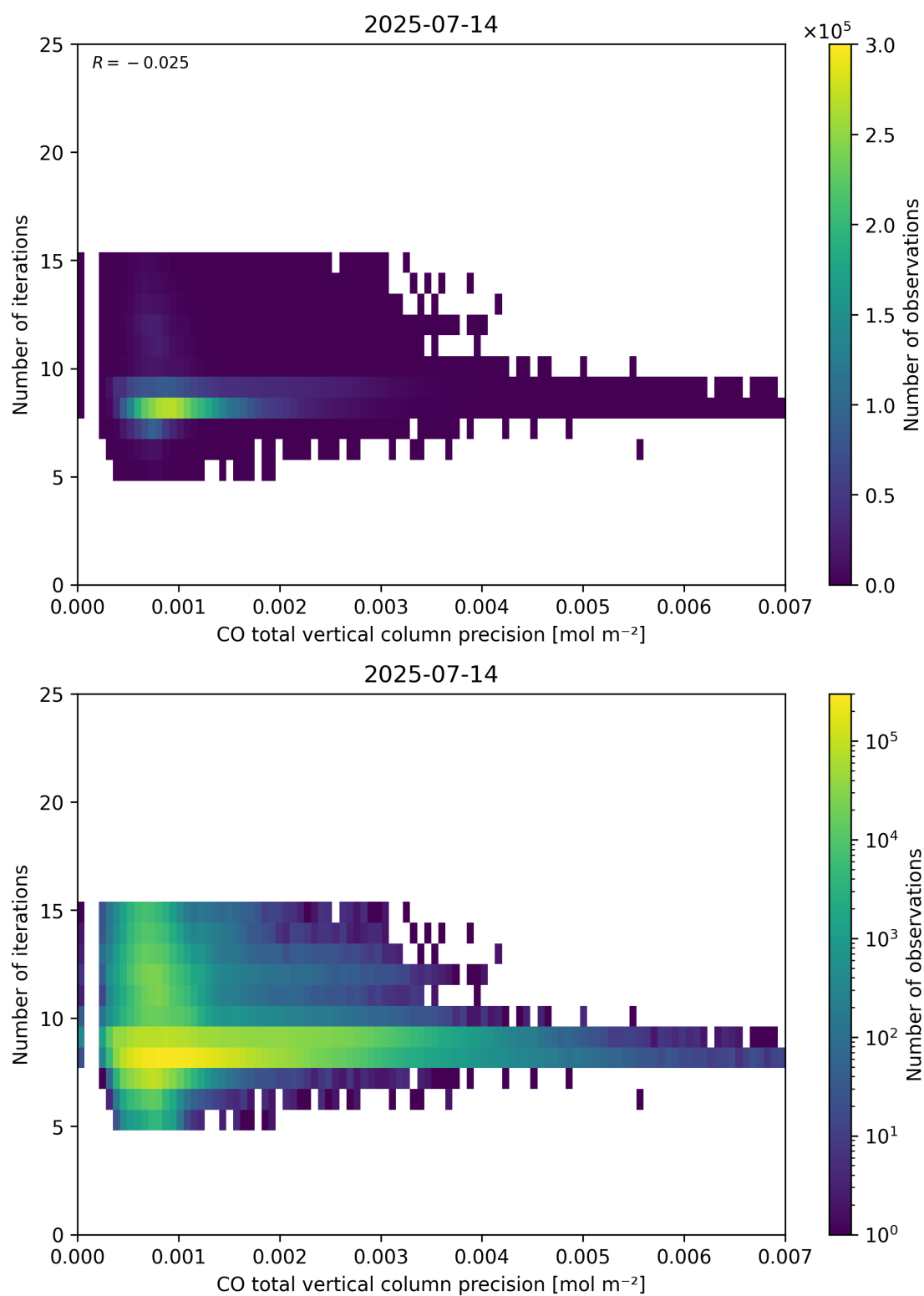
Figure 46: Scatter density plot of “CO total vertical column precision” against “Number of iterations” for 2025-07-13 to 2025-07-15.
