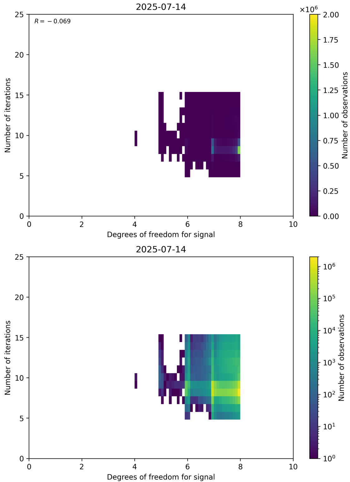
Figure 50: Scatter density plot of “Degrees of freedom for signal” against “Number of iterations” for 2025-07-13 to 2025-07-15.
