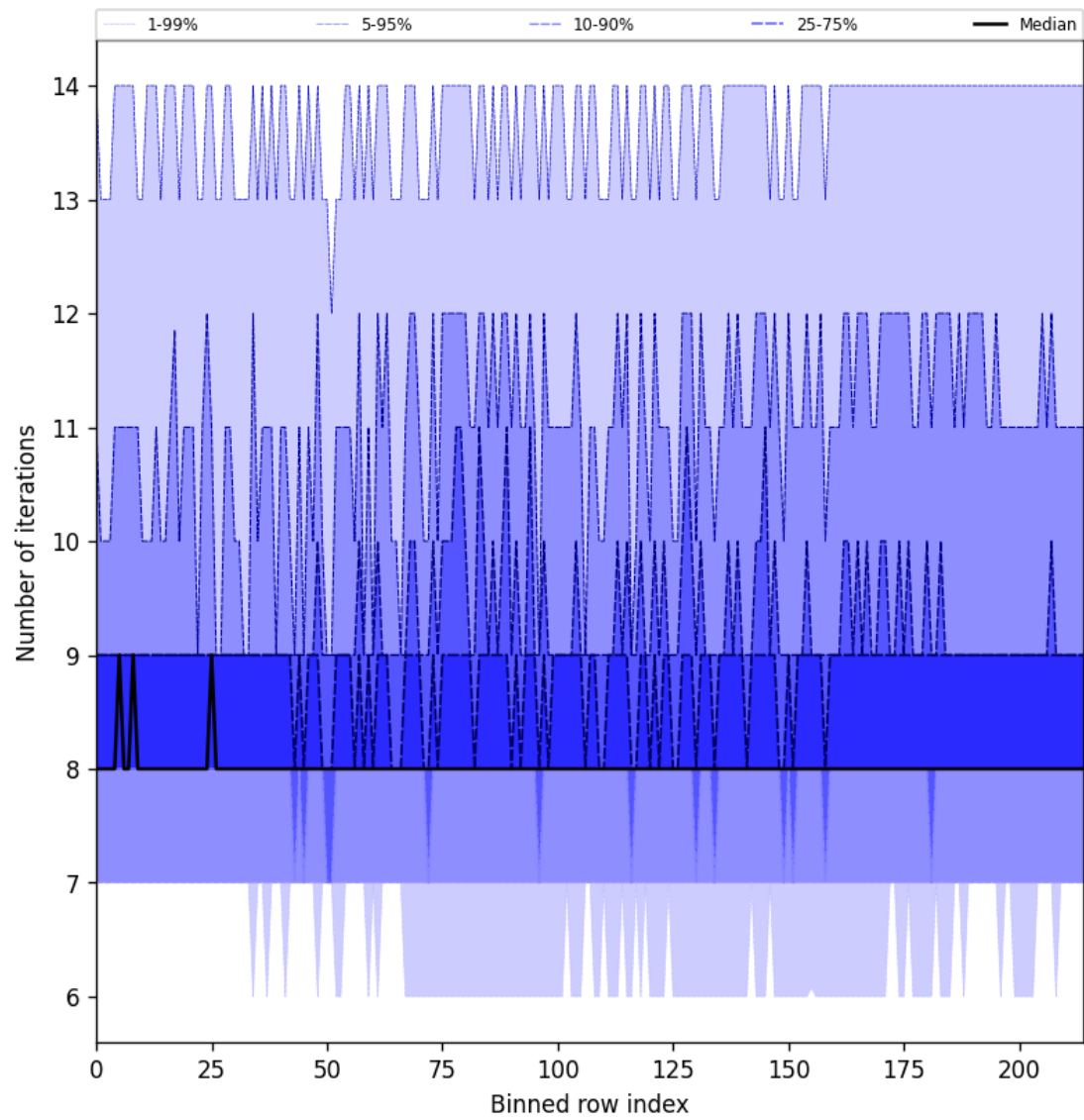
Figure 32: Along track statistics of “Number of iterations” for 2025-07-13 to 2025-07-15
