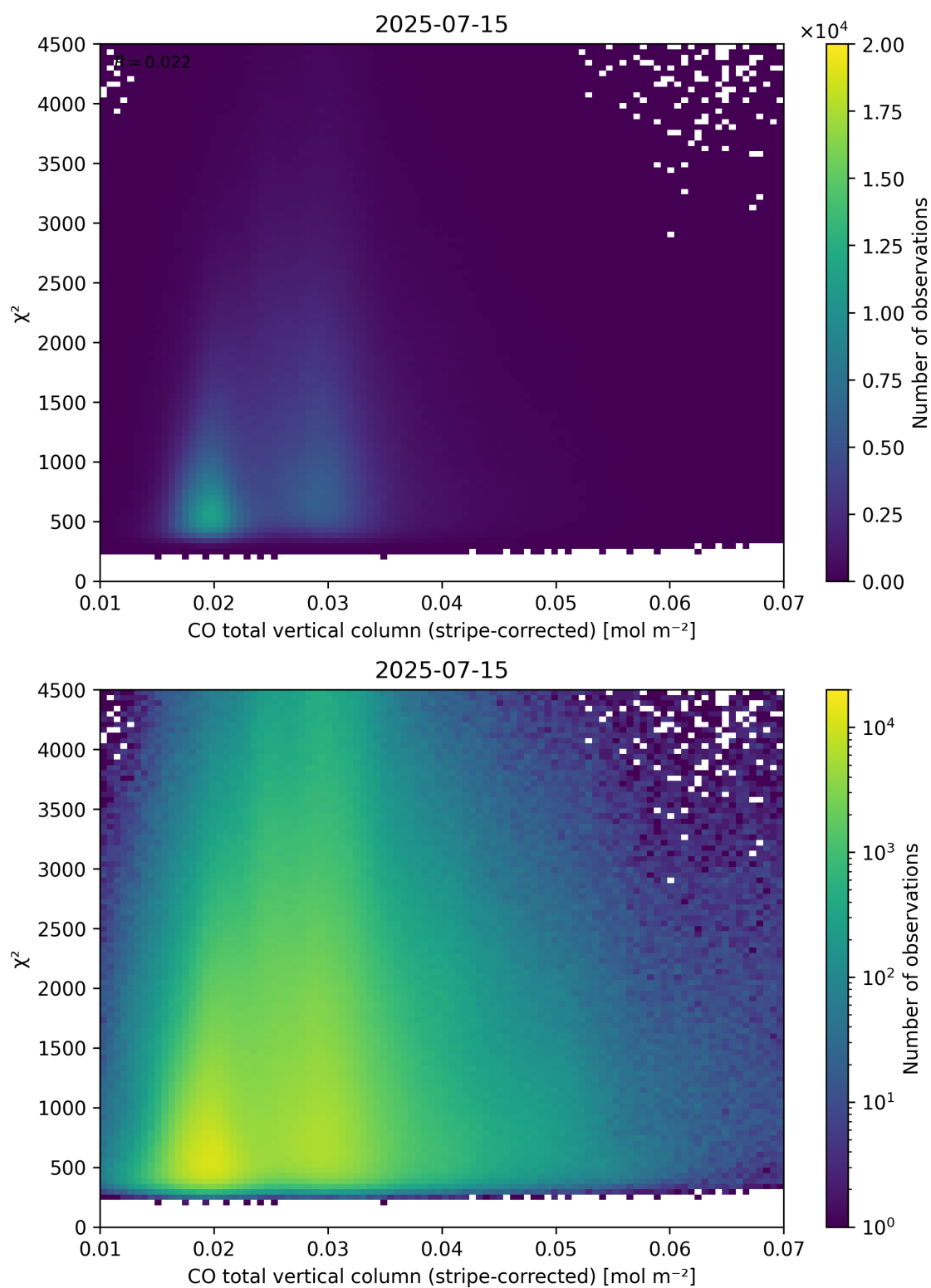
Figure 37: Scatter density plot of “CO total vertical column (stripe-corrected)” against “ \chi^2 ” for 2025-07-14 to 2025-07-16.
