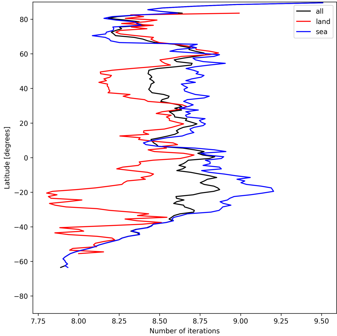
Figure 16: Zonal average of “Number of iterations” for 2025-07-14 to 2025-07-16.
