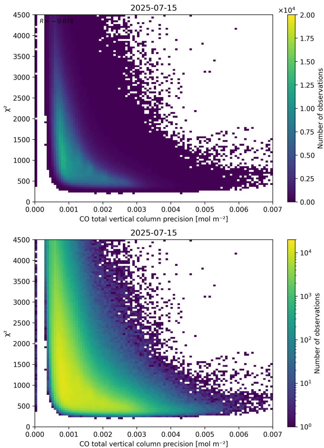
Figure 44: Scatter density plot of “CO total vertical column precision” against “ \chi^2 ” for 2025-07-14 to 2025-07-16.
