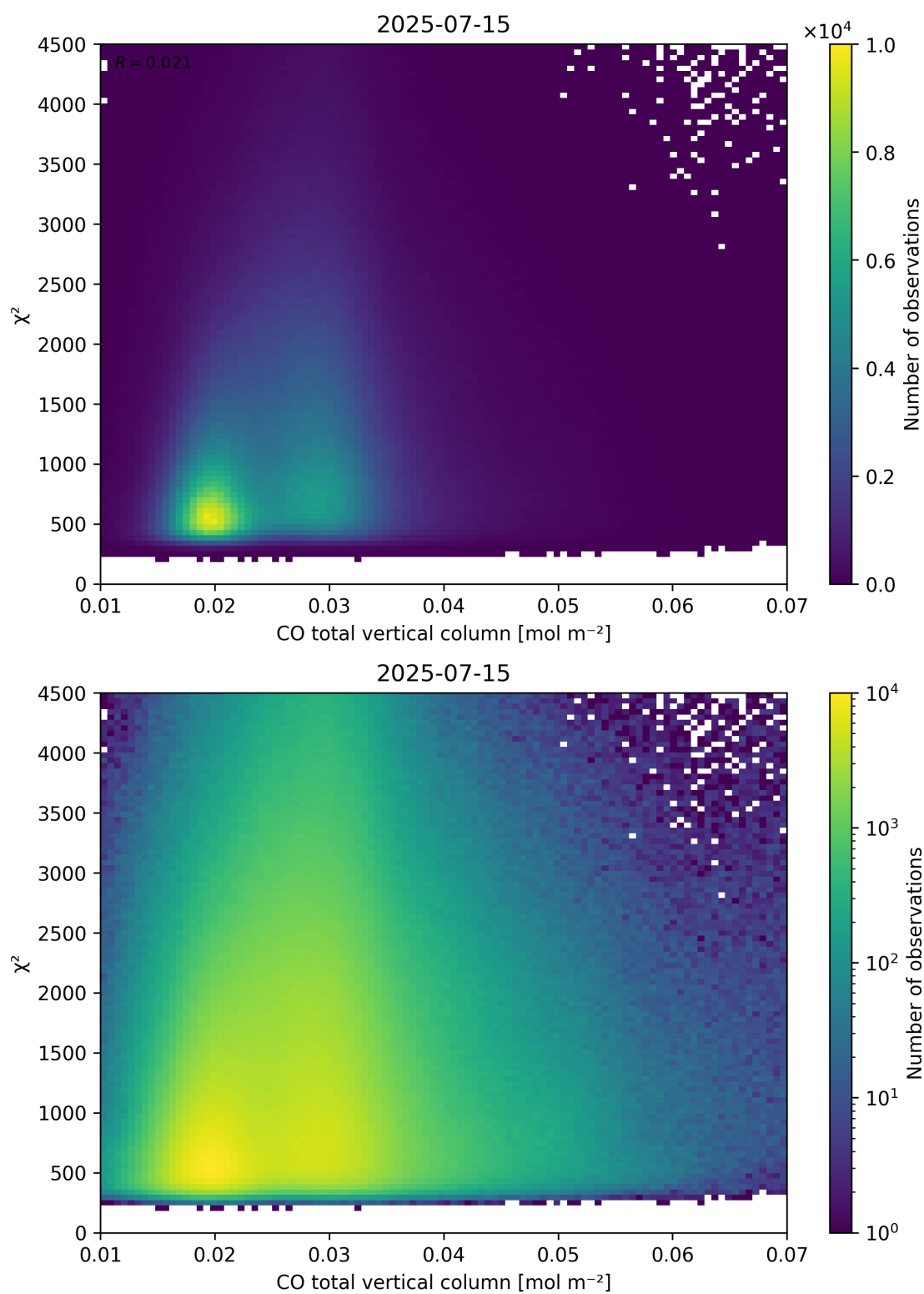
Figure 35: Scatter density plot of “CO total vertical column” against “ \chi^2 ” for 2025-07-14 to 2025-07-16.
