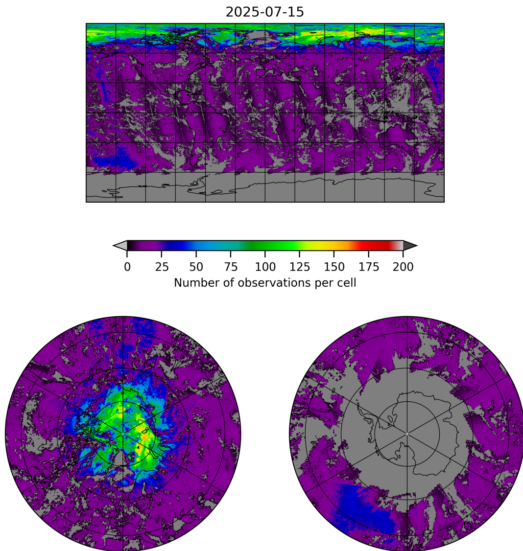
Figure 8: Map of the number of observations for 2025-07-14 to 2025-07-16
