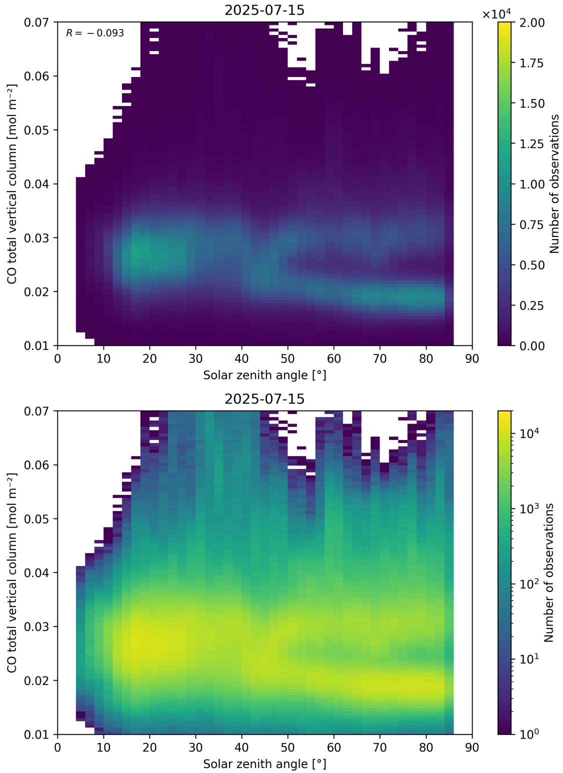
Figure 61: Scatter density plot of “Solar zenith angle” against “CO total vertical column” for 2025-07-14 to 2025-07-16.
