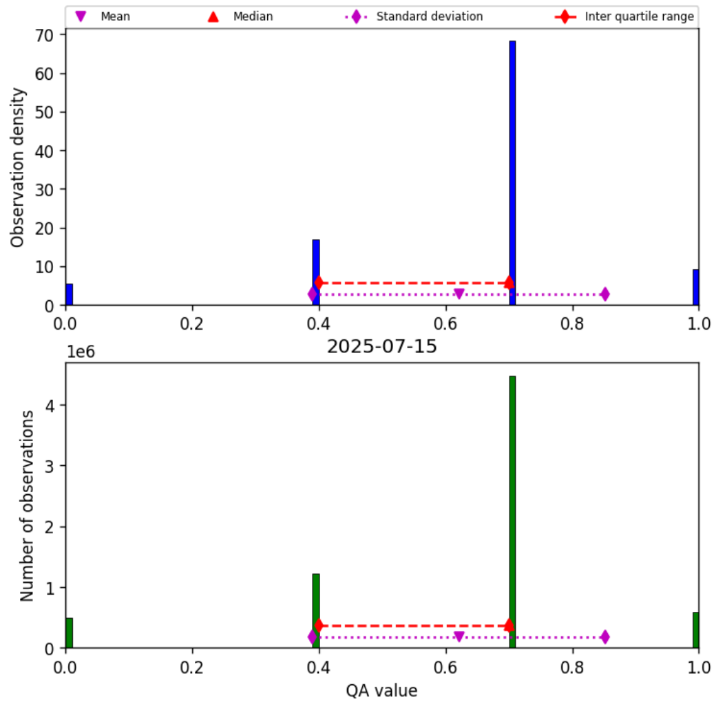
Figure 17: Histogram of “QA value” for 2025-07-14 to 2025-07-16
