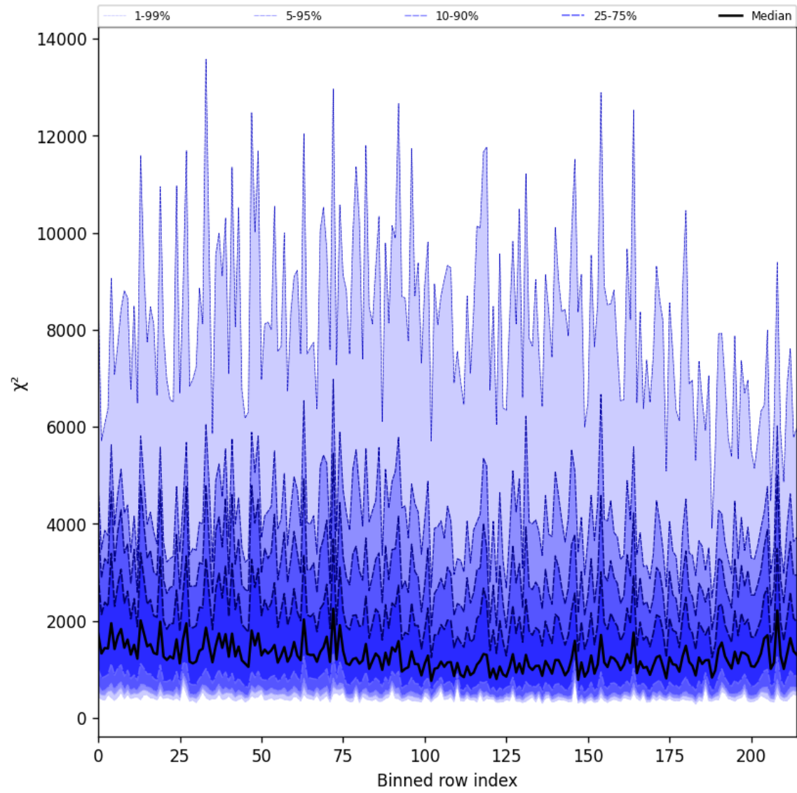
Figure 30: Along track statistics of “ \chi^2 ” for 2025-07-14 to 2025-07-16
