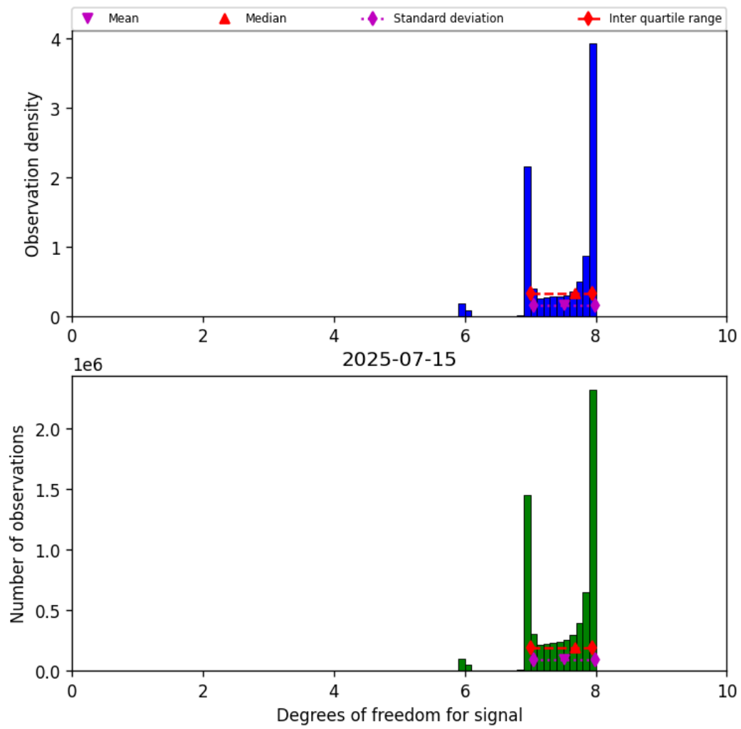
Figure 23: Histogram of “Degrees of freedom for signal” for 2025-07-14 to 2025-07-16
