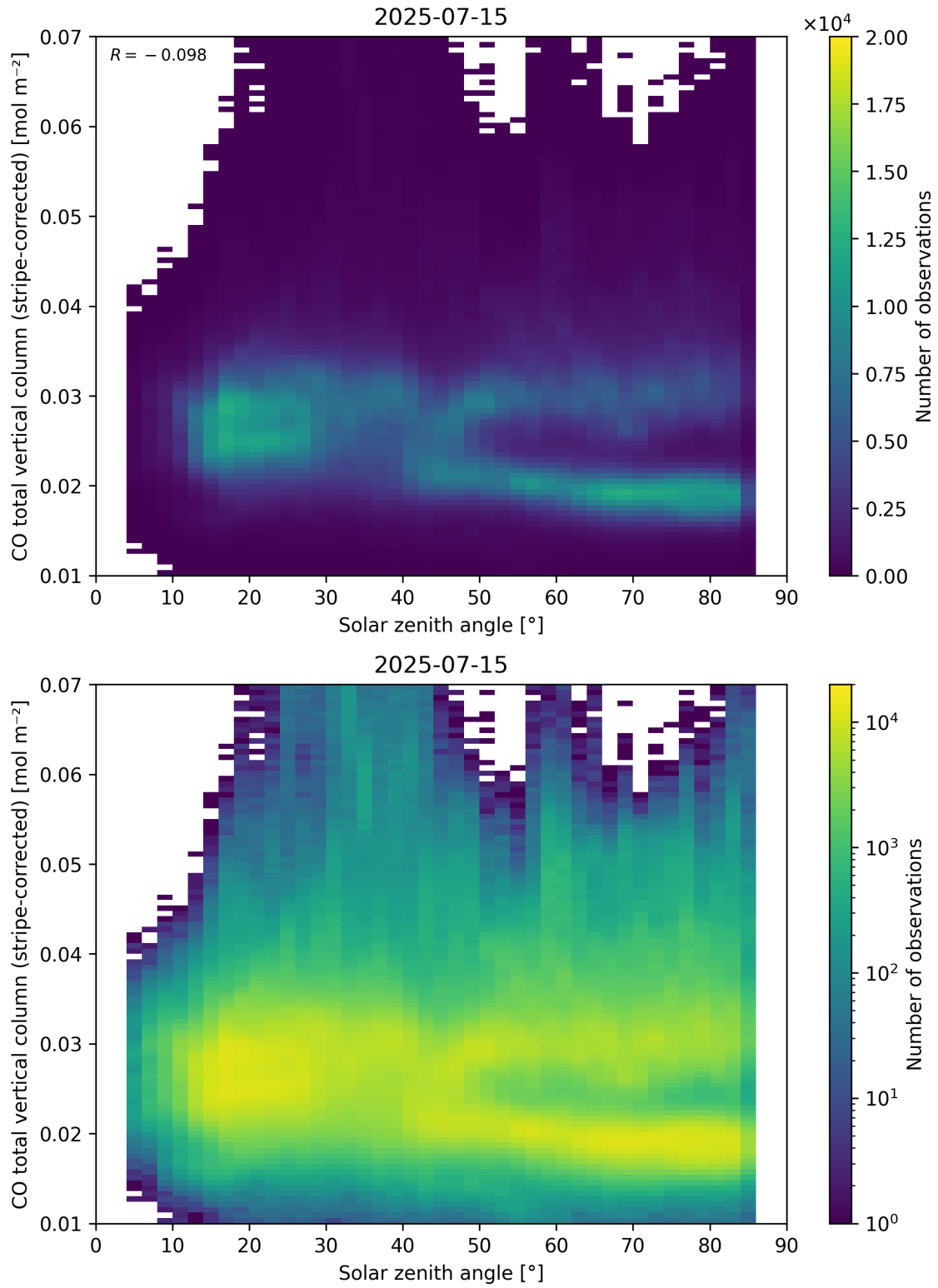
Figure 62: Scatter density plot of “Solar zenith angle” against “CO total vertical column (stripe-corrected)” for 2025-07-14 to 2025-07-16.
