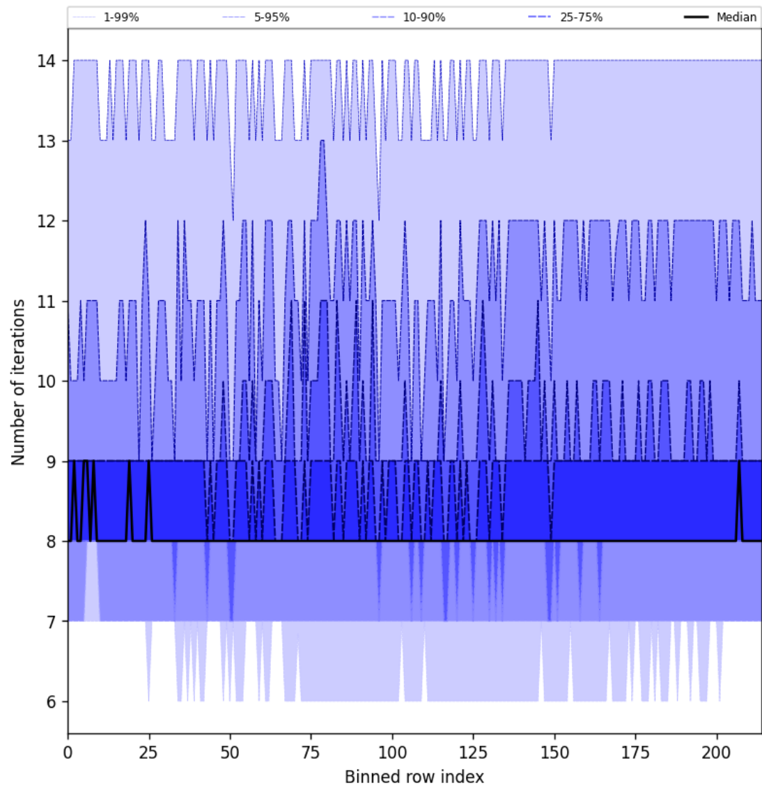
Figure 32: Along track statistics of “Number of iterations” for 2025-07-14 to 2025-07-16
