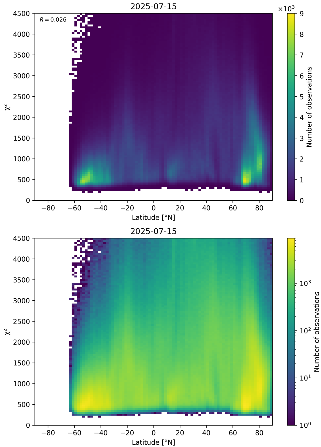
Figure 54: Scatter density plot of “Latitude” against “ \chi^2 ” for 2025-07-14 to 2025-07-16.
