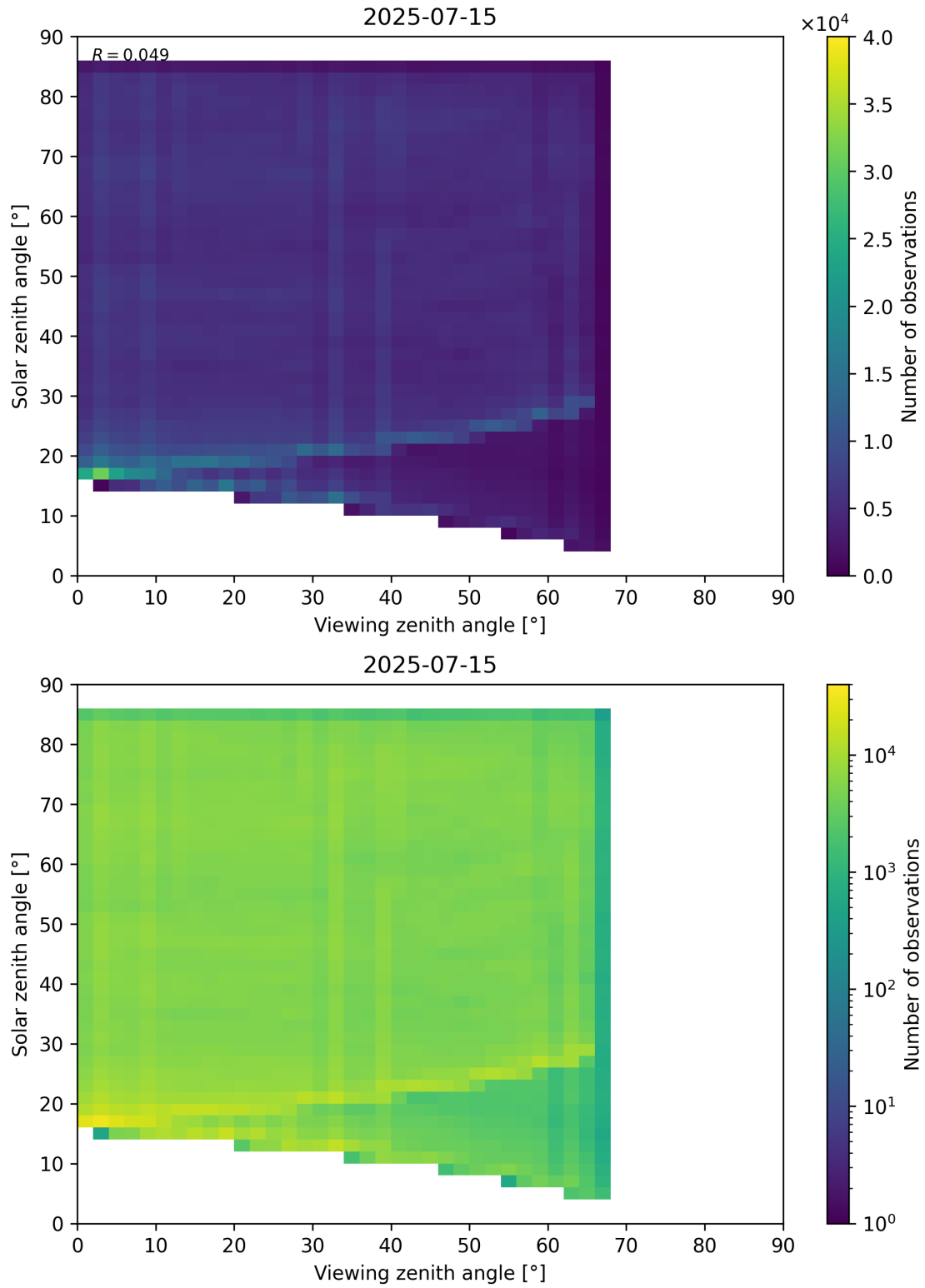
Figure 77: Scatter density plot of “Viewing zenith angle” against “Solar zenith angle” for 2025-07-14 to 2025-07-16.
