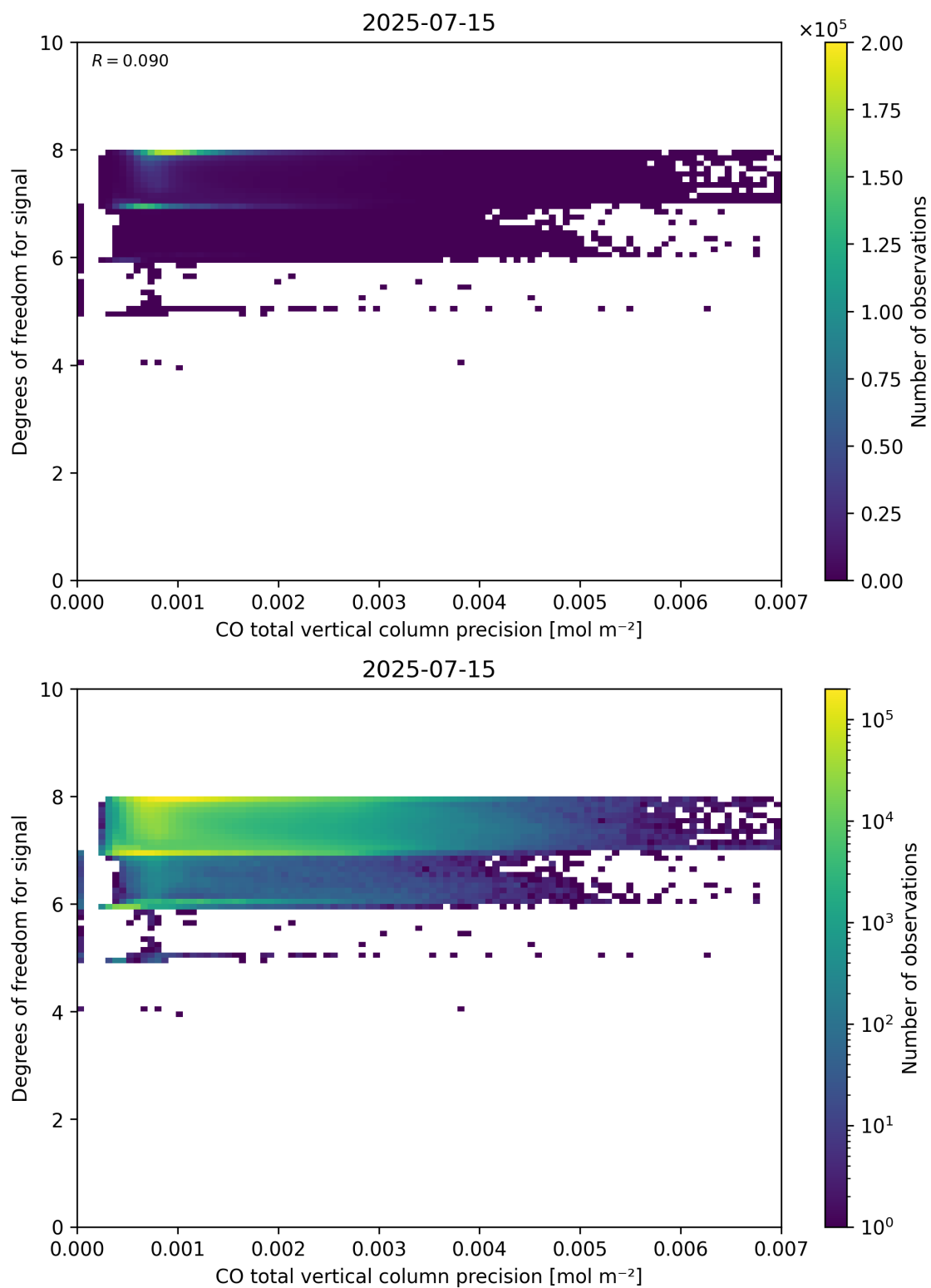
Figure 45: Scatter density plot of “CO total vertical column precision” against “Degrees of freedom for signal” for 2025-07-14 to 2025-07-16.
