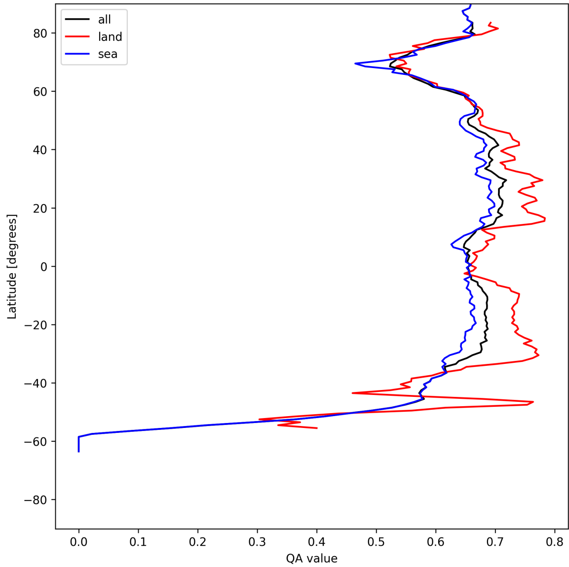
Figure 9: Zonal average of “QA value” for 2025-07-14 to 2025-07-16.
