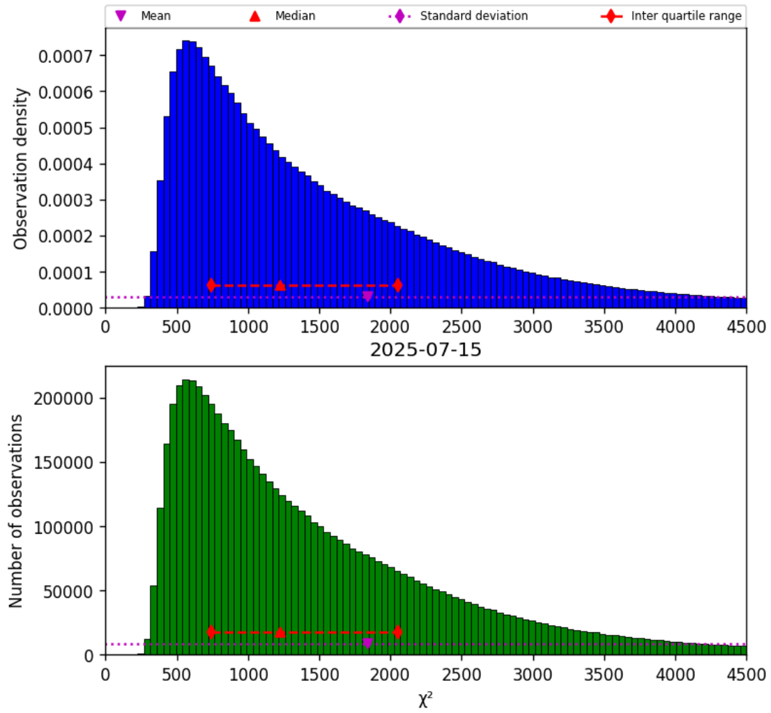
Figure 22: Histogram of “ \chi^2 ” for 2025-07-14 to 2025-07-16
