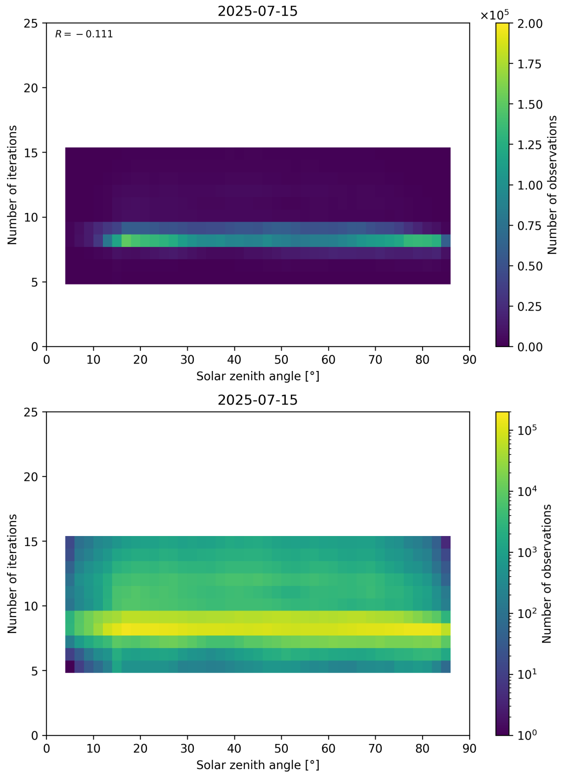
Figure 67: Scatter density plot of “Solar zenith angle” against “Number of iterations” for 2025-07-14 to 2025-07-16.
