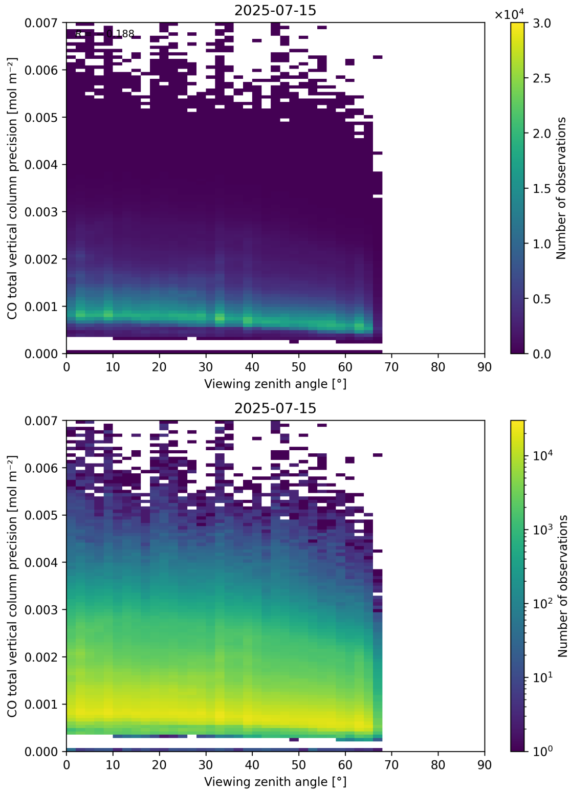
Figure 71: Scatter density plot of “Viewing zenith angle” against “CO total vertical column precision” for 2025-07-14 to 2025-07-16.
