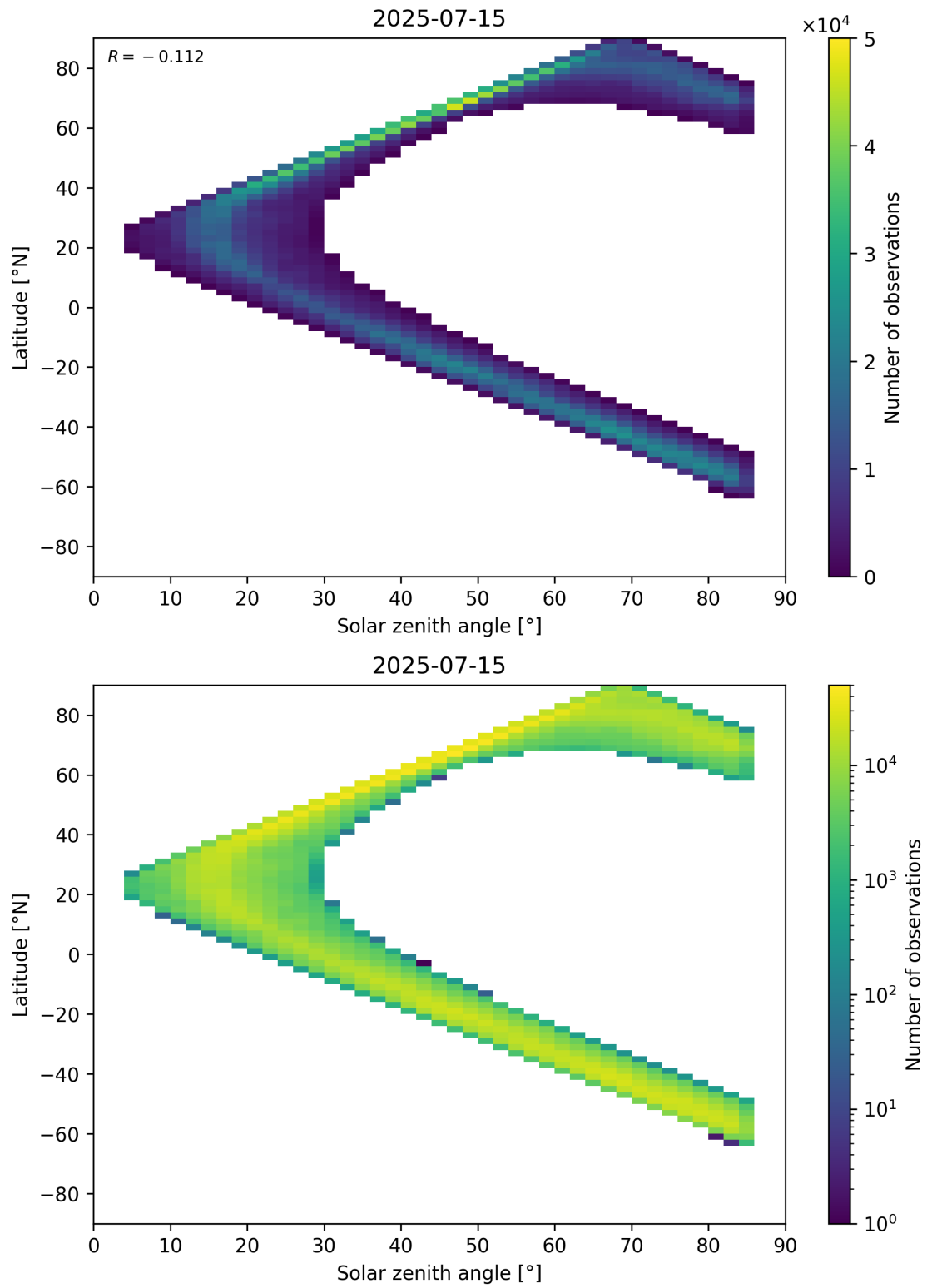
Figure 66: Scatter density plot of “Solar zenith angle” against “Latitude” for 2025-07-14 to 2025-07-16.
