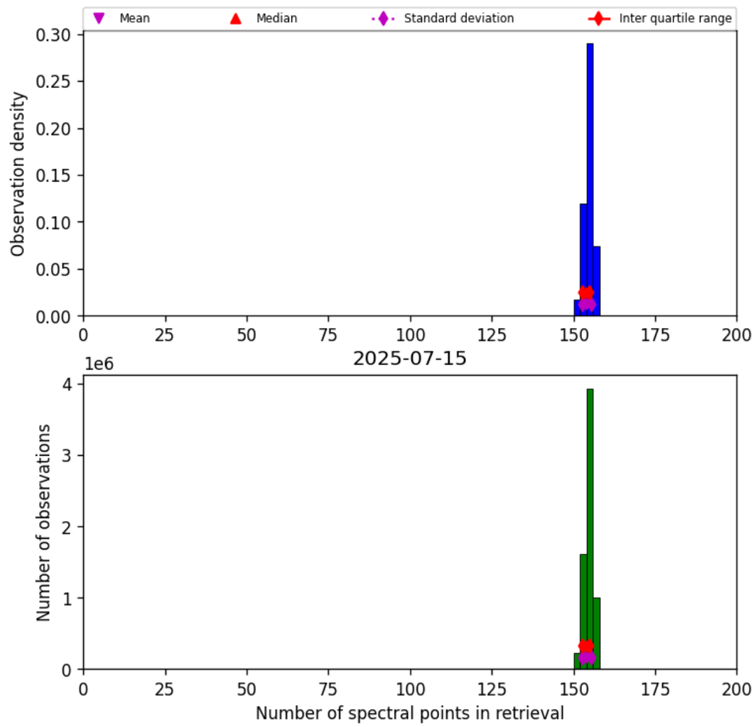
Figure 21: Histogram of "Number of spectral points in retrieval" for 2025-07-14 to 2025-07-16
