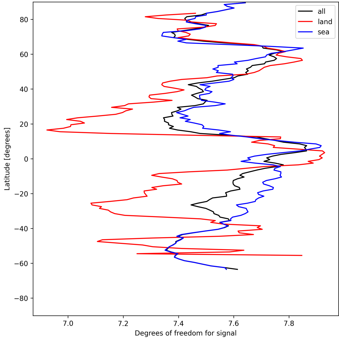
Figure 15: Zonal average of “Degrees of freedom for signal” for 2025-07-14 to 2025-07-16.
