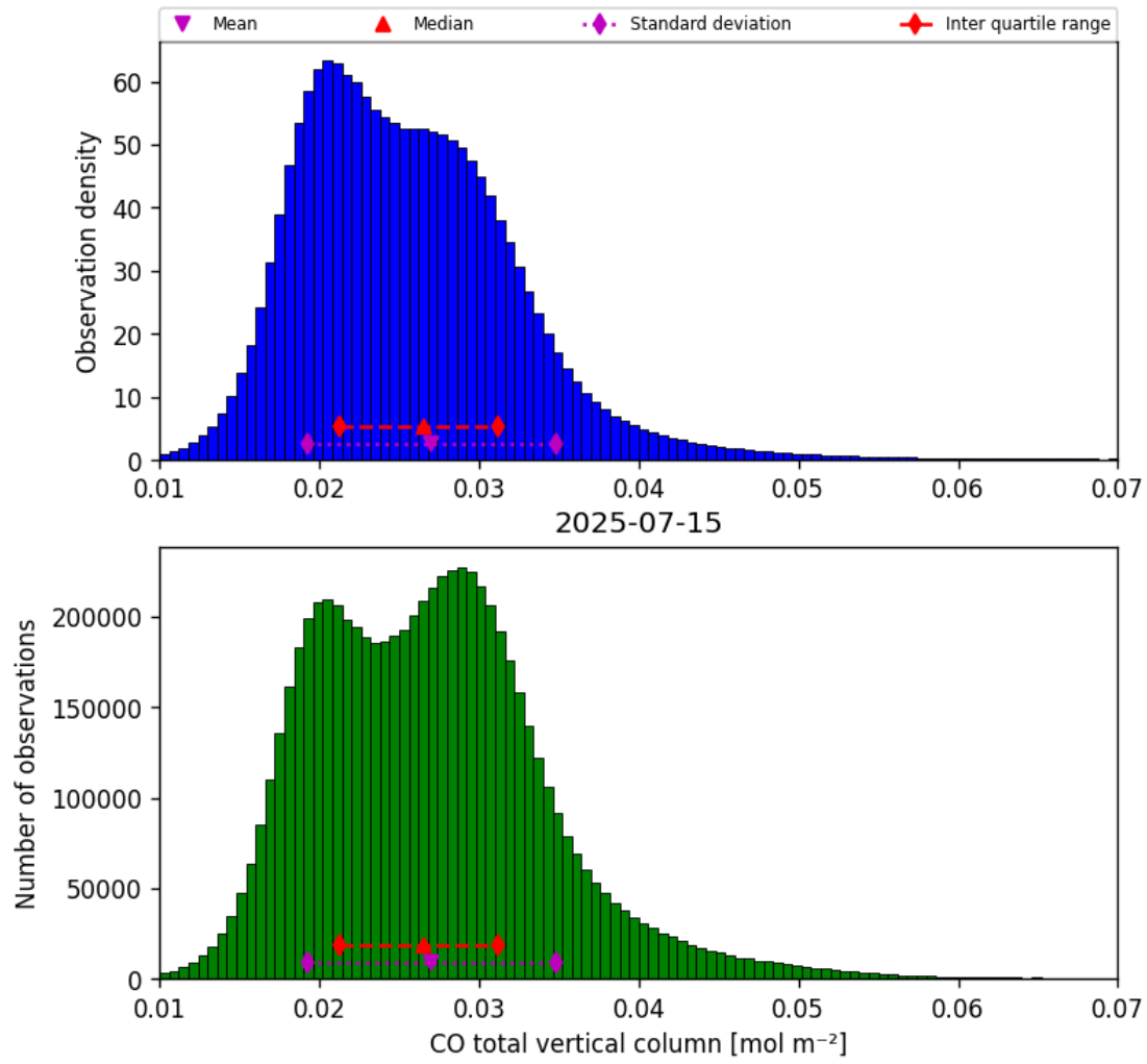
Figure 18: Histogram of “CO total vertical column” for 2025-07-14 to 2025-07-16
