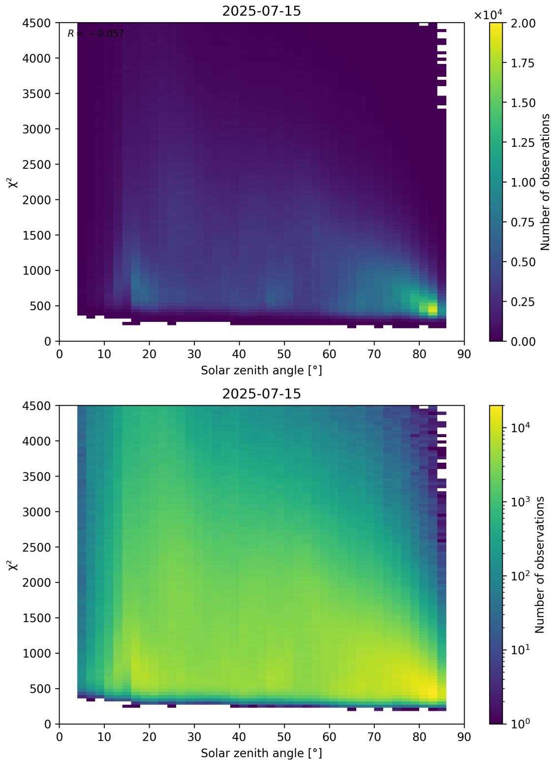
Figure 64: Scatter density plot of “Solar zenith angle” against “ \chi^2 ” for 2025-07-14 to 2025-07-16.
