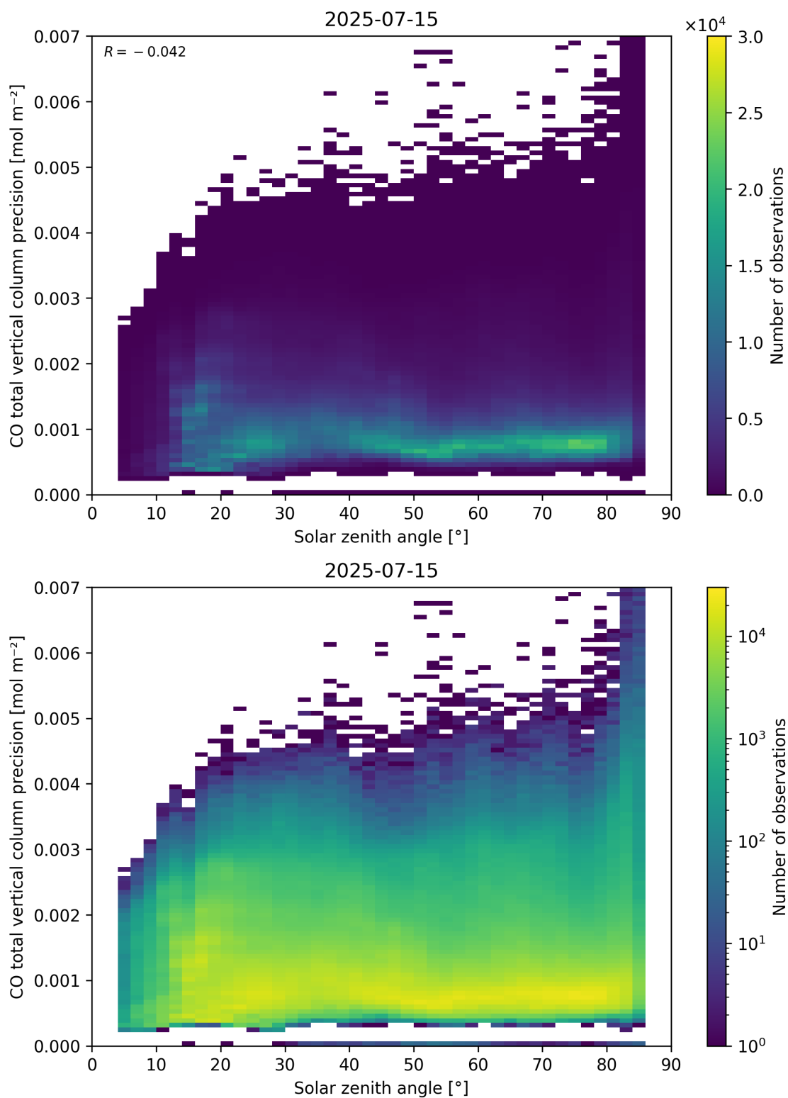
Figure 63: Scatter density plot of “Solar zenith angle” against “CO total vertical column precision” for 2025-07-14 to 2025-07-16.
