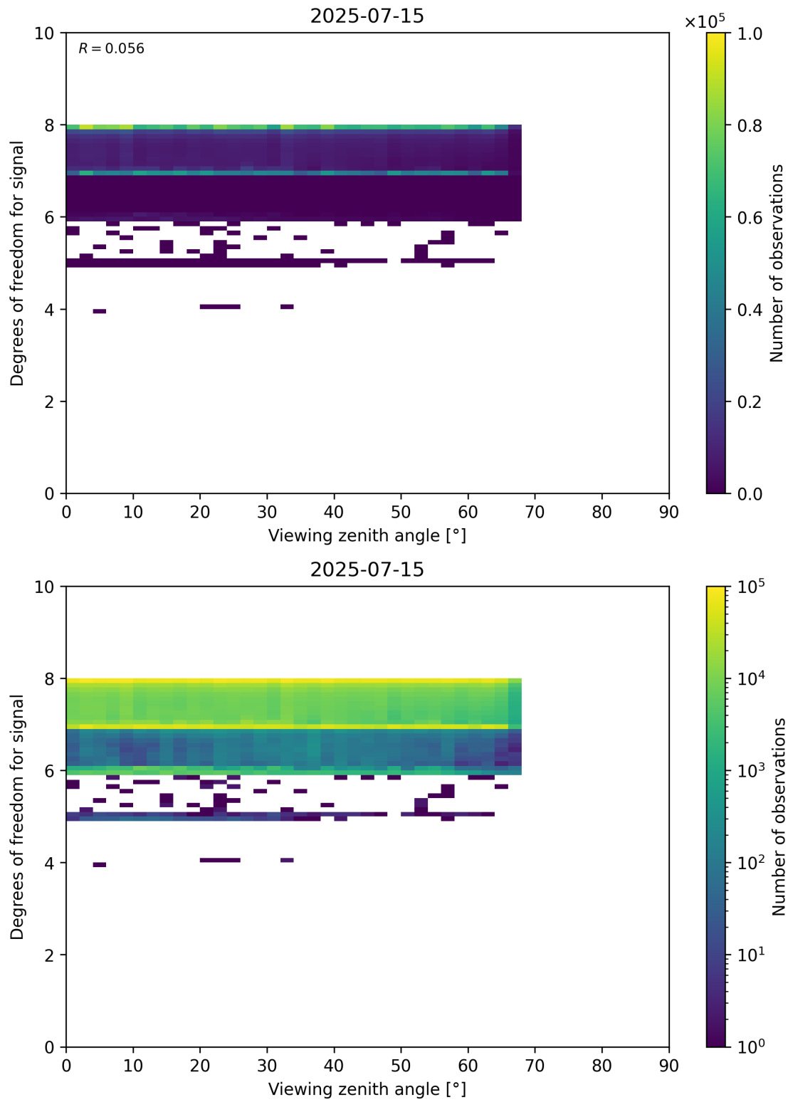
Figure 73: Scatter density plot of “Viewing zenith angle” against “Degrees of freedom for signal” for 2025-07-14 to 2025-07-16.
