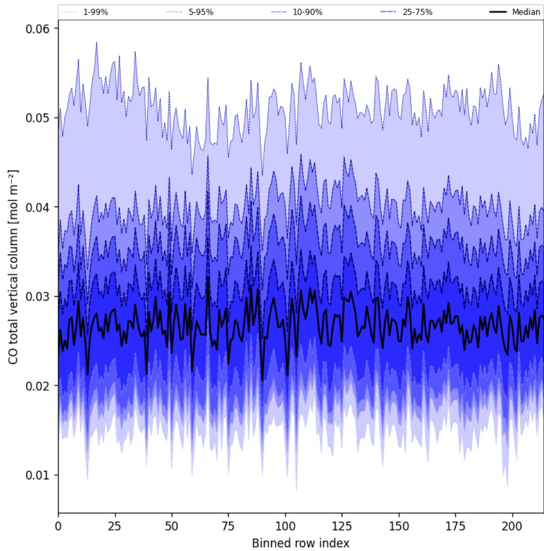
Figure 26: Along track statistics of “CO total vertical column” for 2025-07-14 to 2025-07-16
