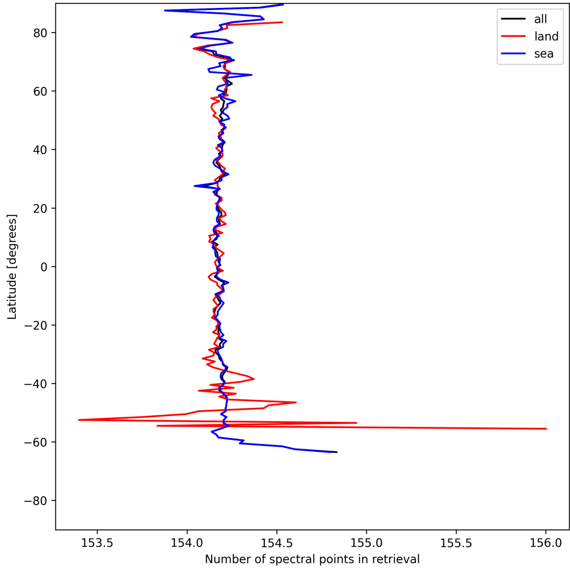
Figure 13: Zonal average of “Number of spectral points in retrieval” for 2025-07-14 to 2025-07-16.
