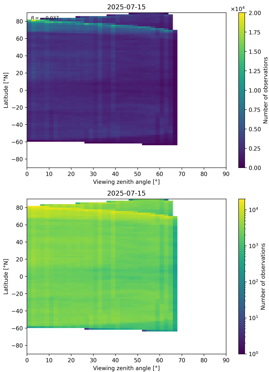
Figure 74: Scatter density plot of “Viewing zenith angle” against “Latitude” for 2025-07-14 to 2025-07-16.
