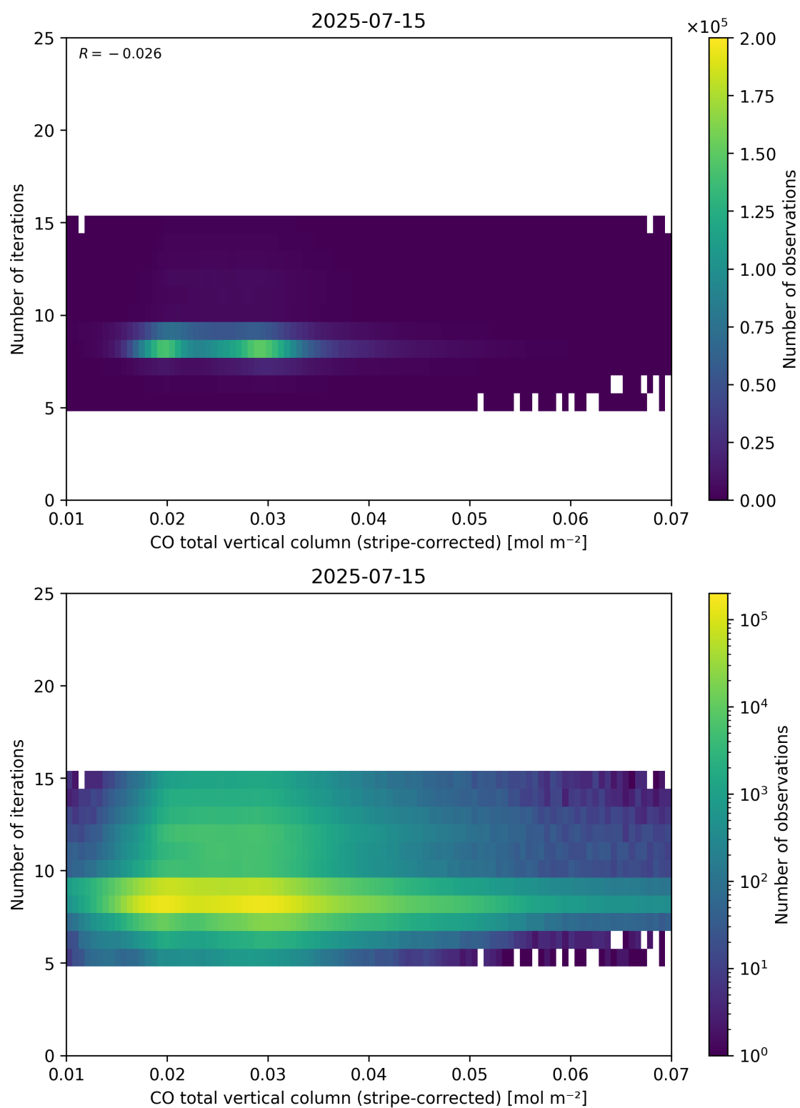
Figure 39: Scatter density plot of “CO total vertical column (stripe-corrected)” against “Number of iterations” for 2025-07-14 to 2025-07-16.
