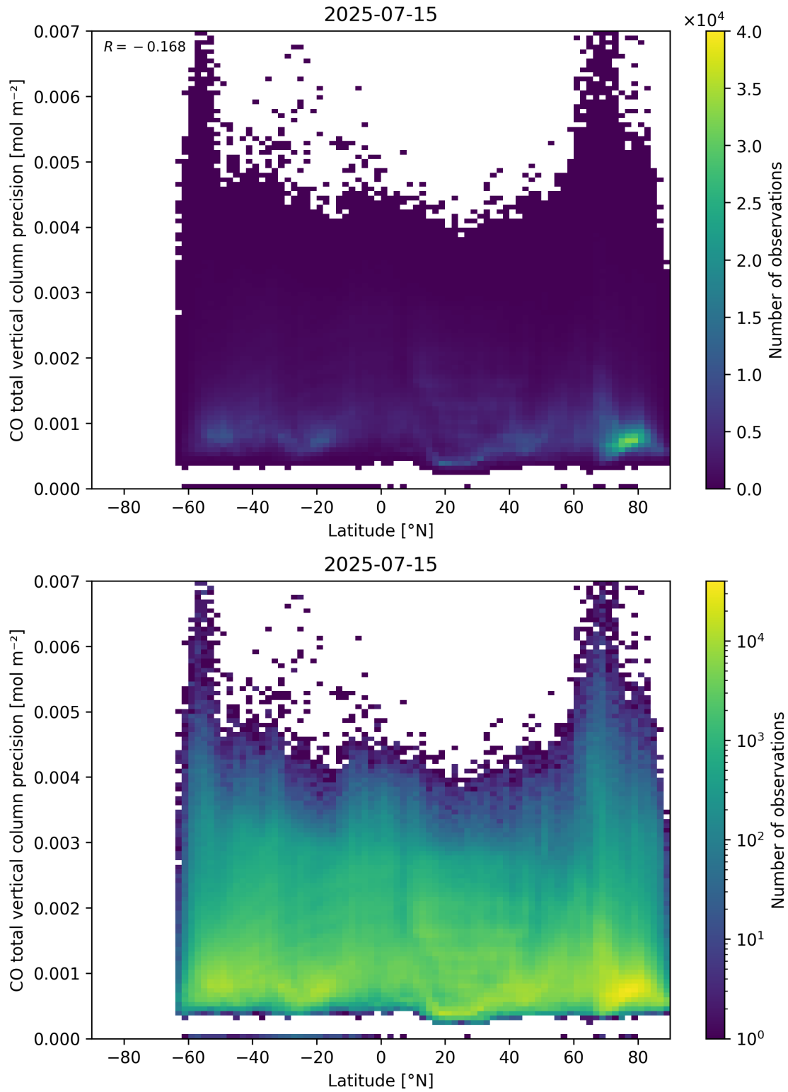
Figure 53: Scatter density plot of “Latitude” against “CO total vertical column precision” for 2025-07-14 to 2025-07-16.
