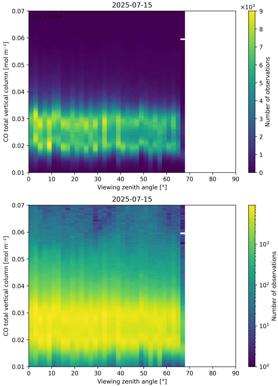
Figure 69: Scatter density plot of “Viewing zenith angle” against “CO total vertical column” for 2025-07-14 to 2025-07-16.
