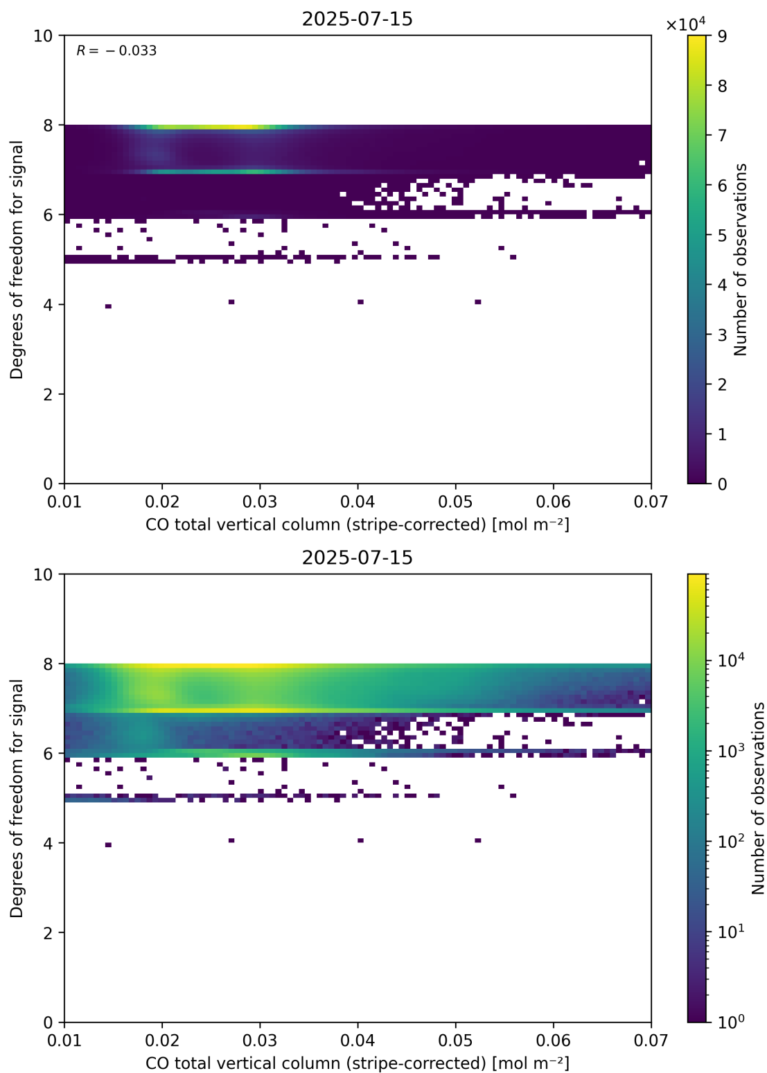
Figure 38: Scatter density plot of “CO total vertical column (stripe-corrected)” against “Degrees of freedom for signal” for 2025-07-14 to 2025-07-16.
