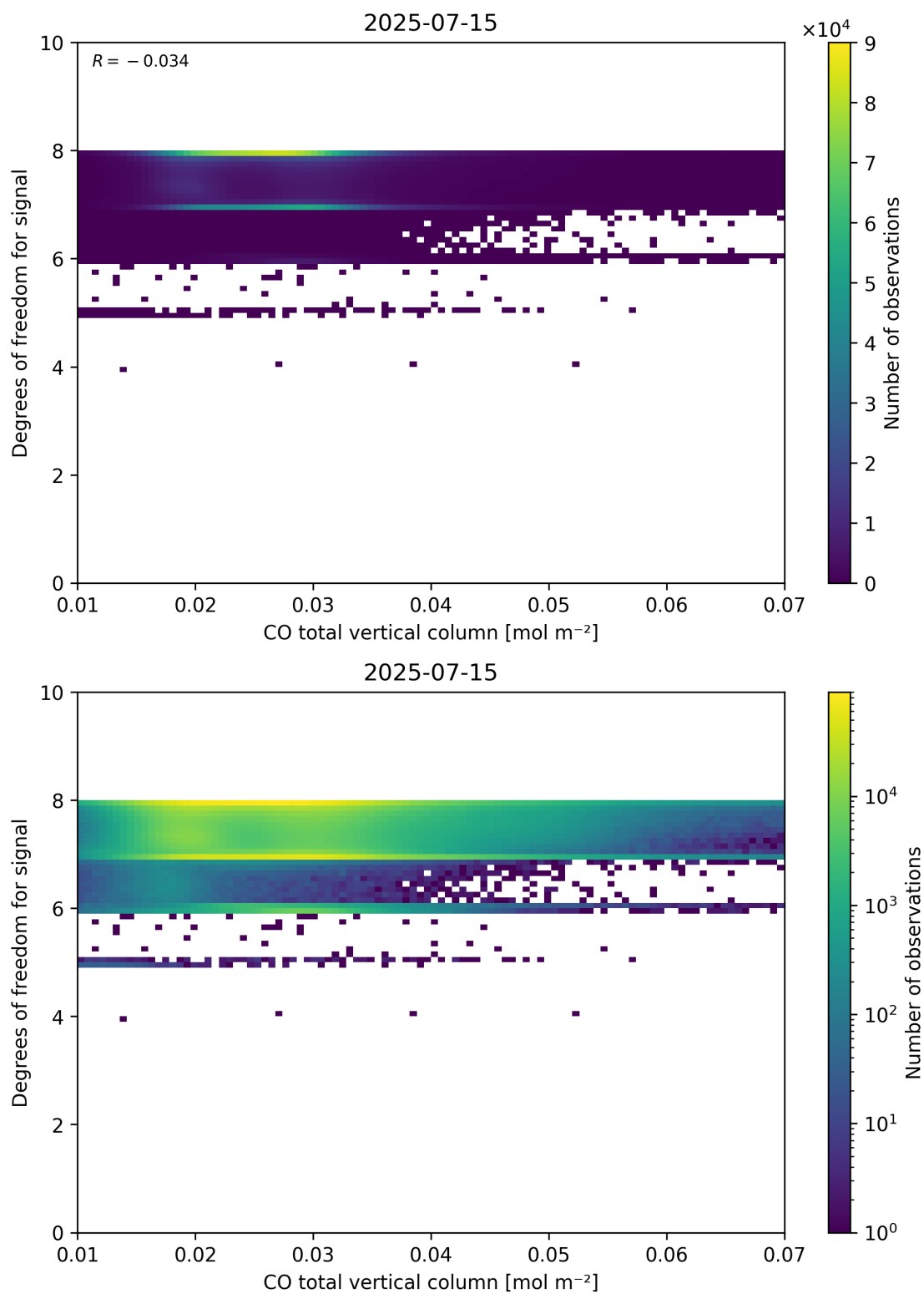
Figure 41: Scatter density plot of “CO total vertical column” against “Degrees of freedom for signal” for 2025-07-14 to 2025-07-16.
