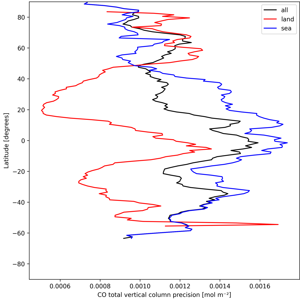
Figure 12: Zonal average of “CO total vertical column precision” for 2025-07-14 to 2025-07-16.
