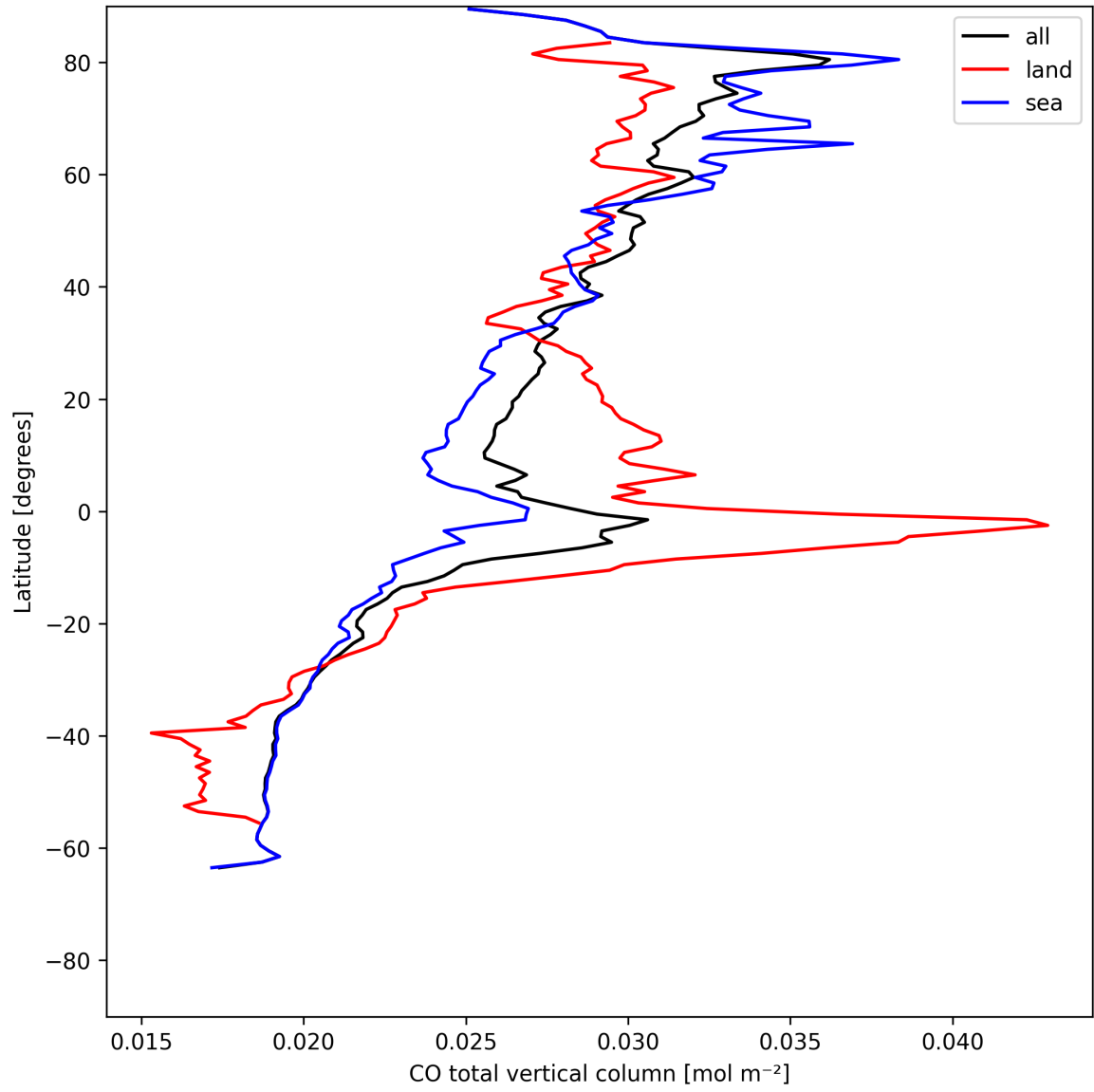
Figure 10: Zonal average of “CO total vertical column” for 2025-07-14 to 2025-07-16.
