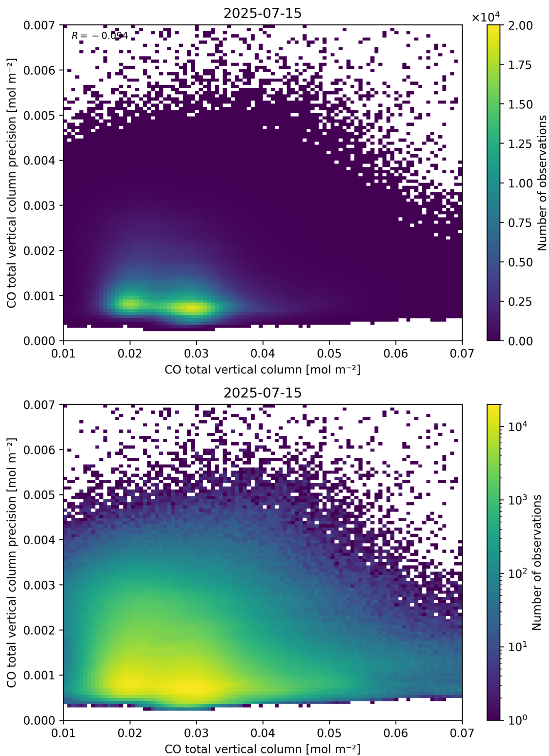
Figure 34: Scatter density plot of “CO total vertical column” against “CO total vertical column precision” for 2025-07-14 to 2025-07-16.
