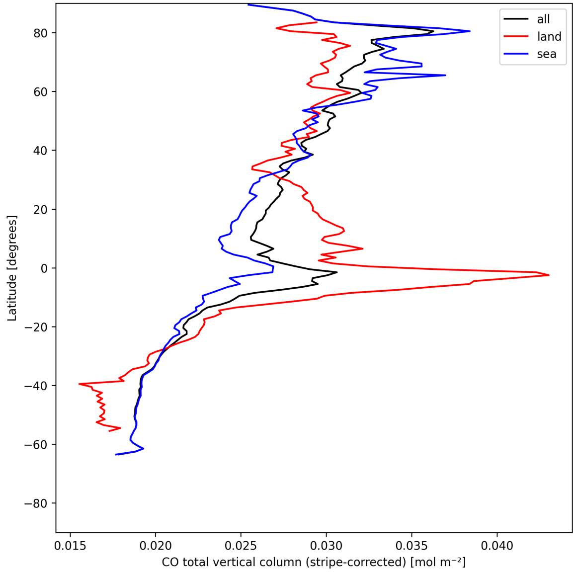
Figure 11: Zonal average of “CO total vertical column (stripe-corrected)” for 2025-07-14 to 2025-07-16.
