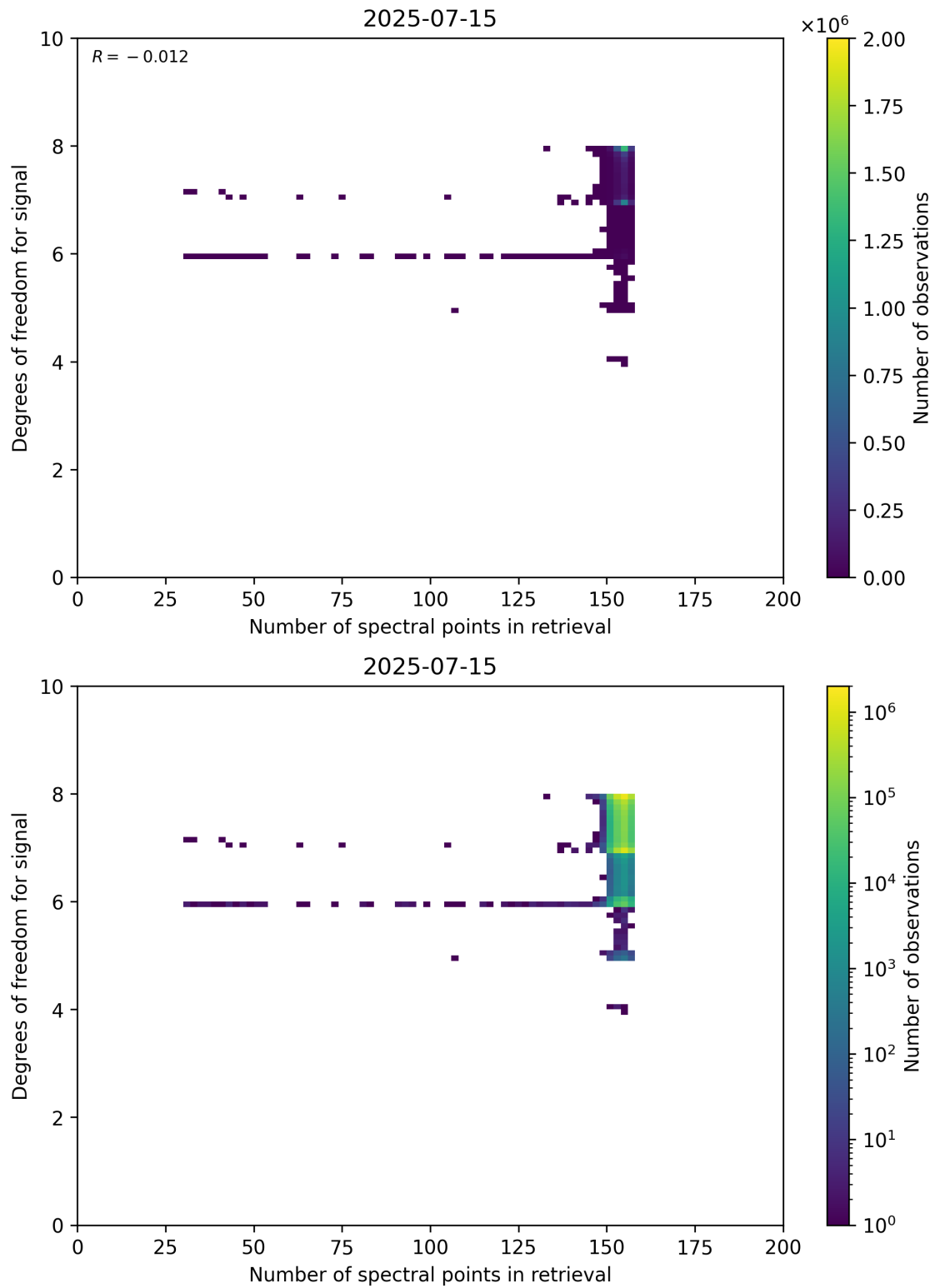
Figure 59: Scatter density plot of “Number of spectral points in retrieval” against “Degrees of freedom for signal” for 2025-07-14 to 2025-07-16.
