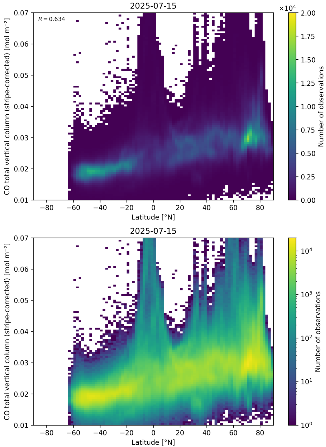
Figure 52: Scatter density plot of “Latitude” against “CO total vertical column (stripe-corrected)” for 2025-07-14 to 2025-07-16.
