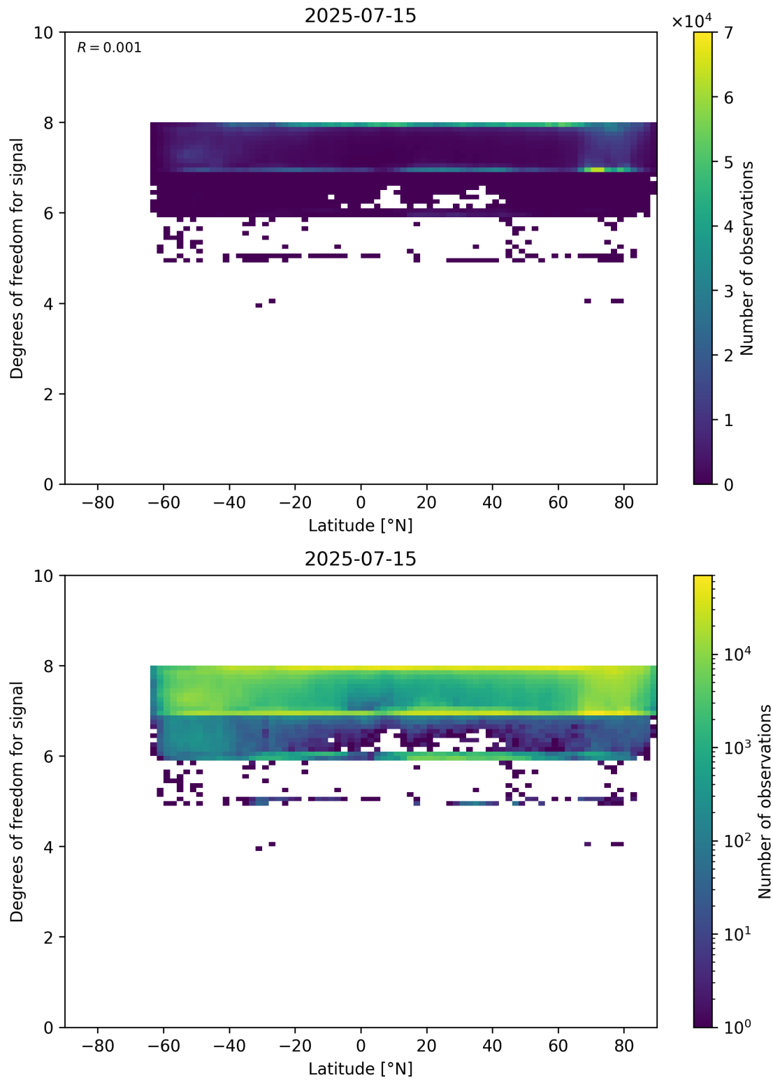
Figure 55: Scatter density plot of “Latitude” against “Degrees of freedom for signal” for 2025-07-14 to 2025-07-16.
