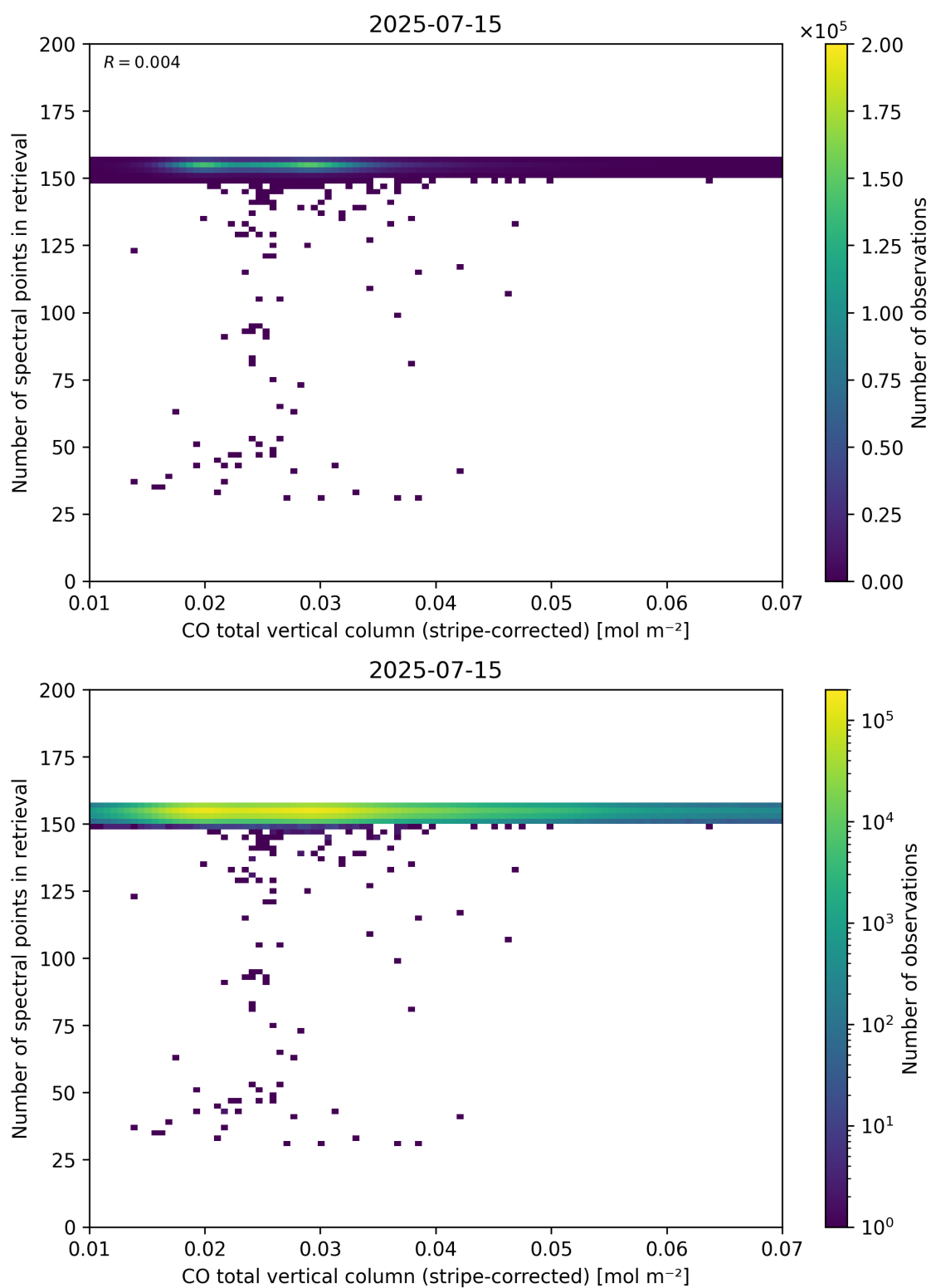
Figure 40: Scatter density plot of “CO total vertical column (stripe-corrected)” against “Number of spectral points in retrieval” for 2025-07-14 to 2025-07-16.
