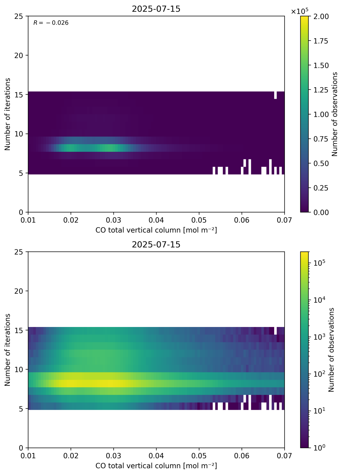
Figure 42: Scatter density plot of “CO total vertical column” against “Number of iterations” for 2025-07-14 to 2025-07-16.
