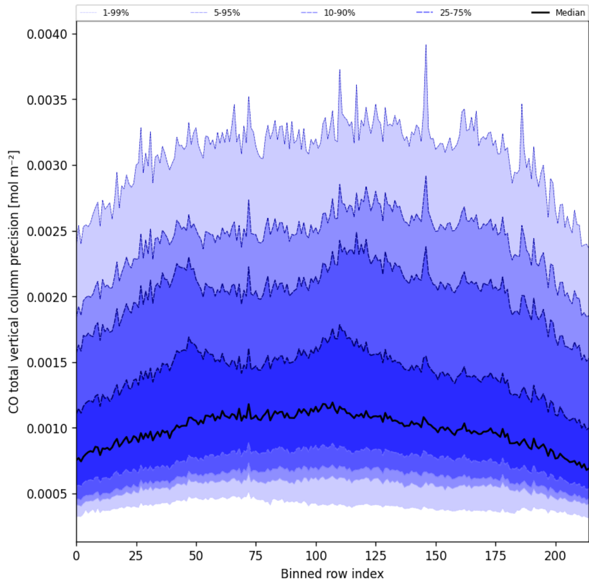
Figure 28: Along track statistics of “CO total vertical column precision” for 2025-07-14 to 2025-07-16
