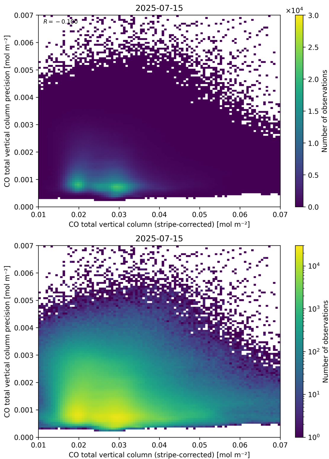
Figure 36: Scatter density plot of “CO total vertical column (stripe-corrected)” against “CO total vertical column precision” for 2025-07-14 to 2025-07-16.
