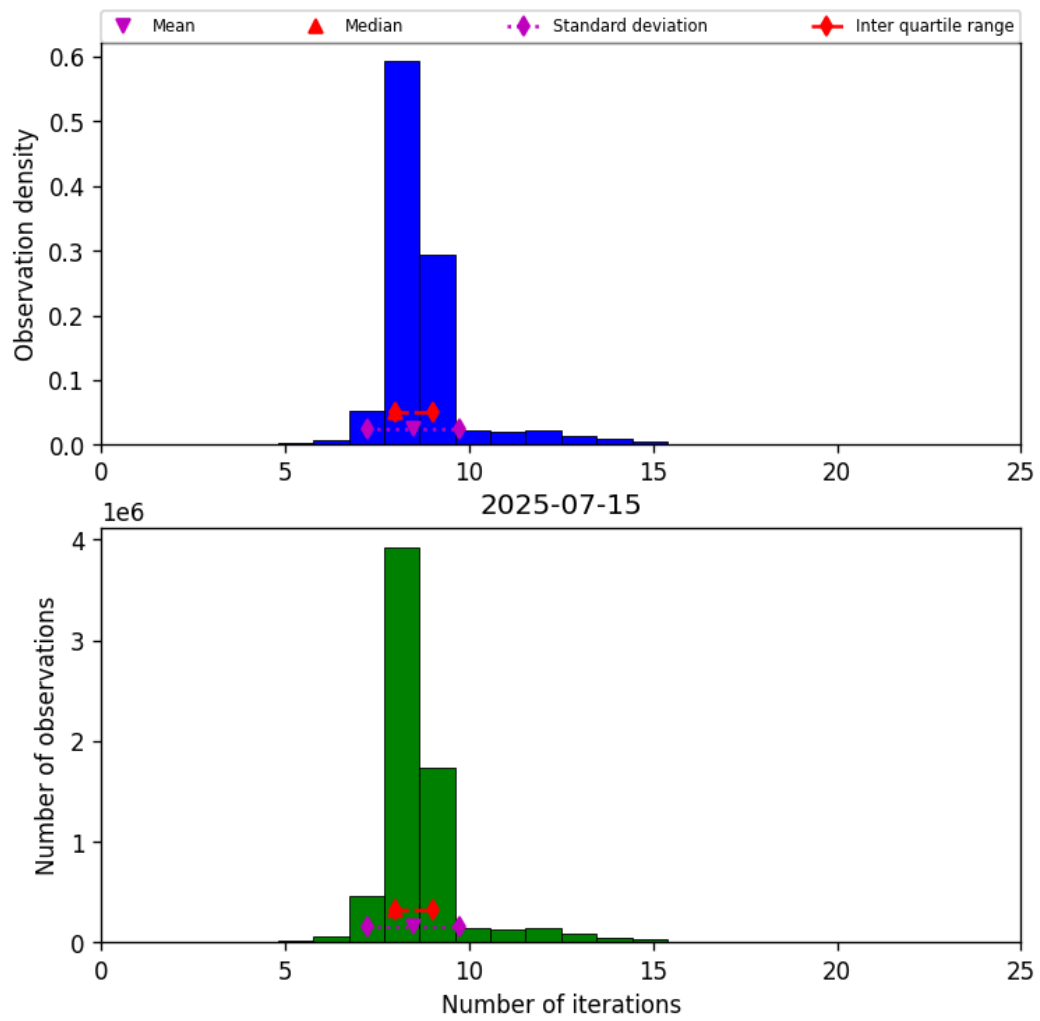
Figure 24: Histogram of “Number of iterations” for 2025-07-14 to 2025-07-16
