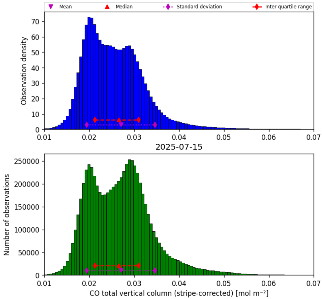
Figure 19: Histogram of “CO total vertical column (stripe-corrected)” for 2025-07-14 to 2025-07-16
