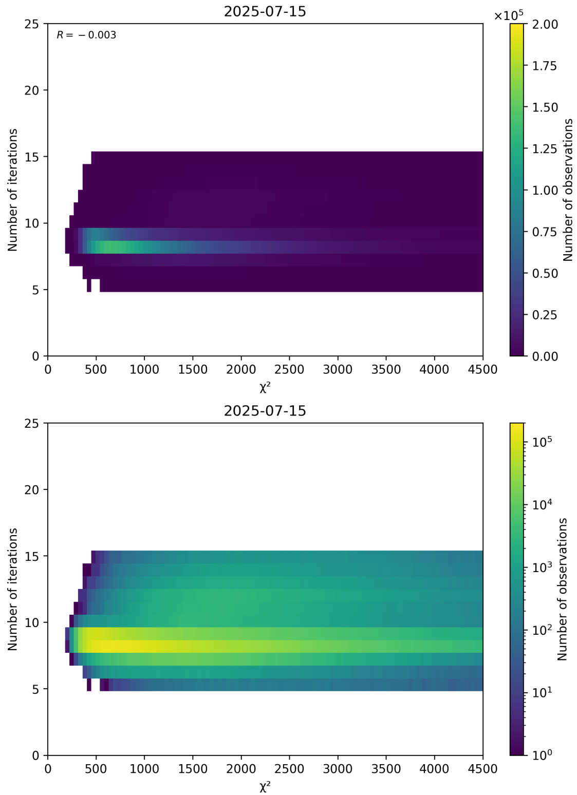
Figure 49: Scatter density plot of “ \chi^2 ” against “Number of iterations” for 2025-07-14 to 2025-07-16.
