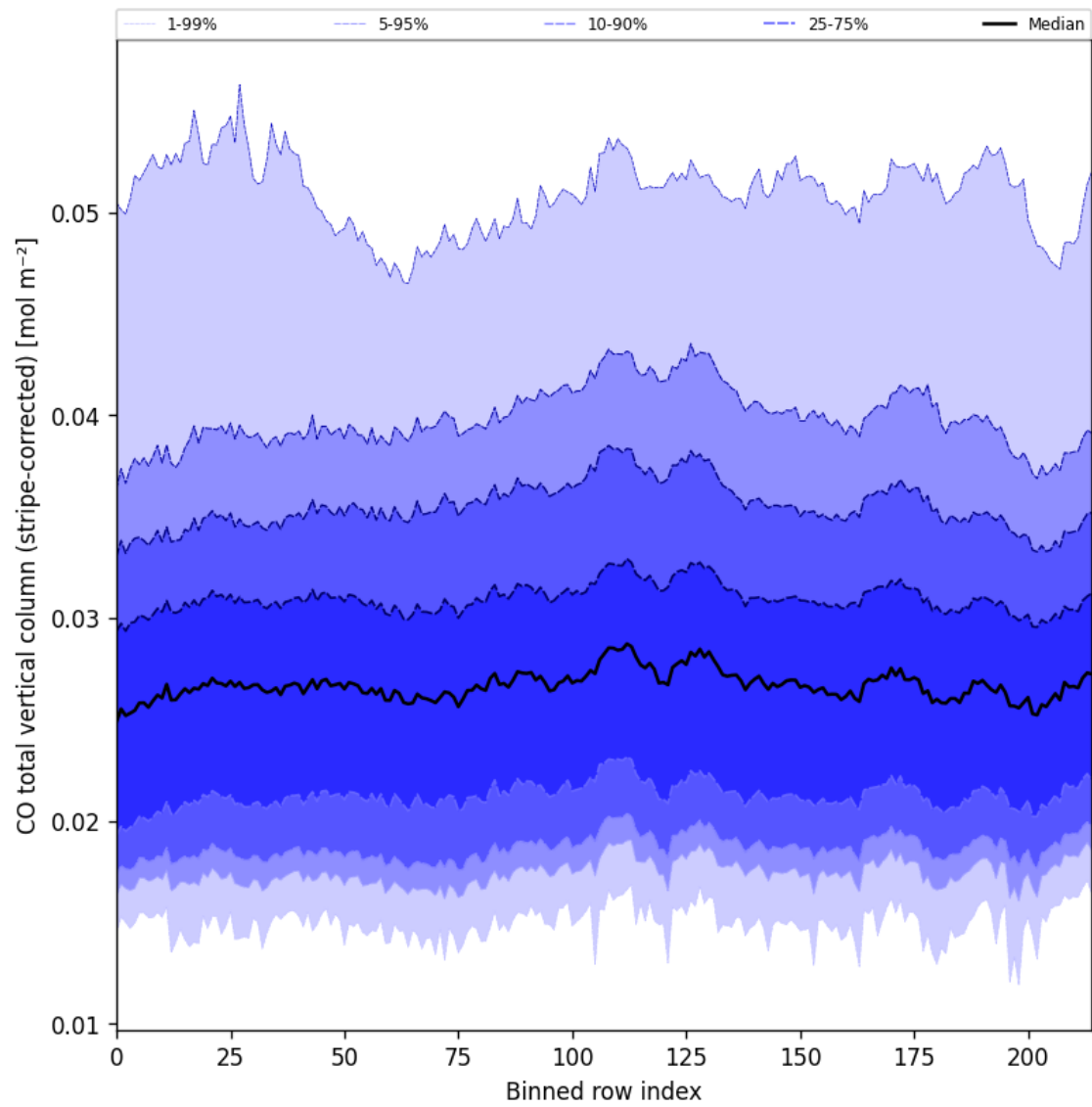
Figure 27: Along track statistics of “CO total vertical column (stripe-corrected)” for 2025-07-14 to 2025-07-16
