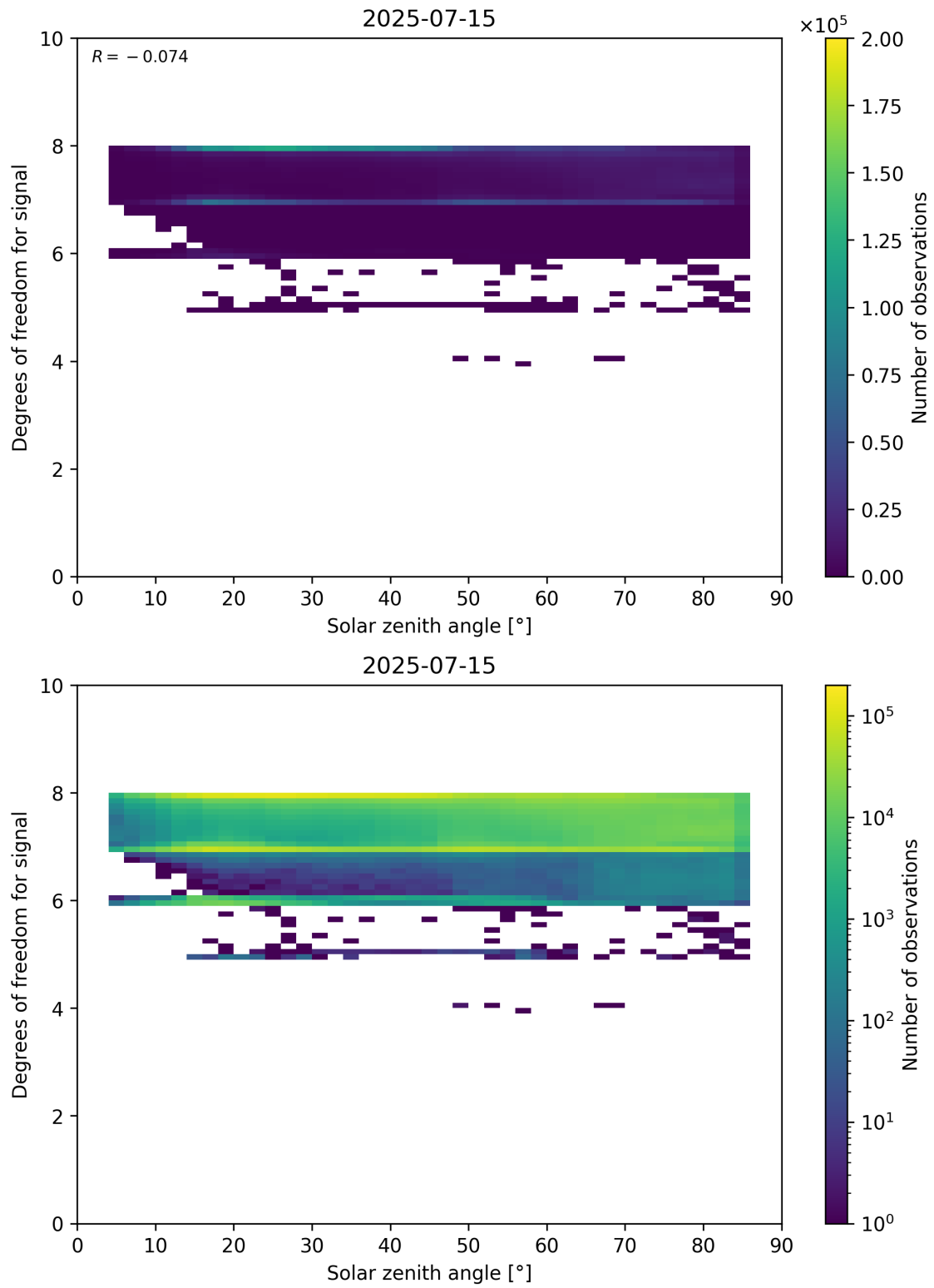
Figure 65: Scatter density plot of “Solar zenith angle” against “Degrees of freedom for signal” for 2025-07-14 to 2025-07-16.
