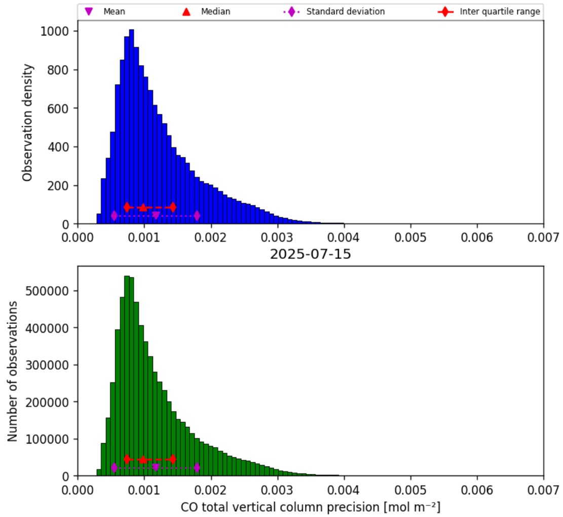
Figure 20: Histogram of “CO total vertical column precision” for 2025-07-14 to 2025-07-16
