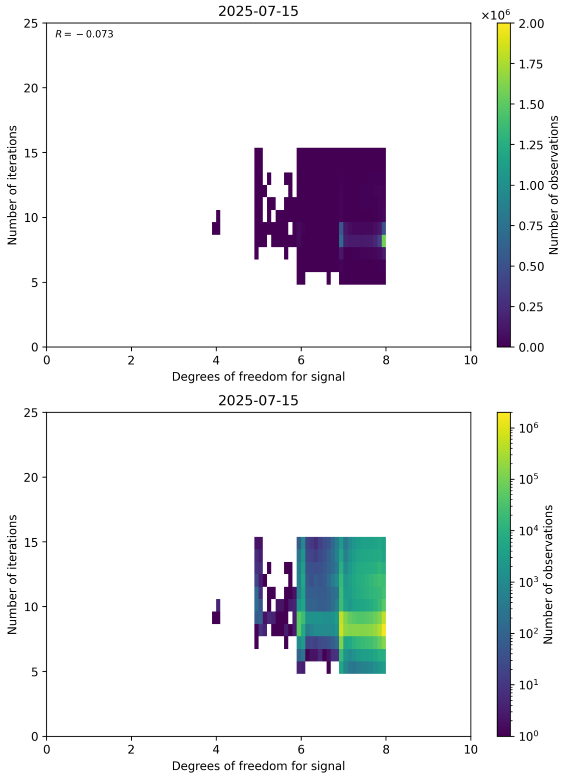
Figure 50: Scatter density plot of “Degrees of freedom for signal” against “Number of iterations” for 2025-07-14 to 2025-07-16.
