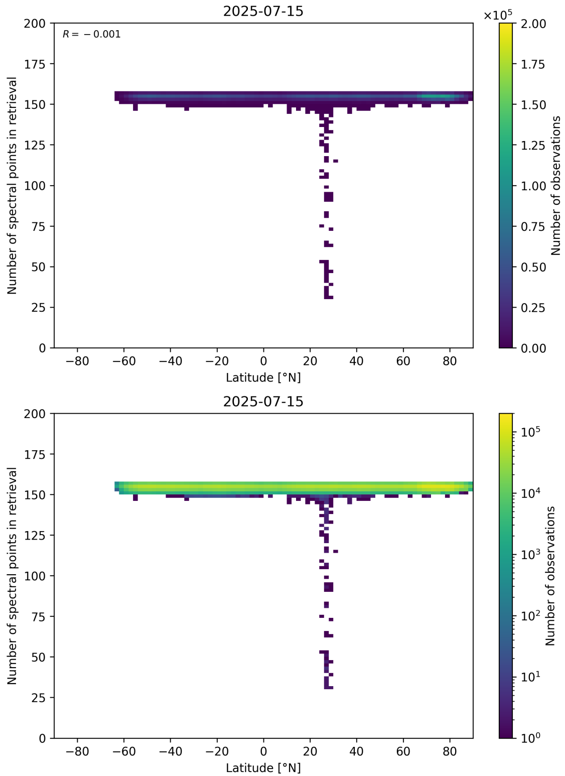
Figure 57: Scatter density plot of “Latitude” against “Number of spectral points in retrieval” for 2025-07-14 to 2025-07-16.
