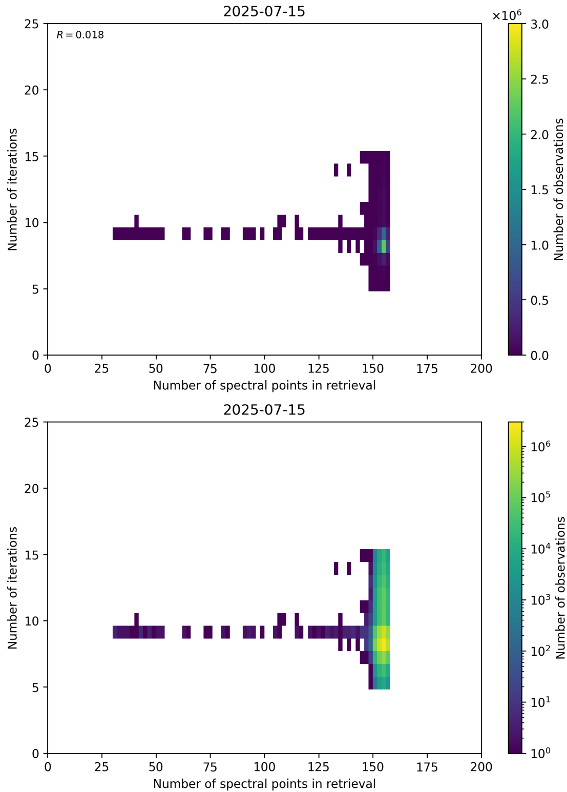
Figure 60: Scatter density plot of “Number of spectral points in retrieval” against “Number of iterations” for 2025-07-14 to 2025-07-16.
