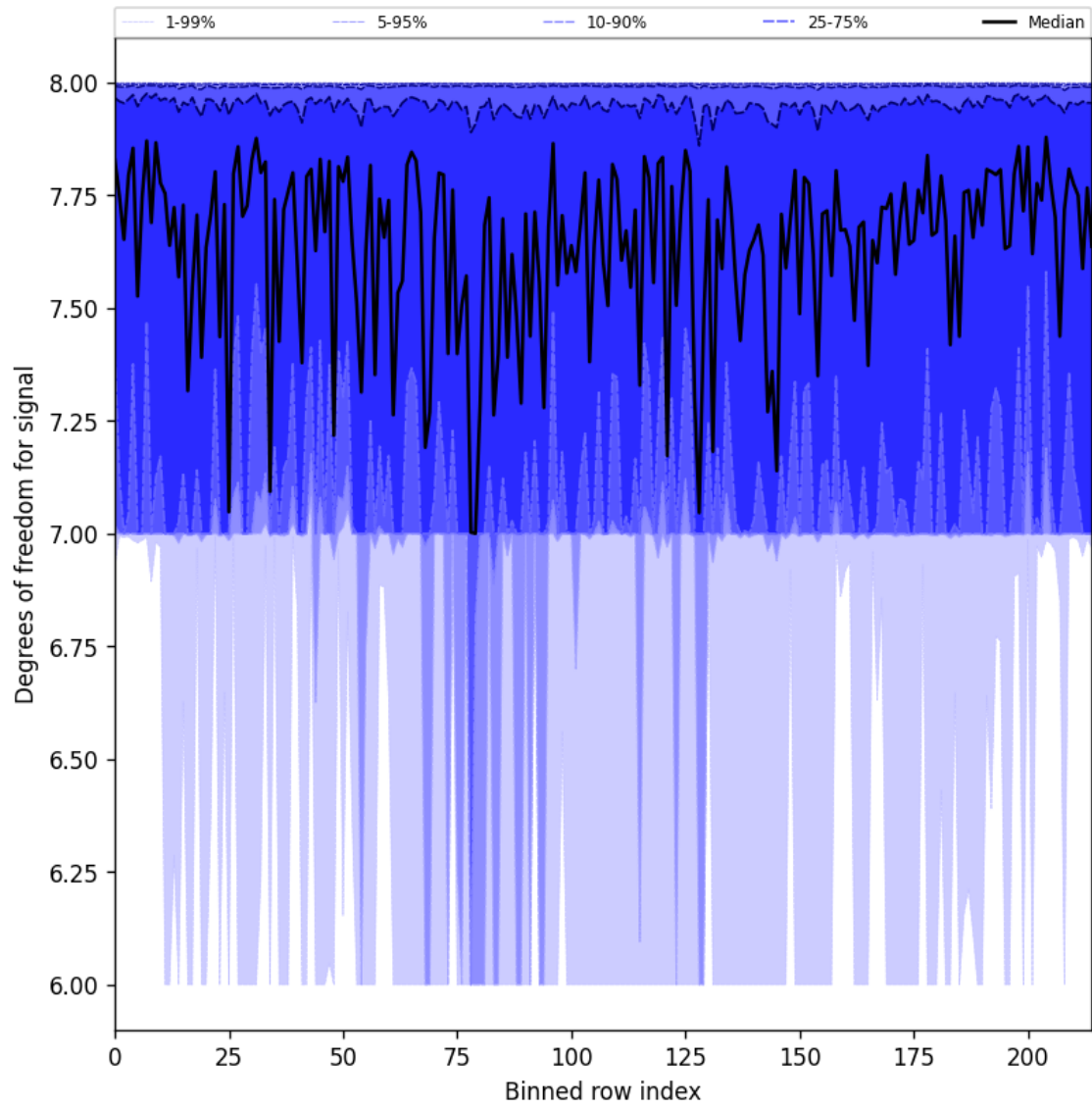
Figure 31: Along track statistics of “Degrees of freedom for signal” for 2025-07-14 to 2025-07-16
