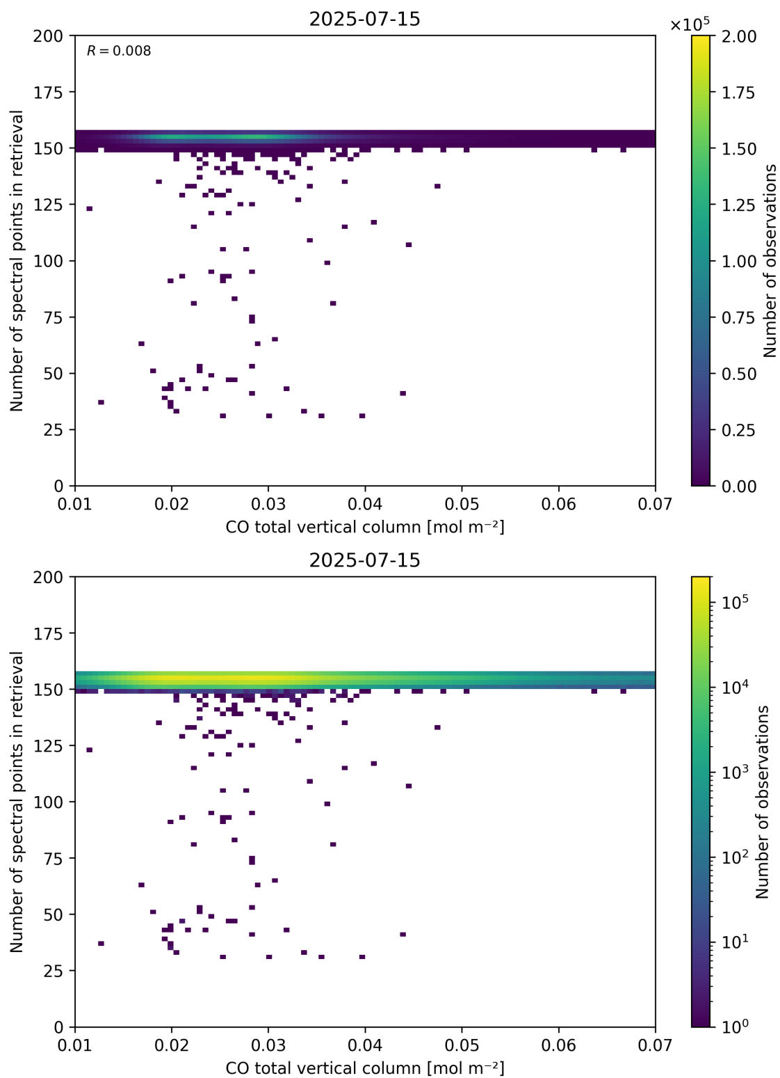
Figure 43: Scatter density plot of “CO total vertical column” against “Number of spectral points in retrieval” for 2025-07-14 to 2025-07-16.
