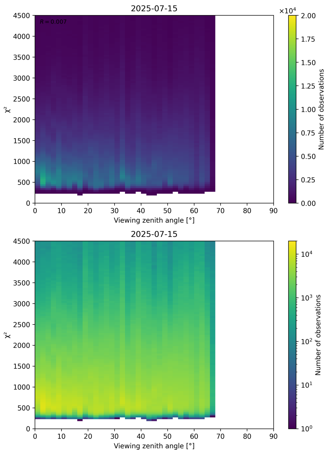
Figure 72: Scatter density plot of “Viewing zenith angle” against “ \chi^2 ” for 2025-07-14 to 2025-07-16.
