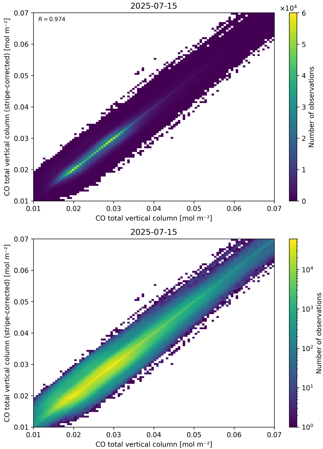
Figure 33: Scatter density plot of “CO total vertical column” against “CO total vertical column (stripe-corrected)” for 2025-07-14 to 2025-07-16.
