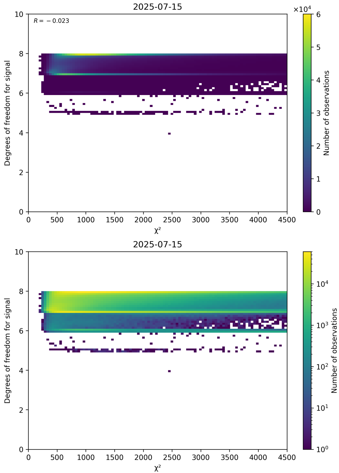
Figure 48: Scatter density plot of “ \chi^2 ” against “Degrees of freedom for signal” for 2025-07-14 to 2025-07-16.
