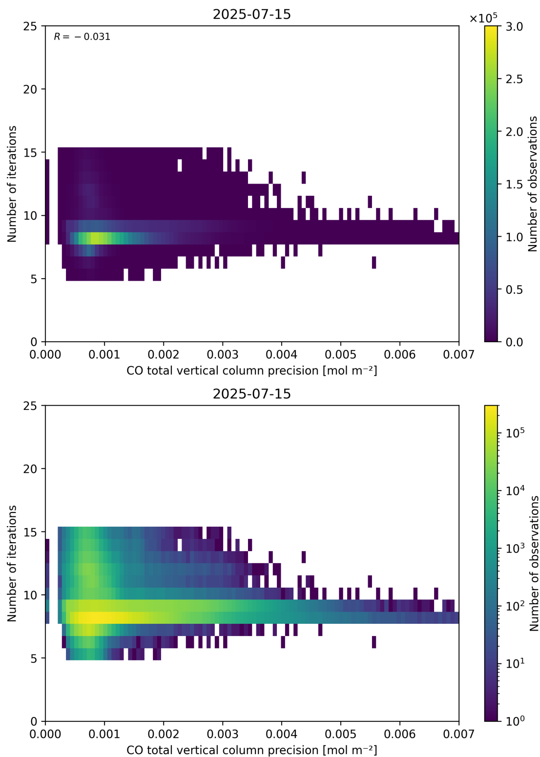
Figure 46: Scatter density plot of “CO total vertical column precision” against “Number of iterations” for 2025-07-14 to 2025-07-16.
