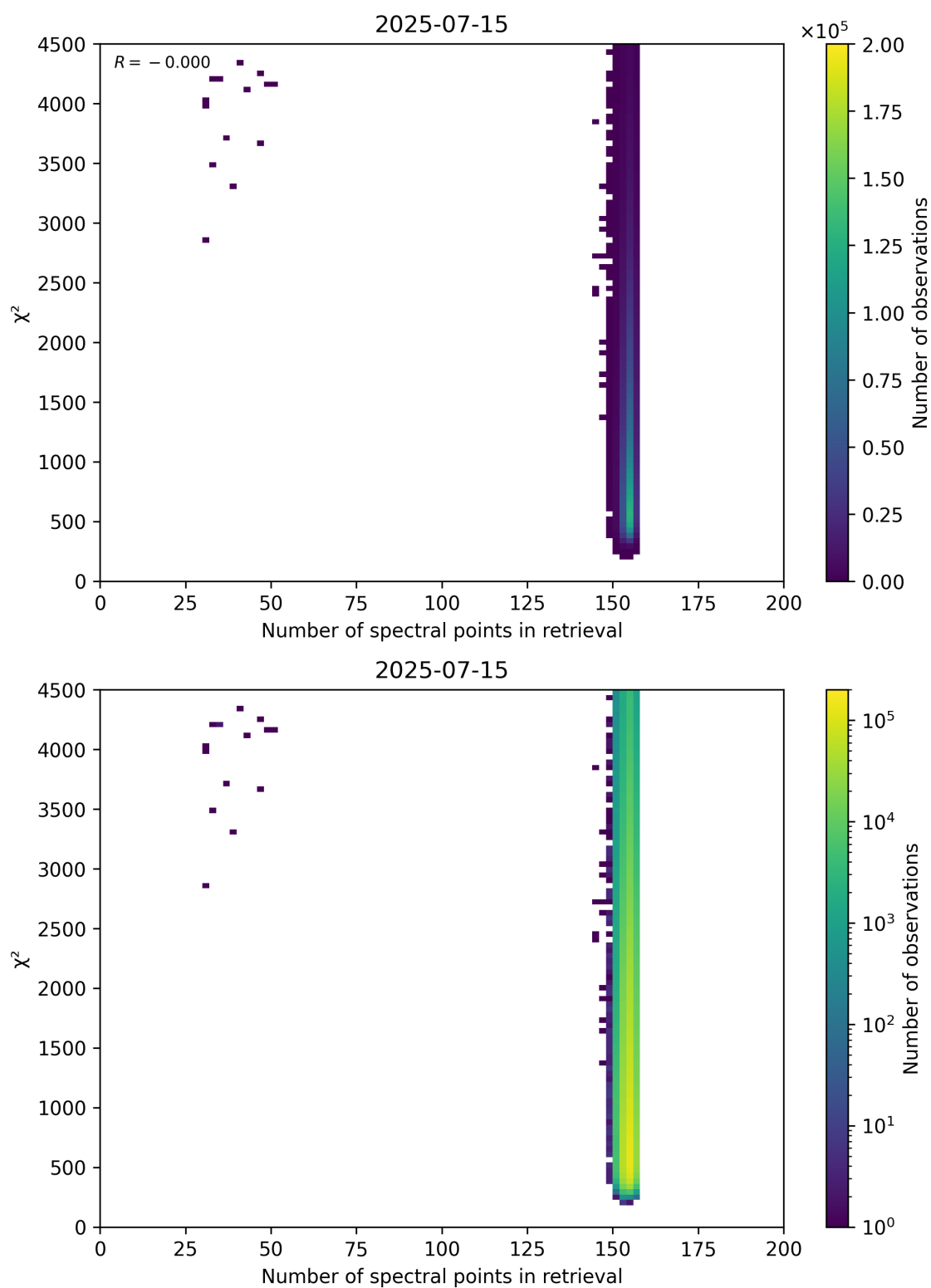
Figure 58: Scatter density plot of “Number of spectral points in retrieval” against “ \chi^2 ” for 2025-07-14 to 2025-07-16.
