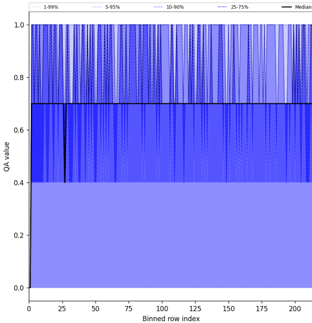
Figure 25: Along track statistics of “QA value” for 2025-07-14 to 2025-07-16
