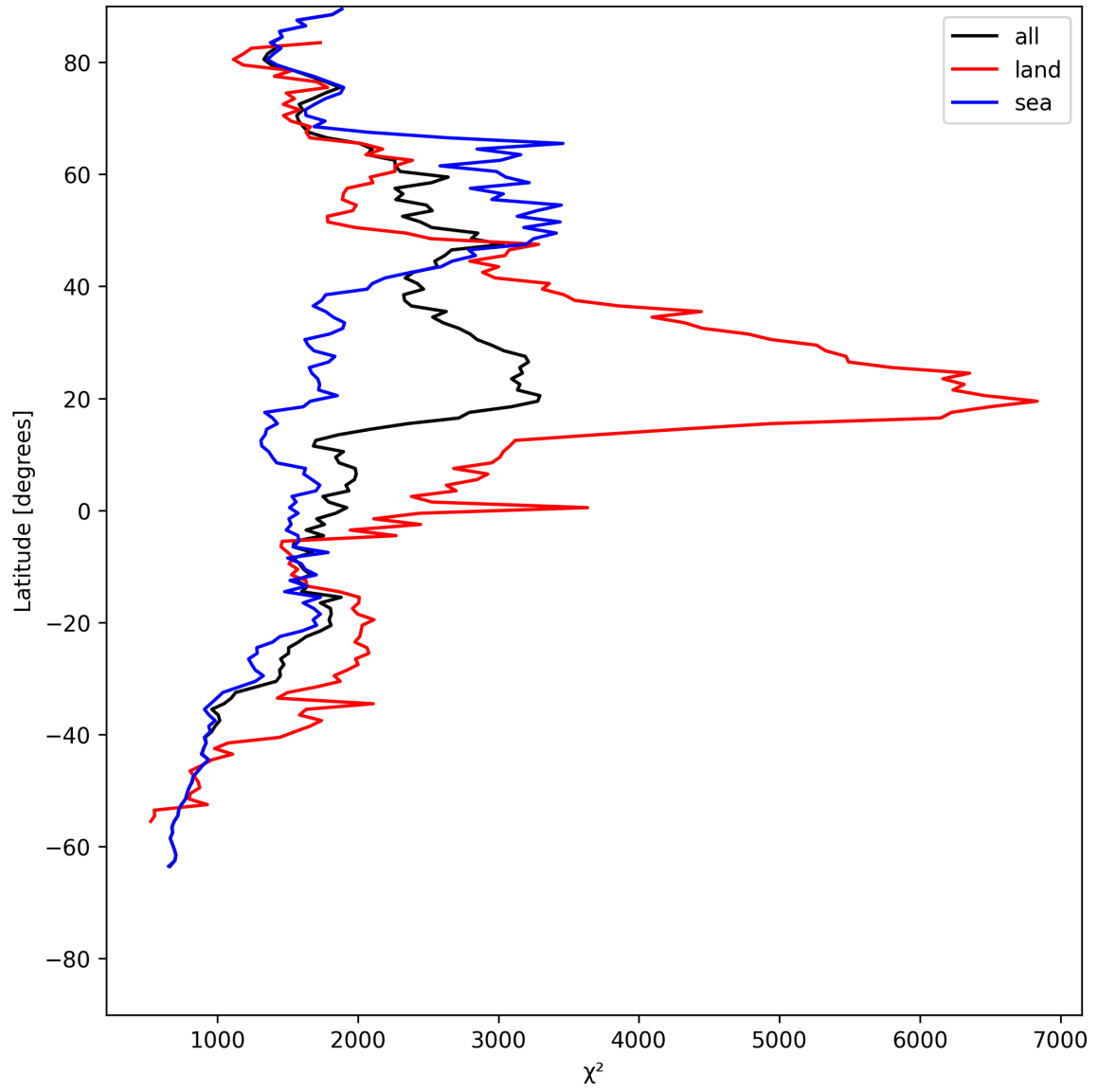
Figure 14: Zonal average of “ \chi^2 ” for 2025-07-14 to 2025-07-16.
