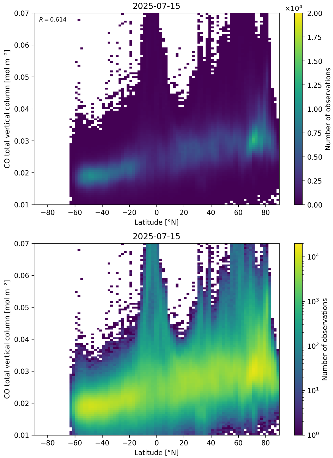
Figure 51: Scatter density plot of “Latitude” against “CO total vertical column” for 2025-07-14 to 2025-07-16.
