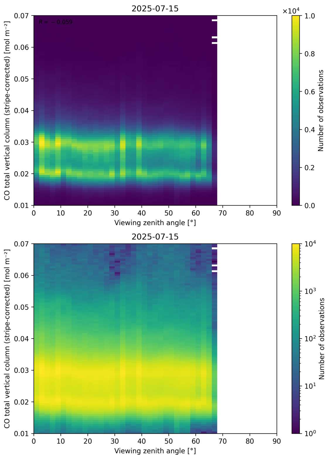
Figure 70: Scatter density plot of “Viewing zenith angle” against “CO total vertical column (stripe-corrected)” for 2025-07-14 to 2025-07-16.
