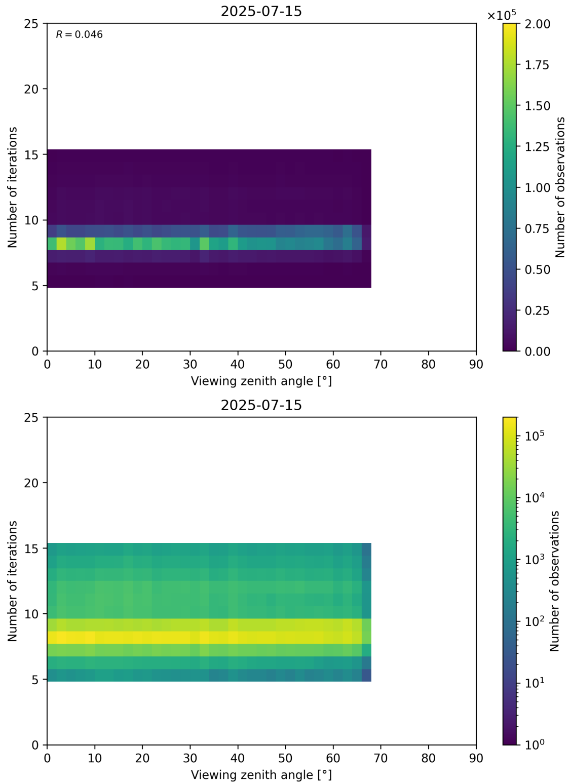
Figure 75: Scatter density plot of “Viewing zenith angle” against “Number of iterations” for 2025-07-14 to 2025-07-16.
