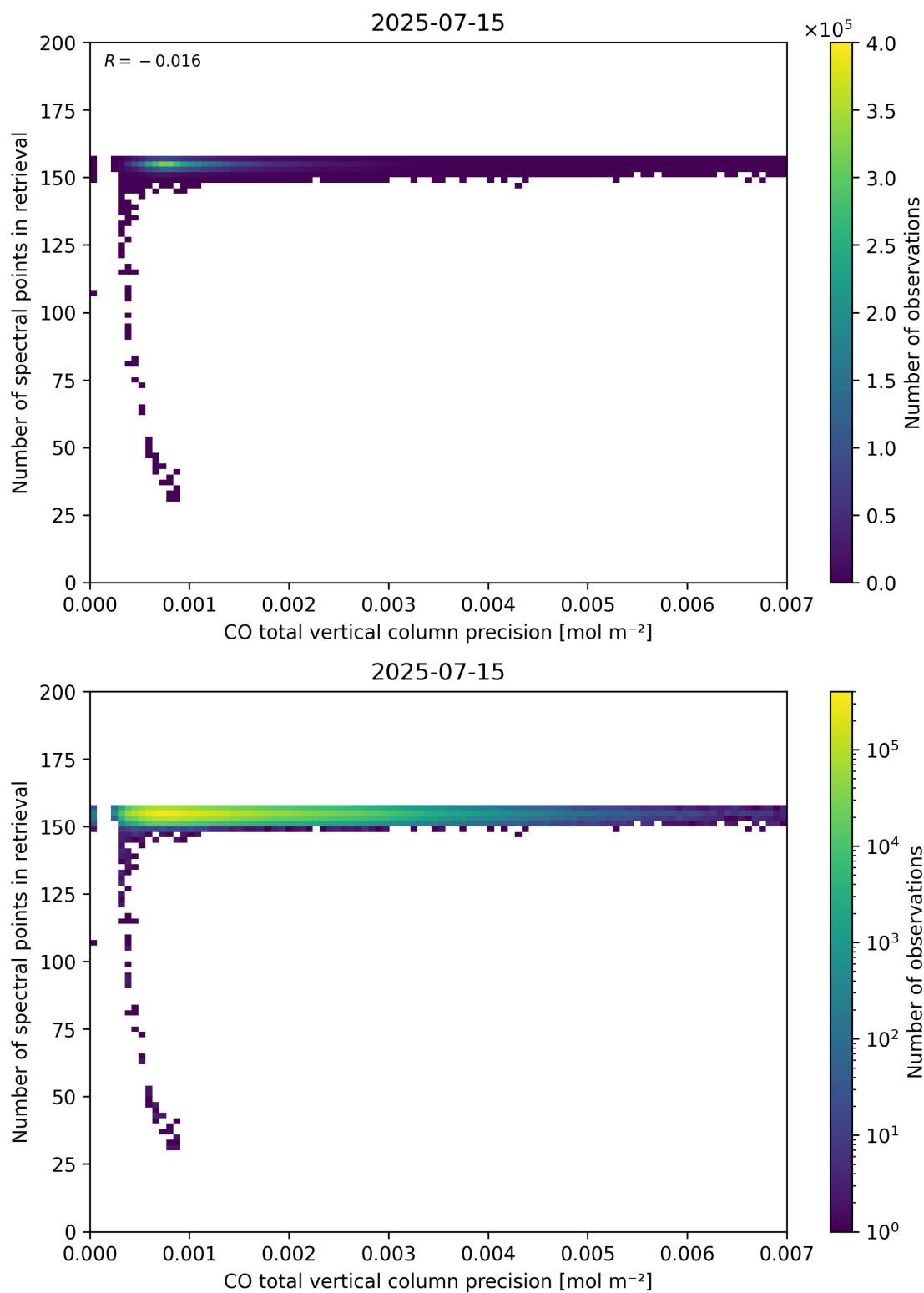
Figure 47: Scatter density plot of “CO total vertical column precision” against “Number of spectral points in retrieval” for 2025-07-14 to 2025-07-16.
