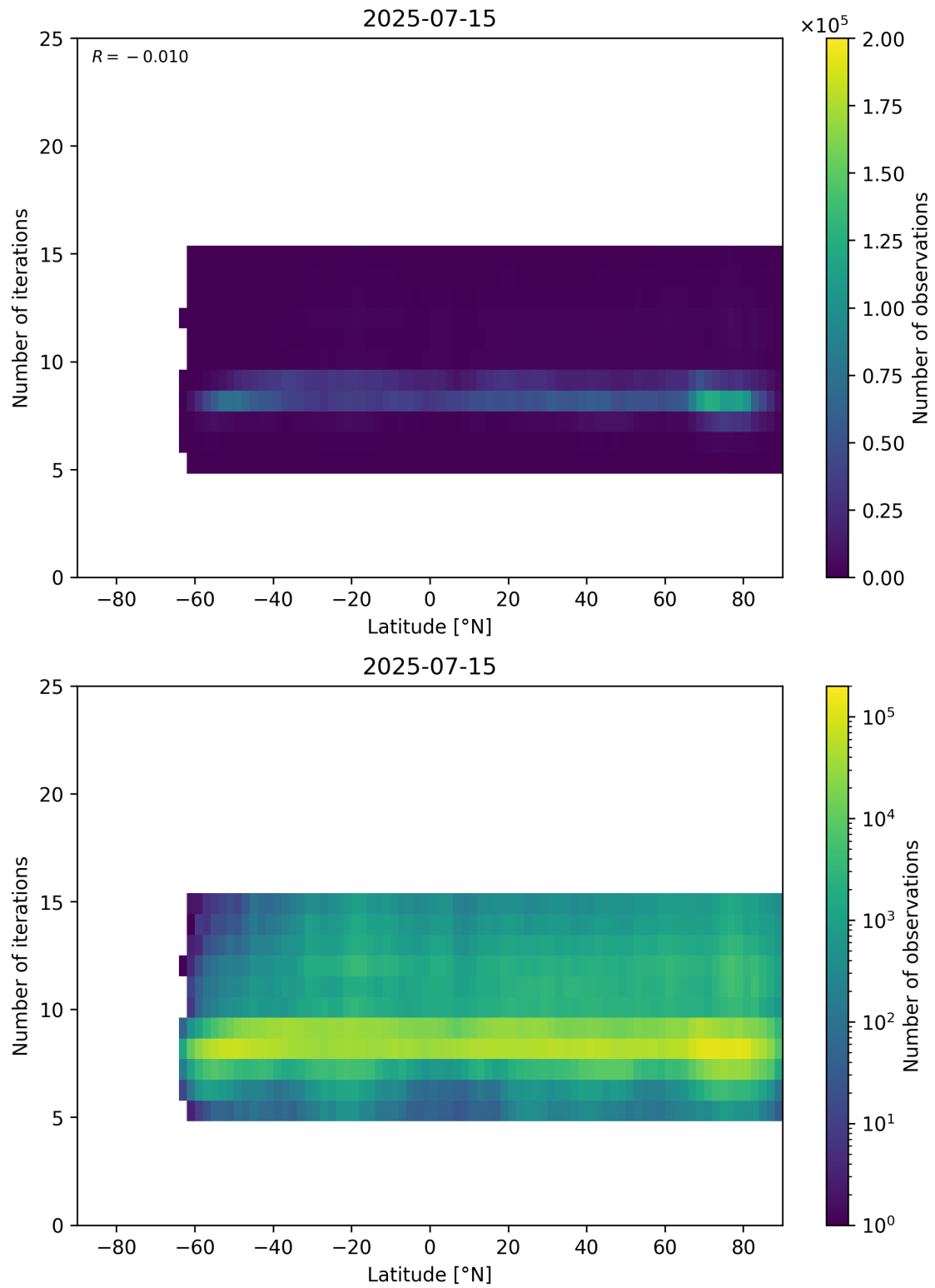
Figure 56: Scatter density plot of “Latitude” against “Number of iterations” for 2025-07-14 to 2025-07-16.
