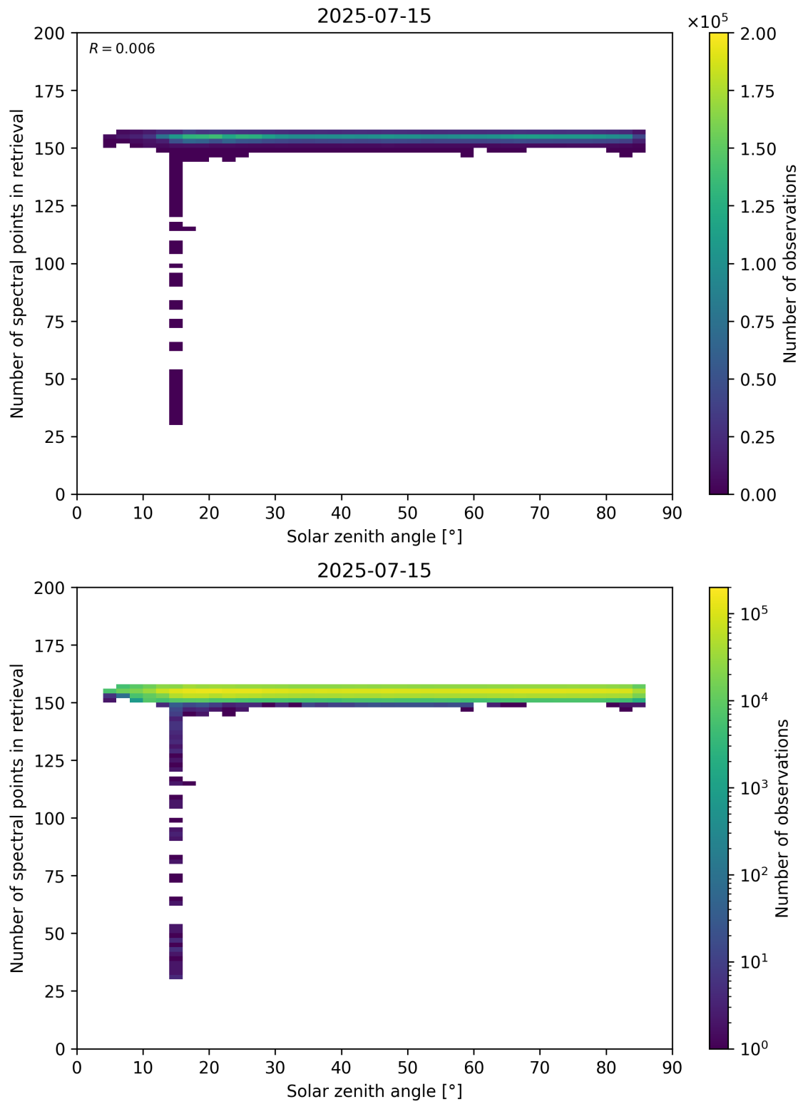
Figure 68: Scatter density plot of “Solar zenith angle” against “Number of spectral points in retrieval” for 2025-07-14 to 2025-07-16.
