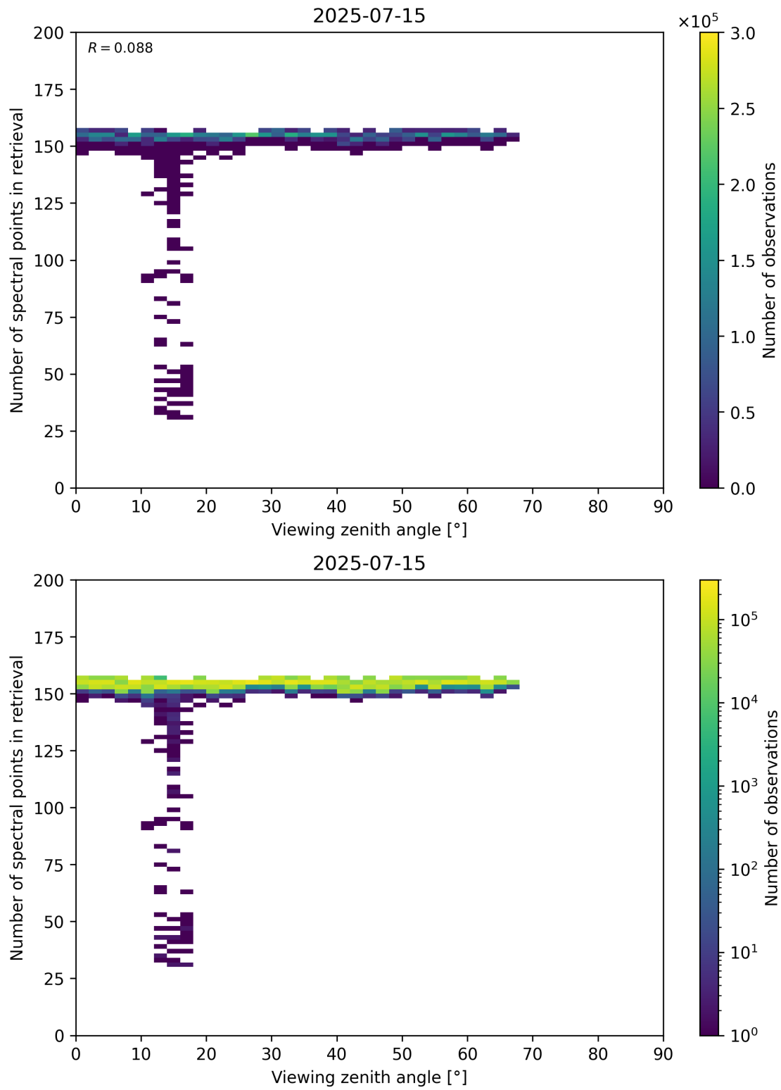
Figure 76: Scatter density plot of “Viewing zenith angle” against “Number of spectral points in retrieval” for 2025-07-14 to 2025-07-16.
